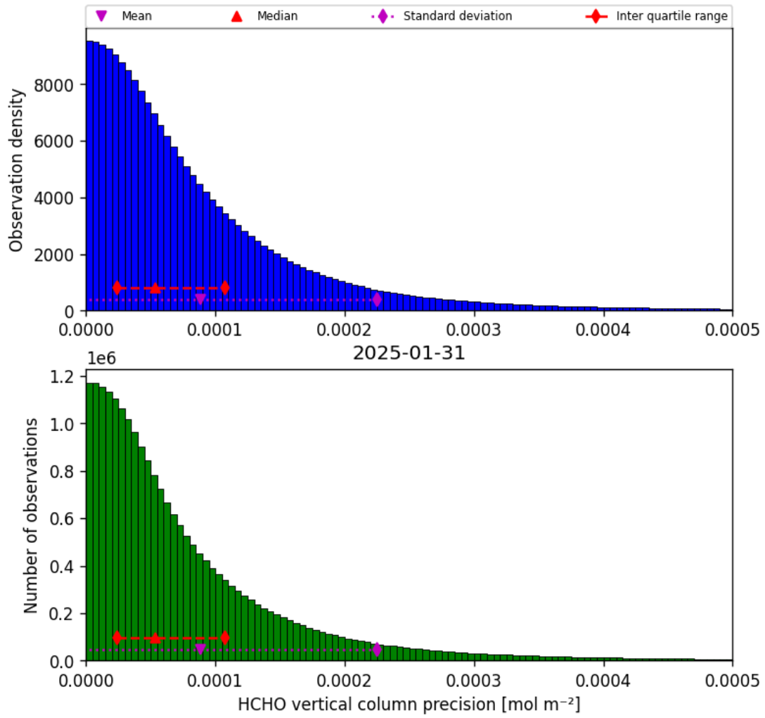
Figure 34: Histogram of “HCHO vertical column precision” for 2025-01-31 to 2025-01-31
