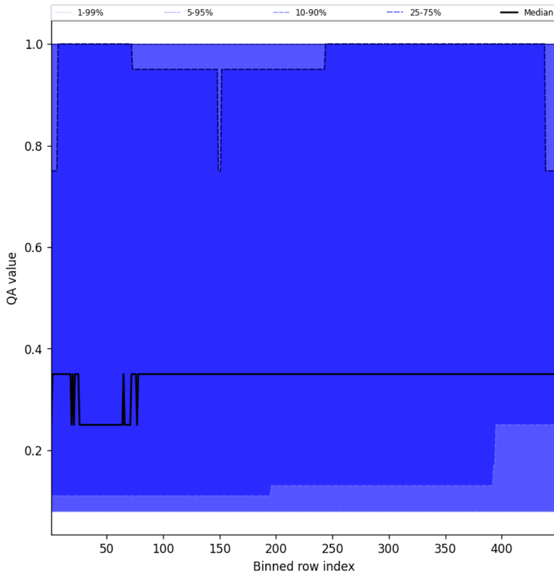
Figure 46: Along track statistics of “QA value” for 2025-01-31 to 2025-01-31
