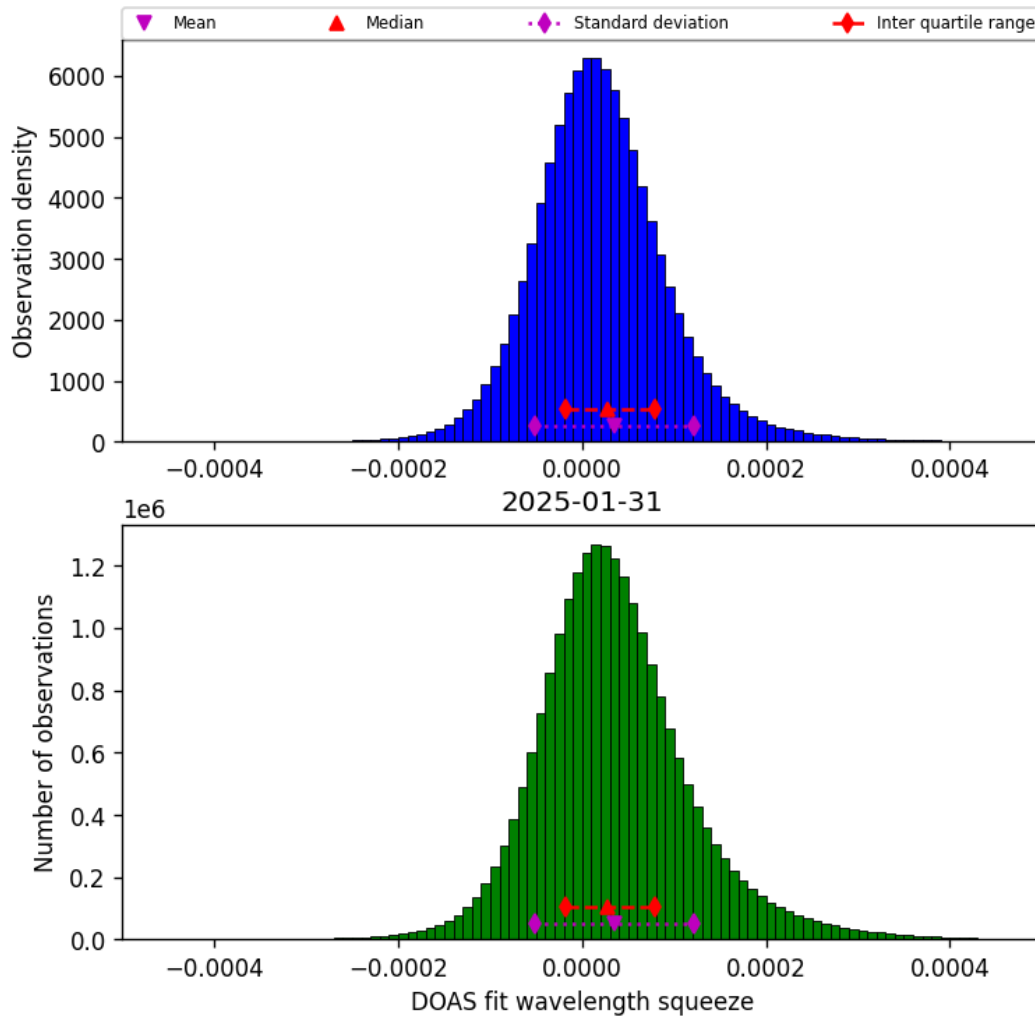
Figure 43: Histogram of “DOAS fit wavelength squeeze” for 2025-01-31 to 2025-01-31
