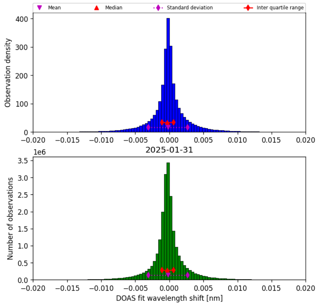
Figure 42: Histogram of “DOAS fit wavelength shift” for 2025-01-31 to 2025-01-31
