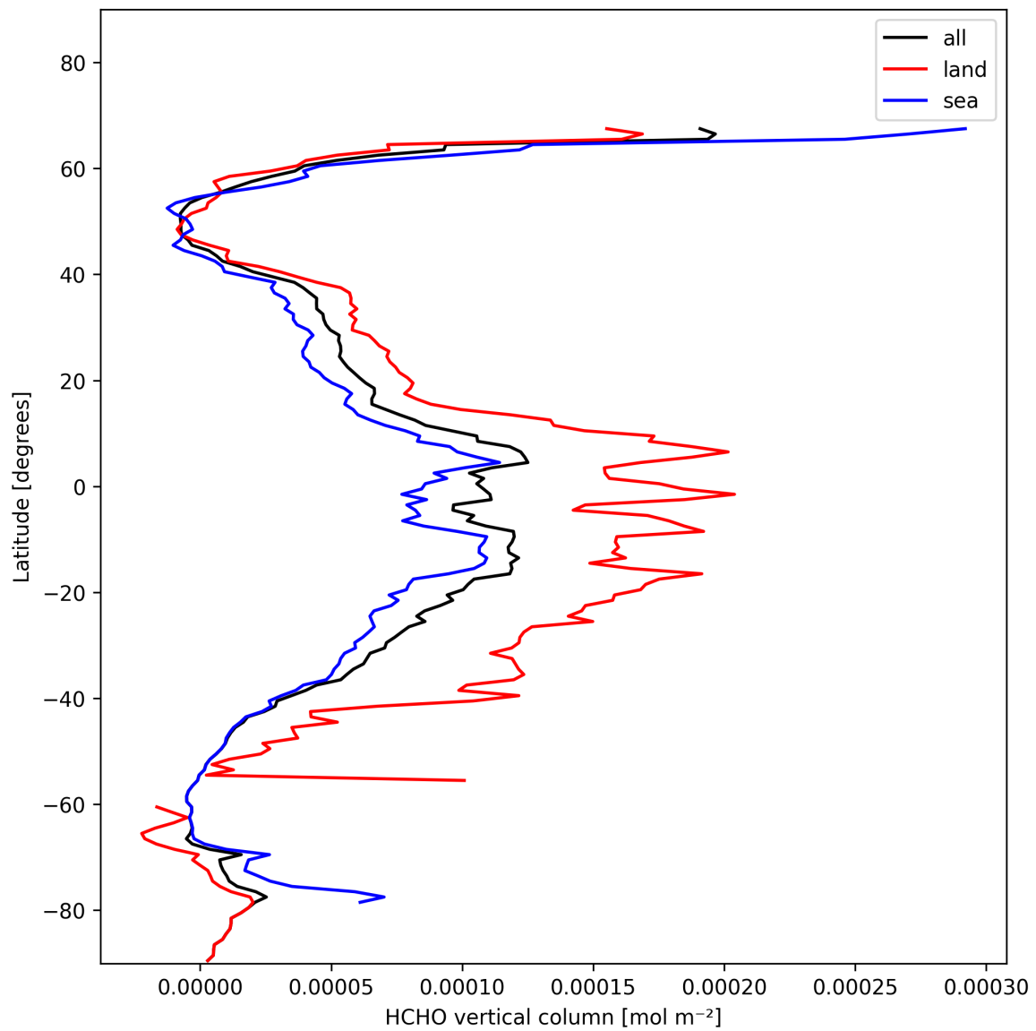
Figure 19: Zonal average of “HCHO vertical column” for 2025-01-31 to 2025-01-31.
