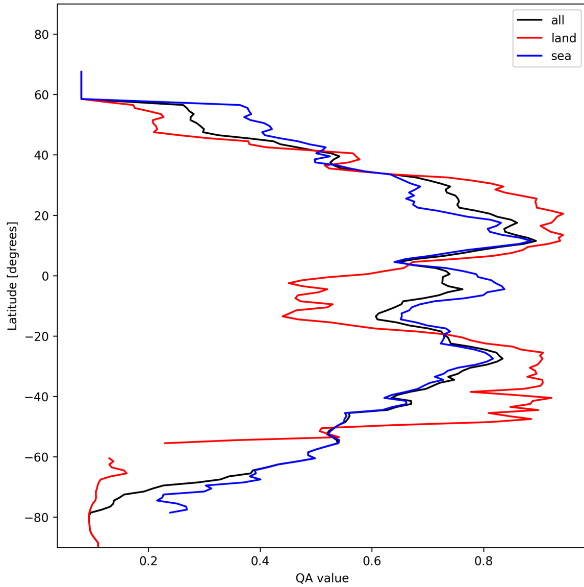
Figure 18: Zonal average of “QA value” for 2025-01-31 to 2025-01-31.
