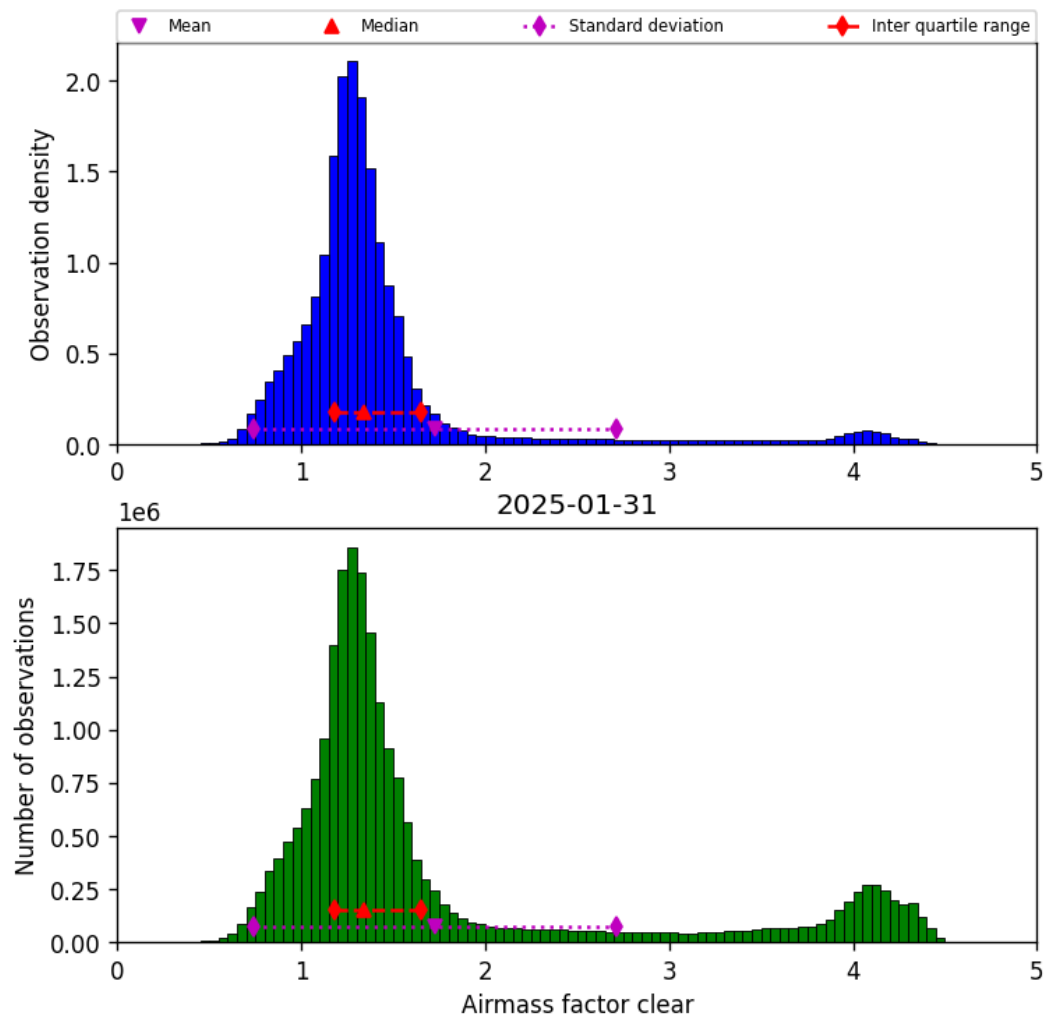
Figure 40: Histogram of “Airmass factor clear” for 2025-01-31 to 2025-01-31
