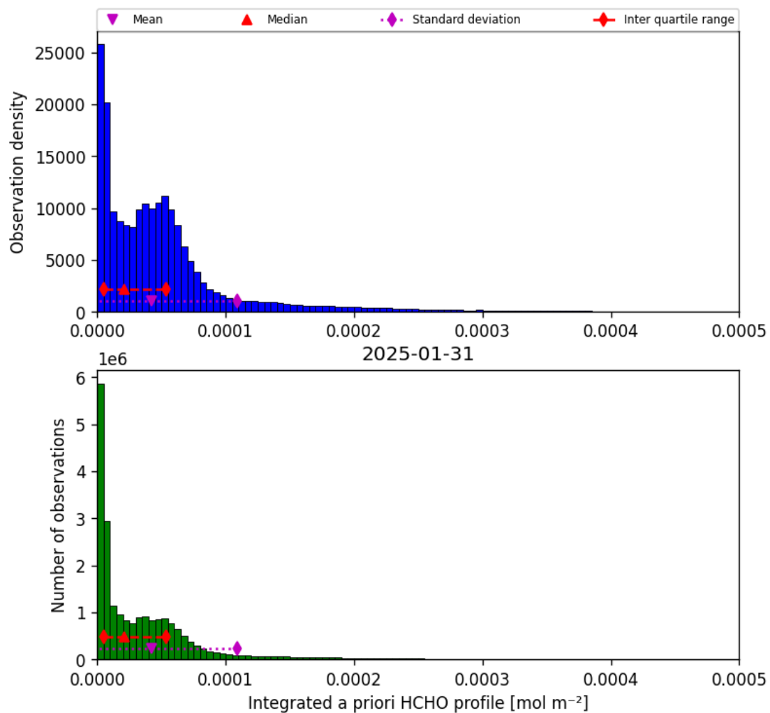
Figure 41: Histogram of “Integrated a priori HCHO profile” for 2025-01-31 to 2025-01-31
