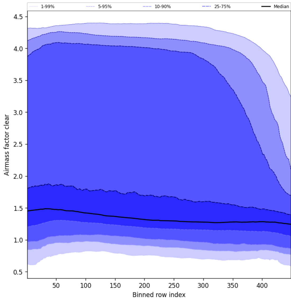
Figure 54: Along track statistics of “Airmass factor clear” for 2025-01-31 to 2025-01-31
