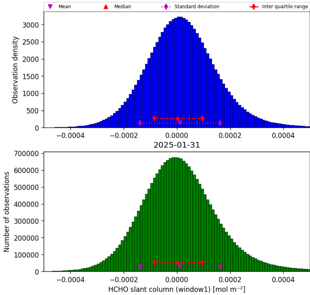
Figure 36: Histogram of “HCHO slant column (window1)” for 2025-01-31 to 2025-01-31
