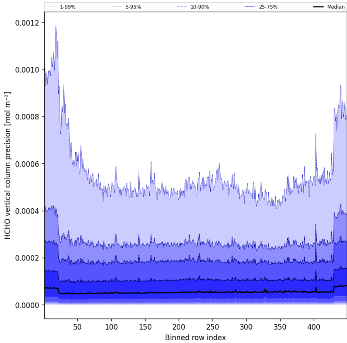
Figure 48: Along track statistics of “HCHO vertical column precision” for 2025-01-31 to 2025-01-31
