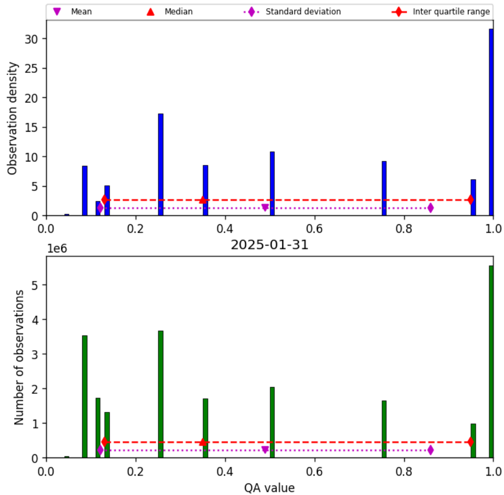
Figure 32: Histogram of “QA value” for 2025-01-31 to 2025-01-31
