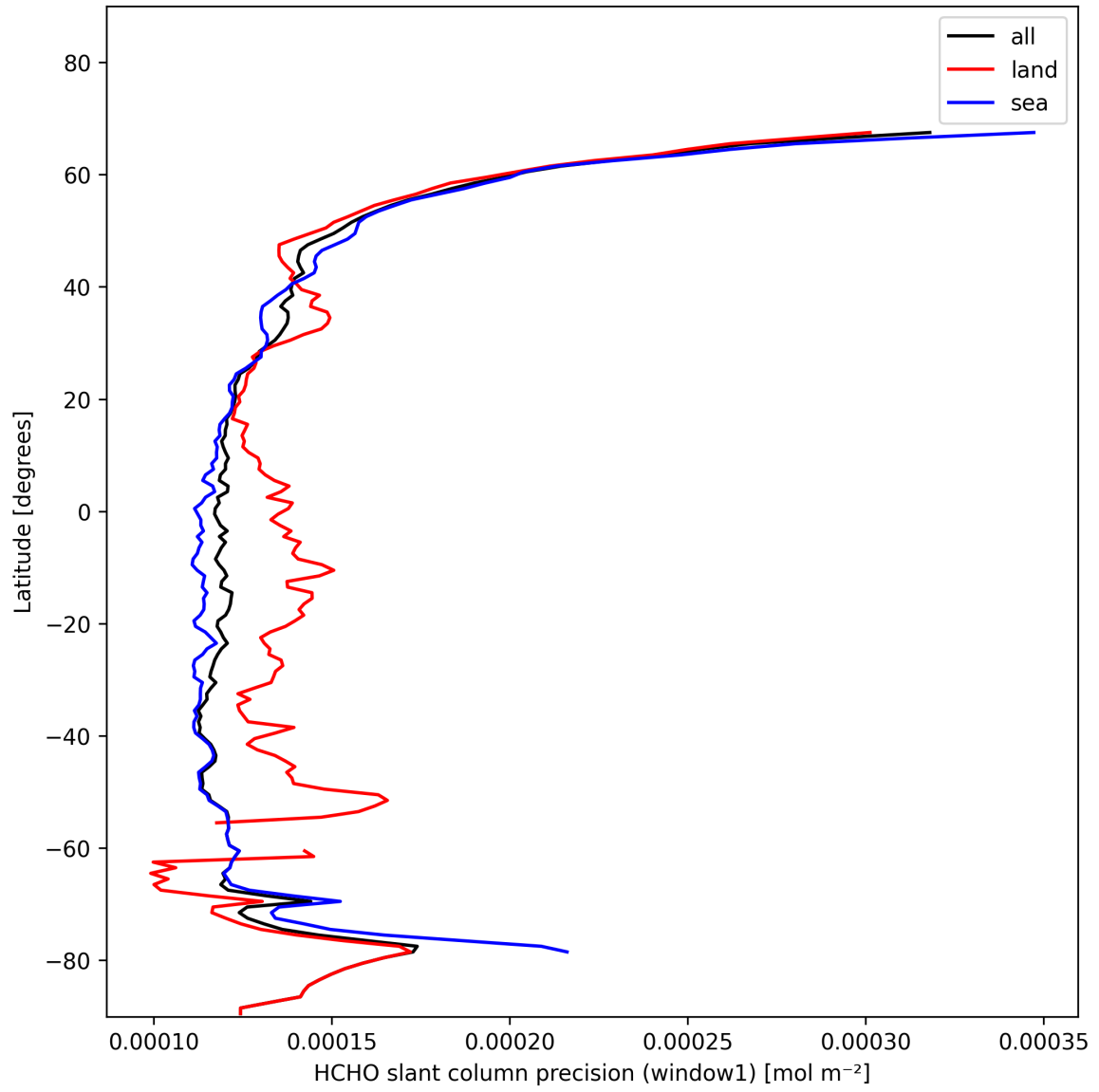
Figure 23: Zonal average of "HCHO slant column precision (window1)" for 2025-01-31 to 2025-01-31.
