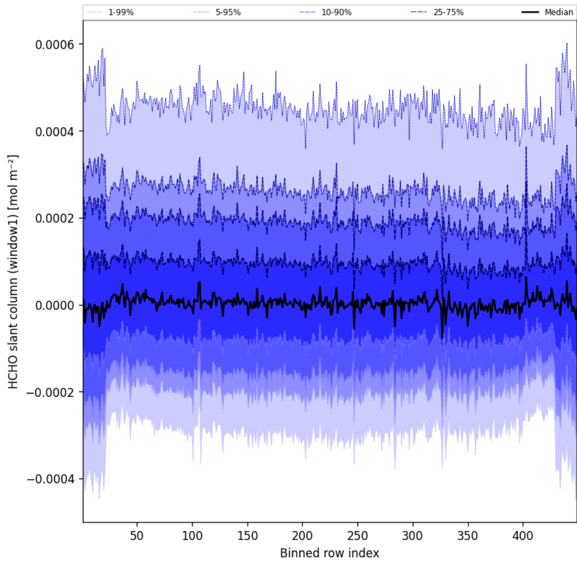
Figure 50: Along track statistics of "HCHO slant column (window1)" for 2025-01-31 to 2025-01-31
