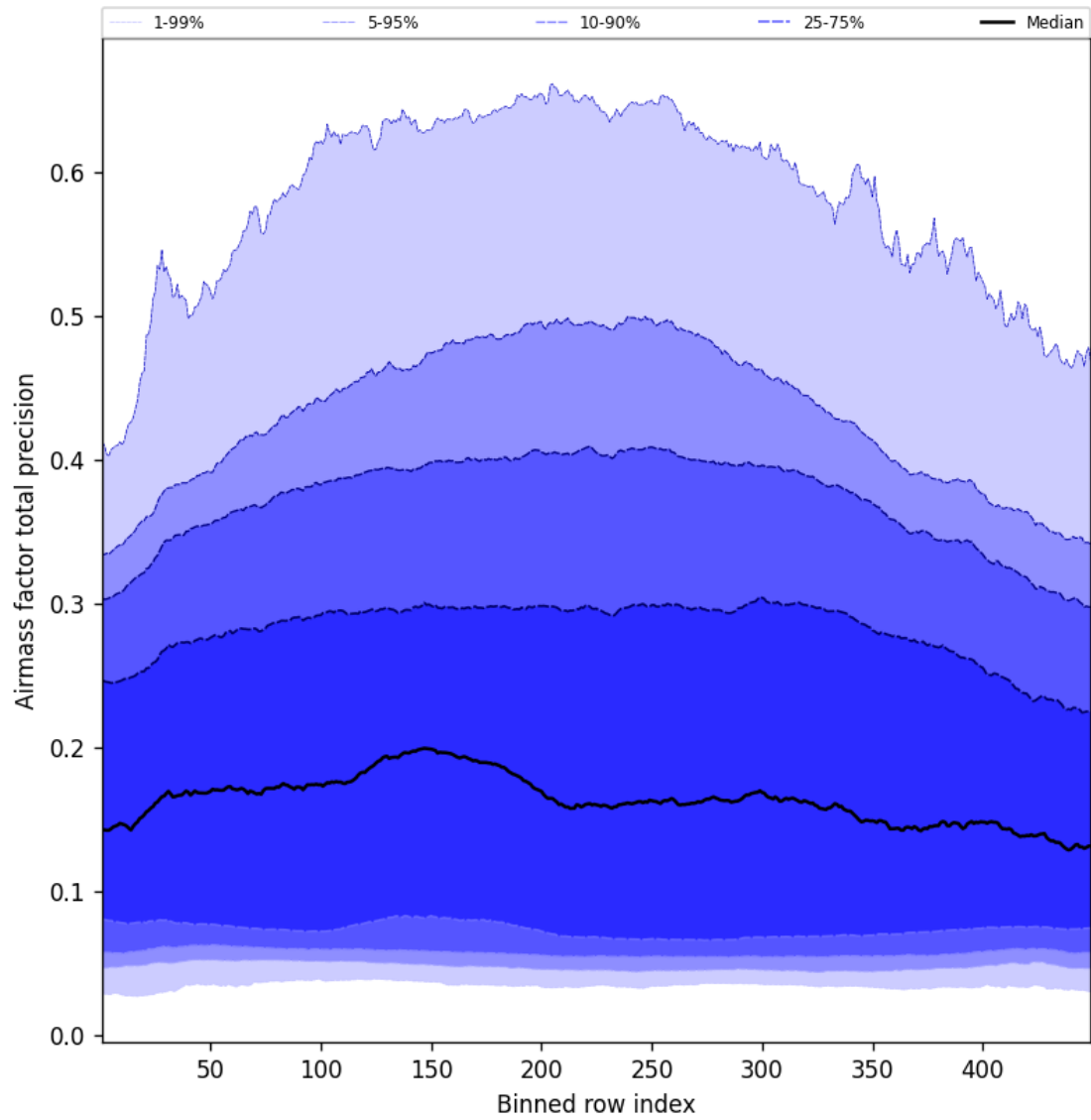
Figure 53: Along track statistics of “Airmass factor total precision” for 2025-01-31 to 2025-01-31
