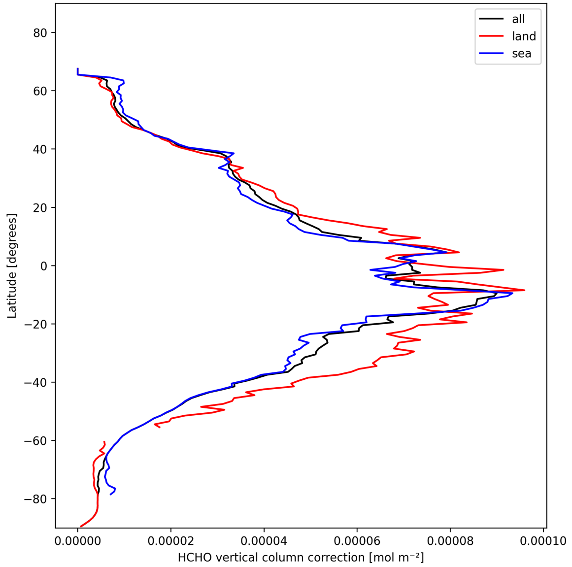
Figure 21: Zonal average of “HCHO vertical column correction” for 2025-01-31 to 2025-01-31.
