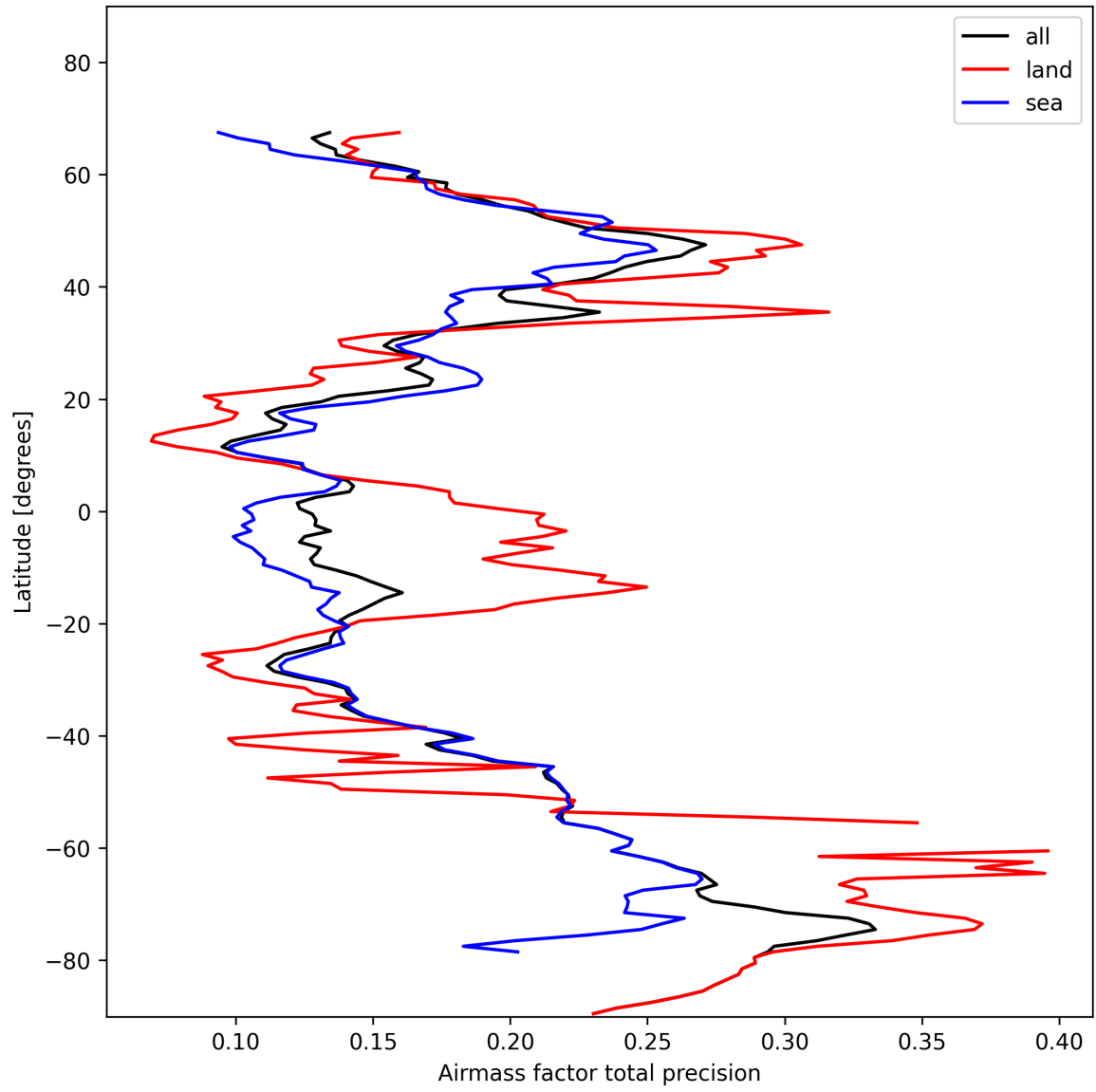
Figure 25: Zonal average of “Airmass factor total precision” for 2025-01-31 to 2025-01-31.
