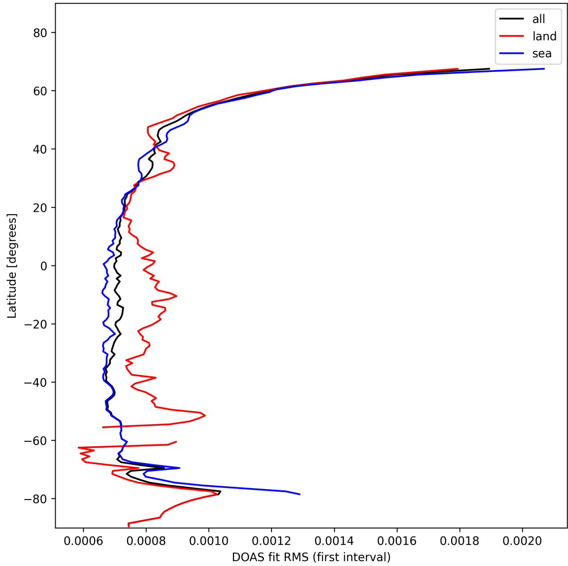
Figure 30: Zonal average of “DOAS fit RMS (first interval)” for 2025-01-31 to 2025-01-31.
