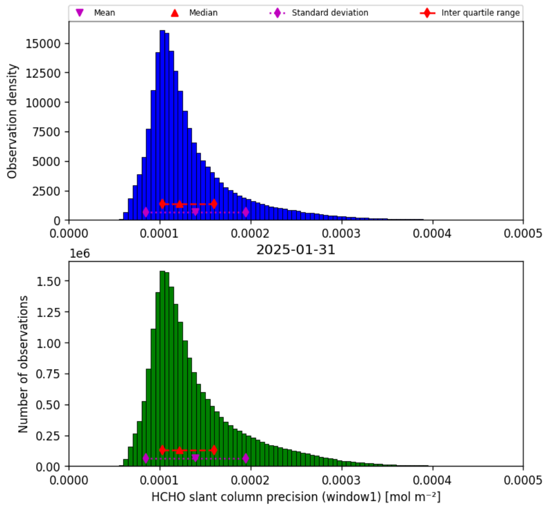
Figure 37: Histogram of “HCHO slant column precision (window1)” for 2025-01-31 to 2025-01-31
