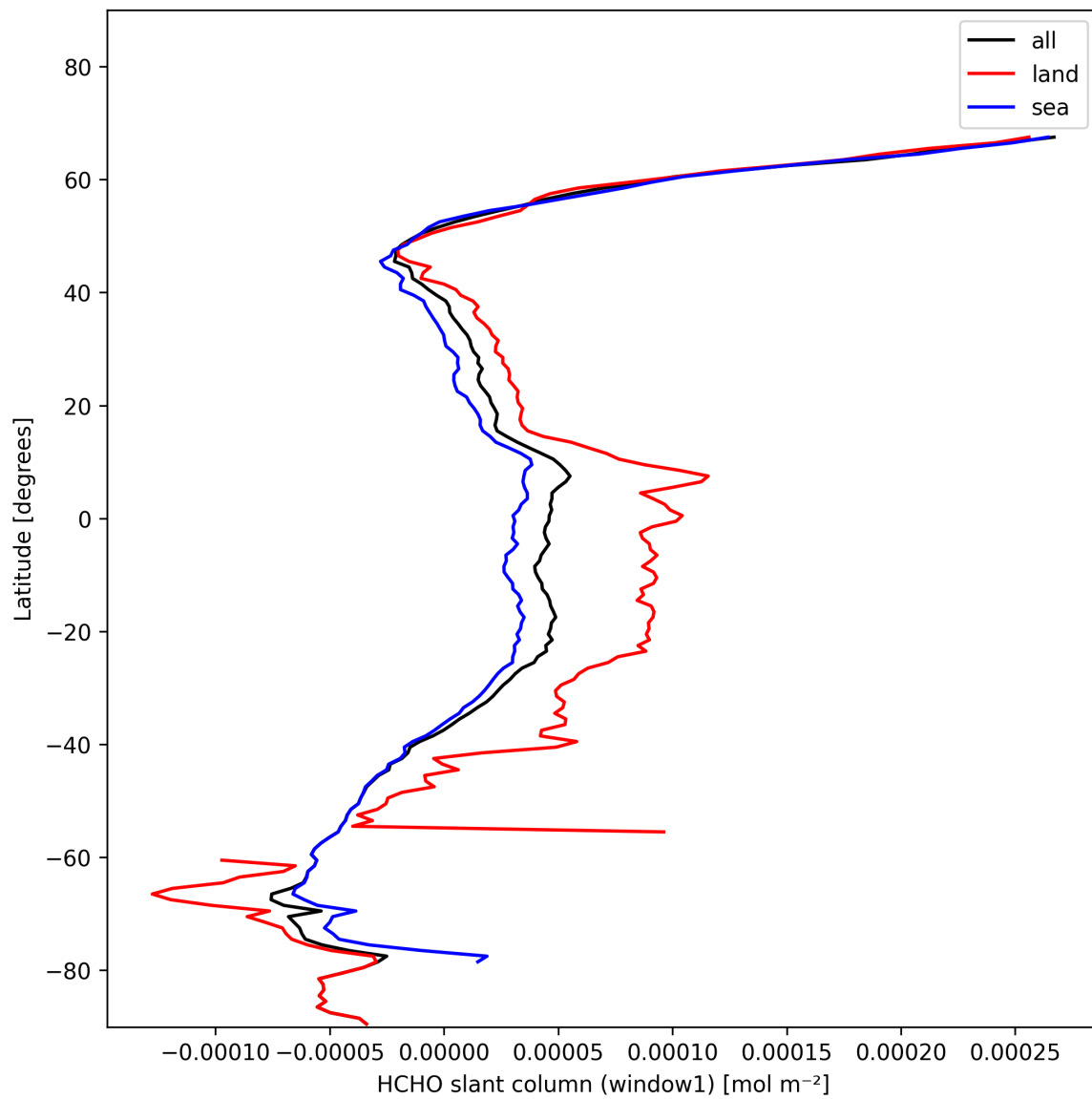
Figure 22: Zonal average of “HCHO slant column (window1)” for 2025-01-31 to 2025-01-31.
