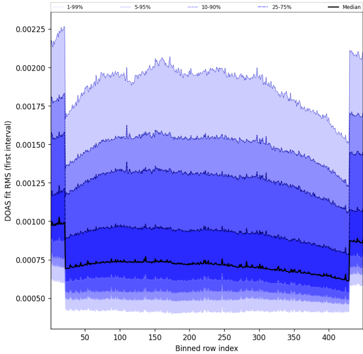
Figure 58: Along track statistics of “DOAS fit RMS (first interval)” for 2025-01-31 to 2025-01-31
