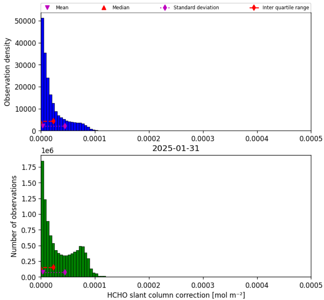
Figure 45: Histogram of “HCHO slant column correction” for 2025-01-31 to 2025-01-31
