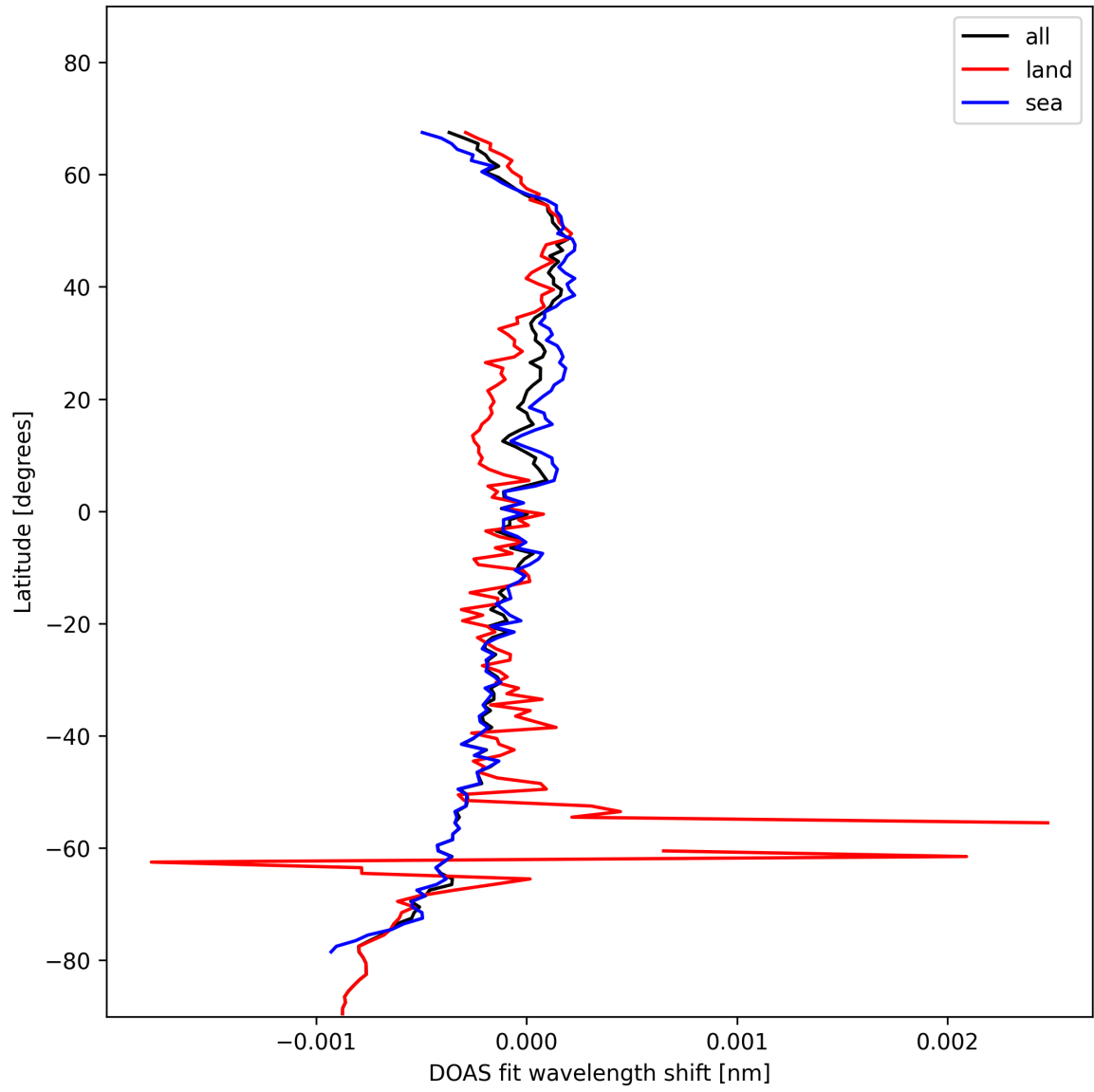
Figure 28: Zonal average of “DOAS fit wavelength shift” for 2025-01-31 to 2025-01-31.
