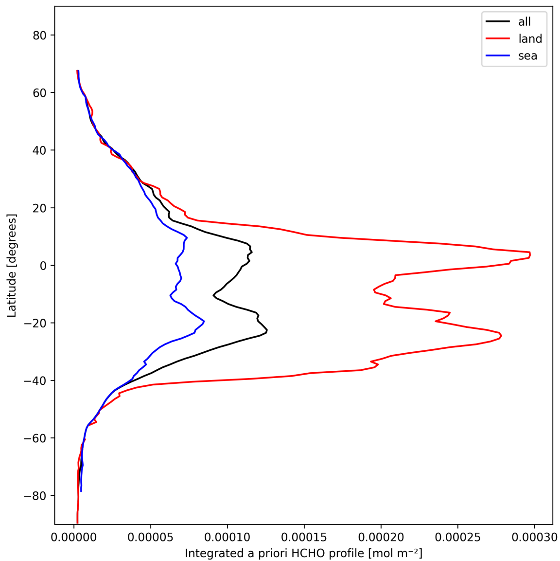
Figure 27: Zonal average of “Integrated a priori HCHO profile” for 2025-01-31 to 2025-01-31.
