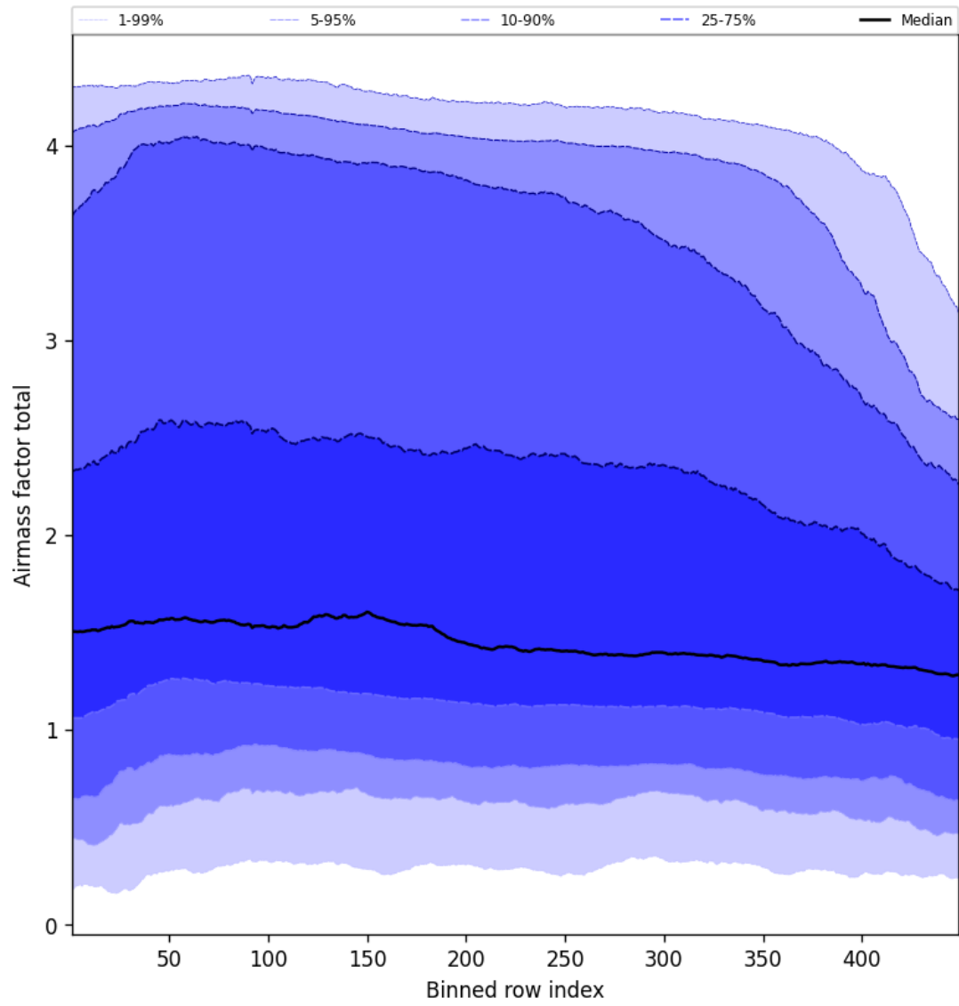
Figure 52: Along track statistics of “Airmass factor total” for 2025-01-31 to 2025-01-31
