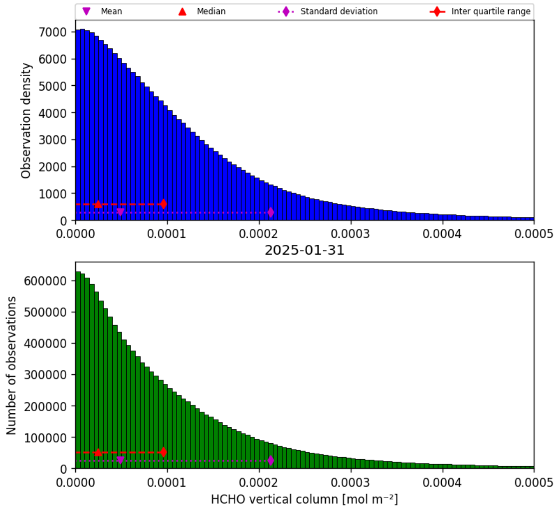
Figure 33: Histogram of “HCHO vertical column” for 2025-01-31 to 2025-01-31
