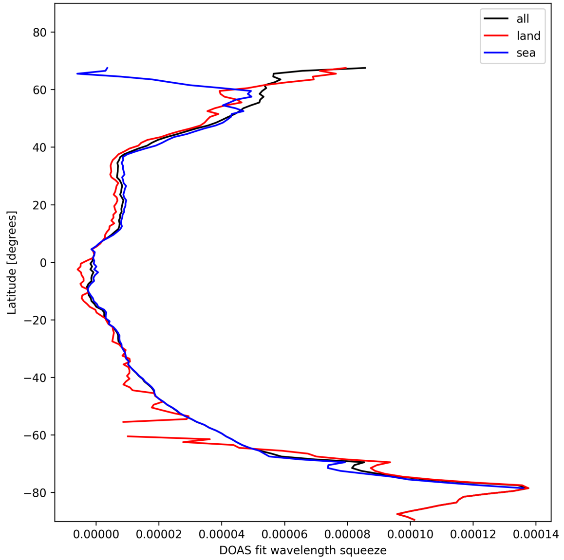
Figure 29: Zonal average of “DOAS fit wavelength squeeze” for 2025-01-31 to 2025-01-31.
