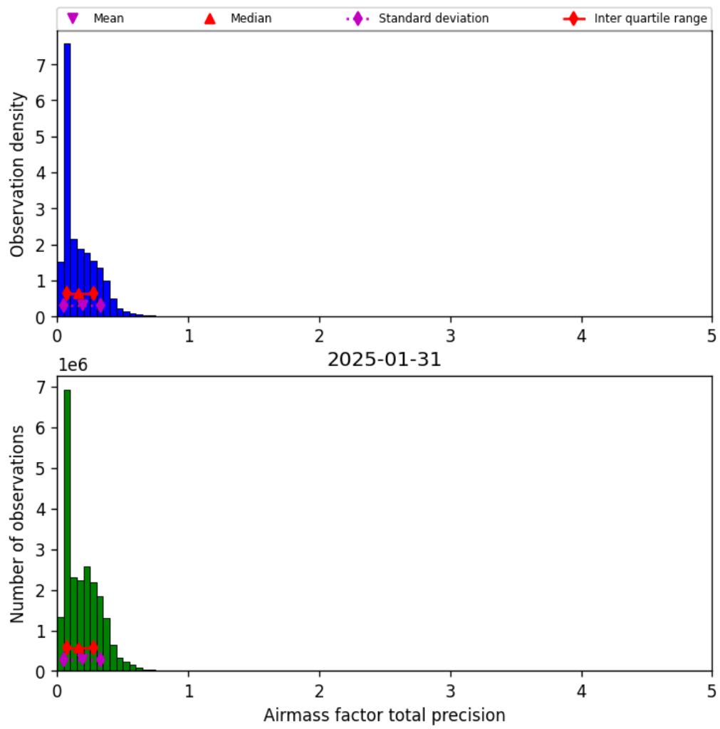
Figure 39: Histogram of “Airmass factor total precision” for 2025-01-31 to 2025-01-31
