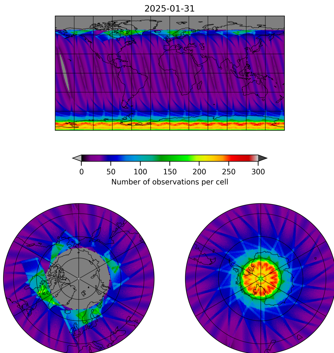
Figure 17: Map of the number of observations for 2025-01-31 to 2025-01-31
