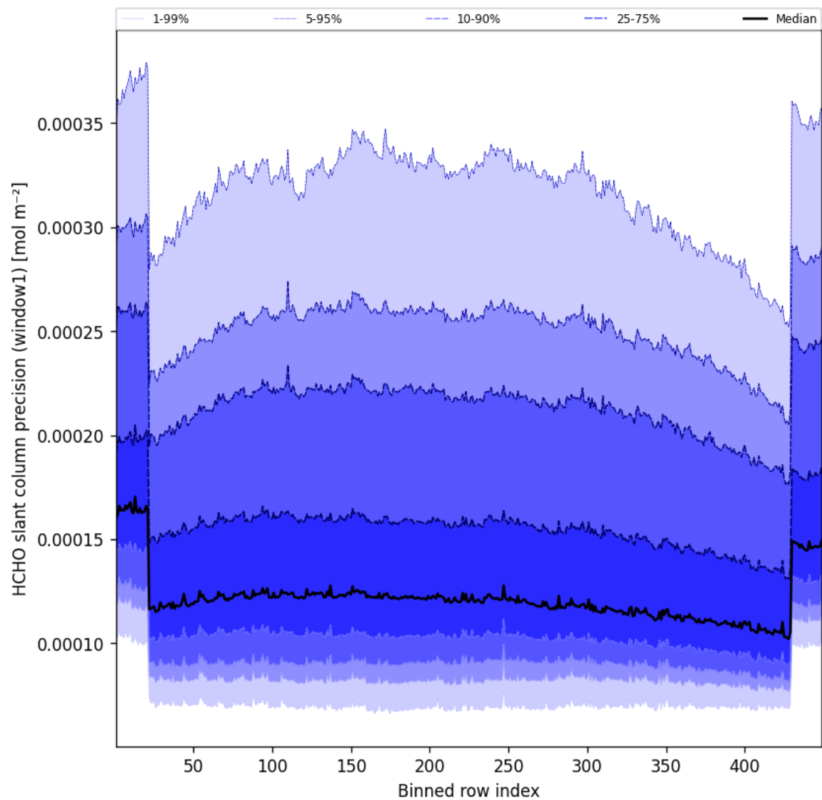
Figure 51: Along track statistics of “HCHO slant column precision (window1)” for 2025-01-31 to 2025-01-31
