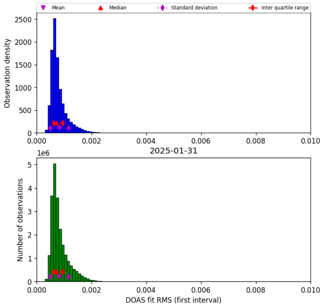
Figure 44: Histogram of “DOAS fit RMS (first interval)” for 2025-01-31 to 2025-01-31
