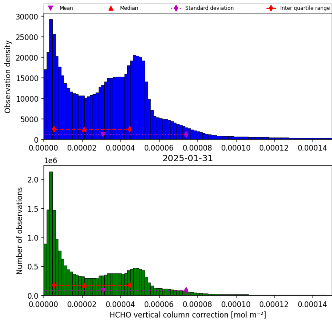
Figure 35: Histogram of “HCHO vertical column correction” for 2025-01-31 to 2025-01-31
