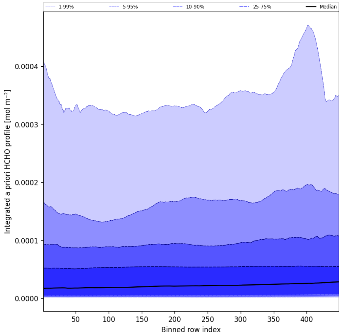
Figure 55: Along track statistics of “Integrated a priori HCHO profile” for 2025-01-31 to 2025-01-31
