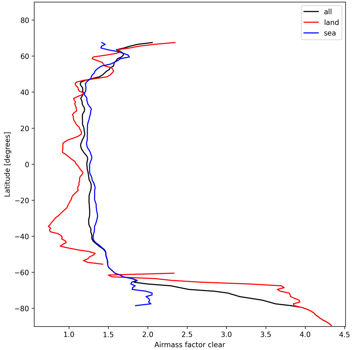
Figure 26: Zonal average of “Airmass factor clear” for 2025-01-31 to 2025-01-31.
