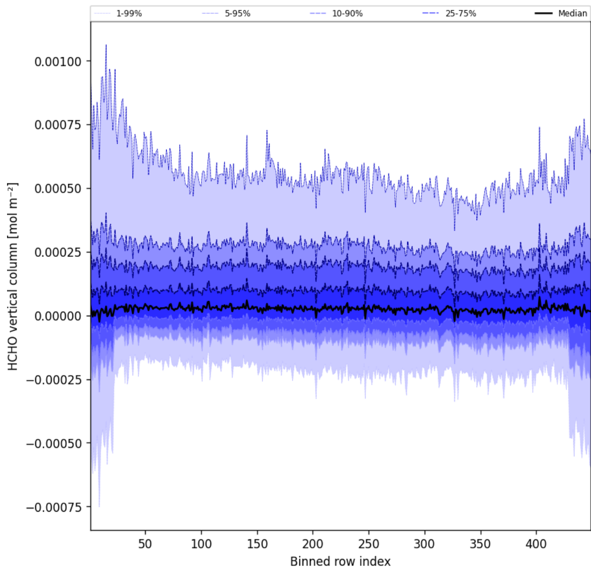
Figure 47: Along track statistics of “HCHO vertical column” for 2025-01-31 to 2025-01-31
