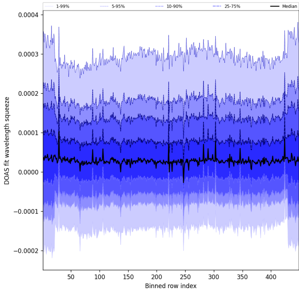
Figure 57: Along track statistics of “DOAS fit wavelength squeeze” for 2025-01-31 to 2025-01-31
