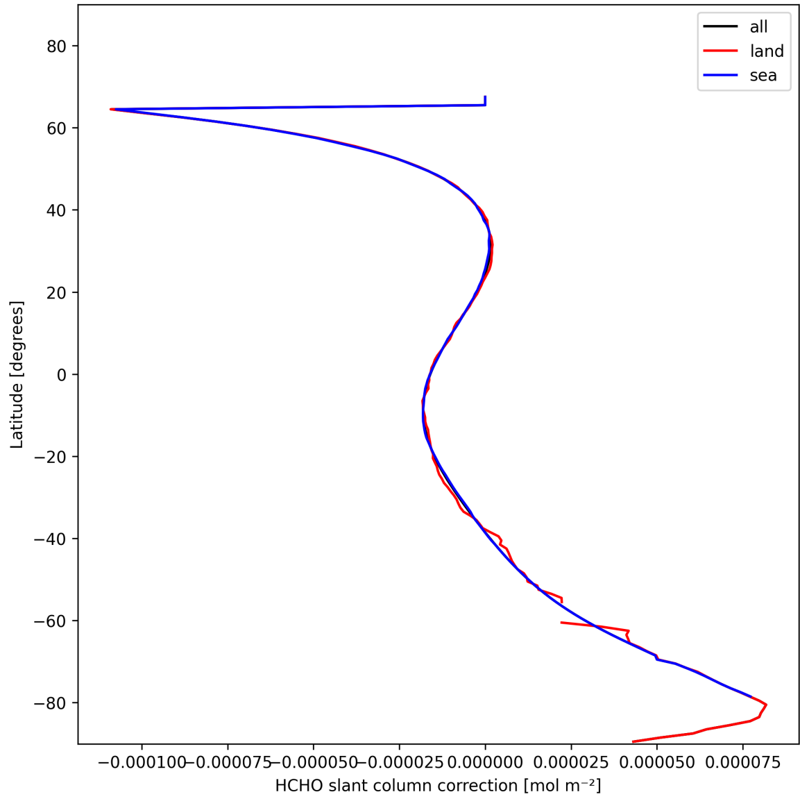
Figure 31: Zonal average of “HCHO slant column correction” for 2025-01-31 to 2025-01-31.
