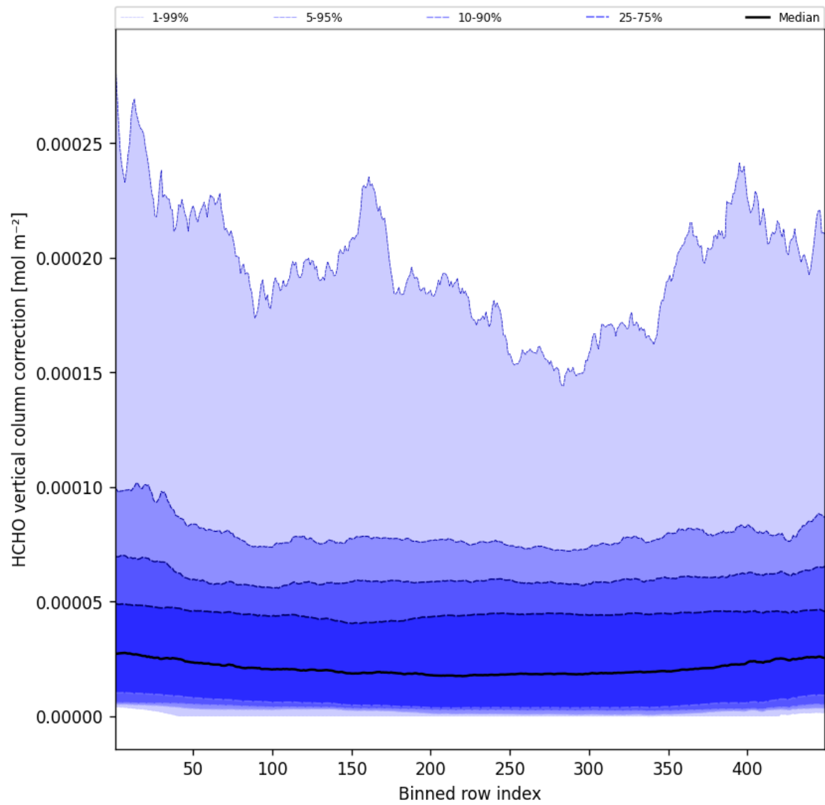
Figure 49: Along track statistics of “HCHO vertical column correction” for 2025-01-31 to 2025-01-31
