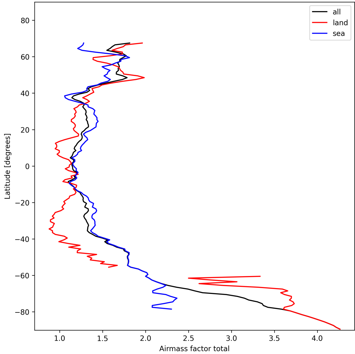
Figure 24: Zonal average of “Airmass factor total” for 2025-01-31 to 2025-01-31.
