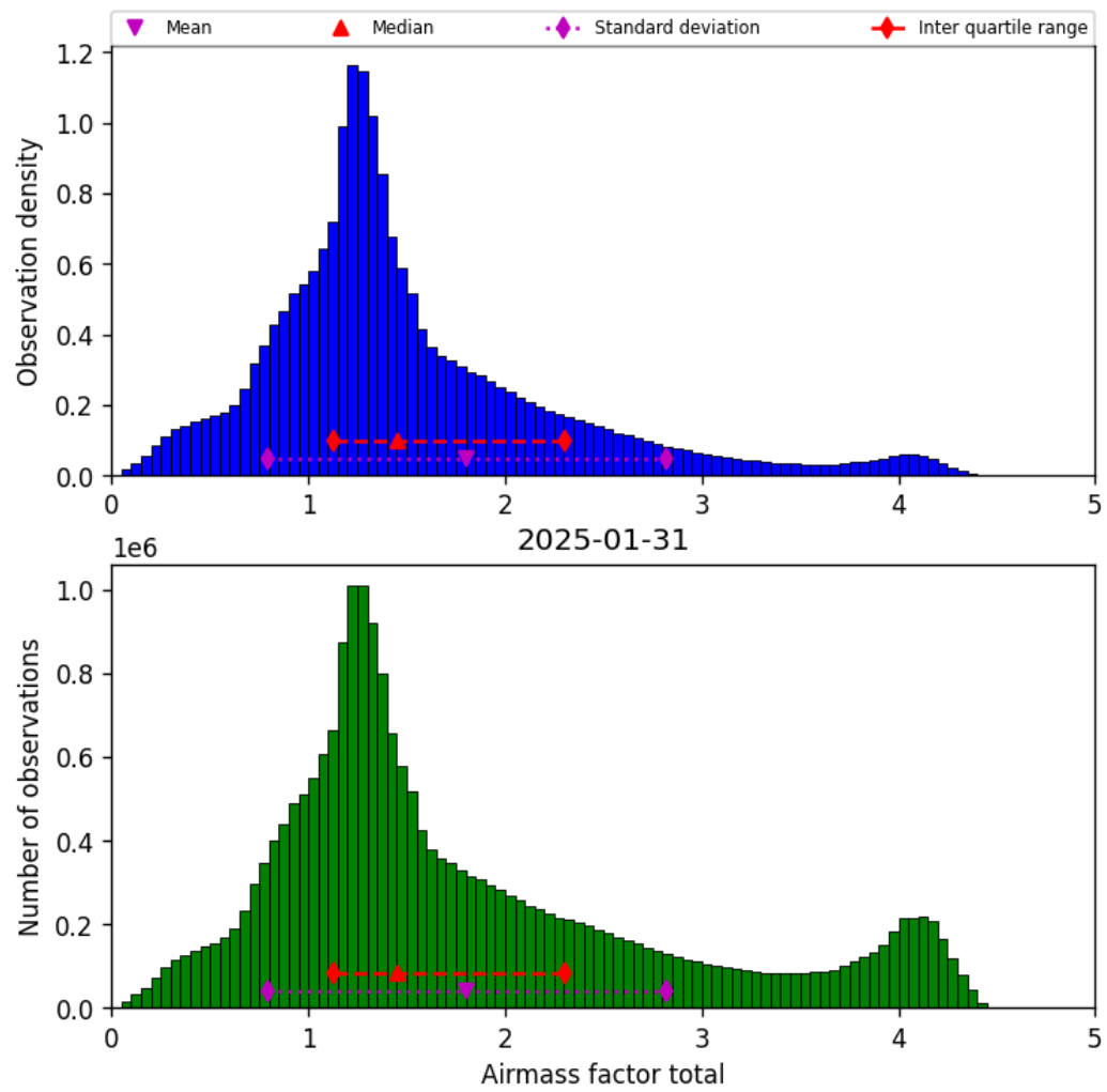
Figure 38: Histogram of “Airmass factor total” for 2025-01-31 to 2025-01-31
