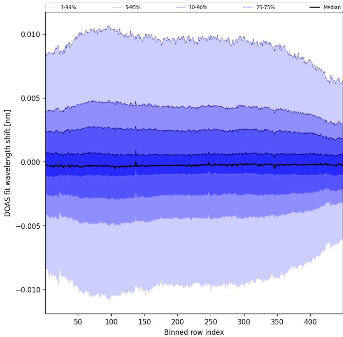
Figure 56: Along track statistics of “DOAS fit wavelength shift” for 2025-01-31 to 2025-01-31
