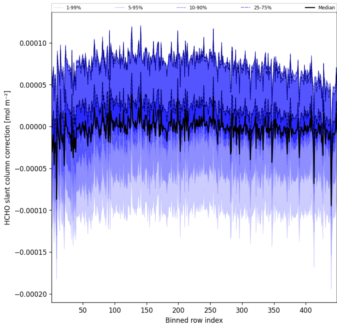
Figure 59: Along track statistics of “HCHO slant column correction” for 2025-01-31 to 2025-01-31
