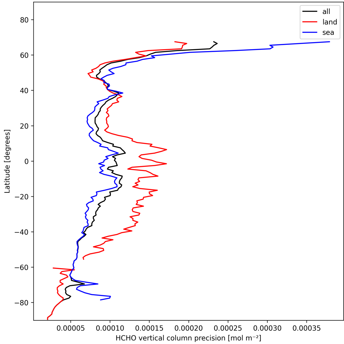
Figure 20: Zonal average of “HCHO vertical column precision” for 2025-01-31 to 2025-01-31.
