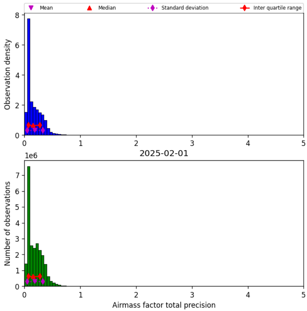
Figure 39: Histogram of “Airmass factor total precision” for 2025-02-01 to 2025-02-02
