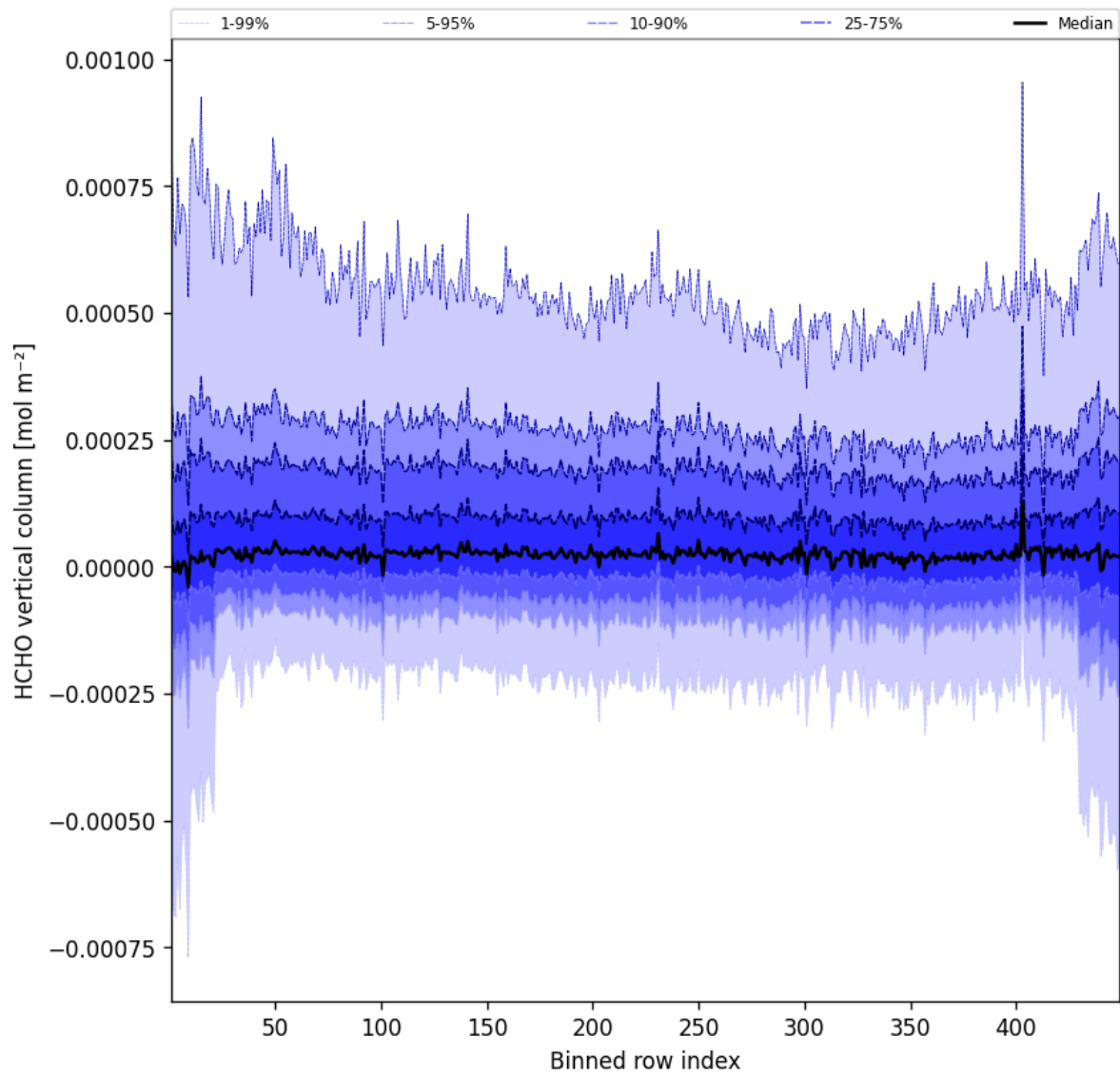
Figure 47: Along track statistics of “HCHO vertical column” for 2025-02-01 to 2025-02-02
