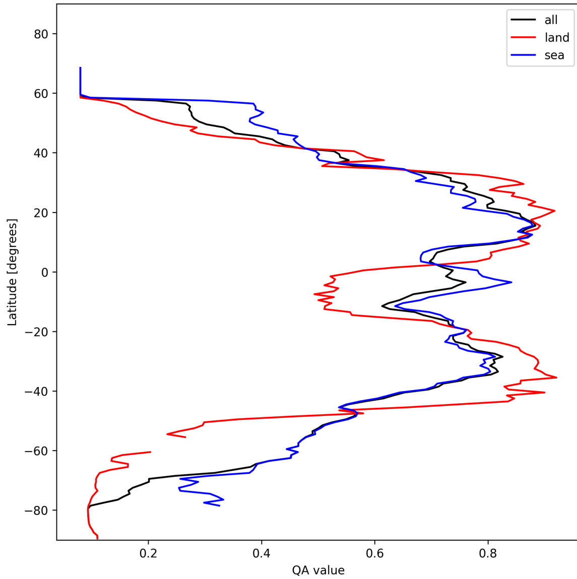
Figure 18: Zonal average of “QA value” for 2025-02-01 to 2025-02-02.
