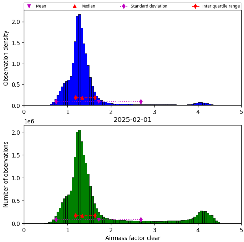
Figure 40: Histogram of “Airmass factor clear” for 2025-02-01 to 2025-02-02
