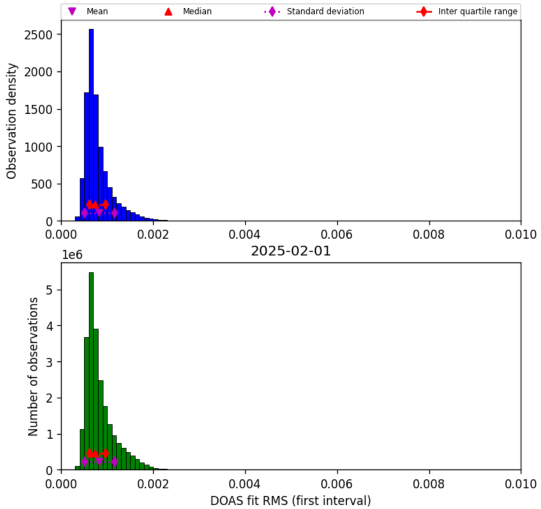
Figure 44: Histogram of “DOAS fit RMS (first interval)” for 2025-02-01 to 2025-02-02
