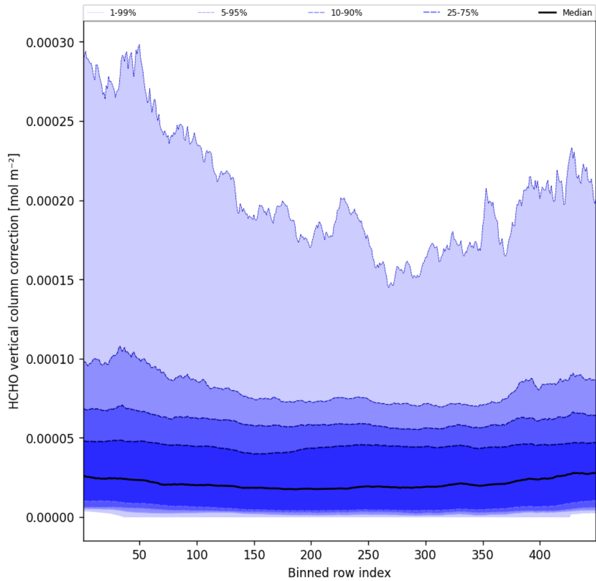
Figure 49: Along track statistics of “HCHO vertical column correction” for 2025-02-01 to 2025-02-02
