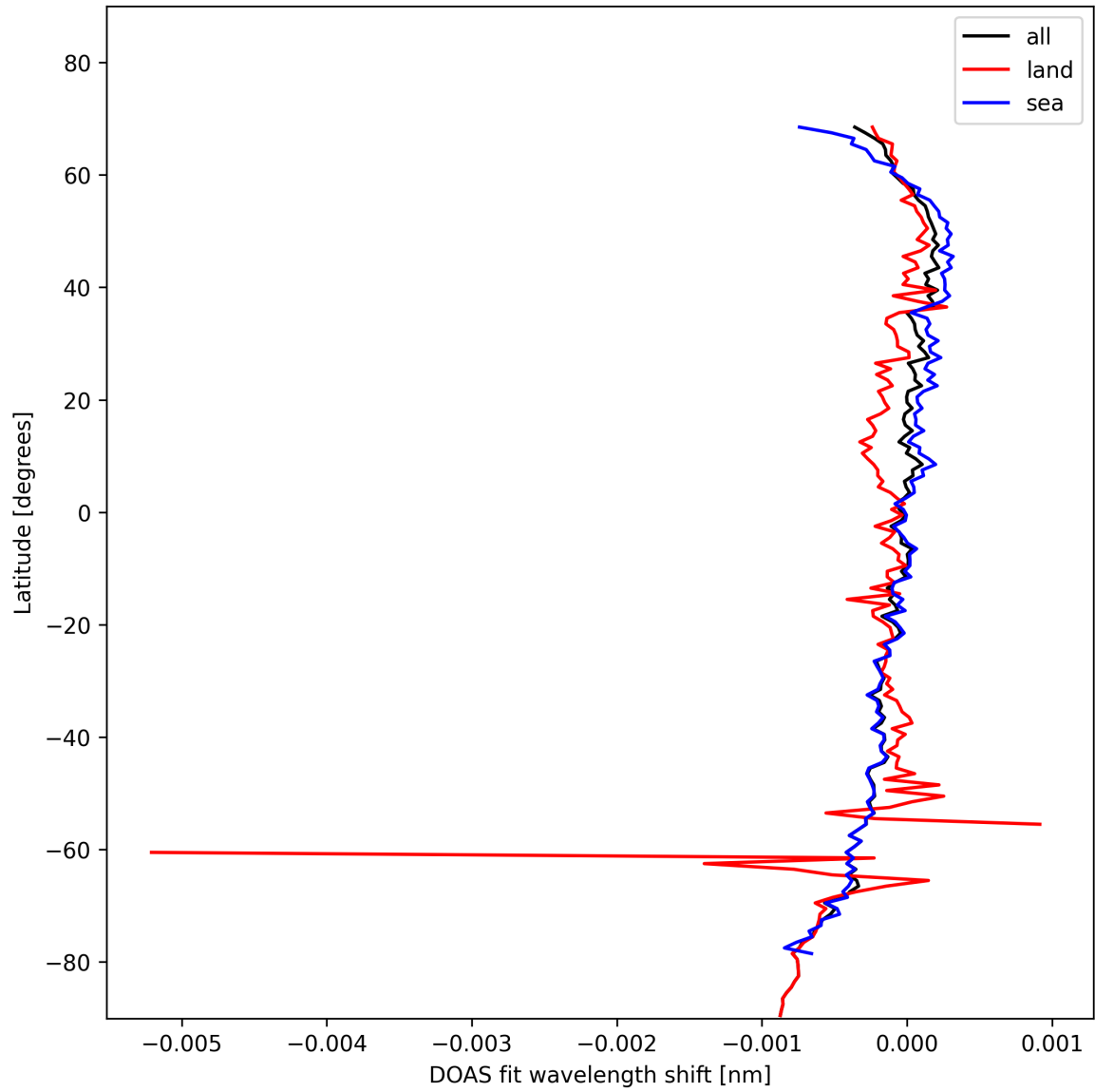
Figure 28: Zonal average of “DOAS fit wavelength shift” for 2025-02-01 to 2025-02-02.
