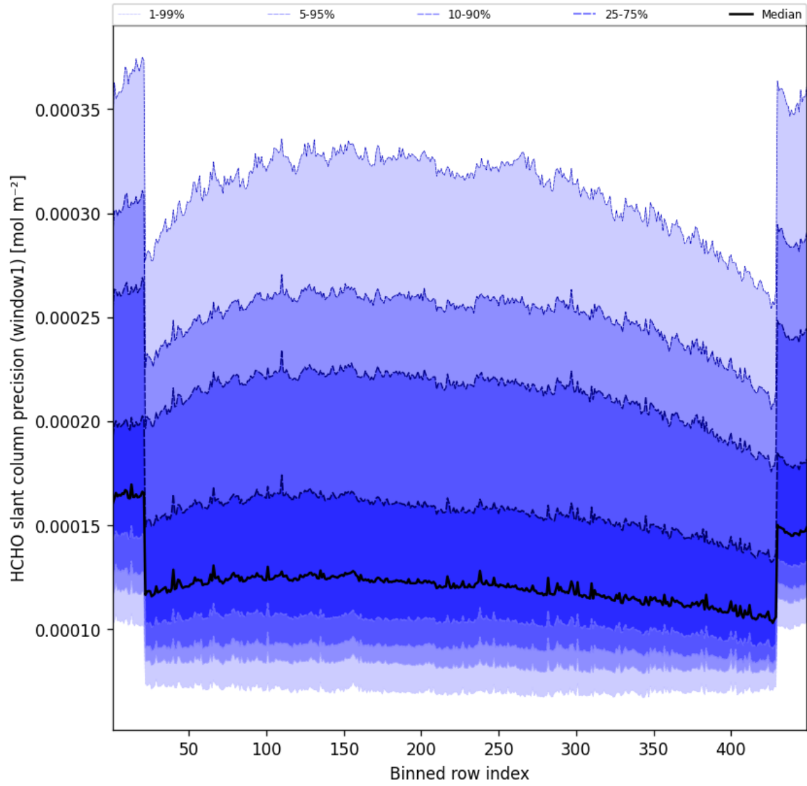
Figure 51: Along track statistics of “HCHO slant column precision (window1)” for 2025-02-01 to 2025-02-02
