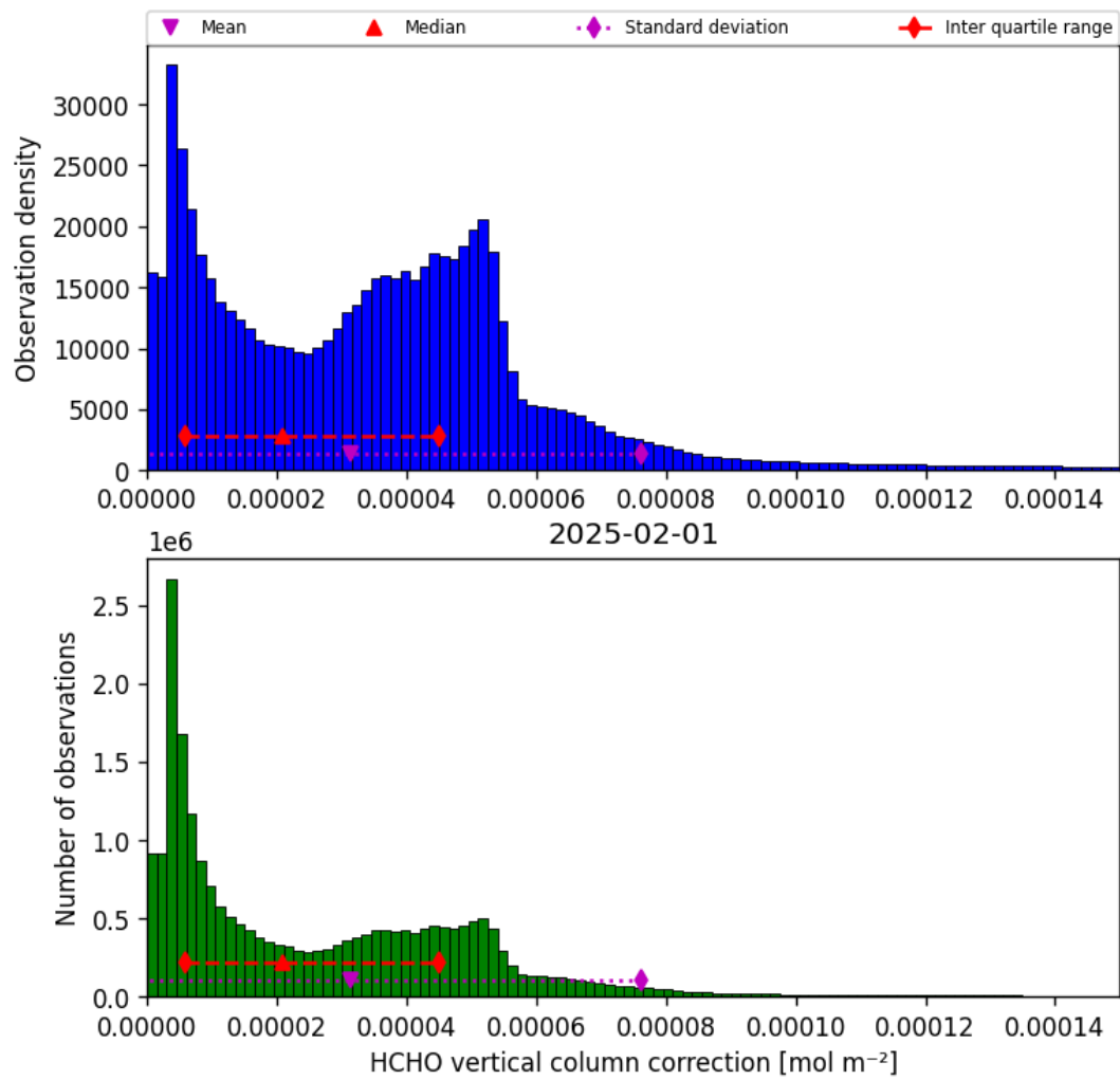
Figure 35: Histogram of “HCHO vertical column correction” for 2025-02-01 to 2025-02-02
