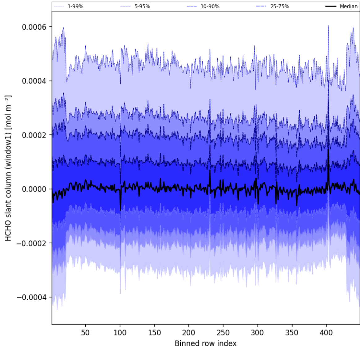
Figure 50: Along track statistics of “HCHO slant column (window1)” for 2025-02-01 to 2025-02-02
