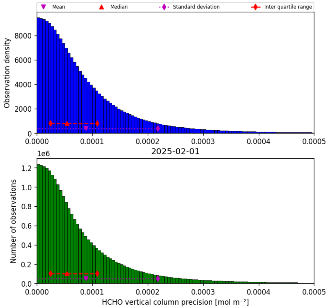
Figure 34: Histogram of “HCHO vertical column precision” for 2025-02-01 to 2025-02-02
