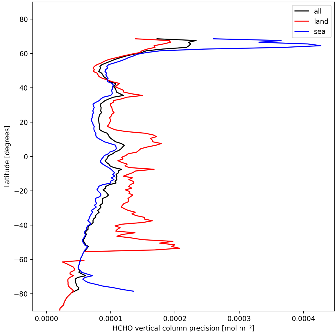
Figure 20: Zonal average of “HCHO vertical column precision” for 2025-02-01 to 2025-02-02.
