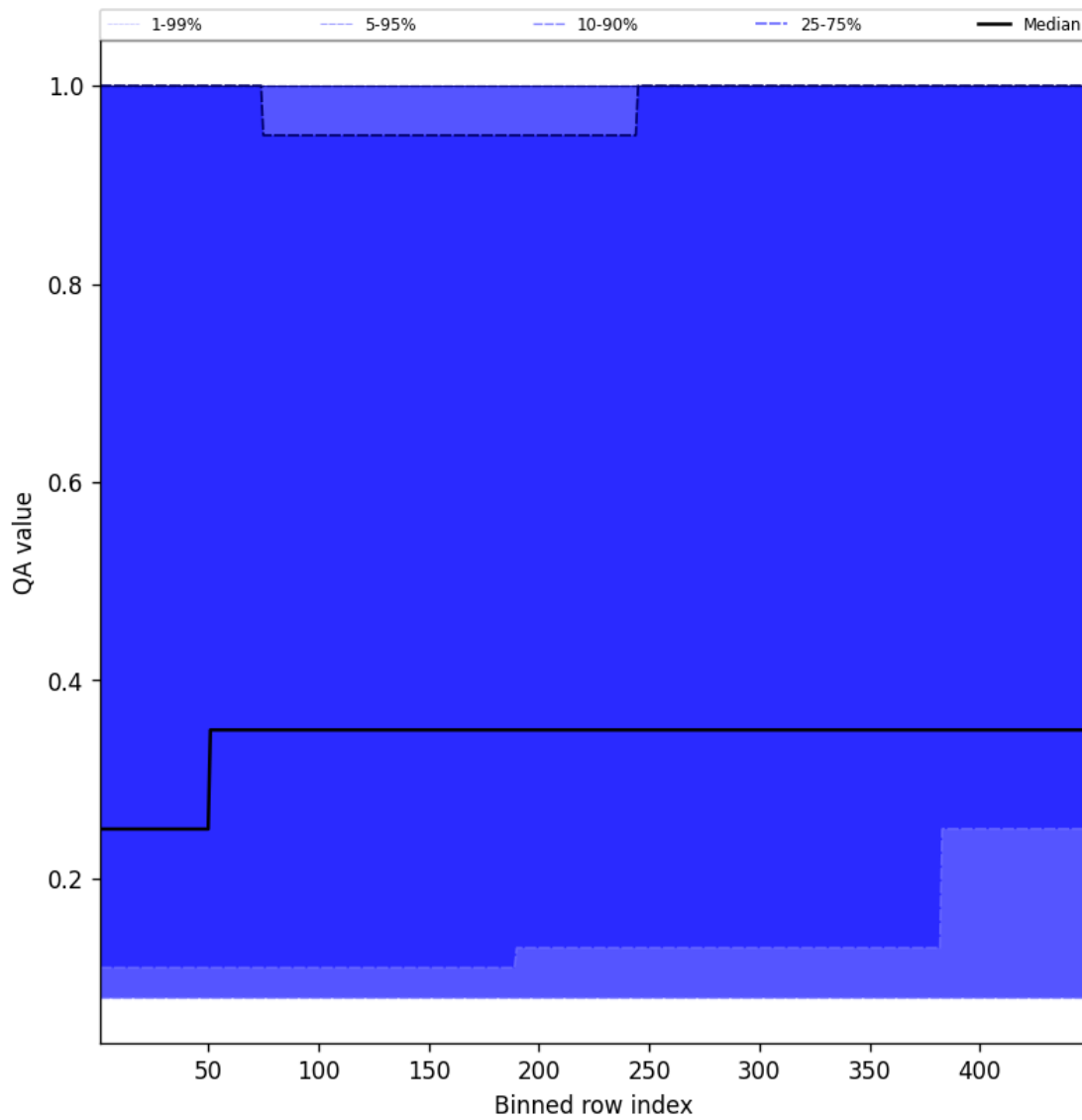
Figure 46: Along track statistics of “QA value” for 2025-02-01 to 2025-02-02
