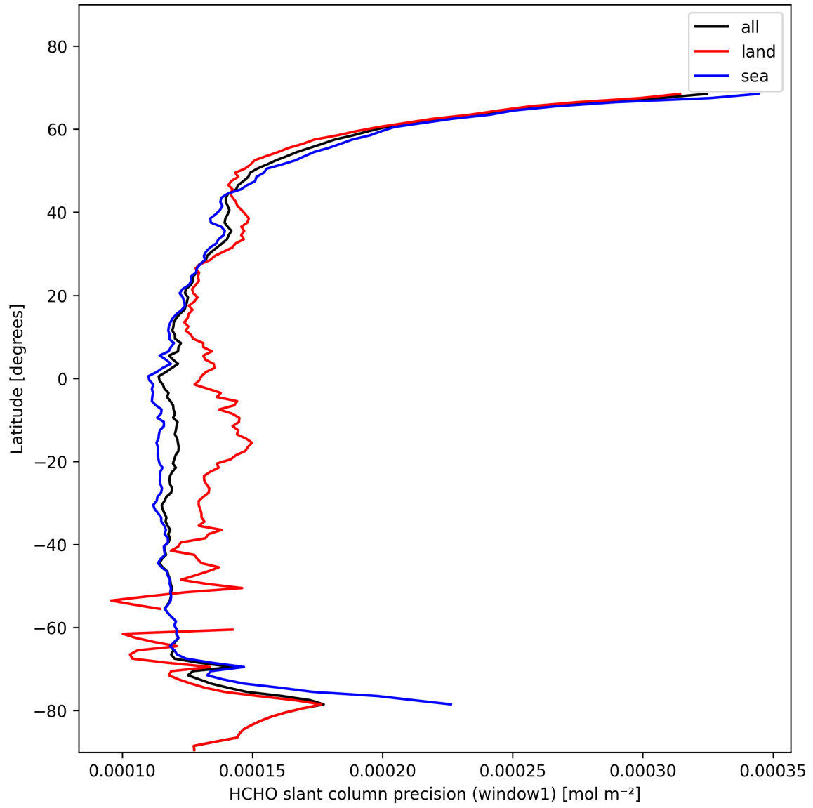
Figure 23: Zonal average of “HCHO slant column precision (window1)” for 2025-02-01 to 2025-02-02.
