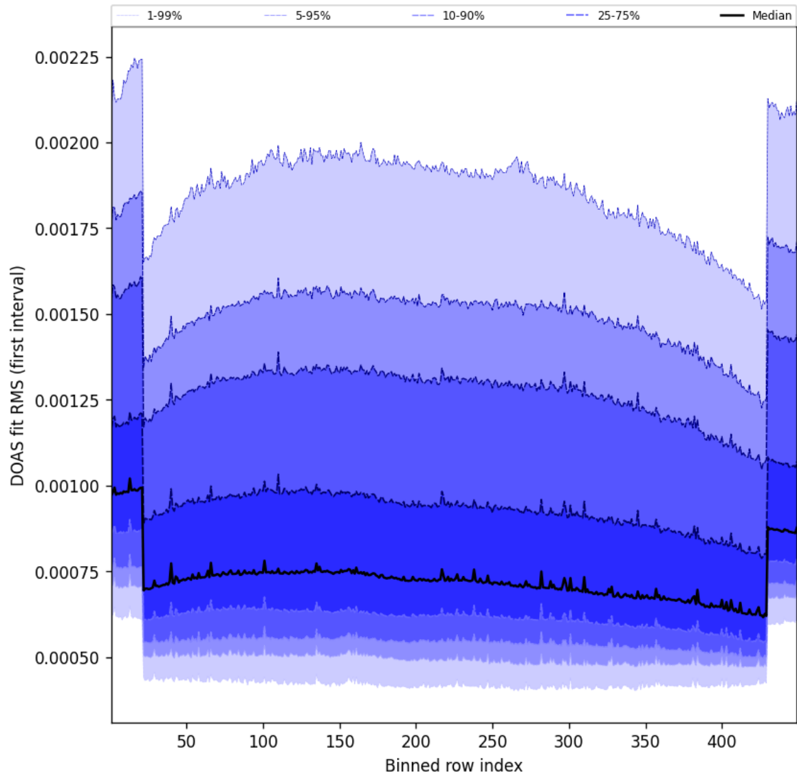
Figure 58: Along track statistics of “DOAS fit RMS (first interval)” for 2025-02-01 to 2025-02-02
