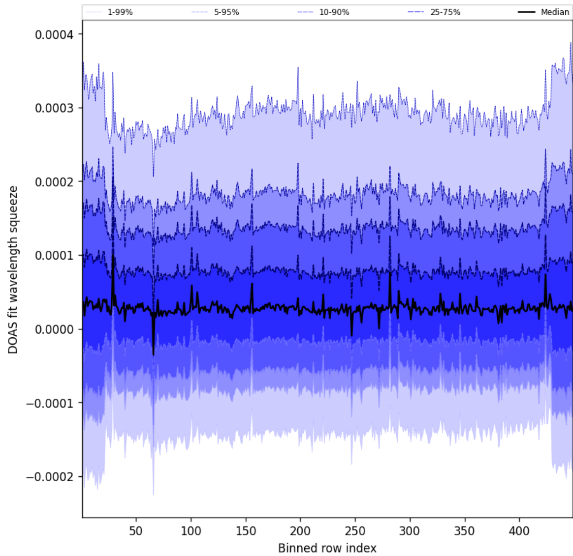
Figure 57: Along track statistics of “DOAS fit wavelength squeeze” for 2025-02-01 to 2025-02-02
