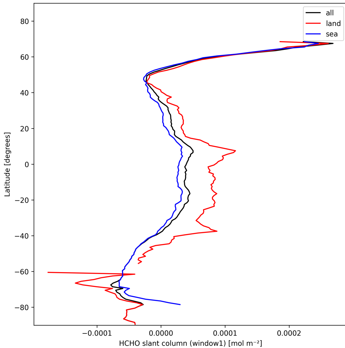
Figure 22: Zonal average of “HCHO slant column (window1)” for 2025-02-01 to 2025-02-02.
