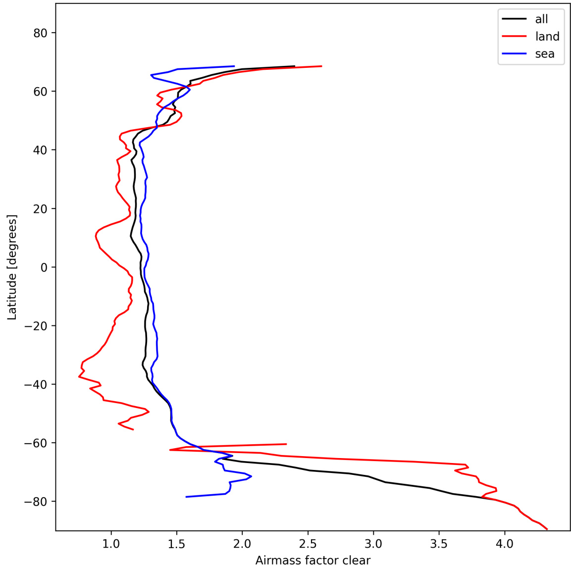
Figure 26: Zonal average of “Airmass factor clear” for 2025-02-01 to 2025-02-02.
