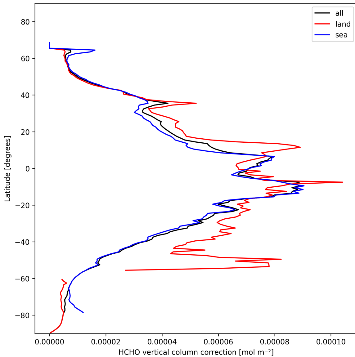
Figure 21: Zonal average of “HCHO vertical column correction” for 2025-02-01 to 2025-02-02.
