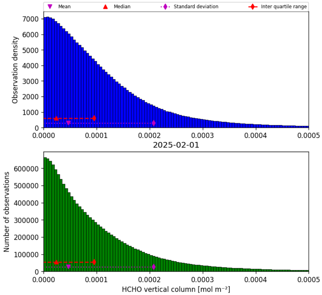
Figure 33: Histogram of “HCHO vertical column” for 2025-02-01 to 2025-02-02
