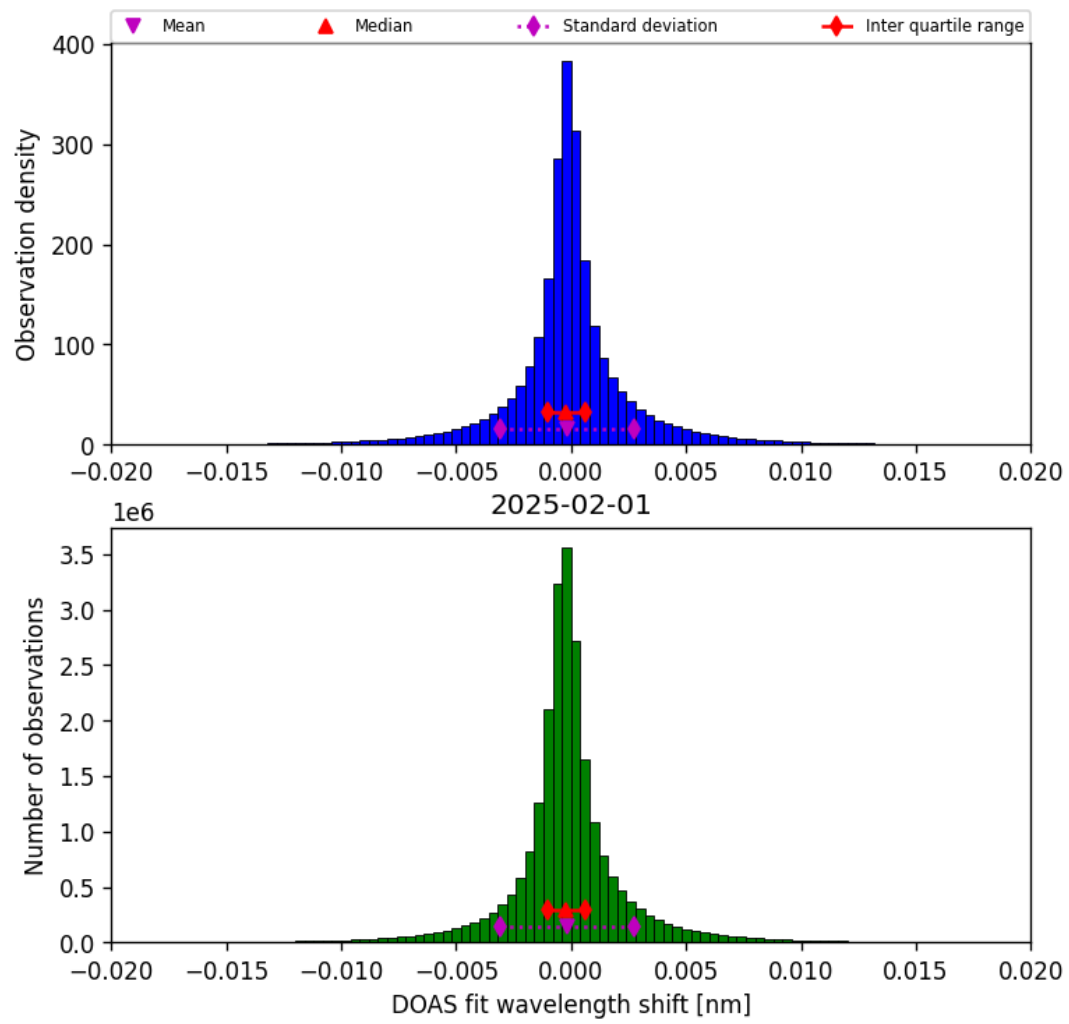
Figure 42: Histogram of “DOAS fit wavelength shift” for 2025-02-01 to 2025-02-02
