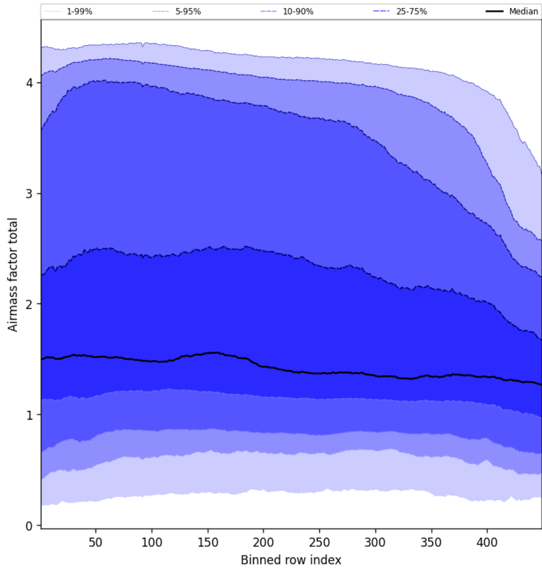
Figure 52: Along track statistics of “Airmass factor total” for 2025-02-01 to 2025-02-02
