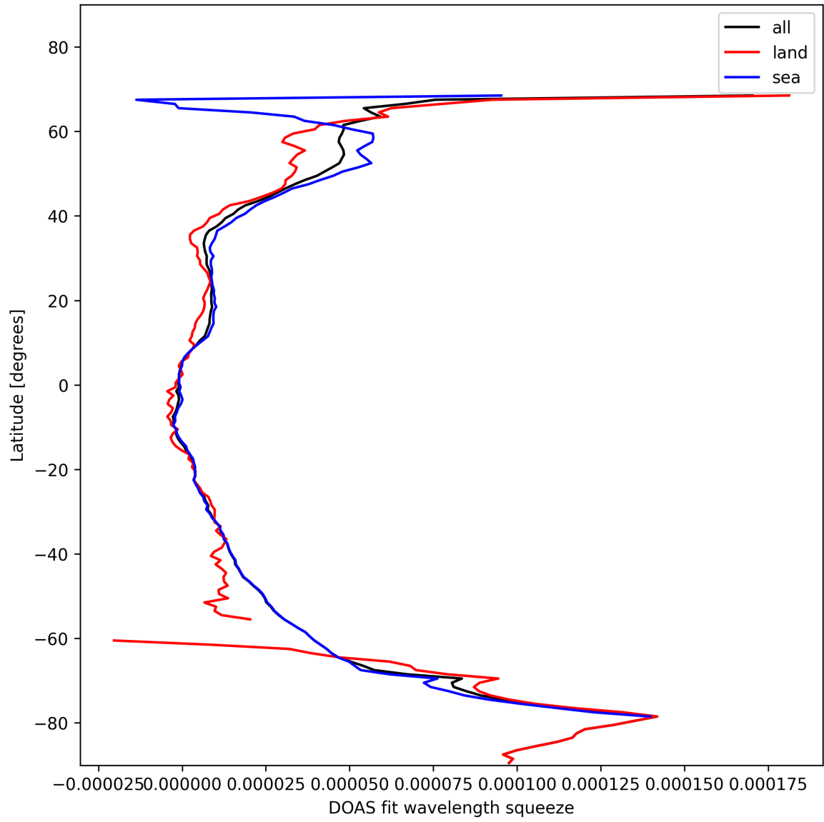
Figure 29: Zonal average of “DOAS fit wavelength squeeze” for 2025-02-01 to 2025-02-02.
