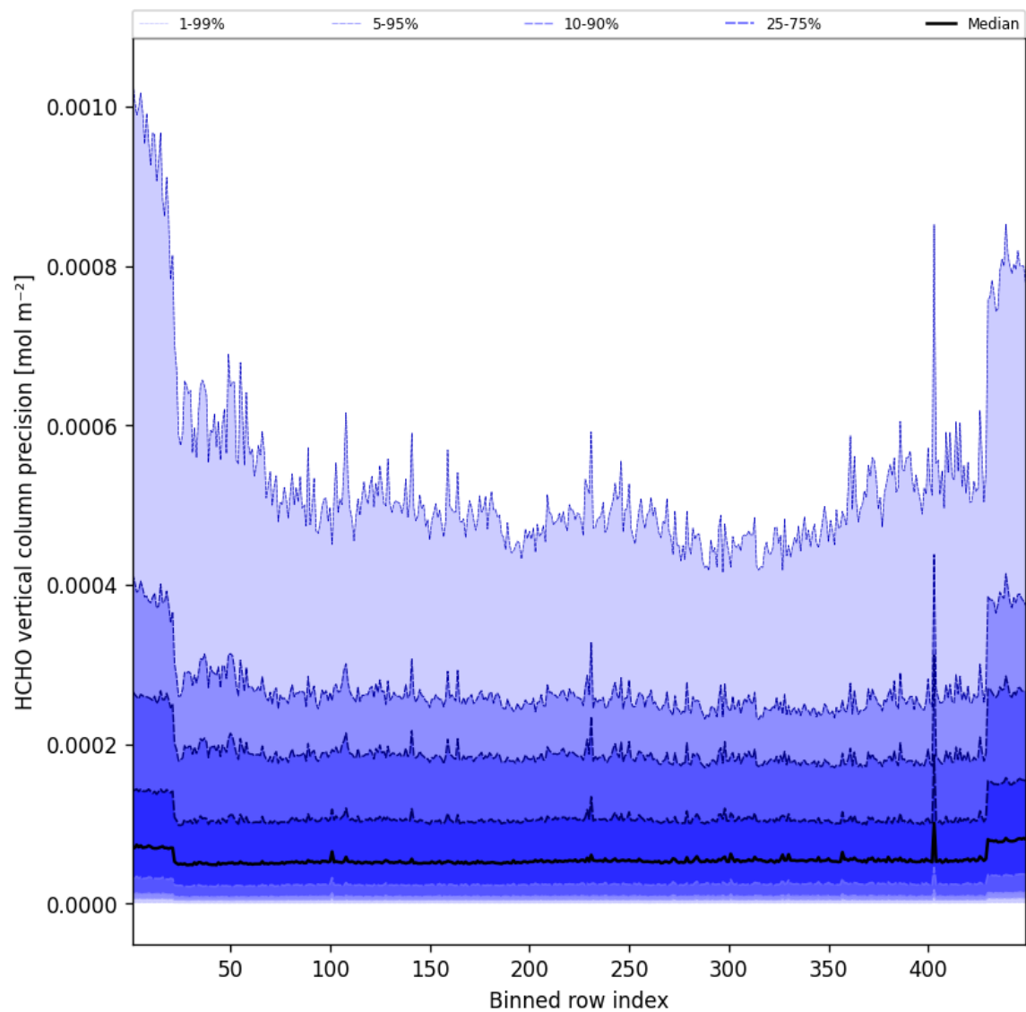
Figure 48: Along track statistics of “HCHO vertical column precision” for 2025-02-01 to 2025-02-02
