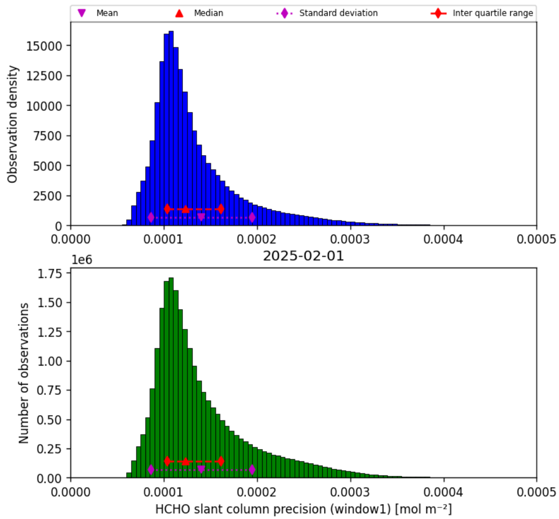
Figure 37: Histogram of “HCHO slant column precision (window1)” for 2025-02-01 to 2025-02-02
