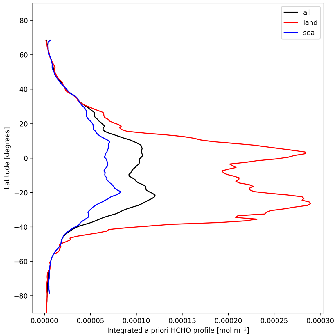
Figure 27: Zonal average of “Integrated a priori HCHO profile” for 2025-02-01 to 2025-02-02.
