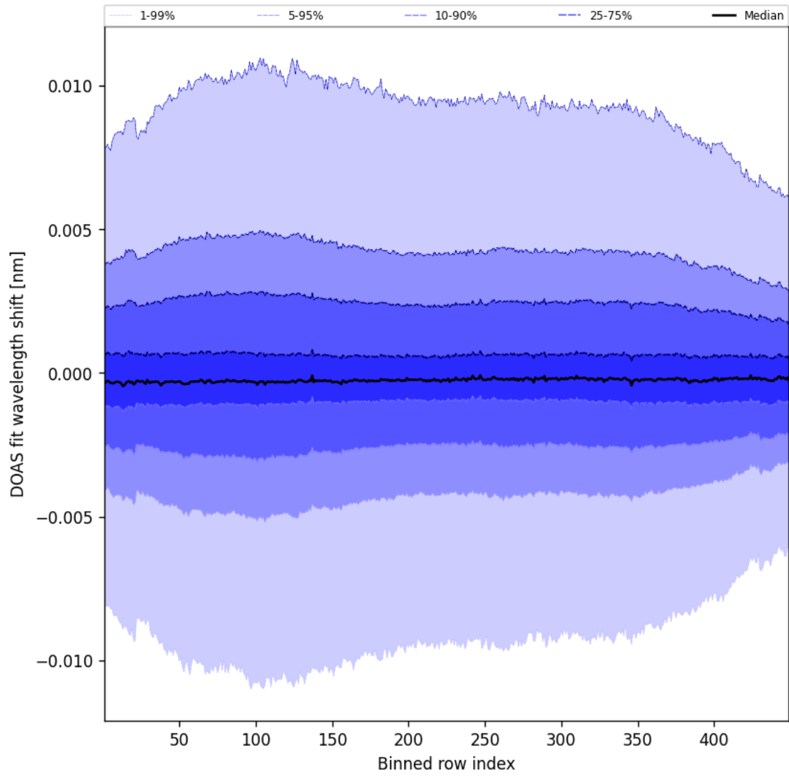
Figure 56: Along track statistics of “DOAS fit wavelength shift” for 2025-02-01 to 2025-02-02
