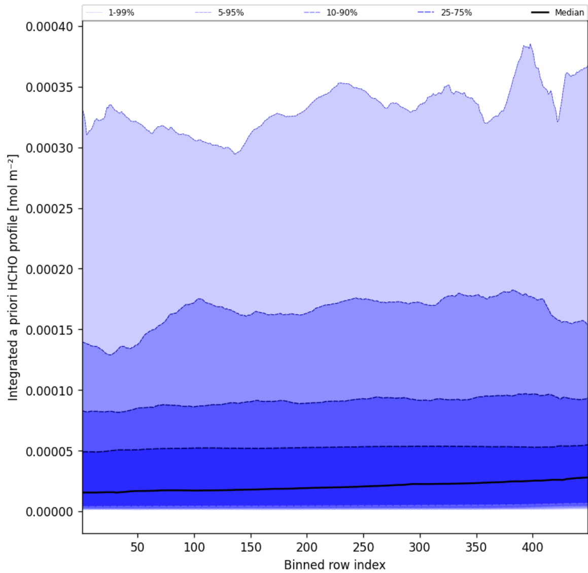
Figure 55: Along track statistics of “Integrated a priori HCHO profile” for 2025-02-01 to 2025-02-02
