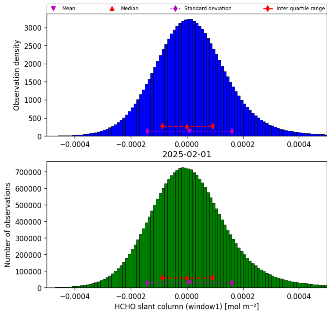
Figure 36: Histogram of “HCHO slant column (window1)” for 2025-02-01 to 2025-02-02
