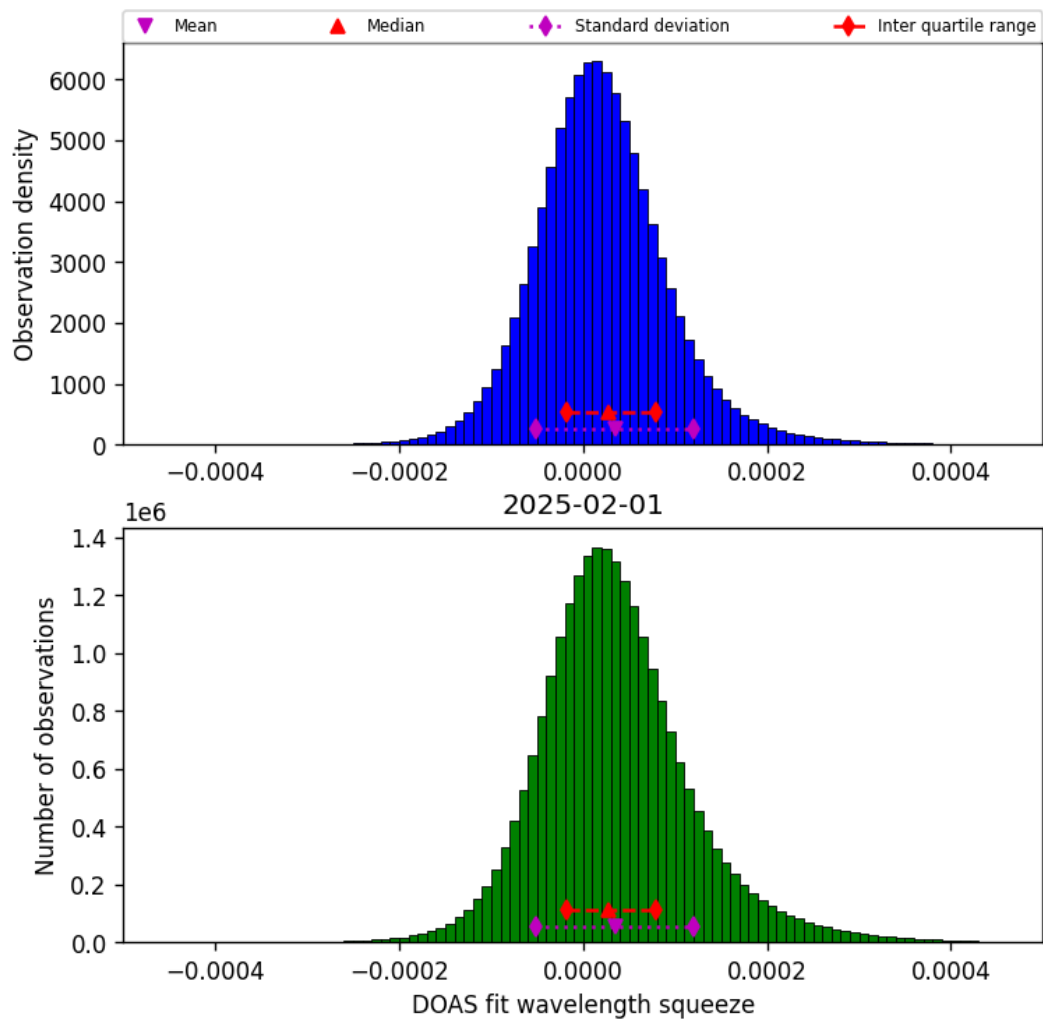
Figure 43: Histogram of “DOAS fit wavelength squeeze” for 2025-02-01 to 2025-02-02
