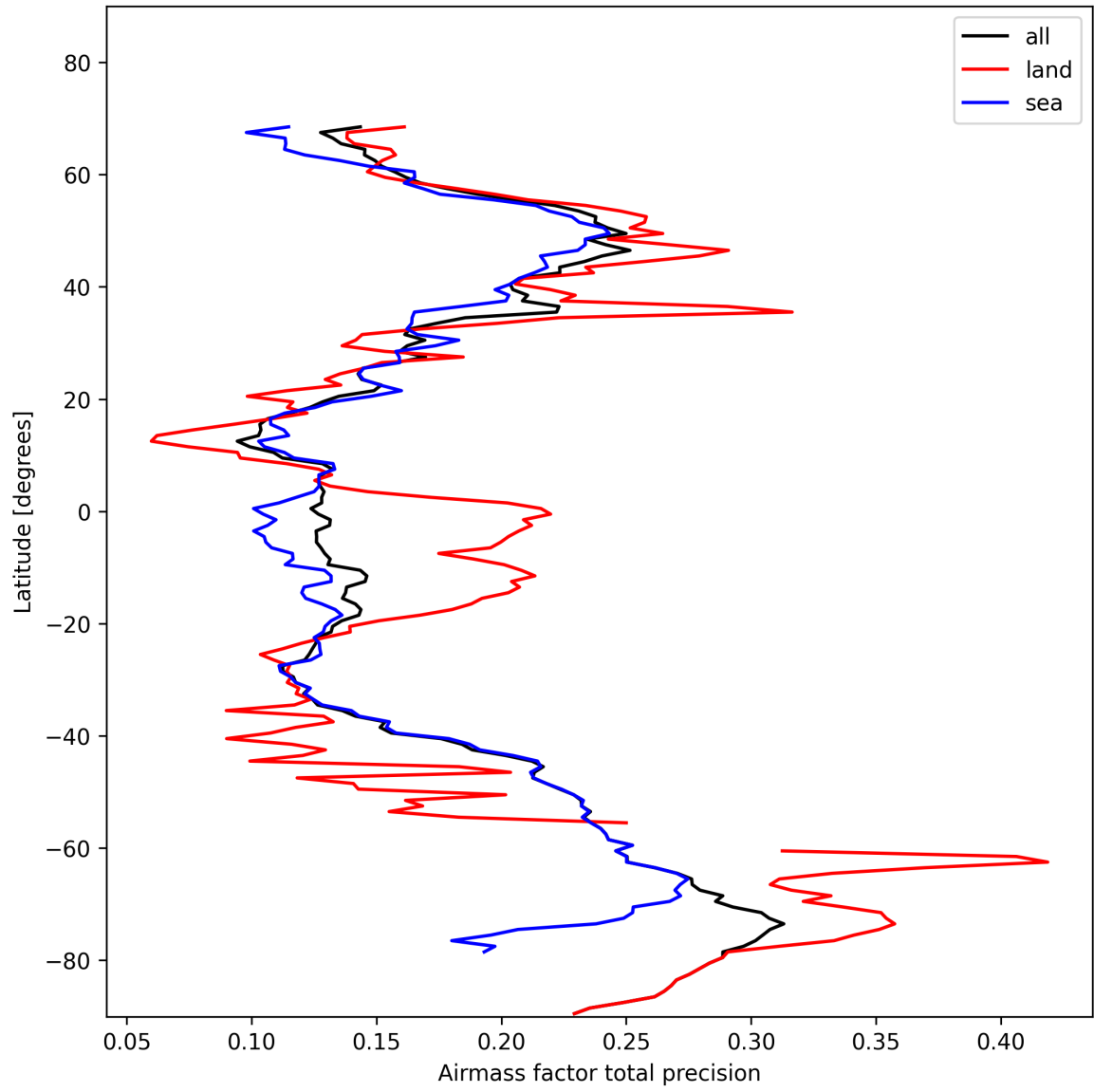
Figure 25: Zonal average of “Airmass factor total precision” for 2025-02-01 to 2025-02-02.
