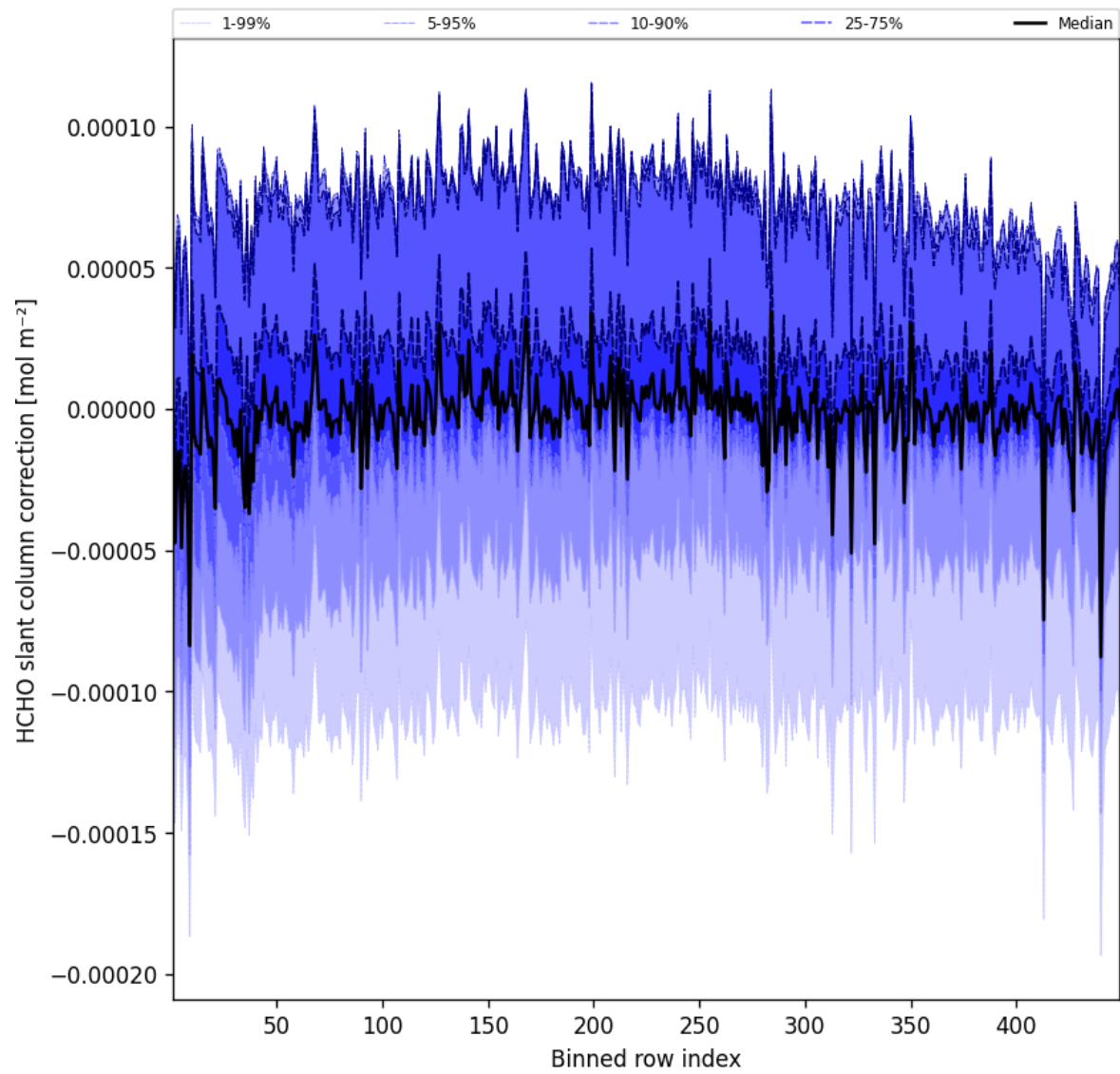
Figure 59: Along track statistics of “HCHO slant column correction” for 2025-02-01 to 2025-02-02
