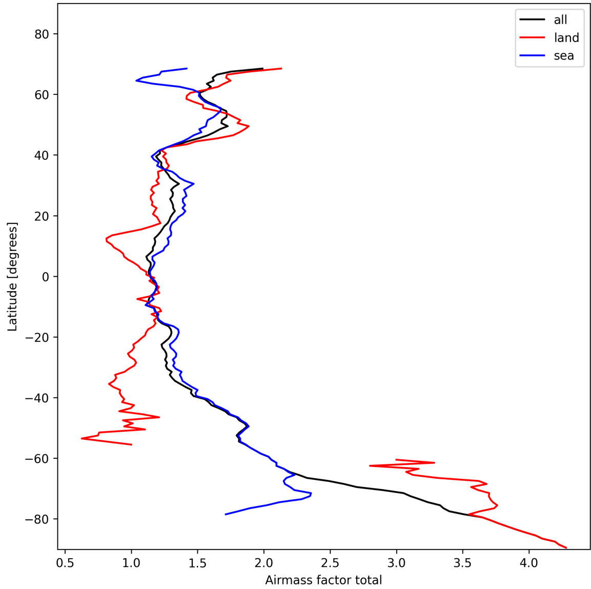
Figure 24: Zonal average of “Airmass factor total” for 2025-02-01 to 2025-02-02.
