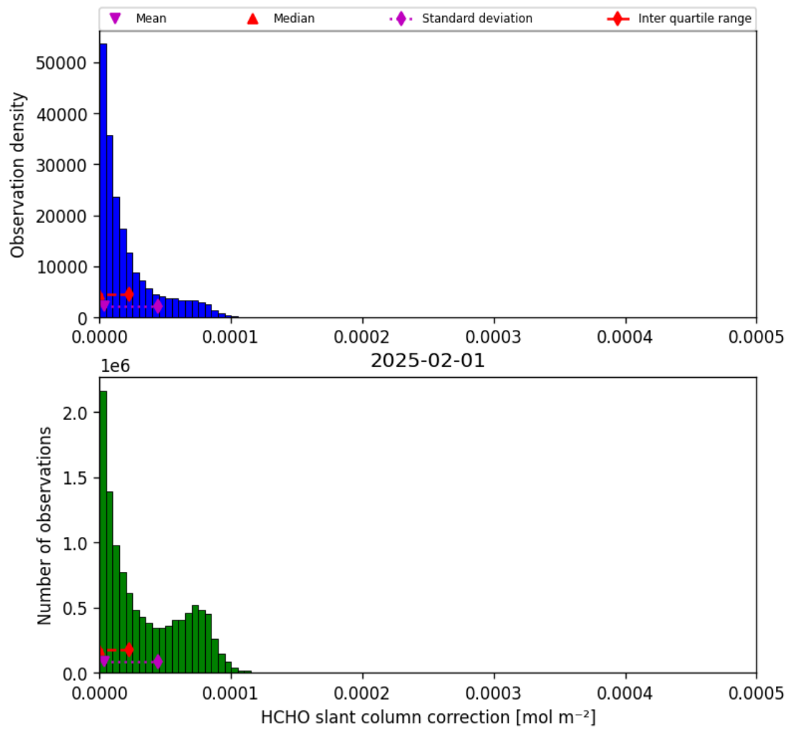
Figure 45: Histogram of “HCHO slant column correction” for 2025-02-01 to 2025-02-02
