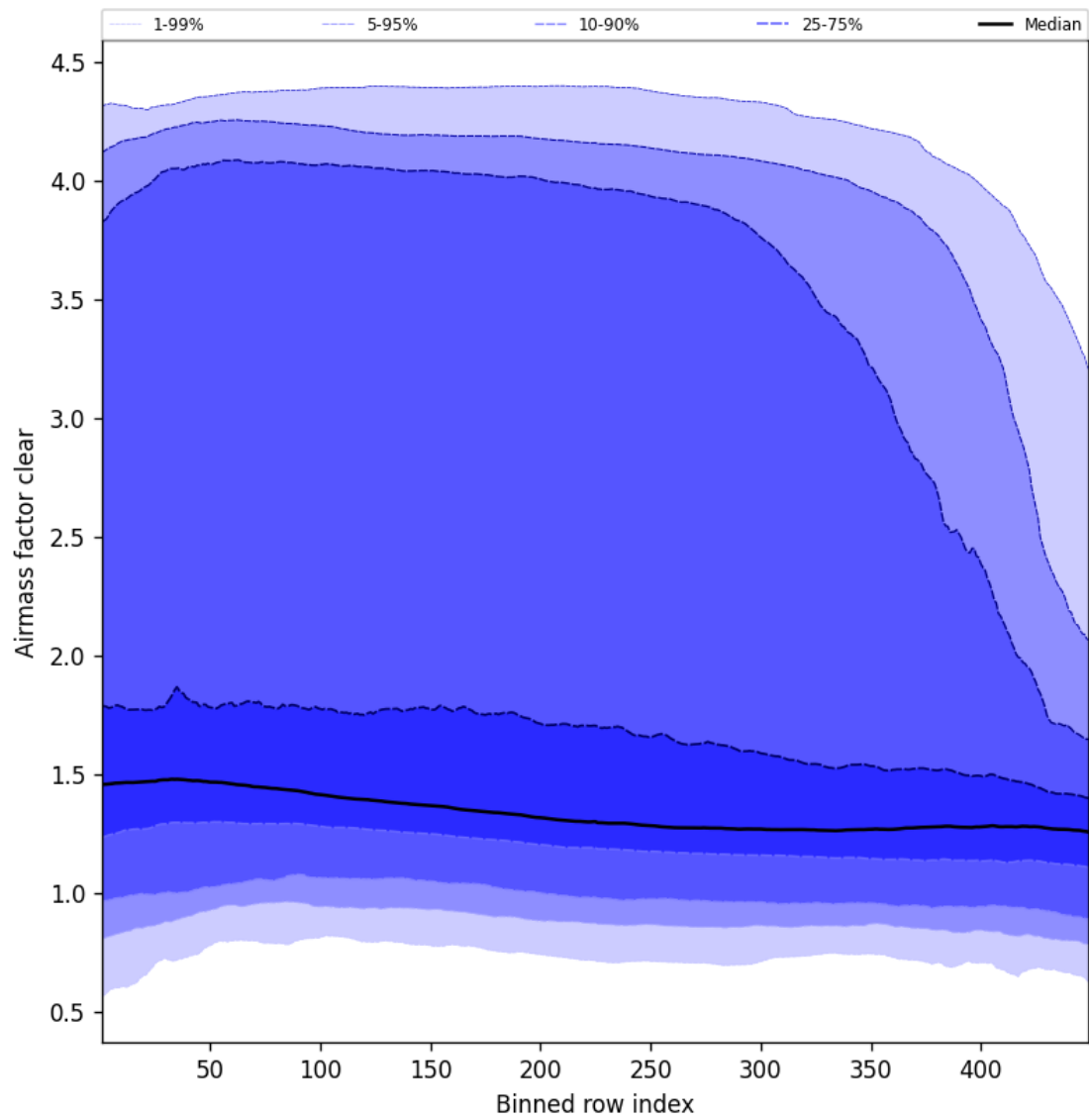
Figure 54: Along track statistics of “Airmass factor clear” for 2025-02-01 to 2025-02-02
