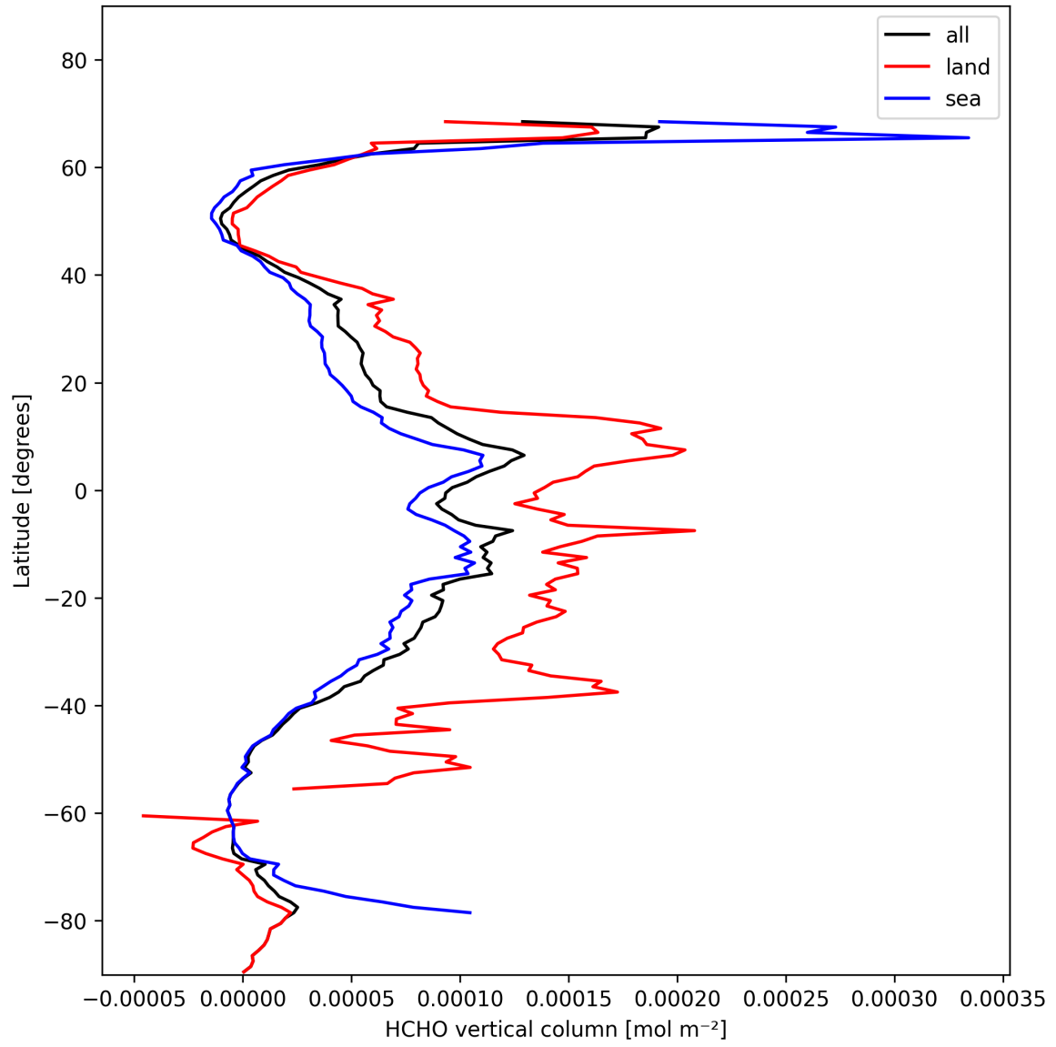
Figure 19: Zonal average of “HCHO vertical column” for 2025-02-01 to 2025-02-02.
