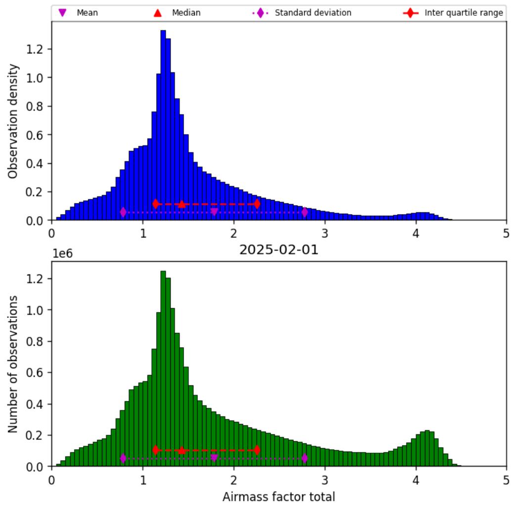
Figure 38: Histogram of “Airmass factor total” for 2025-02-01 to 2025-02-02
