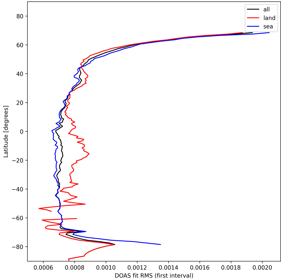
Figure 30: Zonal average of "DOAS fit RMS (first interval)" for 2025-02-01 to 2025-02-02.
