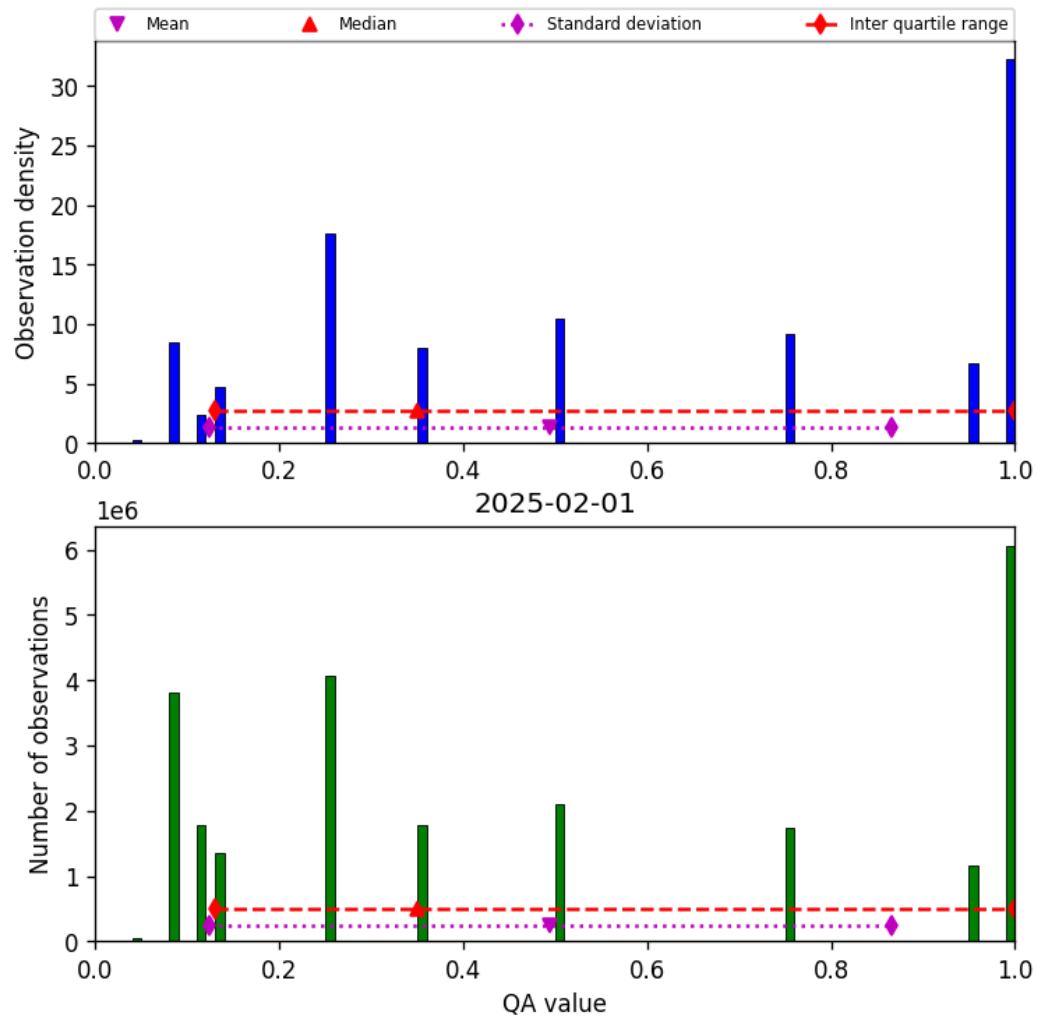
Figure 32: Histogram of “QA value” for 2025-02-01 to 2025-02-02
