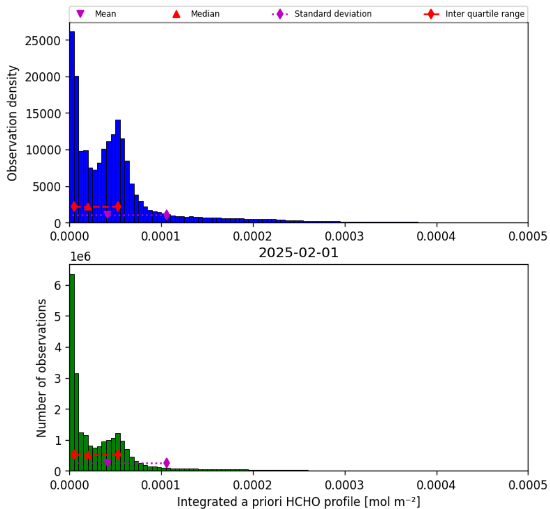
Figure 41: Histogram of “Integrated a priori HCHO profile” for 2025-02-01 to 2025-02-02
