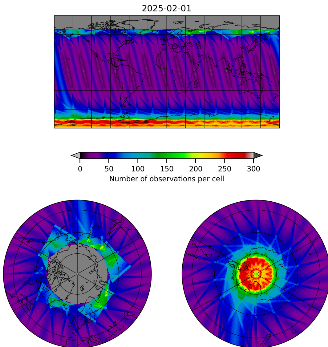
Figure 17: Map of the number of observations for 2025-02-01 to 2025-02-02
