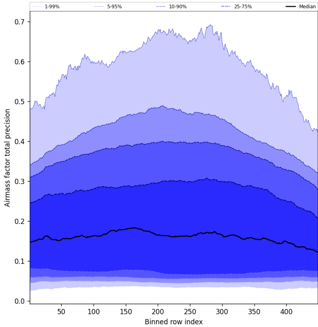
Figure 53: Along track statistics of “Airmass factor total precision” for 2025-02-01 to 2025-02-02
