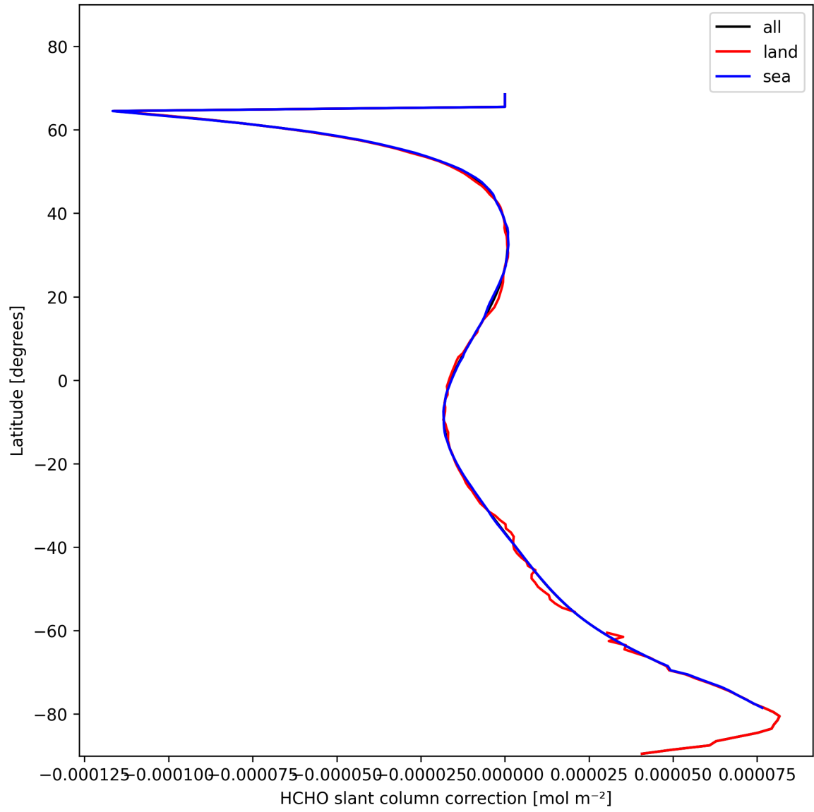
Figure 31: Zonal average of “HCHO slant column correction” for 2025-02-01 to 2025-02-02.
