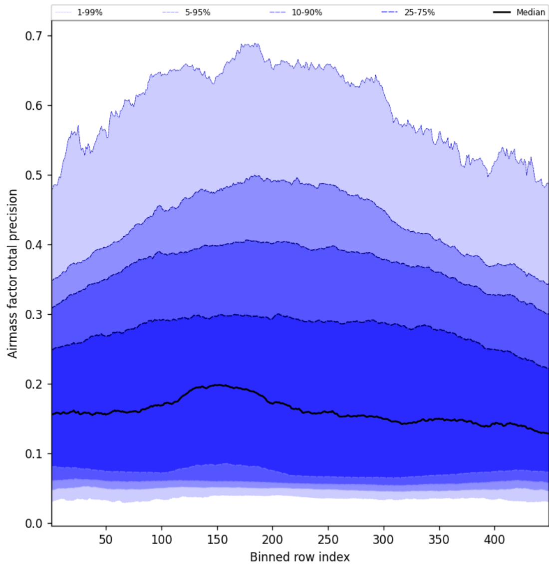
Figure 53: Along track statistics of “Airmass factor total precision” for 2025-02-04 to 2025-02-05
