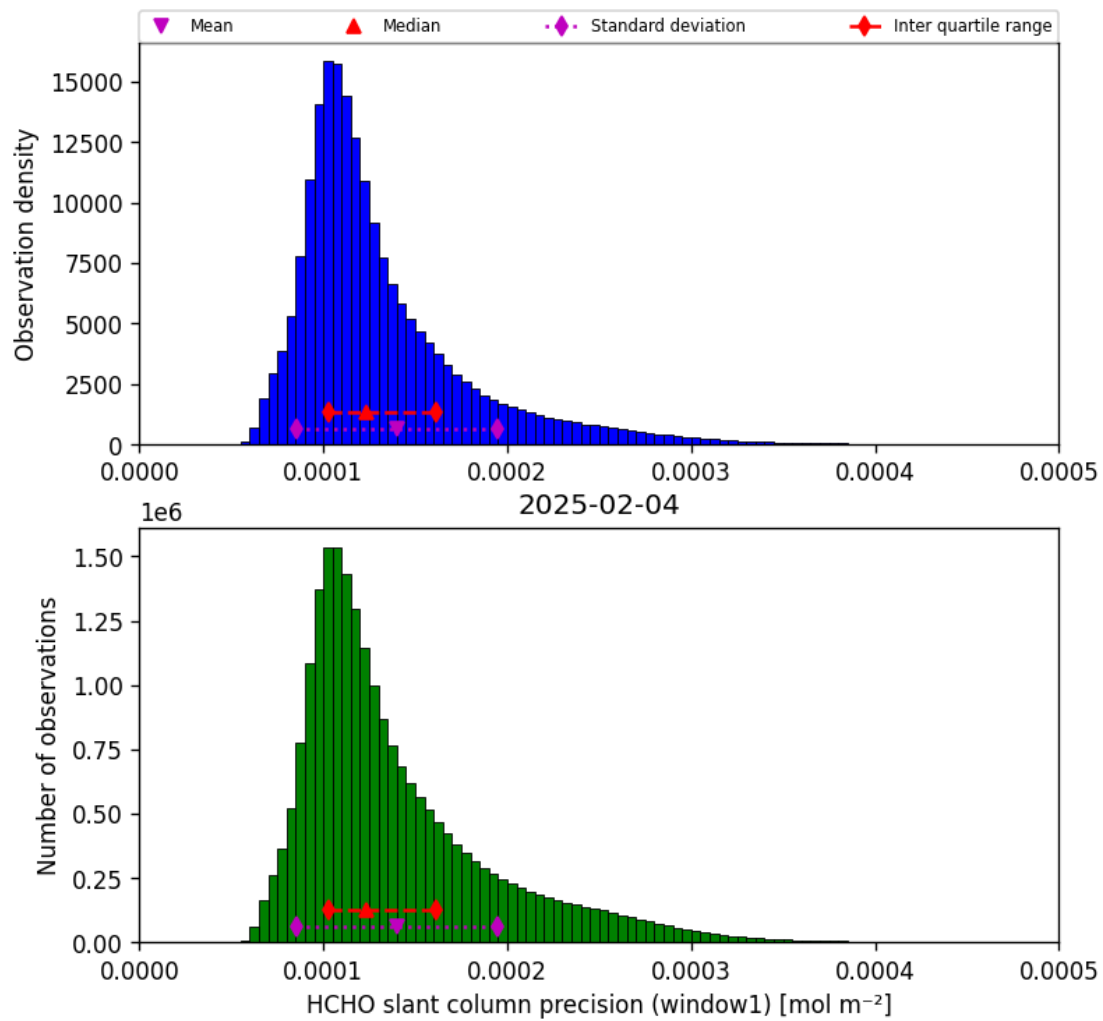
Figure 37: Histogram of “HCHO slant column precision (window1)” for 2025-02-04 to 2025-02-05
