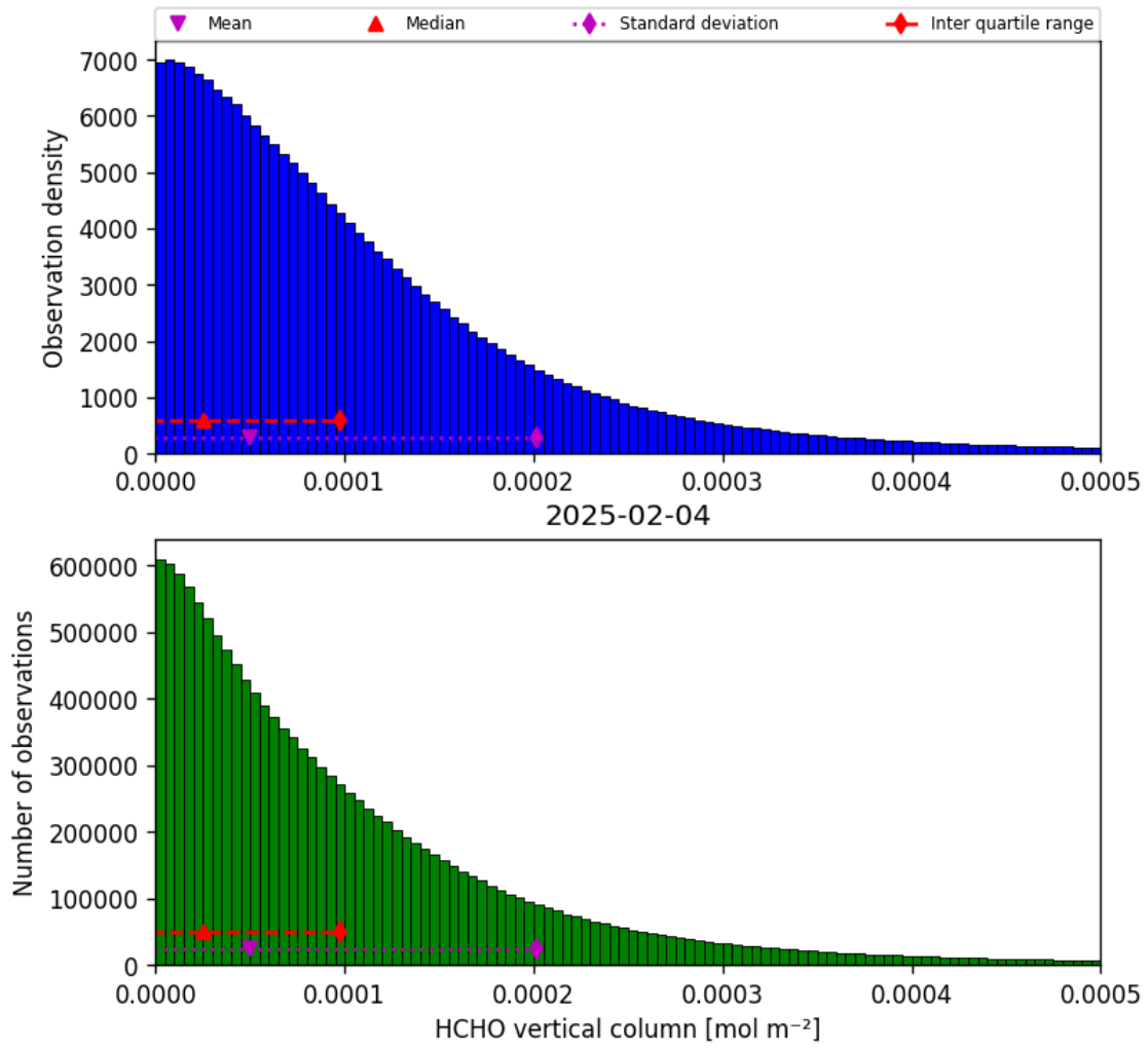
Figure 33: Histogram of “HCHO vertical column” for 2025-02-04 to 2025-02-05
