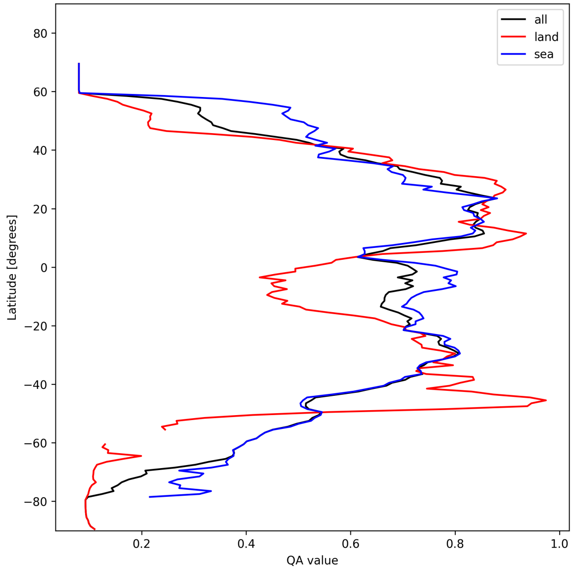
Figure 18: Zonal average of “QA value” for 2025-02-04 to 2025-02-05.
