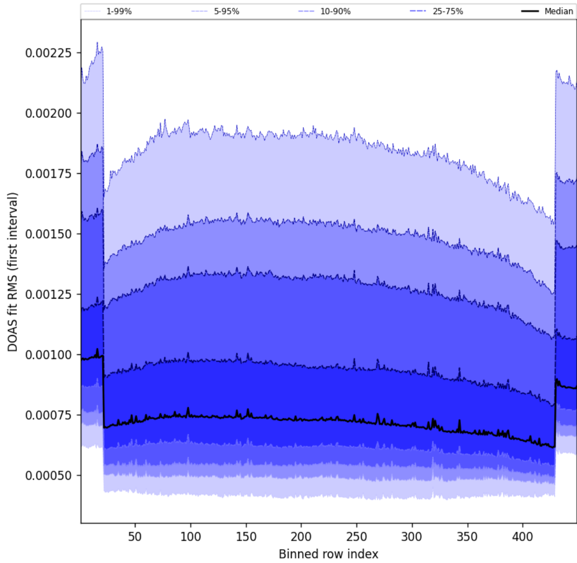
Figure 58: Along track statistics of “DOAS fit RMS (first interval)” for 2025-02-04 to 2025-02-05
