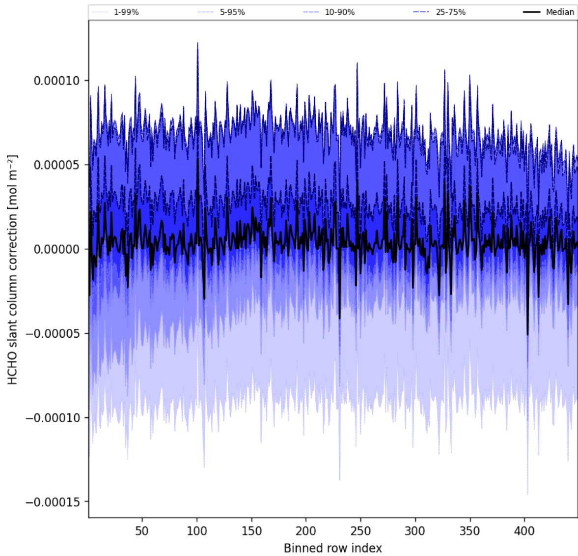
Figure 59: Along track statistics of “HCHO slant column correction” for 2025-02-04 to 2025-02-05
