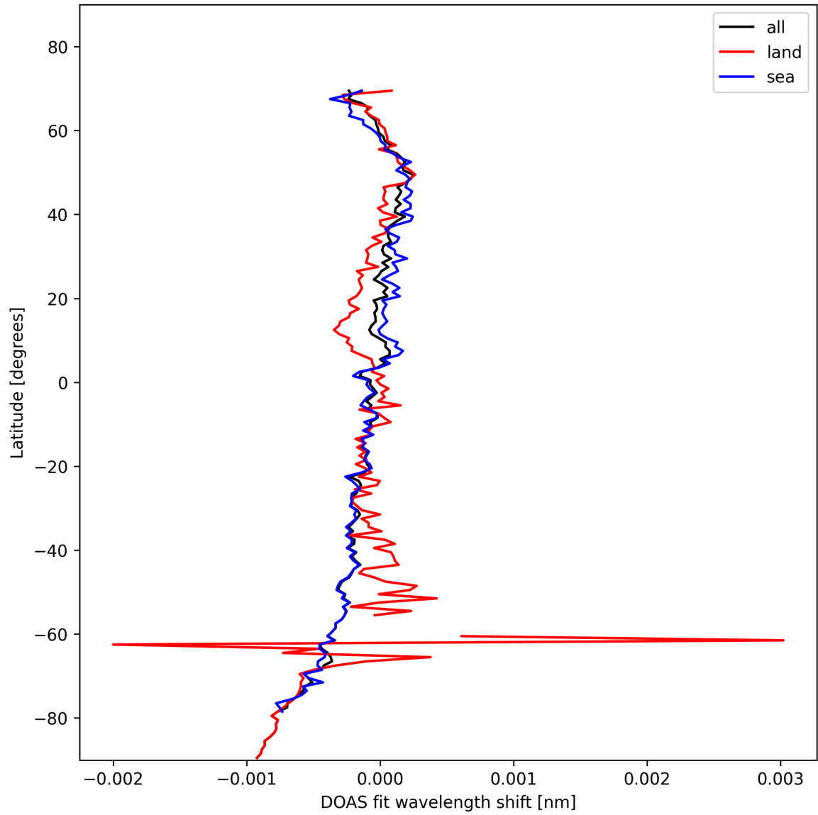
Figure 28: Zonal average of “DOAS fit wavelength shift” for 2025-02-04 to 2025-02-05.
