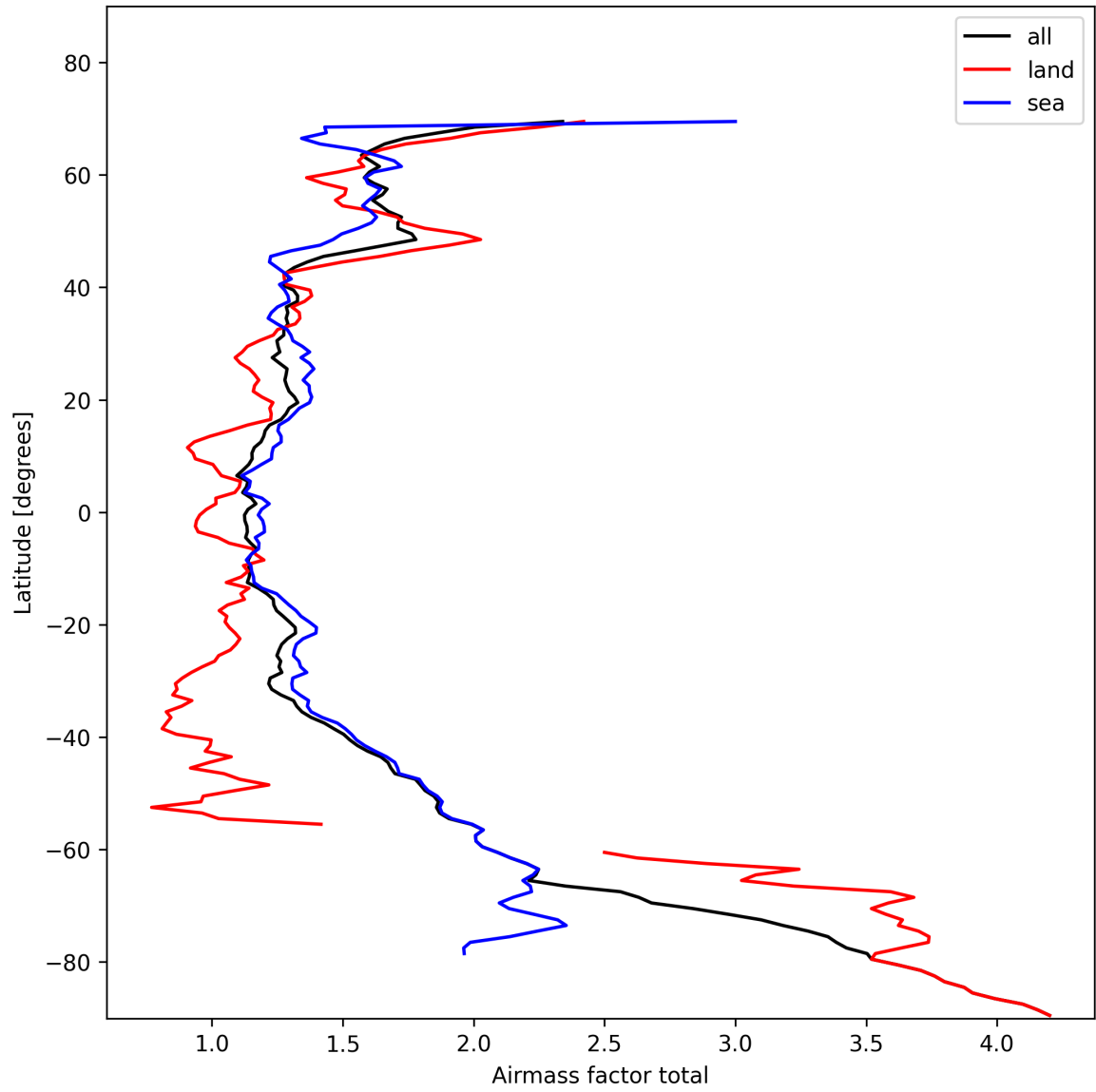
Figure 24: Zonal average of “Airmass factor total” for 2025-02-04 to 2025-02-05.
