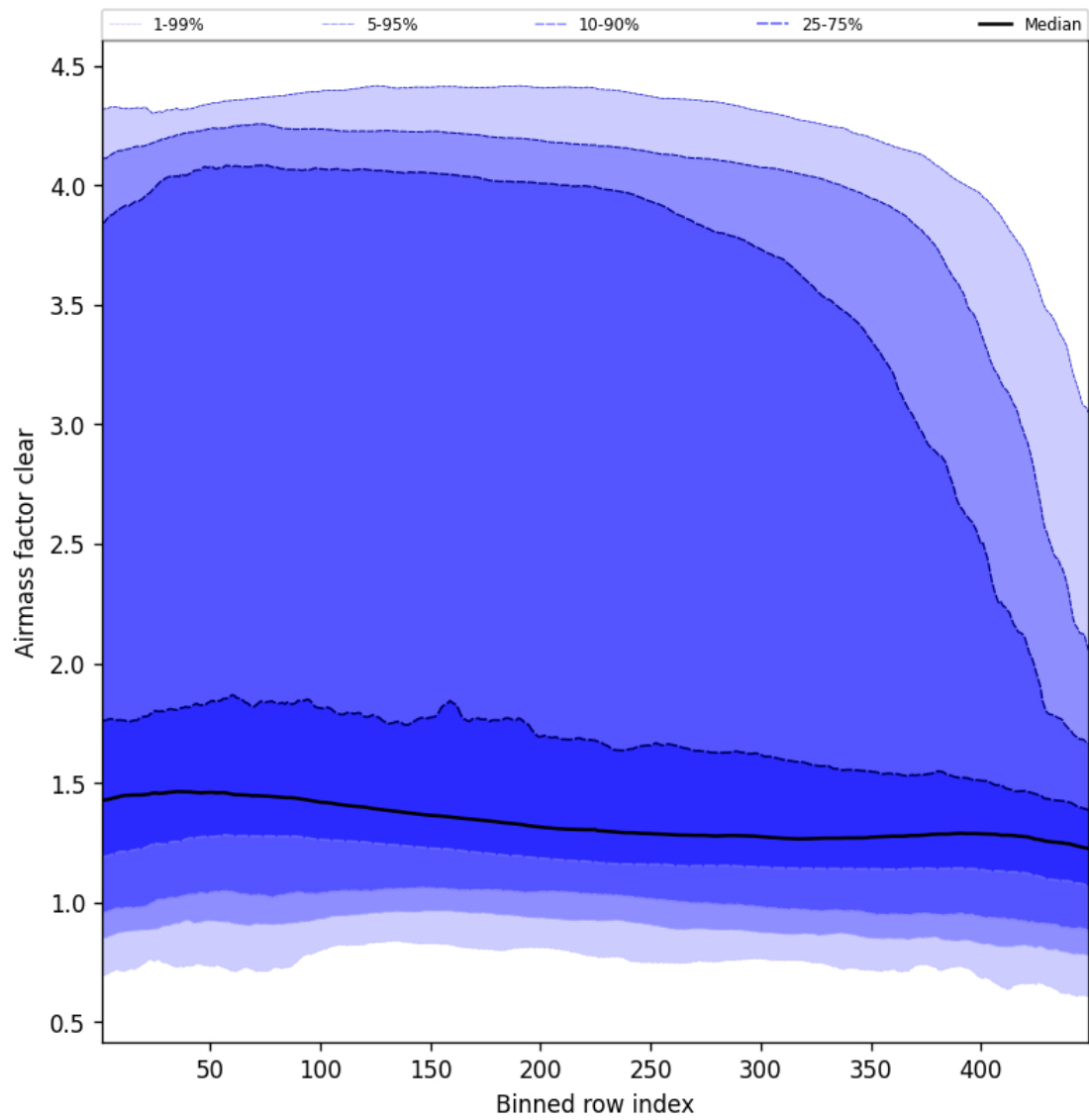
Figure 54: Along track statistics of “Airmass factor clear” for 2025-02-04 to 2025-02-05
