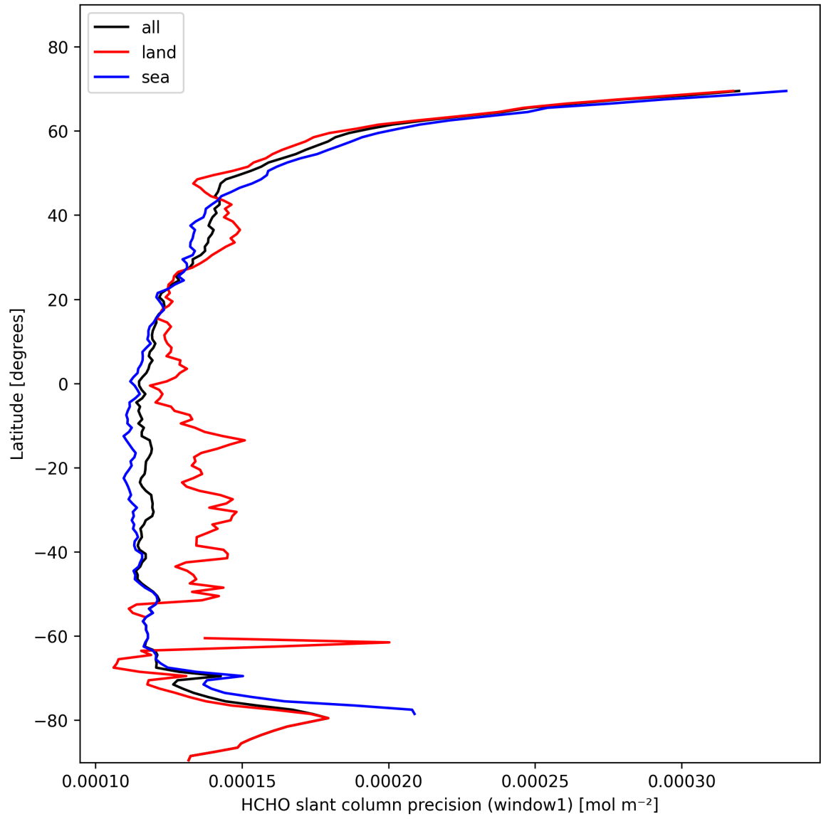
Figure 23: Zonal average of “HCHO slant column precision (window1)” for 2025-02-04 to 2025-02-05.
