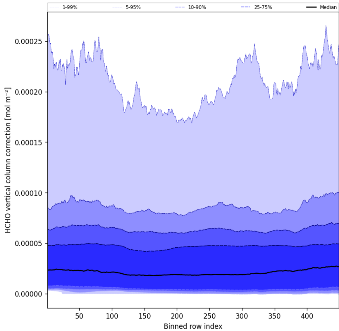
Figure 49: Along track statistics of "HCHO vertical column correction" for 2025-02-04 to 2025-02-05
