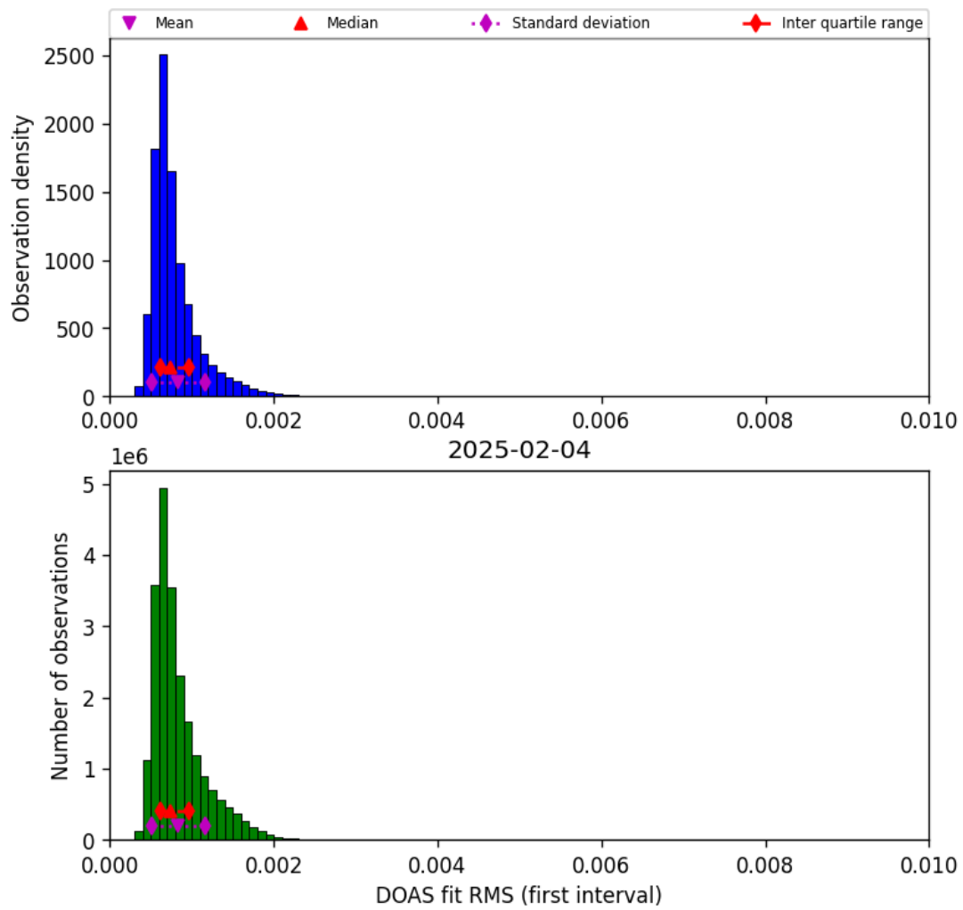
Figure 44: Histogram of “DOAS fit RMS (first interval)” for 2025-02-04 to 2025-02-05
