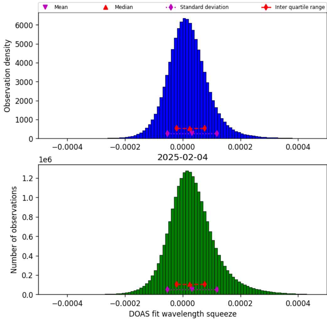
Figure 43: Histogram of “DOAS fit wavelength squeeze” for 2025-02-04 to 2025-02-05
