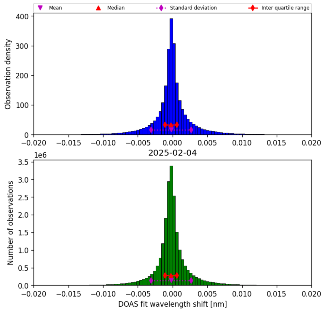
Figure 42: Histogram of “DOAS fit wavelength shift” for 2025-02-04 to 2025-02-05
