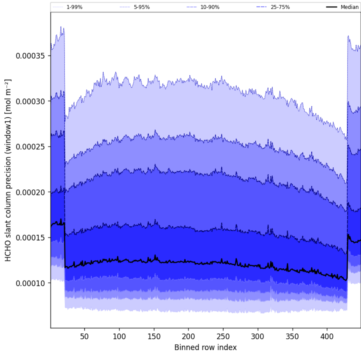
Figure 51: Along track statistics of "HCHO slant column precision (window1)" for 2025-02-04 to 2025-02-05
