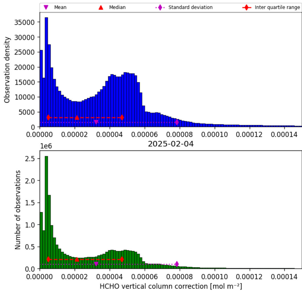
Figure 35: Histogram of “HCHO vertical column correction” for 2025-02-04 to 2025-02-05
