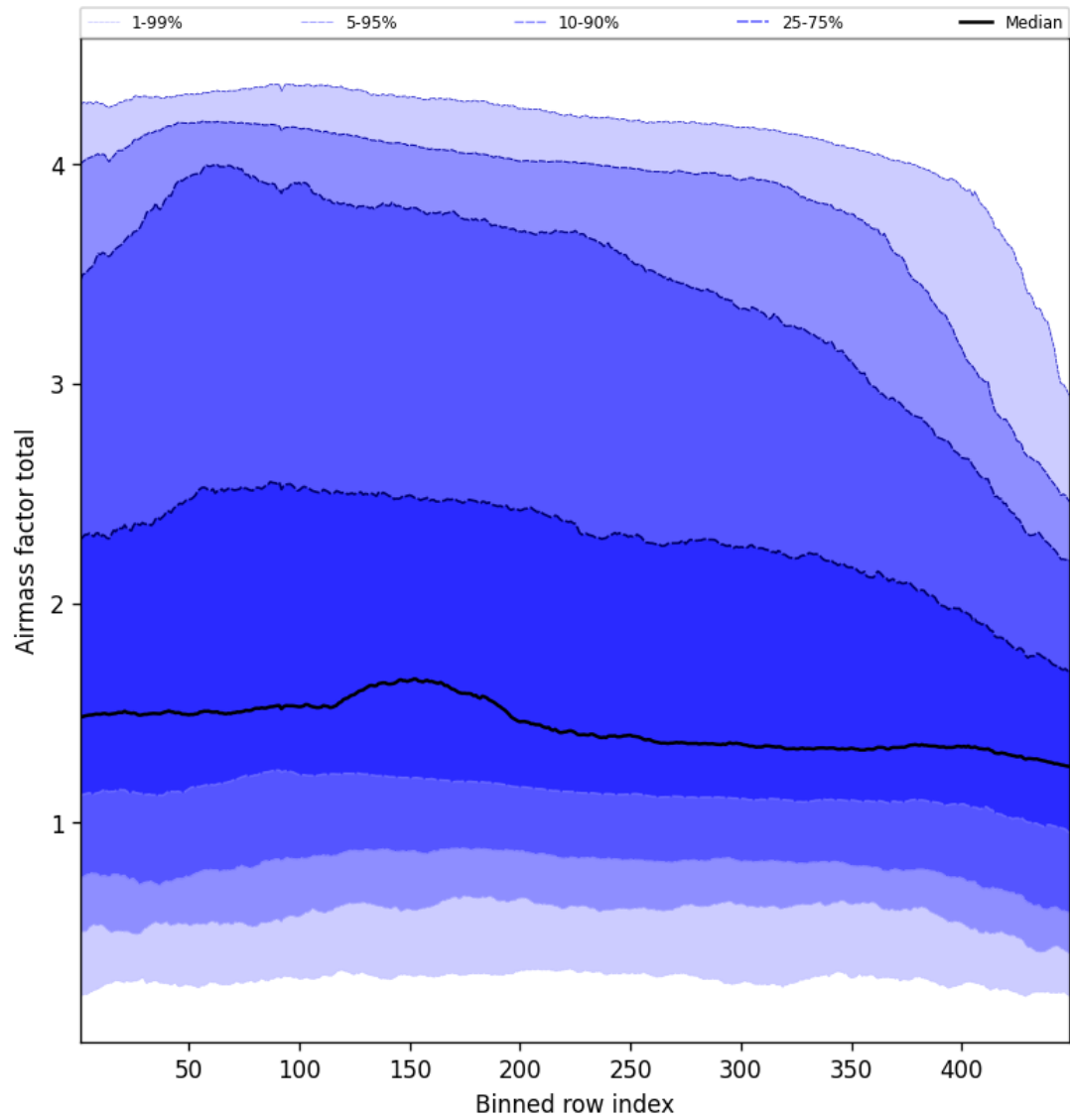
Figure 52: Along track statistics of “Airmass factor total” for 2025-02-04 to 2025-02-05
