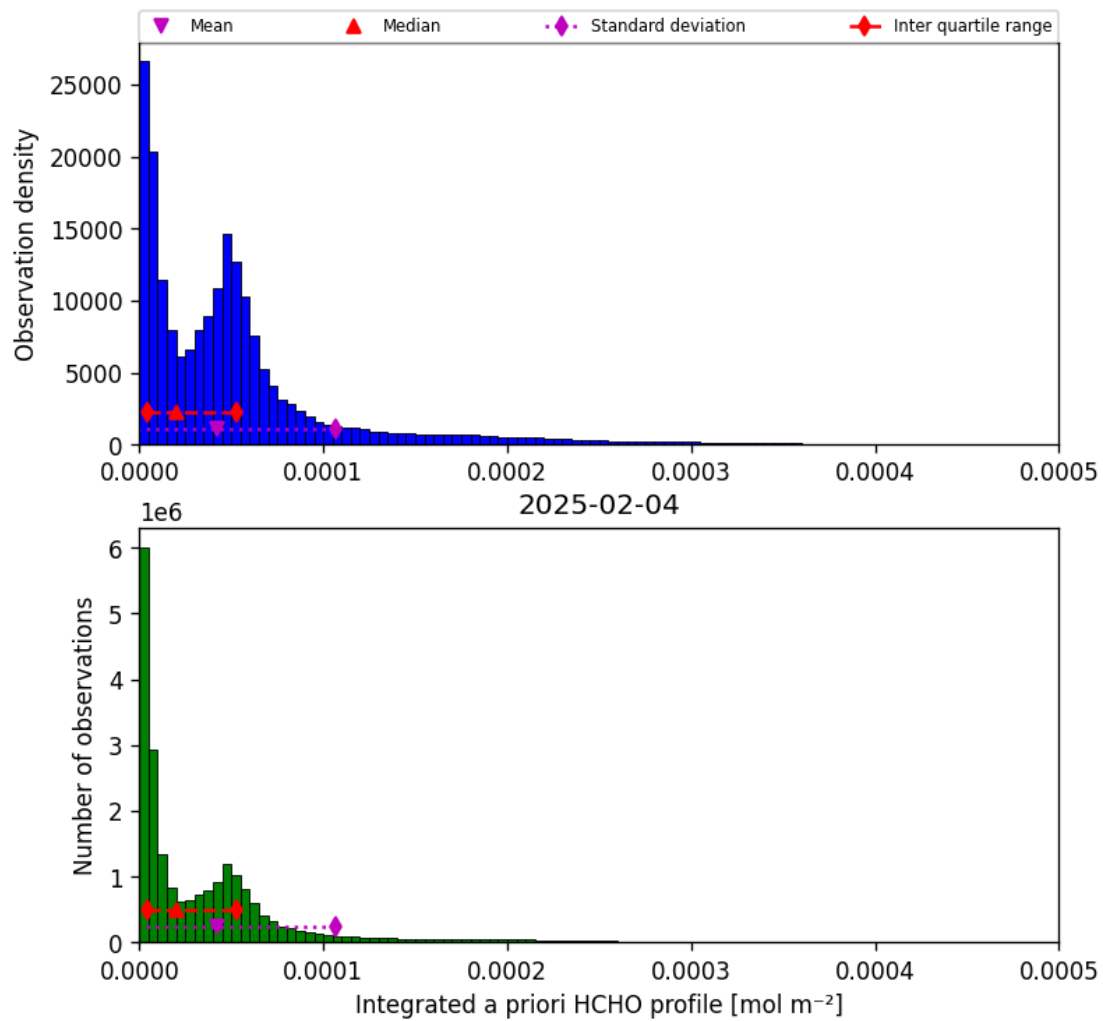
Figure 41: Histogram of “Integrated a priori HCHO profile” for 2025-02-04 to 2025-02-05
