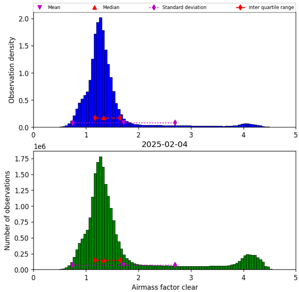
Figure 40: Histogram of “Airmass factor clear” for 2025-02-04 to 2025-02-05
