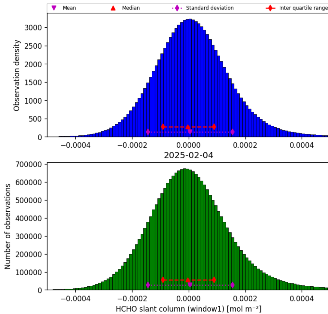
Figure 36: Histogram of “HCHO slant column (window1)” for 2025-02-04 to 2025-02-05
