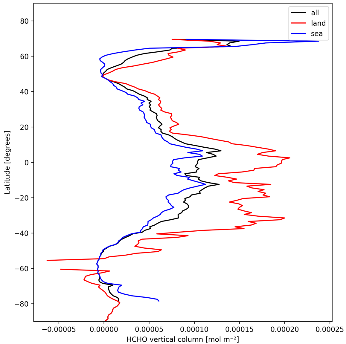
Figure 19: Zonal average of “HCHO vertical column” for 2025-02-04 to 2025-02-05.
