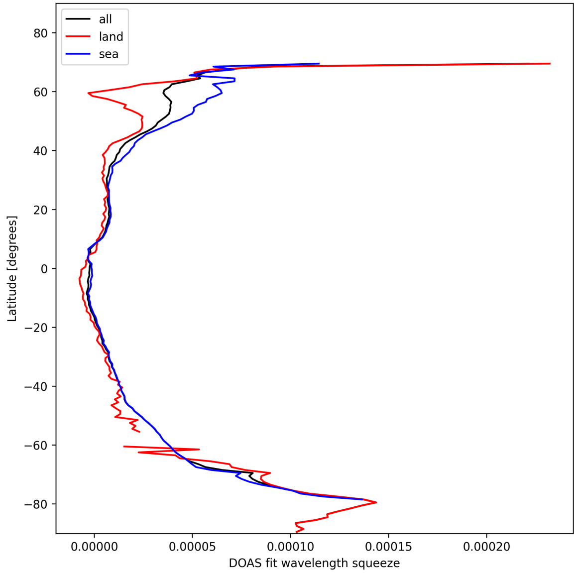
Figure 29: Zonal average of “DOAS fit wavelength squeeze” for 2025-02-04 to 2025-02-05.
