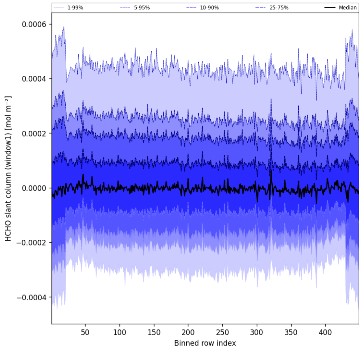
Figure 50: Along track statistics of “HCHO slant column (window1)” for 2025-02-04 to 2025-02-05
