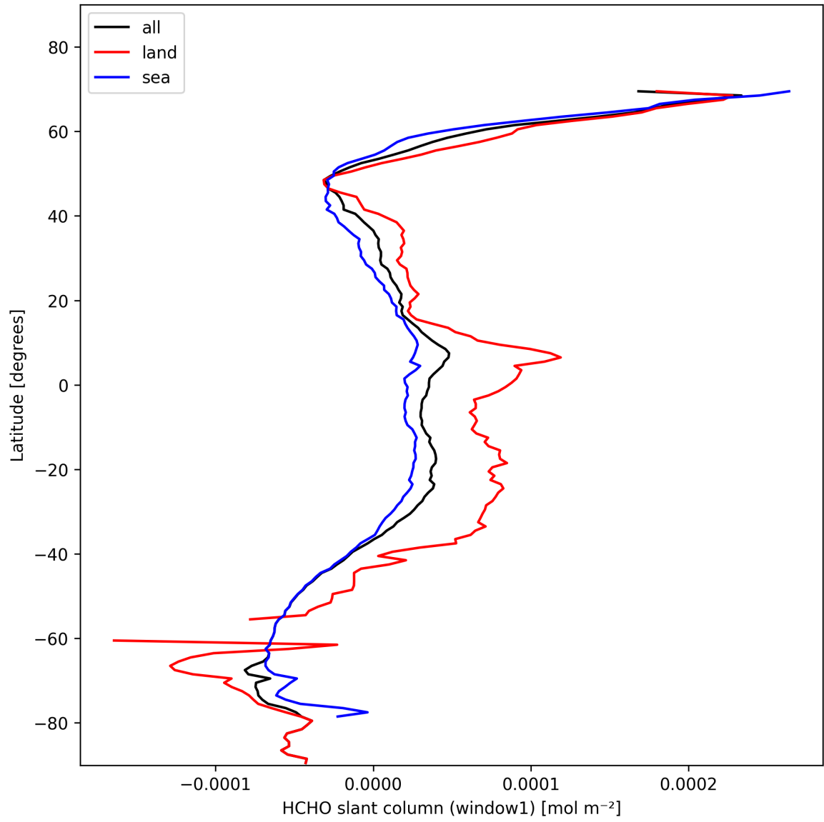
Figure 22: Zonal average of “HCHO slant column (window1)” for 2025-02-04 to 2025-02-05.
