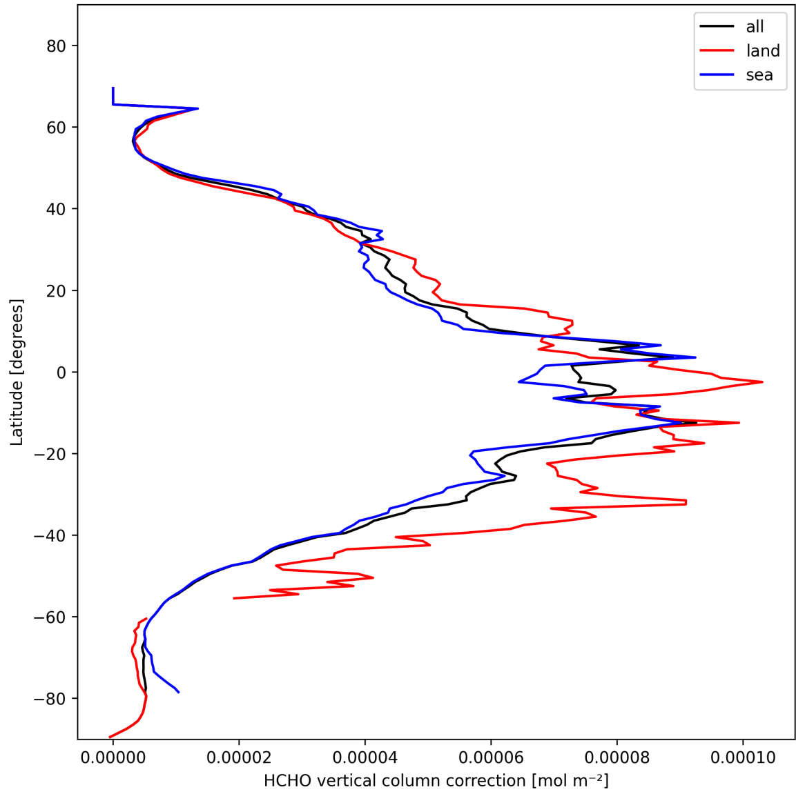
Figure 21: Zonal average of “HCHO vertical column correction” for 2025-02-04 to 2025-02-05.
