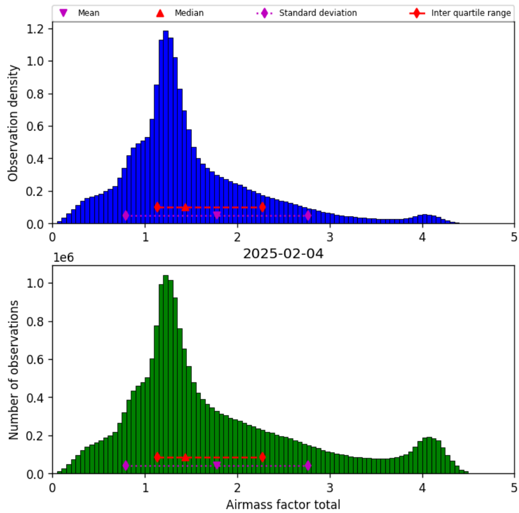
Figure 38: Histogram of “Airmass factor total” for 2025-02-04 to 2025-02-05
