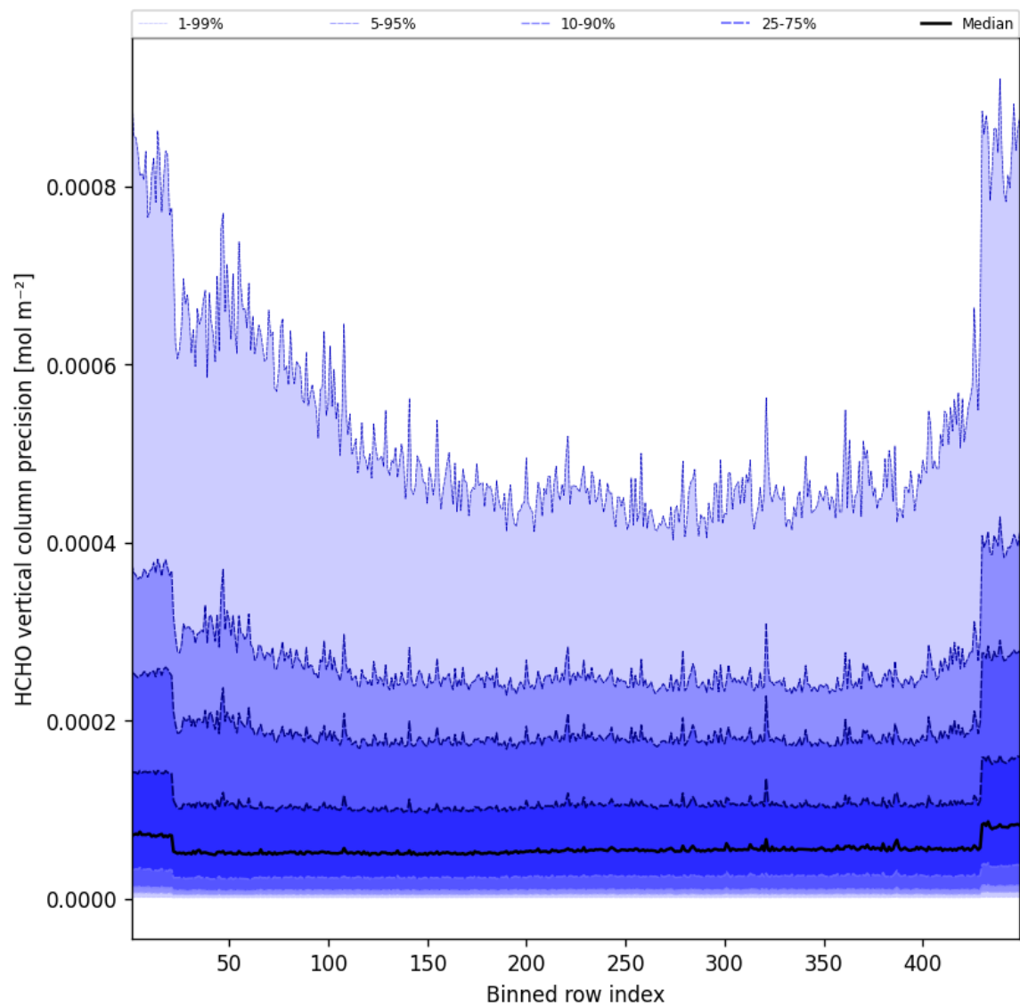
Figure 48: Along track statistics of “HCHO vertical column precision” for 2025-02-04 to 2025-02-05
