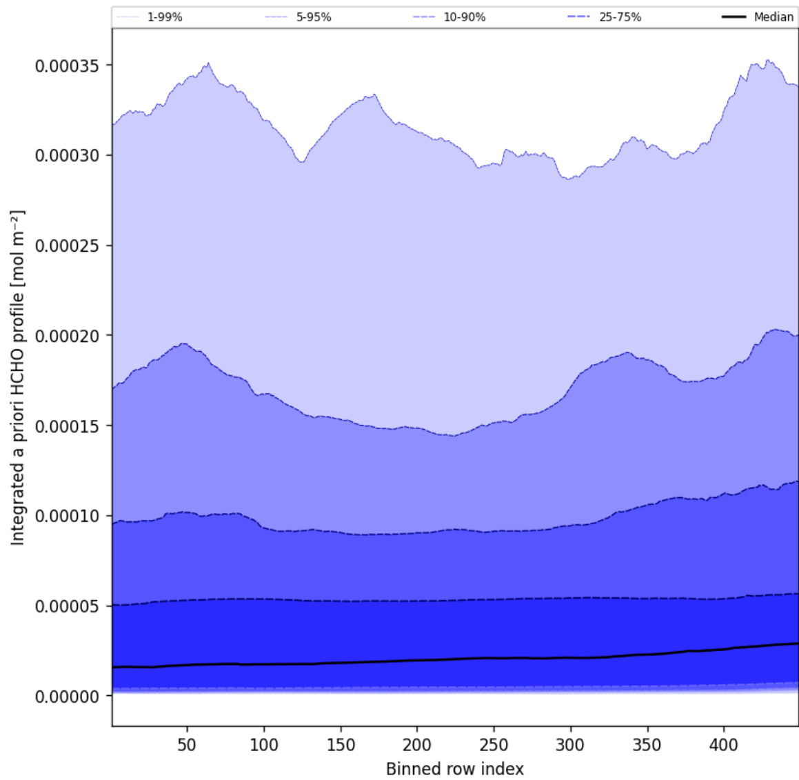
Figure 55: Along track statistics of “Integrated a priori HCHO profile” for 2025-02-04 to 2025-02-05
