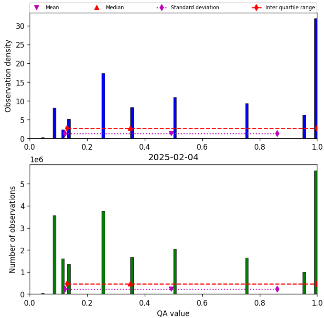
Figure 32: Histogram of “QA value” for 2025-02-04 to 2025-02-05
