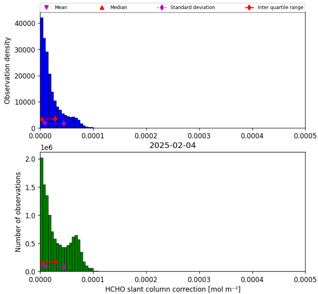
Figure 45: Histogram of “HCHO slant column correction” for 2025-02-04 to 2025-02-05
