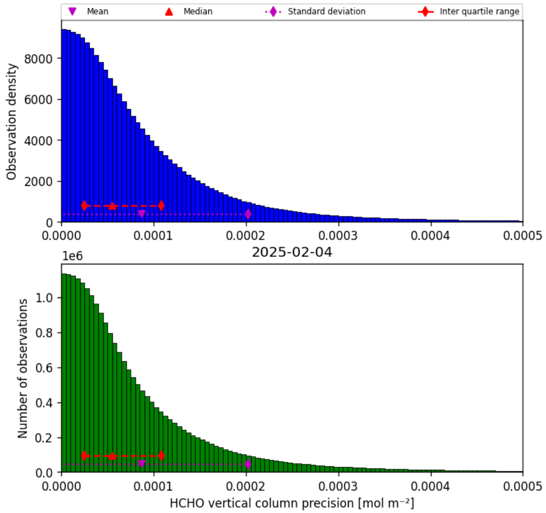
Figure 34: Histogram of “HCHO vertical column precision” for 2025-02-04 to 2025-02-05
