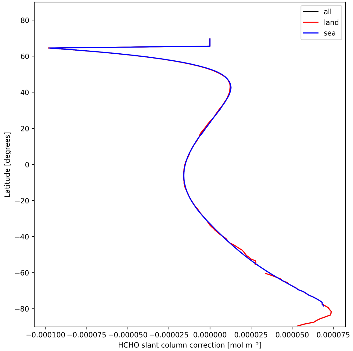
Figure 31: Zonal average of “HCHO slant column correction” for 2025-02-04 to 2025-02-05.
