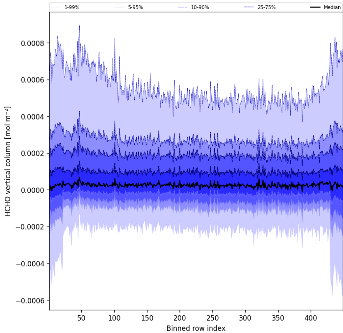
Figure 47: Along track statistics of “HCHO vertical column” for 2025-02-04 to 2025-02-05
