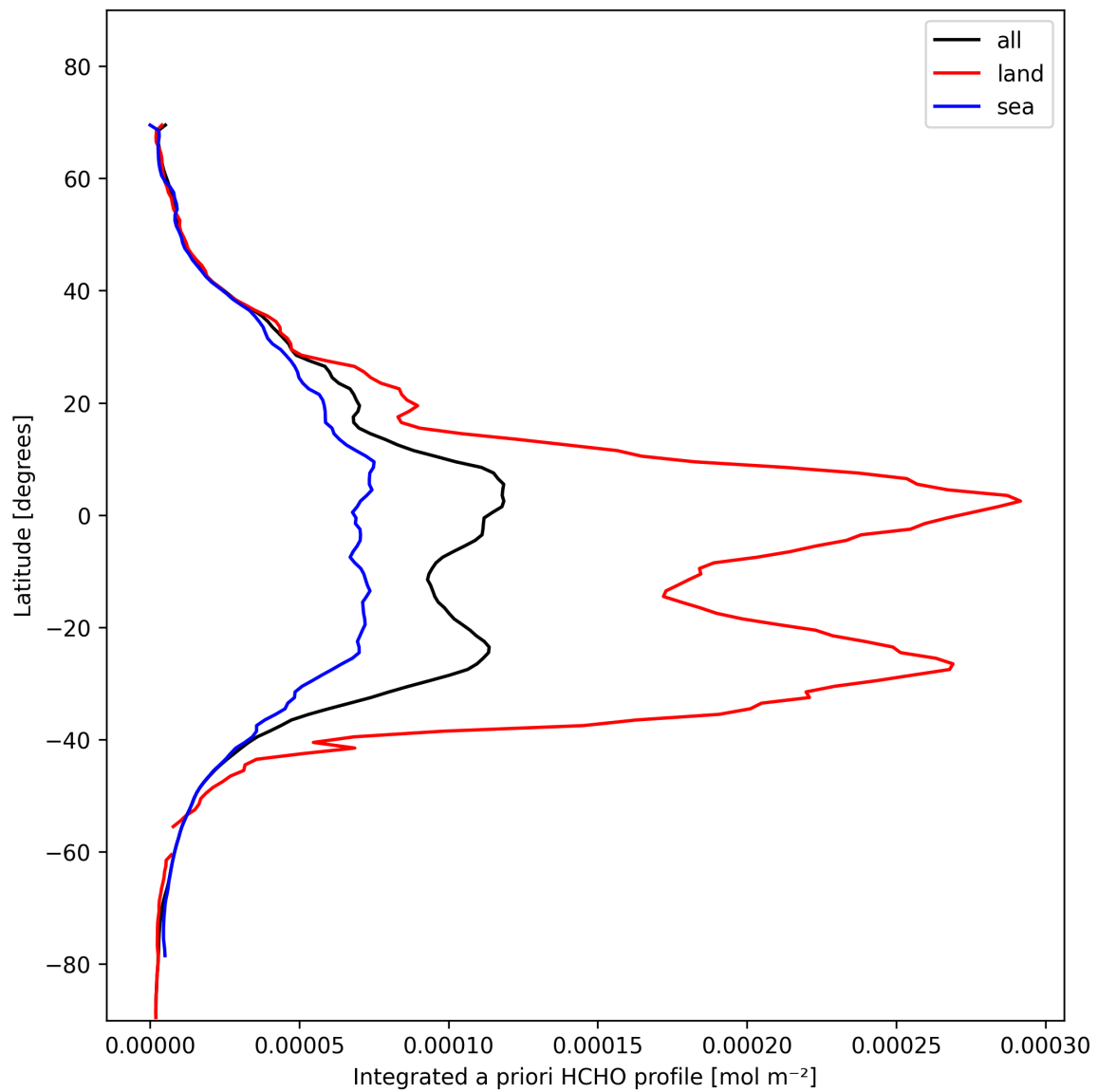
Figure 27: Zonal average of “Integrated a priori HCHO profile” for 2025-02-04 to 2025-02-05.
