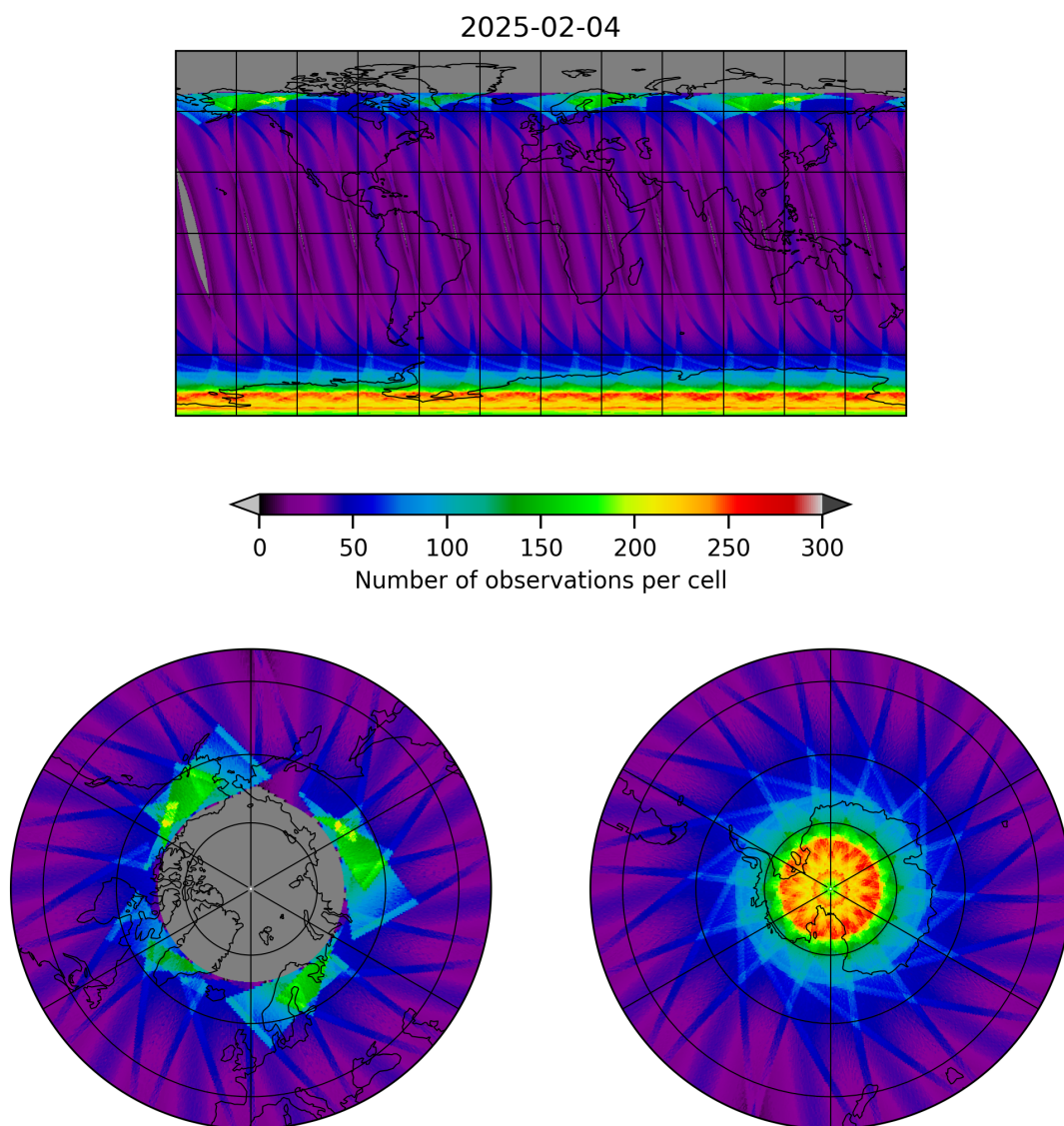
Figure 17: Map of the number of observations for 2025-02-04 to 2025-02-05
