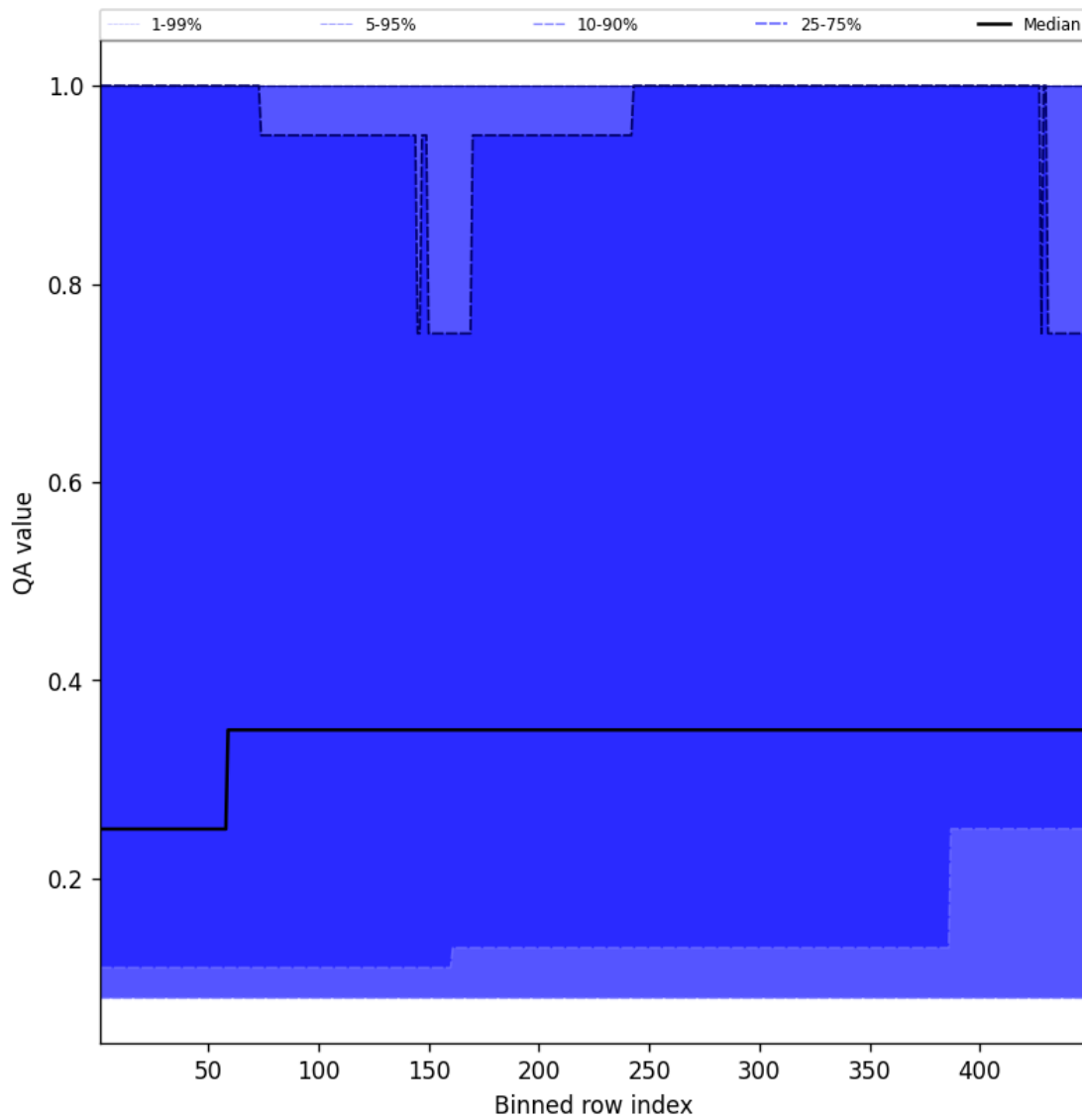
Figure 46: Along track statistics of “QA value” for 2025-02-04 to 2025-02-05
