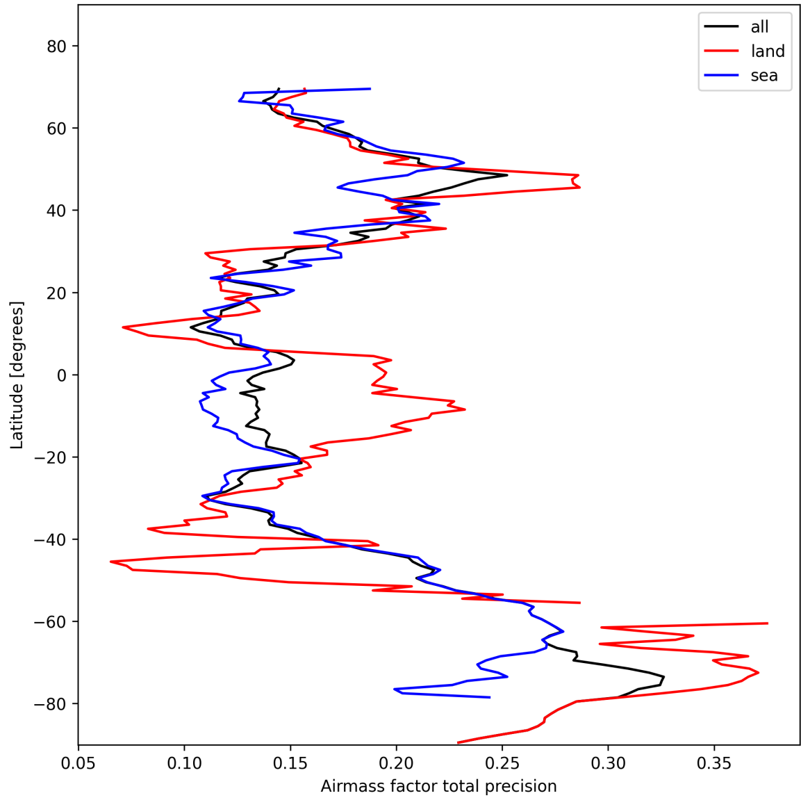
Figure 25: Zonal average of “Airmass factor total precision” for 2025-02-04 to 2025-02-05.
