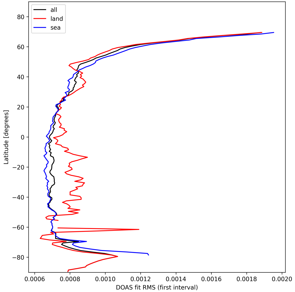
Figure 30: Zonal average of "DOAS fit RMS (first interval)" for 2025-02-04 to 2025-02-05.
