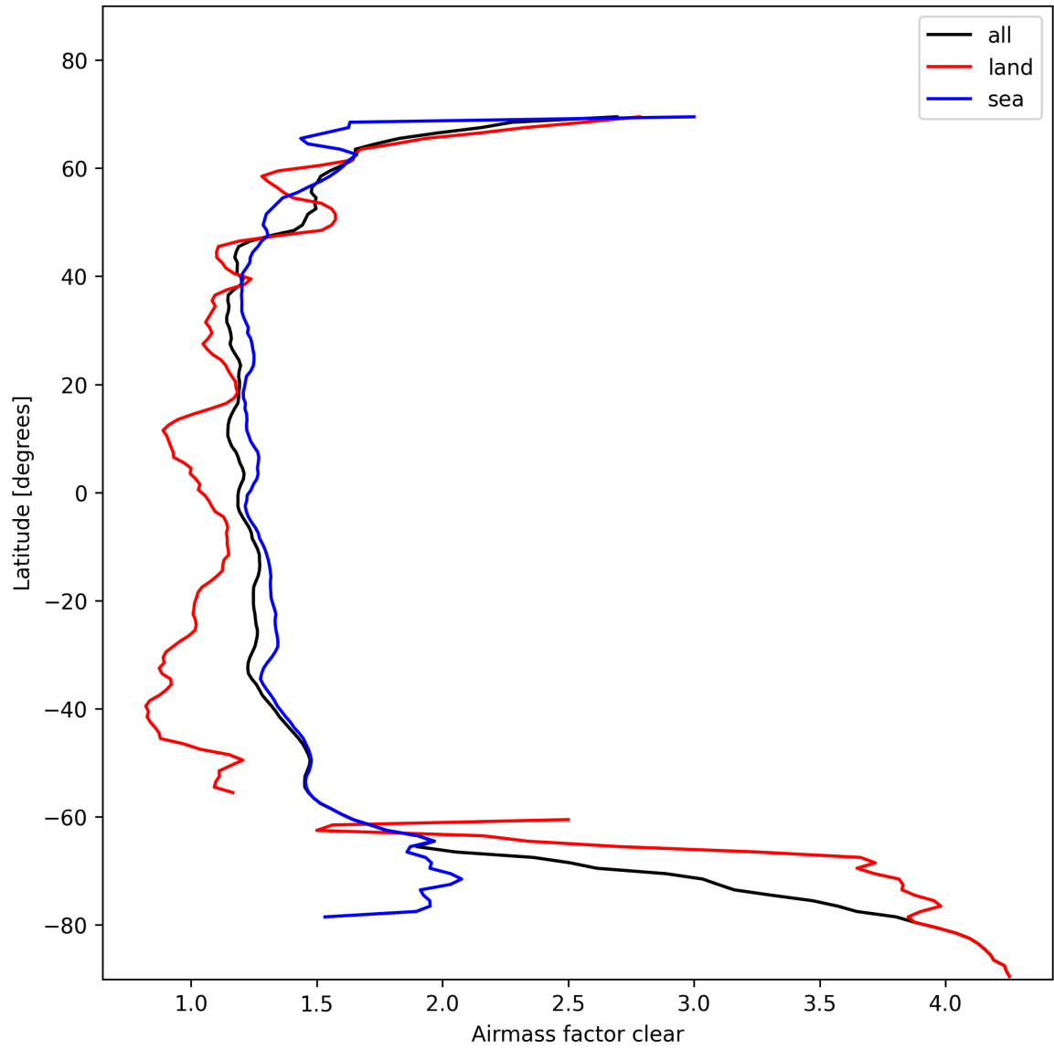
Figure 26: Zonal average of “Airmass factor clear” for 2025-02-04 to 2025-02-05.
