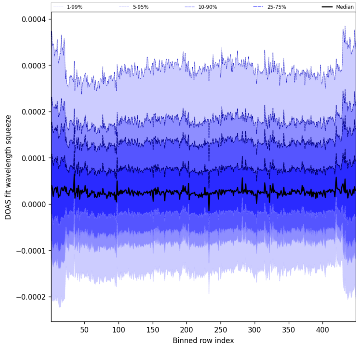
Figure 57: Along track statistics of “DOAS fit wavelength squeeze” for 2025-02-04 to 2025-02-05
