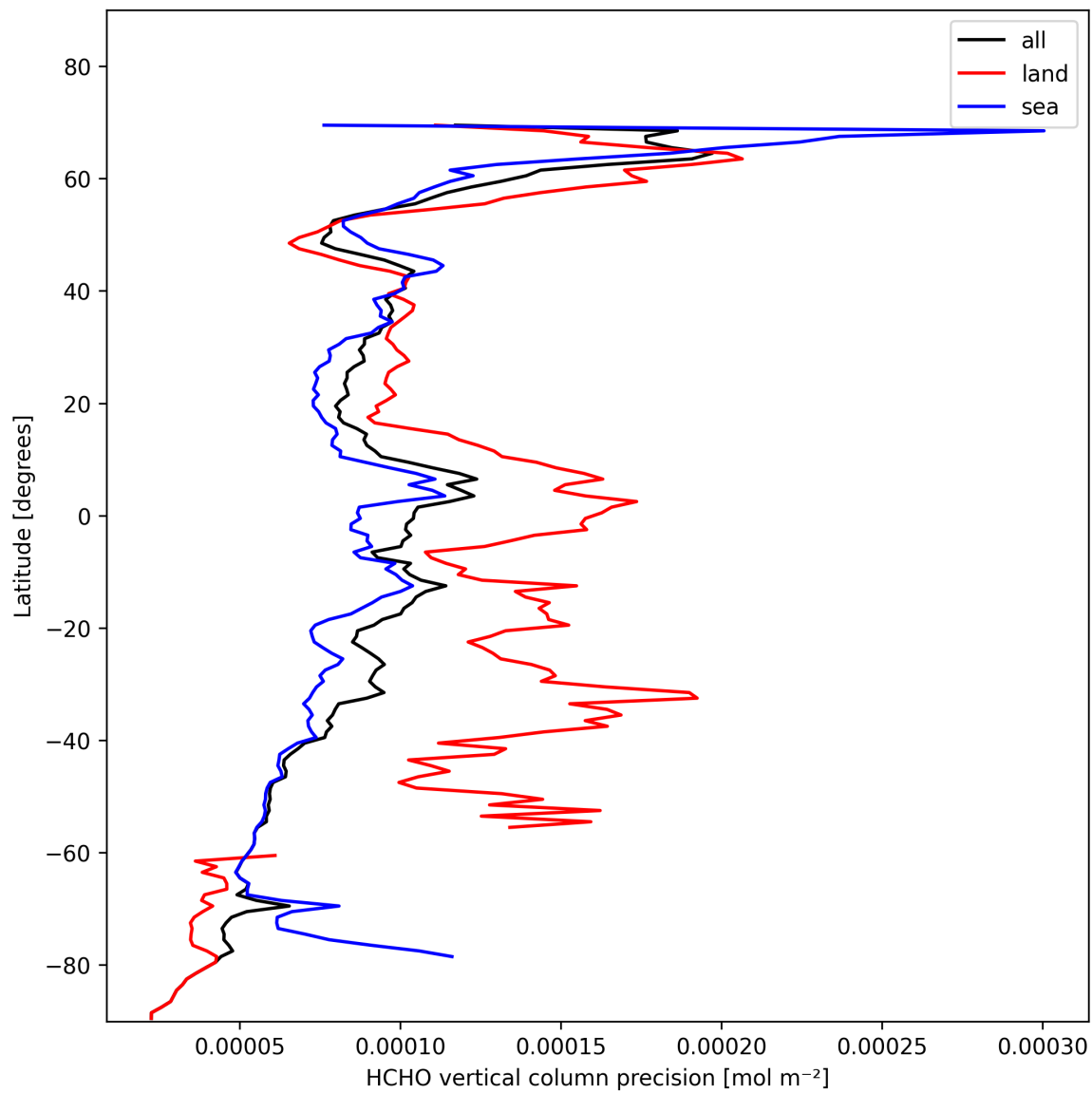
Figure 20: Zonal average of “HCHO vertical column precision” for 2025-02-04 to 2025-02-05.
