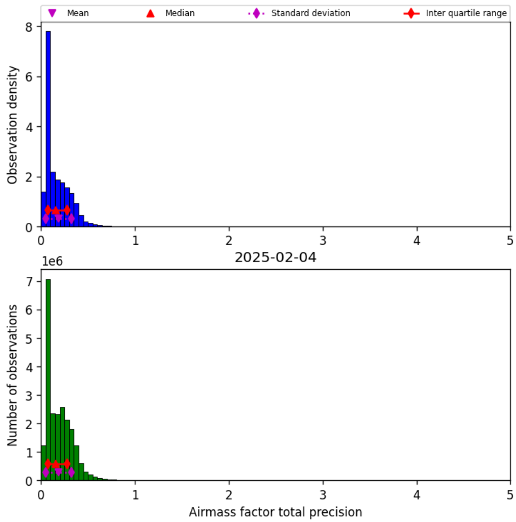
Figure 39: Histogram of “Airmass factor total precision” for 2025-02-04 to 2025-02-05
