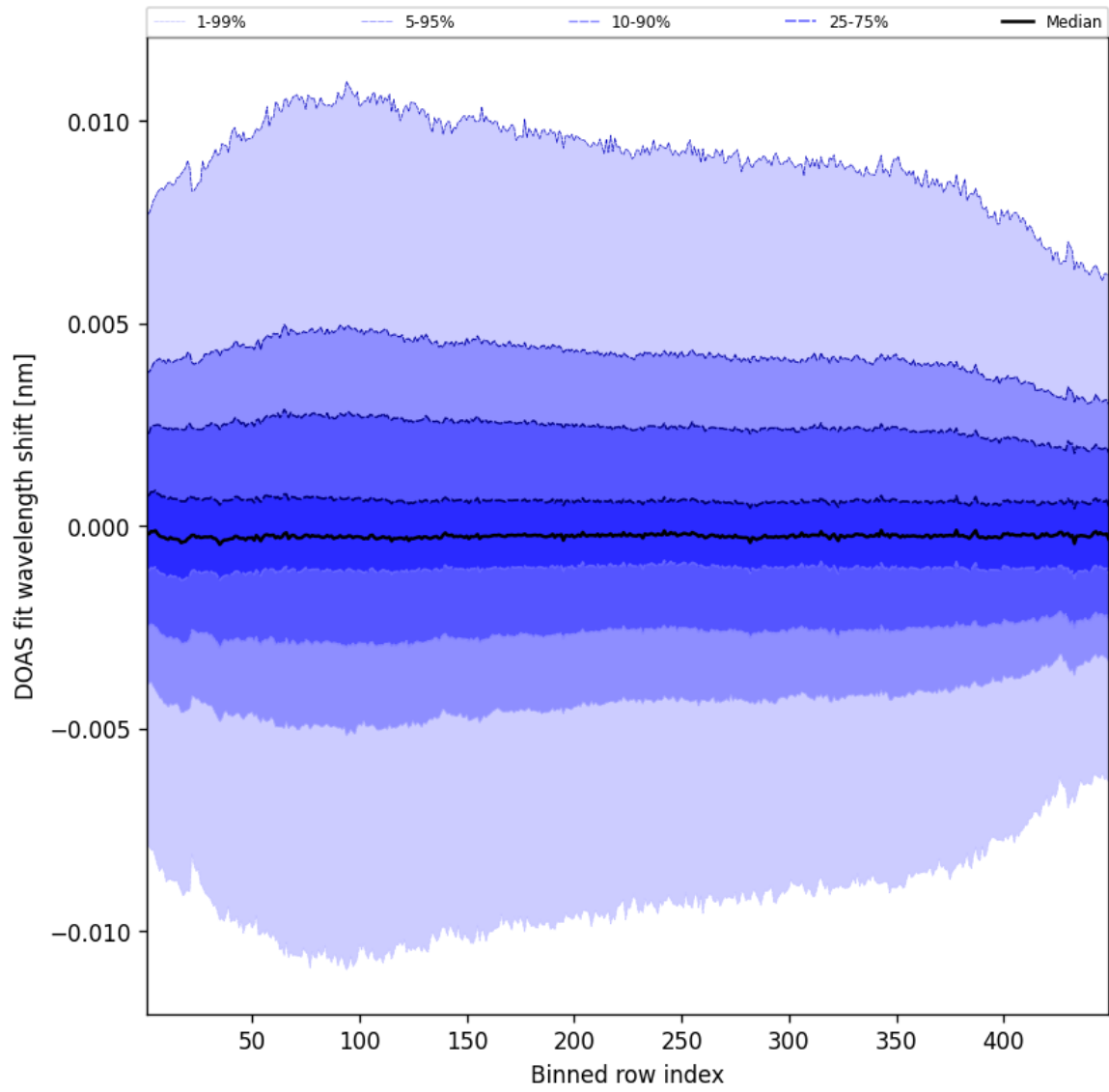
Figure 56: Along track statistics of “DOAS fit wavelength shift” for 2025-02-04 to 2025-02-05
