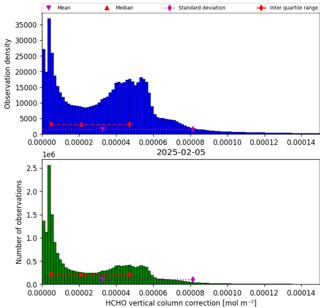
Figure 35: Histogram of “HCHO vertical column correction” for 2025-02-05 to 2025-02-06
