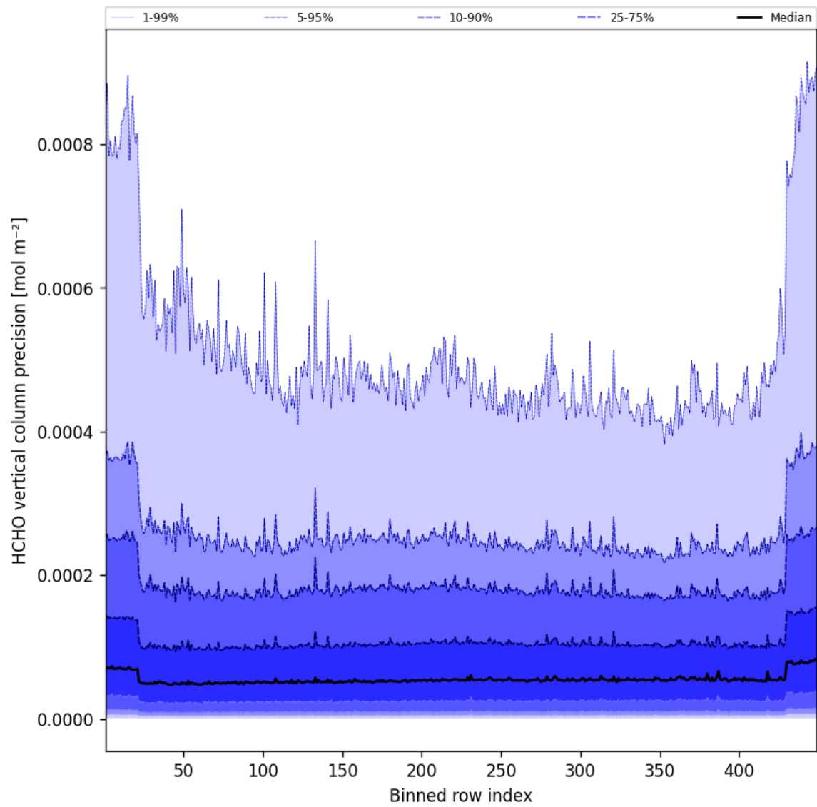
Figure 48: Along track statistics of “HCHO vertical column precision” for 2025-02-05 to 2025-02-06
