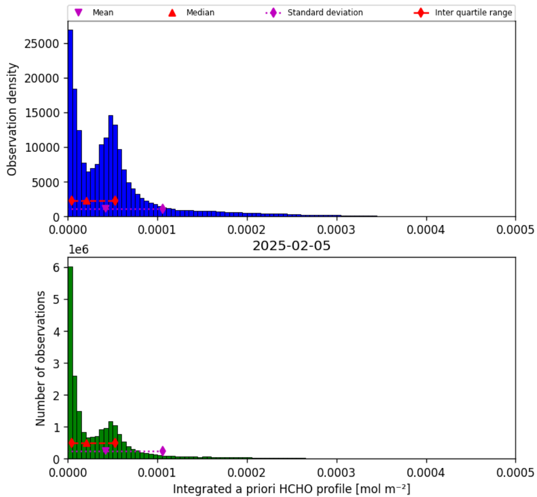
Figure 41: Histogram of “Integrated a priori HCHO profile” for 2025-02-05 to 2025-02-06
