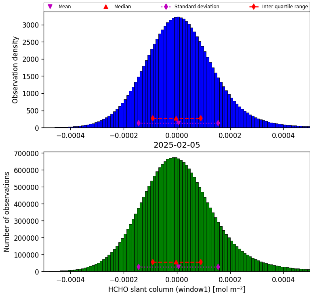
Figure 36: Histogram of "HCHO slant column (window1)" for 2025-02-05 to 2025-02-06
