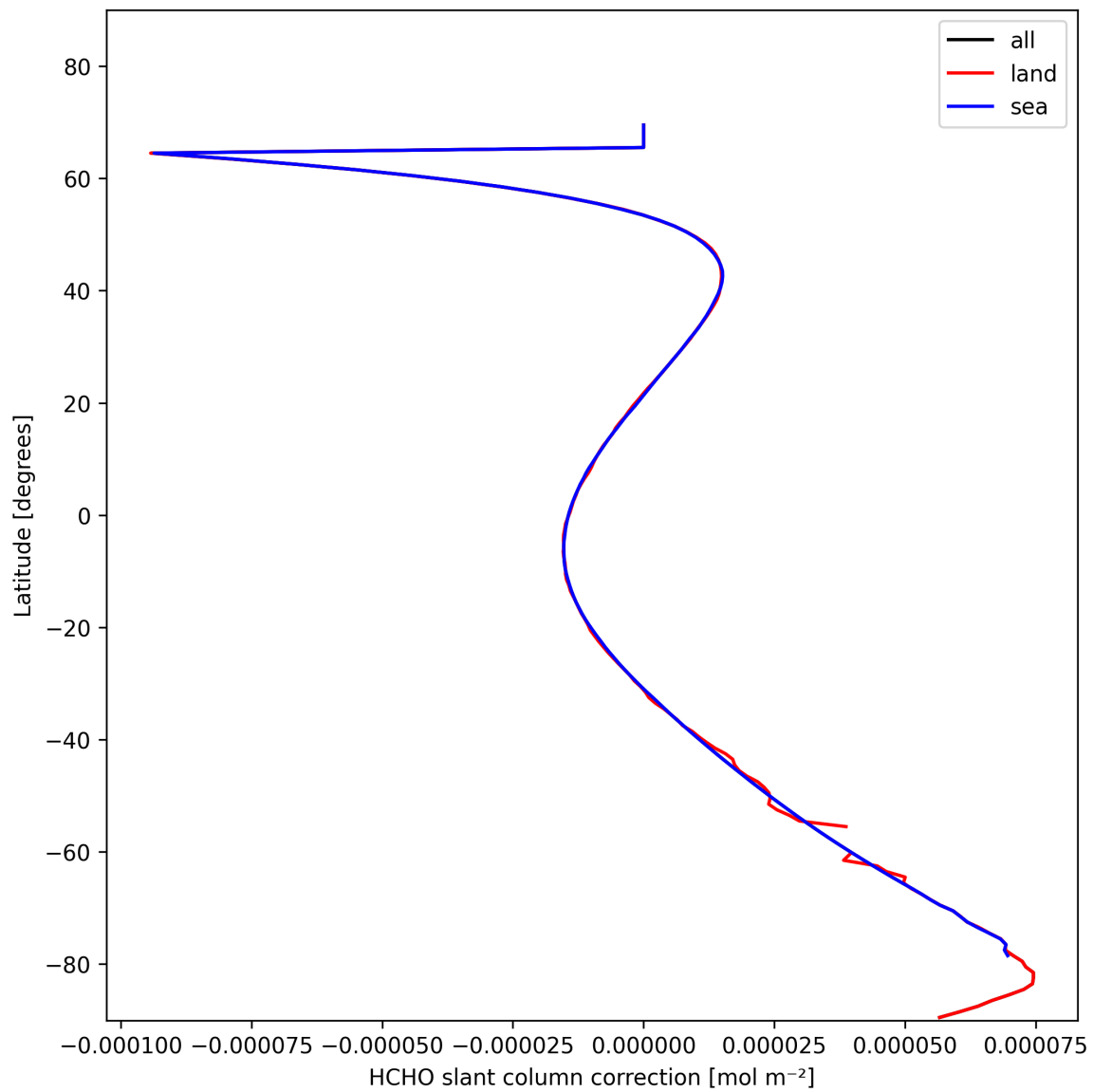
Figure 31: Zonal average of “HCHO slant column correction” for 2025-02-05 to 2025-02-06.
