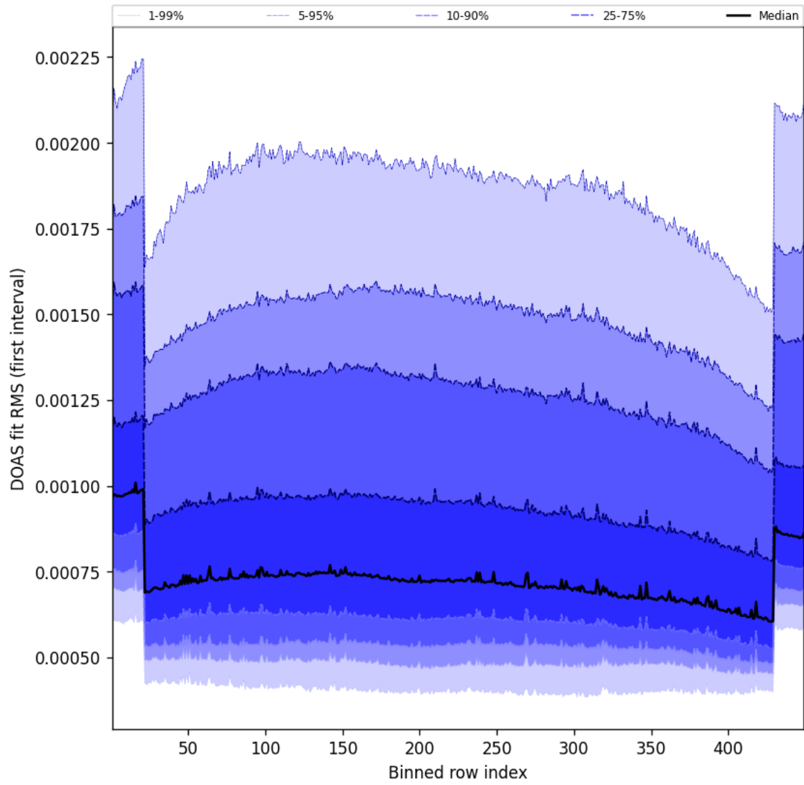
Figure 58: Along track statistics of “DOAS fit RMS (first interval)” for 2025-02-05 to 2025-02-06
