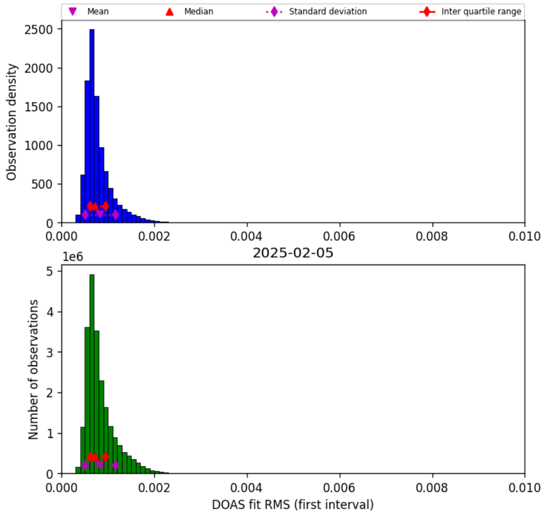
Figure 44: Histogram of “DOAS fit RMS (first interval)” for 2025-02-05 to 2025-02-06
