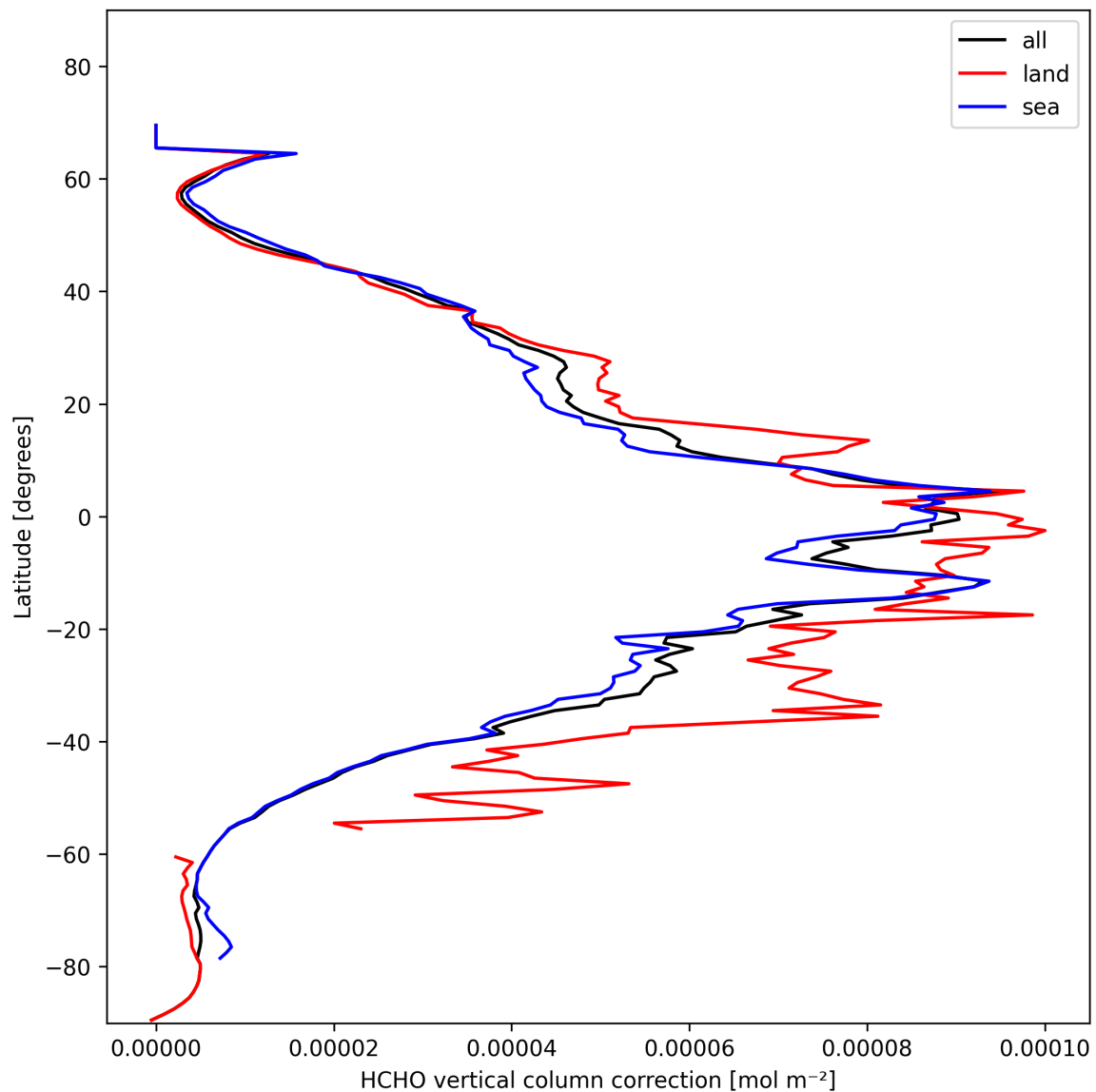
Figure 21: Zonal average of “HCHO vertical column correction” for 2025-02-05 to 2025-02-06.
