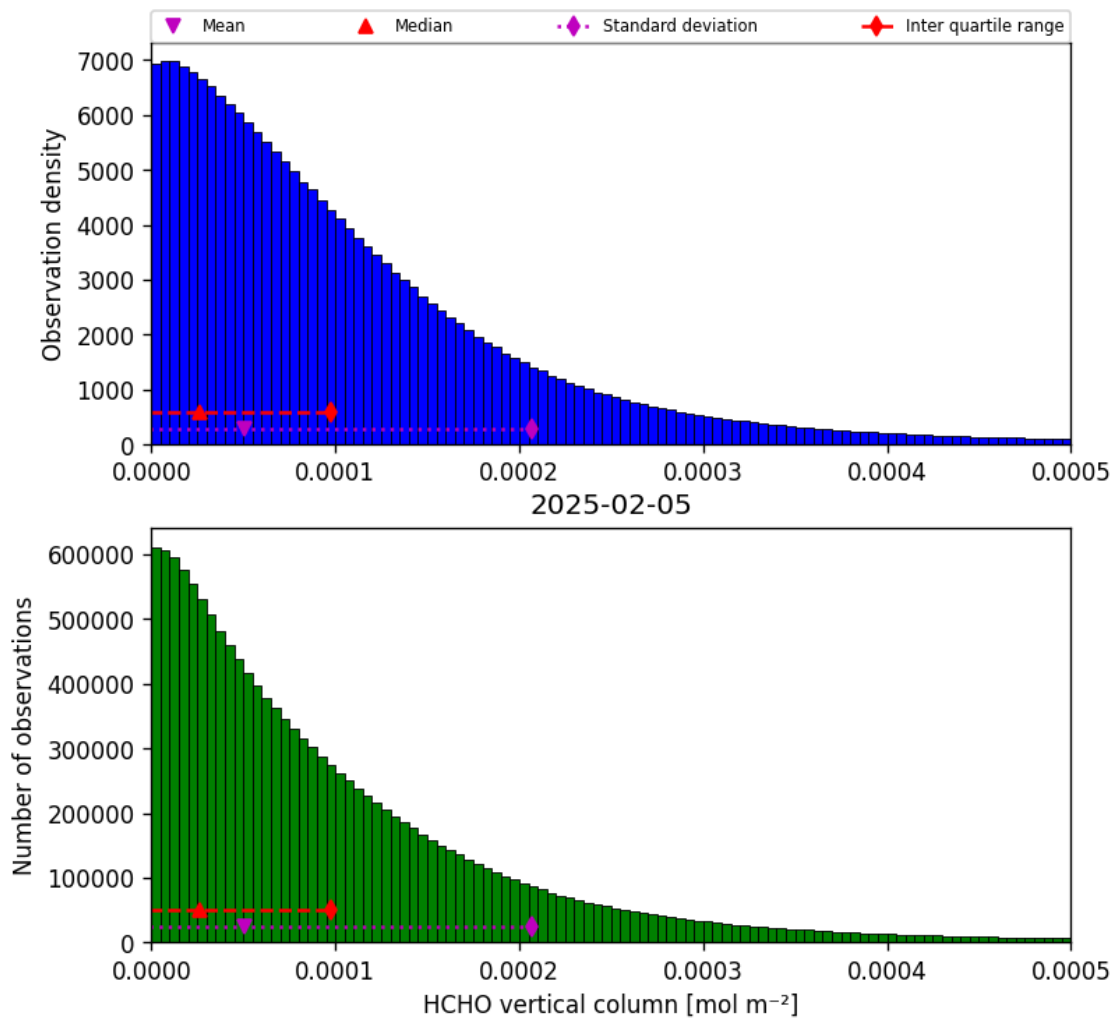
Figure 33: Histogram of “HCHO vertical column” for 2025-02-05 to 2025-02-06
