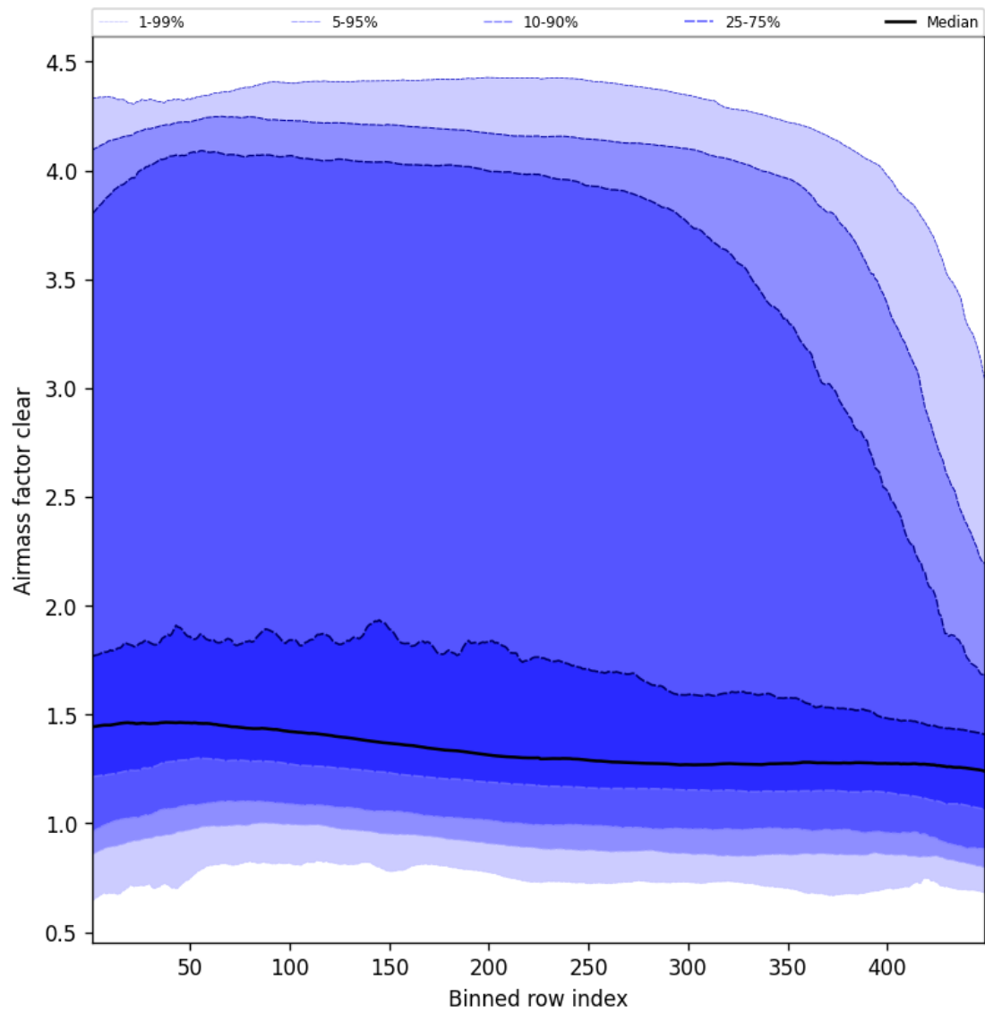
Figure 54: Along track statistics of “Air mass factor clear” for 2025-02-05 to 2025-02-06
