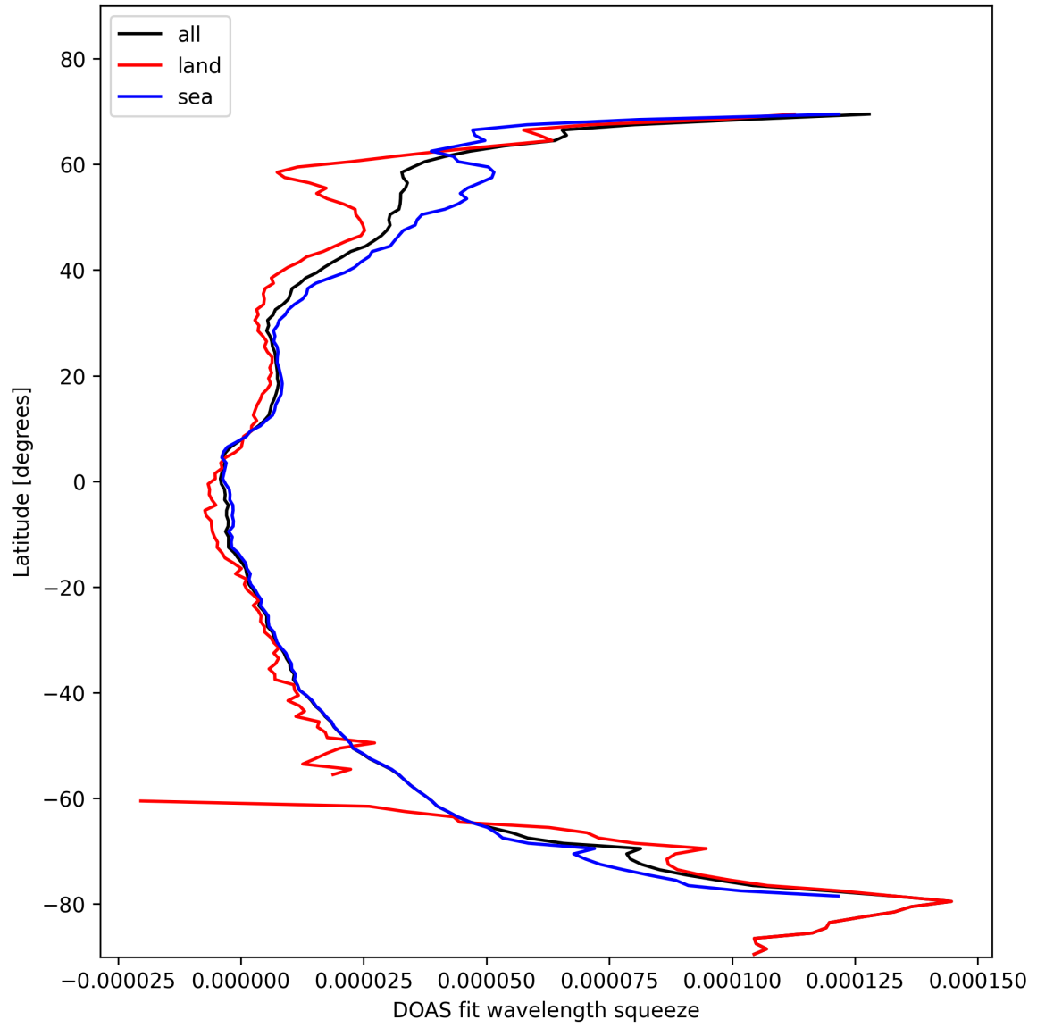
Figure 29: Zonal average of “DOAS fit wavelength squeeze” for 2025-02-05 to 2025-02-06.
