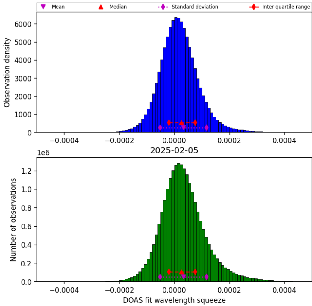
Figure 43: Histogram of “DOAS fit wavelength squeeze” for 2025-02-05 to 2025-02-06
