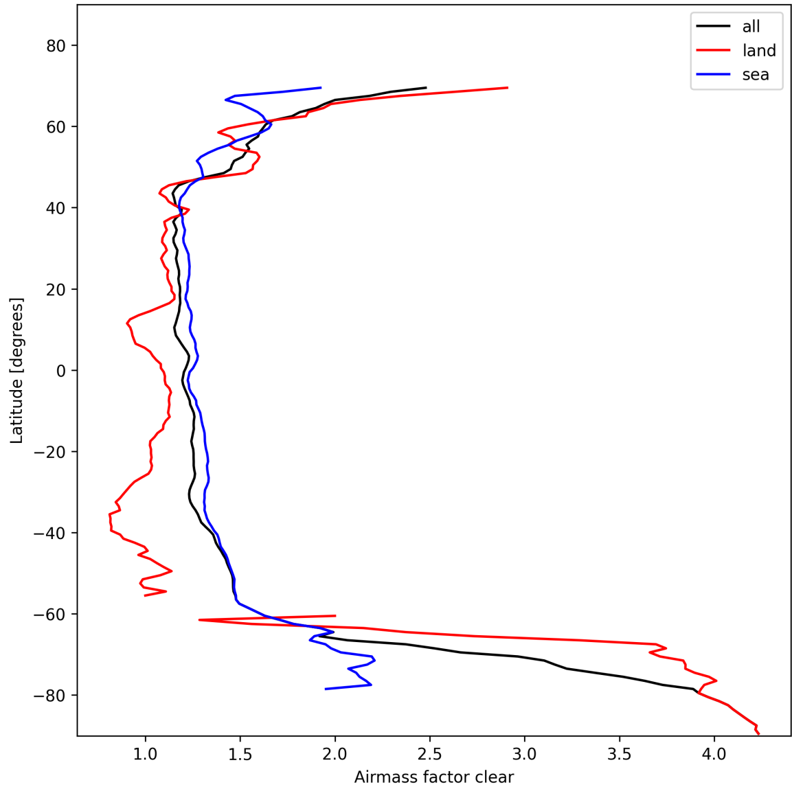
Figure 26: Zonal average of “Airmass factor clear” for 2025-02-05 to 2025-02-06.
