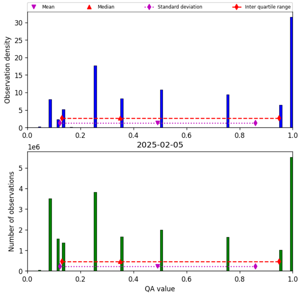
Figure 32: Histogram of “QA value” for 2025-02-05 to 2025-02-06
