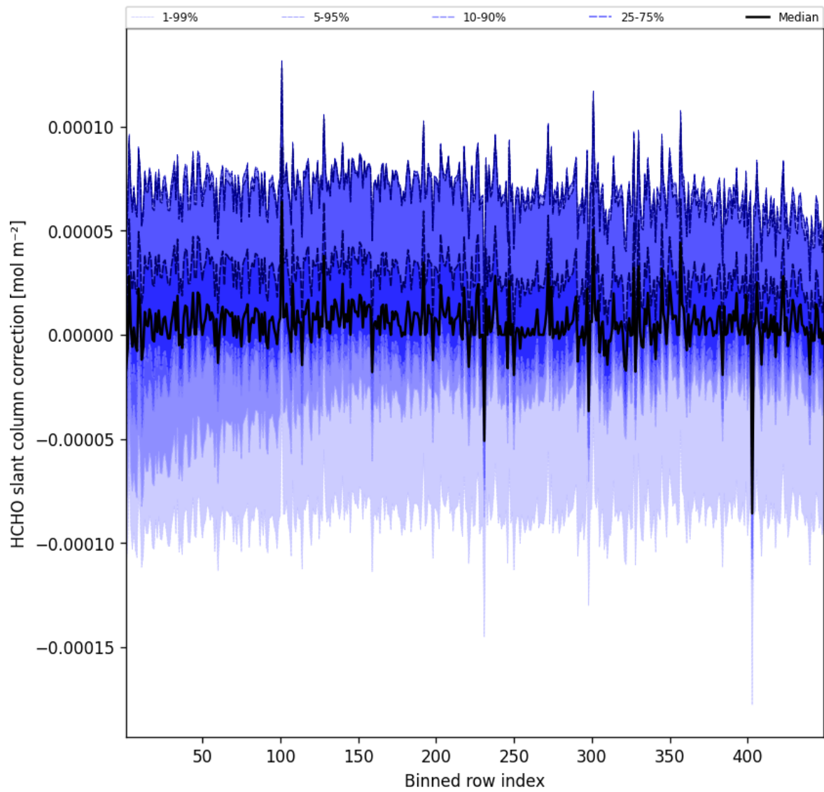
Figure 59: Along track statistics of “HCHO slant column correction” for 2025-02-05 to 2025-02-06
