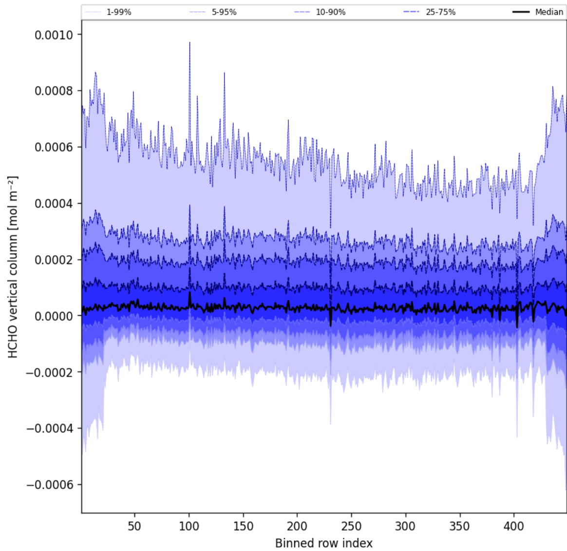
Figure 47: Along track statistics of “HCHO vertical column” for 2025-02-05 to 2025-02-06
