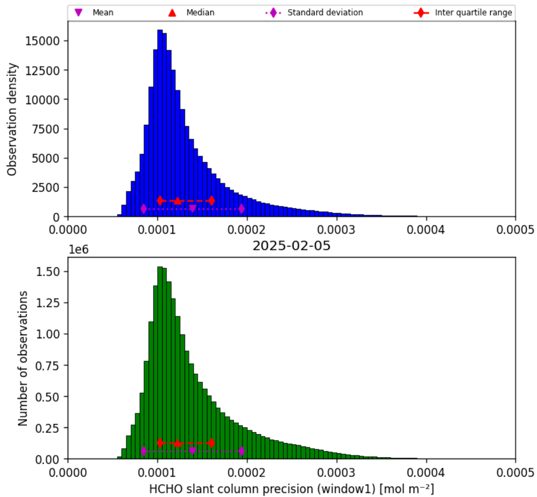
Figure 37: Histogram of “HCHO slant column precision (window1)” for 2025-02-05 to 2025-02-06
