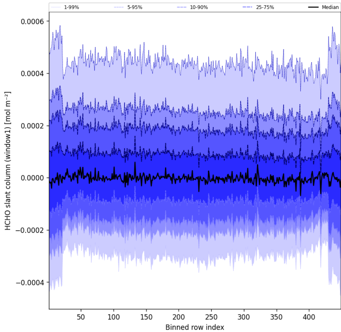
Figure 50: Along track statistics of “HCHO slant column (window1)” for 2025-02-05 to 2025-02-06
