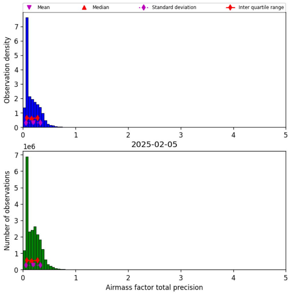
Figure 39: Histogram of “Airmass factor total precision” for 2025-02-05 to 2025-02-06
