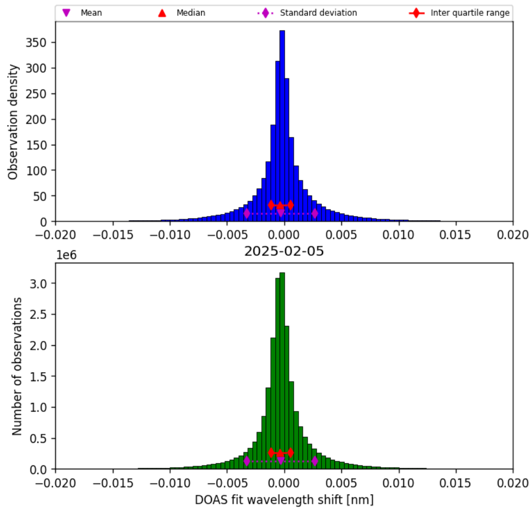
Figure 42: Histogram of “DOAS fit wavelength shift” for 2025-02-05 to 2025-02-06
