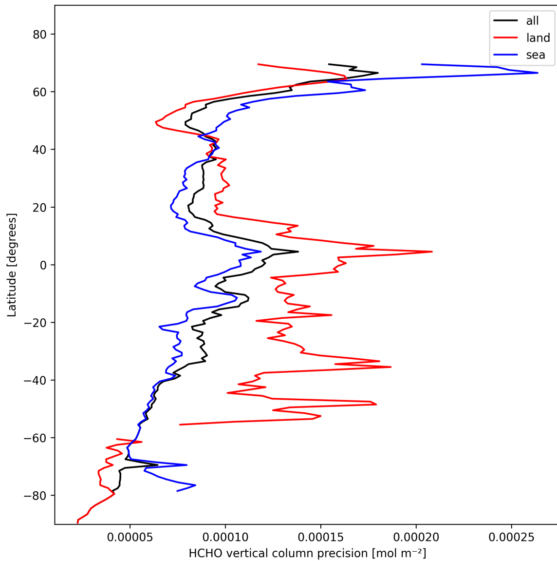
Figure 20: Zonal average of “HCHO vertical column precision” for 2025-02-05 to 2025-02-06.
