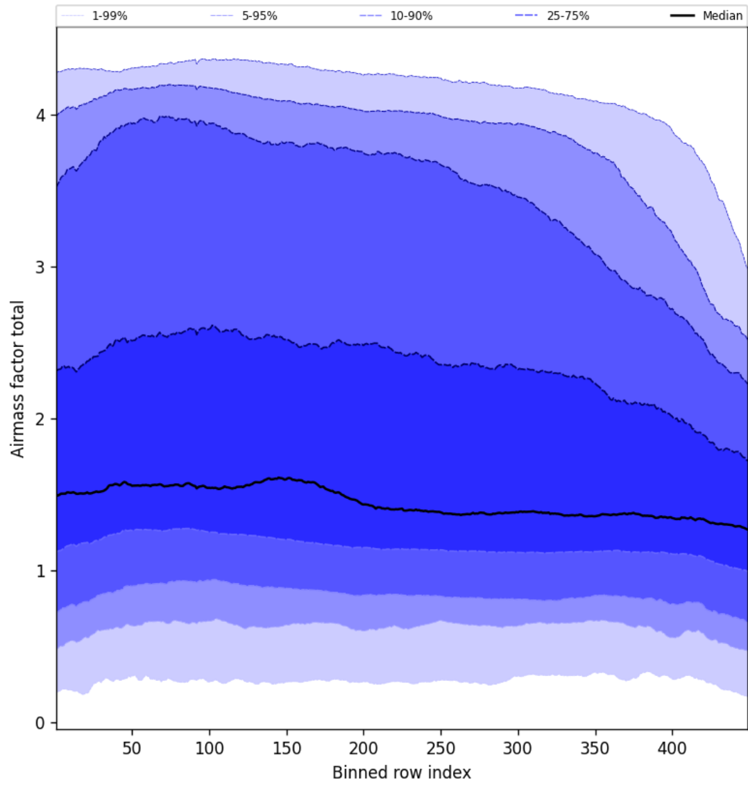
Figure 52: Along track statistics of “Airmass factor total” for 2025-02-05 to 2025-02-06
