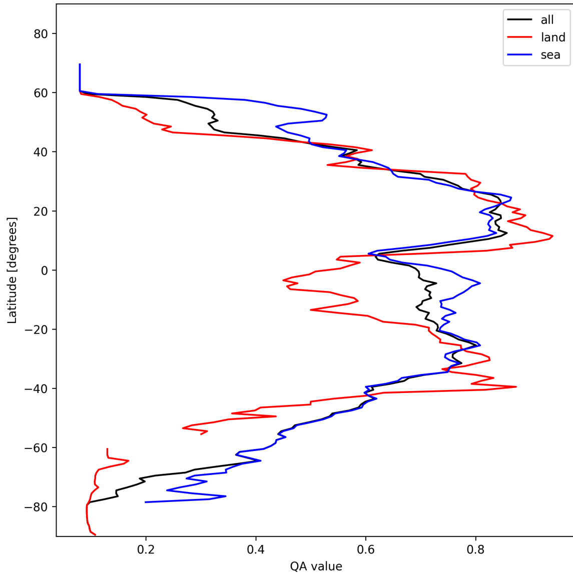
Figure 18: Zonal average of “QA value” for 2025-02-05 to 2025-02-06.
