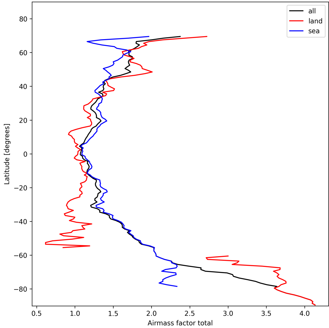
Figure 24: Zonal average of “Airmass factor total” for 2025-02-05 to 2025-02-06.
