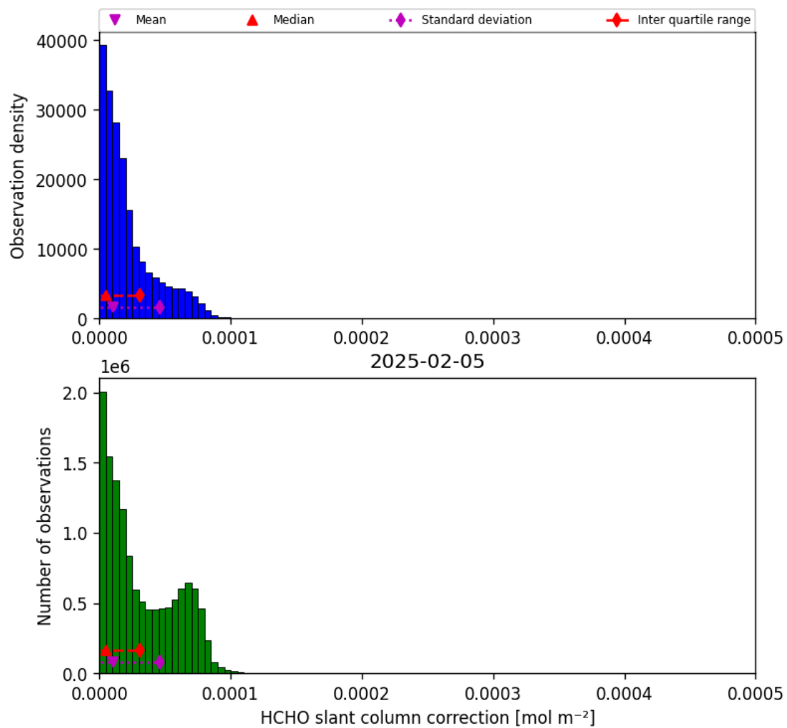
Figure 45: Histogram of “HCHO slant column correction” for 2025-02-05 to 2025-02-06
