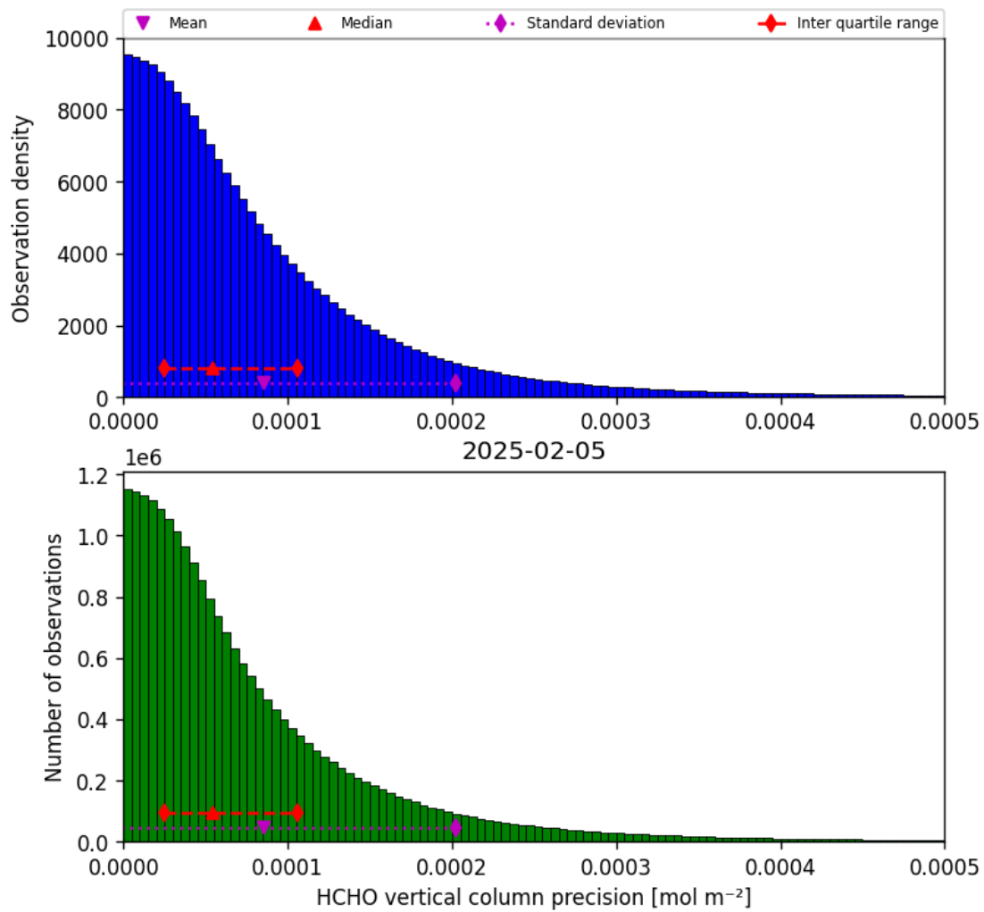
Figure 34: Histogram of "HCHO vertical column precision" for 2025-02-05 to 2025-02-06
