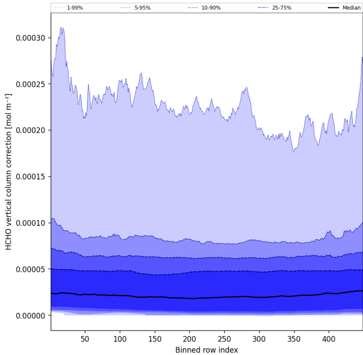
Figure 49: Along track statistics of “HCHO vertical column correction” for 2025-02-05 to 2025-02-06
