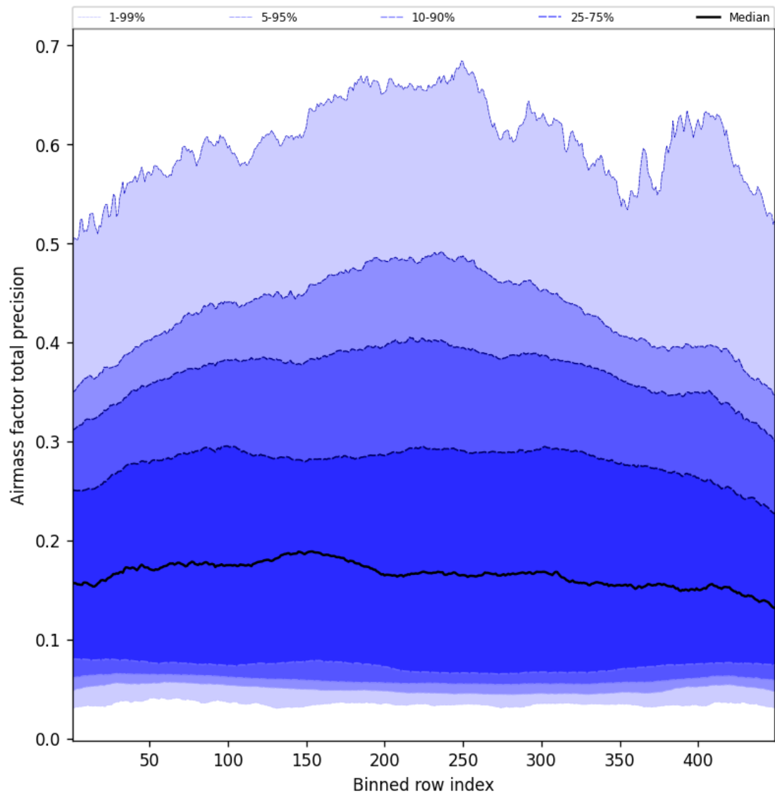
Figure 53: Along track statistics of “Airmass factor total precision” for 2025-02-05 to 2025-02-06
