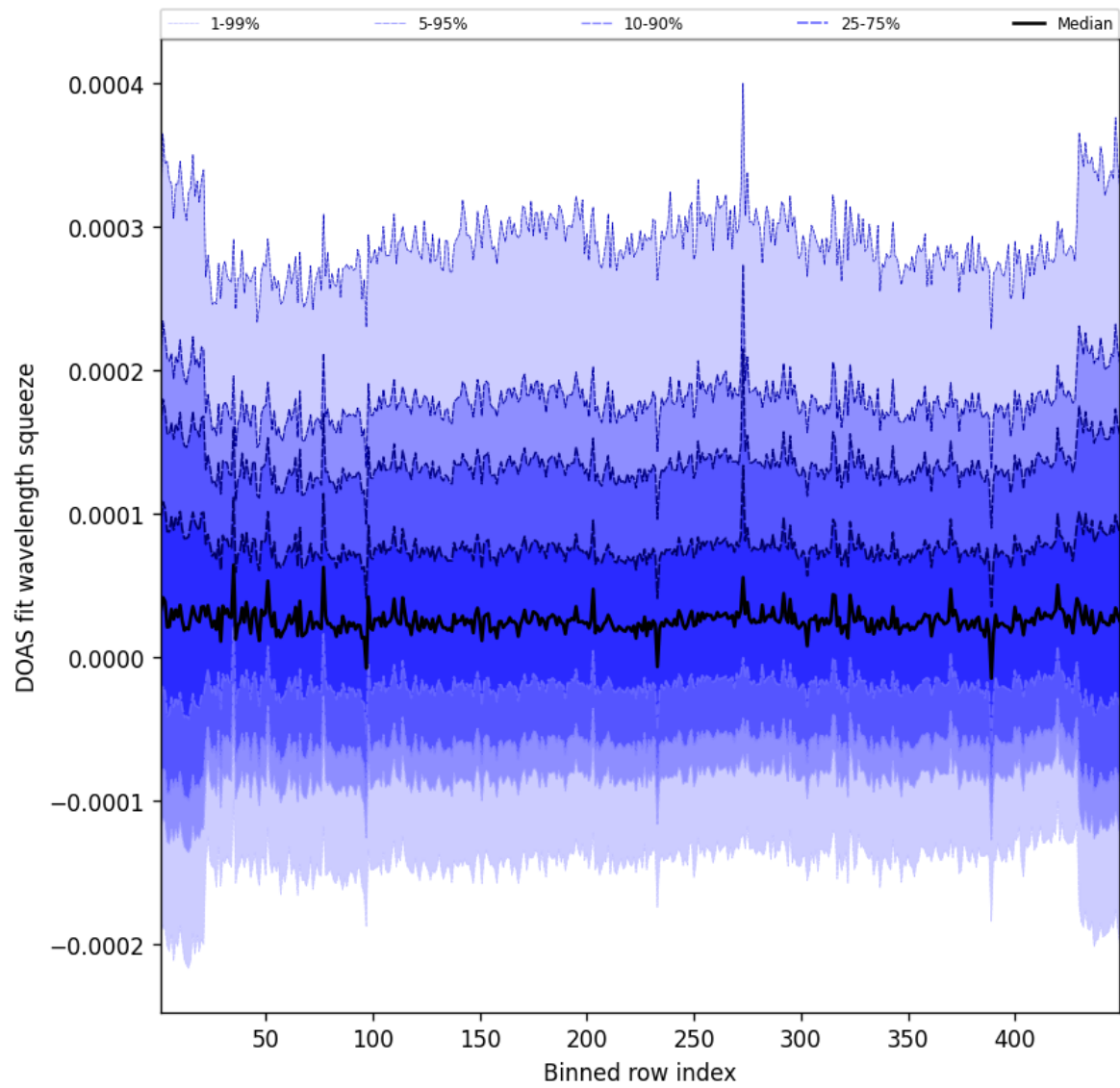
Figure 57: Along track statistics of “DOAS fit wavelength squeeze” for 2025-02-05 to 2025-02-06
