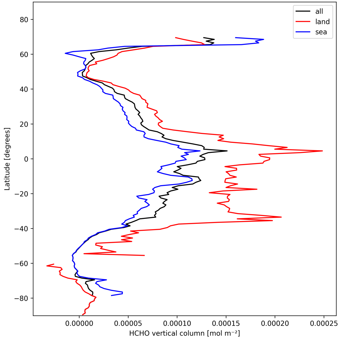
Figure 19: Zonal average of “HCHO vertical column” for 2025-02-05 to 2025-02-06.
