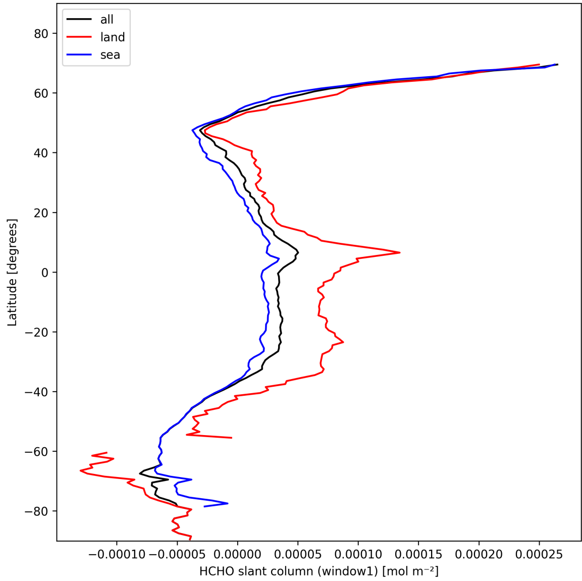
Figure 22: Zonal average of “HCHO slant column (window1)” for 2025-02-05 to 2025-02-06.
