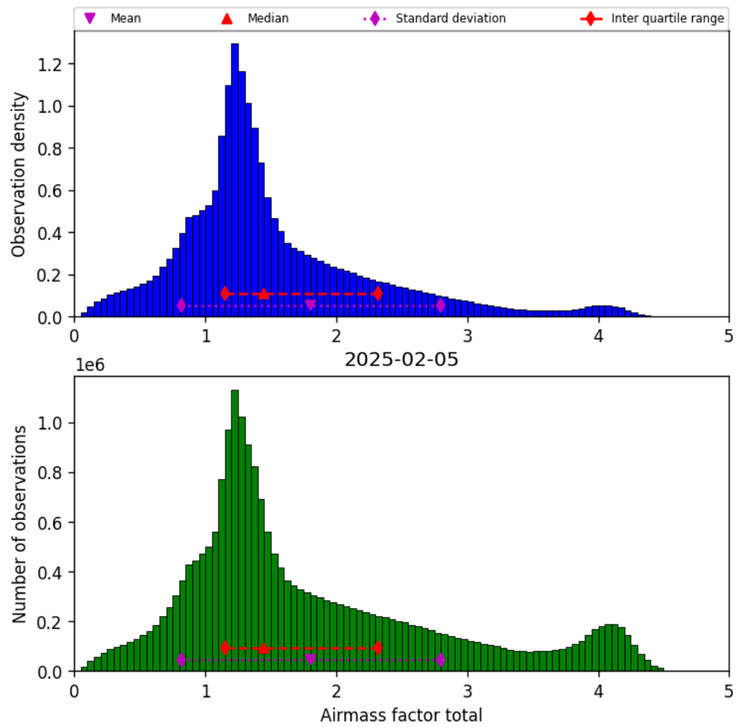
Figure 38: Histogram of “Airmass factor total” for 2025-02-05 to 2025-02-06
