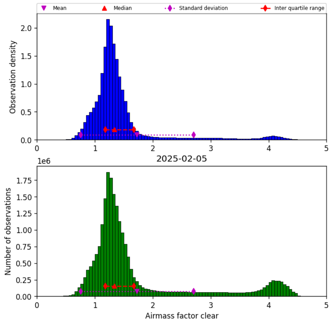
Figure 40: Histogram of “Airmass factor clear” for 2025-02-05 to 2025-02-06
