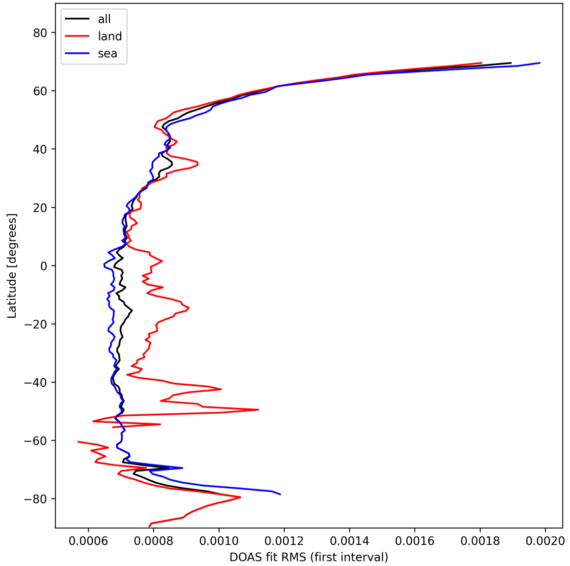
Figure 30: Zonal average of "DOAS fit RMS (first interval)" for 2025-02-05 to 2025-02-06.
