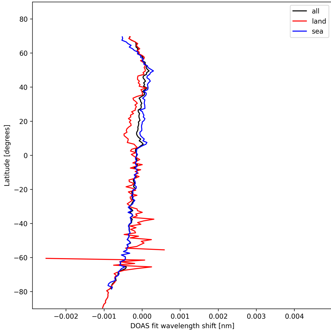
Figure 28: Zonal average of "DOAS fit wavelength shift" for 2025-02-05 to 2025-02-06.
