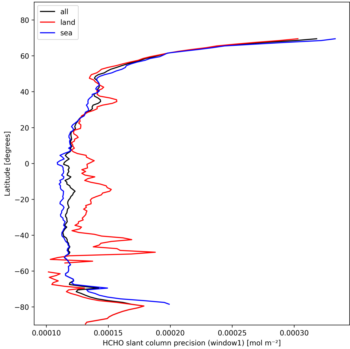
Figure 23: Zonal average of “HCHO slant column precision (window1)” for 2025-02-05 to 2025-02-06.
