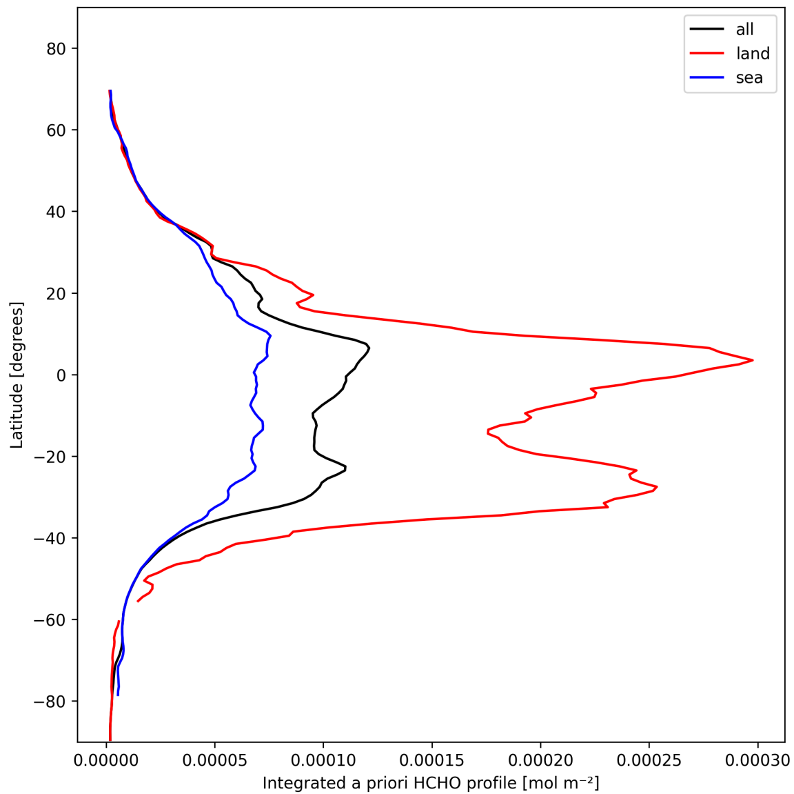
Figure 27: Zonal average of “Integrated a priori HCHO profile” for 2025-02-05 to 2025-02-06.
