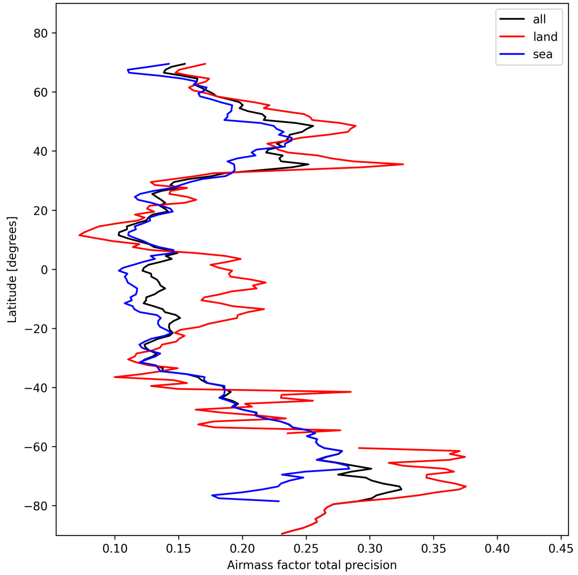
Figure 25: Zonal average of “Airmass factor total precision” for 2025-02-05 to 2025-02-06.
