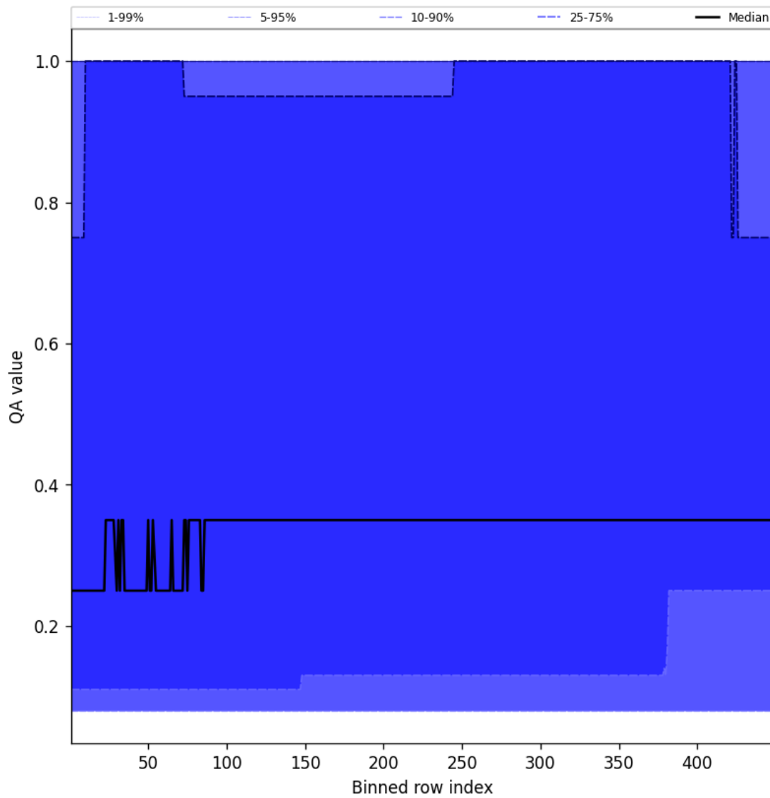
Figure 46: Along track statistics of “QA value” for 2025-02-05 to 2025-02-06
