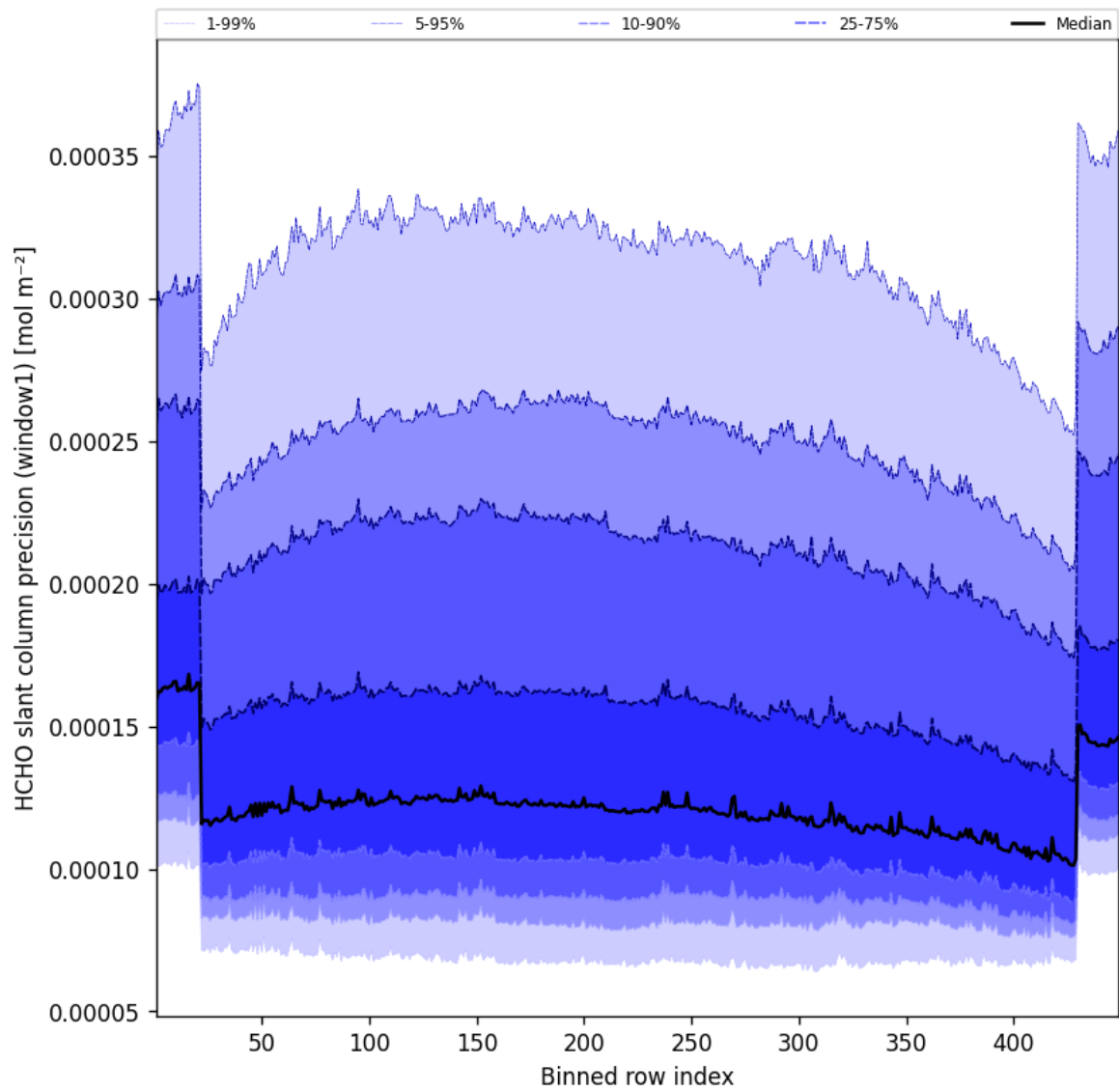
Figure 51: Along track statistics of “HCHO slant column precision (window1)” for 2025-02-05 to 2025-02-06
