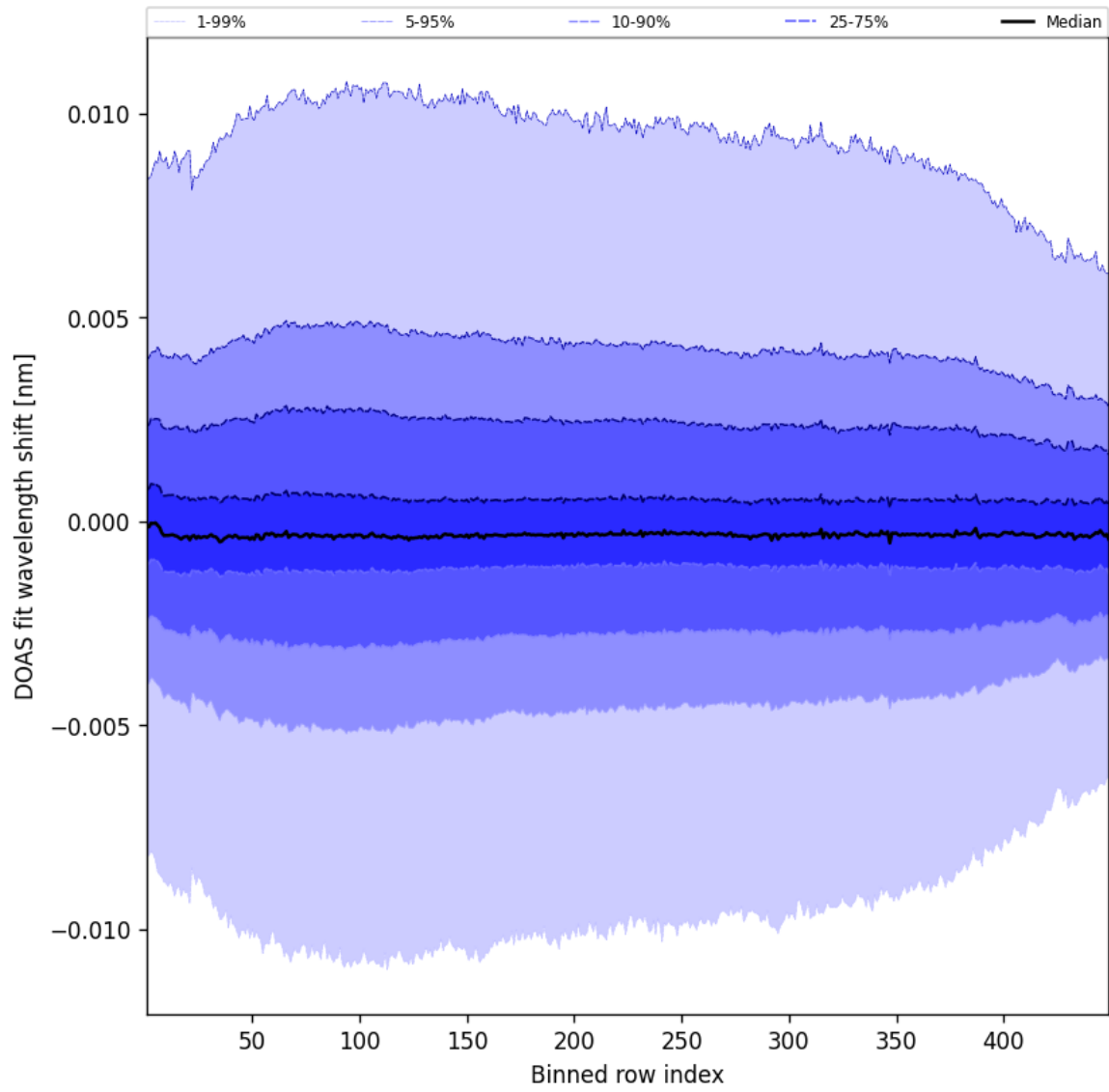
Figure 56: Along track statistics of “DOAS fit wavelength shift” for 2025-02-05 to 2025-02-06
