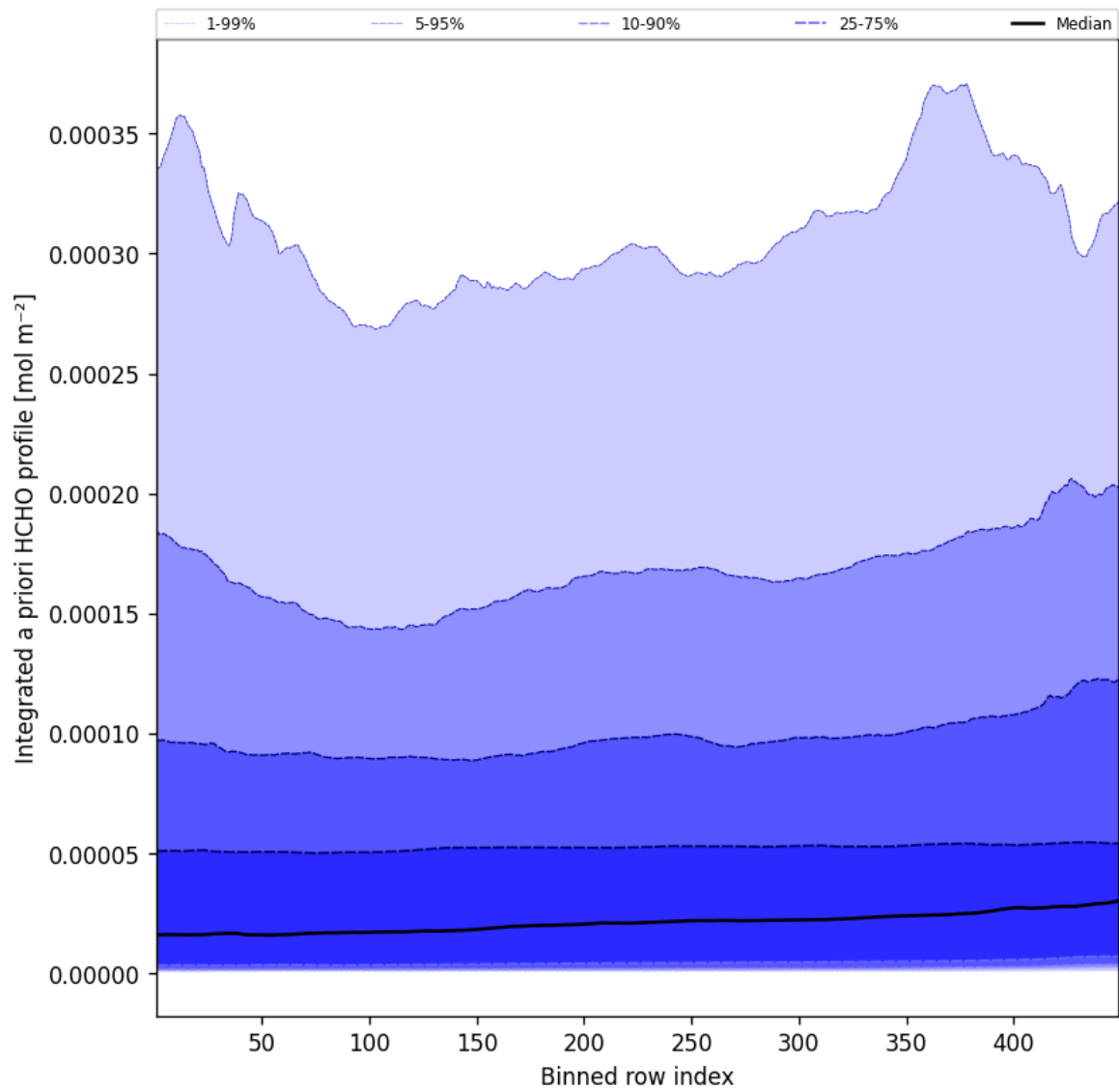
Figure 55: Along track statistics of "Integrated a priori HCHO profile" for 2025-02-05 to 2025-02-06
