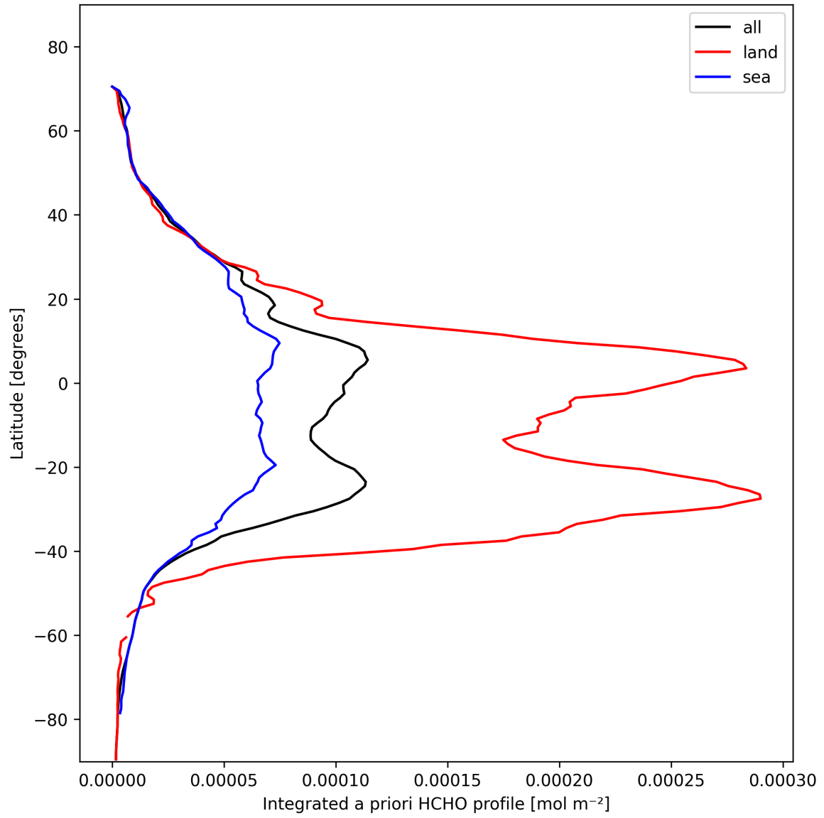
Figure 27: Zonal average of “Integrated a priori HCHO profile” for 2025-02-07 to 2025-02-08.
