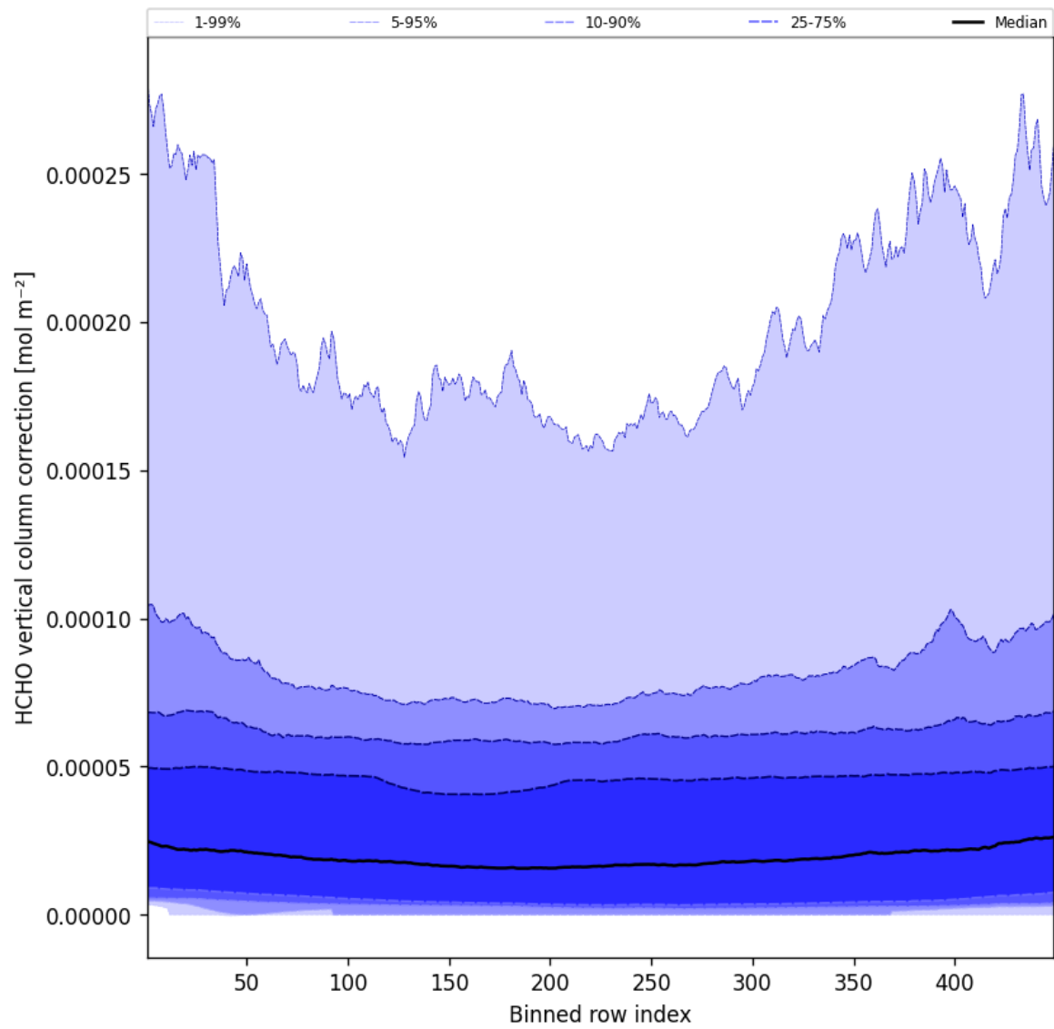
Figure 49: Along track statistics of “HCHO vertical column correction” for 2025-02-07 to 2025-02-08
