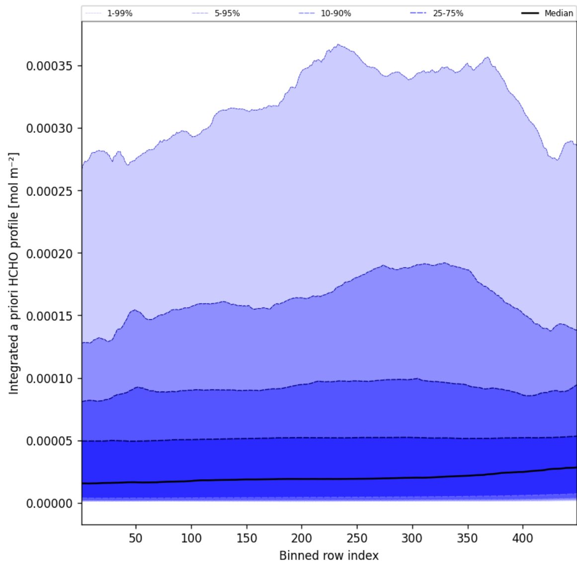
Figure 55: Along track statistics of “Integrated a priori HCHO profile” for 2025-02-07 to 2025-02-08
