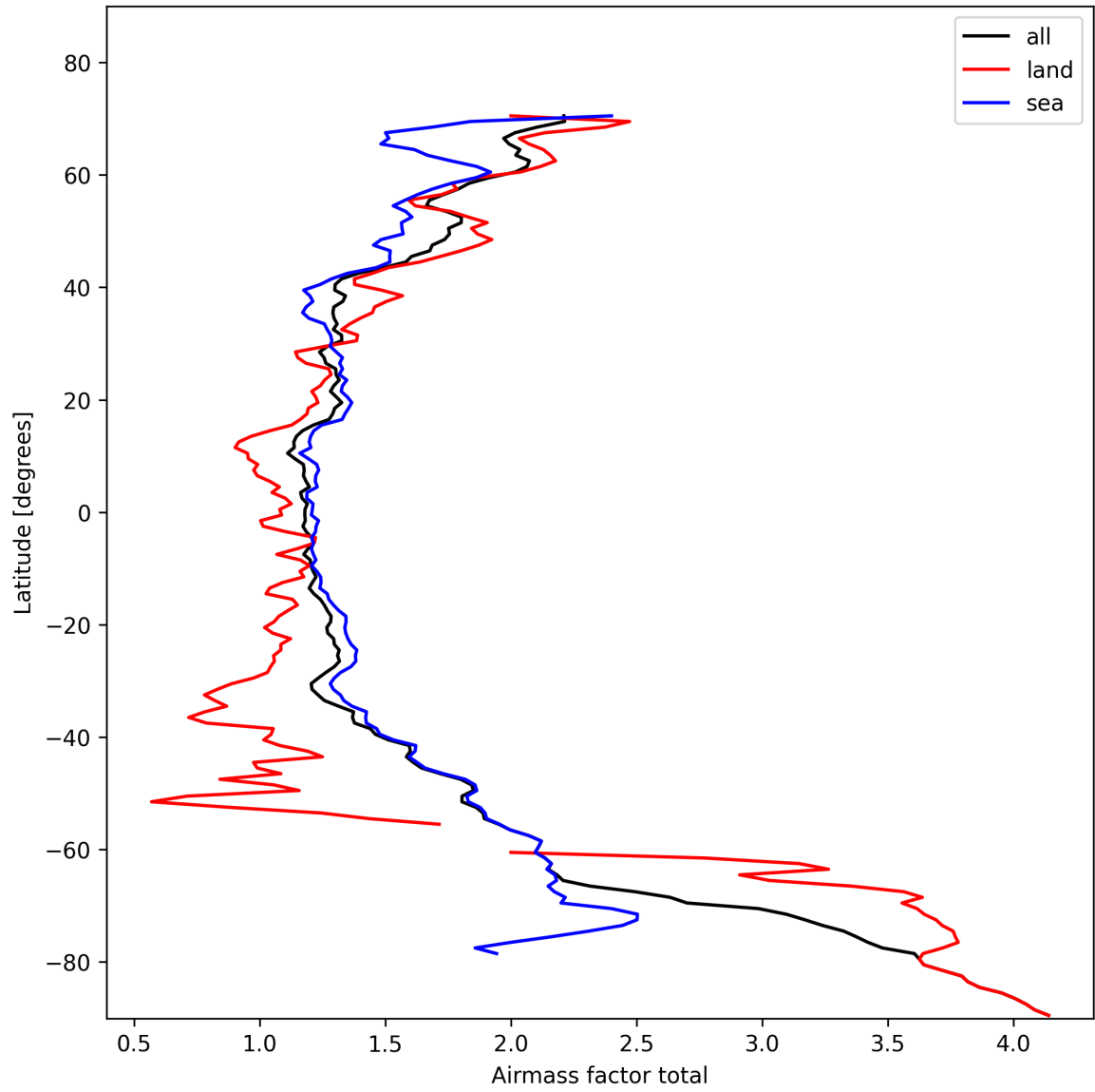
Figure 24: Zonal average of “Airmass factor total” for 2025-02-07 to 2025-02-08.
