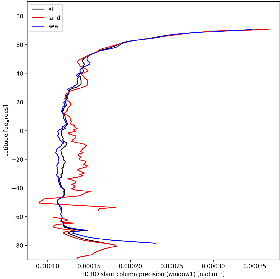
Figure 23: Zonal average of “HCHO slant column precision (window1)” for 2025-02-07 to 2025-02-08.
