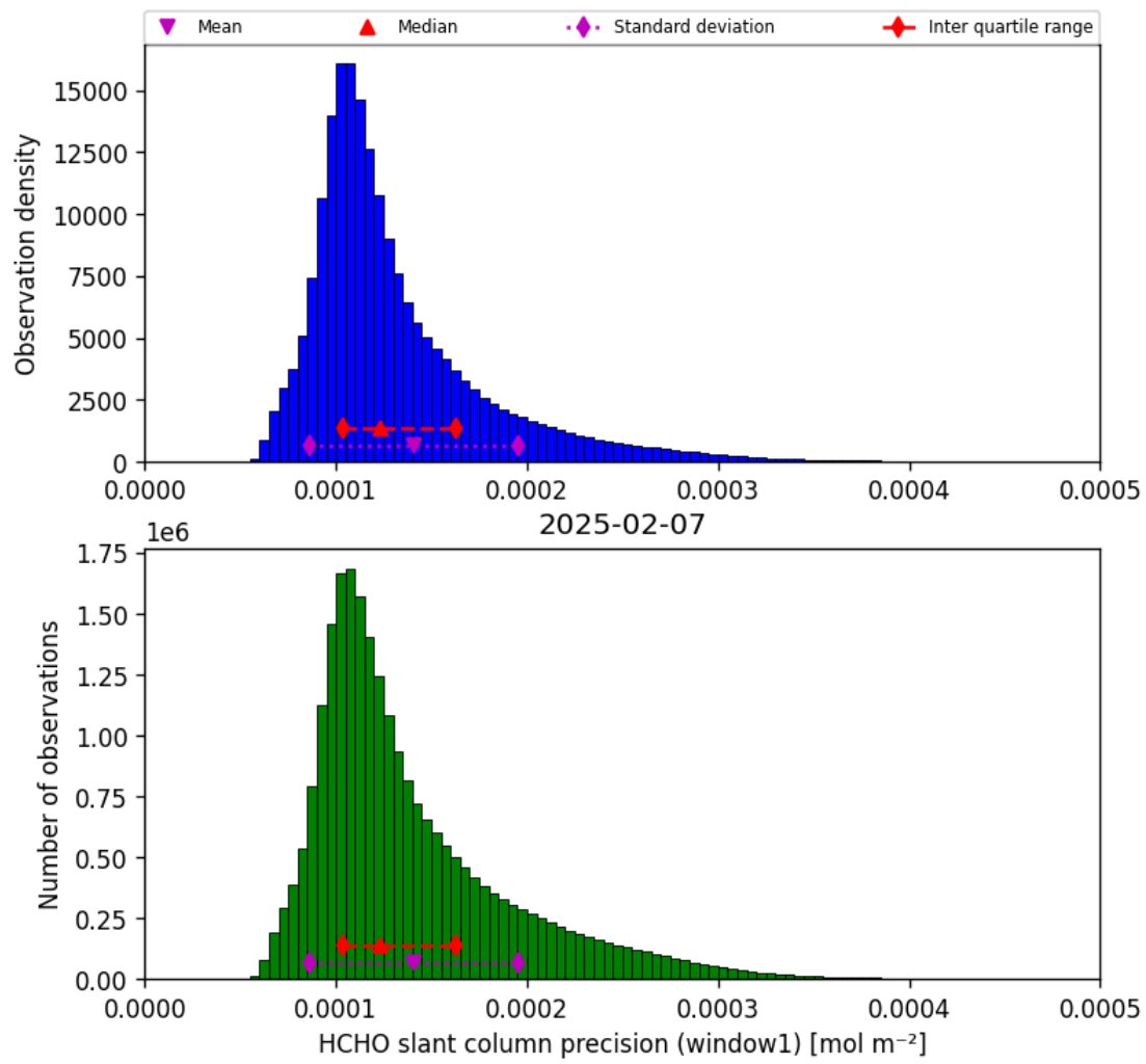
Figure 37: Histogram of “HCHO slant column precision (window1)” for 2025-02-07 to 2025-02-08
