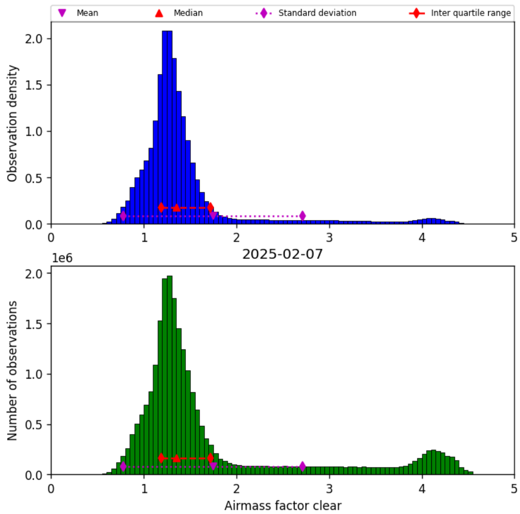
Figure 40: Histogram of “Airmass factor clear” for 2025-02-07 to 2025-02-08
