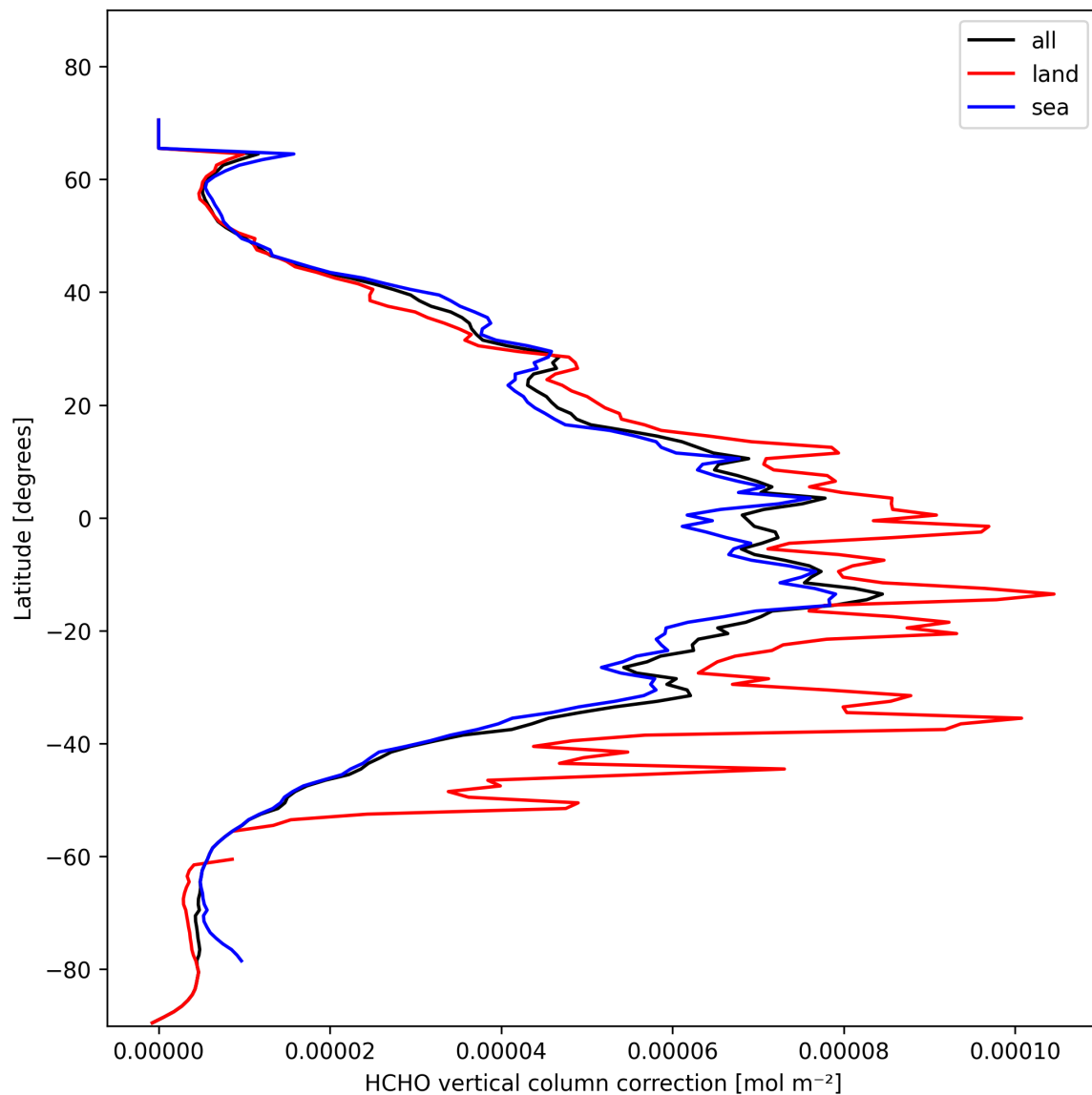
Figure 21: Zonal average of “HCHO vertical column correction” for 2025-02-07 to 2025-02-08.
