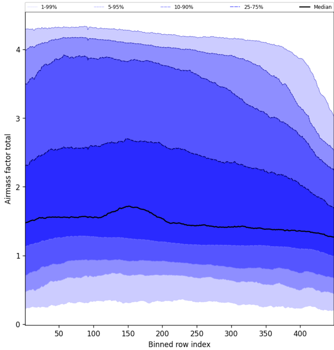
Figure 52: Along track statistics of “Airmass factor total” for 2025-02-07 to 2025-02-08
