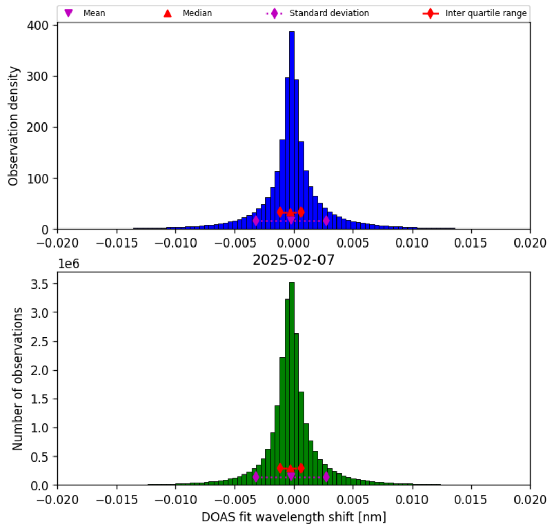
Figure 42: Histogram of “DOAS fit wavelength shift” for 2025-02-07 to 2025-02-08
