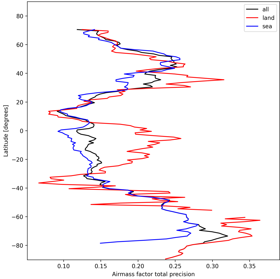
Figure 25: Zonal average of “Airmass factor total precision” for 2025-02-07 to 2025-02-08.
