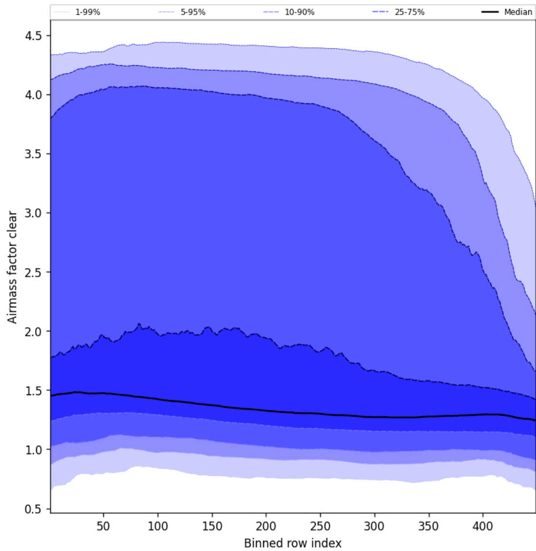
Figure 54: Along track statistics of “Airmass factor clear” for 2025-02-07 to 2025-02-08
