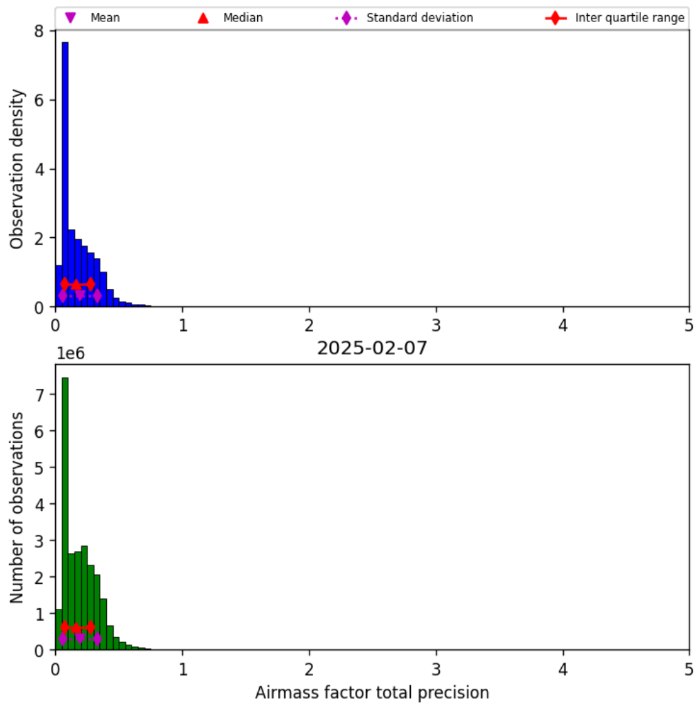
Figure 39: Histogram of “Airmass factor total precision” for 2025-02-07 to 2025-02-08
