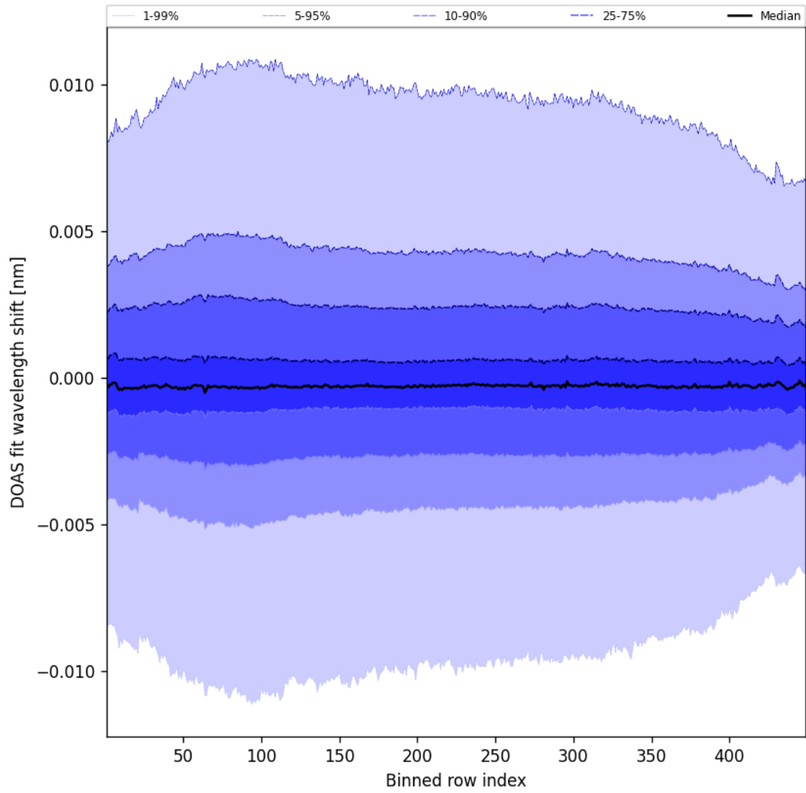
Figure 56: Along track statistics of “DOAS fit wavelength shift” for 2025-02-07 to 2025-02-08
