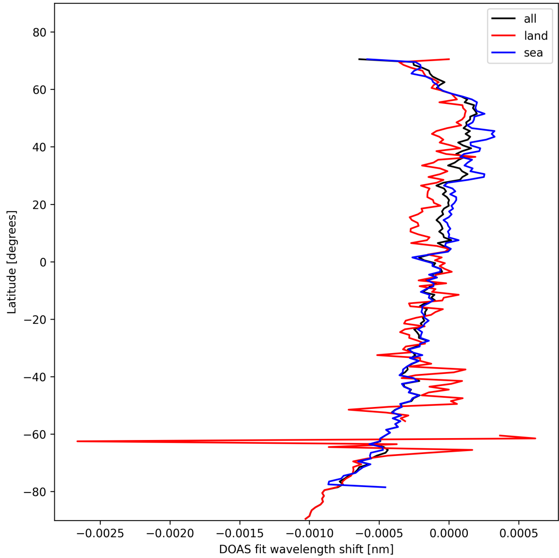
Figure 28: Zonal average of "DOAS fit wavelength shift" for 2025-02-07 to 2025-02-08.
