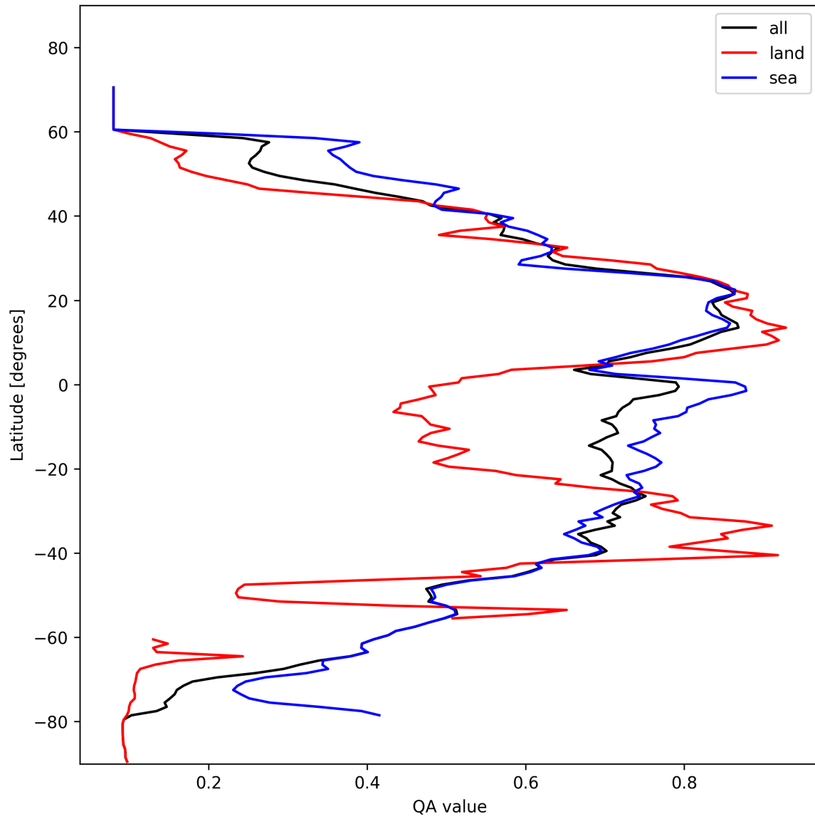
Figure 18: Zonal average of “QA value” for 2025-02-07 to 2025-02-08.
