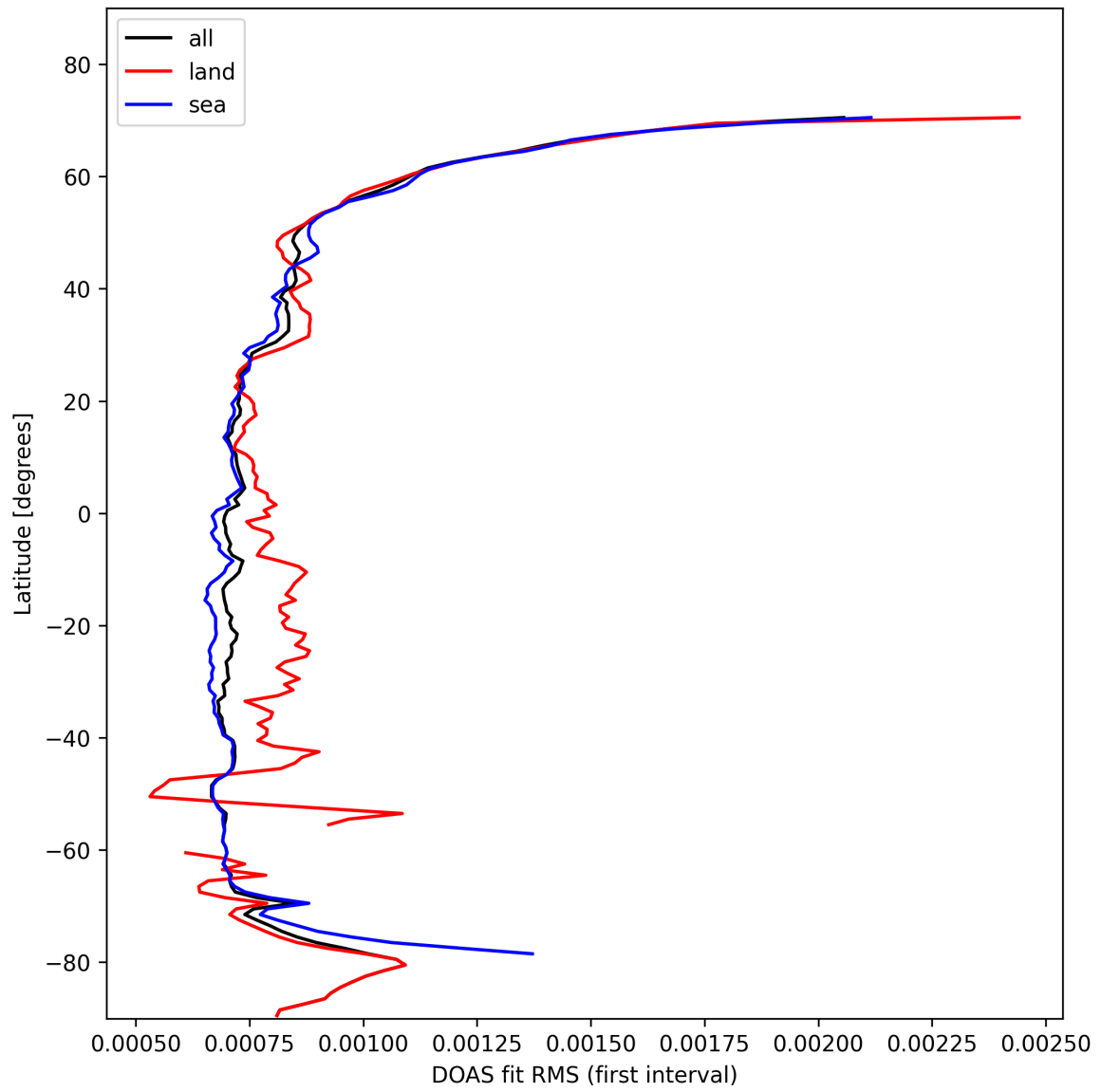
Figure 30: Zonal average of “DOAS fit RMS (first interval)” for 2025-02-07 to 2025-02-08.
