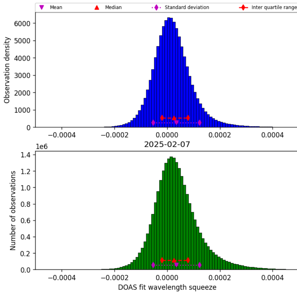
Figure 43: Histogram of “DOAS fit wavelength squeeze” for 2025-02-07 to 2025-02-08
