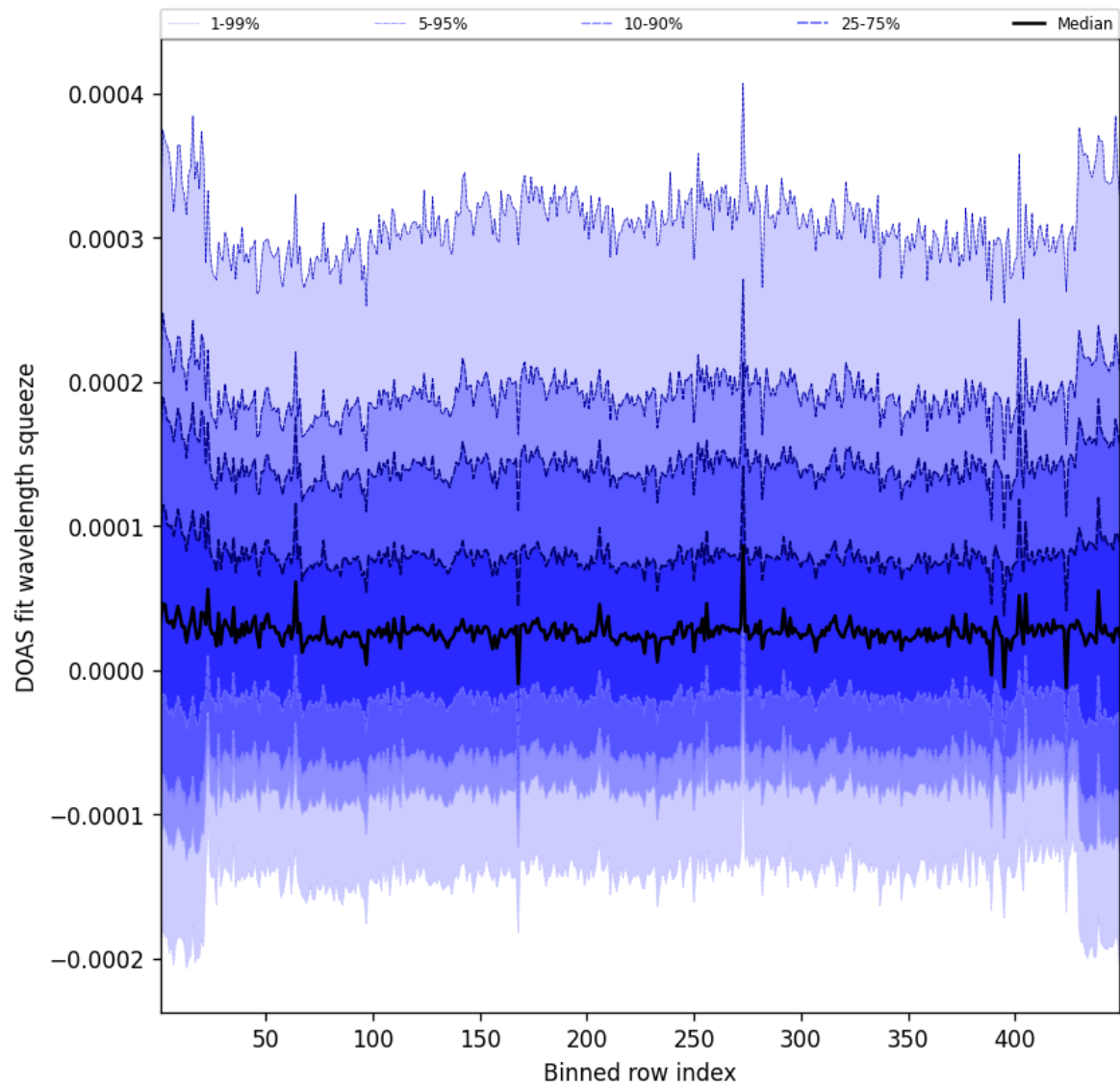
Figure 57: Along track statistics of “DOAS fit wavelength squeeze” for 2025-02-07 to 2025-02-08
