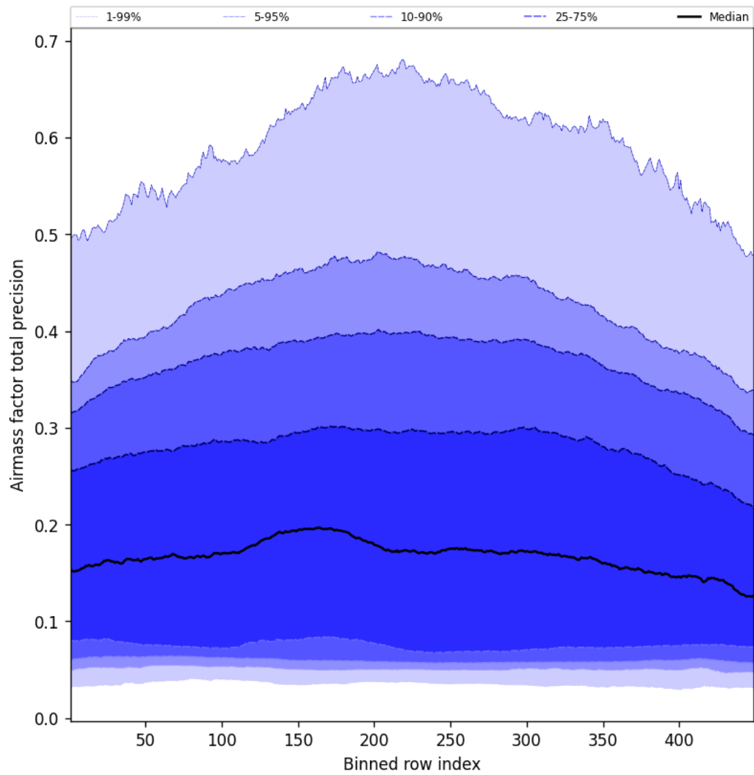
Figure 53: Along track statistics of “Airmass factor total precision” for 2025-02-07 to 2025-02-08
