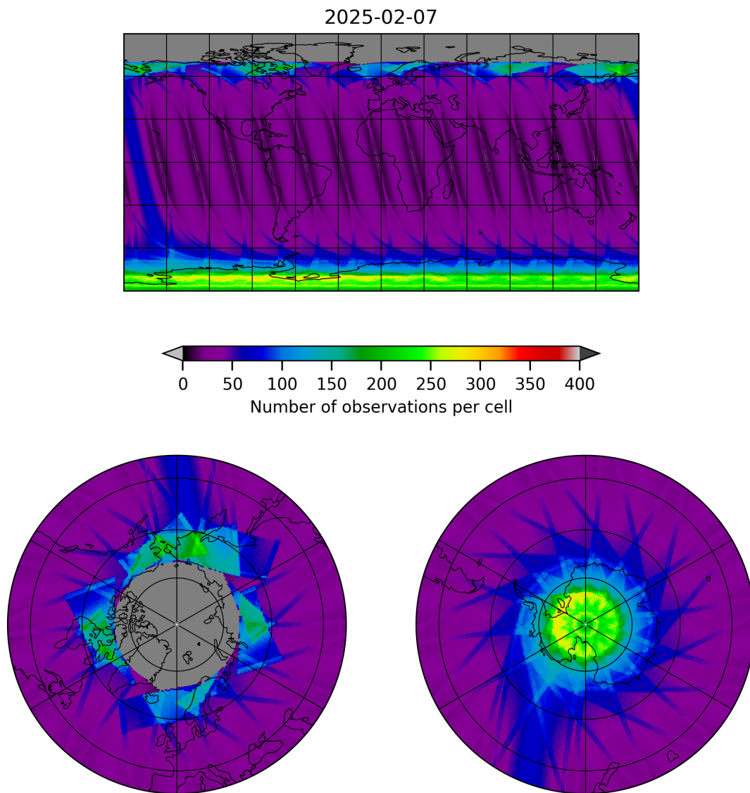
Figure 17: Map of the number of observations for 2025-02-07 to 2025-02-08
