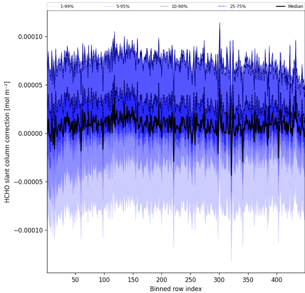
Figure 59: Along track statistics of “HCHO slant column correction” for 2025-02-07 to 2025-02-08
