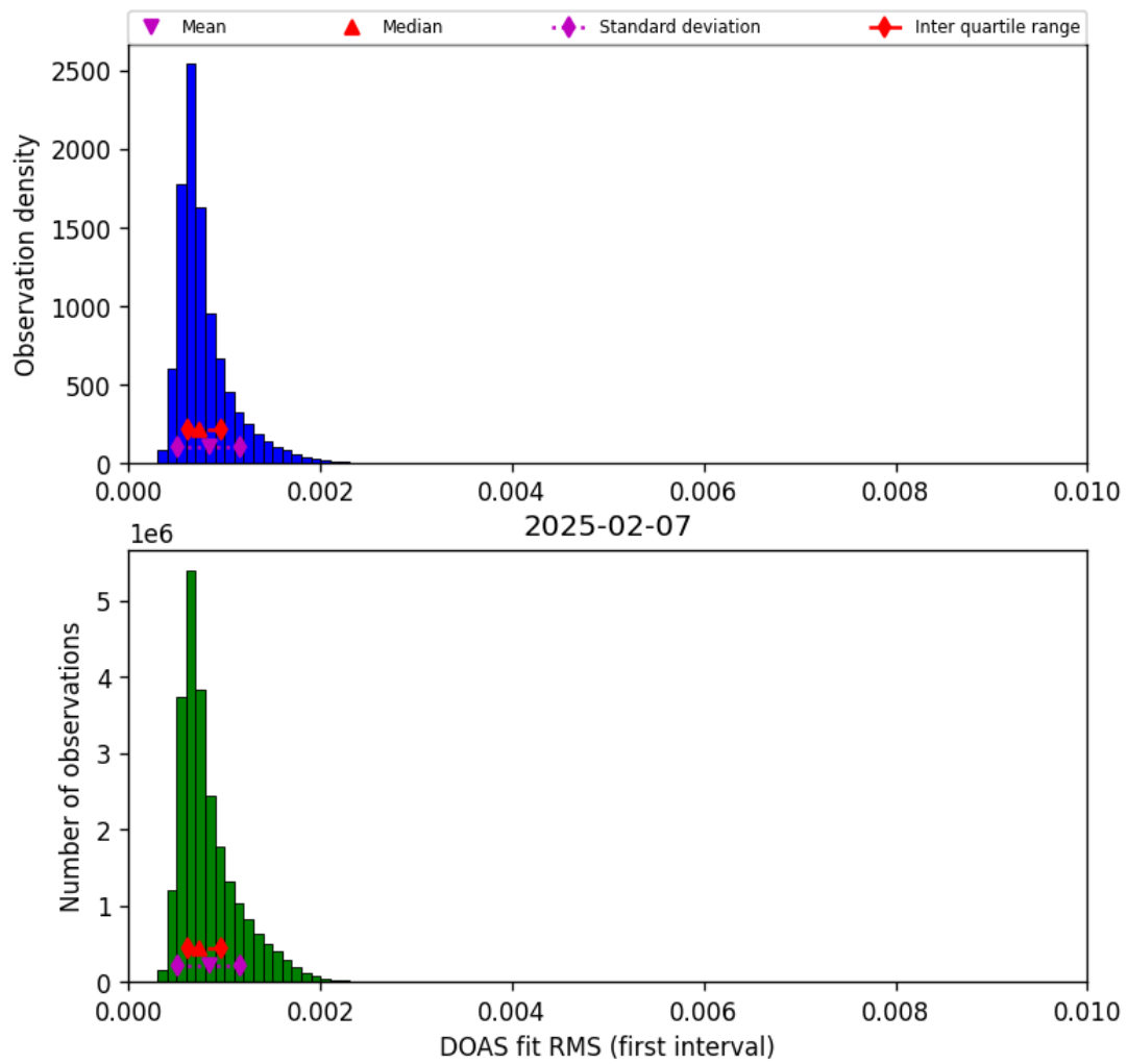
Figure 44: Histogram of “DOAS fit RMS (first interval)” for 2025-02-07 to 2025-02-08
