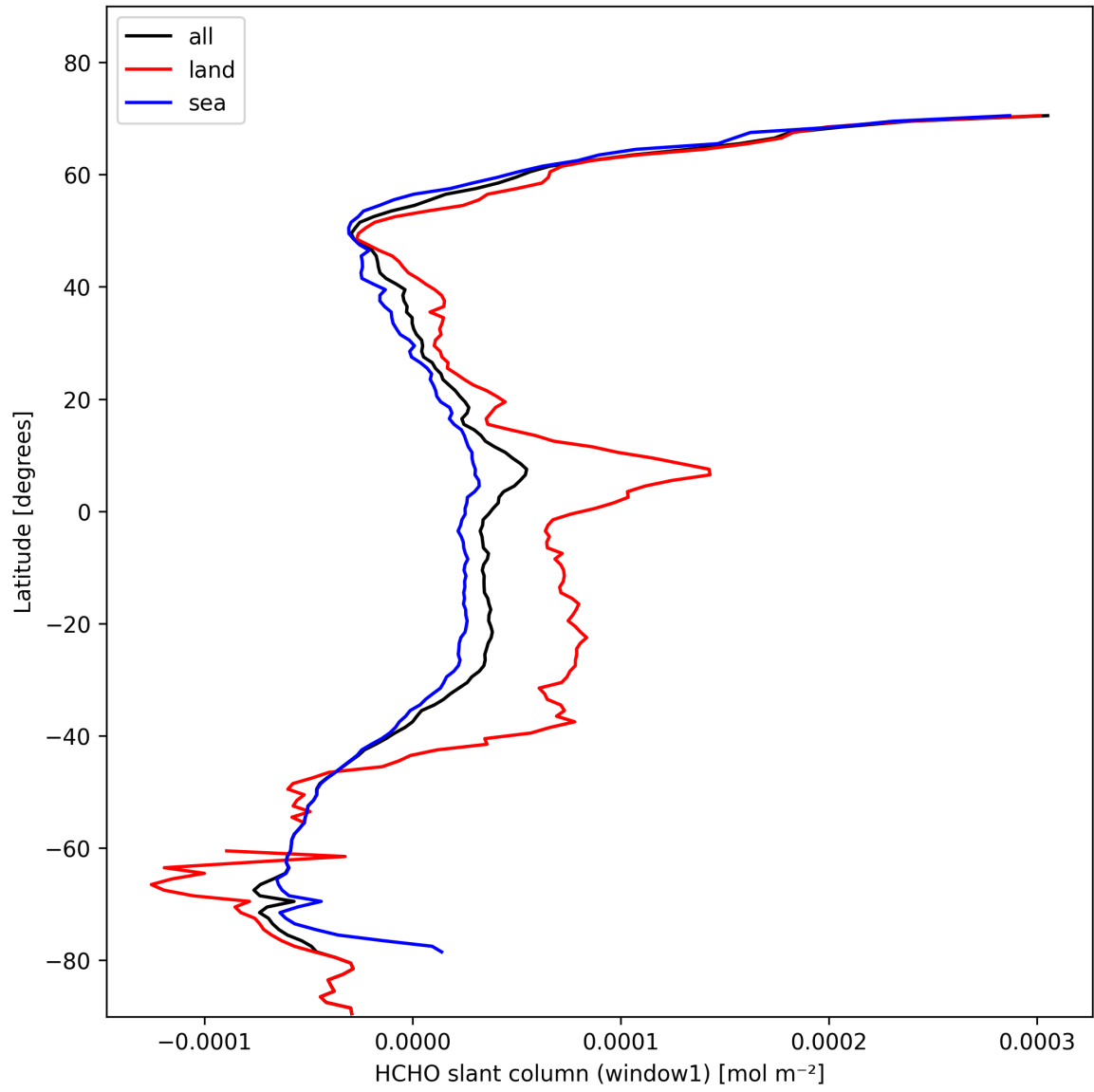
Figure 22: Zonal average of “HCHO slant column (window1)” for 2025-02-07 to 2025-02-08.
