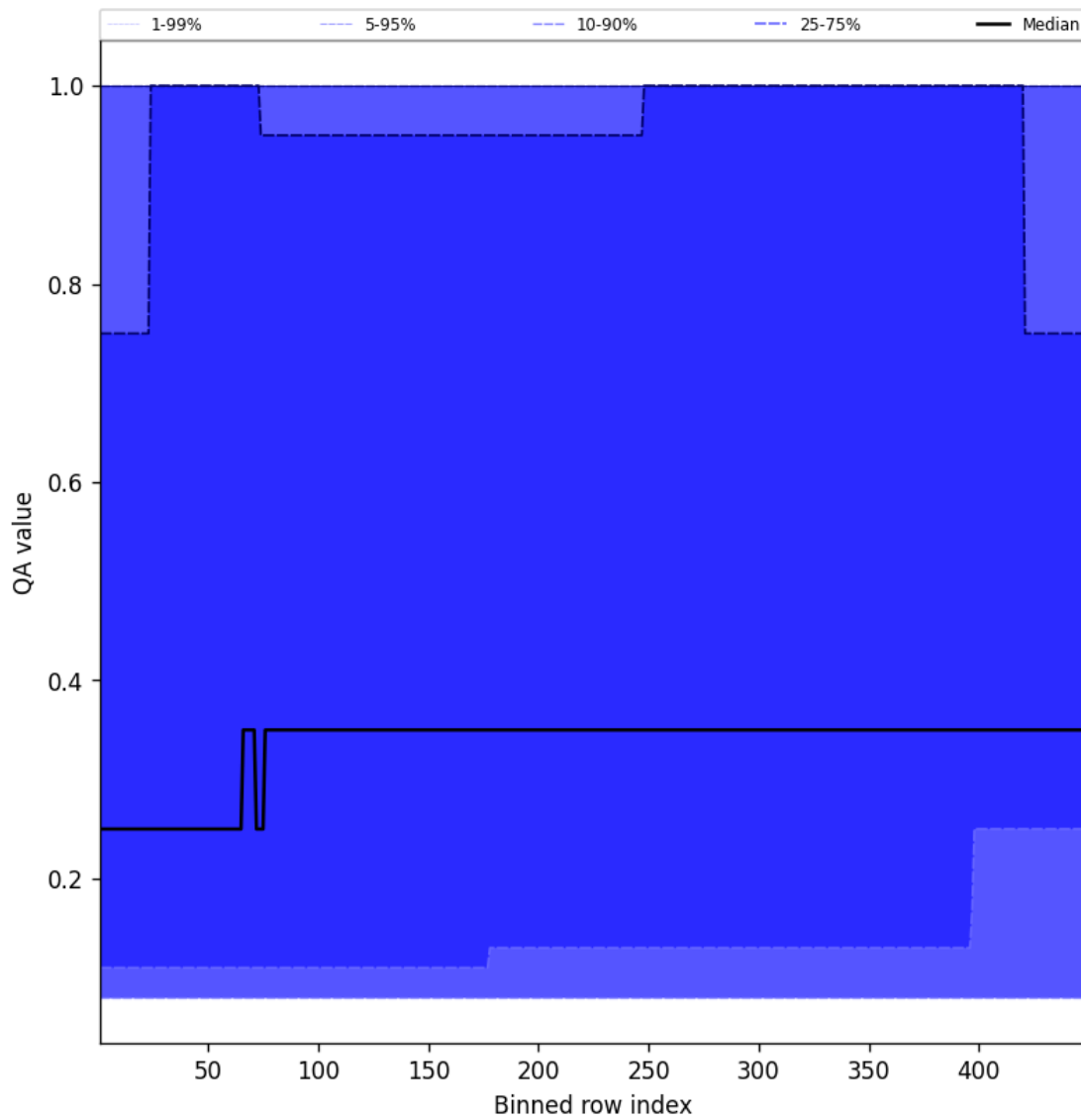
Figure 46: Along track statistics of “QA value” for 2025-02-07 to 2025-02-08
