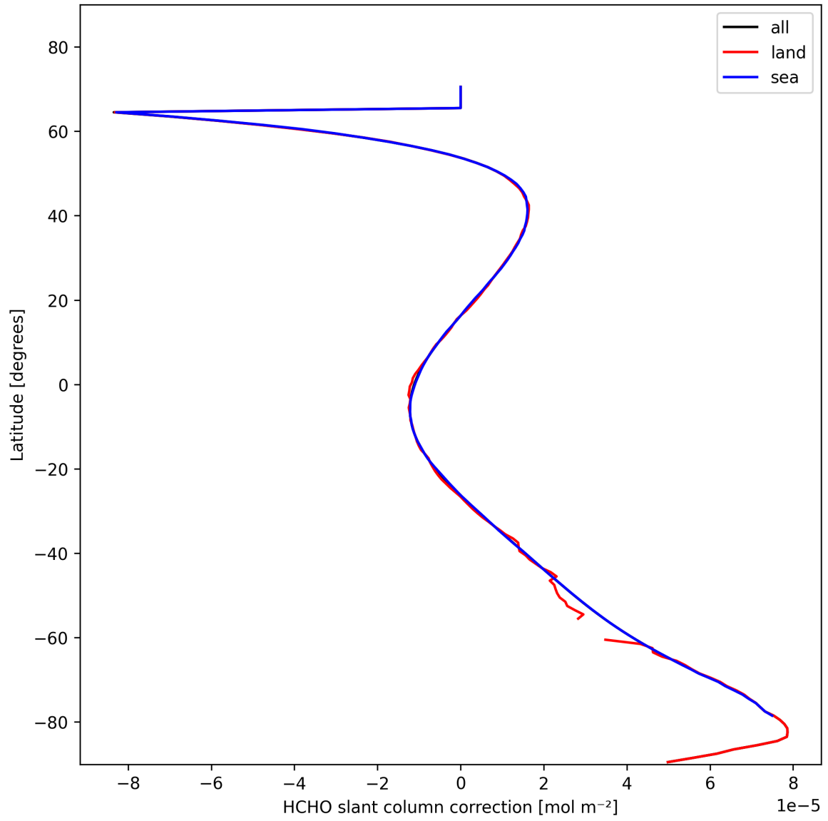
Figure 31: Zonal average of “HCHO slant column correction” for 2025-02-07 to 2025-02-08.
