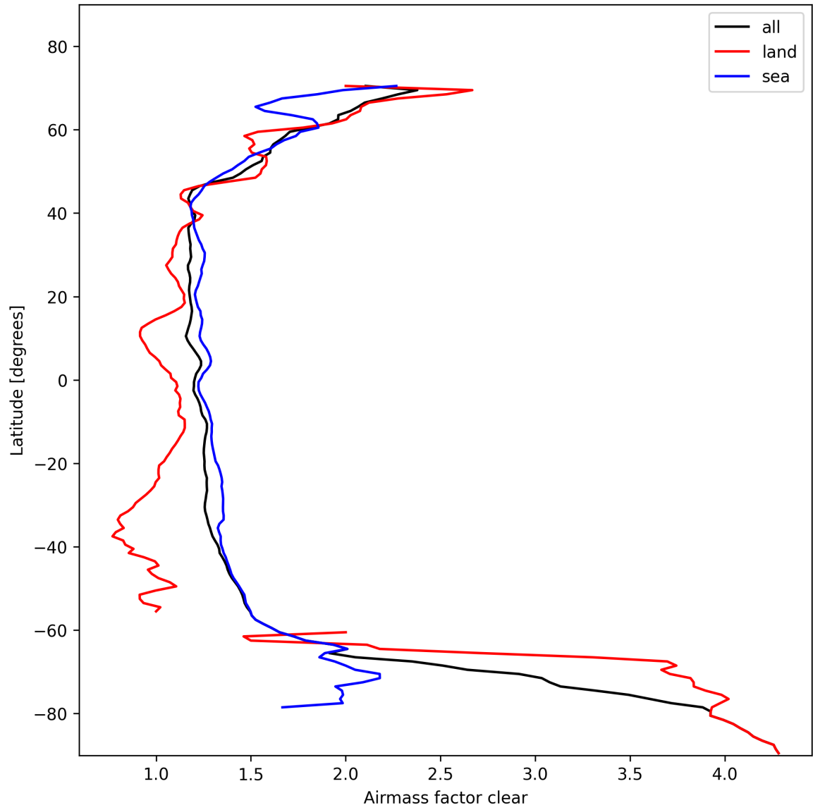
Figure 26: Zonal average of “Airmass factor clear” for 2025-02-07 to 2025-02-08.
