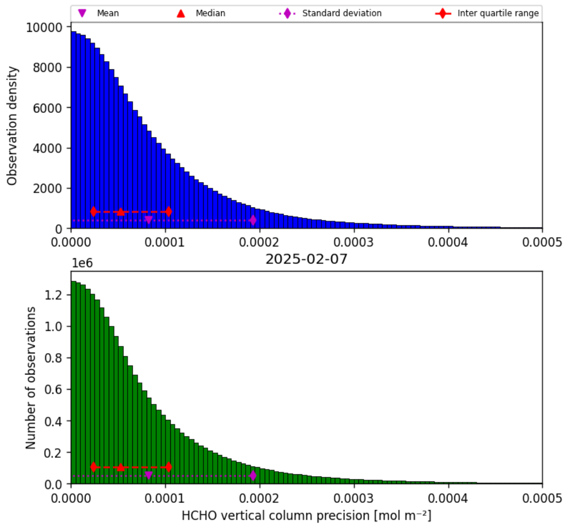
Figure 34: Histogram of “HCHO vertical column precision” for 2025-02-07 to 2025-02-08
