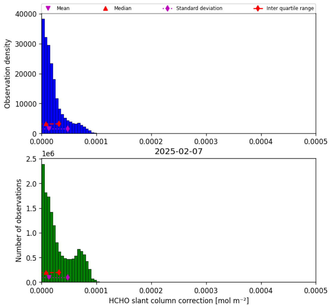
Figure 45: Histogram of “HCHO slant column correction” for 2025-02-07 to 2025-02-08
