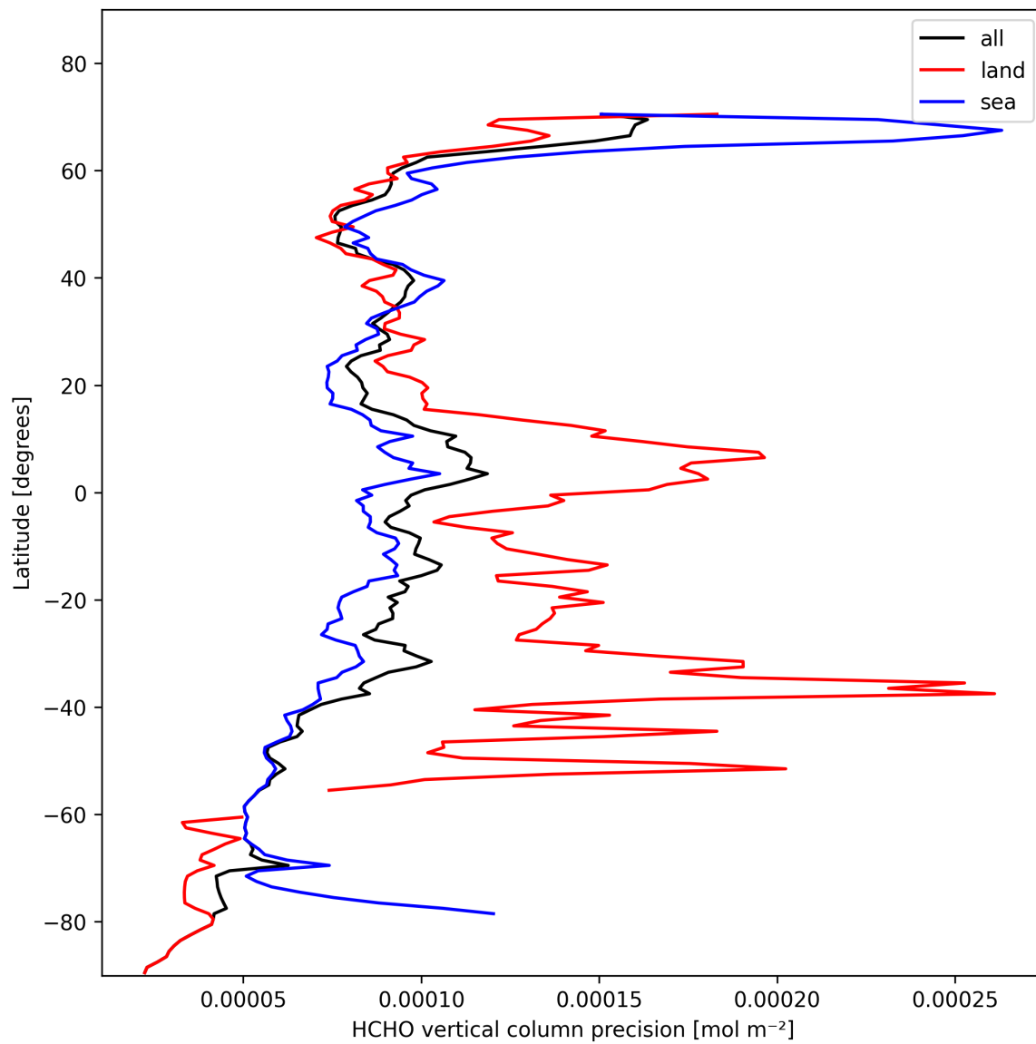
Figure 20: Zonal average of “HCHO vertical column precision” for 2025-02-07 to 2025-02-08.
