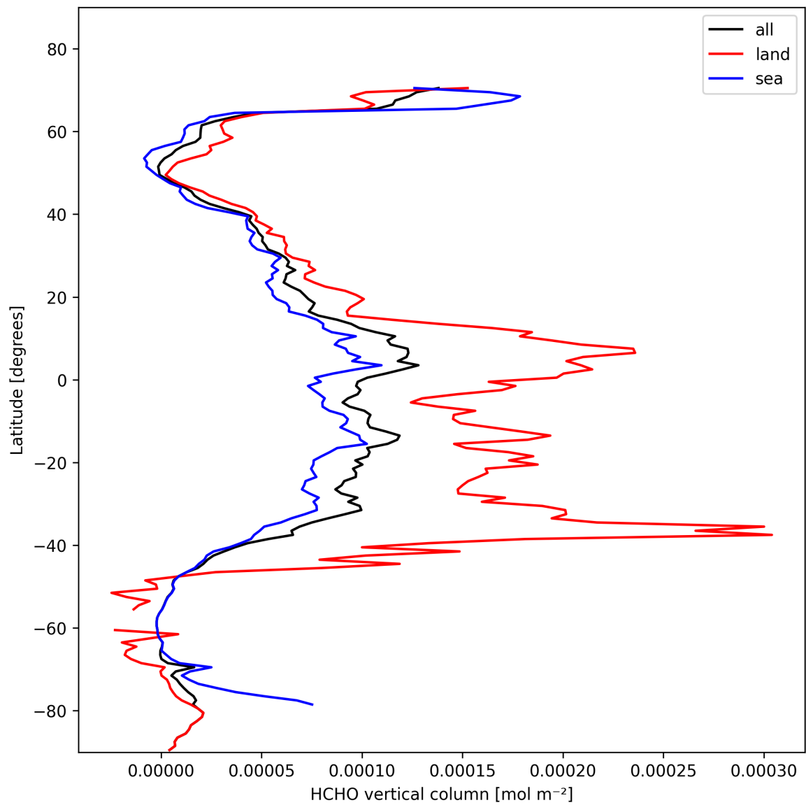
Figure 19: Zonal average of “HCHO vertical column” for 2025-02-07 to 2025-02-08.
