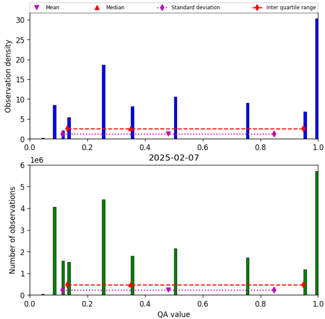
Figure 32: Histogram of “QA value” for 2025-02-07 to 2025-02-08
