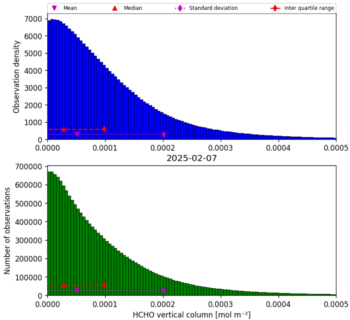
Figure 33: Histogram of “HCHO vertical column” for 2025-02-07 to 2025-02-08
