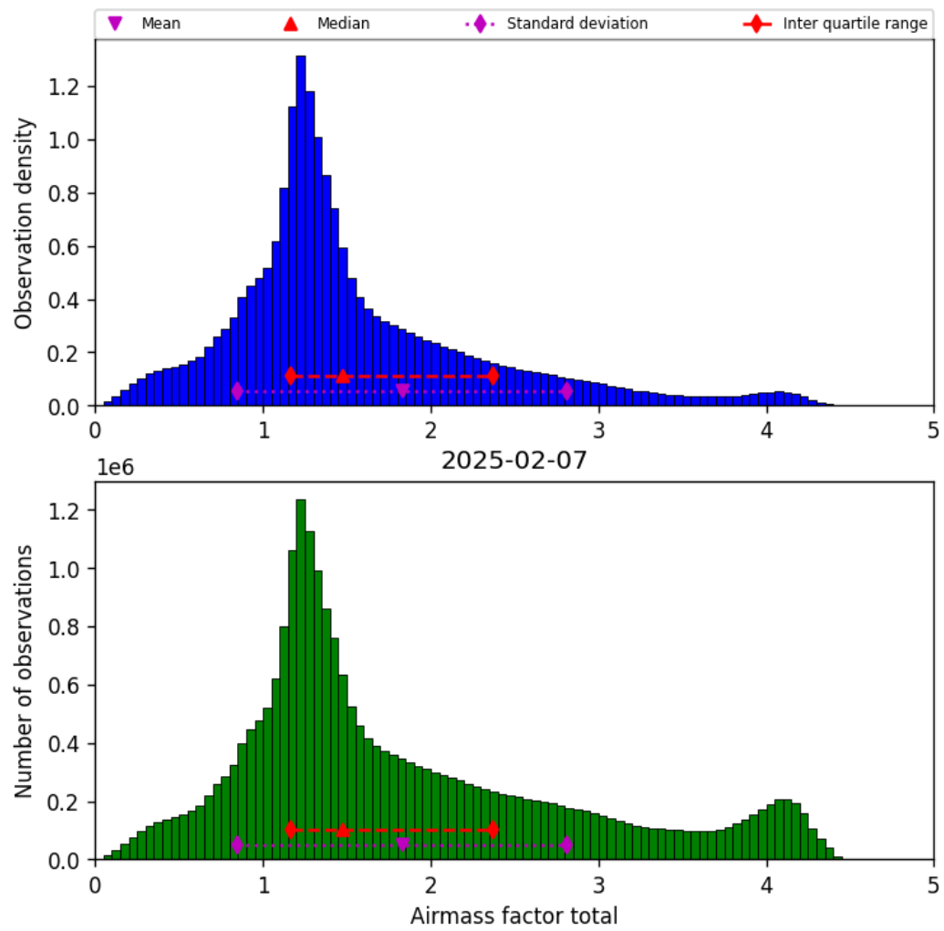
Figure 38: Histogram of “Airmass factor total” for 2025-02-07 to 2025-02-08
