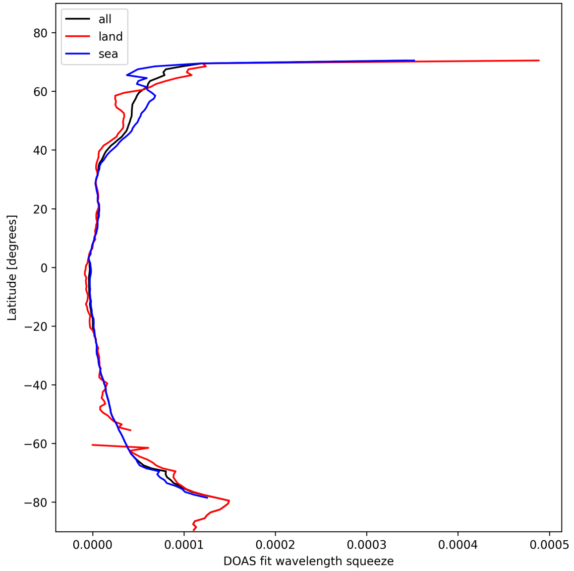
Figure 29: Zonal average of “DOAS fit wavelength squeeze” for 2025-02-07 to 2025-02-08.
