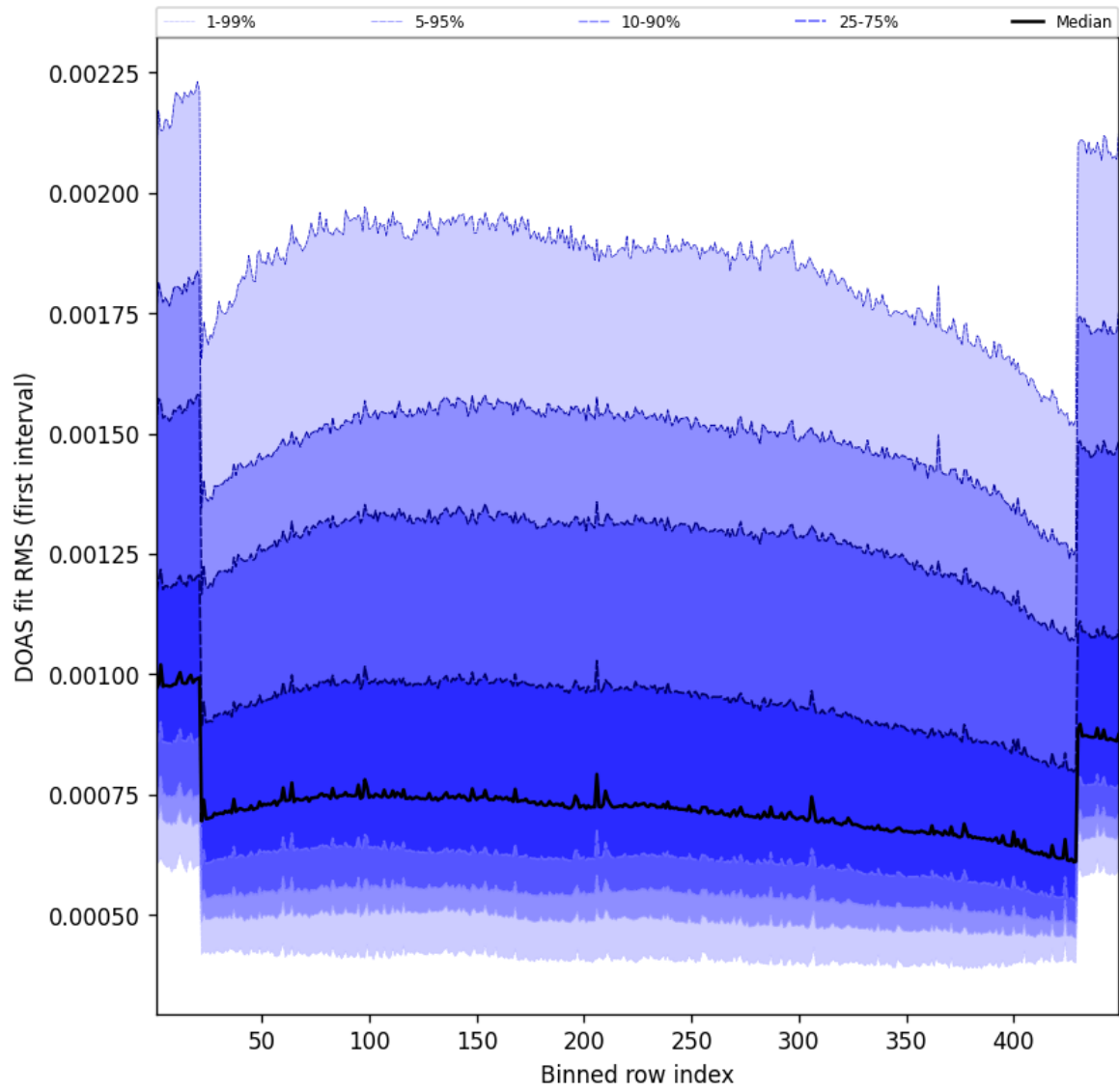
Figure 58: Along track statistics of “DOAS fit RMS (first interval)” for 2025-02-07 to 2025-02-08
