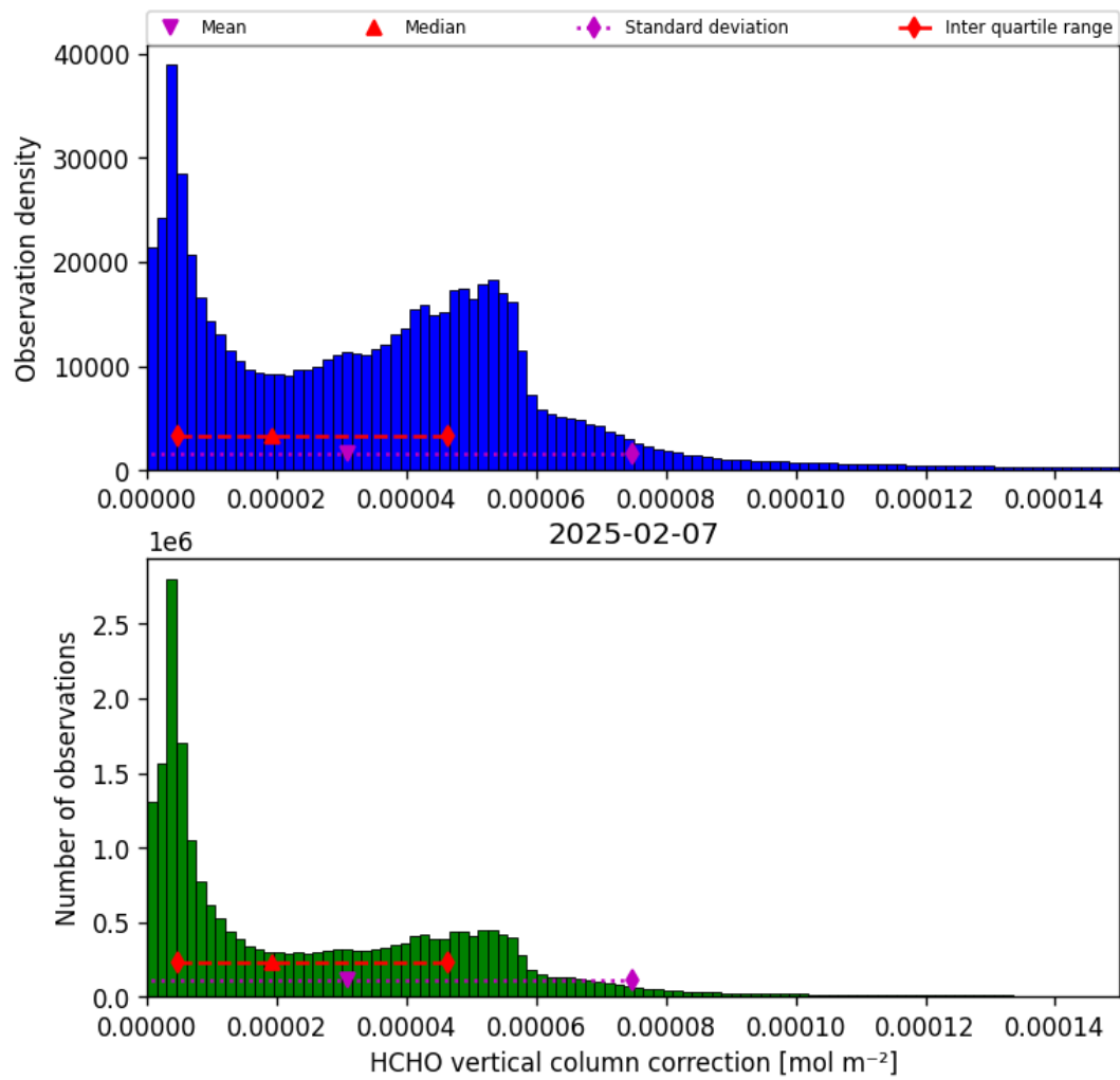
Figure 35: Histogram of “HCHO vertical column correction” for 2025-02-07 to 2025-02-08
