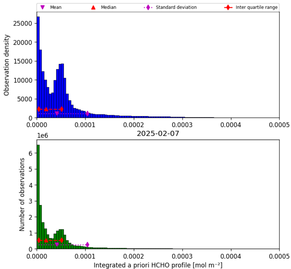
Figure 41: Histogram of “Integrated a priori HCHO profile” for 2025-02-07 to 2025-02-08
