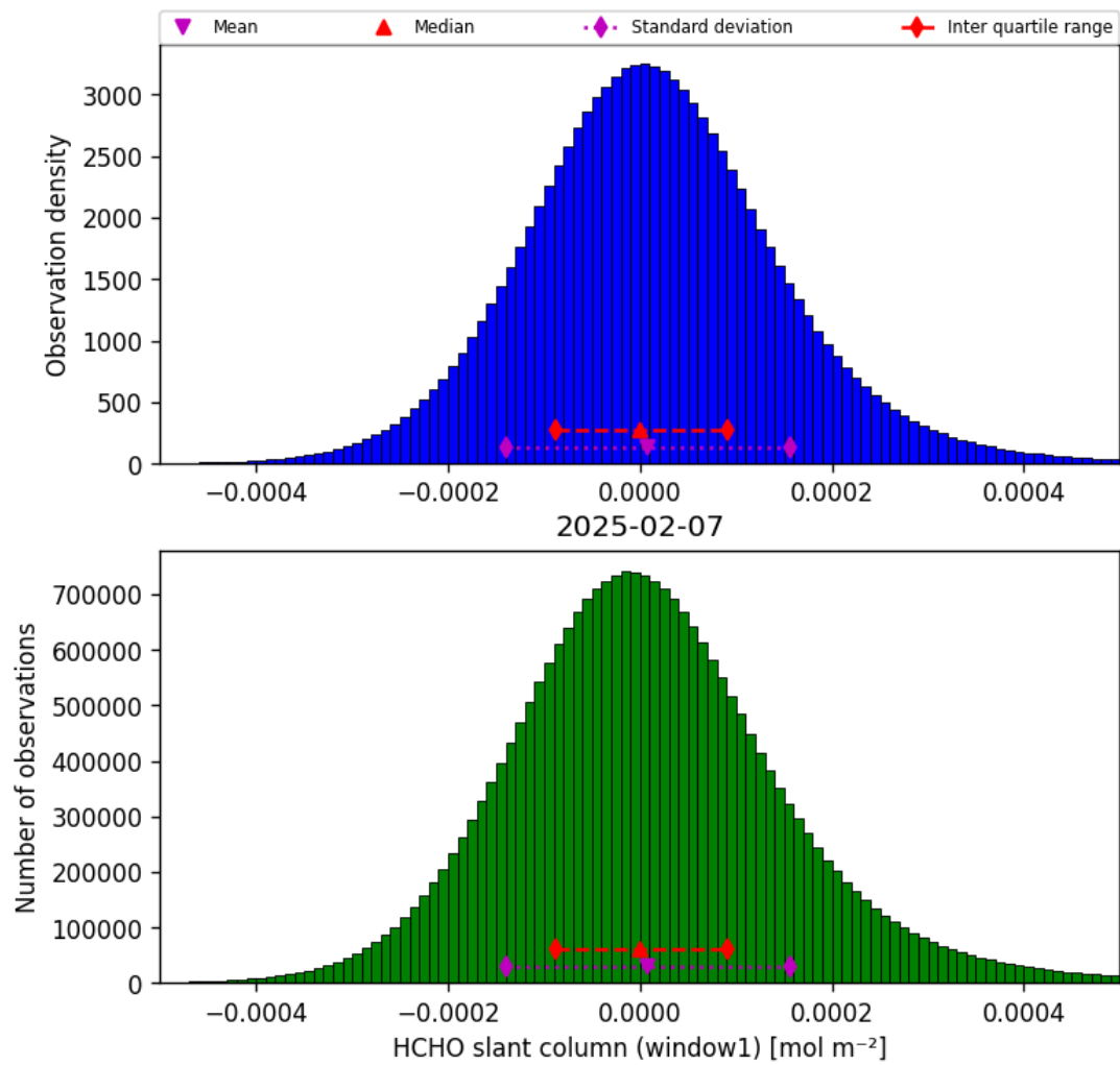
Figure 36: Histogram of “HCHO slant column (window1)” for 2025-02-07 to 2025-02-08
