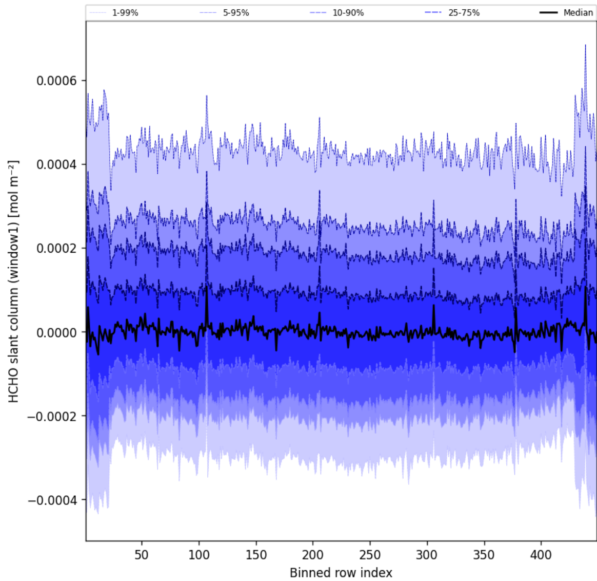
Figure 50: Along track statistics of “HCHO slant column (window1)” for 2025-02-07 to 2025-02-08
