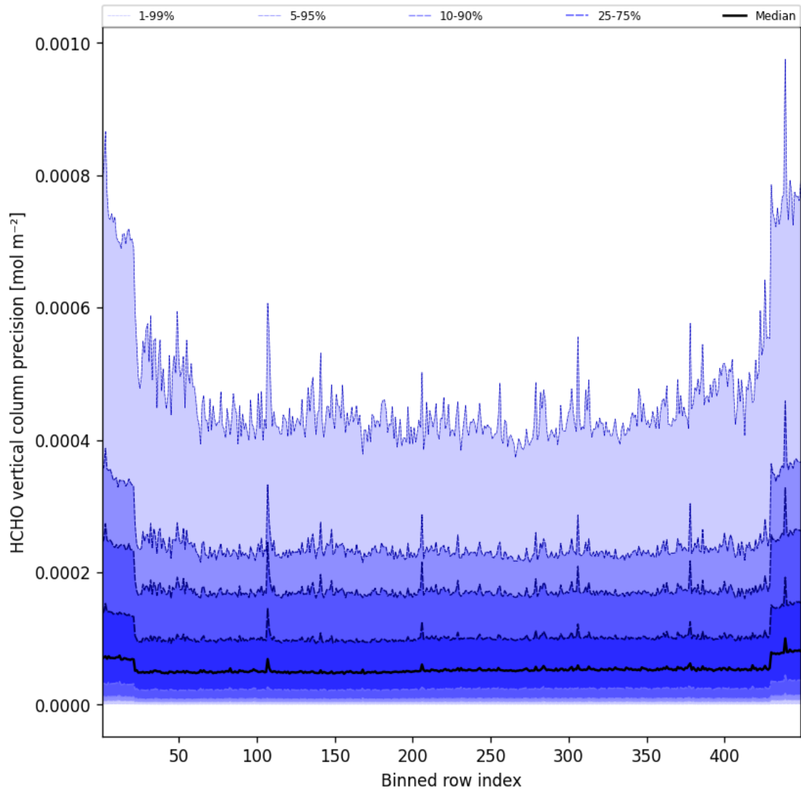
Figure 48: Along track statistics of “HCHO vertical column precision” for 2025-02-07 to 2025-02-08
