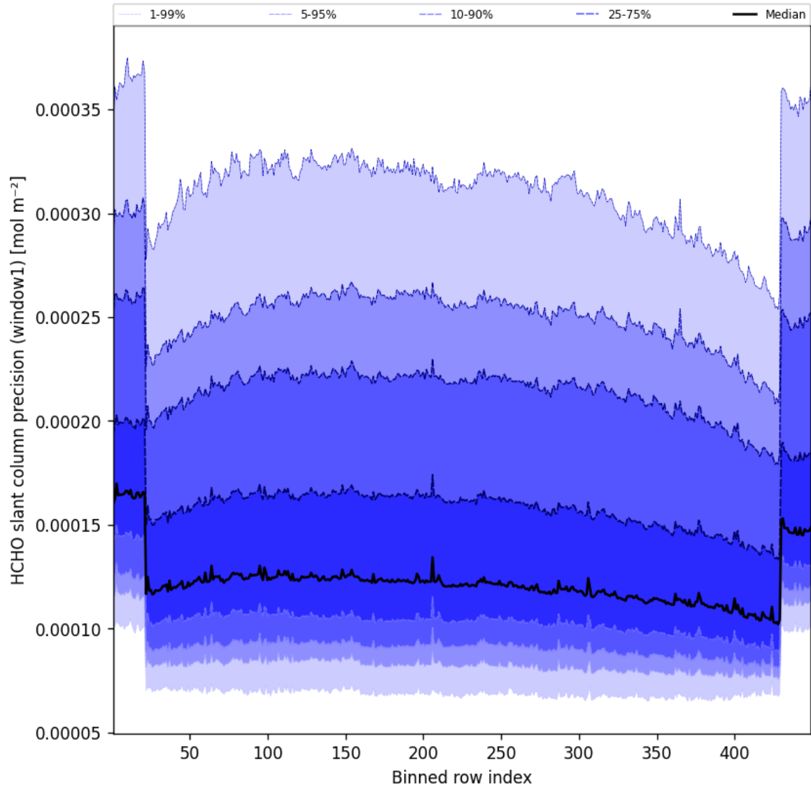
Figure 51: Along track statistics of “HCHO slant column precision (window1)” for 2025-02-07 to 2025-02-08
