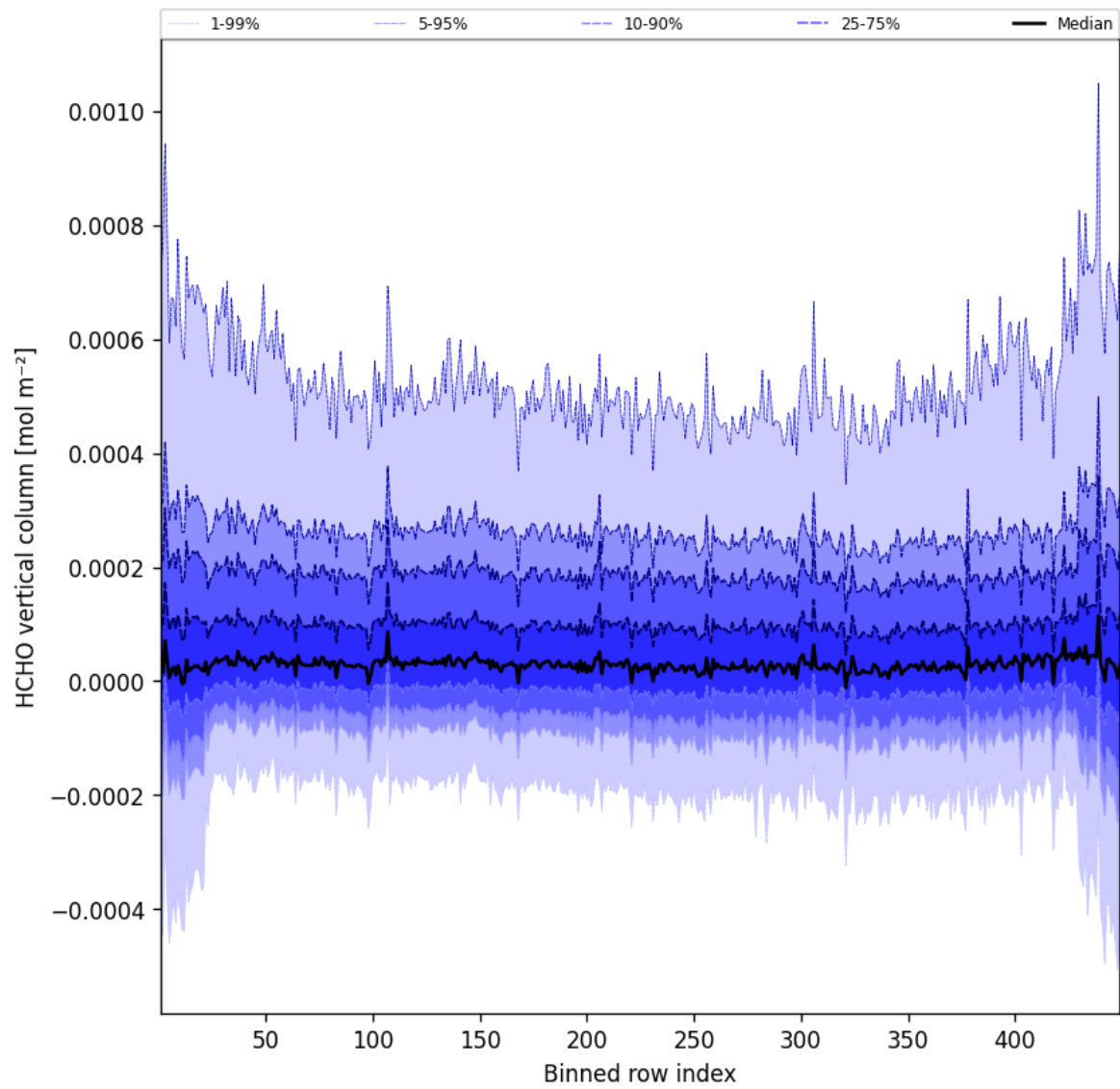
Figure 47: Along track statistics of “HCHO vertical column” for 2025-02-07 to 2025-02-08
