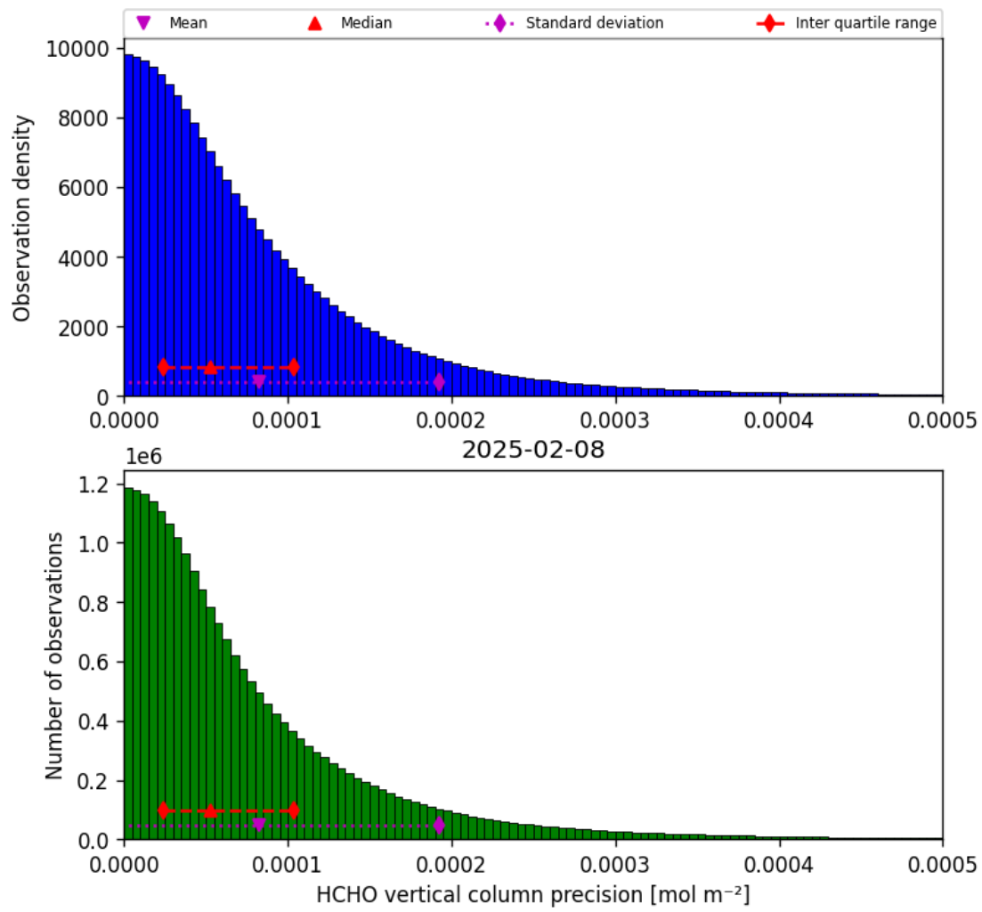
Figure 34: Histogram of “HCHO vertical column precision” for 2025-02-08 to 2025-02-09
