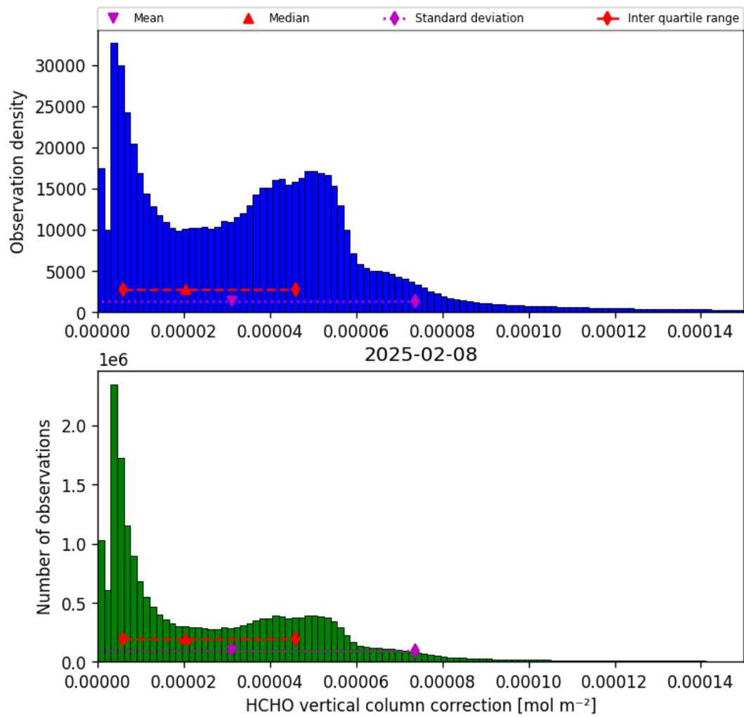
Figure 35: Histogram of “HCHO vertical column correction” for 2025-02-08 to 2025-02-09
