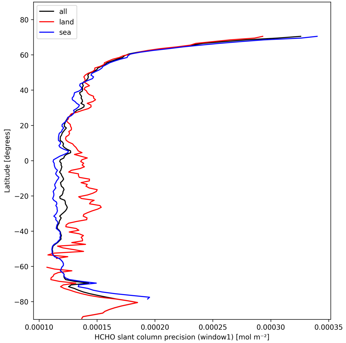
Figure 23: Zonal average of “HCHO slant column precision (window1)” for 2025-02-08 to 2025-02-09.
