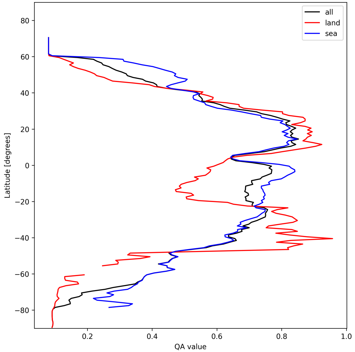
Figure 18: Zonal average of “QA value” for 2025-02-08 to 2025-02-09.
