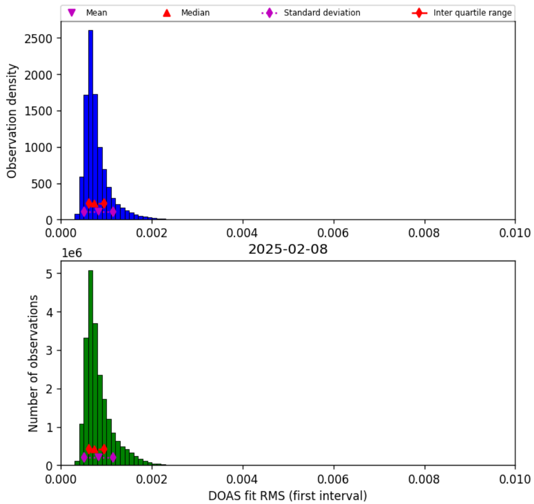
Figure 44: Histogram of “DOAS fit RMS (first interval)” for 2025-02-08 to 2025-02-09
