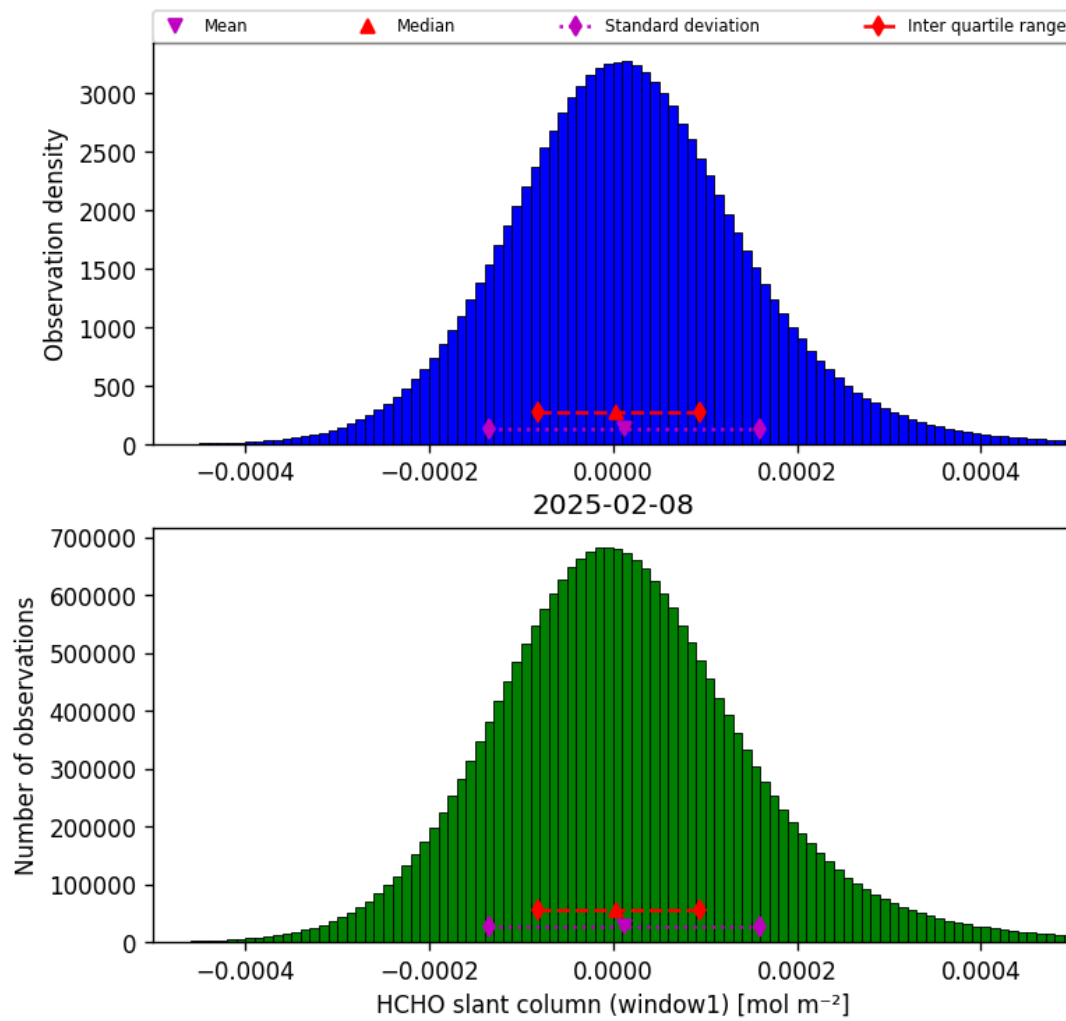
Figure 36: Histogram of “HCHO slant column (window1)” for 2025-02-08 to 2025-02-09
