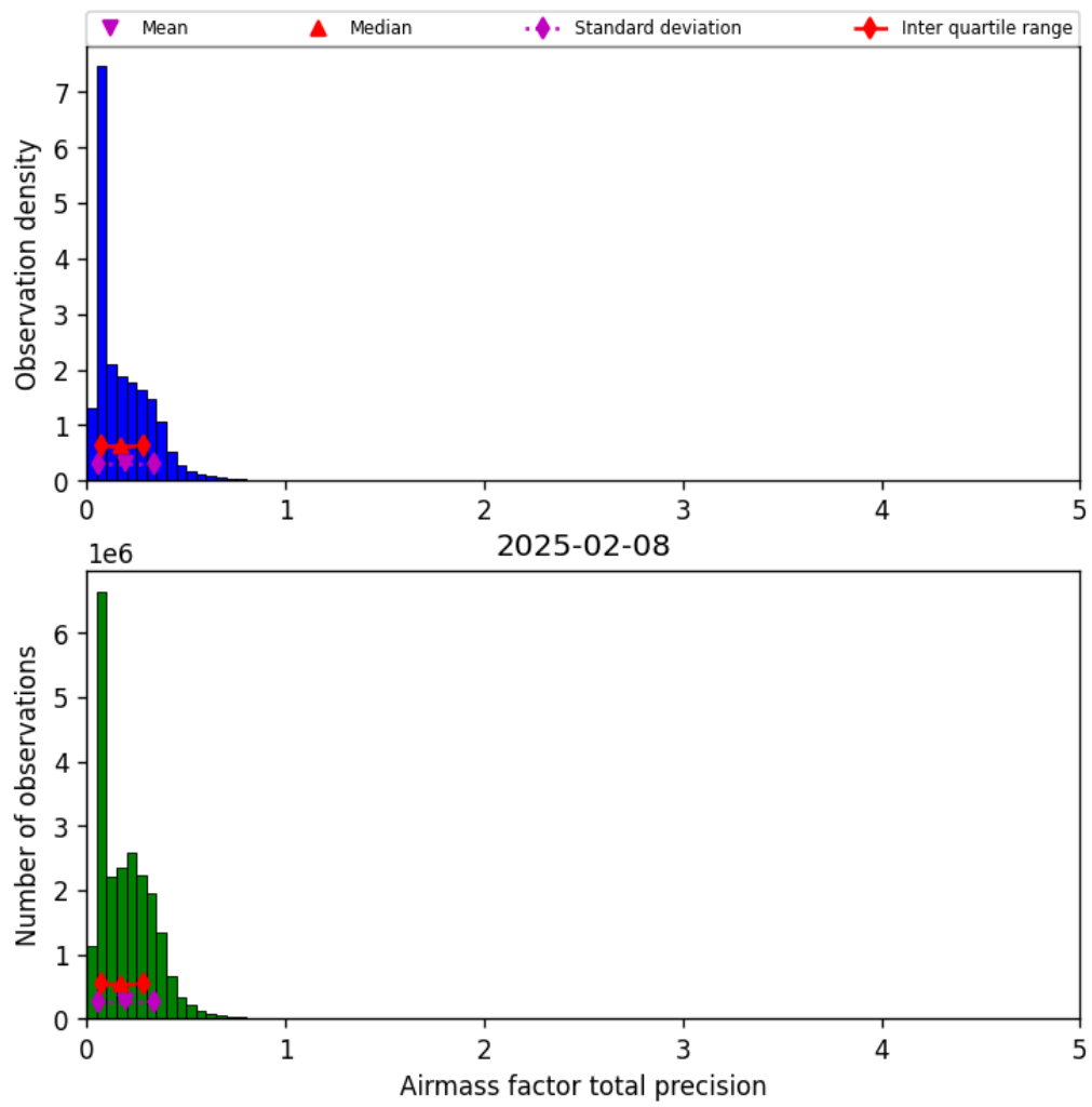
Figure 39: Histogram of “Airmass factor total precision” for 2025-02-08 to 2025-02-09
