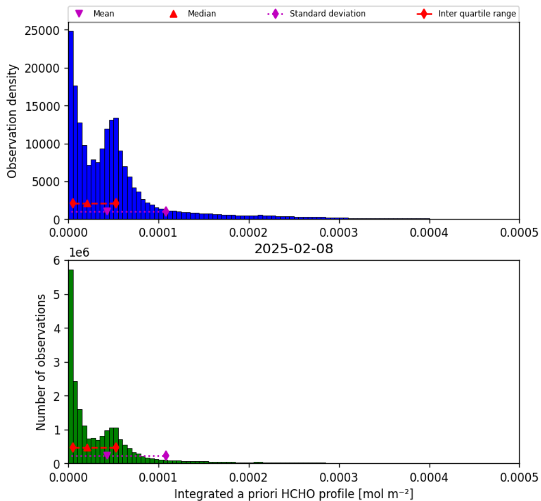
Figure 41: Histogram of “Integrated a priori HCHO profile” for 2025-02-08 to 2025-02-09
