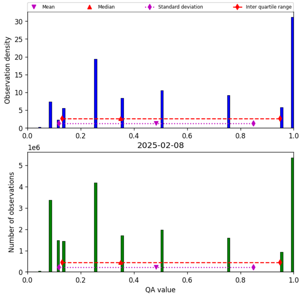
Figure 32: Histogram of “QA value” for 2025-02-08 to 2025-02-09
