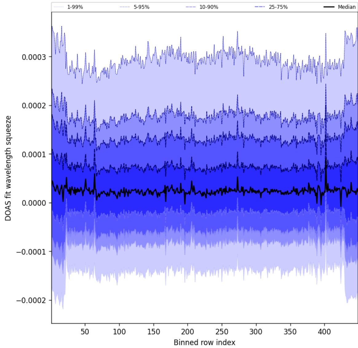
Figure 57: Along track statistics of “DOAS fit wavelength squeeze” for 2025-02-08 to 2025-02-09
