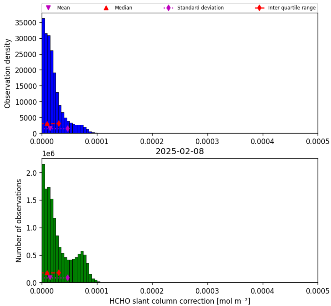
Figure 45: Histogram of “HCHO slant column correction” for 2025-02-08 to 2025-02-09
