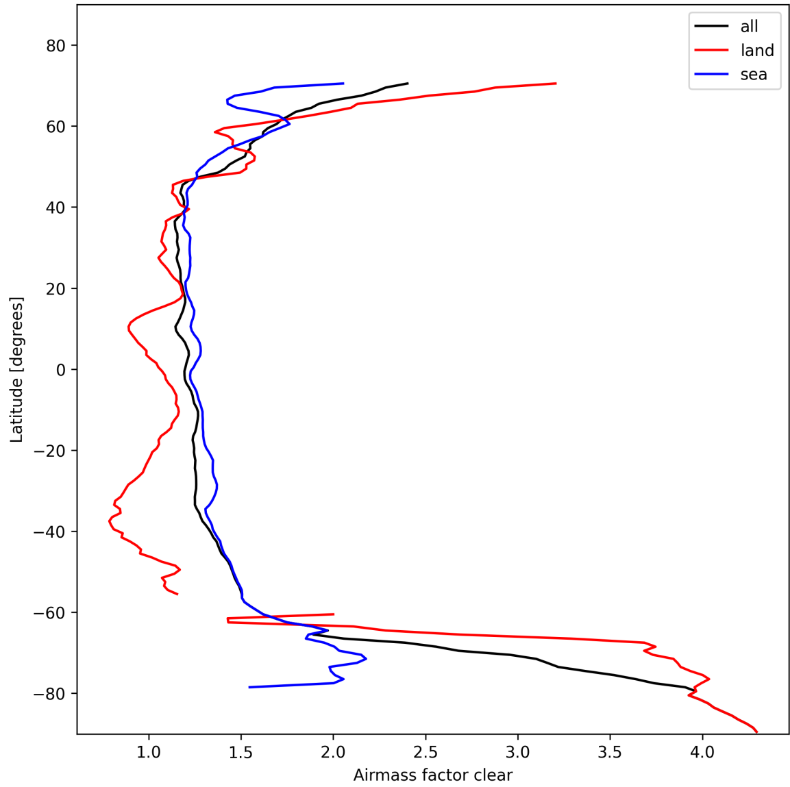
Figure 26: Zonal average of “Airmass factor clear” for 2025-02-08 to 2025-02-09.
