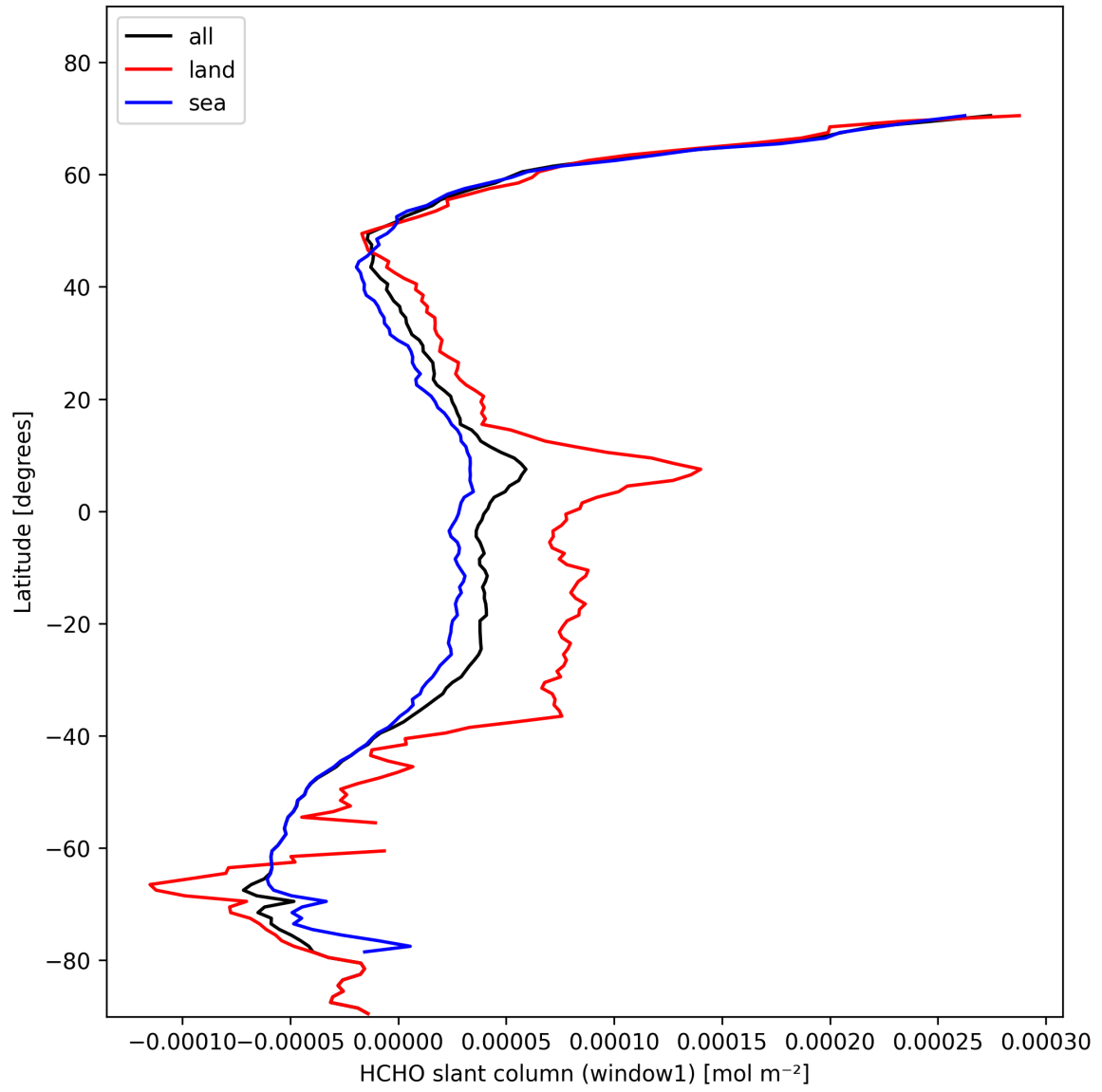
Figure 22: Zonal average of “HCHO slant column (window1)” for 2025-02-08 to 2025-02-09.
