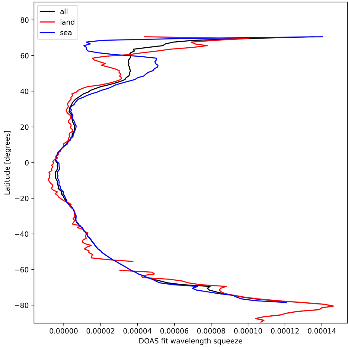
Figure 29: Zonal average of “DOAS fit wavelength squeeze” for 2025-02-08 to 2025-02-09.
