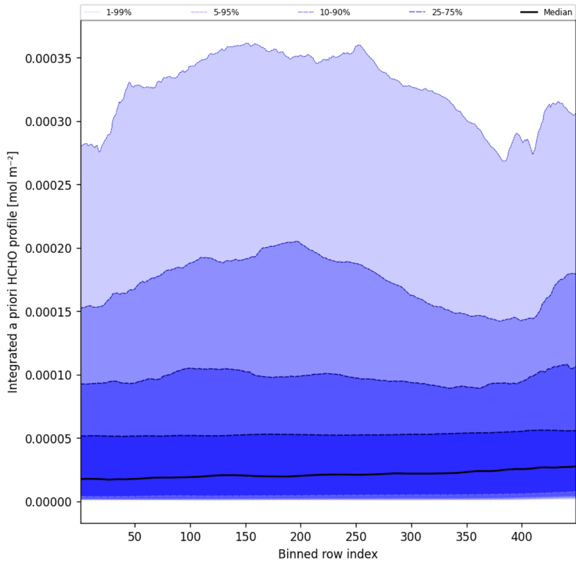
Figure 55: Along track statistics of “Integrated a priori HCHO profile” for 2025-02-08 to 2025-02-09
