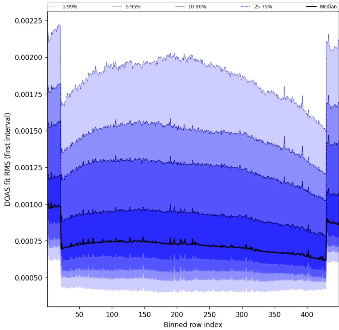
Figure 58: Along track statistics of “DOAS fit RMS (first interval)” for 2025-02-08 to 2025-02-09
