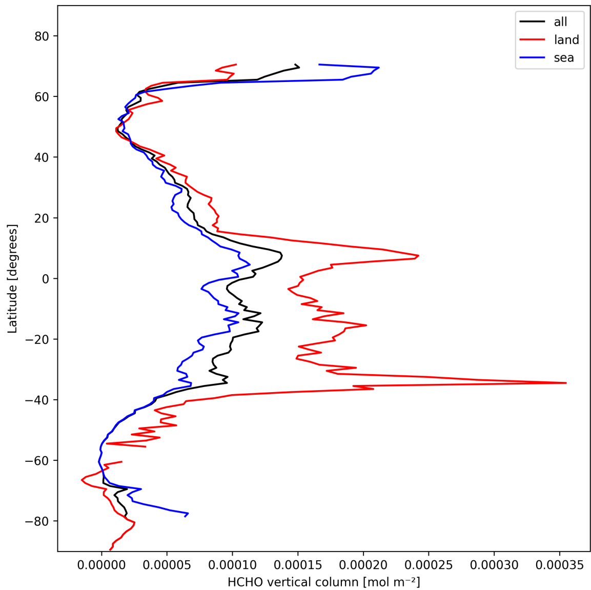
Figure 19: Zonal average of “HCHO vertical column” for 2025-02-08 to 2025-02-09.
