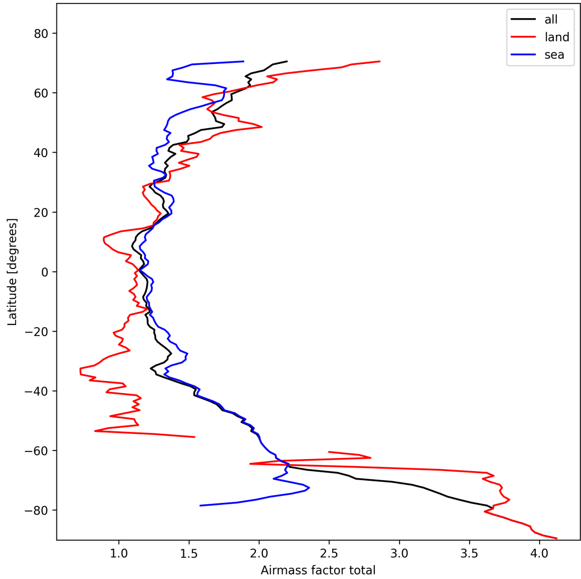
Figure 24: Zonal average of “Airmass factor total” for 2025-02-08 to 2025-02-09.
