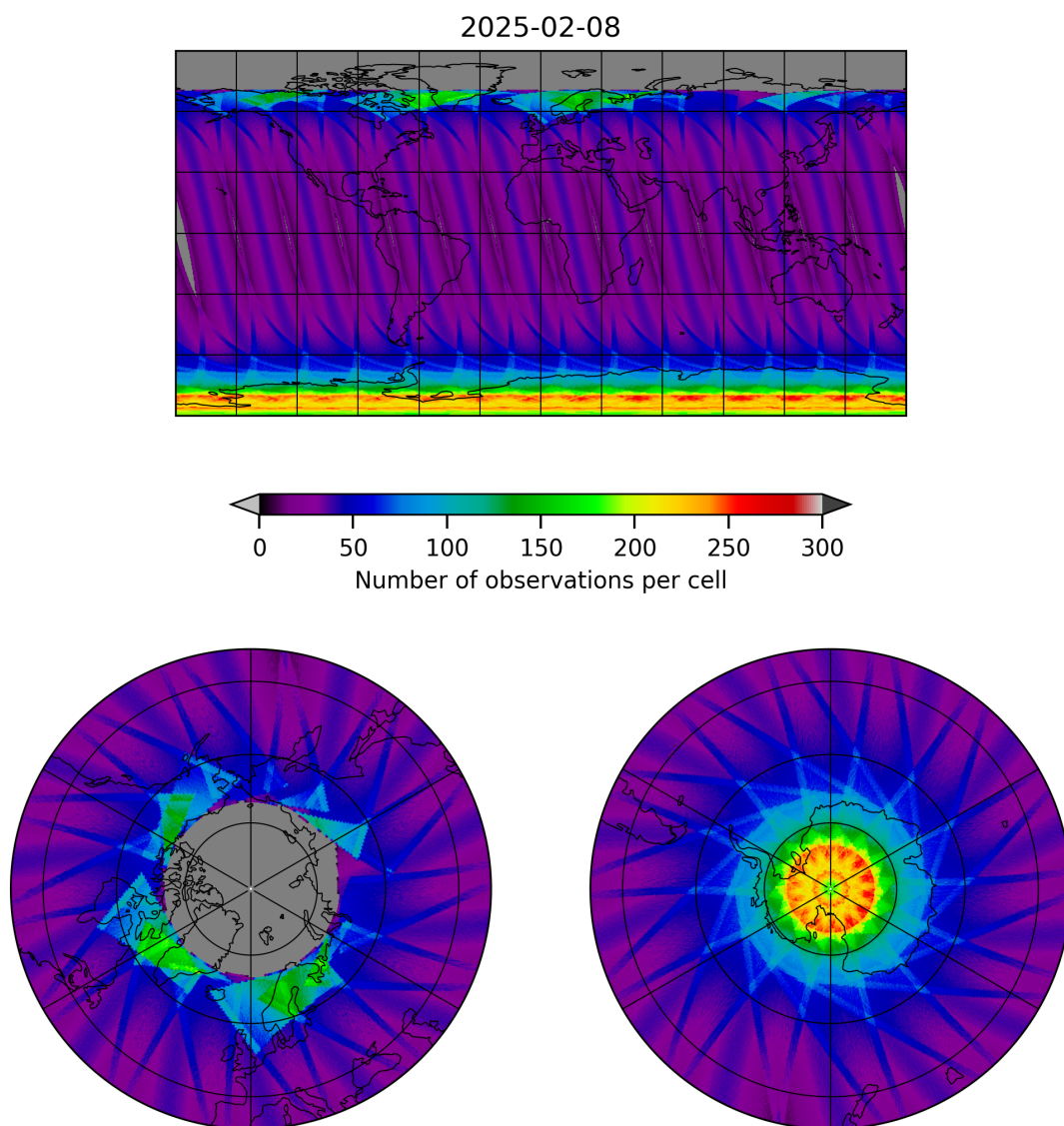
Figure 17: Map of the number of observations for 2025-02-08 to 2025-02-09
