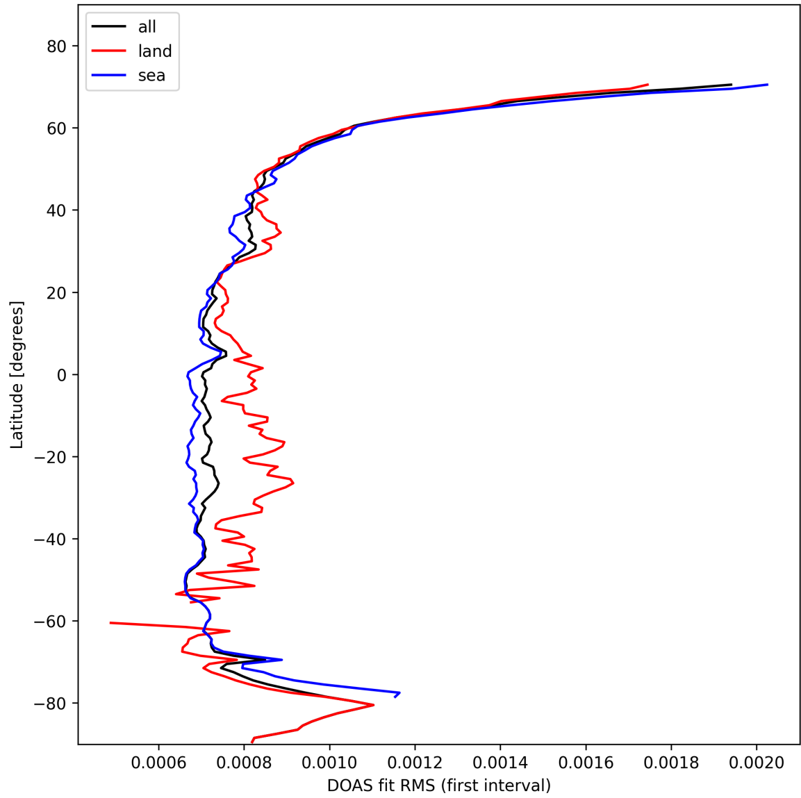
Figure 30: Zonal average of “DOAS fit RMS (first interval)” for 2025-02-08 to 2025-02-09.
