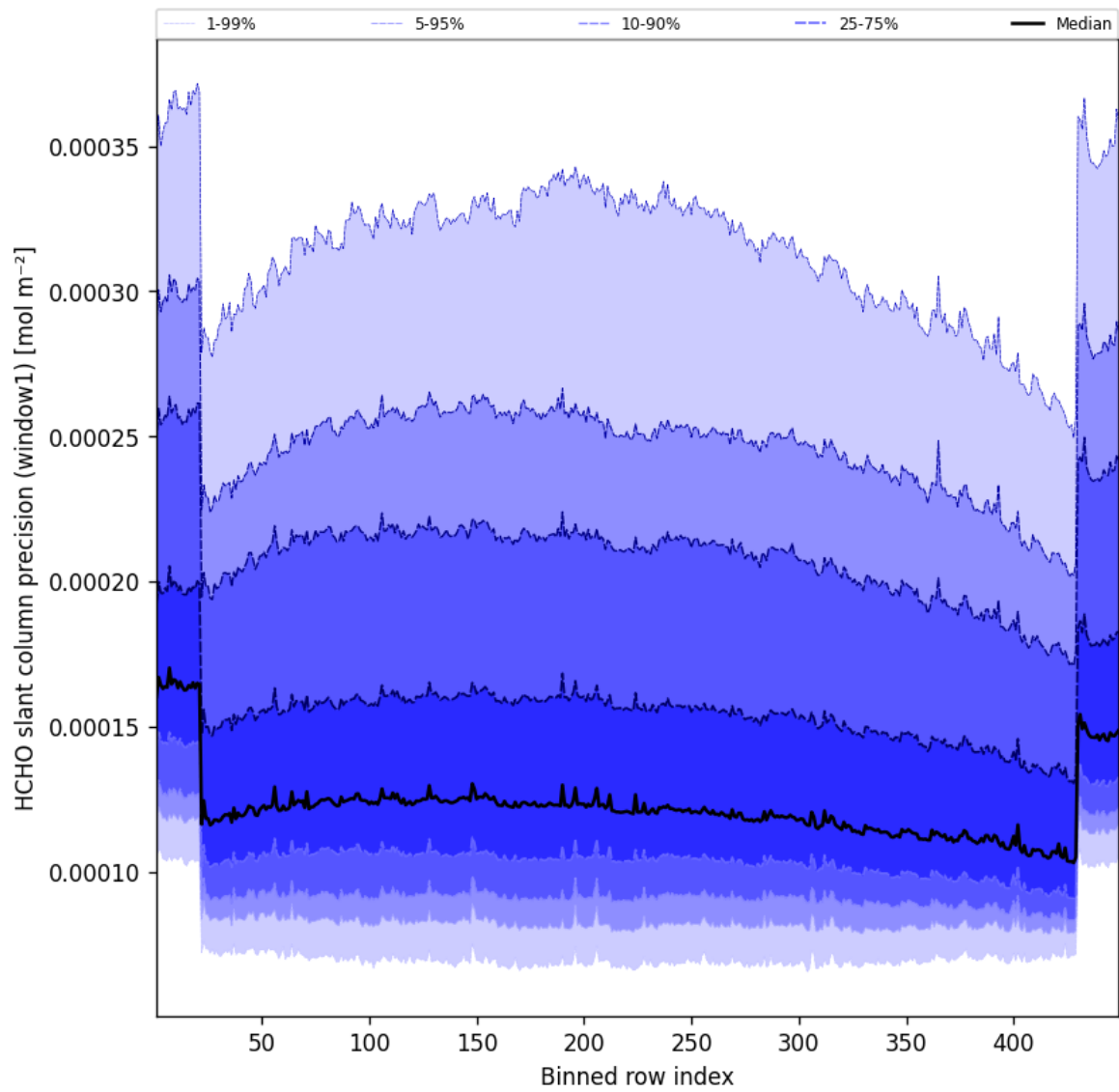
Figure 51: Along track statistics of “HCHO slant column precision (window1)” for 2025-02-08 to 2025-02-09
