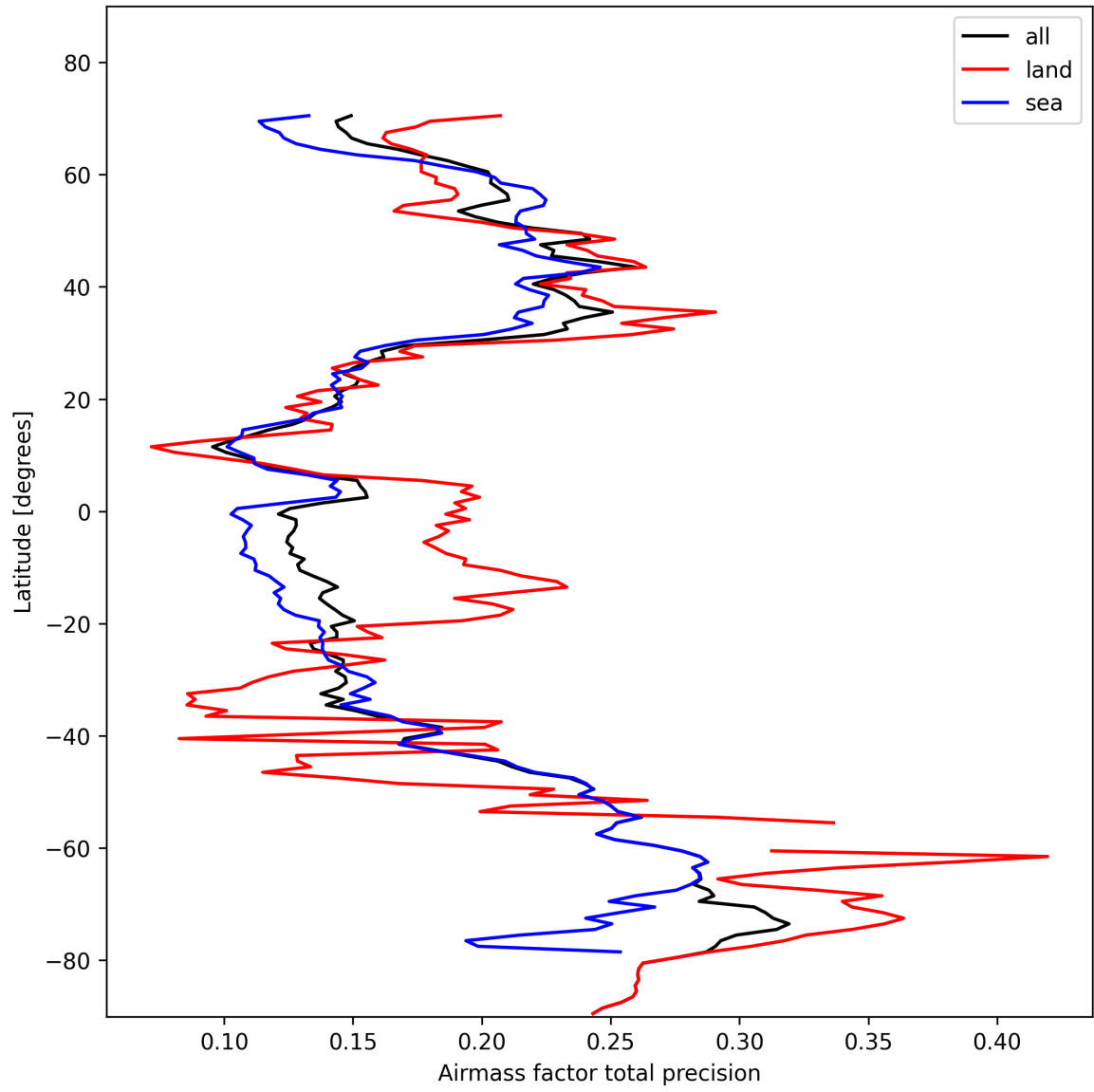
Figure 25: Zonal average of “Airmass factor total precision” for 2025-02-08 to 2025-02-09.
