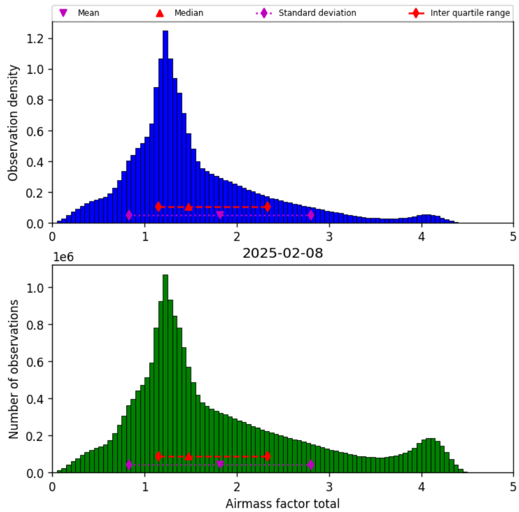
Figure 38: Histogram of “Airmass factor total” for 2025-02-08 to 2025-02-09
