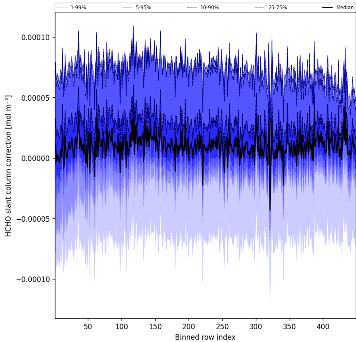
Figure 59: Along track statistics of “HCHO slant column correction” for 2025-02-08 to 2025-02-09
