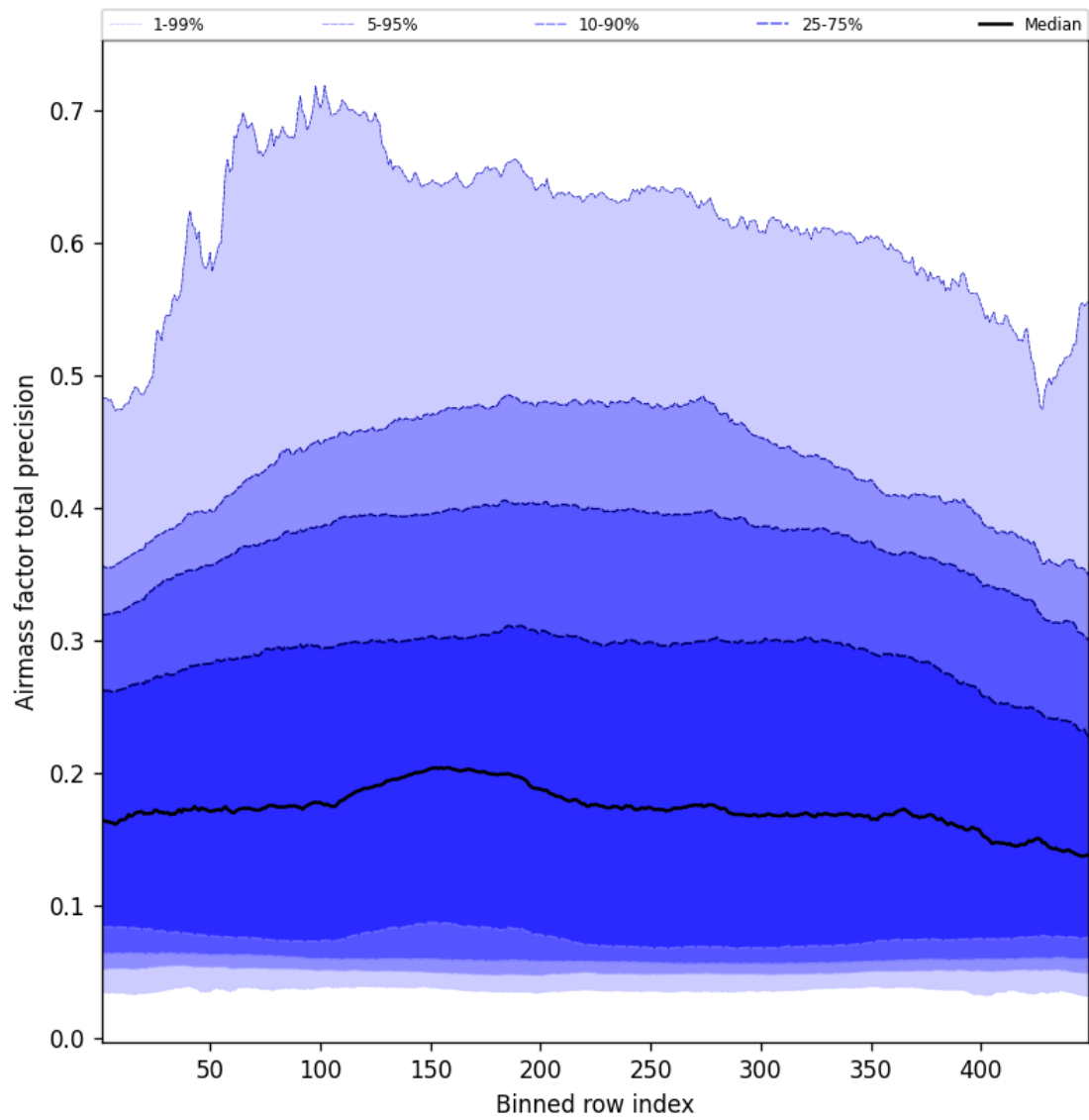
Figure 53: Along track statistics of “Airmass factor total precision” for 2025-02-08 to 2025-02-09
