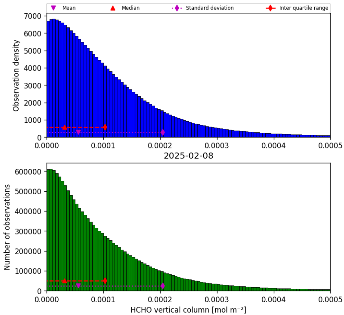
Figure 33: Histogram of “HCHO vertical column” for 2025-02-08 to 2025-02-09
