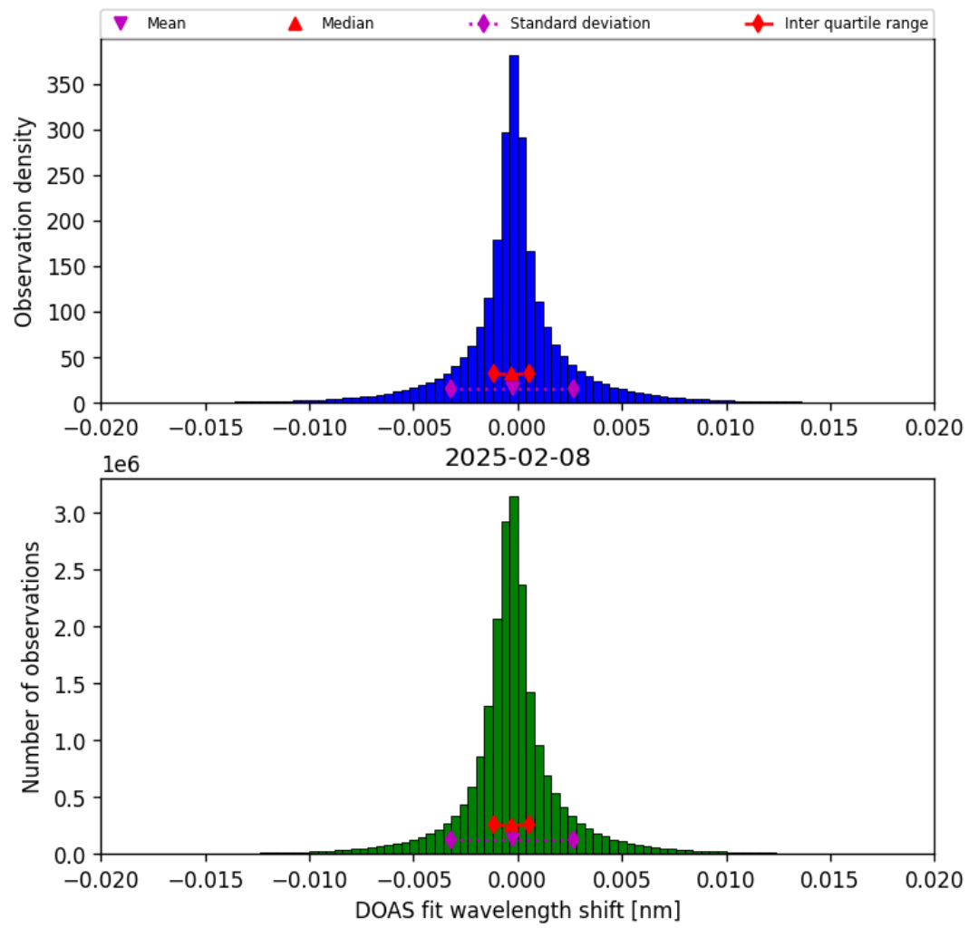
Figure 42: Histogram of “DOAS fit wavelength shift” for 2025-02-08 to 2025-02-09
