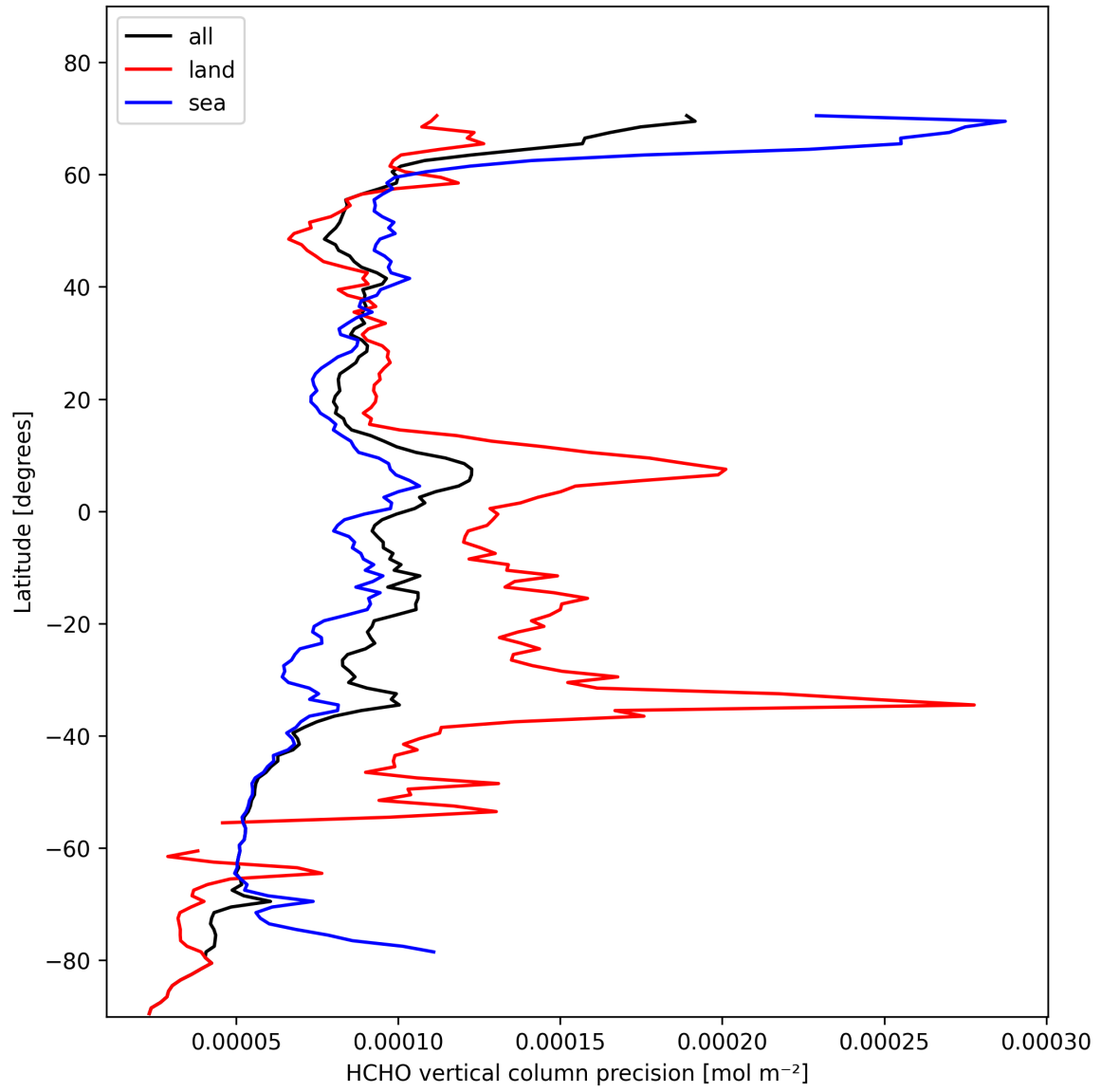
Figure 20: Zonal average of “HCHO vertical column precision” for 2025-02-08 to 2025-02-09.
