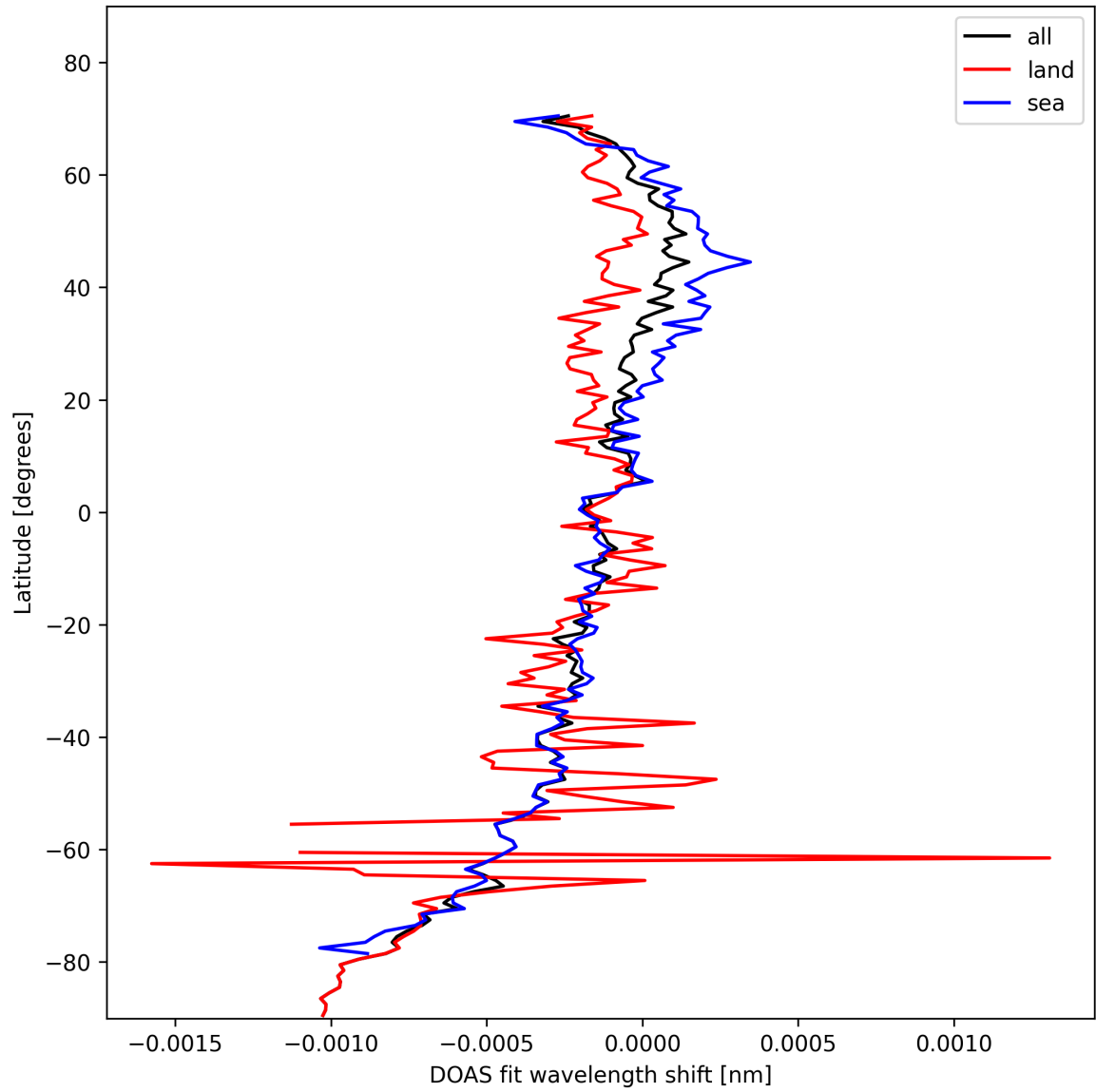
Figure 28: Zonal average of “DOAS fit wavelength shift” for 2025-02-08 to 2025-02-09.
