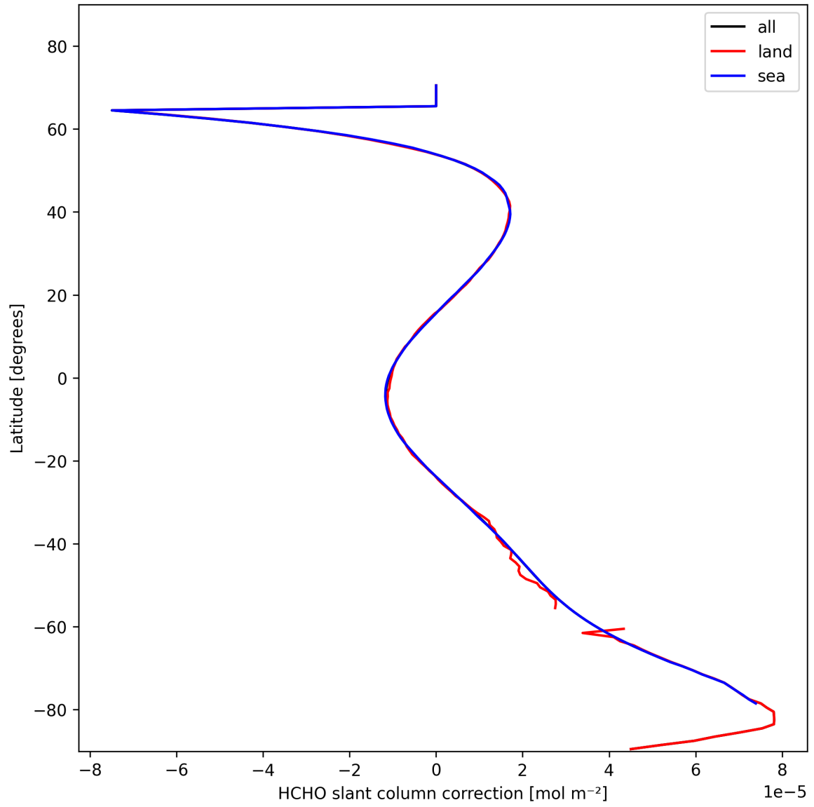
Figure 31: Zonal average of “HCHO slant column correction” for 2025-02-08 to 2025-02-09.
