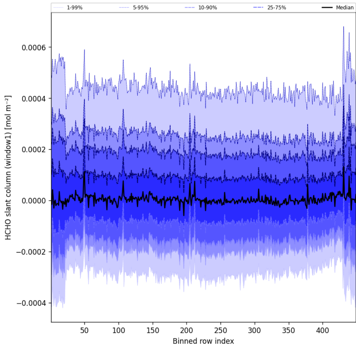
Figure 50: Along track statistics of “HCHO slant column (window1)” for 2025-02-08 to 2025-02-09
