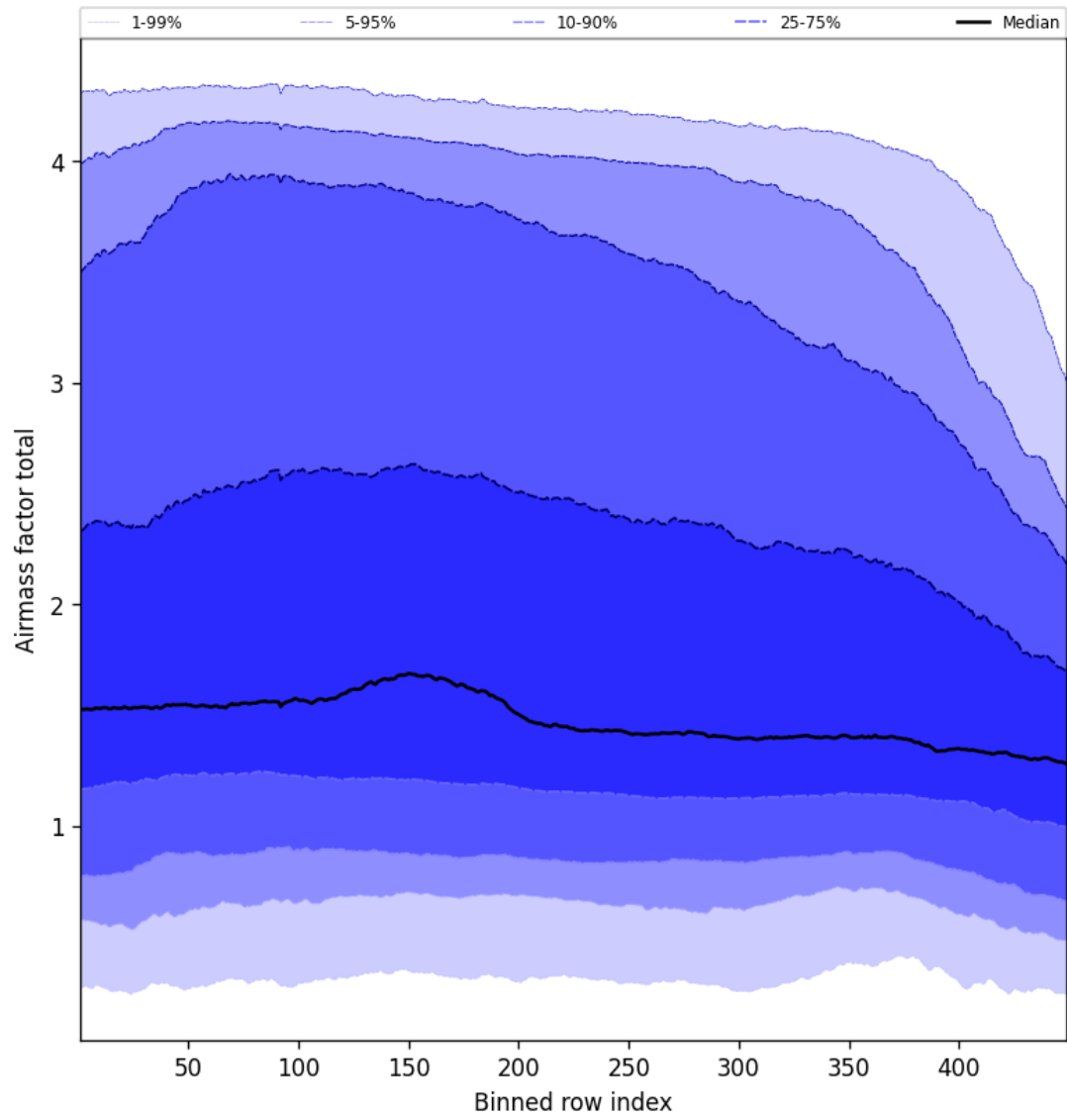
Figure 52: Along track statistics of “Airmass factor total” for 2025-02-08 to 2025-02-09
