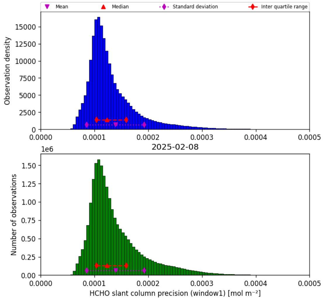
Figure 37: Histogram of “HCHO slant column precision (window1)” for 2025-02-08 to 2025-02-09
