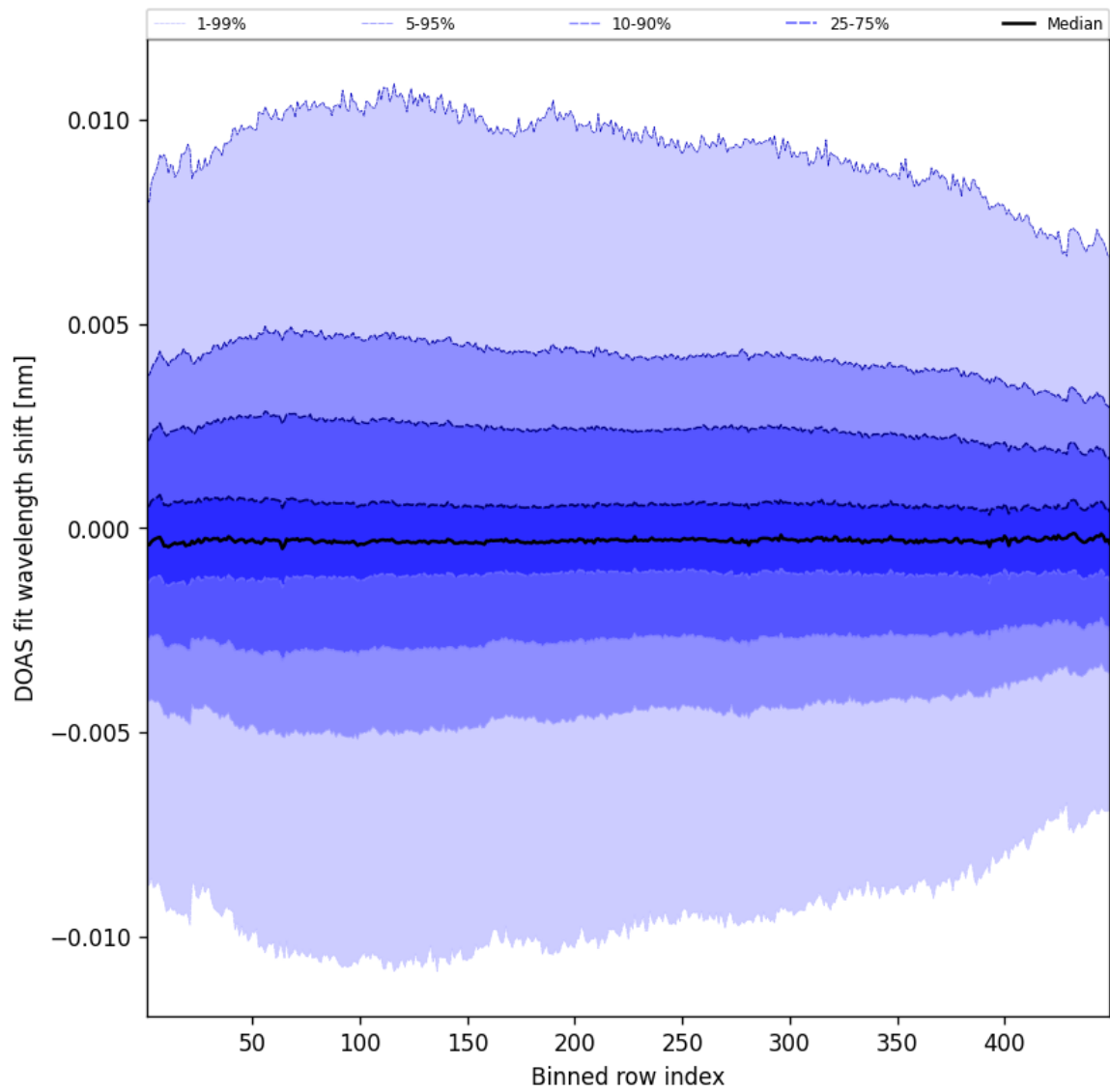
Figure 56: Along track statistics of “DOAS fit wavelength shift” for 2025-02-08 to 2025-02-09
