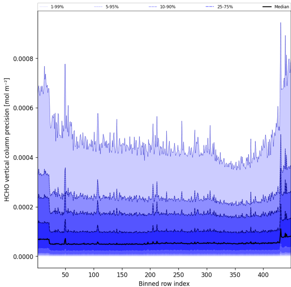
Figure 48: Along track statistics of “HCHO vertical column precision” for 2025-02-08 to 2025-02-09
