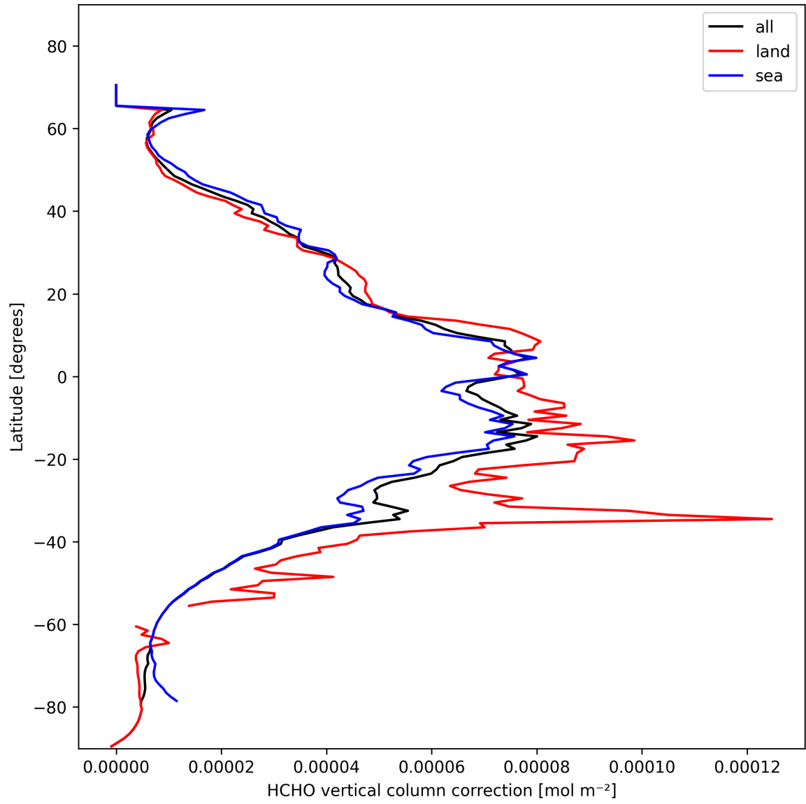
Figure 21: Zonal average of “HCHO vertical column correction” for 2025-02-08 to 2025-02-09.
