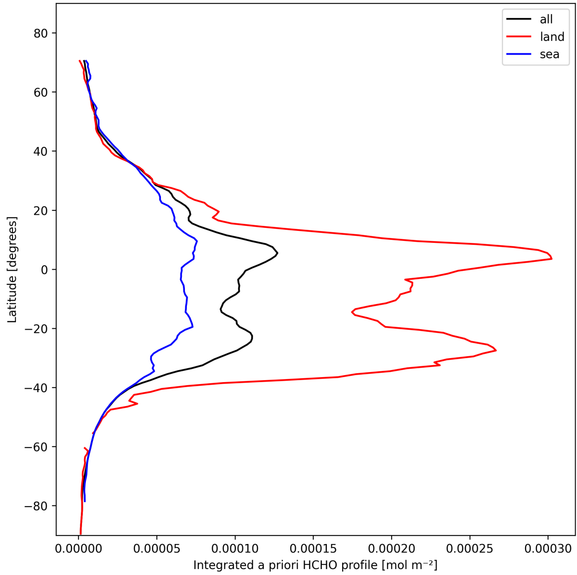
Figure 27: Zonal average of “Integrated a priori HCHO profile” for 2025-02-08 to 2025-02-09.
