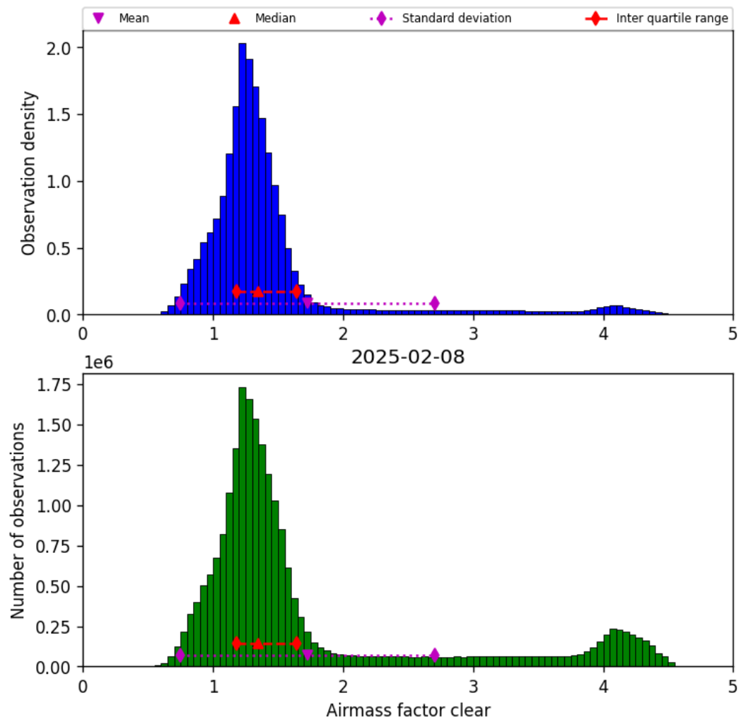
Figure 40: Histogram of “Airmass factor clear” for 2025-02-08 to 2025-02-09
