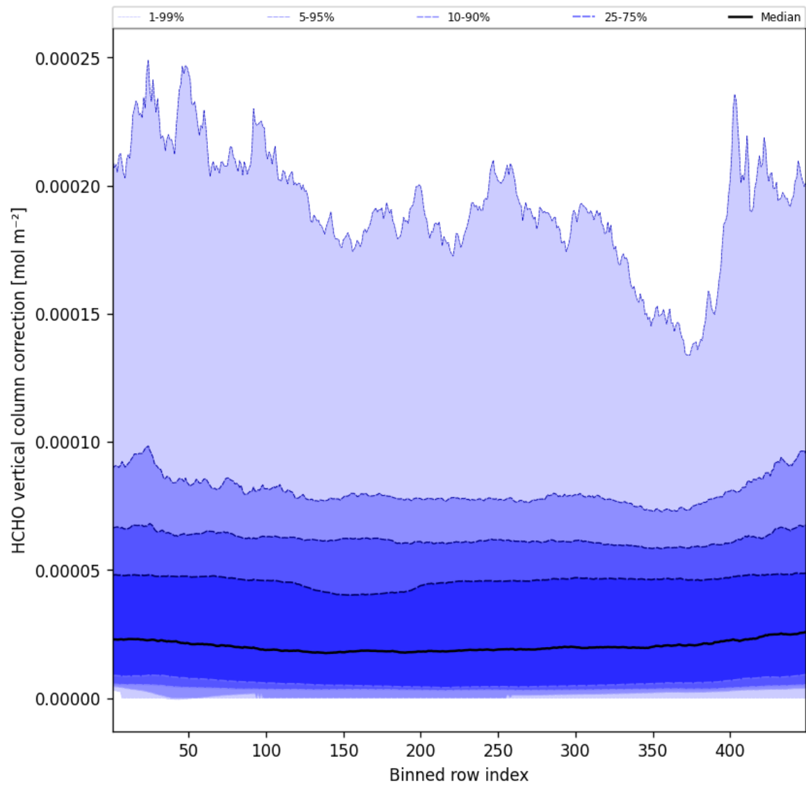
Figure 49: Along track statistics of “HCHO vertical column correction” for 2025-02-08 to 2025-02-09
