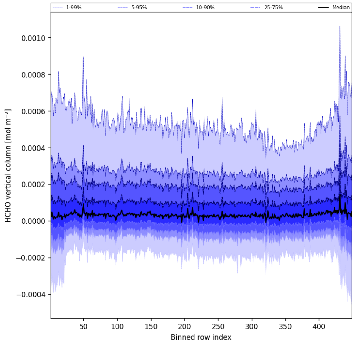
Figure 47: Along track statistics of “HCHO vertical column” for 2025-02-08 to 2025-02-09
