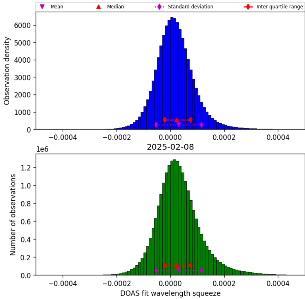
Figure 43: Histogram of “DOAS fit wavelength squeeze” for 2025-02-08 to 2025-02-09
