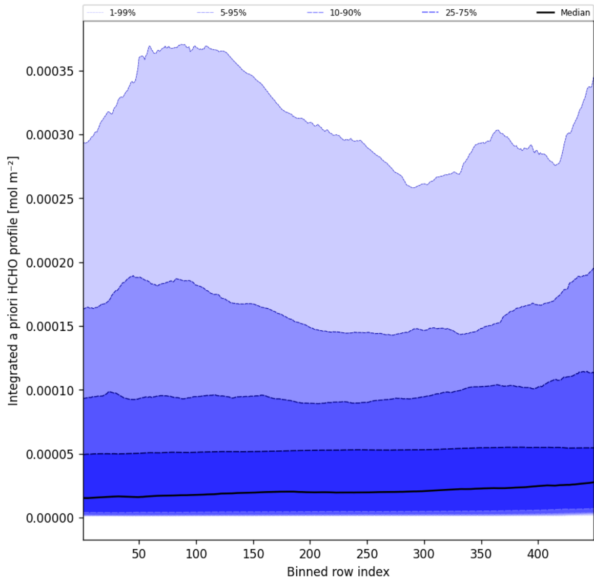
Figure 55: Along track statistics of "Integrated a priori HCHO profile" for 2025-02-09 to 2025-02-10
