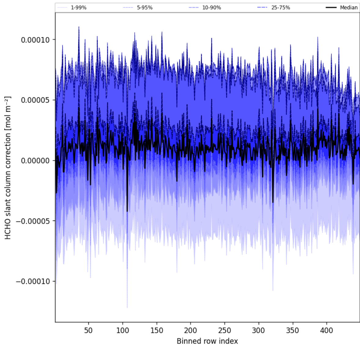
Figure 59: Along track statistics of “HCHO slant column correction” for 2025-02-09 to 2025-02-10
