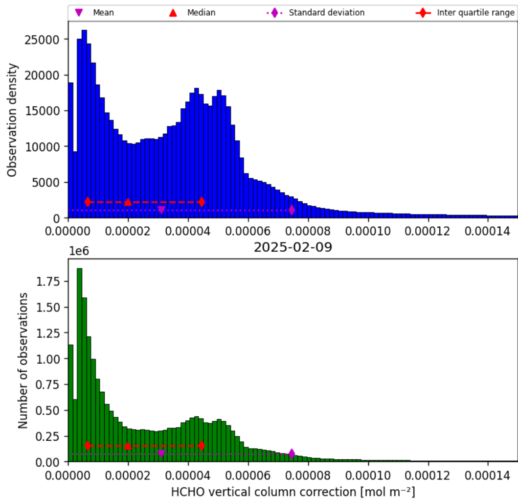
Figure 35: Histogram of “HCHO vertical column correction” for 2025-02-09 to 2025-02-10
