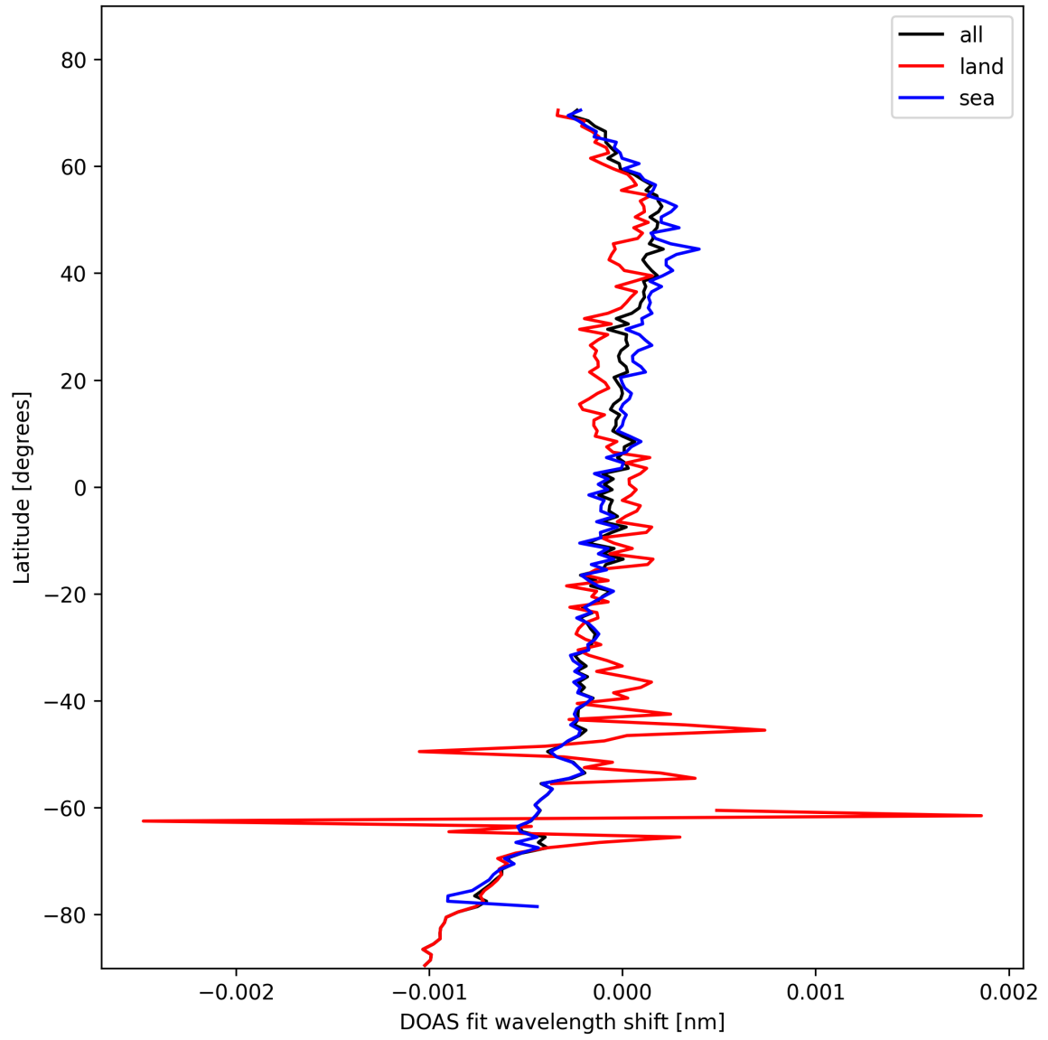
Figure 28: Zonal average of “DOAS fit wavelength shift” for 2025-02-09 to 2025-02-10.
