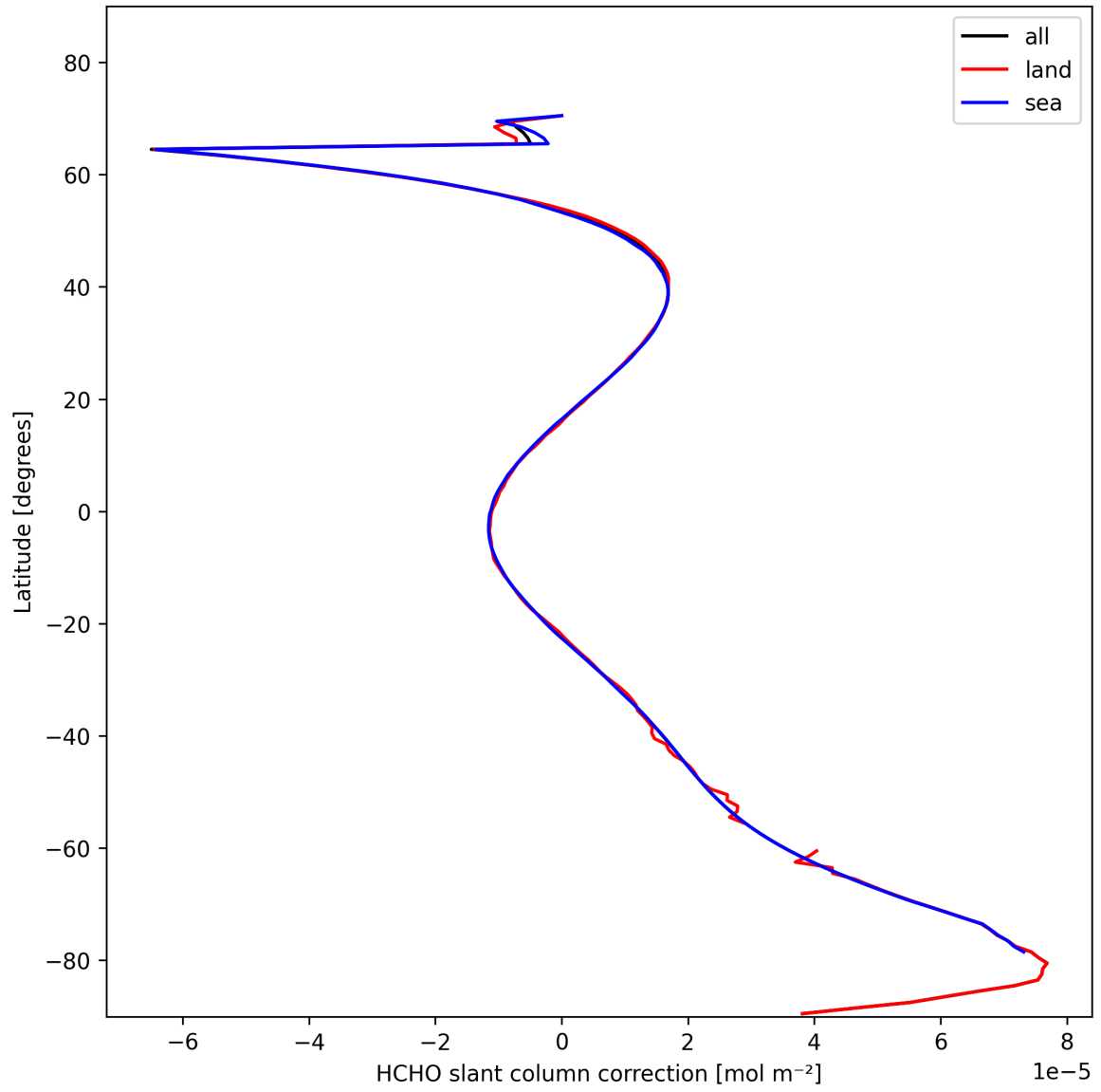
Figure 31: Zonal average of “HCHO slant column correction” for 2025-02-09 to 2025-02-10.
