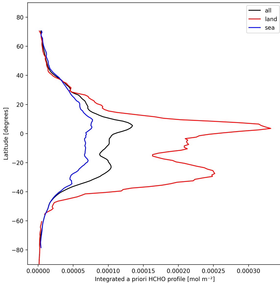
Figure 27: Zonal average of “Integrated a priori HCHO profile” for 2025-02-09 to 2025-02-10.
