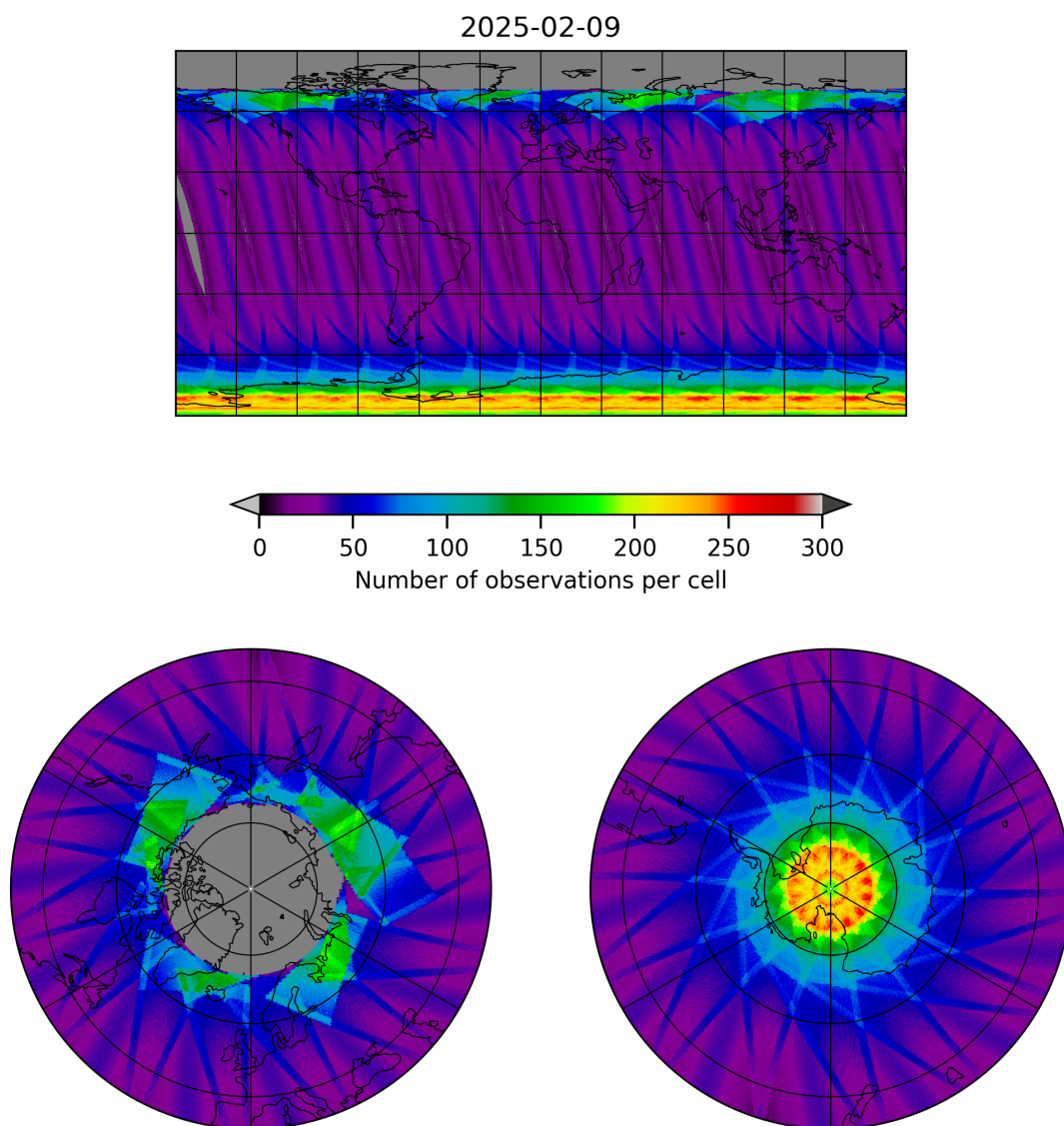
Figure 17: Map of the number of observations for 2025-02-09 to 2025-02-10
