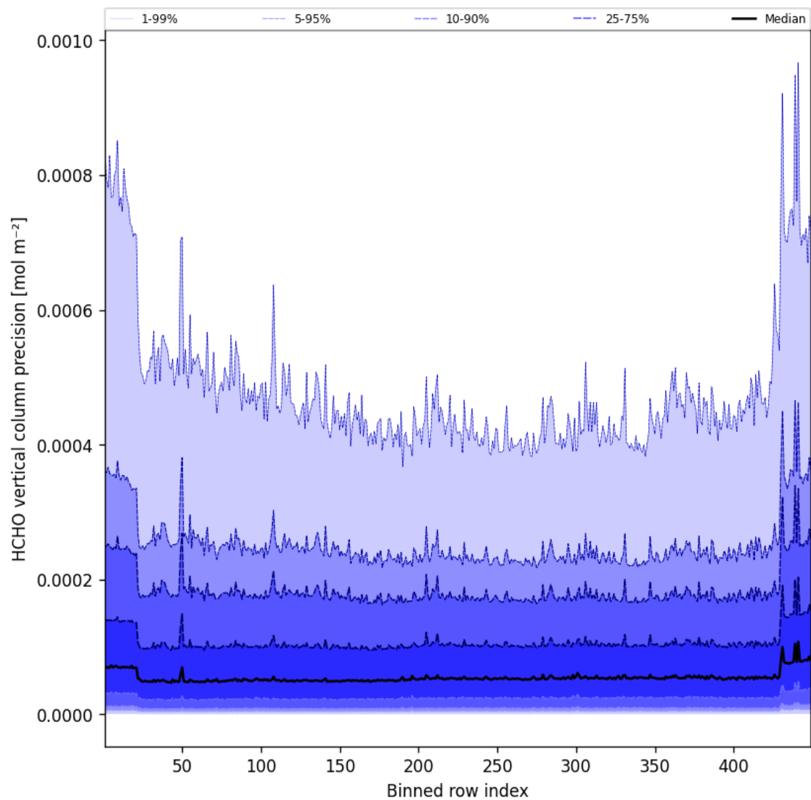
Figure 48: Along track statistics of “HCHO vertical column precision” for 2025-02-09 to 2025-02-10
