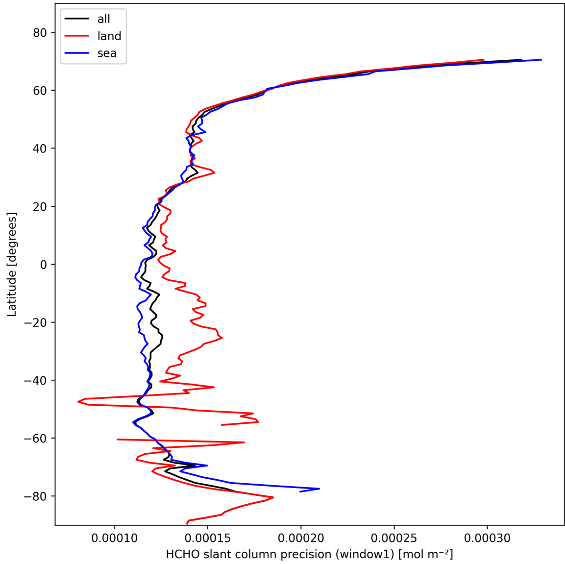
Figure 23: Zonal average of “HCHO slant column precision (window1)” for 2025-02-09 to 2025-02-10.
