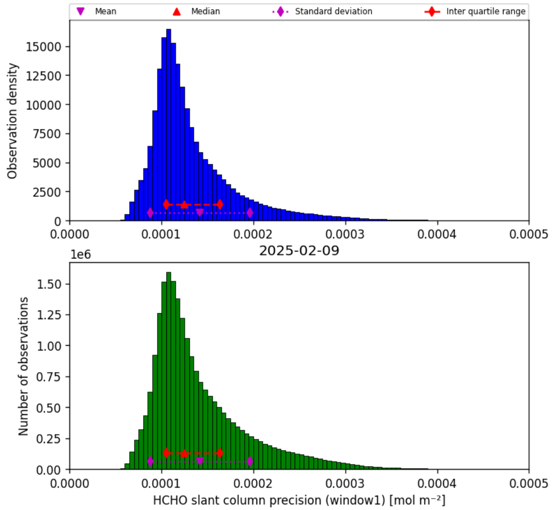
Figure 37: Histogram of “HCHO slant column precision (window1)” for 2025-02-09 to 2025-02-10
