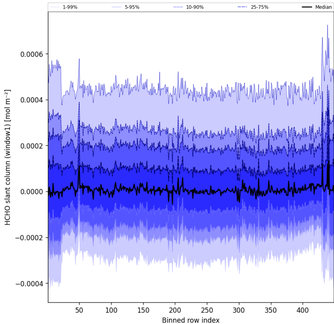
Figure 50: Along track statistics of “HCHO slant column (window1)” for 2025-02-09 to 2025-02-10
