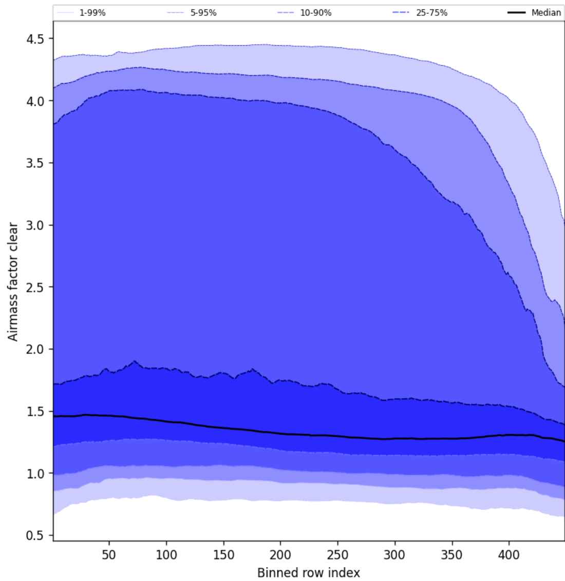
Figure 54: Along track statistics of “Airmass factor clear” for 2025-02-09 to 2025-02-10
