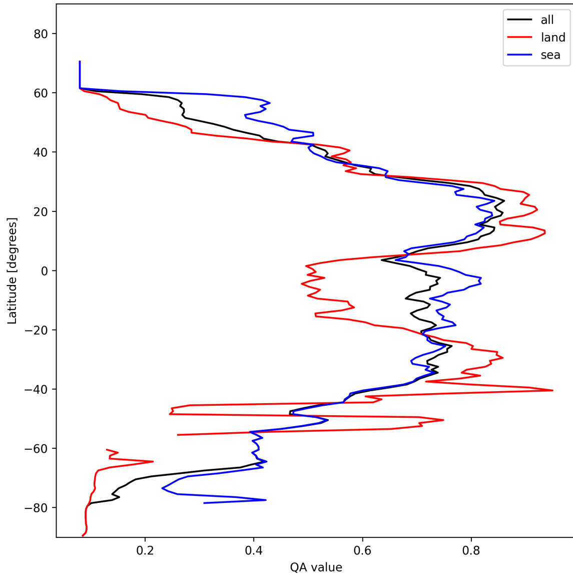
Figure 18: Zonal average of “QA value” for 2025-02-09 to 2025-02-10.
