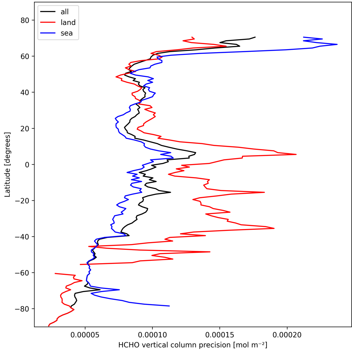
Figure 20: Zonal average of “HCHO vertical column precision” for 2025-02-09 to 2025-02-10.
