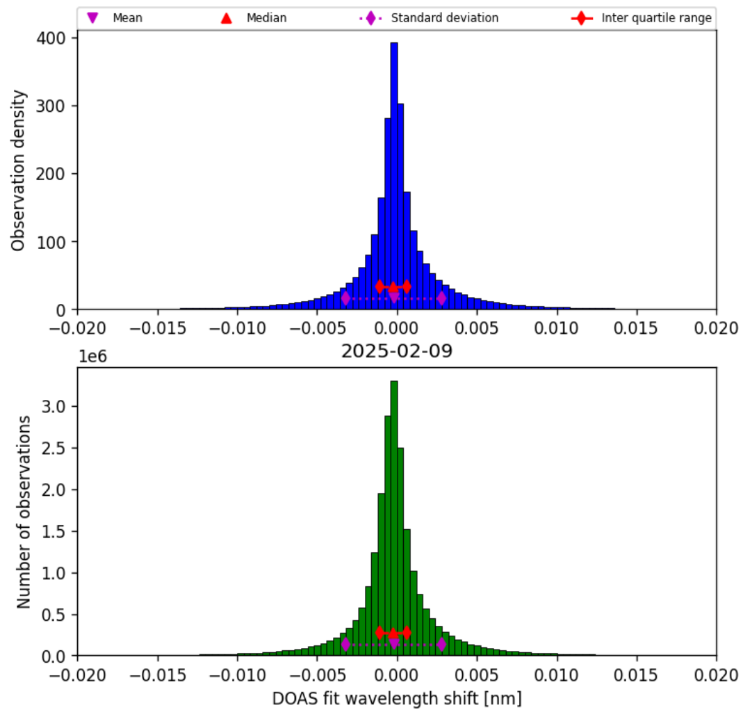
Figure 42: Histogram of “DOAS fit wavelength shift” for 2025-02-09 to 2025-02-10
