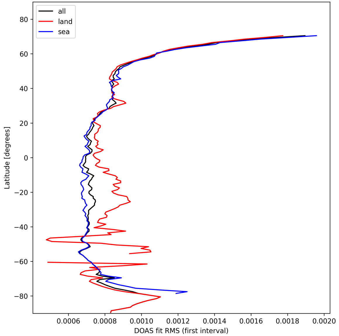
Figure 30: Zonal average of “DOAS fit RMS (first interval)” for 2025-02-09 to 2025-02-10.
