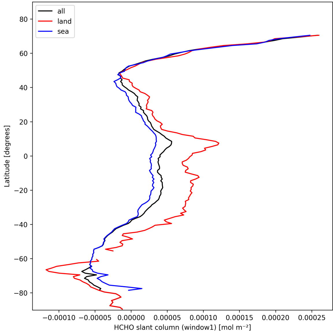
Figure 22: Zonal average of “HCHO slant column (window1)” for 2025-02-09 to 2025-02-10.
