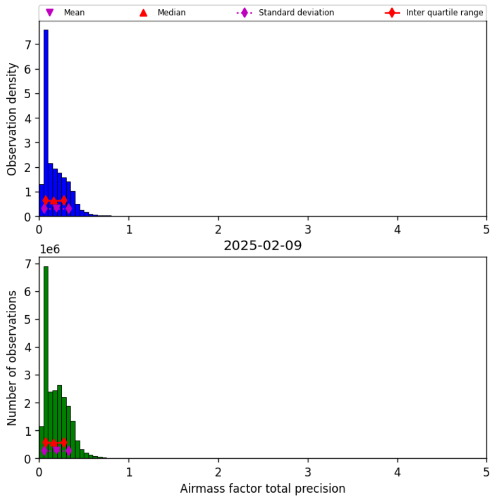
Figure 39: Histogram of “Airmass factor total precision” for 2025-02-09 to 2025-02-10
