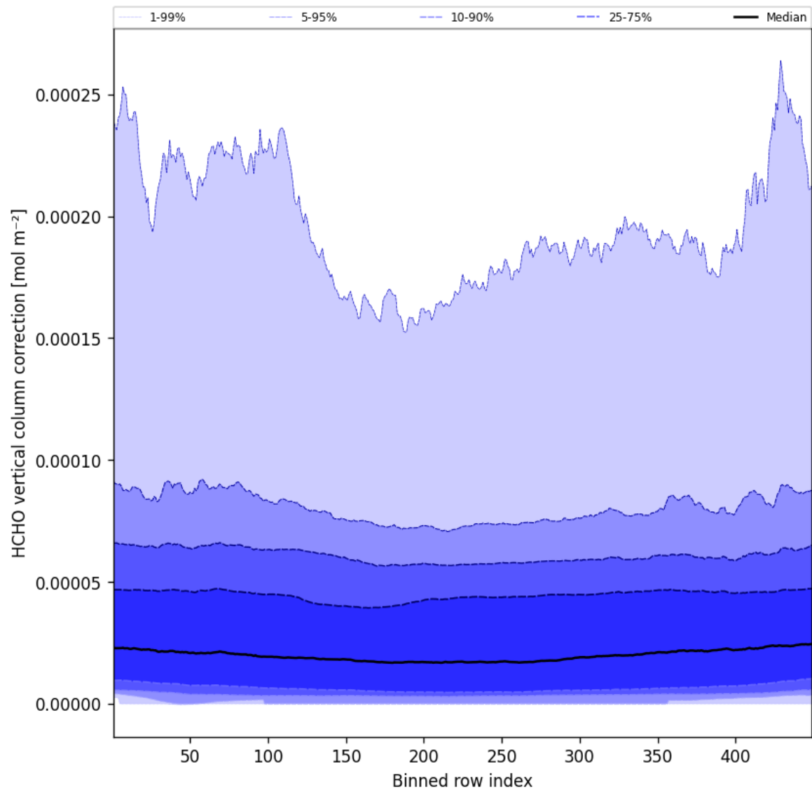
Figure 49: Along track statistics of “HCHO vertical column correction” for 2025-02-09 to 2025-02-10
