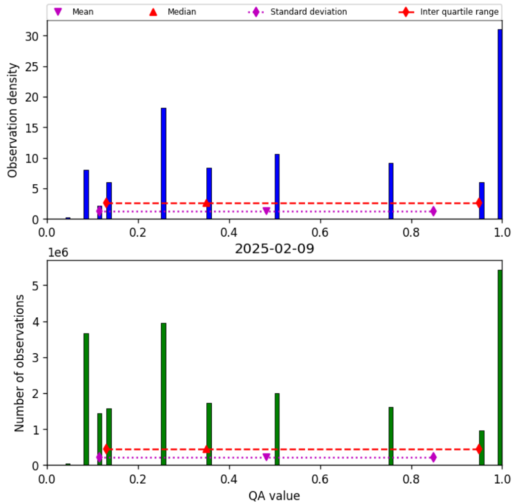
Figure 32: Histogram of “QA value” for 2025-02-09 to 2025-02-10
