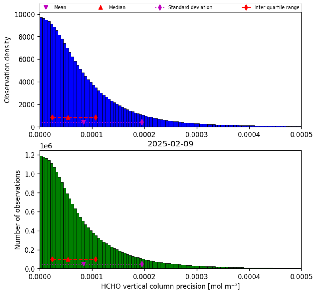
Figure 34: Histogram of "HCHO vertical column precision" for 2025-02-09 to 2025-02-10
