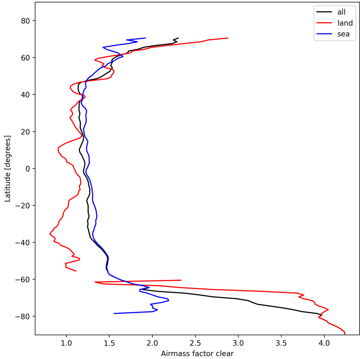
Figure 26: Zonal average of “Airmass factor clear” for 2025-02-09 to 2025-02-10.
