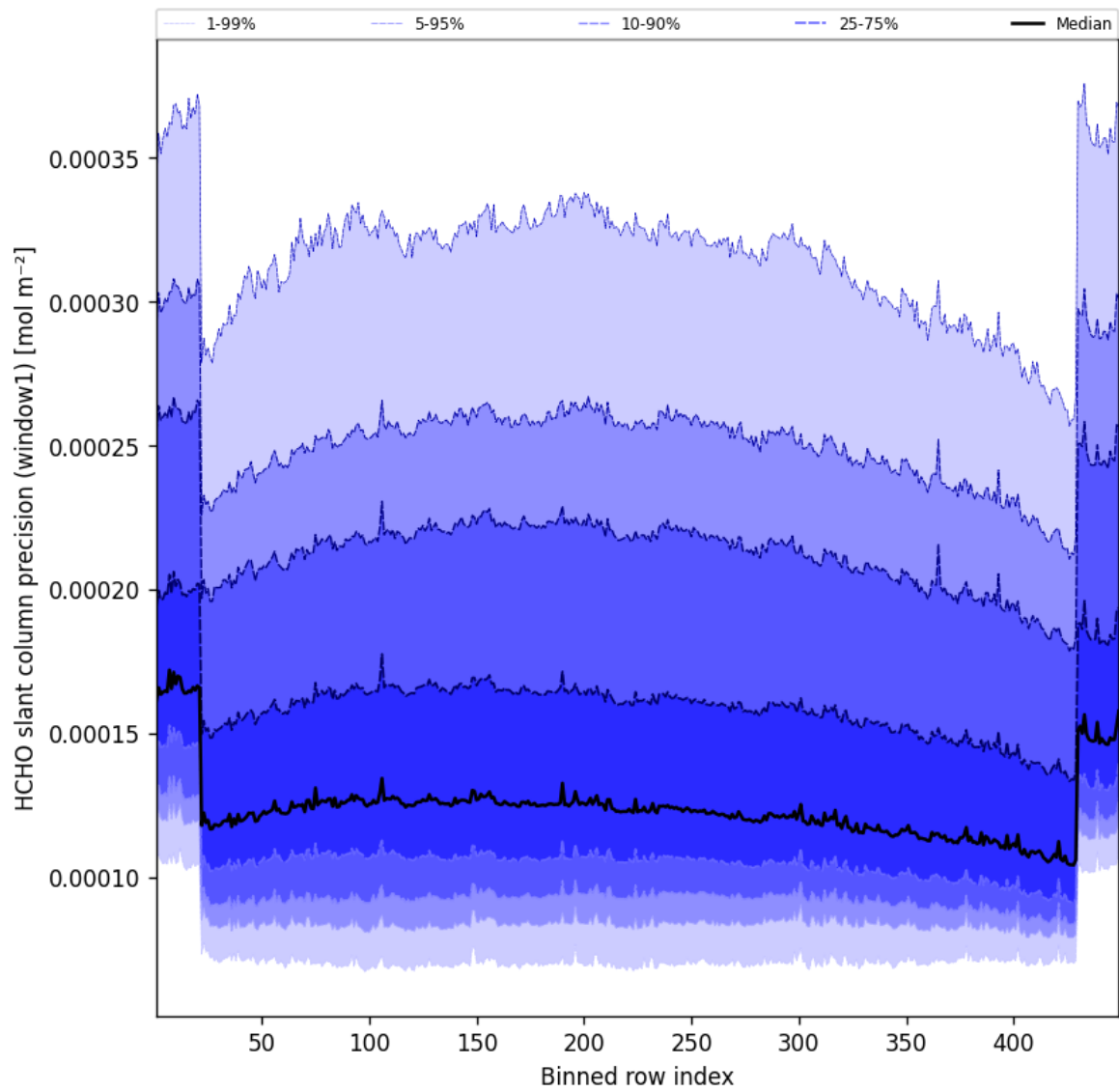
Figure 51: Along track statistics of “HCHO slant column precision (window1)” for 2025-02-09 to 2025-02-10
