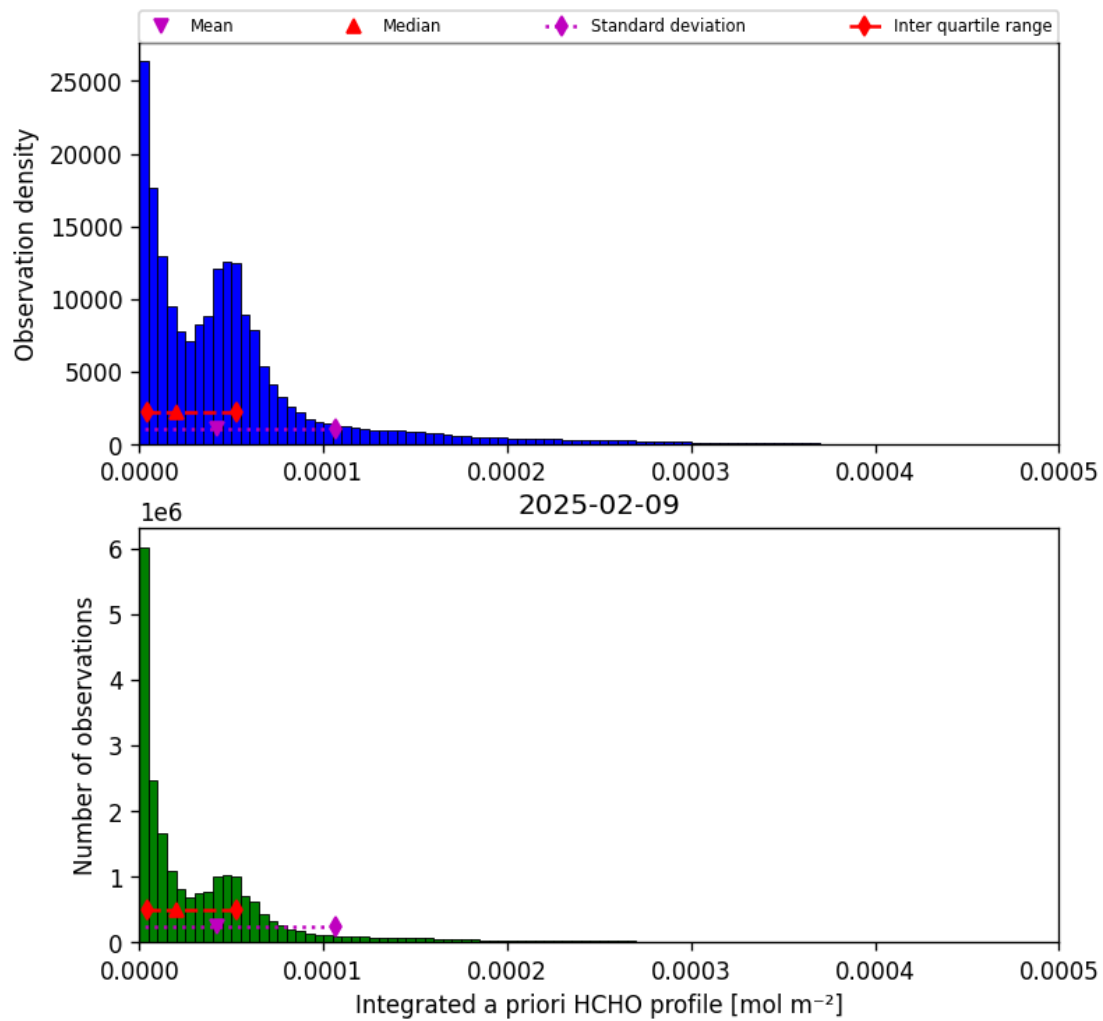
Figure 41: Histogram of “Integrated a priori HCHO profile” for 2025-02-09 to 2025-02-10
