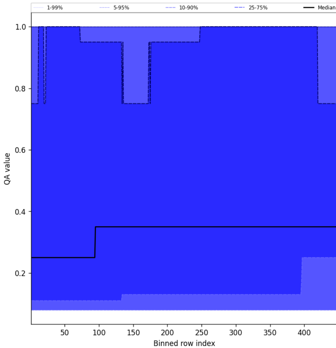
Figure 46: Along track statistics of “QA value” for 2025-02-09 to 2025-02-10
