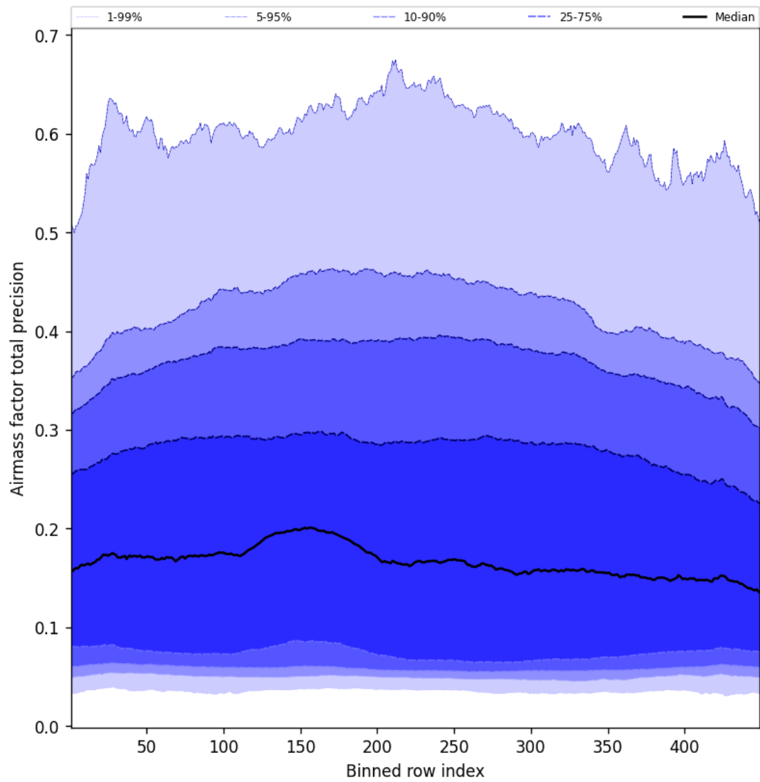
Figure 53: Along track statistics of “Airmass factor total precision” for 2025-02-09 to 2025-02-10
