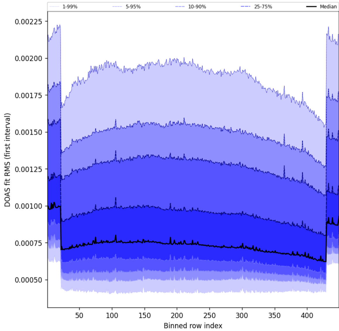
Figure 58: Along track statistics of “DOAS fit RMS (first interval)” for 2025-02-09 to 2025-02-10
