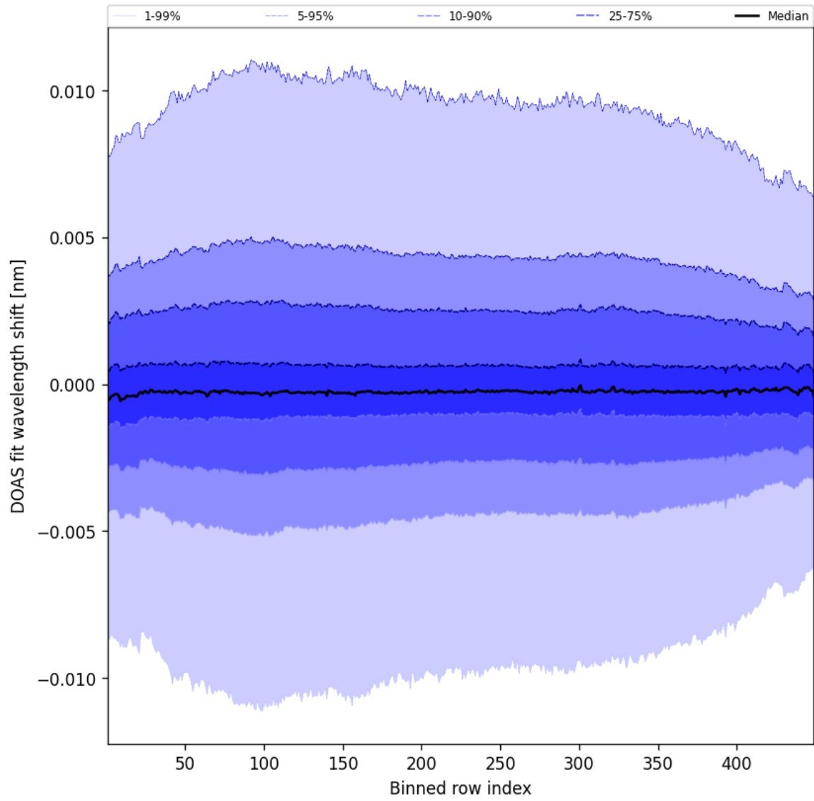
Figure 56: Along track statistics of “DOAS fit wavelength shift” for 2025-02-09 to 2025-02-10
