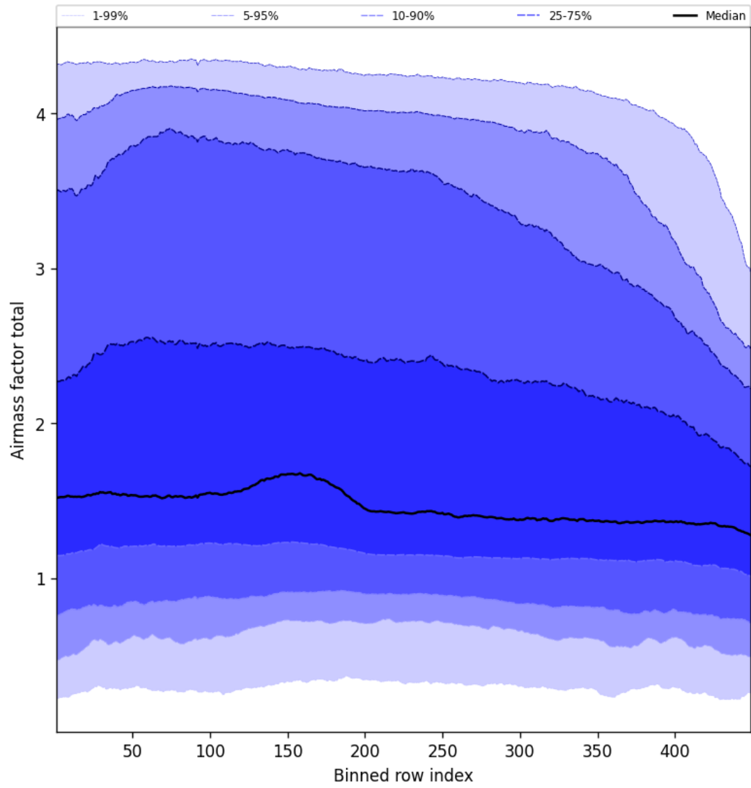
Figure 52: Along track statistics of “Airmass factor total” for 2025-02-09 to 2025-02-10
