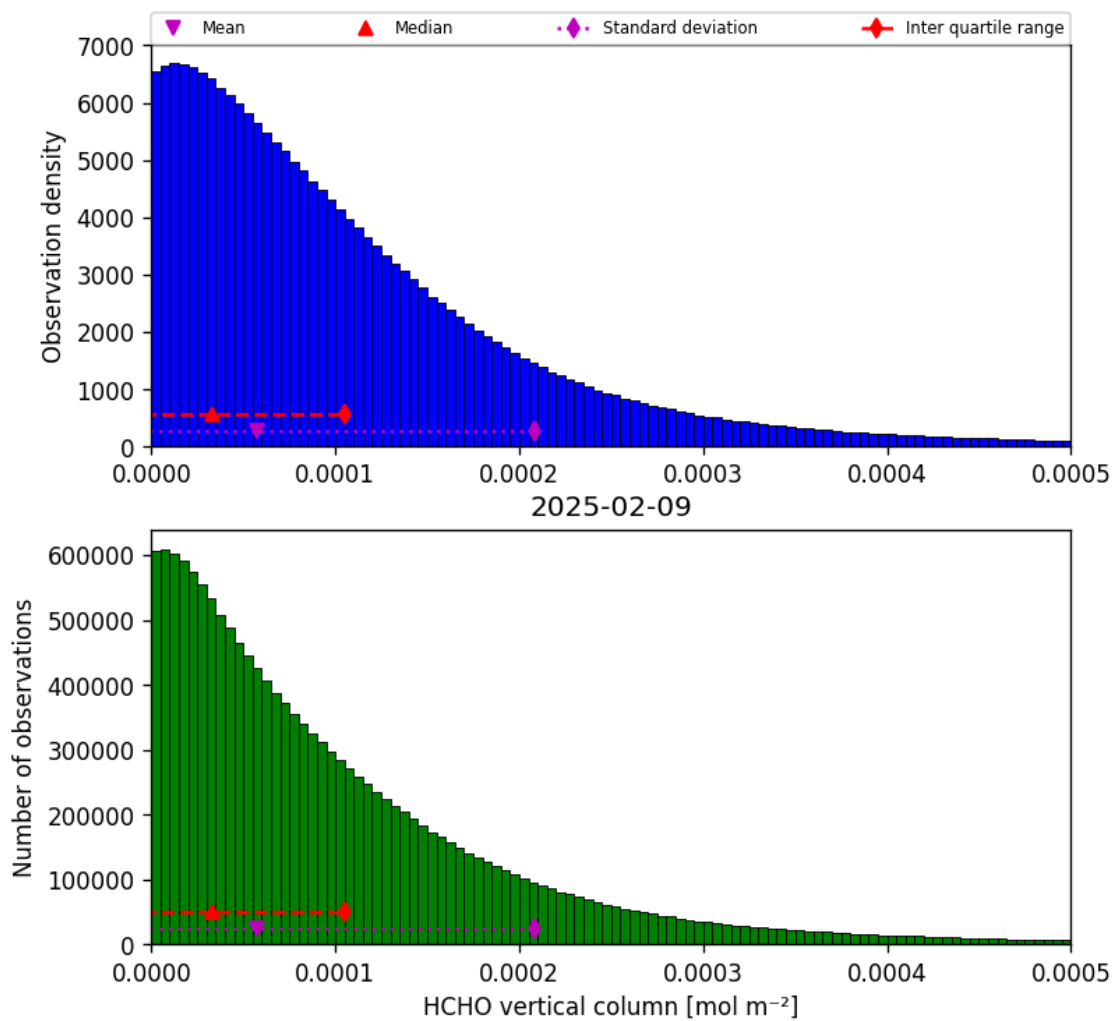
Figure 33: Histogram of “HCHO vertical column” for 2025-02-09 to 2025-02-10
