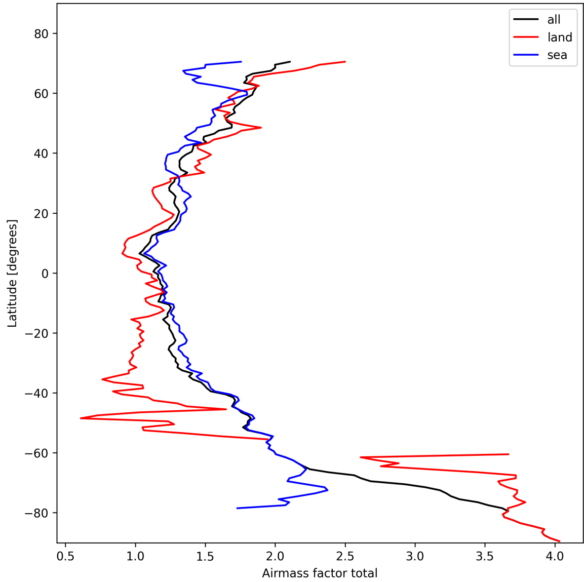
Figure 24: Zonal average of “Airmass factor total” for 2025-02-09 to 2025-02-10.
