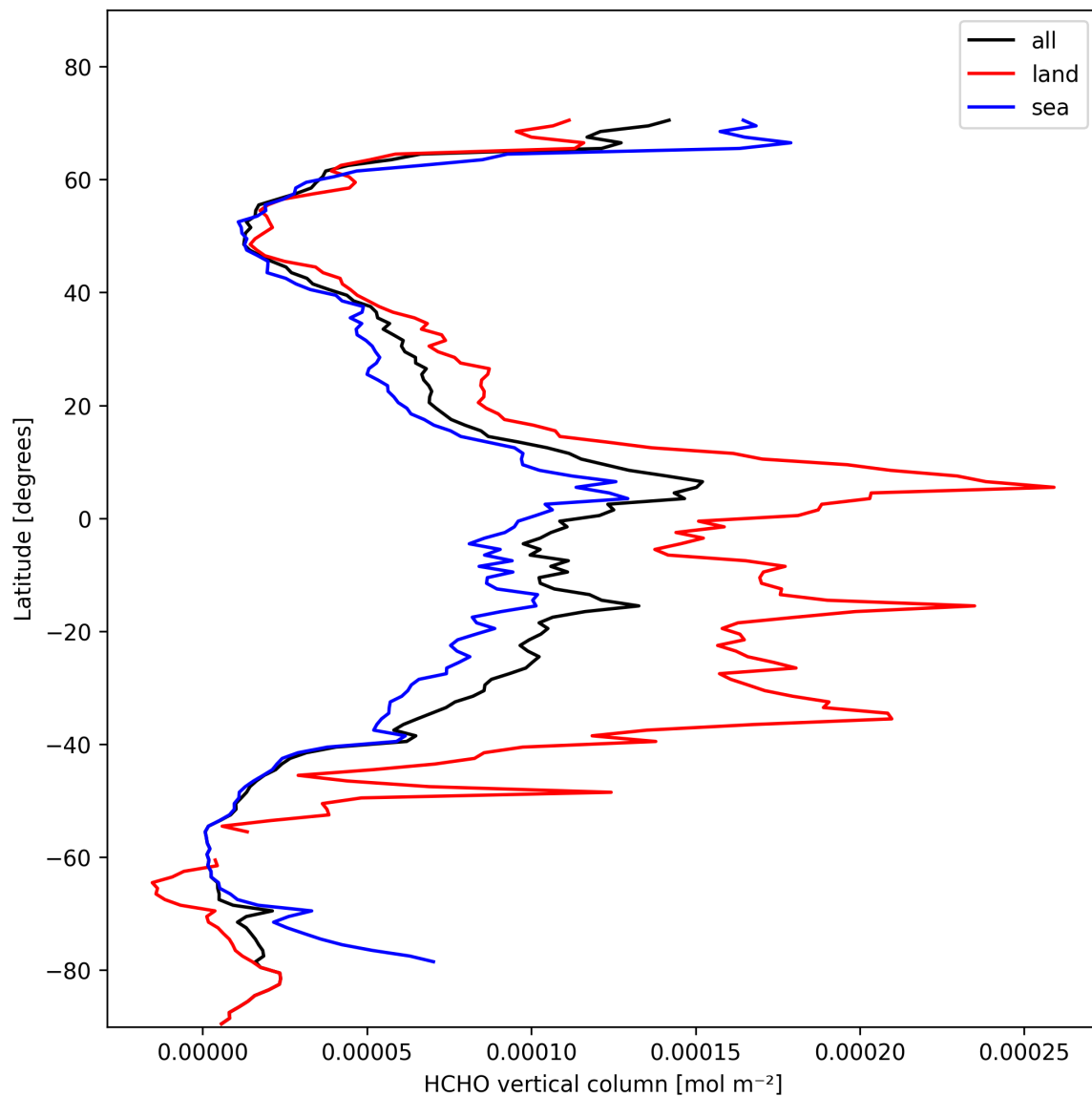
Figure 19: Zonal average of “HCHO vertical column” for 2025-02-09 to 2025-02-10.
