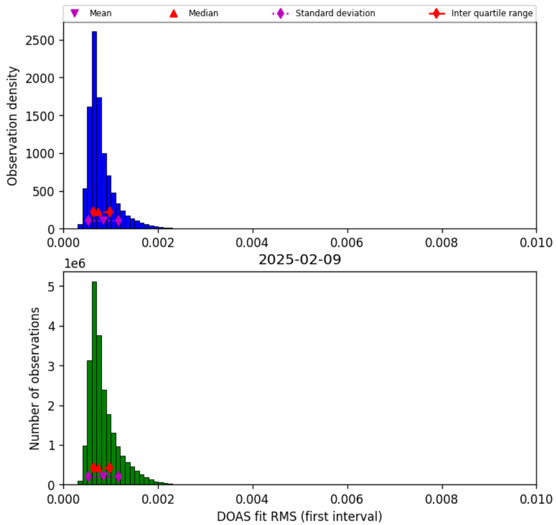
Figure 44: Histogram of “DOAS fit RMS (first interval)” for 2025-02-09 to 2025-02-10
