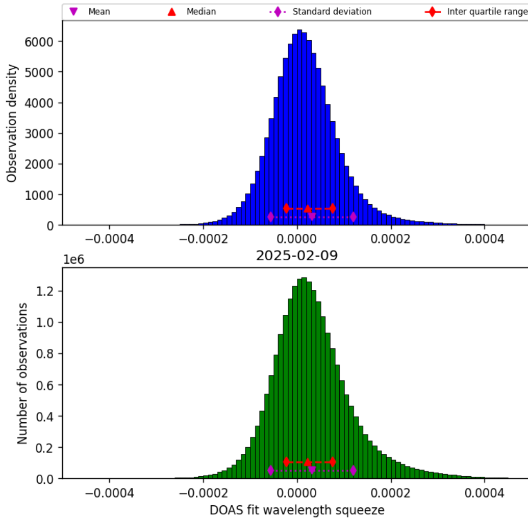
Figure 43: Histogram of “DOAS fit wavelength squeeze” for 2025-02-09 to 2025-02-10
