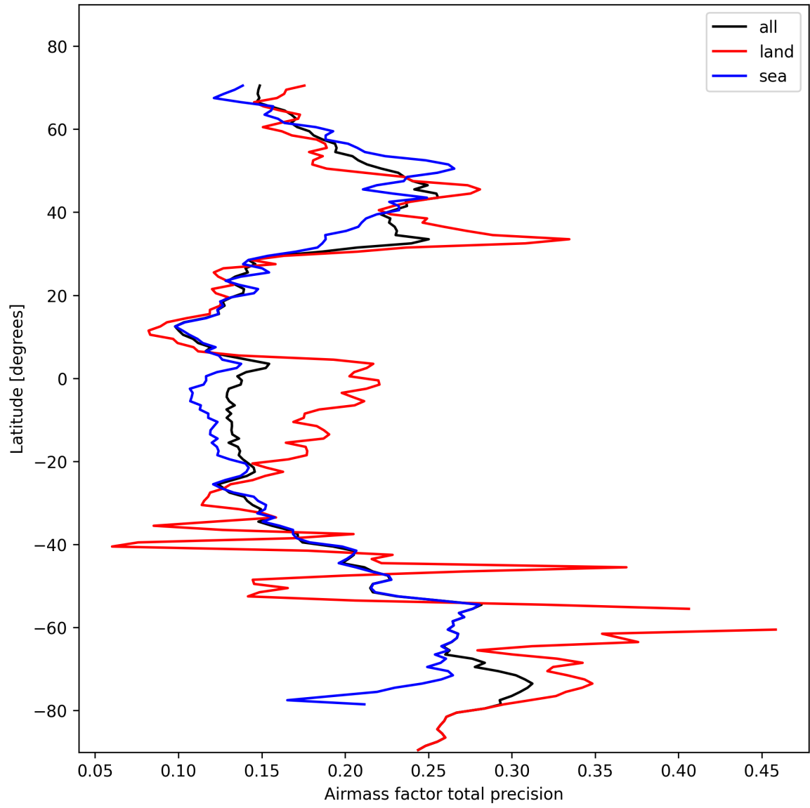
Figure 25: Zonal average of “Airmass factor total precision” for 2025-02-09 to 2025-02-10.
