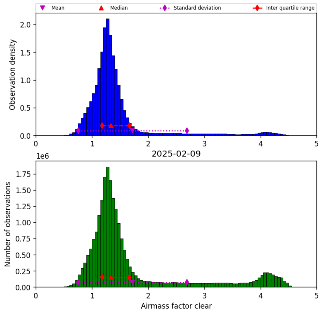
Figure 40: Histogram of “Airmass factor clear” for 2025-02-09 to 2025-02-10
