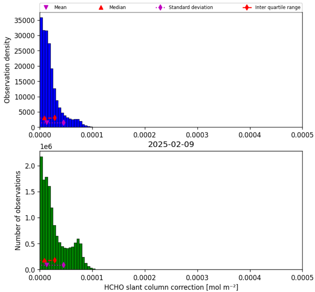
Figure 45: Histogram of “HCHO slant column correction” for 2025-02-09 to 2025-02-10
