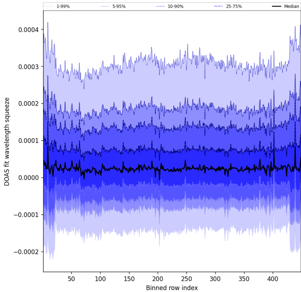
Figure 57: Along track statistics of “DOAS fit wavelength squeeze” for 2025-02-09 to 2025-02-10
