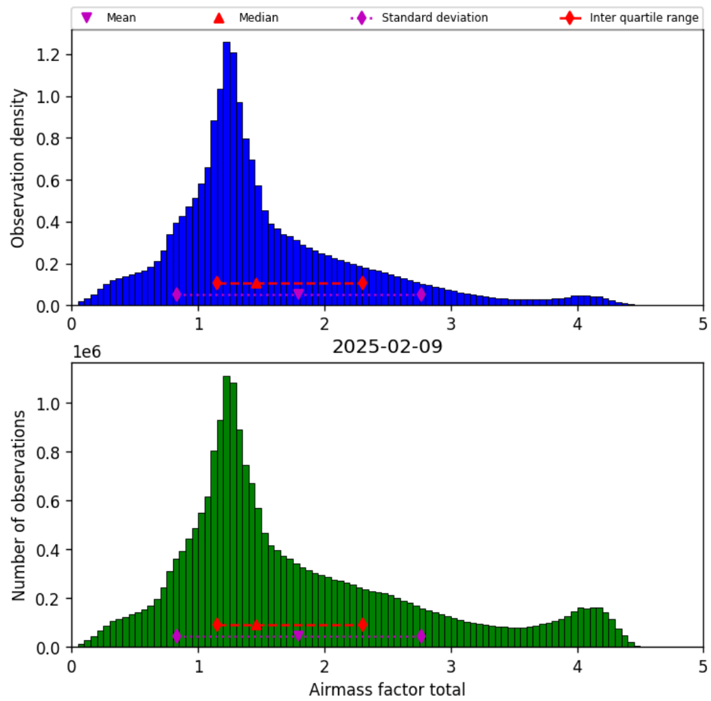
Figure 38: Histogram of “Airmass factor total” for 2025-02-09 to 2025-02-10
