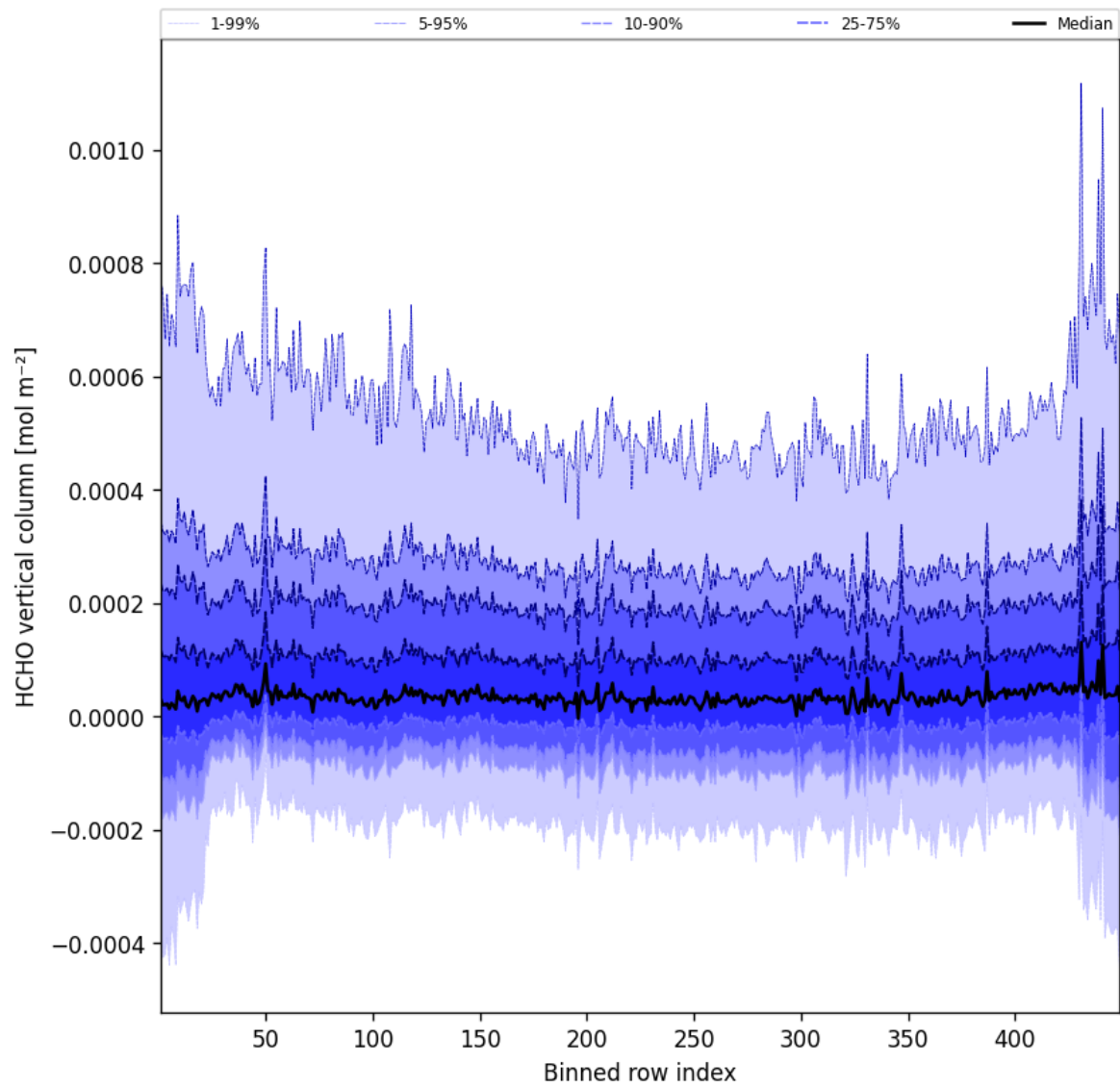
Figure 47: Along track statistics of “HCHO vertical column” for 2025-02-09 to 2025-02-10
