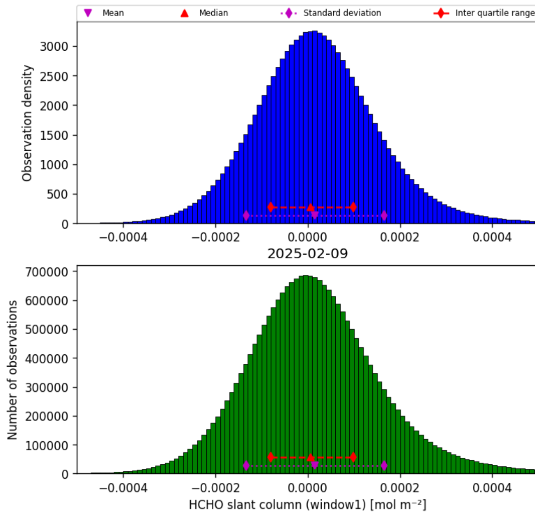
Figure 36: Histogram of “HCHO slant column (window1)” for 2025-02-09 to 2025-02-10
