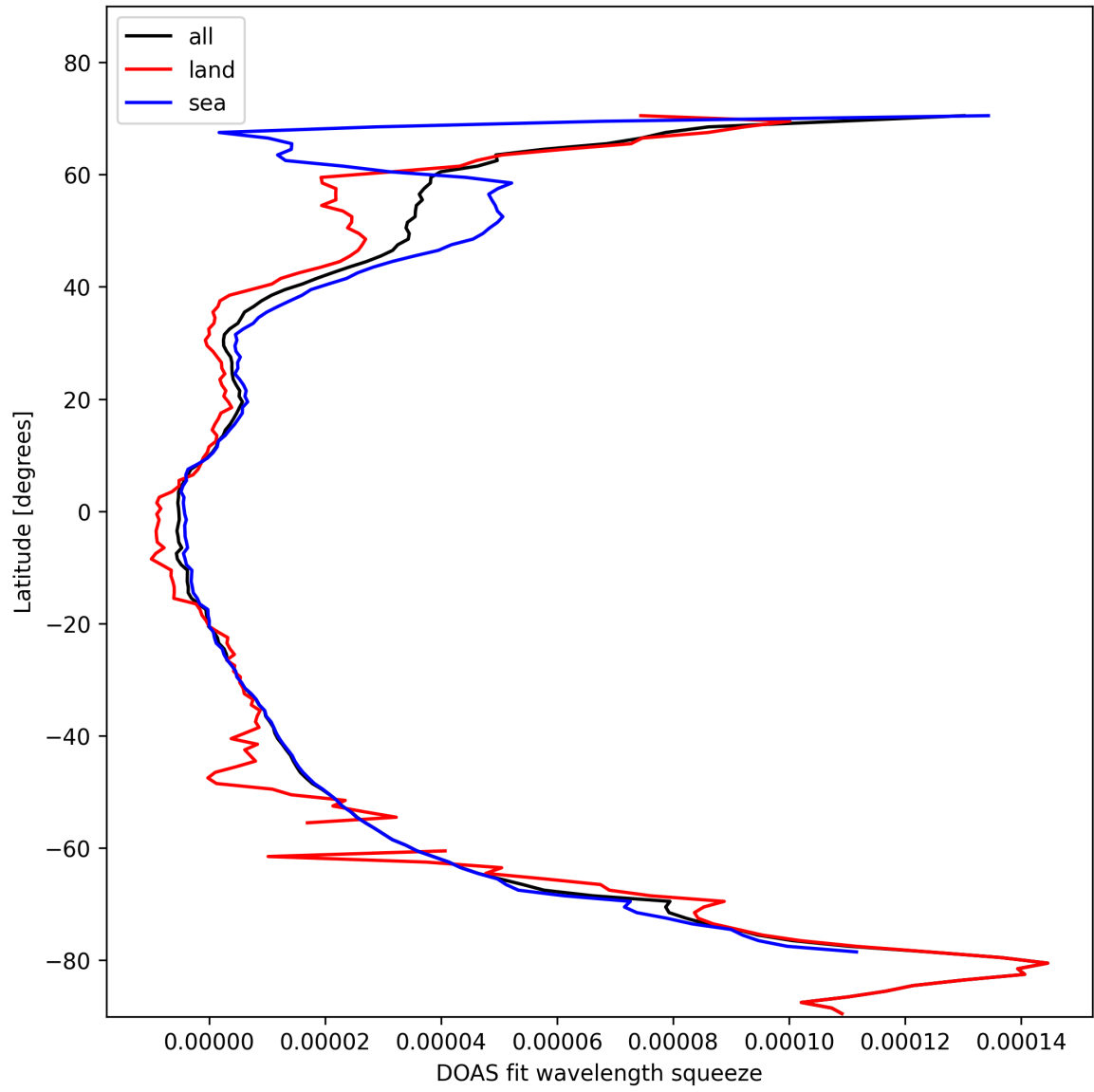
Figure 29: Zonal average of "DOAS fit wavelength squeeze" for 2025-02-09 to 2025-02-10.
