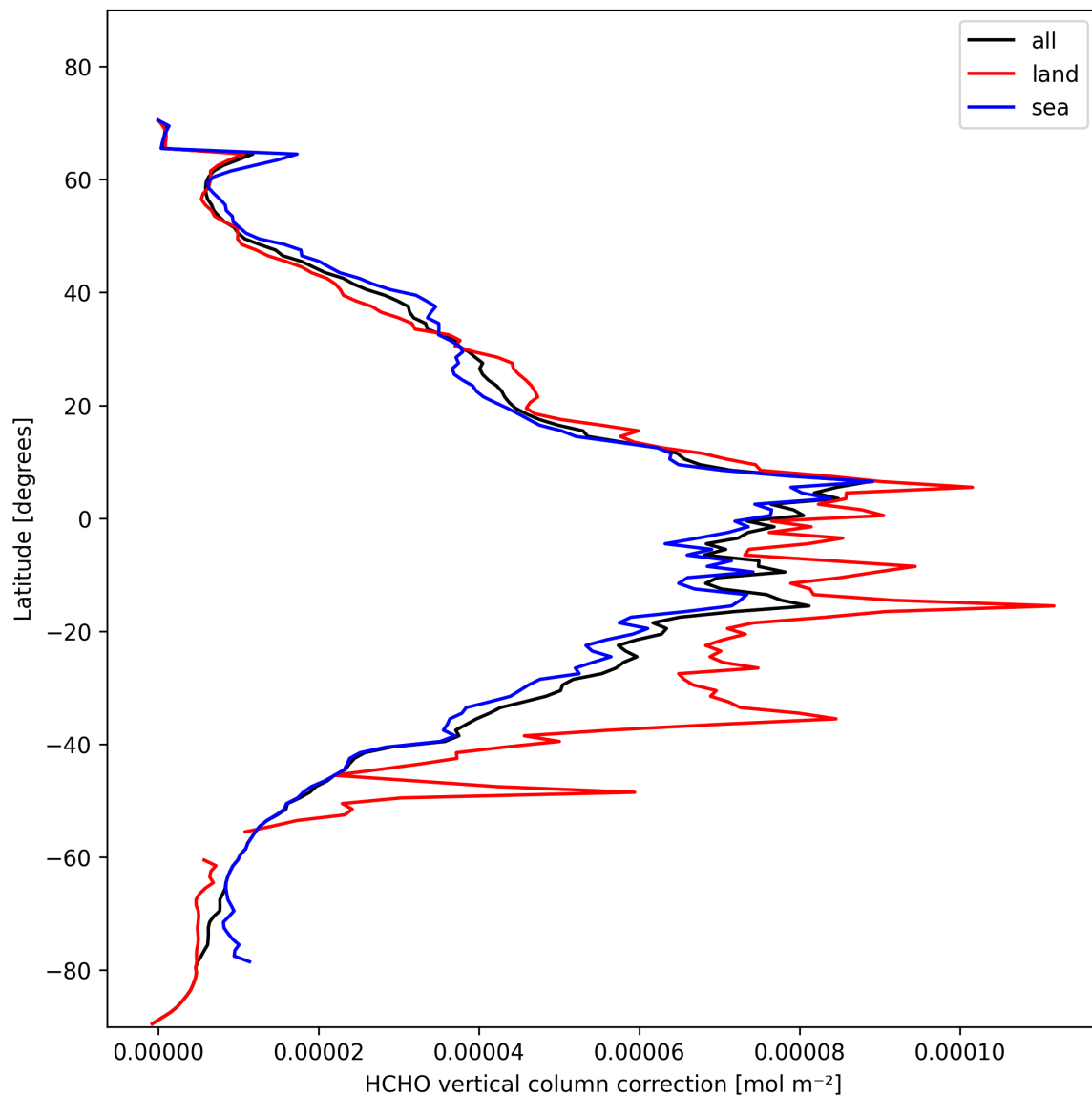
Figure 21: Zonal average of “HCHO vertical column correction” for 2025-02-09 to 2025-02-10.
