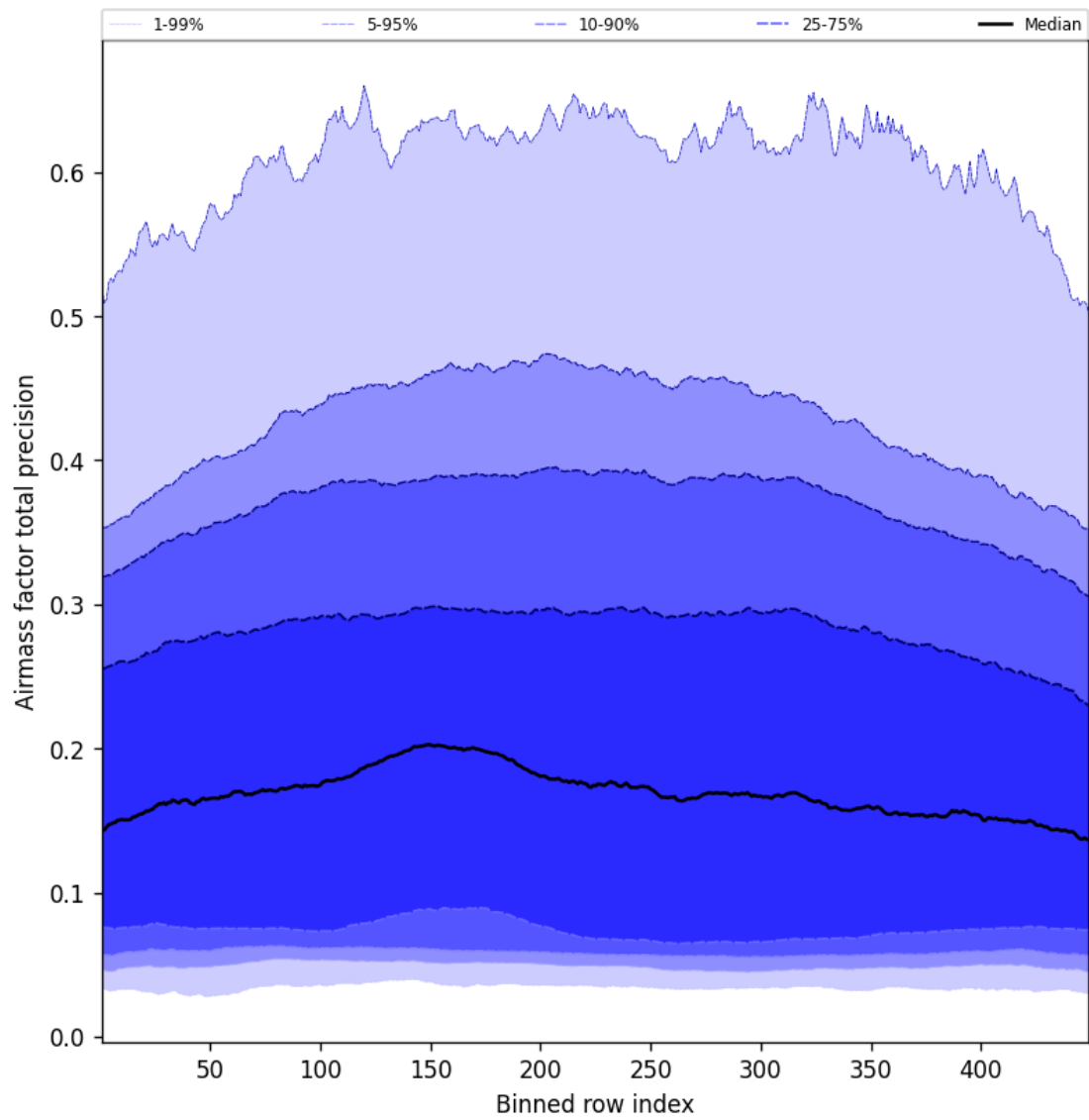
Figure 53: Along track statistics of “Airmass factor total precision” for 2025-02-10 to 2025-02-11
