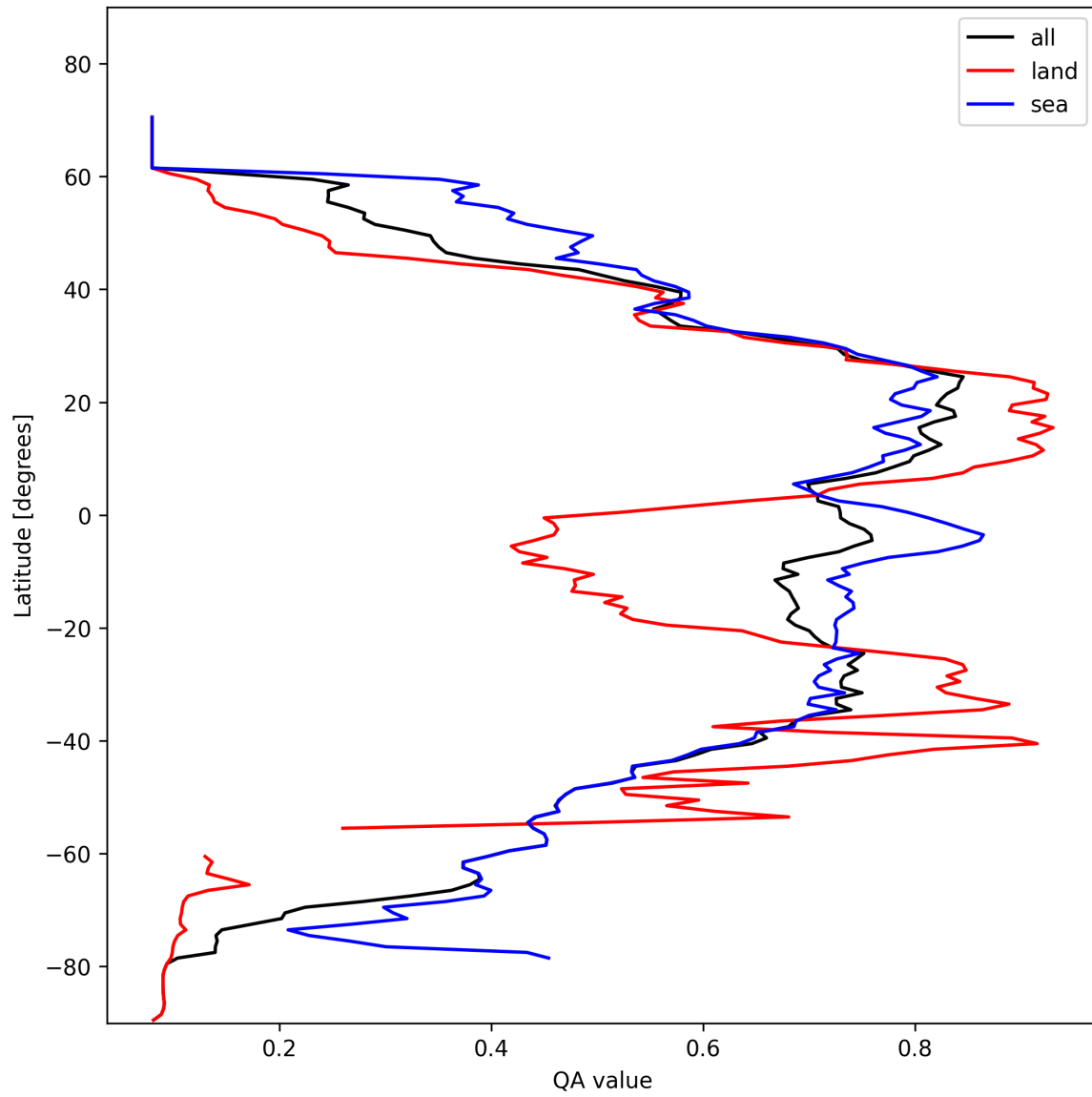
Figure 18: Zonal average of “QA value” for 2025-02-10 to 2025-02-11.
