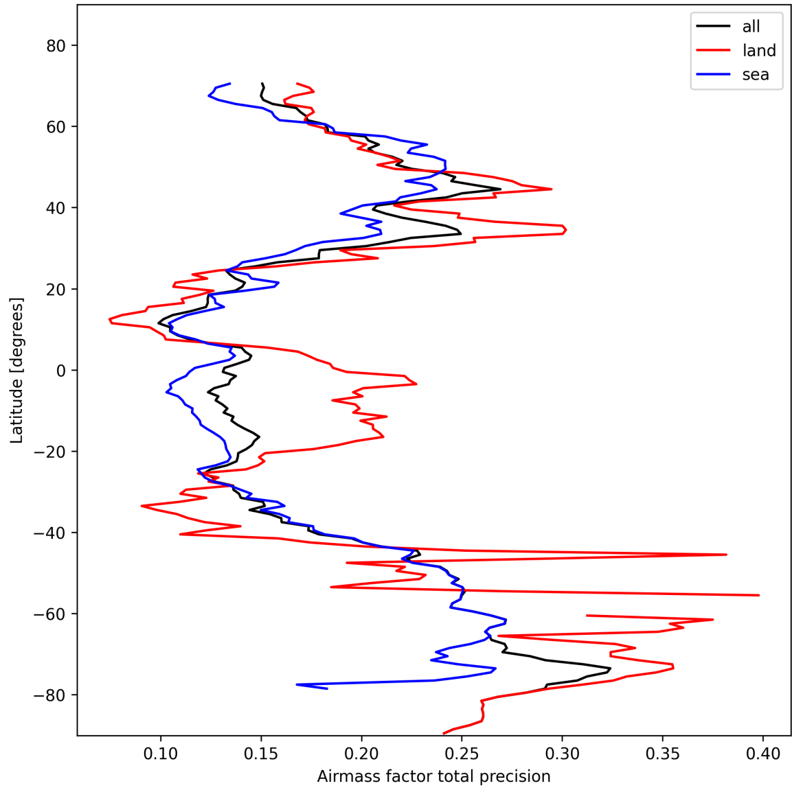
Figure 25: Zonal average of “Airmass factor total precision” for 2025-02-10 to 2025-02-11.
