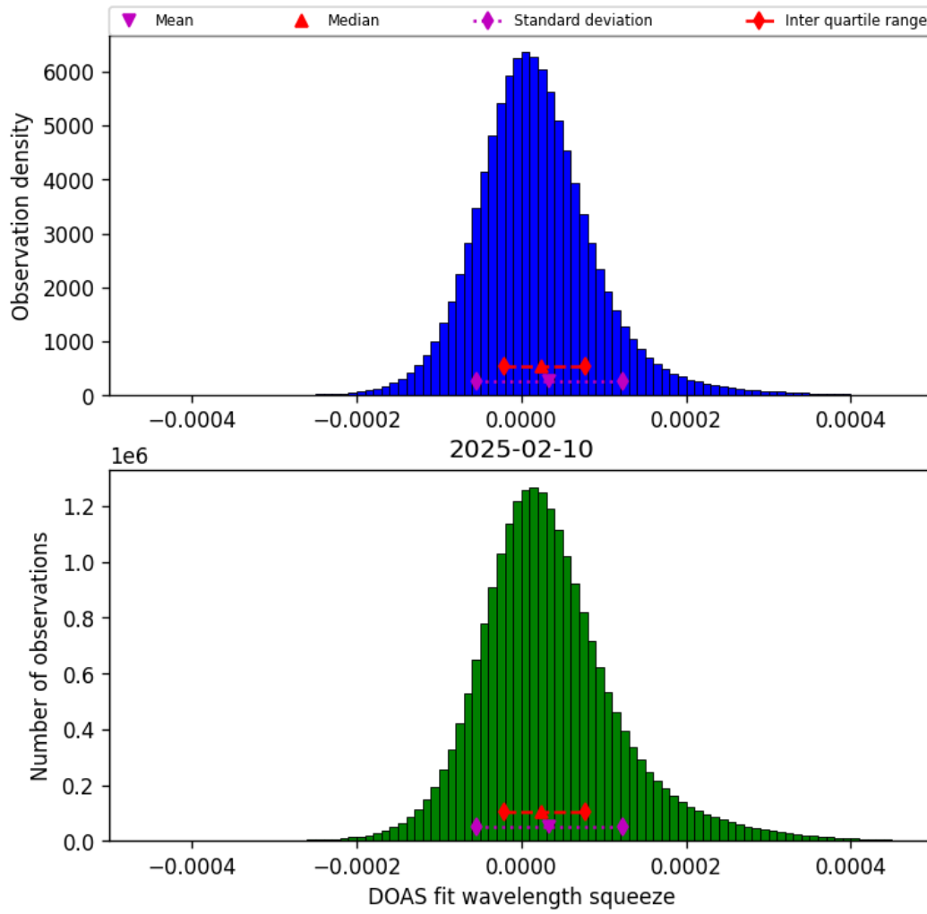
Figure 43: Histogram of “DOAS fit wavelength squeeze” for 2025-02-10 to 2025-02-11
