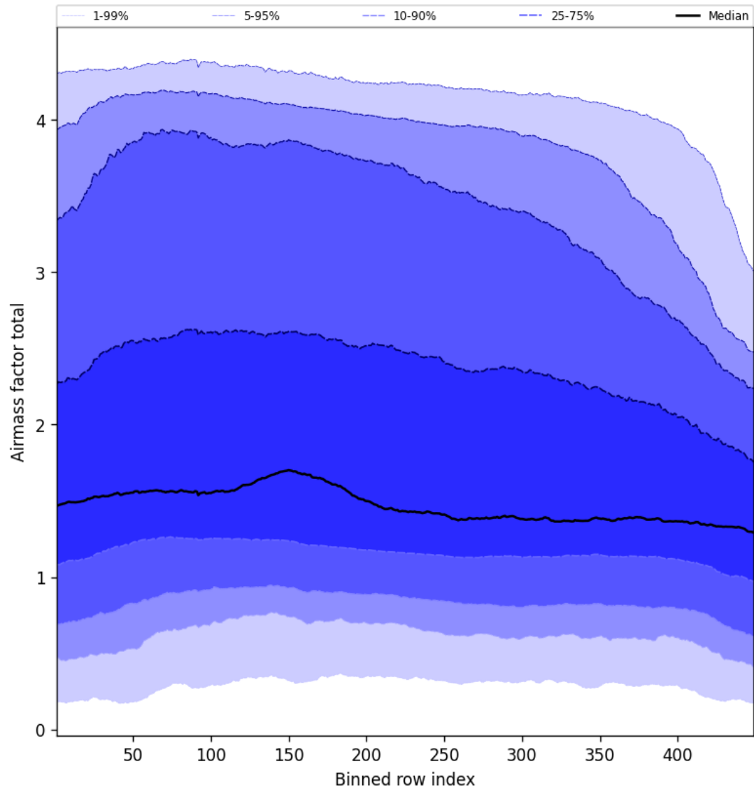
Figure 52: Along track statistics of “Airmass factor total” for 2025-02-10 to 2025-02-11
