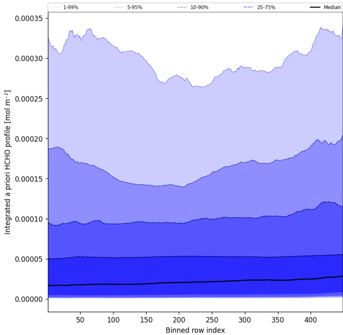
Figure 55: Along track statistics of “Integrated a priori HCHO profile” for 2025-02-10 to 2025-02-11
