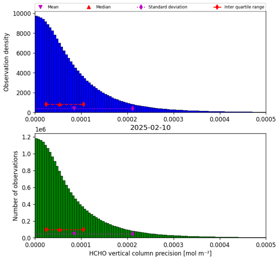
Figure 34: Histogram of “HCHO vertical column precision” for 2025-02-10 to 2025-02-11
