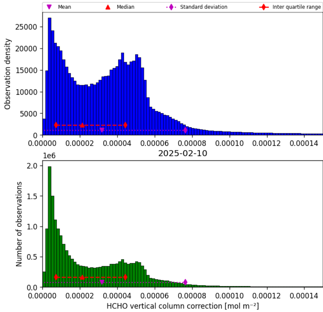
Figure 35: Histogram of “HCHO vertical column correction” for 2025-02-10 to 2025-02-11
