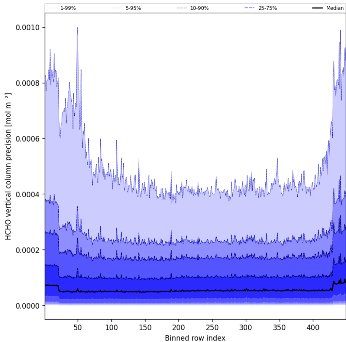
Figure 48: Along track statistics of “HCHO vertical column precision” for 2025-02-10 to 2025-02-11
