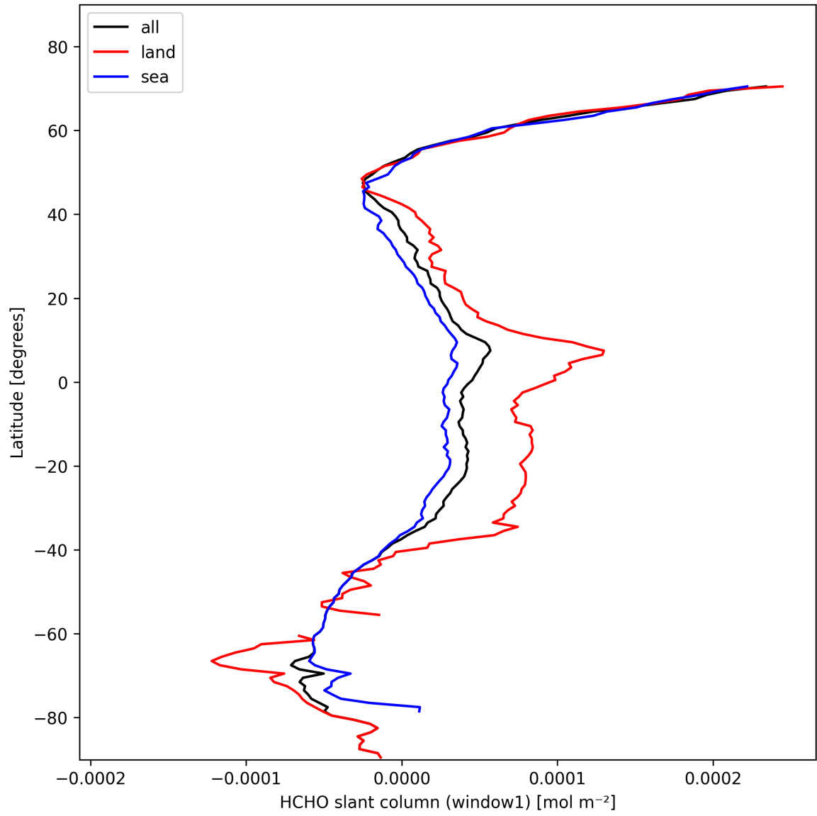
Figure 22: Zonal average of “HCHO slant column (window1)” for 2025-02-10 to 2025-02-11.
