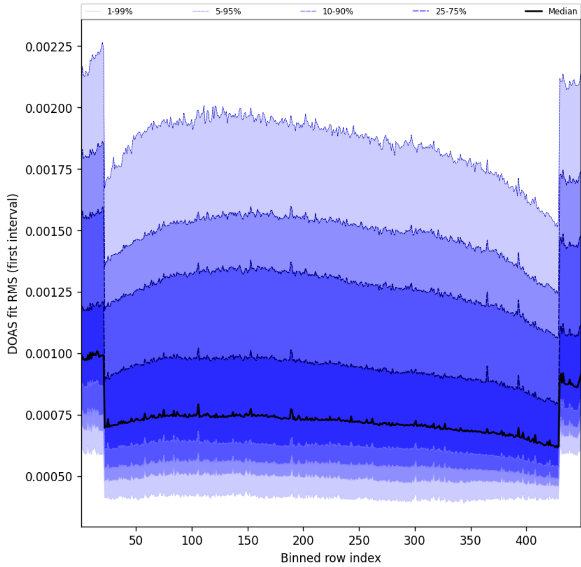
Figure 58: Along track statistics of “DOAS fit RMS (first interval)” for 2025-02-10 to 2025-02-11
