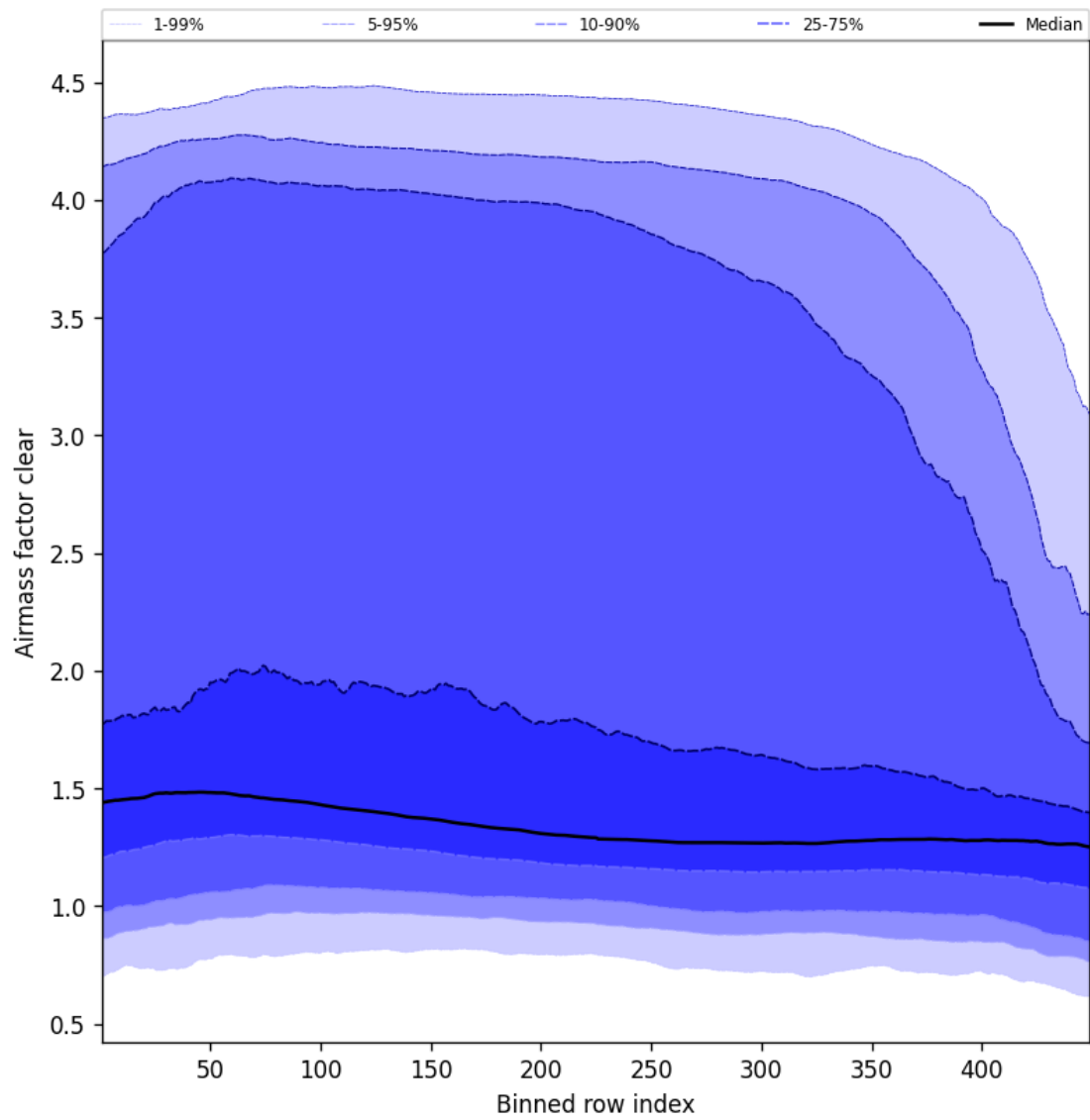
Figure 54: Along track statistics of “Air mass factor clear” for 2025-02-10 to 2025-02-11
