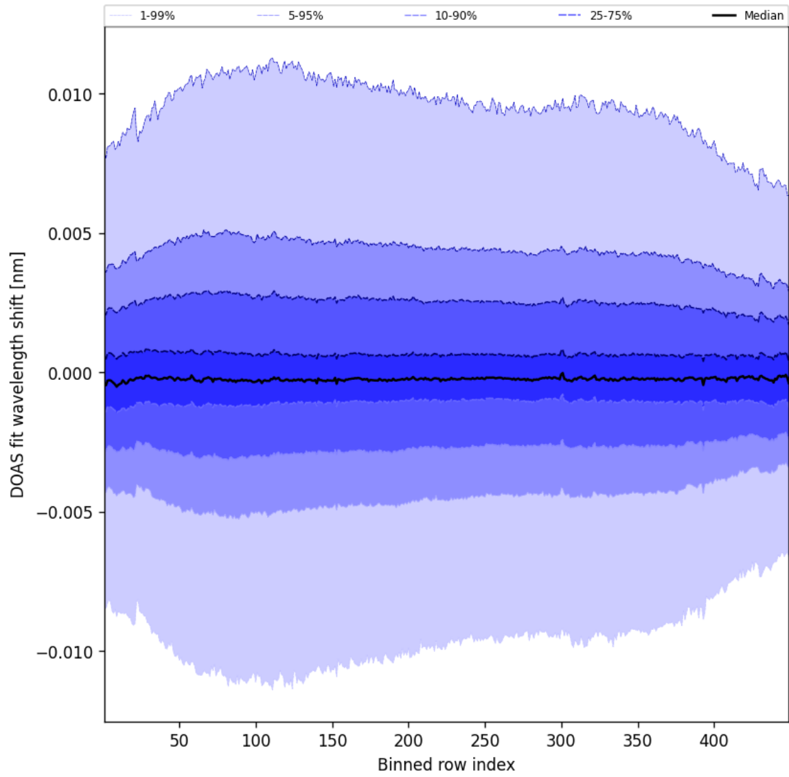
Figure 56: Along track statistics of “DOAS fit wavelength shift” for 2025-02-10 to 2025-02-11
