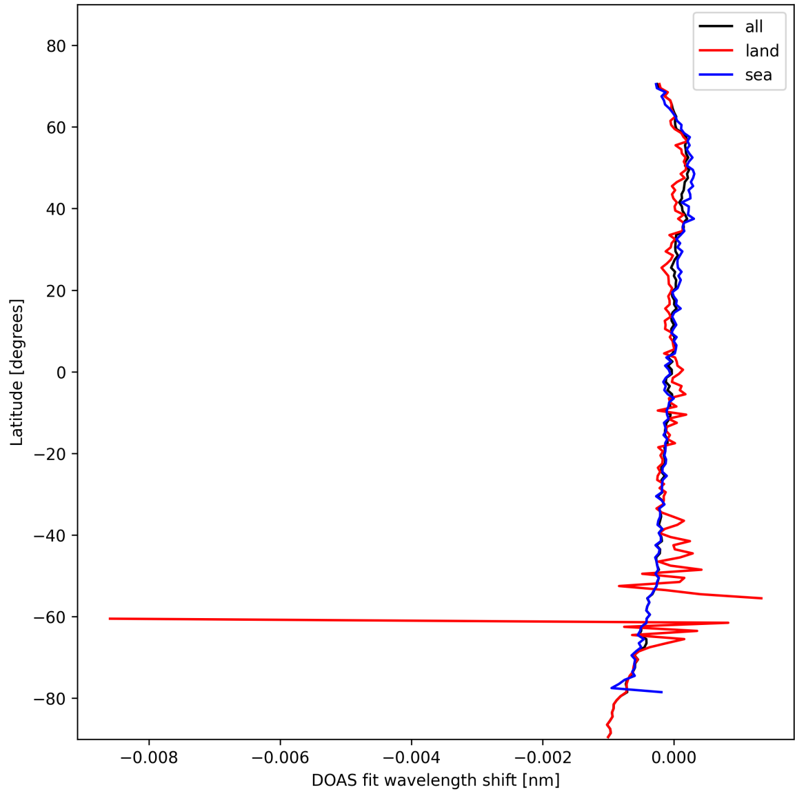
Figure 28: Zonal average of "DOAS fit wavelength shift" for 2025-02-10 to 2025-02-11.
