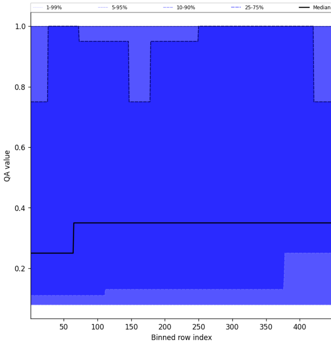
Figure 46: Along track statistics of “QA value” for 2025-02-10 to 2025-02-11
