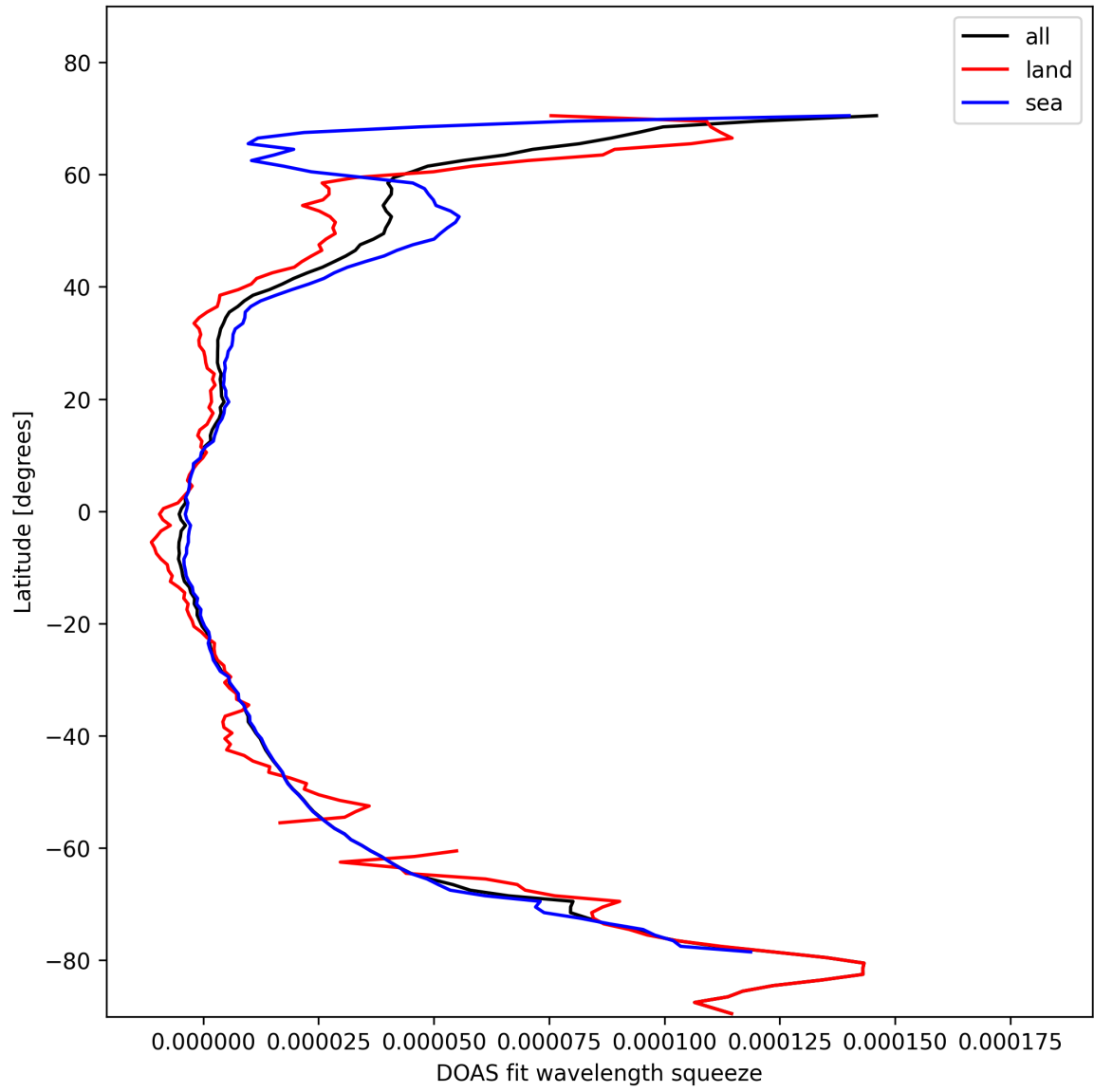
Figure 29: Zonal average of “DOAS fit wavelength squeeze” for 2025-02-10 to 2025-02-11.
