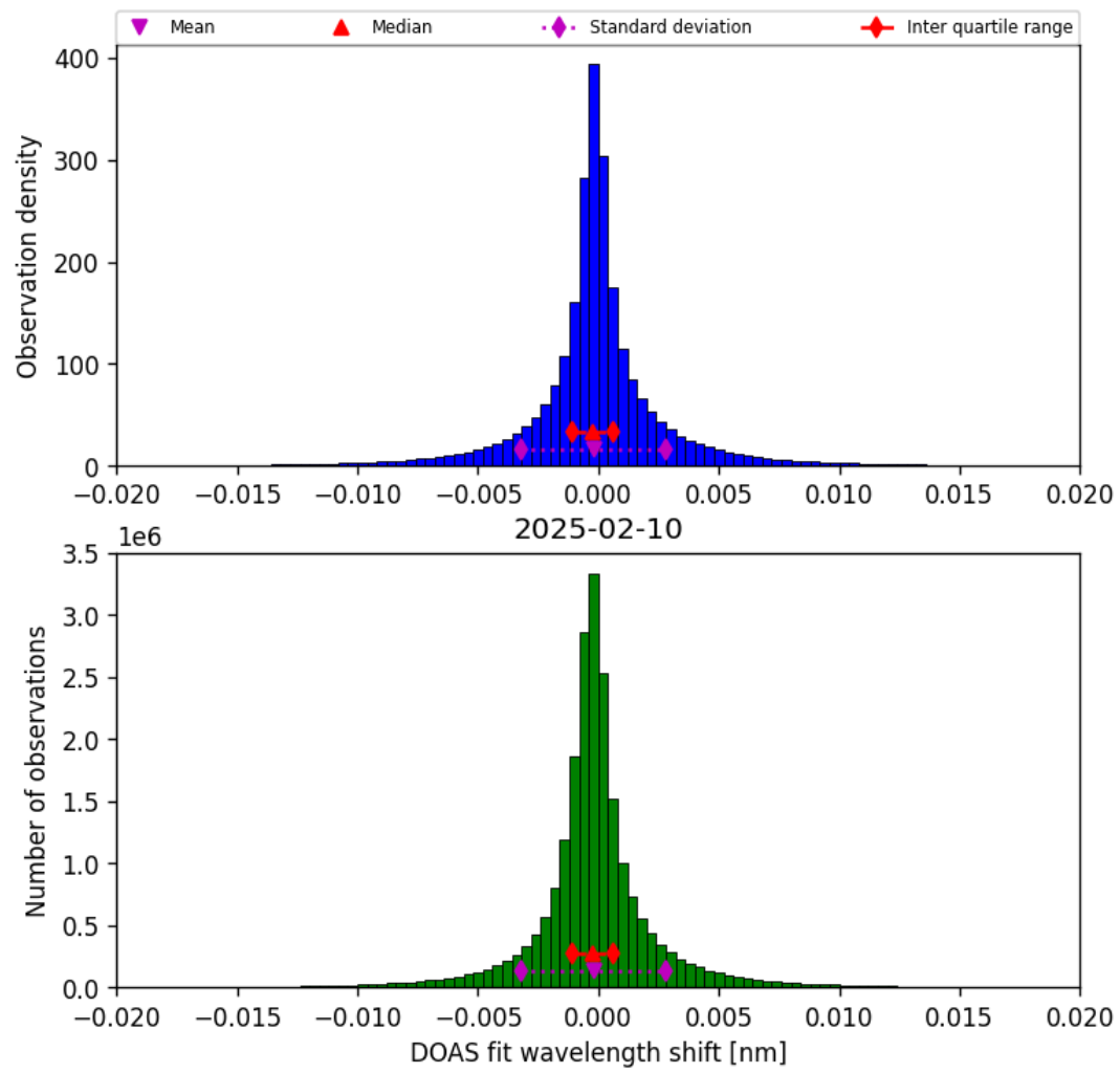
Figure 42: Histogram of “DOAS fit wavelength shift” for 2025-02-10 to 2025-02-11
