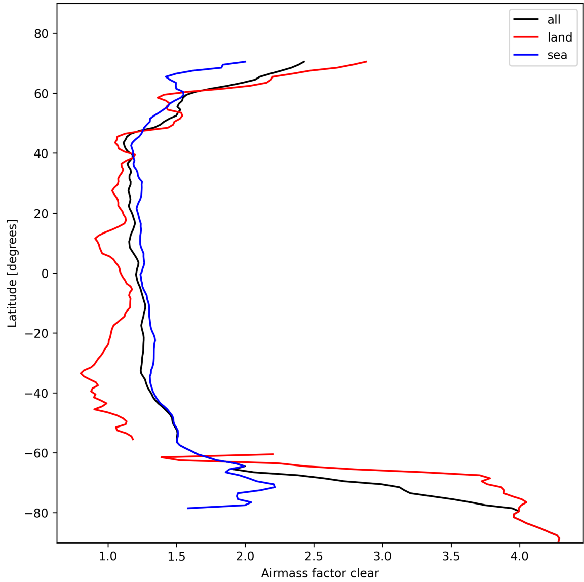
Figure 26: Zonal average of “Airmass factor clear” for 2025-02-10 to 2025-02-11.
