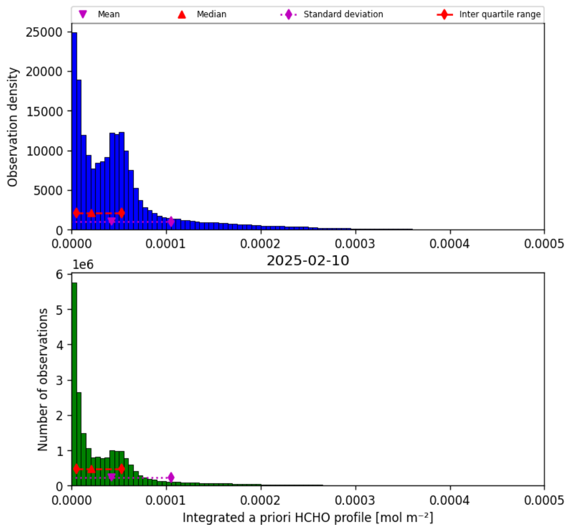
Figure 41: Histogram of “Integrated a priori HCHO profile” for 2025-02-10 to 2025-02-11
