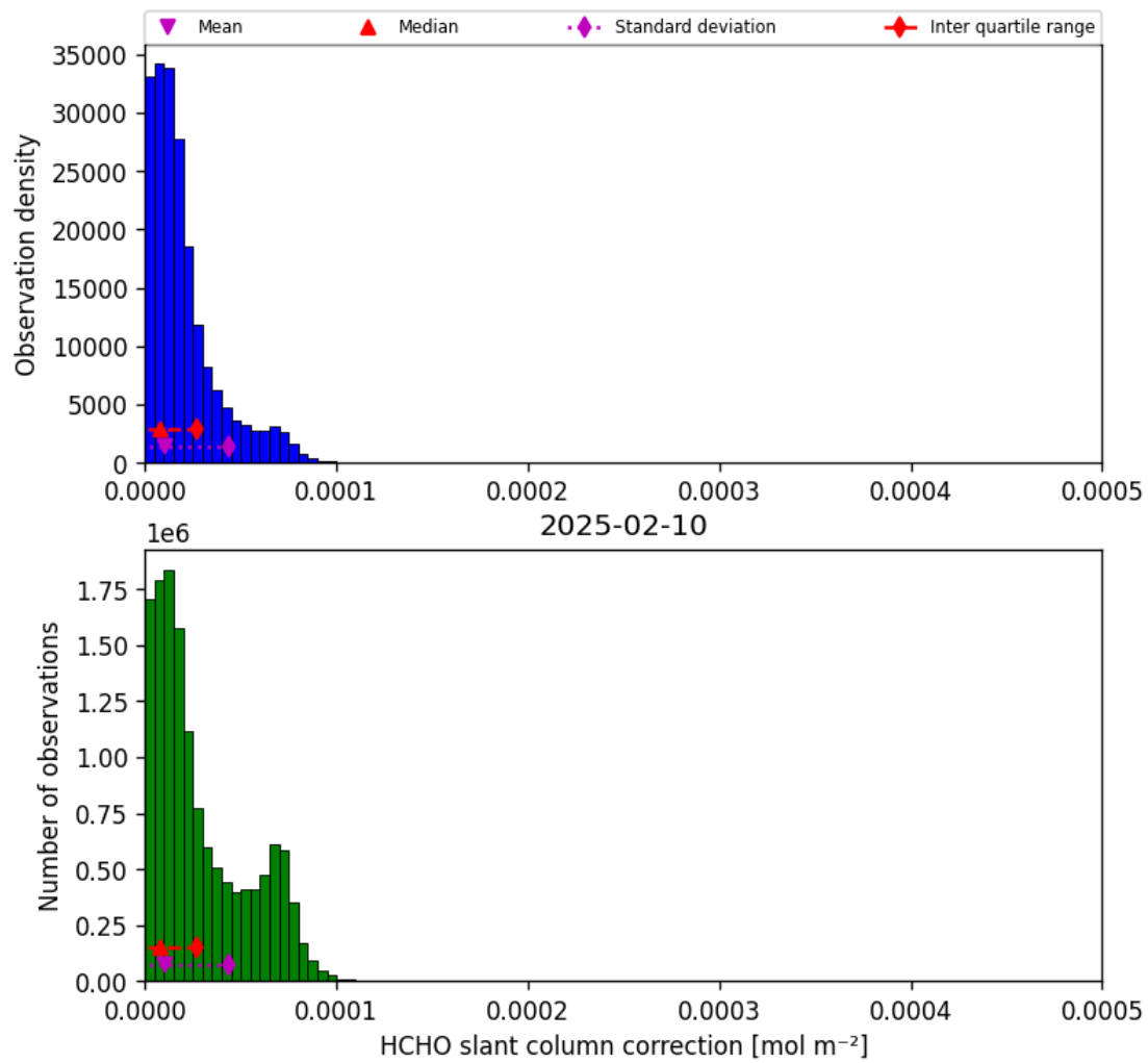
Figure 45: Histogram of “HCHO slant column correction” for 2025-02-10 to 2025-02-11
