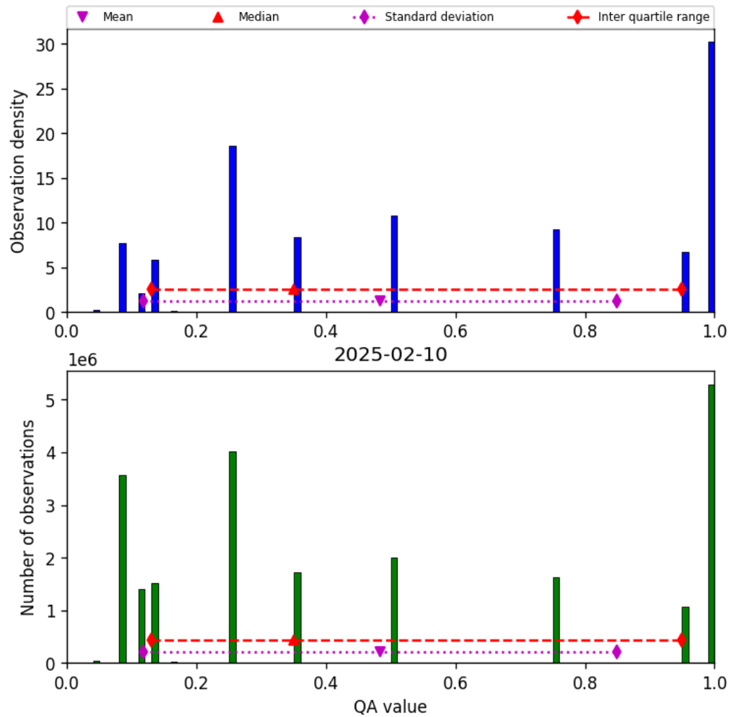
Figure 32: Histogram of “QA value” for 2025-02-10 to 2025-02-11
