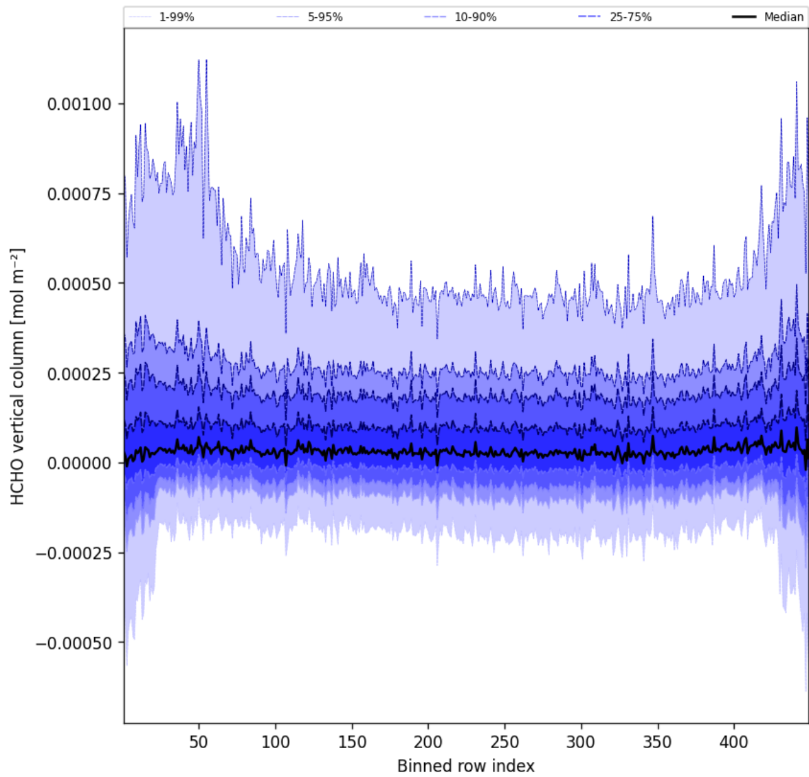
Figure 47: Along track statistics of “HCHO vertical column” for 2025-02-10 to 2025-02-11
