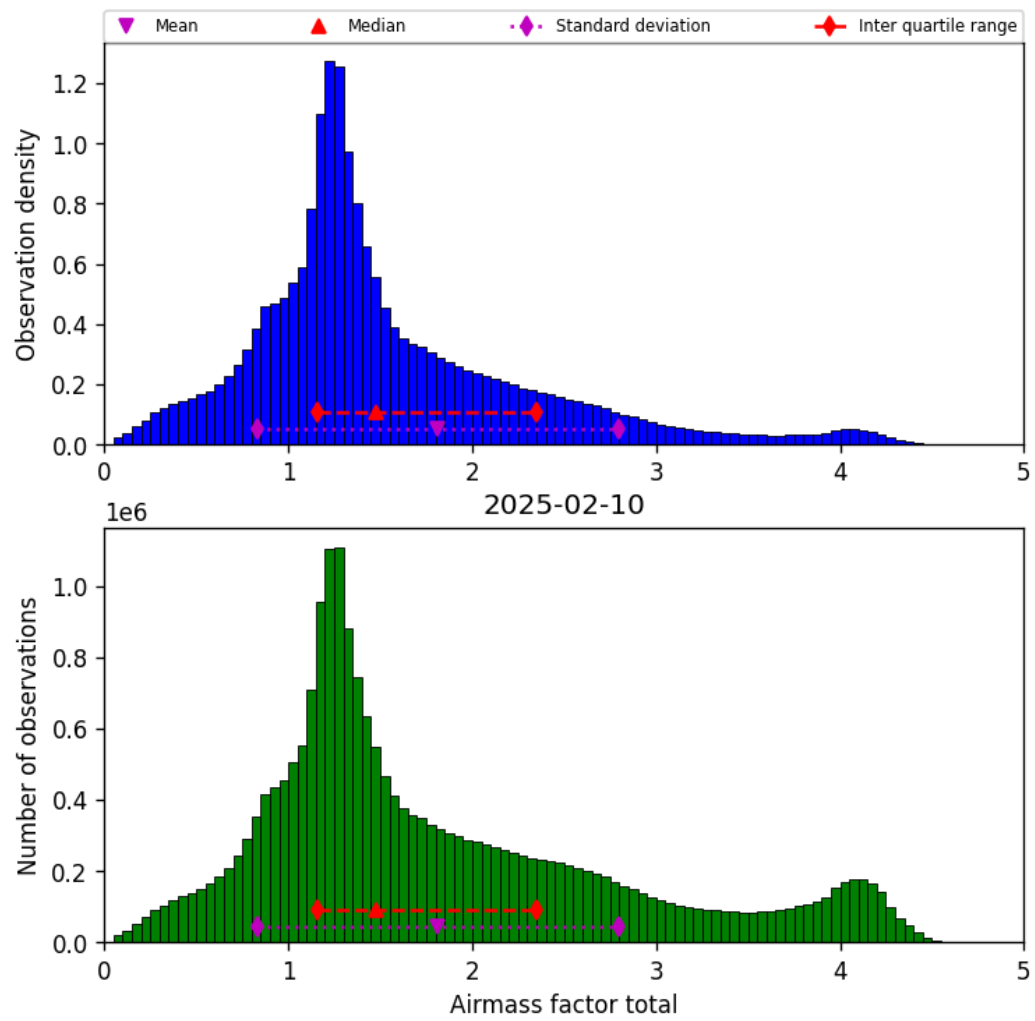
Figure 38: Histogram of “Airmass factor total” for 2025-02-10 to 2025-02-11
