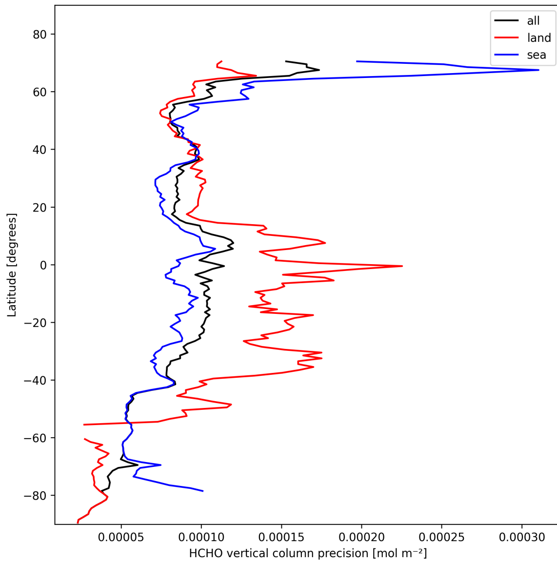
Figure 20: Zonal average of “HCHO vertical column precision” for 2025-02-10 to 2025-02-11.
