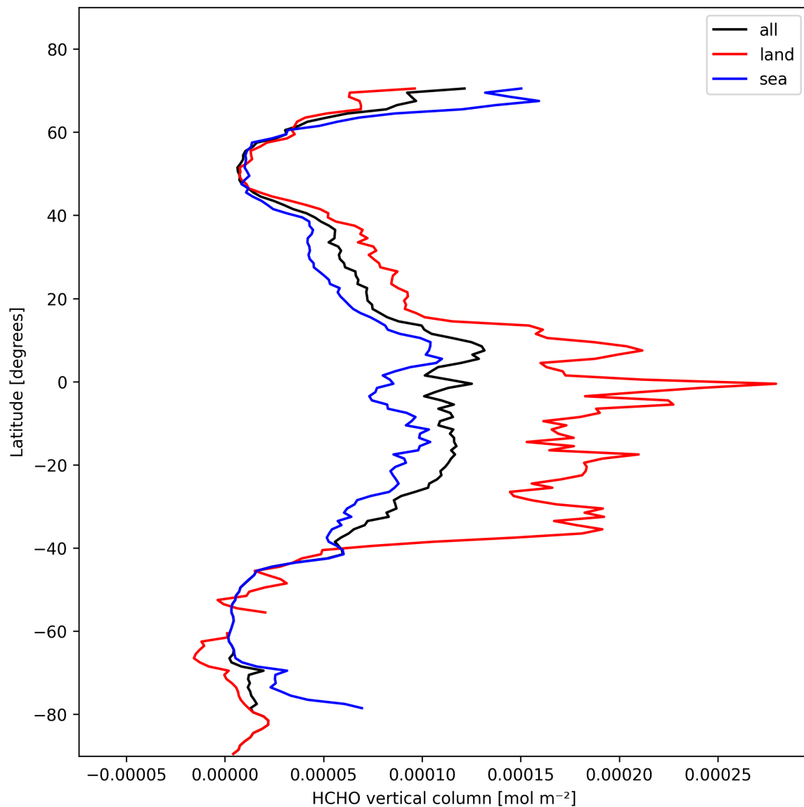
Figure 19: Zonal average of “HCHO vertical column” for 2025-02-10 to 2025-02-11.
