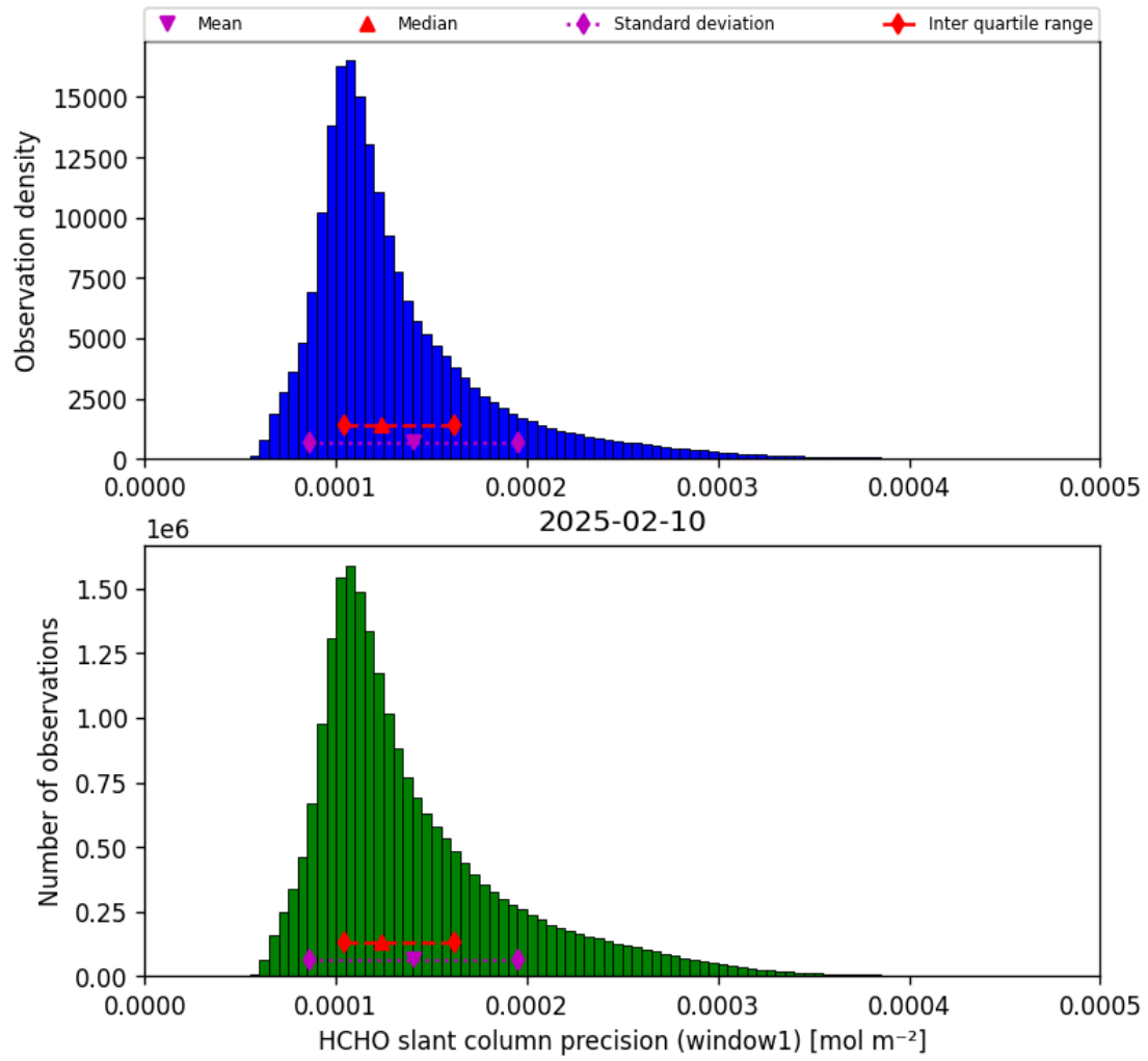
Figure 37: Histogram of “HCHO slant column precision (window1)” for 2025-02-10 to 2025-02-11
