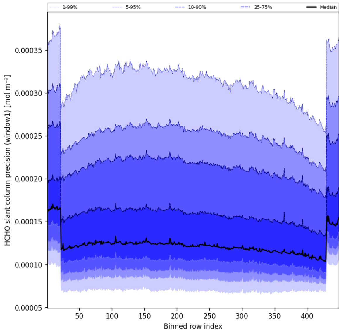
Figure 51: Along track statistics of “HCHO slant column precision (window1)” for 2025-02-10 to 2025-02-11
