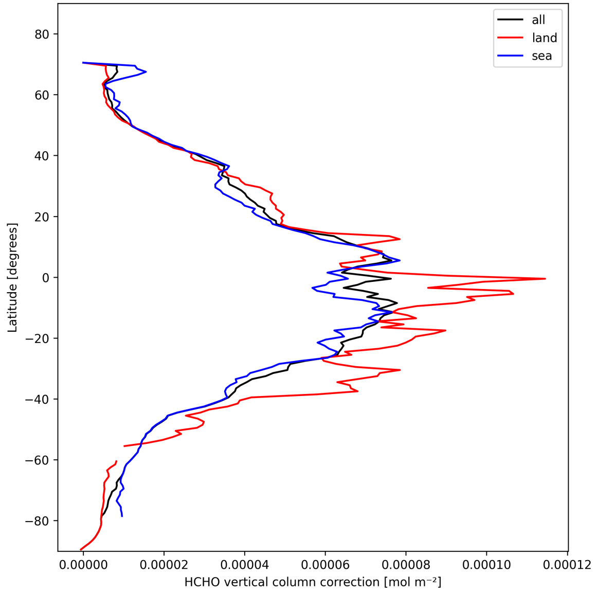
Figure 21: Zonal average of “HCHO vertical column correction” for 2025-02-10 to 2025-02-11.
