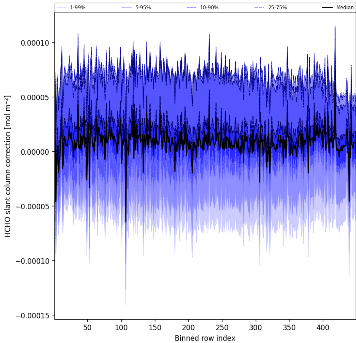
Figure 59: Along track statistics of “HCHO slant column correction” for 2025-02-10 to 2025-02-11
