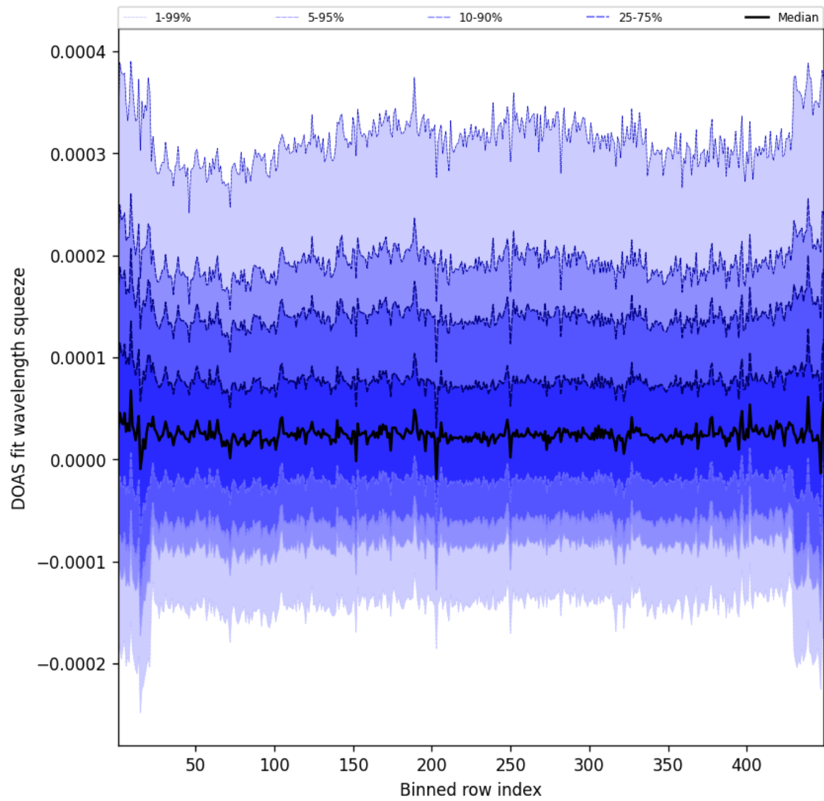
Figure 57: Along track statistics of “DOAS fit wavelength squeeze” for 2025-02-10 to 2025-02-11
