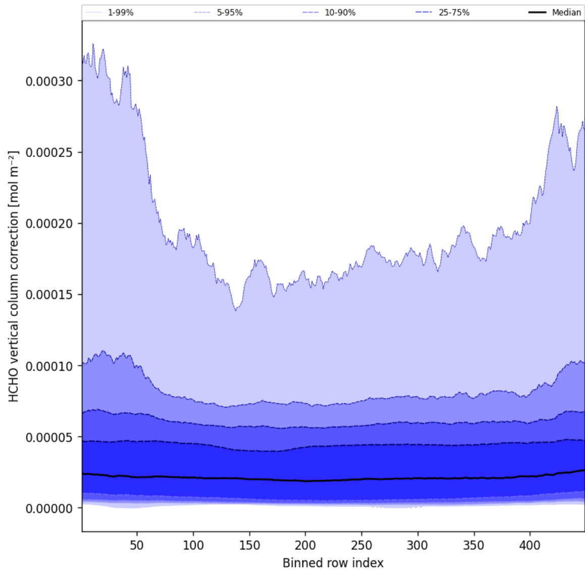
Figure 49: Along track statistics of “HCHO vertical column correction” for 2025-02-10 to 2025-02-11
