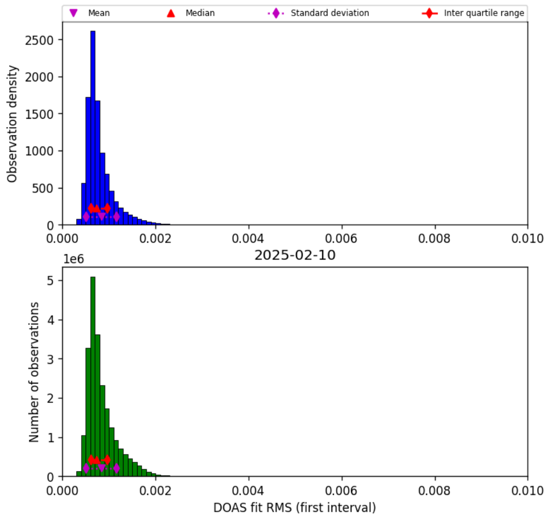
Figure 44: Histogram of “DOAS fit RMS (first interval)” for 2025-02-10 to 2025-02-11
