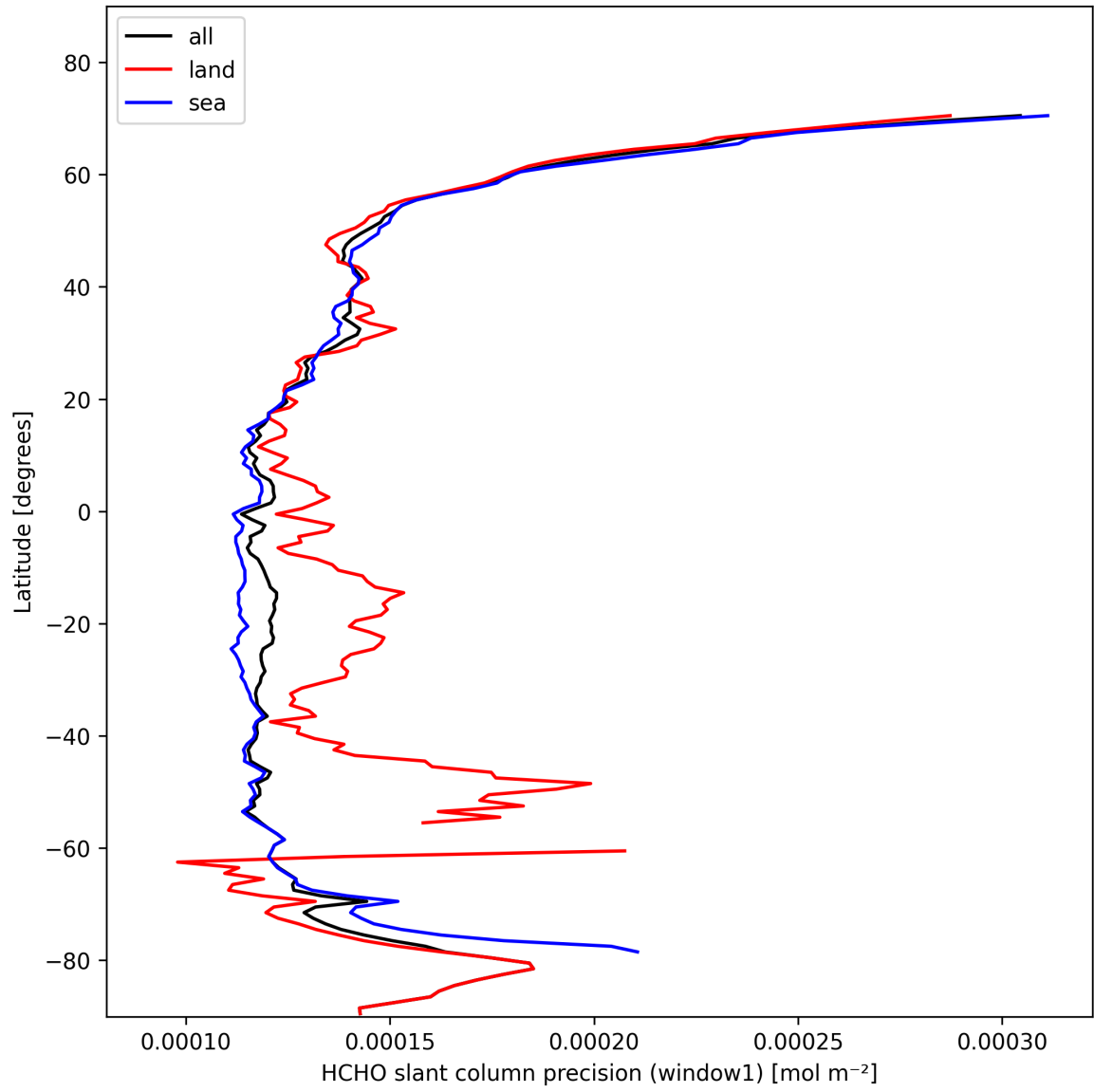
Figure 23: Zonal average of “HCHO slant column precision (window1)” for 2025-02-10 to 2025-02-11.
