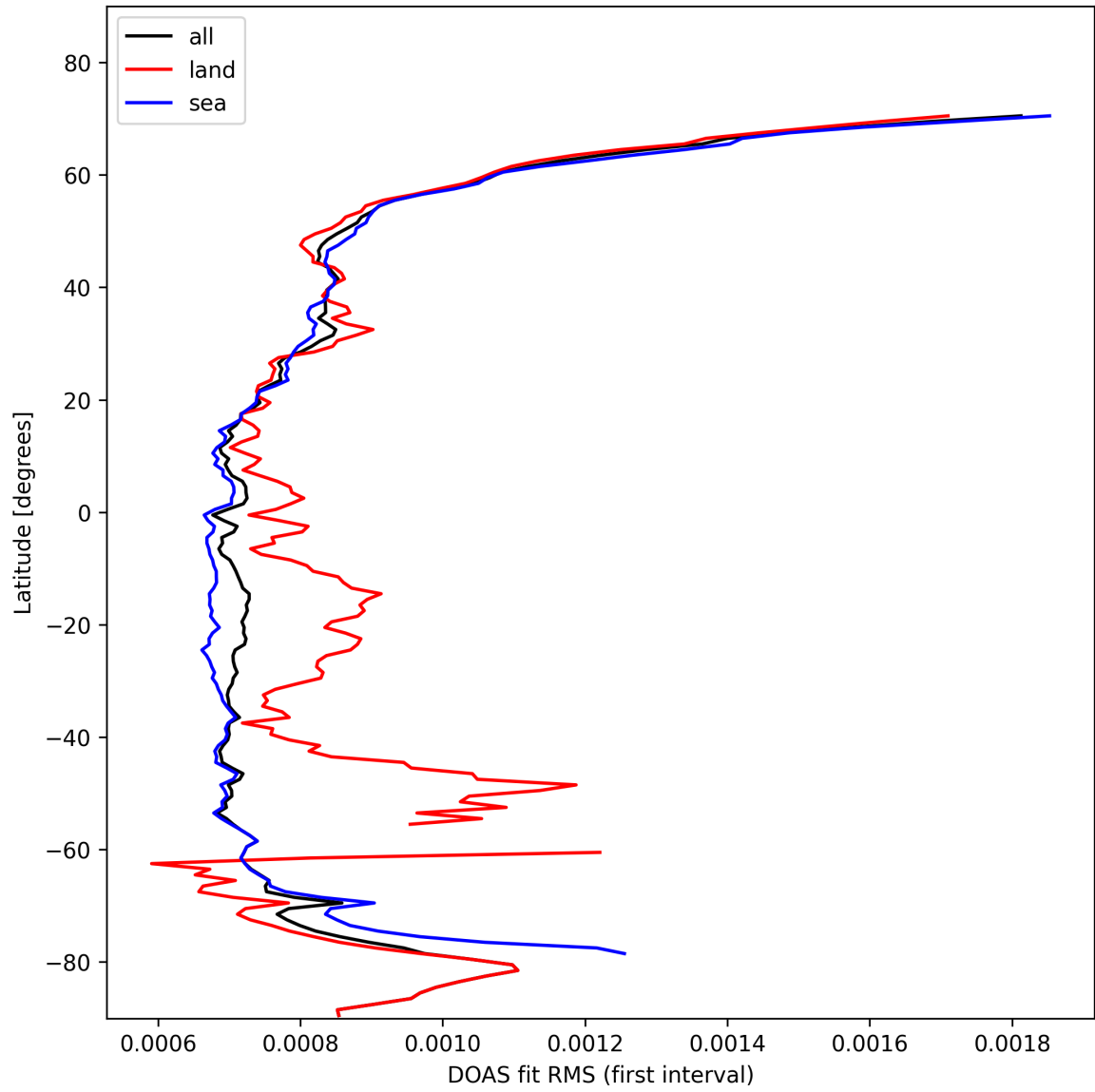
Figure 30: Zonal average of “DOAS fit RMS (first interval)” for 2025-02-10 to 2025-02-11.
