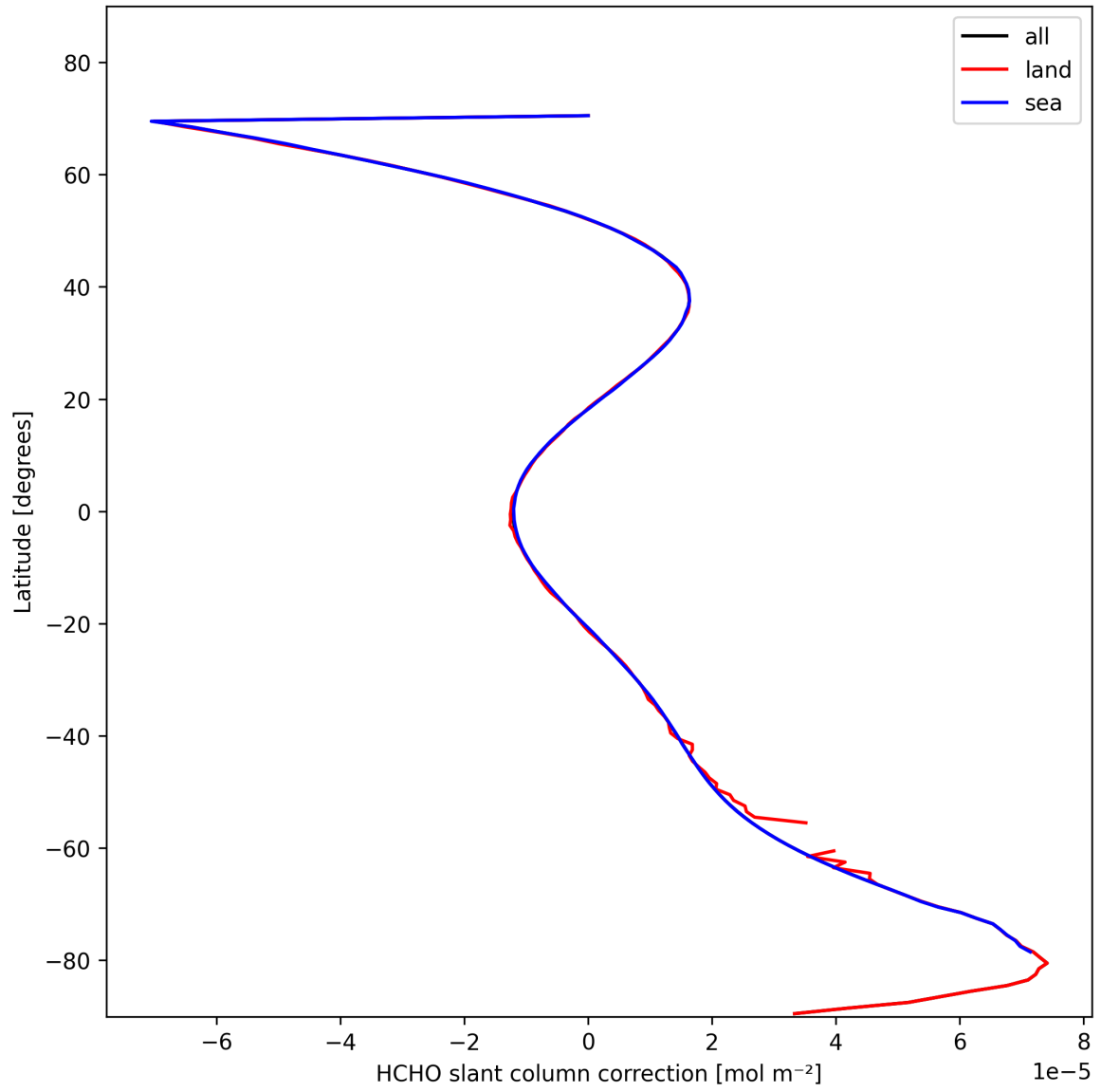
Figure 31: Zonal average of “HCHO slant column correction” for 2025-02-10 to 2025-02-11.
