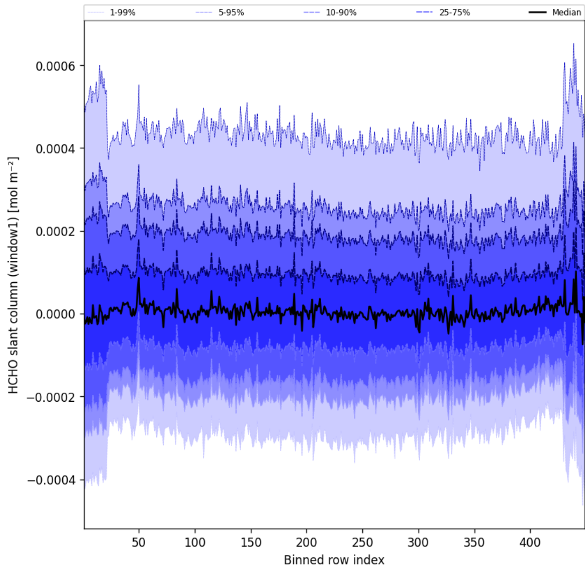
Figure 50: Along track statistics of “HCHO slant column (window1)” for 2025-02-10 to 2025-02-11
