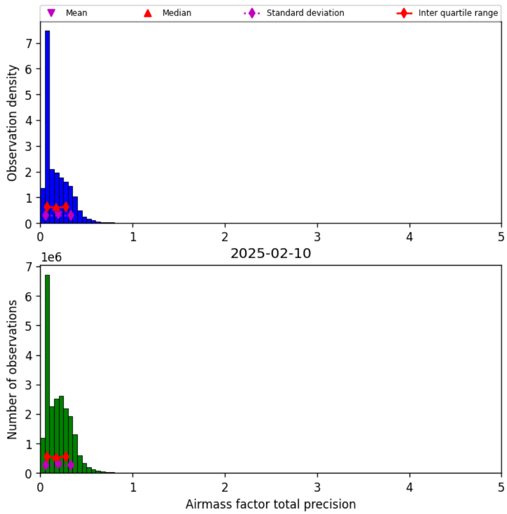
Figure 39: Histogram of “Airmass factor total precision” for 2025-02-10 to 2025-02-11
