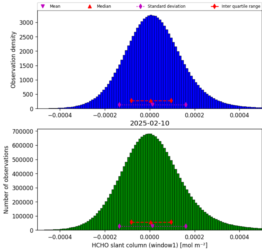
Figure 36: Histogram of “HCHO slant column (window1)” for 2025-02-10 to 2025-02-11
