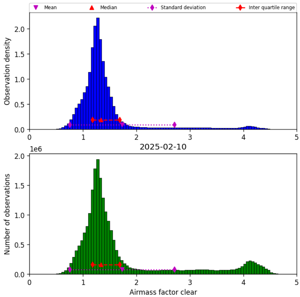
Figure 40: Histogram of “Airmass factor clear” for 2025-02-10 to 2025-02-11
