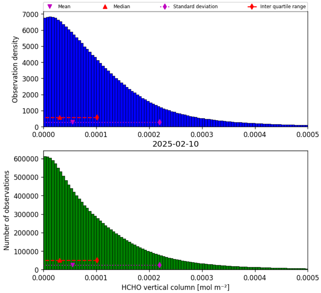
Figure 33: Histogram of “HCHO vertical column” for 2025-02-10 to 2025-02-11
