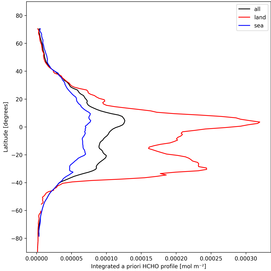
Figure 27: Zonal average of “Integrated a priori HCHO profile” for 2025-02-10 to 2025-02-11.
