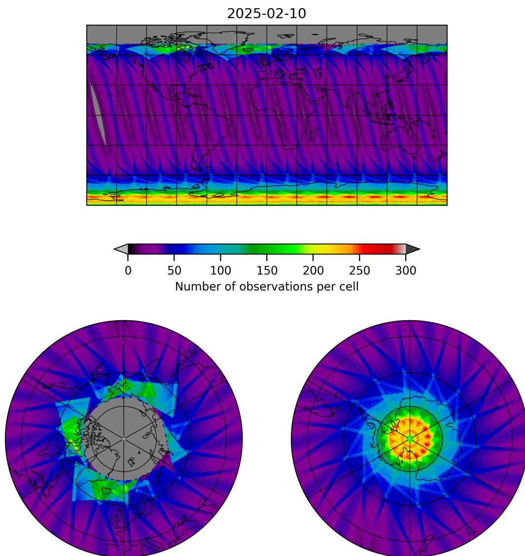
Figure 17: Map of the number of observations for 2025-02-10 to 2025-02-11
