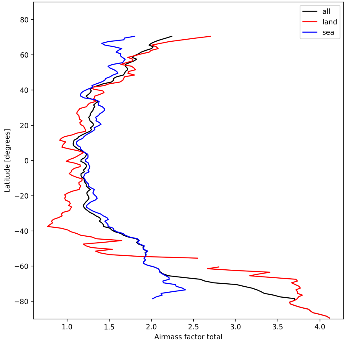
Figure 24: Zonal average of “Airmass factor total” for 2025-02-10 to 2025-02-11.
