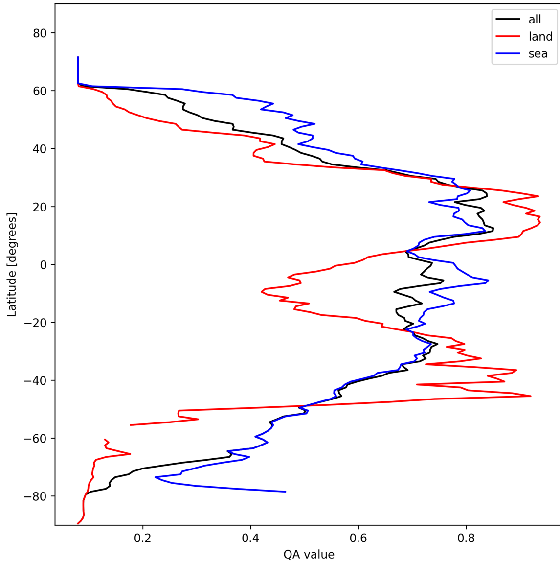
Figure 18: Zonal average of “QA value” for 2025-02-11 to 2025-02-11.
