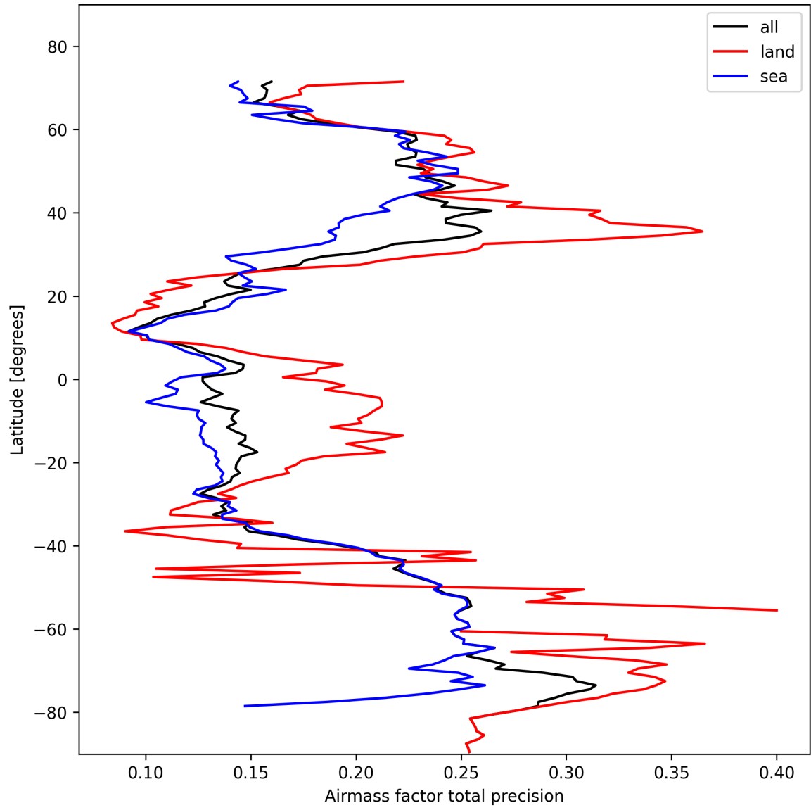
Figure 25: Zonal average of “Airmass factor total precision” for 2025-02-11 to 2025-02-11.
