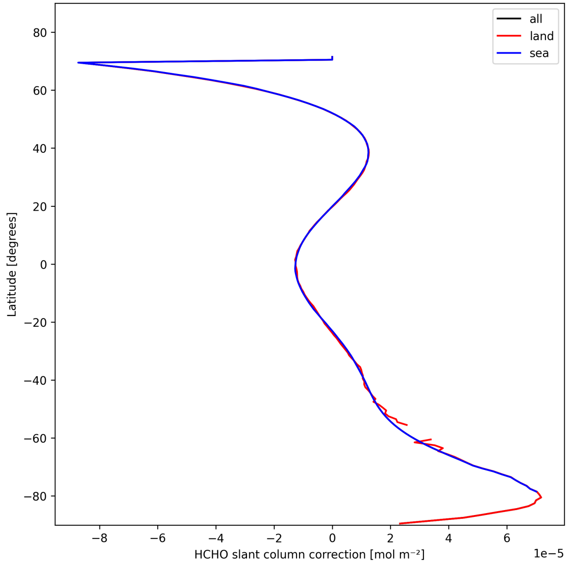
Figure 31: Zonal average of “HCHO slant column correction” for 2025-02-11 to 2025-02-11.
