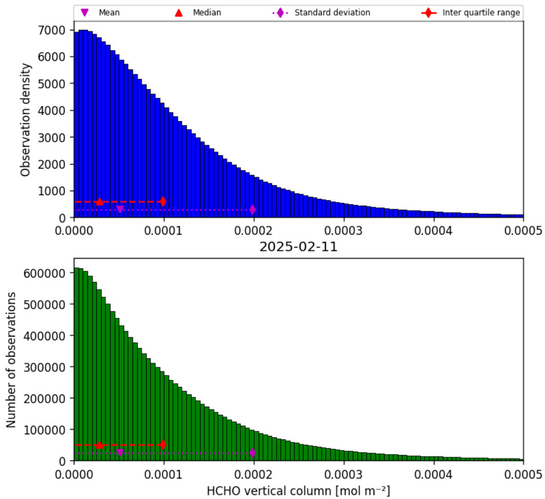
Figure 33: Histogram of “HCHO vertical column” for 2025-02-11 to 2025-02-11
