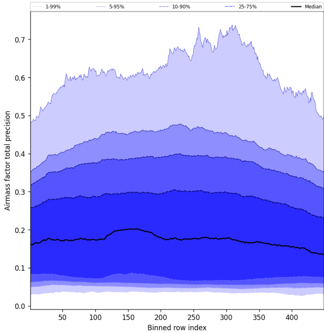
Figure 53: Along track statistics of “Airmass factor total precision” for 2025-02-11 to 2025-02-11
