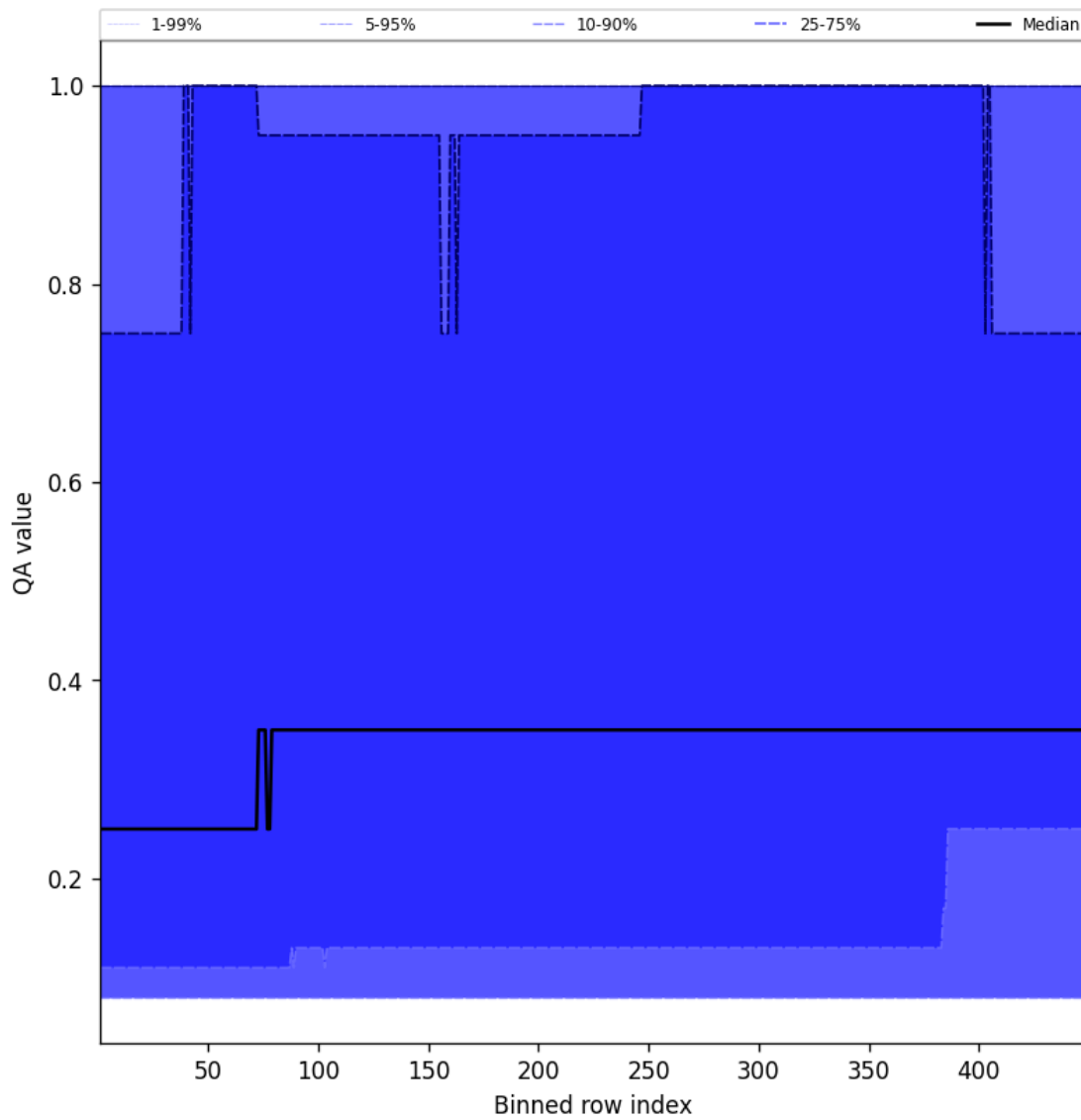
Figure 46: Along track statistics of “QA value” for 2025-02-11 to 2025-02-11
