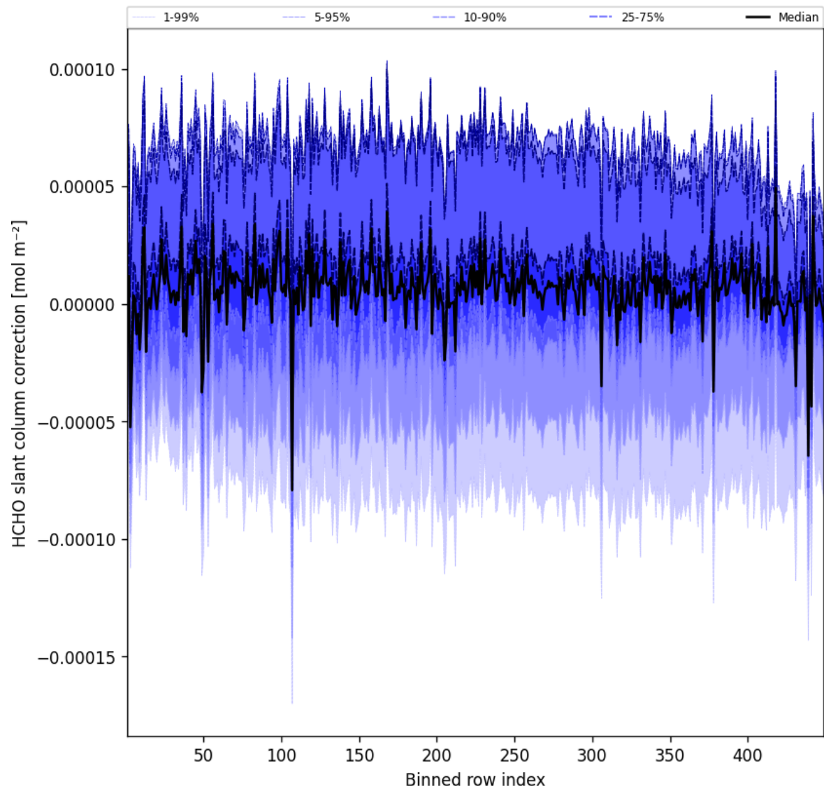
Figure 59: Along track statistics of “HCHO slant column correction” for 2025-02-11 to 2025-02-11
