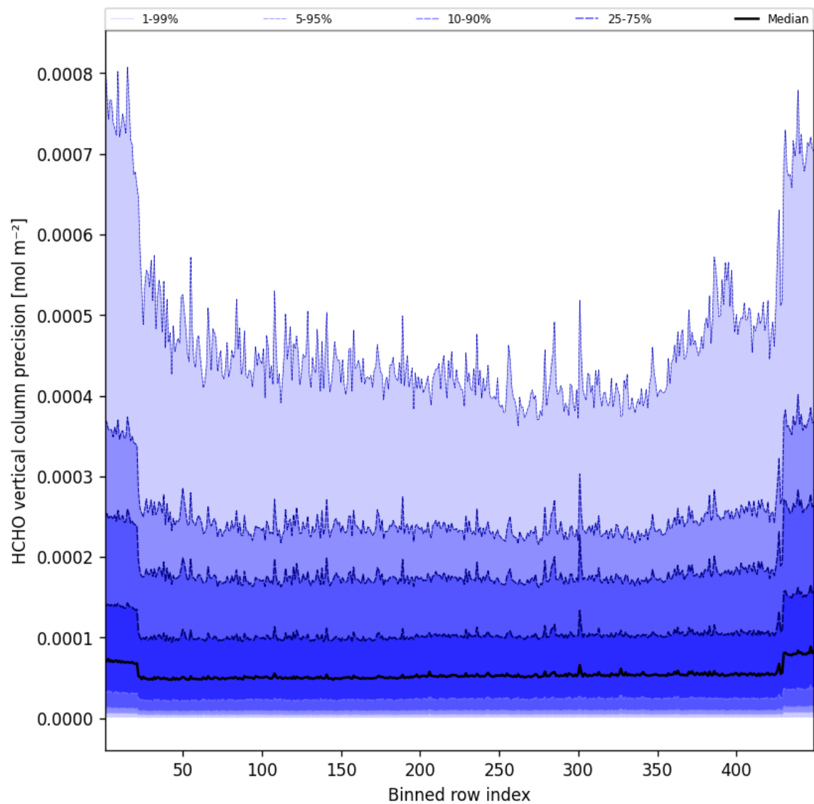
Figure 48: Along track statistics of “HCHO vertical column precision” for 2025-02-11 to 2025-02-11
