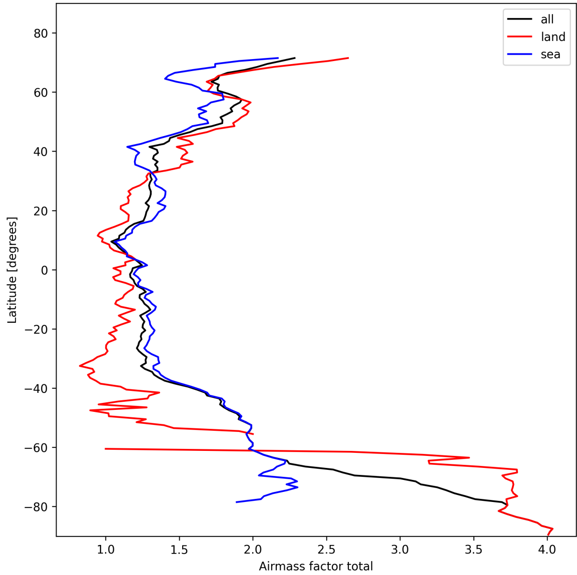
Figure 24: Zonal average of “Airmass factor total” for 2025-02-11 to 2025-02-11.
