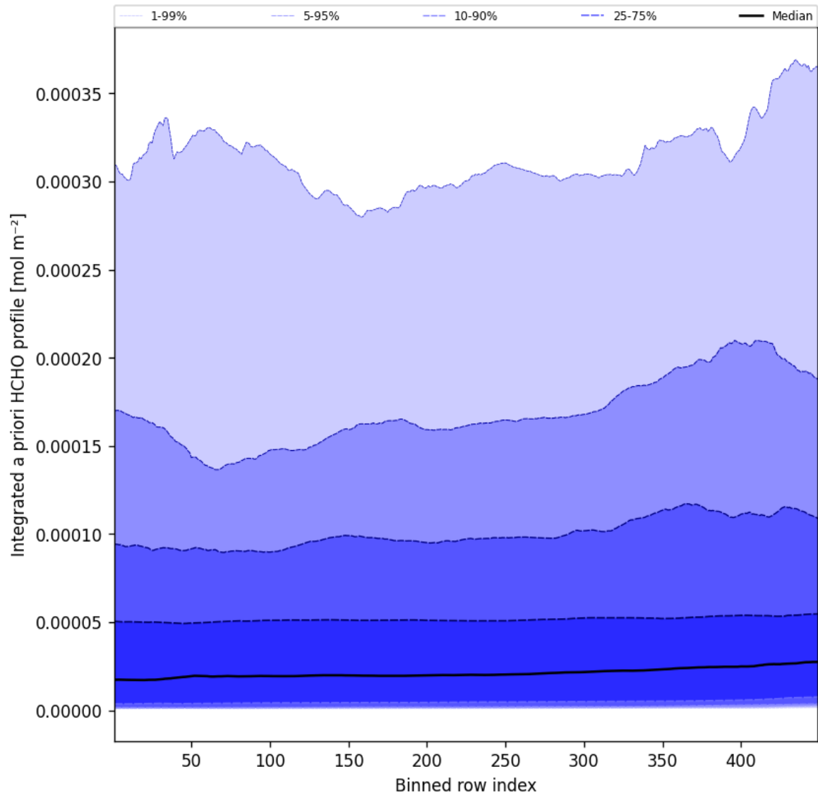
Figure 55: Along track statistics of "Integrated a priori HCHO profile" for 2025-02-11 to 2025-02-11
