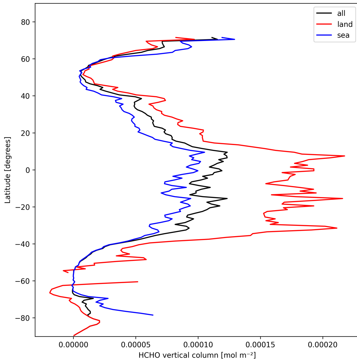
Figure 19: Zonal average of “HCHO vertical column” for 2025-02-11 to 2025-02-11.
