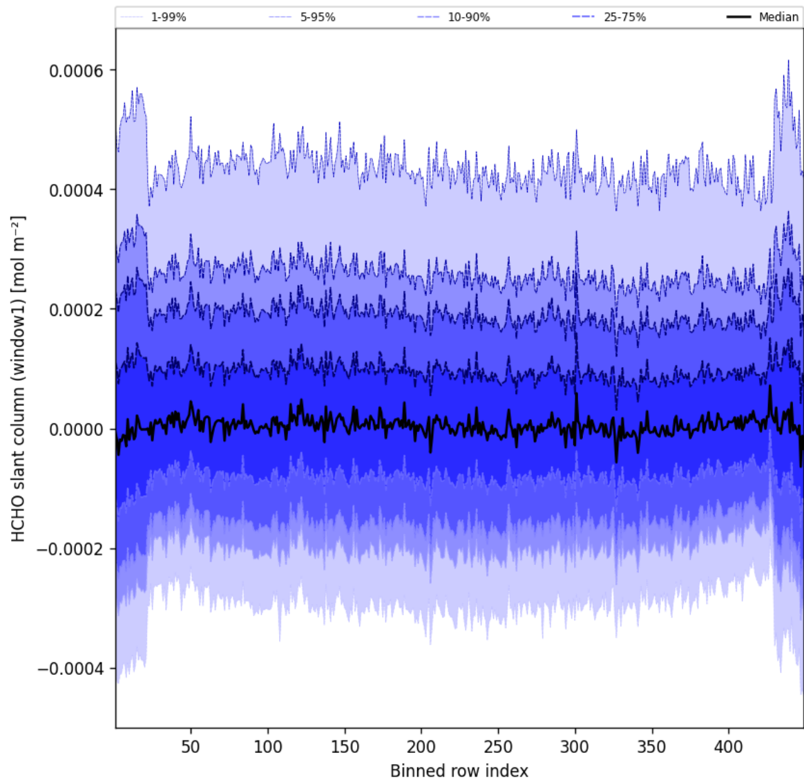
Figure 50: Along track statistics of “HCHO slant column (window1)” for 2025-02-11 to 2025-02-11
