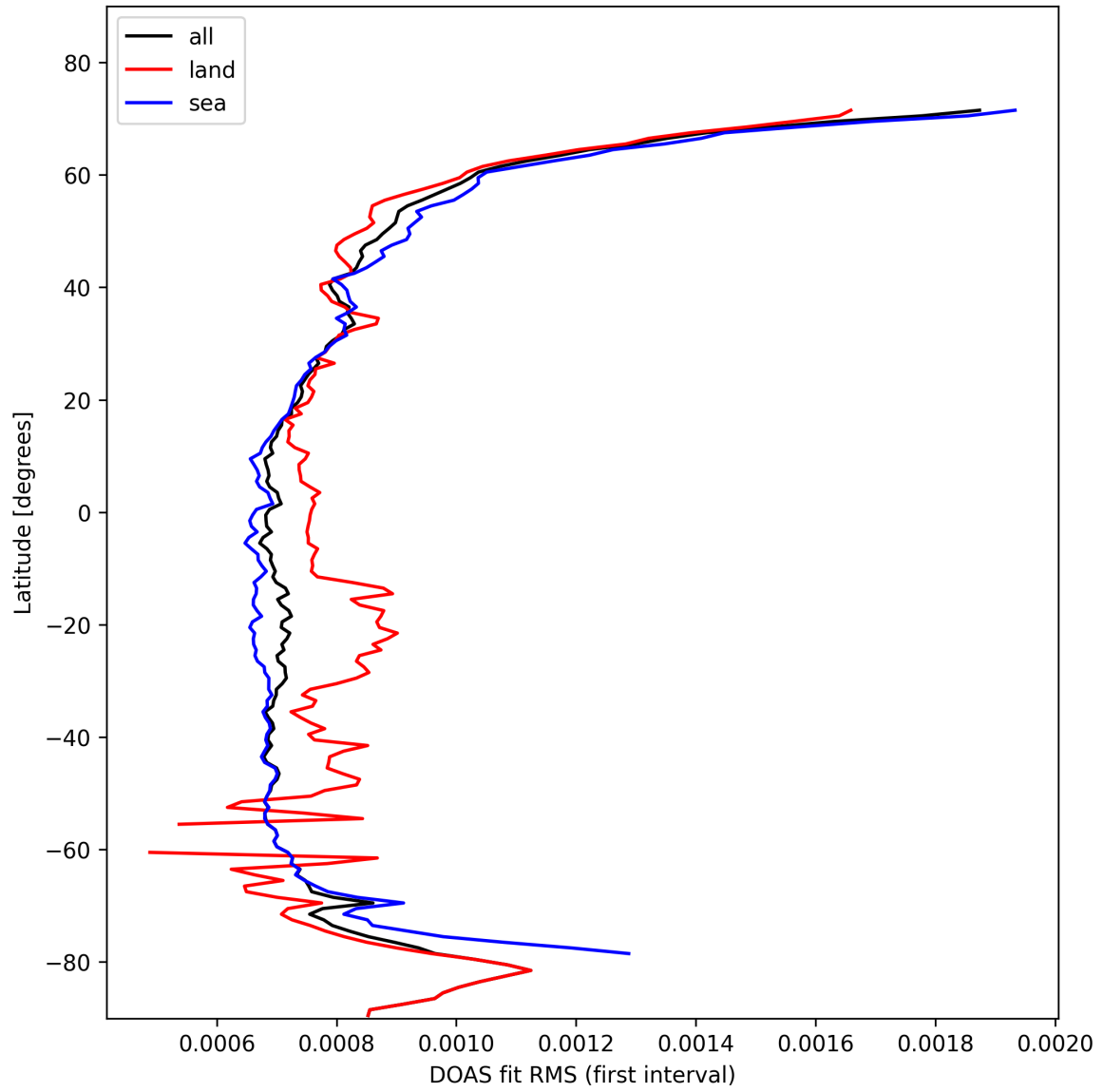
Figure 30: Zonal average of “DOAS fit RMS (first interval)” for 2025-02-11 to 2025-02-11.
