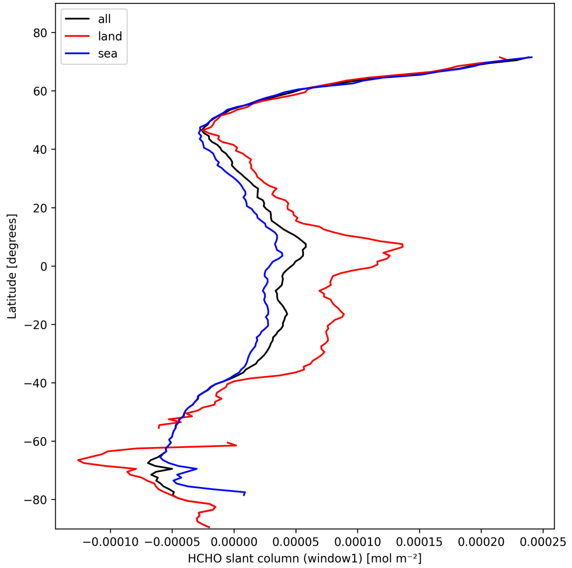
Figure 22: Zonal average of “HCHO slant column (window1)” for 2025-02-11 to 2025-02-11.
