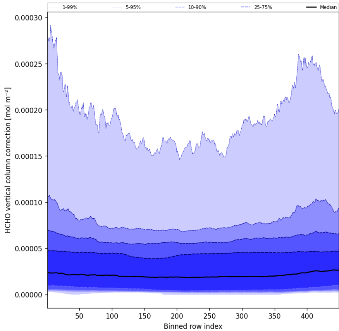
Figure 49: Along track statistics of “HCHO vertical column correction” for 2025-02-11 to 2025-02-11
