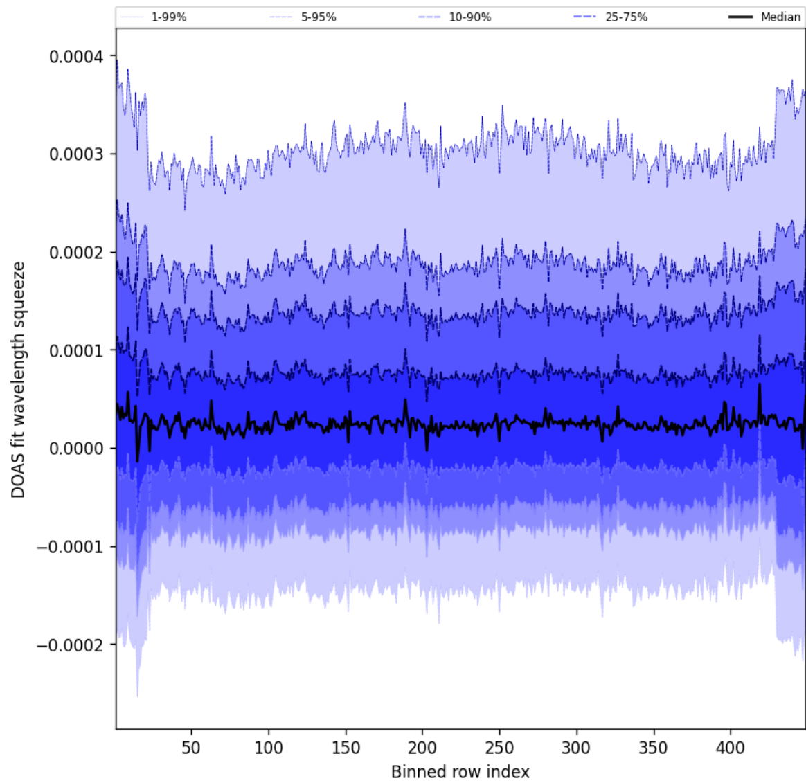
Figure 57: Along track statistics of “DOAS fit wavelength squeeze” for 2025-02-11 to 2025-02-11
