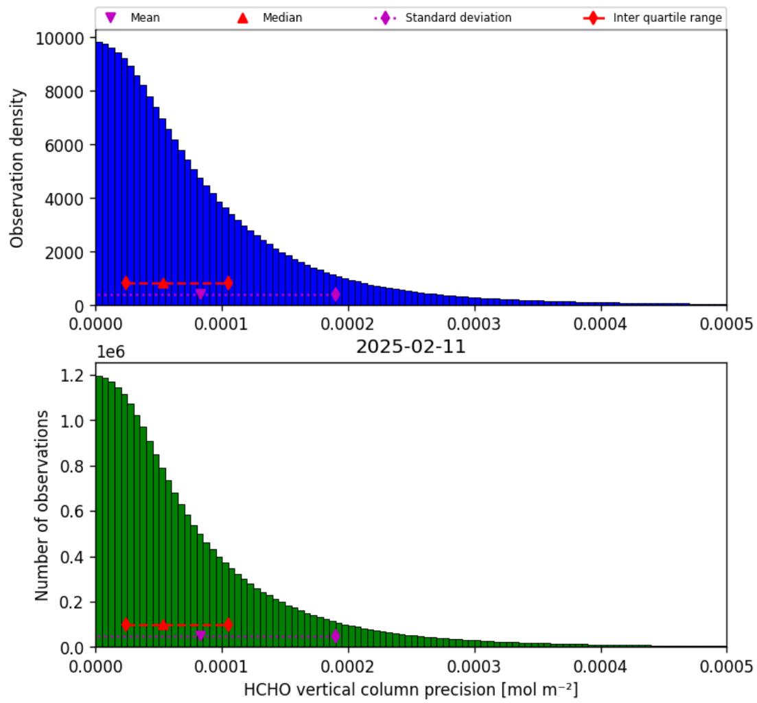
Figure 34: Histogram of “HCHO vertical column precision” for 2025-02-11 to 2025-02-11
