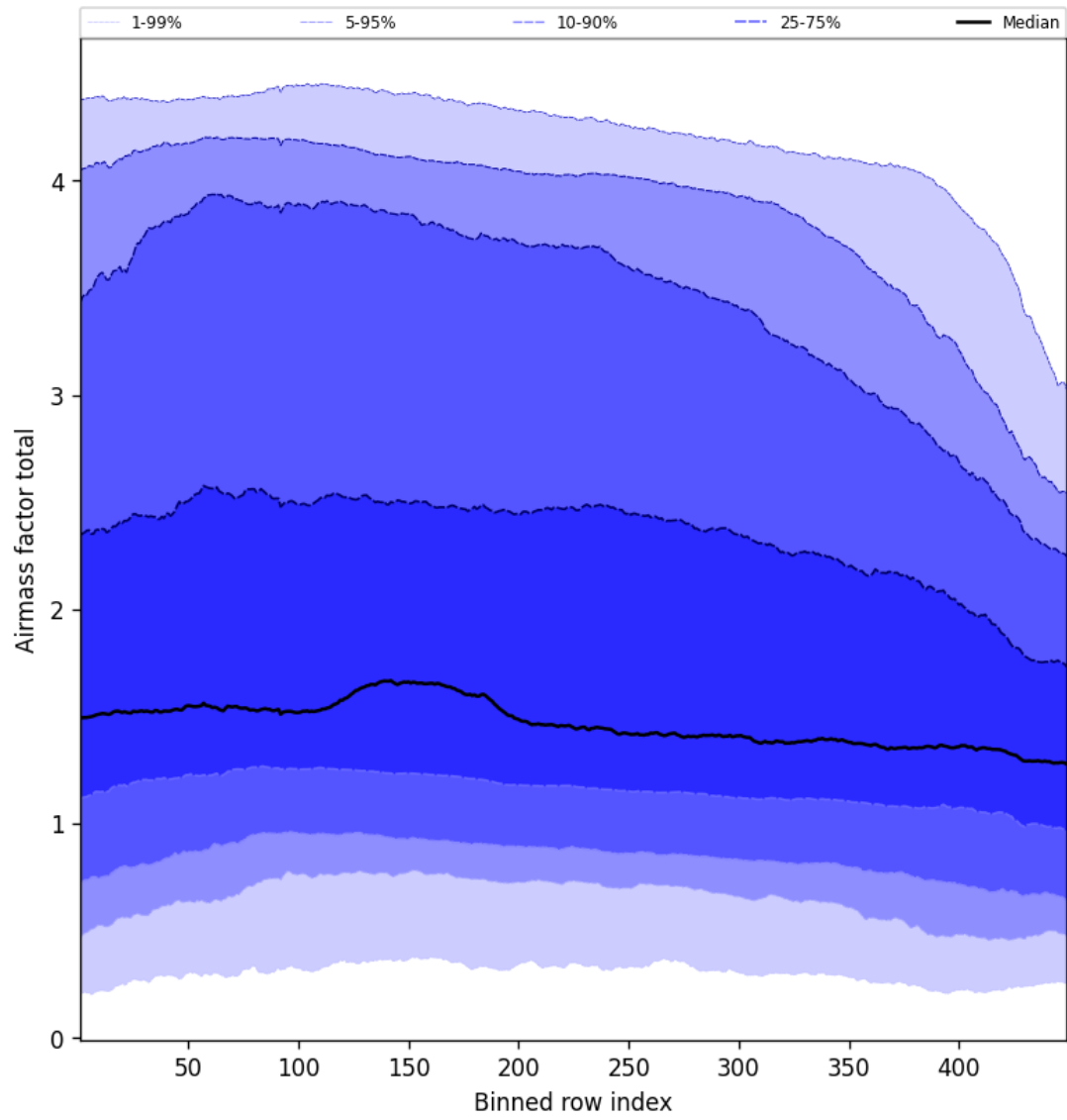
Figure 52: Along track statistics of “Airmass factor total” for 2025-02-11 to 2025-02-11
