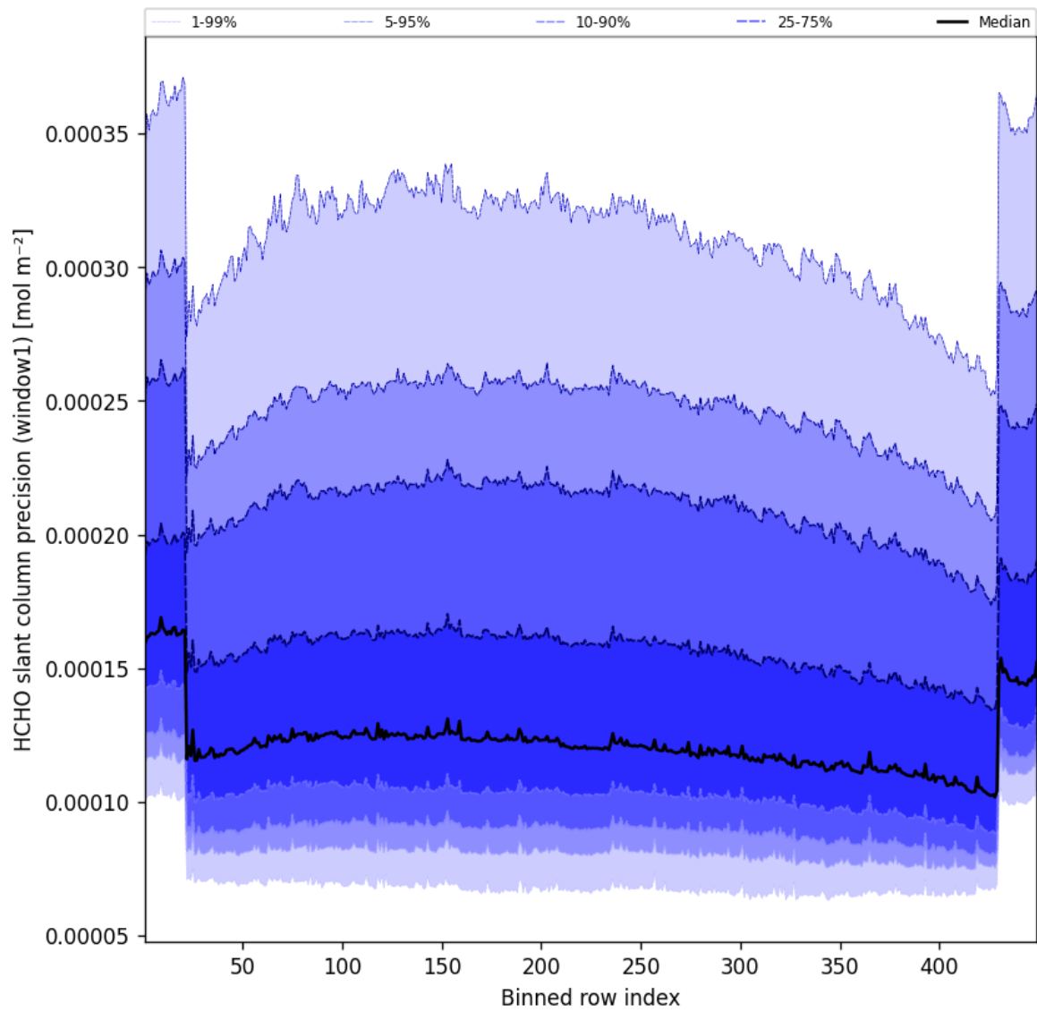
Figure 51: Along track statistics of “HCHO slant column precision (window1)” for 2025-02-11 to 2025-02-11
