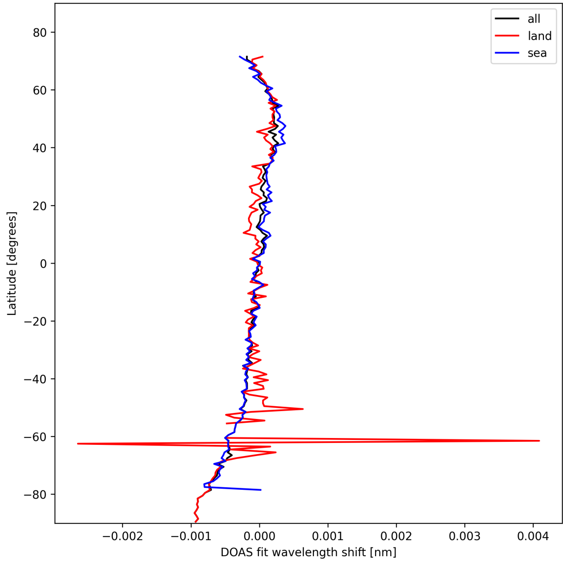
Figure 28: Zonal average of “DOAS fit wavelength shift” for 2025-02-11 to 2025-02-11.
