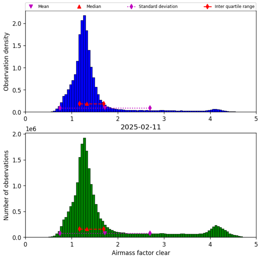
Figure 40: Histogram of “Airmass factor clear” for 2025-02-11 to 2025-02-11
