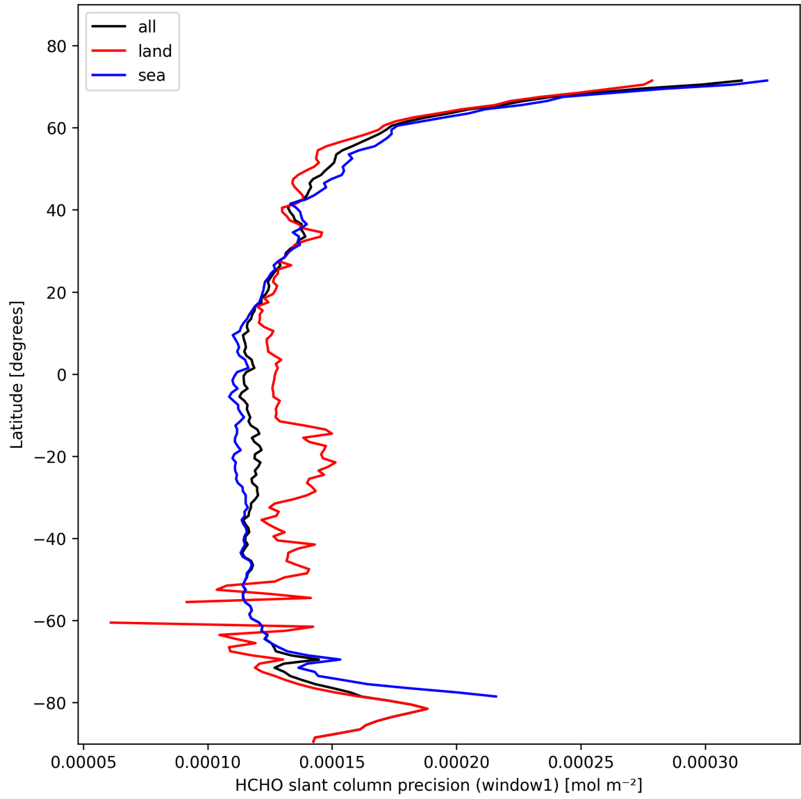
Figure 23: Zonal average of “HCHO slant column precision (window1)” for 2025-02-11 to 2025-02-11.
