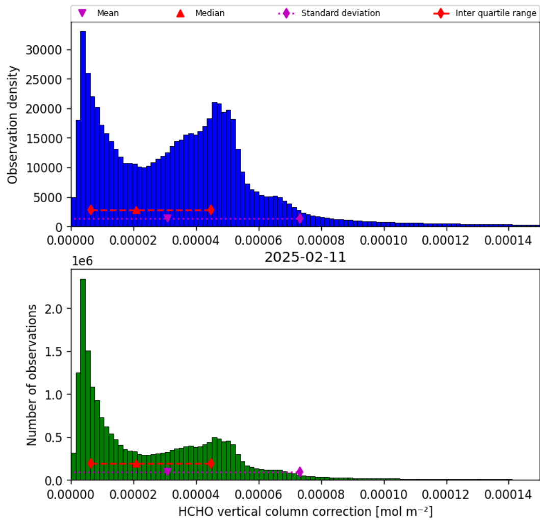
Figure 35: Histogram of “HCHO vertical column correction” for 2025-02-11 to 2025-02-11
