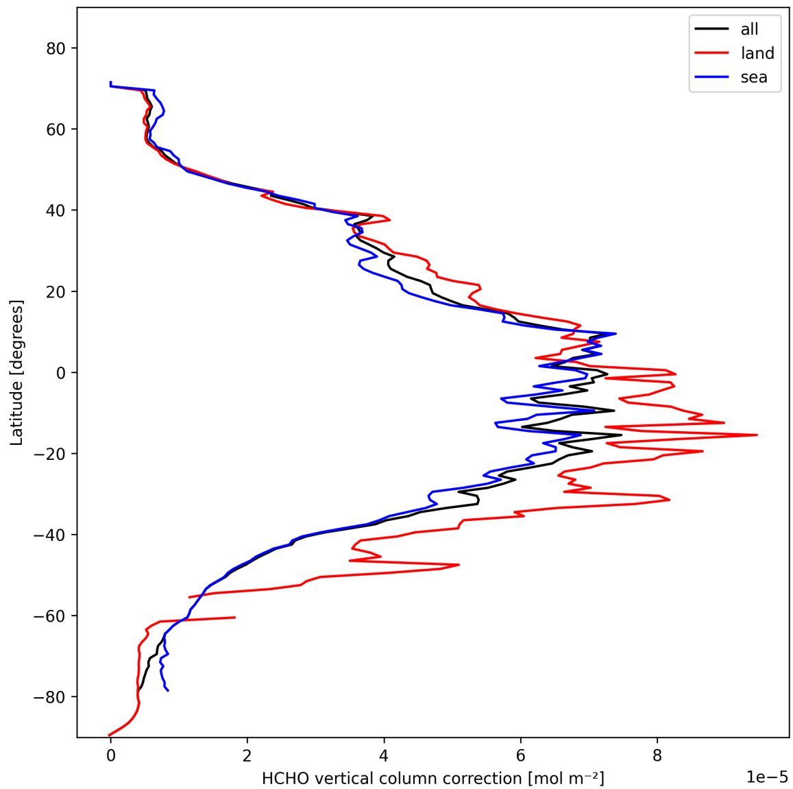
Figure 21: Zonal average of “HCHO vertical column correction” for 2025-02-11 to 2025-02-11.
