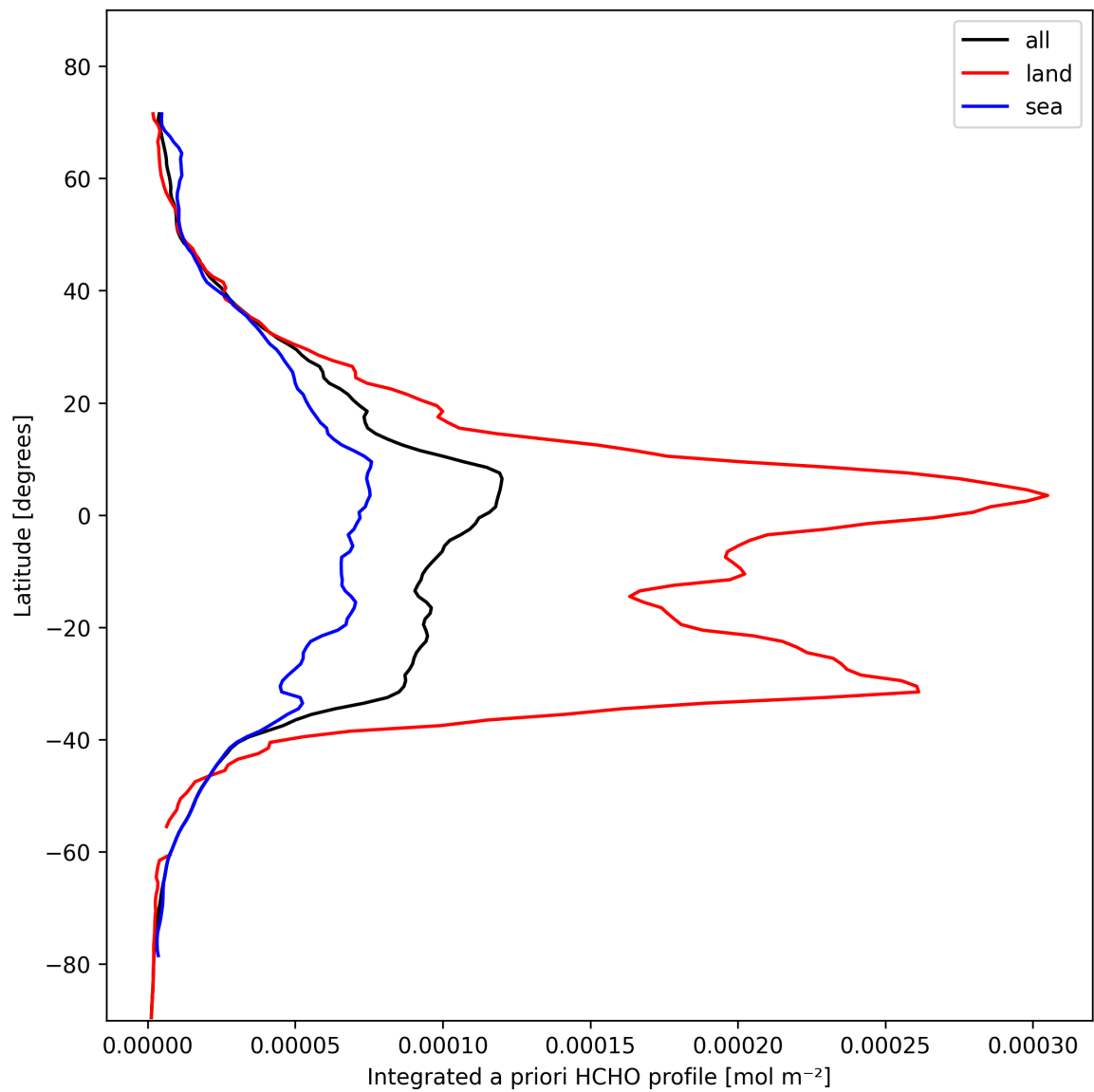
Figure 27: Zonal average of “Integrated a priori HCHO profile” for 2025-02-11 to 2025-02-11.
