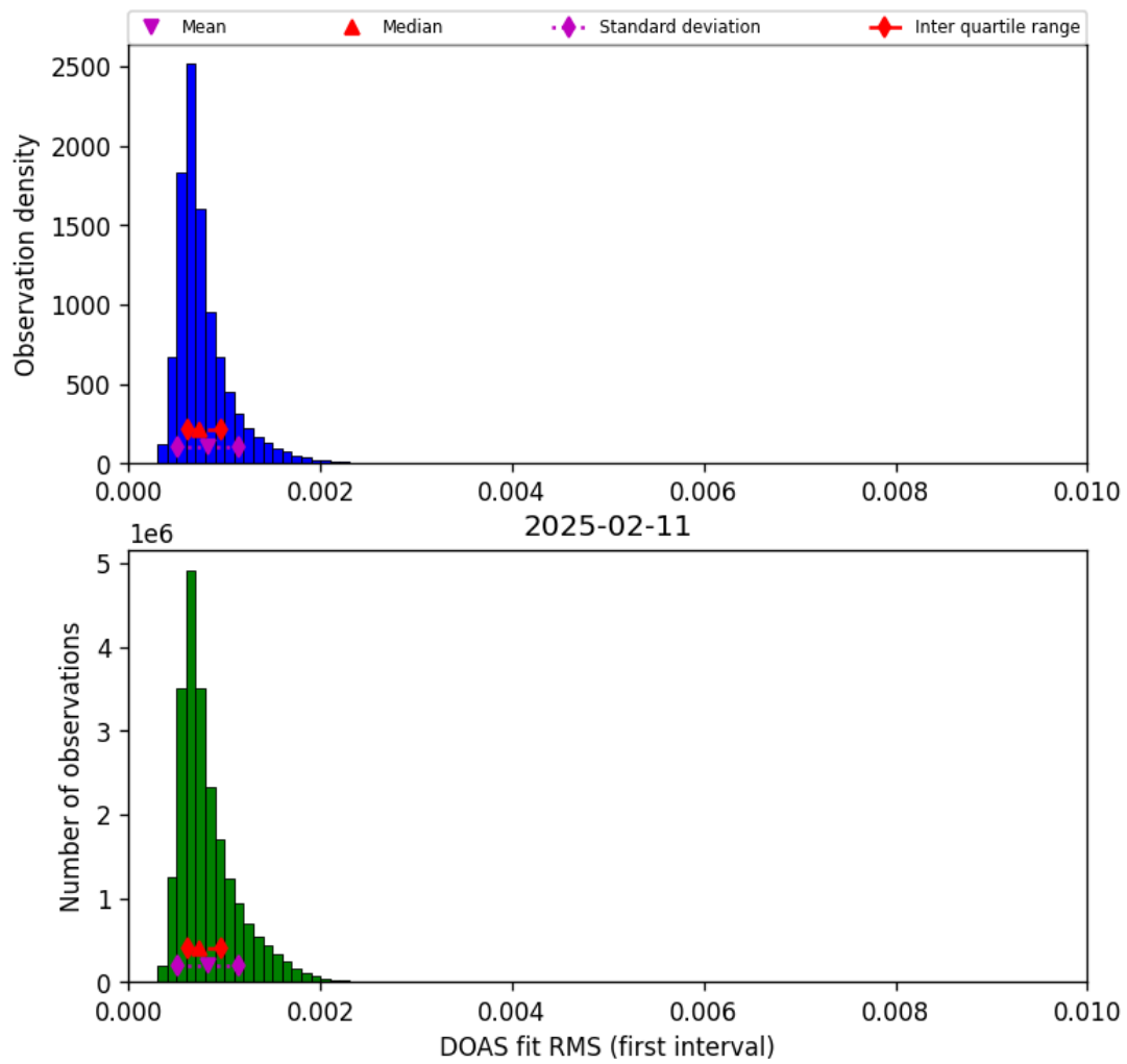
Figure 44: Histogram of “DOAS fit RMS (first interval)” for 2025-02-11 to 2025-02-11
