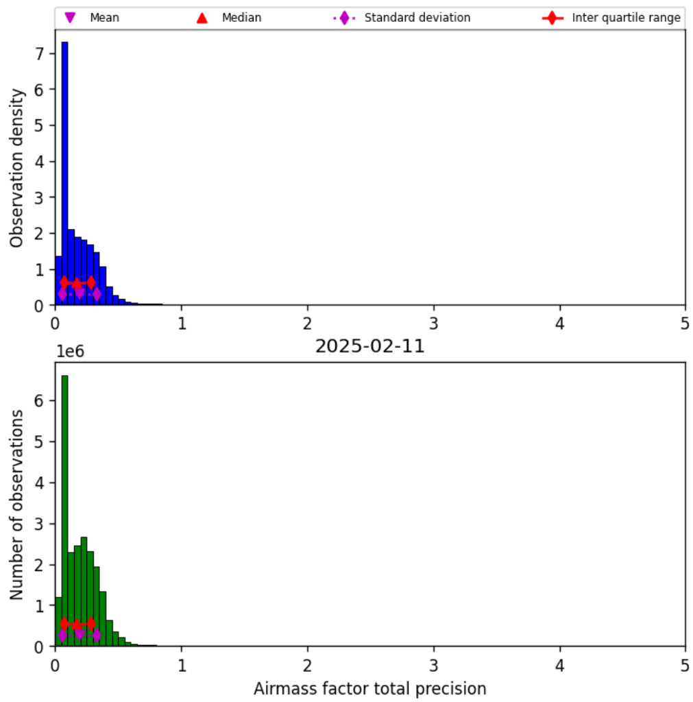
Figure 39: Histogram of “Airmass factor total precision” for 2025-02-11 to 2025-02-11
