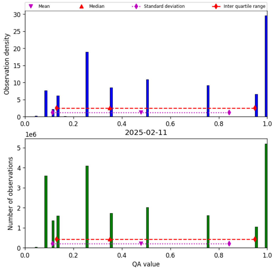
Figure 32: Histogram of “QA value” for 2025-02-11 to 2025-02-11
