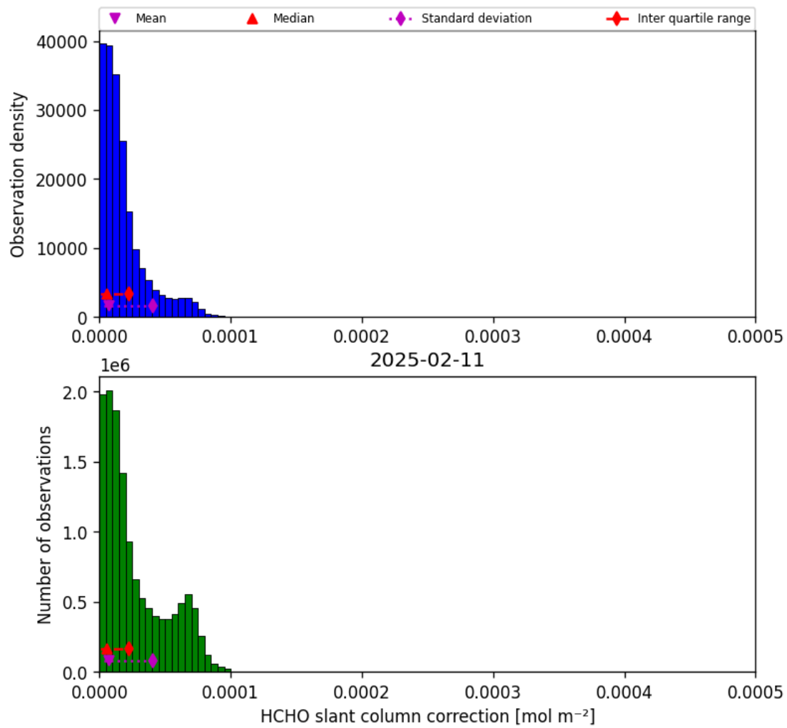
Figure 45: Histogram of “HCHO slant column correction” for 2025-02-11 to 2025-02-11
