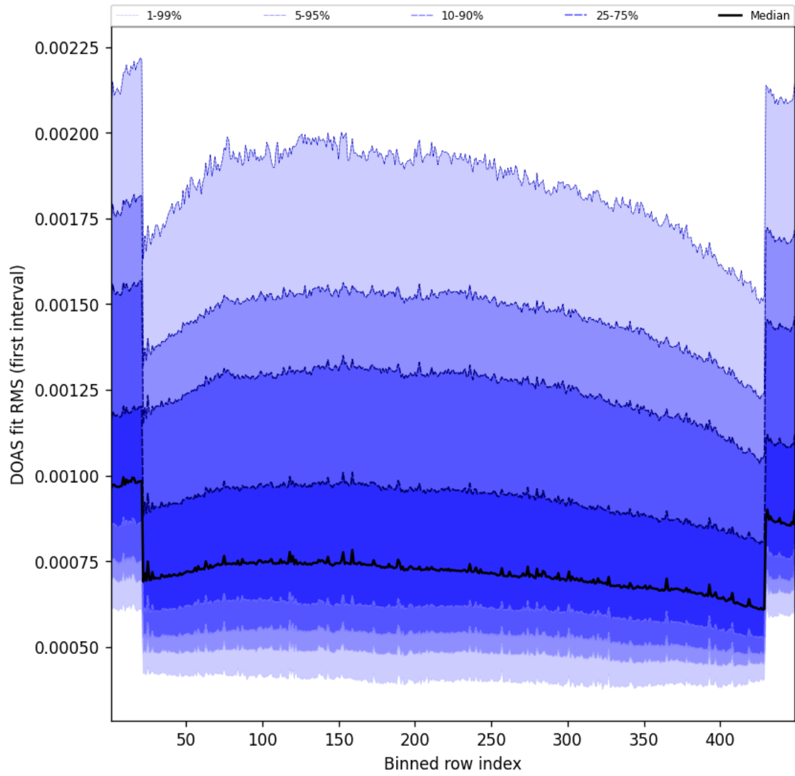
Figure 58: Along track statistics of “DOAS fit RMS (first interval)” for 2025-02-11 to 2025-02-11
