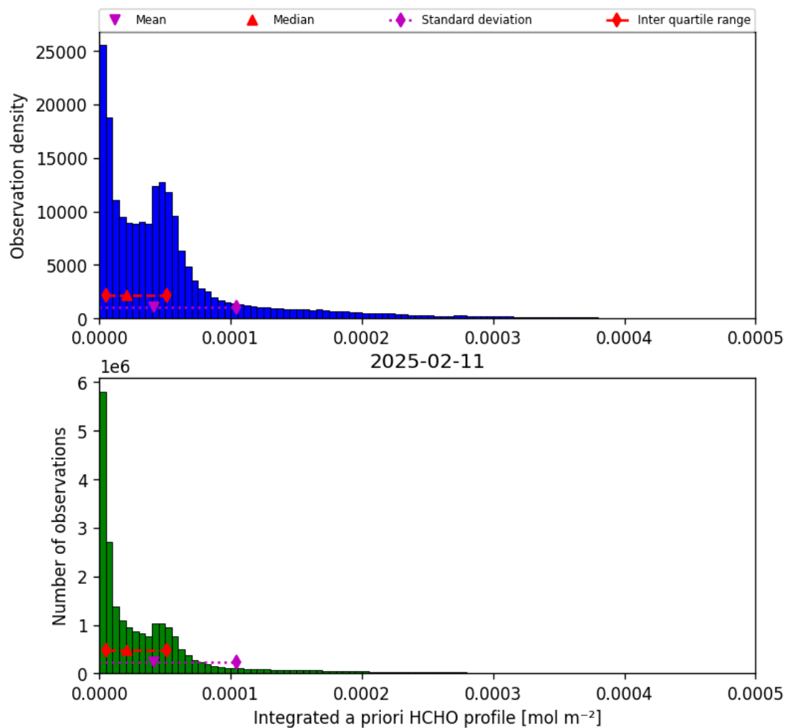
Figure 41: Histogram of “Integrated a priori HCHO profile” for 2025-02-11 to 2025-02-11
