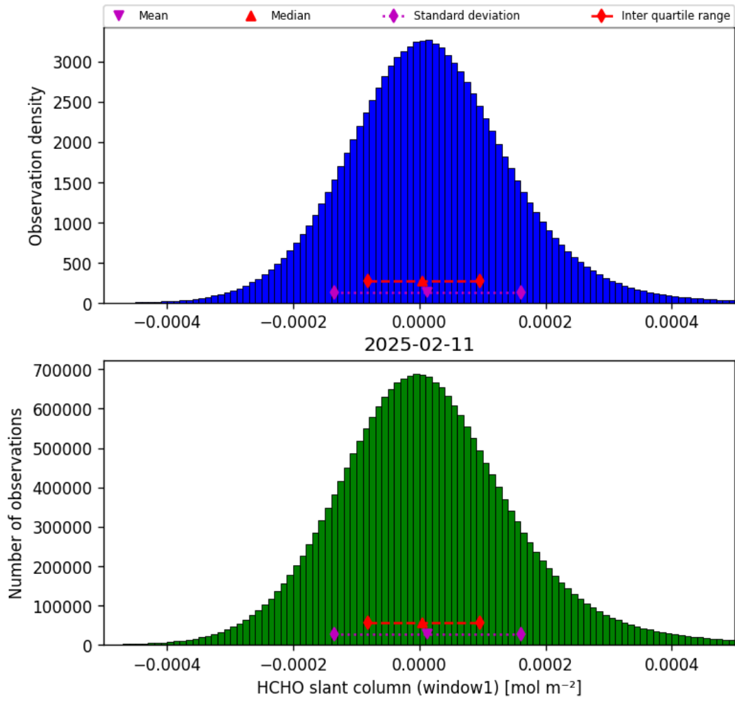
Figure 36: Histogram of “HCHO slant column (window1)” for 2025-02-11 to 2025-02-11
