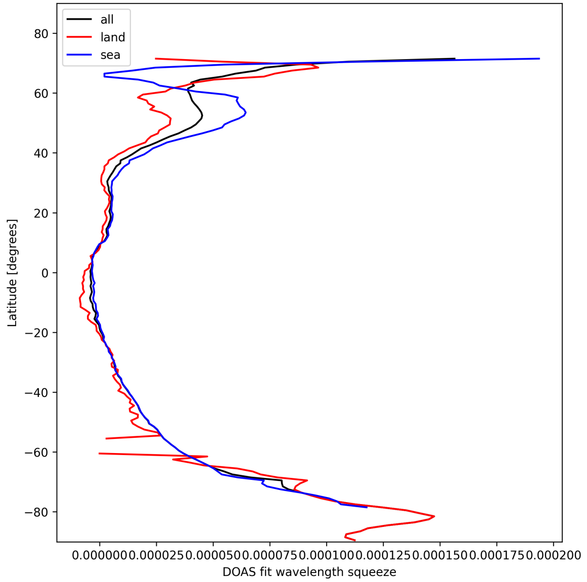
Figure 29: Zonal average of “DOAS fit wavelength squeeze” for 2025-02-11 to 2025-02-11.
