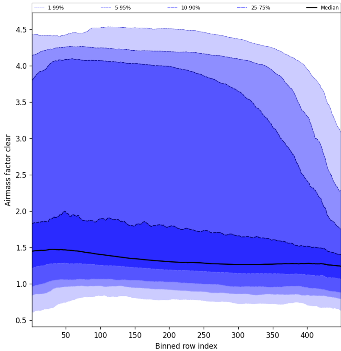
Figure 54: Along track statistics of “Airmass factor clear” for 2025-02-11 to 2025-02-11
