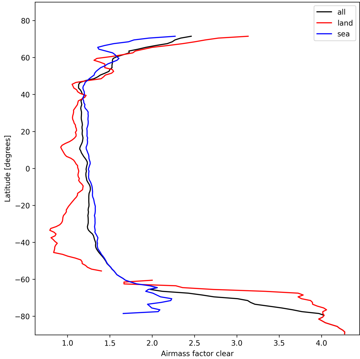
Figure 26: Zonal average of “Airmass factor clear” for 2025-02-11 to 2025-02-11.
