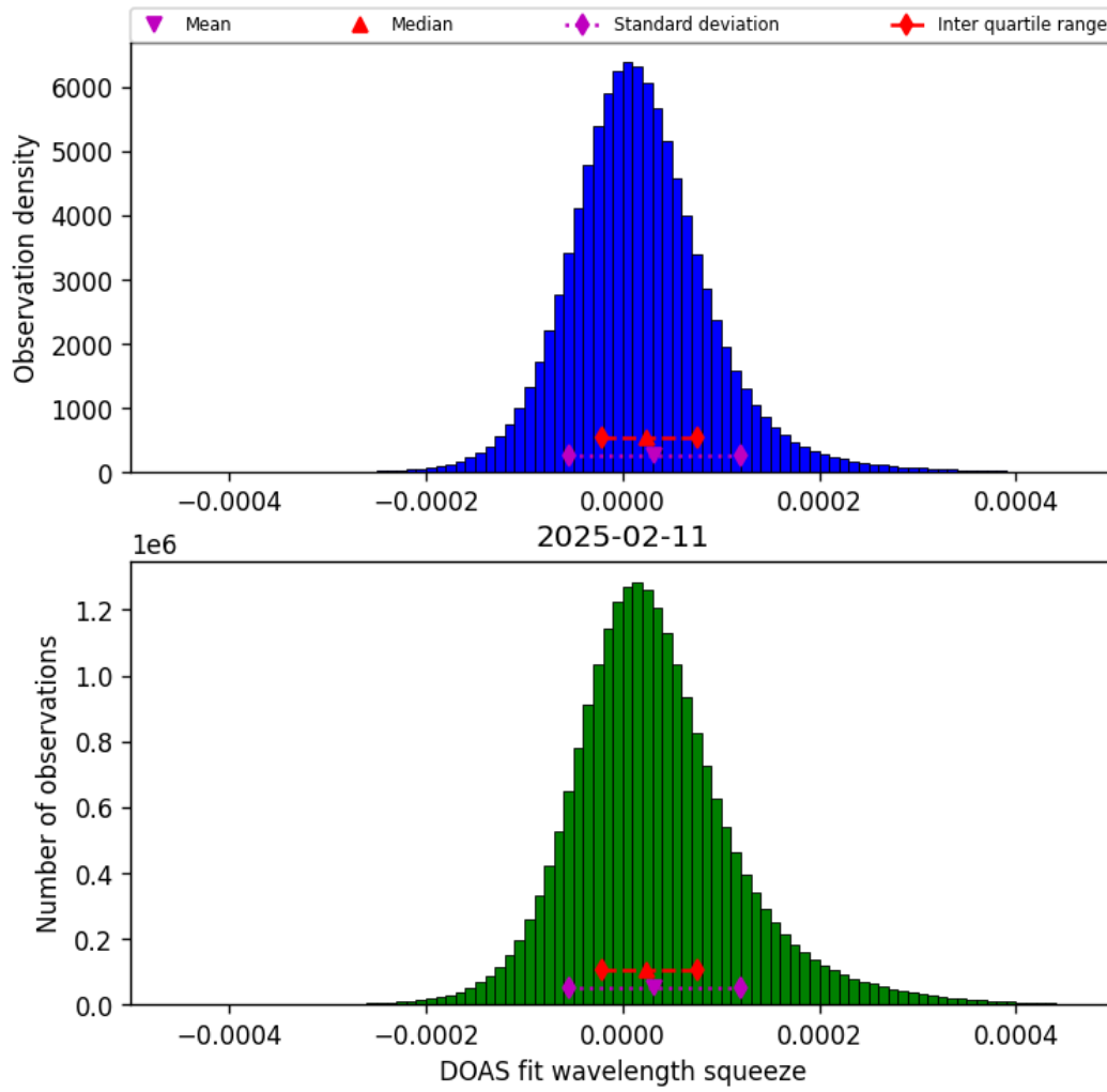
Figure 43: Histogram of “DOAS fit wavelength squeeze” for 2025-02-11 to 2025-02-11
