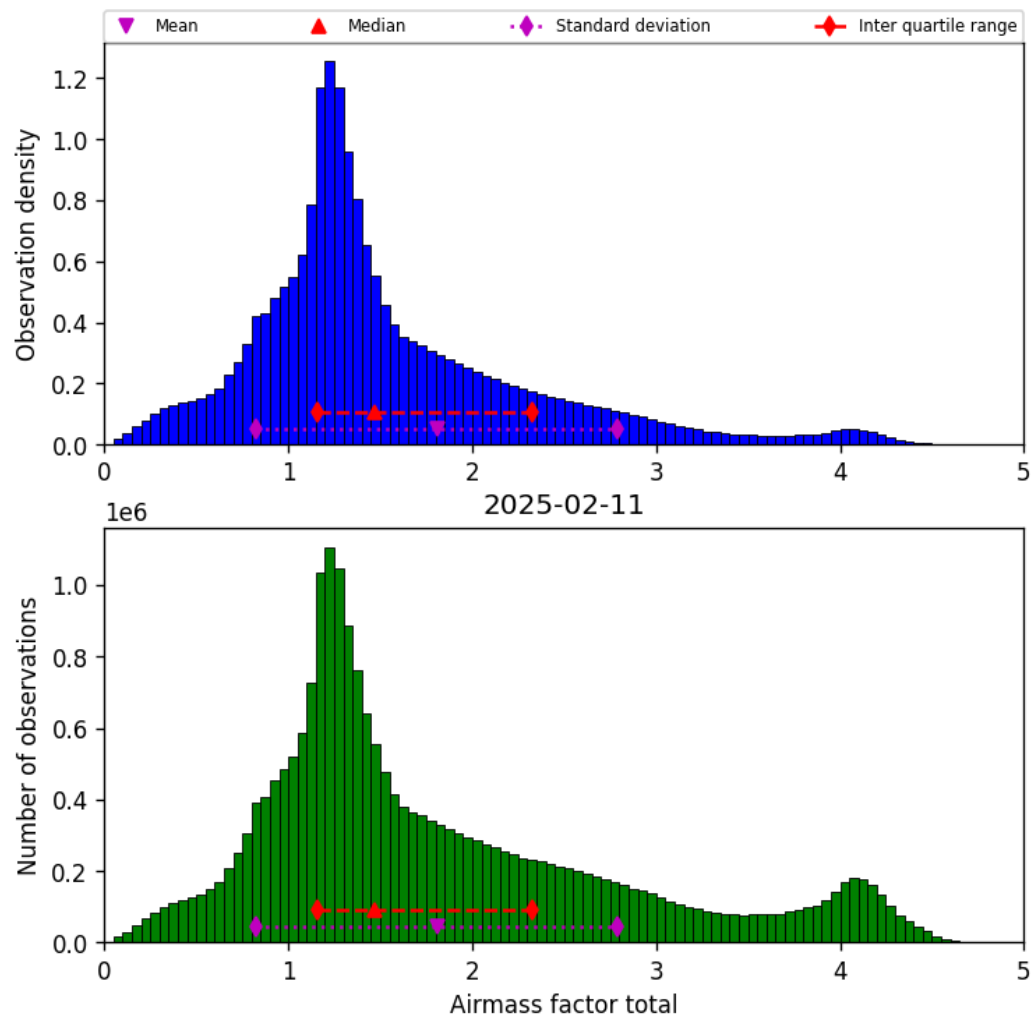
Figure 38: Histogram of “Airmass factor total” for 2025-02-11 to 2025-02-11
