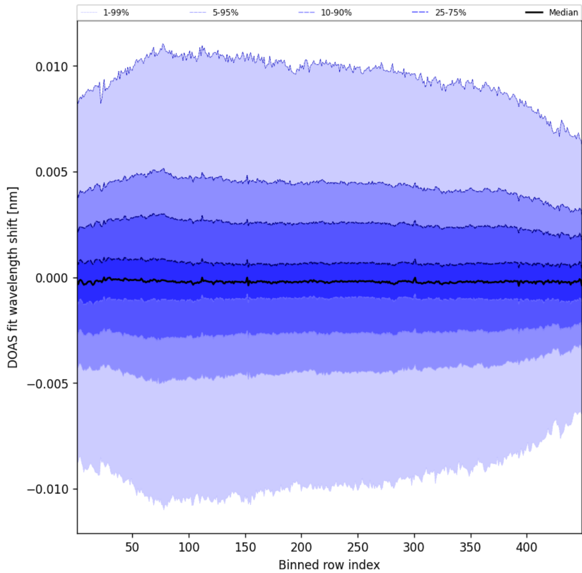
Figure 56: Along track statistics of “DOAS fit wavelength shift” for 2025-02-11 to 2025-02-11
