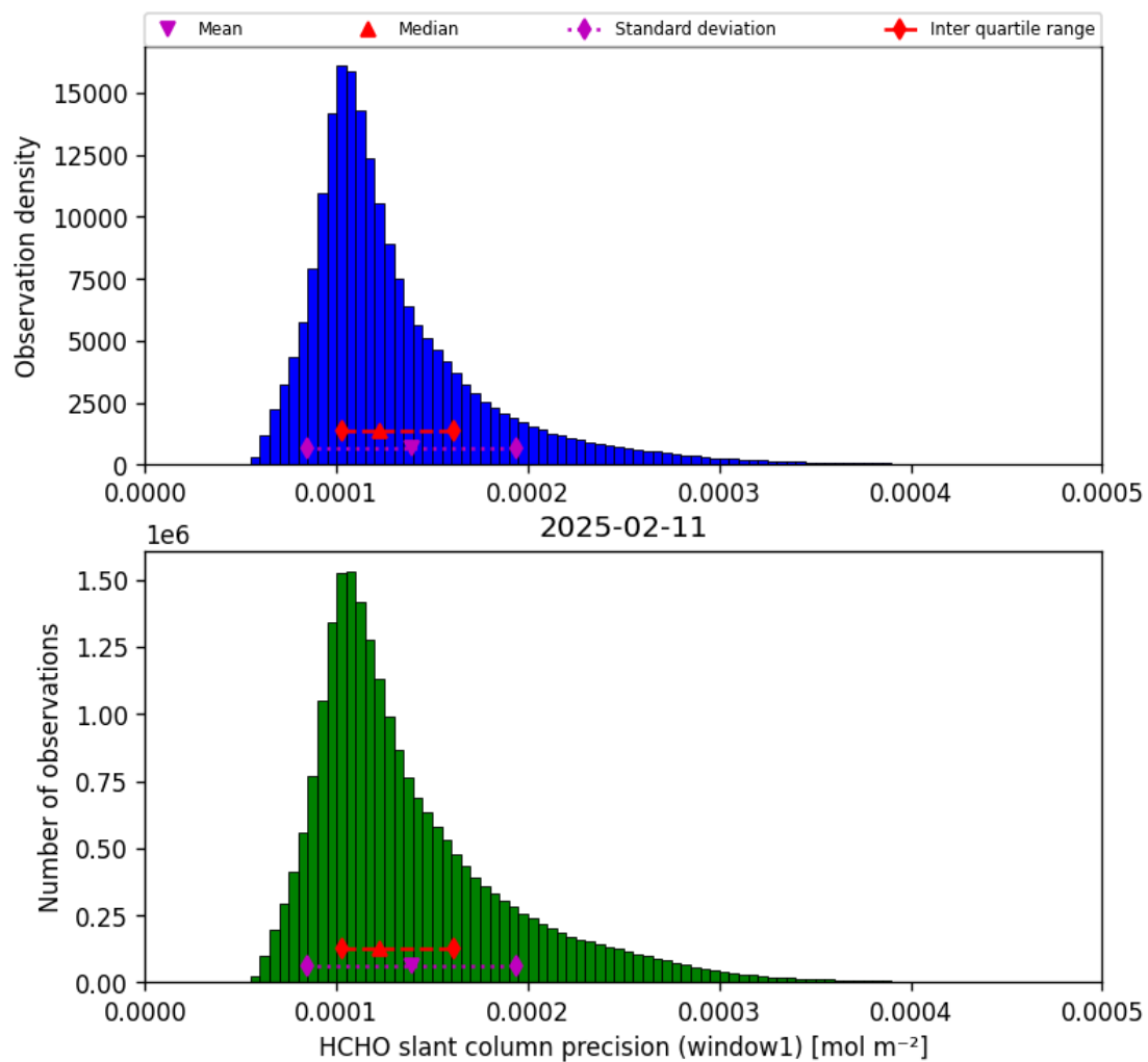
Figure 37: Histogram of “HCHO slant column precision (window1)” for 2025-02-11 to 2025-02-11
