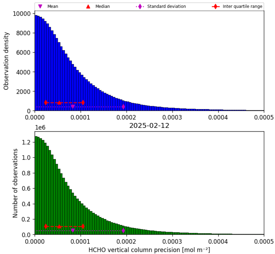
Figure 34: Histogram of “HCHO vertical column precision” for 2025-02-12 to 2025-02-13
