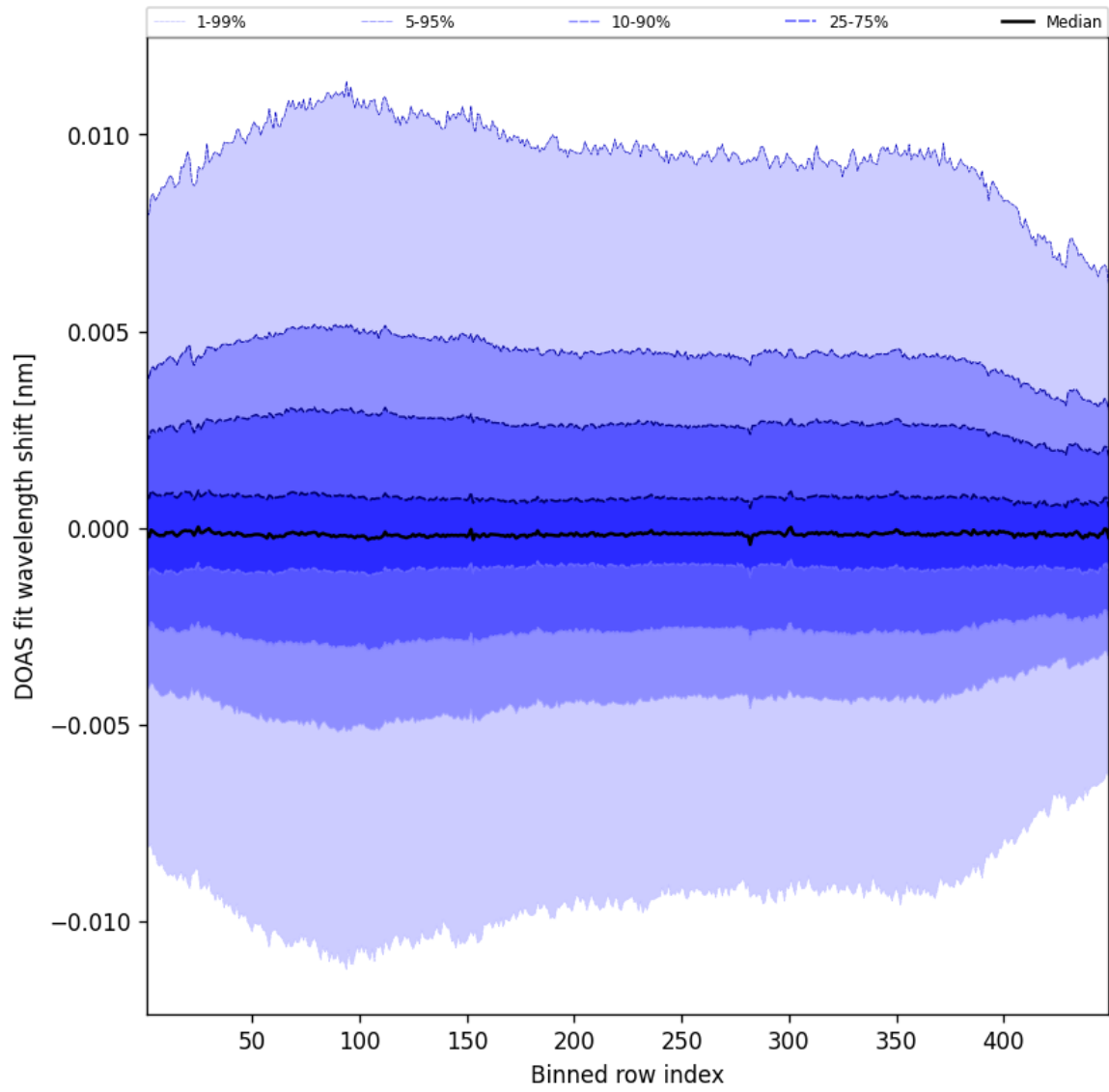
Figure 56: Along track statistics of “DOAS fit wavelength shift” for 2025-02-12 to 2025-02-13
