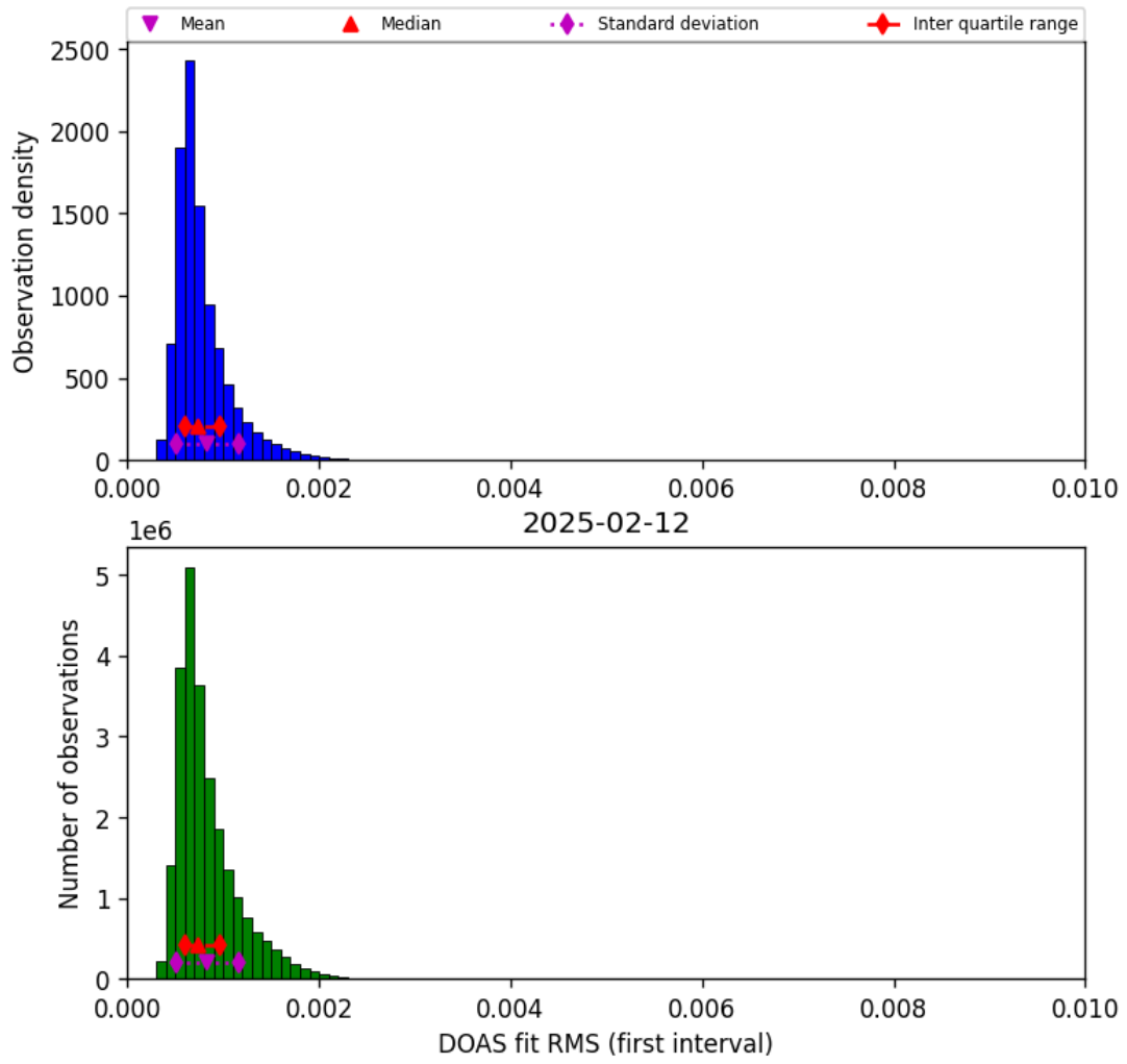
Figure 44: Histogram of “DOAS fit RMS (first interval)” for 2025-02-12 to 2025-02-13
