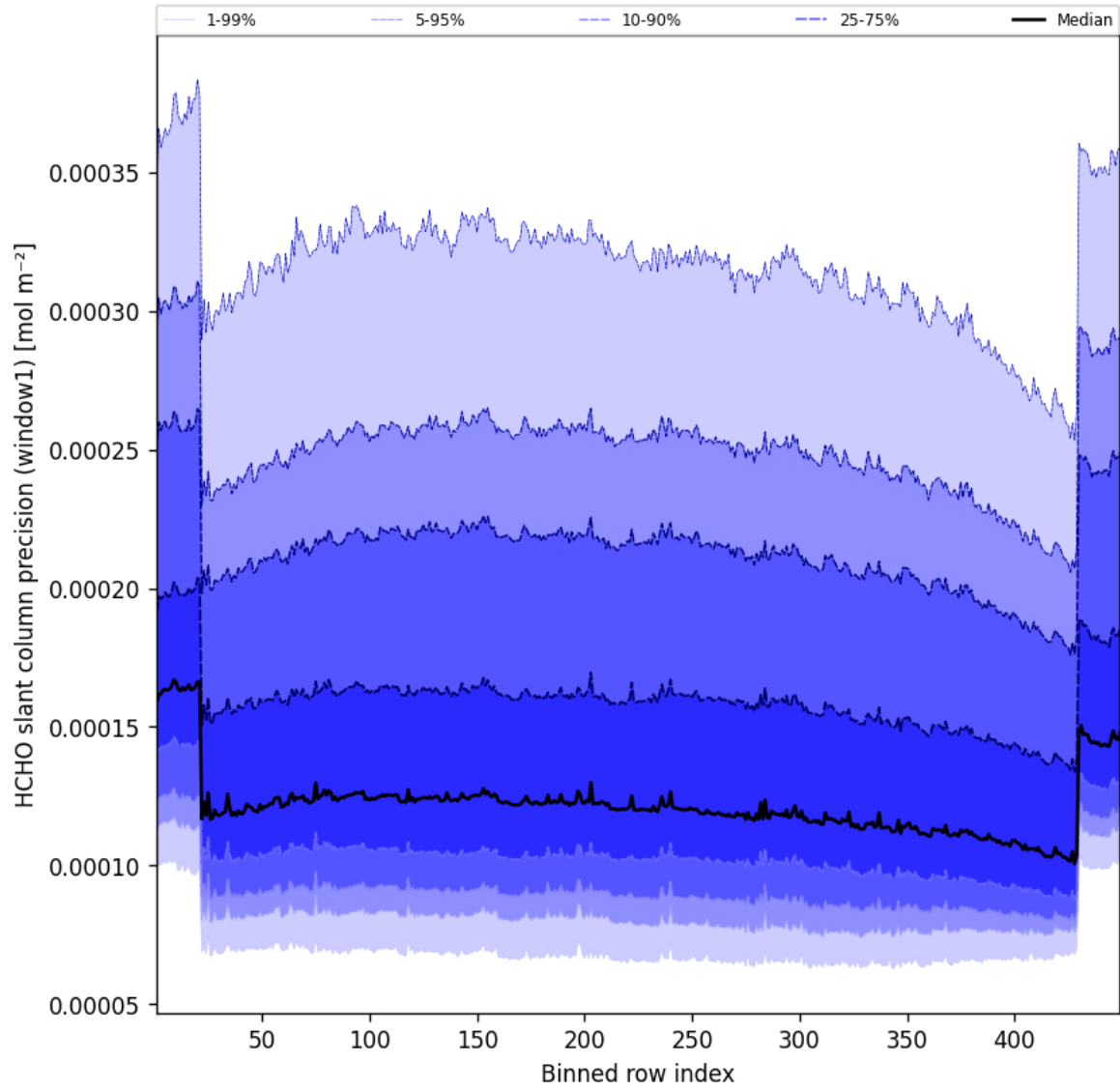
Figure 51: Along track statistics of “HCHO slant column precision (window1)” for 2025-02-12 to 2025-02-13
