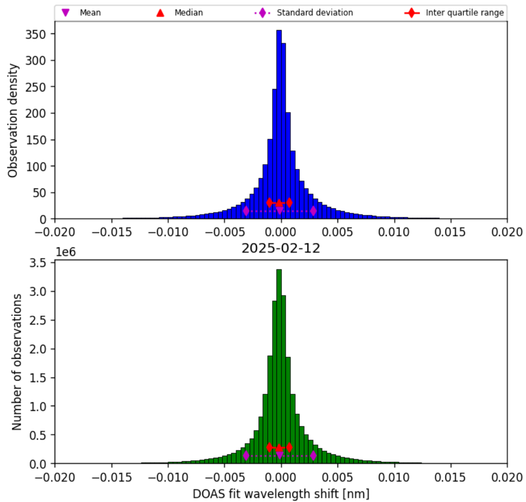
Figure 42: Histogram of “DOAS fit wavelength shift” for 2025-02-12 to 2025-02-13
