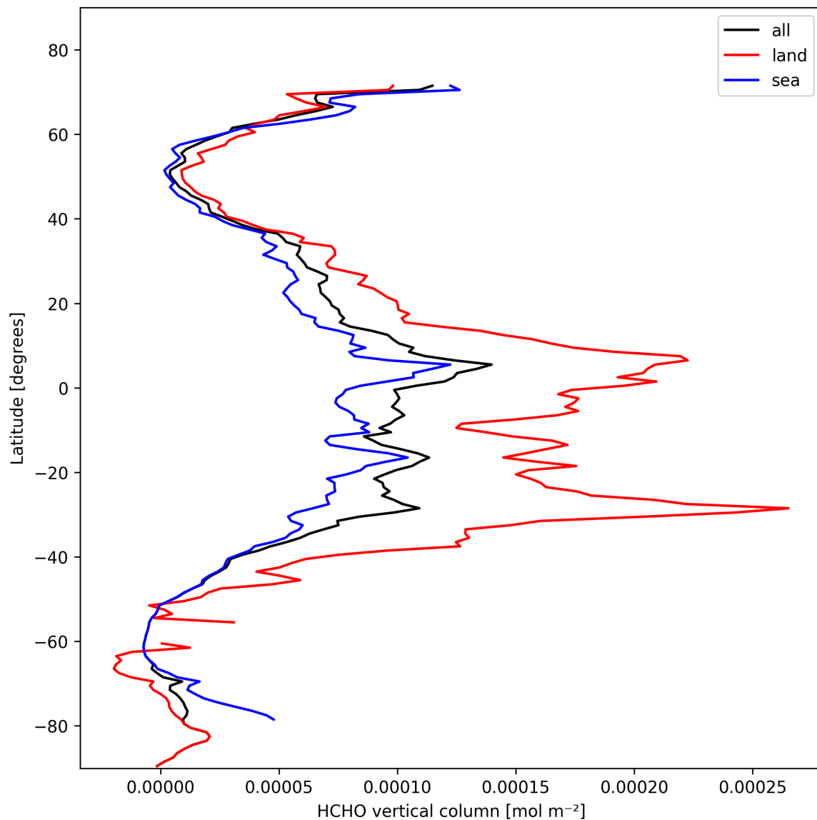
Figure 19: Zonal average of “HCHO vertical column” for 2025-02-12 to 2025-02-13.
