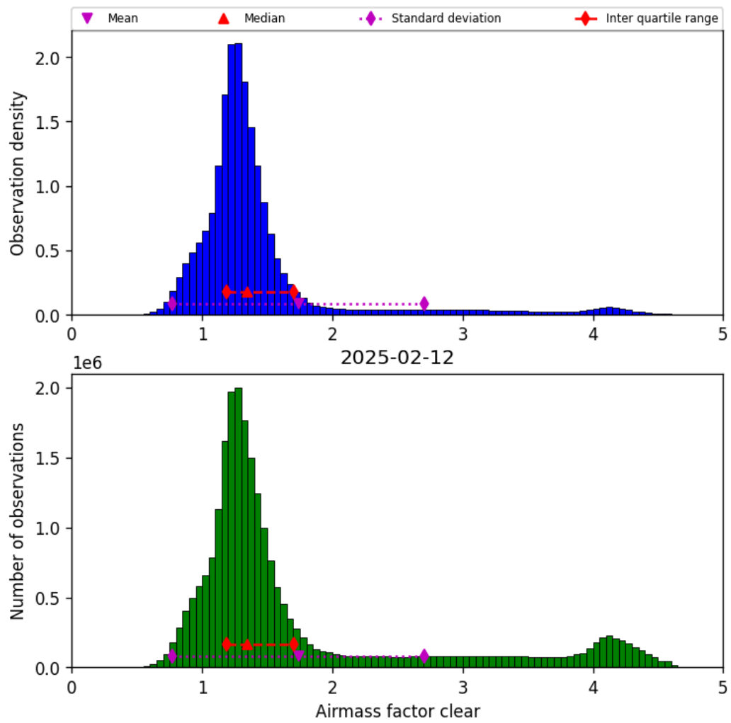
Figure 40: Histogram of “Airmass factor clear” for 2025-02-12 to 2025-02-13
