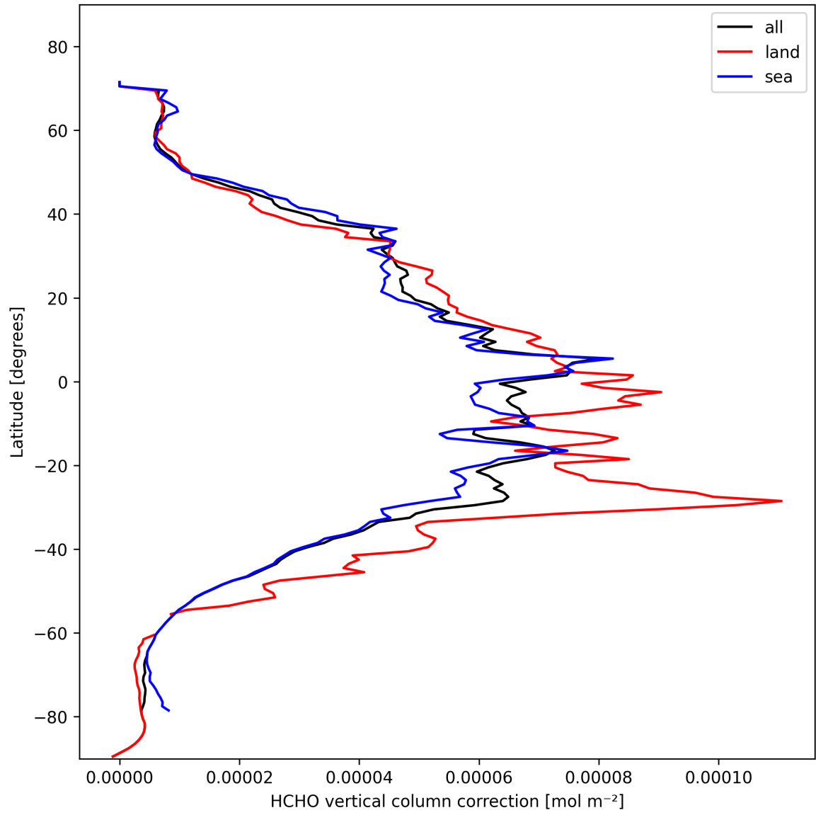
Figure 21: Zonal average of “HCHO vertical column correction” for 2025-02-12 to 2025-02-13.
