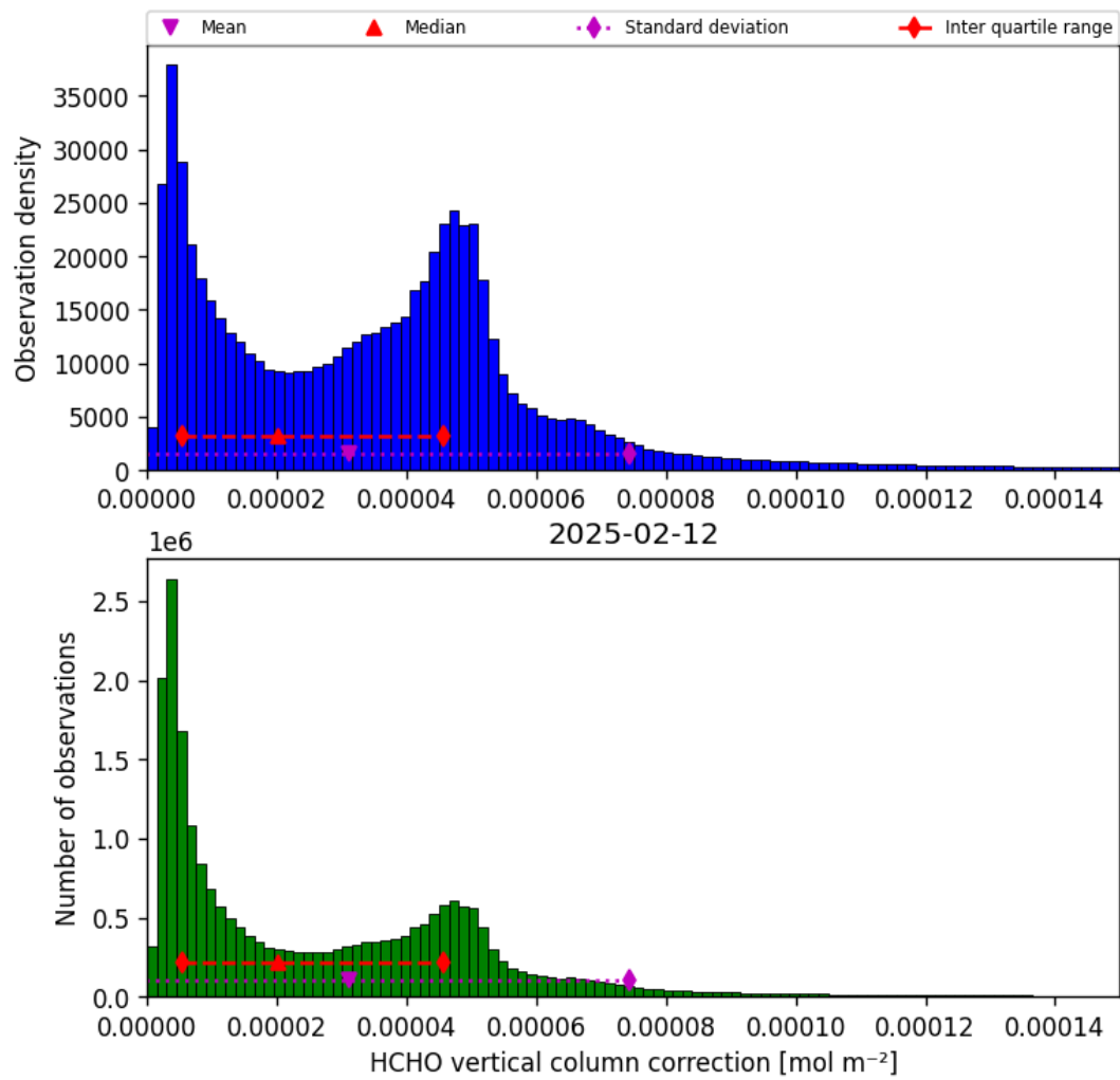
Figure 35: Histogram of “HCHO vertical column correction” for 2025-02-12 to 2025-02-13
