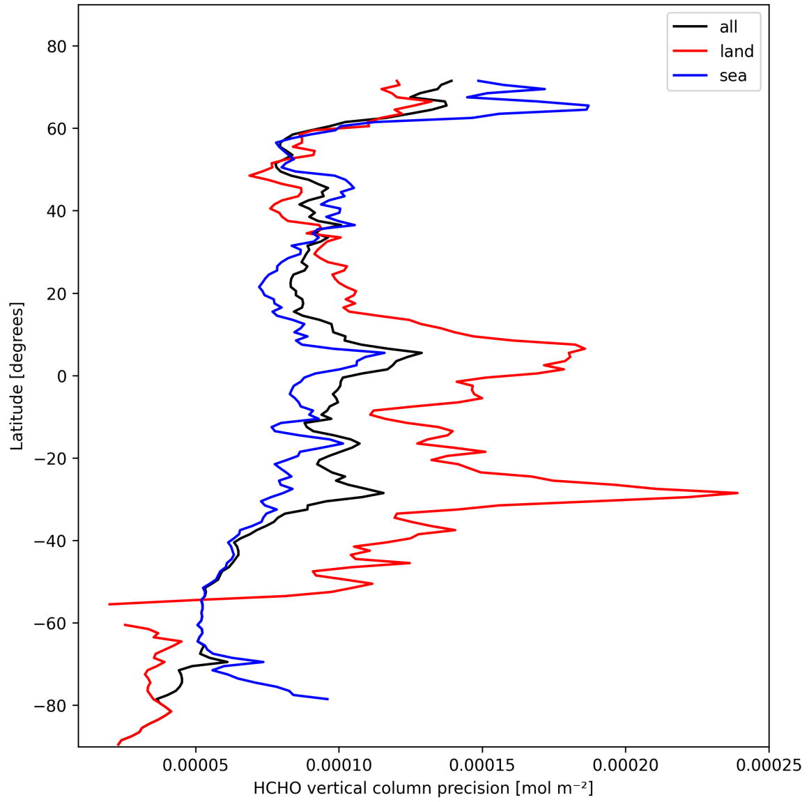
Figure 20: Zonal average of "HCHO vertical column precision" for 2025-02-12 to 2025-02-13.
