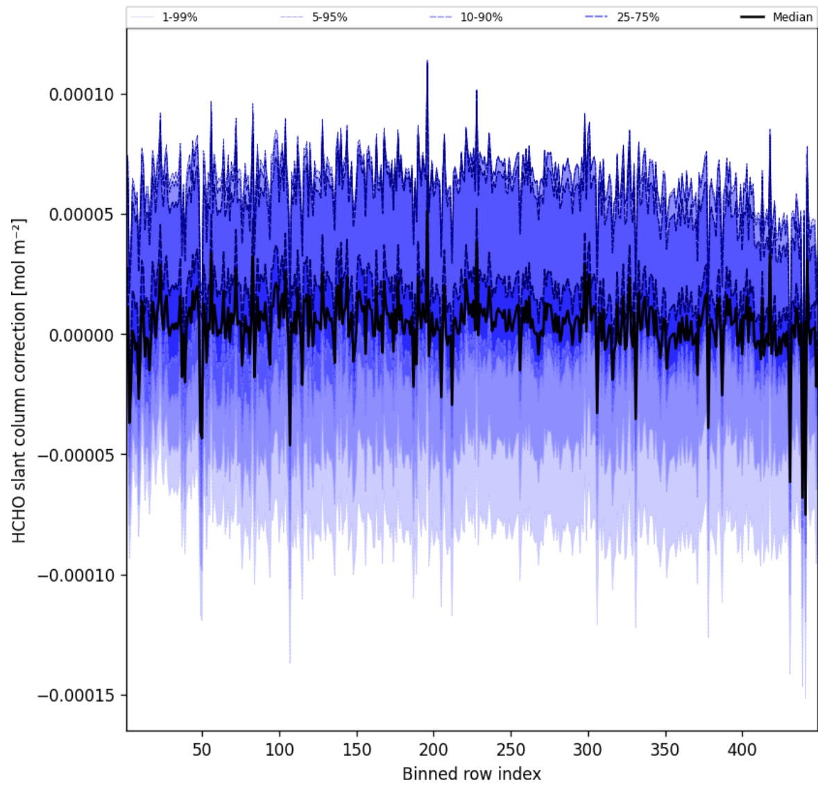
Figure 59: Along track statistics of “HCHO slant column correction” for 2025-02-12 to 2025-02-13
