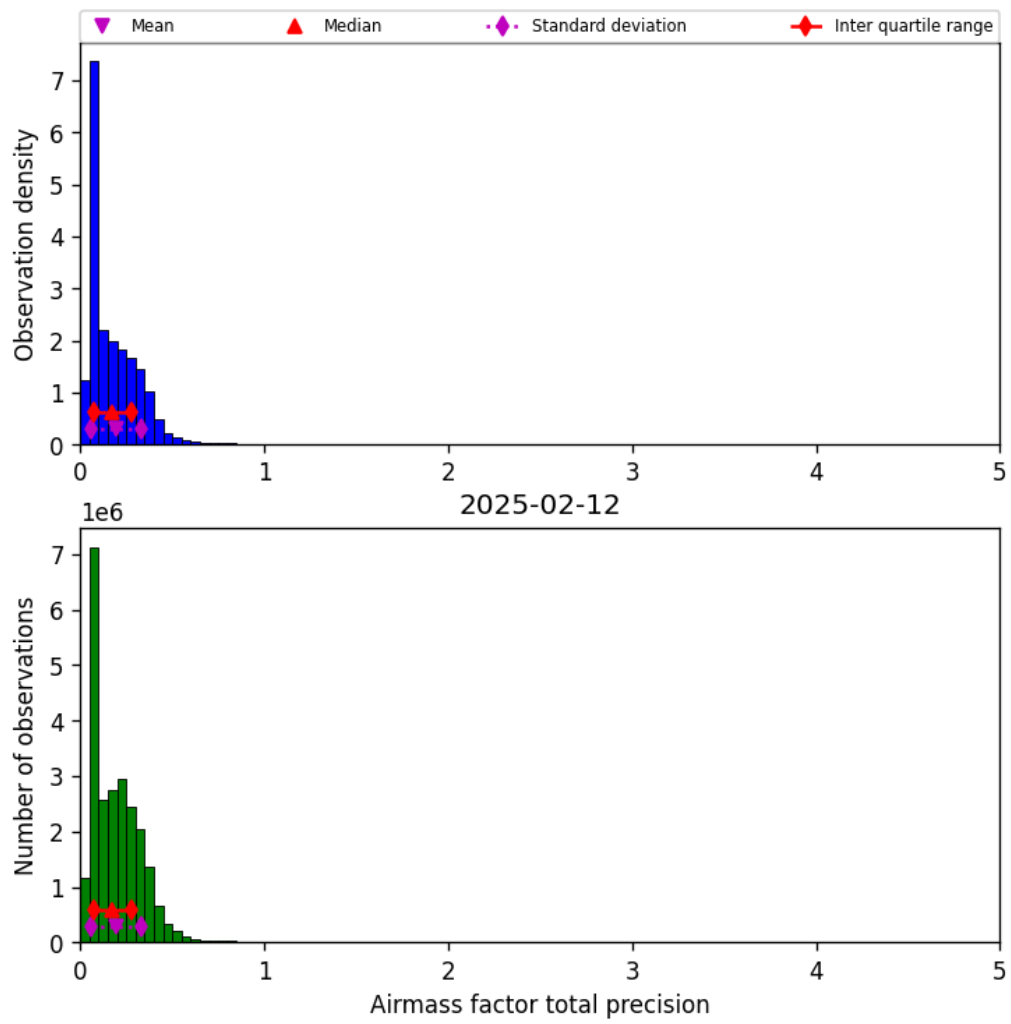
Figure 39: Histogram of “Airmass factor total precision” for 2025-02-12 to 2025-02-13
