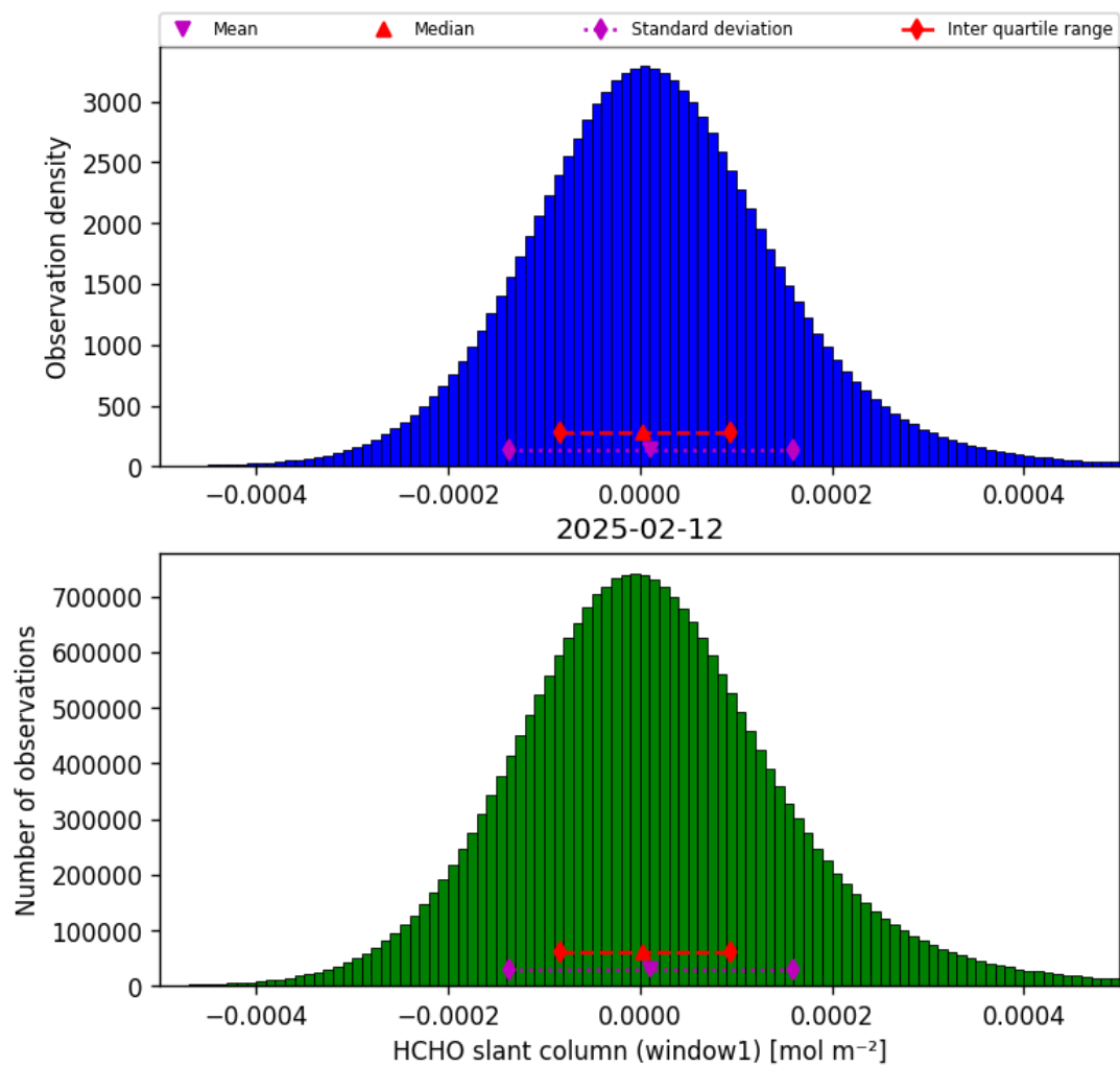
Figure 36: Histogram of “HCHO slant column (window1)” for 2025-02-12 to 2025-02-13
