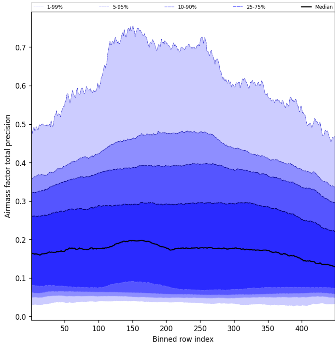
Figure 53: Along track statistics of “Airmass factor total precision” for 2025-02-12 to 2025-02-13
