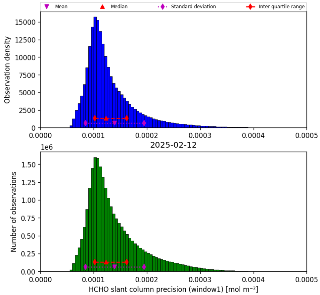
Figure 37: Histogram of “HCHO slant column precision (window1)” for 2025-02-12 to 2025-02-13
