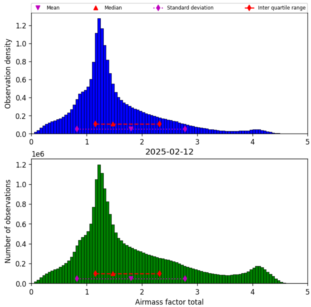
Figure 38: Histogram of “Airmass factor total” for 2025-02-12 to 2025-02-13
