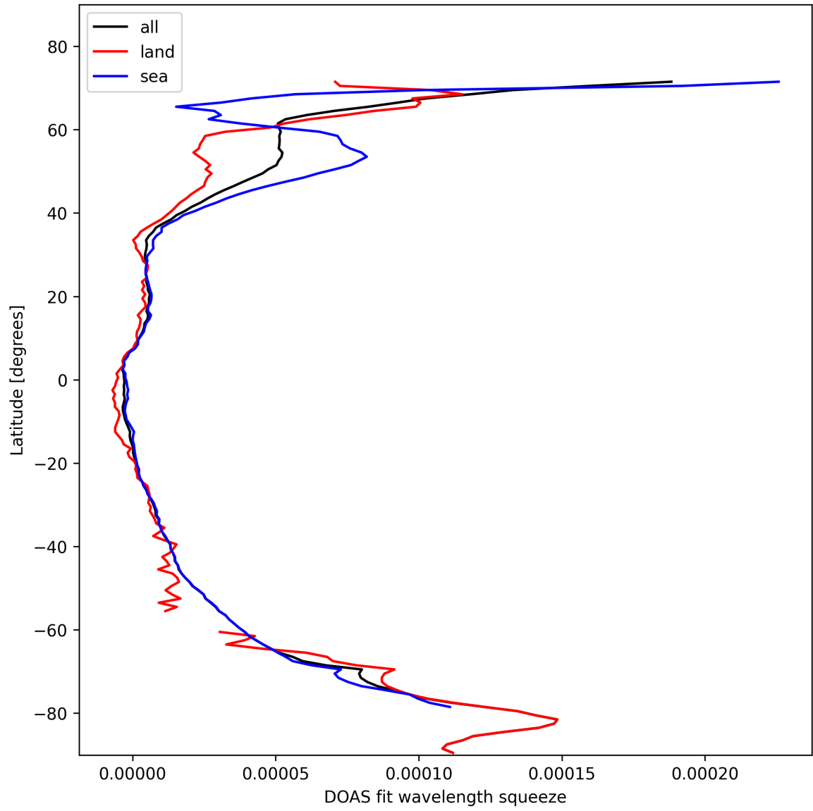
Figure 29: Zonal average of “DOAS fit wavelength squeeze” for 2025-02-12 to 2025-02-13.
