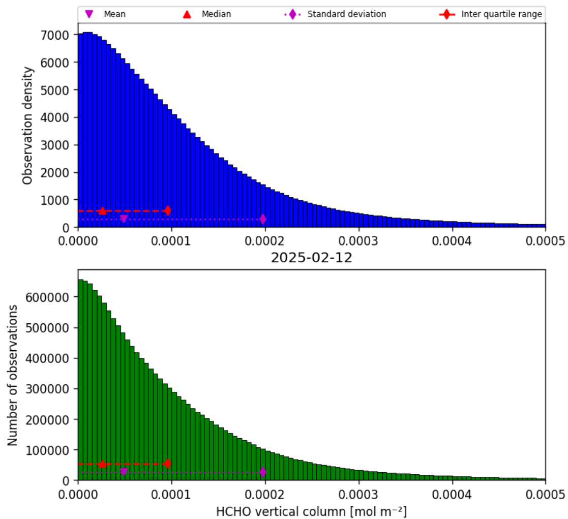
Figure 33: Histogram of “HCHO vertical column” for 2025-02-12 to 2025-02-13
