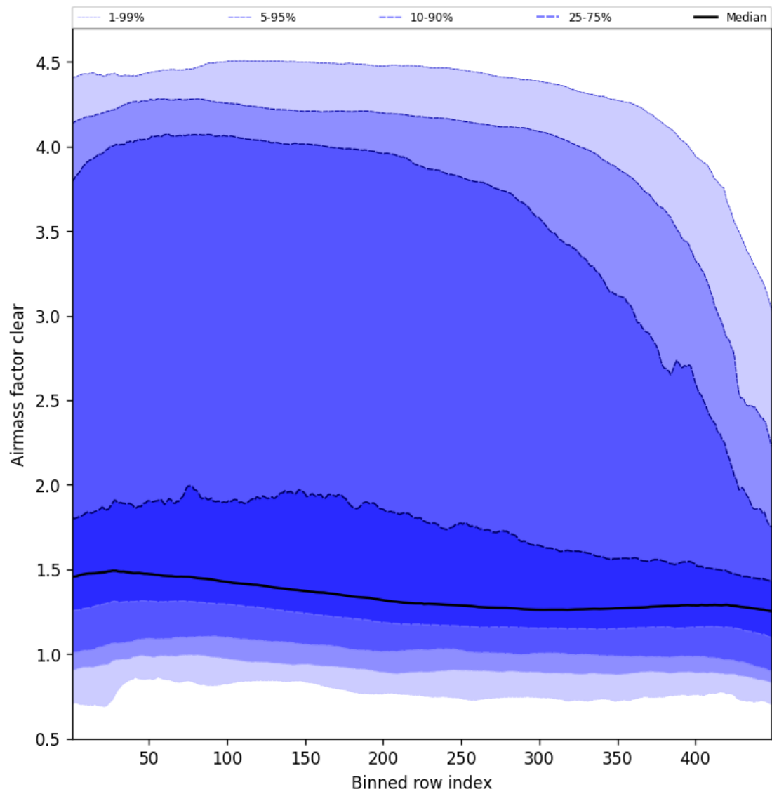
Figure 54: Along track statistics of “Airmass factor clear” for 2025-02-12 to 2025-02-13
