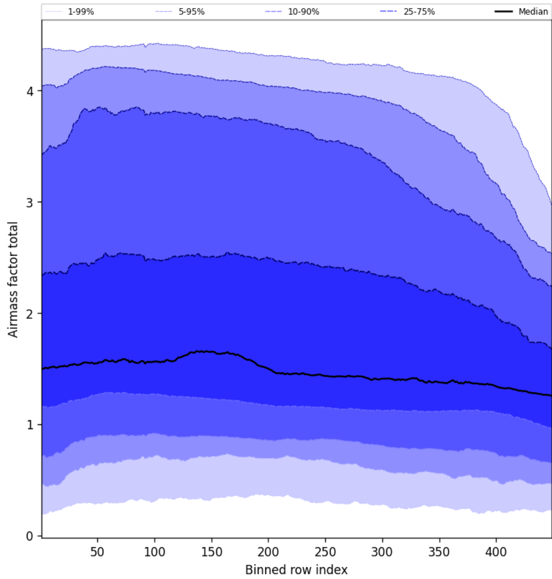
Figure 52: Along track statistics of “Airmass factor total” for 2025-02-12 to 2025-02-13
