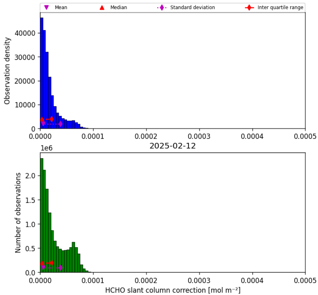
Figure 45: Histogram of “HCHO slant column correction” for 2025-02-12 to 2025-02-13
