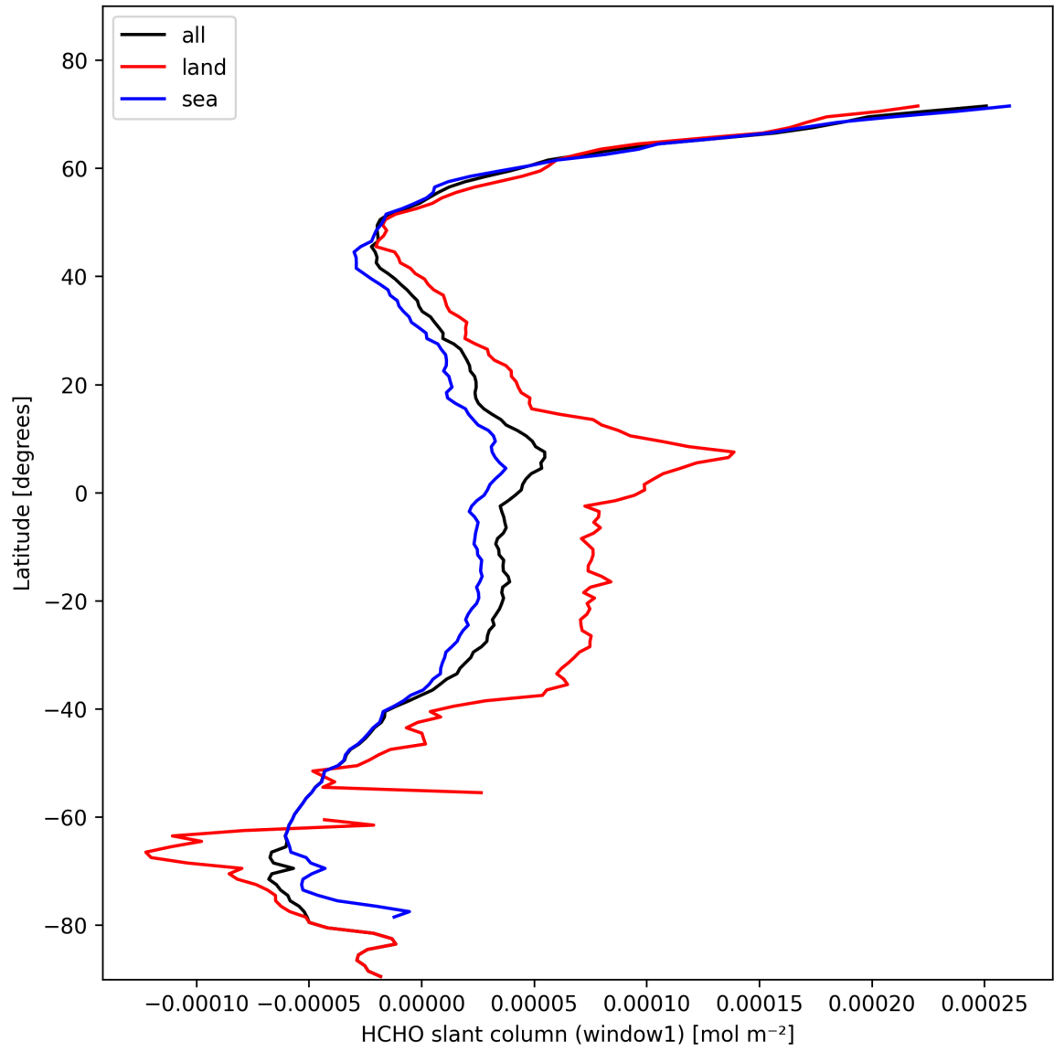
Figure 22: Zonal average of “HCHO slant column (window1)” for 2025-02-12 to 2025-02-13.
