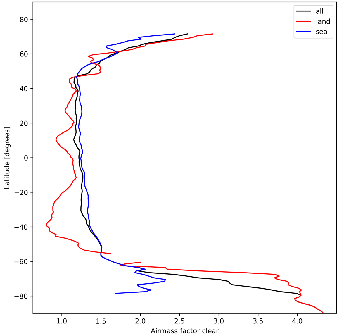
Figure 26: Zonal average of “Airmass factor clear” for 2025-02-12 to 2025-02-13.
