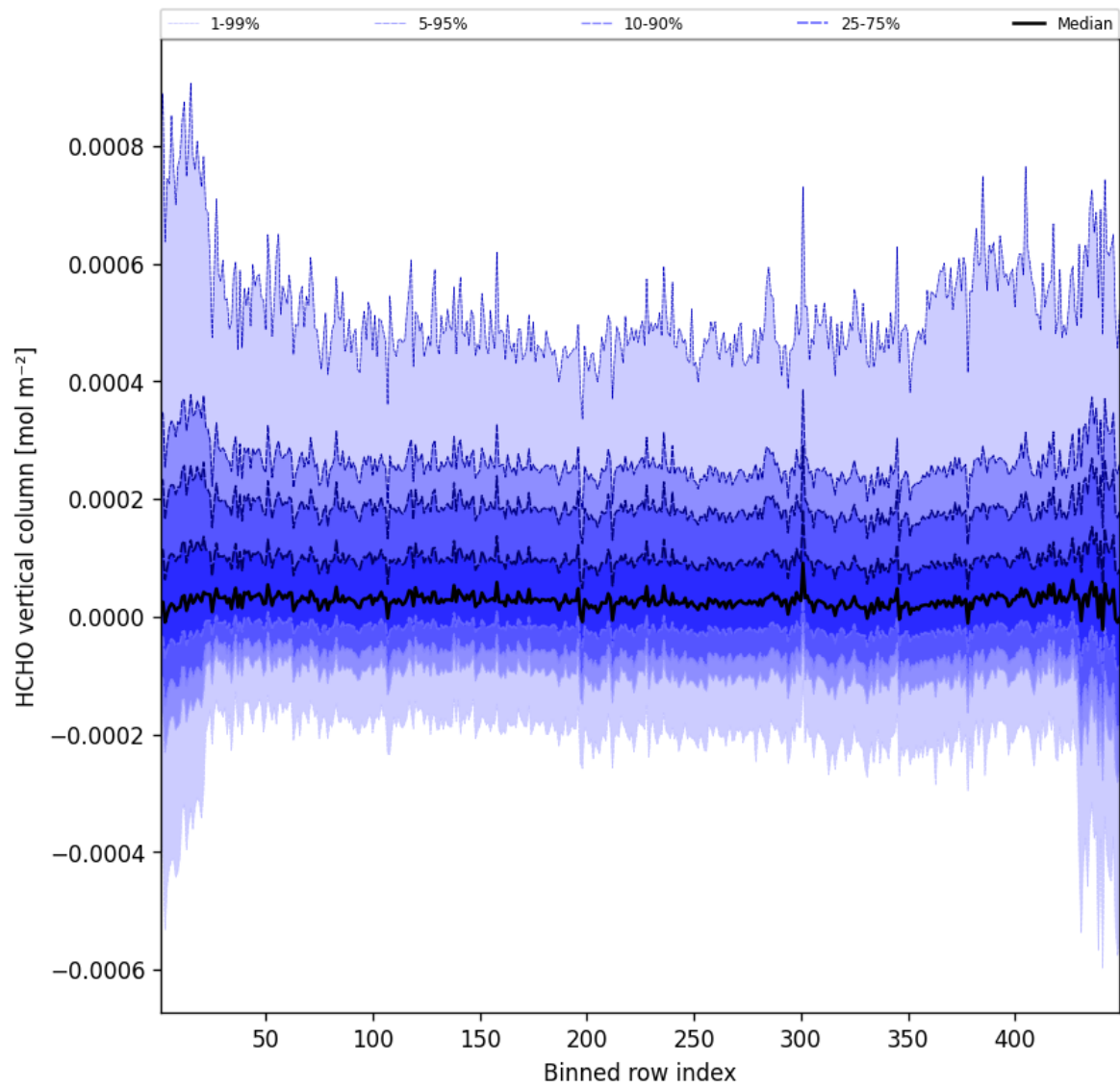
Figure 47: Along track statistics of “HCHO vertical column” for 2025-02-12 to 2025-02-13
