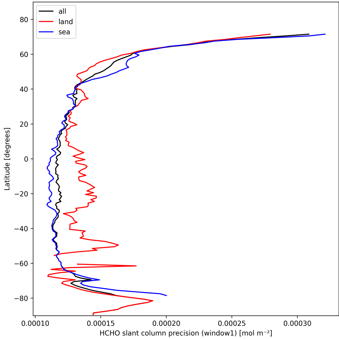
Figure 23: Zonal average of "HCHO slant column precision (window1)" for 2025-02-12 to 2025-02-13.
