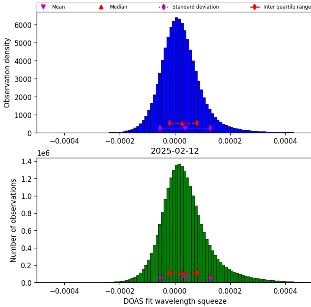
Figure 43: Histogram of “DOAS fit wavelength squeeze” for 2025-02-12 to 2025-02-13
