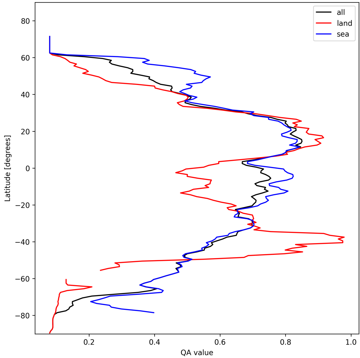
Figure 18: Zonal average of “QA value” for 2025-02-12 to 2025-02-13.
