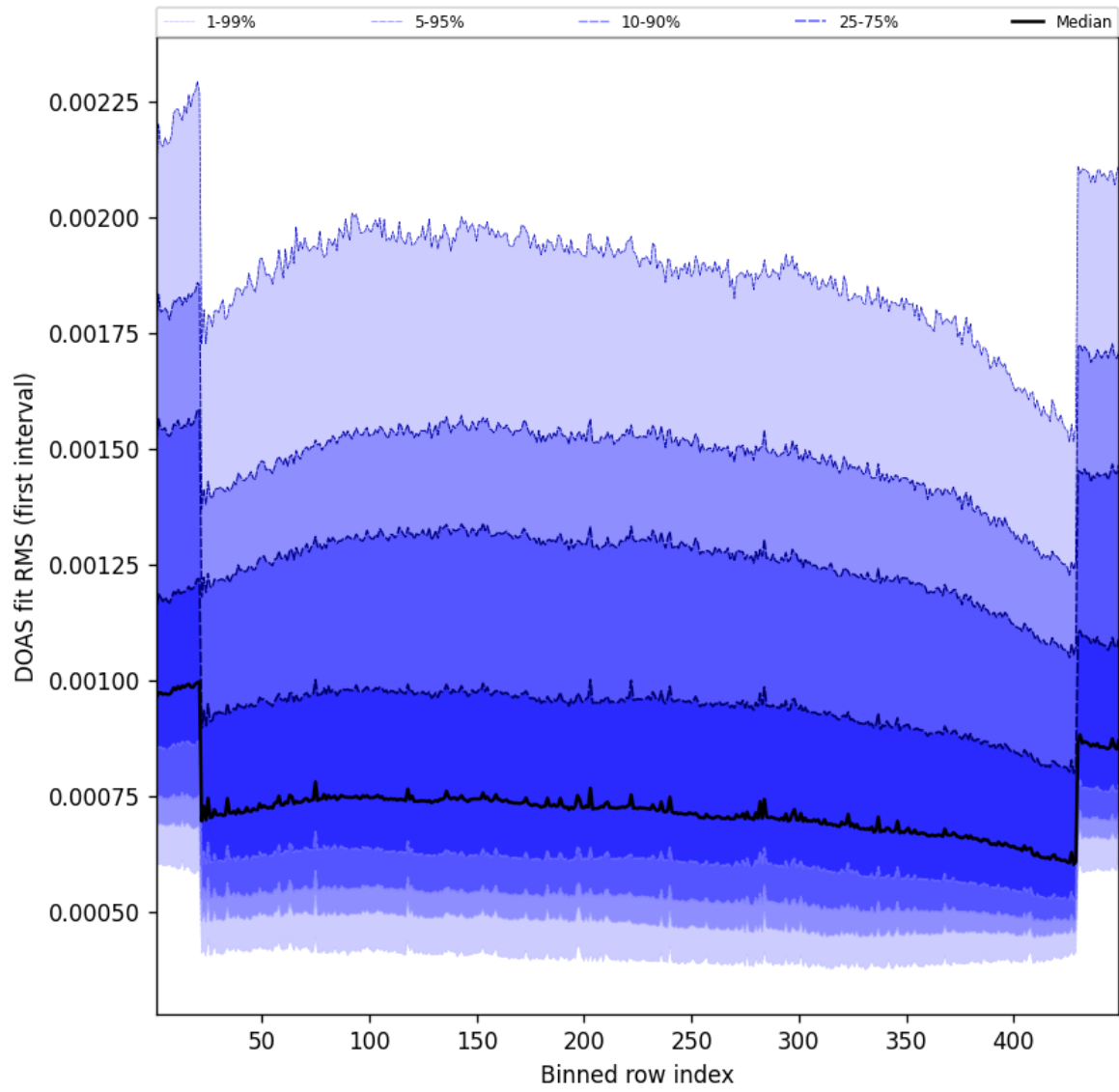
Figure 58: Along track statistics of “DOAS fit RMS (first interval)” for 2025-02-12 to 2025-02-13
