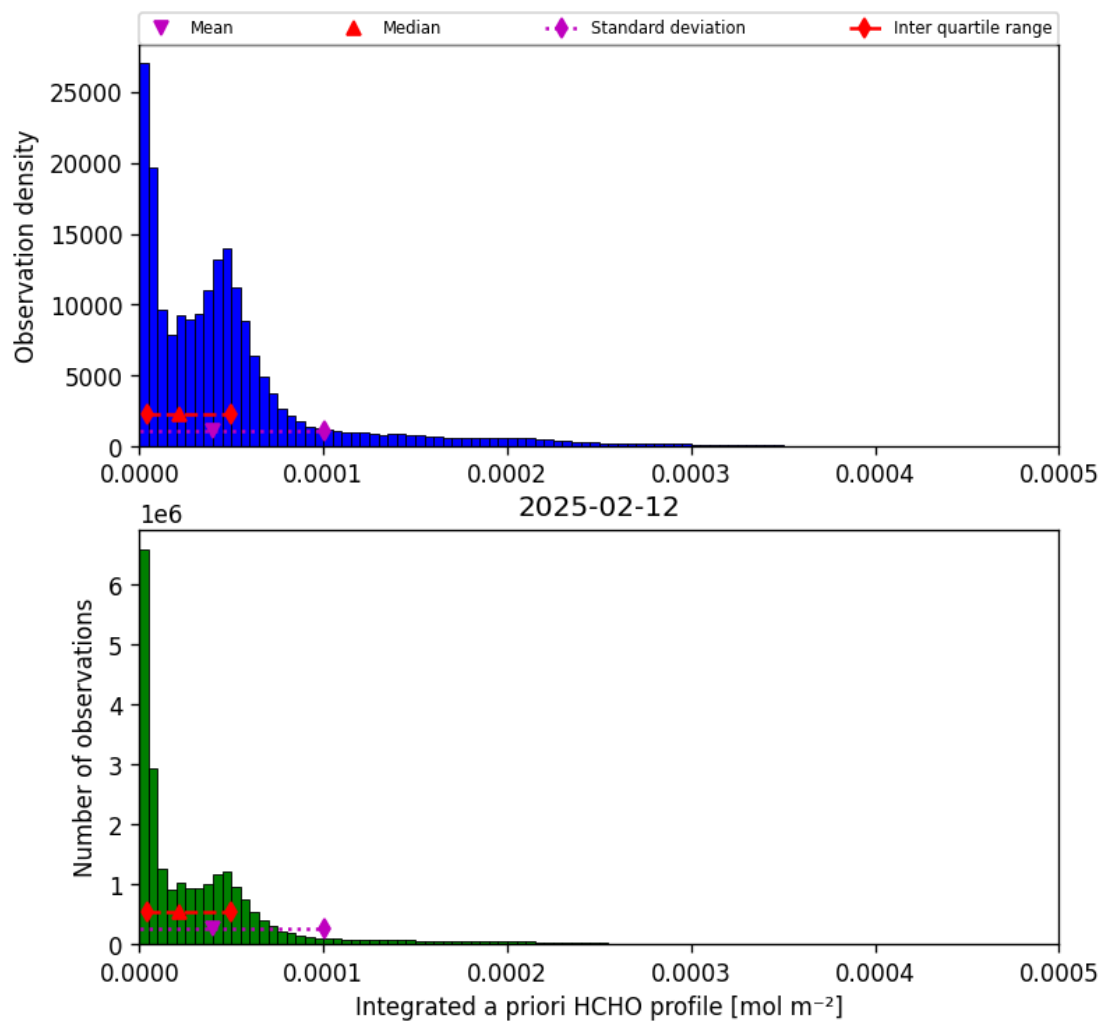
Figure 41: Histogram of “Integrated a priori HCHO profile” for 2025-02-12 to 2025-02-13
