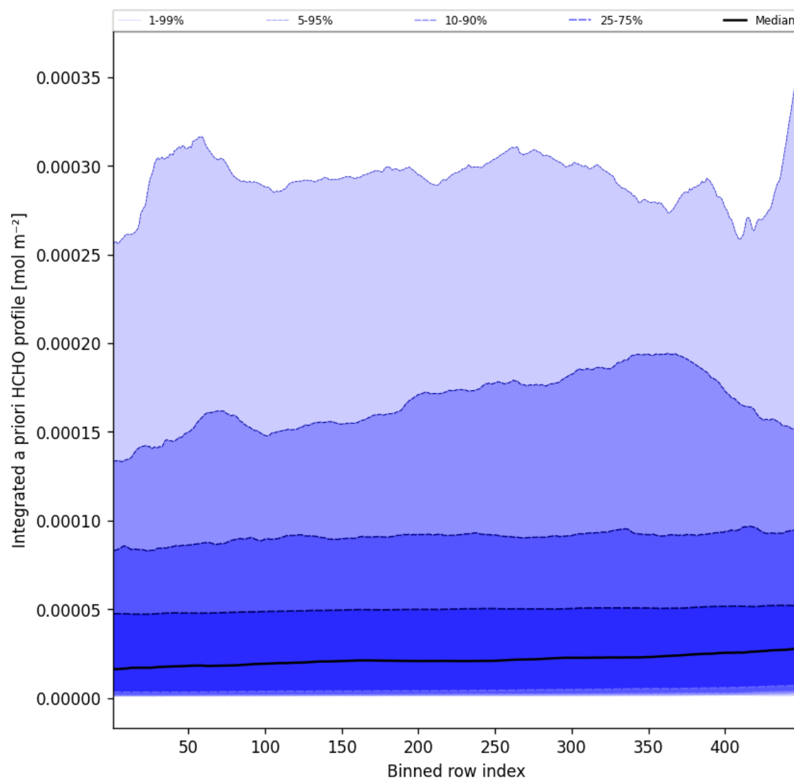
Figure 55: Along track statistics of "Integrated a priori HCHO profile" for 2025-02-12 to 2025-02-13
