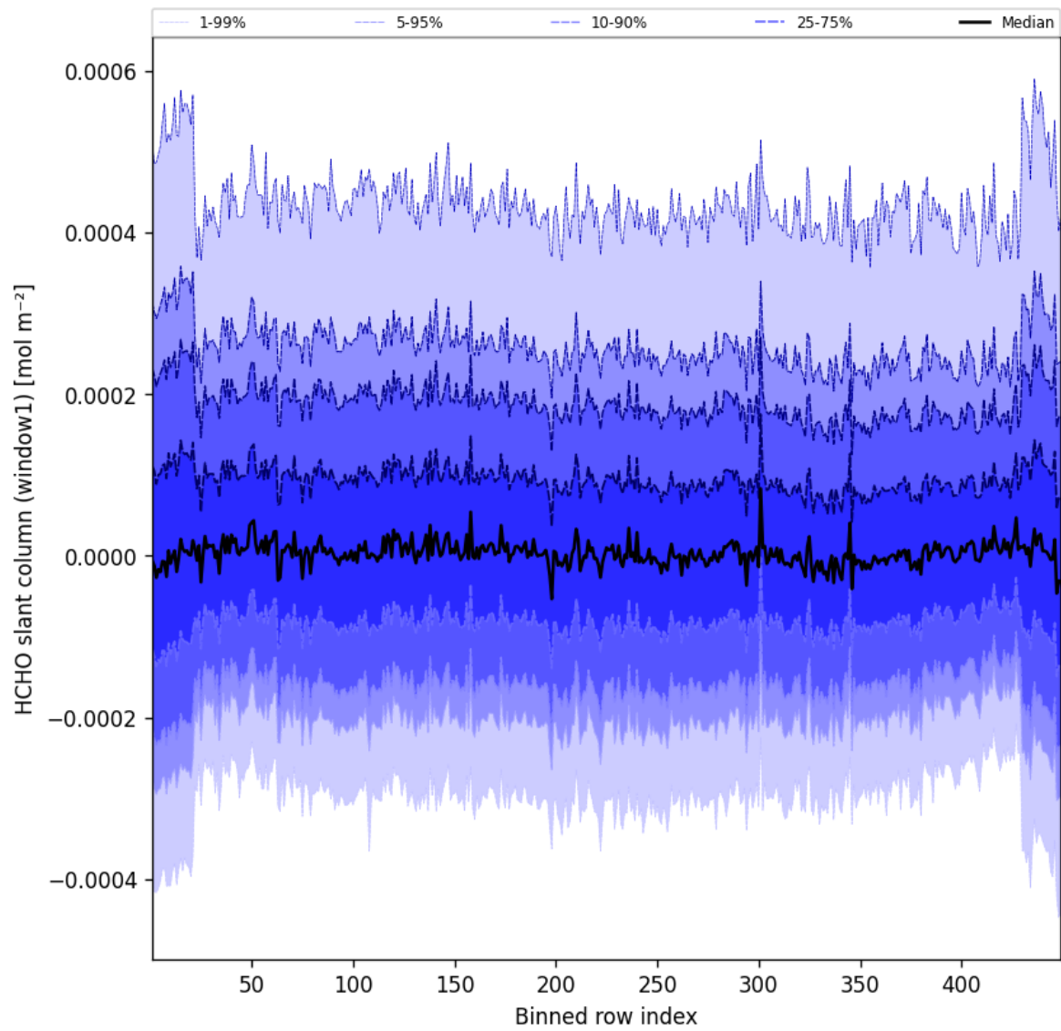
Figure 50: Along track statistics of “HCHO slant column (window1)” for 2025-02-12 to 2025-02-13
