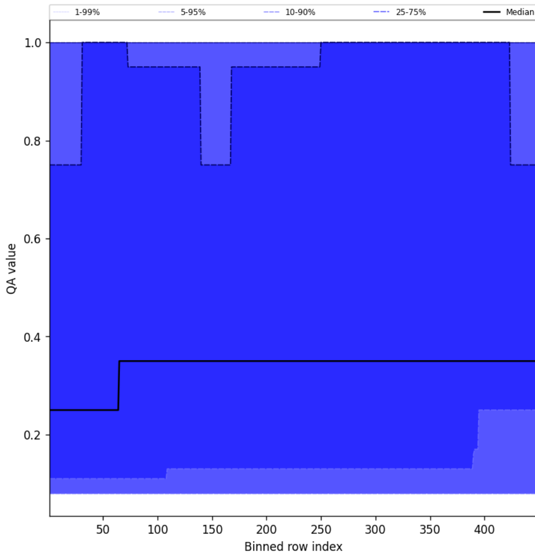
Figure 46: Along track statistics of “QA value” for 2025-02-12 to 2025-02-13
