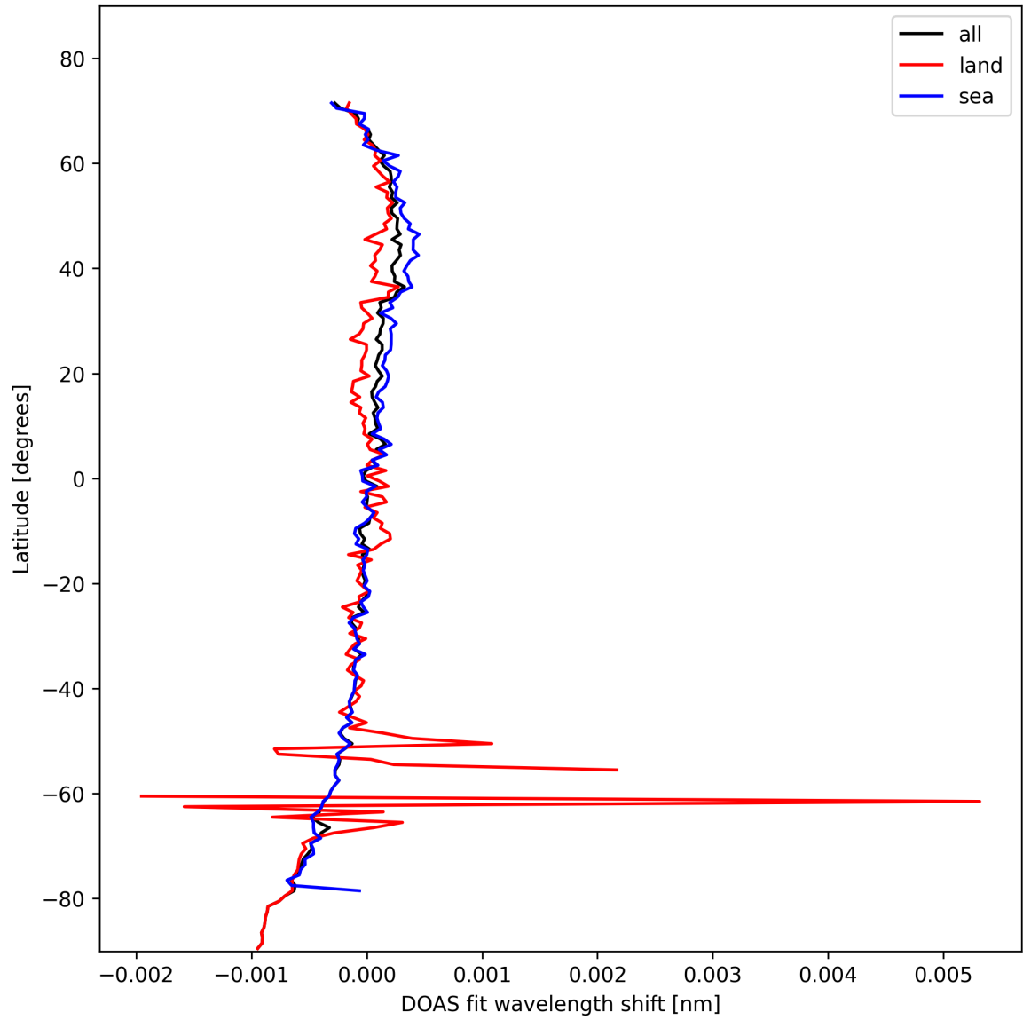
Figure 28: Zonal average of "DOAS fit wavelength shift" for 2025-02-12 to 2025-02-13.
