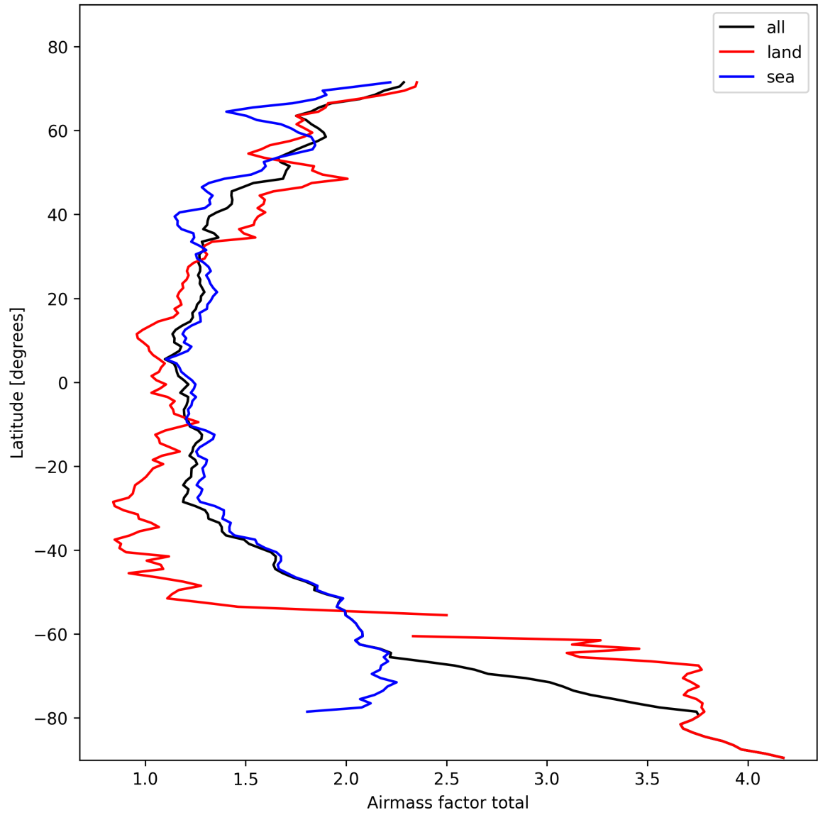
Figure 24: Zonal average of “Airmass factor total” for 2025-02-12 to 2025-02-13.
