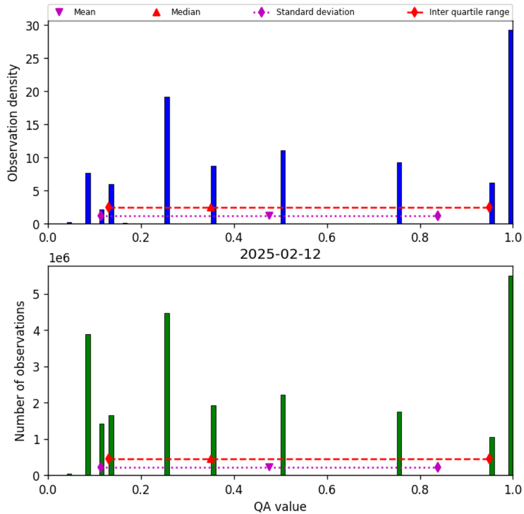
Figure 32: Histogram of “QA value” for 2025-02-12 to 2025-02-13
