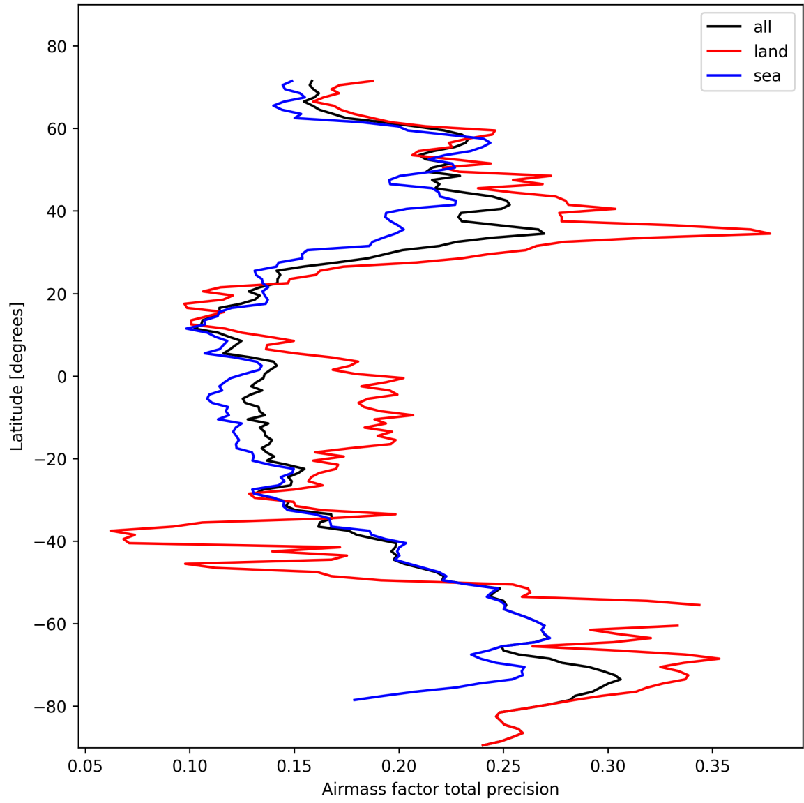
Figure 25: Zonal average of “Airmass factor total precision” for 2025-02-12 to 2025-02-13.
