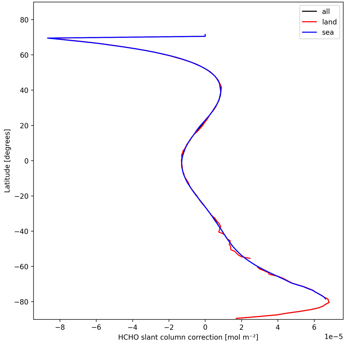
Figure 31: Zonal average of “HCHO slant column correction” for 2025-02-12 to 2025-02-13.
