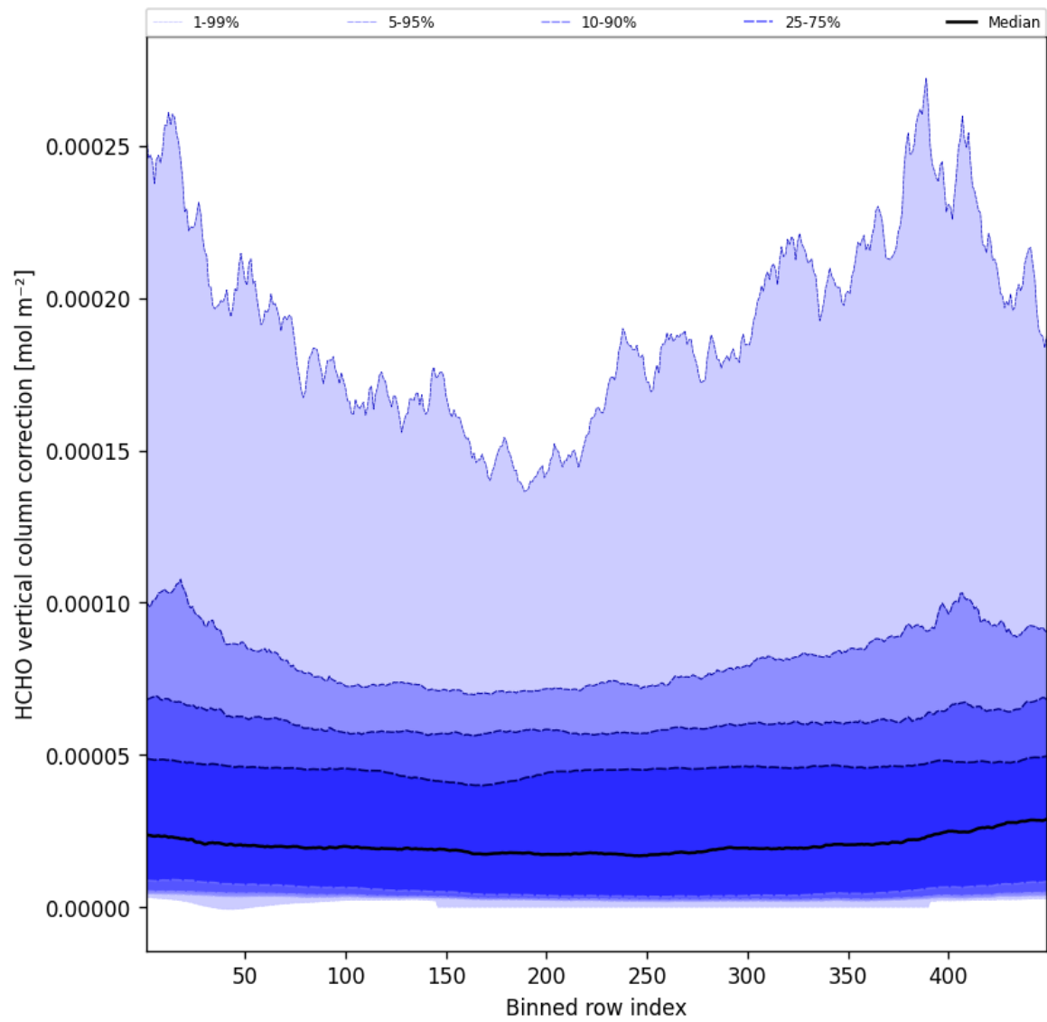
Figure 49: Along track statistics of “HCHO vertical column correction” for 2025-02-12 to 2025-02-13
