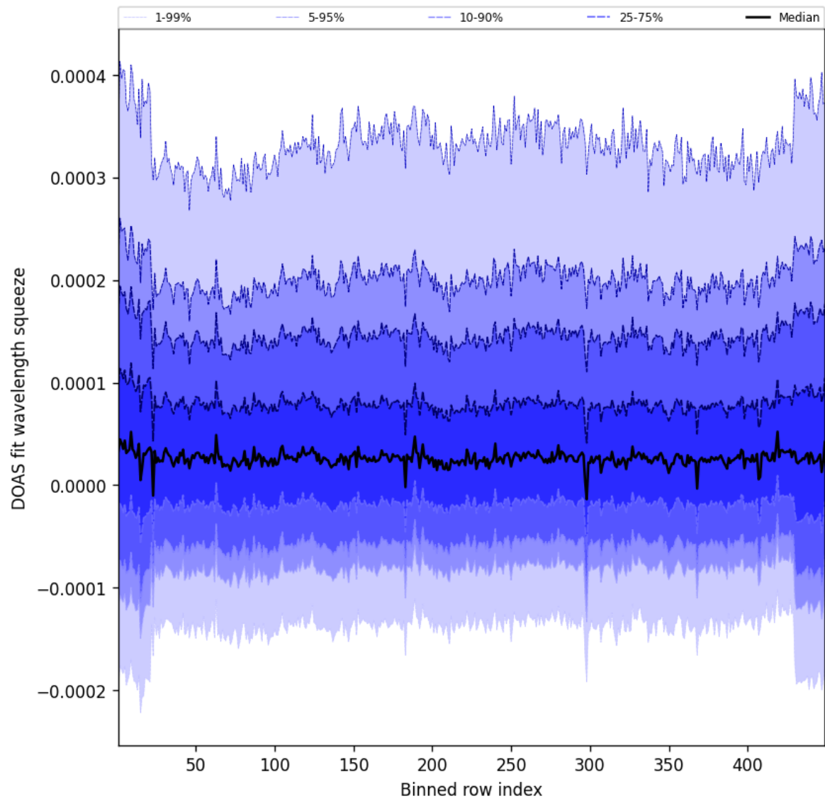
Figure 57: Along track statistics of “DOAS fit wavelength squeeze” for 2025-02-12 to 2025-02-13
