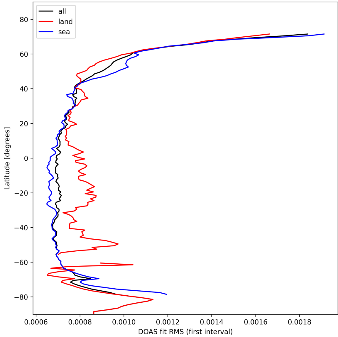
Figure 30: Zonal average of “DOAS fit RMS (first interval)” for 2025-02-12 to 2025-02-13.
