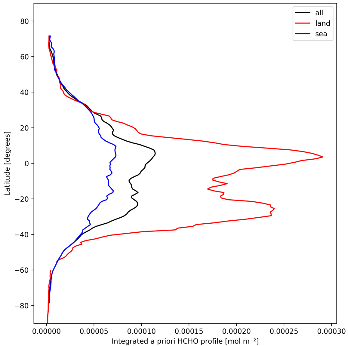
Figure 27: Zonal average of “Integrated a priori HCHO profile” for 2025-02-12 to 2025-02-13.
