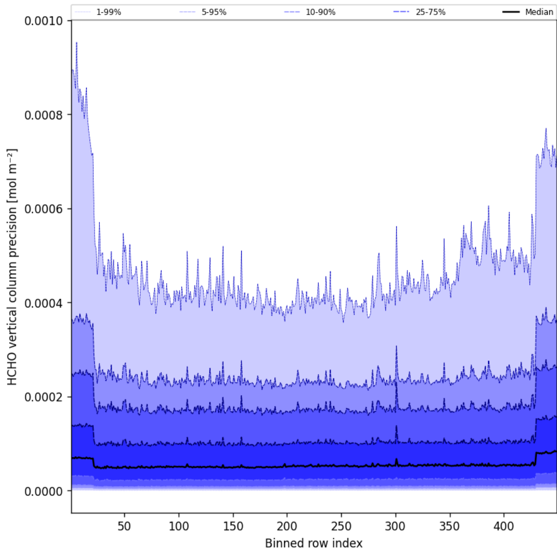
Figure 48: Along track statistics of “HCHO vertical column precision” for 2025-02-12 to 2025-02-13
