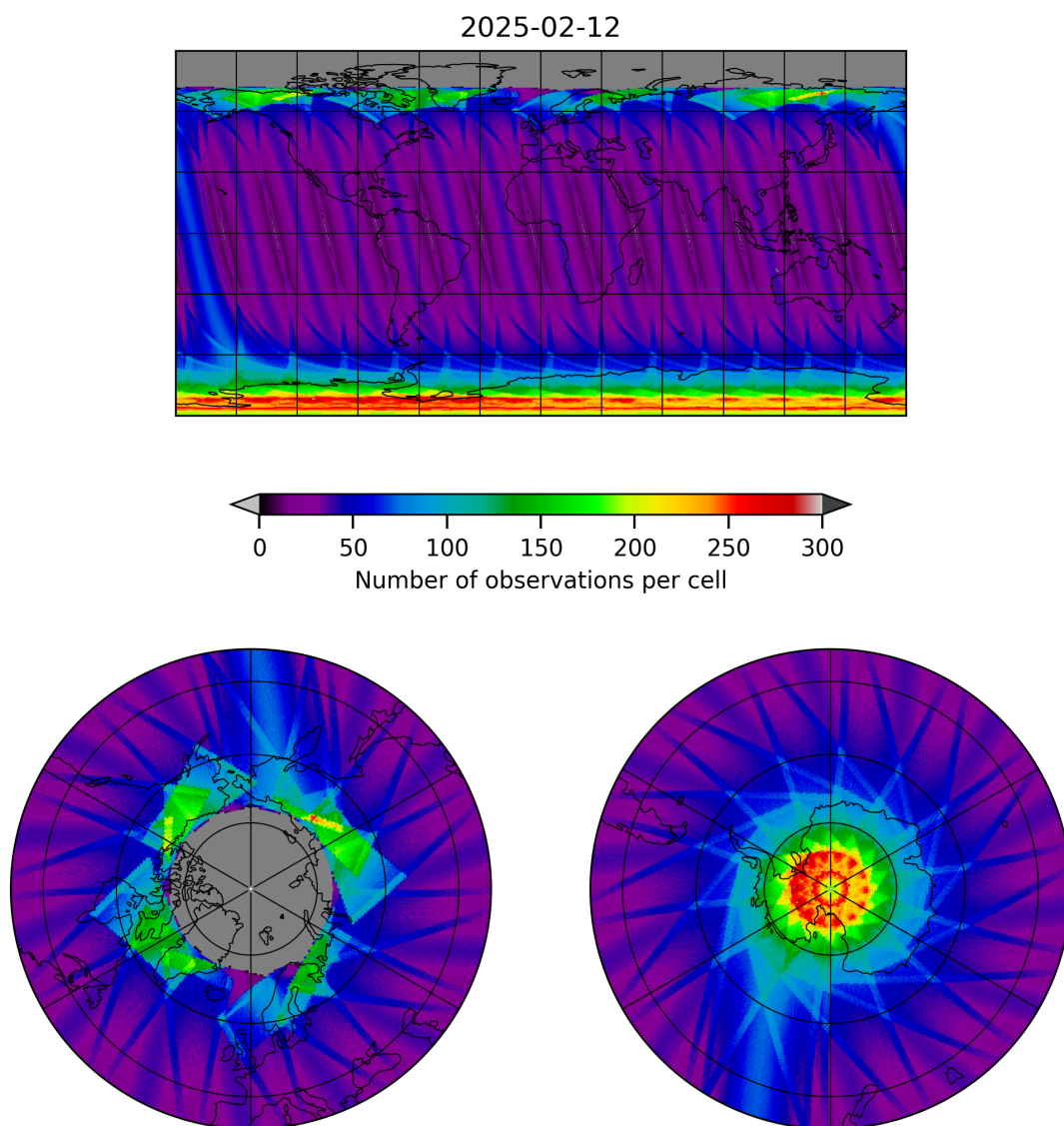
Figure 17: Map of the number of observations for 2025-02-12 to 2025-02-13
