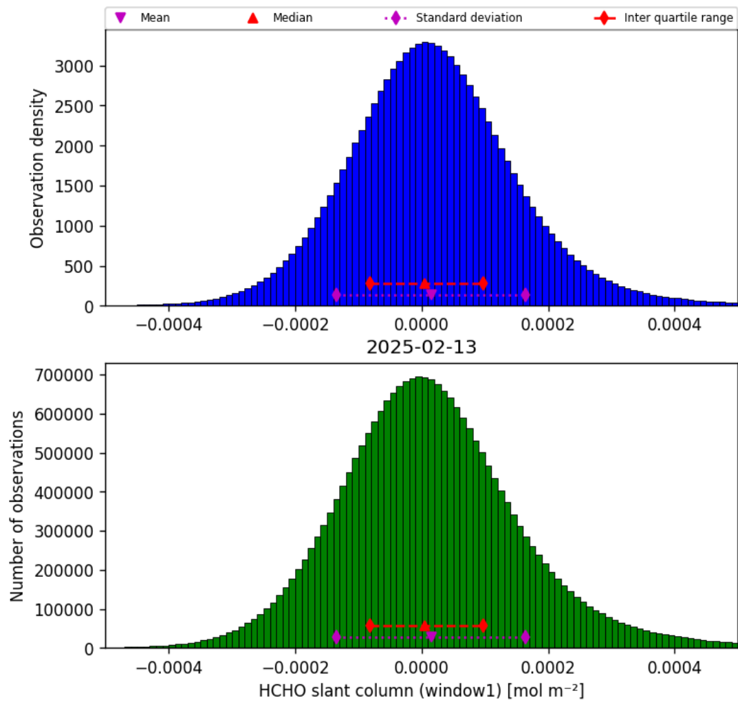
Figure 36: Histogram of "HCHO slant column (window1)" for 2025-02-13 to 2025-02-14
