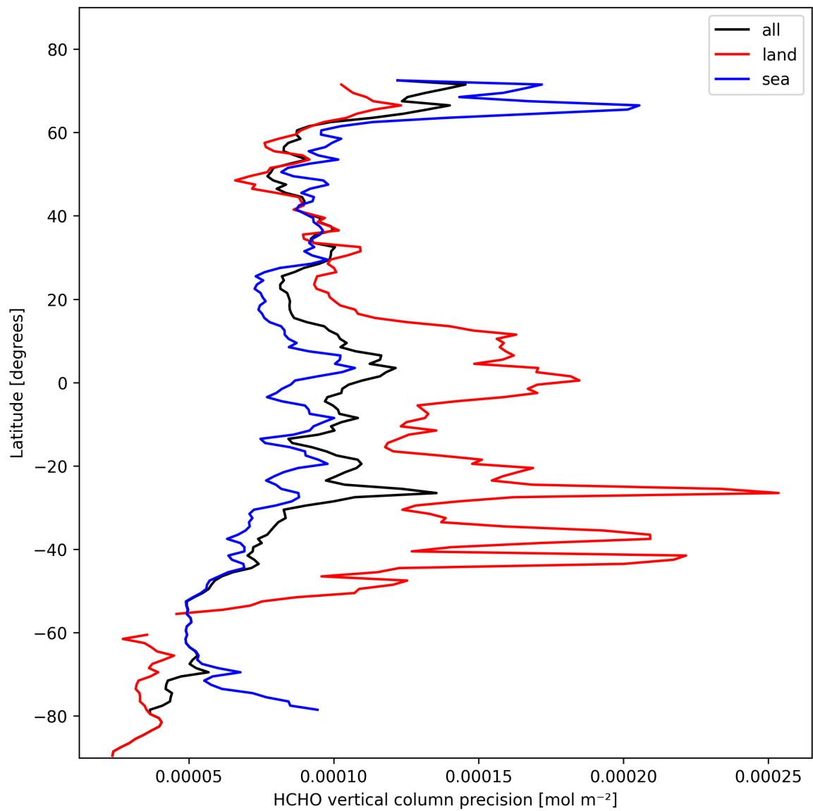
Figure 20: Zonal average of “HCHO vertical column precision” for 2025-02-13 to 2025-02-14.
