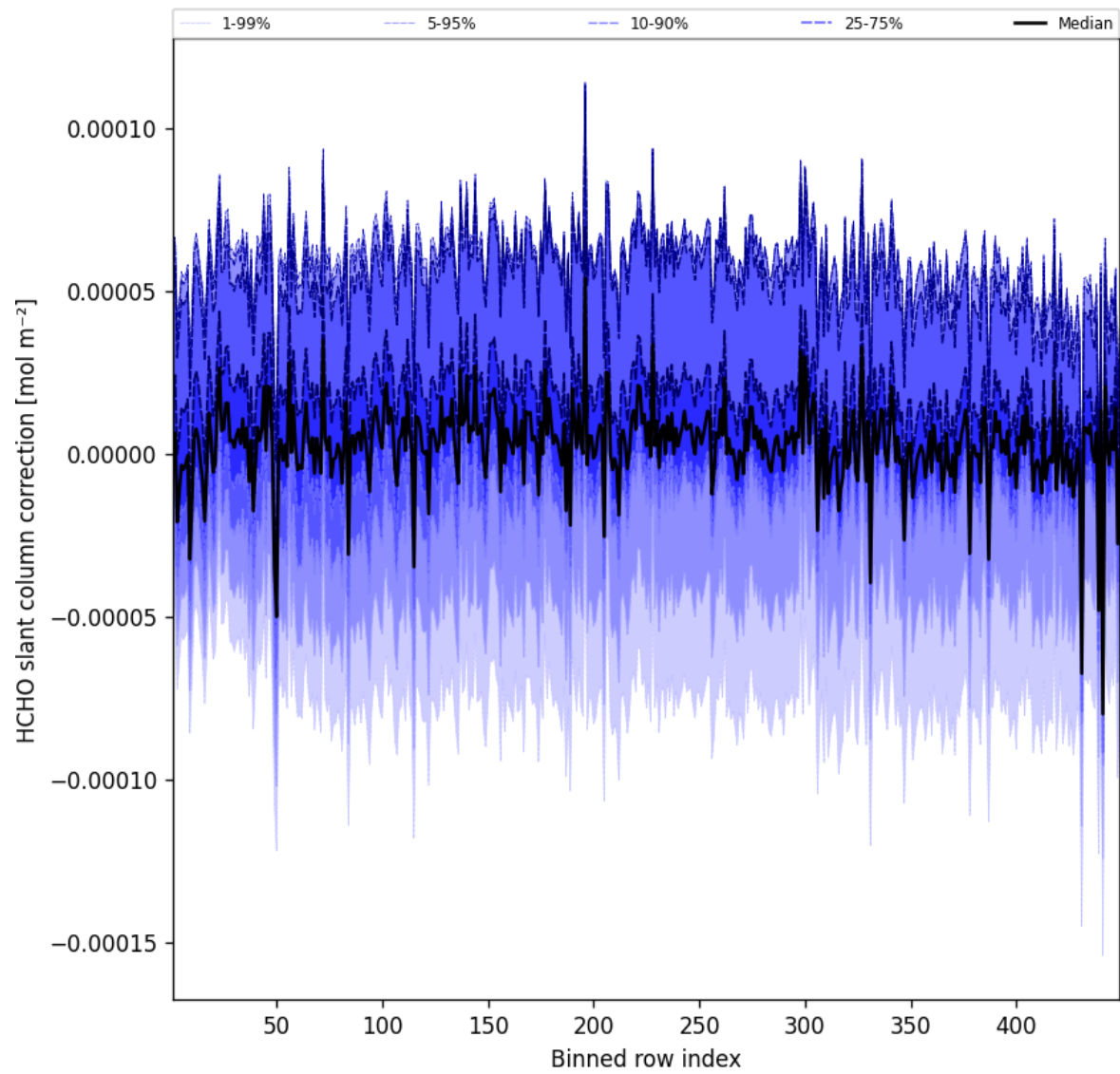
Figure 59: Along track statistics of “HCHO slant column correction” for 2025-02-13 to 2025-02-14
