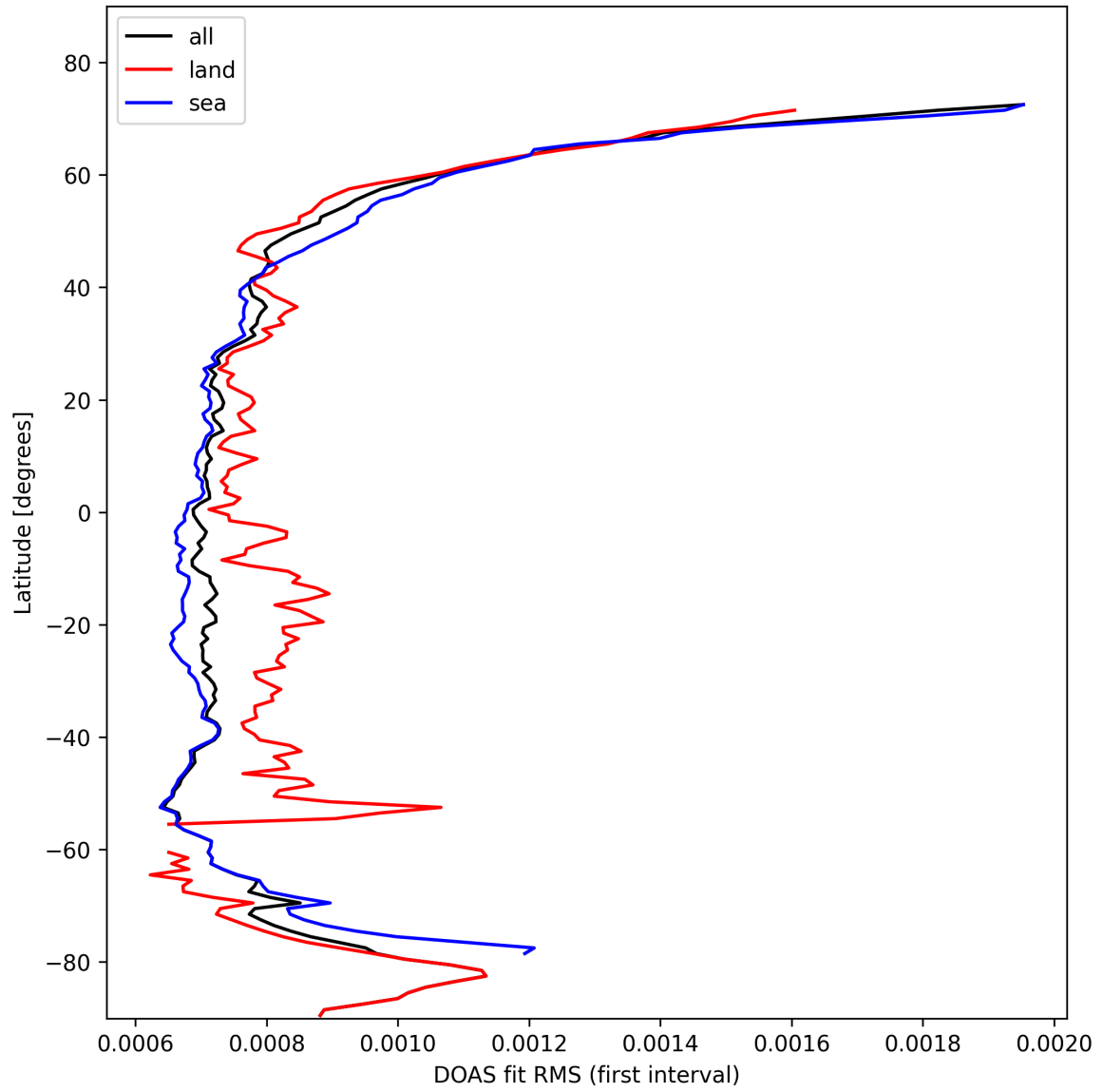
Figure 30: Zonal average of “DOAS fit RMS (first interval)” for 2025-02-13 to 2025-02-14.
