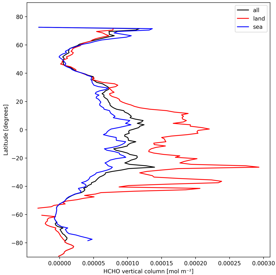
Figure 19: Zonal average of “HCHO vertical column” for 2025-02-13 to 2025-02-14.
