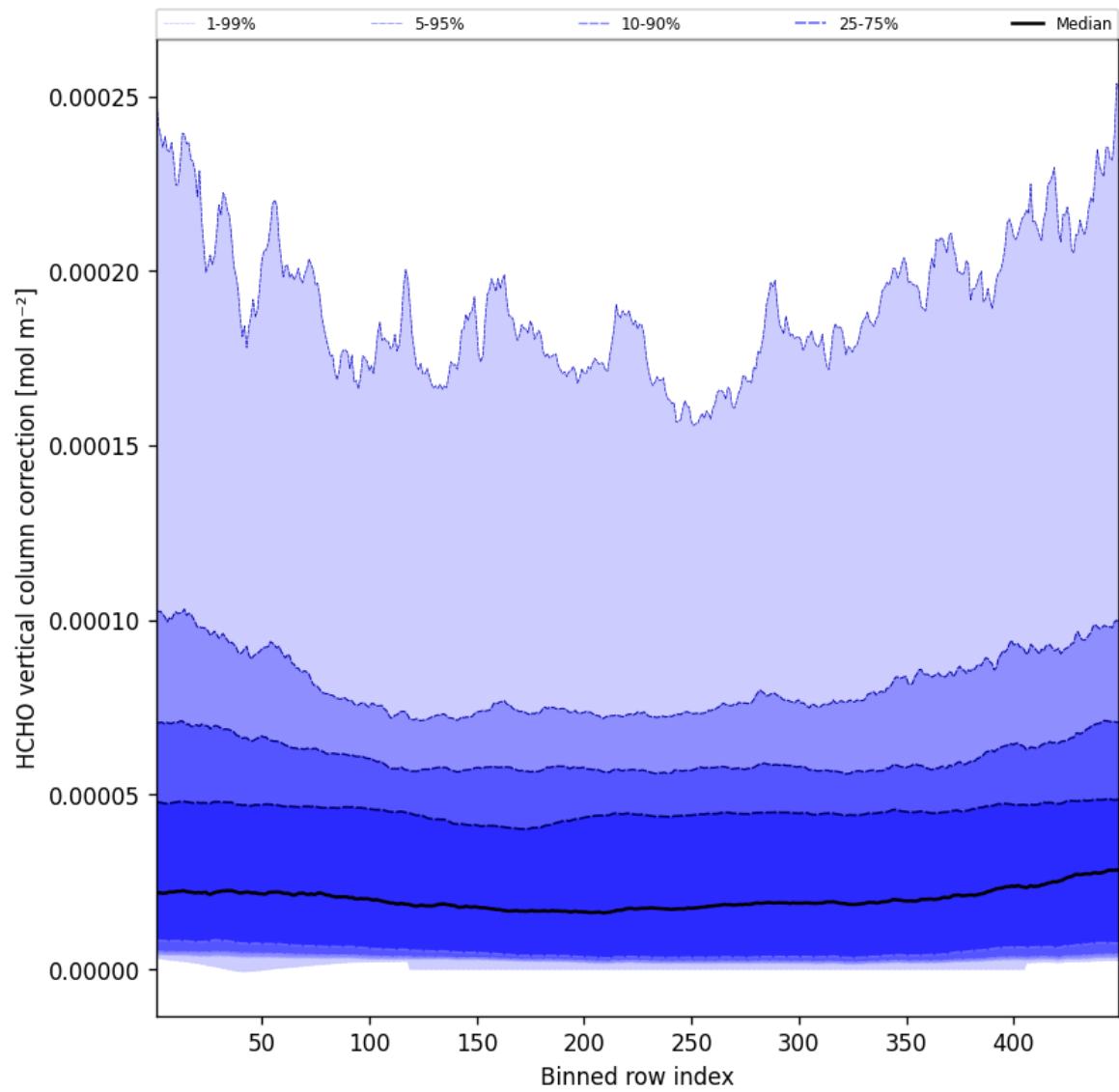
Figure 49: Along track statistics of “HCHO vertical column correction” for 2025-02-13 to 2025-02-14
