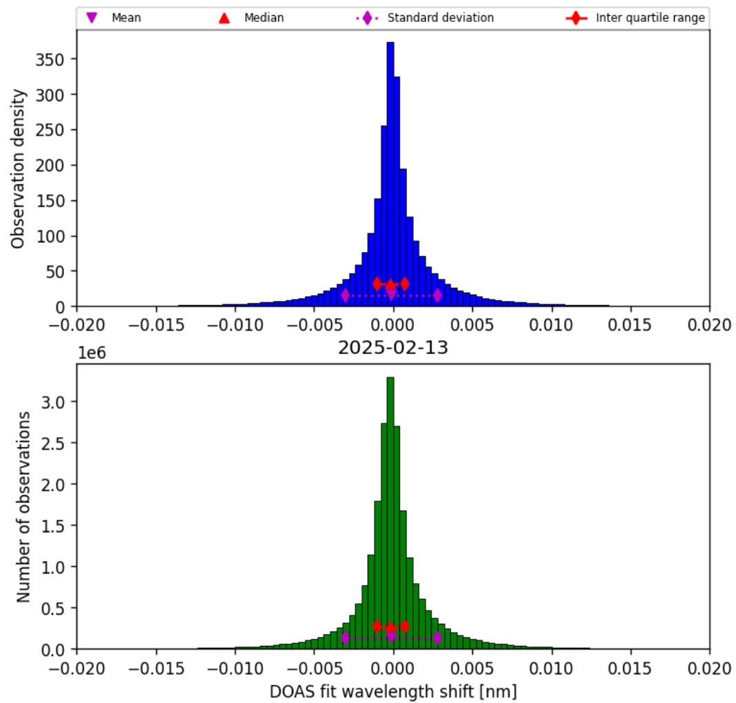
Figure 42: Histogram of “DOAS fit wavelength shift” for 2025-02-13 to 2025-02-14
