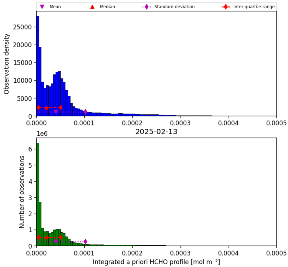
Figure 41: Histogram of “Integrated a priori HCHO profile” for 2025-02-13 to 2025-02-14
