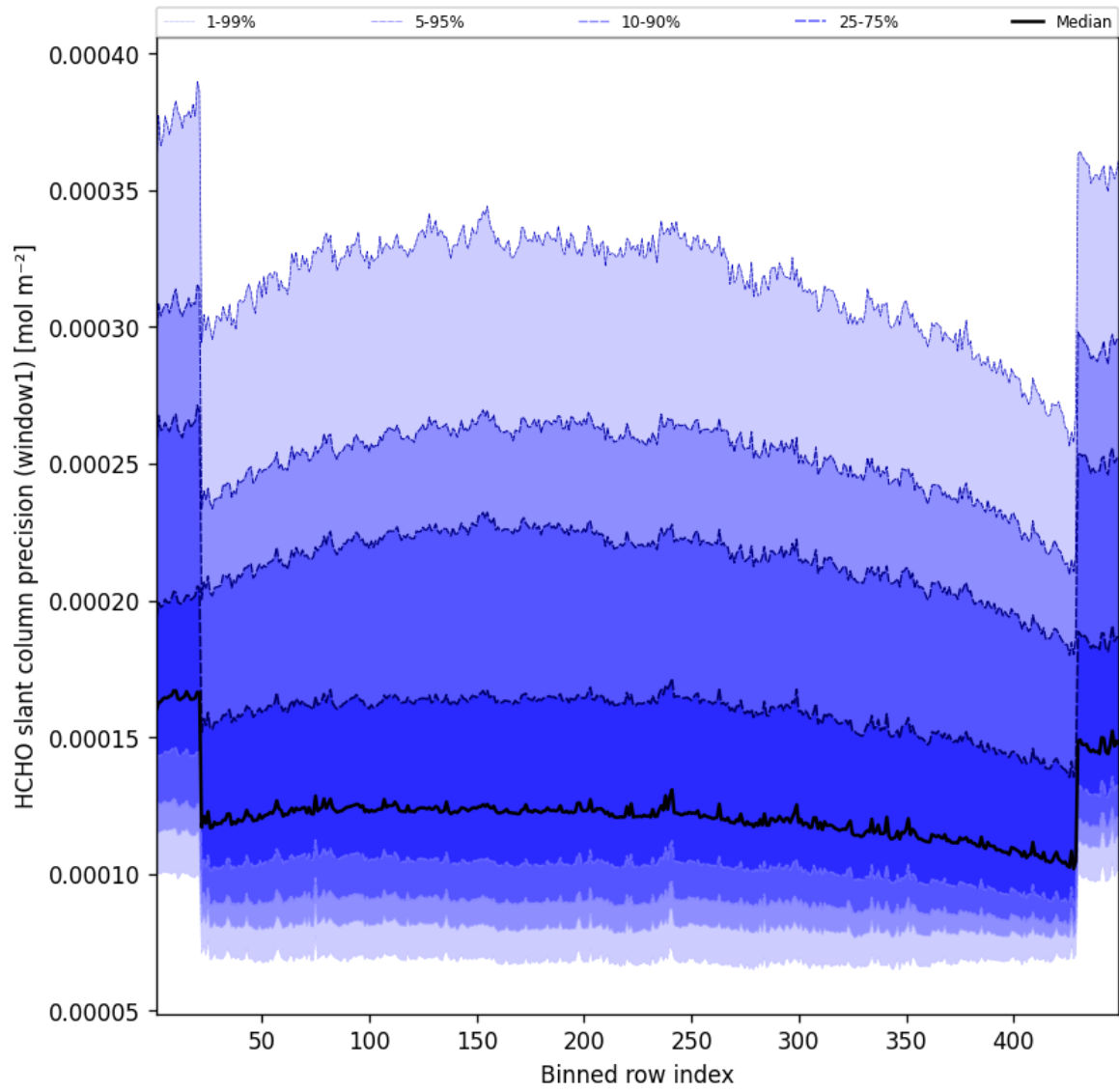
Figure 51: Along track statistics of “HCHO slant column precision (window1)” for 2025-02-13 to 2025-02-14
