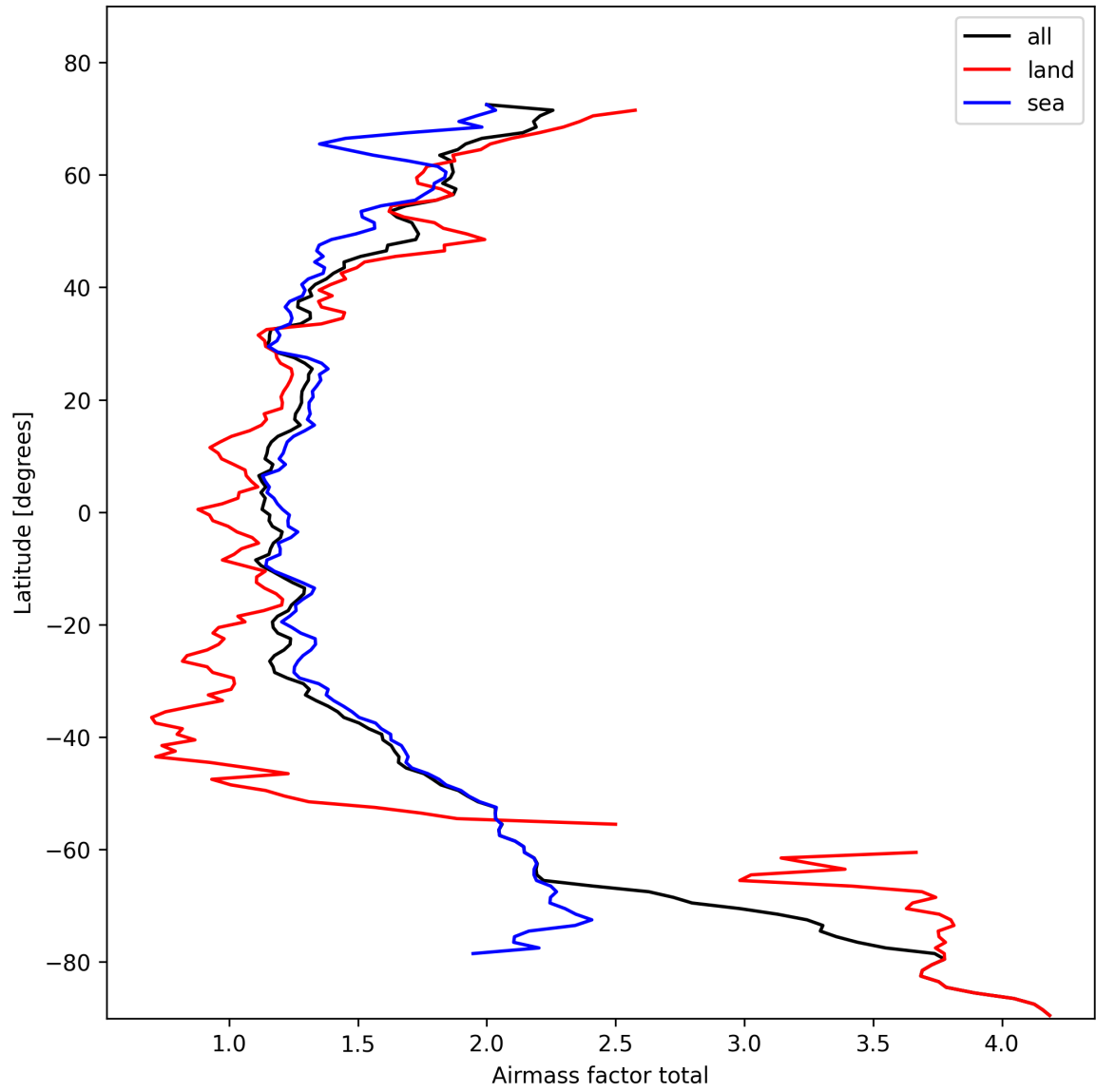
Figure 24: Zonal average of “Airmass factor total” for 2025-02-13 to 2025-02-14.
