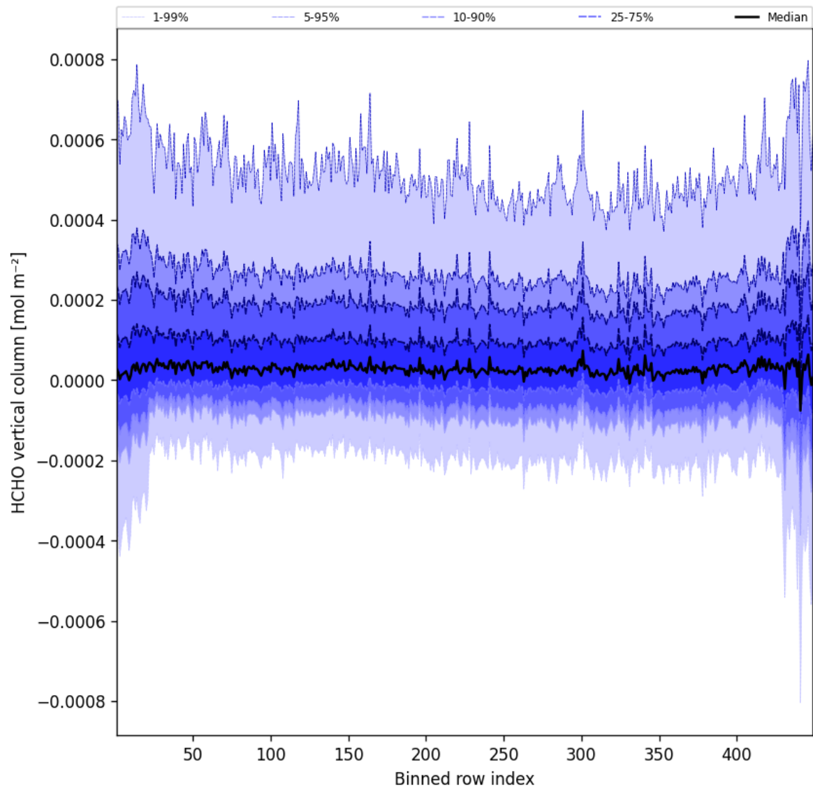
Figure 47: Along track statistics of “HCHO vertical column” for 2025-02-13 to 2025-02-14
