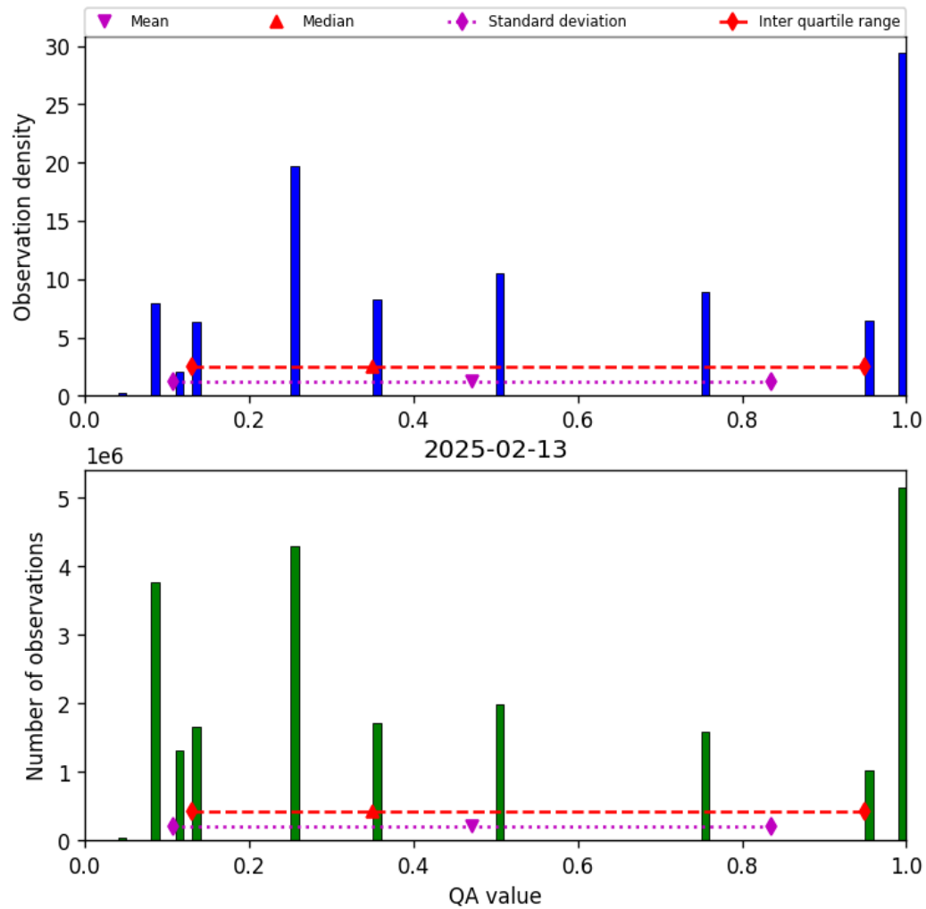
Figure 32: Histogram of “QA value” for 2025-02-13 to 2025-02-14
