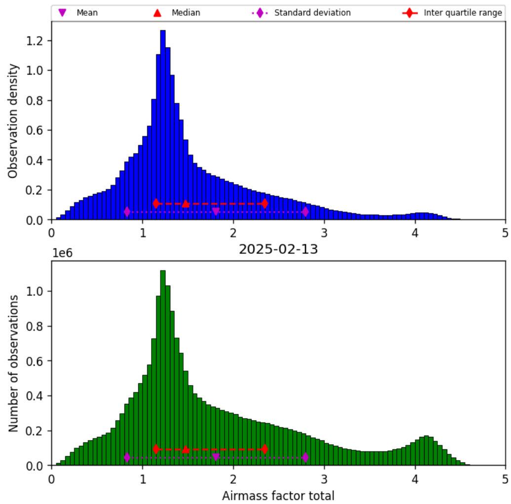
Figure 38: Histogram of “Airmass factor total” for 2025-02-13 to 2025-02-14
