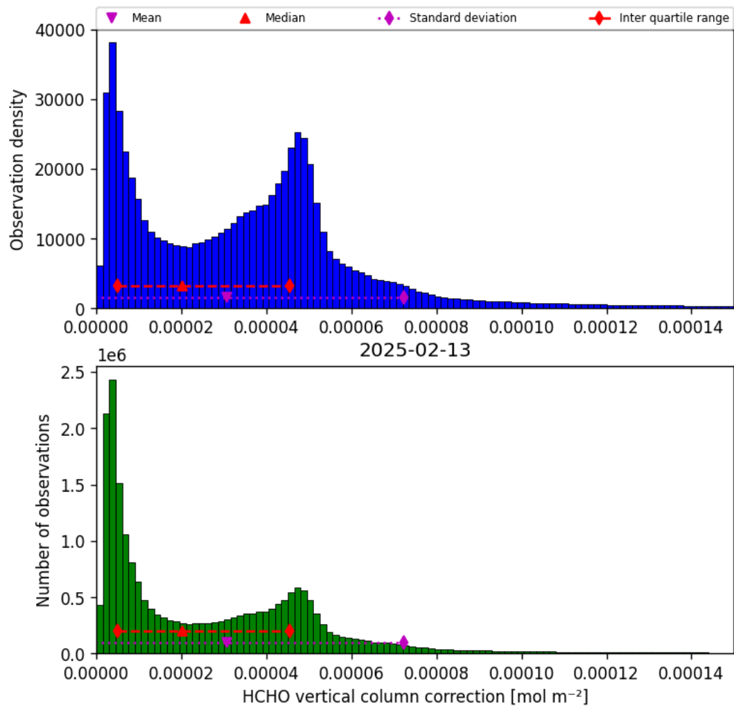
Figure 35: Histogram of “HCHO vertical column correction” for 2025-02-13 to 2025-02-14
