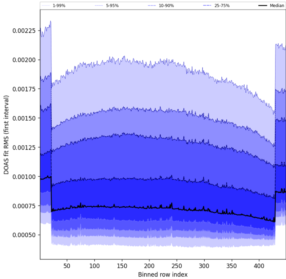
Figure 58: Along track statistics of “DOAS fit RMS (first interval)” for 2025-02-13 to 2025-02-14
