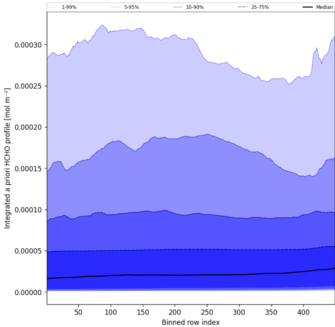
Figure 55: Along track statistics of “Integrated a priori HCHO profile” for 2025-02-13 to 2025-02-14
