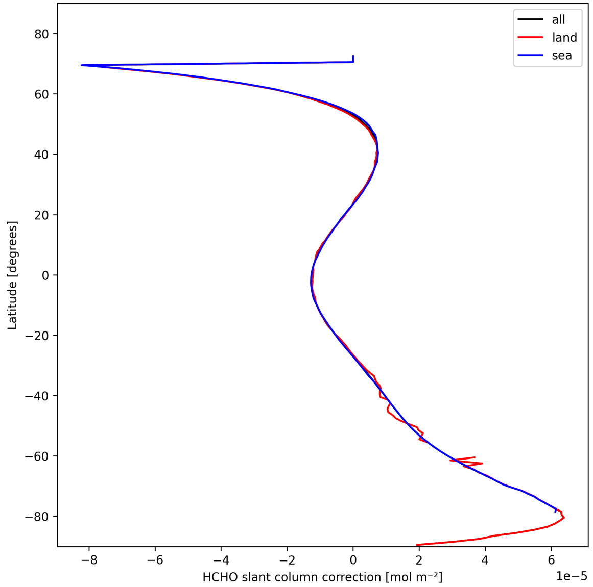
Figure 31: Zonal average of “HCHO slant column correction” for 2025-02-13 to 2025-02-14.
