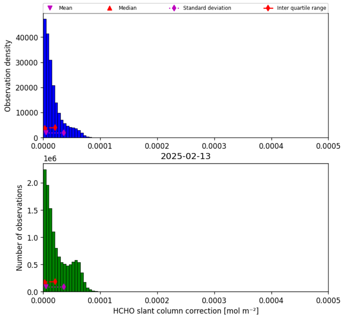
Figure 45: Histogram of “HCHO slant column correction” for 2025-02-13 to 2025-02-14
