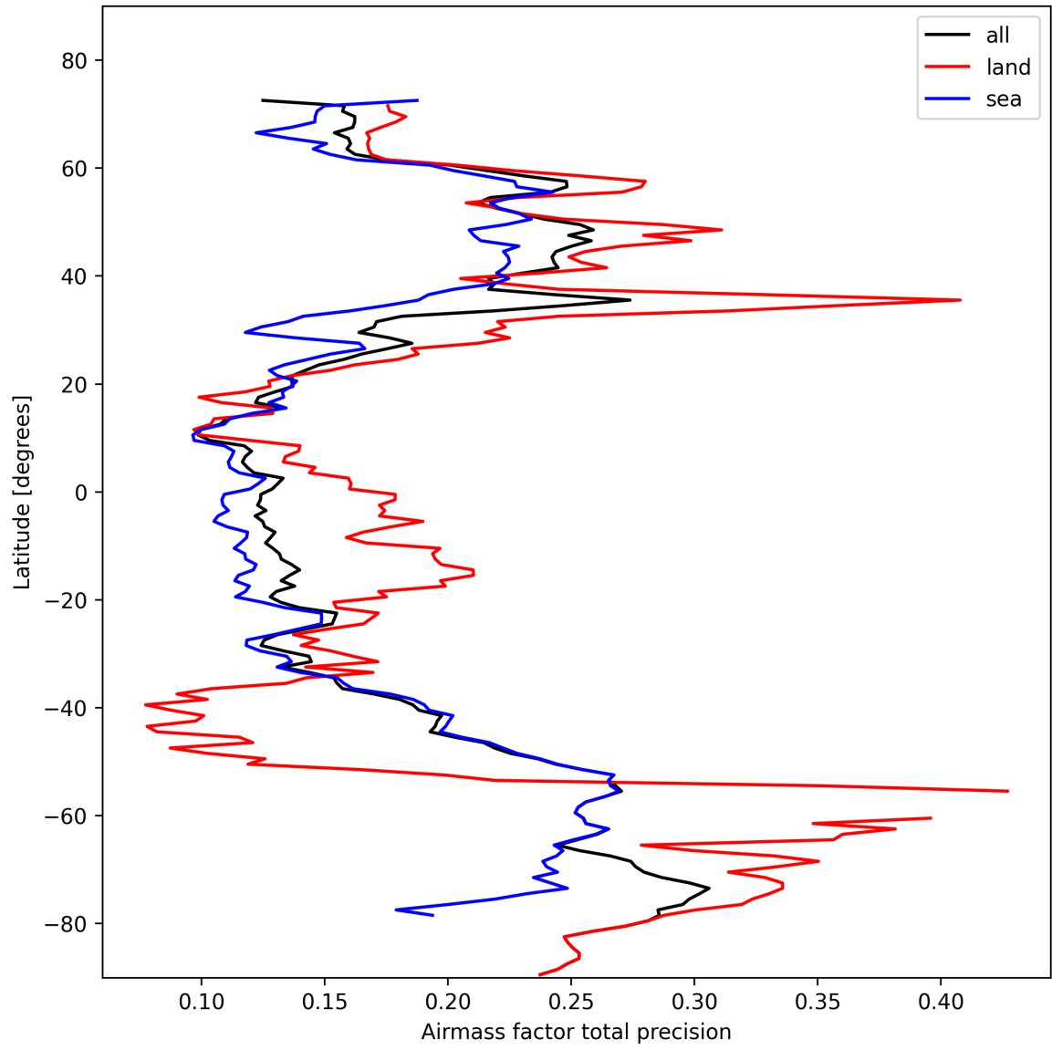
Figure 25: Zonal average of “Airmass factor total precision” for 2025-02-13 to 2025-02-14.
