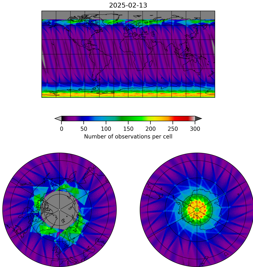
Figure 17: Map of the number of observations for 2025-02-13 to 2025-02-14
