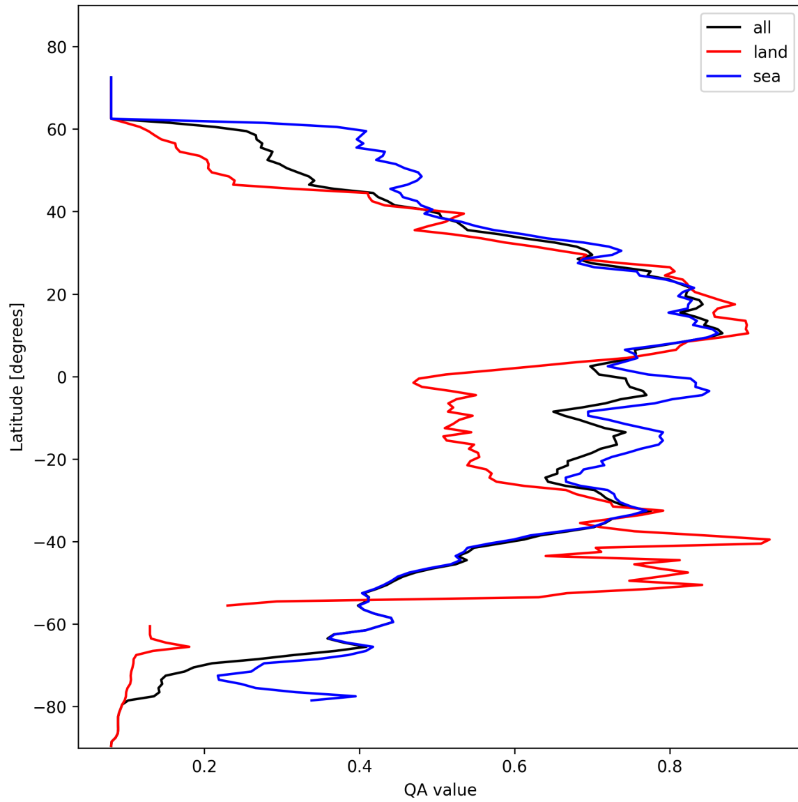
Figure 18: Zonal average of “QA value” for 2025-02-13 to 2025-02-14.
