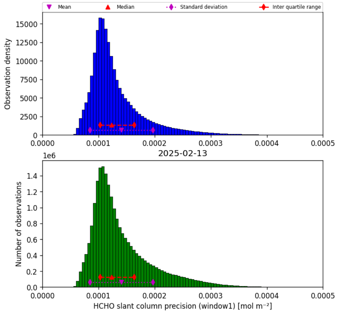
Figure 37: Histogram of “HCHO slant column precision (window1)” for 2025-02-13 to 2025-02-14
