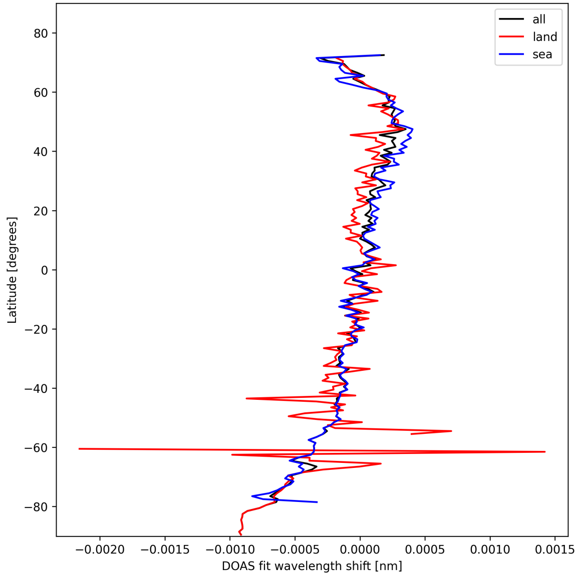
Figure 28: Zonal average of “DOAS fit wavelength shift” for 2025-02-13 to 2025-02-14.
