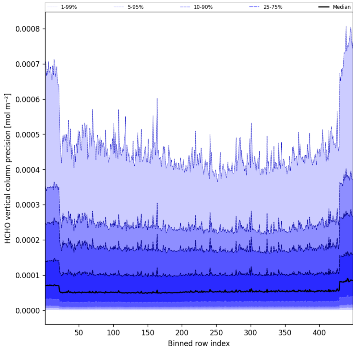
Figure 48: Along track statistics of “HCHO vertical column precision” for 2025-02-13 to 2025-02-14
