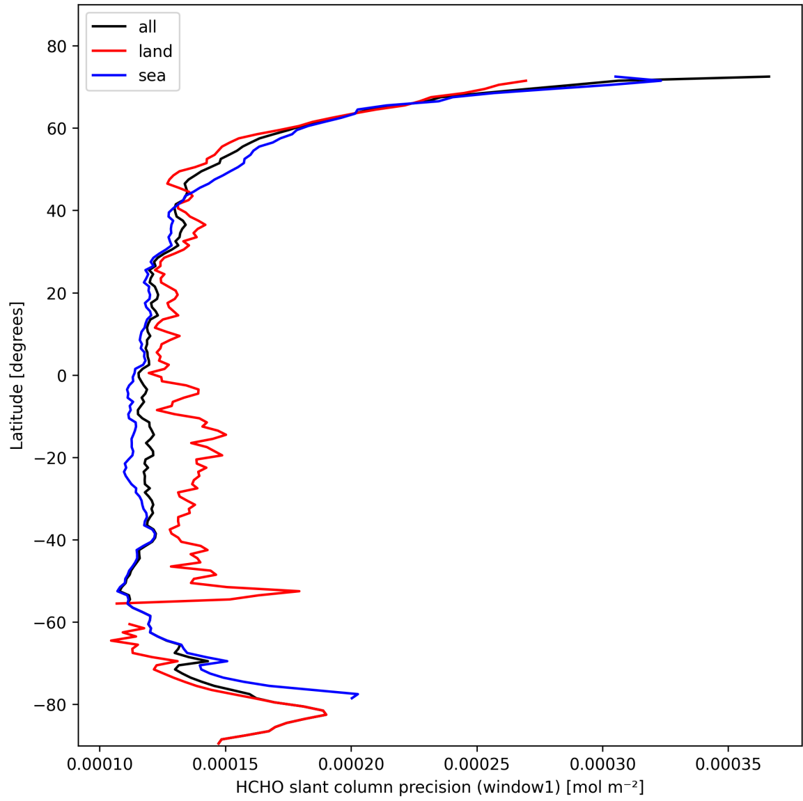
Figure 23: Zonal average of “HCHO slant column precision (window1)” for 2025-02-13 to 2025-02-14.
