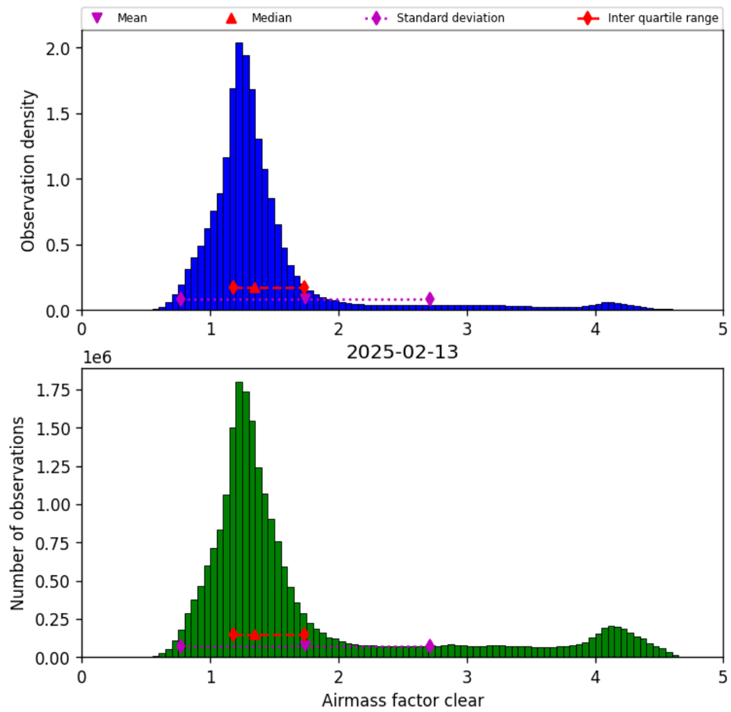
Figure 40: Histogram of “Airmass factor clear” for 2025-02-13 to 2025-02-14
