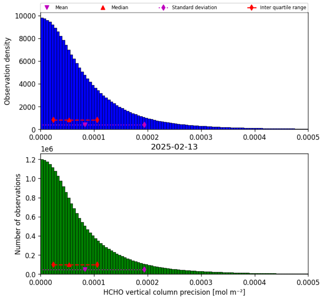
Figure 34: Histogram of “HCHO vertical column precision” for 2025-02-13 to 2025-02-14
