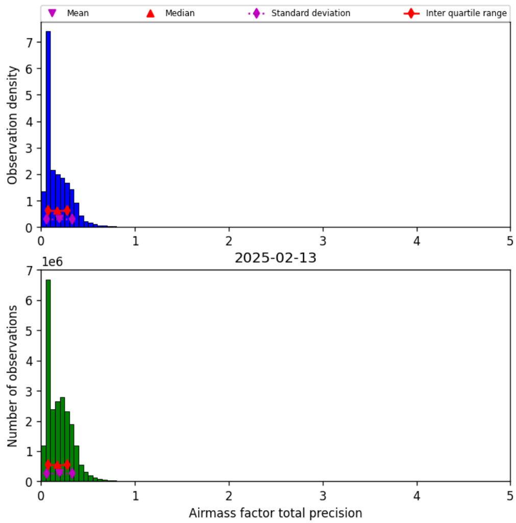
Figure 39: Histogram of “Airmass factor total precision” for 2025-02-13 to 2025-02-14
