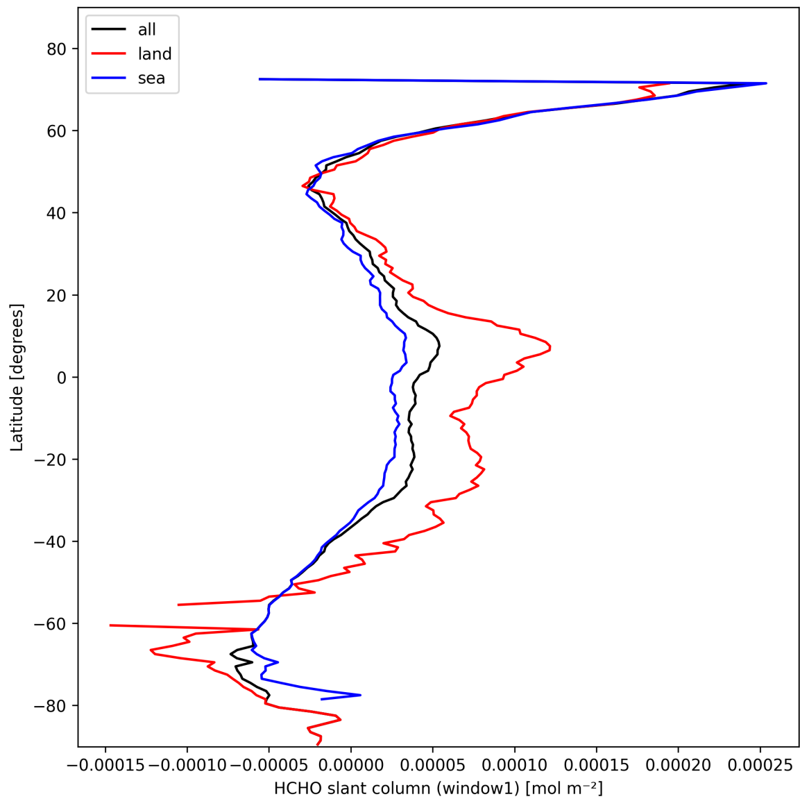
Figure 22: Zonal average of “HCHO slant column (window1)” for 2025-02-13 to 2025-02-14.
