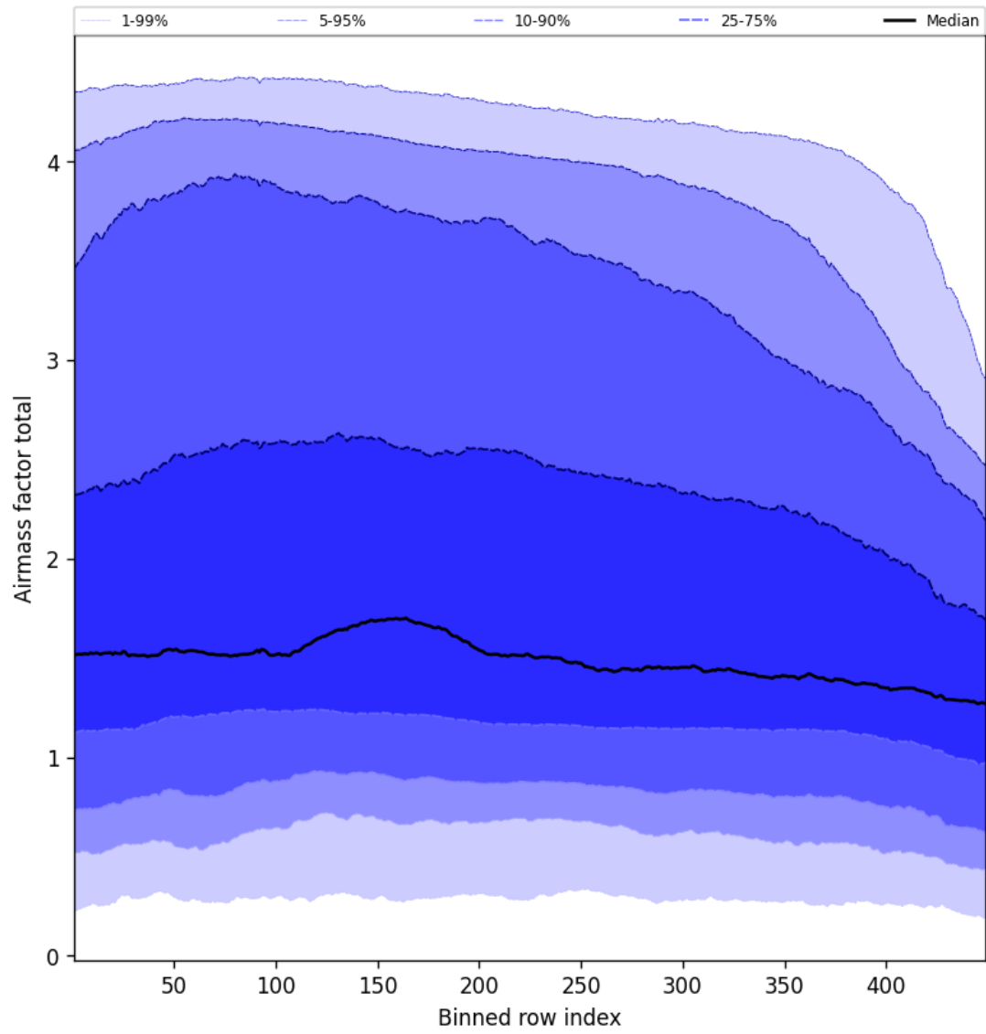
Figure 52: Along track statistics of “Airmass factor total” for 2025-02-13 to 2025-02-14
