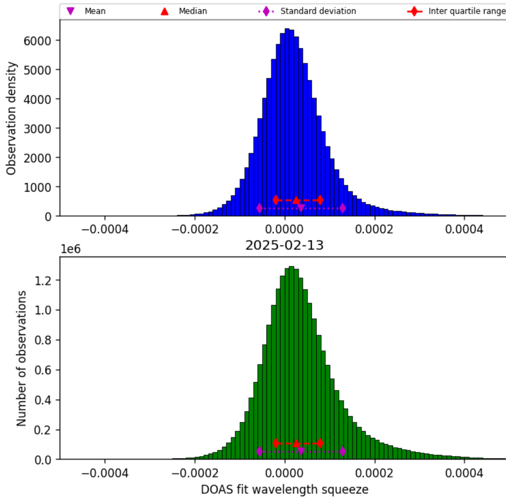
Figure 43: Histogram of “DOAS fit wavelength squeeze” for 2025-02-13 to 2025-02-14
