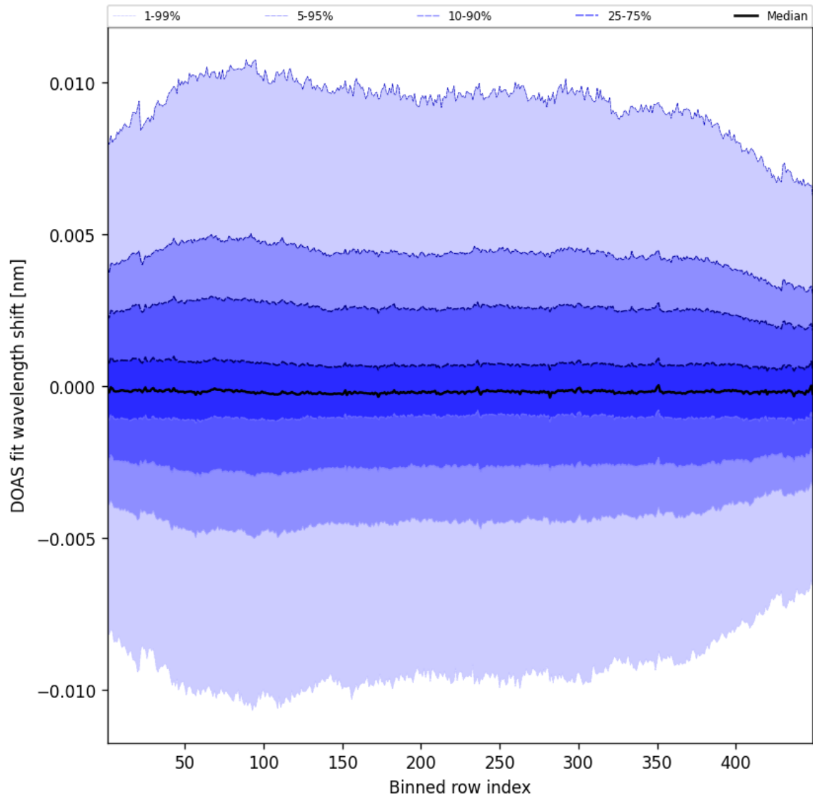
Figure 56: Along track statistics of “DOAS fit wavelength shift” for 2025-02-13 to 2025-02-14
