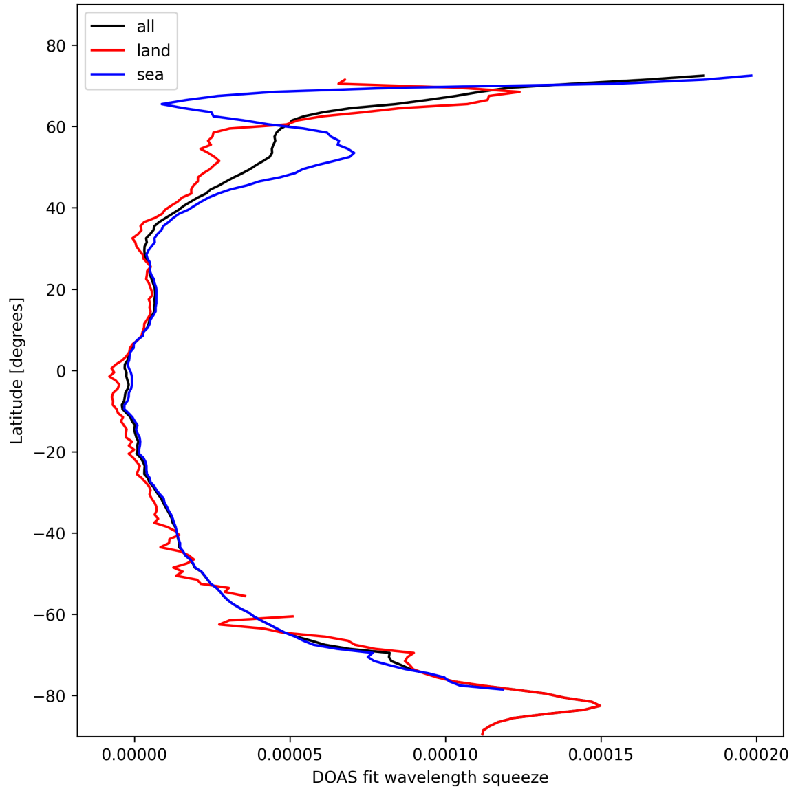
Figure 29: Zonal average of “DOAS fit wavelength squeeze” for 2025-02-13 to 2025-02-14.
