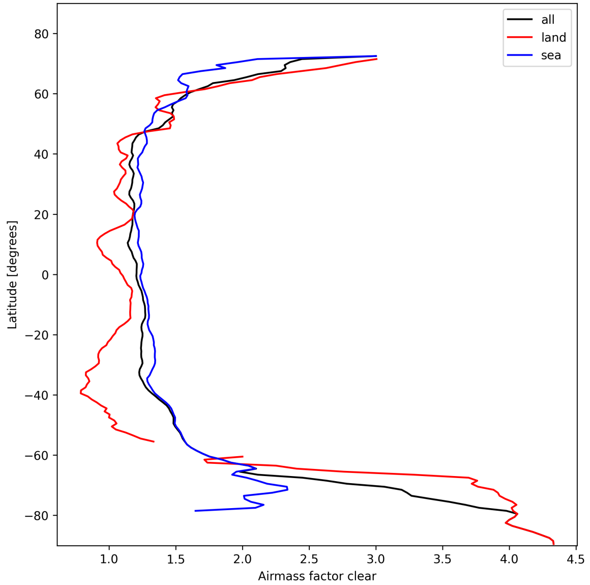
Figure 26: Zonal average of “Airmass factor clear” for 2025-02-13 to 2025-02-14.
