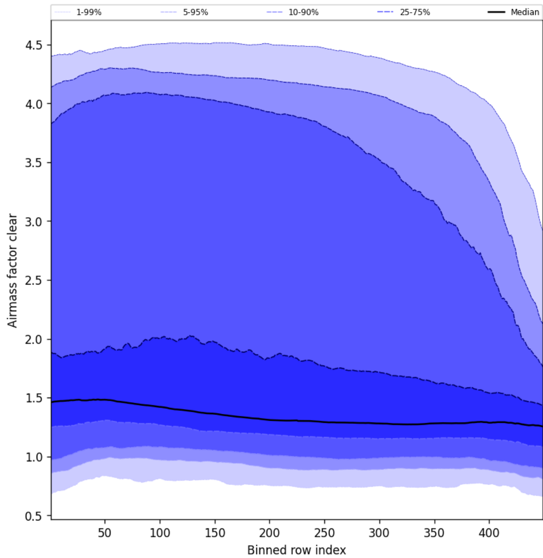
Figure 54: Along track statistics of “Airmass factor clear” for 2025-02-13 to 2025-02-14
