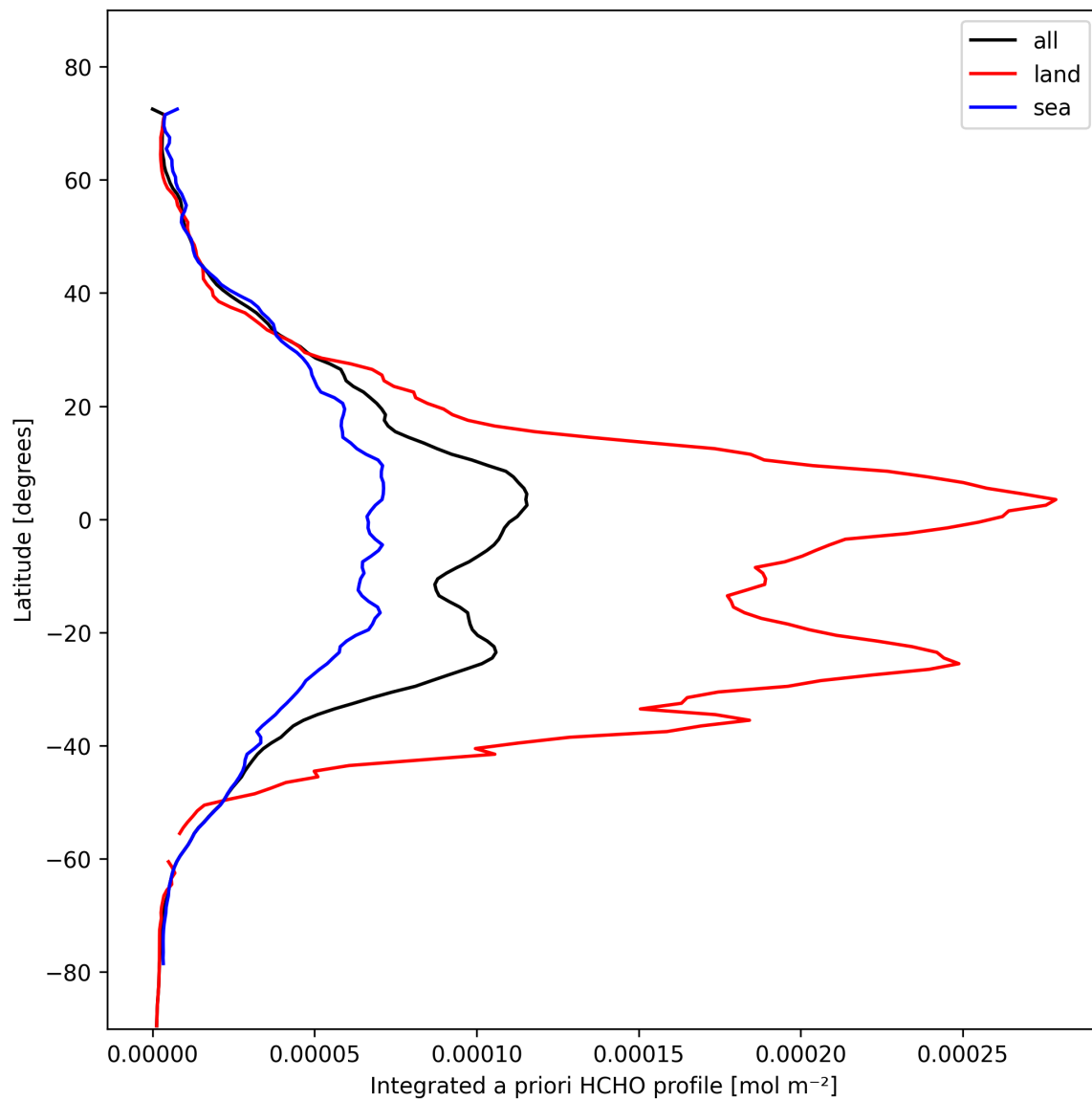
Figure 27: Zonal average of “Integrated a priori HCHO profile” for 2025-02-13 to 2025-02-14.
