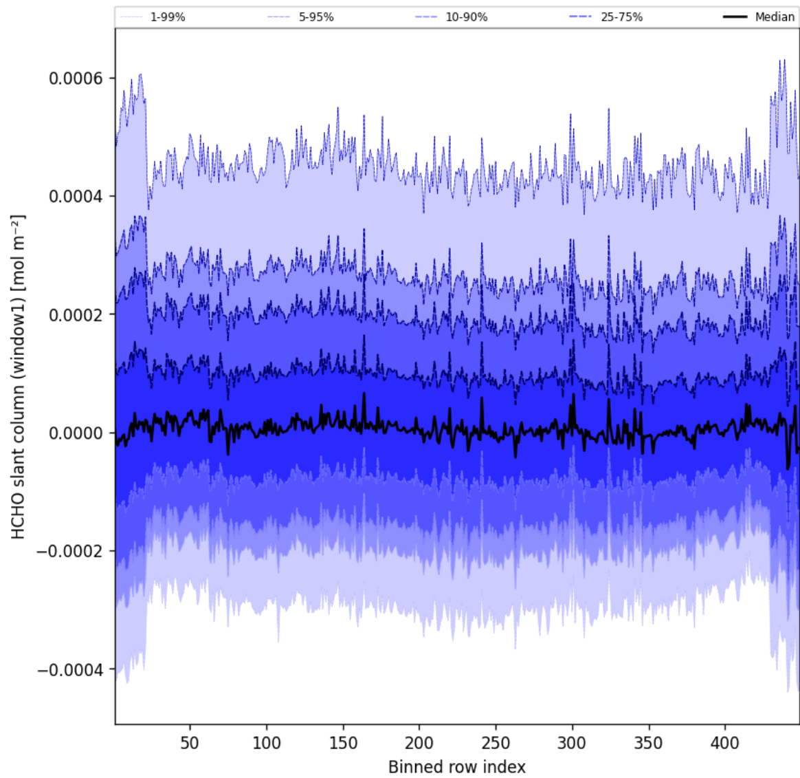
Figure 50: Along track statistics of “HCHO slant column (window1)” for 2025-02-13 to 2025-02-14
