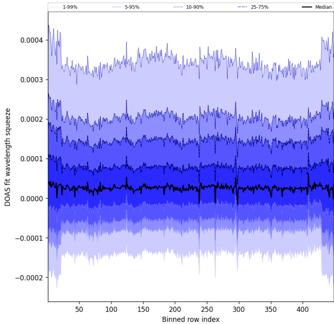
Figure 57: Along track statistics of “DOAS fit wavelength squeeze” for 2025-02-13 to 2025-02-14
