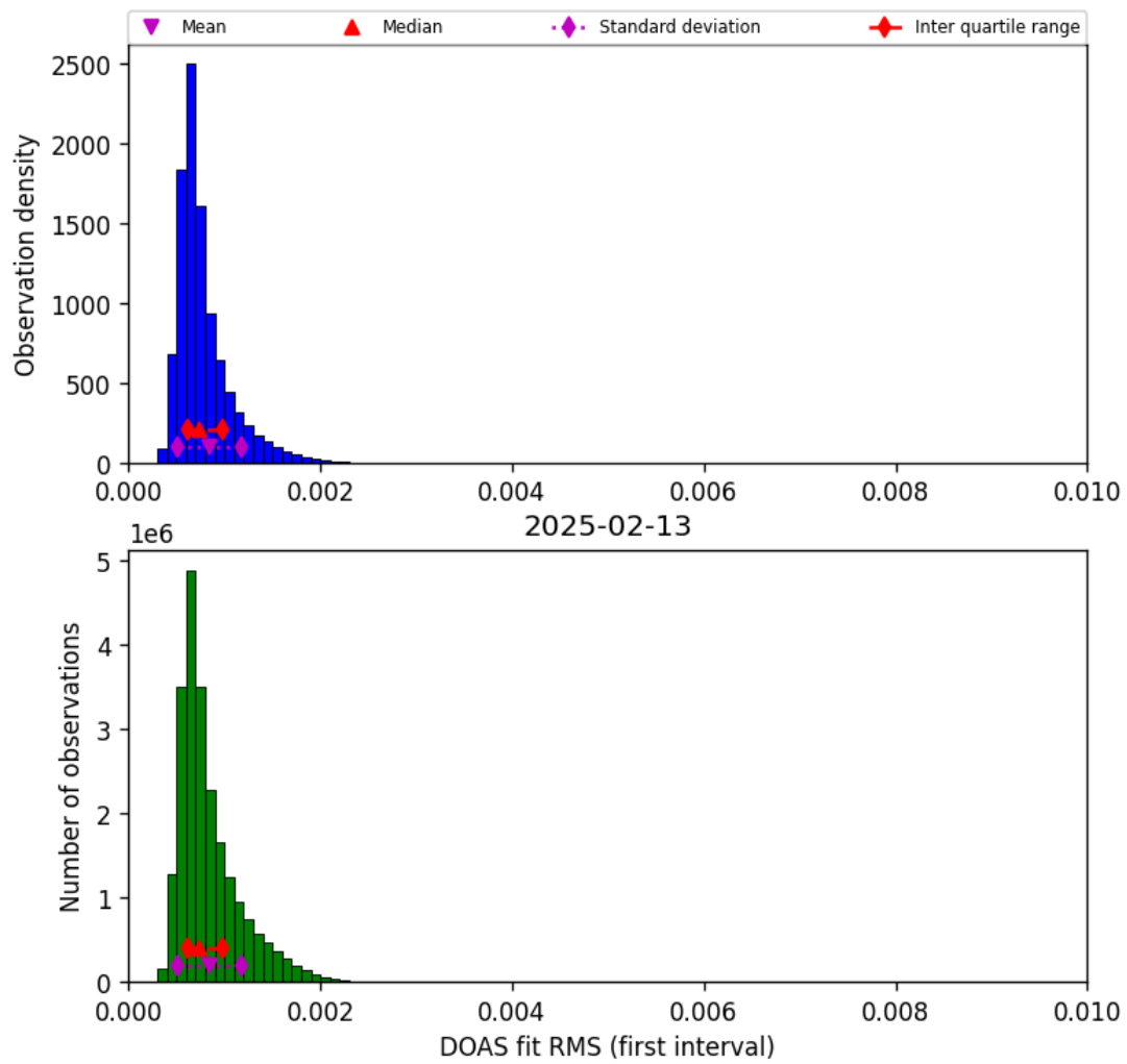
Figure 44: Histogram of “DOAS fit RMS (first interval)” for 2025-02-13 to 2025-02-14
