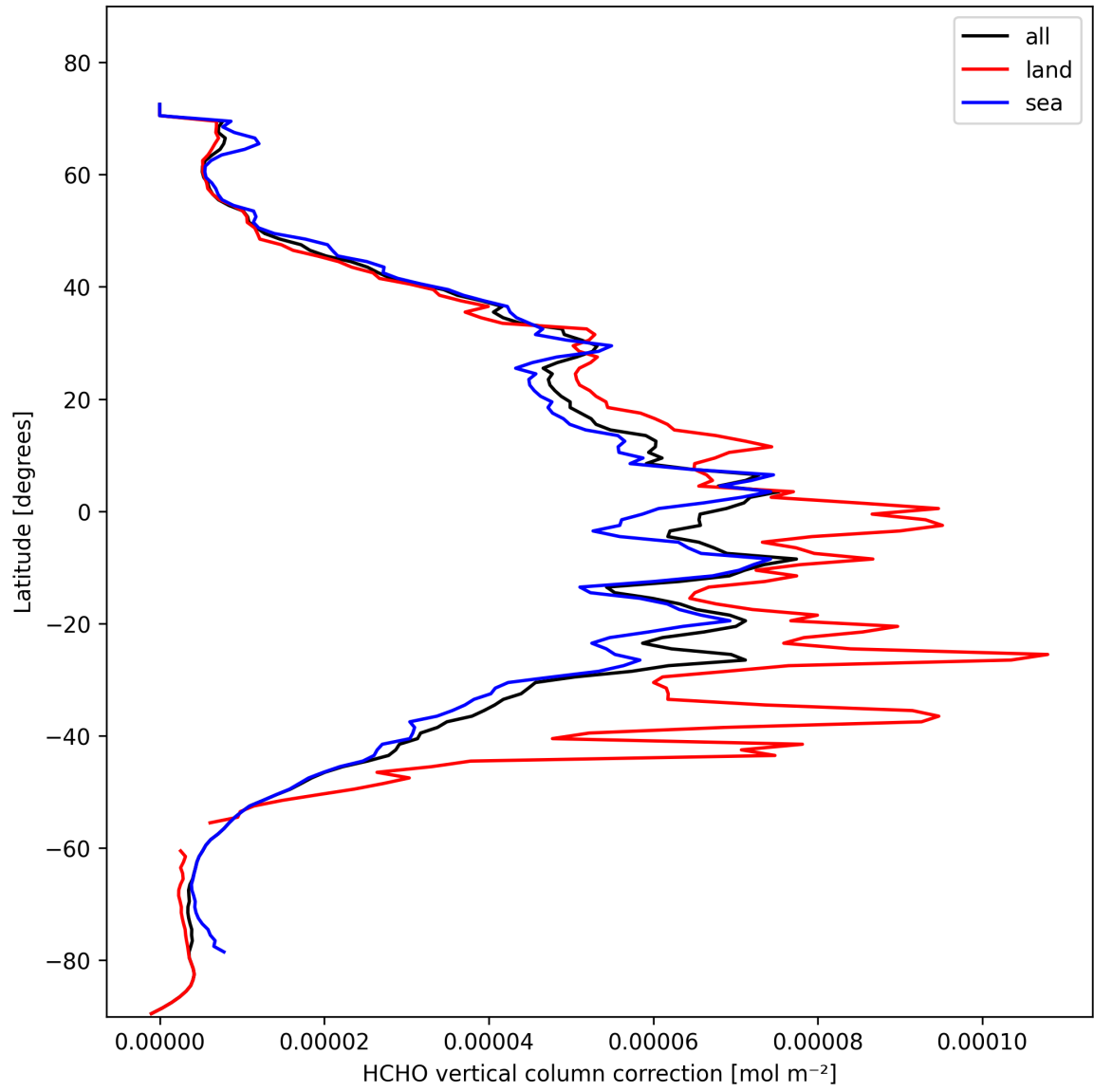
Figure 21: Zonal average of “HCHO vertical column correction” for 2025-02-13 to 2025-02-14.
