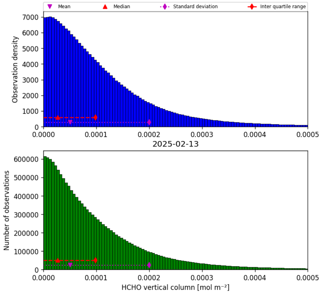
Figure 33: Histogram of “HCHO vertical column” for 2025-02-13 to 2025-02-14
