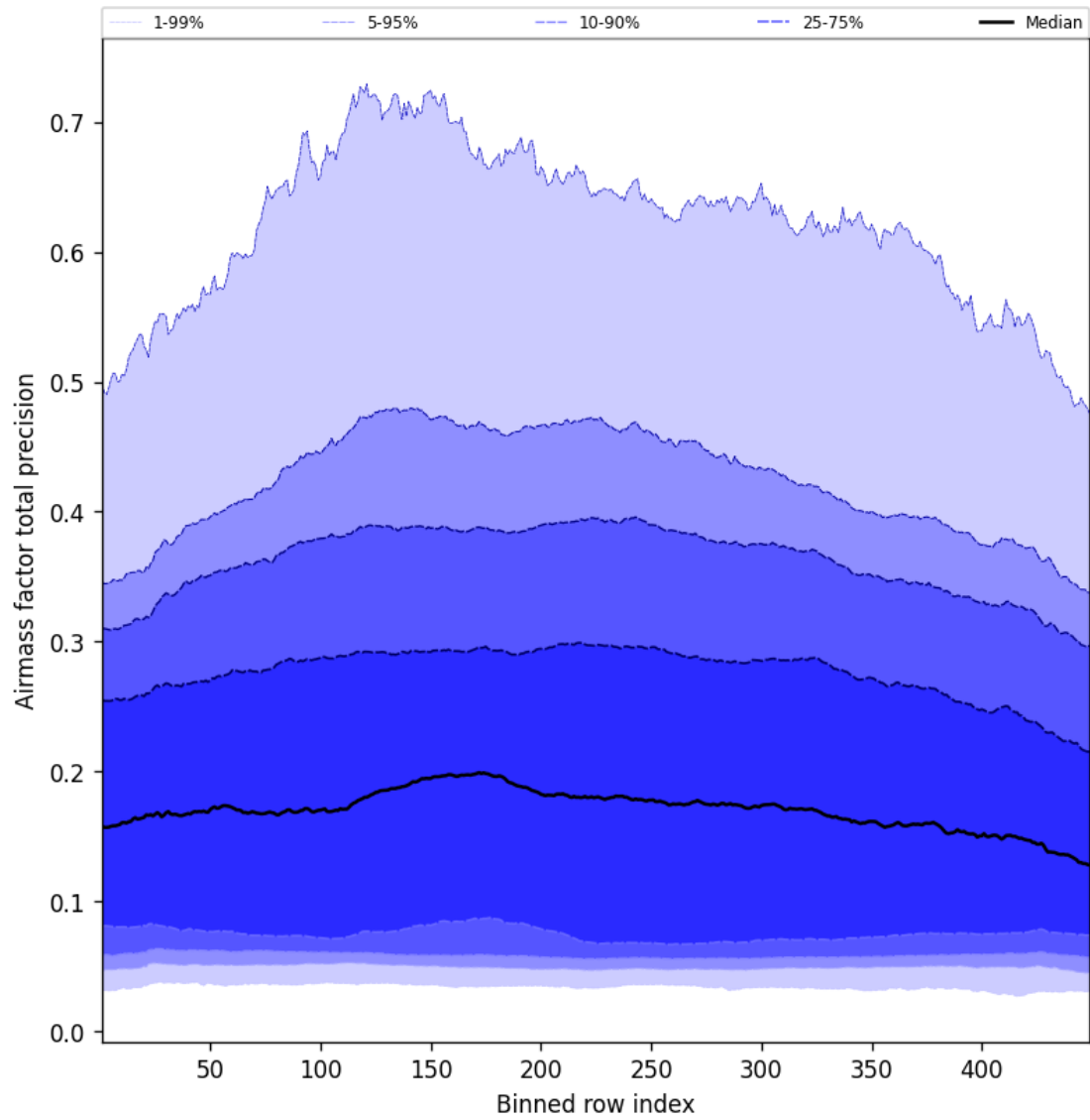
Figure 53: Along track statistics of “Airmass factor total precision” for 2025-02-13 to 2025-02-14
