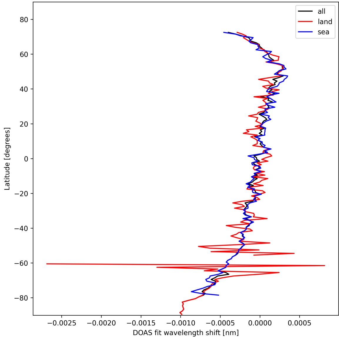
Figure 28: Zonal average of "DOAS fit wavelength shift" for 2025-02-14 to 2025-02-15.
