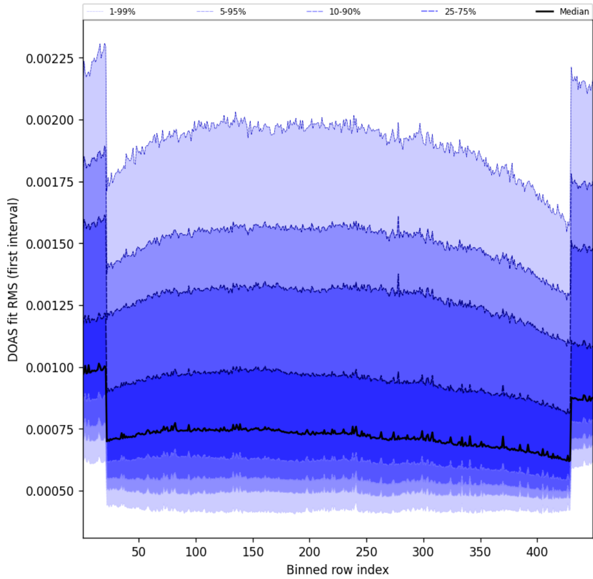
Figure 58: Along track statistics of “DOAS fit RMS (first interval)” for 2025-02-14 to 2025-02-15
