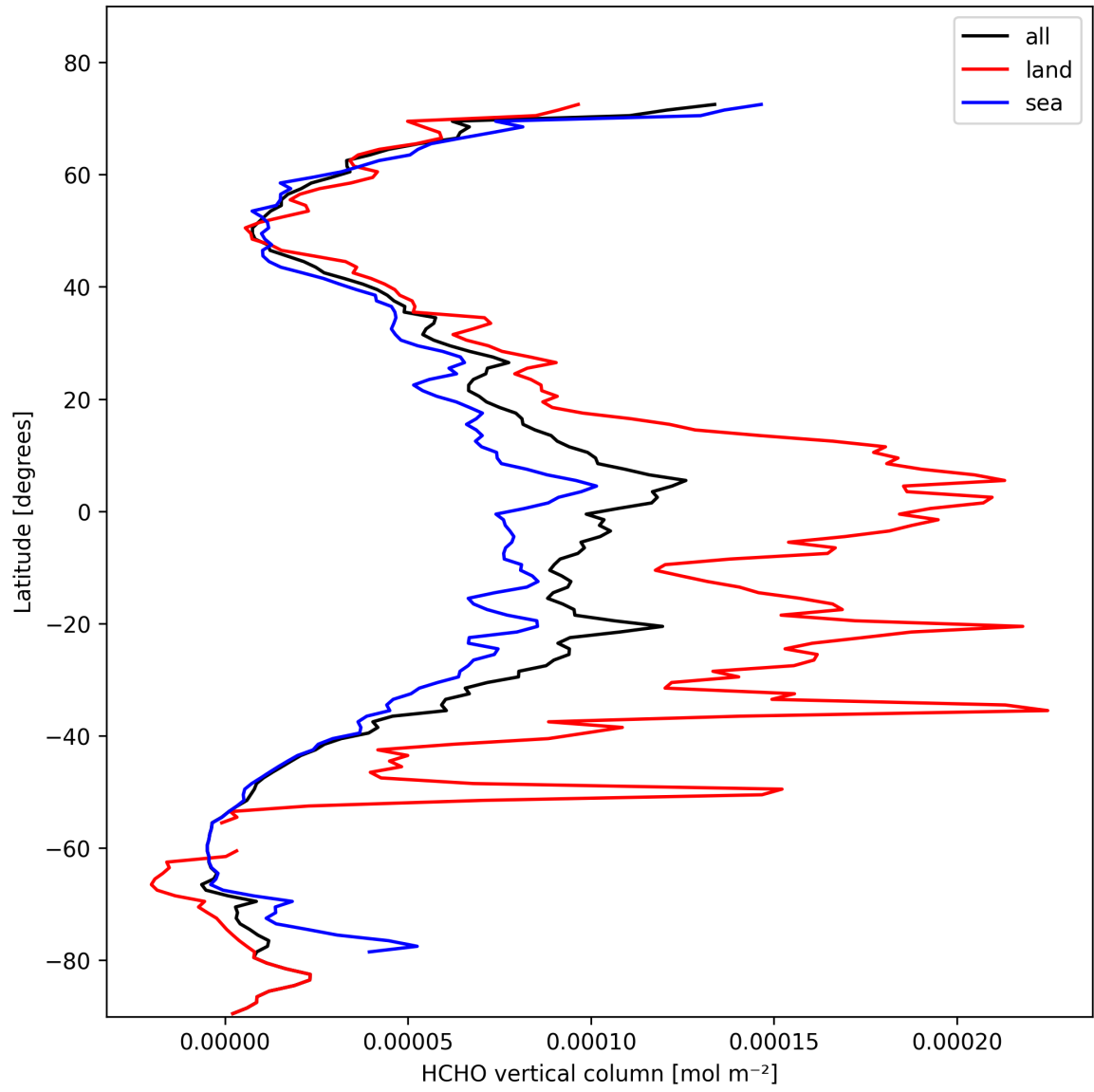
Figure 19: Zonal average of “HCHO vertical column” for 2025-02-14 to 2025-02-15.
