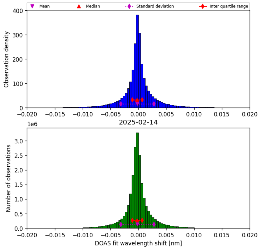
Figure 42: Histogram of “DOAS fit wavelength shift” for 2025-02-14 to 2025-02-15
