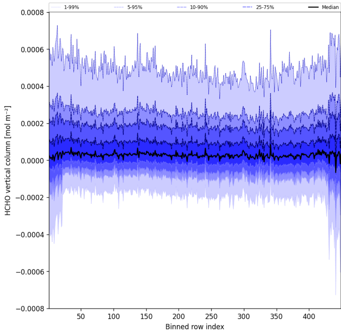
Figure 47: Along track statistics of “HCHO vertical column” for 2025-02-14 to 2025-02-15
