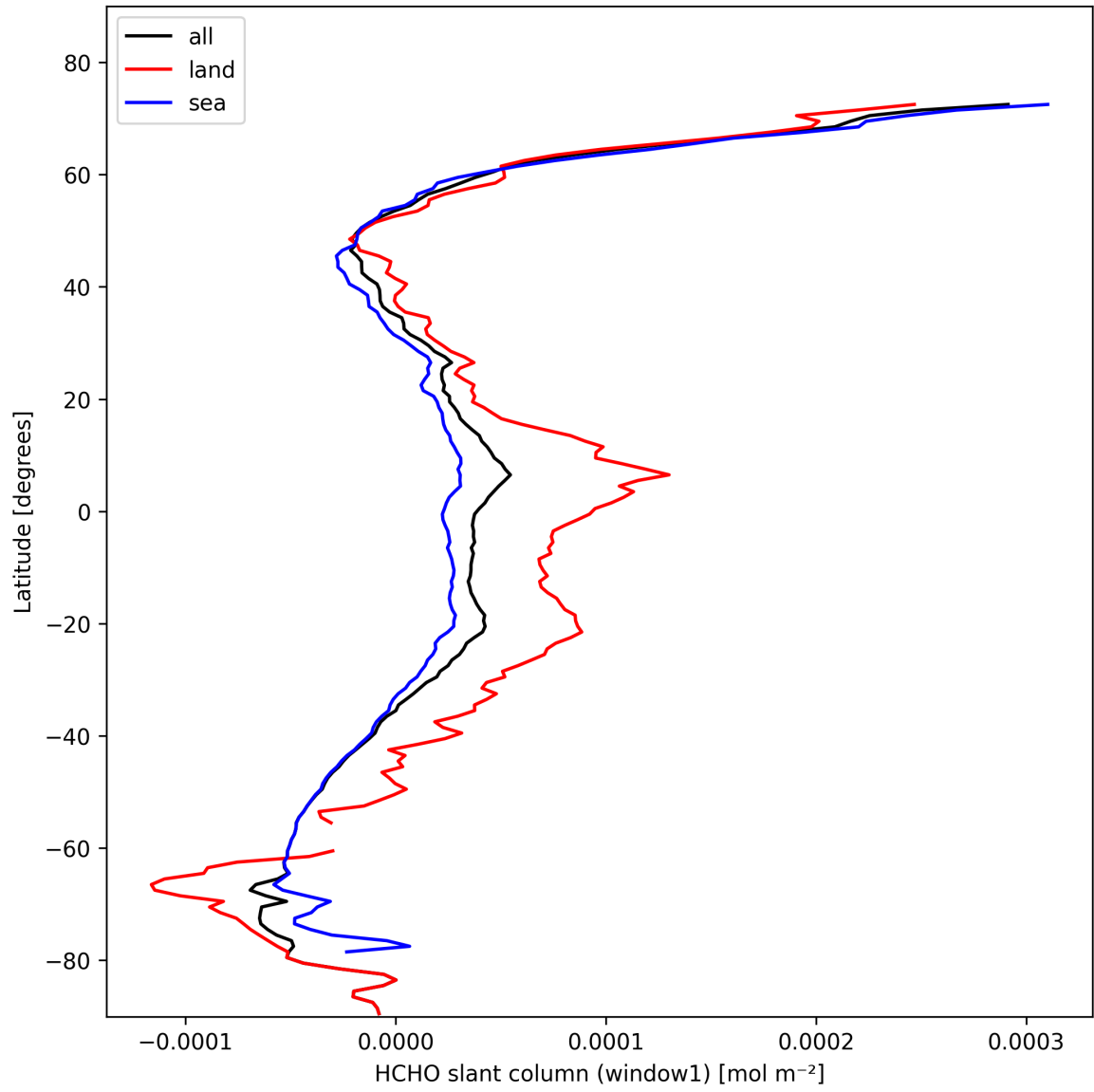
Figure 22: Zonal average of “HCHO slant column (window1)” for 2025-02-14 to 2025-02-15.
