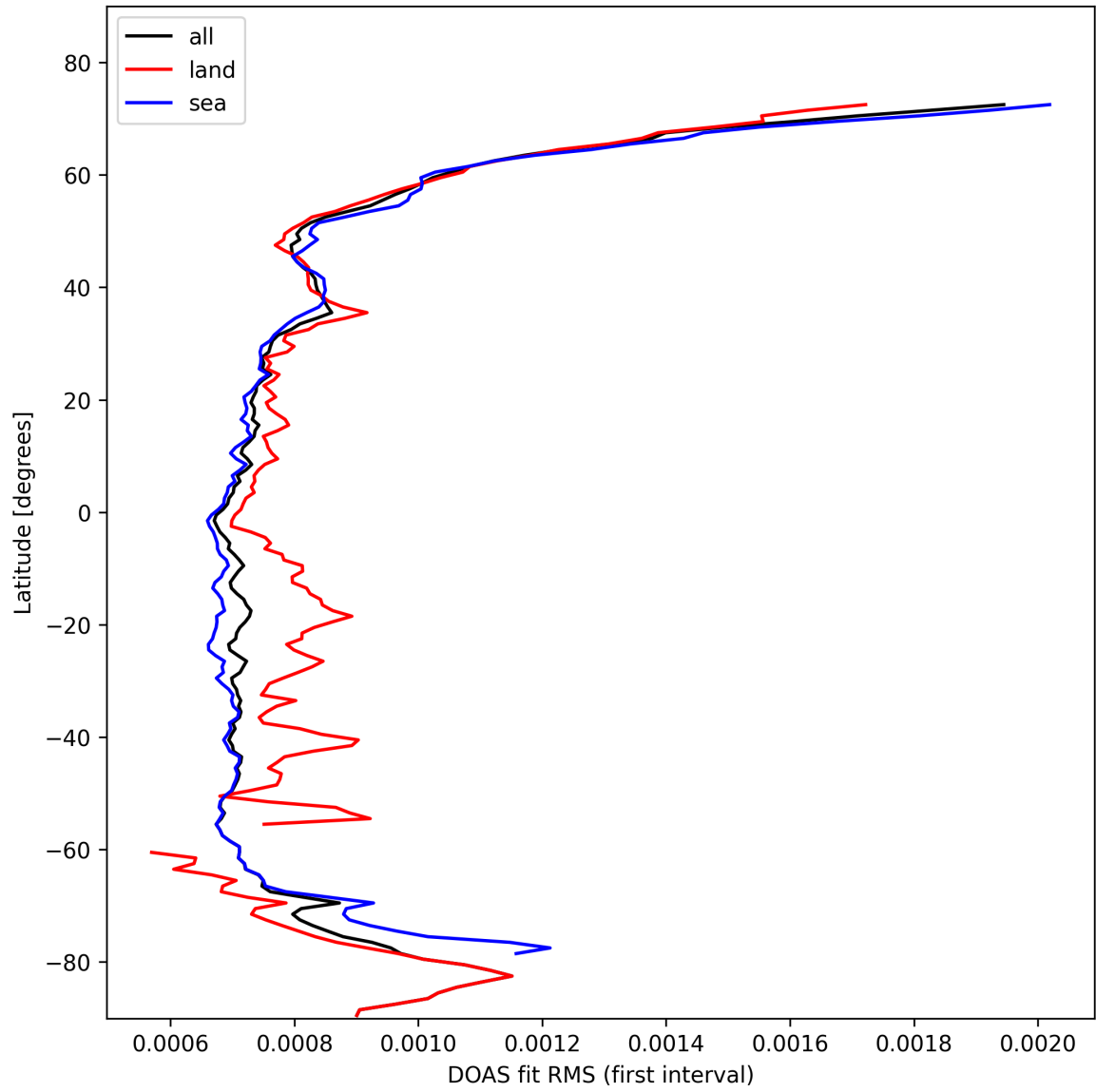
Figure 30: Zonal average of "DOAS fit RMS (first interval)" for 2025-02-14 to 2025-02-15.
