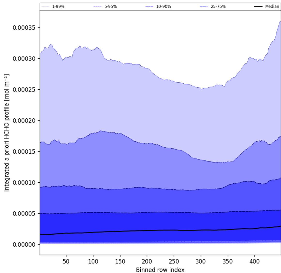
Figure 55: Along track statistics of "Integrated a priori HCHO profile" for 2025-02-14 to 2025-02-15
