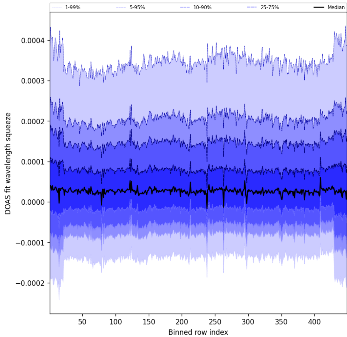
Figure 57: Along track statistics of “DOAS fit wavelength squeeze” for 2025-02-14 to 2025-02-15
