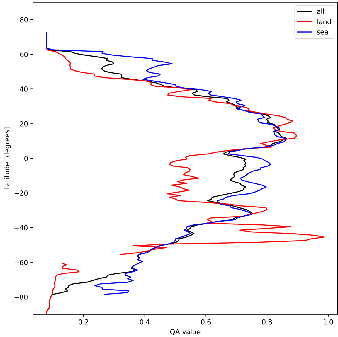
Figure 18: Zonal average of “QA value” for 2025-02-14 to 2025-02-15.
