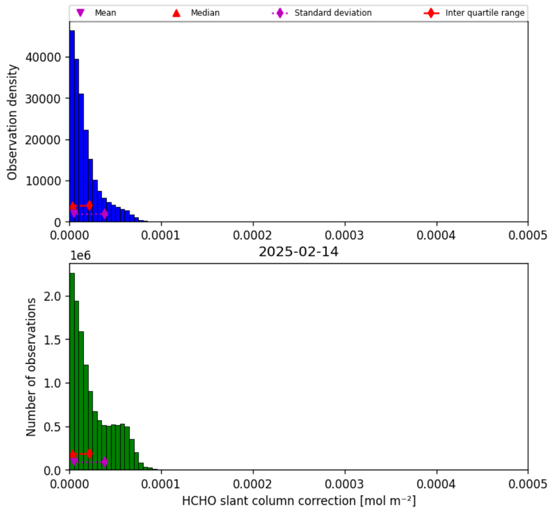
Figure 45: Histogram of “HCHO slant column correction” for 2025-02-14 to 2025-02-15
