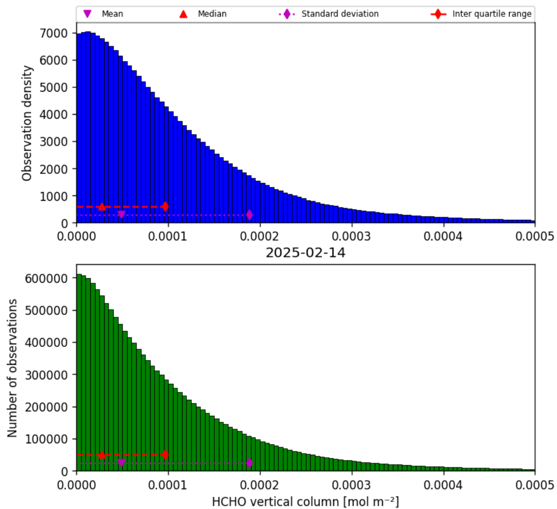
Figure 33: Histogram of “HCHO vertical column” for 2025-02-14 to 2025-02-15
