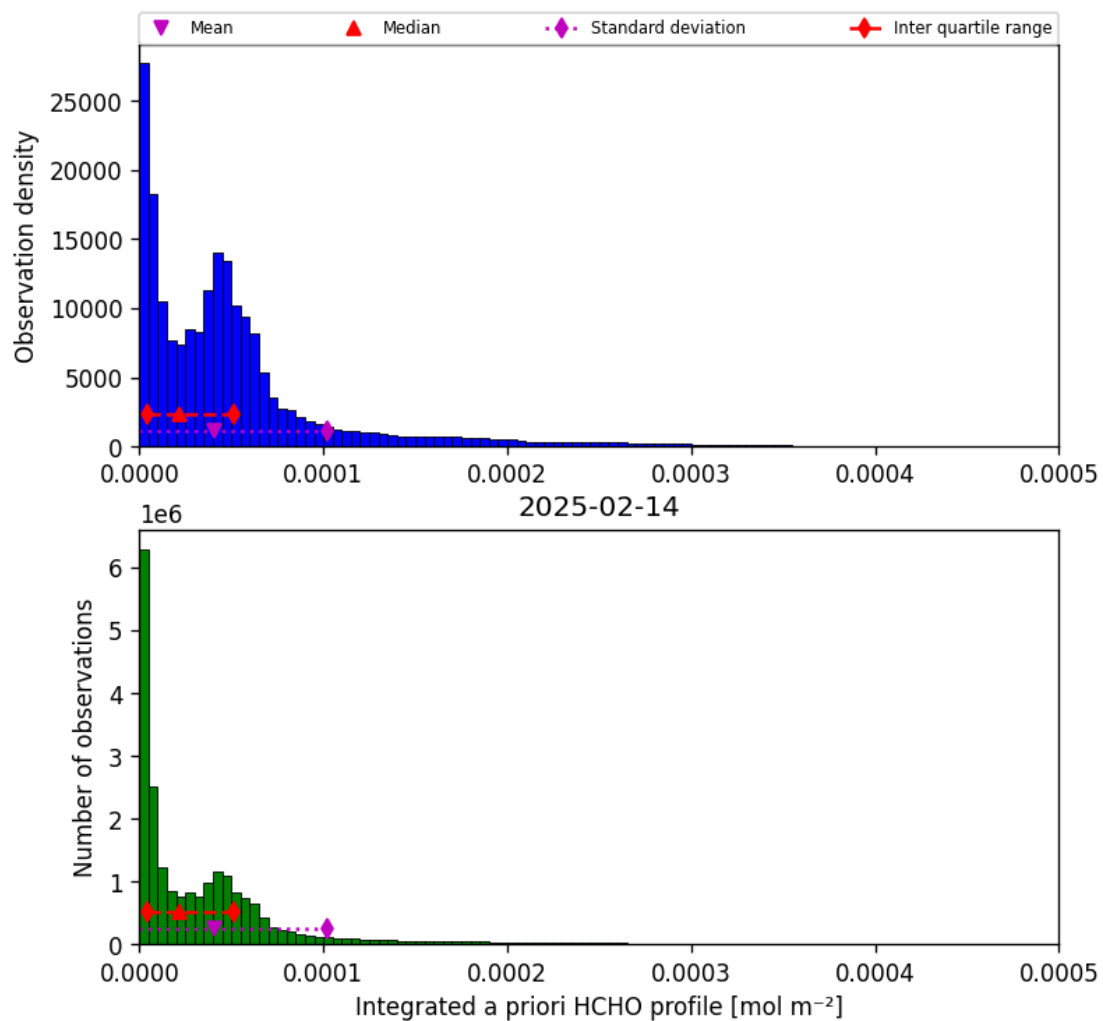
Figure 41: Histogram of “Integrated a priori HCHO profile” for 2025-02-14 to 2025-02-15
