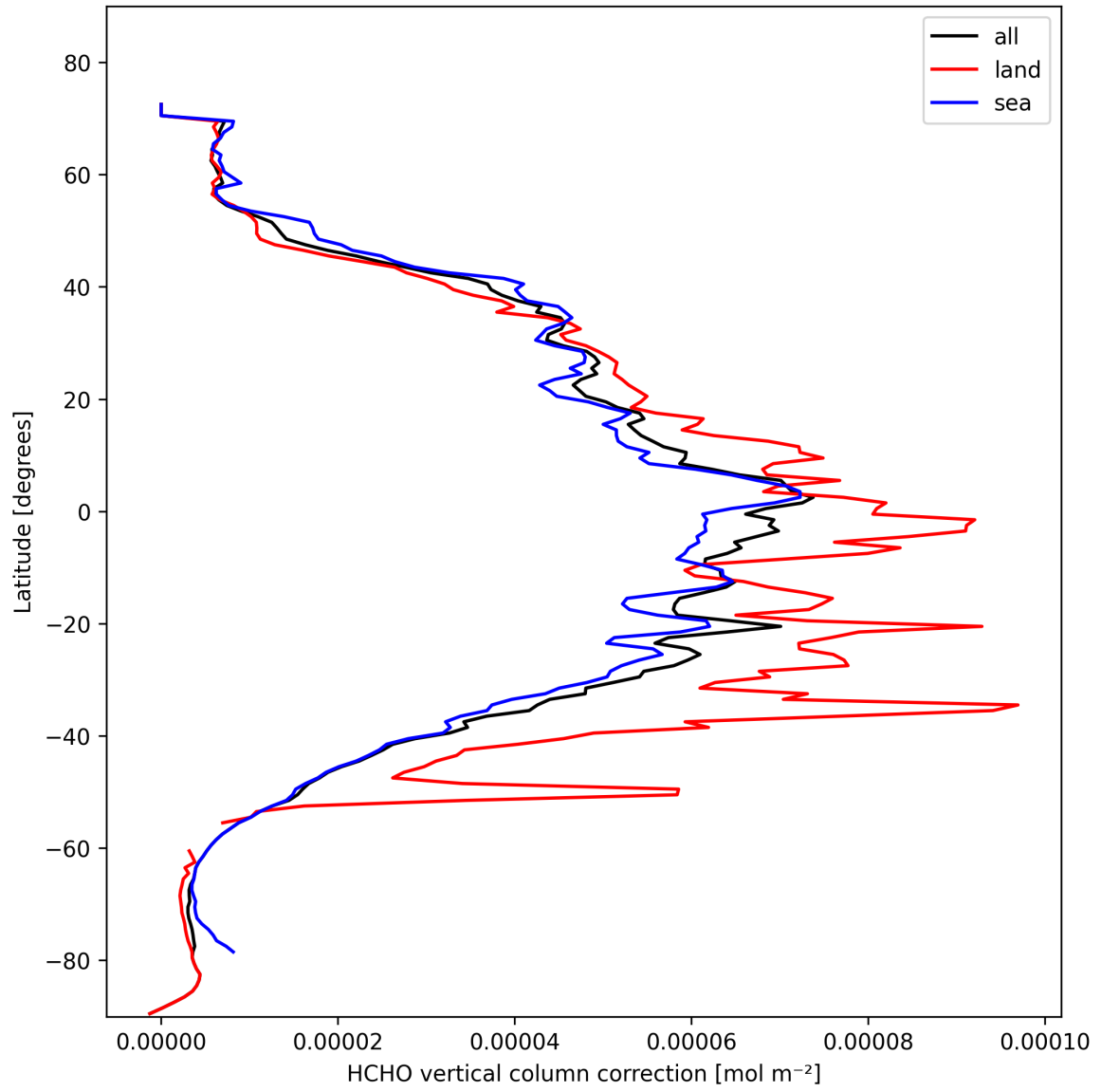
Figure 21: Zonal average of “HCHO vertical column correction” for 2025-02-14 to 2025-02-15.
