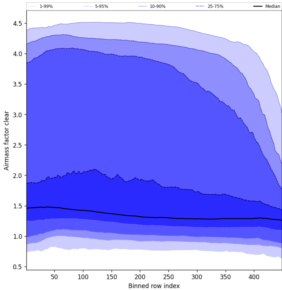
Figure 54: Along track statistics of “Airmass factor clear” for 2025-02-14 to 2025-02-15
