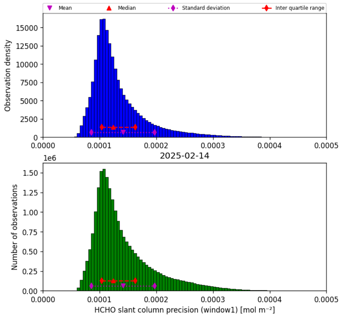
Figure 37: Histogram of “HCHO slant column precision (window1)” for 2025-02-14 to 2025-02-15
