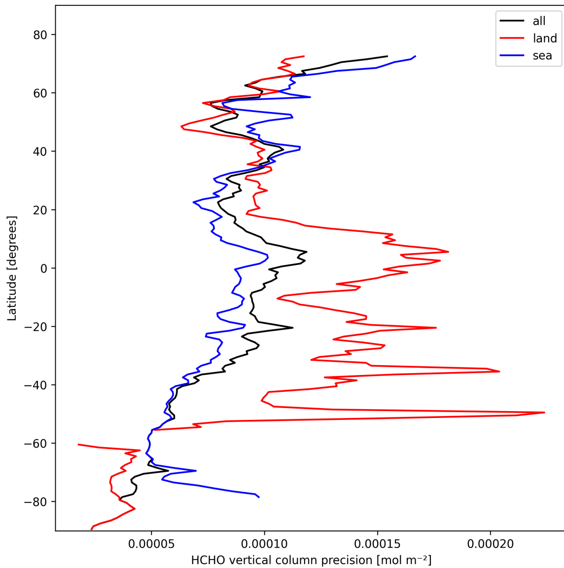
Figure 20: Zonal average of “HCHO vertical column precision” for 2025-02-14 to 2025-02-15.
