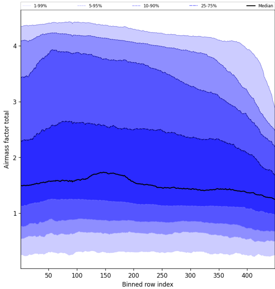
Figure 52: Along track statistics of “Airmass factor total” for 2025-02-14 to 2025-02-15
