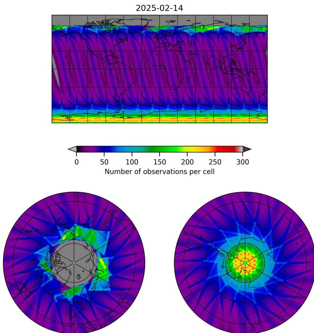
Figure 17: Map of the number of observations for 2025-02-14 to 2025-02-15
