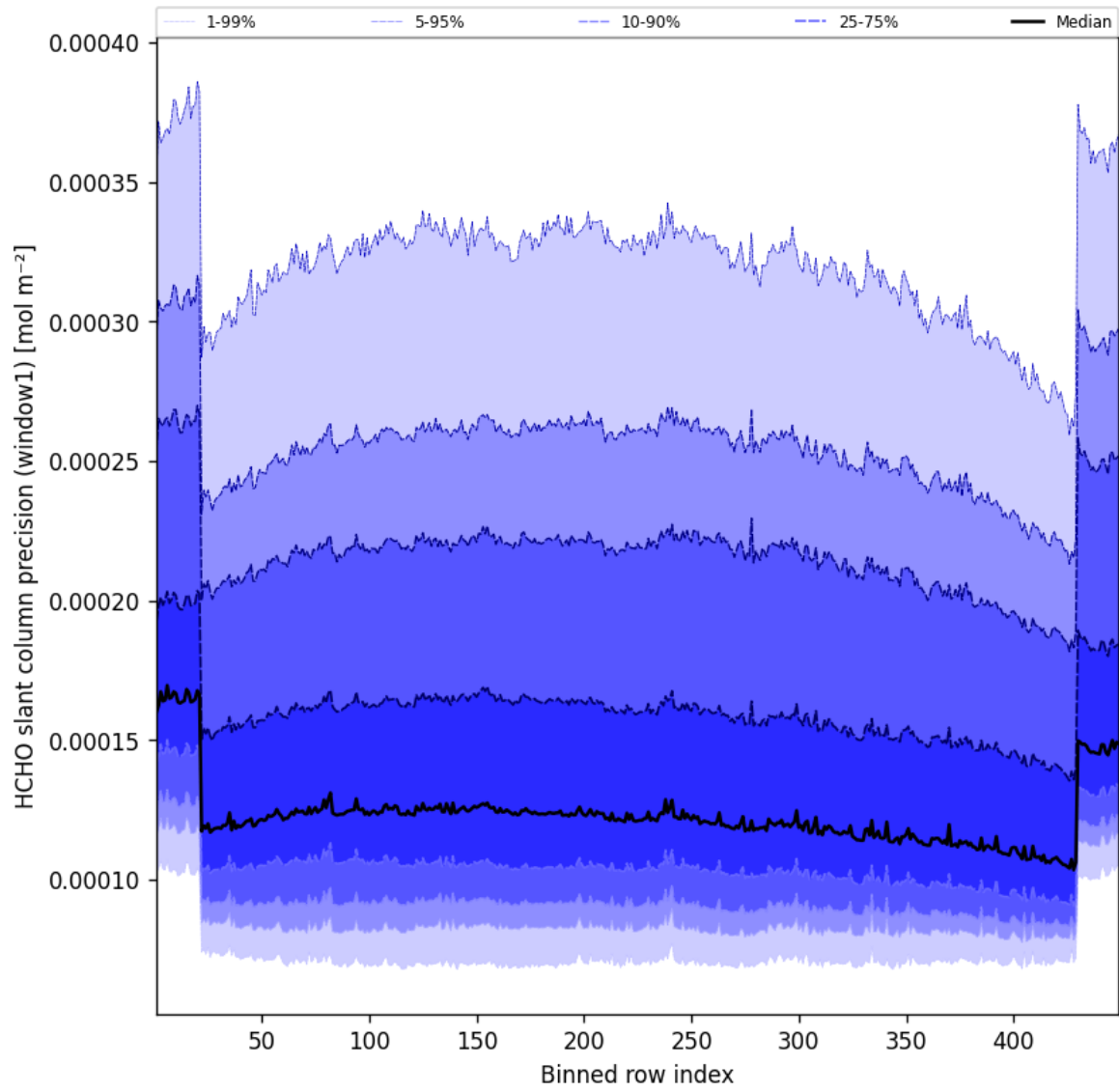
Figure 51: Along track statistics of “HCHO slant column precision (window1)” for 2025-02-14 to 2025-02-15
