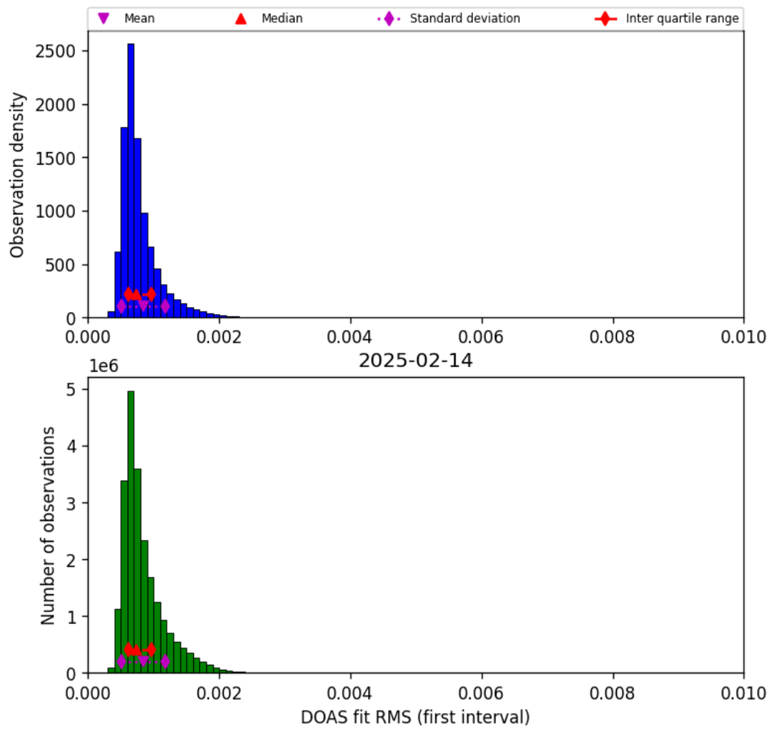
Figure 44: Histogram of “DOAS fit RMS (first interval)” for 2025-02-14 to 2025-02-15
