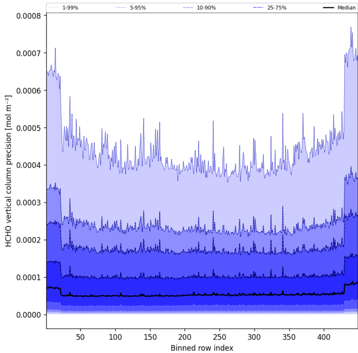
Figure 48: Along track statistics of “HCHO vertical column precision” for 2025-02-14 to 2025-02-15
