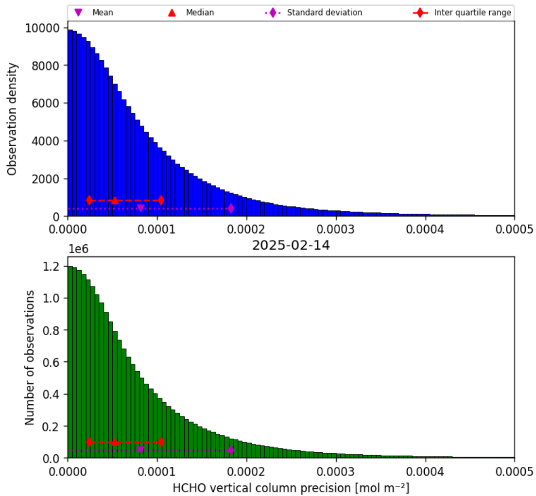
Figure 34: Histogram of “HCHO vertical column precision” for 2025-02-14 to 2025-02-15
