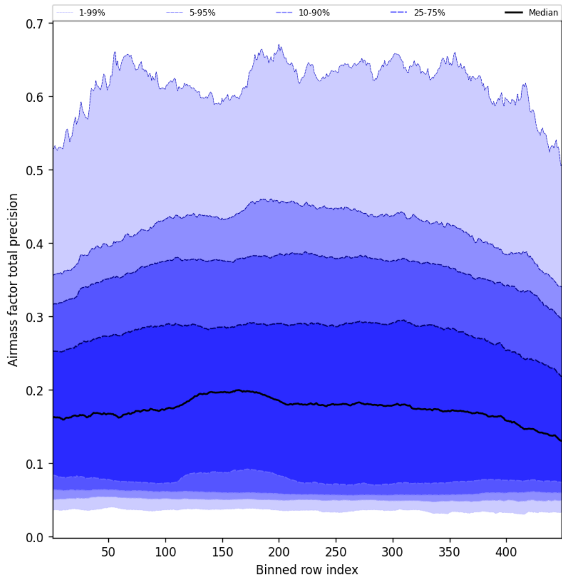
Figure 53: Along track statistics of “Airmass factor total precision” for 2025-02-14 to 2025-02-15
