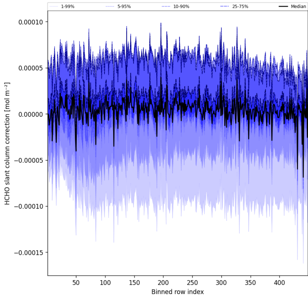
Figure 59: Along track statistics of “HCHO slant column correction” for 2025-02-14 to 2025-02-15
