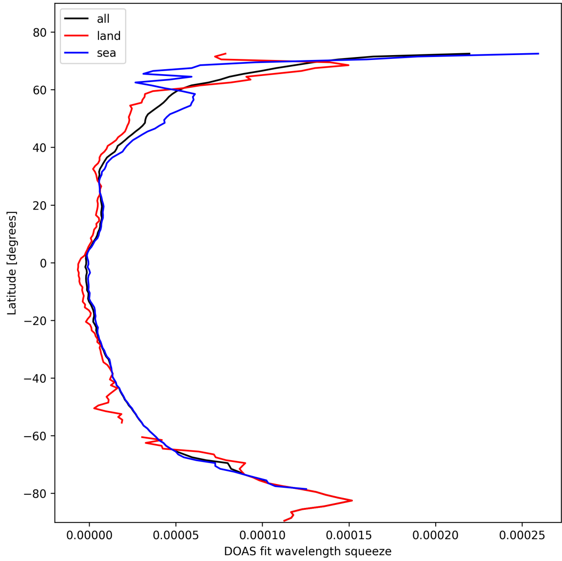
Figure 29: Zonal average of “DOAS fit wavelength squeeze” for 2025-02-14 to 2025-02-15.
