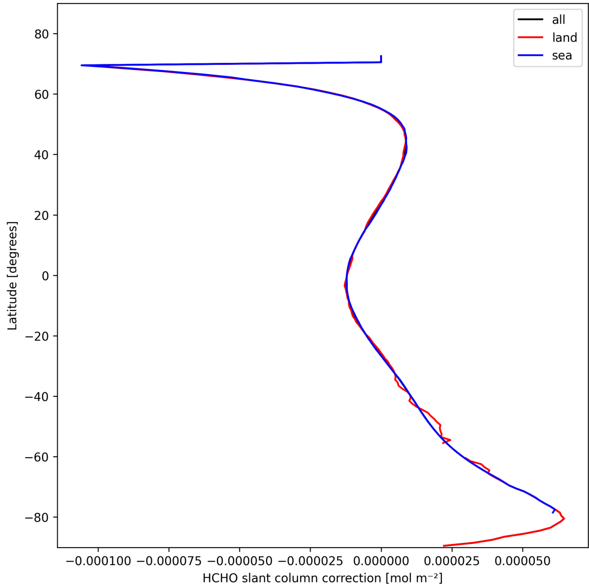
Figure 31: Zonal average of “HCHO slant column correction” for 2025-02-14 to 2025-02-15.
