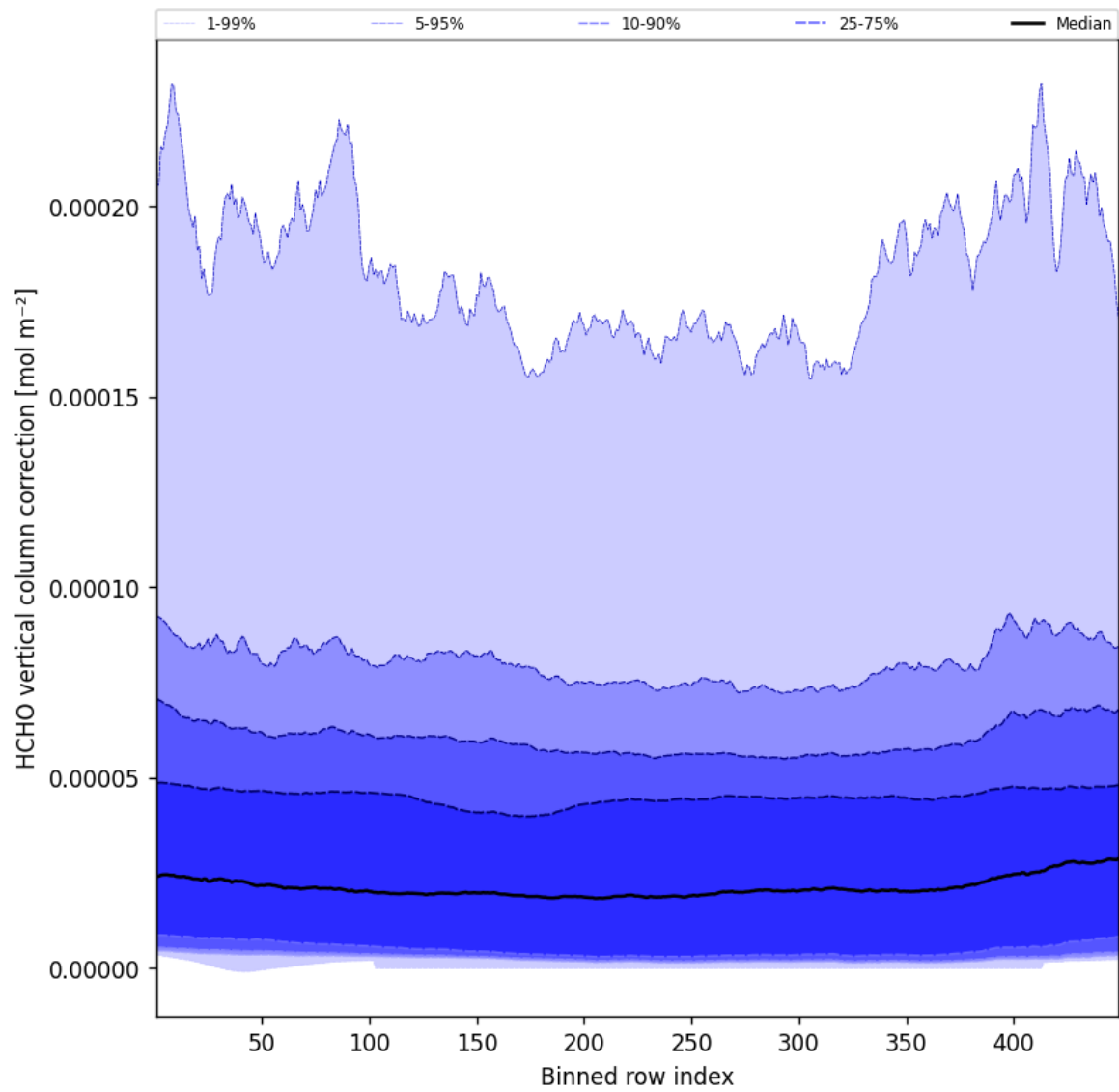
Figure 49: Along track statistics of “HCHO vertical column correction” for 2025-02-14 to 2025-02-15
