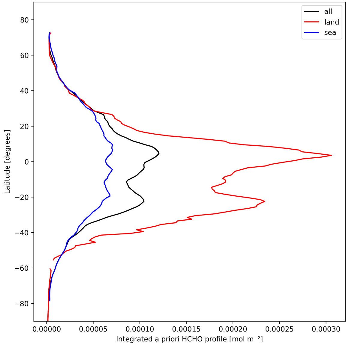
Figure 27: Zonal average of “Integrated a priori HCHO profile” for 2025-02-14 to 2025-02-15.
