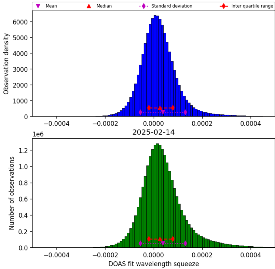
Figure 43: Histogram of “DOAS fit wavelength squeeze” for 2025-02-14 to 2025-02-15
