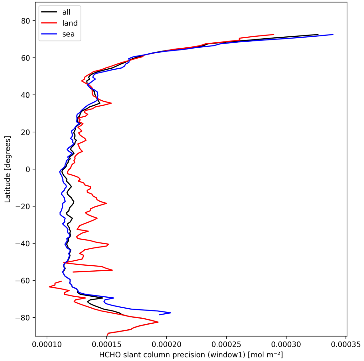
Figure 23: Zonal average of “HCHO slant column precision (window1)” for 2025-02-14 to 2025-02-15.
