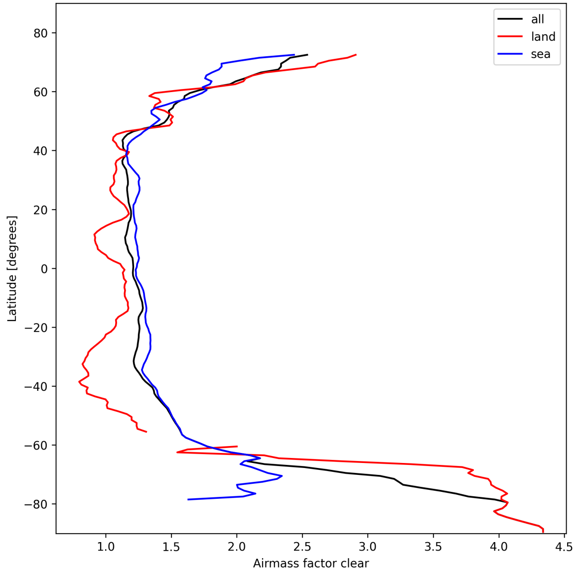
Figure 26: Zonal average of “Airmass factor clear” for 2025-02-14 to 2025-02-15.
