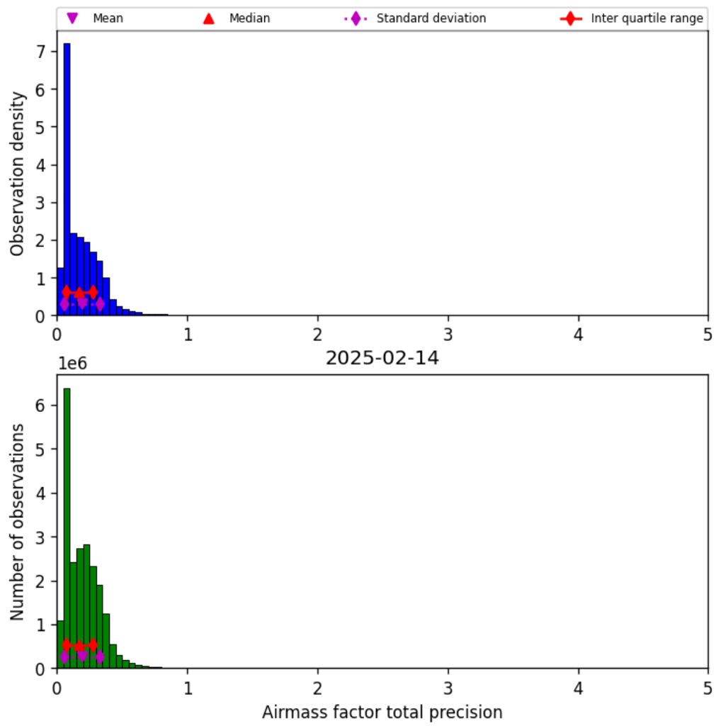
Figure 39: Histogram of “Airmass factor total precision” for 2025-02-14 to 2025-02-15
