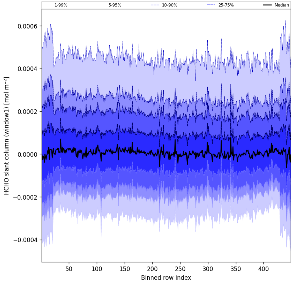
Figure 50: Along track statistics of “HCHO slant column (window1)” for 2025-02-14 to 2025-02-15
