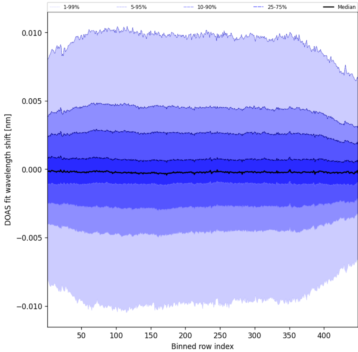
Figure 56: Along track statistics of “DOAS fit wavelength shift” for 2025-02-14 to 2025-02-15
