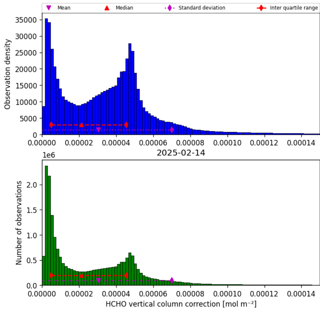
Figure 35: Histogram of “HCHO vertical column correction” for 2025-02-14 to 2025-02-15
