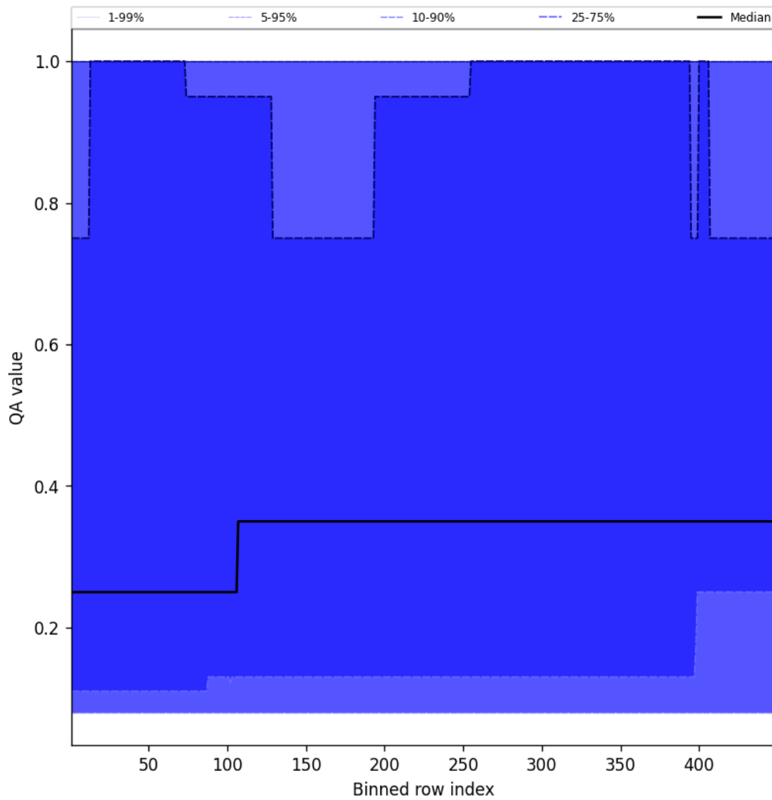
Figure 46: Along track statistics of “QA value” for 2025-02-14 to 2025-02-15
