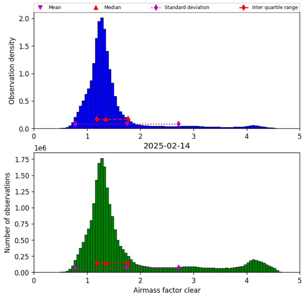
Figure 40: Histogram of “Airmass factor clear” for 2025-02-14 to 2025-02-15
