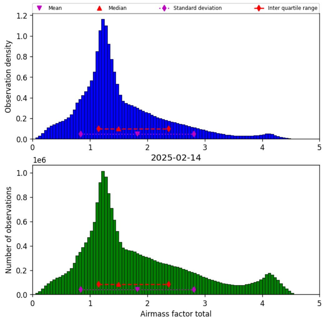
Figure 38: Histogram of “Airmass factor total” for 2025-02-14 to 2025-02-15
