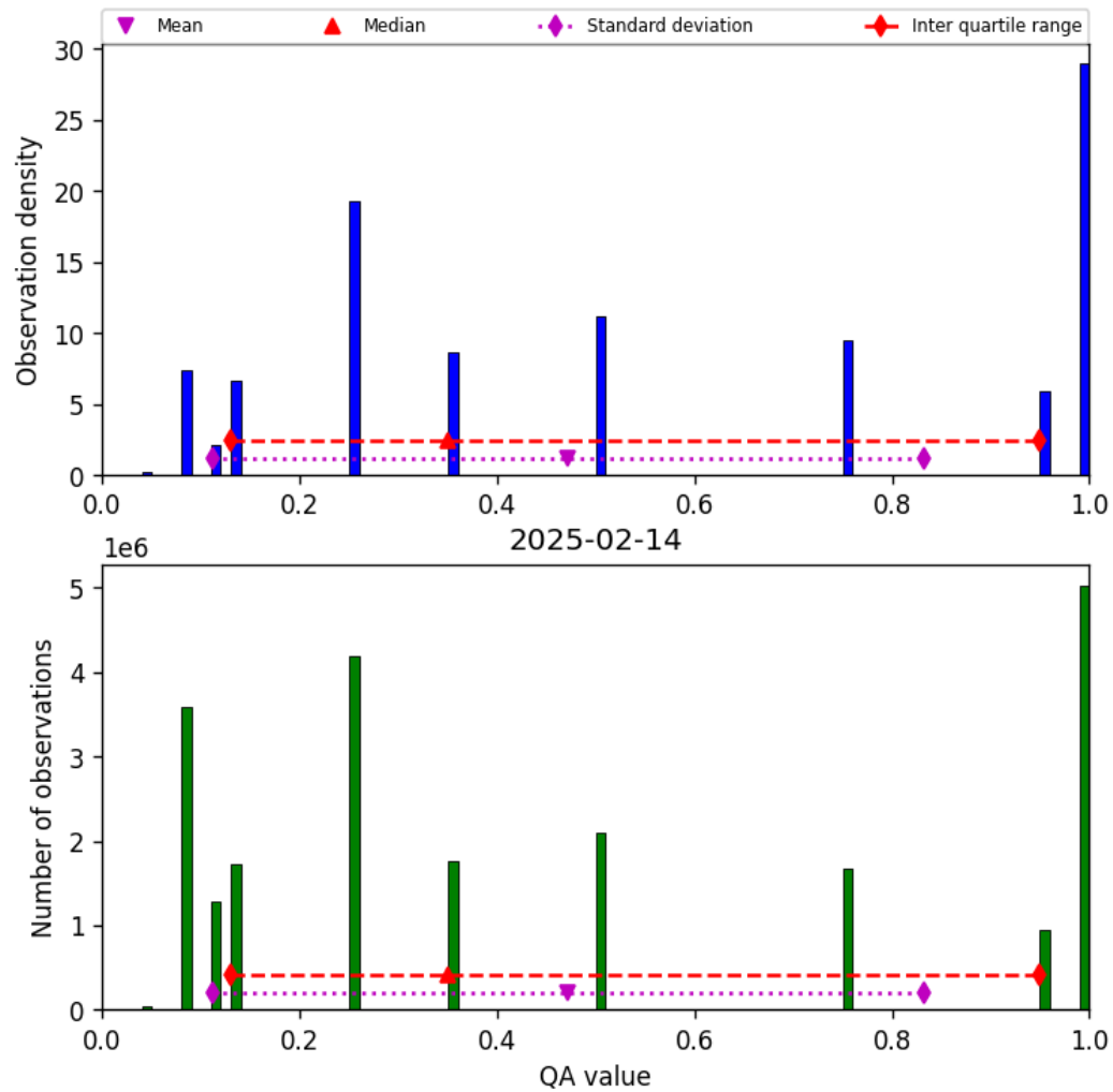
Figure 32: Histogram of “QA value” for 2025-02-14 to 2025-02-15
