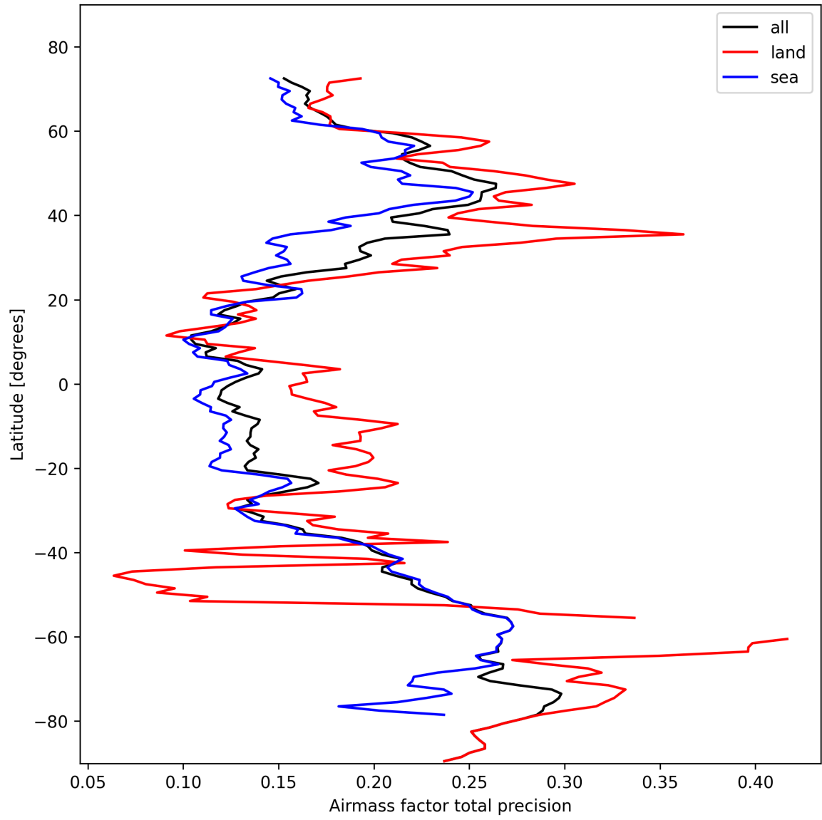
Figure 25: Zonal average of “Airmass factor total precision” for 2025-02-14 to 2025-02-15.
