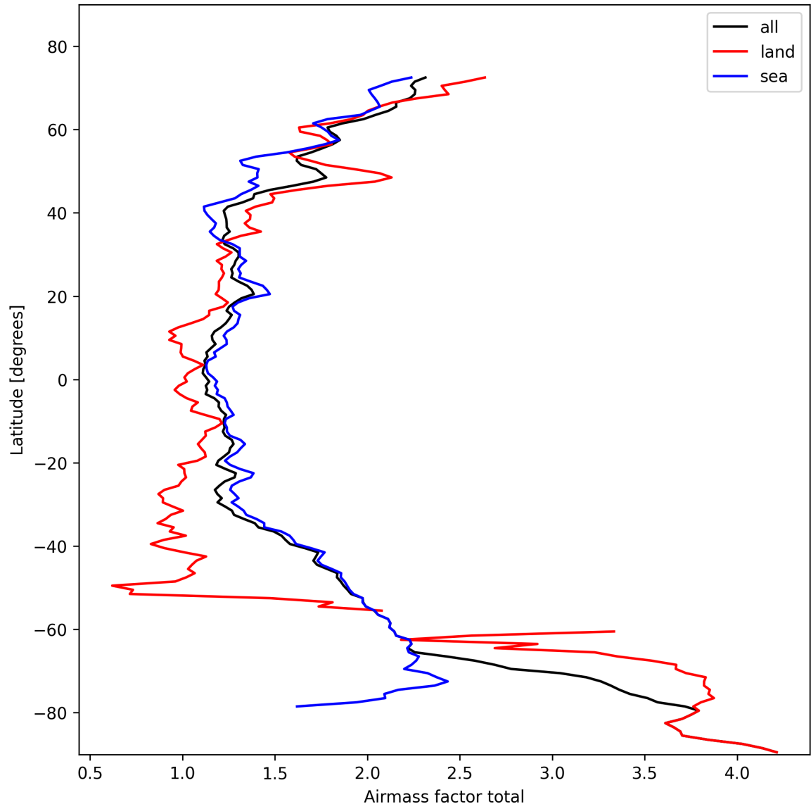
Figure 24: Zonal average of “Airmass factor total” for 2025-02-14 to 2025-02-15.
