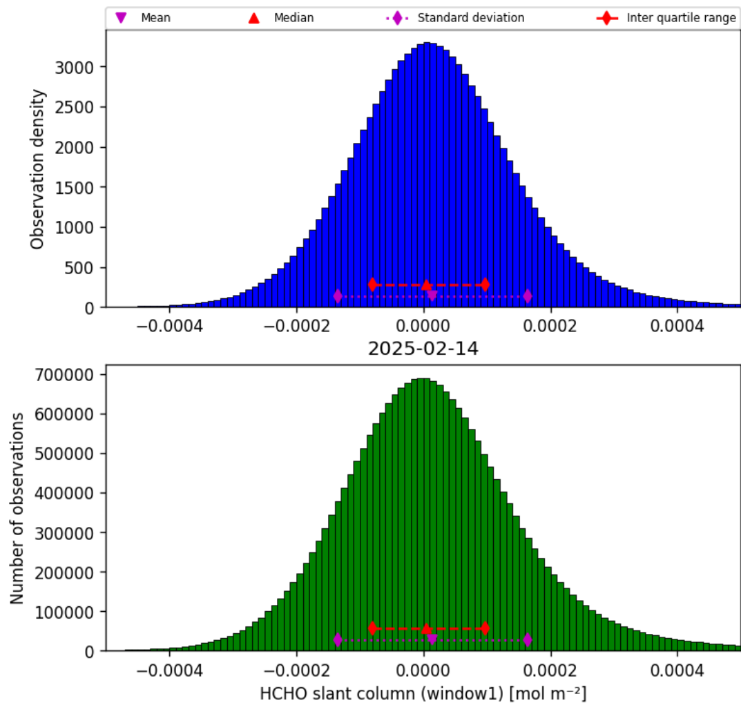
Figure 36: Histogram of “HCHO slant column (window1)” for 2025-02-14 to 2025-02-15
