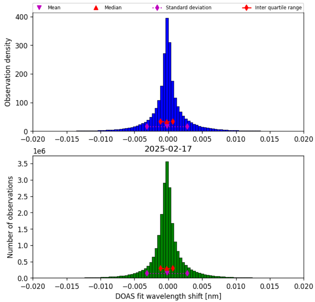
Figure 42: Histogram of “DOAS fit wavelength shift” for 2025-02-17 to 2025-02-18
