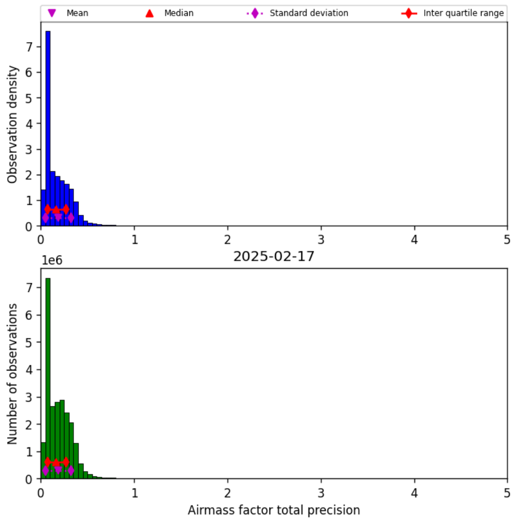
Figure 39: Histogram of “Airmass factor total precision” for 2025-02-17 to 2025-02-18
