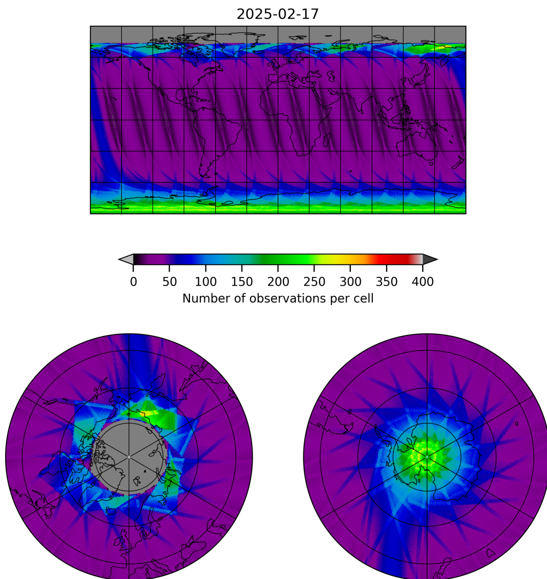
Figure 17: Map of the number of observations for 2025-02-17 to 2025-02-18
