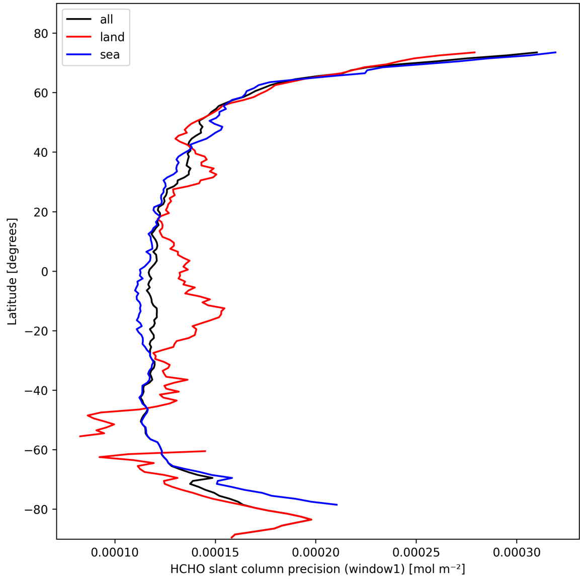
Figure 23: Zonal average of “HCHO slant column precision (window1)” for 2025-02-17 to 2025-02-18.
