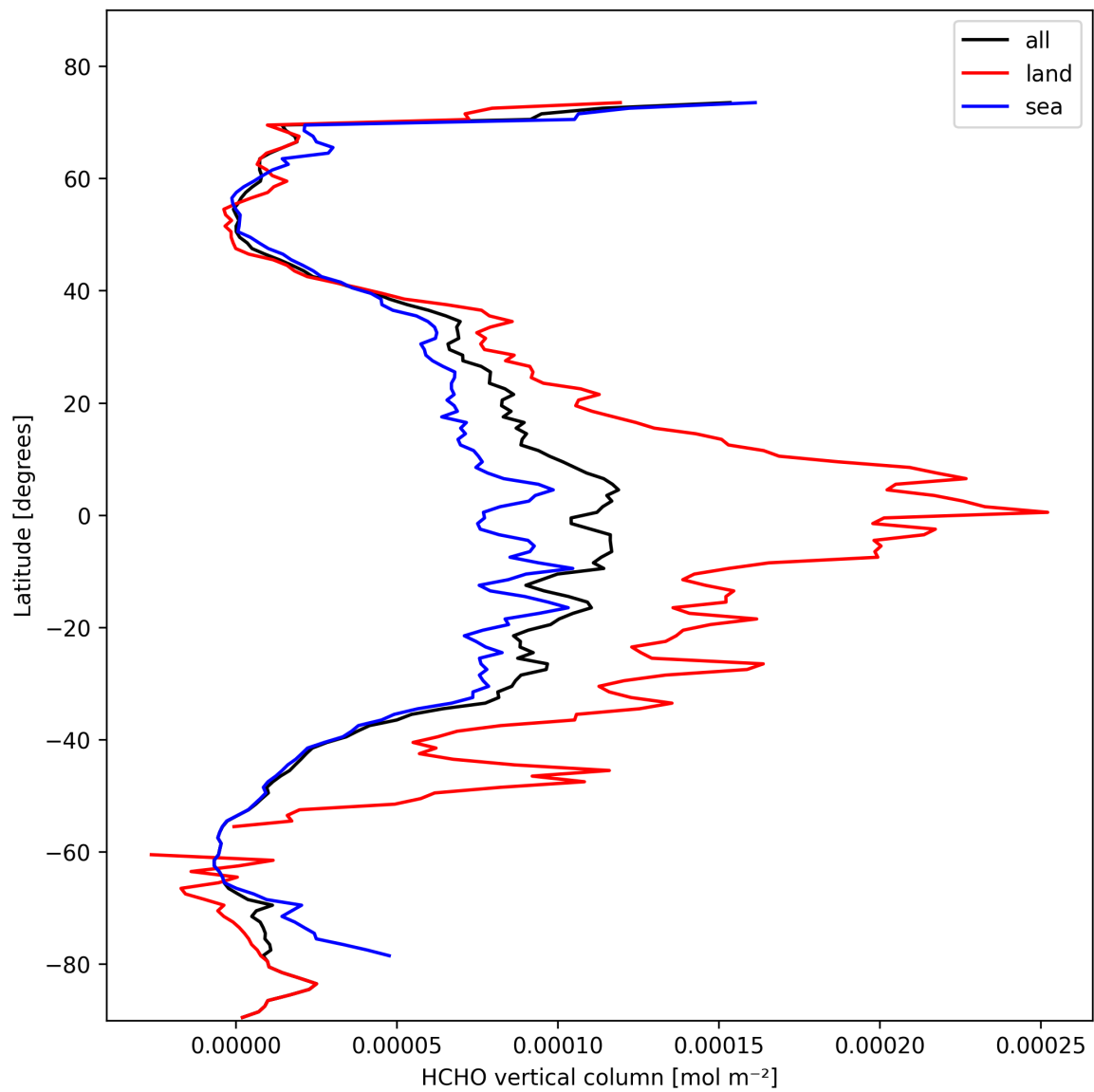
Figure 19: Zonal average of “HCHO vertical column” for 2025-02-17 to 2025-02-18.
