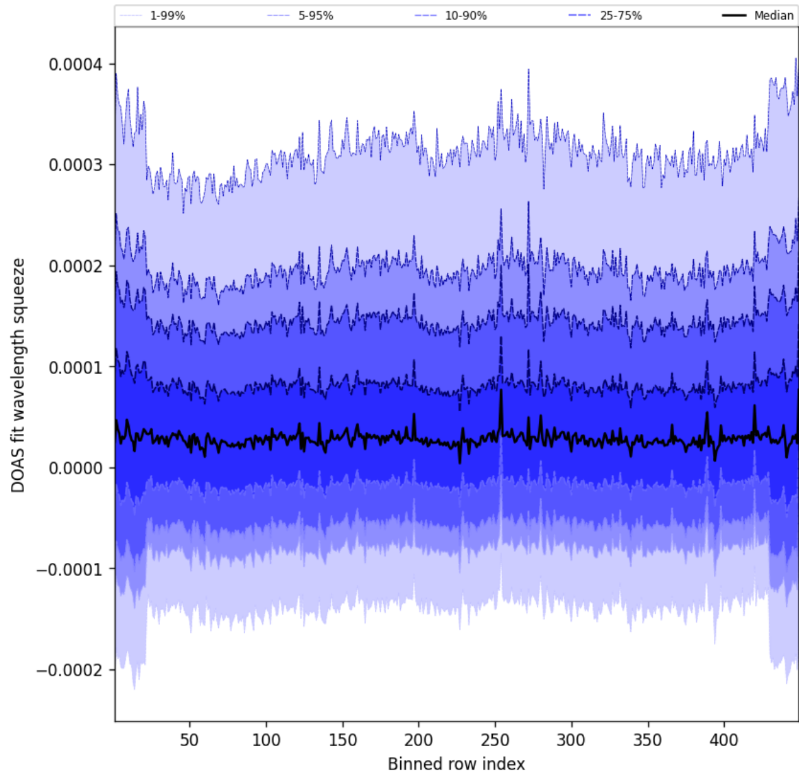
Figure 57: Along track statistics of “DOAS fit wavelength squeeze” for 2025-02-17 to 2025-02-18
