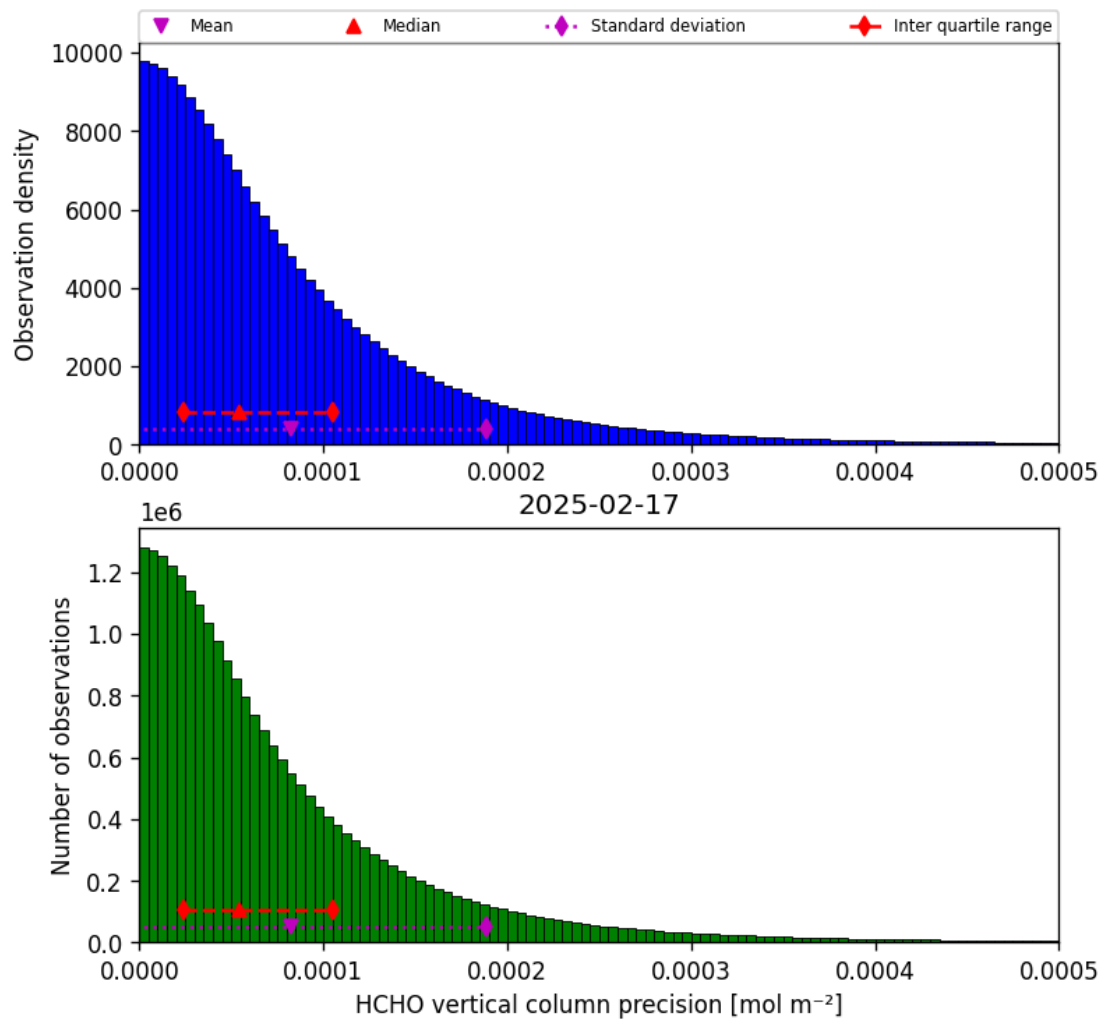
Figure 34: Histogram of “HCHO vertical column precision” for 2025-02-17 to 2025-02-18
