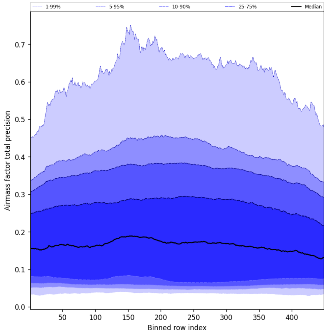
Figure 53: Along track statistics of “Airmass factor total precision” for 2025-02-17 to 2025-02-18
