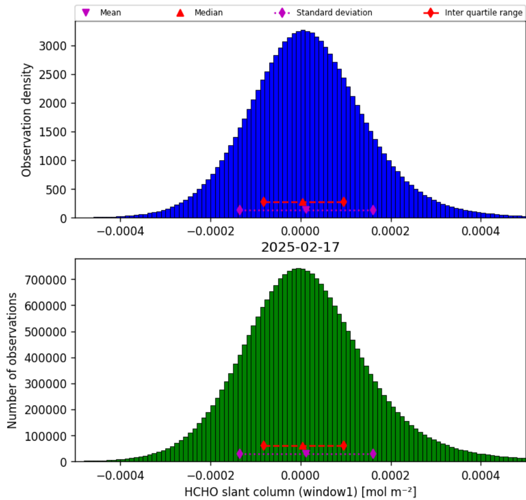
Figure 36: Histogram of “HCHO slant column (window1)” for 2025-02-17 to 2025-02-18
