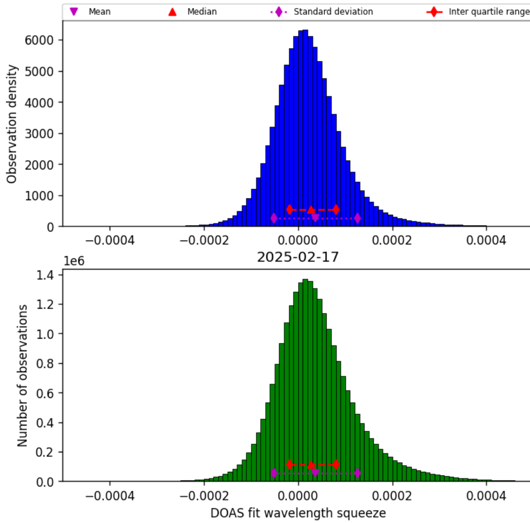
Figure 43: Histogram of “DOAS fit wavelength squeeze” for 2025-02-17 to 2025-02-18
