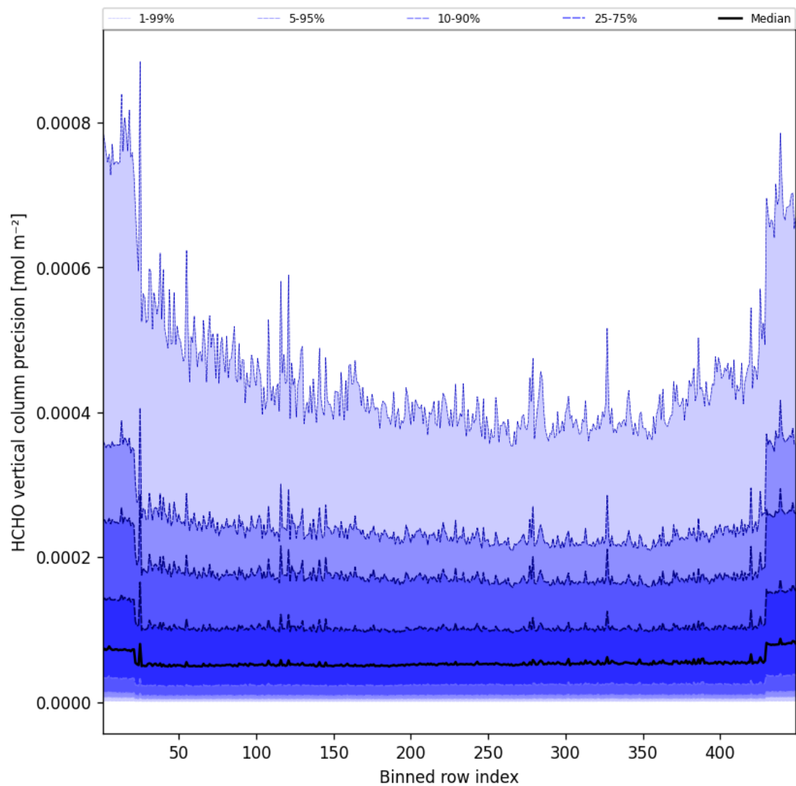
Figure 48: Along track statistics of “HCHO vertical column precision” for 2025-02-17 to 2025-02-18
