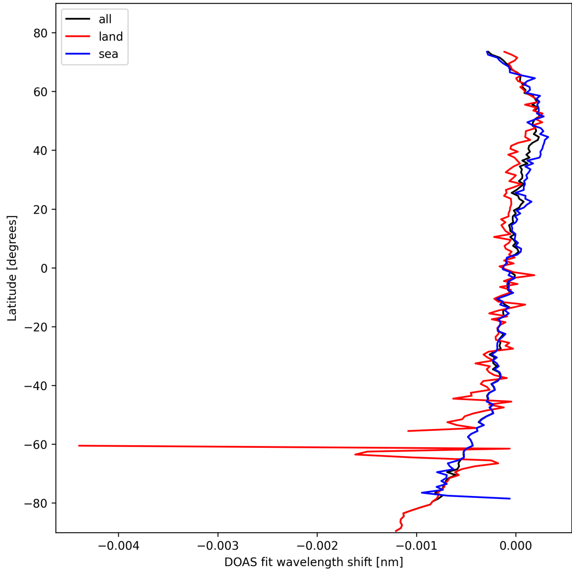
Figure 28: Zonal average of “DOAS fit wavelength shift” for 2025-02-17 to 2025-02-18.
