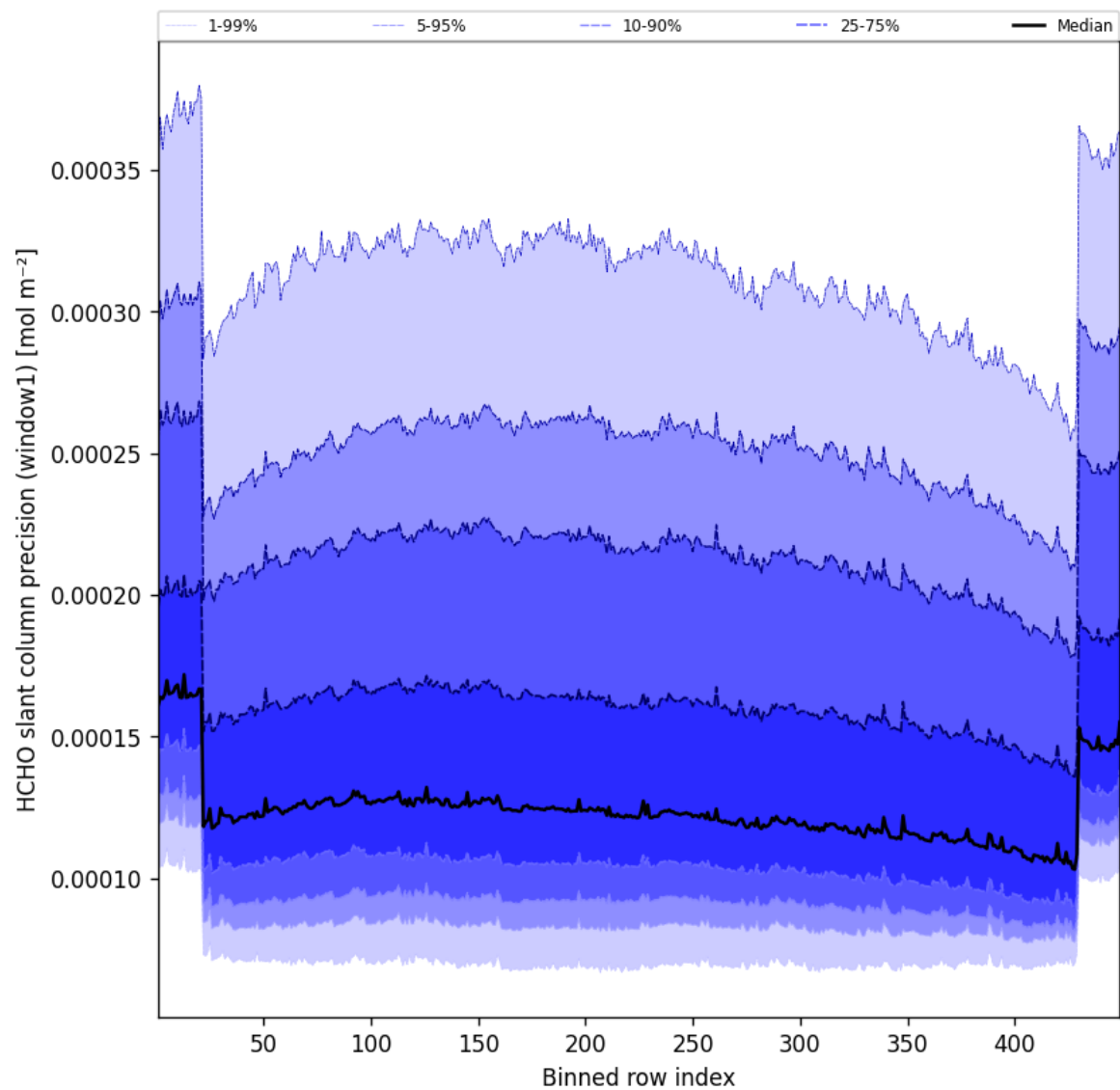
Figure 51: Along track statistics of “HCHO slant column precision (window1)” for 2025-02-17 to 2025-02-18
