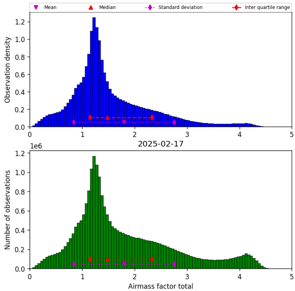
Figure 38: Histogram of “Airmass factor total” for 2025-02-17 to 2025-02-18
