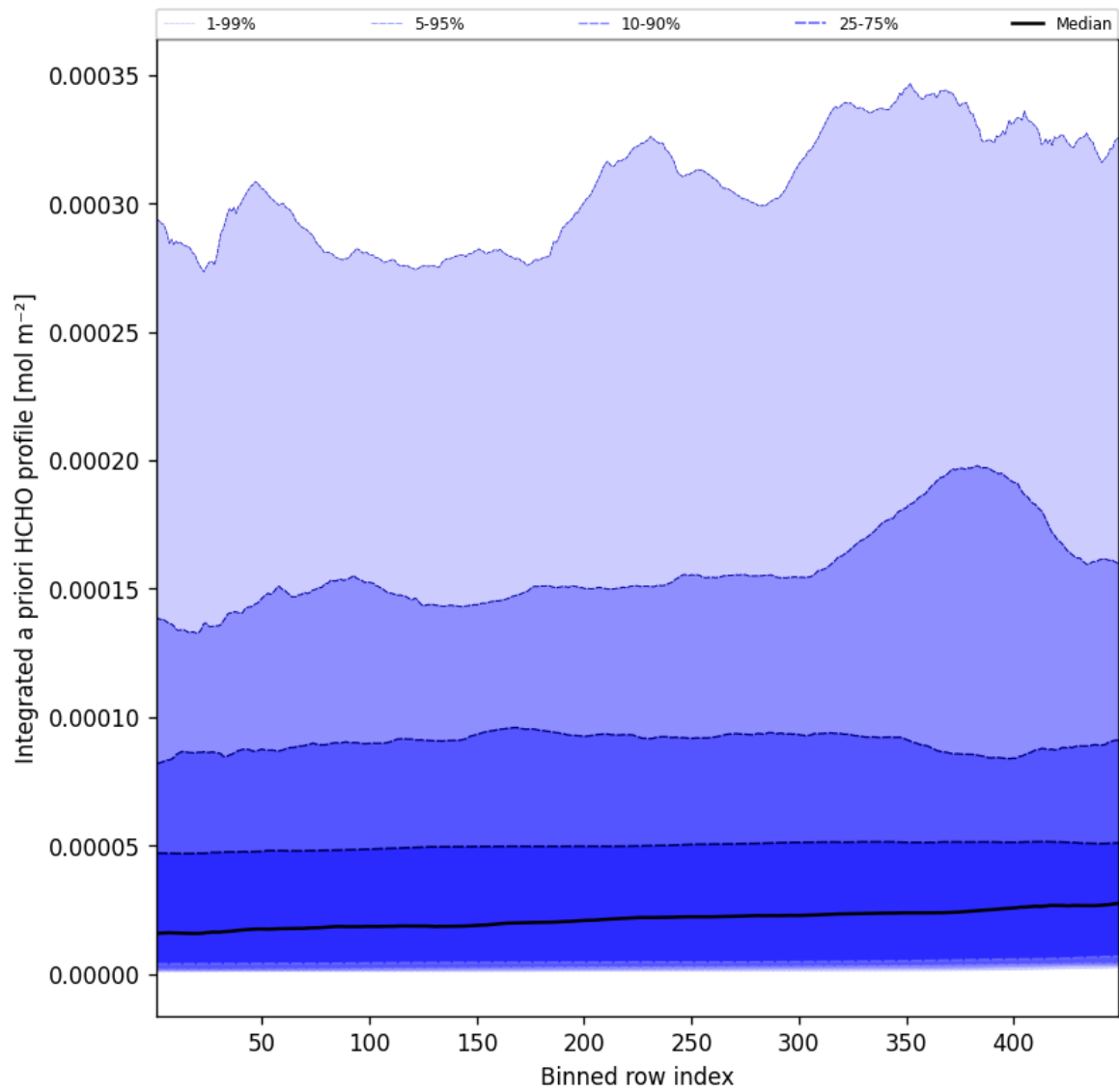
Figure 55: Along track statistics of “Integrated a priori HCHO profile” for 2025-02-17 to 2025-02-18
