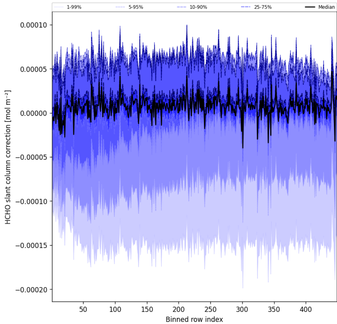
Figure 59: Along track statistics of “HCHO slant column correction” for 2025-02-17 to 2025-02-18
