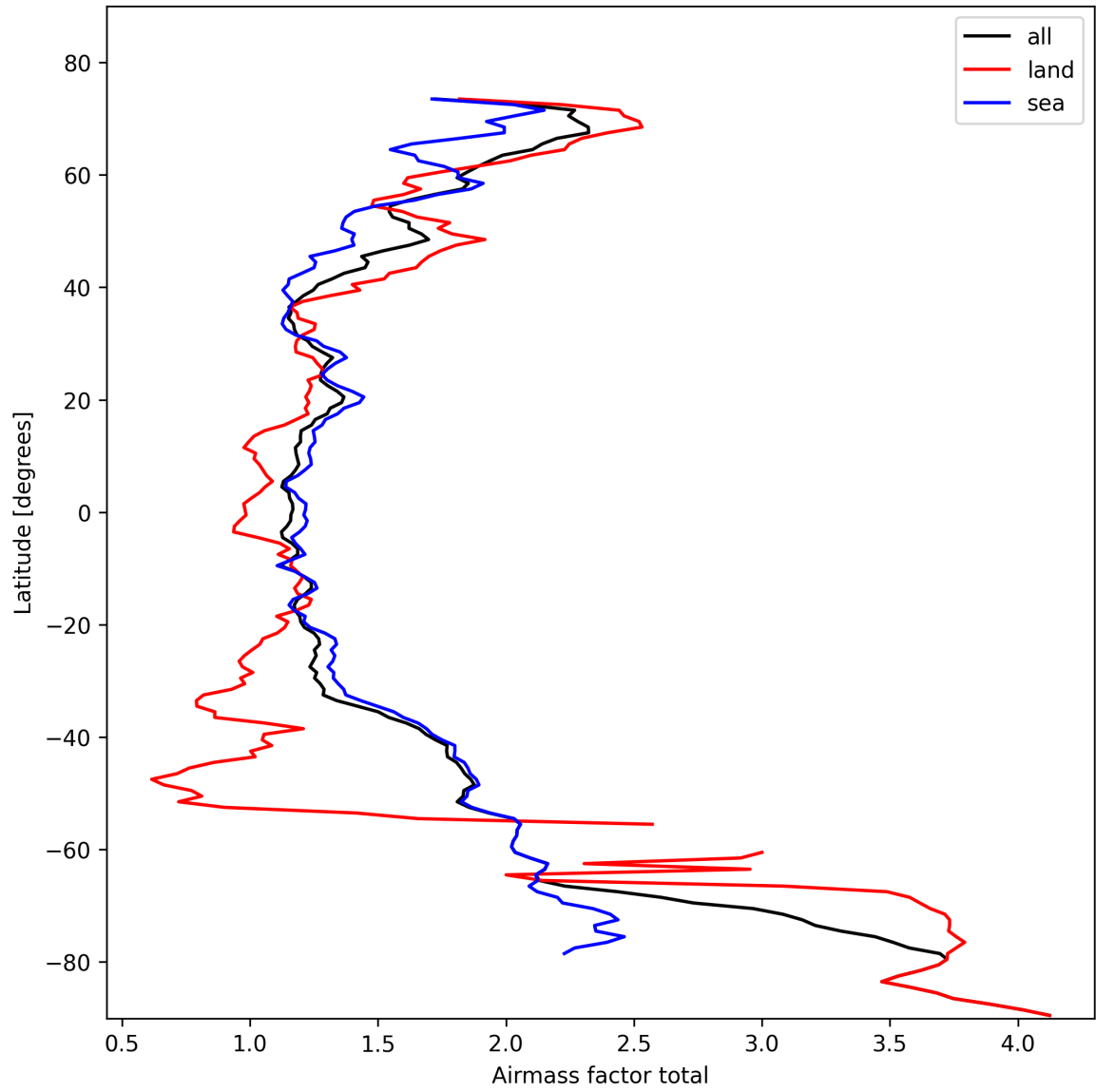
Figure 24: Zonal average of “Airmass factor total” for 2025-02-17 to 2025-02-18.
