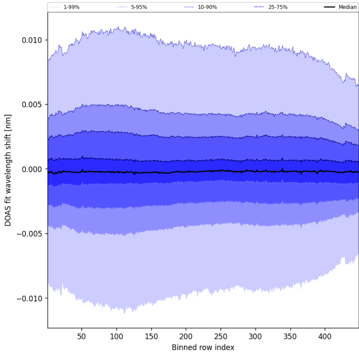
Figure 56: Along track statistics of “DOAS fit wavelength shift” for 2025-02-17 to 2025-02-18
