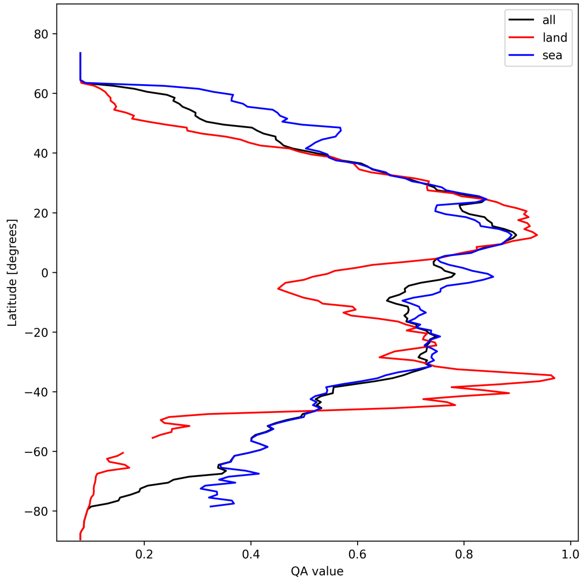
Figure 18: Zonal average of “QA value” for 2025-02-17 to 2025-02-18.
