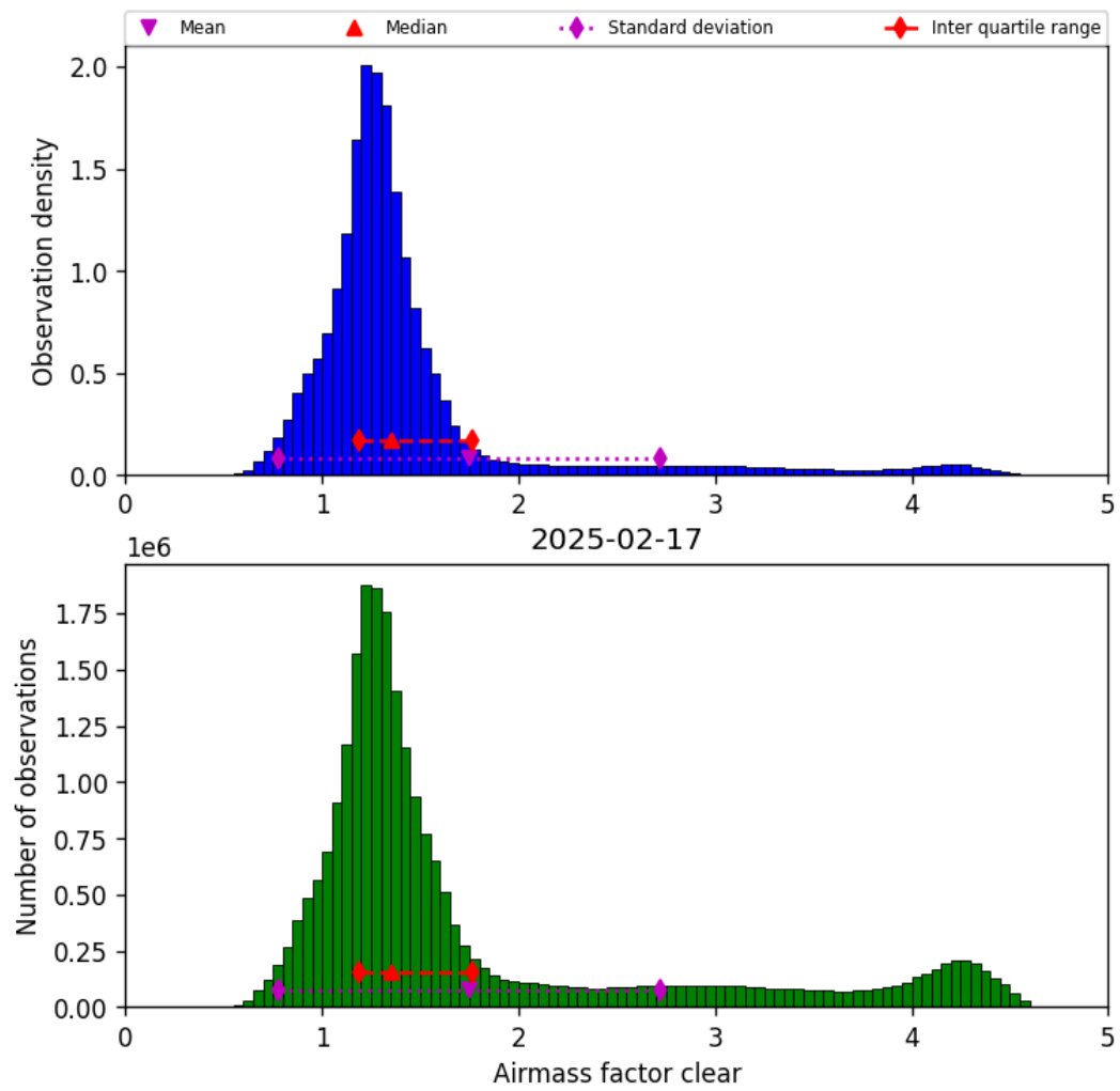
Figure 40: Histogram of “Airmass factor clear” for 2025-02-17 to 2025-02-18
