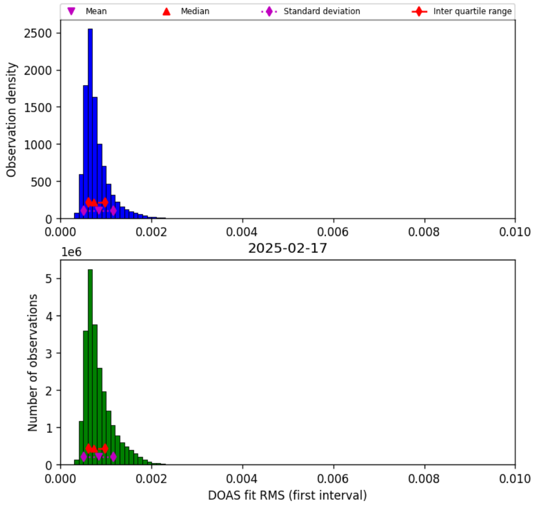
Figure 44: Histogram of “DOAS fit RMS (first interval)” for 2025-02-17 to 2025-02-18
