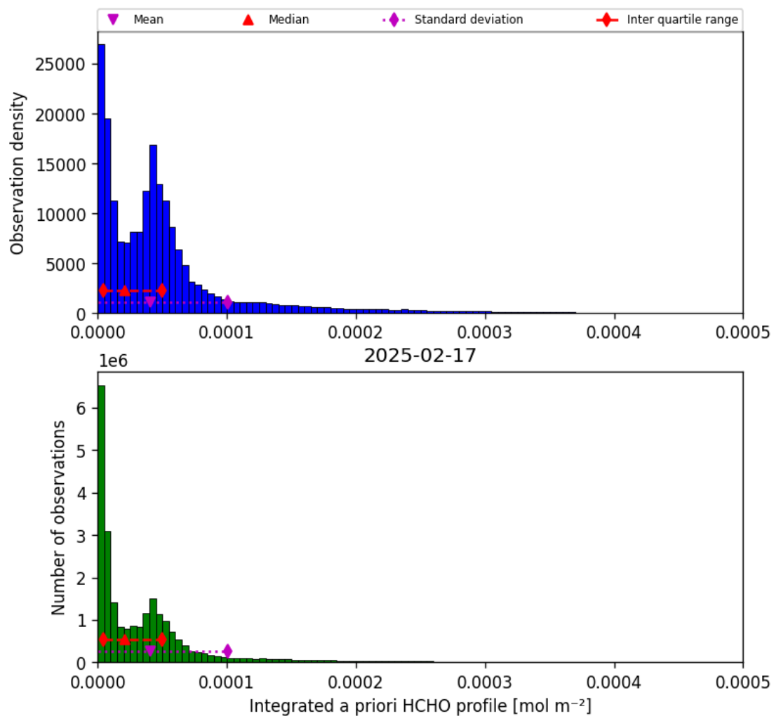
Figure 41: Histogram of “Integrated a priori HCHO profile” for 2025-02-17 to 2025-02-18
