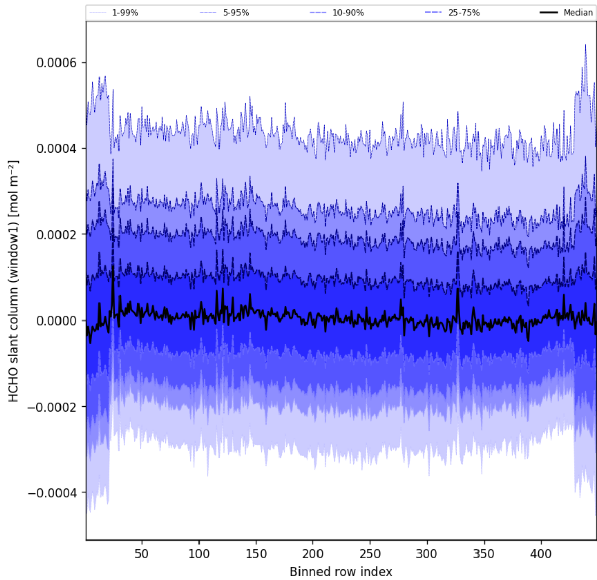
Figure 50: Along track statistics of "HCHO slant column (window1)" for 2025-02-17 to 2025-02-18
