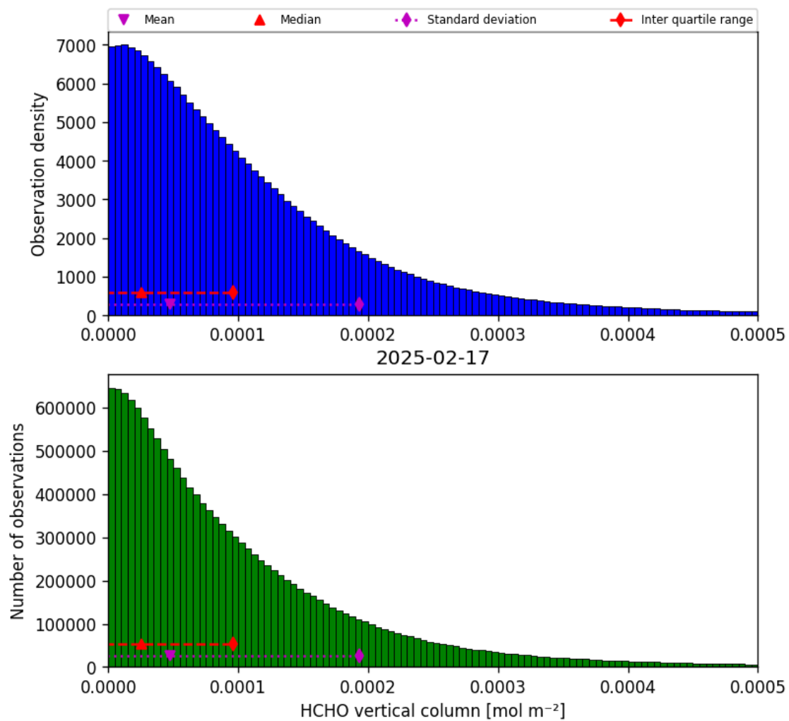
Figure 33: Histogram of “HCHO vertical column” for 2025-02-17 to 2025-02-18
