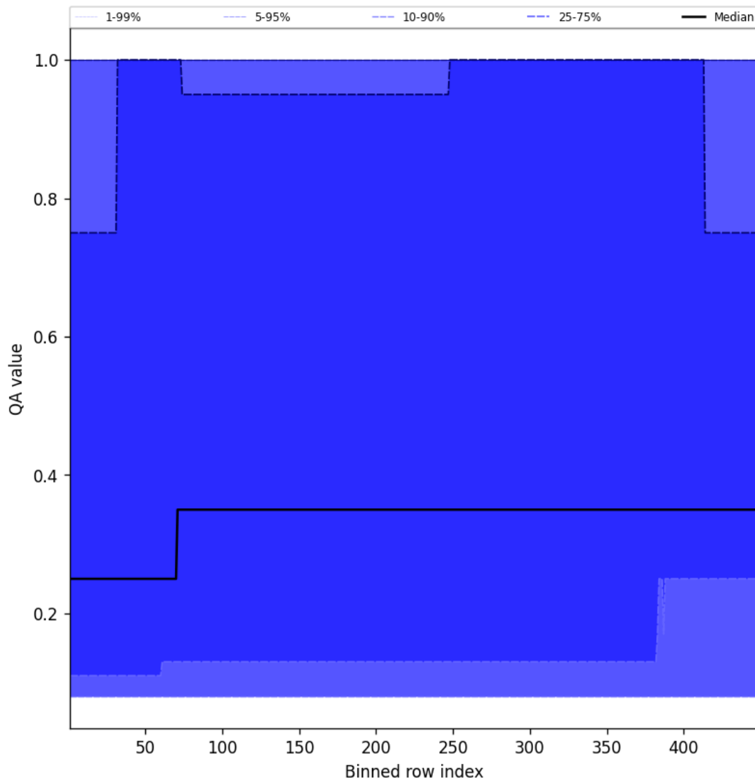
Figure 46: Along track statistics of “QA value” for 2025-02-17 to 2025-02-18
