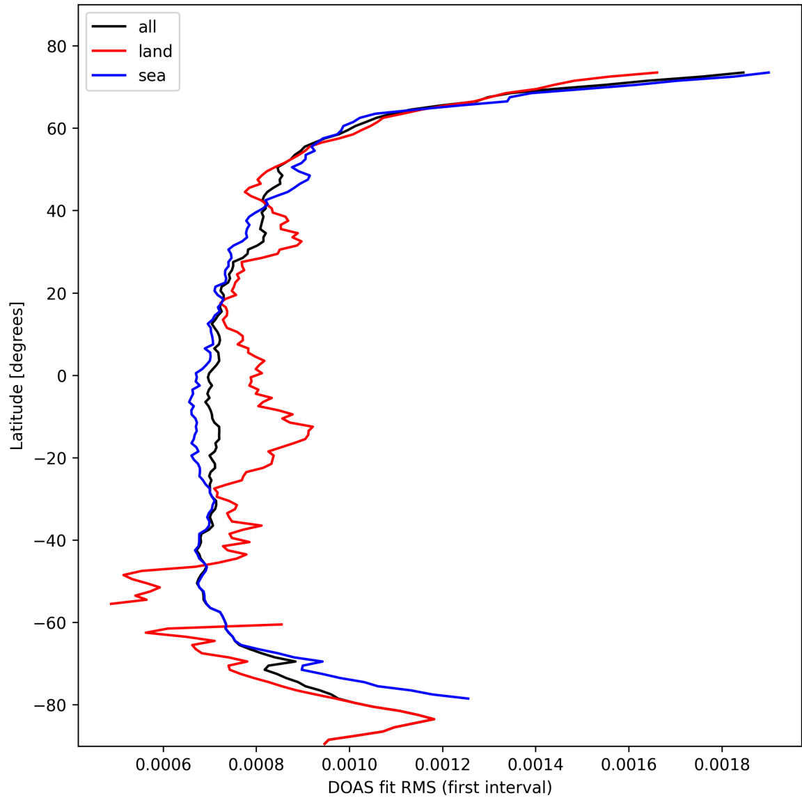
Figure 30: Zonal average of “DOAS fit RMS (first interval)” for 2025-02-17 to 2025-02-18.
