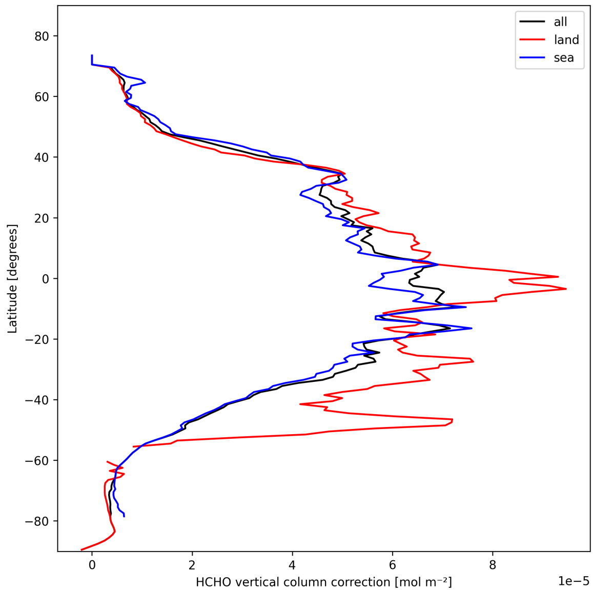
Figure 21: Zonal average of “HCHO vertical column correction” for 2025-02-17 to 2025-02-18.
