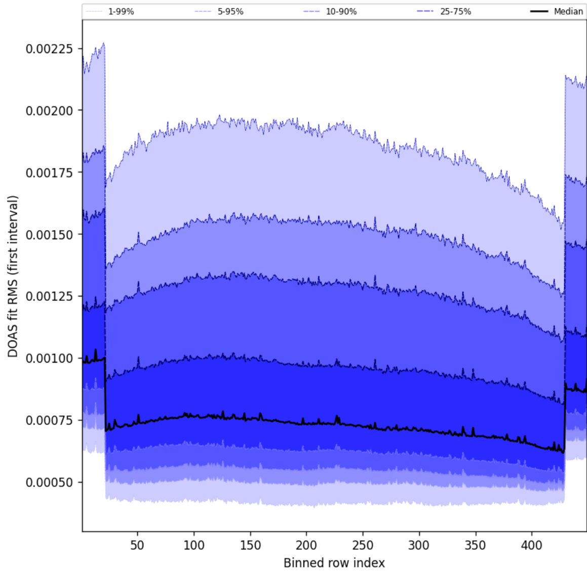
Figure 58: Along track statistics of “DOAS fit RMS (first interval)” for 2025-02-17 to 2025-02-18
