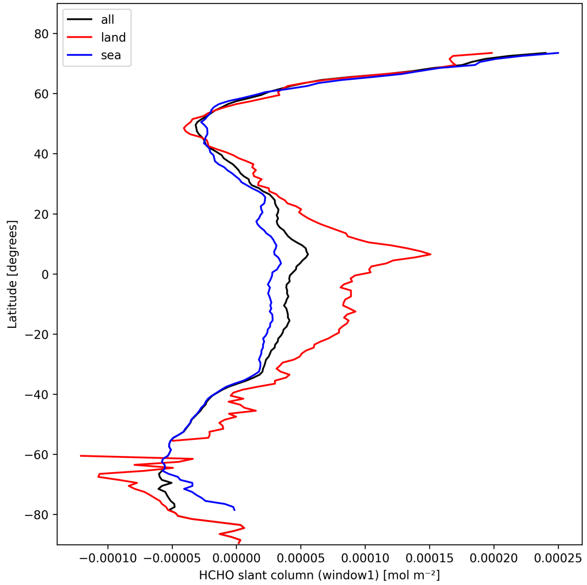
Figure 22: Zonal average of “HCHO slant column (window1)” for 2025-02-17 to 2025-02-18.
