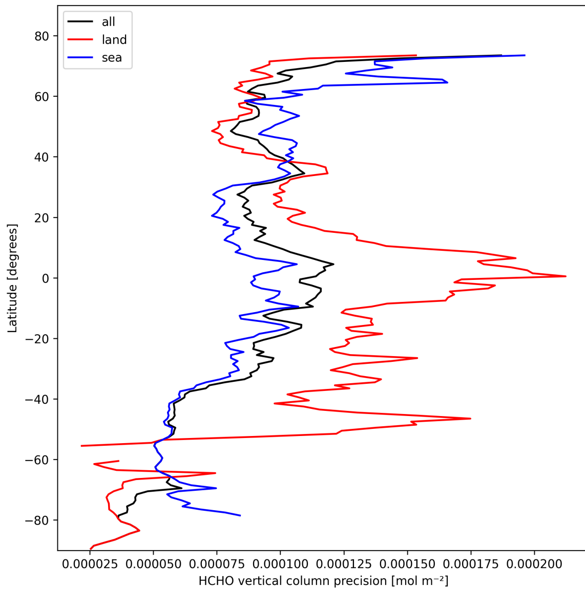
Figure 20: Zonal average of “HCHO vertical column precision” for 2025-02-17 to 2025-02-18.
