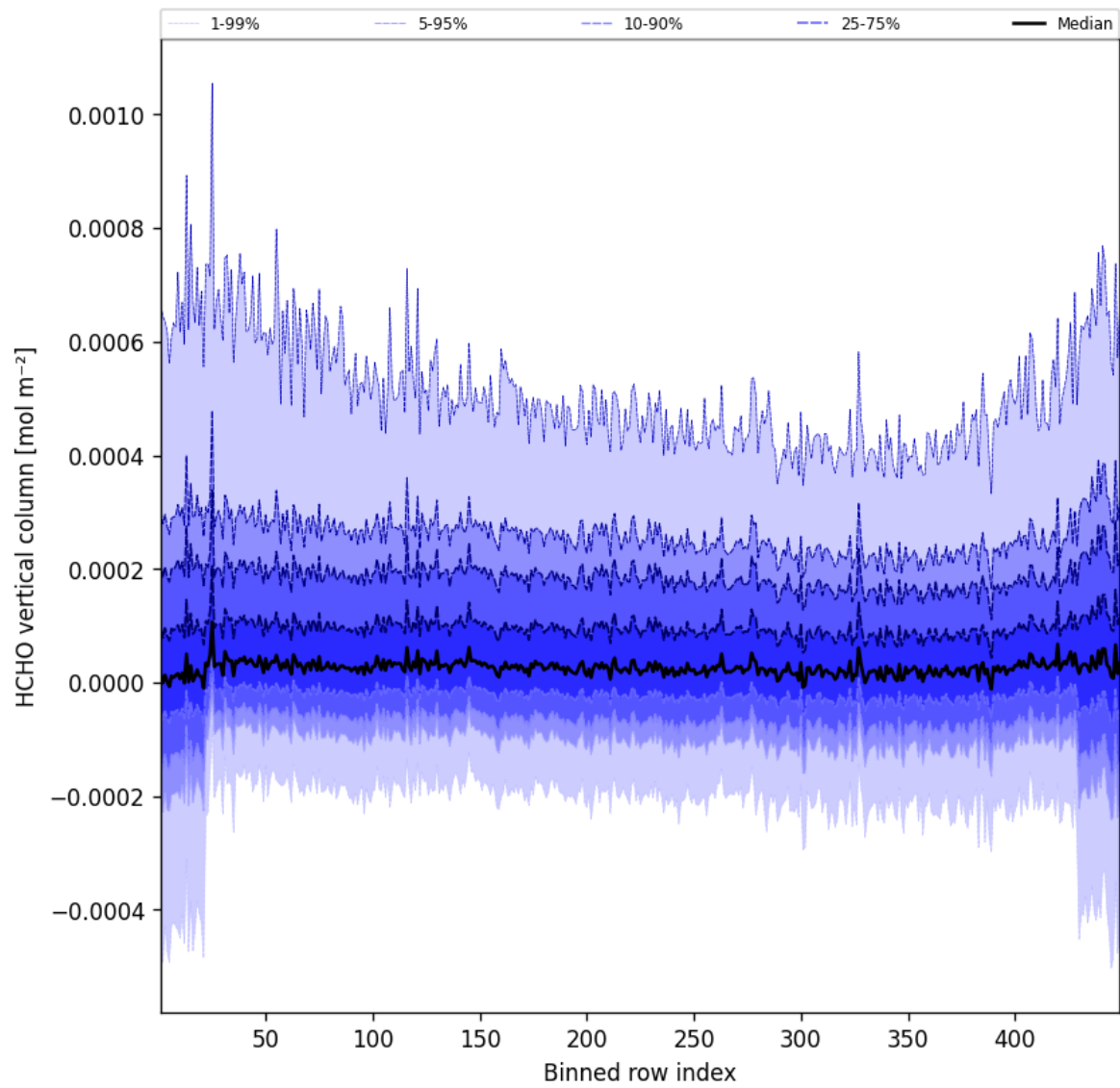
Figure 47: Along track statistics of “HCHO vertical column” for 2025-02-17 to 2025-02-18
