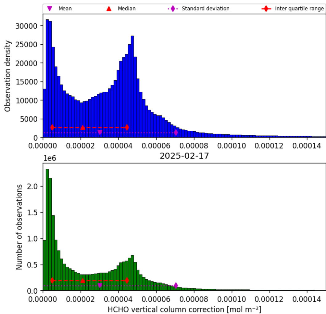
Figure 35: Histogram of “HCHO vertical column correction” for 2025-02-17 to 2025-02-18
