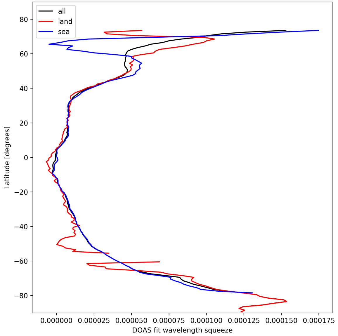
Figure 29: Zonal average of “DOAS fit wavelength squeeze” for 2025-02-17 to 2025-02-18.
