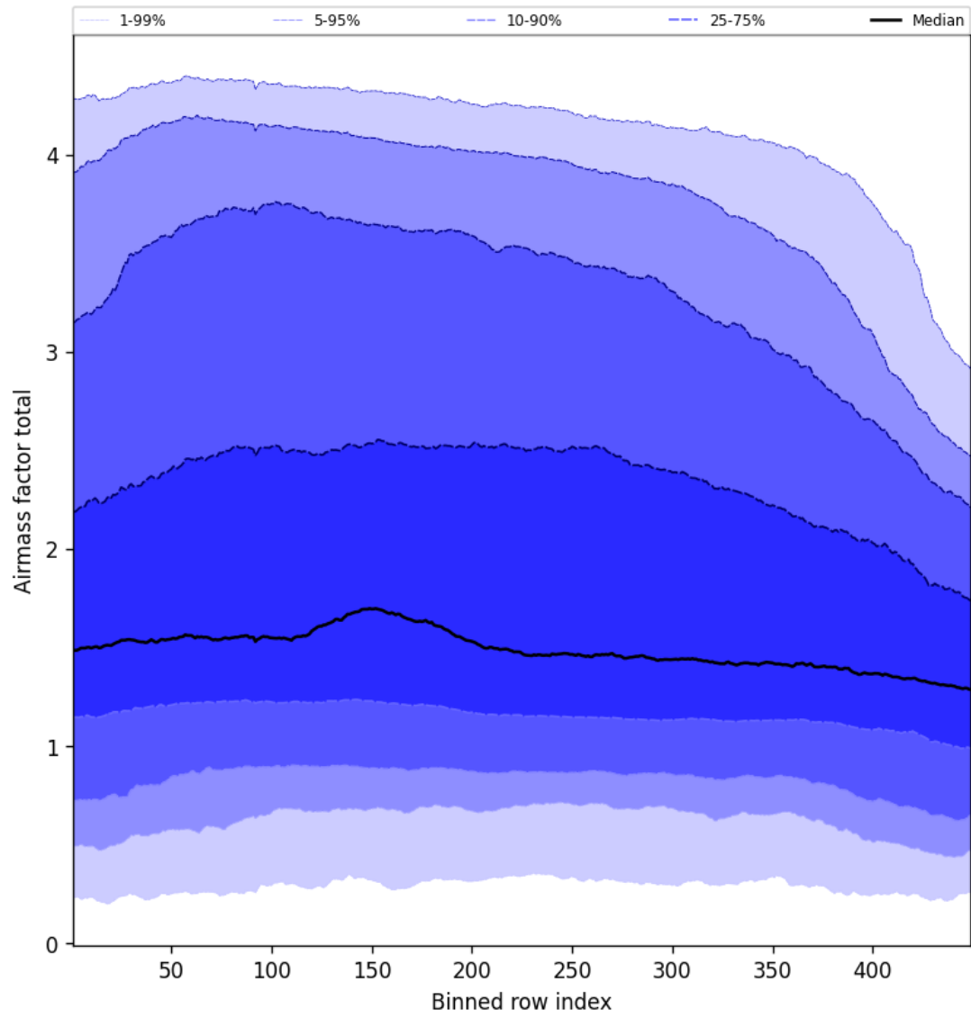
Figure 52: Along track statistics of “Airmass factor total” for 2025-02-17 to 2025-02-18
