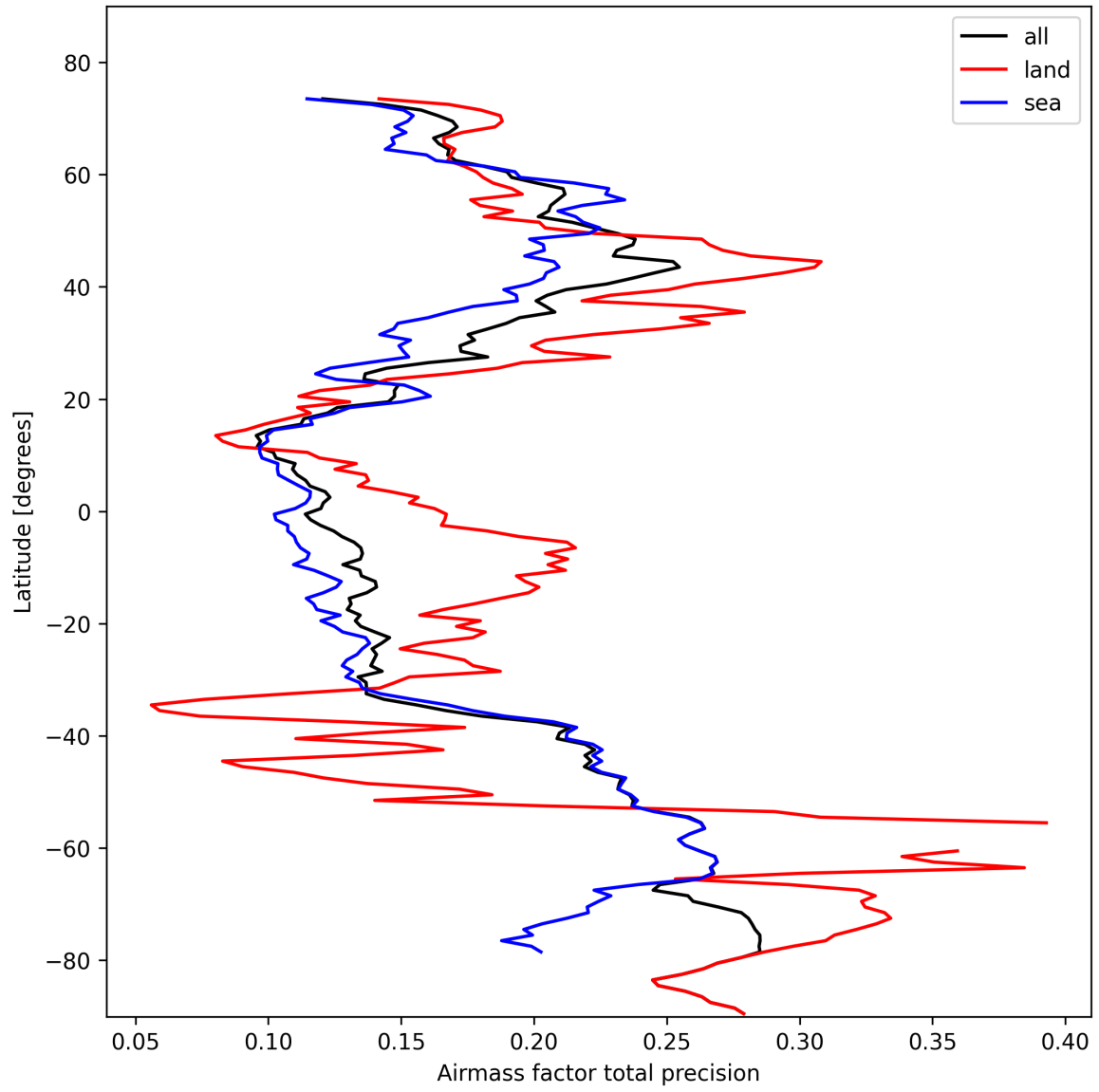
Figure 25: Zonal average of “Airmass factor total precision” for 2025-02-17 to 2025-02-18.
