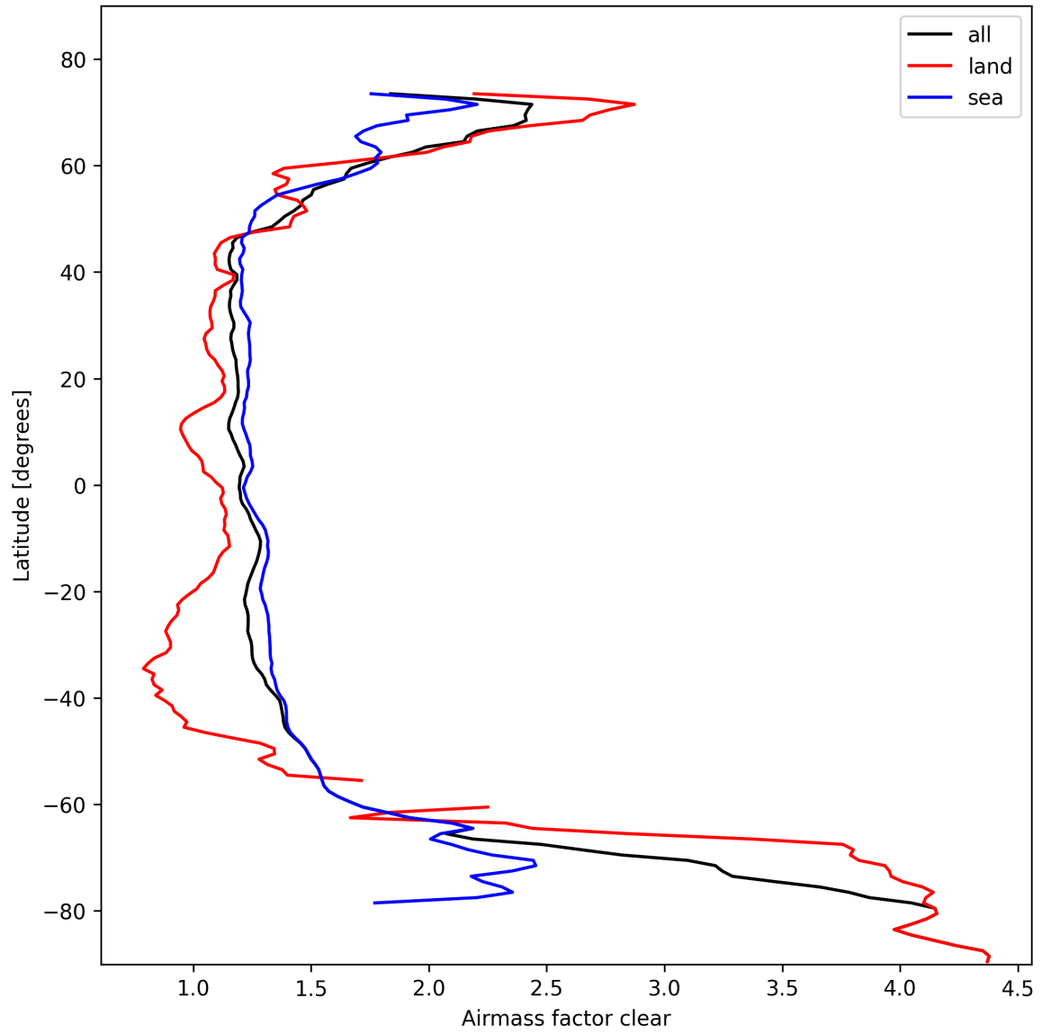
Figure 26: Zonal average of “Airmass factor clear” for 2025-02-17 to 2025-02-18.
