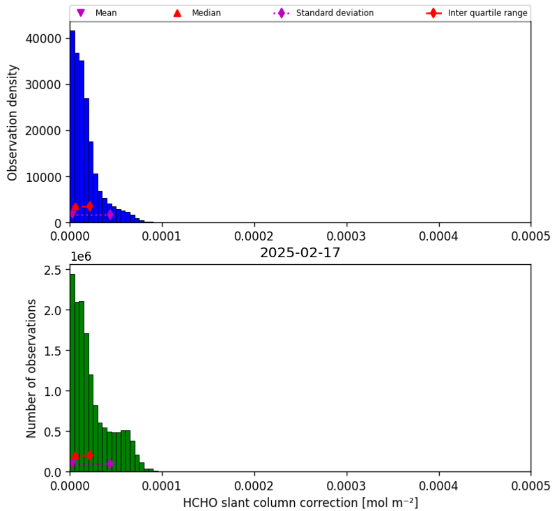
Figure 45: Histogram of “HCHO slant column correction” for 2025-02-17 to 2025-02-18
