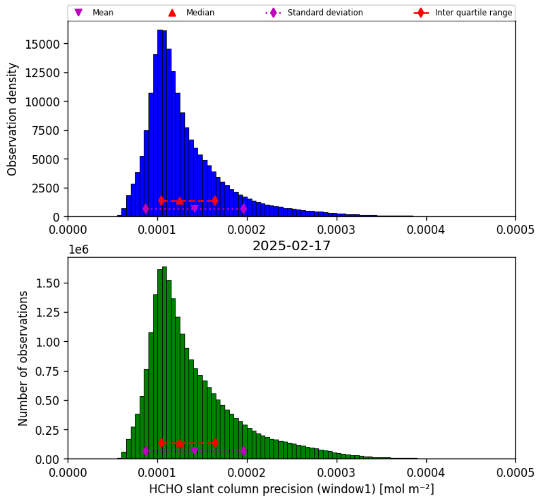
Figure 37: Histogram of “HCHO slant column precision (window1)” for 2025-02-17 to 2025-02-18
