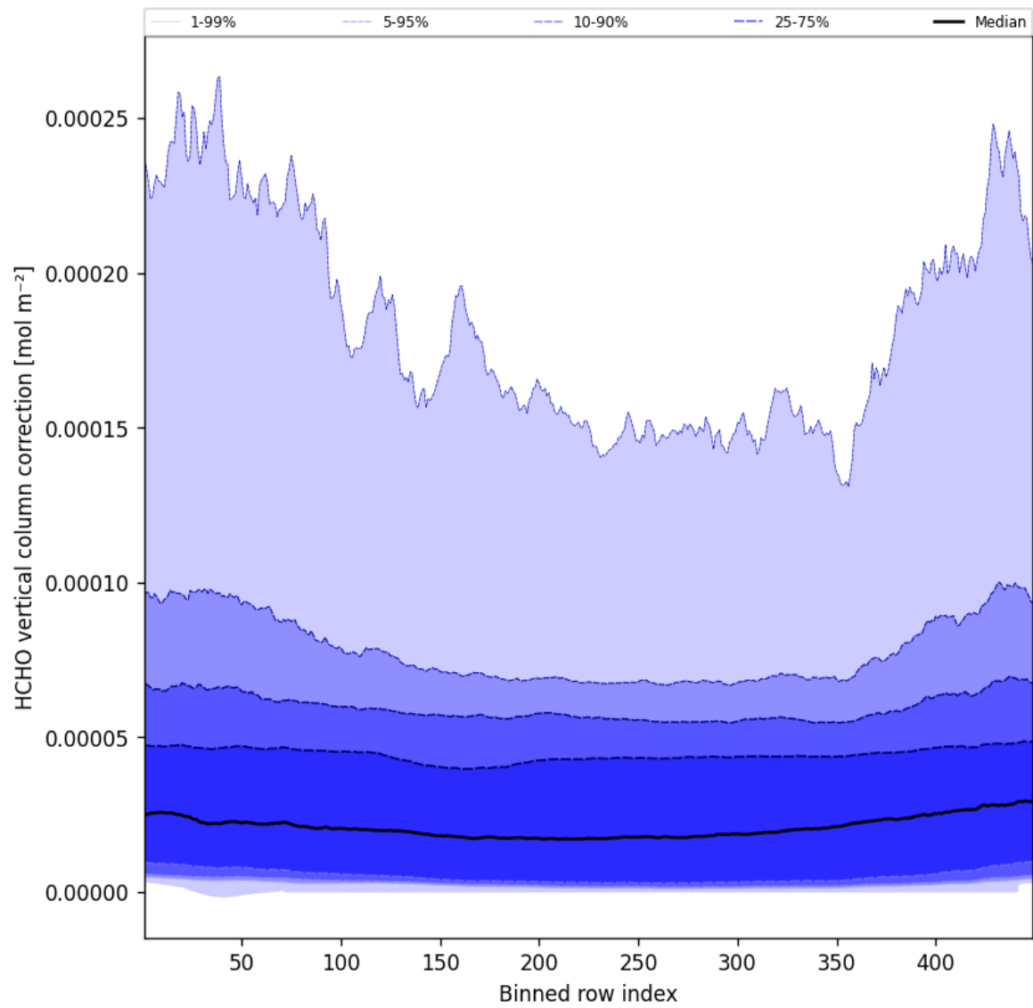
Figure 49: Along track statistics of “HCHO vertical column correction” for 2025-02-17 to 2025-02-18
