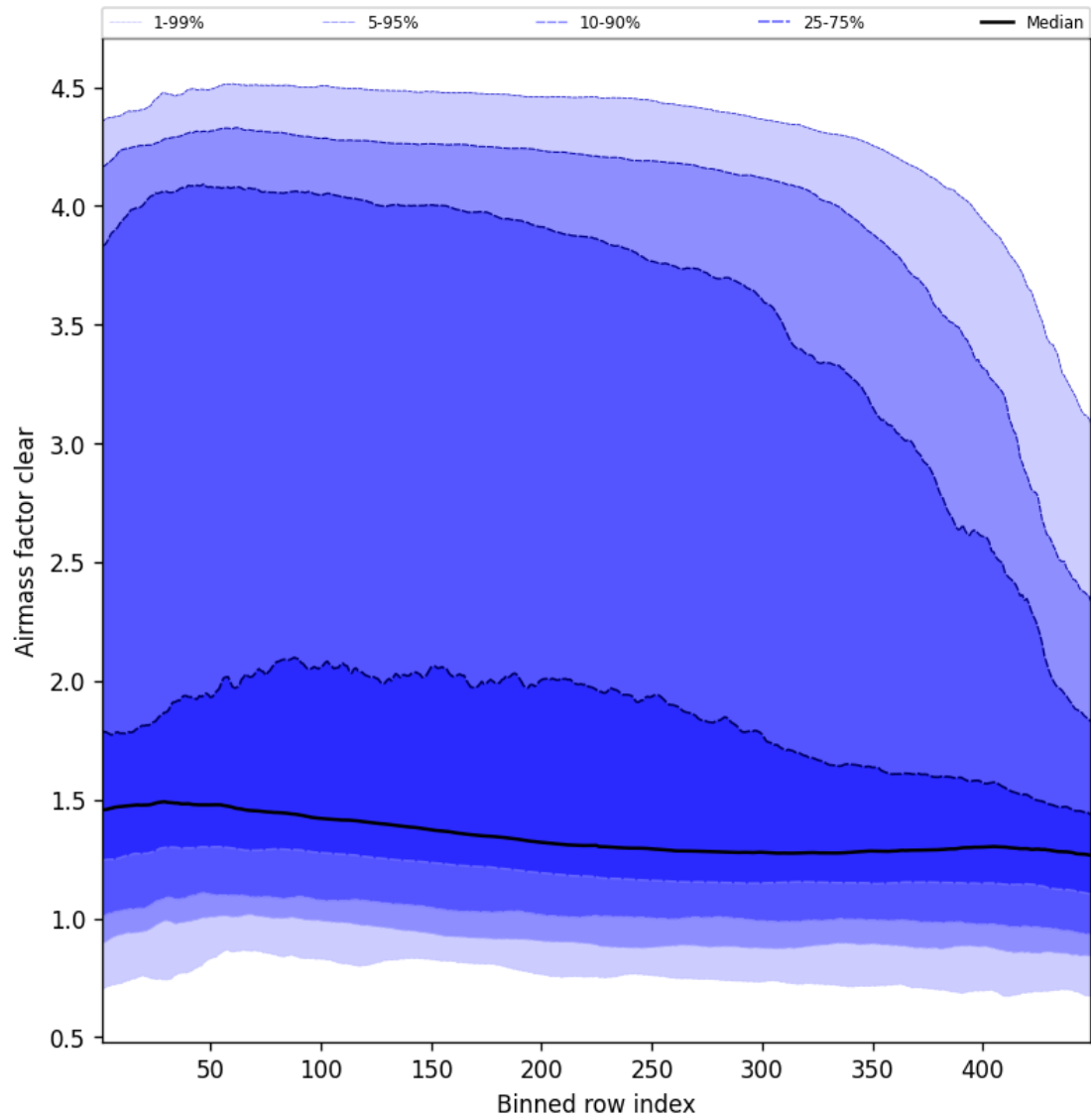
Figure 54: Along track statistics of “Airmass factor clear” for 2025-02-17 to 2025-02-18
