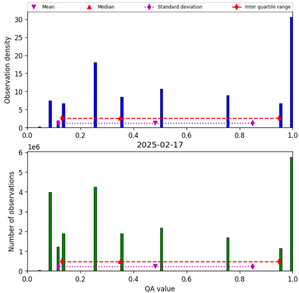
Figure 32: Histogram of “QA value” for 2025-02-17 to 2025-02-18
