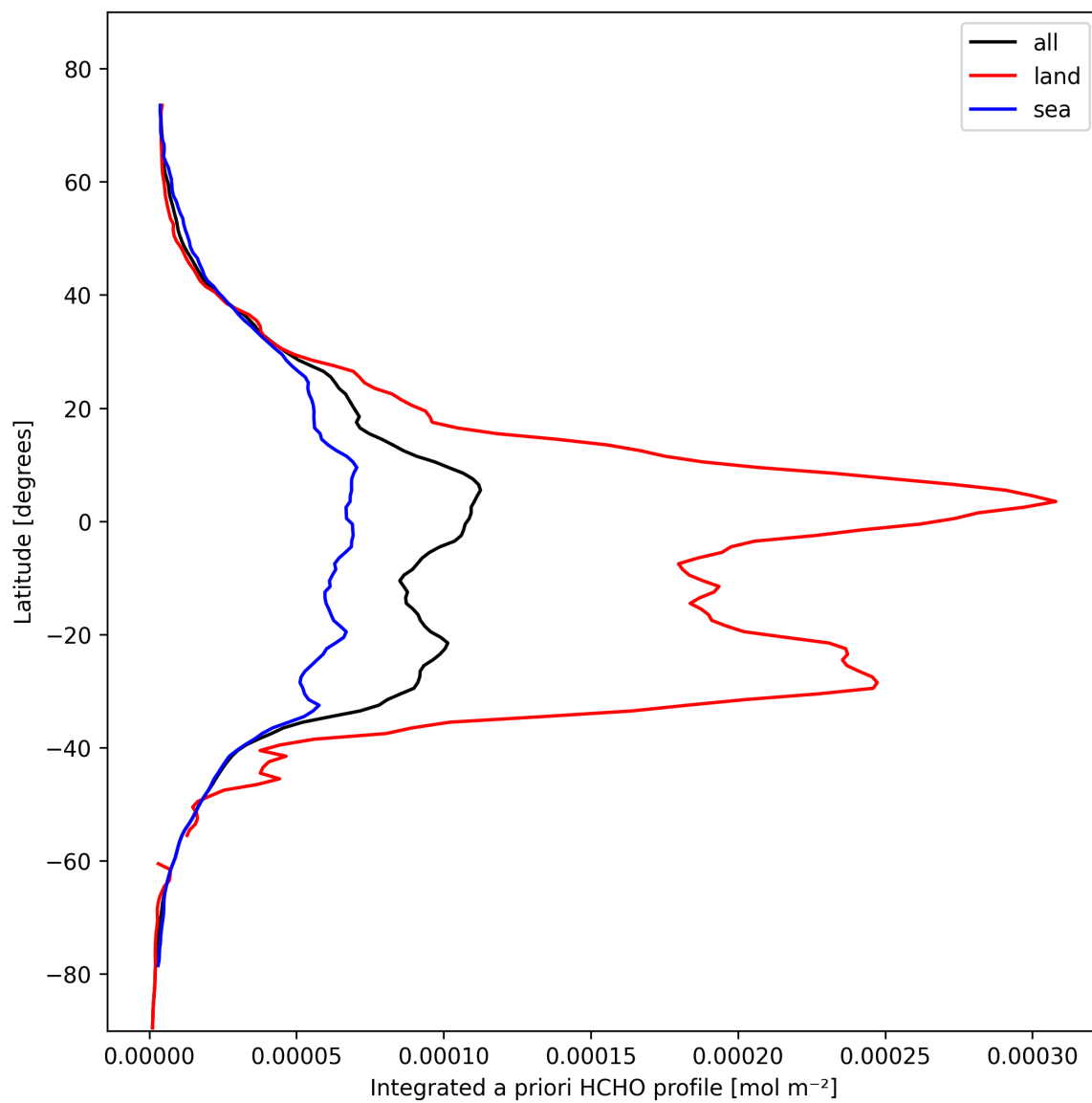
Figure 27: Zonal average of “Integrated a priori HCHO profile” for 2025-02-17 to 2025-02-18.
