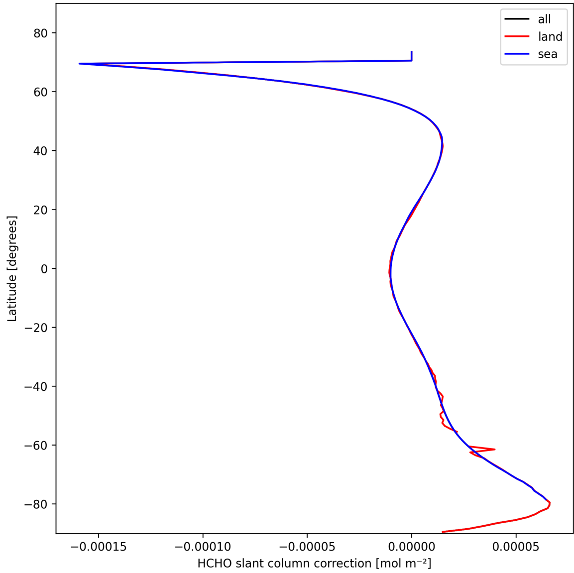
Figure 31: Zonal average of "HCHO slant column correction" for 2025-02-17 to 2025-02-18.
