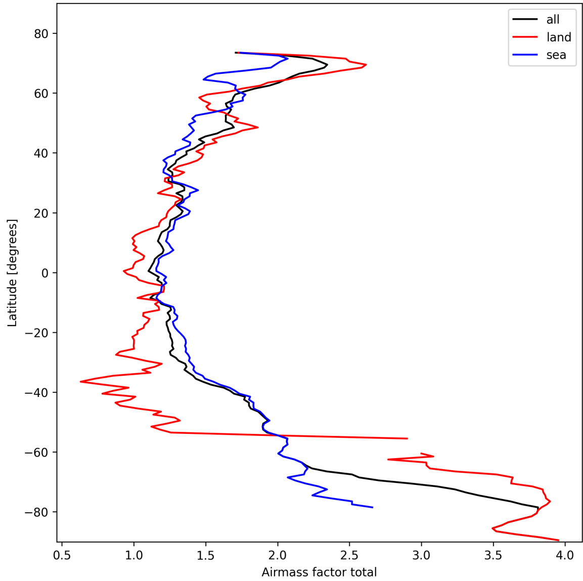
Figure 24: Zonal average of “Airmass factor total” for 2025-02-18 to 2025-02-19.
