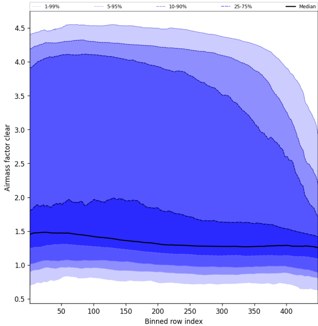
Figure 54: Along track statistics of “Air mass factor clear” for 2025-02-18 to 2025-02-19
