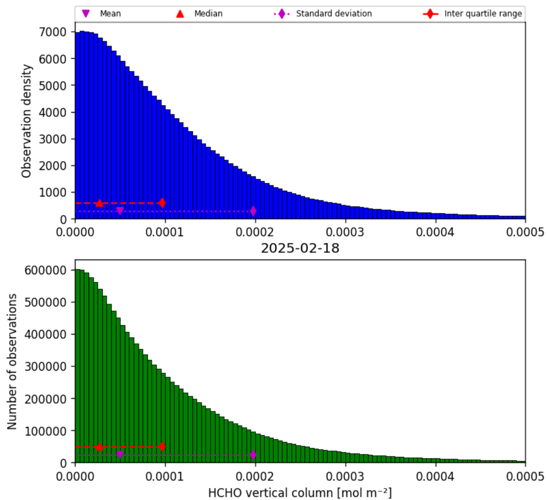
Figure 33: Histogram of “HCHO vertical column” for 2025-02-18 to 2025-02-19
