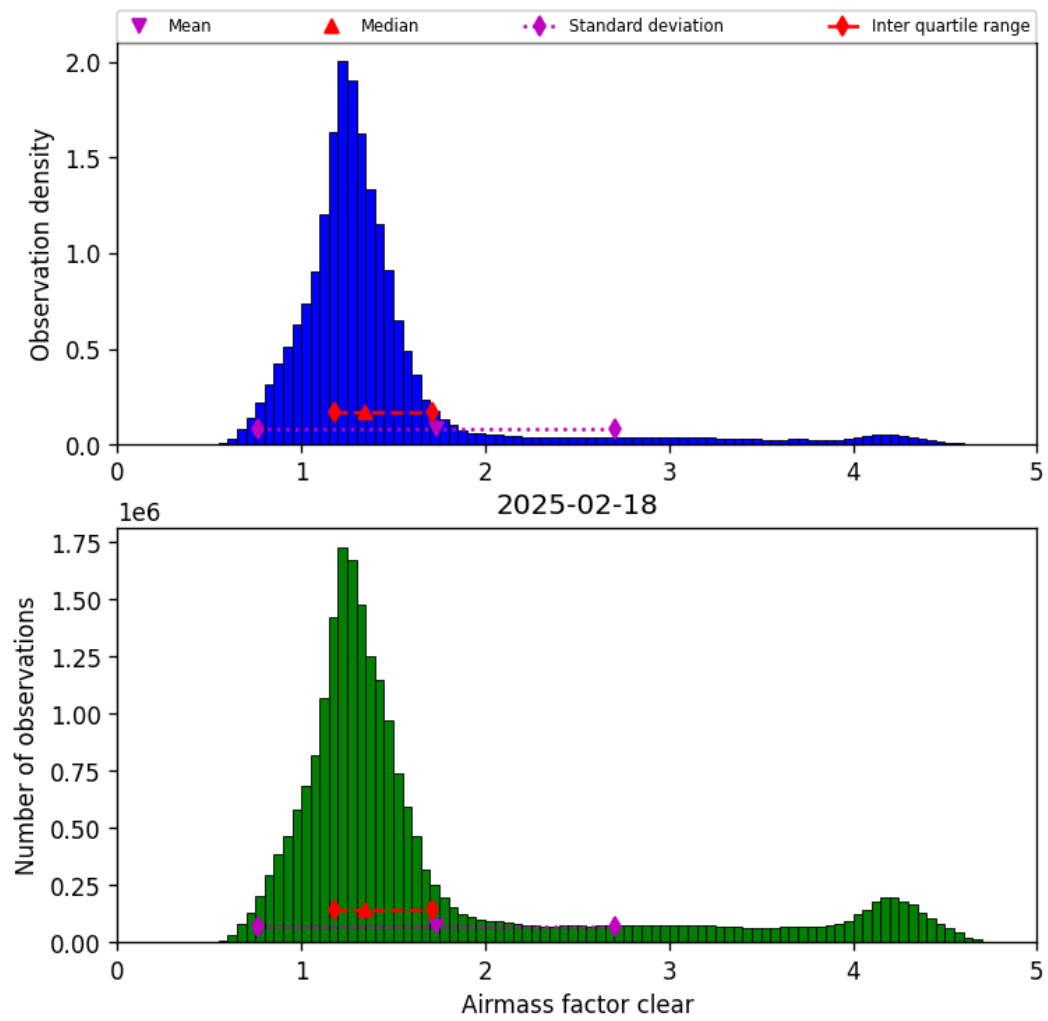
Figure 40: Histogram of “Airmass factor clear” for 2025-02-18 to 2025-02-19
