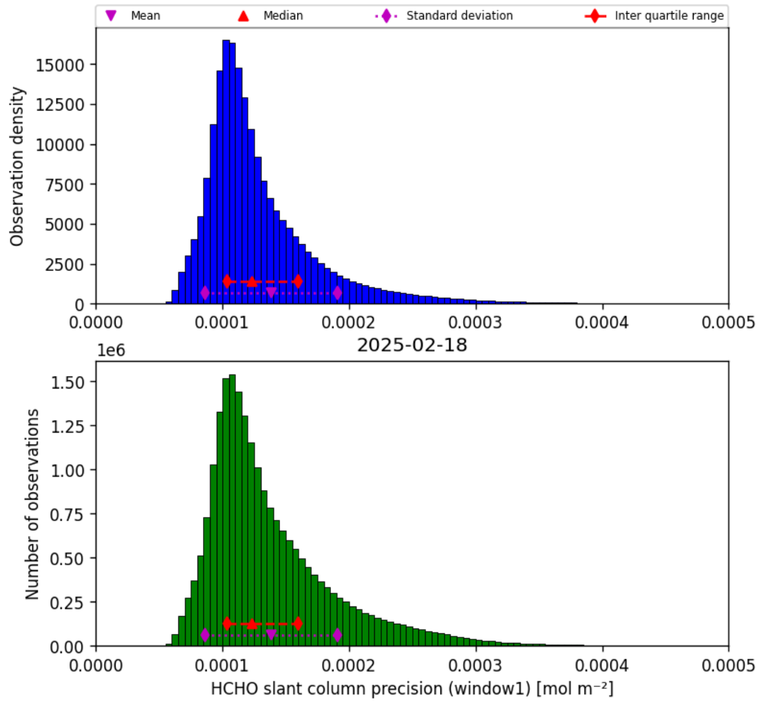
Figure 37: Histogram of “HCHO slant column precision (window1)” for 2025-02-18 to 2025-02-19
