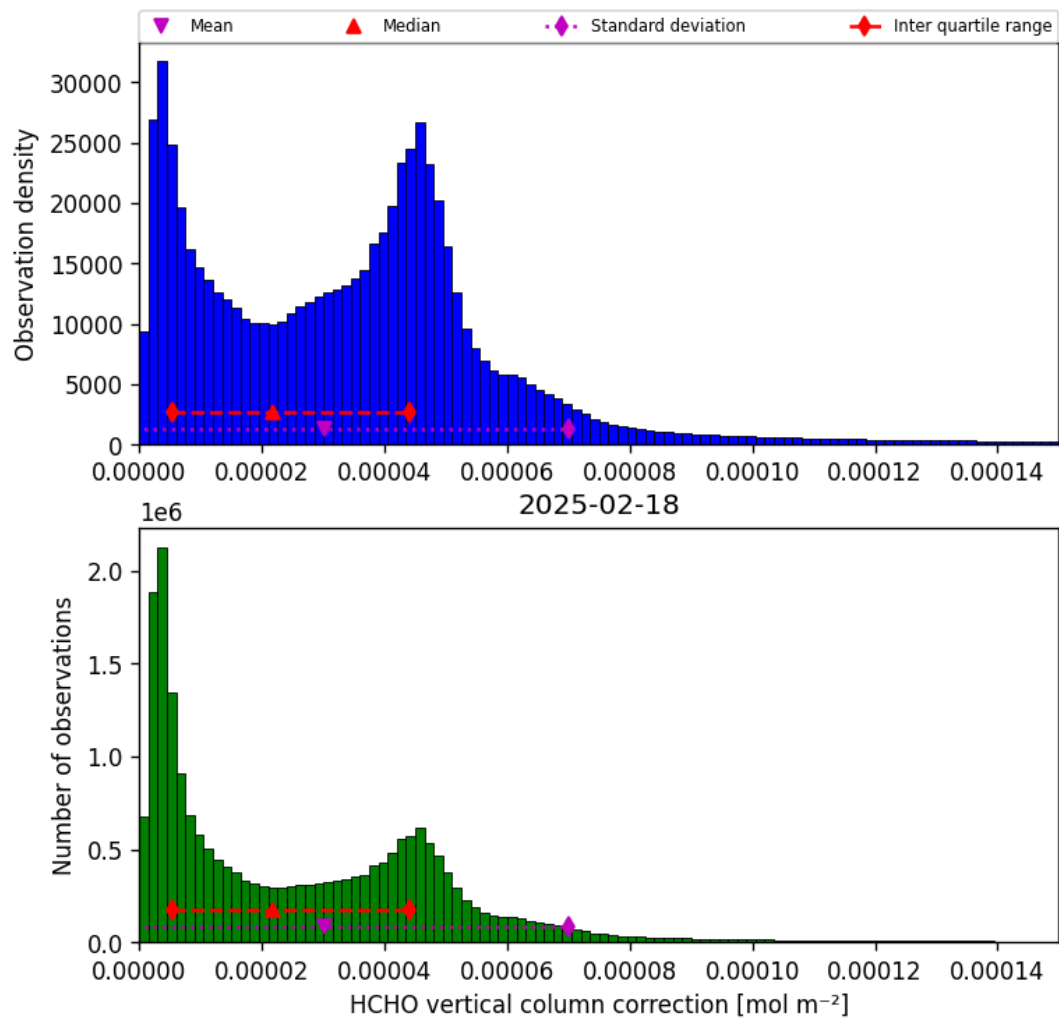
Figure 35: Histogram of “HCHO vertical column correction” for 2025-02-18 to 2025-02-19
