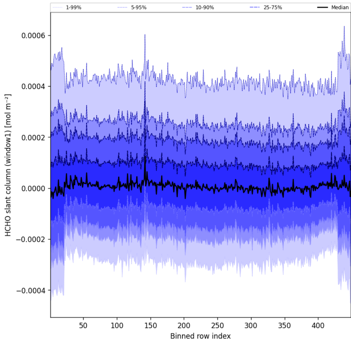
Figure 50: Along track statistics of "HCHO slant column (window1)" for 2025-02-18 to 2025-02-19
