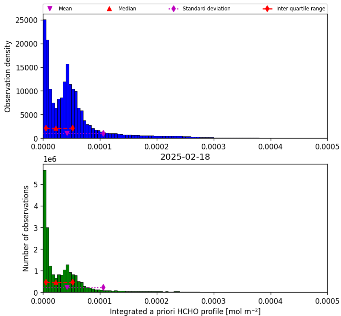
Figure 41: Histogram of “Integrated a priori HCHO profile” for 2025-02-18 to 2025-02-19
