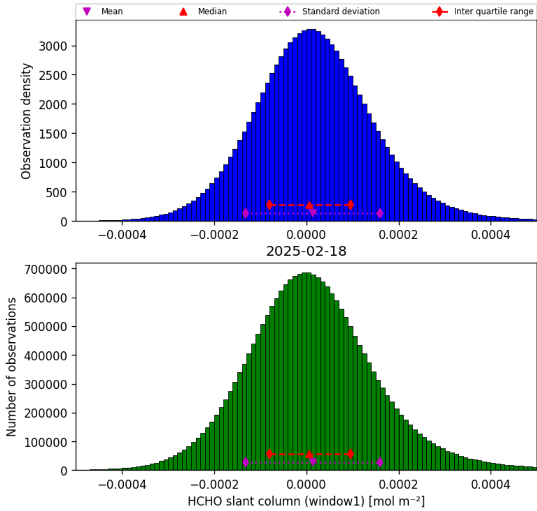
Figure 36: Histogram of “HCHO slant column (window1)” for 2025-02-18 to 2025-02-19
