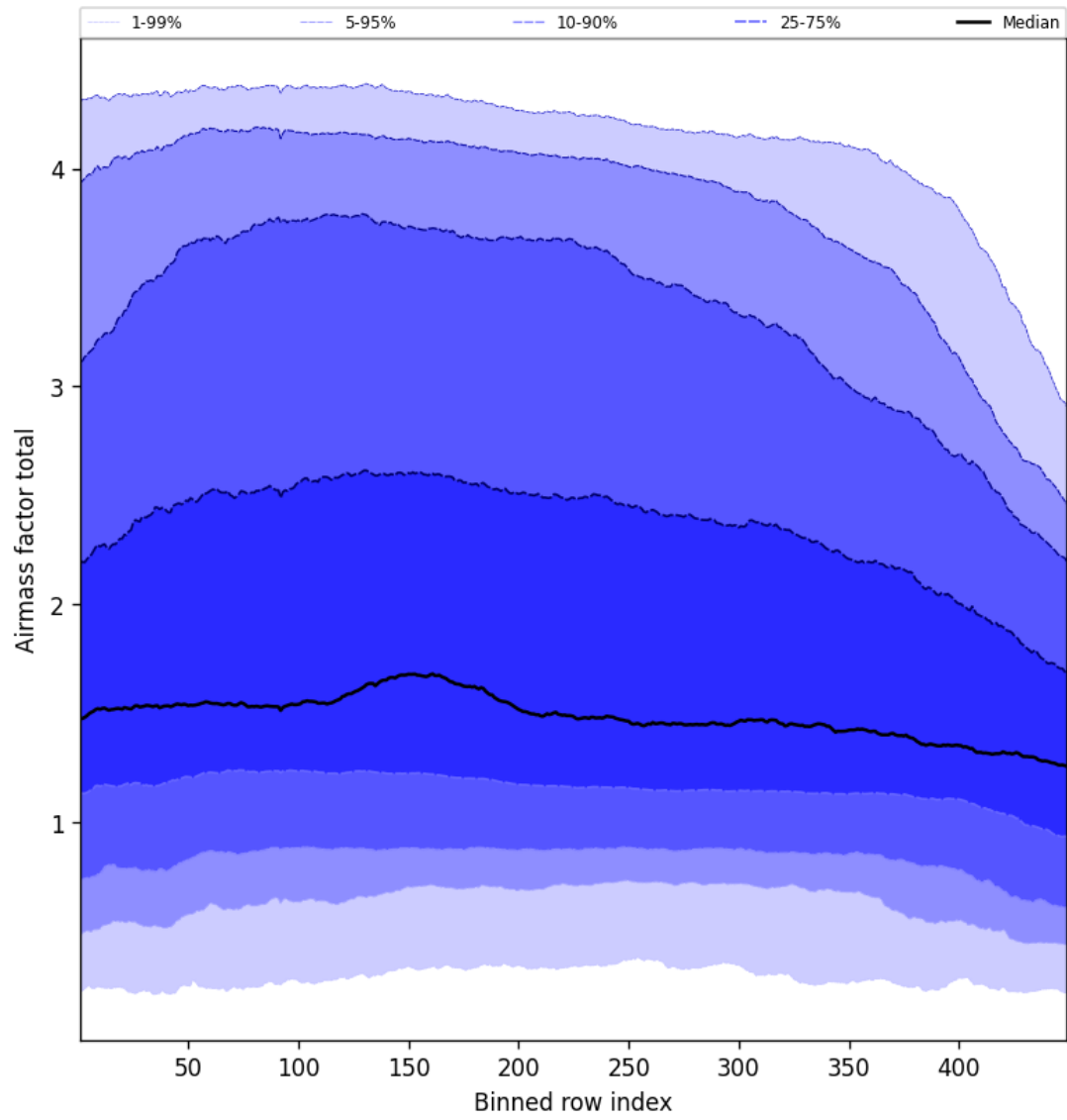
Figure 52: Along track statistics of “Airmass factor total” for 2025-02-18 to 2025-02-19
