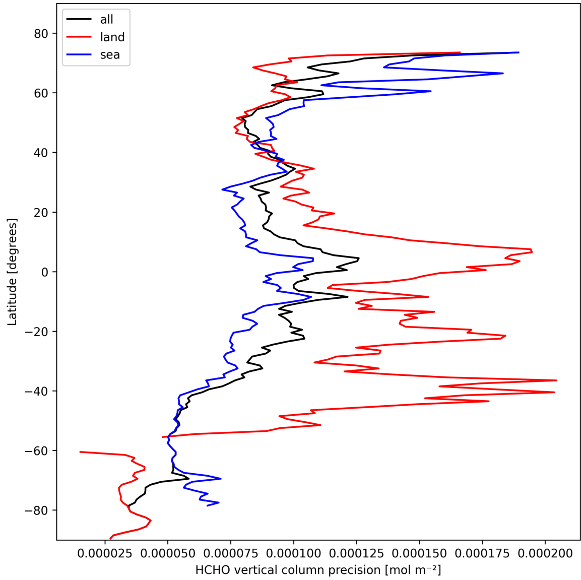
Figure 20: Zonal average of “HCHO vertical column precision” for 2025-02-18 to 2025-02-19.
