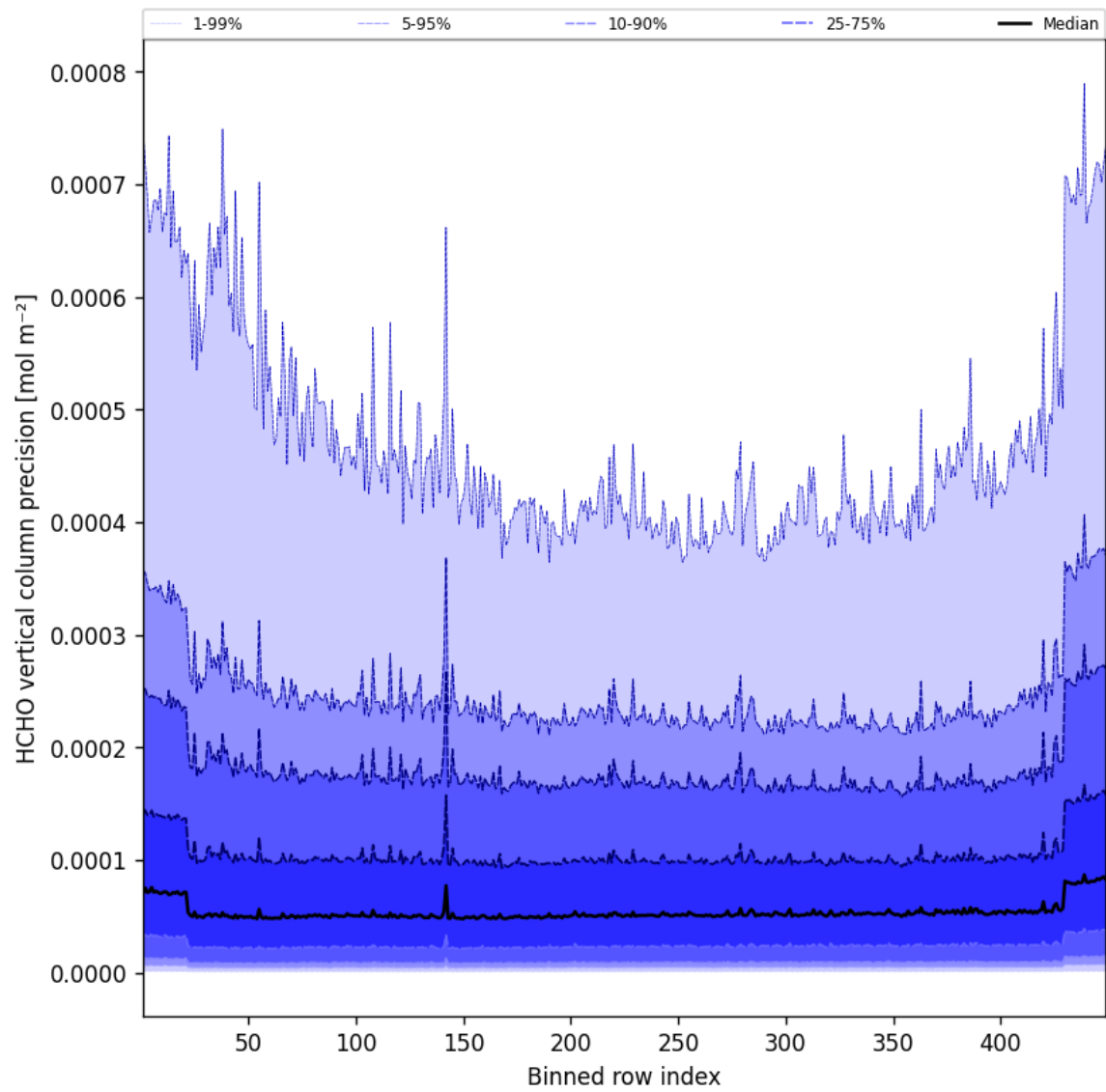
Figure 48: Along track statistics of "HCHO vertical column precision" for 2025-02-18 to 2025-02-19
