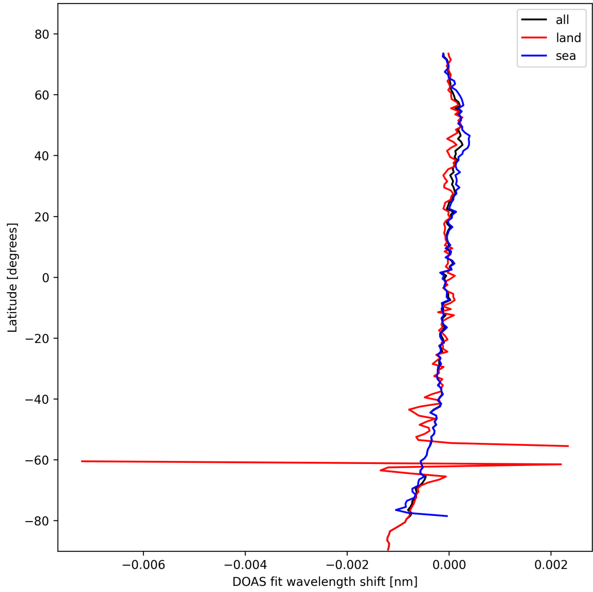
Figure 28: Zonal average of “DOAS fit wavelength shift” for 2025-02-18 to 2025-02-19.
