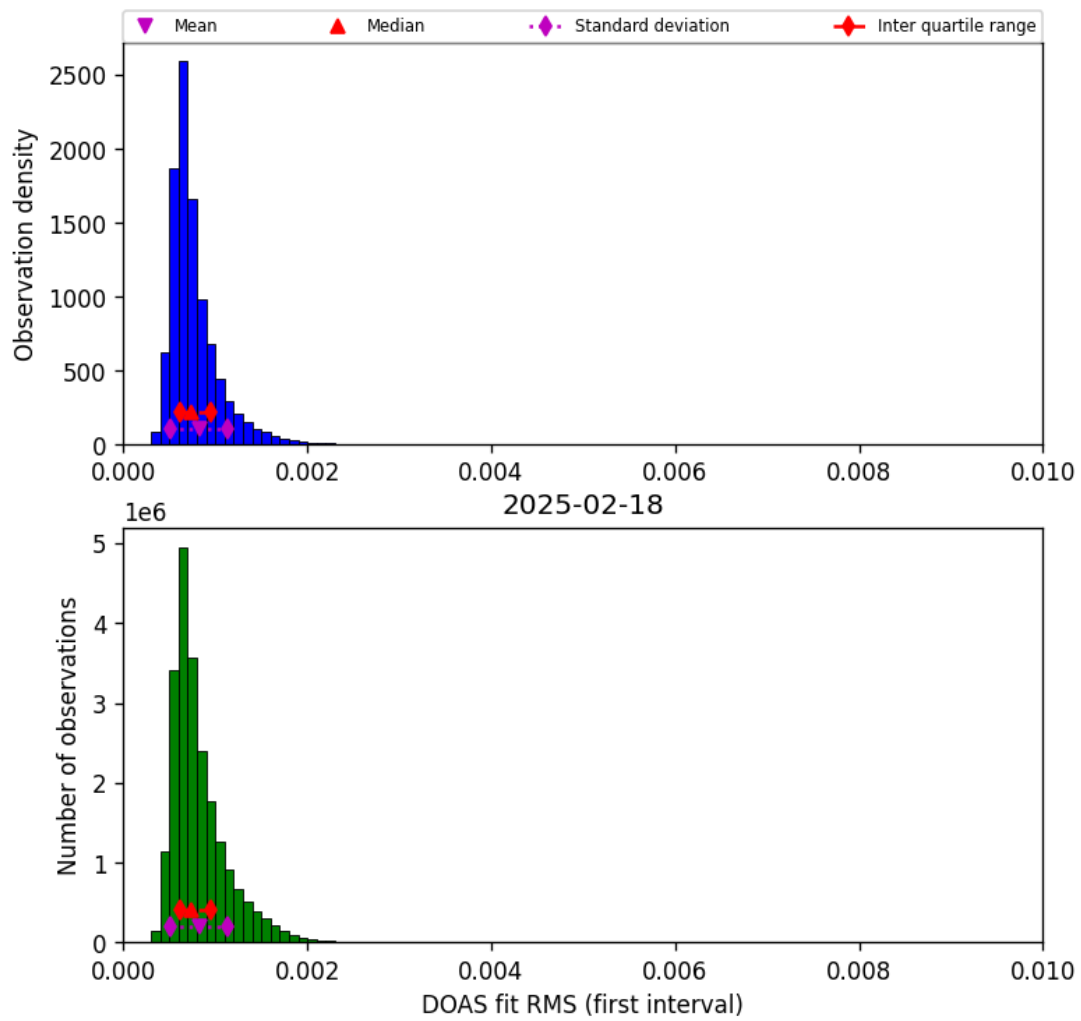
Figure 44: Histogram of “DOAS fit RMS (first interval)” for 2025-02-18 to 2025-02-19
