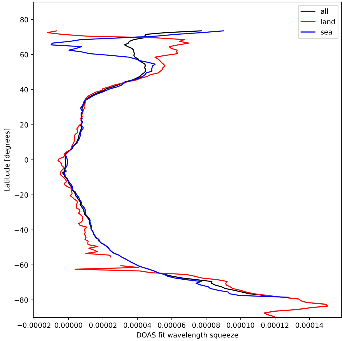
Figure 29: Zonal average of “DOAS fit wavelength squeeze” for 2025-02-18 to 2025-02-19.
