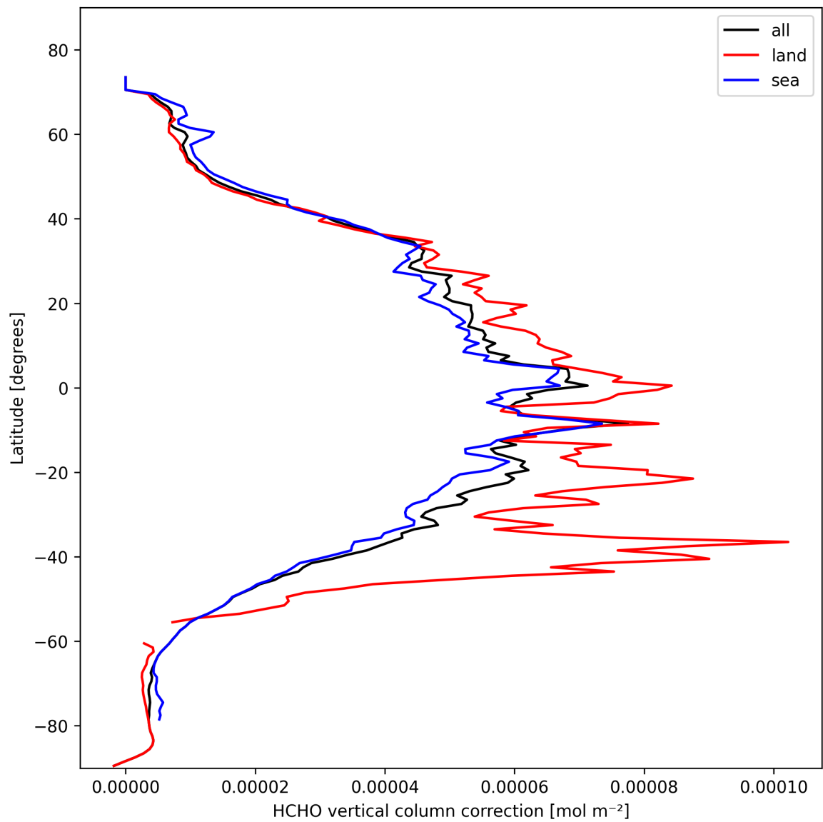
Figure 21: Zonal average of “HCHO vertical column correction” for 2025-02-18 to 2025-02-19.
