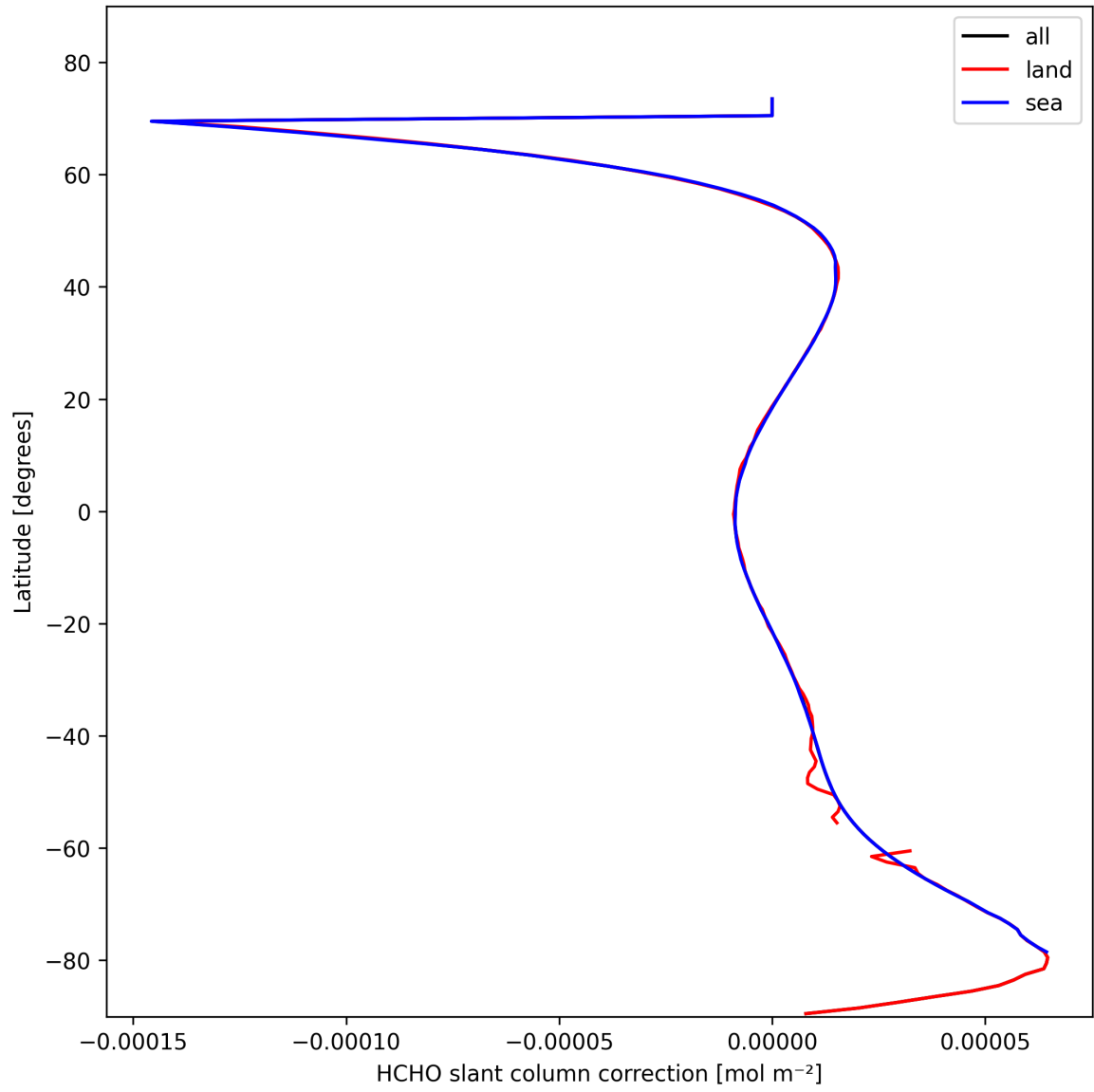
Figure 31: Zonal average of “HCHO slant column correction” for 2025-02-18 to 2025-02-19.
