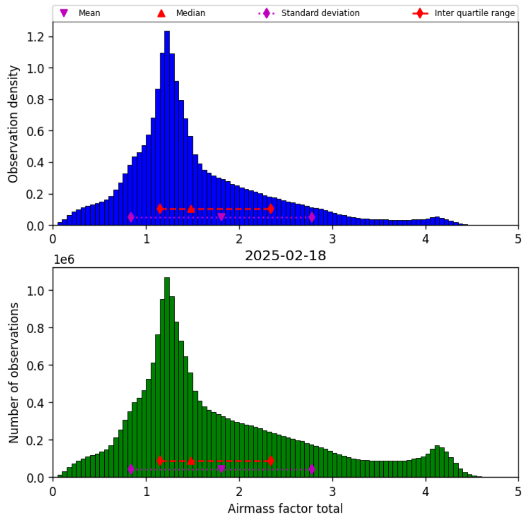
Figure 38: Histogram of “Airmass factor total” for 2025-02-18 to 2025-02-19
