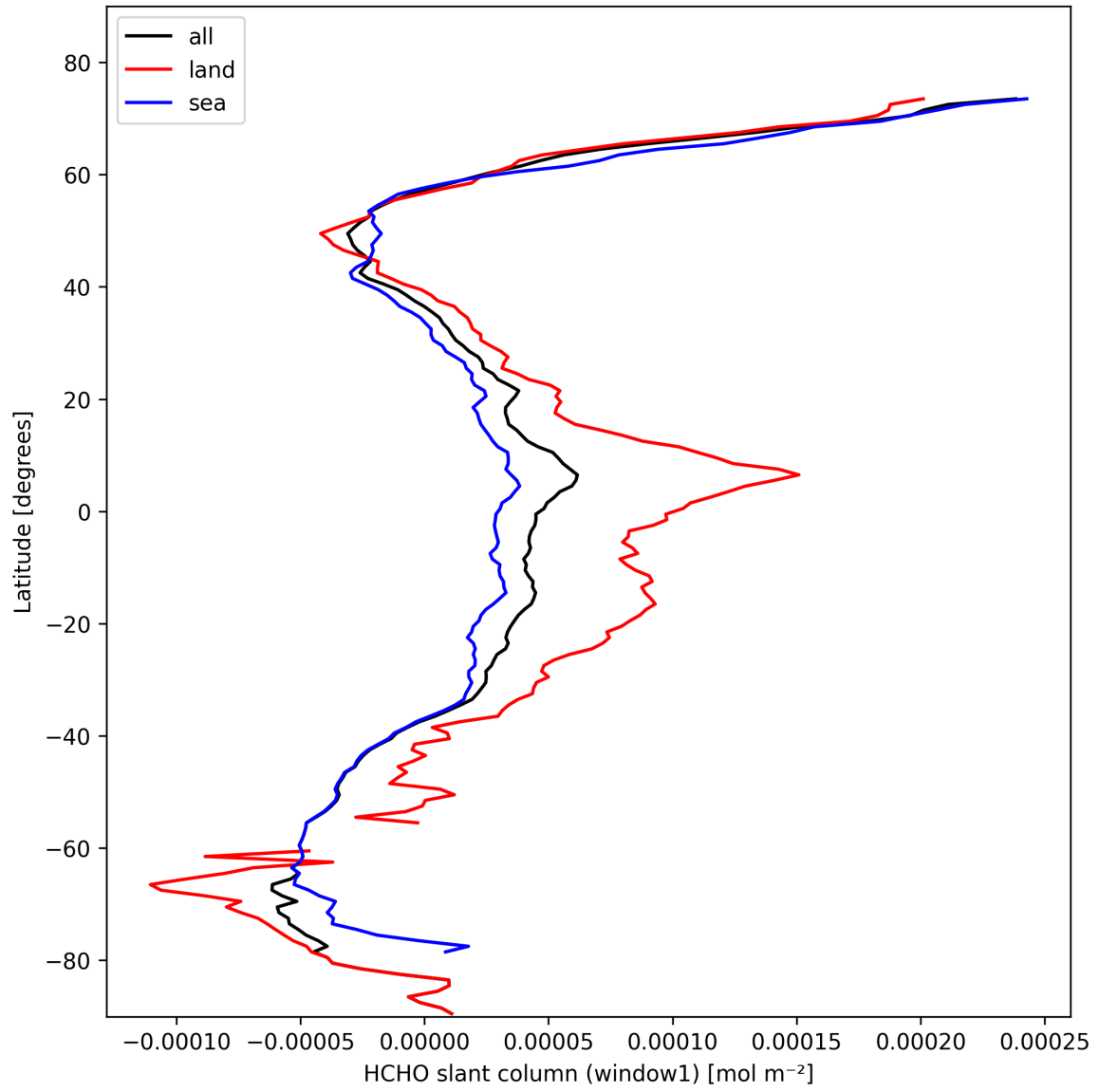
Figure 22: Zonal average of “HCHO slant column (window1)” for 2025-02-18 to 2025-02-19.
