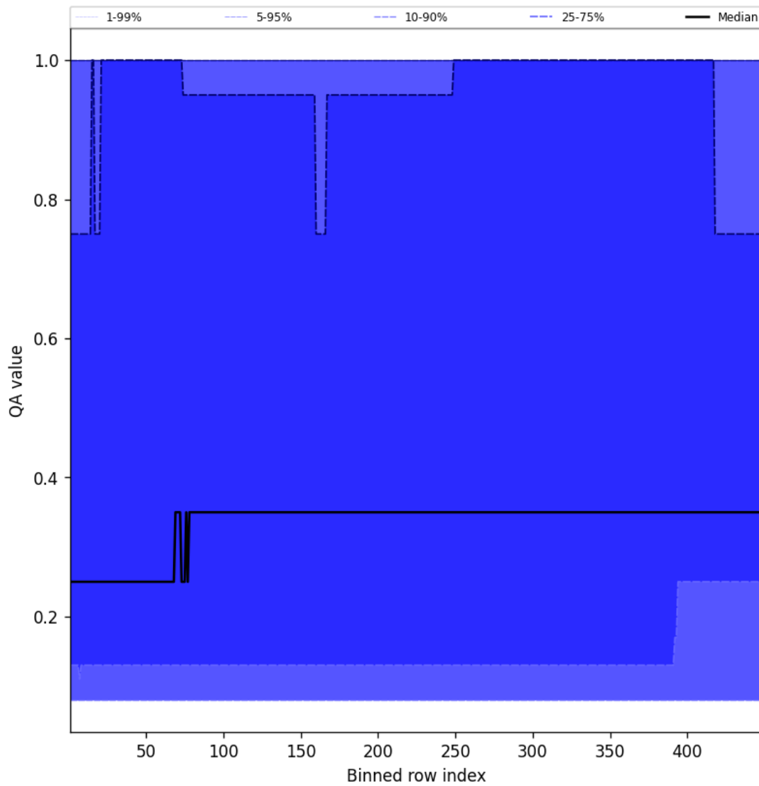
Figure 46: Along track statistics of “QA value” for 2025-02-18 to 2025-02-19
