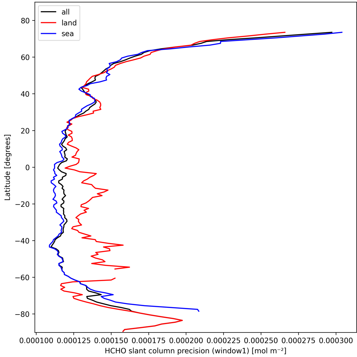
Figure 23: Zonal average of “HCHO slant column precision (window1)” for 2025-02-18 to 2025-02-19.
