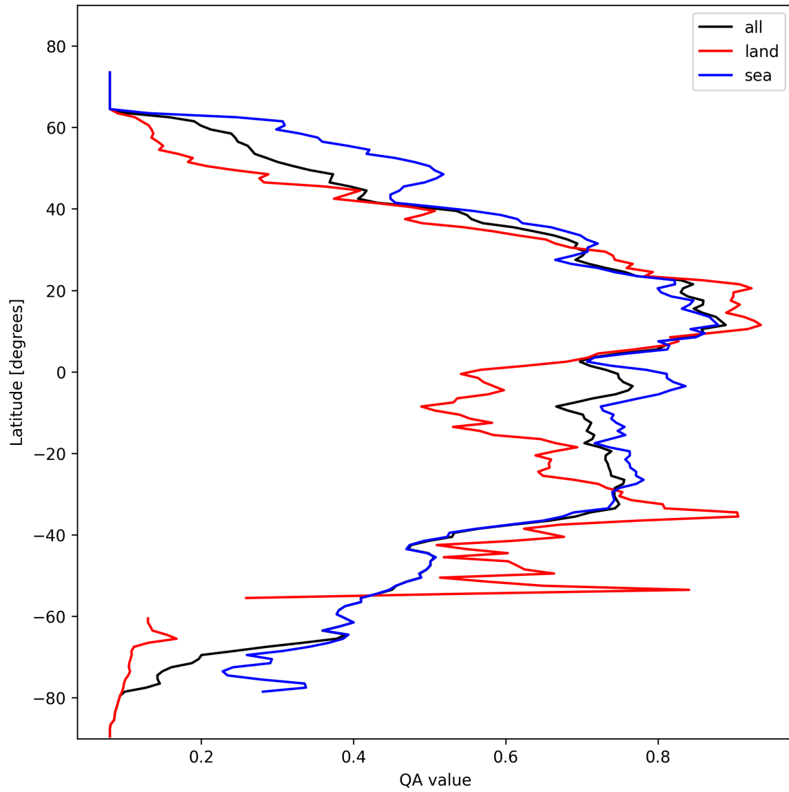
Figure 18: Zonal average of “QA value” for 2025-02-18 to 2025-02-19.
