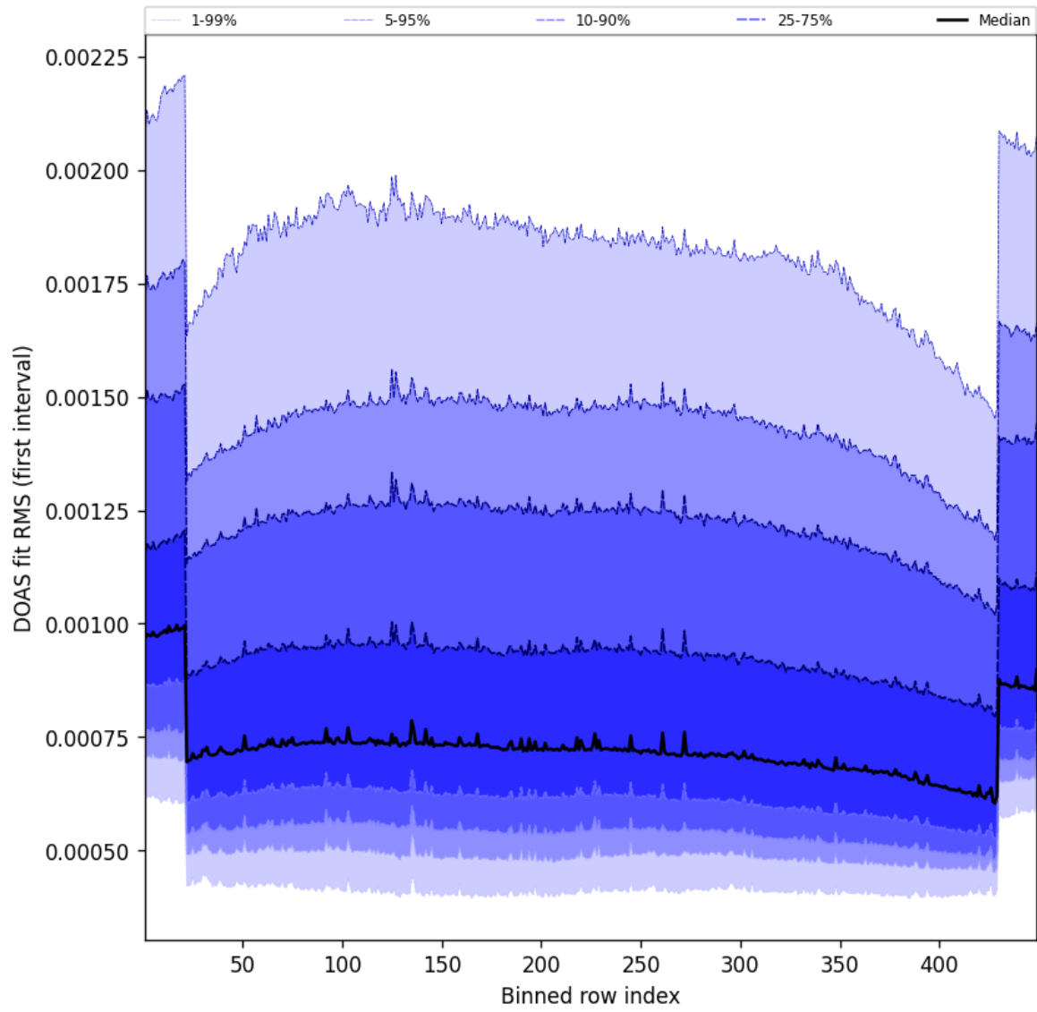
Figure 58: Along track statistics of “DOAS fit RMS (first interval)” for 2025-02-18 to 2025-02-19
