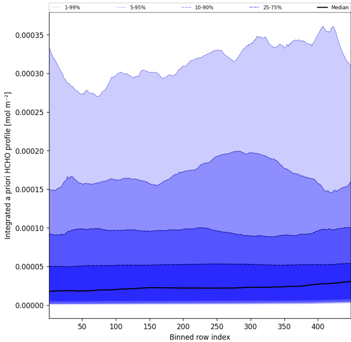
Figure 55: Along track statistics of “Integrated a priori HCHO profile” for 2025-02-18 to 2025-02-19
