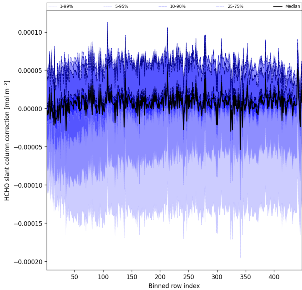
Figure 59: Along track statistics of “HCHO slant column correction” for 2025-02-18 to 2025-02-19
