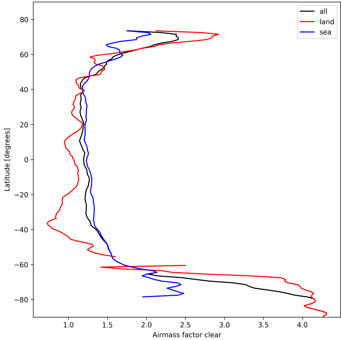
Figure 26: Zonal average of “Airmass factor clear” for 2025-02-18 to 2025-02-19.
