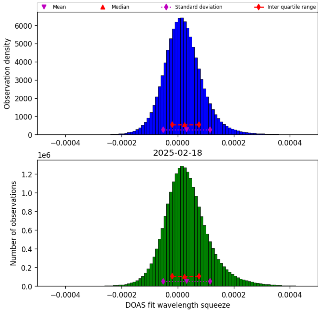
Figure 43: Histogram of “DOAS fit wavelength squeeze” for 2025-02-18 to 2025-02-19
