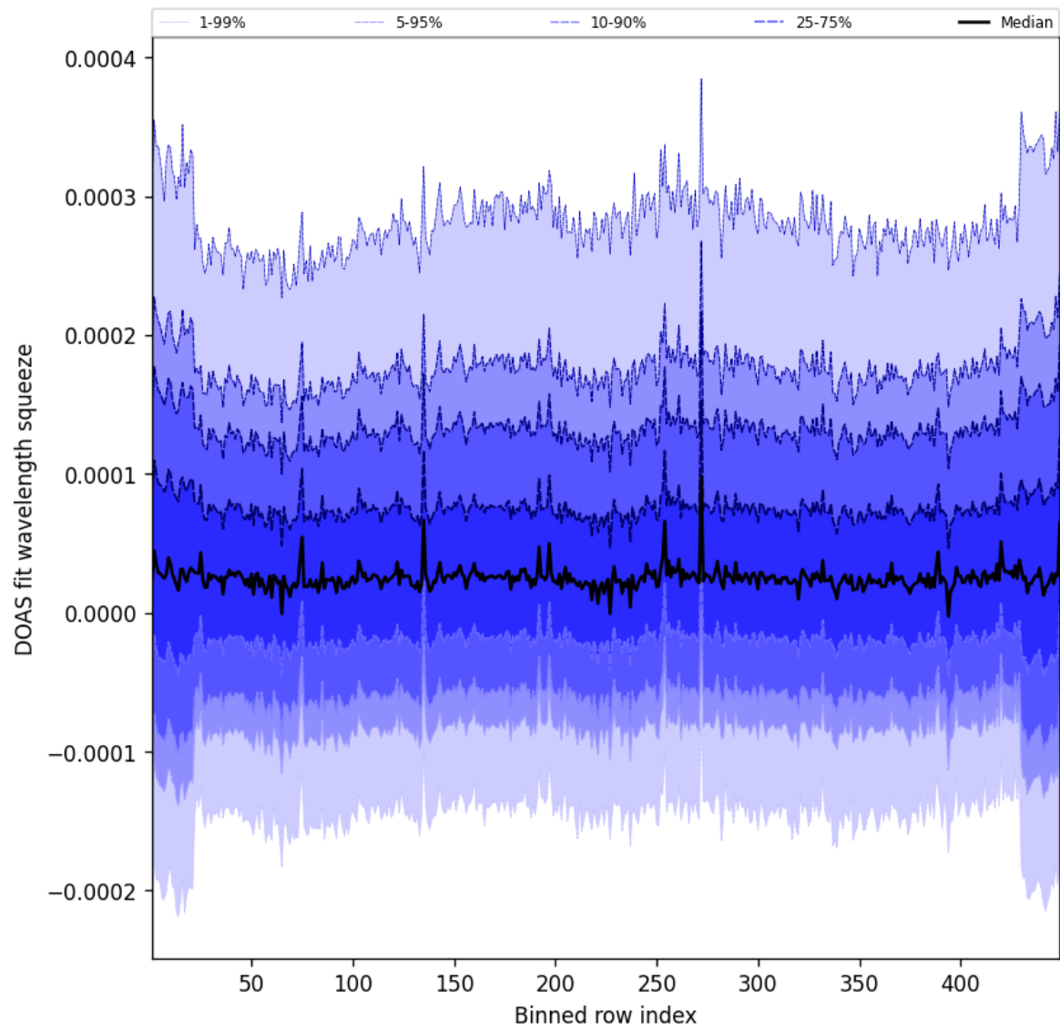
Figure 57: Along track statistics of “DOAS fit wavelength squeeze” for 2025-02-18 to 2025-02-19
