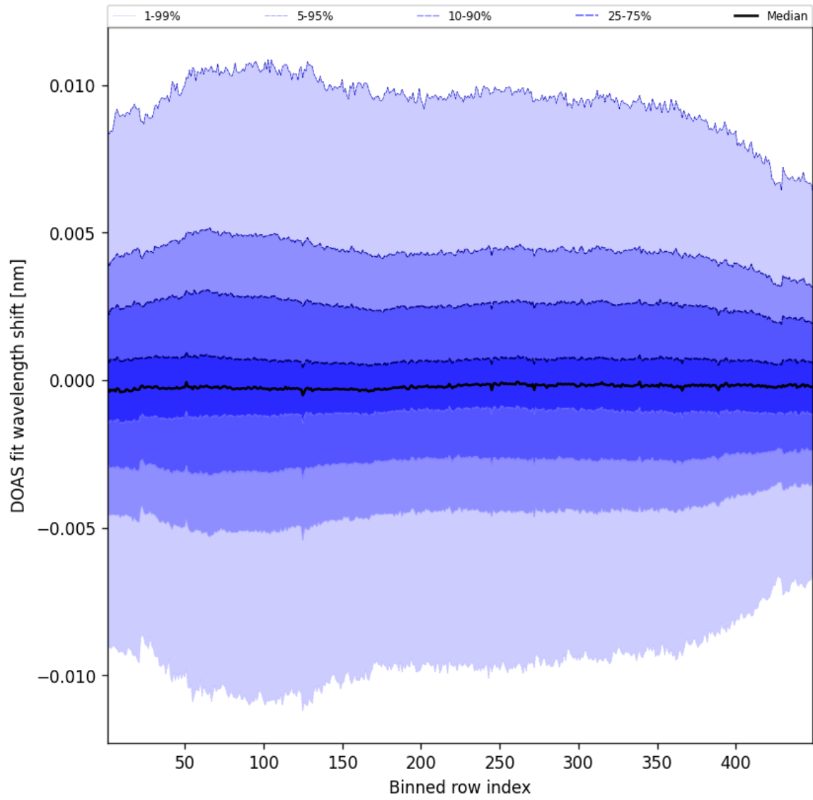
Figure 56: Along track statistics of “DOAS fit wavelength shift” for 2025-02-18 to 2025-02-19
