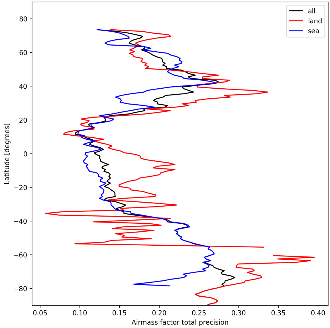
Figure 25: Zonal average of “Airmass factor total precision” for 2025-02-18 to 2025-02-19.
