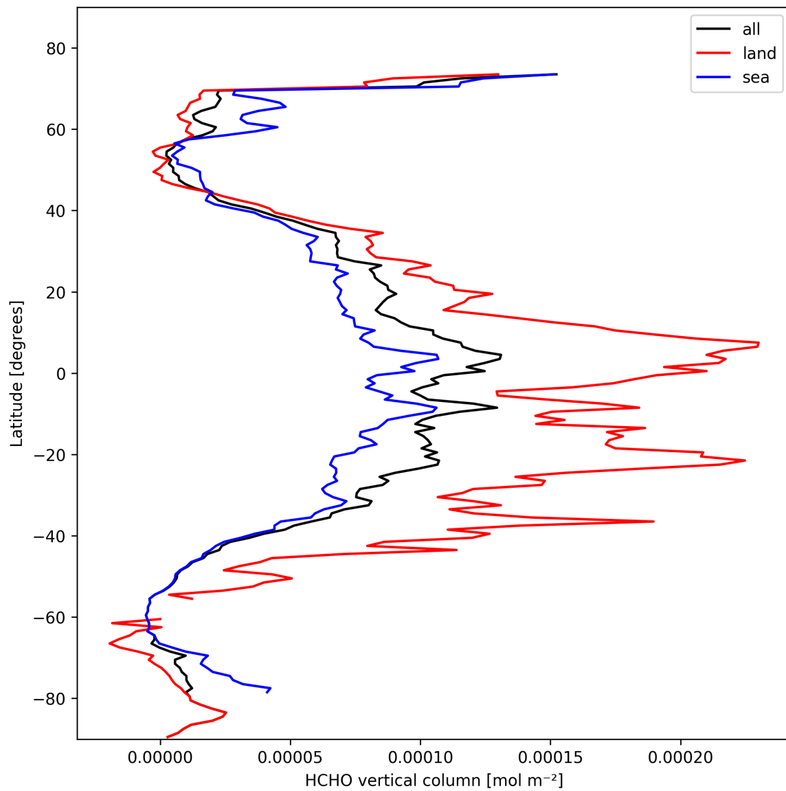
Figure 19: Zonal average of “HCHO vertical column” for 2025-02-18 to 2025-02-19.
