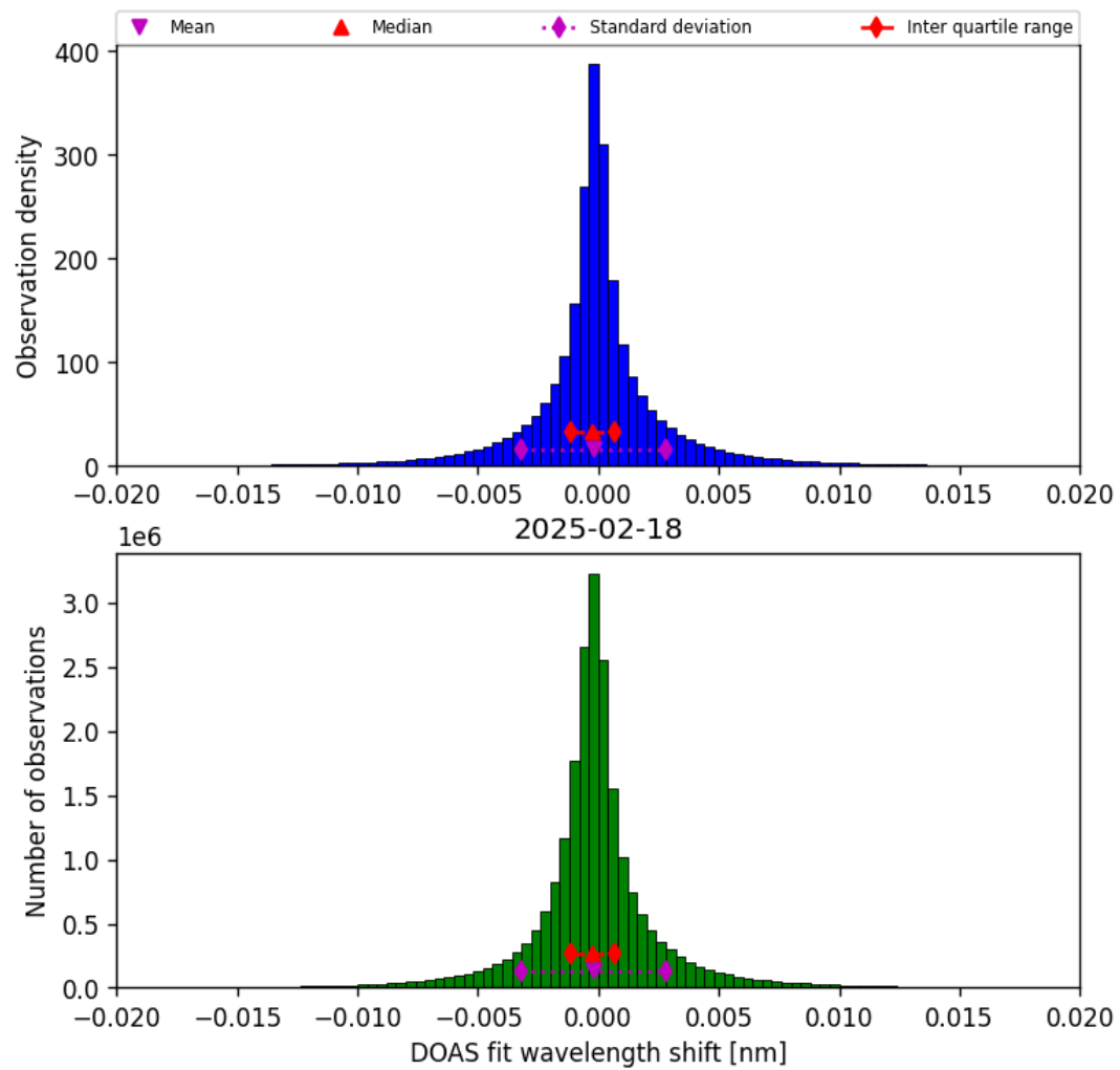
Figure 42: Histogram of “DOAS fit wavelength shift” for 2025-02-18 to 2025-02-19
