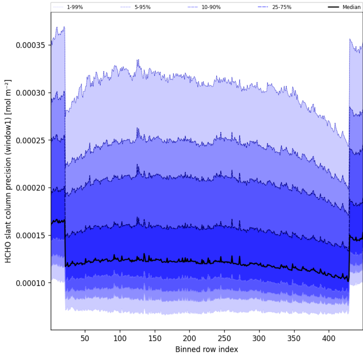
Figure 51: Along track statistics of “HCHO slant column precision (window1)” for 2025-02-18 to 2025-02-19
