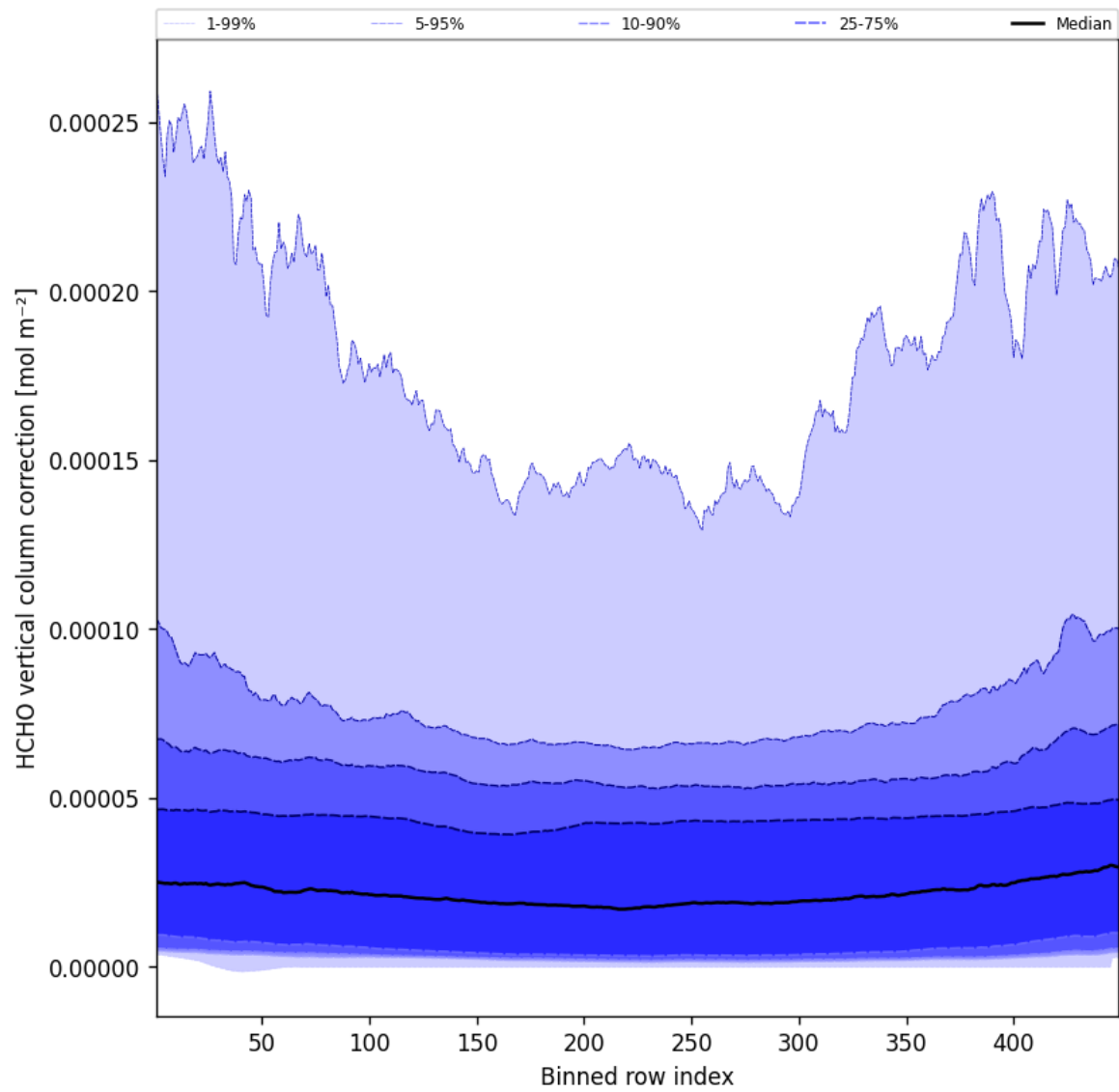
Figure 49: Along track statistics of “HCHO vertical column correction” for 2025-02-18 to 2025-02-19
