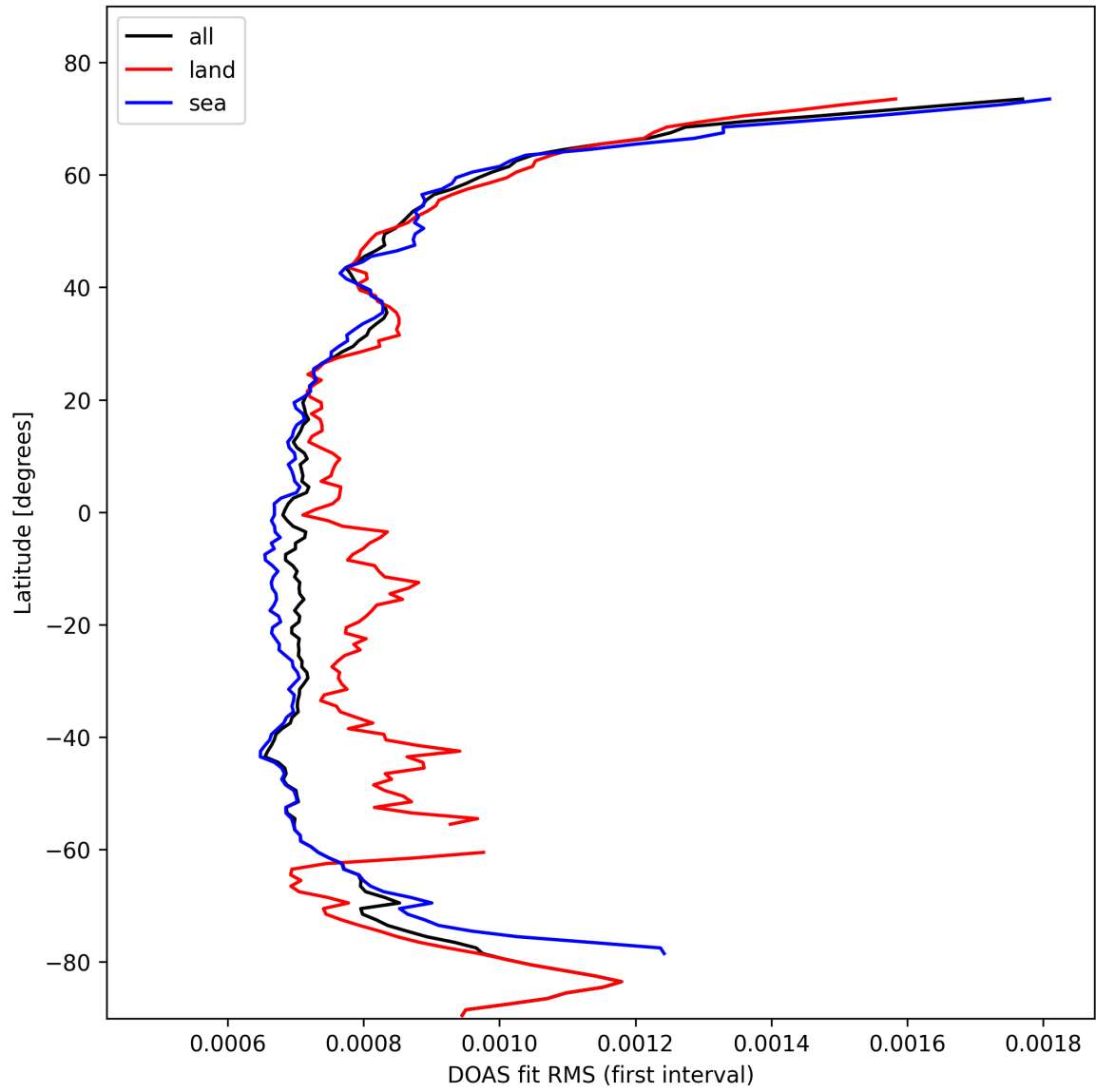
Figure 30: Zonal average of “DOAS fit RMS (first interval)” for 2025-02-18 to 2025-02-19.
