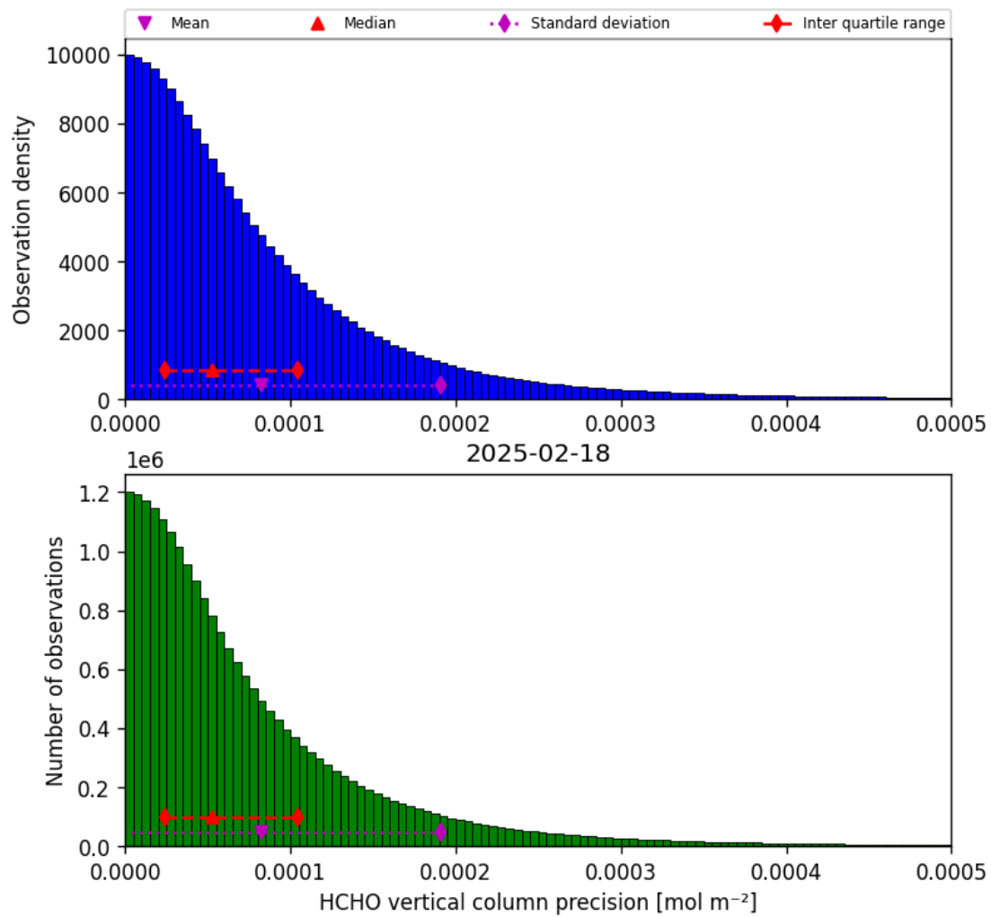
Figure 34: Histogram of “HCHO vertical column precision” for 2025-02-18 to 2025-02-19
