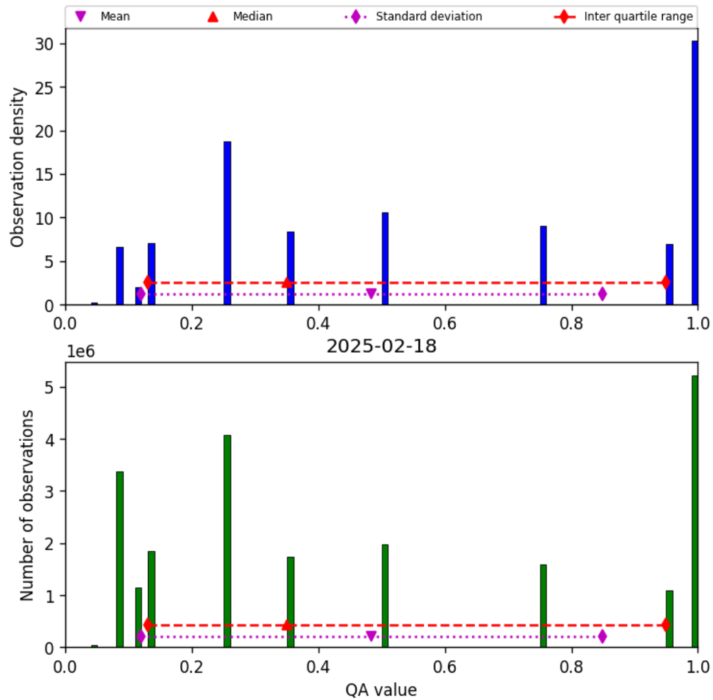
Figure 32: Histogram of “QA value” for 2025-02-18 to 2025-02-19
