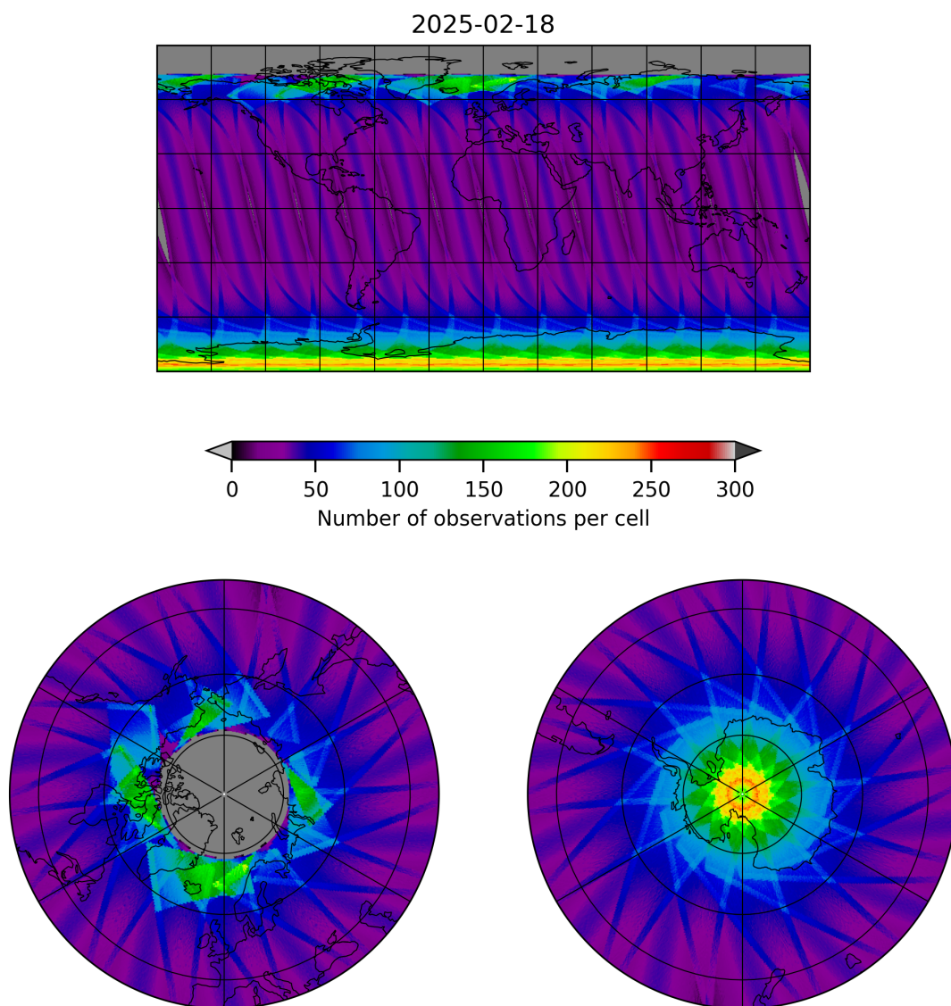
Figure 17: Map of the number of observations for 2025-02-18 to 2025-02-19
