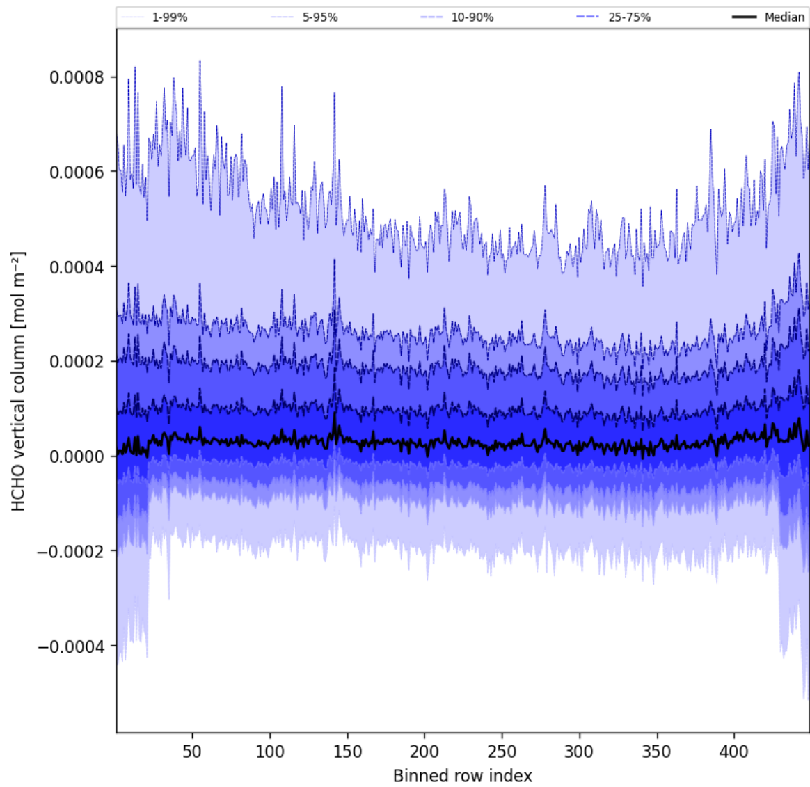
Figure 47: Along track statistics of “HCHO vertical column” for 2025-02-18 to 2025-02-19
