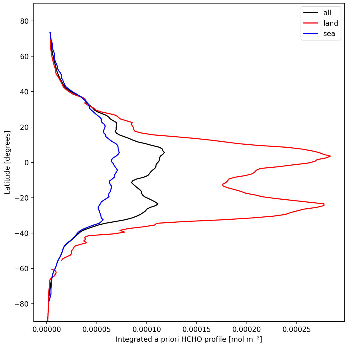
Figure 27: Zonal average of “Integrated a priori HCHO profile” for 2025-02-18 to 2025-02-19.
