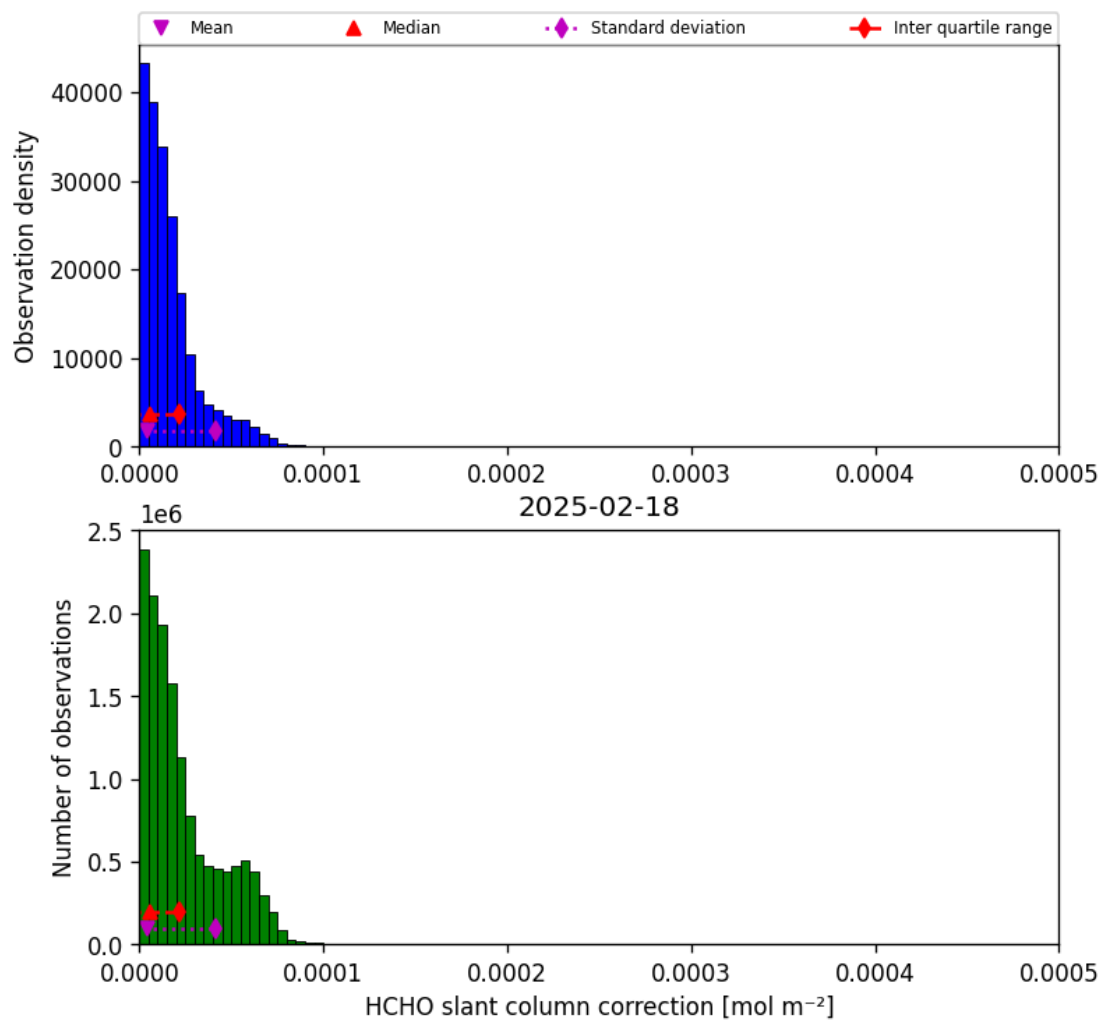
Figure 45: Histogram of “HCHO slant column correction” for 2025-02-18 to 2025-02-19
