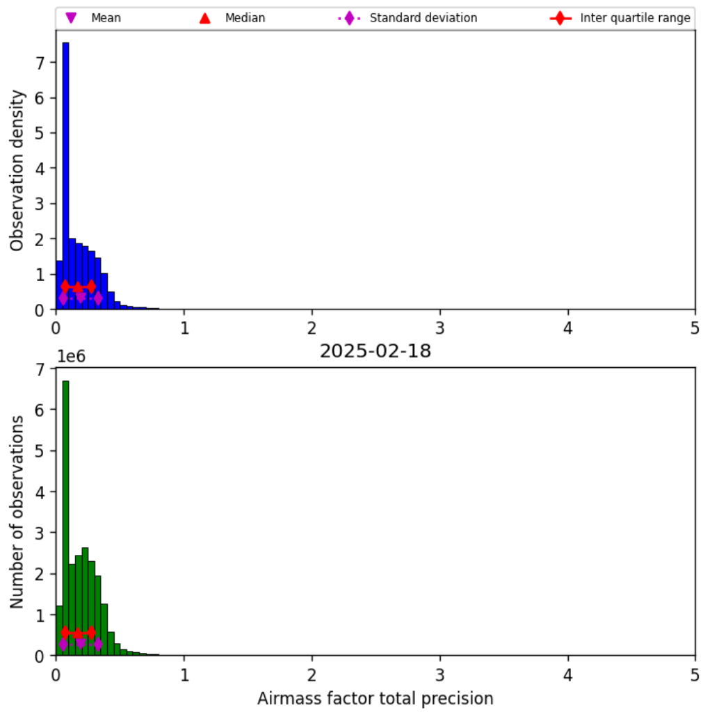
Figure 39: Histogram of “Airmass factor total precision” for 2025-02-18 to 2025-02-19
