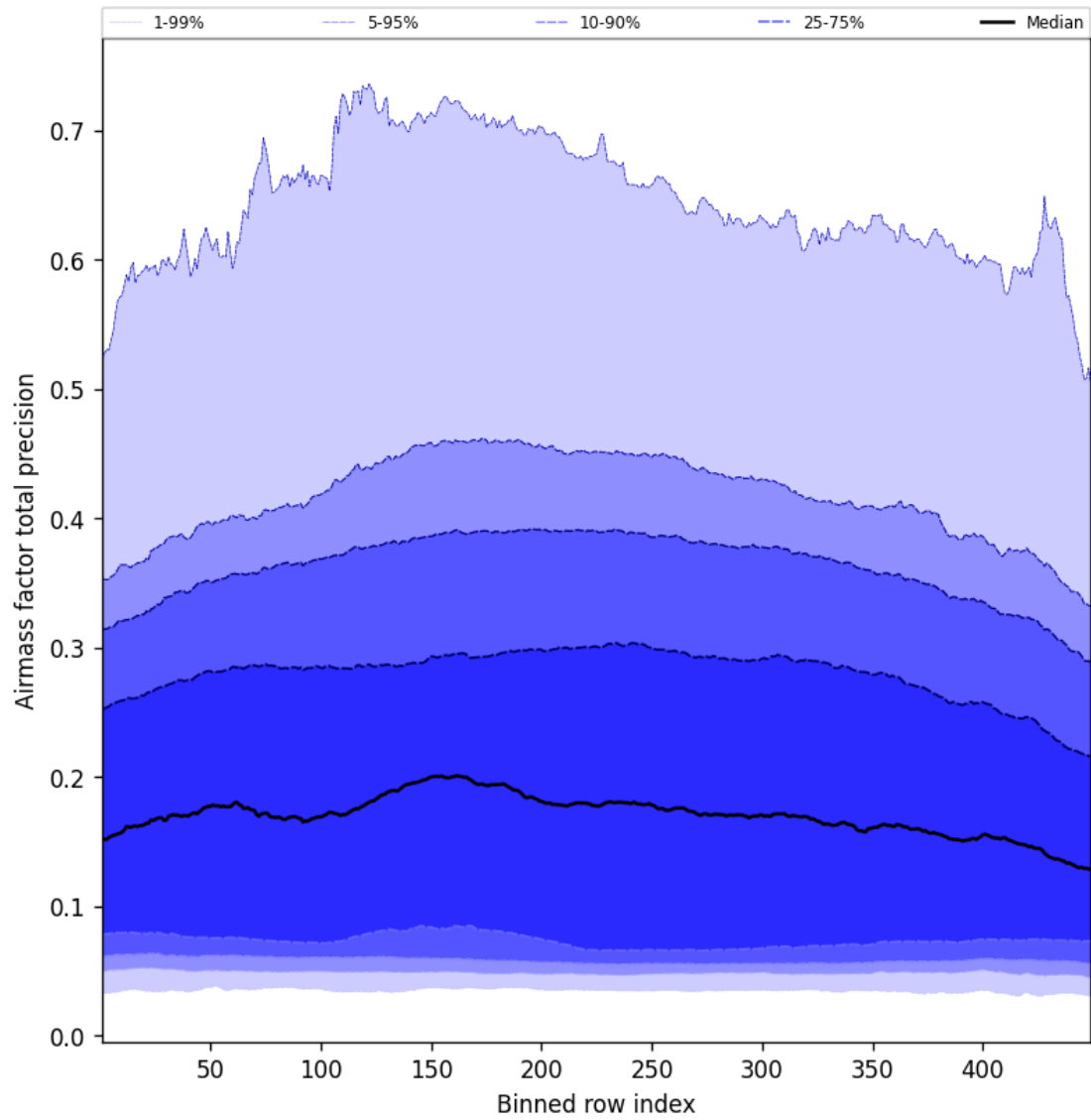
Figure 53: Along track statistics of “Airmass factor total precision” for 2025-02-18 to 2025-02-19
