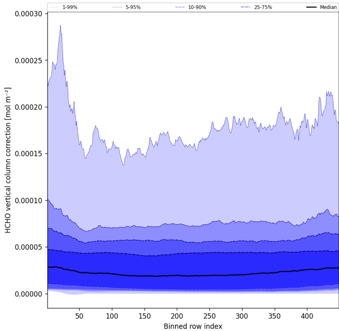
Figure 49: Along track statistics of “HCHO vertical column correction” for 2025-02-19 to 2025-02-20
