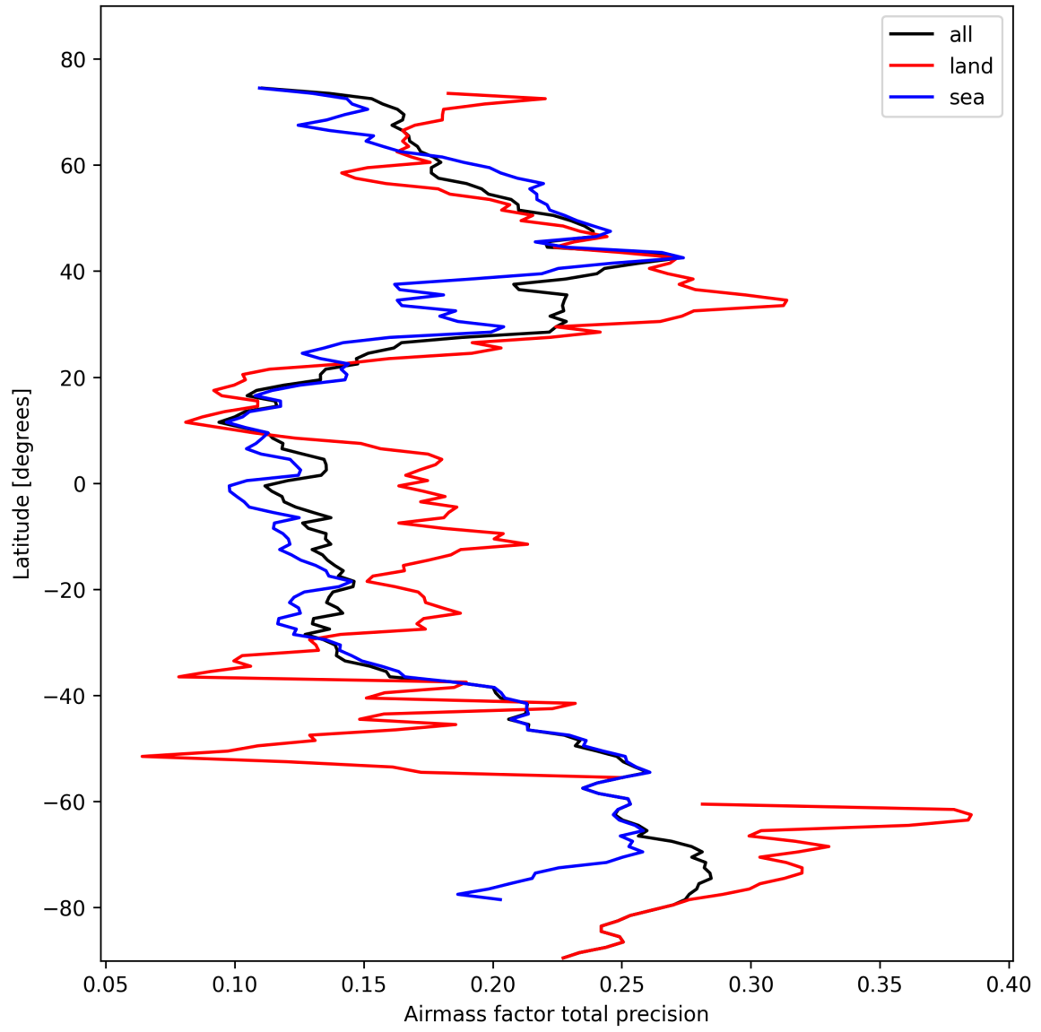
Figure 25: Zonal average of “Airmass factor total precision” for 2025-02-19 to 2025-02-20.
