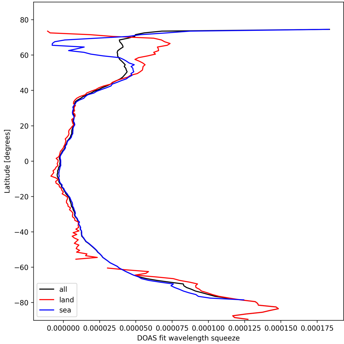
Figure 29: Zonal average of “DOAS fit wavelength squeeze” for 2025-02-19 to 2025-02-20.
