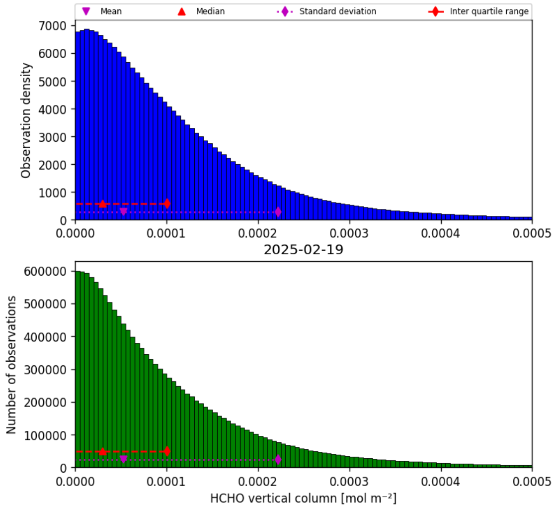
Figure 33: Histogram of “HCHO vertical column” for 2025-02-19 to 2025-02-20
