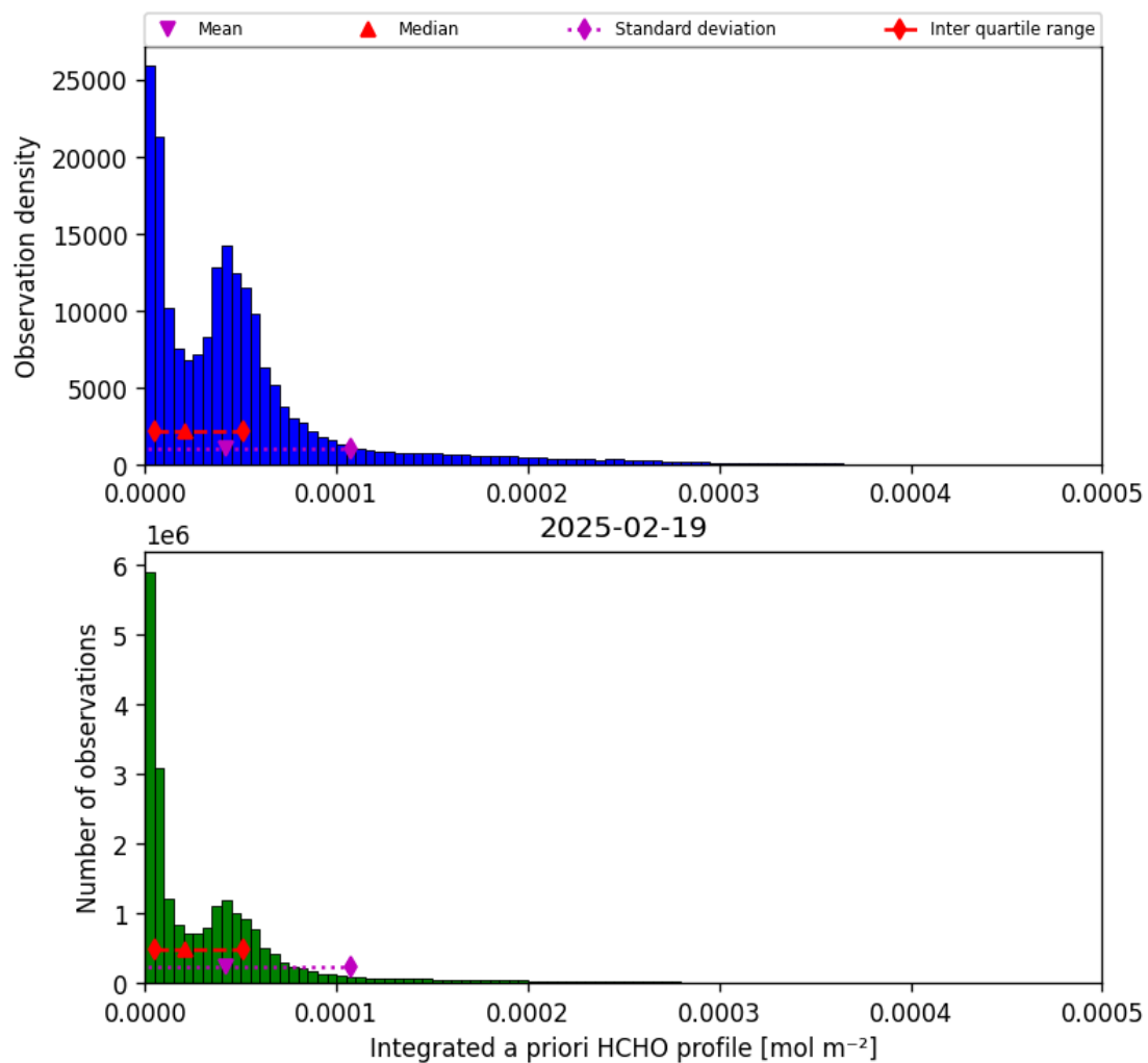
Figure 41: Histogram of “Integrated a priori HCHO profile” for 2025-02-19 to 2025-02-20
