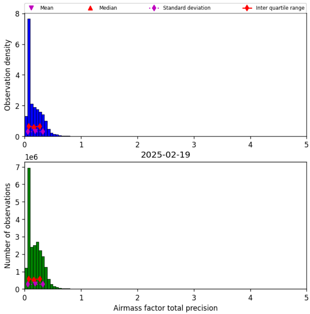
Figure 39: Histogram of “Airmass factor total precision” for 2025-02-19 to 2025-02-20
