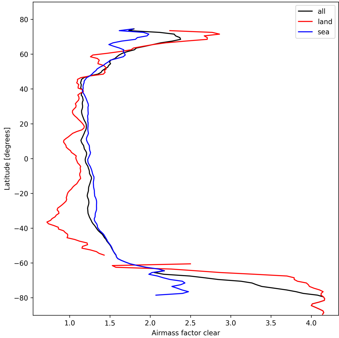
Figure 26: Zonal average of “Airmass factor clear” for 2025-02-19 to 2025-02-20.
