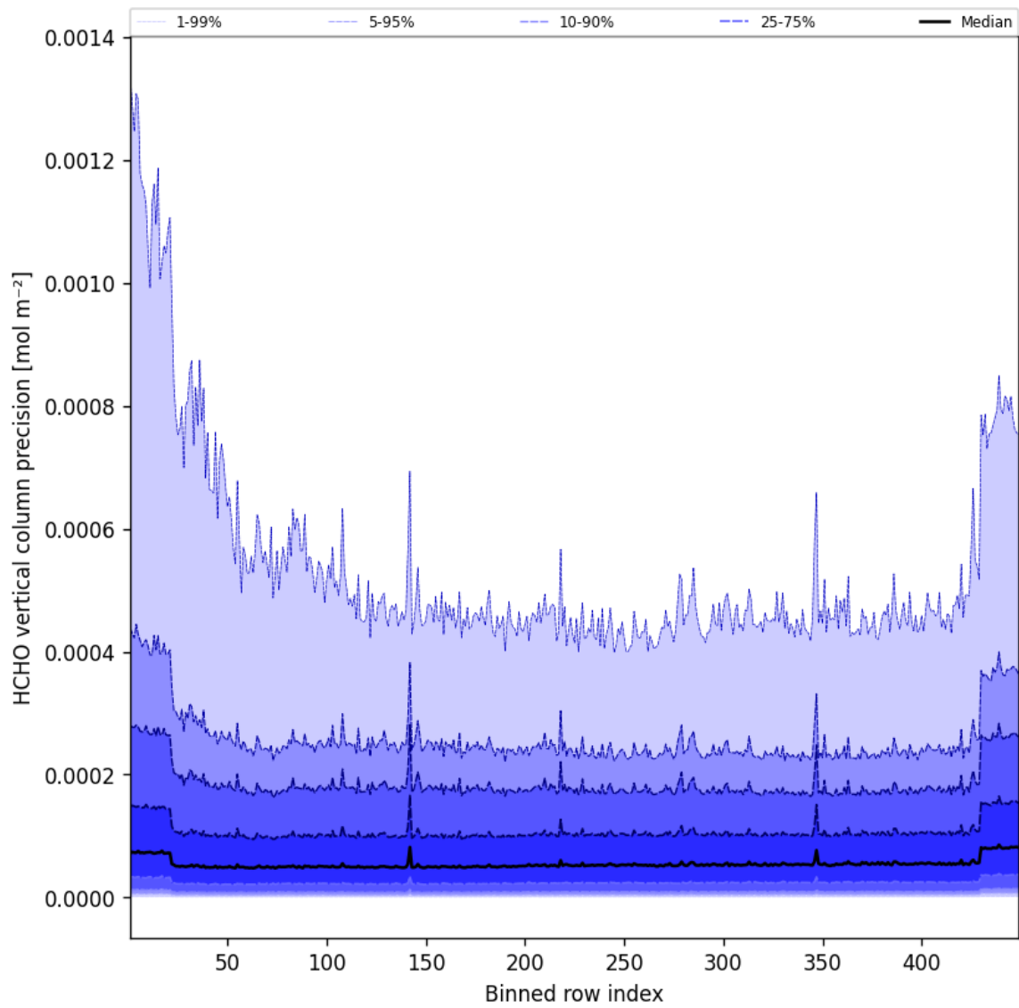
Figure 48: Along track statistics of “HCHO vertical column precision” for 2025-02-19 to 2025-02-20
