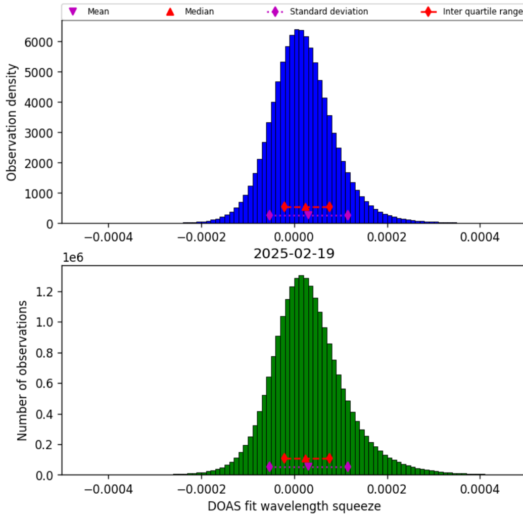
Figure 43: Histogram of “DOAS fit wavelength squeeze” for 2025-02-19 to 2025-02-20
