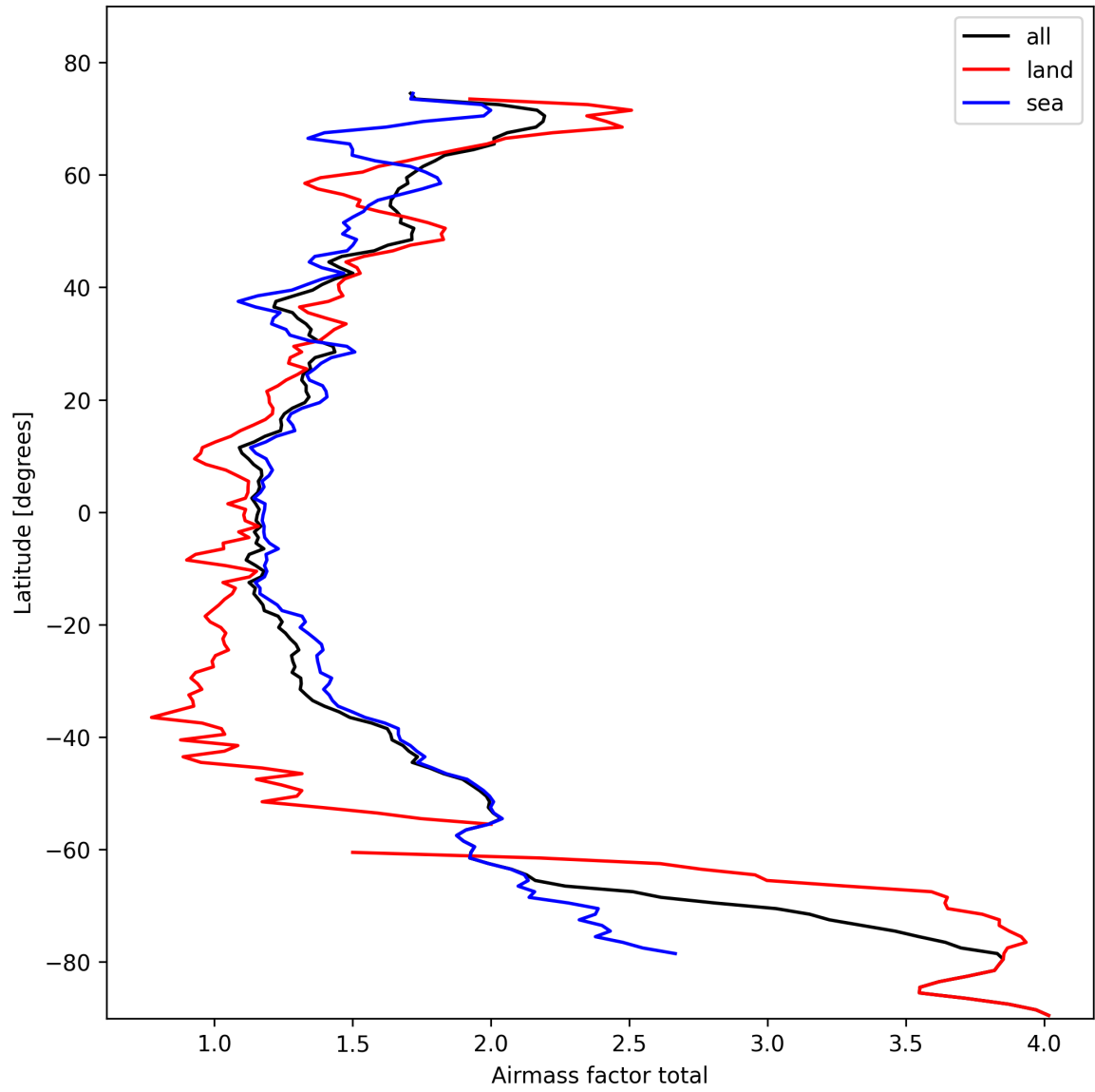
Figure 24: Zonal average of “Airmass factor total” for 2025-02-19 to 2025-02-20.
