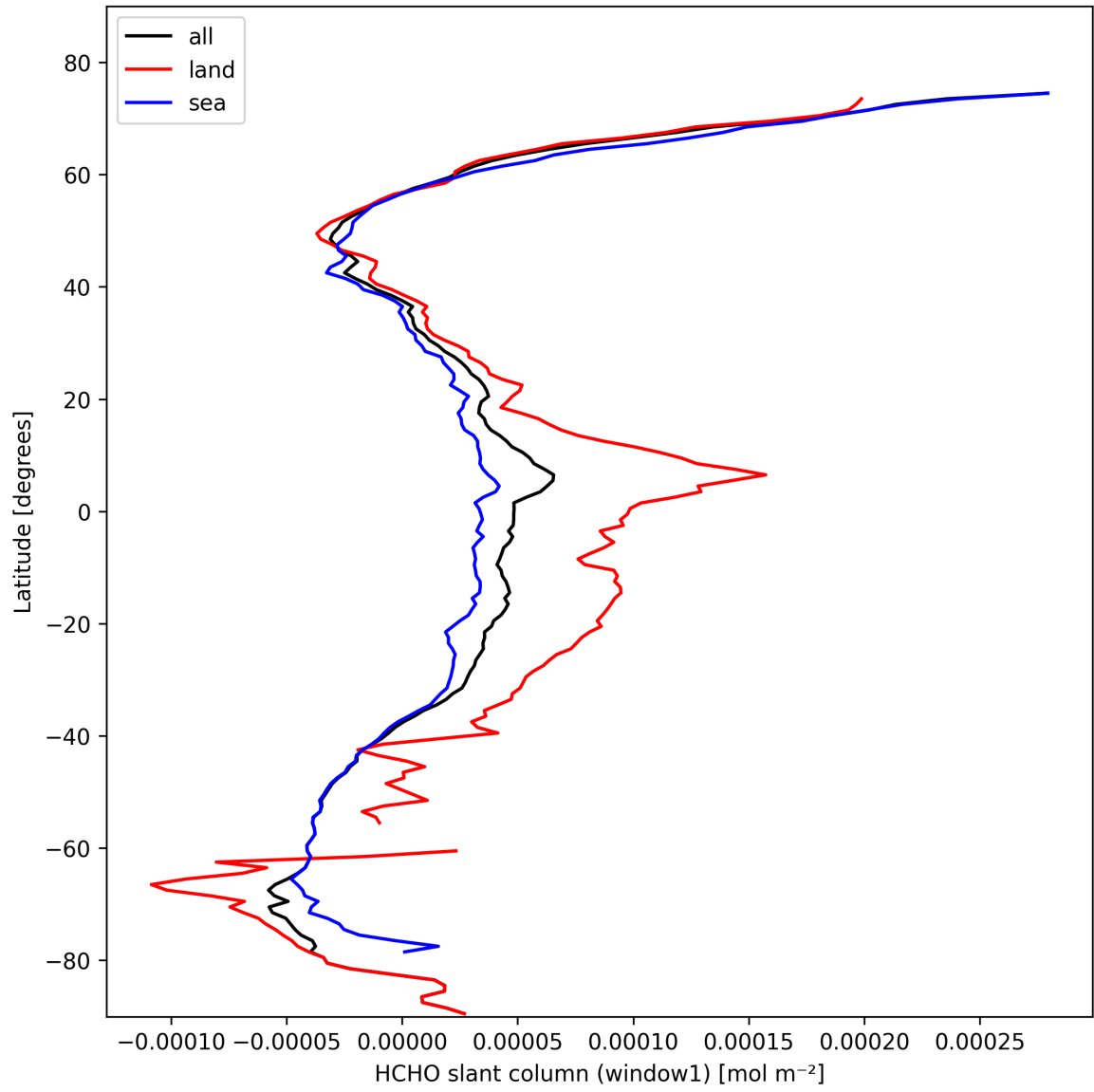
Figure 22: Zonal average of “HCHO slant column (window1)” for 2025-02-19 to 2025-02-20.
