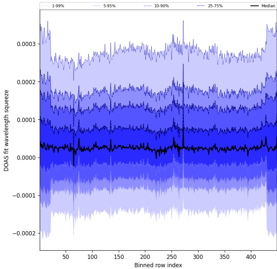
Figure 57: Along track statistics of “DOAS fit wavelength squeeze” for 2025-02-19 to 2025-02-20
