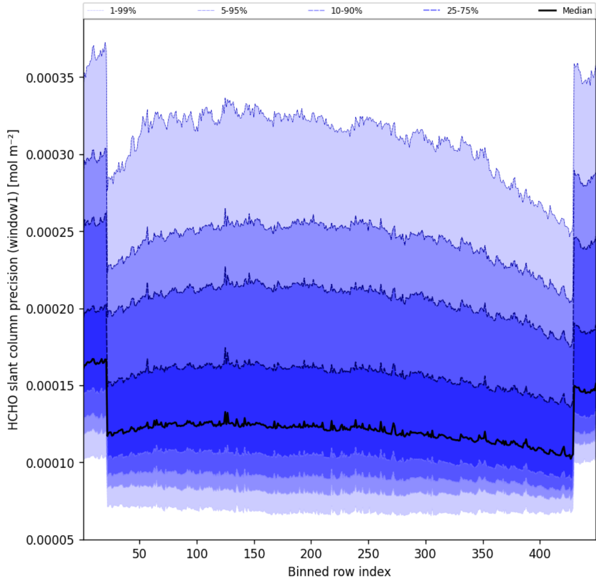
Figure 51: Along track statistics of “HCHO slant column precision (window1)” for 2025-02-19 to 2025-02-20
