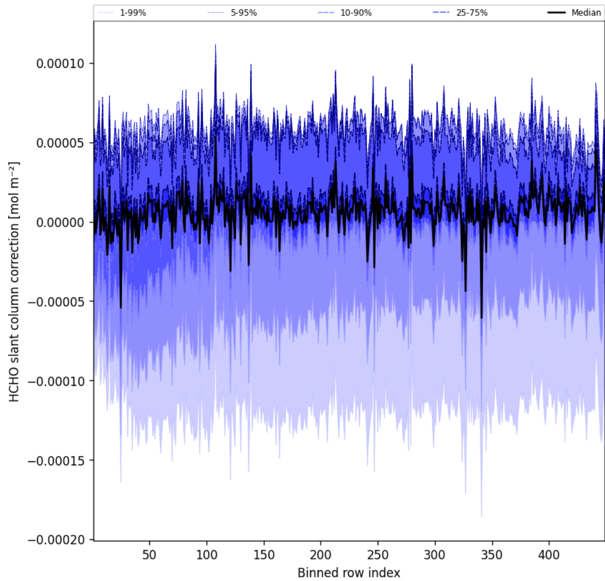
Figure 59: Along track statistics of “HCHO slant column correction” for 2025-02-19 to 2025-02-20
