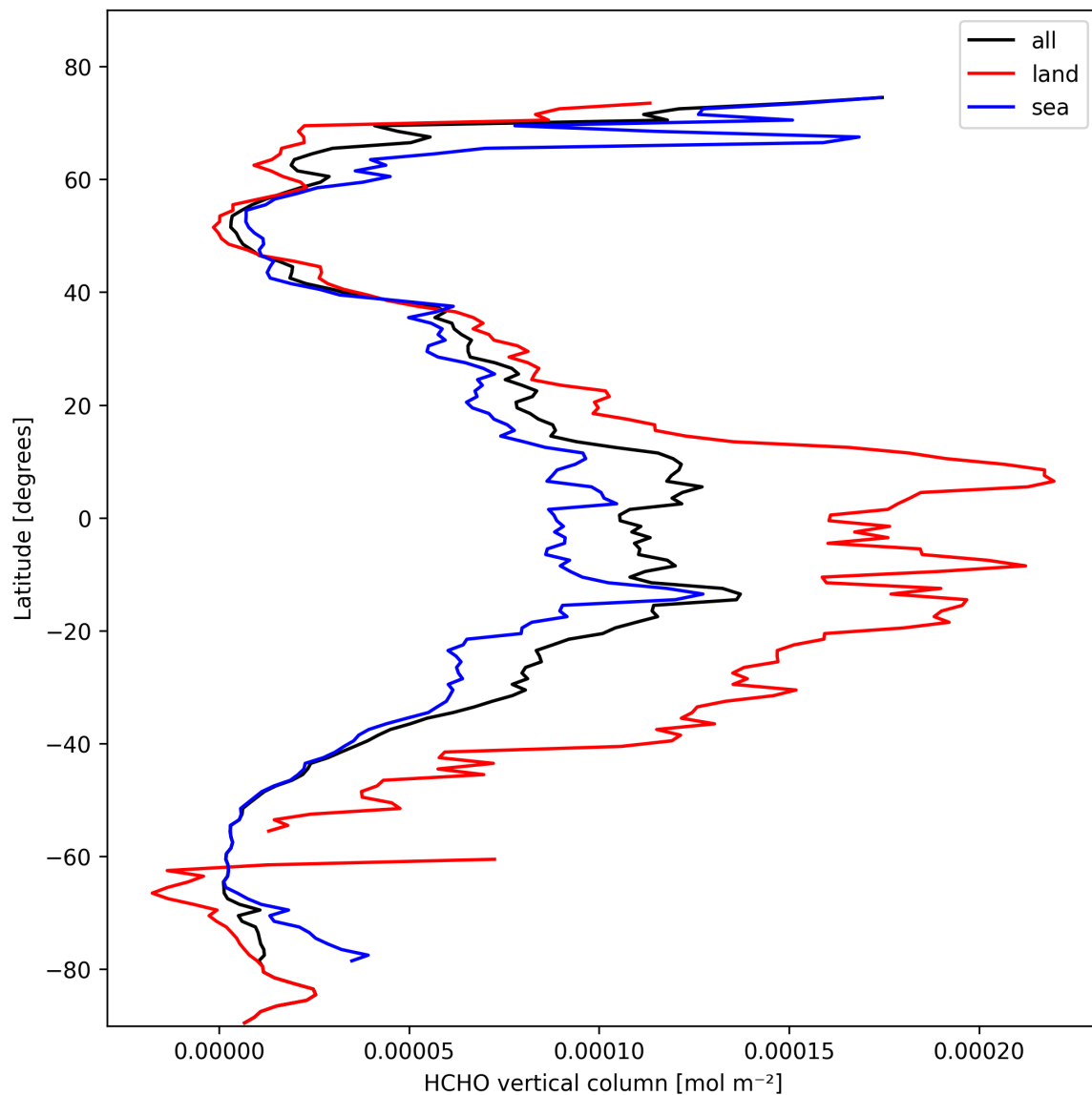
Figure 19: Zonal average of “HCHO vertical column” for 2025-02-19 to 2025-02-20.
