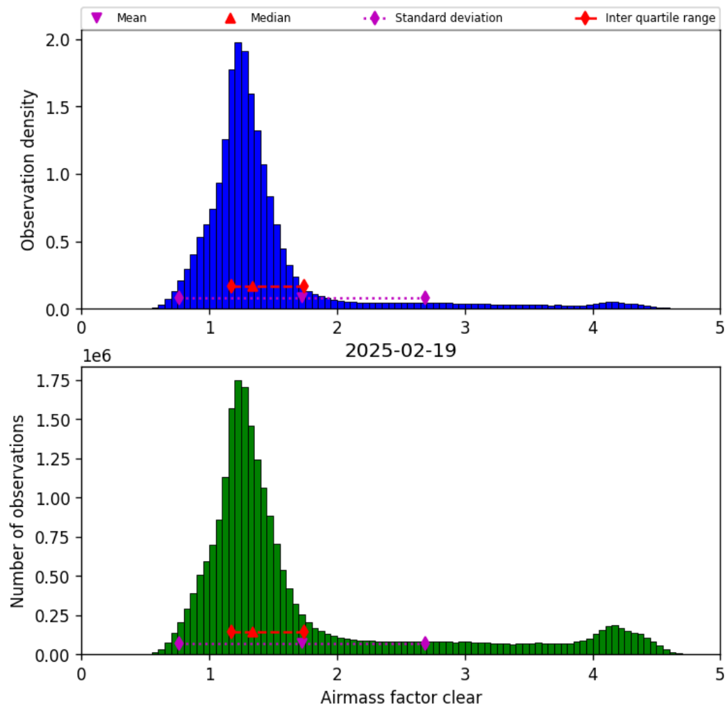
Figure 40: Histogram of “Airmass factor clear” for 2025-02-19 to 2025-02-20
