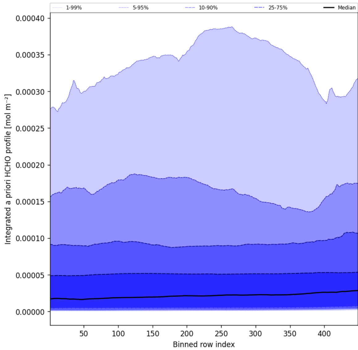
Figure 55: Along track statistics of "Integrated a priori HCHO profile" for 2025-02-19 to 2025-02-20
