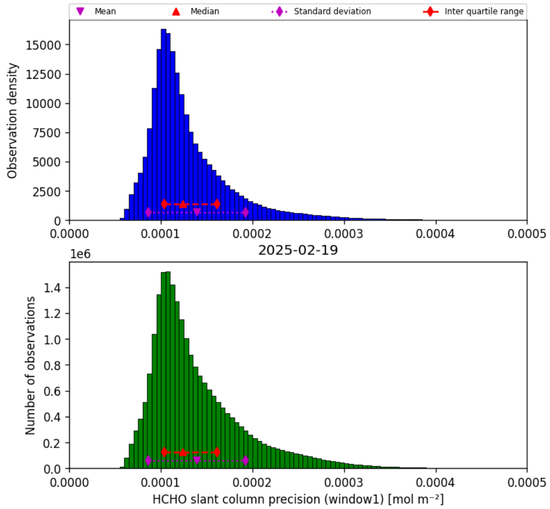
Figure 37: Histogram of “HCHO slant column precision (window1)” for 2025-02-19 to 2025-02-20
