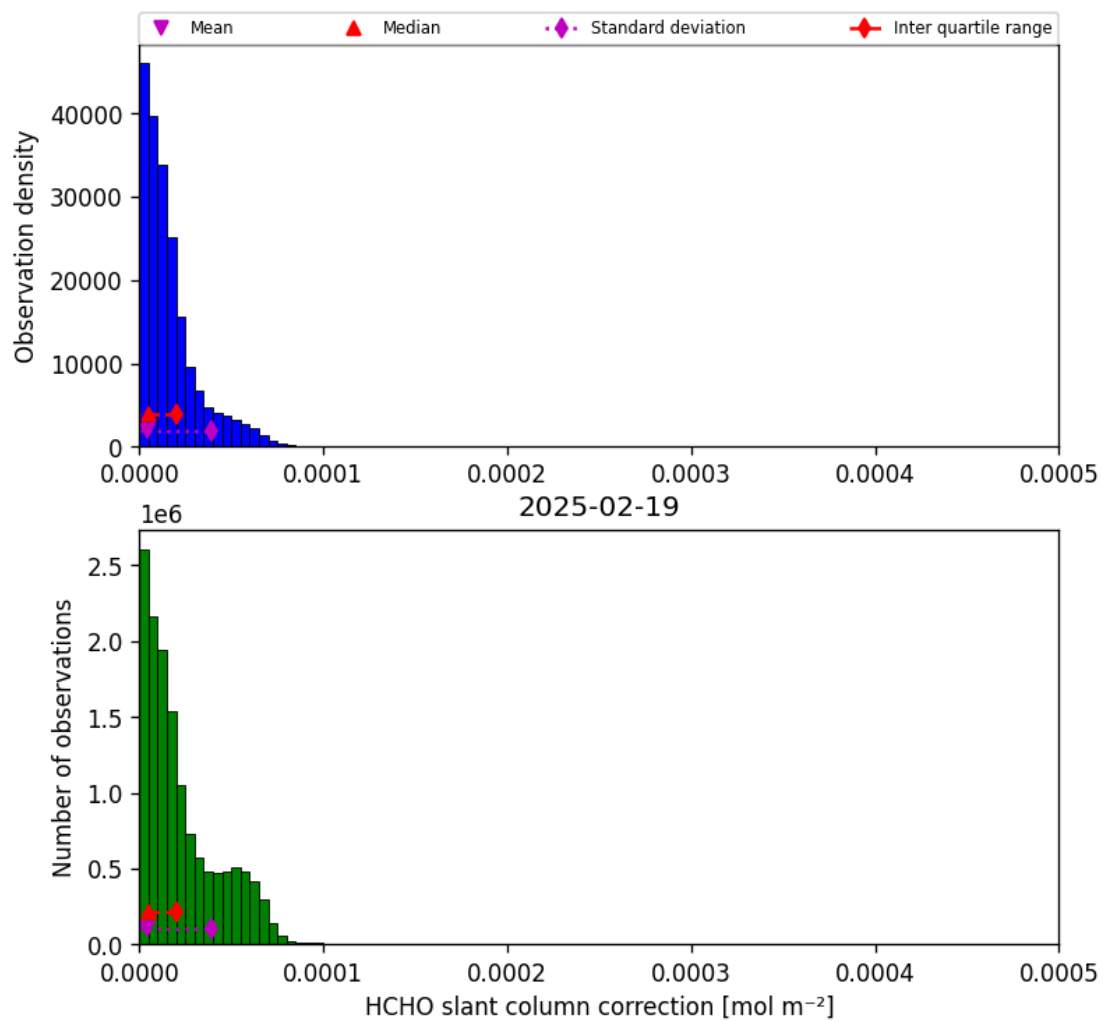
Figure 45: Histogram of “HCHO slant column correction” for 2025-02-19 to 2025-02-20
