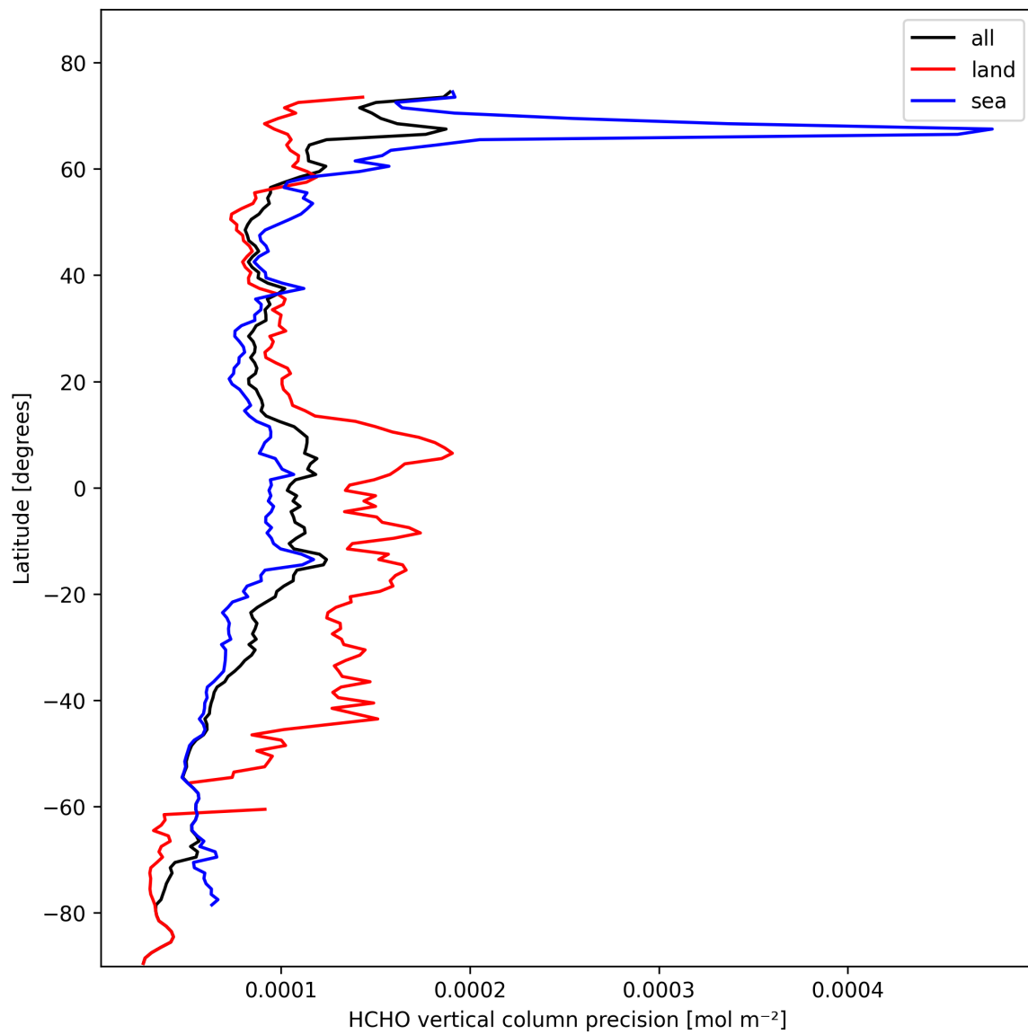
Figure 20: Zonal average of “HCHO vertical column precision” for 2025-02-19 to 2025-02-20.
