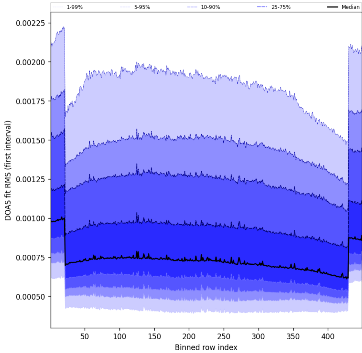
Figure 58: Along track statistics of “DOAS fit RMS (first interval)” for 2025-02-19 to 2025-02-20
