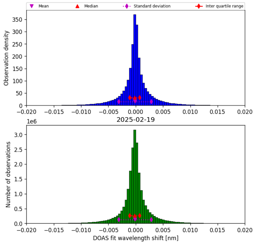
Figure 42: Histogram of “DOAS fit wavelength shift” for 2025-02-19 to 2025-02-20
