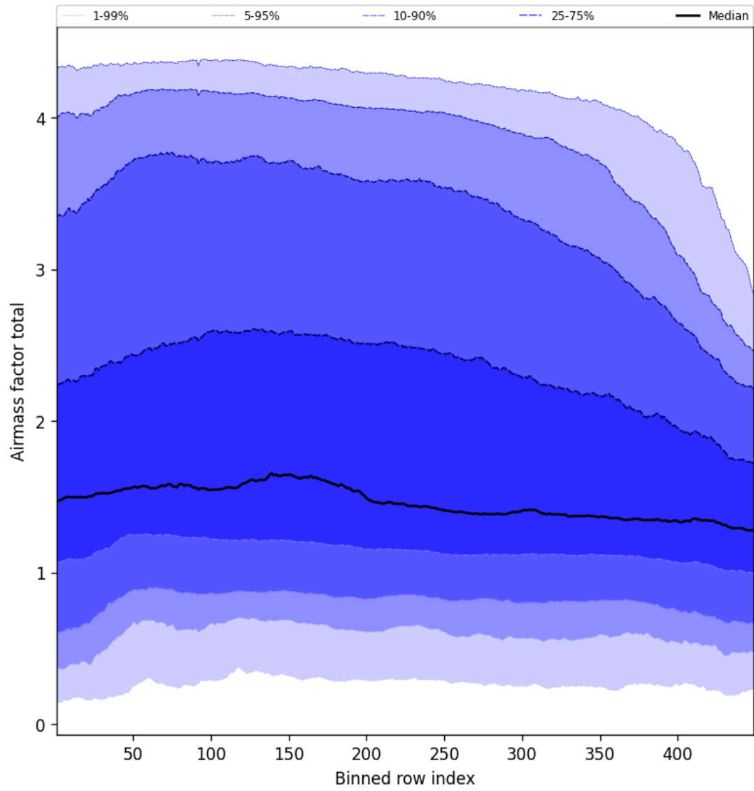
Figure 52: Along track statistics of “Airmass factor total” for 2025-02-19 to 2025-02-20
