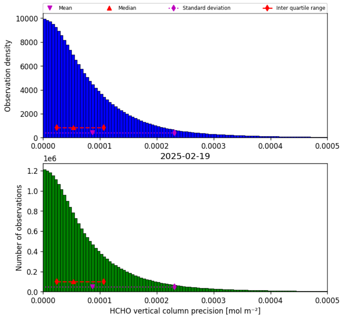
Figure 34: Histogram of “HCHO vertical column precision” for 2025-02-19 to 2025-02-20
