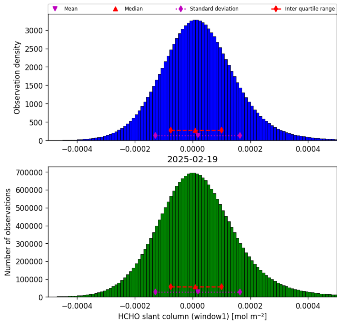
Figure 36: Histogram of “HCHO slant column (window1)” for 2025-02-19 to 2025-02-20
