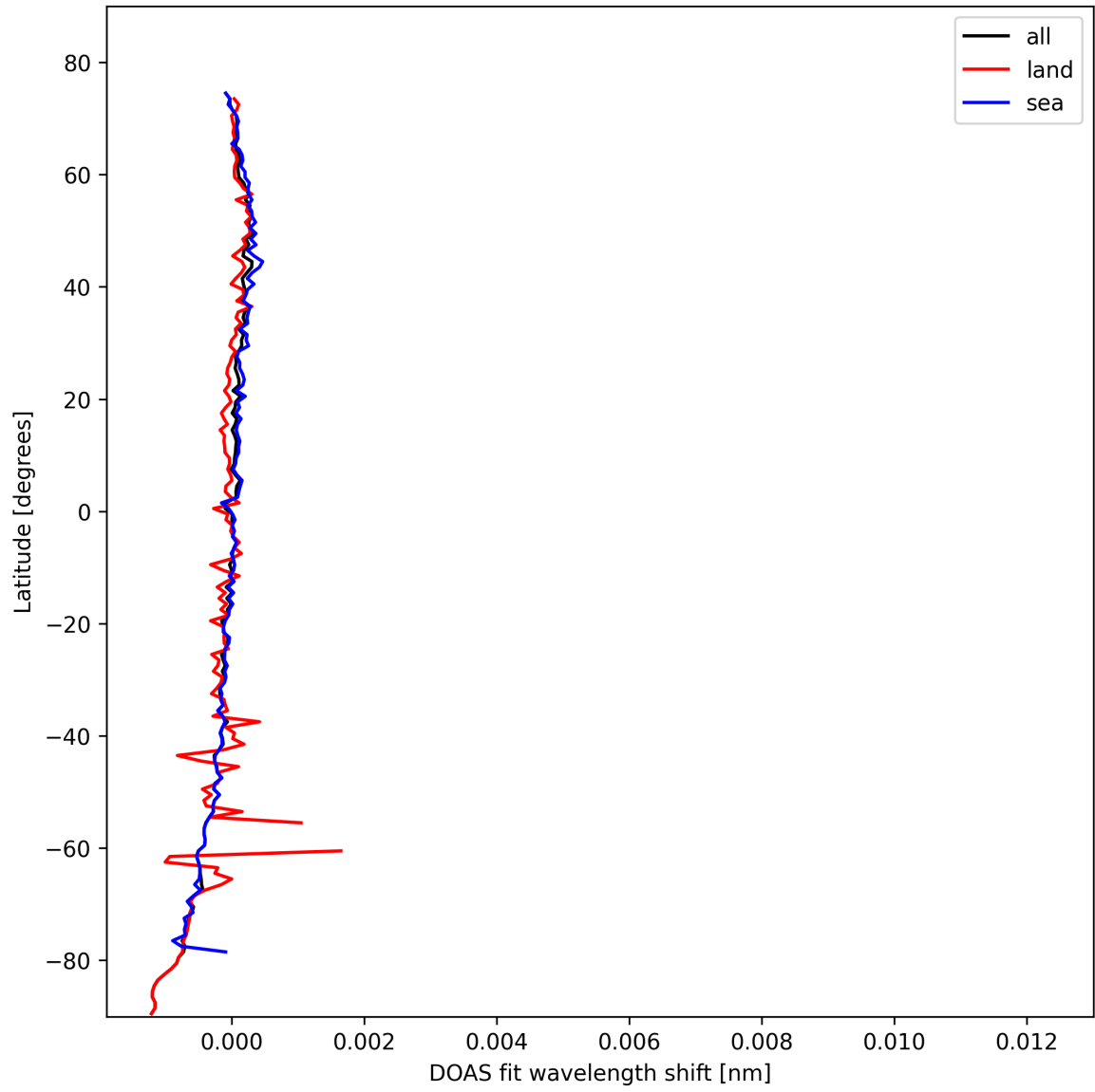
Figure 28: Zonal average of "DOAS fit wavelength shift" for 2025-02-19 to 2025-02-20.
