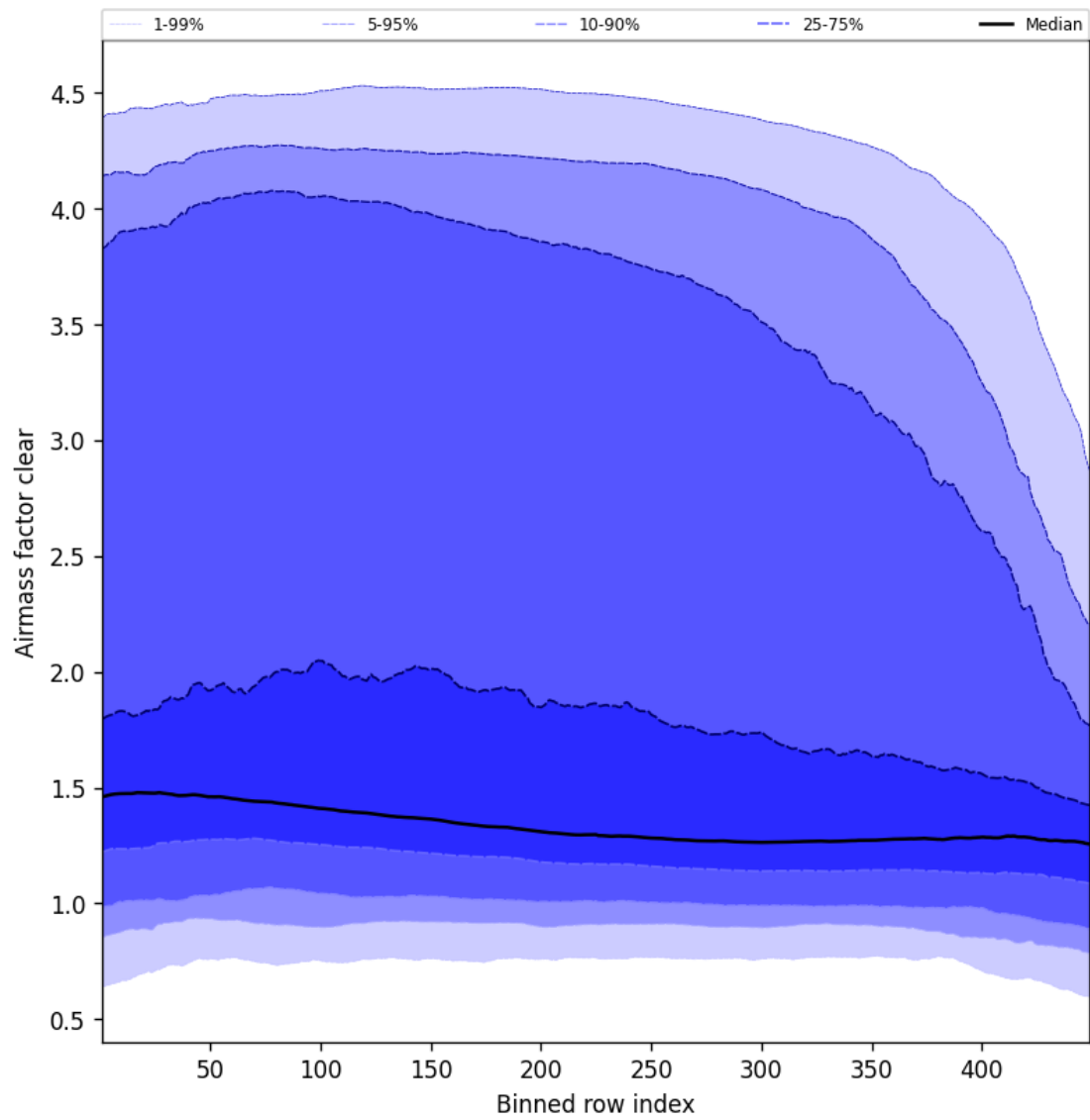
Figure 54: Along track statistics of “Airmass factor clear” for 2025-02-19 to 2025-02-20
