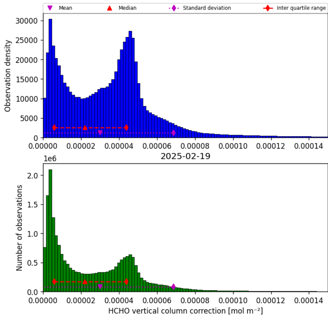
Figure 35: Histogram of “HCHO vertical column correction” for 2025-02-19 to 2025-02-20
