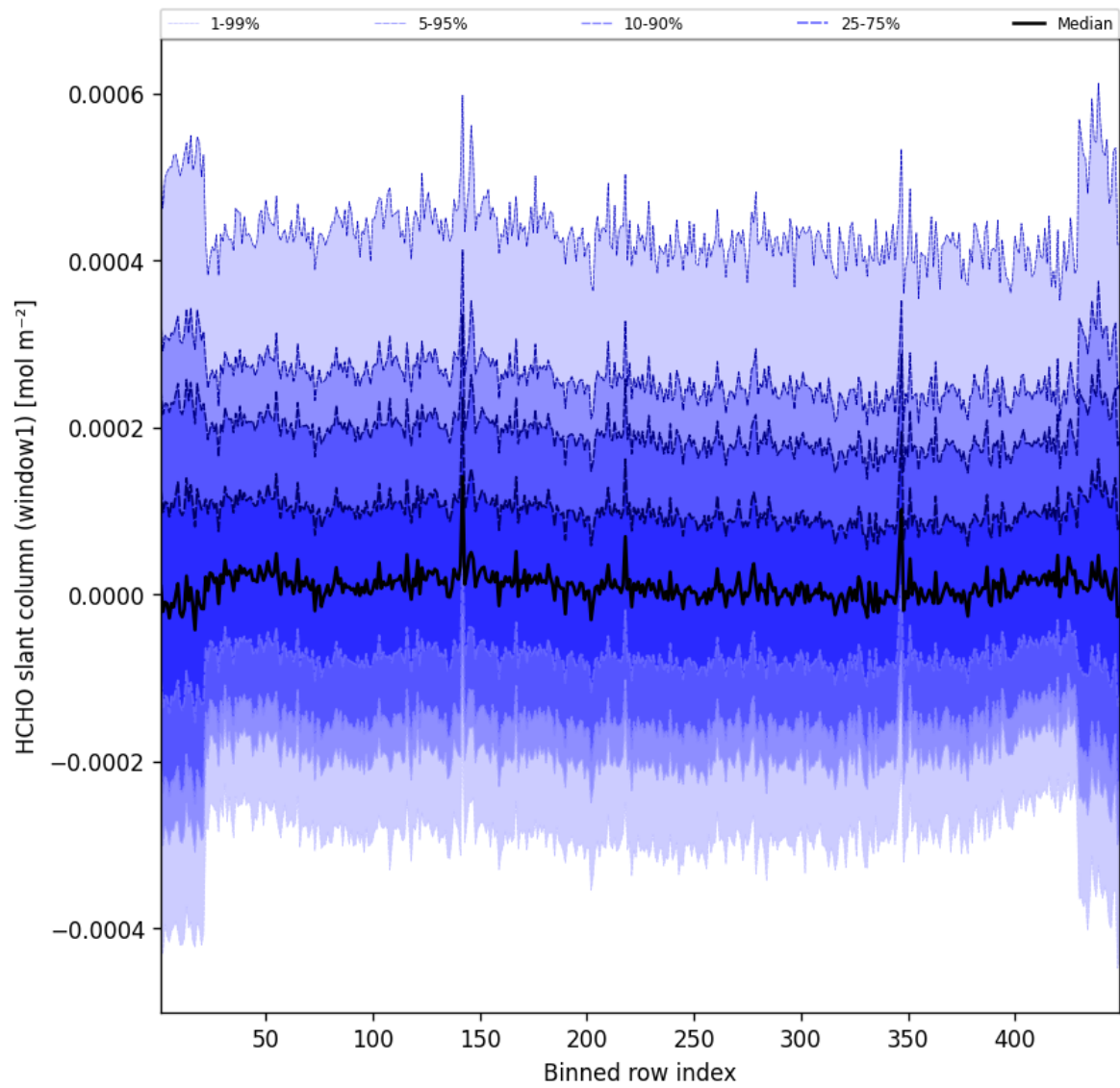
Figure 50: Along track statistics of “HCHO slant column (window1)” for 2025-02-19 to 2025-02-20
