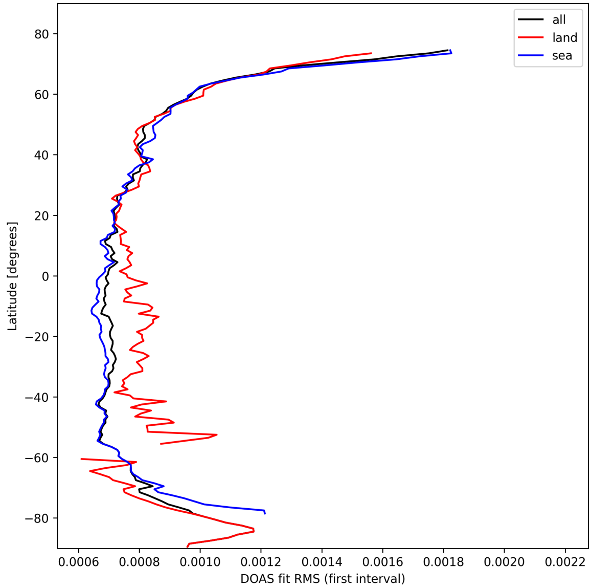
Figure 30: Zonal average of “DOAS fit RMS (first interval)” for 2025-02-19 to 2025-02-20.
