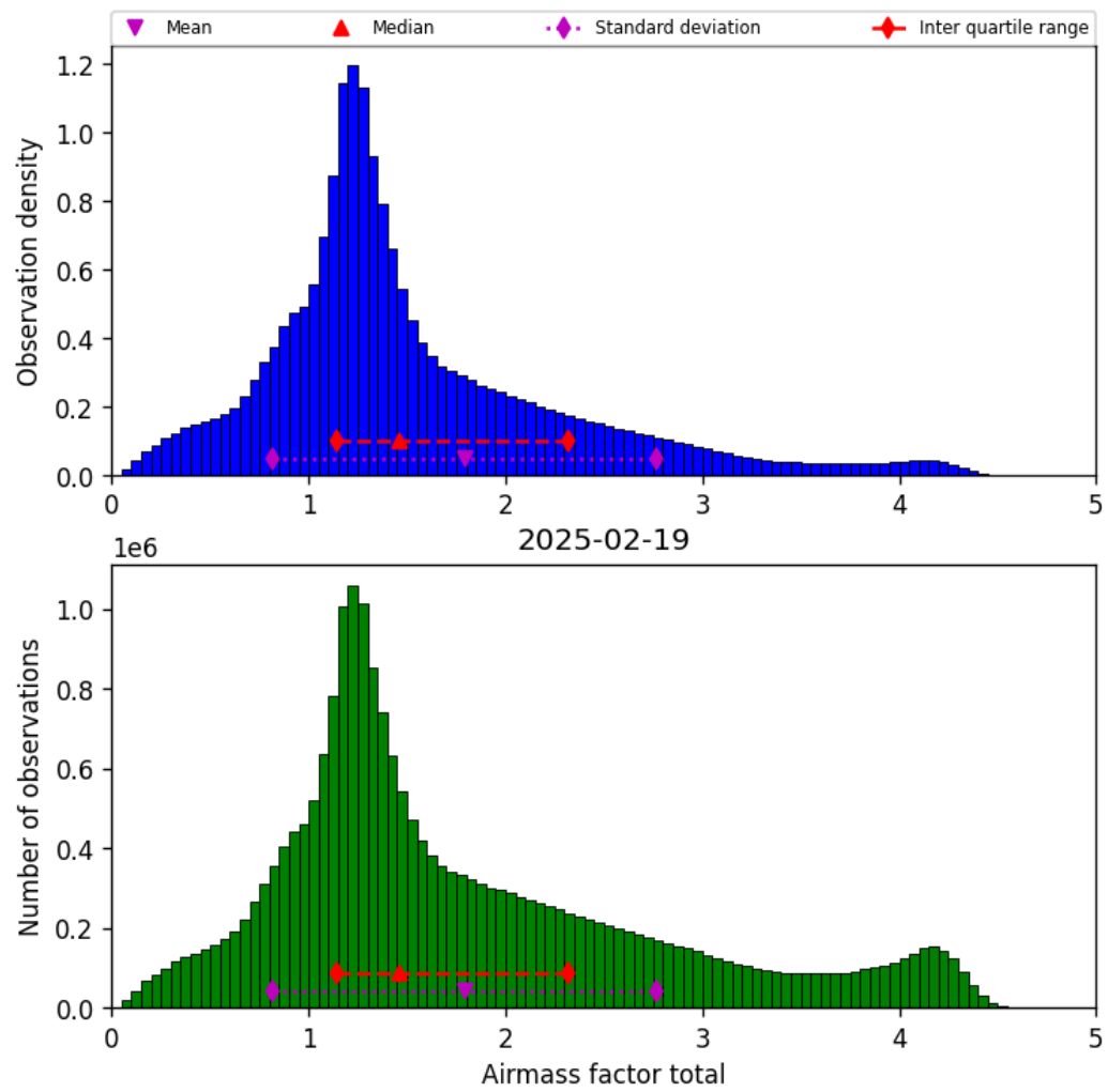
Figure 38: Histogram of “Airmass factor total” for 2025-02-19 to 2025-02-20
