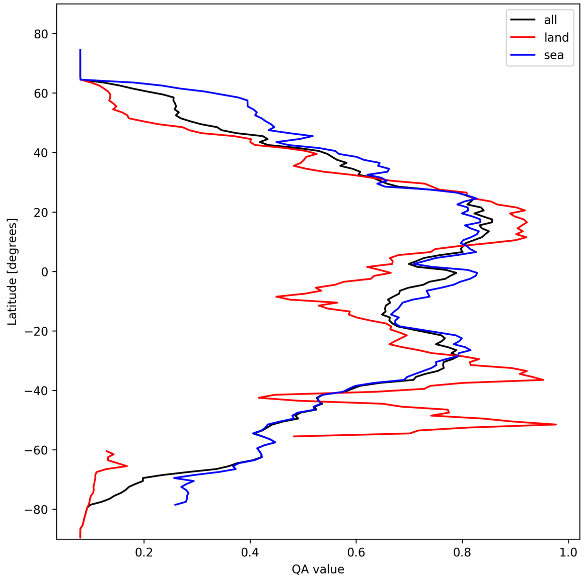
Figure 18: Zonal average of “QA value” for 2025-02-19 to 2025-02-20.
