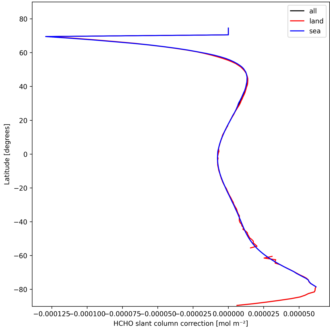
Figure 31: Zonal average of “HCHO slant column correction” for 2025-02-19 to 2025-02-20.
