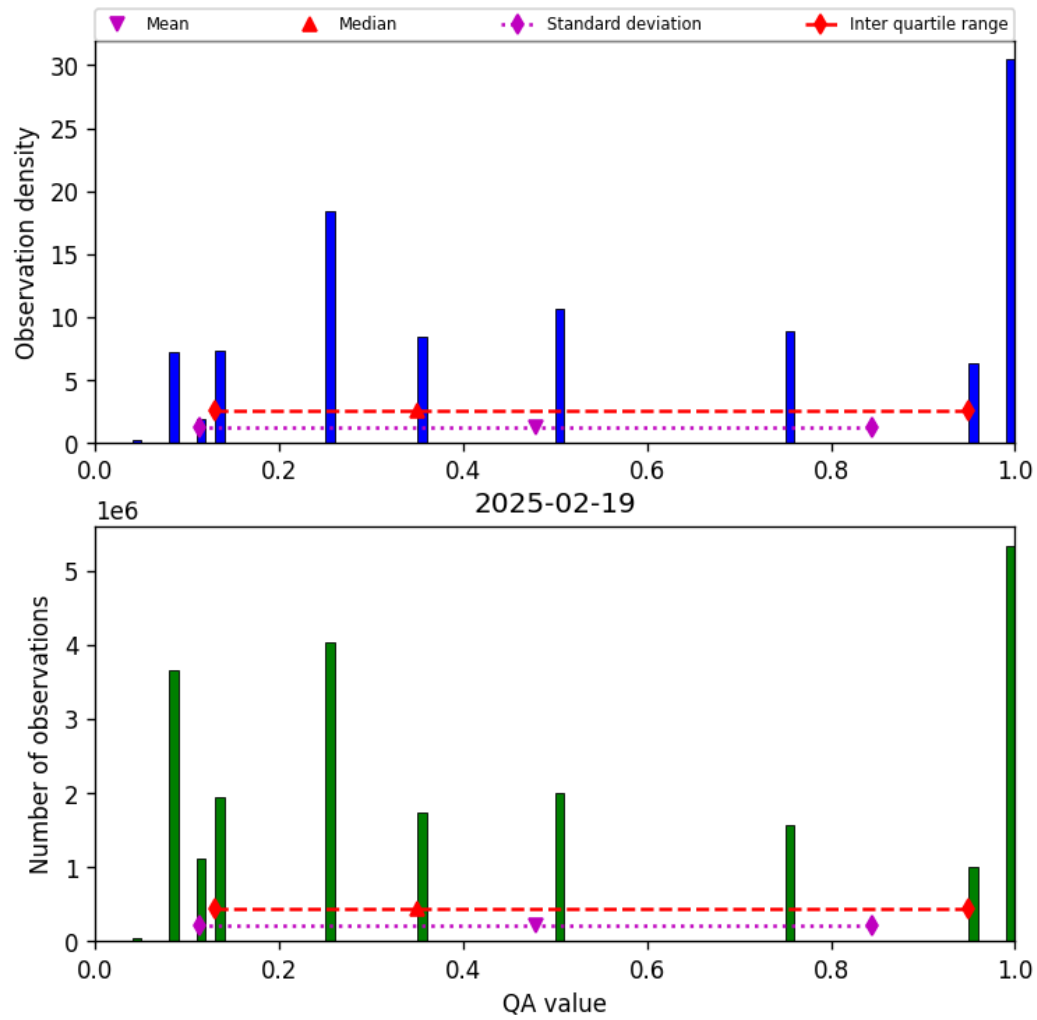
Figure 32: Histogram of “QA value” for 2025-02-19 to 2025-02-20
