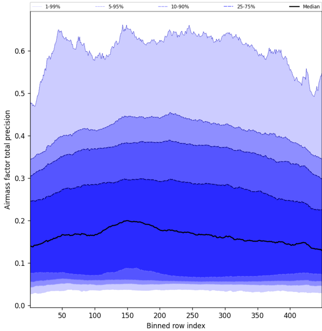
Figure 53: Along track statistics of “Airmass factor total precision” for 2025-02-19 to 2025-02-20
