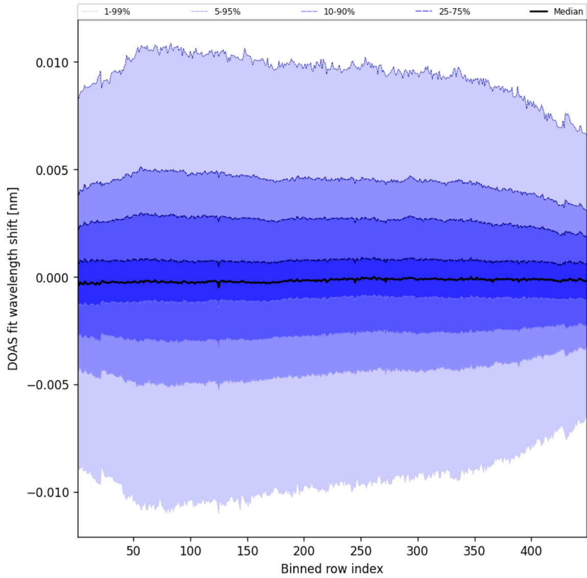
Figure 56: Along track statistics of “DOAS fit wavelength shift” for 2025-02-19 to 2025-02-20
