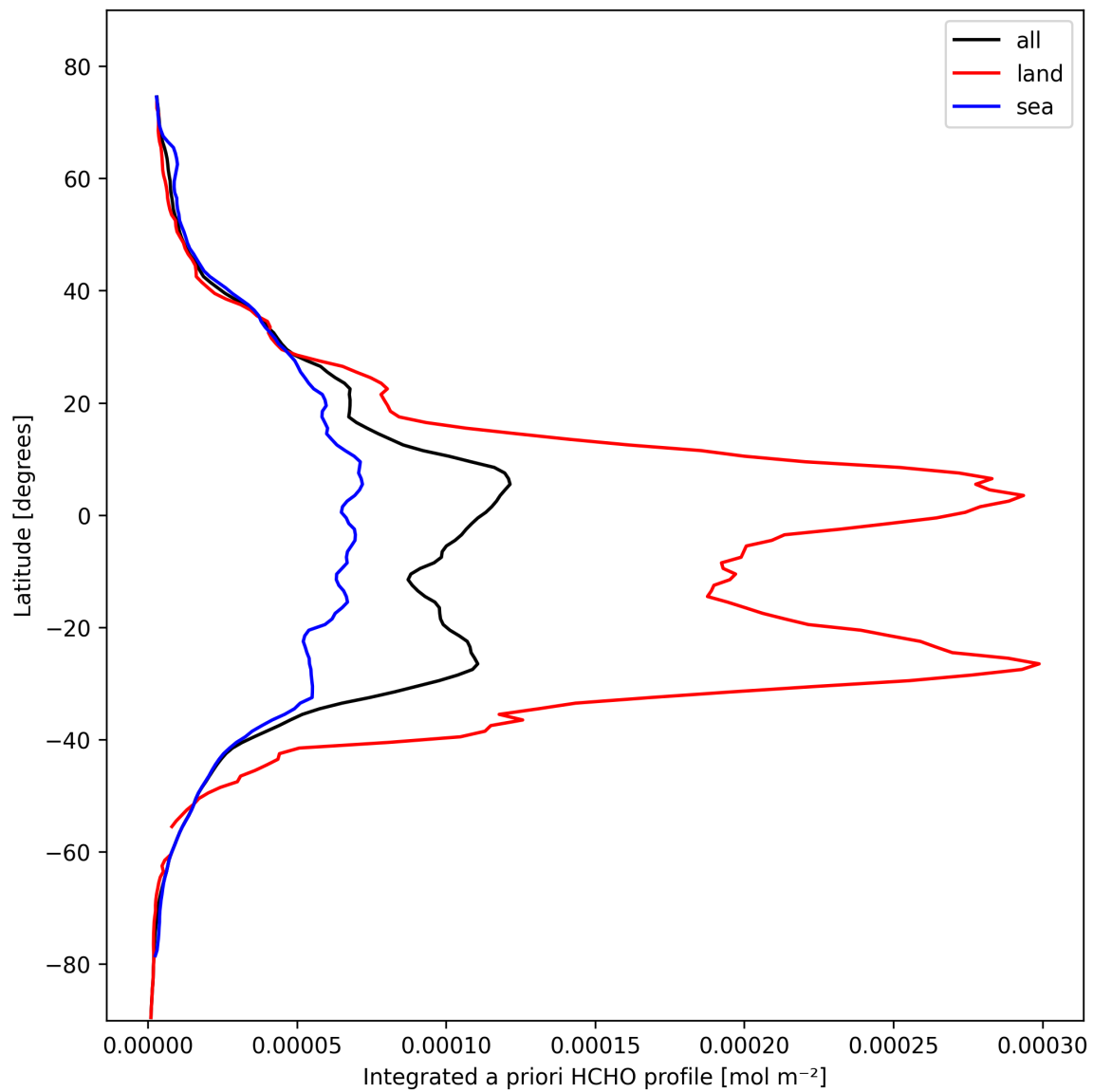
Figure 27: Zonal average of “Integrated a priori HCHO profile” for 2025-02-19 to 2025-02-20.
