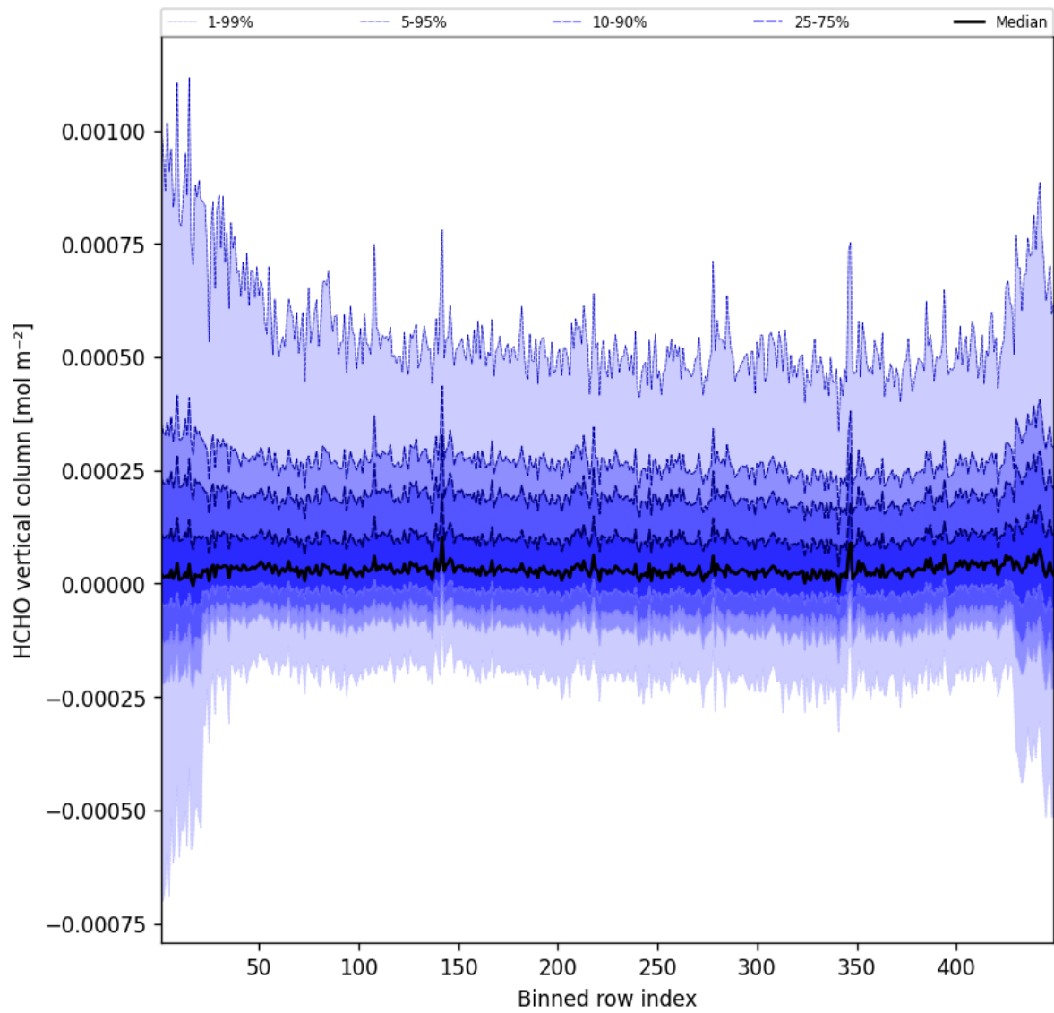
Figure 47: Along track statistics of “HCHO vertical column” for 2025-02-19 to 2025-02-20
