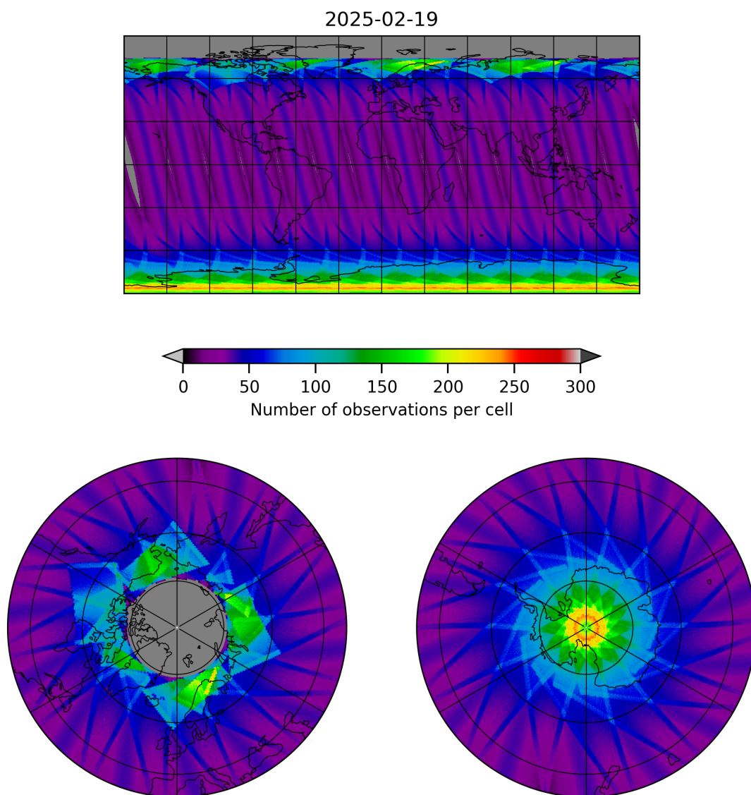
Figure 17: Map of the number of observations for 2025-02-19 to 2025-02-20
