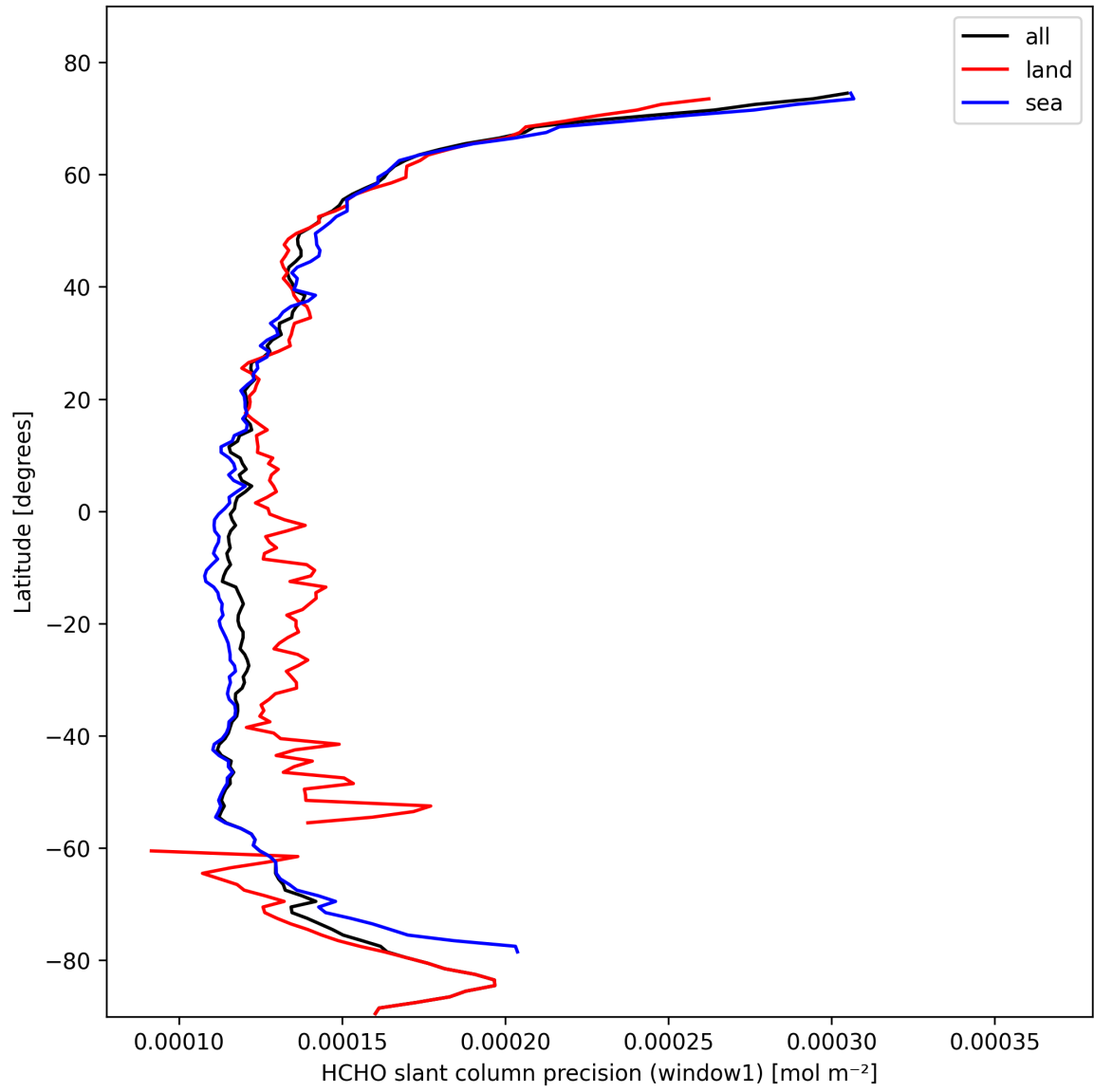
Figure 23: Zonal average of “HCHO slant column precision (window1)” for 2025-02-19 to 2025-02-20.
