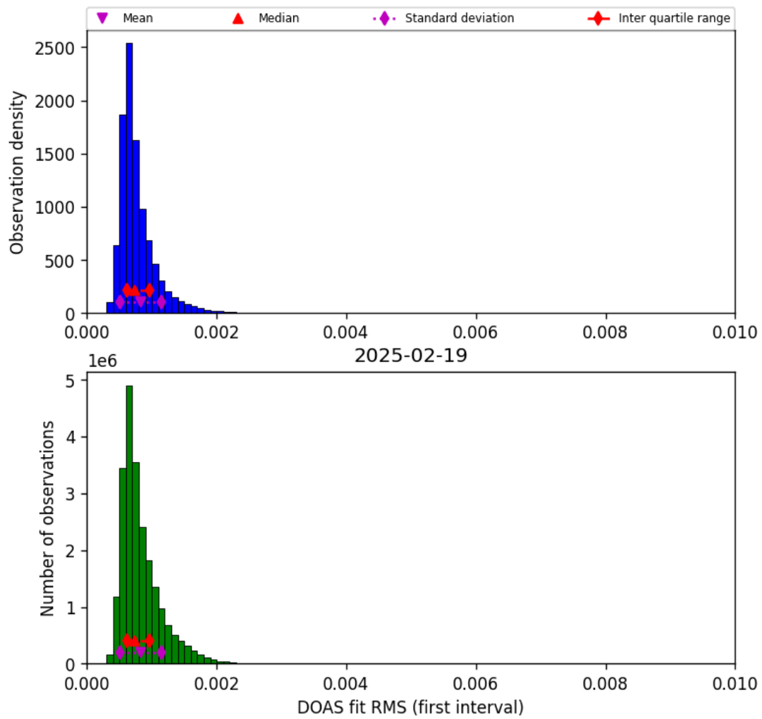
Figure 44: Histogram of "DOAS fit RMS (first interval)" for 2025-02-19 to 2025-02-20
