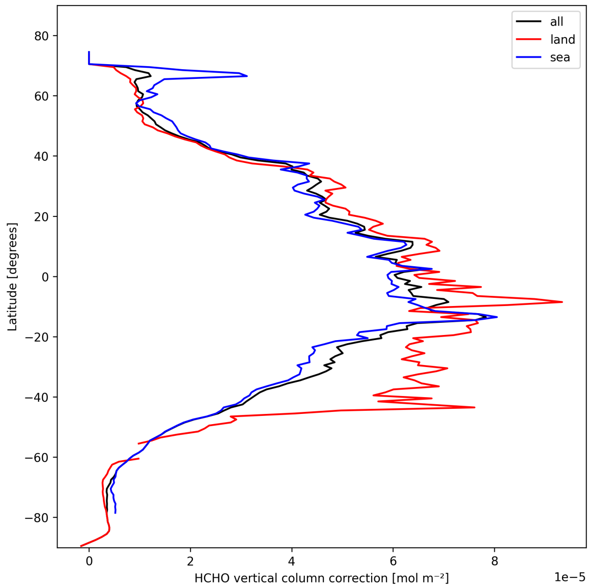
Figure 21: Zonal average of “HCHO vertical column correction” for 2025-02-19 to 2025-02-20.
