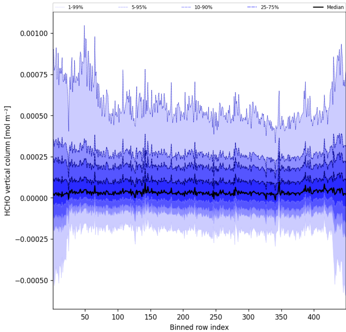
Figure 47: Along track statistics of “HCHO vertical column” for 2025-02-20 to 2025-02-21
