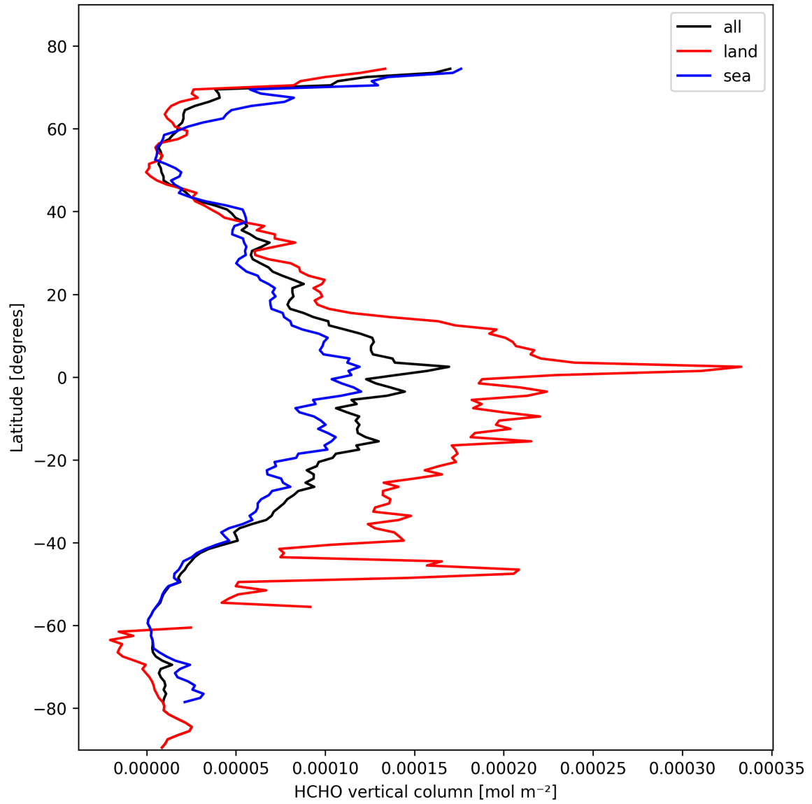
Figure 19: Zonal average of “HCHO vertical column” for 2025-02-20 to 2025-02-21.
