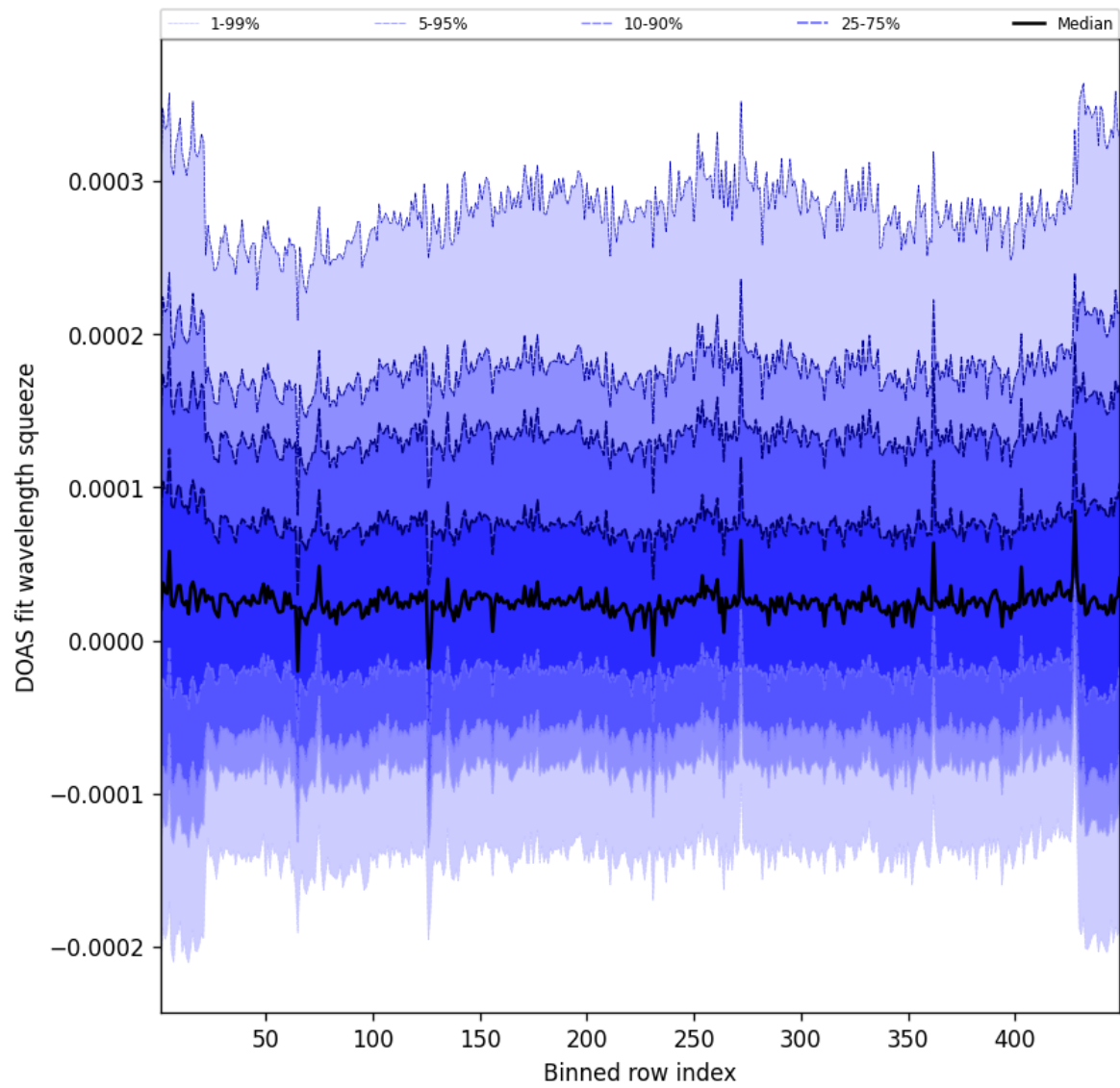
Figure 57: Along track statistics of “DOAS fit wavelength squeeze” for 2025-02-20 to 2025-02-21
