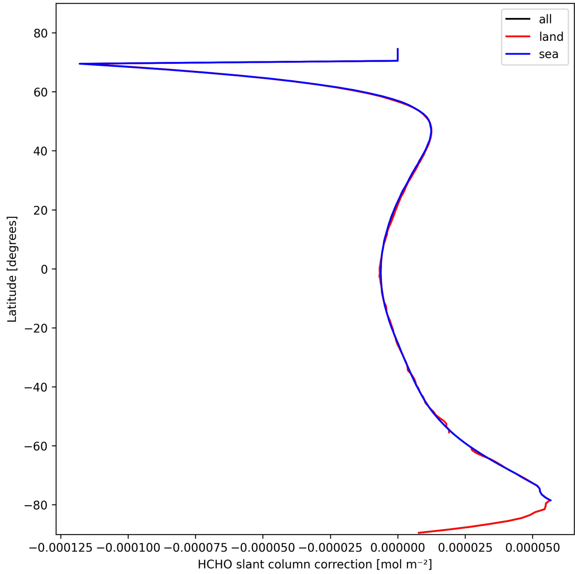
Figure 31: Zonal average of “HCHO slant column correction” for 2025-02-20 to 2025-02-21.
