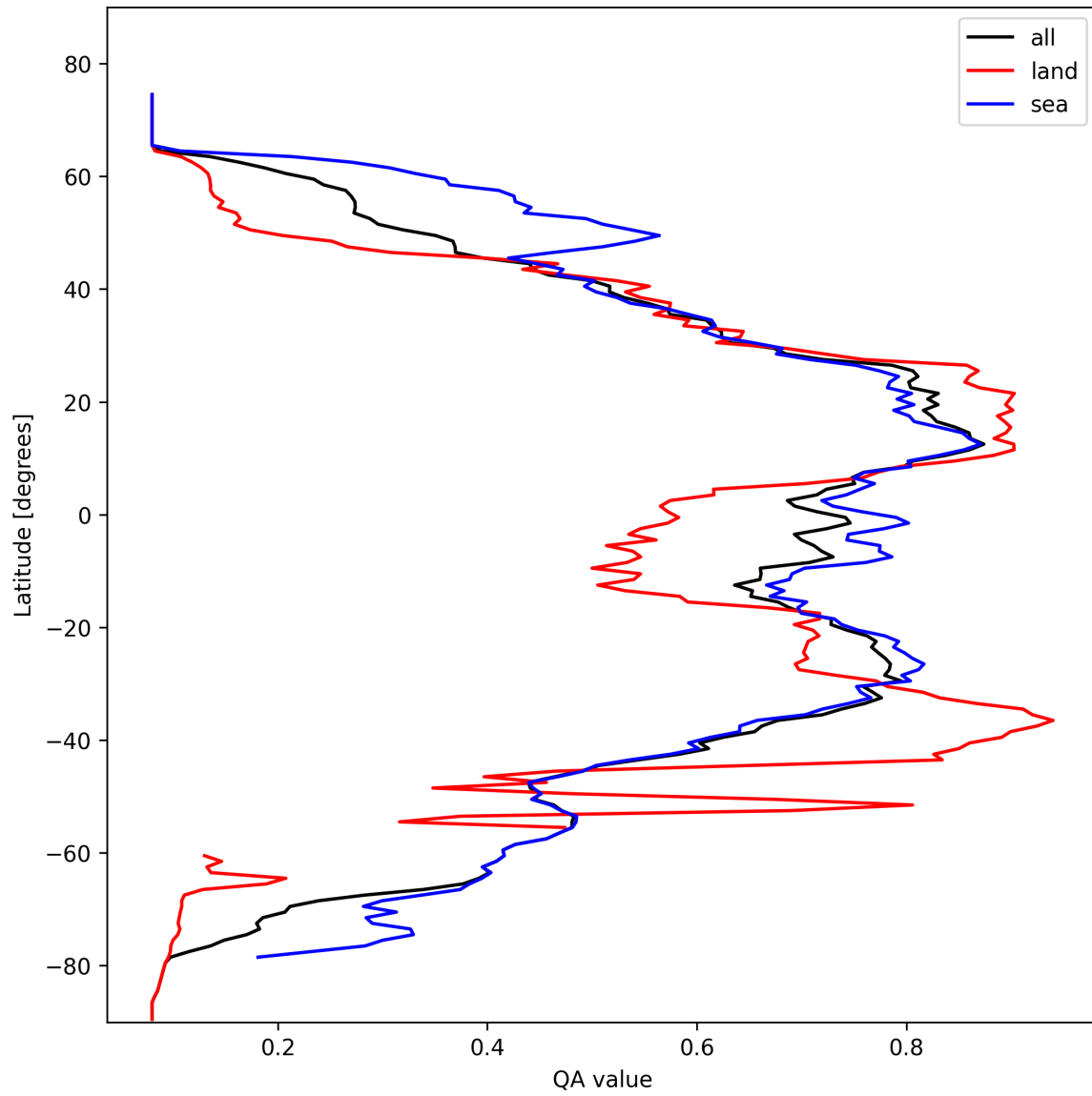
Figure 18: Zonal average of “QA value” for 2025-02-20 to 2025-02-21.
