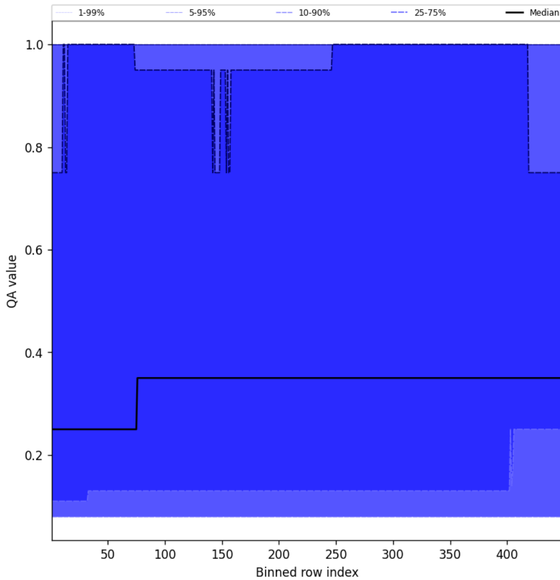
Figure 46: Along track statistics of “QA value” for 2025-02-20 to 2025-02-21
