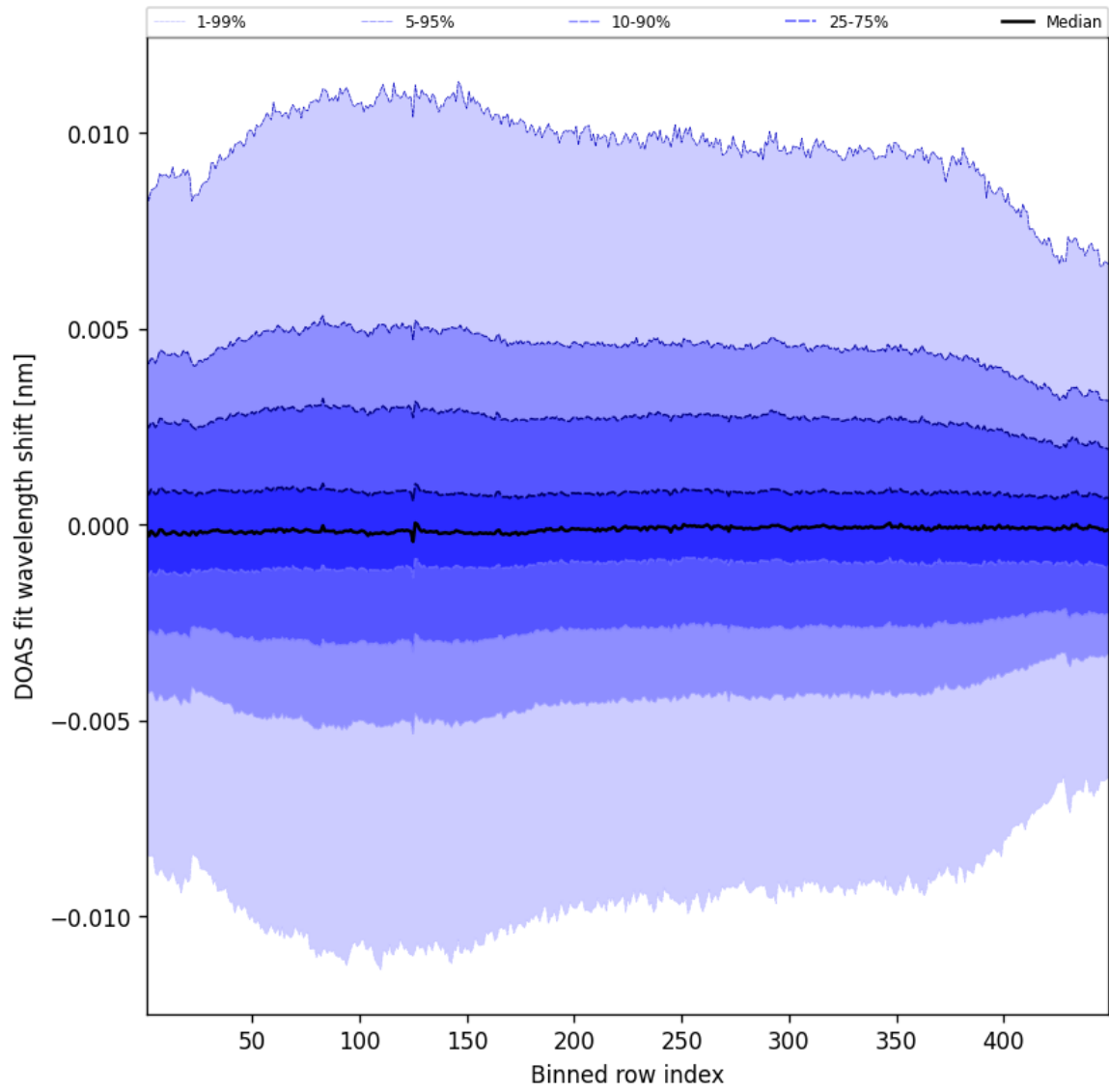
Figure 56: Along track statistics of “DOAS fit wavelength shift” for 2025-02-20 to 2025-02-21
