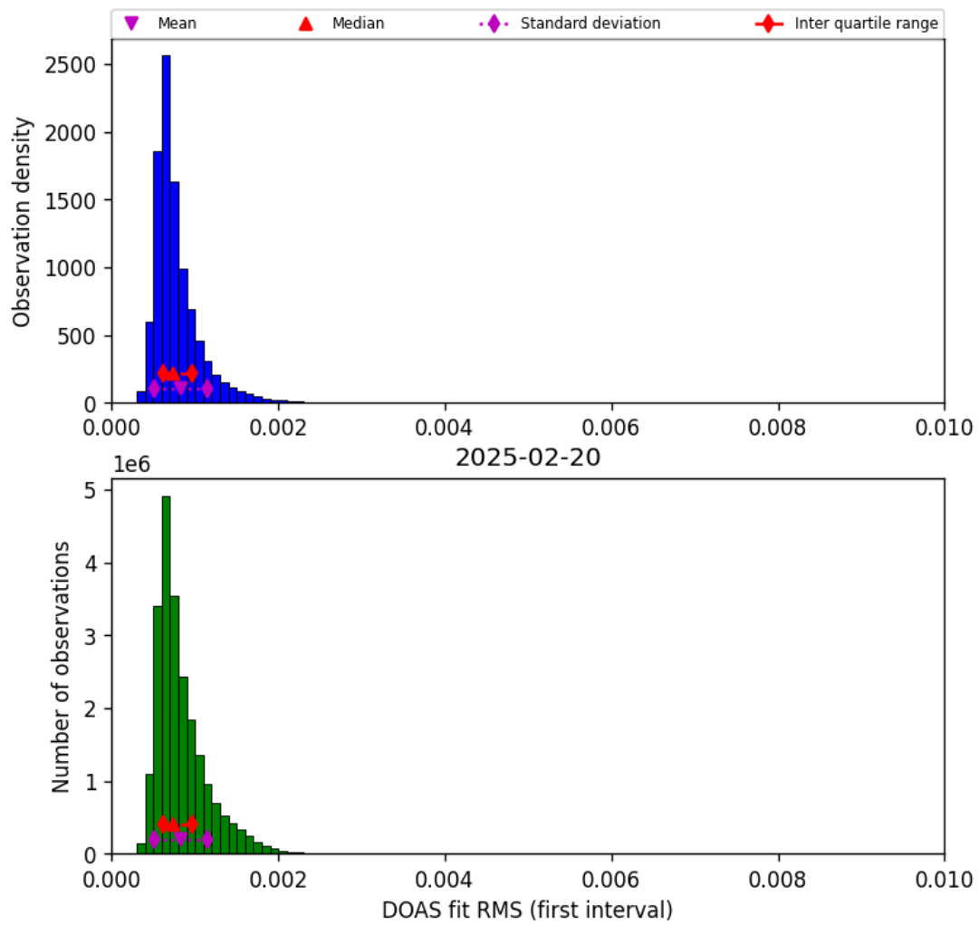
Figure 44: Histogram of “DOAS fit RMS (first interval)” for 2025-02-20 to 2025-02-21
