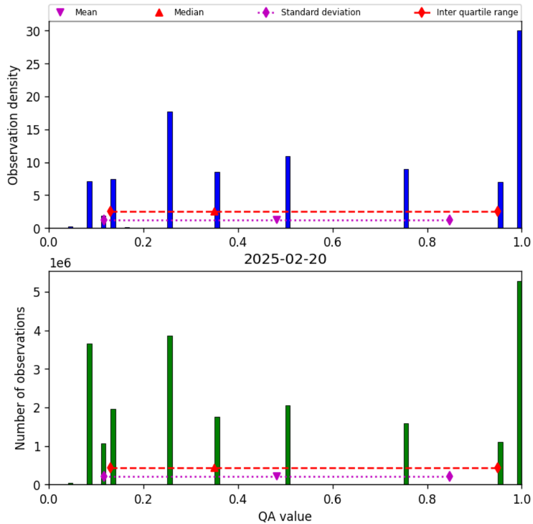
Figure 32: Histogram of “QA value” for 2025-02-20 to 2025-02-21
