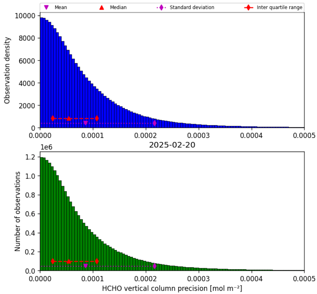
Figure 34: Histogram of “HCHO vertical column precision” for 2025-02-20 to 2025-02-21
