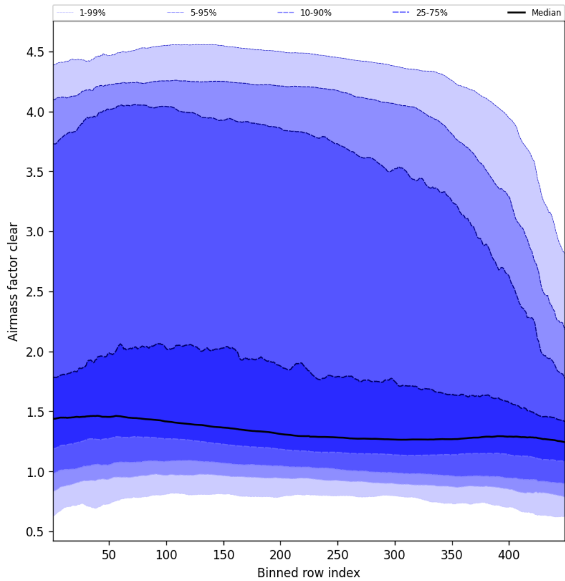
Figure 54: Along track statistics of “Airmass factor clear” for 2025-02-20 to 2025-02-21
