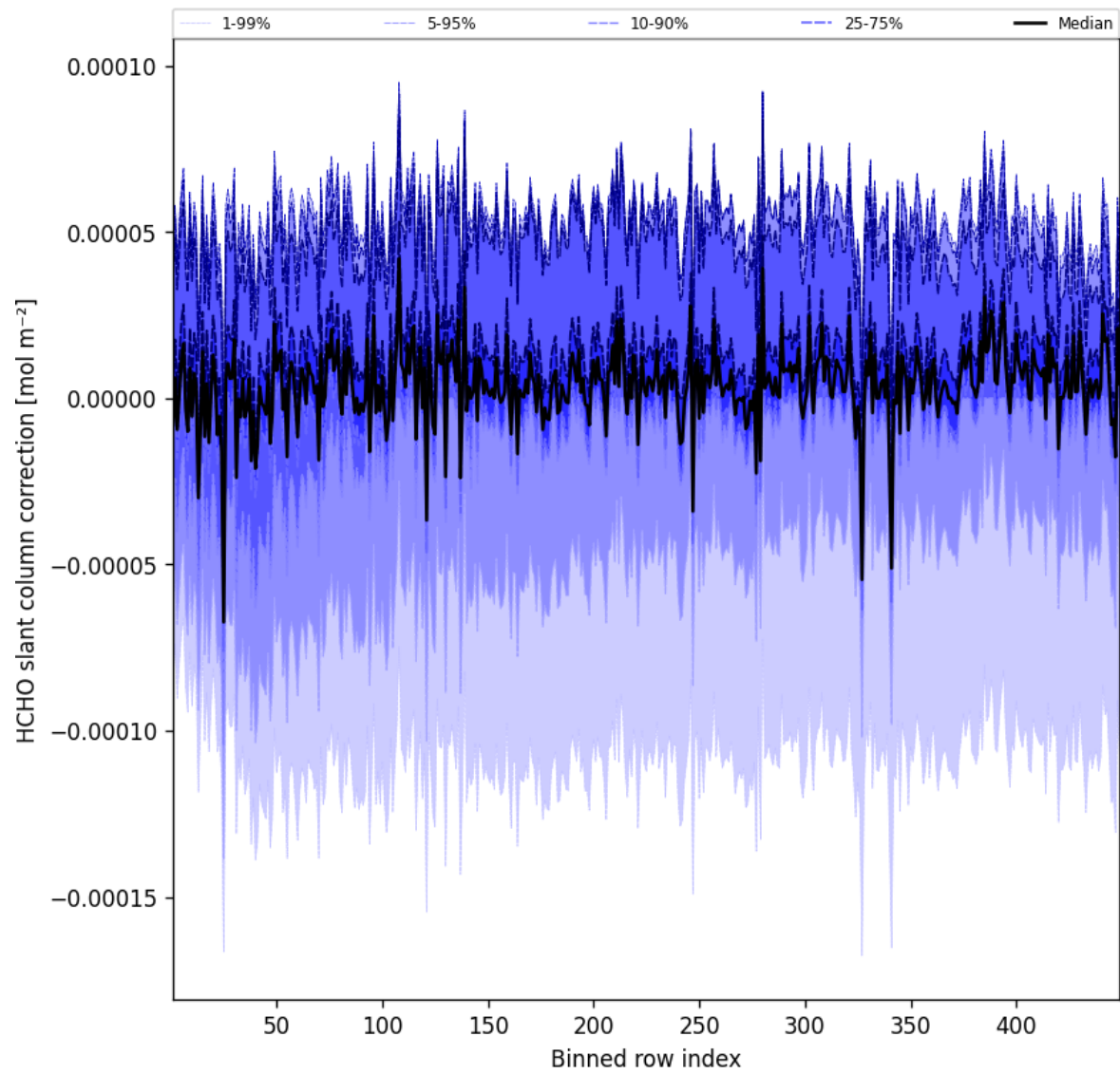
Figure 59: Along track statistics of “HCHO slant column correction” for 2025-02-20 to 2025-02-21
