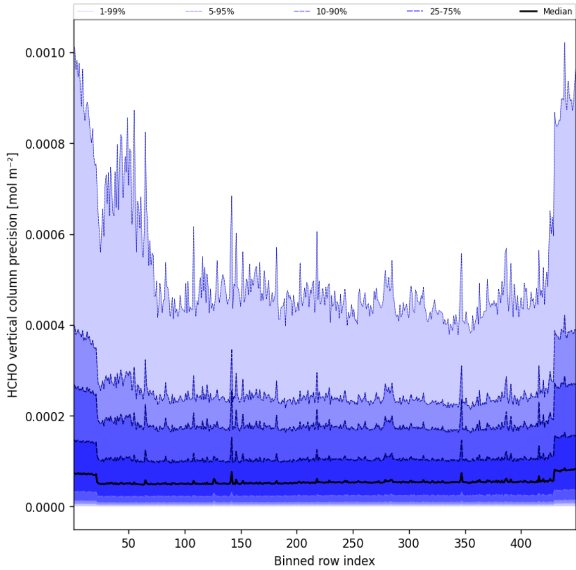
Figure 48: Along track statistics of “HCHO vertical column precision” for 2025-02-20 to 2025-02-21
