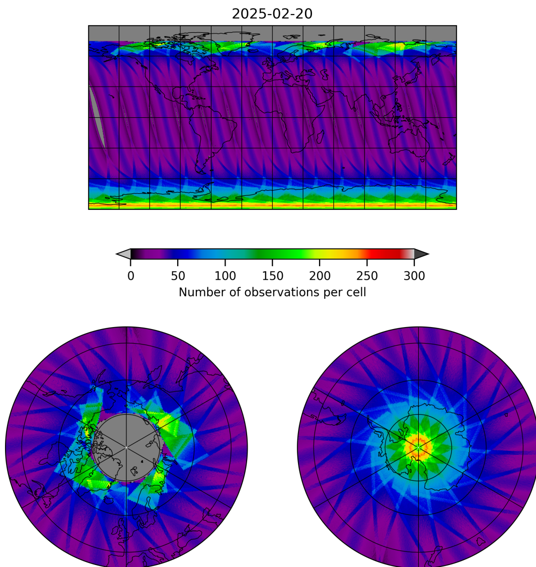
Figure 17: Map of the number of observations for 2025-02-20 to 2025-02-21
