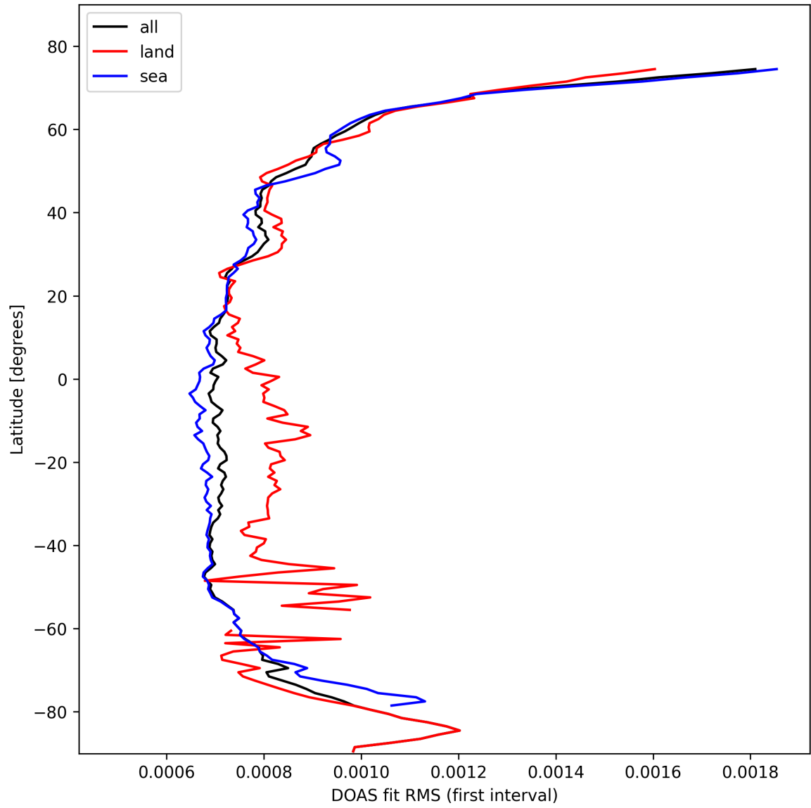
Figure 30: Zonal average of "DOAS fit RMS (first interval)" for 2025-02-20 to 2025-02-21.
