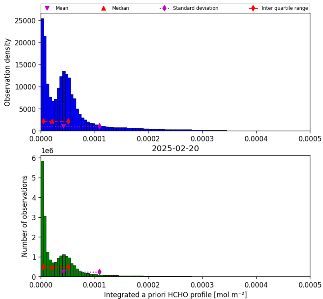
Figure 41: Histogram of “Integrated a priori HCHO profile” for 2025-02-20 to 2025-02-21
