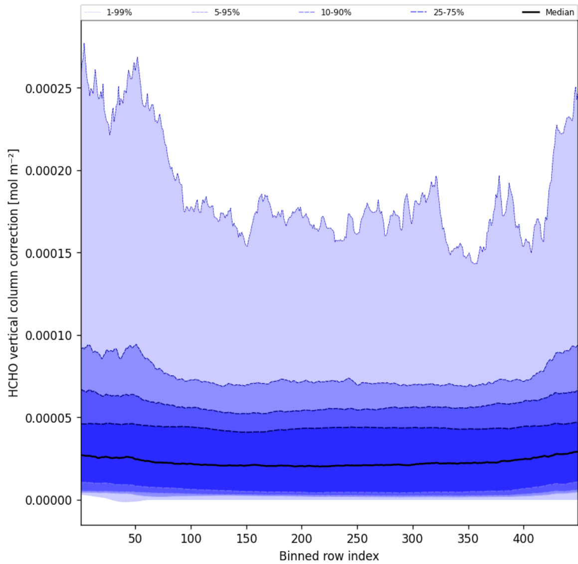
Figure 49: Along track statistics of “HCHO vertical column correction” for 2025-02-20 to 2025-02-21
