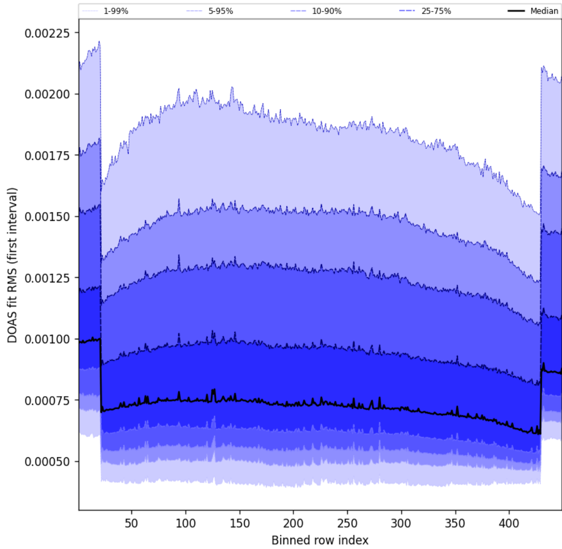
Figure 58: Along track statistics of “DOAS fit RMS (first interval)” for 2025-02-20 to 2025-02-21
