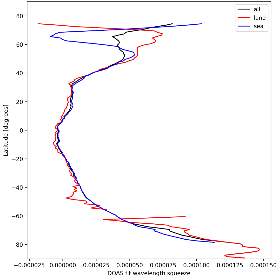
Figure 29: Zonal average of “DOAS fit wavelength squeeze” for 2025-02-20 to 2025-02-21.
