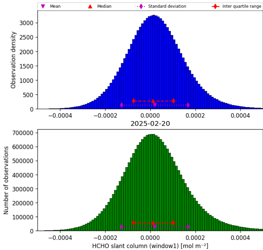
Figure 36: Histogram of “HCHO slant column (window1)” for 2025-02-20 to 2025-02-21
