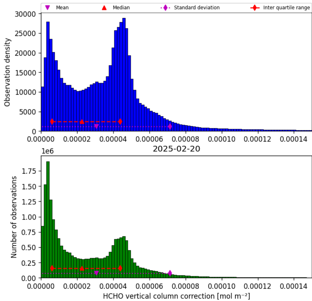
Figure 35: Histogram of “HCHO vertical column correction” for 2025-02-20 to 2025-02-21
