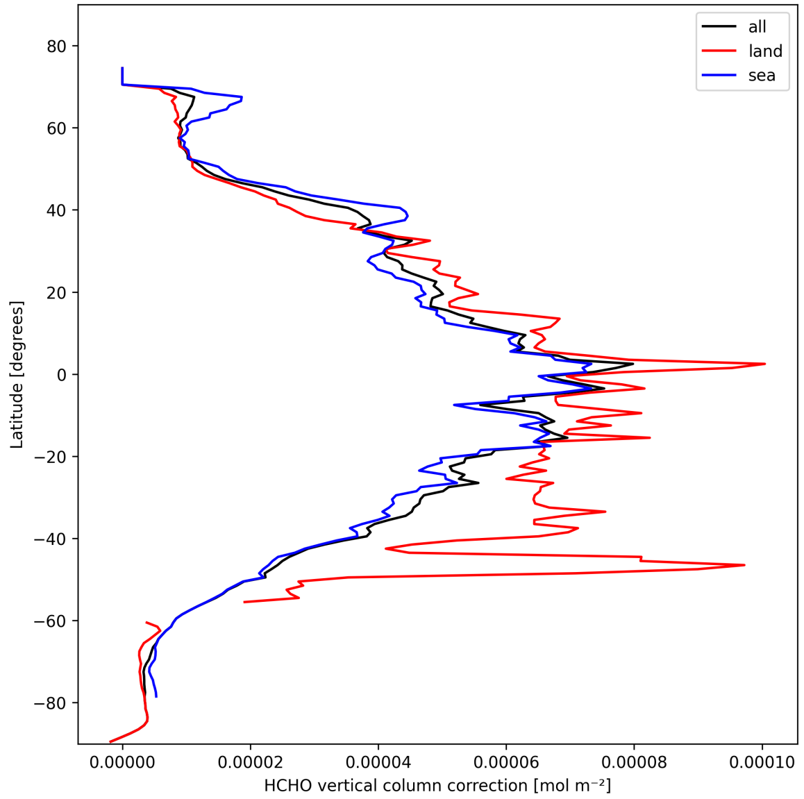
Figure 21: Zonal average of “HCHO vertical column correction” for 2025-02-20 to 2025-02-21.
