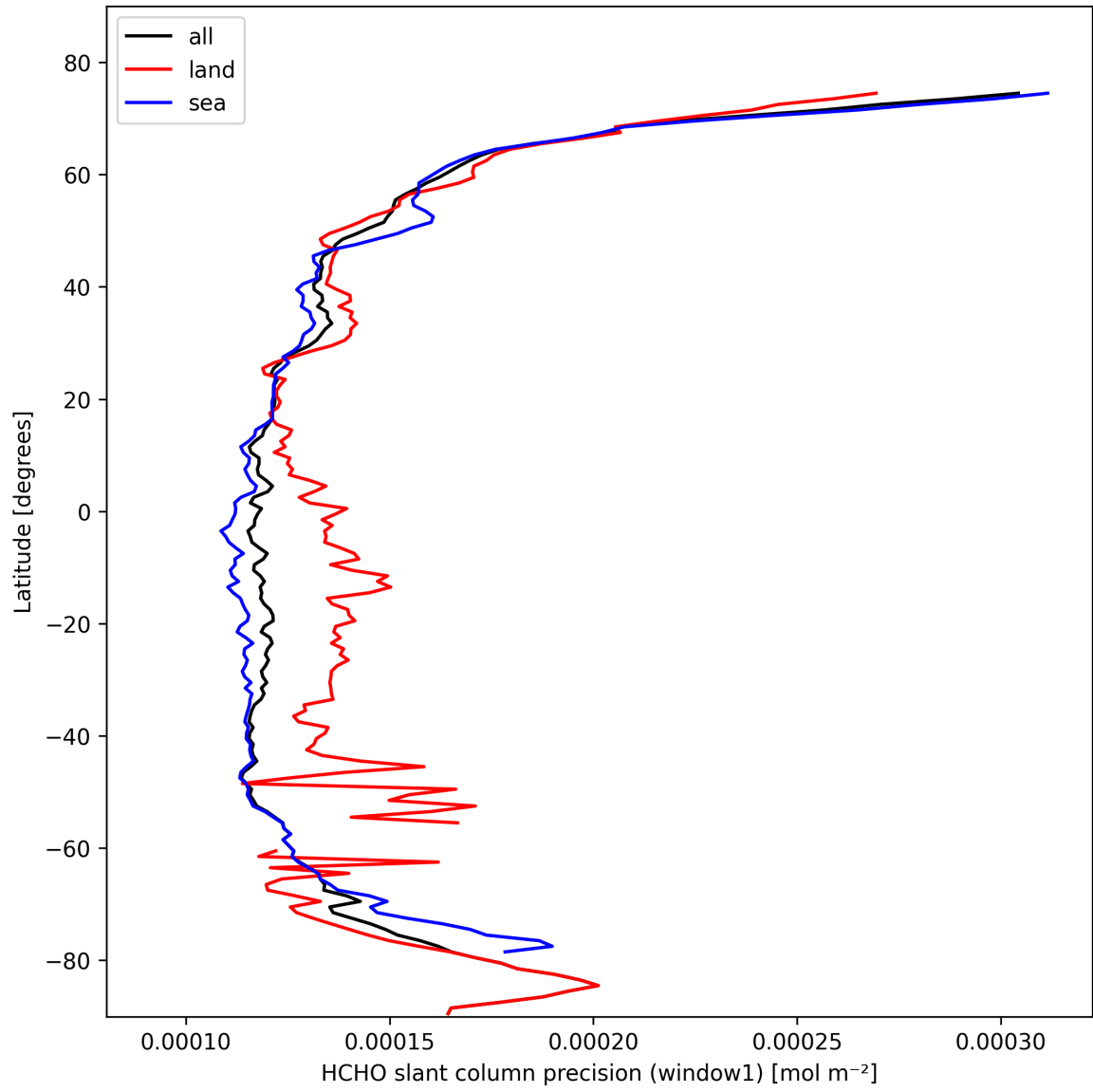
Figure 23: Zonal average of “HCHO slant column precision (window1)” for 2025-02-20 to 2025-02-21.
