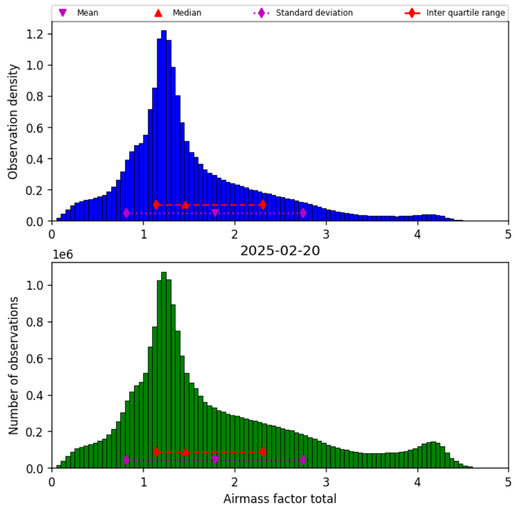
Figure 38: Histogram of “Airmass factor total” for 2025-02-20 to 2025-02-21
