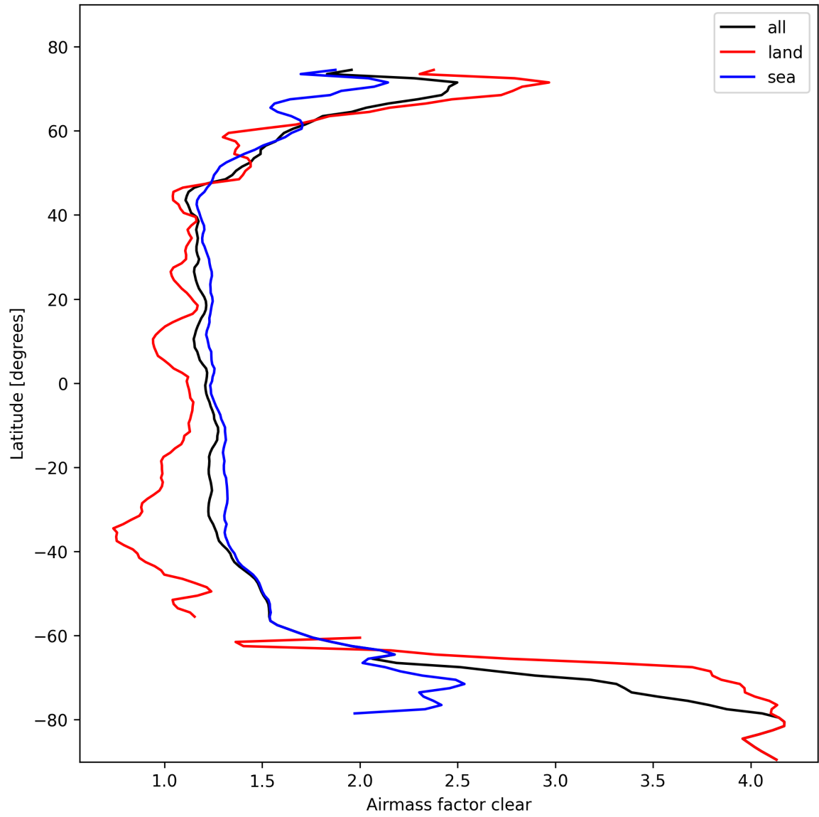
Figure 26: Zonal average of “Airmass factor clear” for 2025-02-20 to 2025-02-21.
