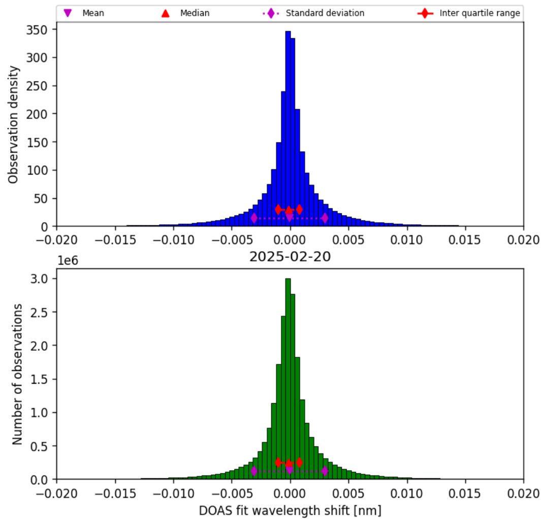
Figure 42: Histogram of “DOAS fit wavelength shift” for 2025-02-20 to 2025-02-21
