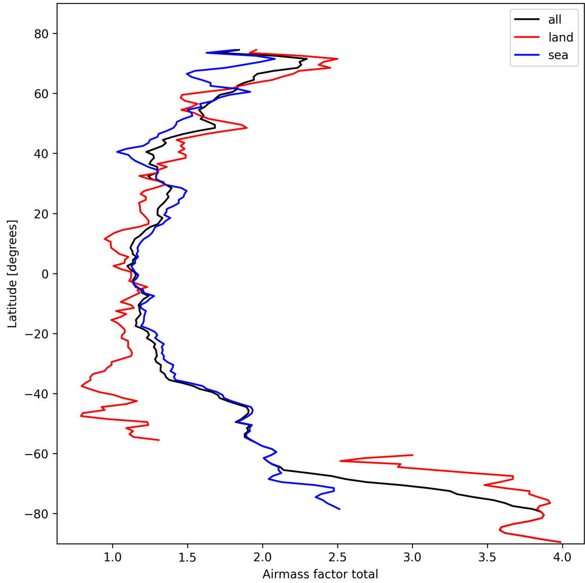
Figure 24: Zonal average of “Airmass factor total” for 2025-02-20 to 2025-02-21.
