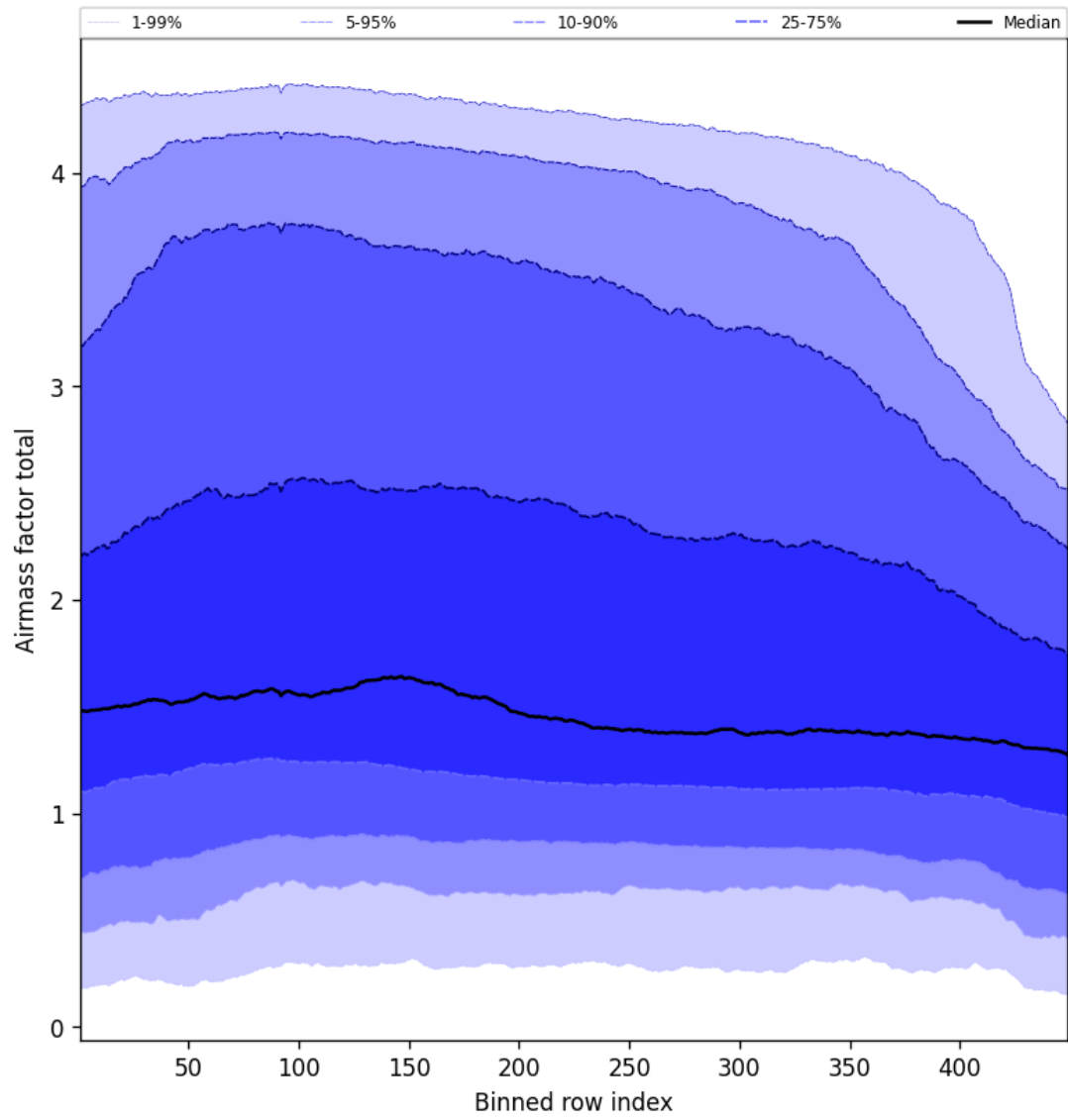
Figure 52: Along track statistics of “Airmass factor total” for 2025-02-20 to 2025-02-21
