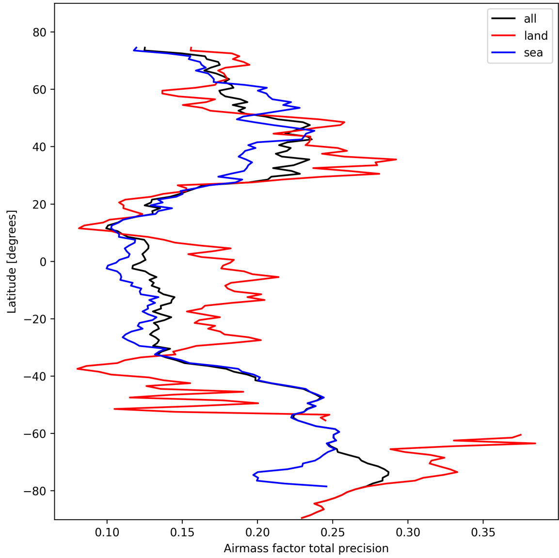
Figure 25: Zonal average of “Airmass factor total precision” for 2025-02-20 to 2025-02-21.
