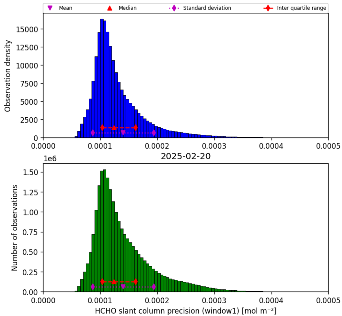
Figure 37: Histogram of “HCHO slant column precision (window1)” for 2025-02-20 to 2025-02-21
