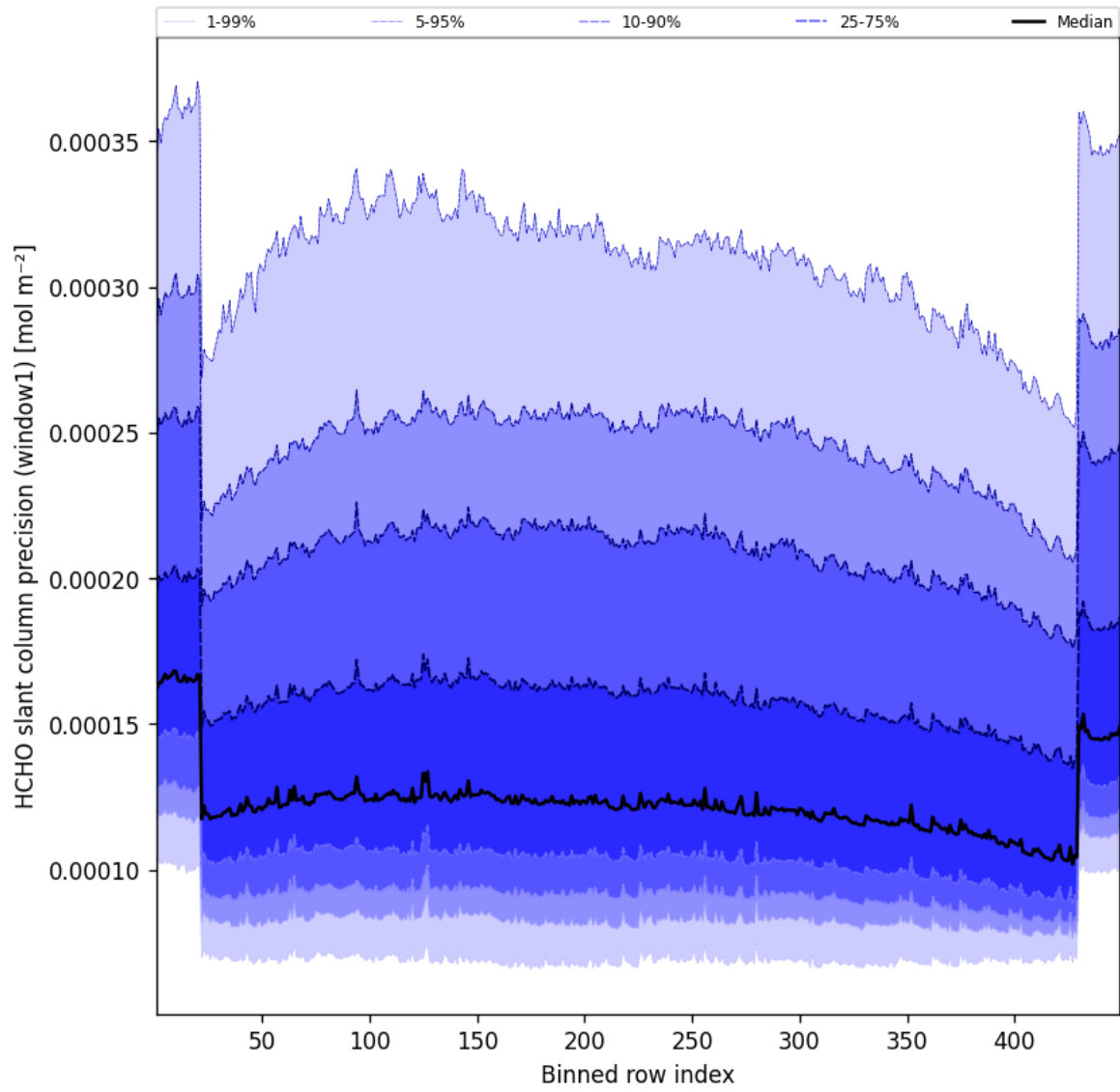
Figure 51: Along track statistics of “HCHO slant column precision (window1)” for 2025-02-20 to 2025-02-21
