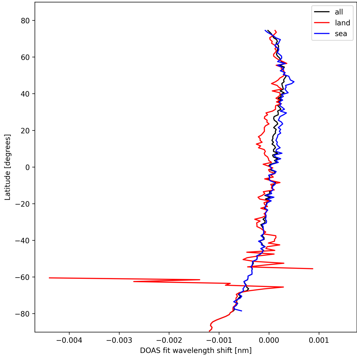
Figure 28: Zonal average of “DOAS fit wavelength shift” for 2025-02-20 to 2025-02-21.
