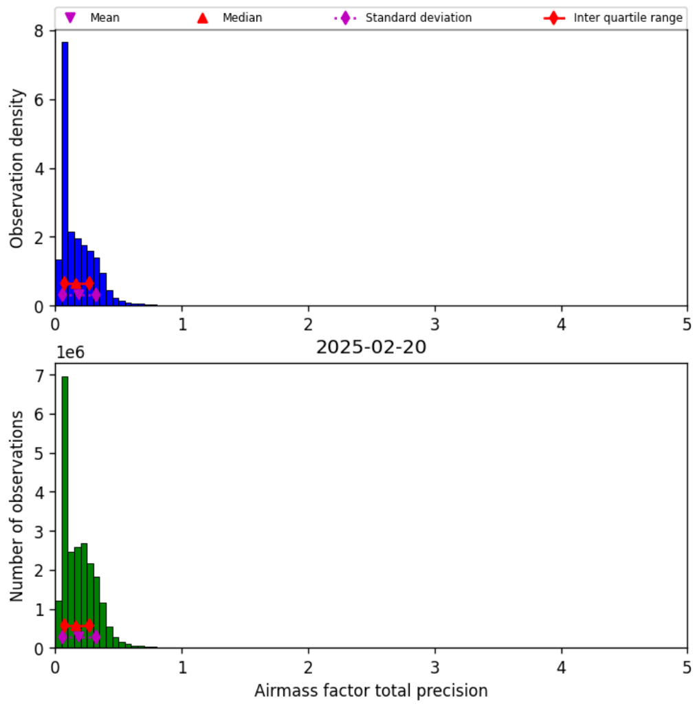
Figure 39: Histogram of “Airmass factor total precision” for 2025-02-20 to 2025-02-21
