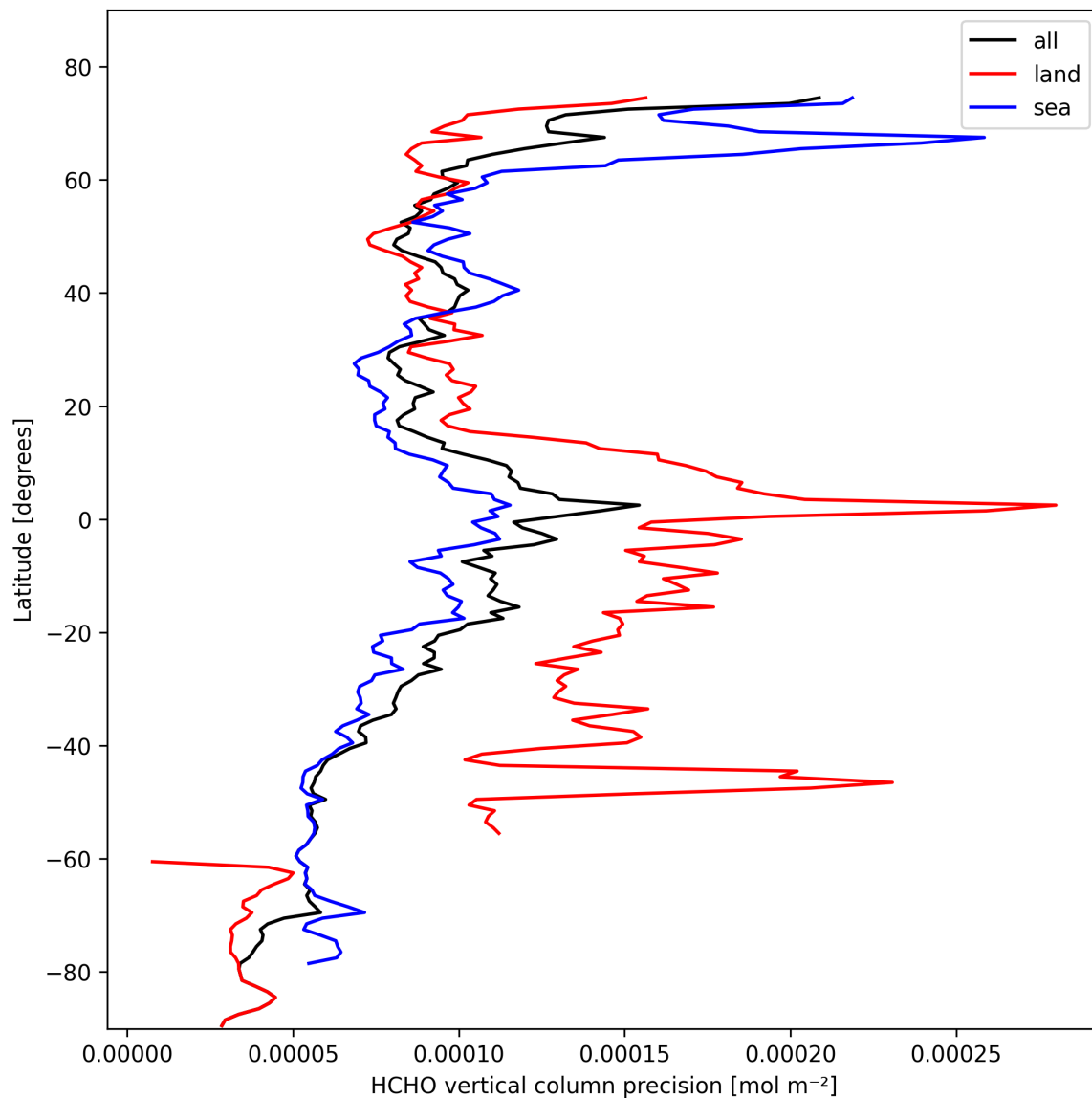
Figure 20: Zonal average of “HCHO vertical column precision” for 2025-02-20 to 2025-02-21.
