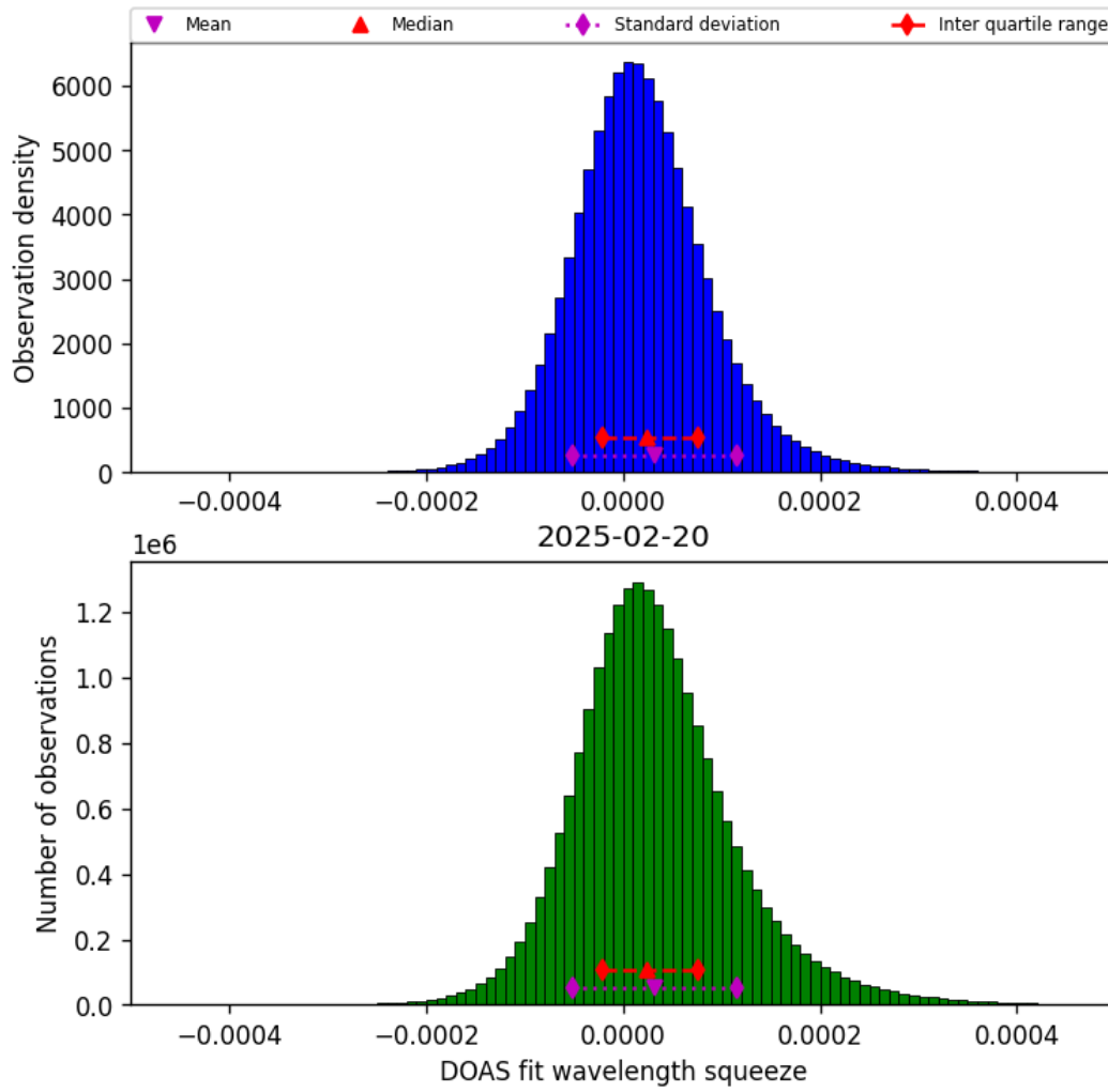
Figure 43: Histogram of “DOAS fit wavelength squeeze” for 2025-02-20 to 2025-02-21
