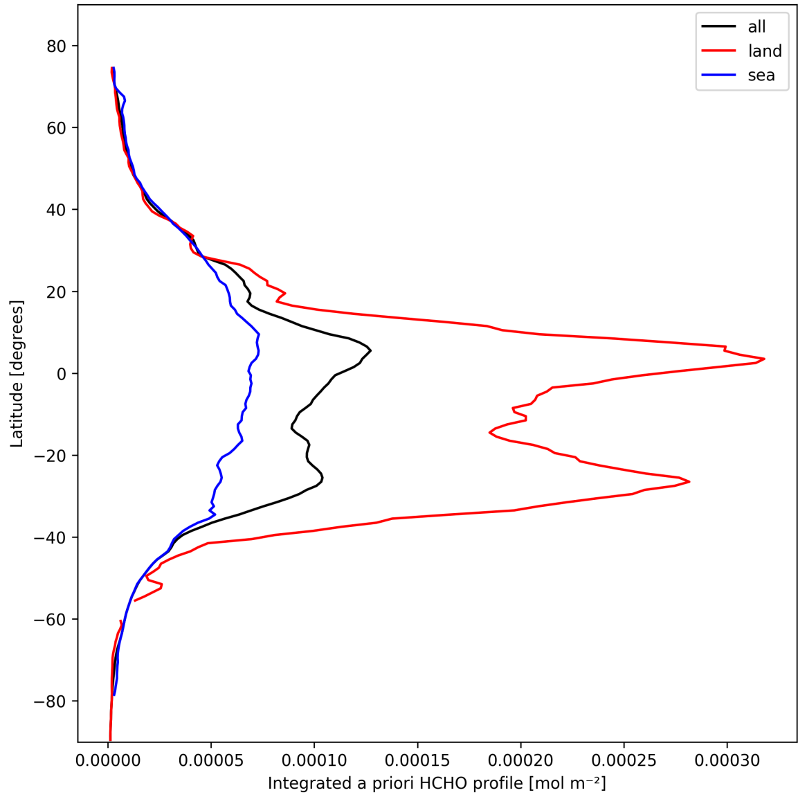
Figure 27: Zonal average of “Integrated a priori HCHO profile” for 2025-02-20 to 2025-02-21.
