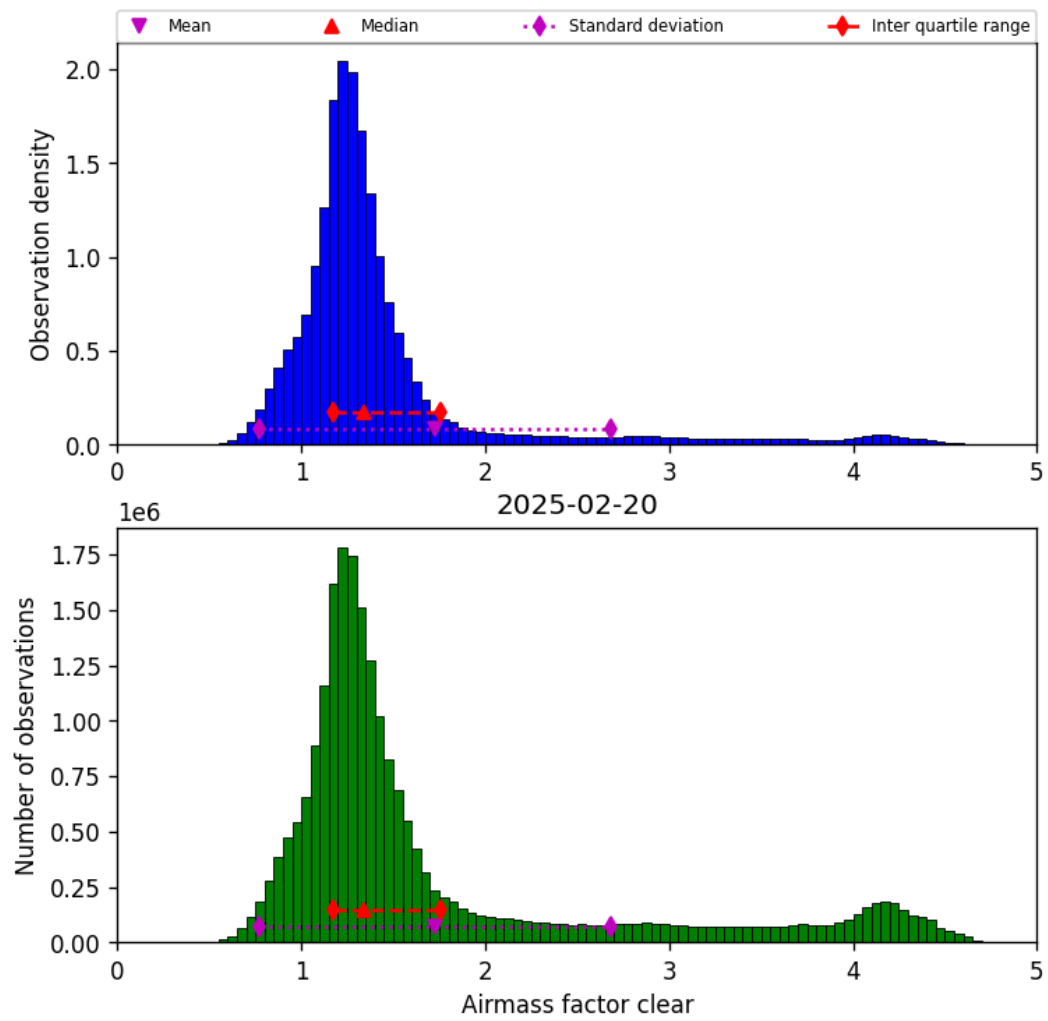
Figure 40: Histogram of “Airmass factor clear” for 2025-02-20 to 2025-02-21
