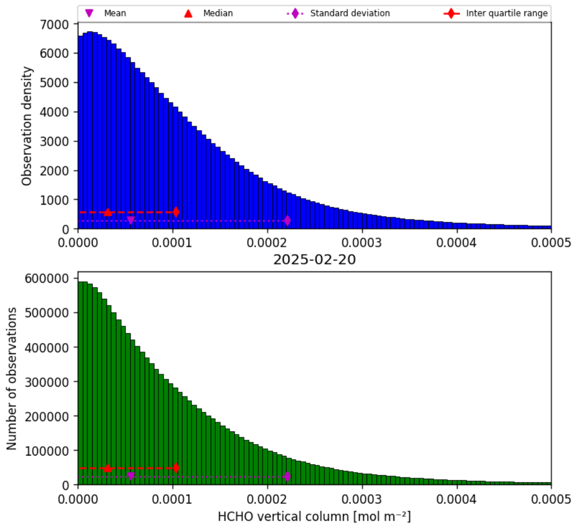
Figure 33: Histogram of “HCHO vertical column” for 2025-02-20 to 2025-02-21
