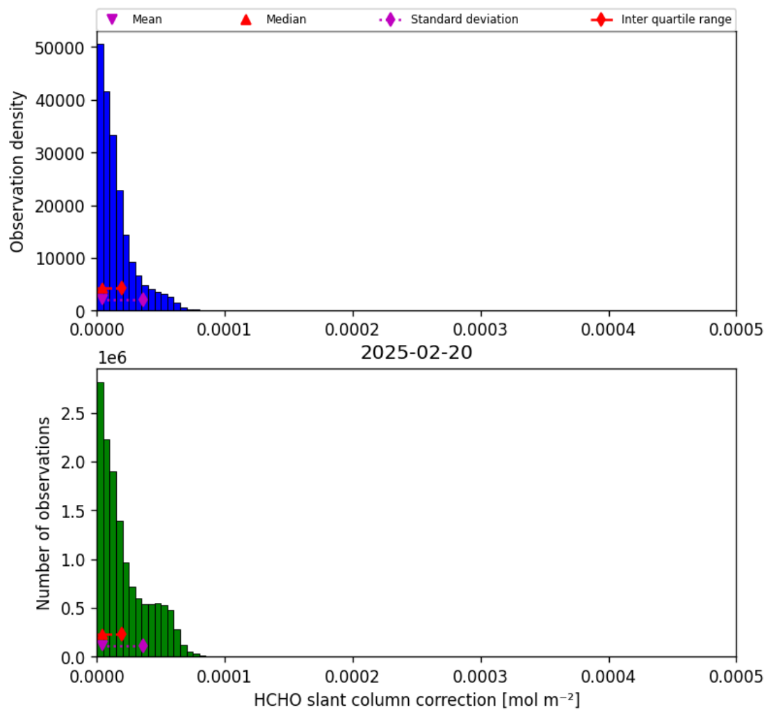
Figure 45: Histogram of “HCHO slant column correction” for 2025-02-20 to 2025-02-21
