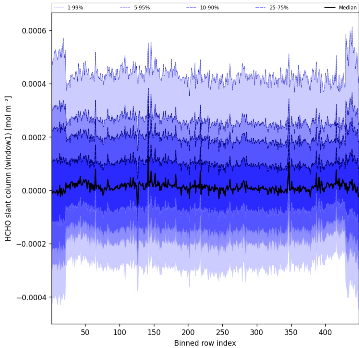
Figure 50: Along track statistics of “HCHO slant column (window1)” for 2025-02-20 to 2025-02-21
