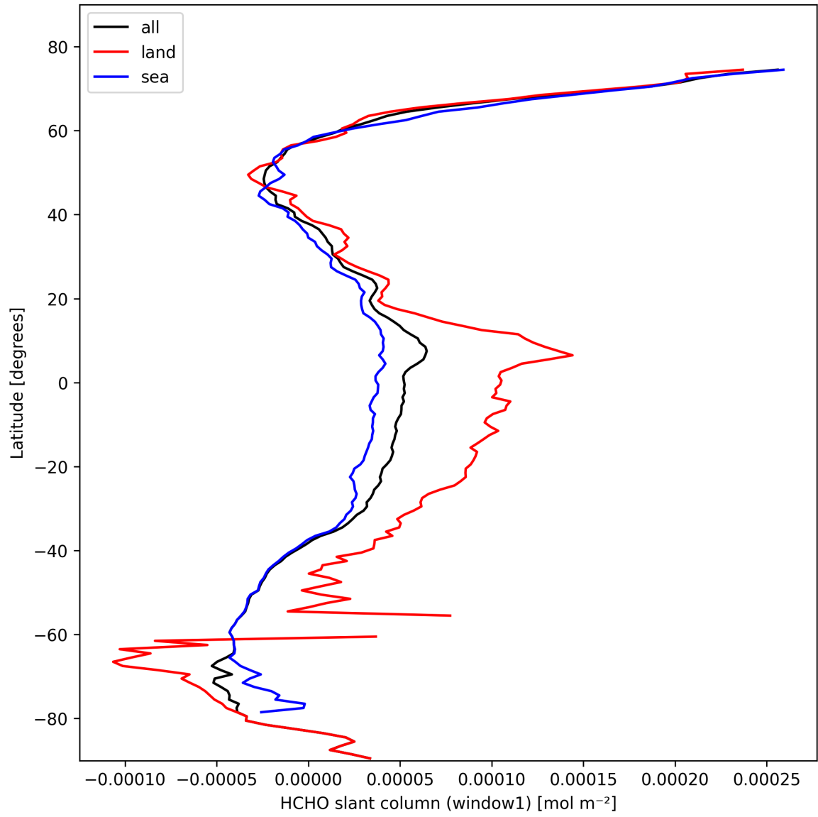
Figure 22: Zonal average of “HCHO slant column (window1)” for 2025-02-20 to 2025-02-21.
