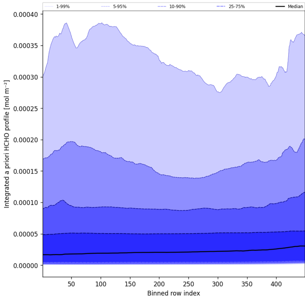
Figure 55: Along track statistics of “Integrated a priori HCHO profile” for 2025-02-20 to 2025-02-21
