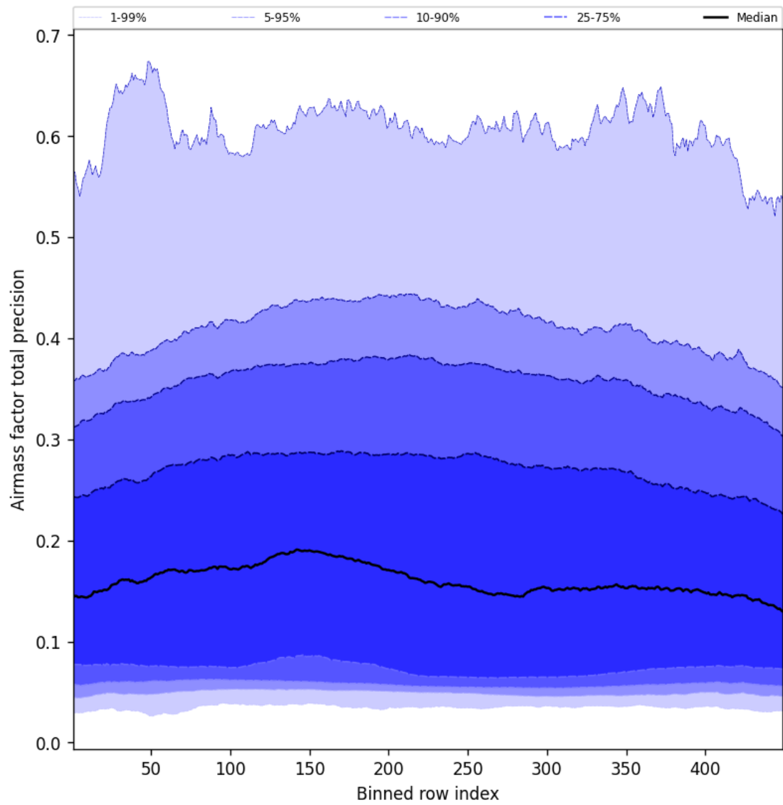
Figure 53: Along track statistics of “Airmass factor total precision” for 2025-02-20 to 2025-02-21
