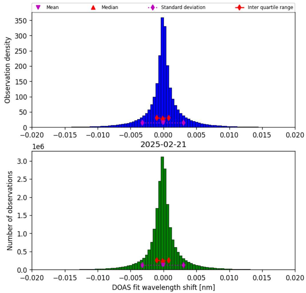
Figure 42: Histogram of “DOAS fit wavelength shift” for 2025-02-21 to 2025-02-22
