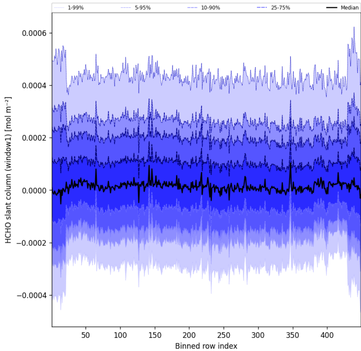
Figure 50: Along track statistics of “HCHO slant column (window1)” for 2025-02-21 to 2025-02-22
