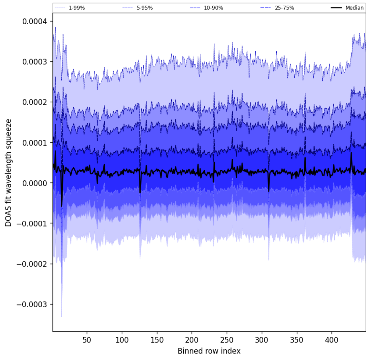
Figure 57: Along track statistics of “DOAS fit wavelength squeeze” for 2025-02-21 to 2025-02-22
