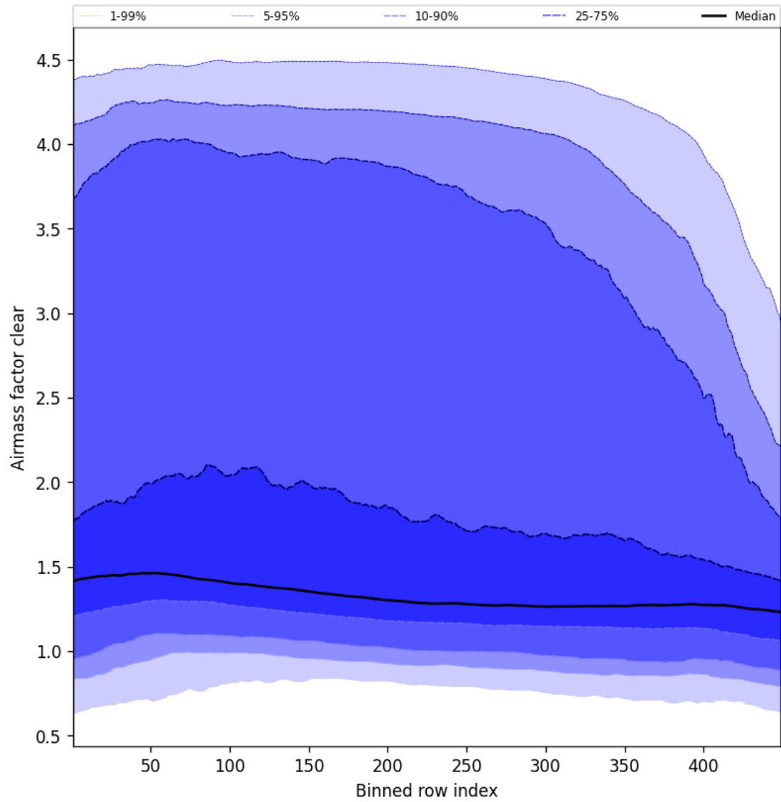
Figure 54: Along track statistics of “Airmass factor clear” for 2025-02-21 to 2025-02-22
