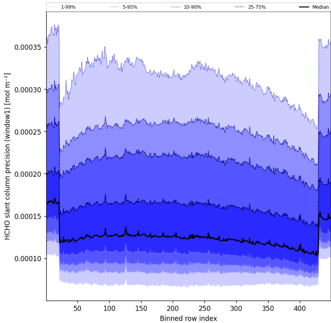
Figure 51: Along track statistics of “HCHO slant column precision (window1)” for 2025-02-21 to 2025-02-22
