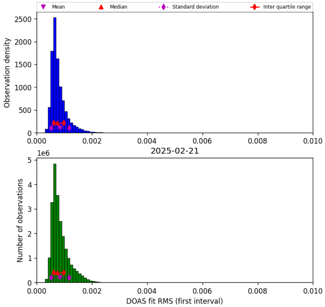
Figure 44: Histogram of “DOAS fit RMS (first interval)” for 2025-02-21 to 2025-02-22
