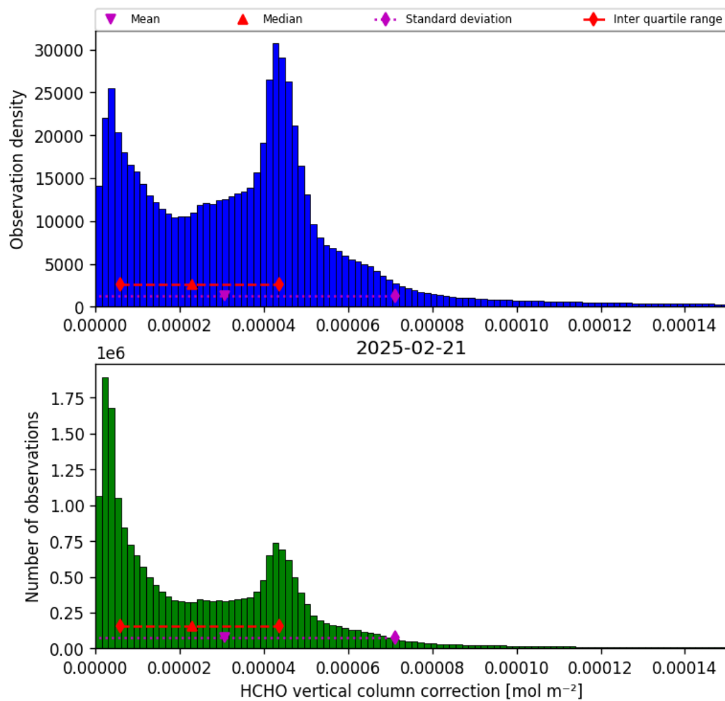
Figure 35: Histogram of “HCHO vertical column correction” for 2025-02-21 to 2025-02-22
