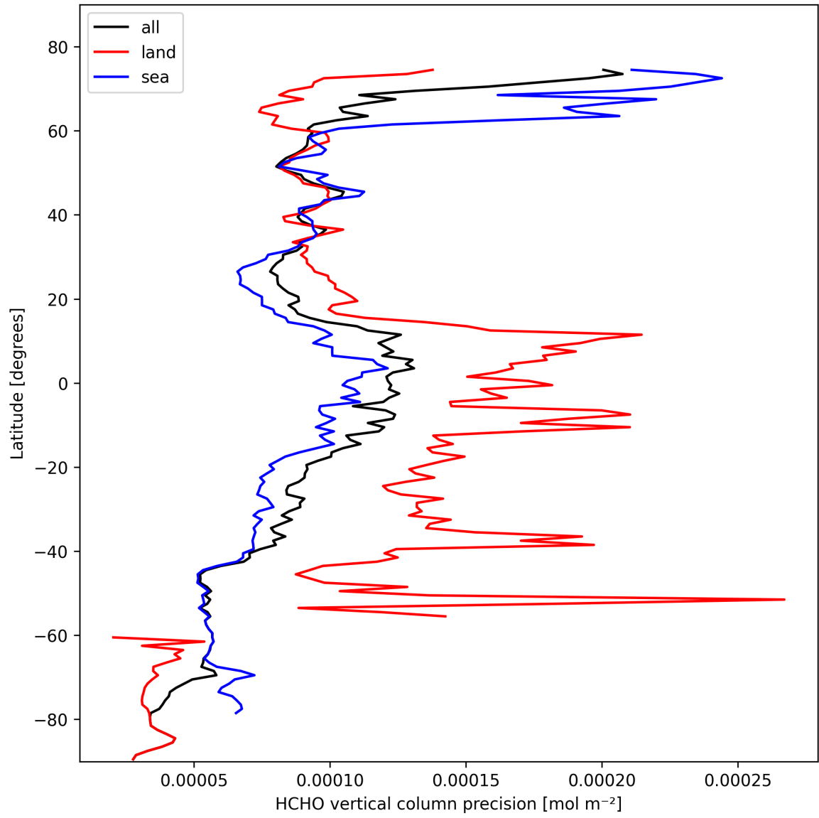
Figure 20: Zonal average of “HCHO vertical column precision” for 2025-02-21 to 2025-02-22.
