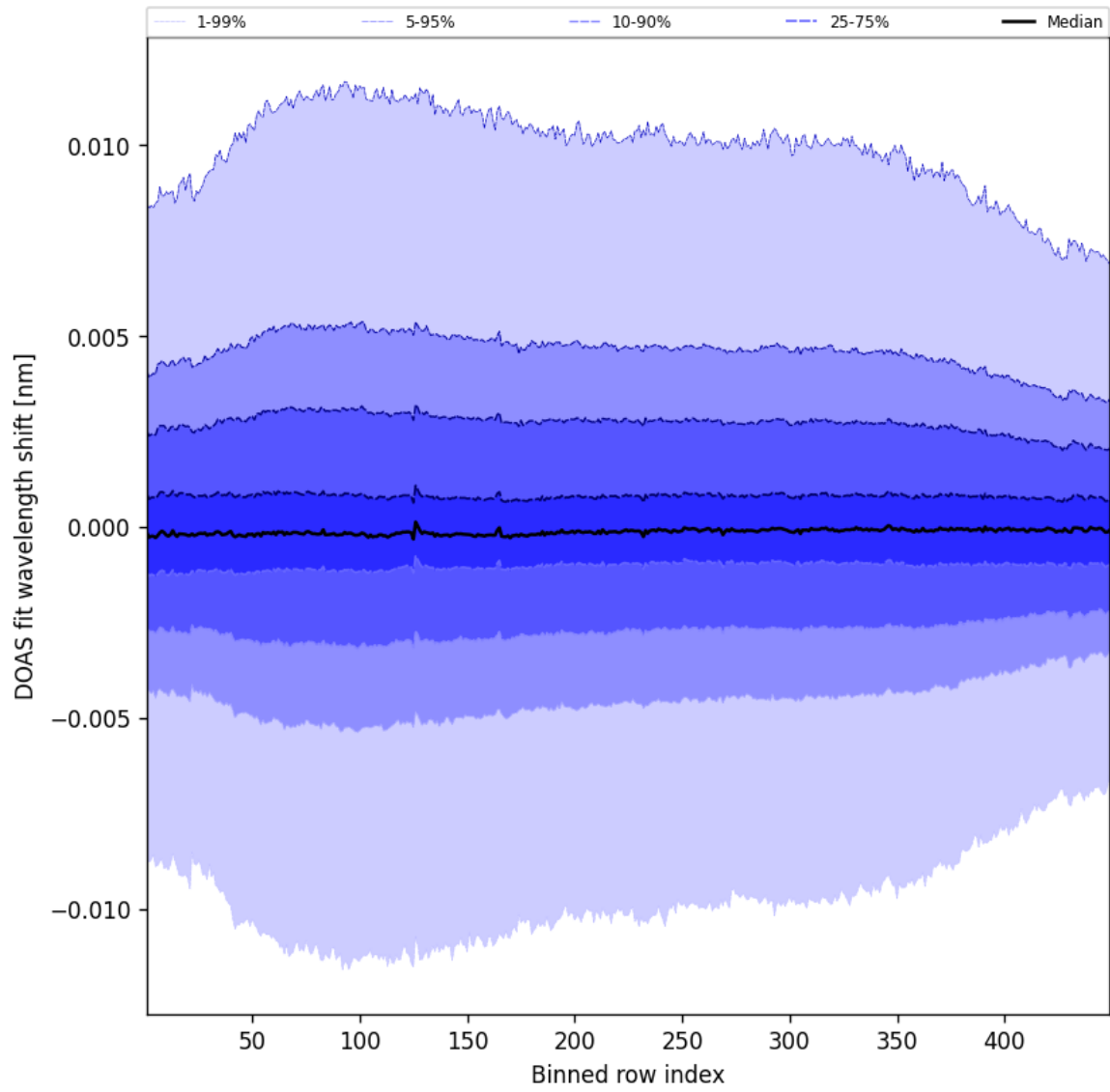
Figure 56: Along track statistics of “DOAS fit wavelength shift” for 2025-02-21 to 2025-02-22
