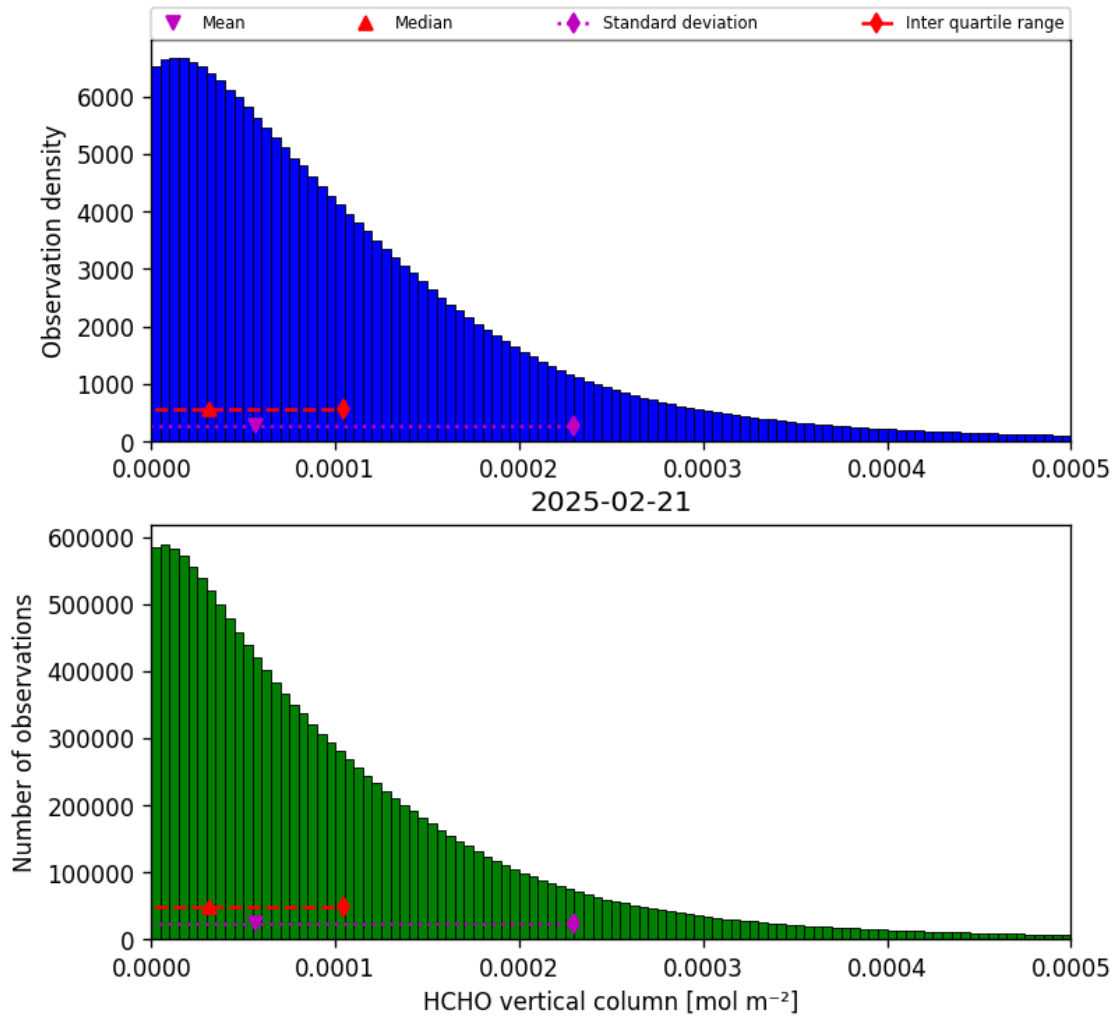
Figure 33: Histogram of “HCHO vertical column” for 2025-02-21 to 2025-02-22
