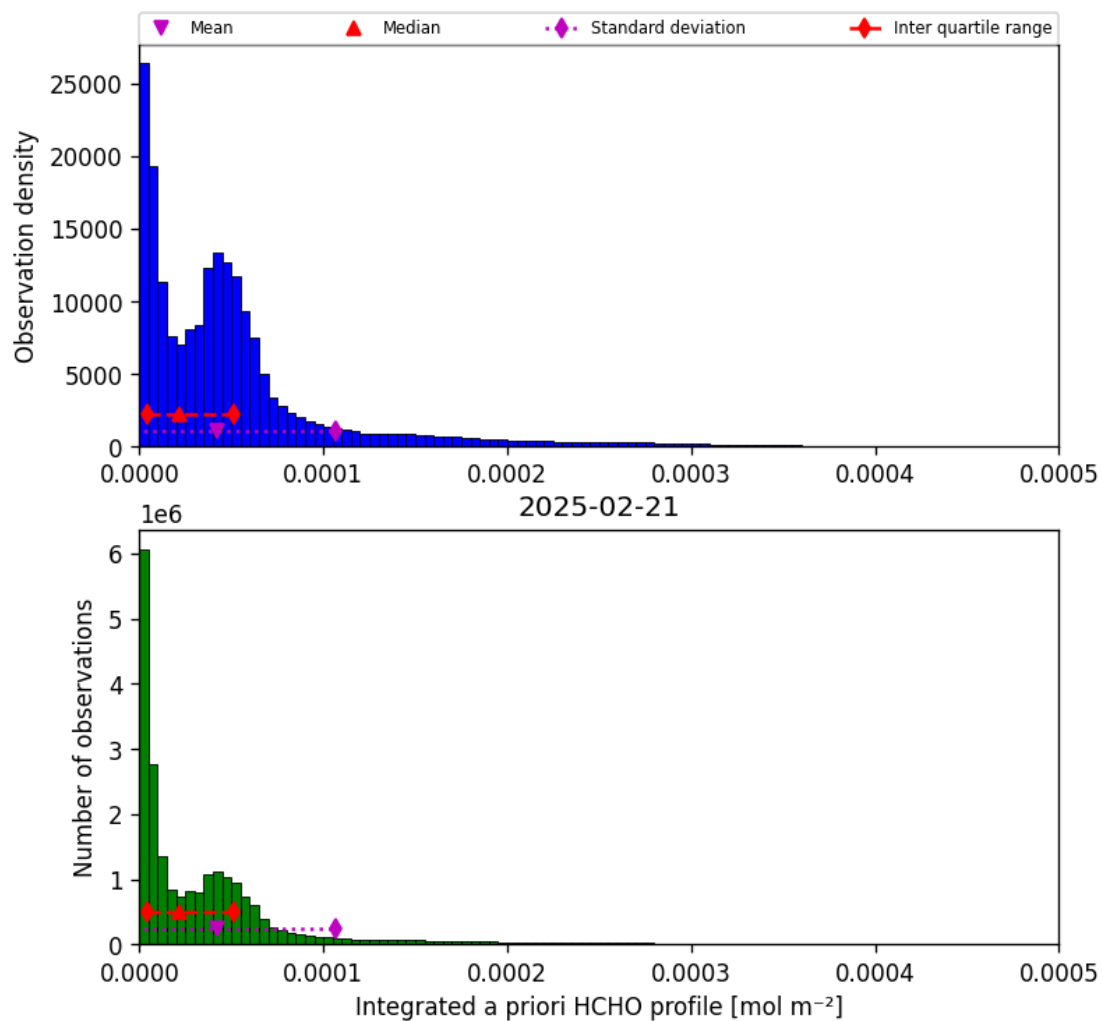
Figure 41: Histogram of “Integrated a priori HCHO profile” for 2025-02-21 to 2025-02-22
