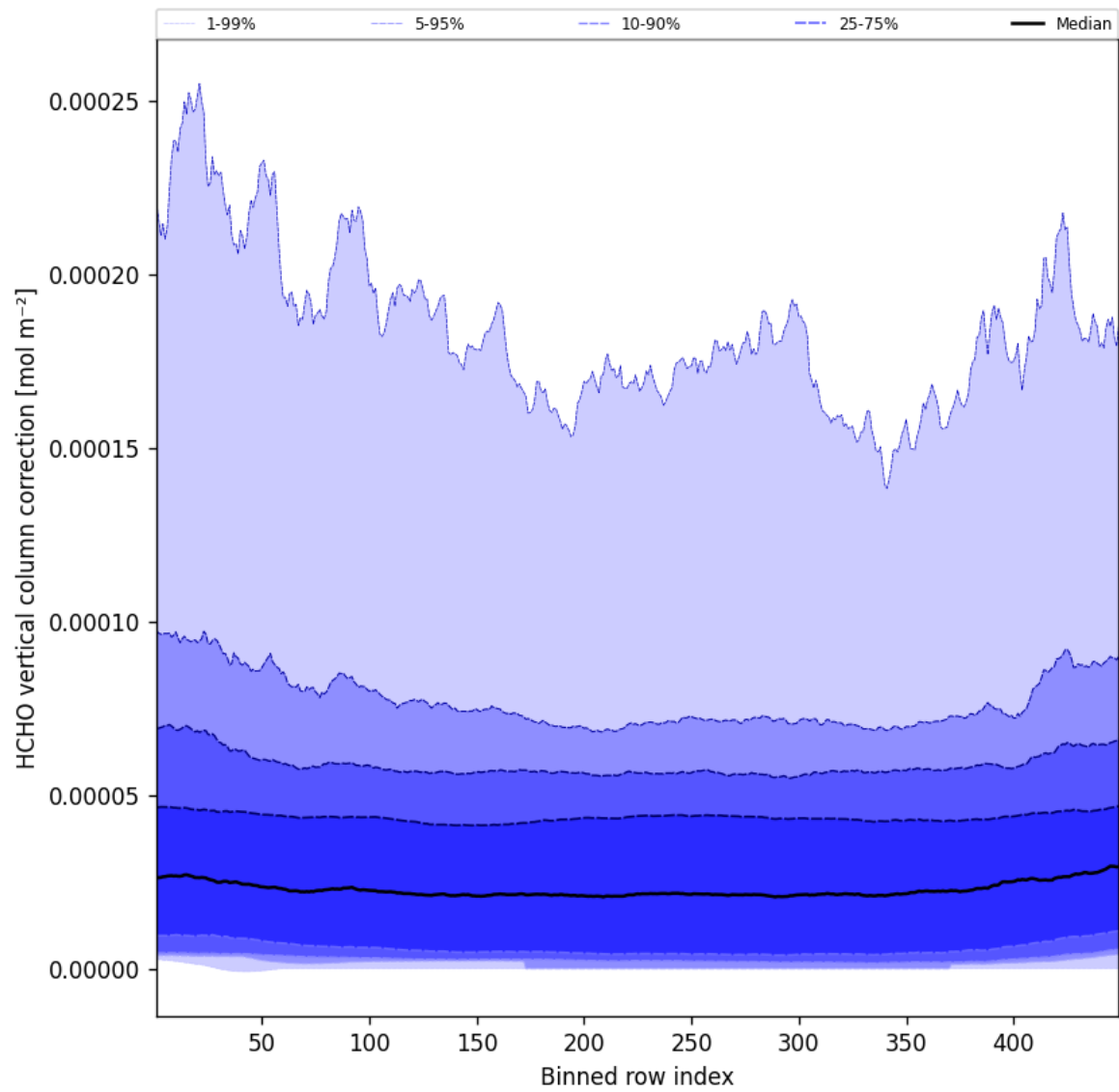
Figure 49: Along track statistics of “HCHO vertical column correction” for 2025-02-21 to 2025-02-22
