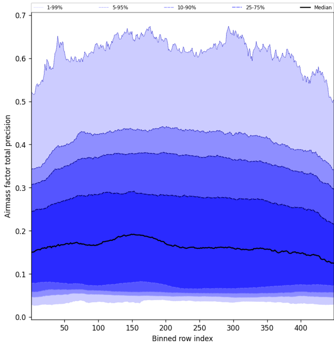
Figure 53: Along track statistics of “Airmass factor total precision” for 2025-02-21 to 2025-02-22
