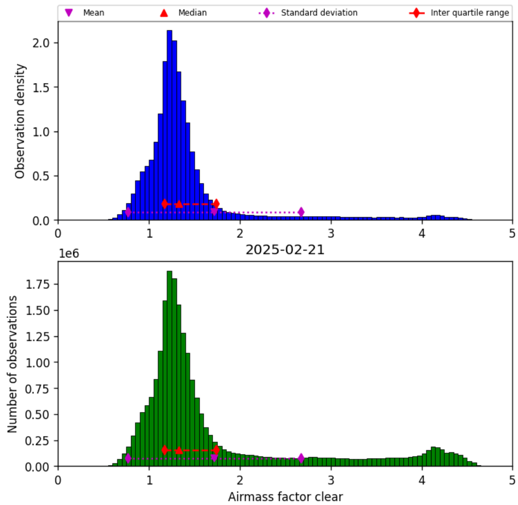
Figure 40: Histogram of “Airmass factor clear” for 2025-02-21 to 2025-02-22
