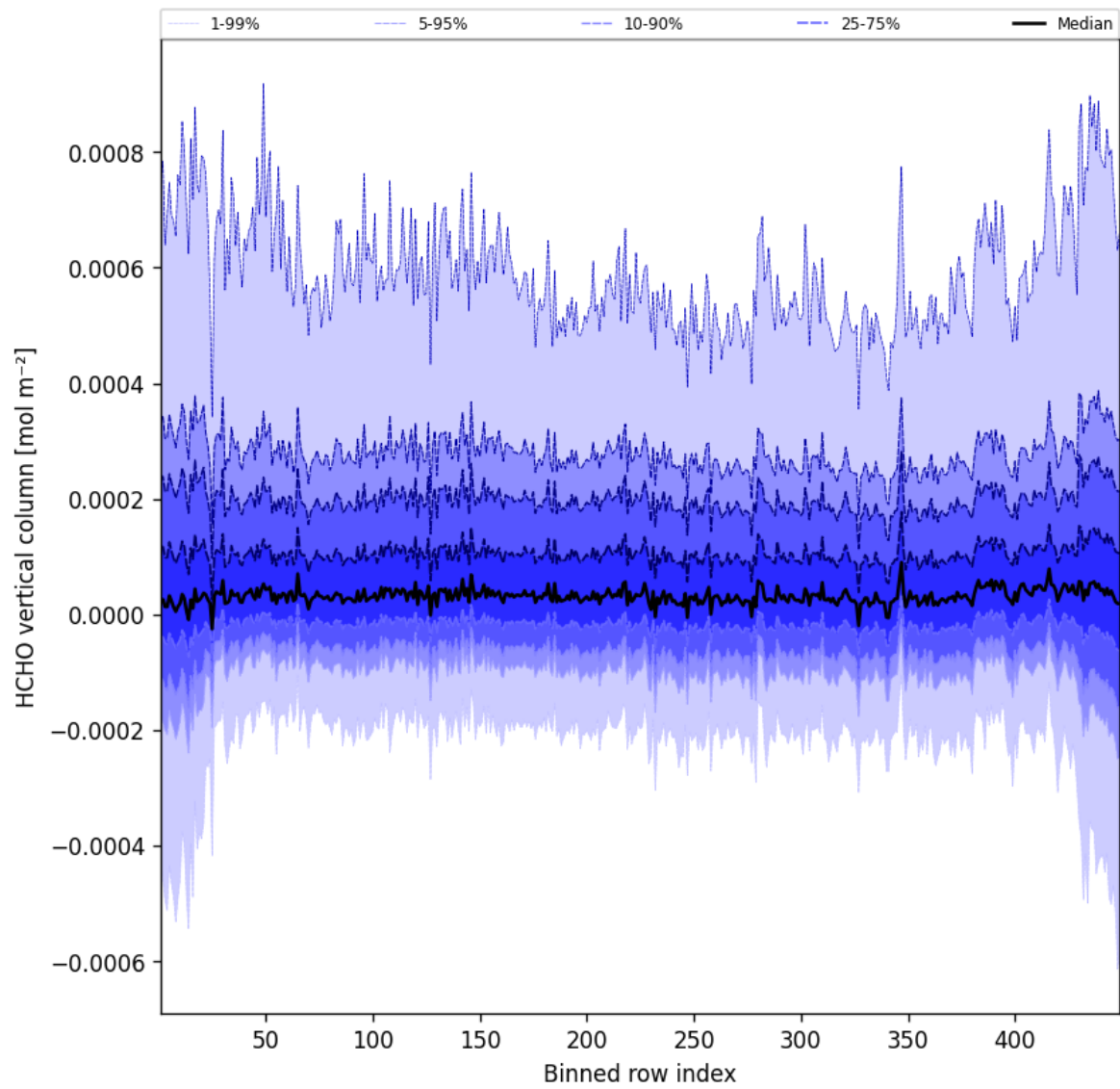
Figure 47: Along track statistics of “HCHO vertical column” for 2025-02-21 to 2025-02-22
