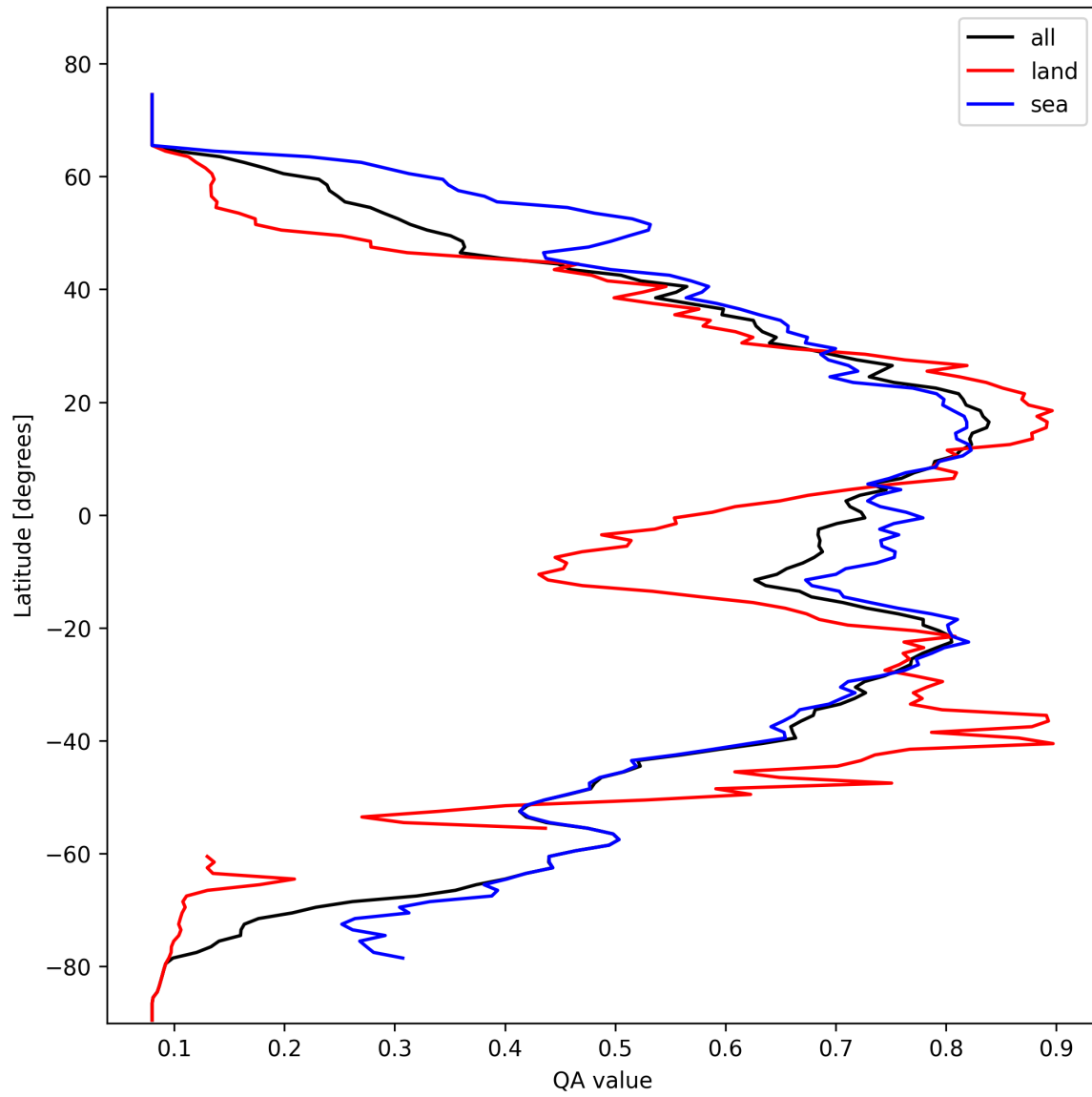
Figure 18: Zonal average of “QA value” for 2025-02-21 to 2025-02-22.
