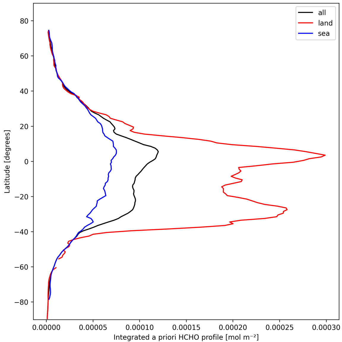
Figure 27: Zonal average of “Integrated a priori HCHO profile” for 2025-02-21 to 2025-02-22.
