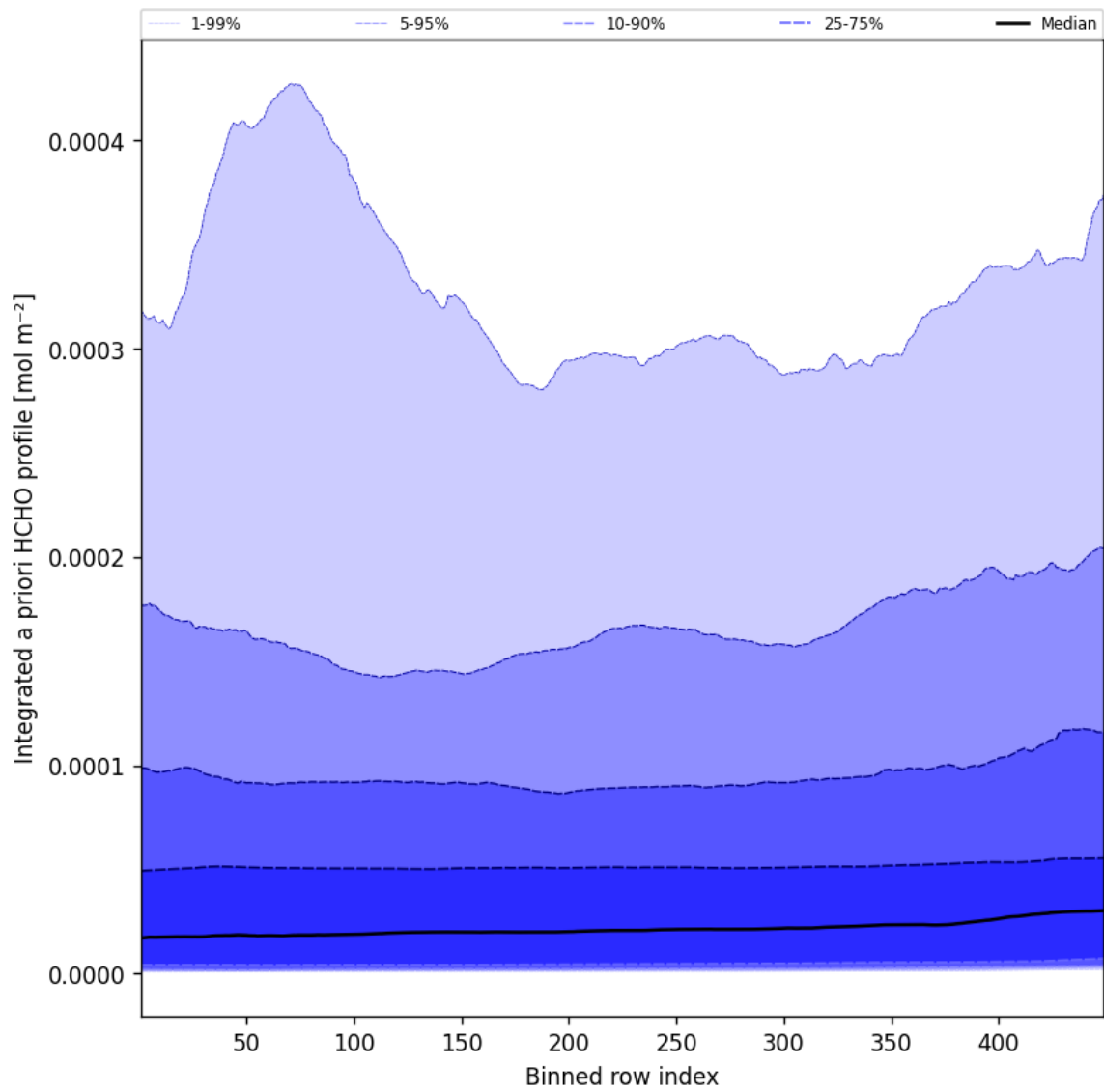
Figure 55: Along track statistics of “Integrated a priori HCHO profile” for 2025-02-21 to 2025-02-22
