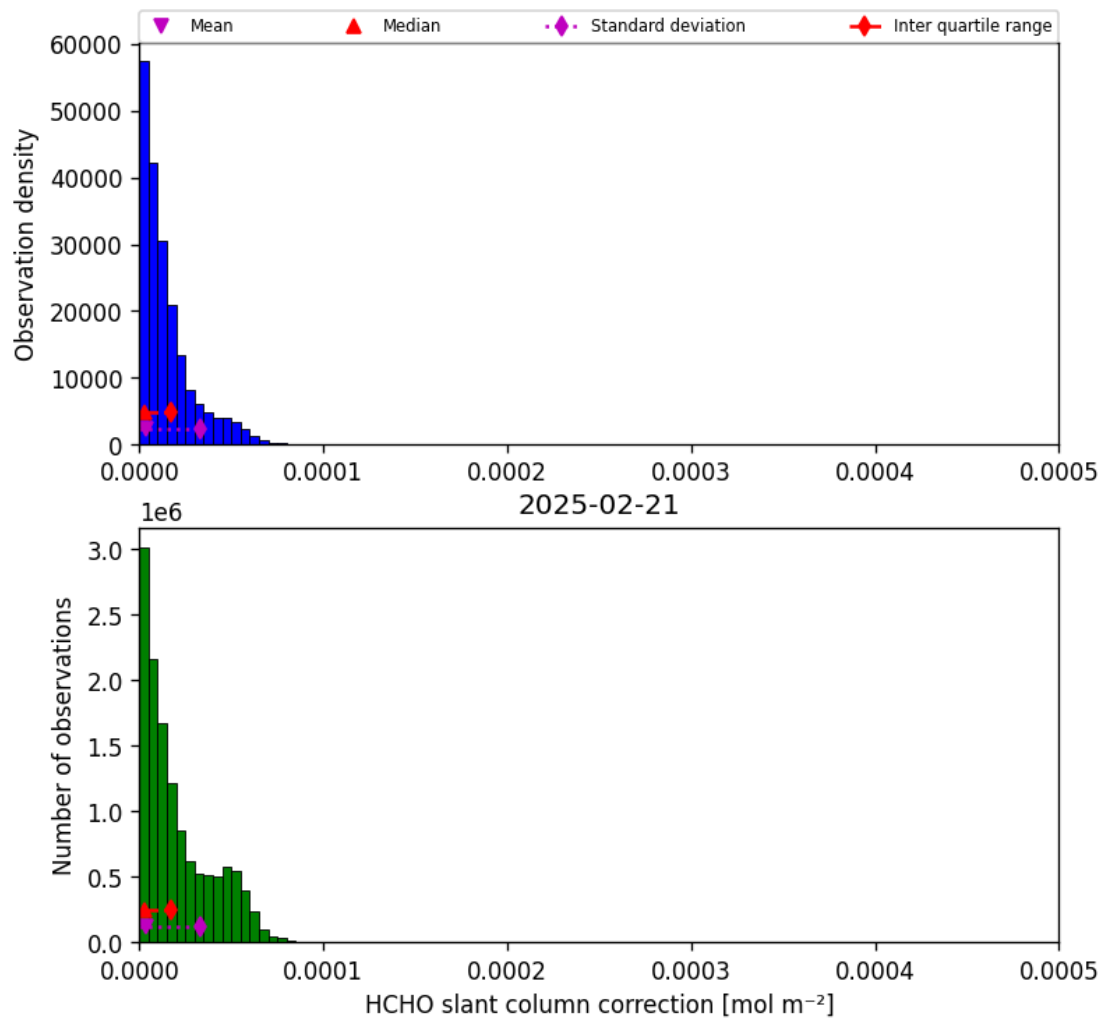
Figure 45: Histogram of “HCHO slant column correction” for 2025-02-21 to 2025-02-22
