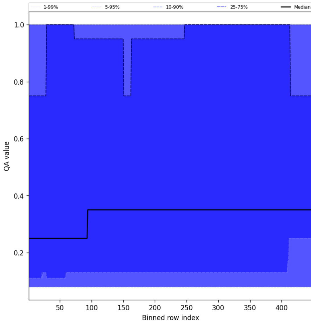
Figure 46: Along track statistics of “QA value” for 2025-02-21 to 2025-02-22
