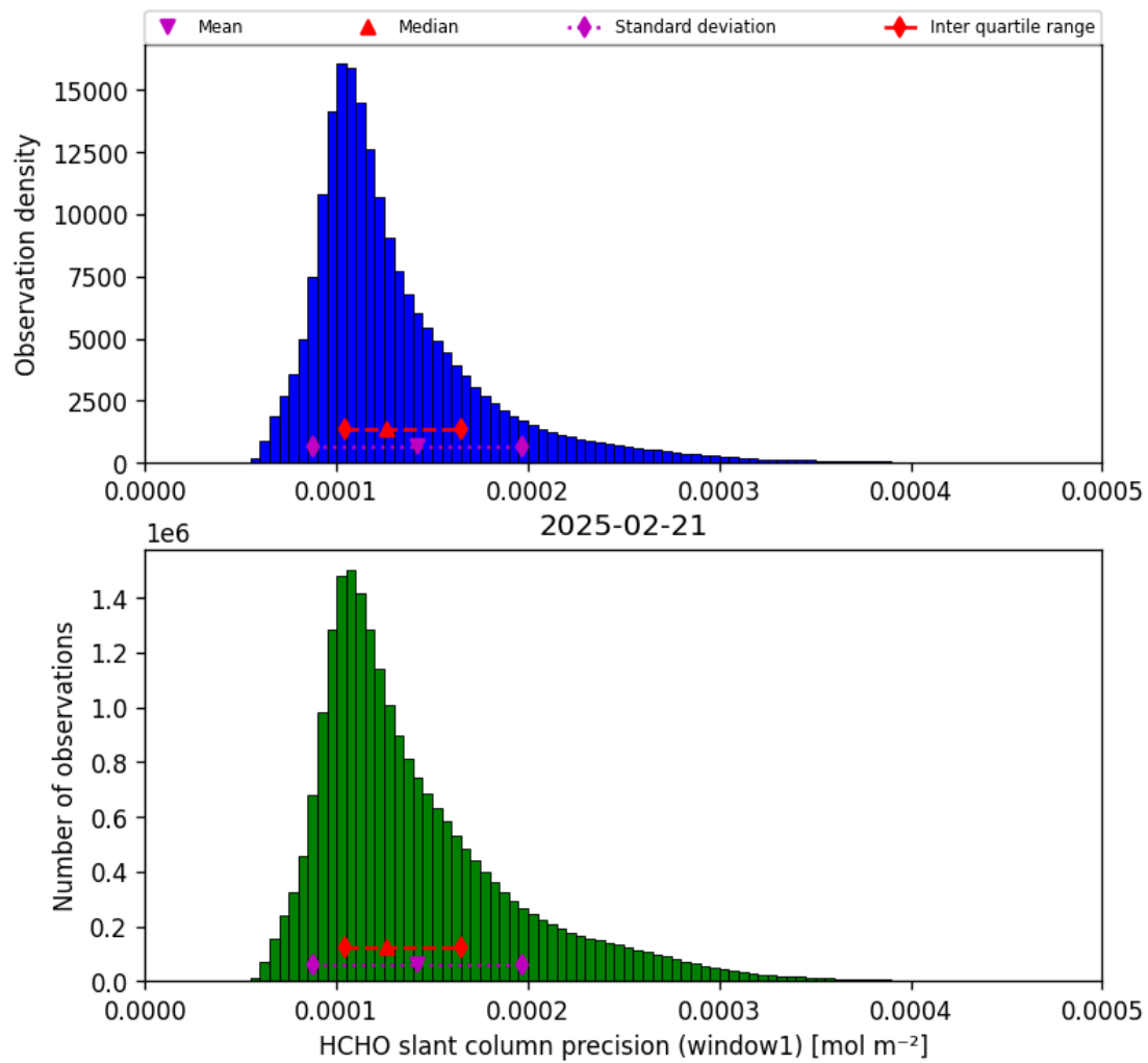
Figure 37: Histogram of “HCHO slant column precision (window1)” for 2025-02-21 to 2025-02-22
