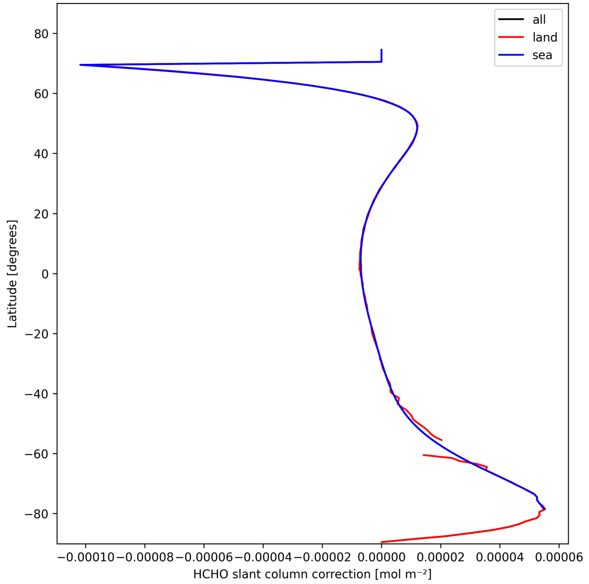
Figure 31: Zonal average of “HCHO slant column correction” for 2025-02-21 to 2025-02-22.
