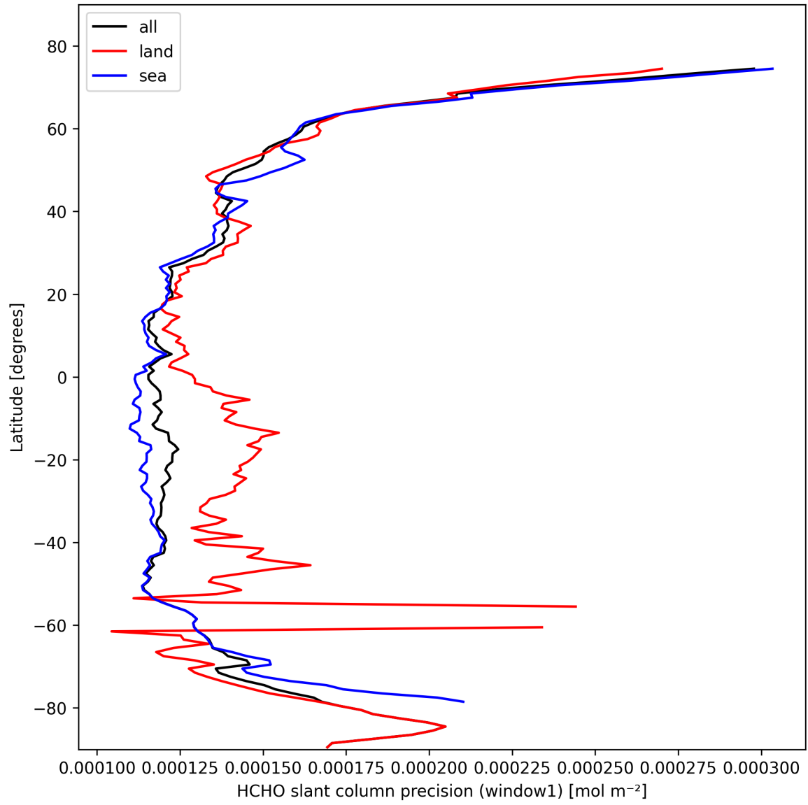
Figure 23: Zonal average of “HCHO slant column precision (window1)” for 2025-02-21 to 2025-02-22.
