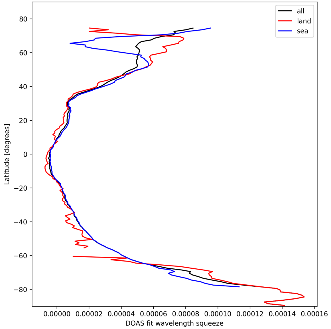
Figure 29: Zonal average of “DOAS fit wavelength squeeze” for 2025-02-21 to 2025-02-22.
