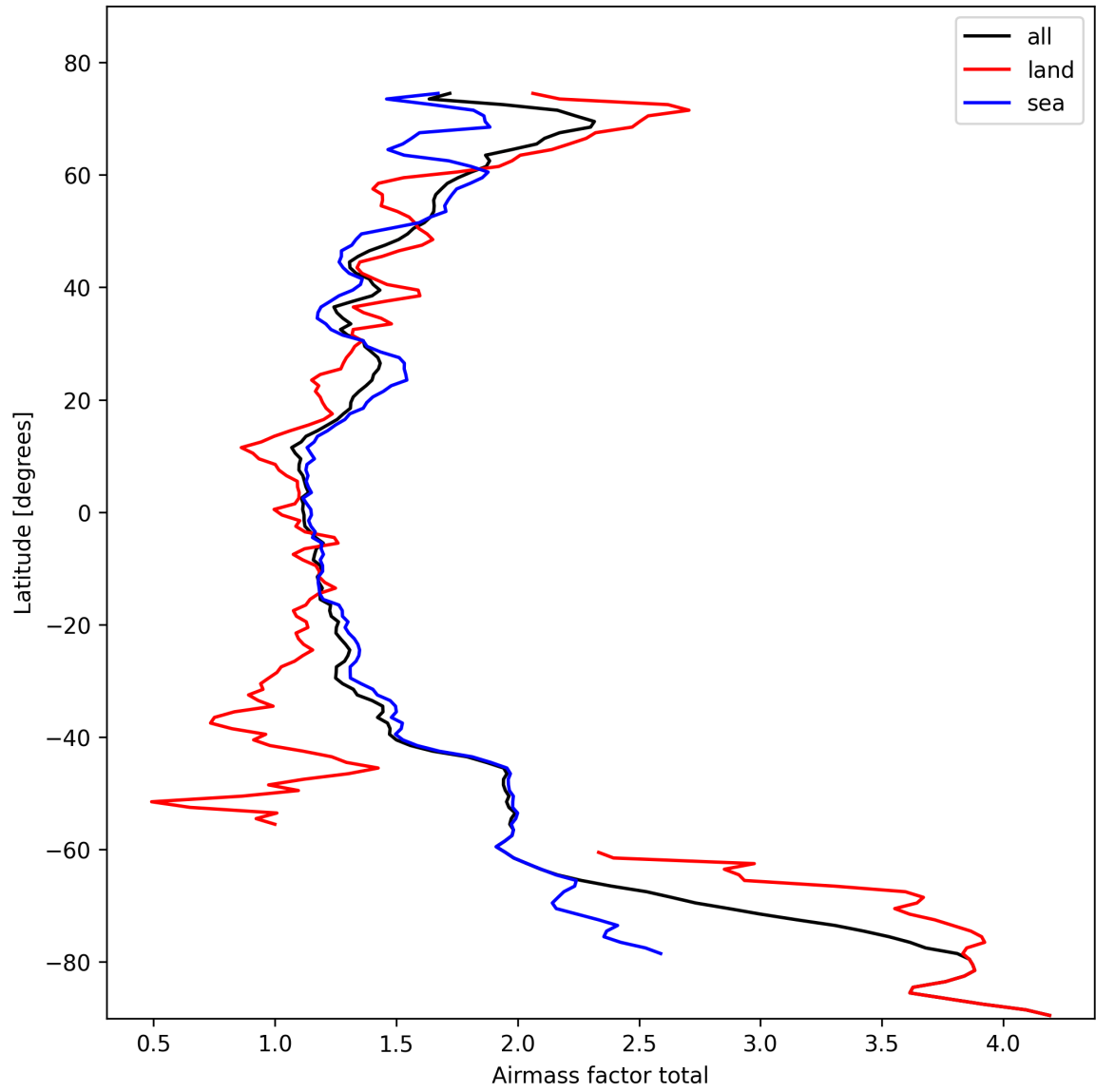
Figure 24: Zonal average of “Airmass factor total” for 2025-02-21 to 2025-02-22.
