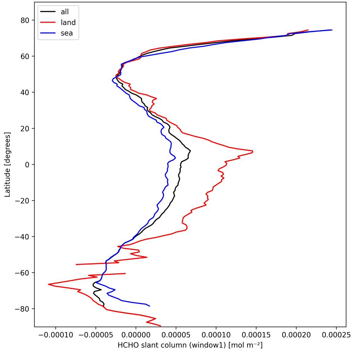
Figure 22: Zonal average of “HCHO slant column (window1)” for 2025-02-21 to 2025-02-22.
