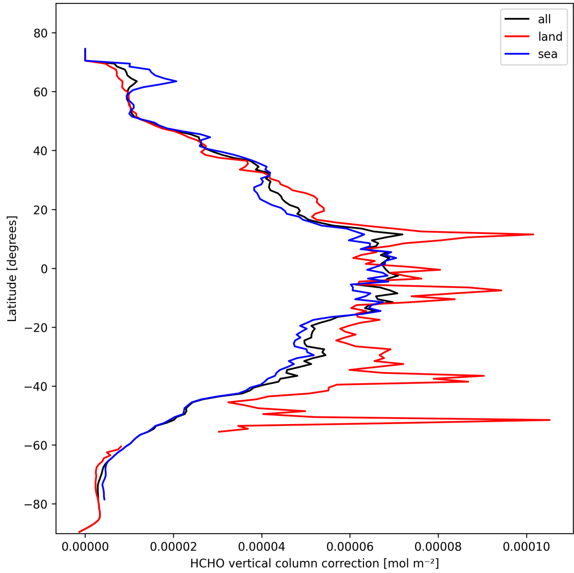
Figure 21: Zonal average of “HCHO vertical column correction” for 2025-02-21 to 2025-02-22.
