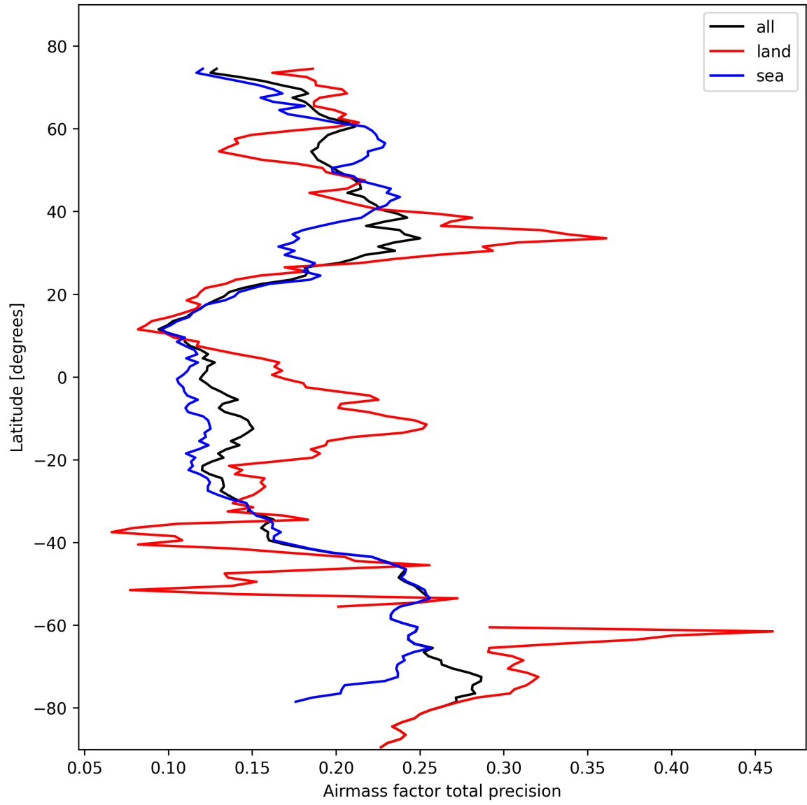
Figure 25: Zonal average of “Airmass factor total precision” for 2025-02-21 to 2025-02-22.
