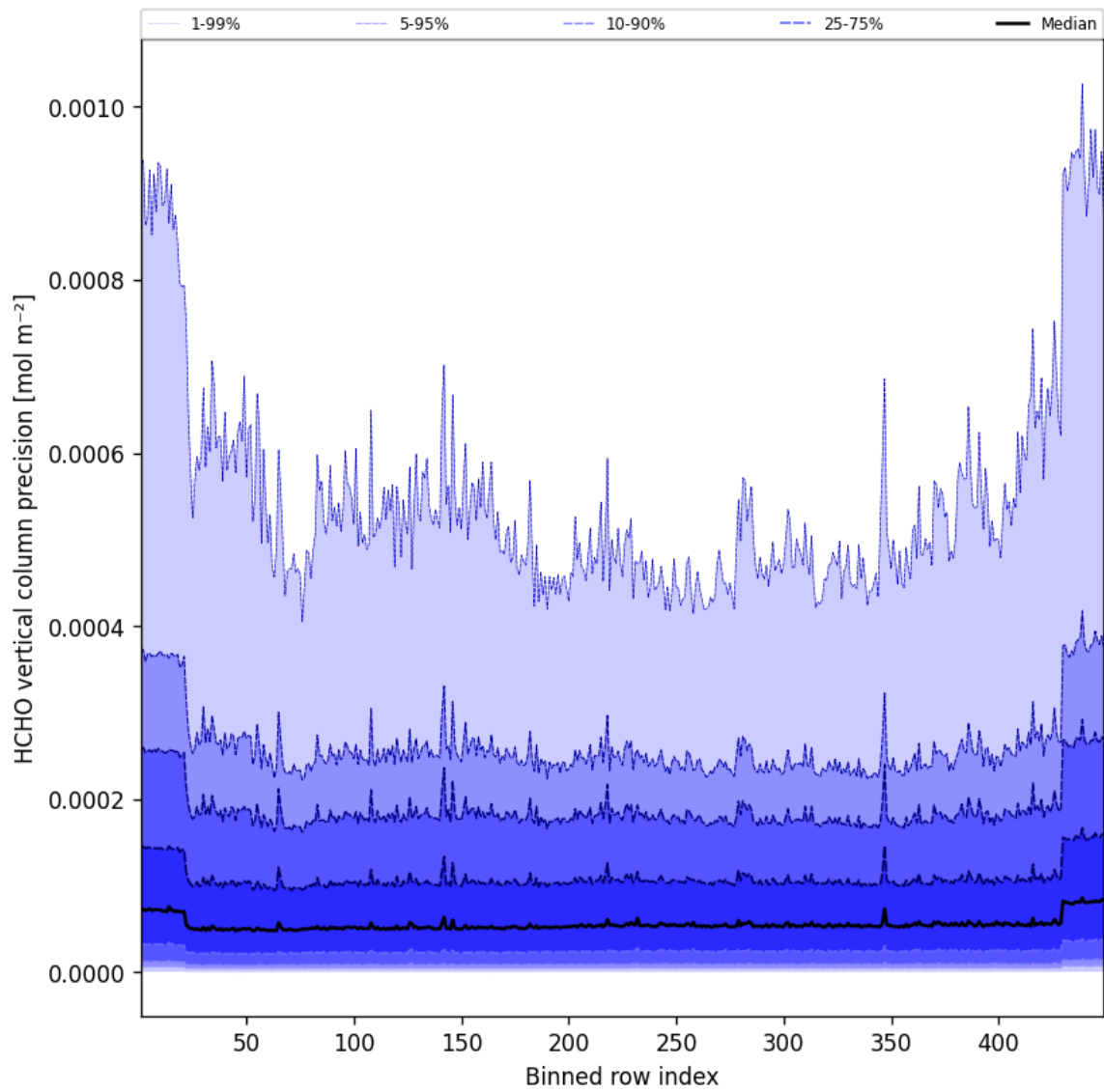
Figure 48: Along track statistics of “HCHO vertical column precision” for 2025-02-21 to 2025-02-22
