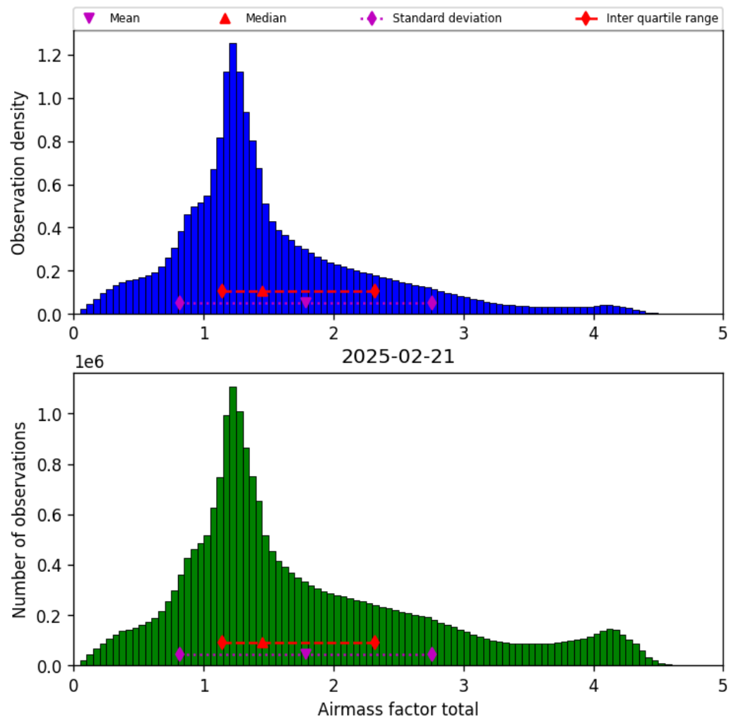
Figure 38: Histogram of “Airmass factor total” for 2025-02-21 to 2025-02-22
