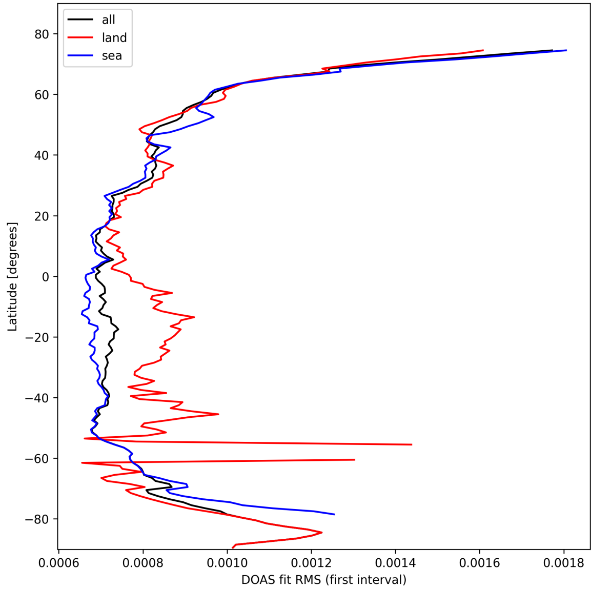
Figure 30: Zonal average of “DOAS fit RMS (first interval)” for 2025-02-21 to 2025-02-22.
