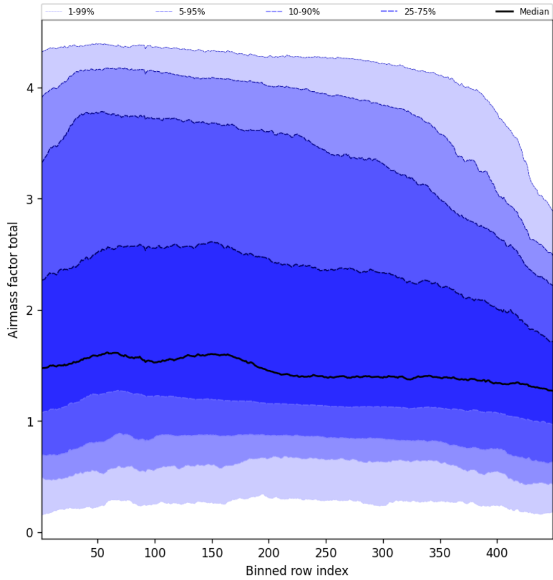
Figure 52: Along track statistics of “Airmass factor total” for 2025-02-21 to 2025-02-22
