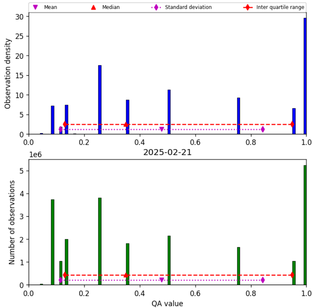
Figure 32: Histogram of “QA value” for 2025-02-21 to 2025-02-22
