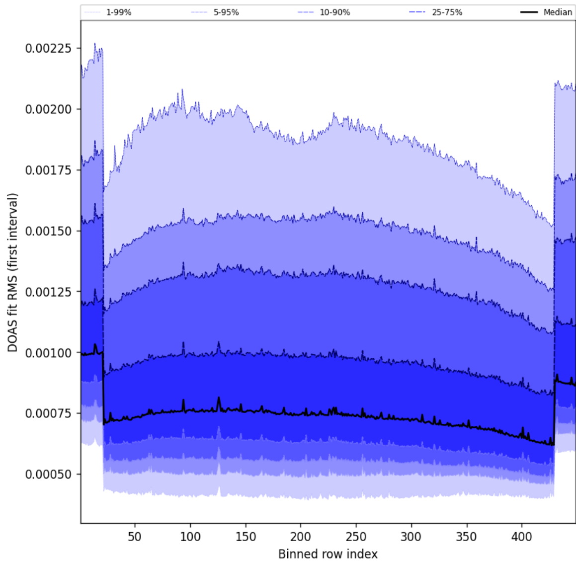
Figure 58: Along track statistics of “DOAS fit RMS (first interval)” for 2025-02-21 to 2025-02-22
