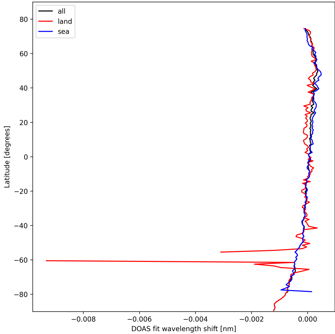
Figure 28: Zonal average of “DOAS fit wavelength shift” for 2025-02-21 to 2025-02-22.
