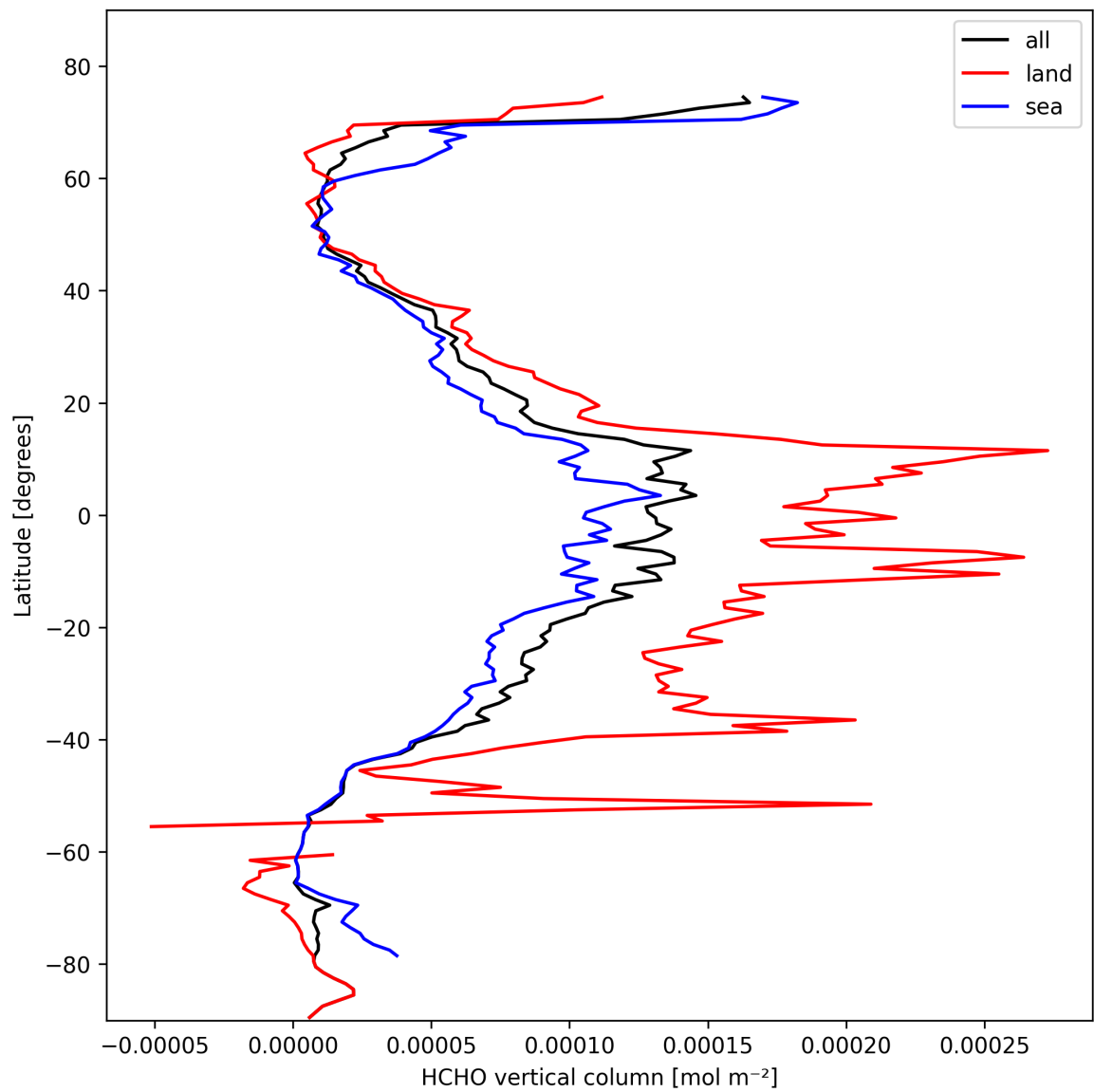
Figure 19: Zonal average of “HCHO vertical column” for 2025-02-21 to 2025-02-22.
