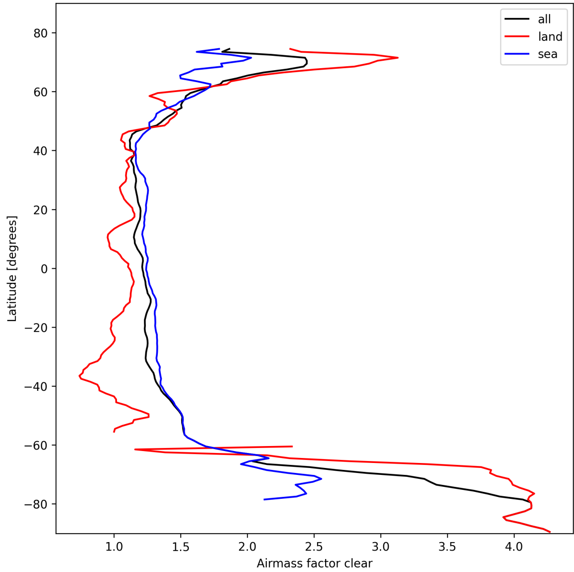
Figure 26: Zonal average of “Airmass factor clear” for 2025-02-21 to 2025-02-22.
