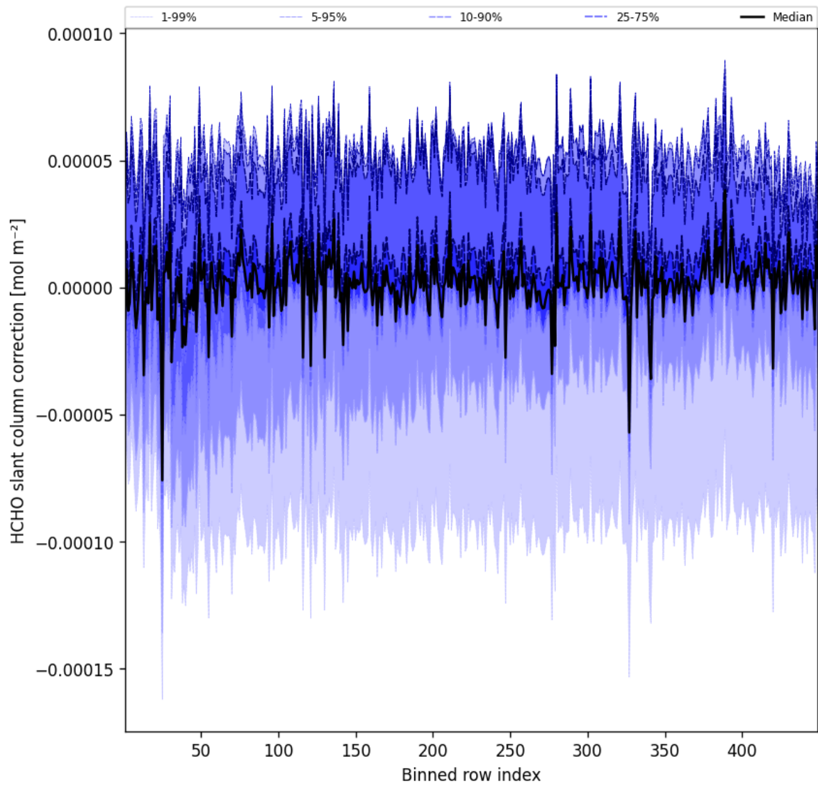
Figure 59: Along track statistics of “HCHO slant column correction” for 2025-02-21 to 2025-02-22
