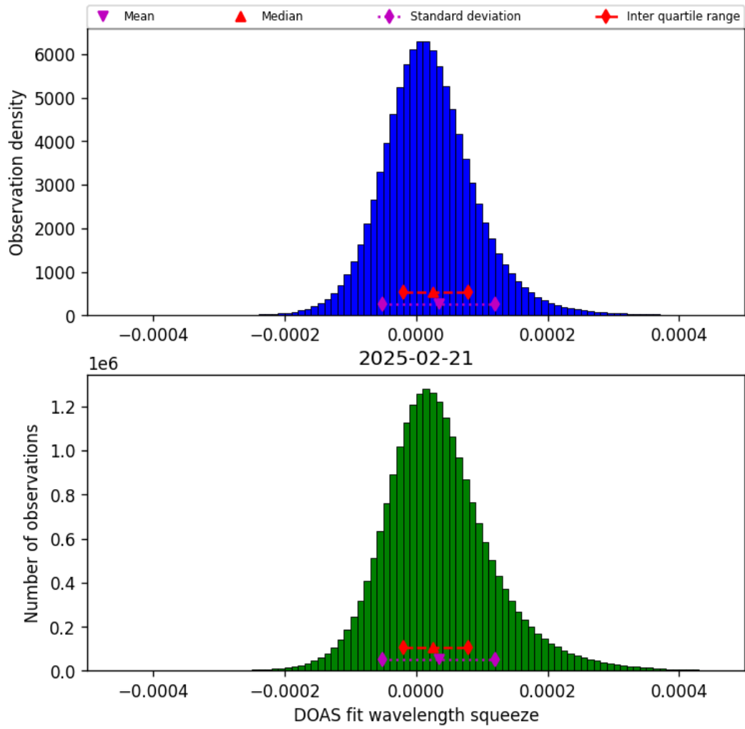
Figure 43: Histogram of “DOAS fit wavelength squeeze” for 2025-02-21 to 2025-02-22
