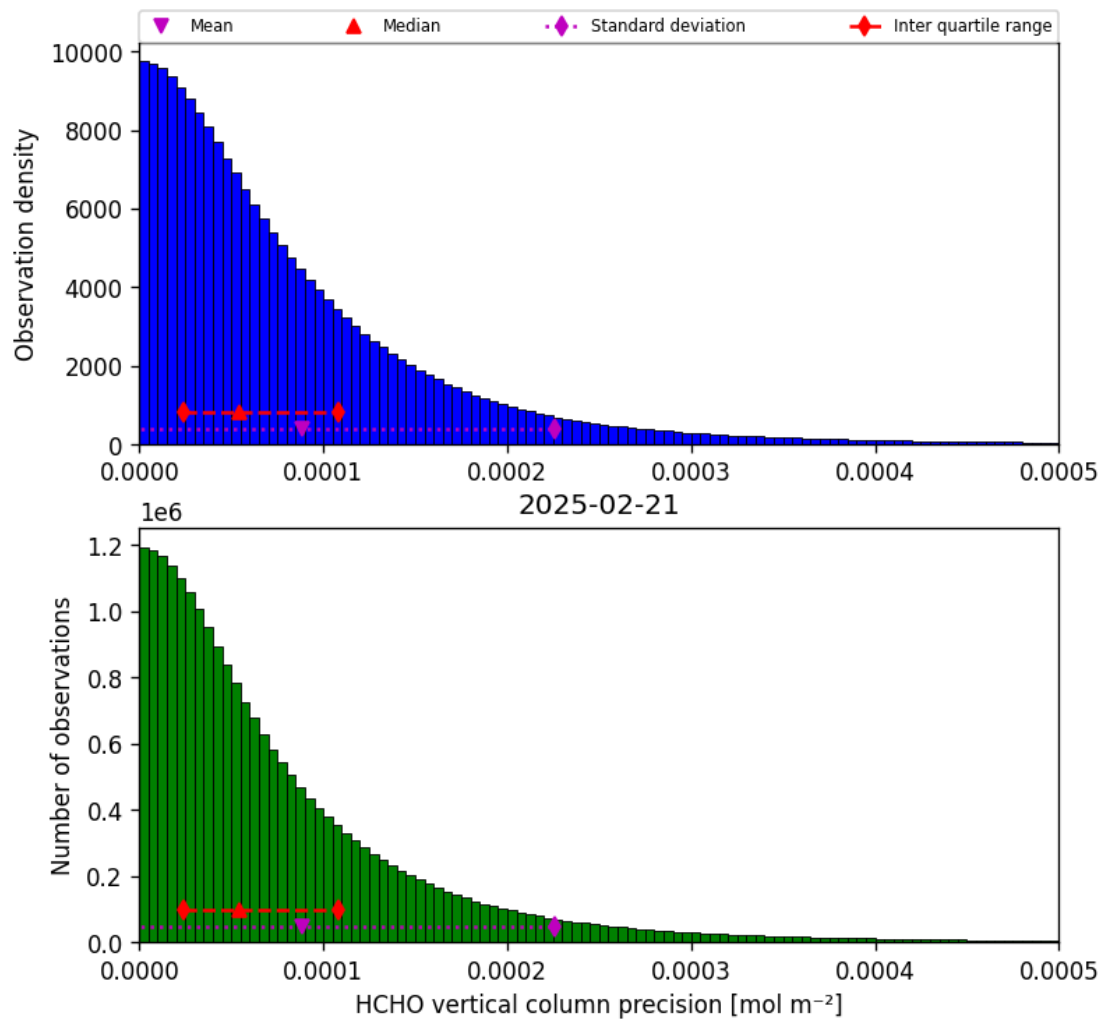
Figure 34: Histogram of “HCHO vertical column precision” for 2025-02-21 to 2025-02-22
