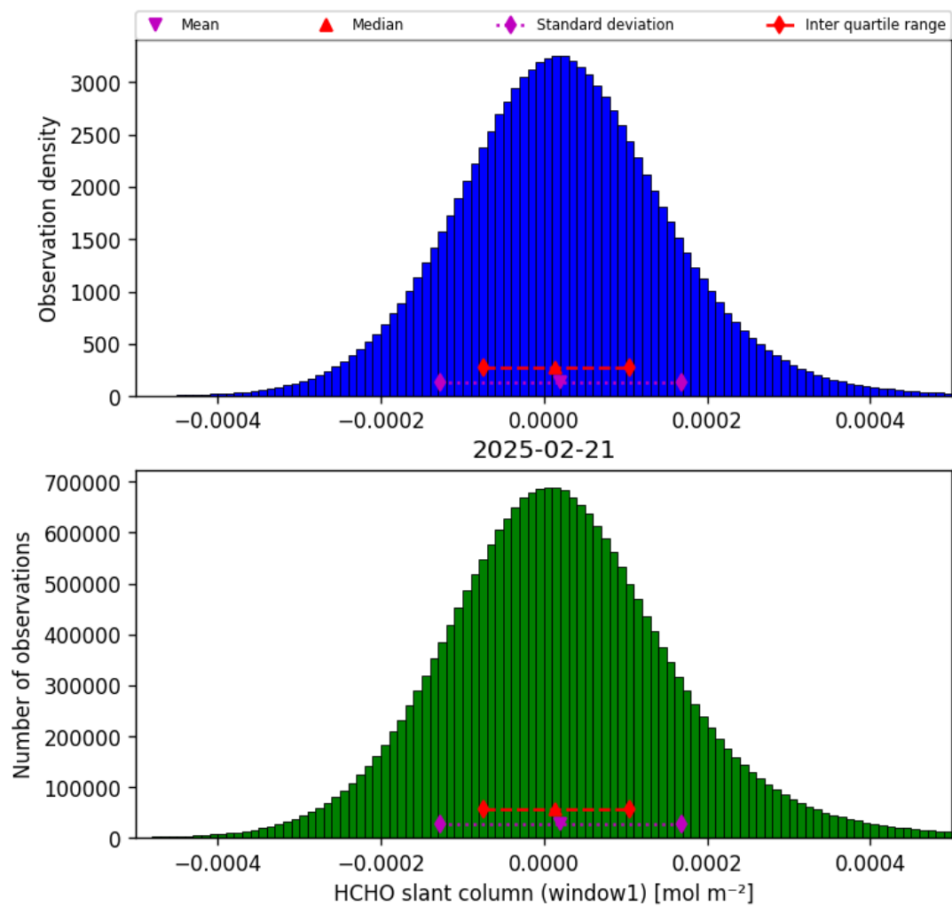
Figure 36: Histogram of “HCHO slant column (window1)” for 2025-02-21 to 2025-02-22
