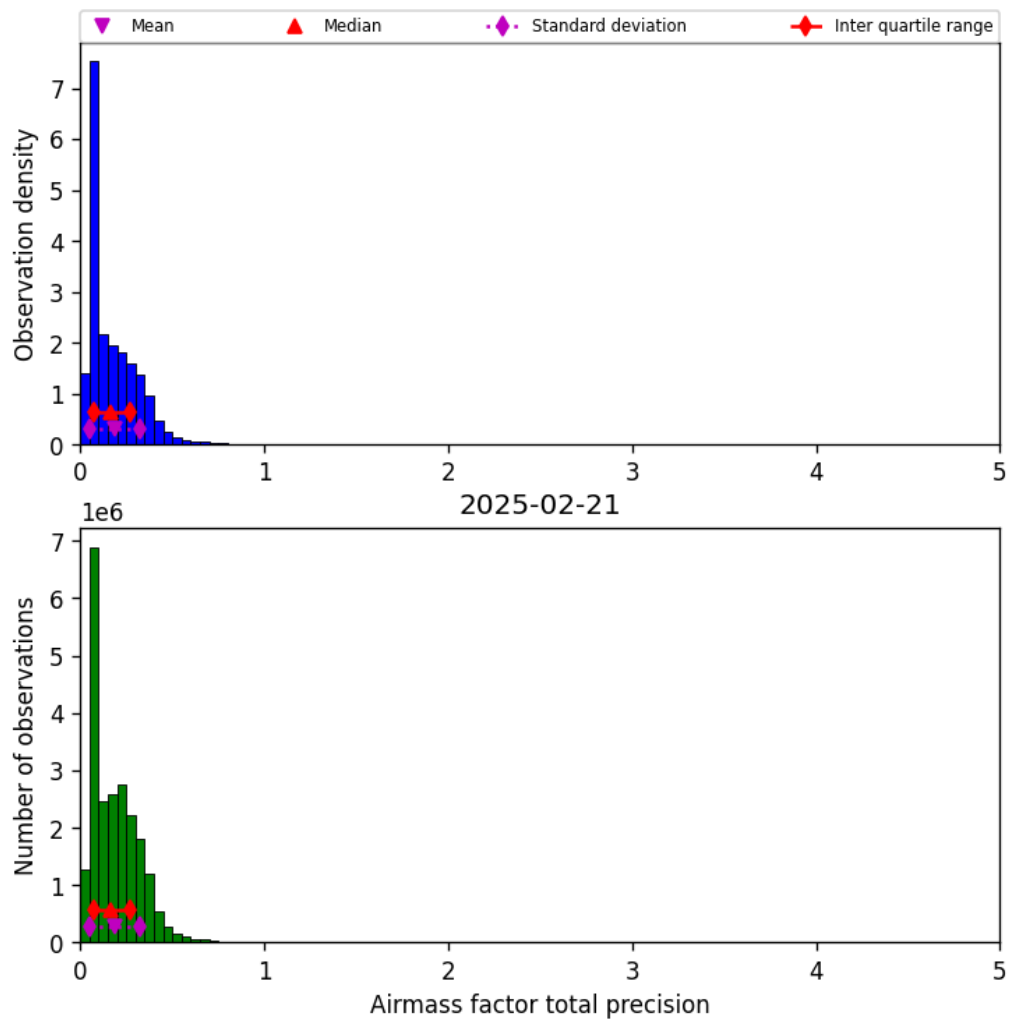
Figure 39: Histogram of “Airmass factor total precision” for 2025-02-21 to 2025-02-22
