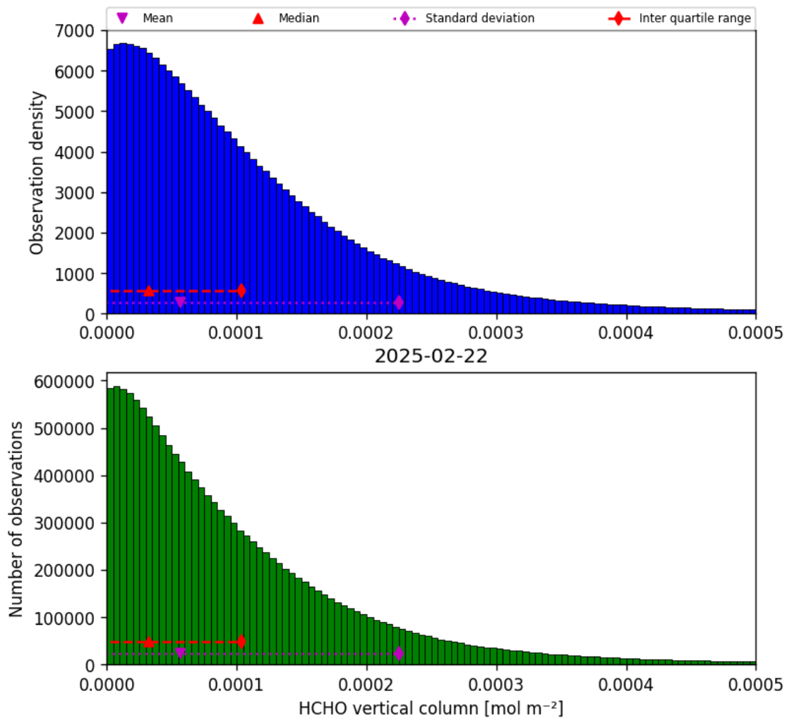
Figure 33: Histogram of “HCHO vertical column” for 2025-02-22 to 2025-02-22
