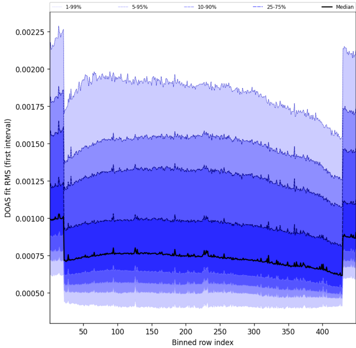
Figure 58: Along track statistics of “DOAS fit RMS (first interval)” for 2025-02-22 to 2025-02-22
