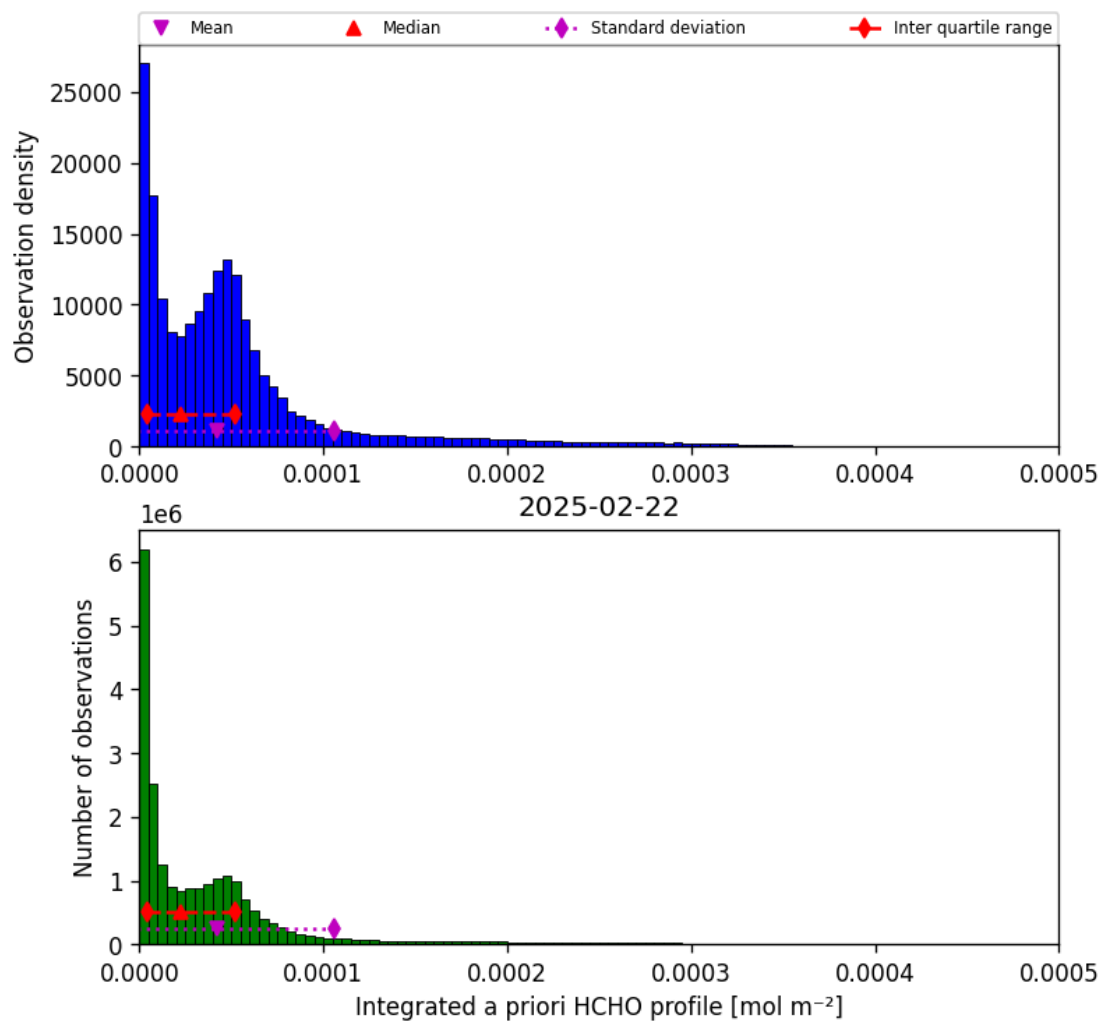
Figure 41: Histogram of “Integrated a priori HCHO profile” for 2025-02-22 to 2025-02-22
