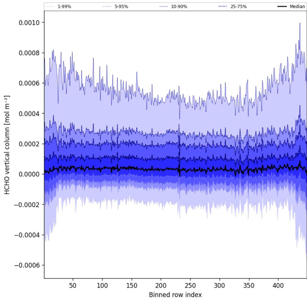
Figure 47: Along track statistics of “HCHO vertical column” for 2025-02-22 to 2025-02-22
