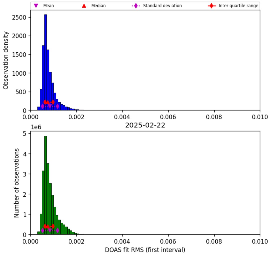
Figure 44: Histogram of “DOAS fit RMS (first interval)” for 2025-02-22 to 2025-02-22
