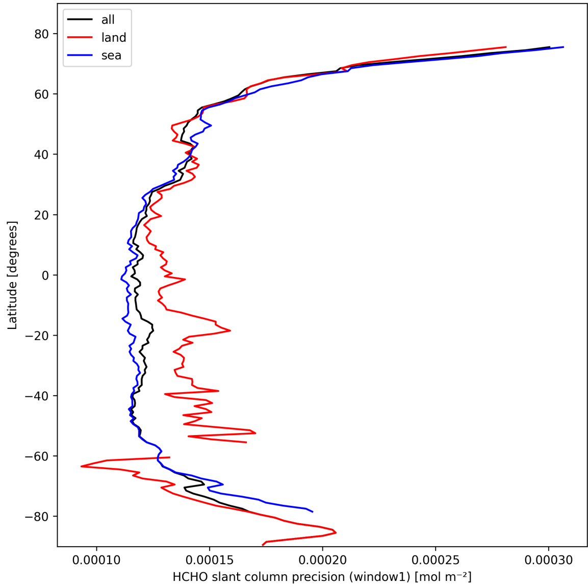
Figure 23: Zonal average of “HCHO slant column precision (window1)” for 2025-02-22 to 2025-02-22.
