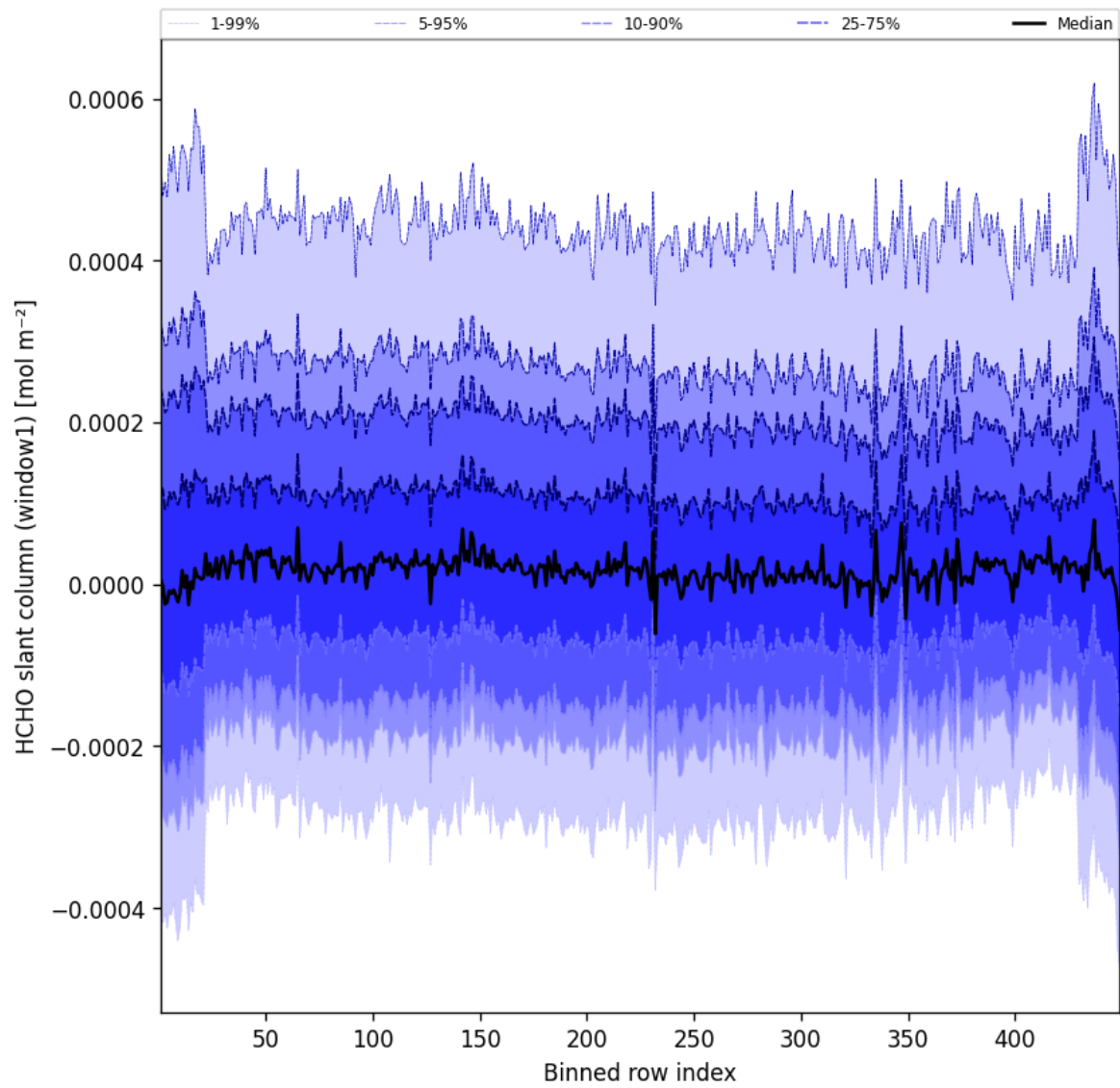
Figure 50: Along track statistics of “HCHO slant column (window1)” for 2025-02-22 to 2025-02-22
