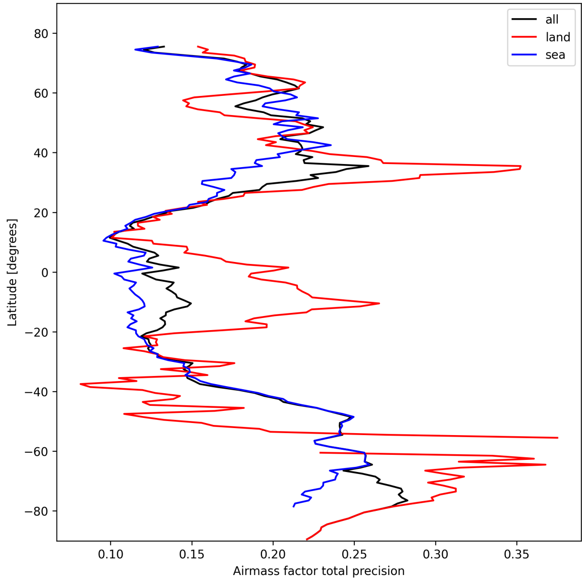
Figure 25: Zonal average of “Airmass factor total precision” for 2025-02-22 to 2025-02-22.
