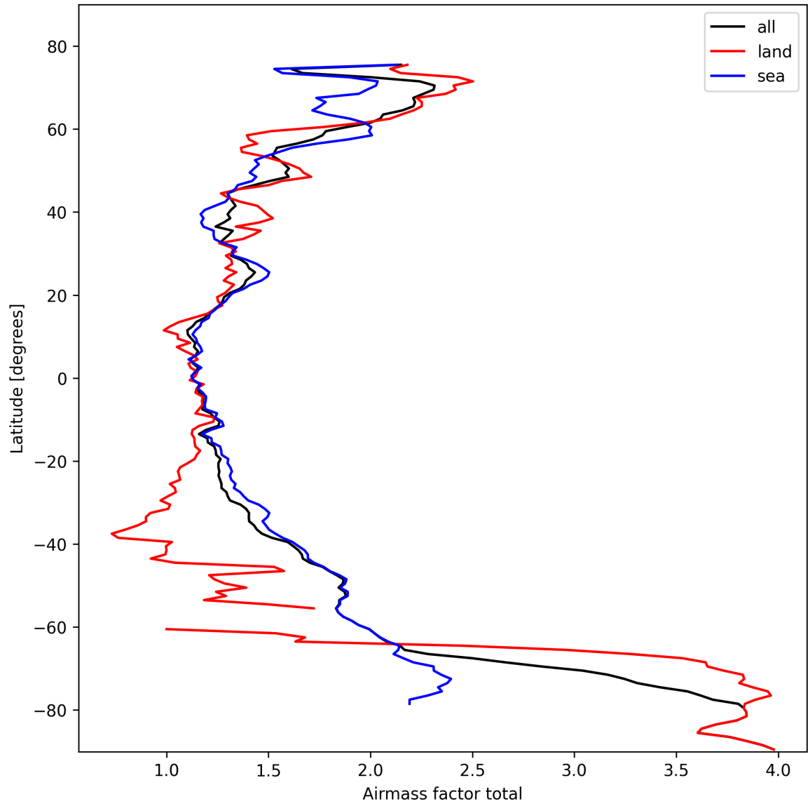
Figure 24: Zonal average of “Airmass factor total” for 2025-02-22 to 2025-02-22.
