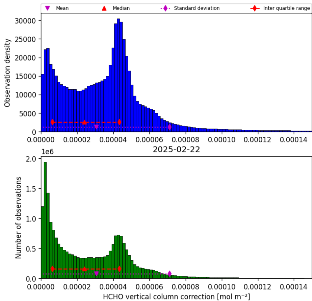
Figure 35: Histogram of “HCHO vertical column correction” for 2025-02-22 to 2025-02-22
