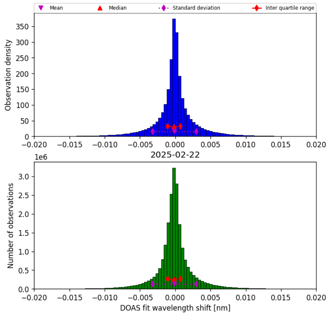
Figure 42: Histogram of “DOAS fit wavelength shift” for 2025-02-22 to 2025-02-22
