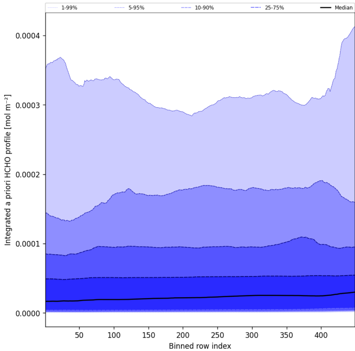
Figure 55: Along track statistics of “Integrated a priori HCHO profile” for 2025-02-22 to 2025-02-22
