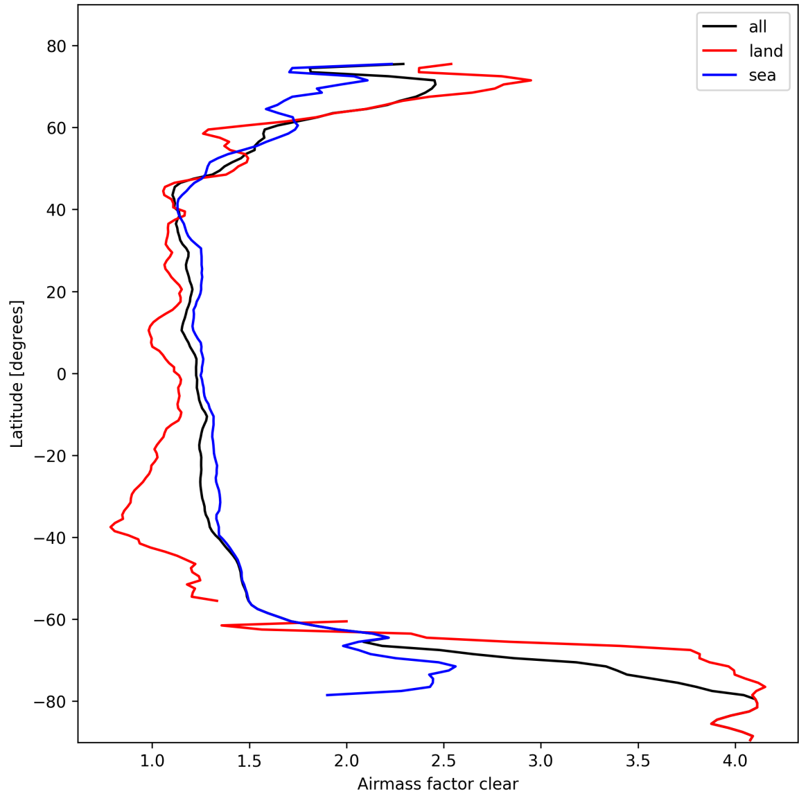
Figure 26: Zonal average of “Airmass factor clear” for 2025-02-22 to 2025-02-22.
