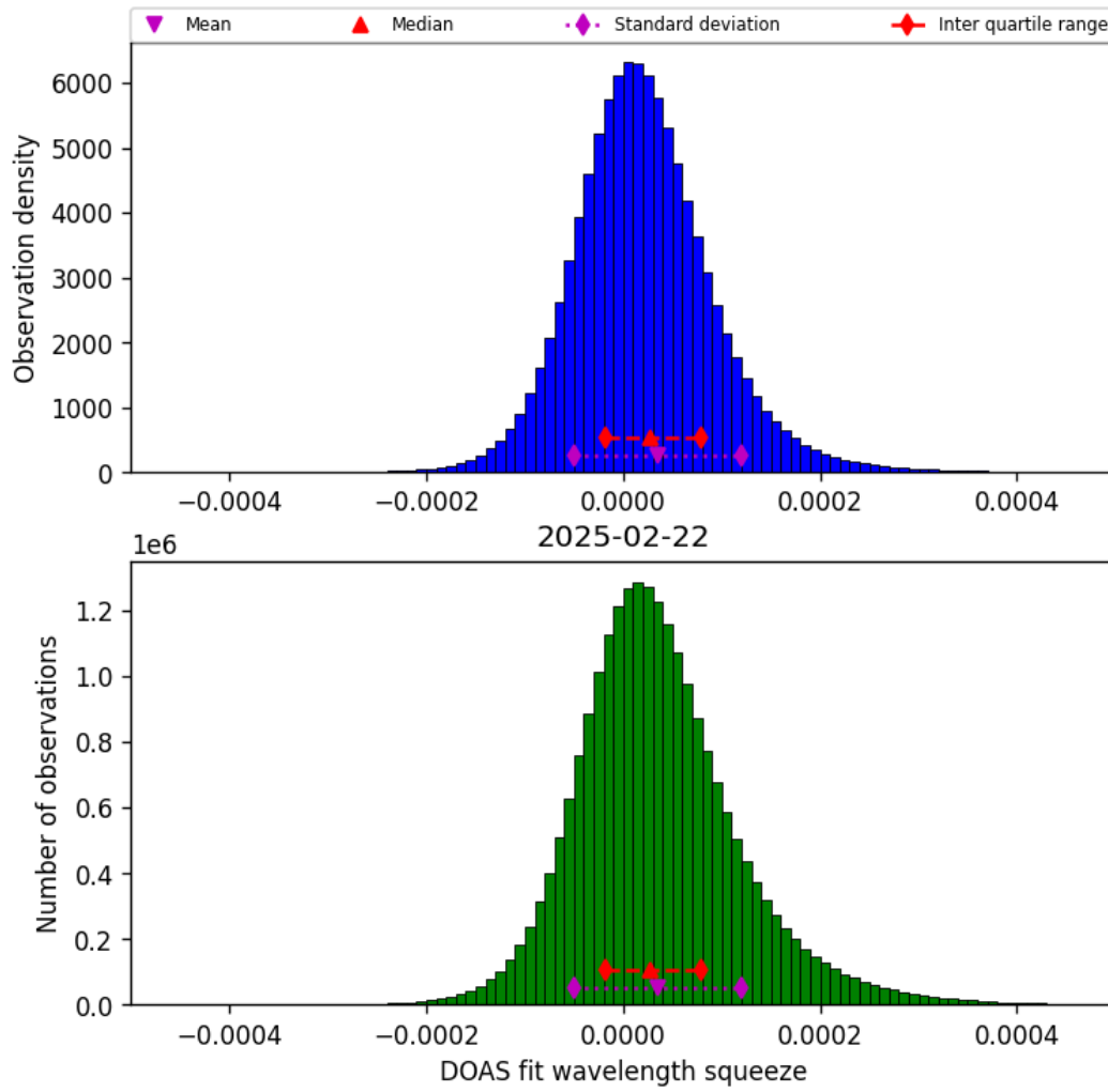
Figure 43: Histogram of “DOAS fit wavelength squeeze” for 2025-02-22 to 2025-02-22
