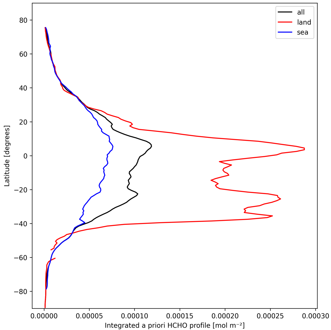
Figure 27: Zonal average of “Integrated a priori HCHO profile” for 2025-02-22 to 2025-02-22.
