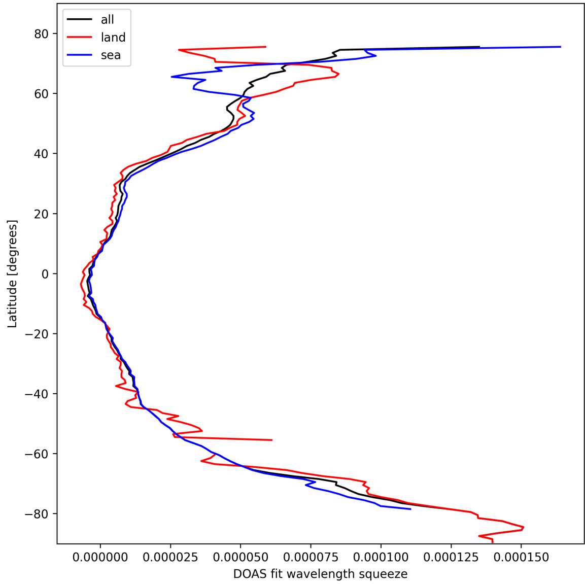
Figure 29: Zonal average of “DOAS fit wavelength squeeze” for 2025-02-22 to 2025-02-22.
