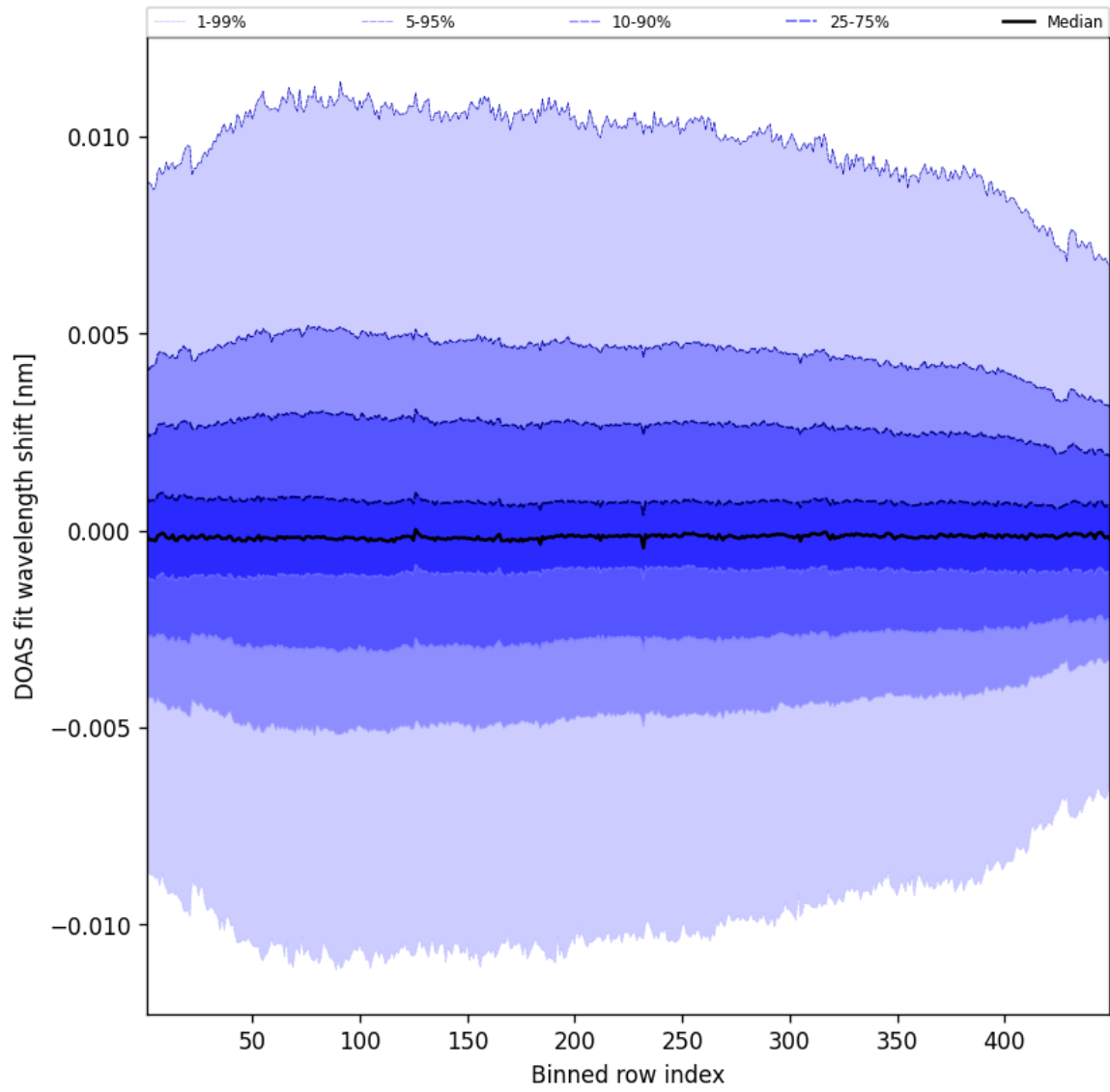
Figure 56: Along track statistics of “DOAS fit wavelength shift” for 2025-02-22 to 2025-02-22
