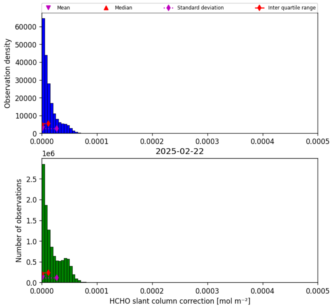
Figure 45: Histogram of “HCHO slant column correction” for 2025-02-22 to 2025-02-22
