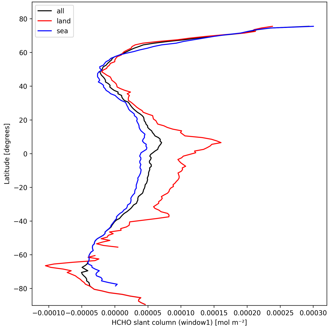
Figure 22: Zonal average of “HCHO slant column (window1)” for 2025-02-22 to 2025-02-22.
