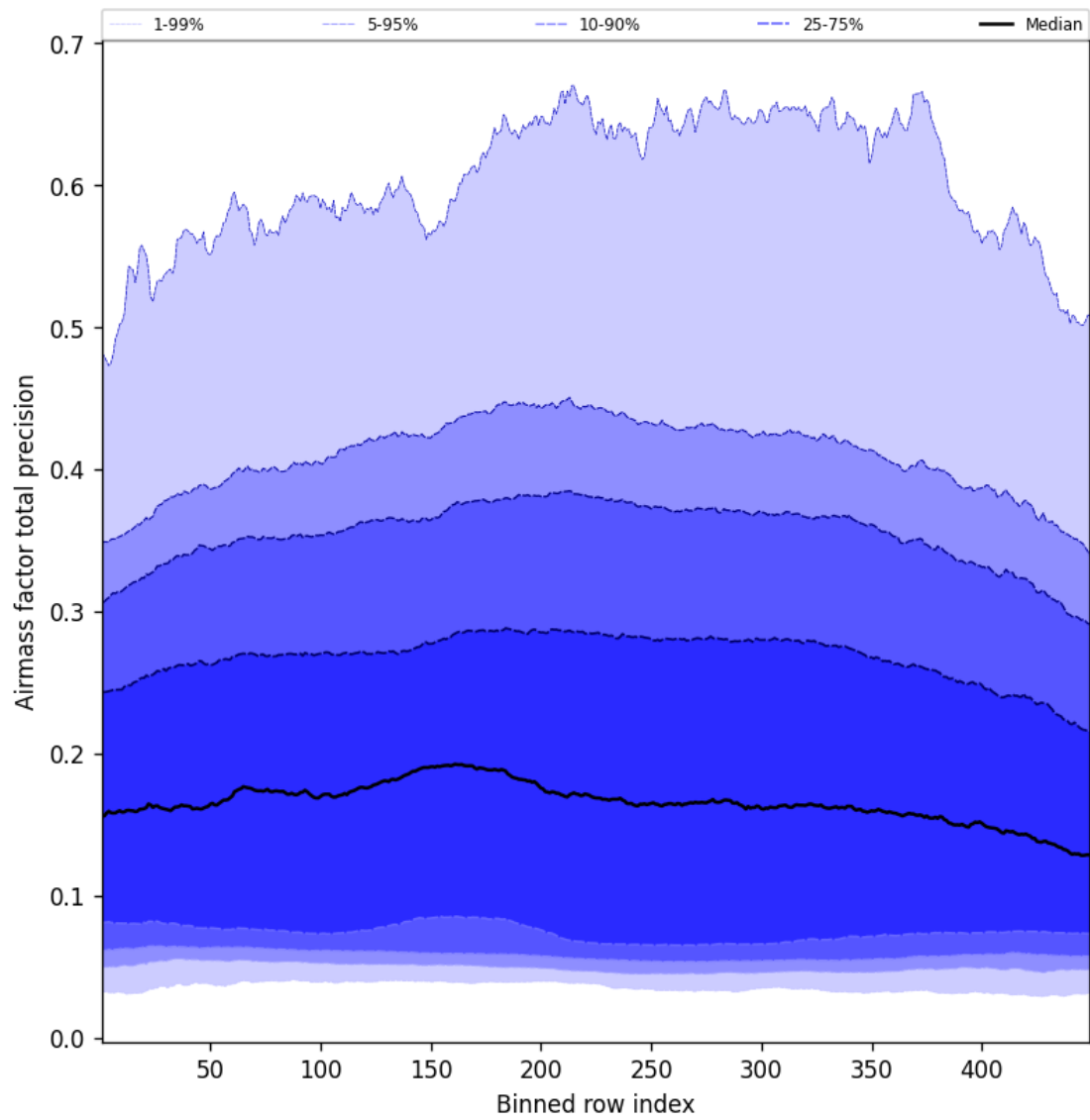
Figure 53: Along track statistics of “Airmass factor total precision” for 2025-02-22 to 2025-02-22
