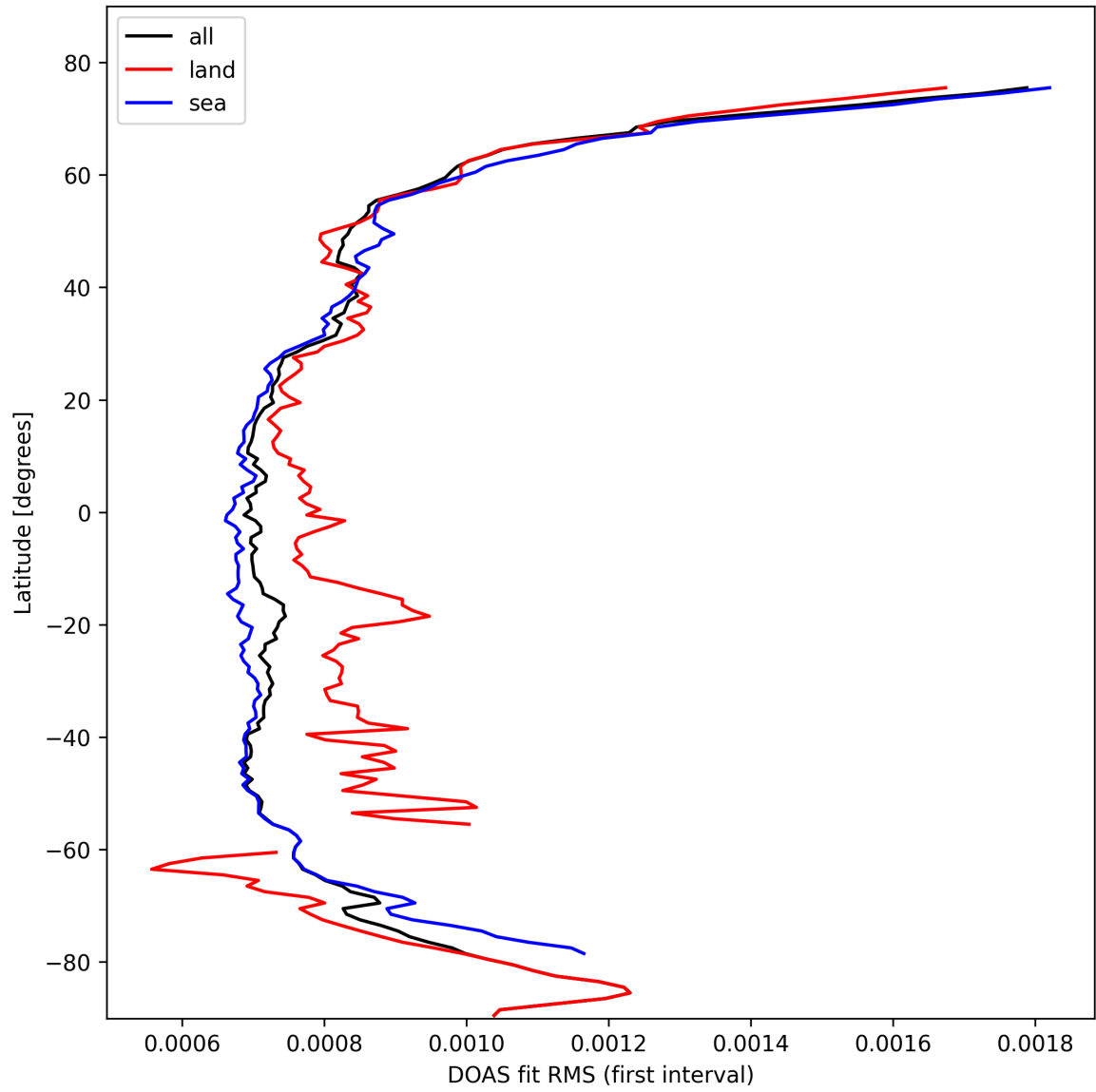
Figure 30: Zonal average of “DOAS fit RMS (first interval)” for 2025-02-22 to 2025-02-22.
