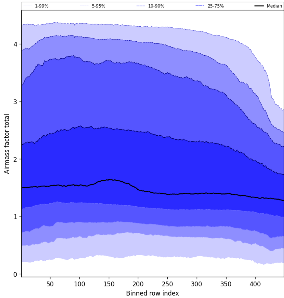
Figure 52: Along track statistics of “Airmass factor total” for 2025-02-22 to 2025-02-22
