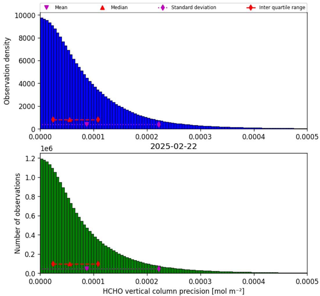
Figure 34: Histogram of “HCHO vertical column precision” for 2025-02-22 to 2025-02-22
