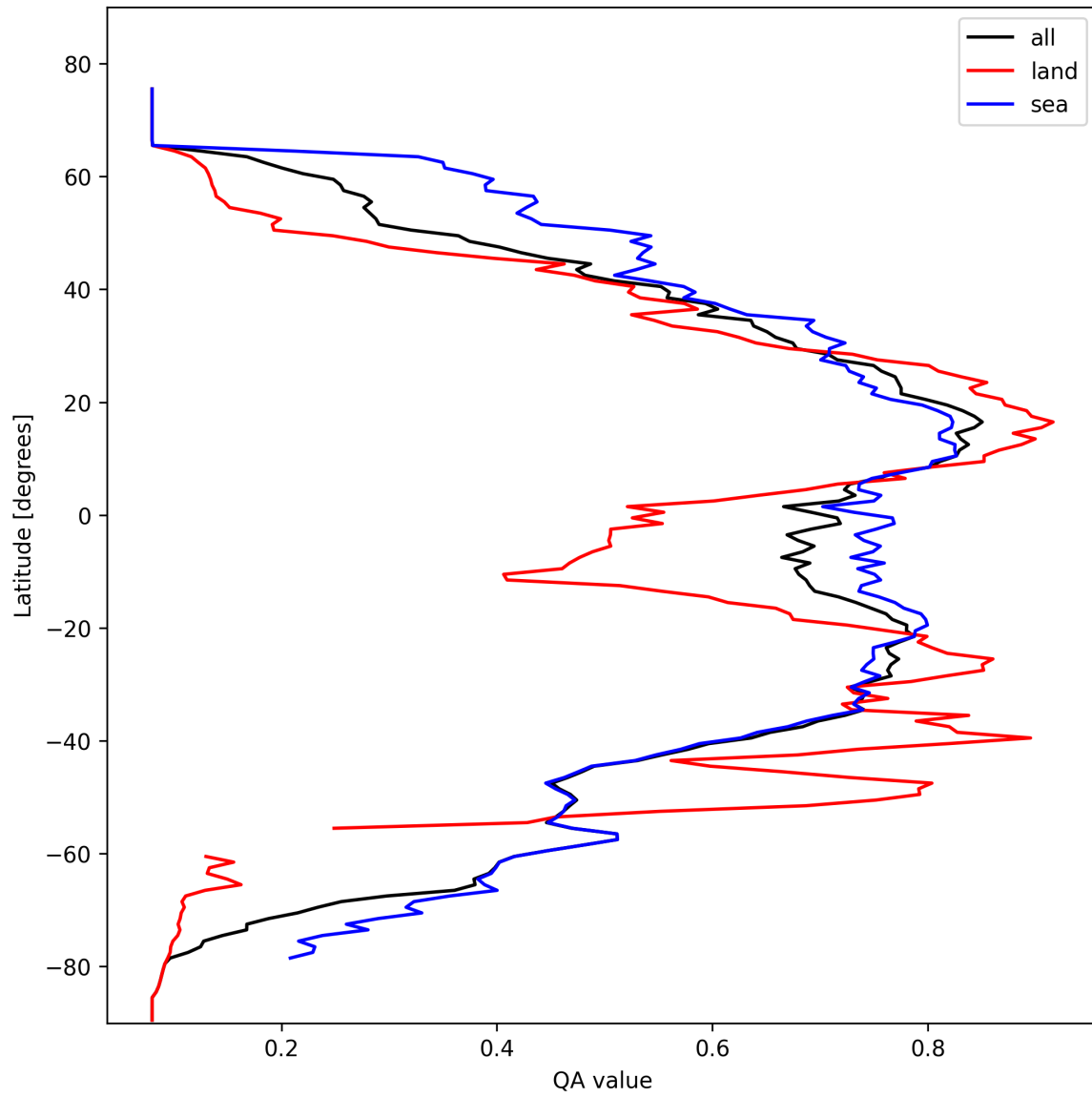
Figure 18: Zonal average of “QA value” for 2025-02-22 to 2025-02-22.
