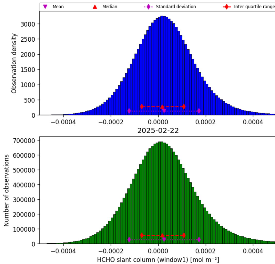
Figure 36: Histogram of “HCHO slant column (window1)” for 2025-02-22 to 2025-02-22
