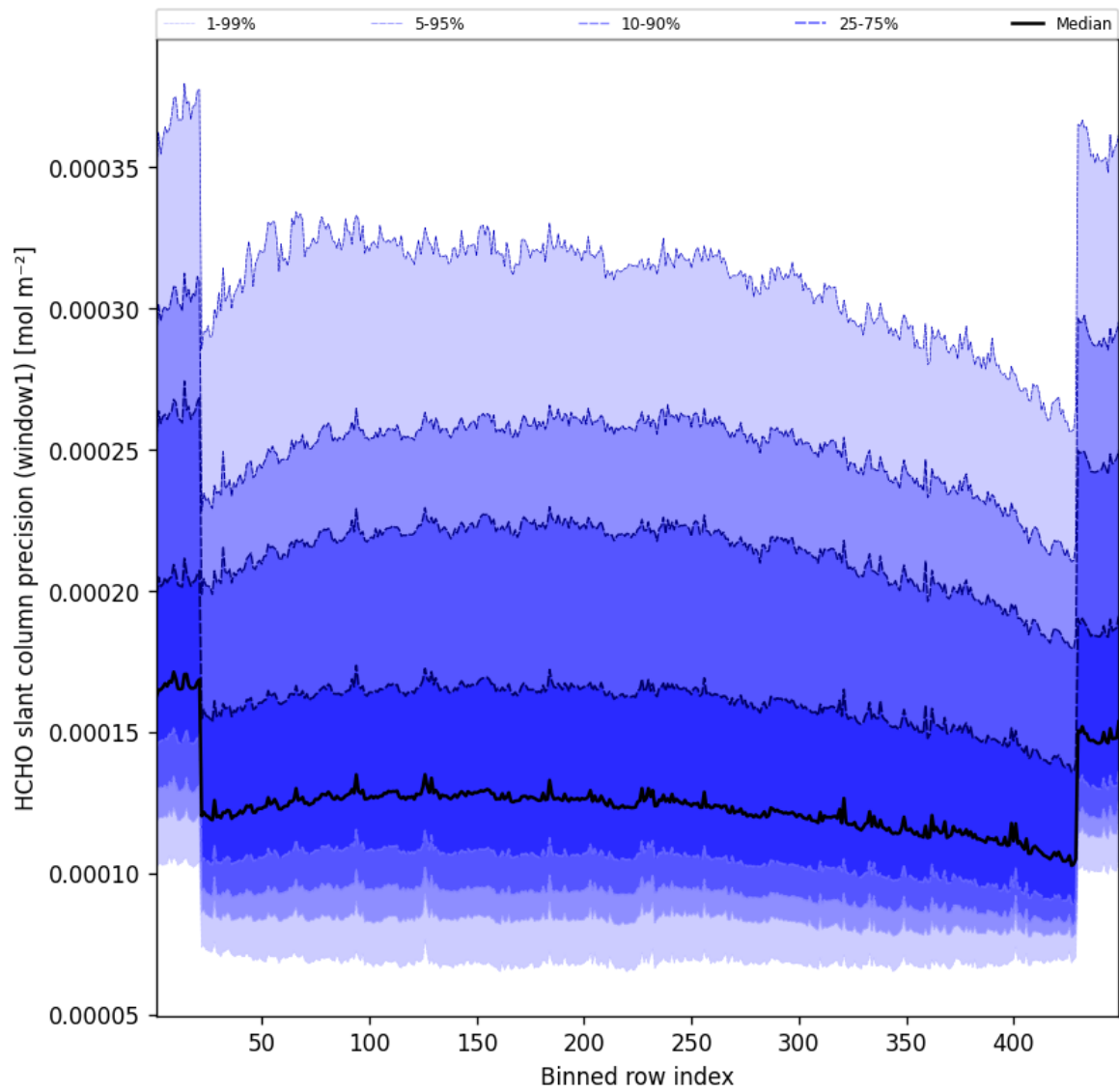
Figure 51: Along track statistics of “HCHO slant column precision (window1)” for 2025-02-22 to 2025-02-22
