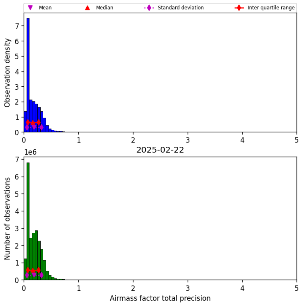
Figure 39: Histogram of “Airmass factor total precision” for 2025-02-22 to 2025-02-22
