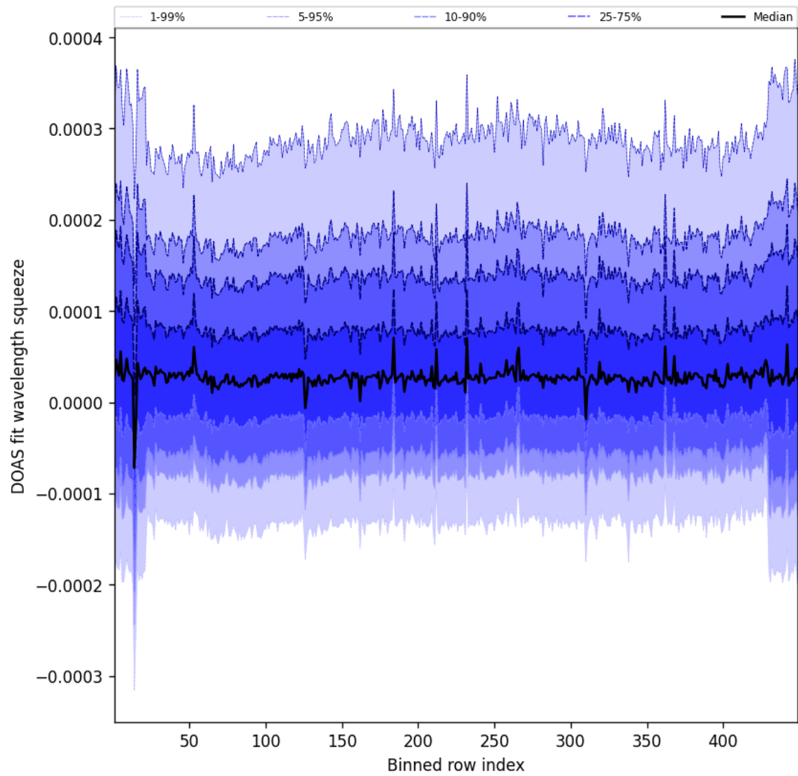
Figure 57: Along track statistics of “DOAS fit wavelength squeeze” for 2025-02-22 to 2025-02-22
