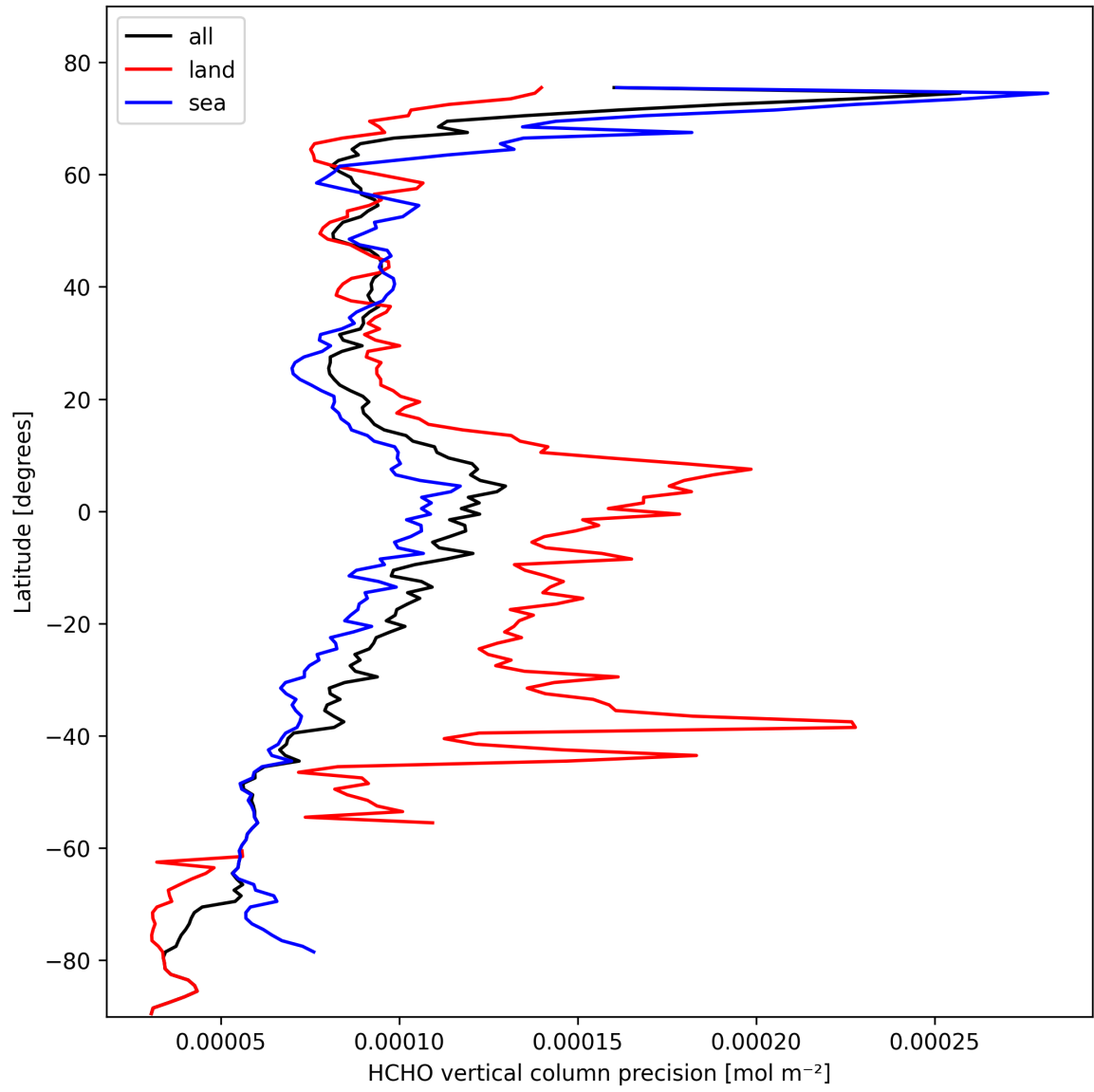
Figure 20: Zonal average of “HCHO vertical column precision” for 2025-02-22 to 2025-02-22.
