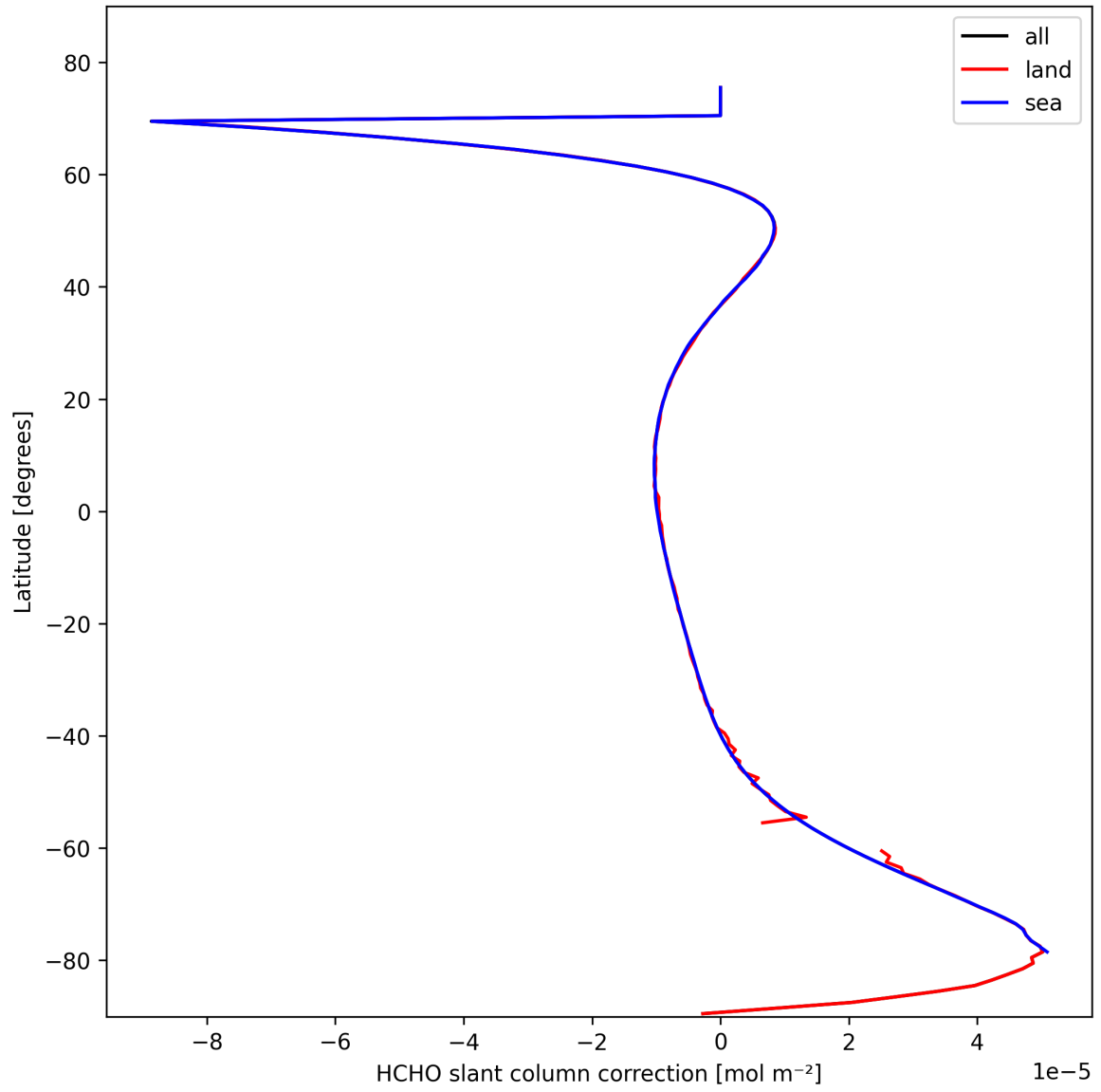
Figure 31: Zonal average of “HCHO slant column correction” for 2025-02-22 to 2025-02-22.
