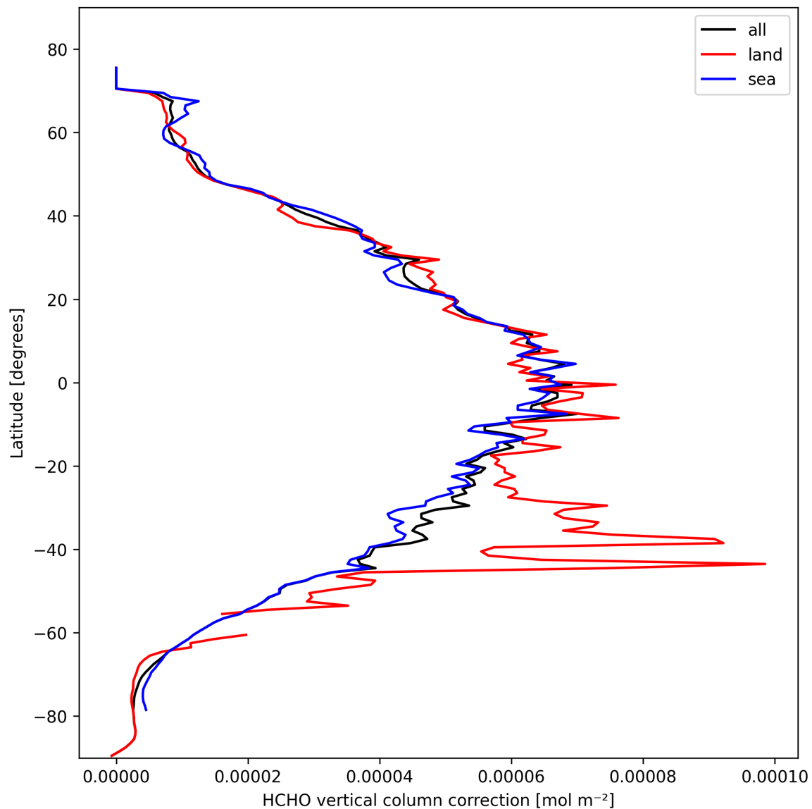
Figure 21: Zonal average of “HCHO vertical column correction” for 2025-02-22 to 2025-02-22.
