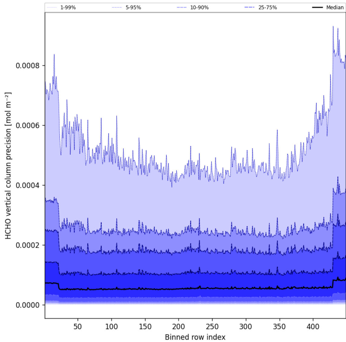
Figure 48: Along track statistics of “HCHO vertical column precision” for 2025-02-22 to 2025-02-22
