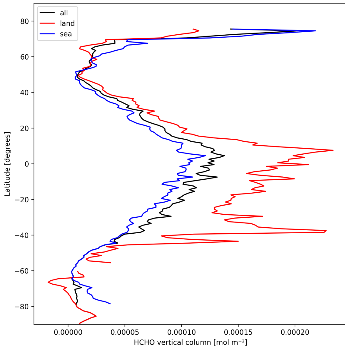
Figure 19: Zonal average of “HCHO vertical column” for 2025-02-22 to 2025-02-22.
