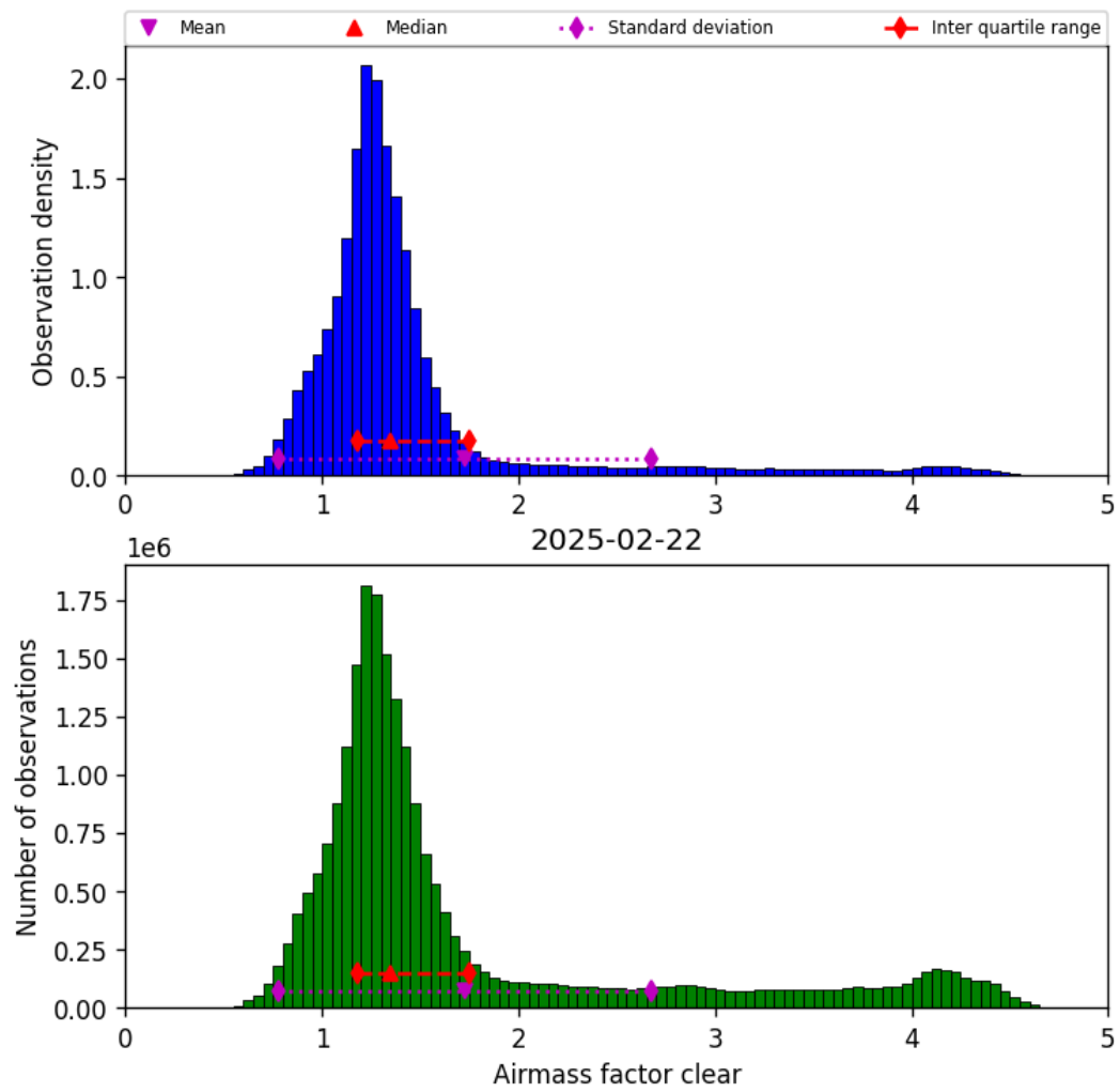
Figure 40: Histogram of “Airmass factor clear” for 2025-02-22 to 2025-02-22
