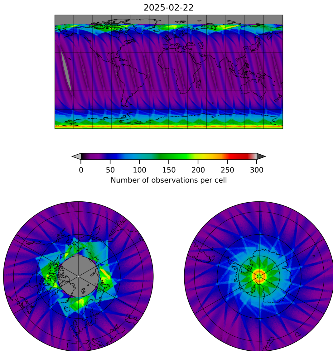
Figure 17: Map of the number of observations for 2025-02-22 to 2025-02-22
