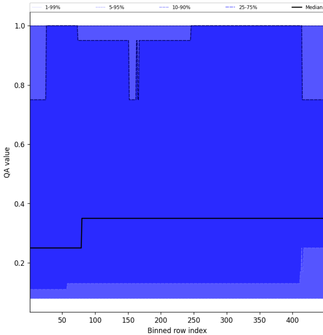
Figure 46: Along track statistics of “QA value” for 2025-02-22 to 2025-02-22
