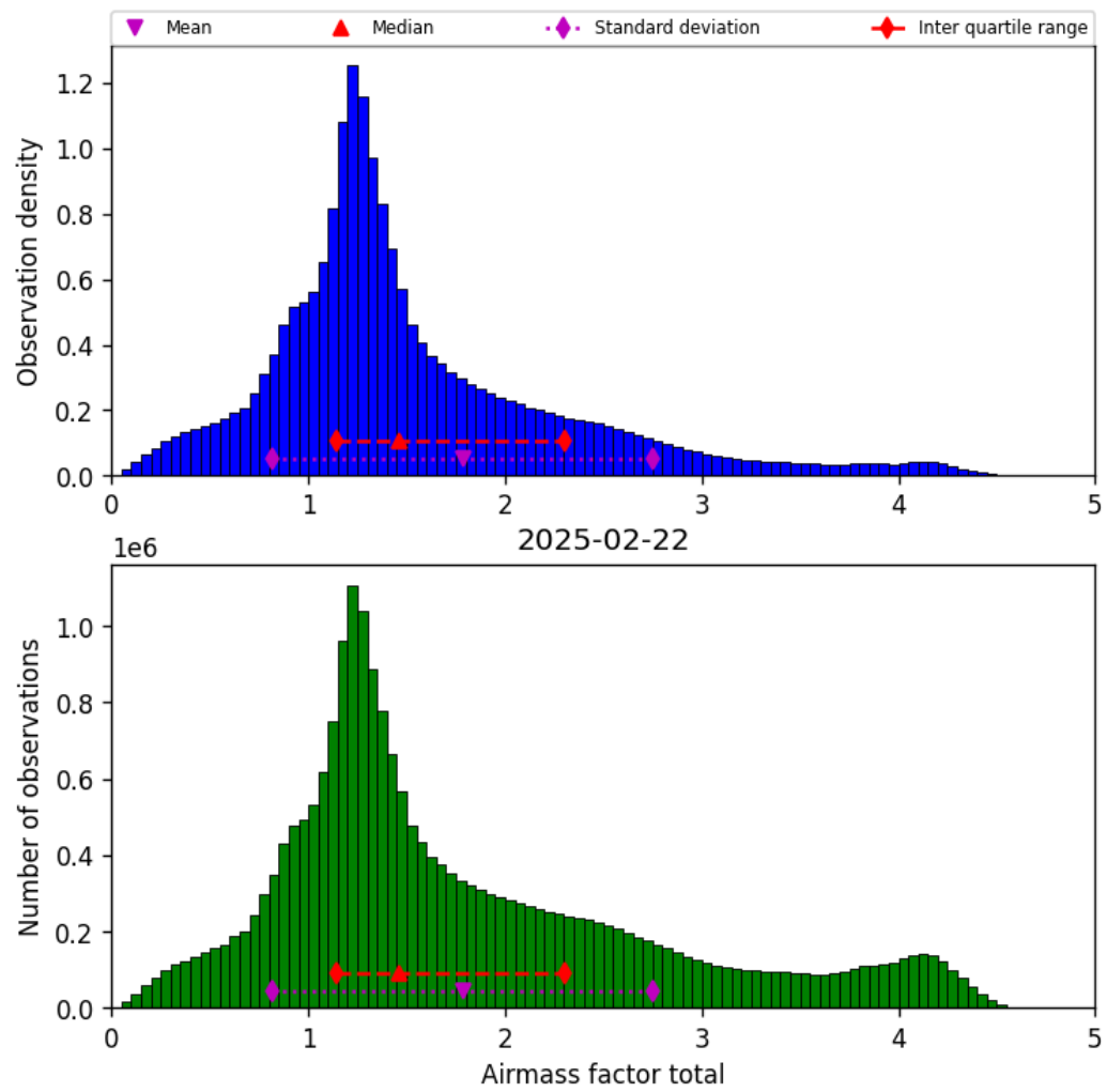
Figure 38: Histogram of “Airmass factor total” for 2025-02-22 to 2025-02-22
