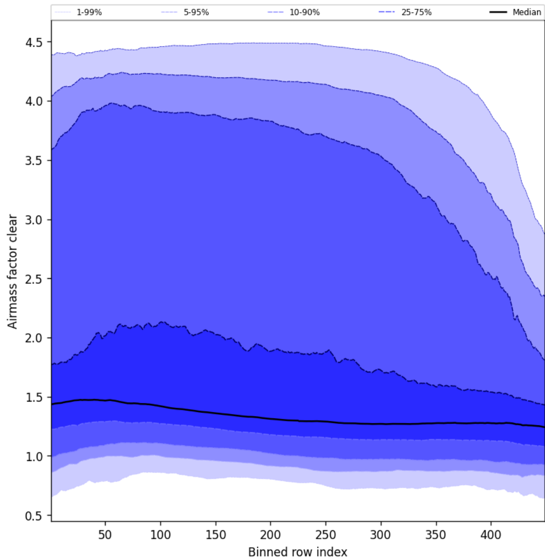
Figure 54: Along track statistics of “Airmass factor clear” for 2025-02-22 to 2025-02-22
