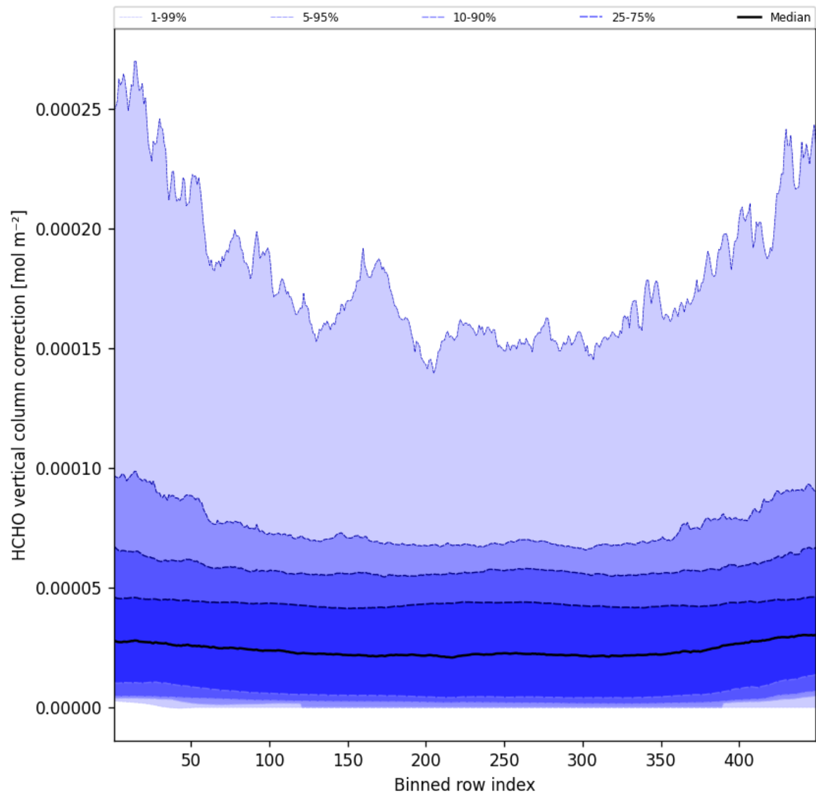
Figure 49: Along track statistics of “HCHO vertical column correction” for 2025-02-22 to 2025-02-22
