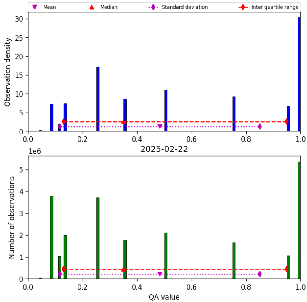
Figure 32: Histogram of “QA value” for 2025-02-22 to 2025-02-22
