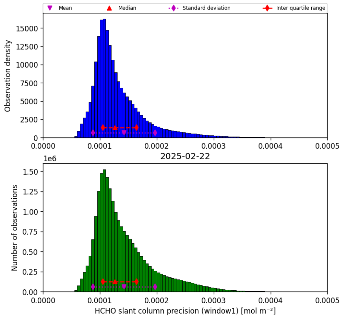
Figure 37: Histogram of “HCHO slant column precision (window1)” for 2025-02-22 to 2025-02-22
