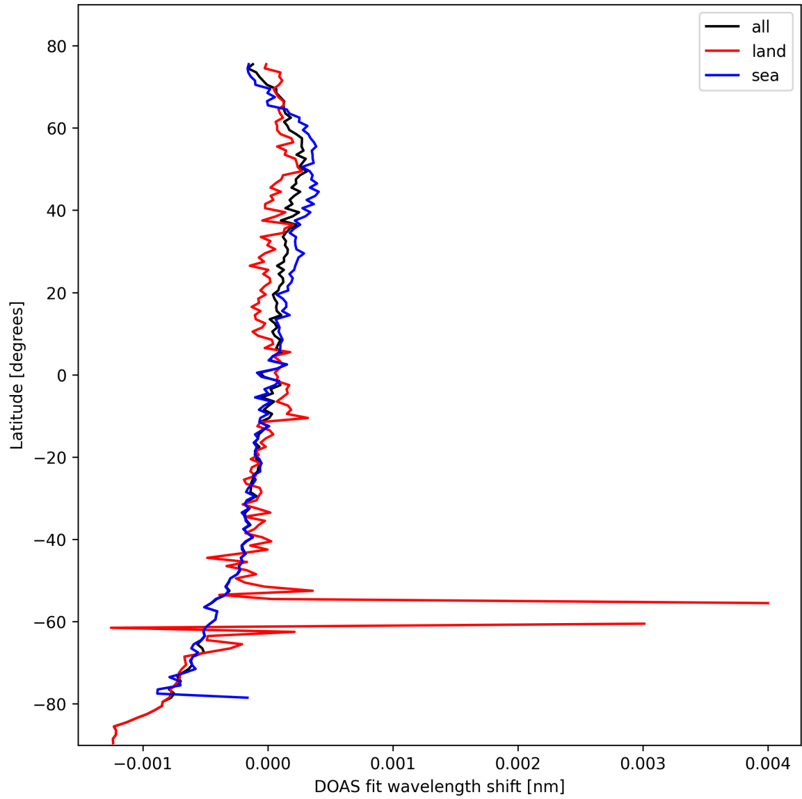
Figure 28: Zonal average of "DOAS fit wavelength shift" for 2025-02-22 to 2025-02-22.
