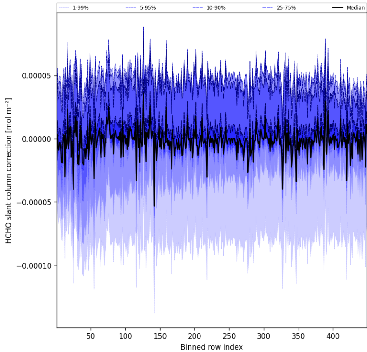
Figure 59: Along track statistics of “HCHO slant column correction” for 2025-02-22 to 2025-02-22
