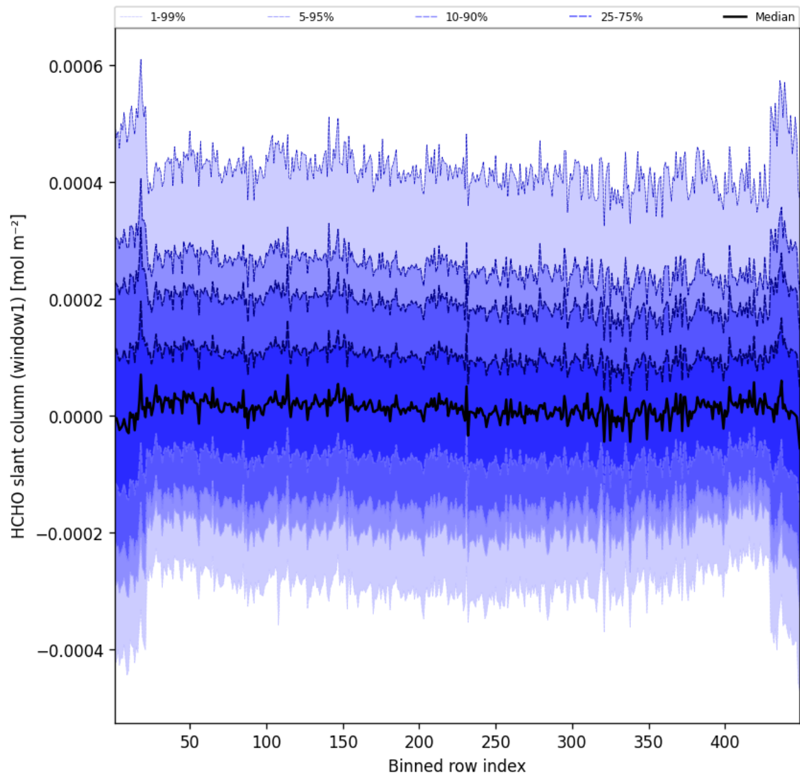
Figure 50: Along track statistics of “HCHO slant column (window1)” for 2025-02-23 to 2025-02-24
