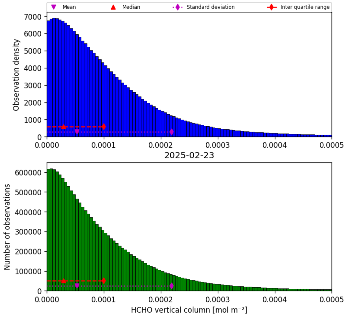
Figure 33: Histogram of “HCHO vertical column” for 2025-02-23 to 2025-02-24
