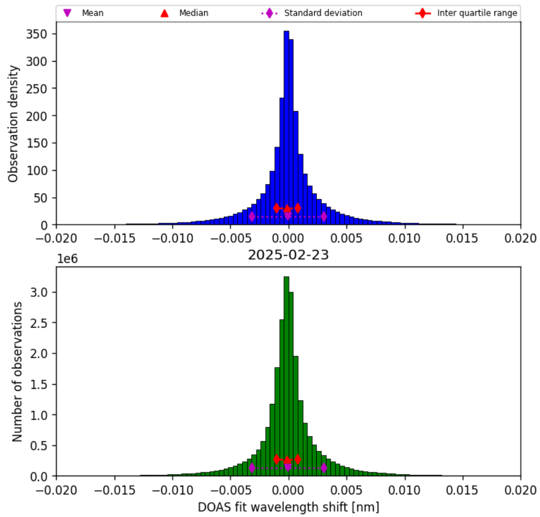
Figure 42: Histogram of “DOAS fit wavelength shift” for 2025-02-23 to 2025-02-24
