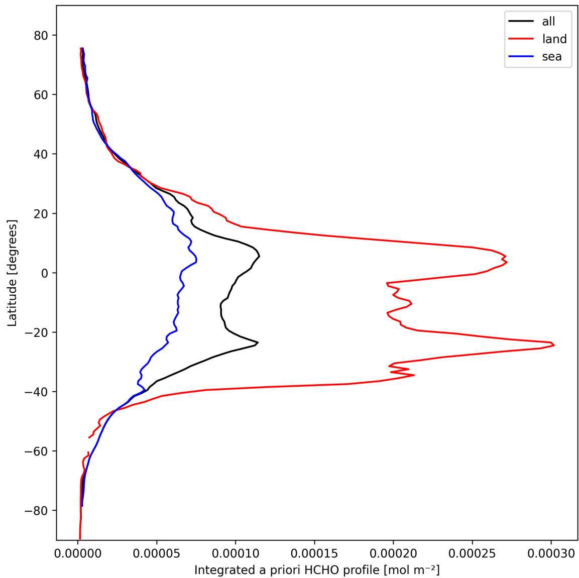
Figure 27: Zonal average of “Integrated a priori HCHO profile” for 2025-02-23 to 2025-02-24.
