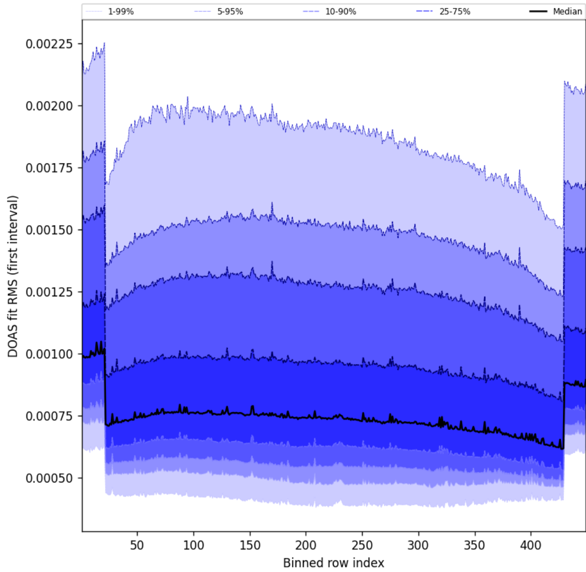
Figure 58: Along track statistics of “DOAS fit RMS (first interval)” for 2025-02-23 to 2025-02-24
