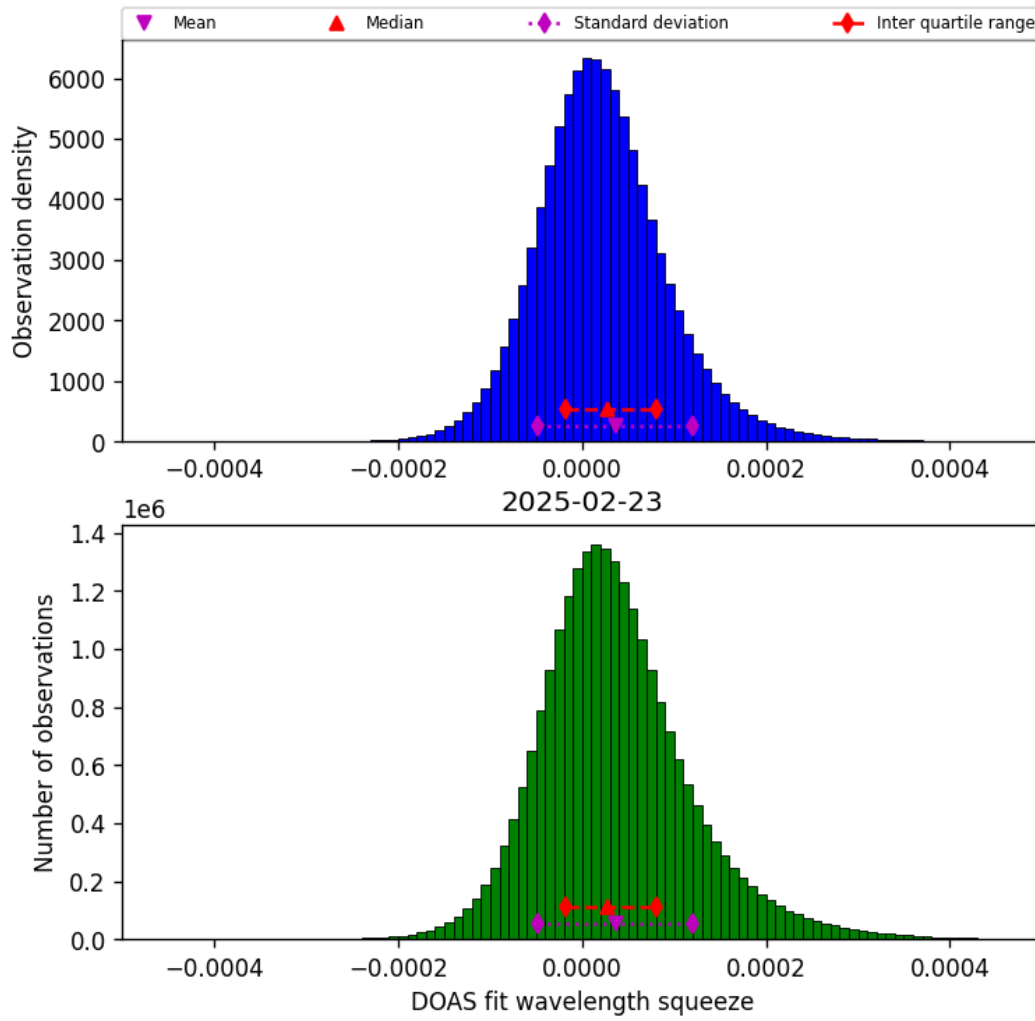
Figure 43: Histogram of “DOAS fit wavelength squeeze” for 2025-02-23 to 2025-02-24
