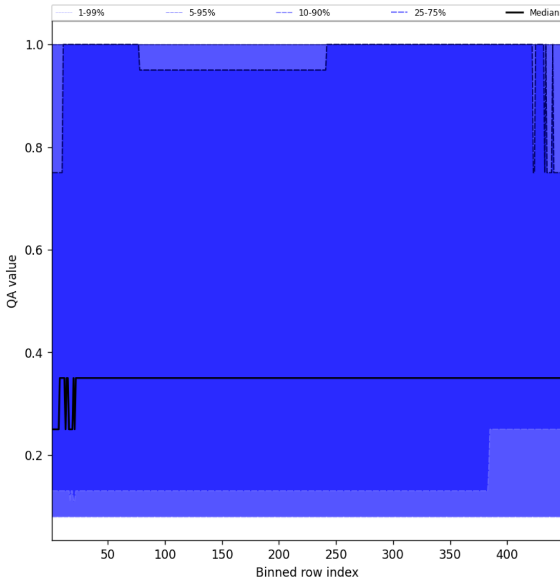
Figure 46: Along track statistics of “QA value” for 2025-02-23 to 2025-02-24
