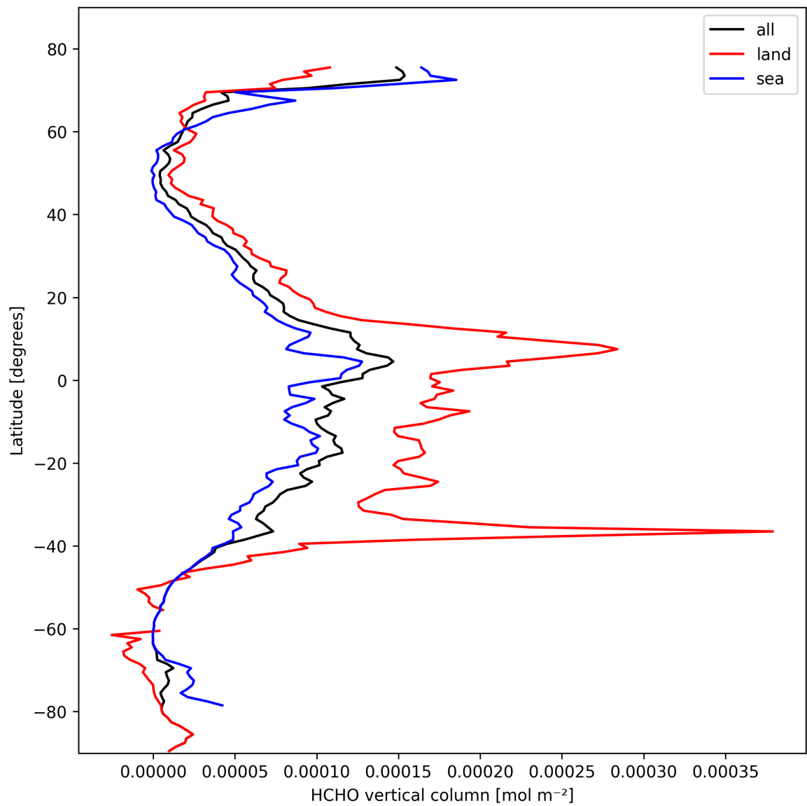
Figure 19: Zonal average of “HCHO vertical column” for 2025-02-23 to 2025-02-24.
