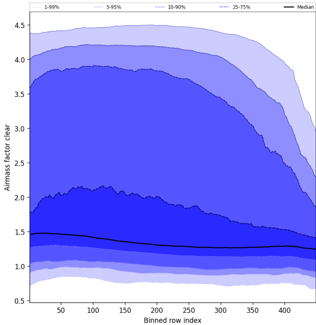
Figure 54: Along track statistics of “Airmass factor clear” for 2025-02-23 to 2025-02-24
