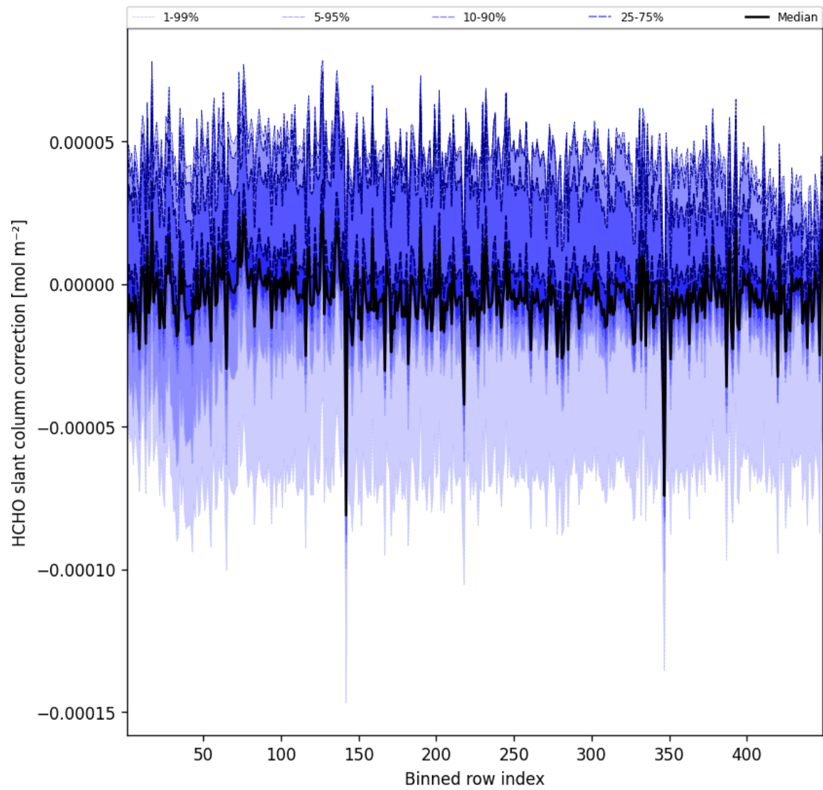
Figure 59: Along track statistics of “HCHO slant column correction” for 2025-02-23 to 2025-02-24
