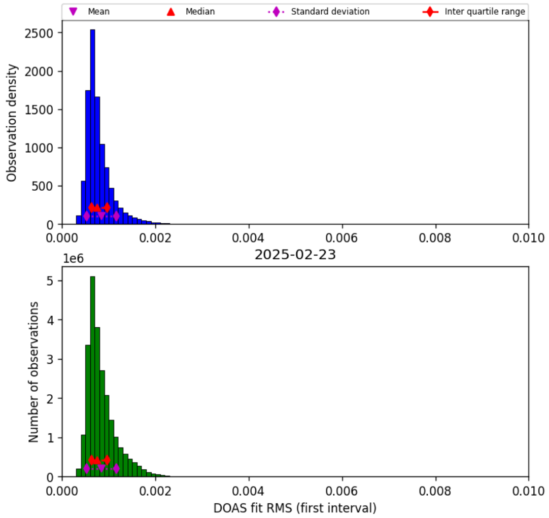
Figure 44: Histogram of “DOAS fit RMS (first interval)” for 2025-02-23 to 2025-02-24
