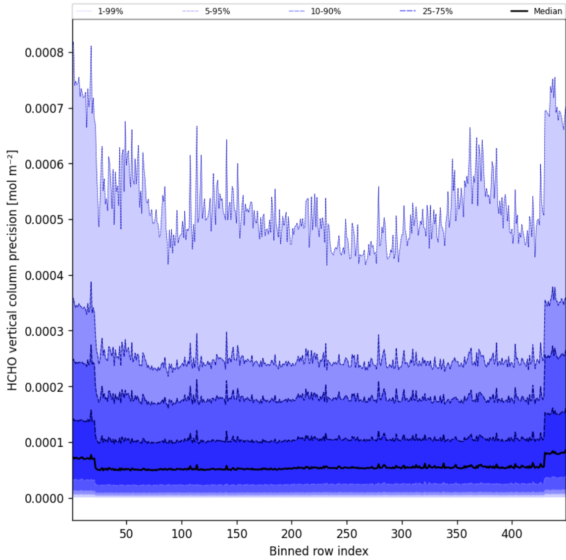
Figure 48: Along track statistics of “HCHO vertical column precision” for 2025-02-23 to 2025-02-24
