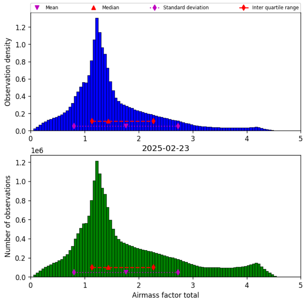
Figure 38: Histogram of “Airmass factor total” for 2025-02-23 to 2025-02-24
