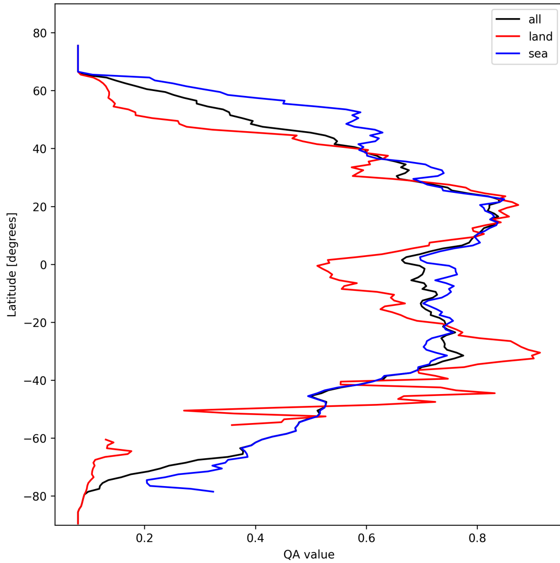
Figure 18: Zonal average of “QA value” for 2025-02-23 to 2025-02-24.
