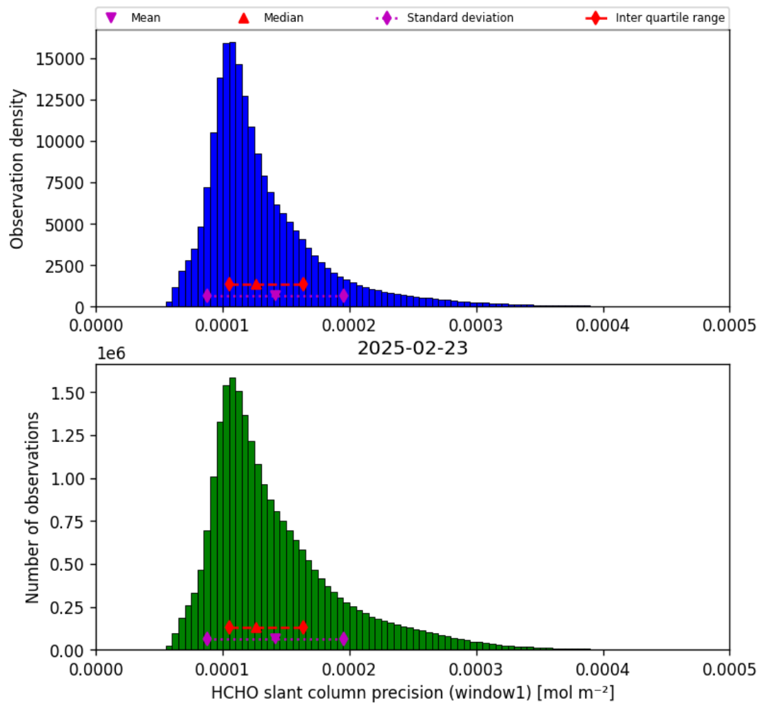
Figure 37: Histogram of “HCHO slant column precision (window1)” for 2025-02-23 to 2025-02-24
