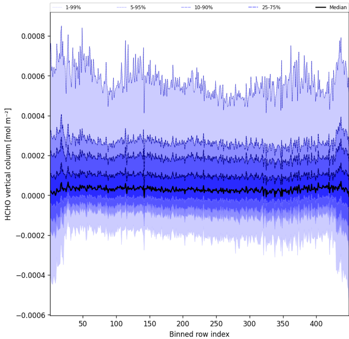
Figure 47: Along track statistics of “HCHO vertical column” for 2025-02-23 to 2025-02-24
