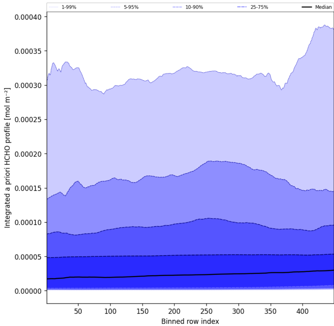
Figure 55: Along track statistics of "Integrated a priori HCHO profile" for 2025-02-23 to 2025-02-24
