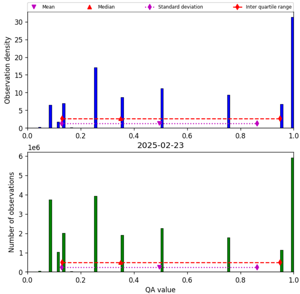
Figure 32: Histogram of “QA value” for 2025-02-23 to 2025-02-24
