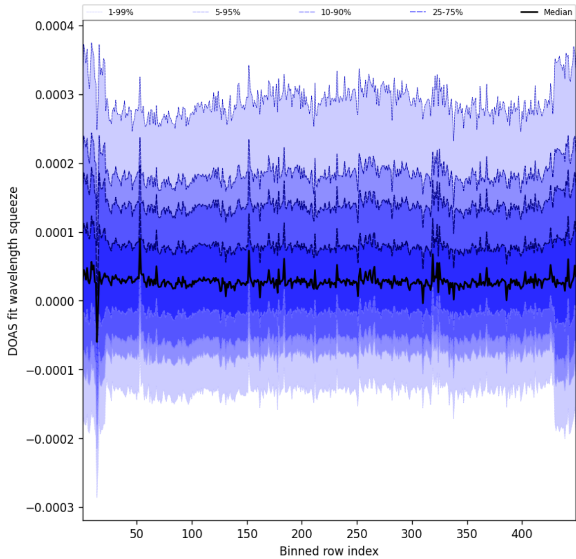
Figure 57: Along track statistics of “DOAS fit wavelength squeeze” for 2025-02-23 to 2025-02-24
