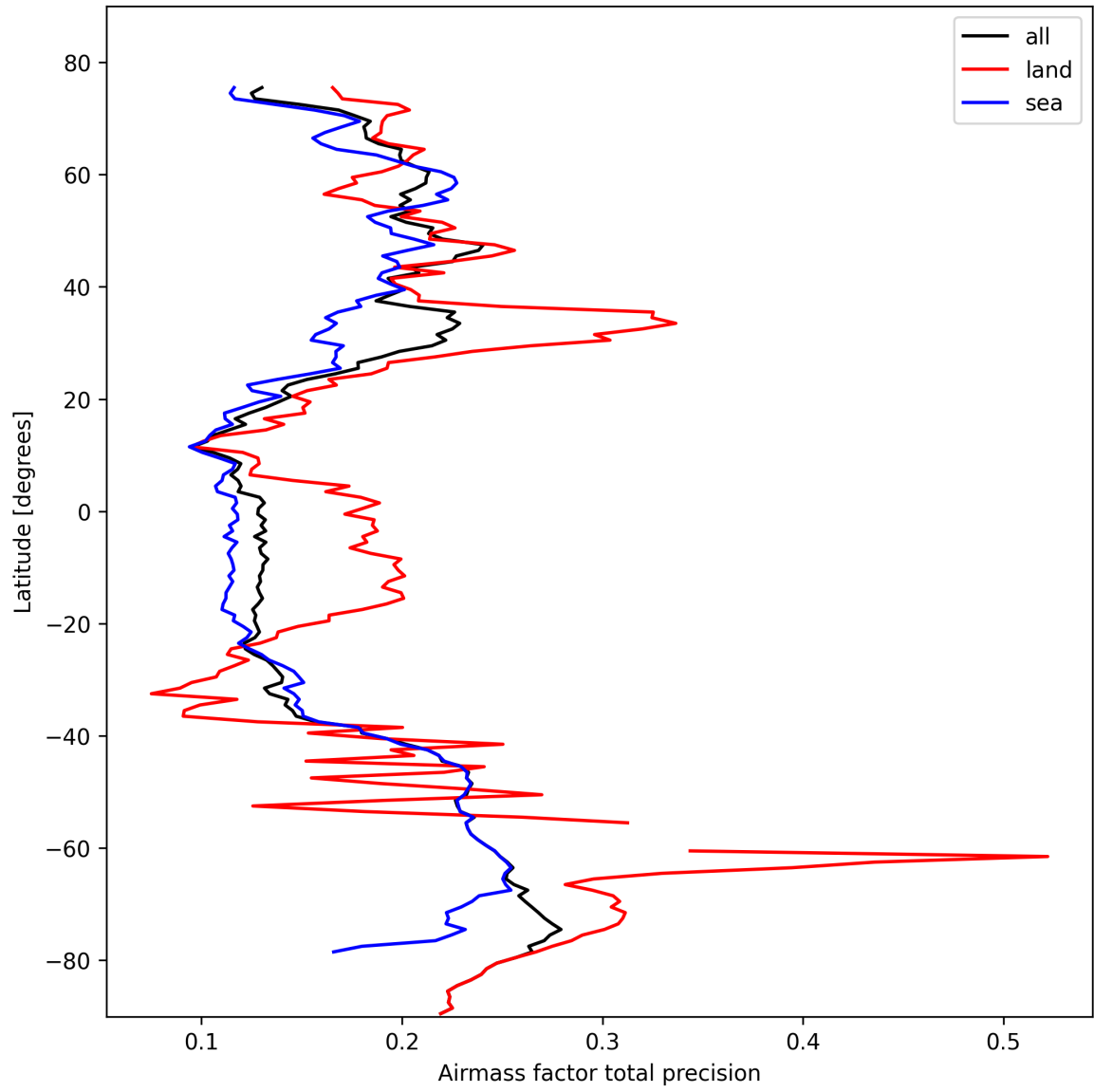
Figure 25: Zonal average of “Airmass factor total precision” for 2025-02-23 to 2025-02-24.
