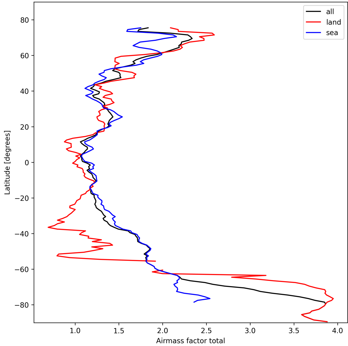
Figure 24: Zonal average of “Airmass factor total” for 2025-02-23 to 2025-02-24.
