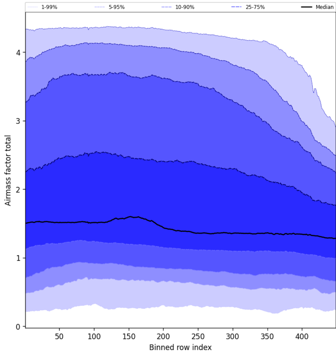
Figure 52: Along track statistics of “Airmass factor total” for 2025-02-23 to 2025-02-24
