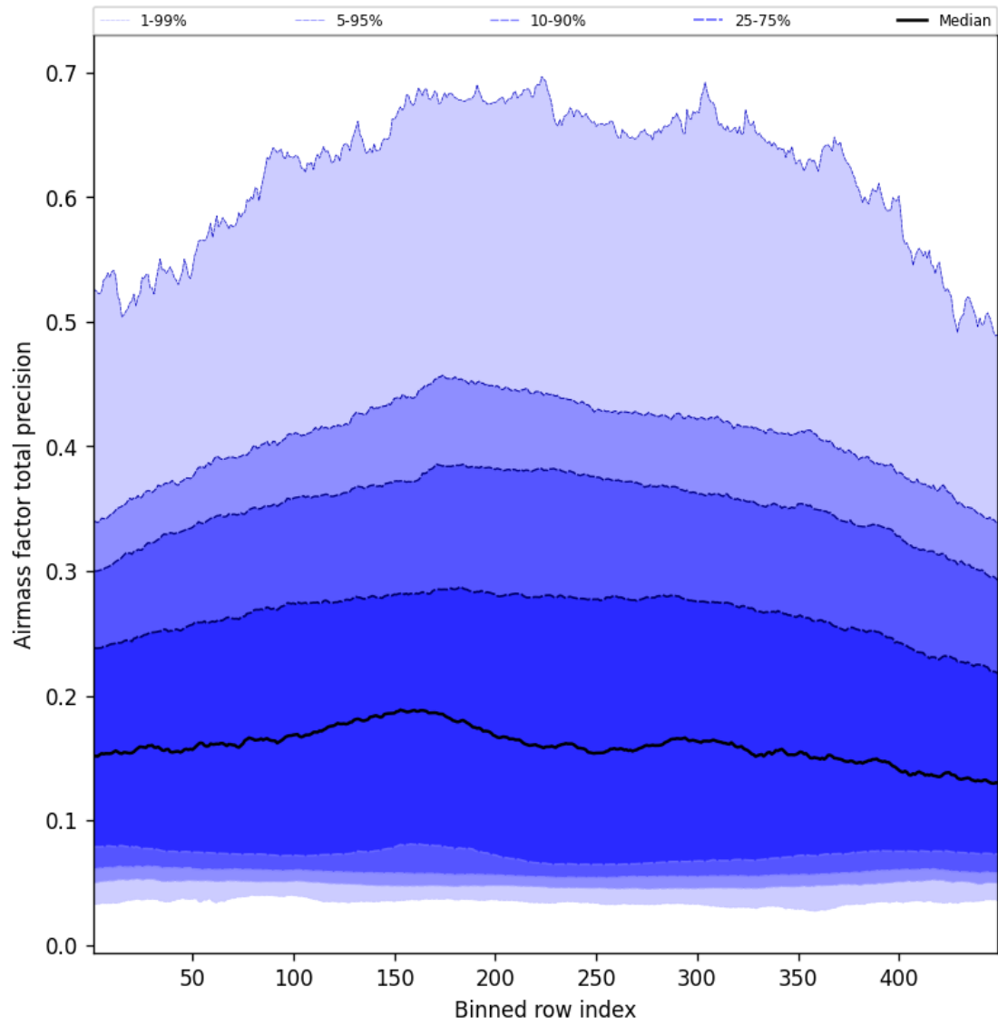
Figure 53: Along track statistics of “Airmass factor total precision” for 2025-02-23 to 2025-02-24
