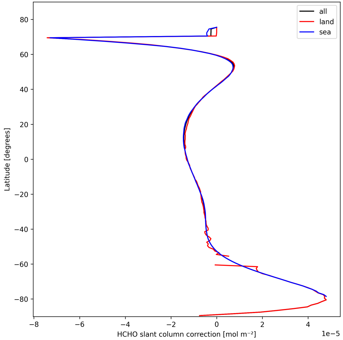
Figure 31: Zonal average of “HCHO slant column correction” for 2025-02-23 to 2025-02-24.
