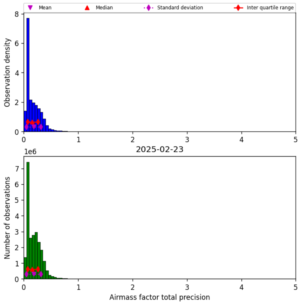
Figure 39: Histogram of “Airmass factor total precision” for 2025-02-23 to 2025-02-24
