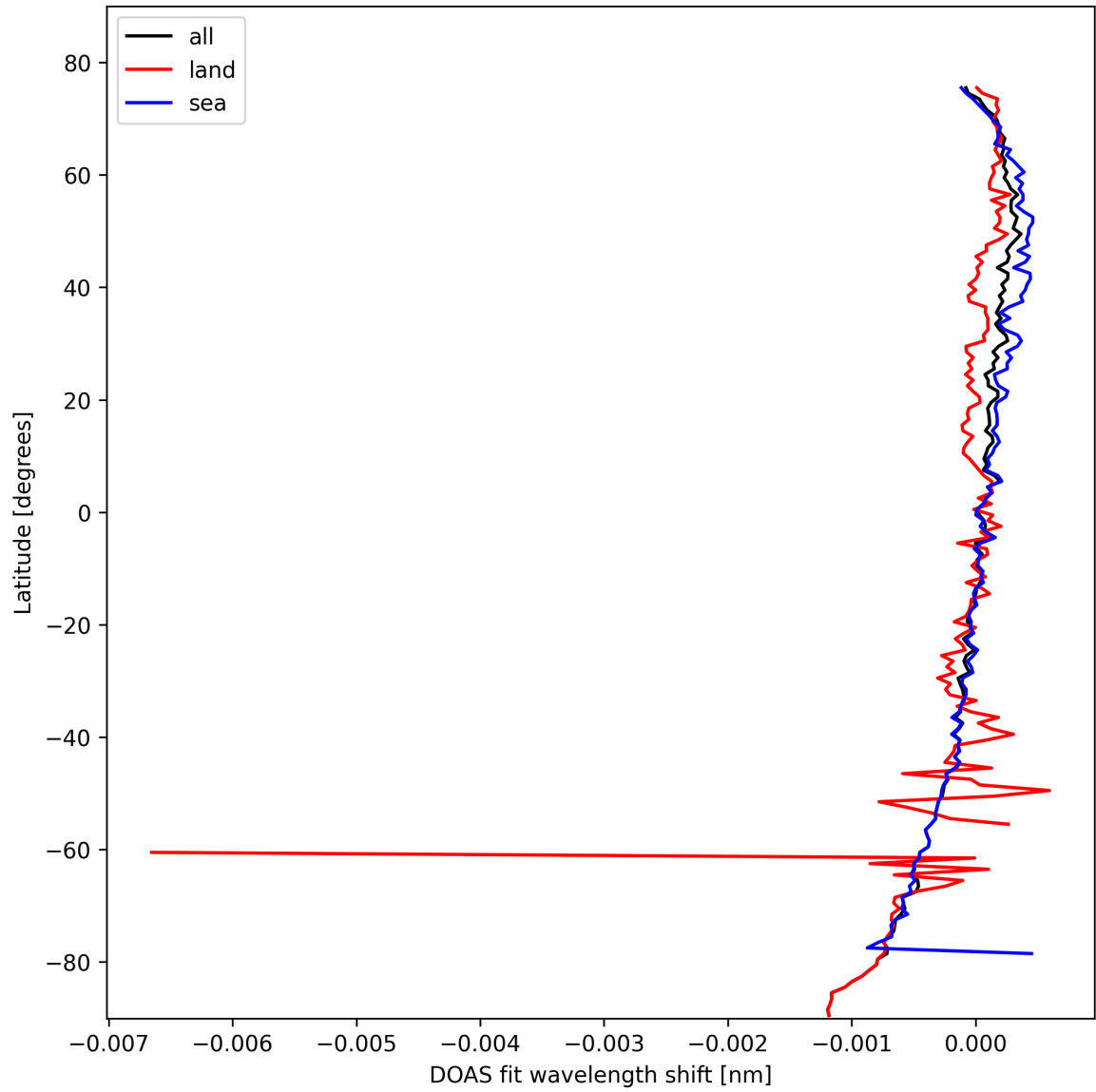
Figure 28: Zonal average of “DOAS fit wavelength shift” for 2025-02-23 to 2025-02-24.
