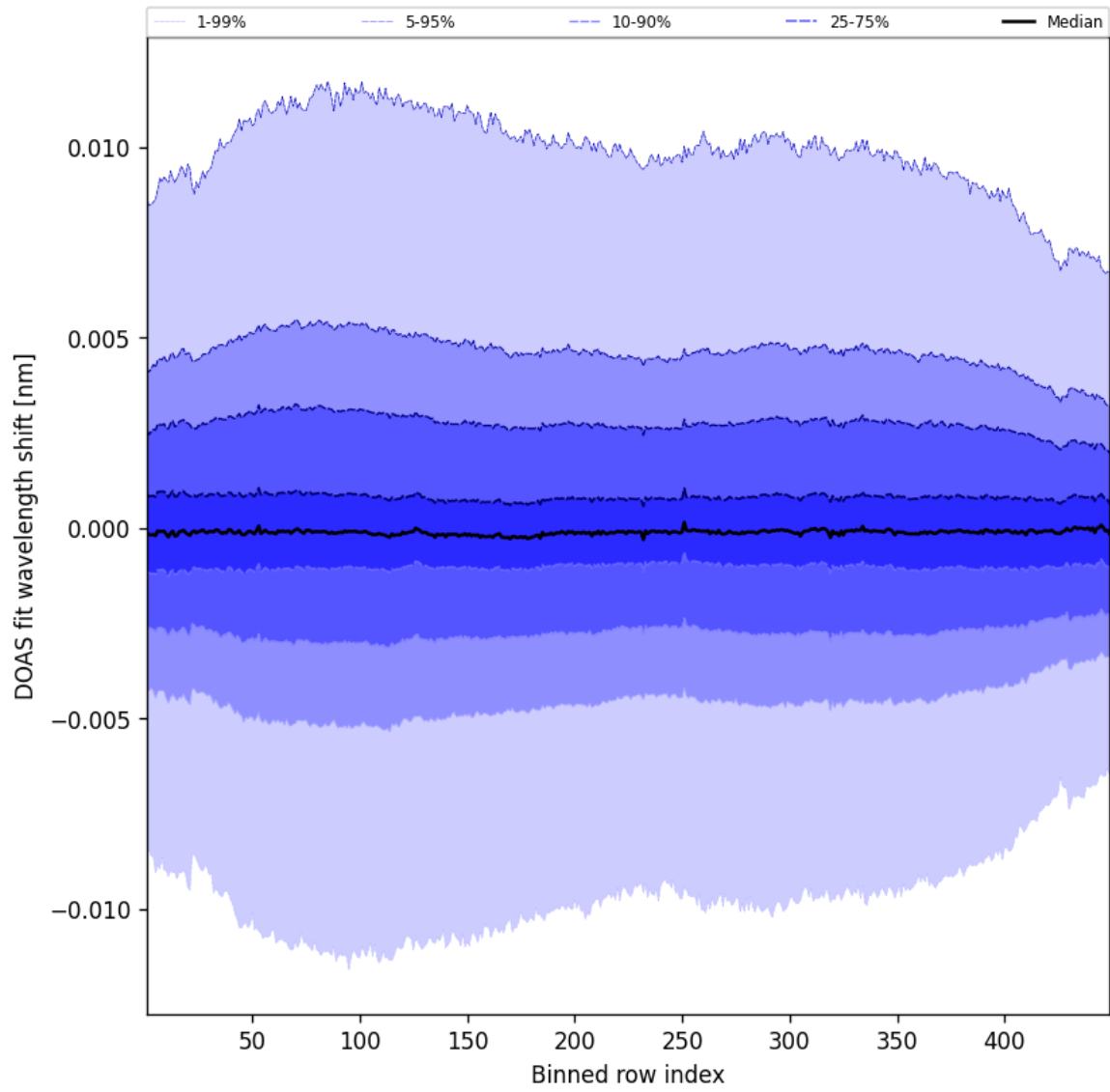
Figure 56: Along track statistics of “DOAS fit wavelength shift” for 2025-02-23 to 2025-02-24
