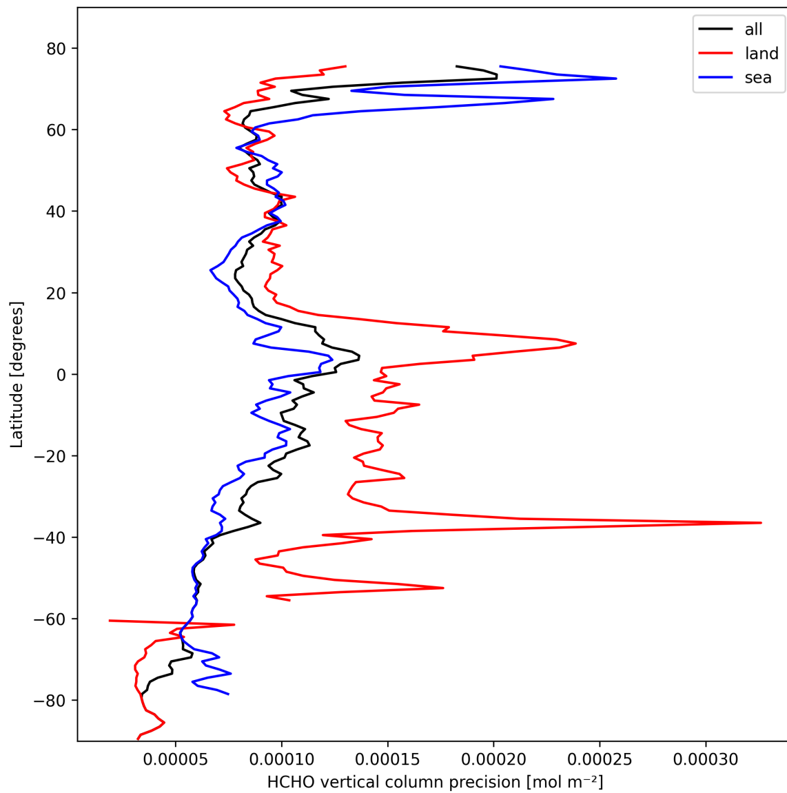
Figure 20: Zonal average of “HCHO vertical column precision” for 2025-02-23 to 2025-02-24.
