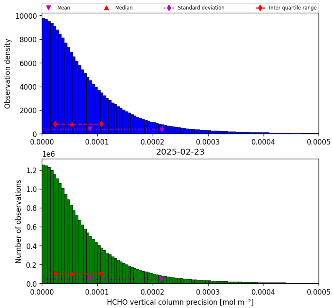
Figure 34: Histogram of “HCHO vertical column precision” for 2025-02-23 to 2025-02-24
