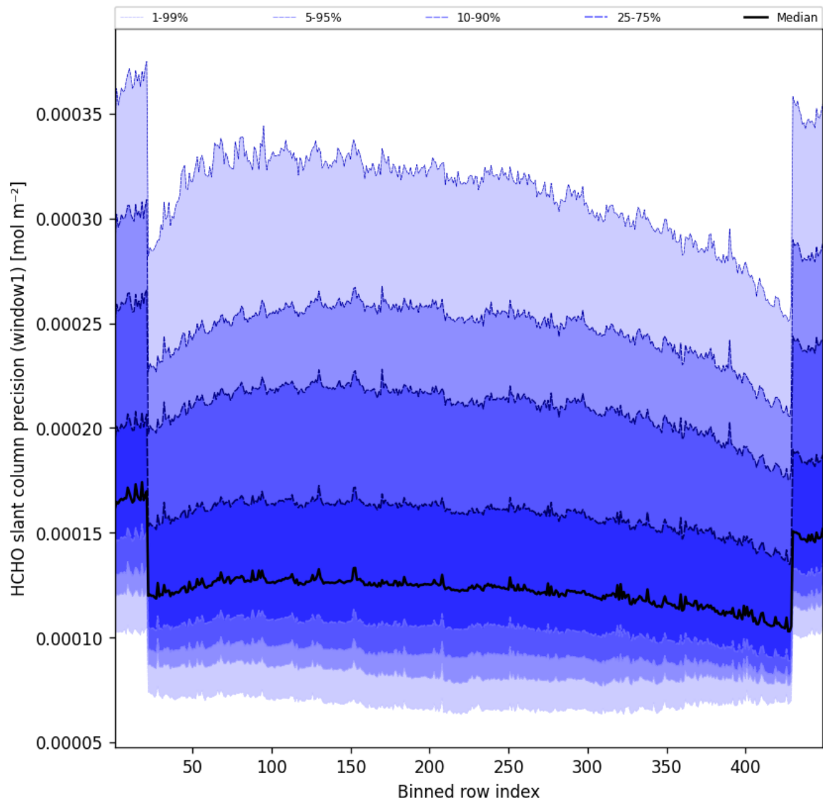
Figure 51: Along track statistics of “HCHO slant column precision (window1)” for 2025-02-23 to 2025-02-24
