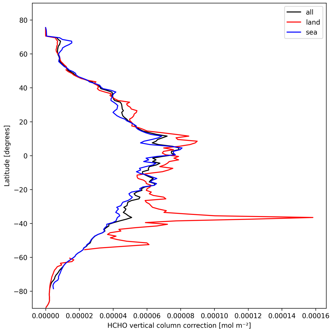
Figure 21: Zonal average of “HCHO vertical column correction” for 2025-02-23 to 2025-02-24.
