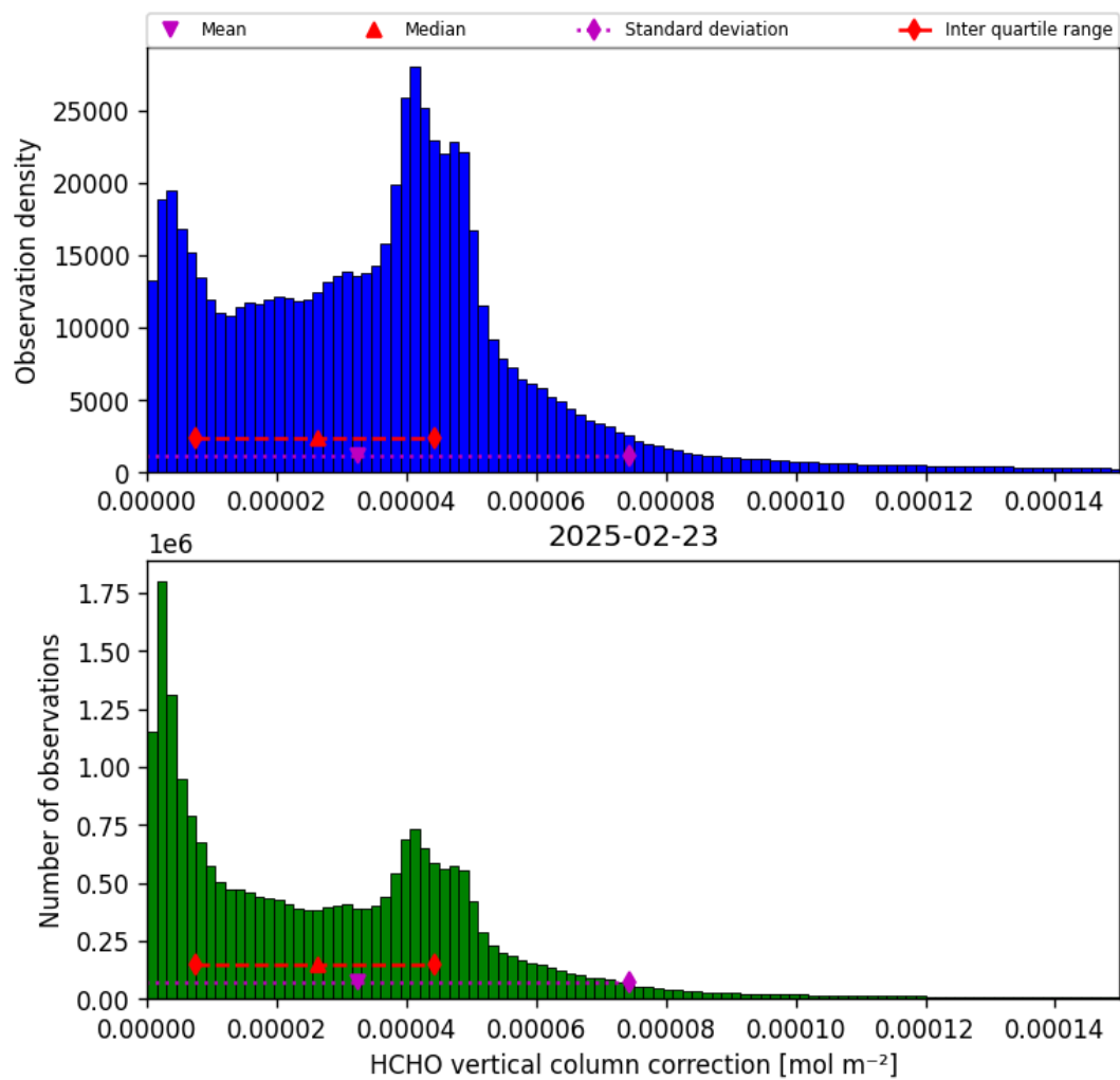
Figure 35: Histogram of “HCHO vertical column correction” for 2025-02-23 to 2025-02-24
