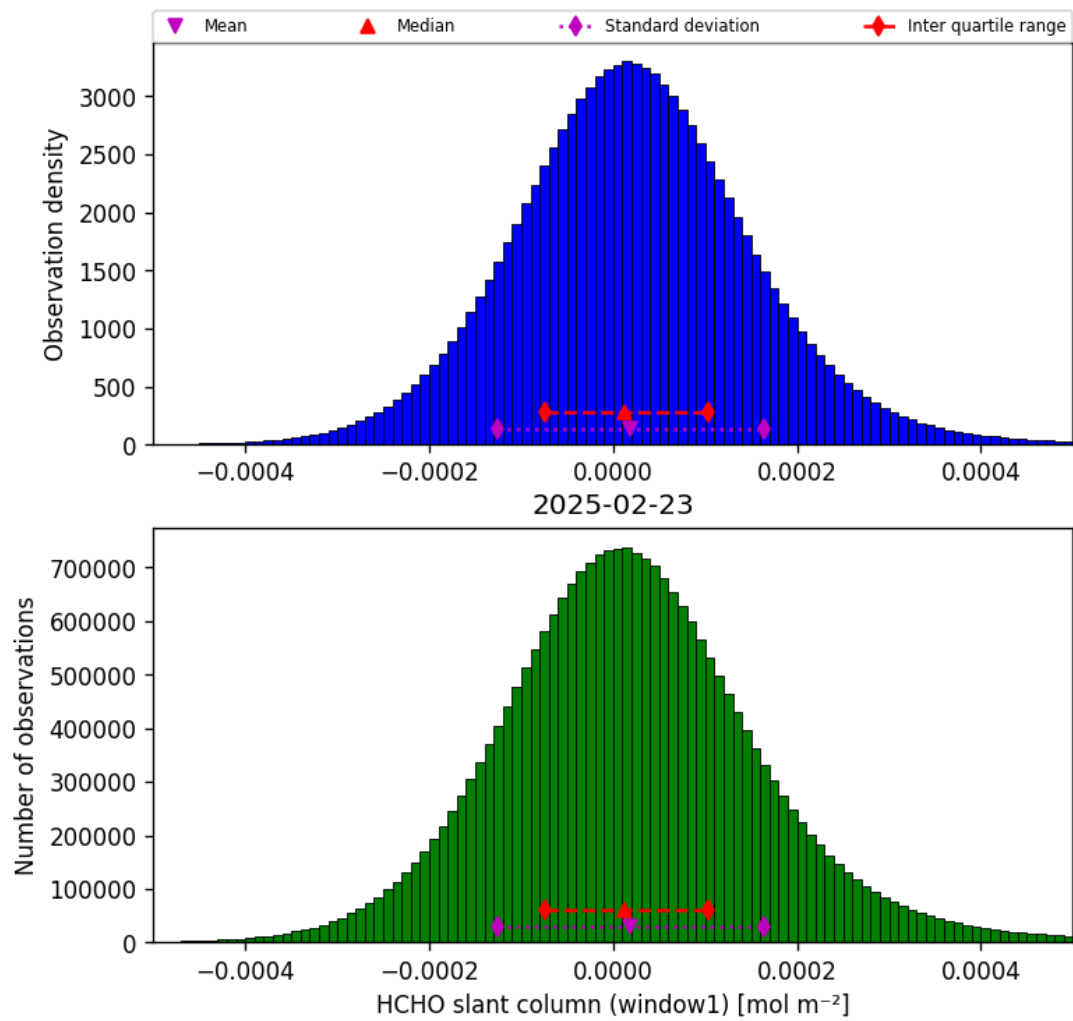
Figure 36: Histogram of “HCHO slant column (window1)” for 2025-02-23 to 2025-02-24
