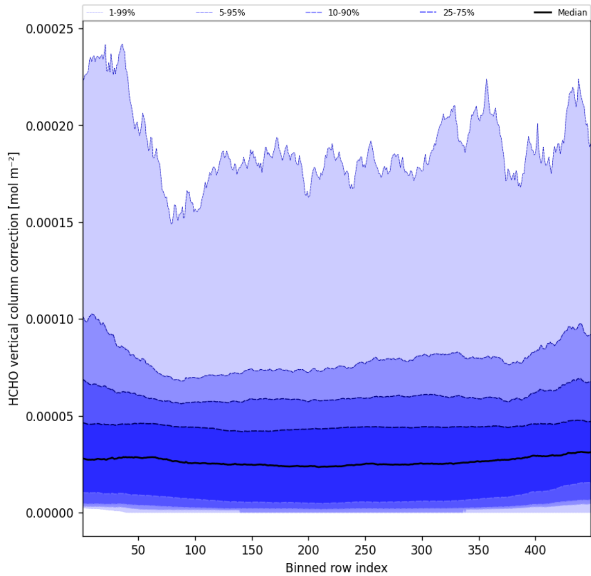
Figure 49: Along track statistics of “HCHO vertical column correction” for 2025-02-23 to 2025-02-24
