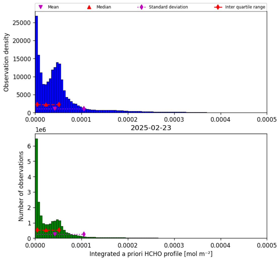
Figure 41: Histogram of “Integrated a priori HCHO profile” for 2025-02-23 to 2025-02-24
