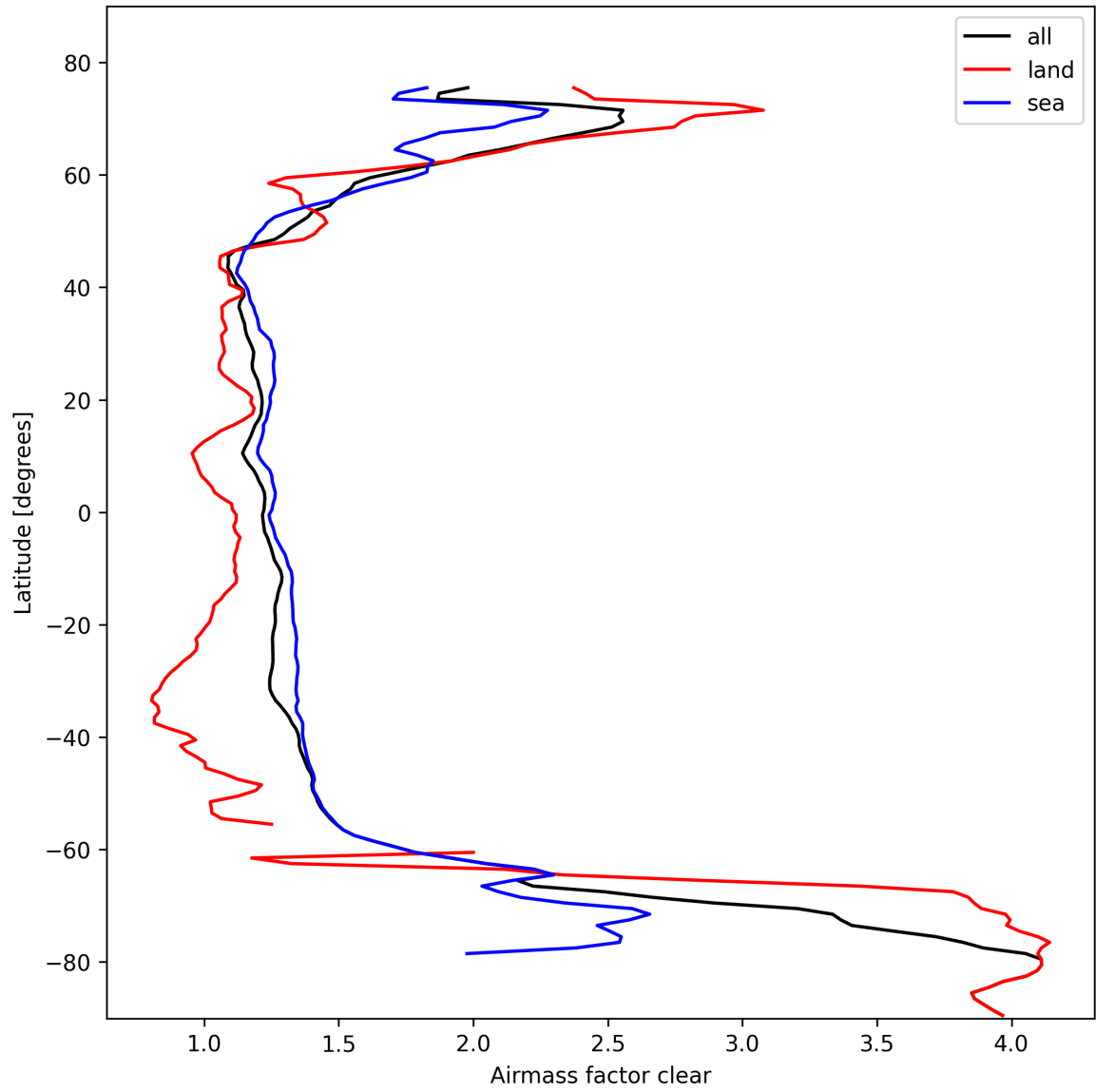
Figure 26: Zonal average of “Airmass factor clear” for 2025-02-23 to 2025-02-24.
