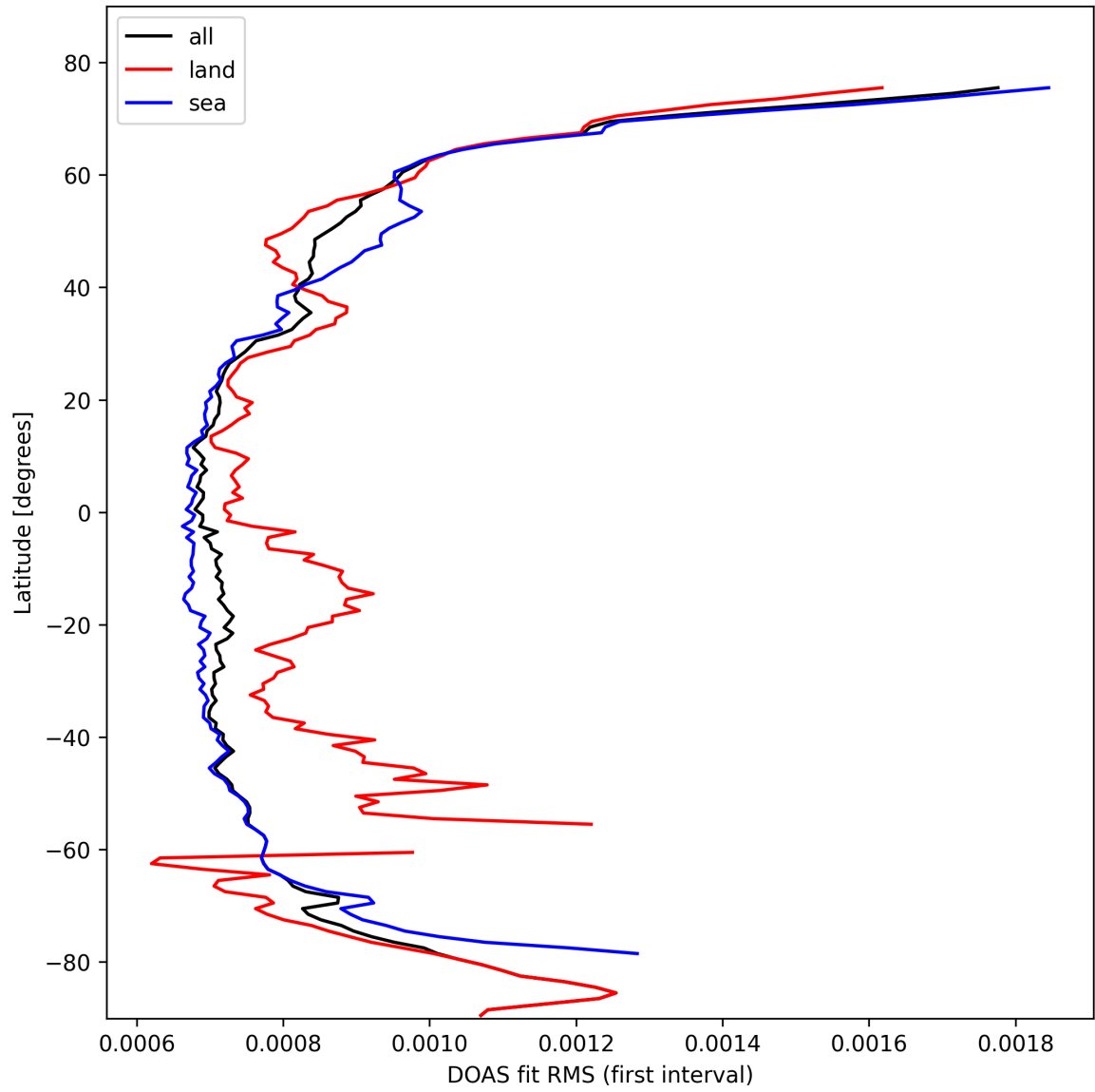
Figure 30: Zonal average of “DOAS fit RMS (first interval)” for 2025-02-23 to 2025-02-24.
