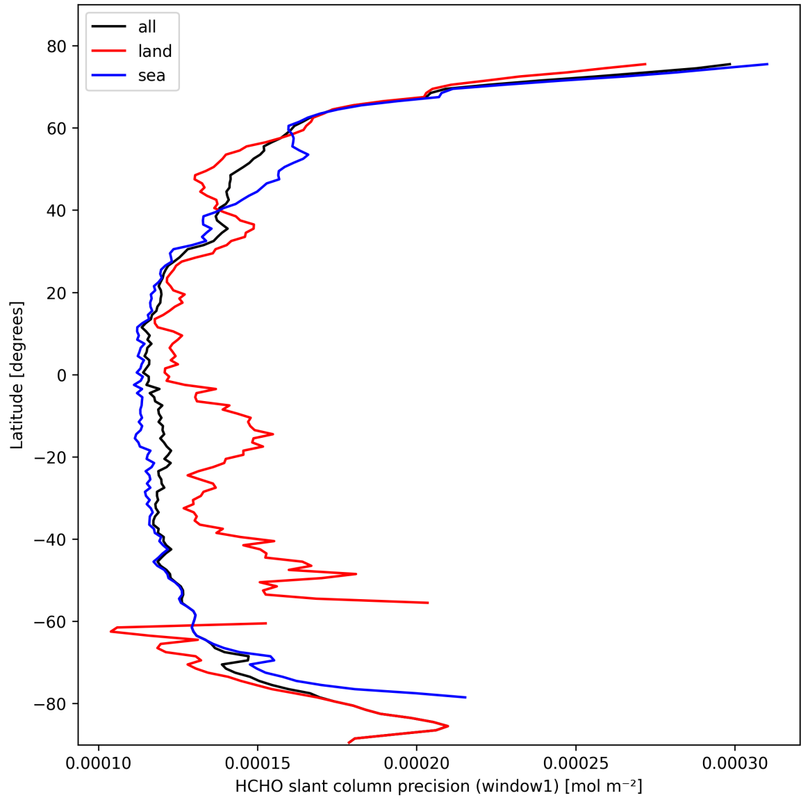
Figure 23: Zonal average of “HCHO slant column precision (window1)” for 2025-02-23 to 2025-02-24.
