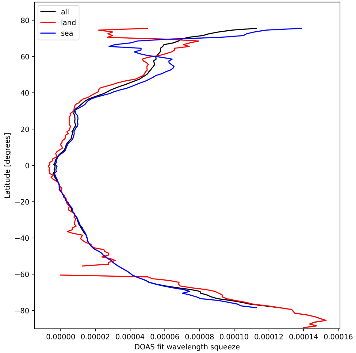
Figure 29: Zonal average of “DOAS fit wavelength squeeze” for 2025-02-23 to 2025-02-24.
