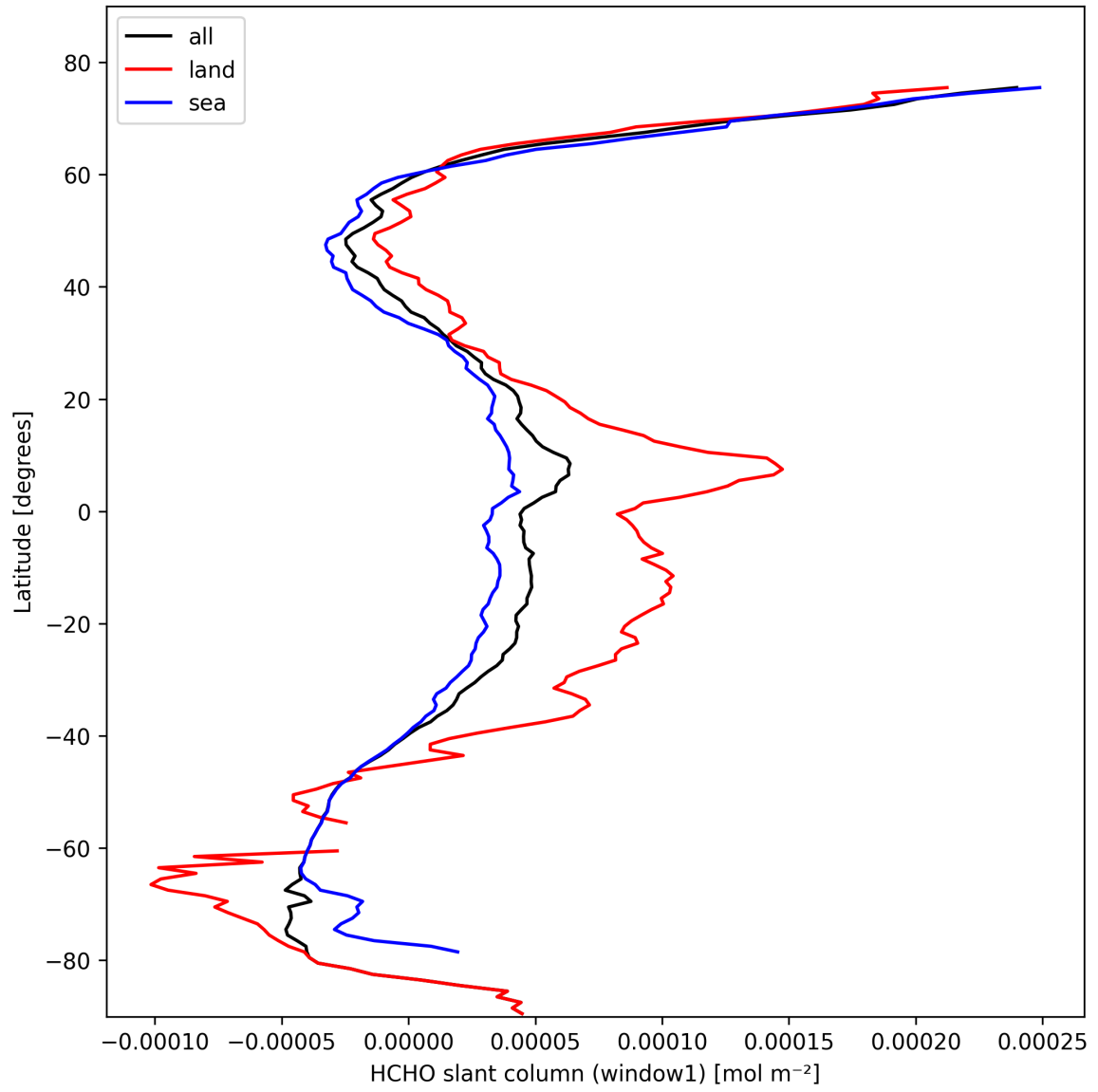
Figure 22: Zonal average of “HCHO slant column (window1)” for 2025-02-23 to 2025-02-24.
