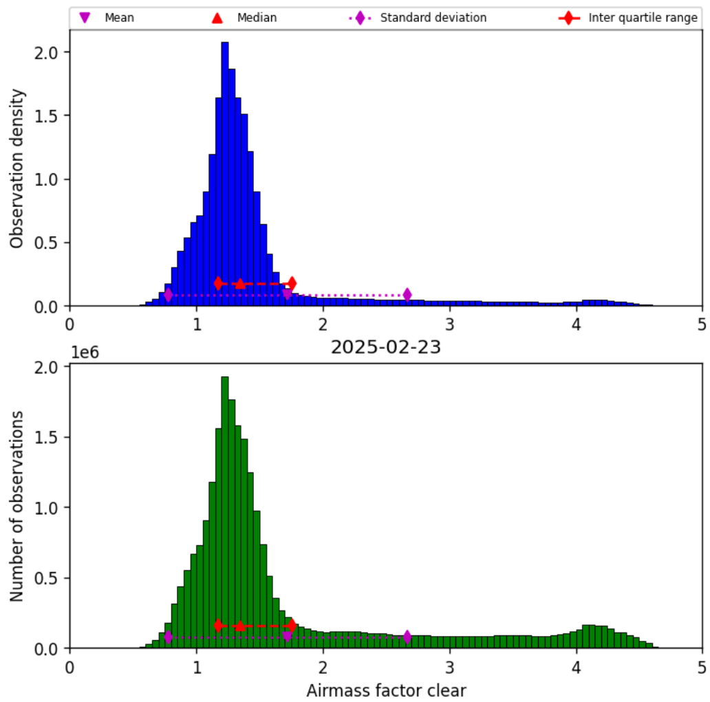
Figure 40: Histogram of “Airmass factor clear” for 2025-02-23 to 2025-02-24
