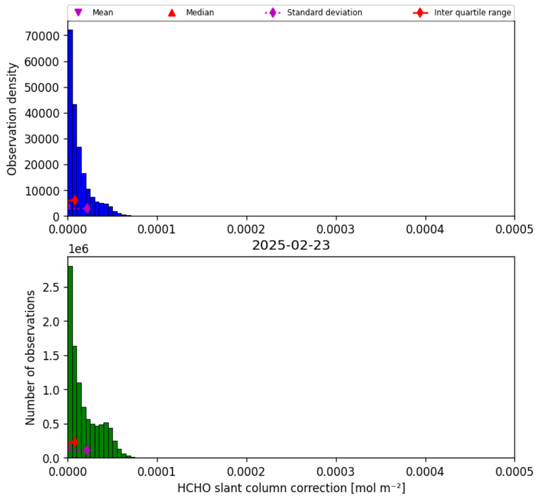
Figure 45: Histogram of "HCHO slant column correction" for 2025-02-23 to 2025-02-24
