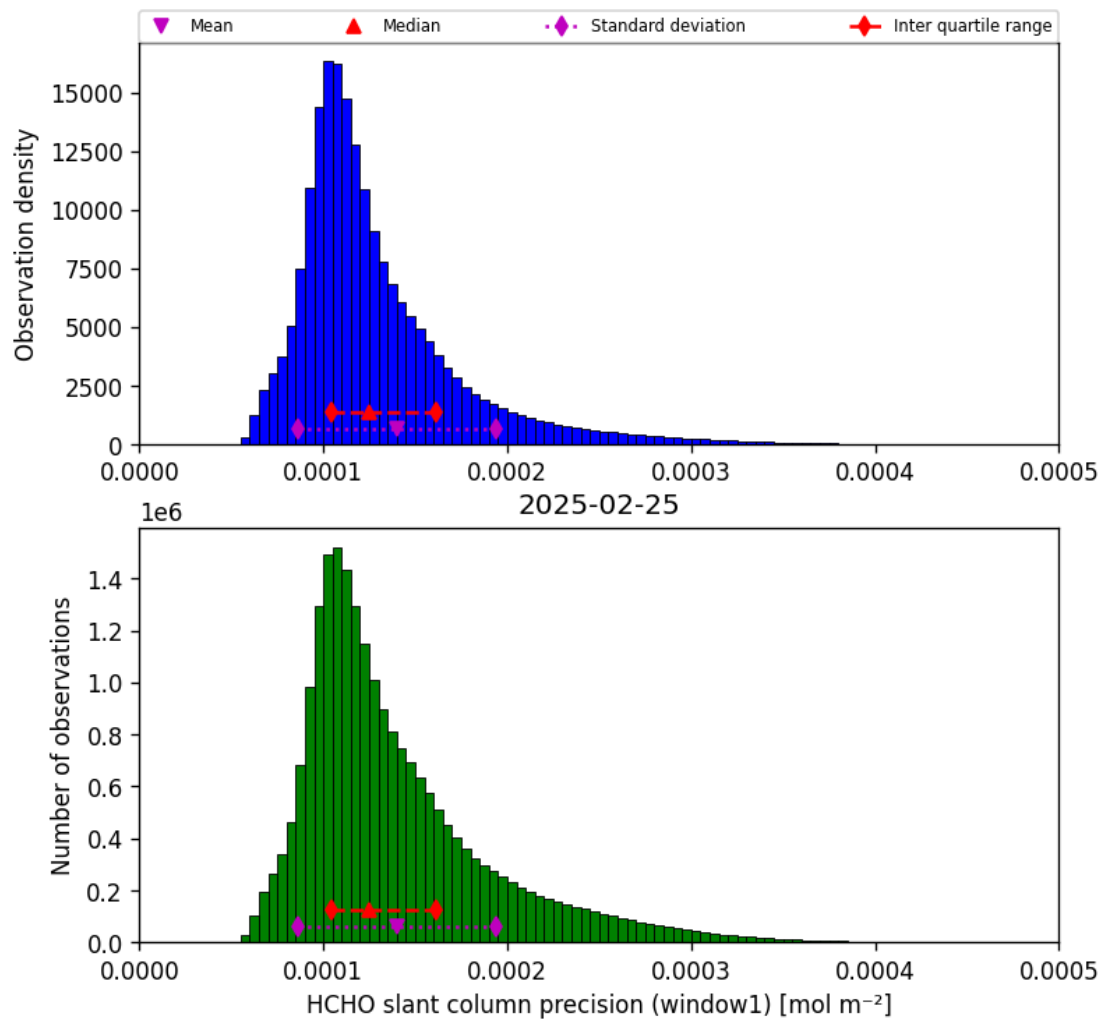
Figure 37: Histogram of “HCHO slant column precision (window1)” for 2025-02-25 to 2025-02-26
