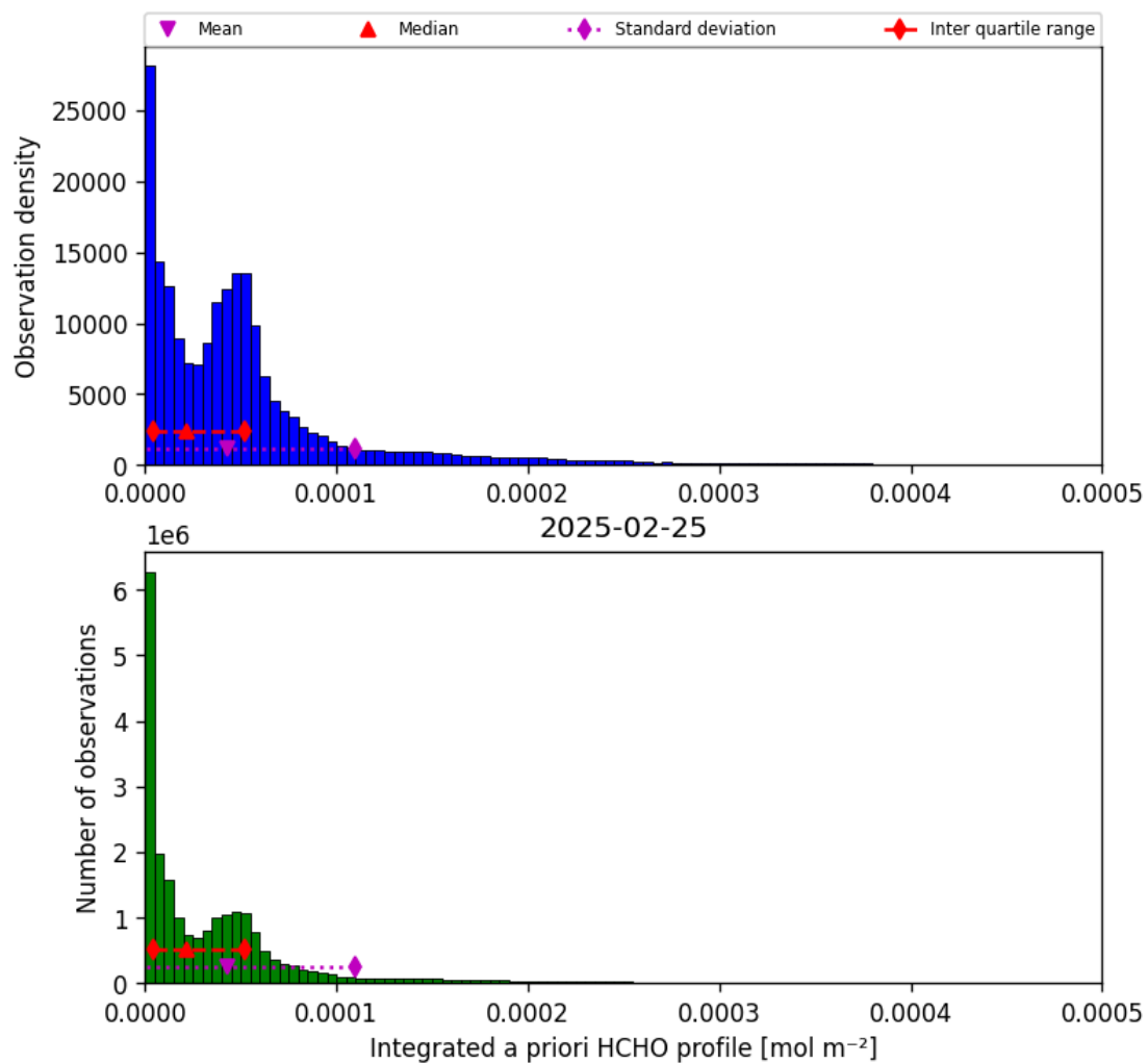
Figure 41: Histogram of “Integrated a priori HCHO profile” for 2025-02-25 to 2025-02-26
