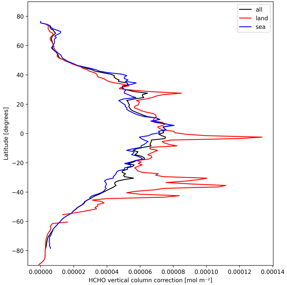
Figure 21: Zonal average of “HCHO vertical column correction” for 2025-02-25 to 2025-02-26.
