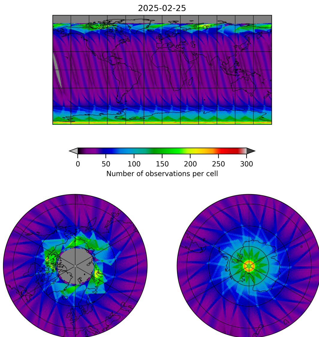
Figure 17: Map of the number of observations for 2025-02-25 to 2025-02-26
