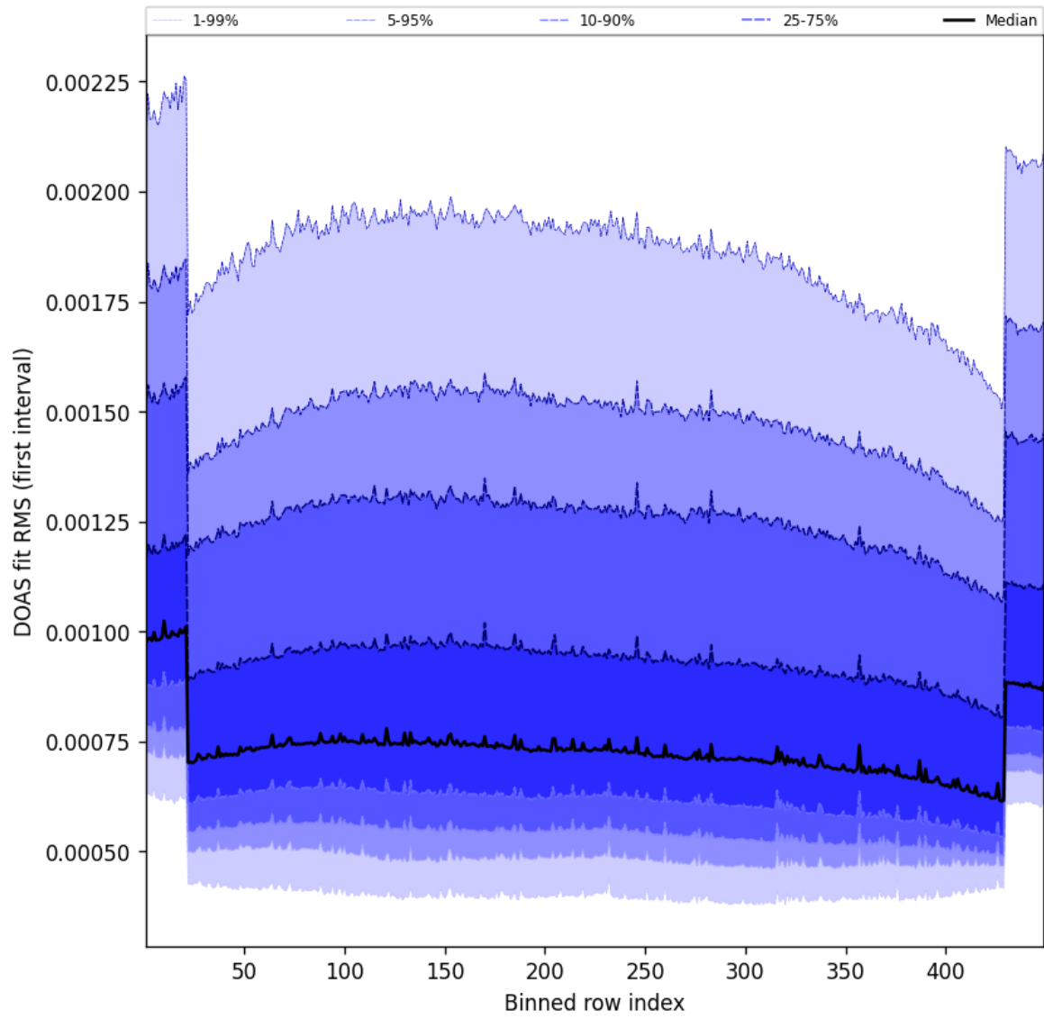
Figure 58: Along track statistics of “DOAS fit RMS (first interval)” for 2025-02-25 to 2025-02-26
