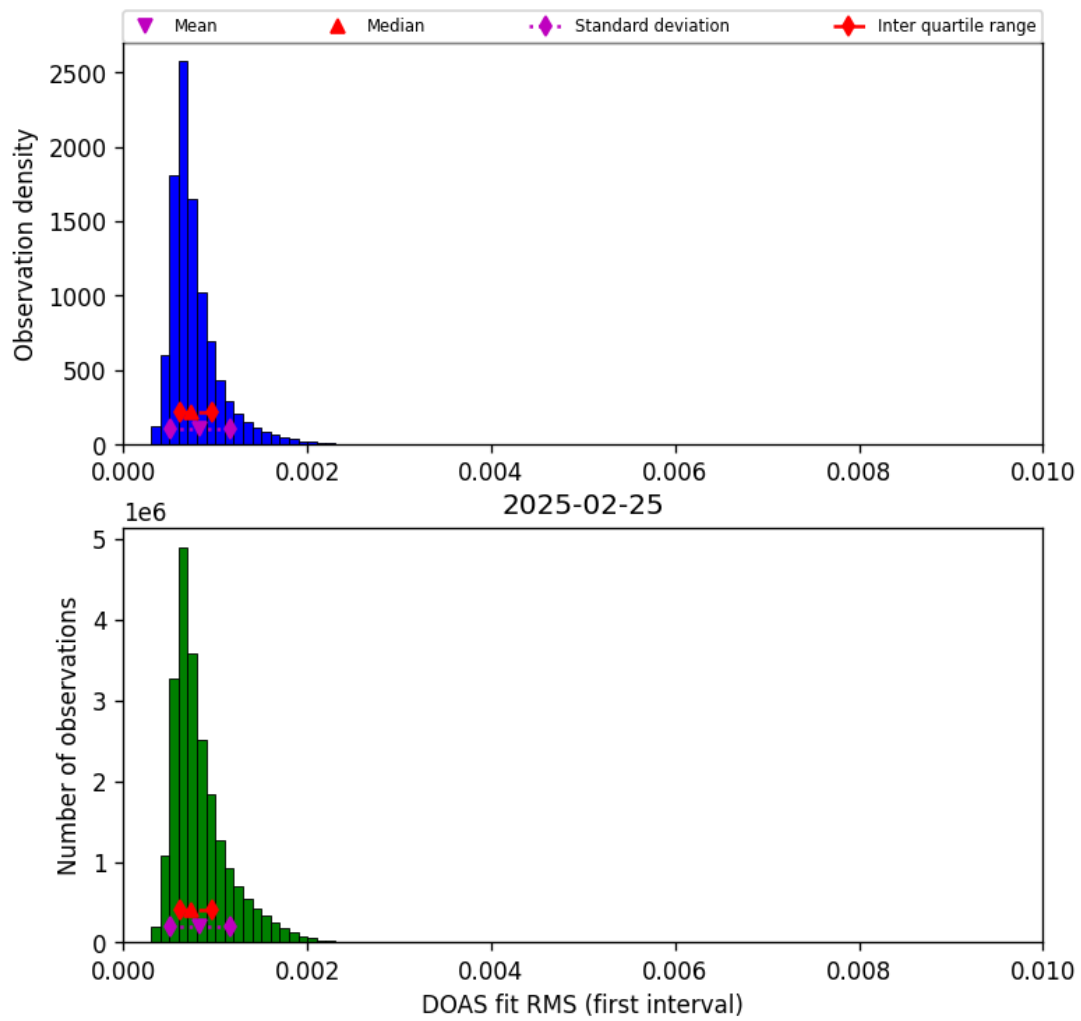
Figure 44: Histogram of “DOAS fit RMS (first interval)” for 2025-02-25 to 2025-02-26
