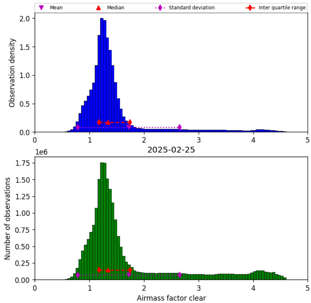
Figure 40: Histogram of “Airmass factor clear” for 2025-02-25 to 2025-02-26
