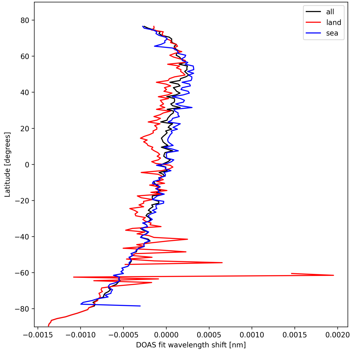
Figure 28: Zonal average of "DOAS fit wavelength shift" for 2025-02-25 to 2025-02-26.
