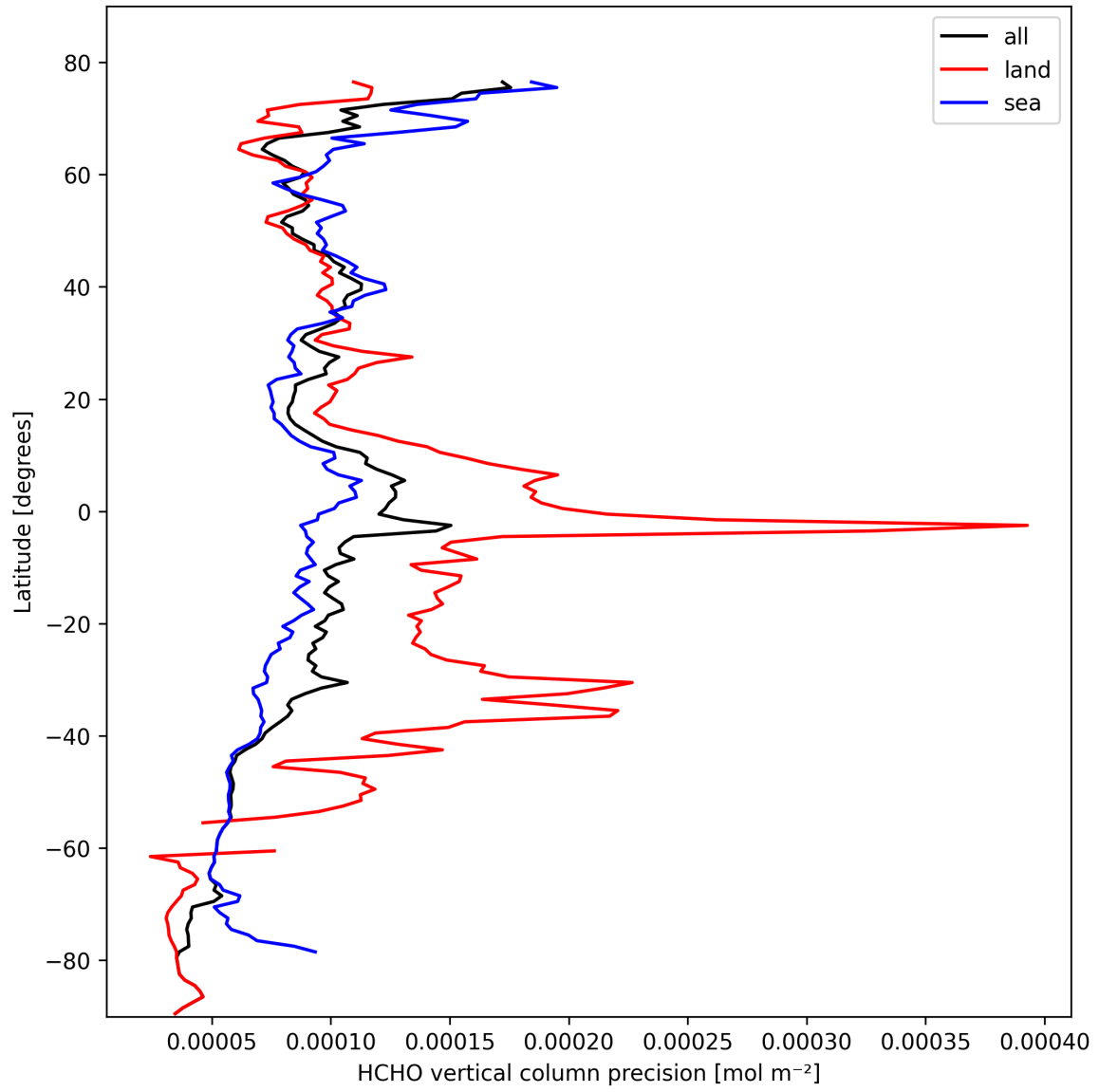
Figure 20: Zonal average of “HCHO vertical column precision” for 2025-02-25 to 2025-02-26.
