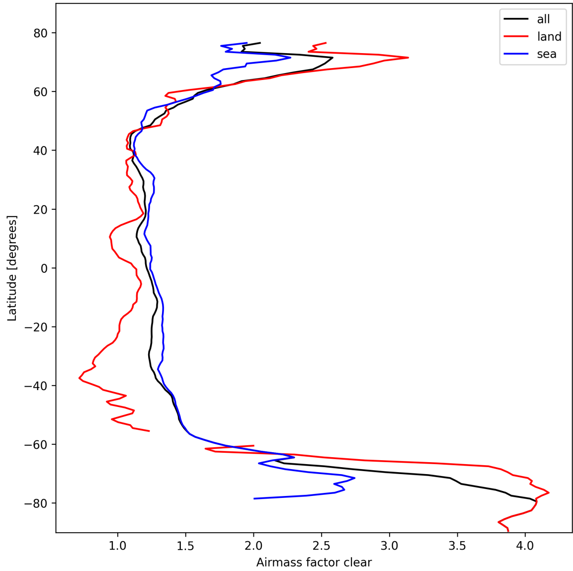
Figure 26: Zonal average of “Airmass factor clear” for 2025-02-25 to 2025-02-26.
