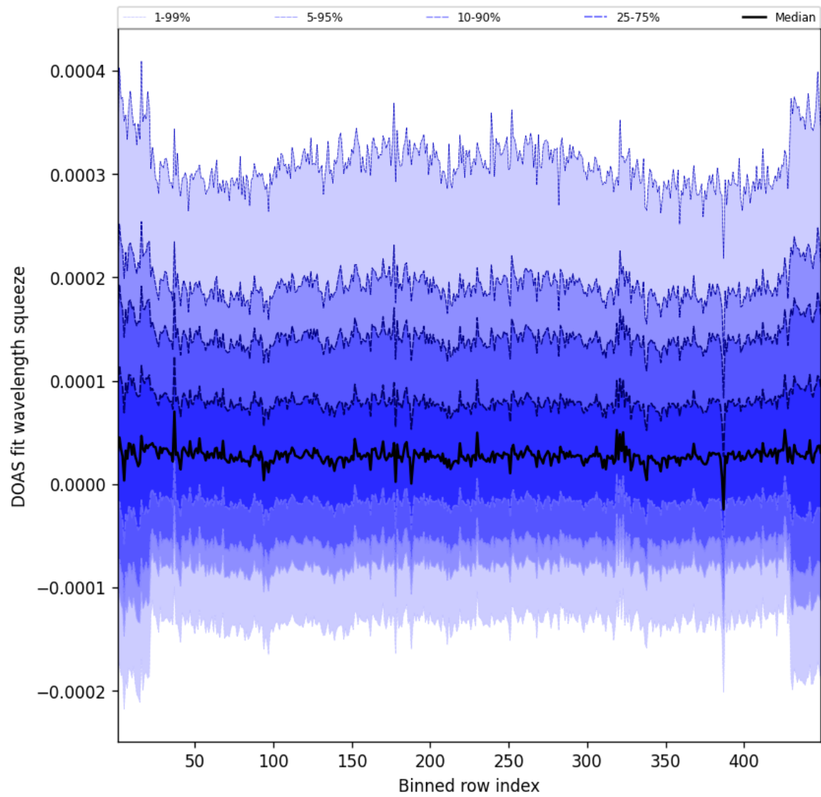
Figure 57: Along track statistics of “DOAS fit wavelength squeeze” for 2025-02-25 to 2025-02-26
