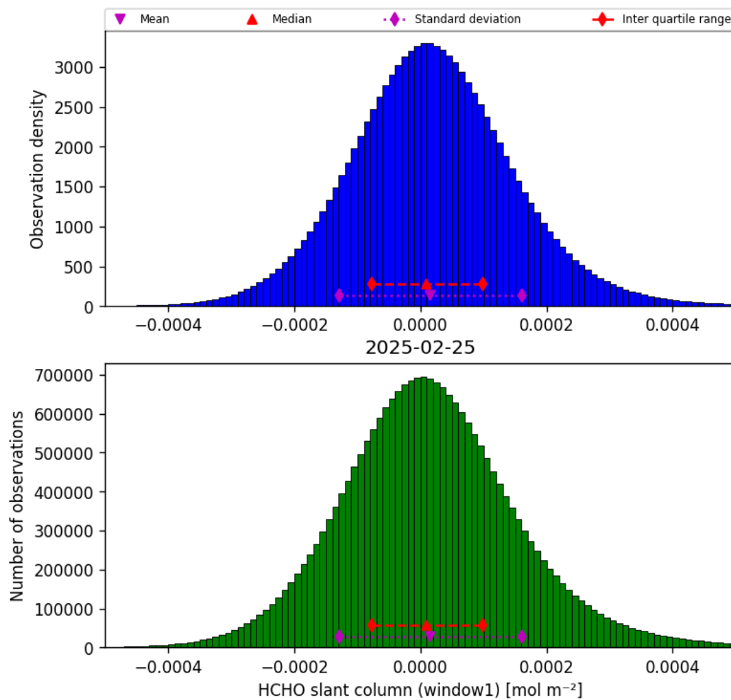
Figure 36: Histogram of “HCHO slant column (window1)” for 2025-02-25 to 2025-02-26
