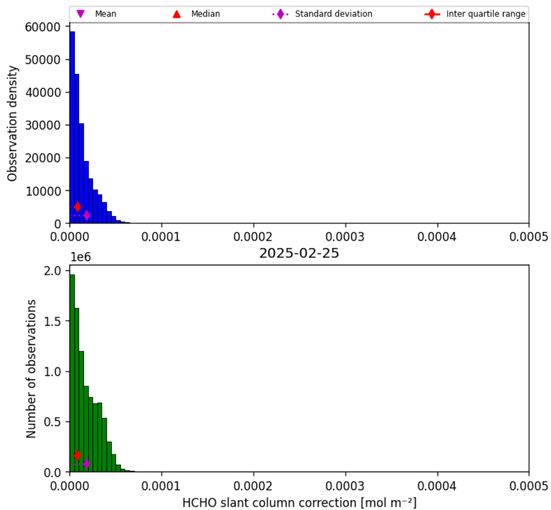
Figure 45: Histogram of “HCHO slant column correction” for 2025-02-25 to 2025-02-26
