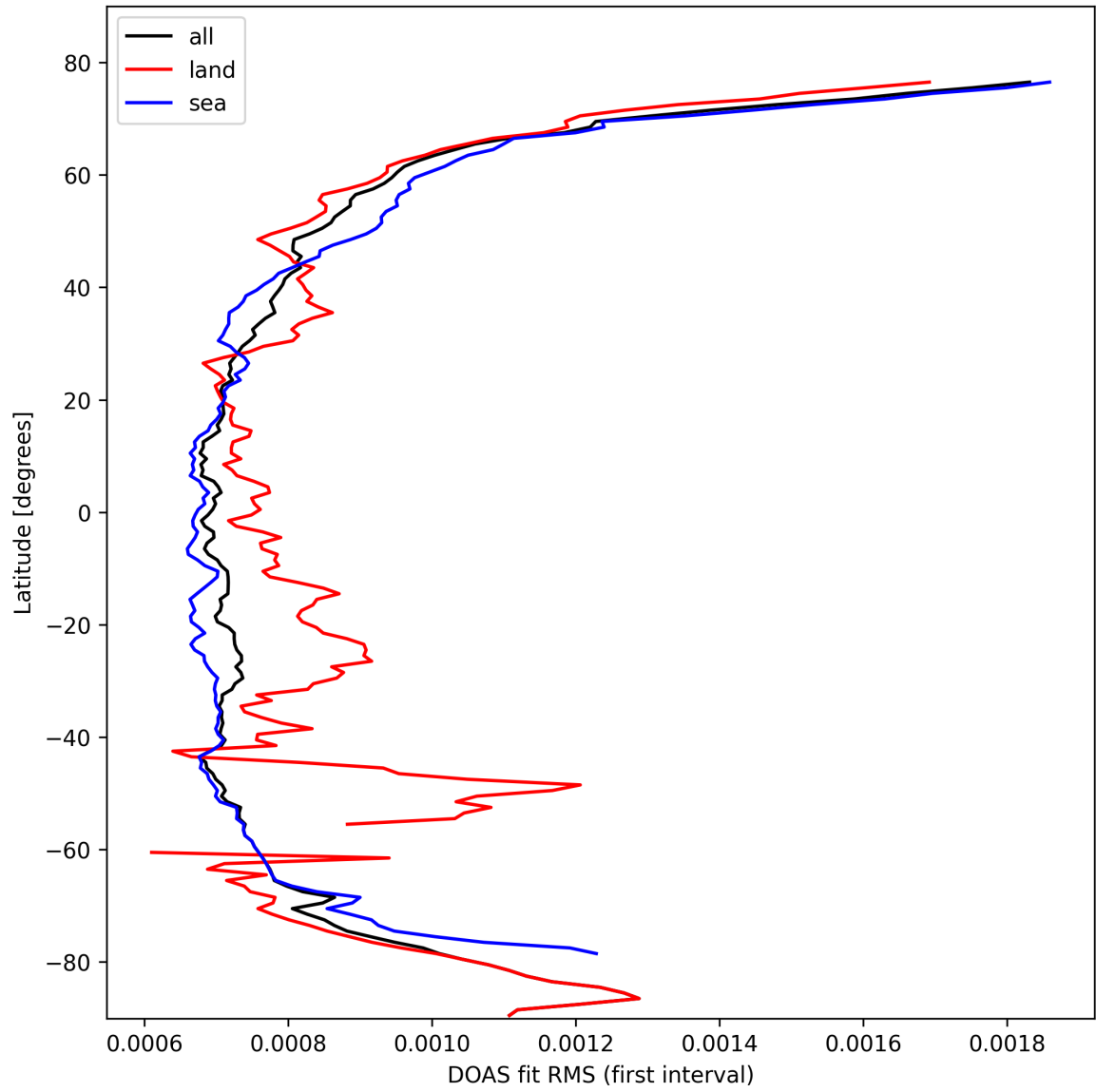
Figure 30: Zonal average of "DOAS fit RMS (first interval)" for 2025-02-25 to 2025-02-26.
