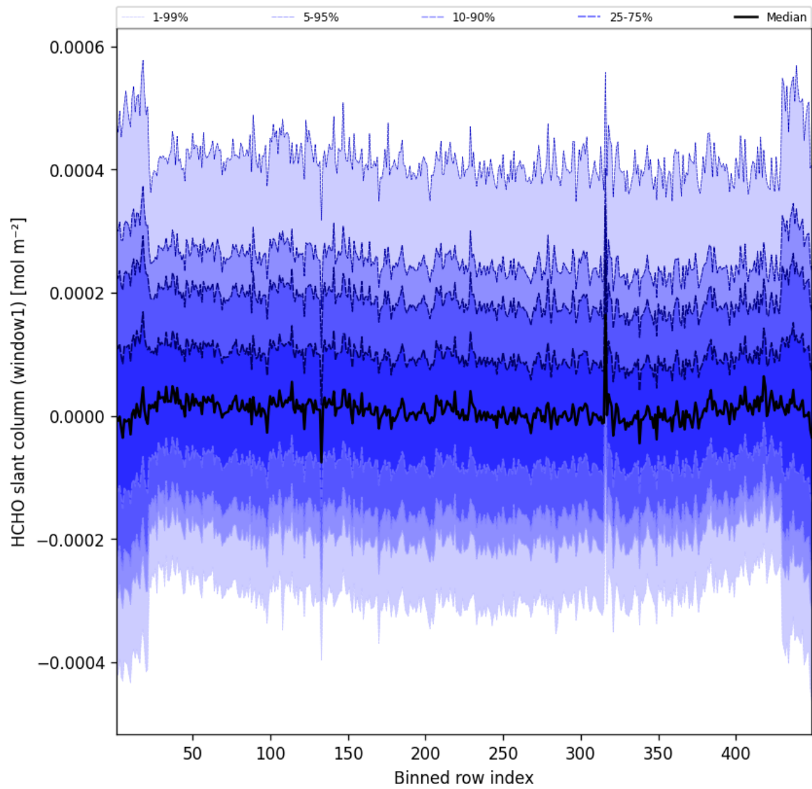
Figure 50: Along track statistics of “HCHO slant column (window1)” for 2025-02-25 to 2025-02-26
