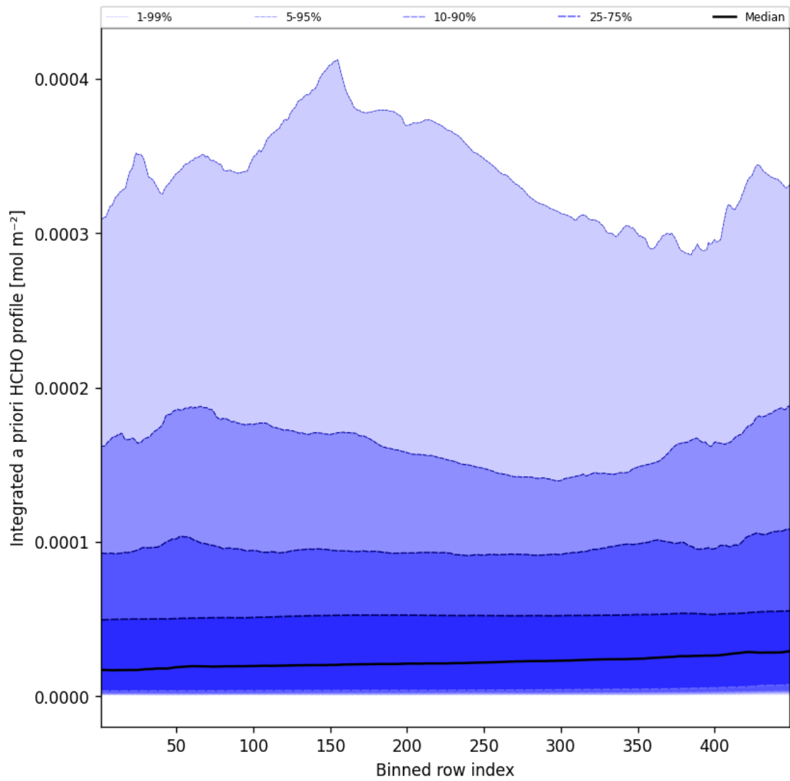
Figure 55: Along track statistics of "Integrated a priori HCHO profile" for 2025-02-25 to 2025-02-26
