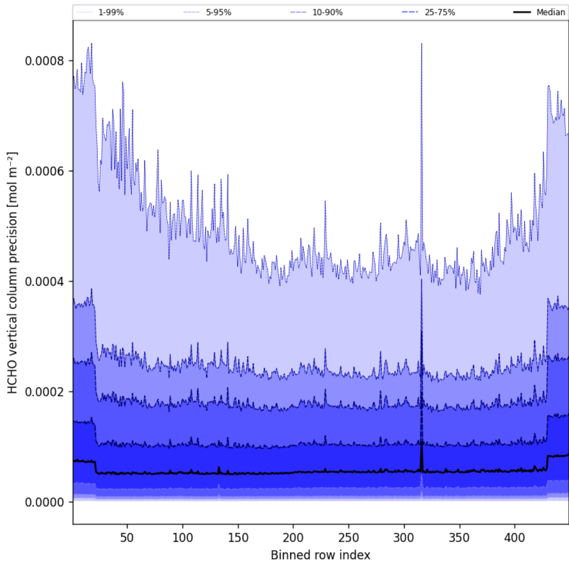
Figure 48: Along track statistics of “HCHO vertical column precision” for 2025-02-25 to 2025-02-26
