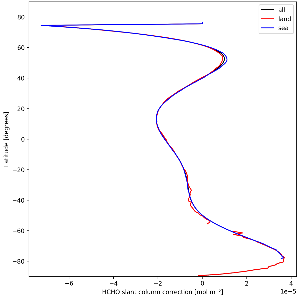
Figure 31: Zonal average of “HCHO slant column correction” for 2025-02-25 to 2025-02-26.
