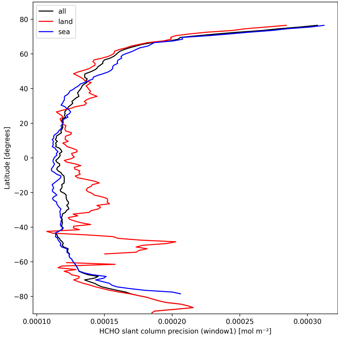
Figure 23: Zonal average of “HCHO slant column precision (window1)” for 2025-02-25 to 2025-02-26.
