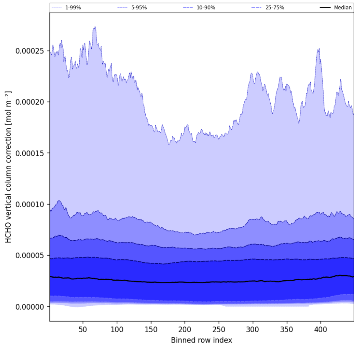
Figure 49: Along track statistics of “HCHO vertical column correction” for 2025-02-25 to 2025-02-26
