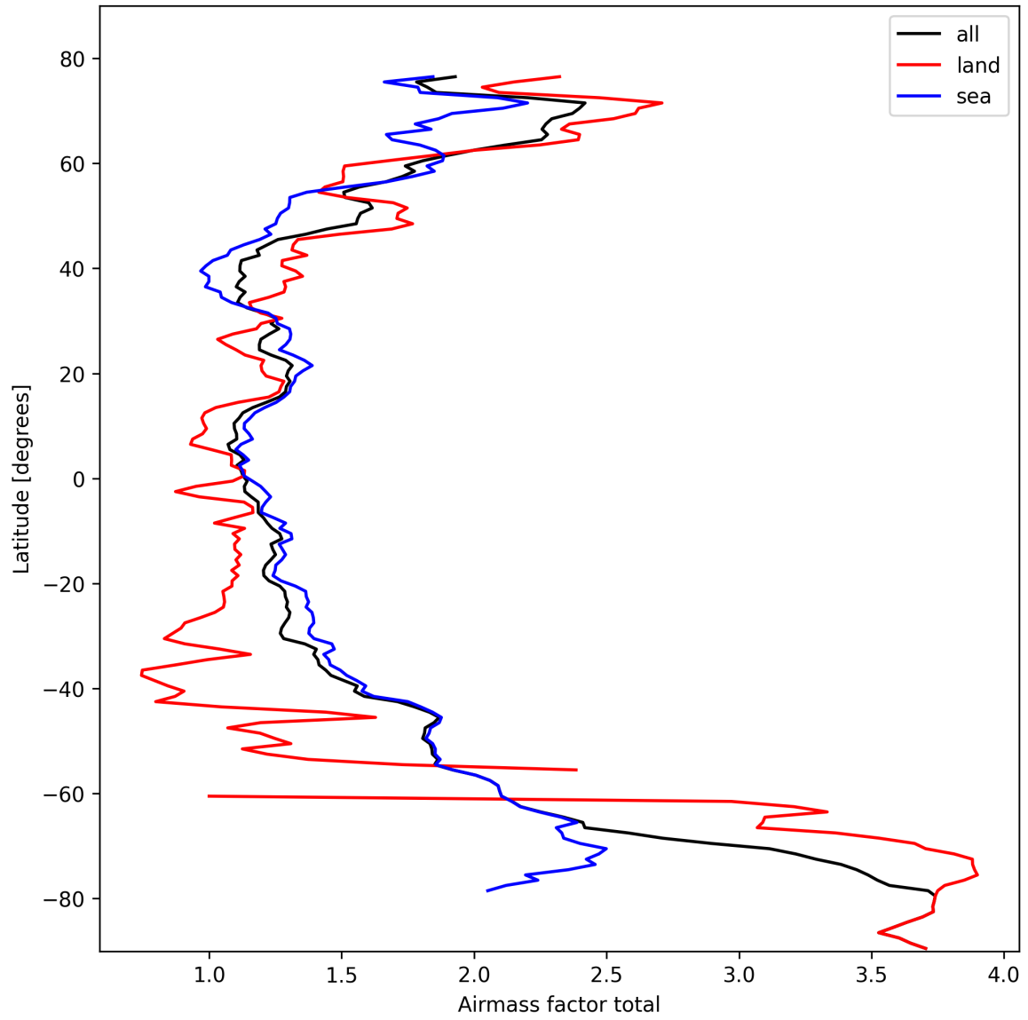
Figure 24: Zonal average of “Airmass factor total” for 2025-02-25 to 2025-02-26.
