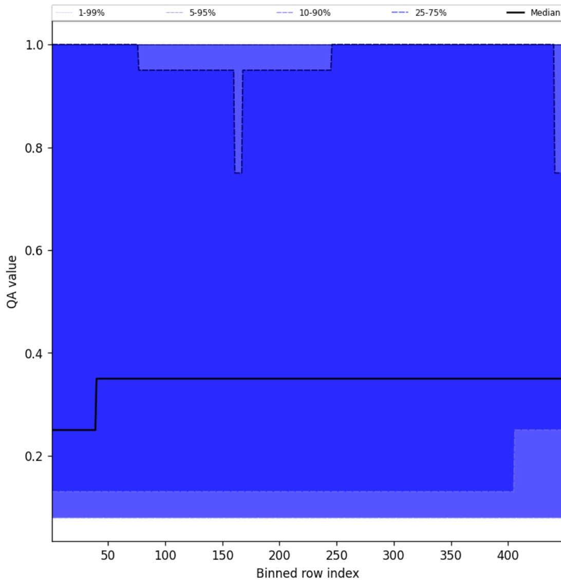
Figure 46: Along track statistics of “QA value” for 2025-02-25 to 2025-02-26
