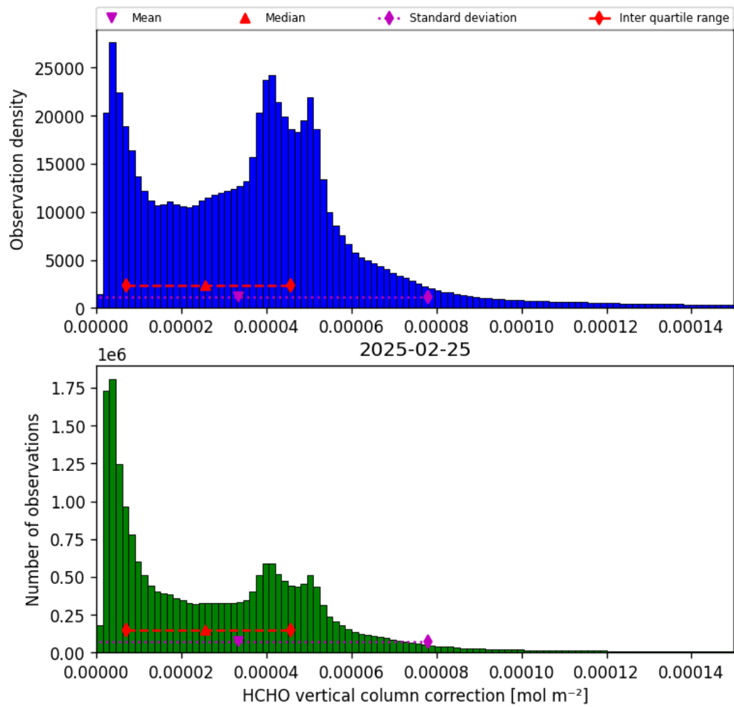
Figure 35: Histogram of “HCHO vertical column correction” for 2025-02-25 to 2025-02-26
