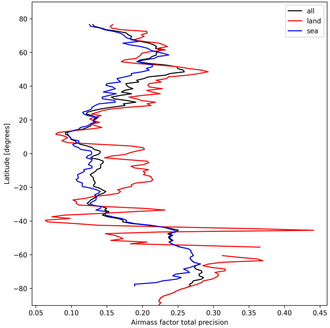
Figure 25: Zonal average of “Airmass factor total precision” for 2025-02-25 to 2025-02-26.
