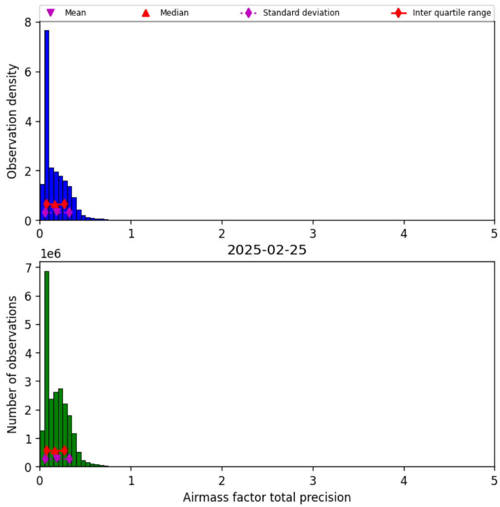
Figure 39: Histogram of “Airmass factor total precision” for 2025-02-25 to 2025-02-26
