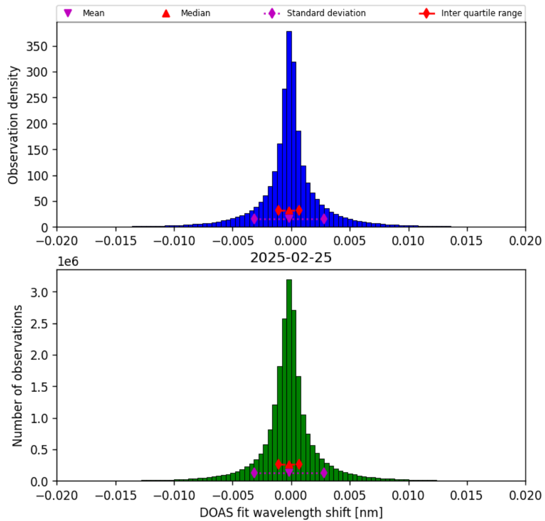
Figure 42: Histogram of “DOAS fit wavelength shift” for 2025-02-25 to 2025-02-26
