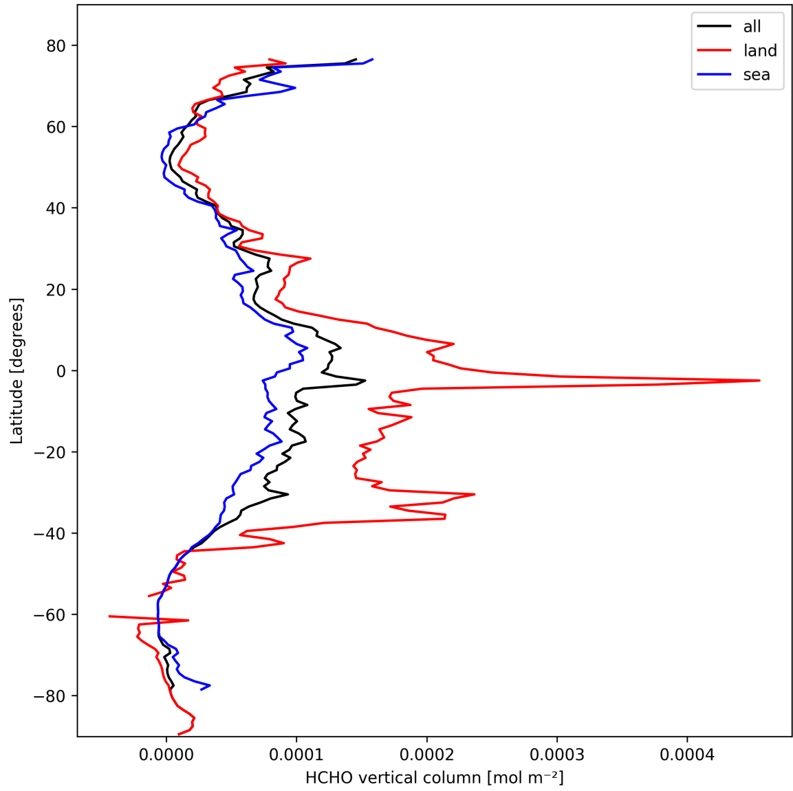
Figure 19: Zonal average of “HCHO vertical column” for 2025-02-25 to 2025-02-26.
