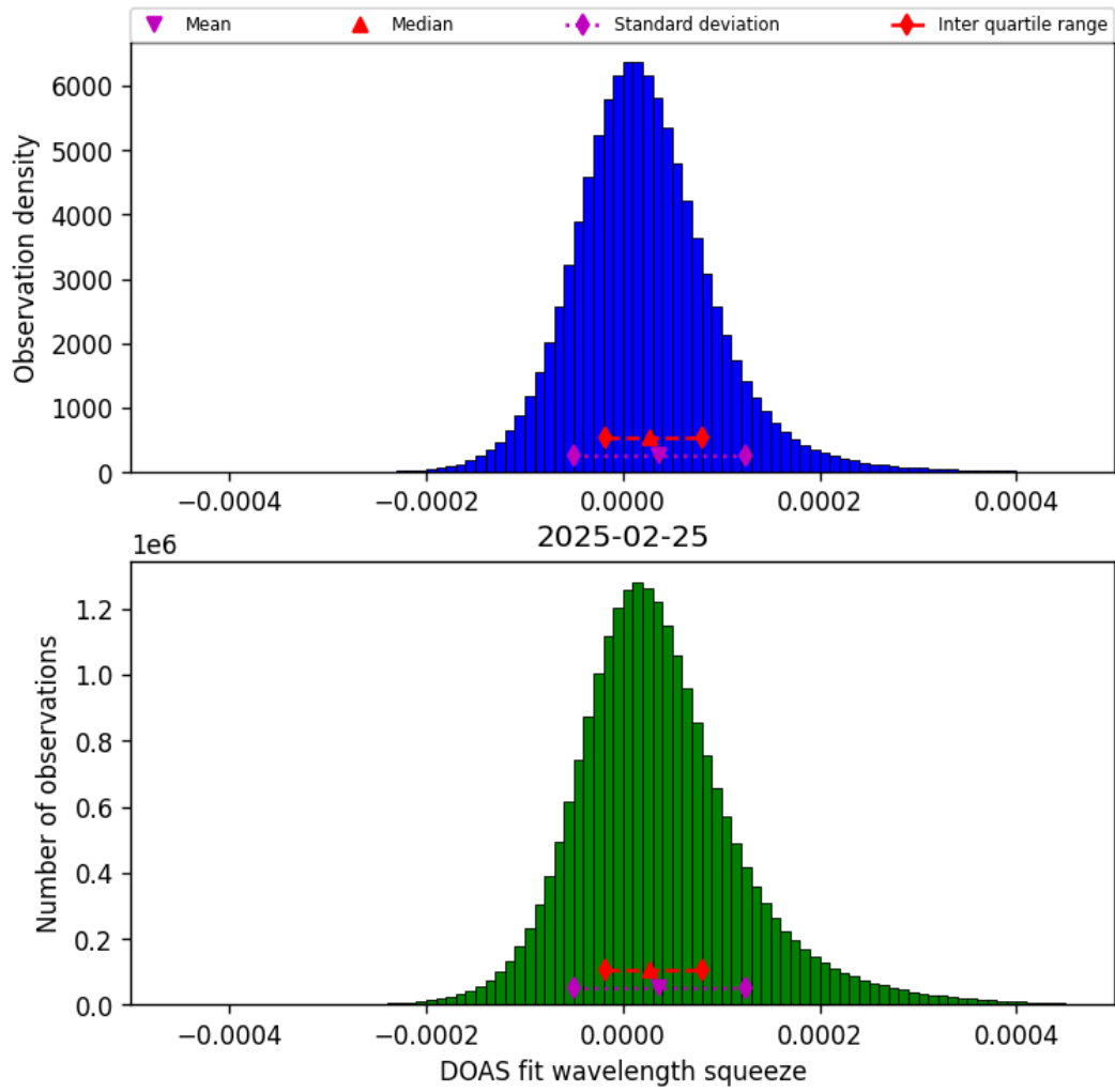
Figure 43: Histogram of “DOAS fit wavelength squeeze” for 2025-02-25 to 2025-02-26
