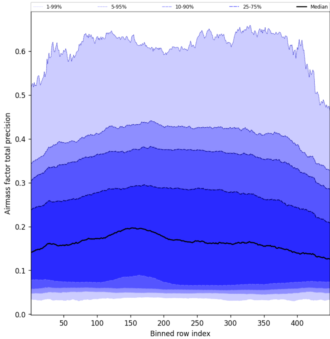
Figure 53: Along track statistics of “Airmass factor total precision” for 2025-02-25 to 2025-02-26
