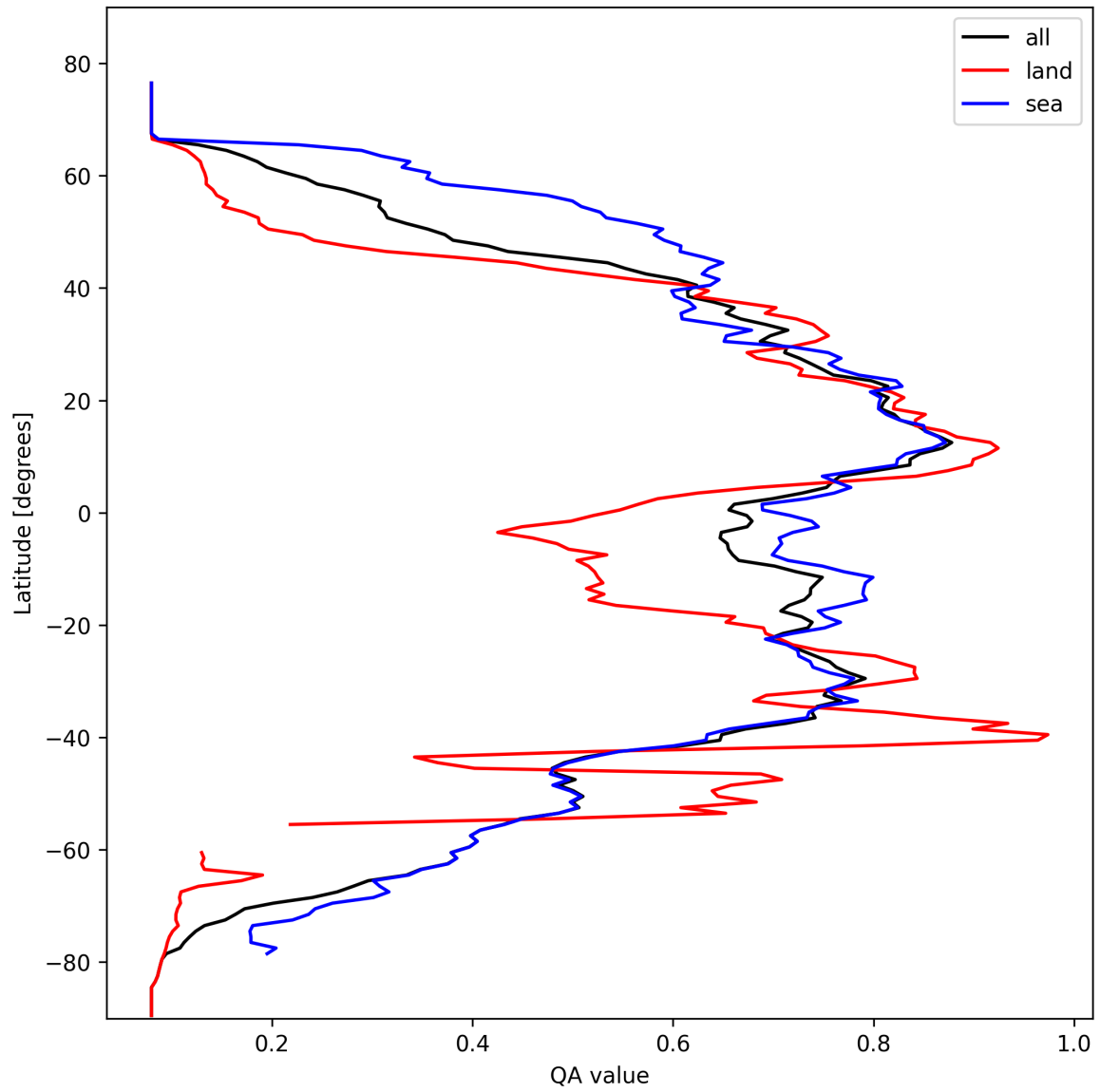
Figure 18: Zonal average of “QA value” for 2025-02-25 to 2025-02-26.
