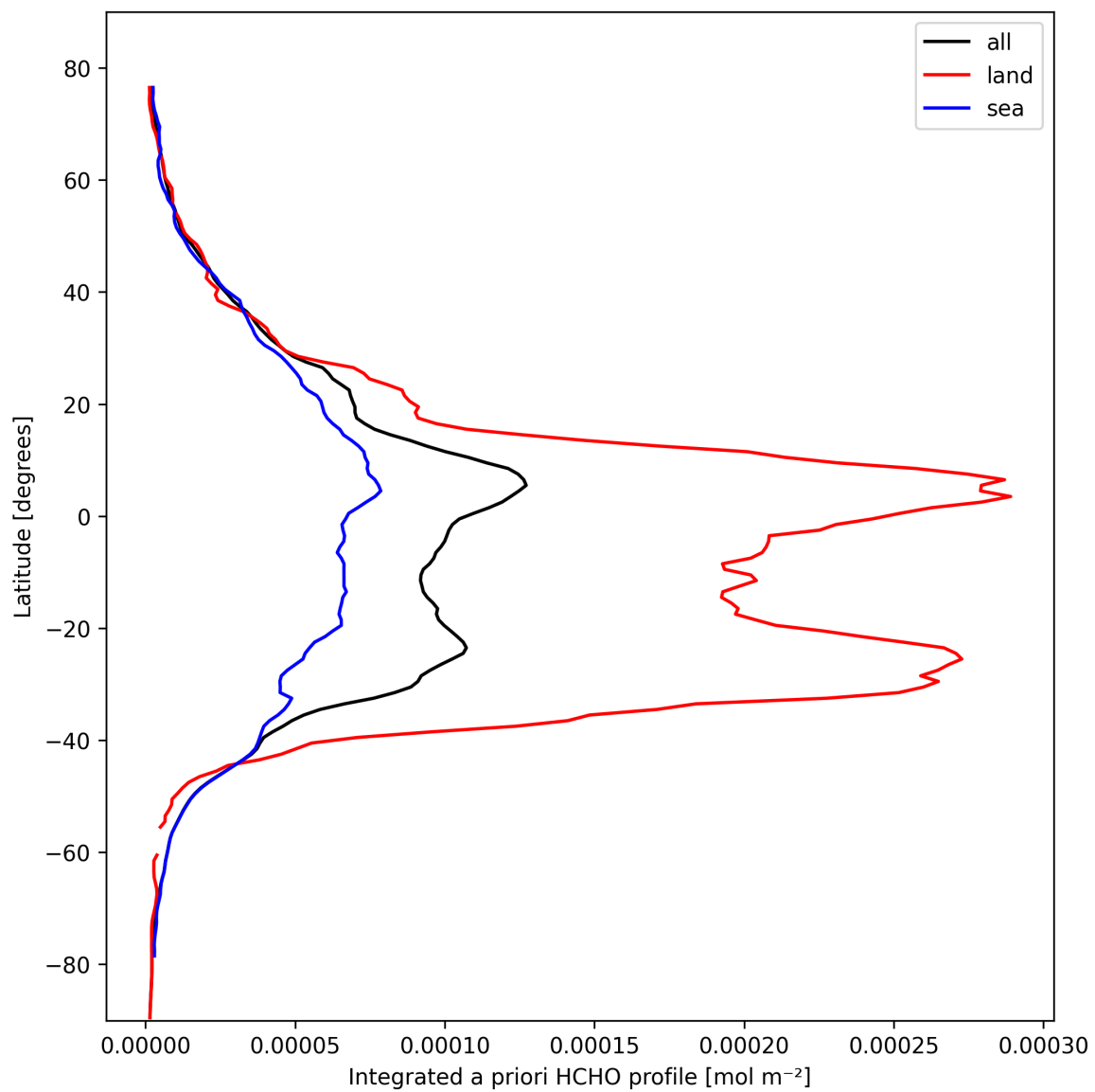
Figure 27: Zonal average of “Integrated a priori HCHO profile” for 2025-02-25 to 2025-02-26.
