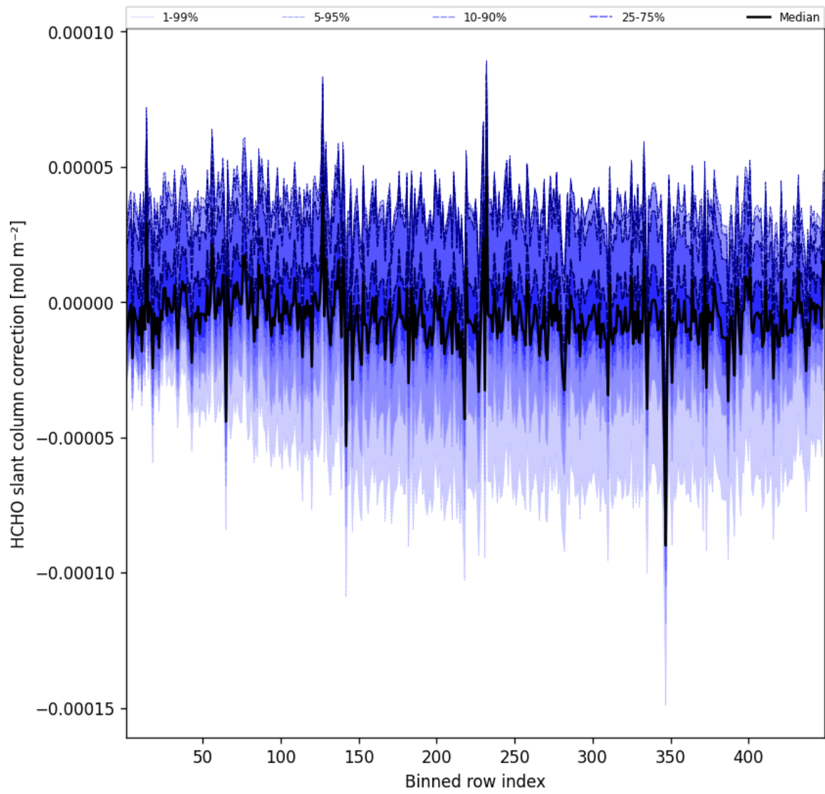
Figure 59: Along track statistics of “HCHO slant column correction” for 2025-02-25 to 2025-02-26
