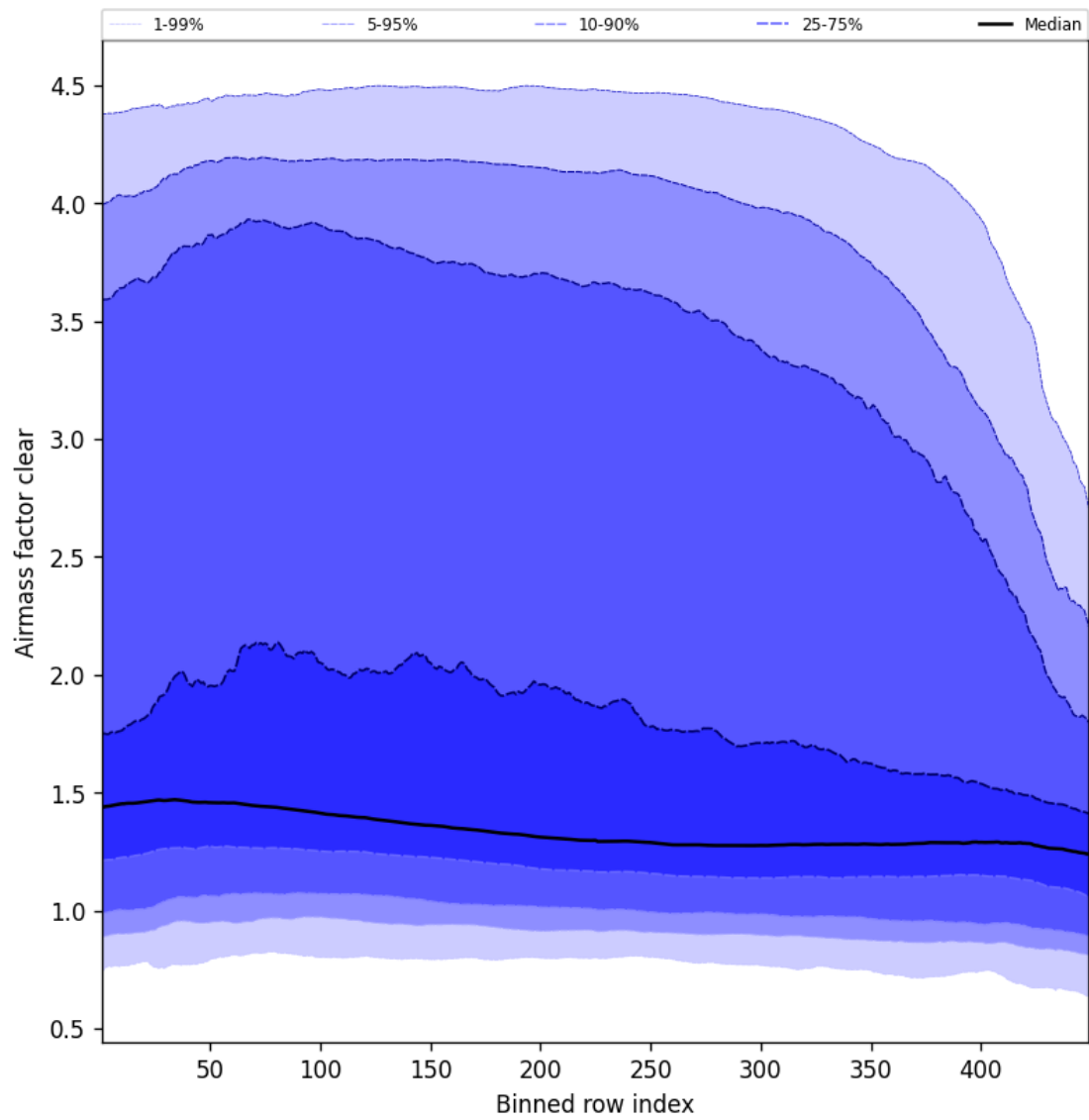
Figure 54: Along track statistics of “Air mass factor clear” for 2025-02-25 to 2025-02-26
