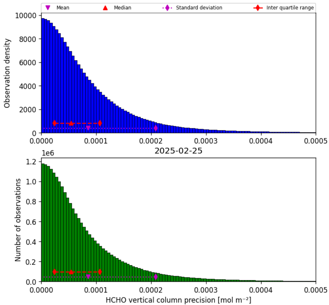
Figure 34: Histogram of “HCHO vertical column precision” for 2025-02-25 to 2025-02-26
