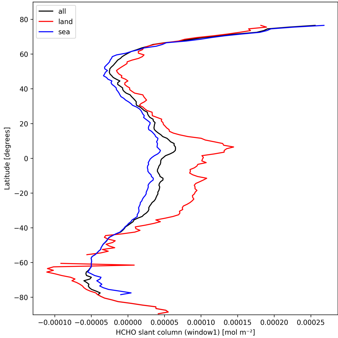
Figure 22: Zonal average of “HCHO slant column (window1)” for 2025-02-25 to 2025-02-26.
