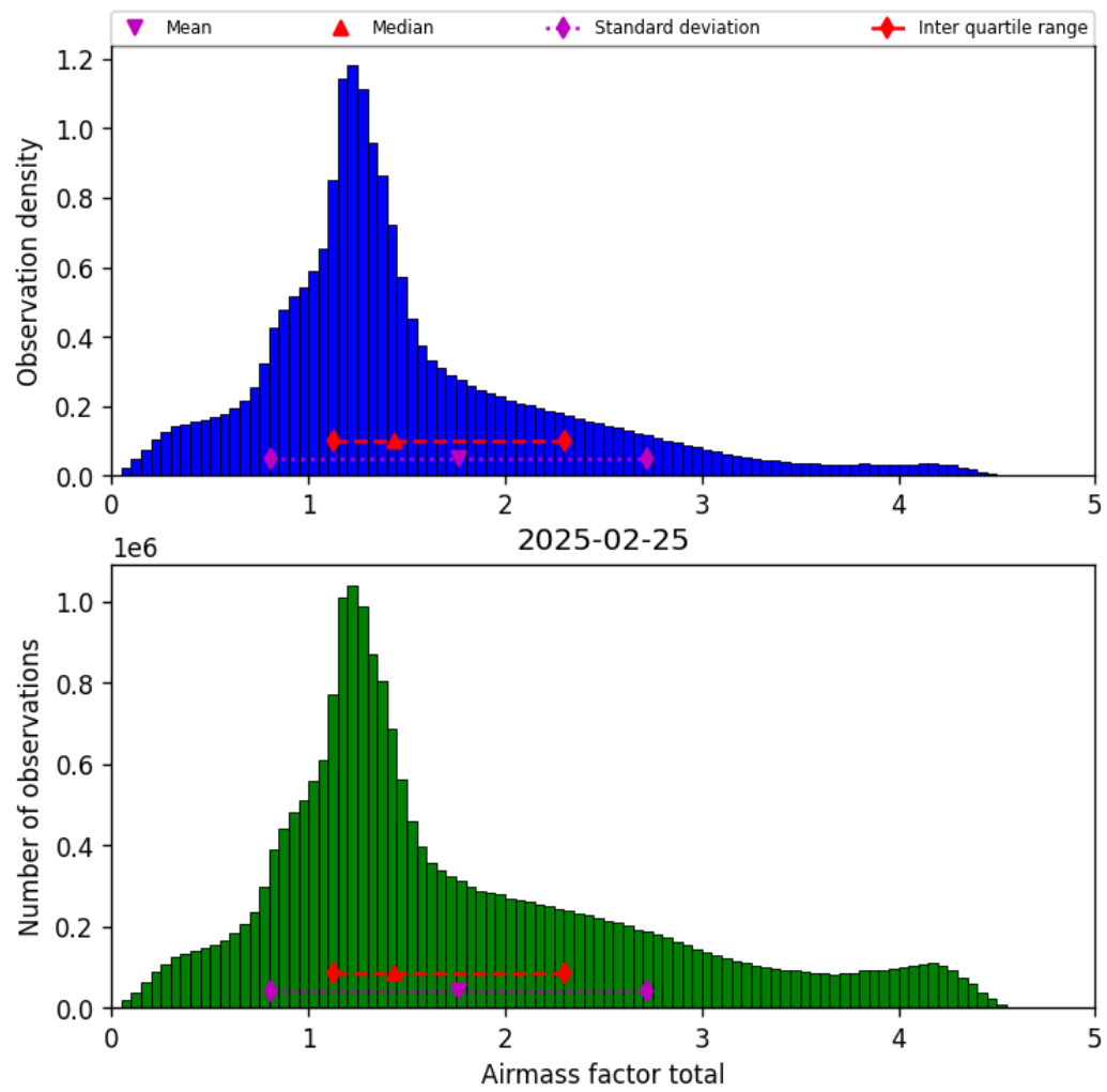
Figure 38: Histogram of “Airmass factor total” for 2025-02-25 to 2025-02-26
