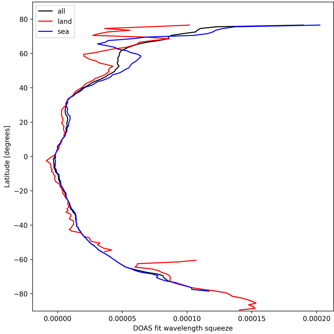
Figure 29: Zonal average of “DOAS fit wavelength squeeze” for 2025-02-25 to 2025-02-26.
