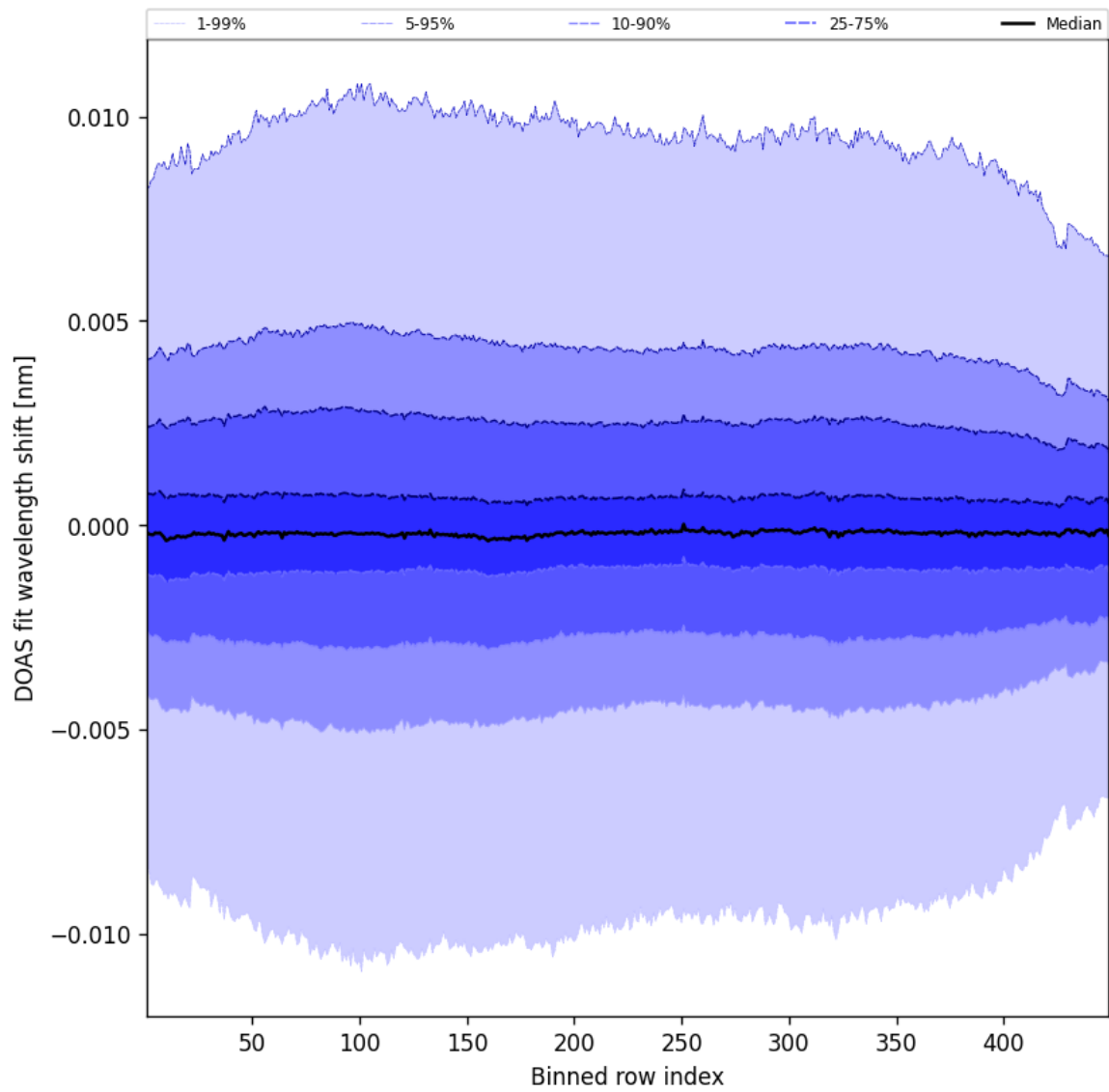
Figure 56: Along track statistics of “DOAS fit wavelength shift” for 2025-02-25 to 2025-02-26
