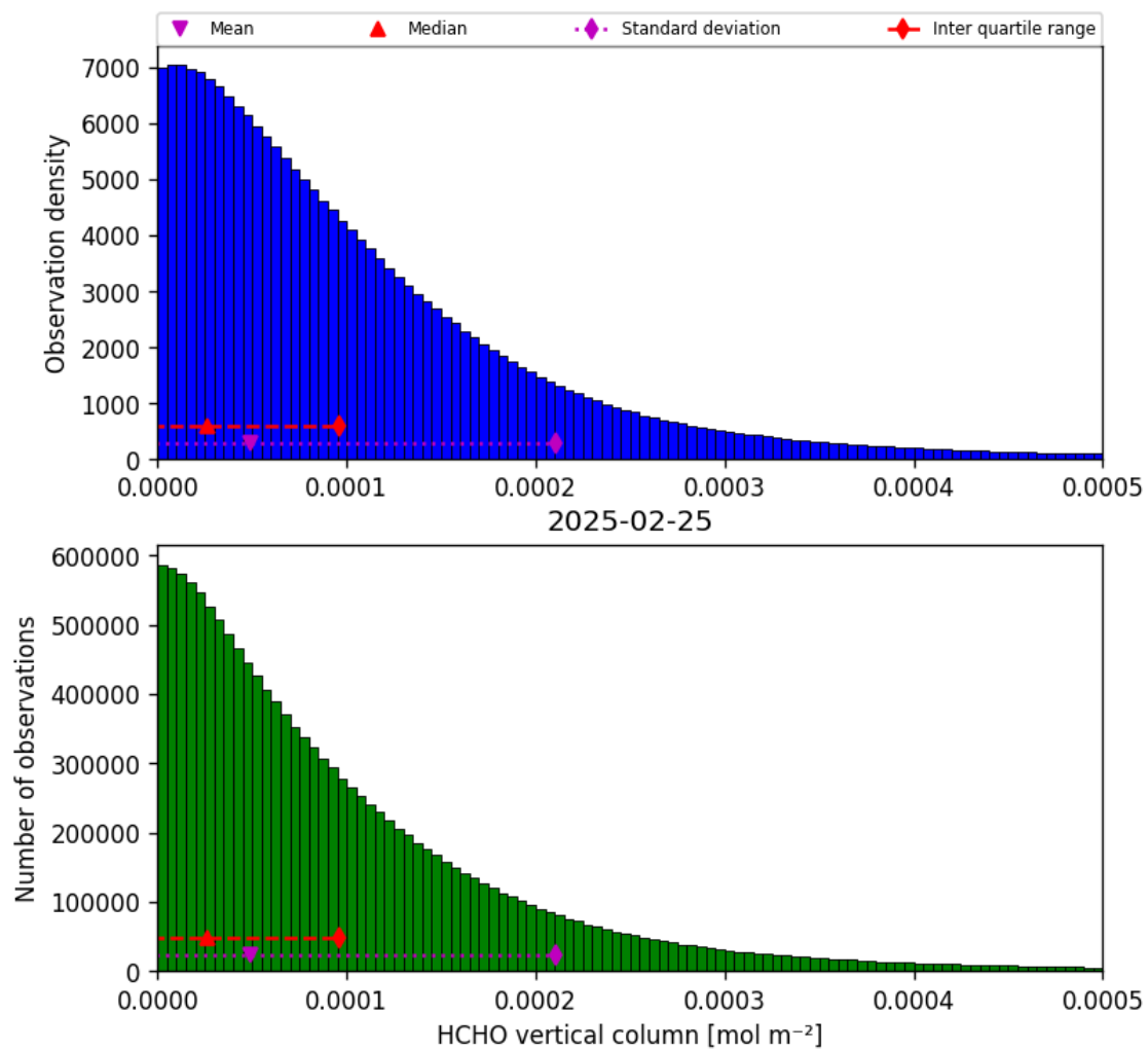
Figure 33: Histogram of “HCHO vertical column” for 2025-02-25 to 2025-02-26
