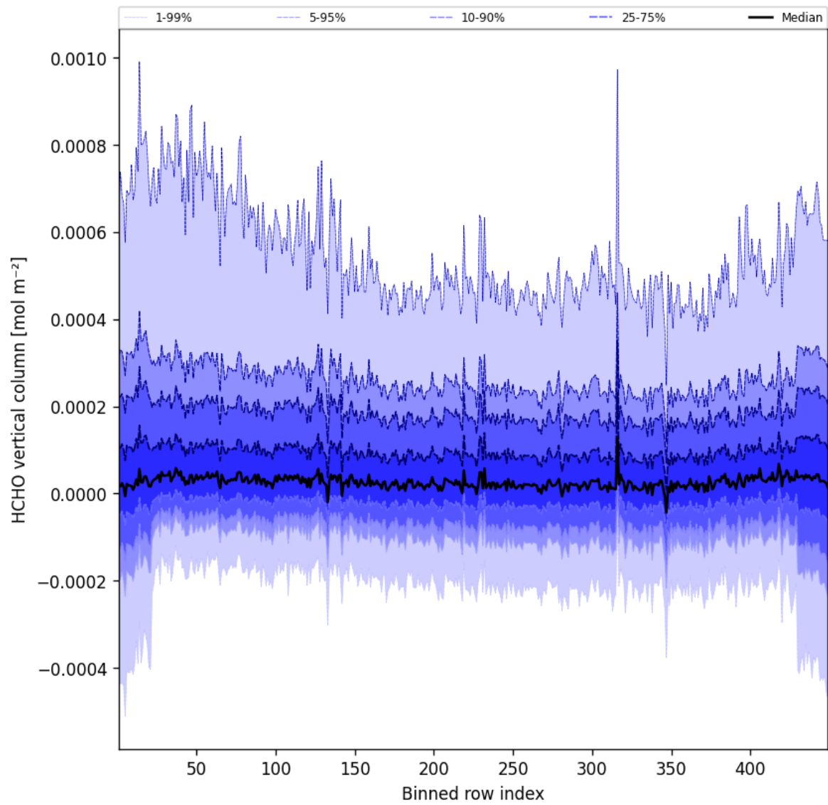
Figure 47: Along track statistics of “HCHO vertical column” for 2025-02-25 to 2025-02-26
