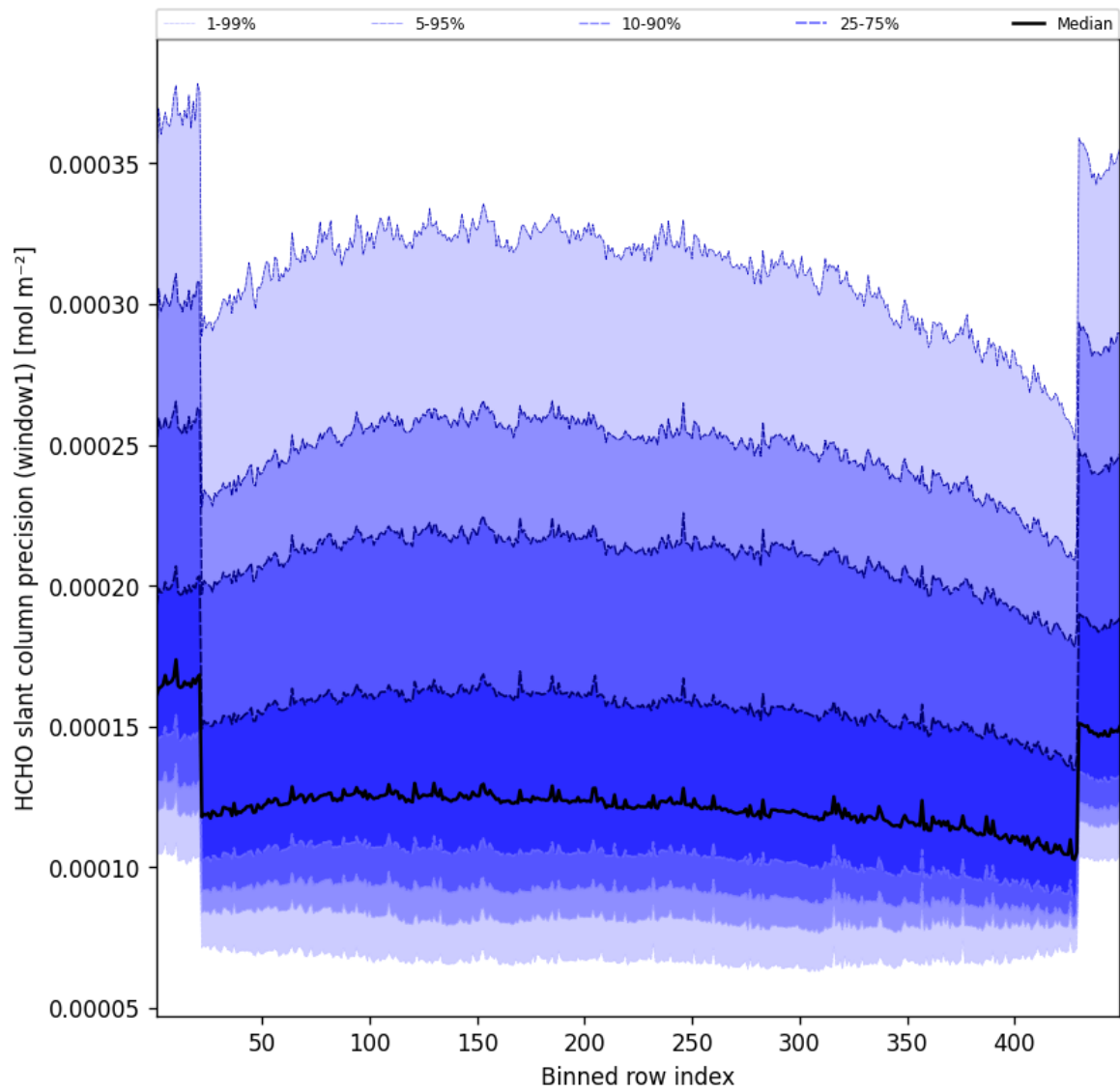
Figure 51: Along track statistics of “HCHO slant column precision (window1)” for 2025-02-25 to 2025-02-26
