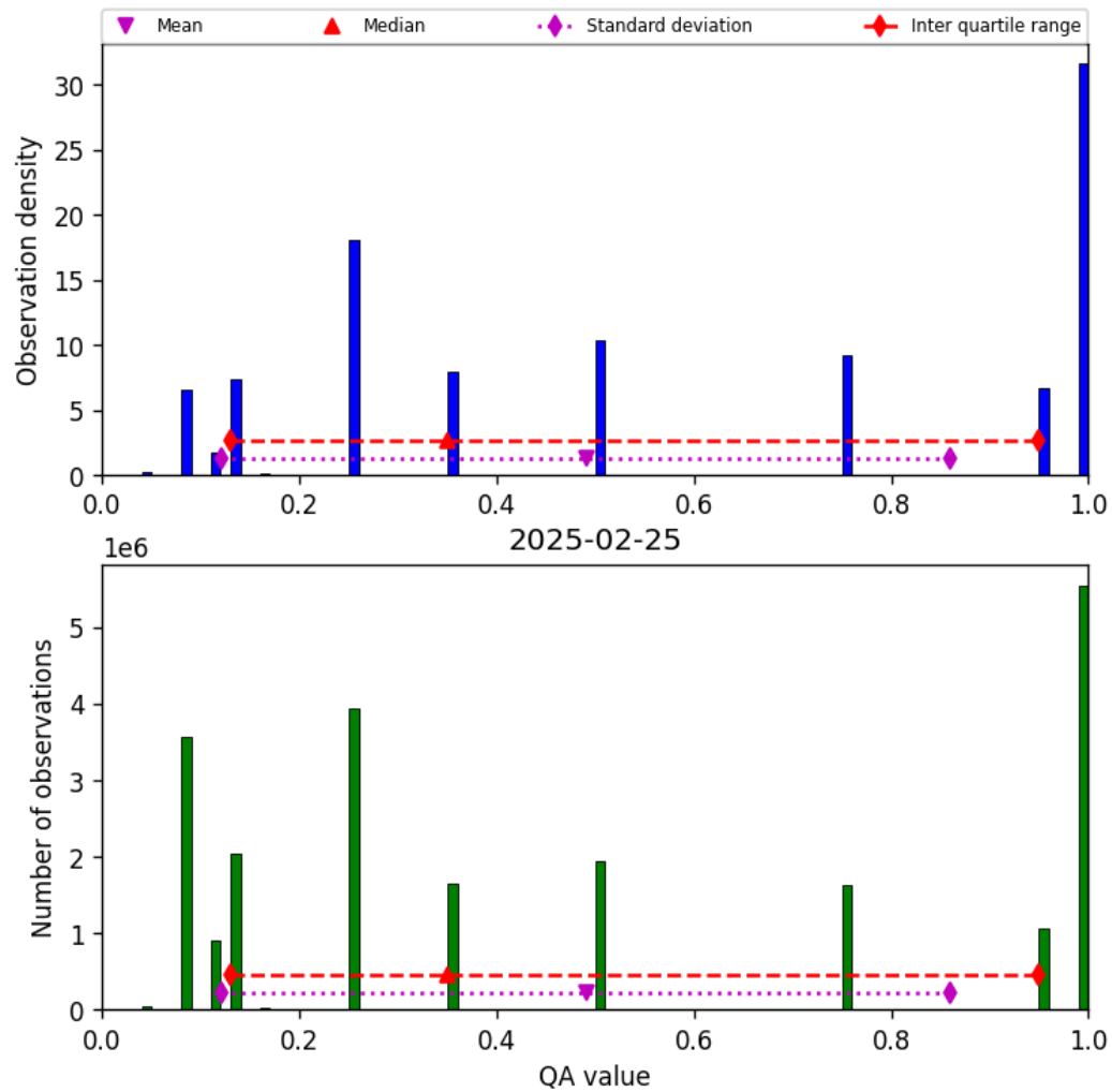
Figure 32: Histogram of “QA value” for 2025-02-25 to 2025-02-26
