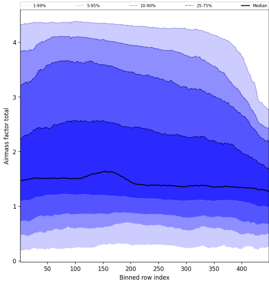
Figure 52: Along track statistics of “Airmass factor total” for 2025-02-25 to 2025-02-26
