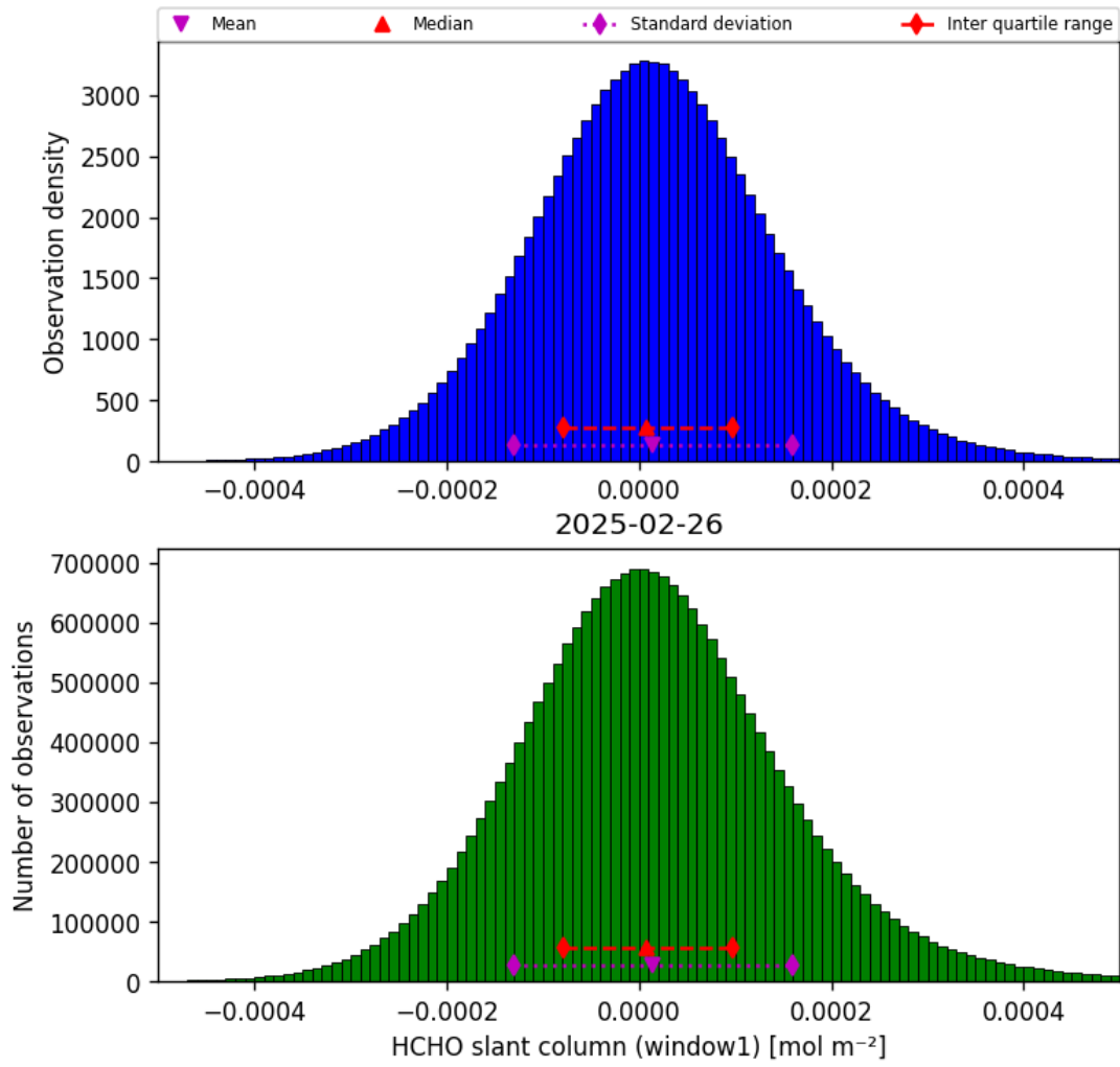
Figure 36: Histogram of “HCHO slant column (window1)” for 2025-02-26 to 2025-02-27
