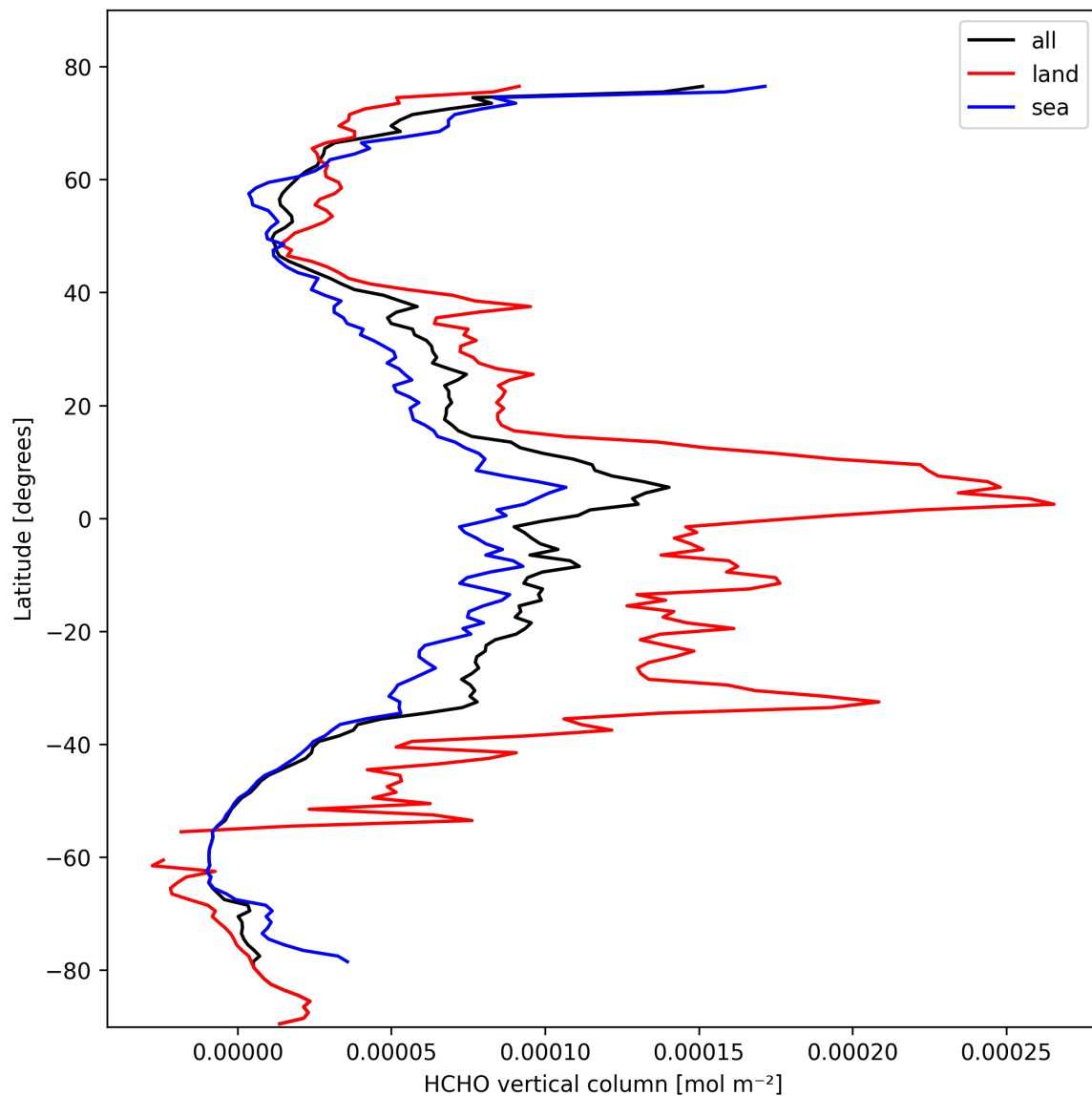
Figure 19: Zonal average of “HCHO vertical column” for 2025-02-26 to 2025-02-27.
