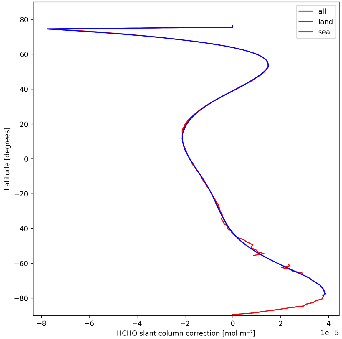
Figure 31: Zonal average of “HCHO slant column correction” for 2025-02-26 to 2025-02-27.
