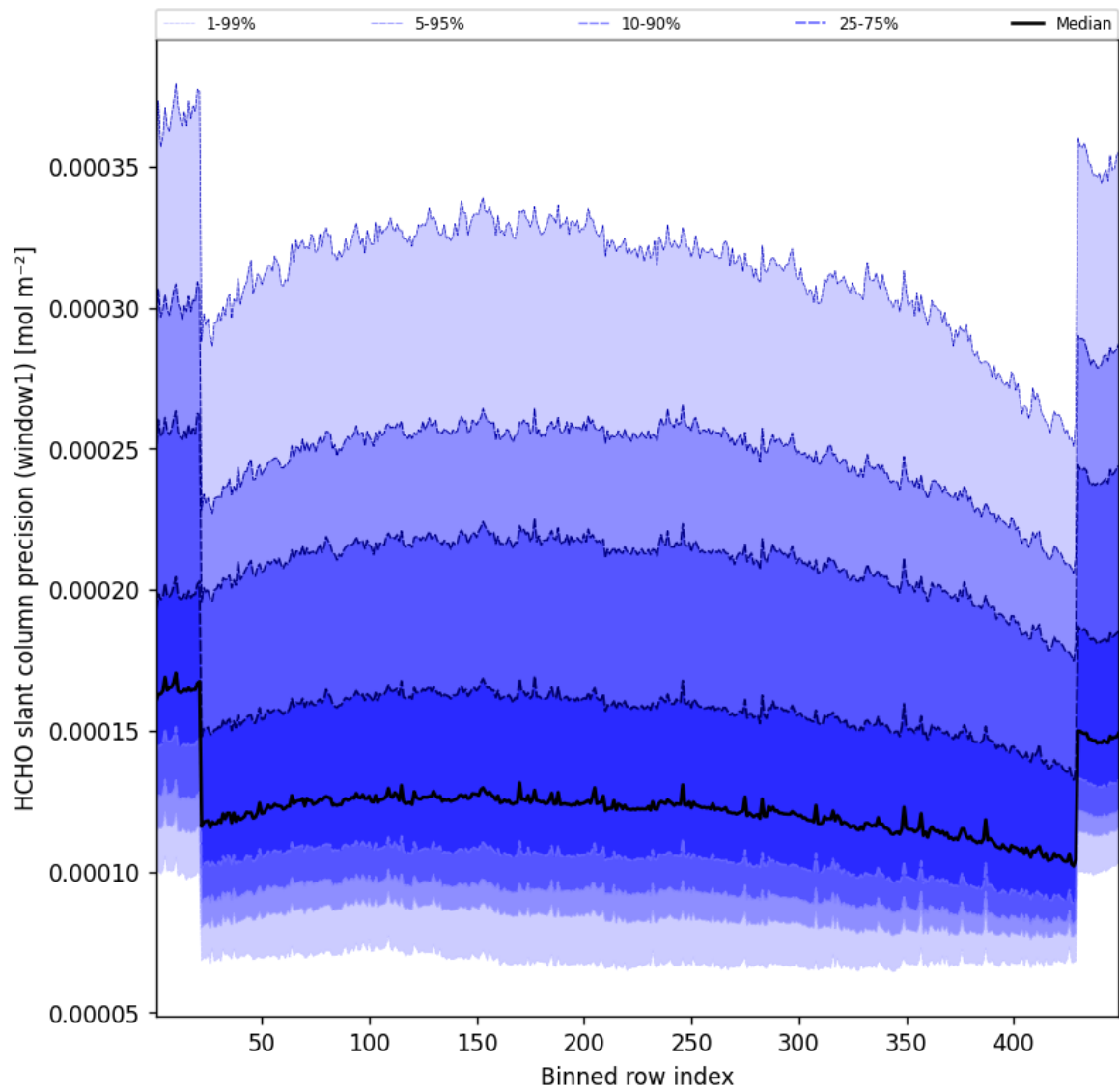
Figure 51: Along track statistics of “HCHO slant column precision (window1)” for 2025-02-26 to 2025-02-27
