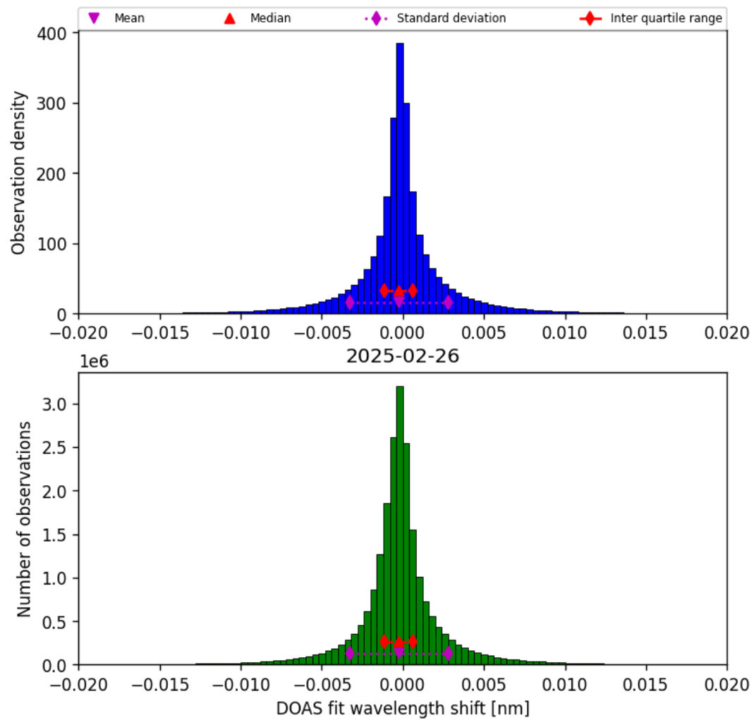
Figure 42: Histogram of “DOAS fit wavelength shift” for 2025-02-26 to 2025-02-27
