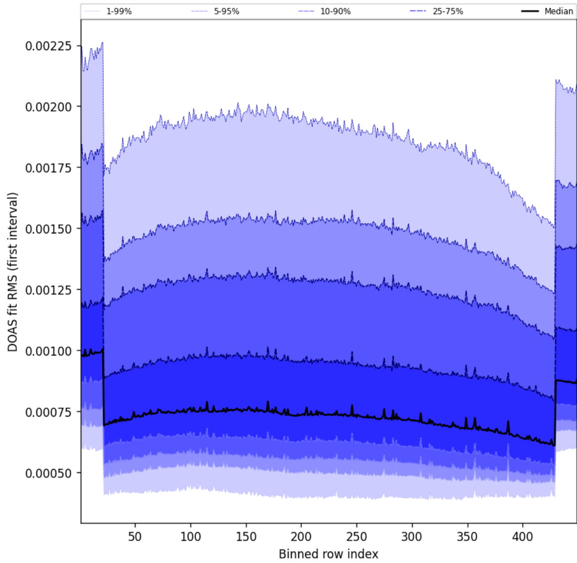
Figure 58: Along track statistics of “DOAS fit RMS (first interval)” for 2025-02-26 to 2025-02-27
