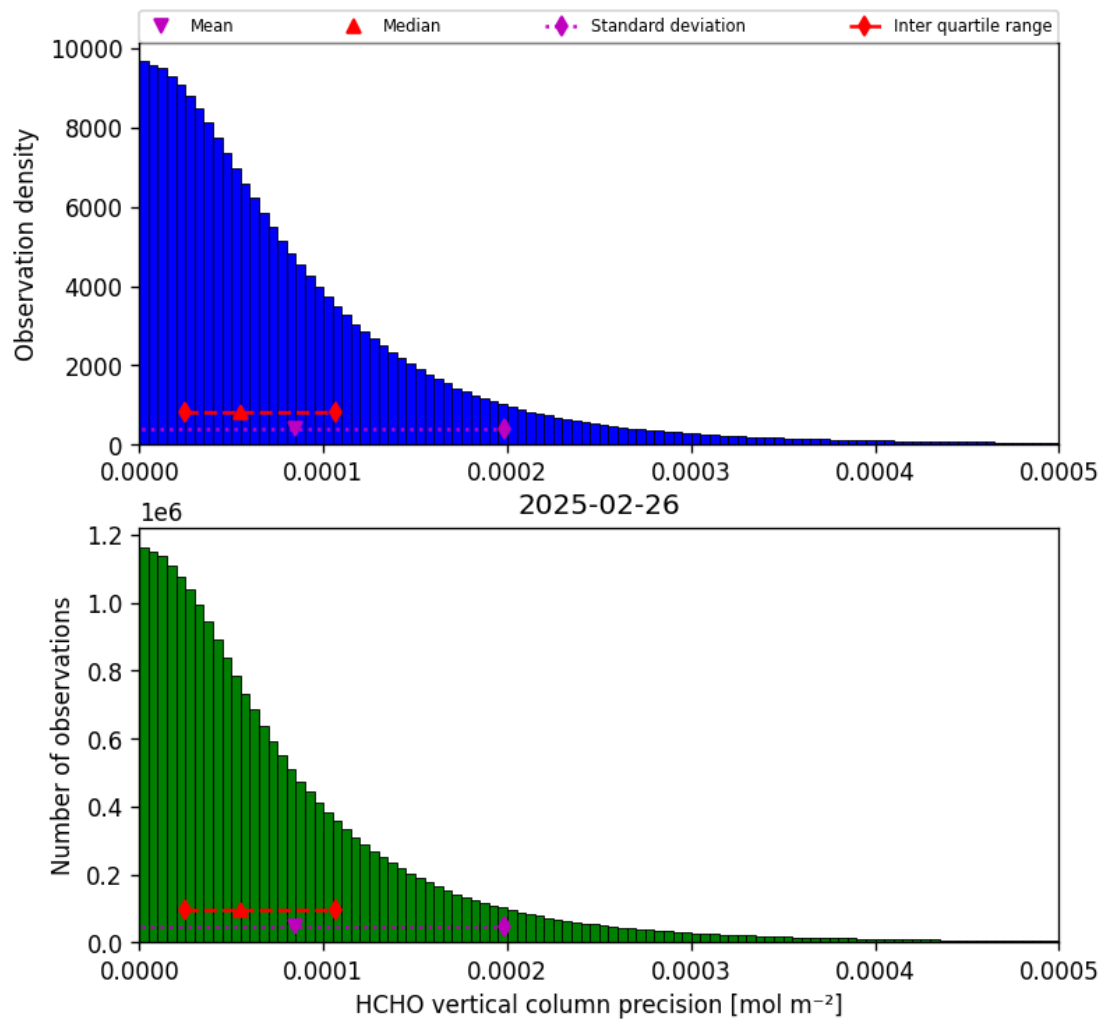
Figure 34: Histogram of “HCHO vertical column precision” for 2025-02-26 to 2025-02-27
