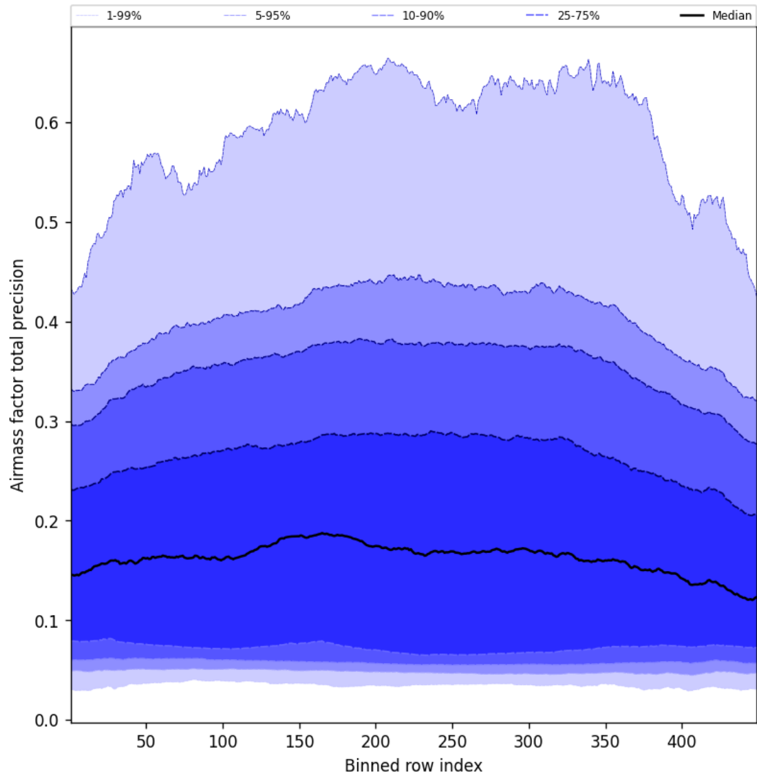
Figure 53: Along track statistics of “Airmass factor total precision” for 2025-02-26 to 2025-02-27
