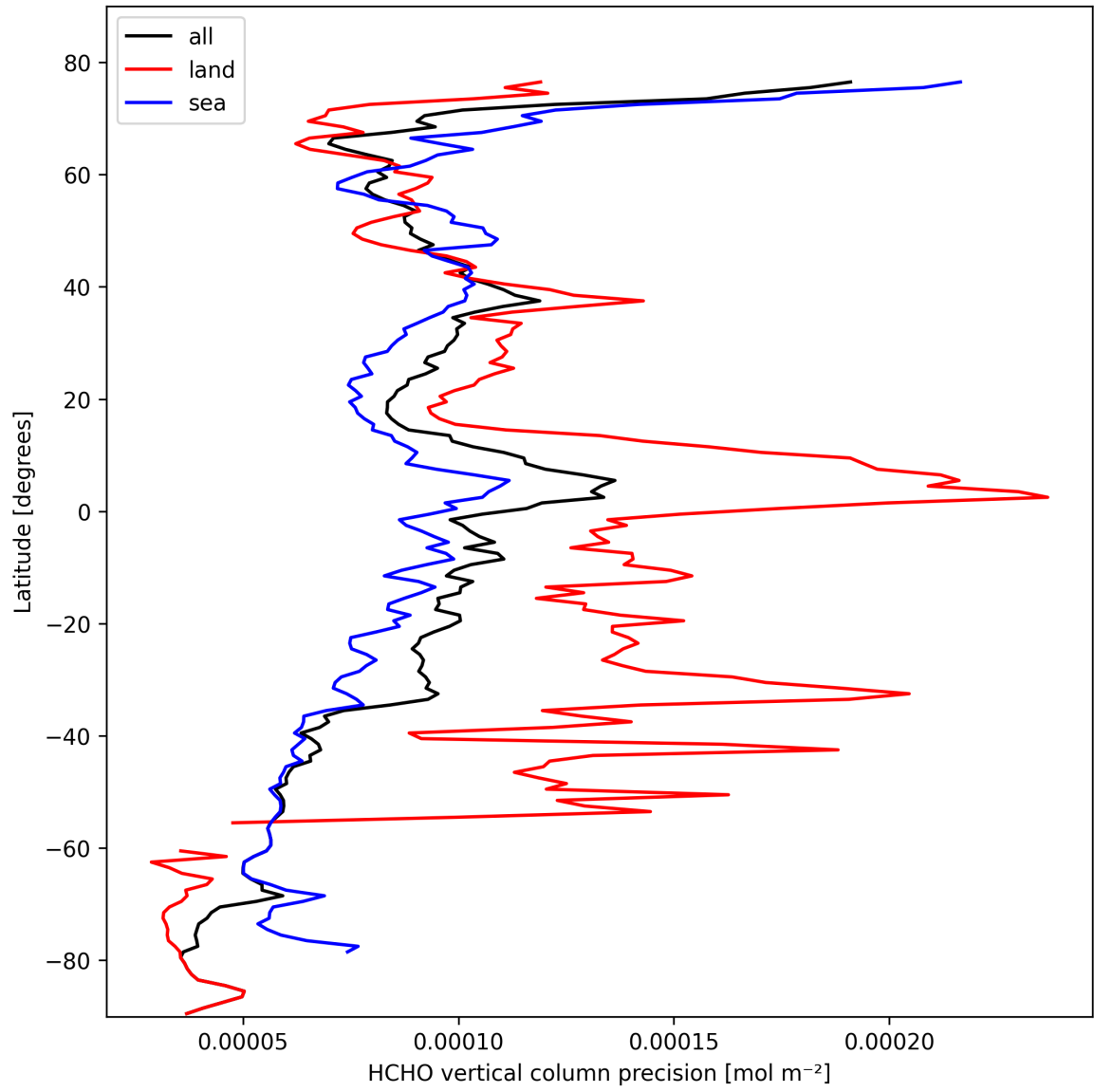
Figure 20: Zonal average of “HCHO vertical column precision” for 2025-02-26 to 2025-02-27.
