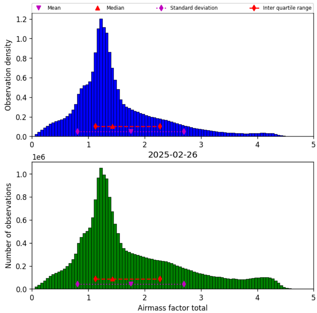
Figure 38: Histogram of “Airmass factor total” for 2025-02-26 to 2025-02-27
