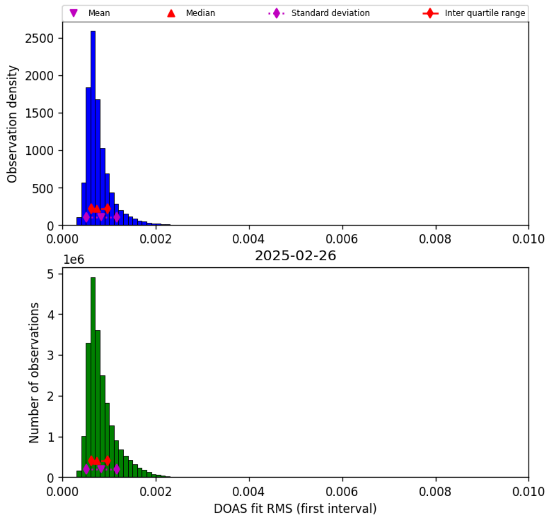
Figure 44: Histogram of “DOAS fit RMS (first interval)” for 2025-02-26 to 2025-02-27
