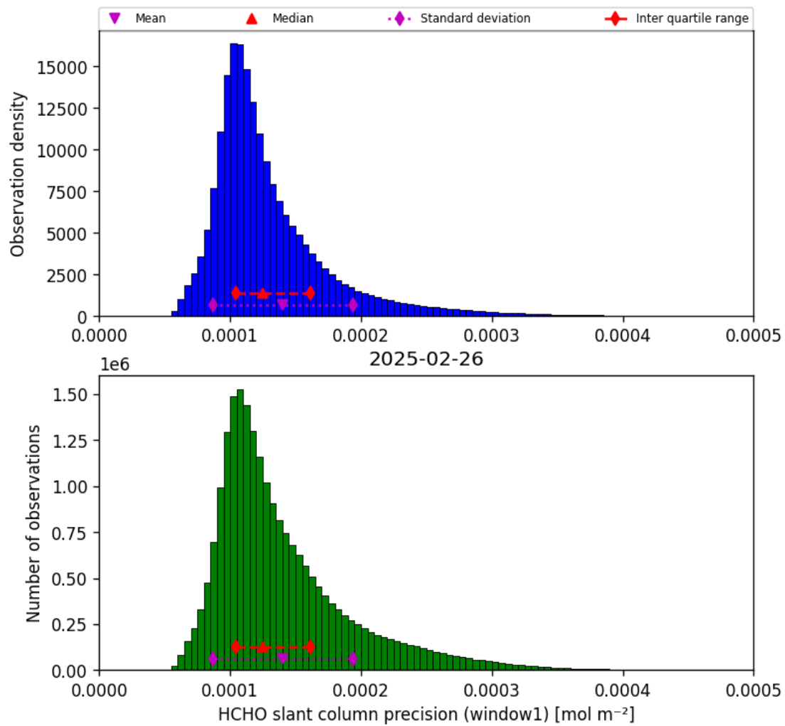
Figure 37: Histogram of “HCHO slant column precision (window1)” for 2025-02-26 to 2025-02-27
