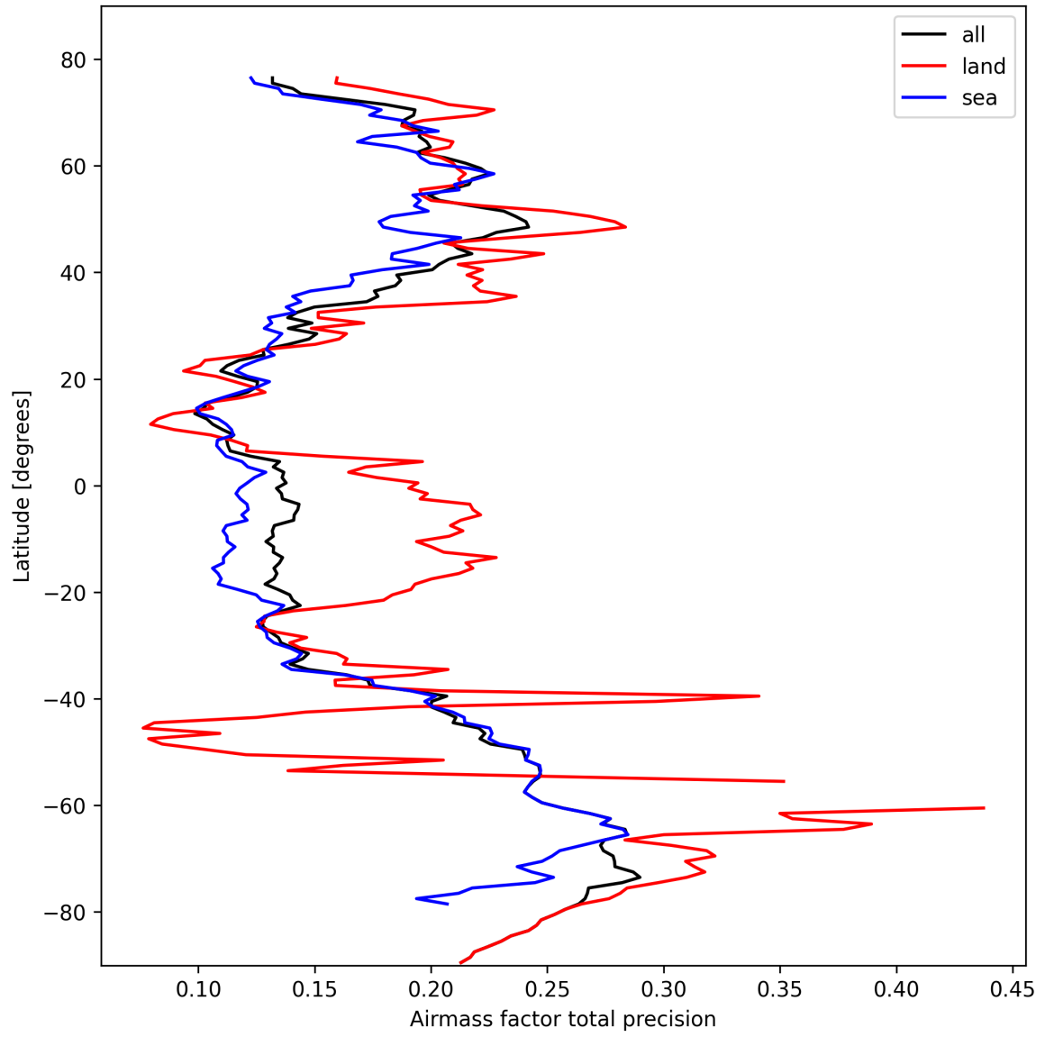
Figure 25: Zonal average of “Airmass factor total precision” for 2025-02-26 to 2025-02-27.
