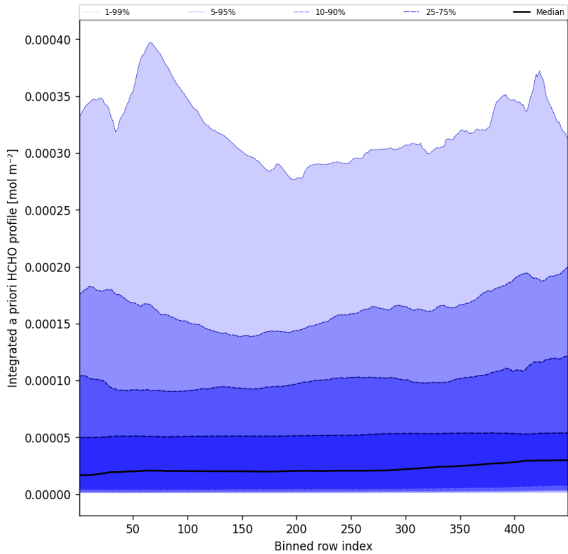
Figure 55: Along track statistics of “Integrated a priori HCHO profile” for 2025-02-26 to 2025-02-27
