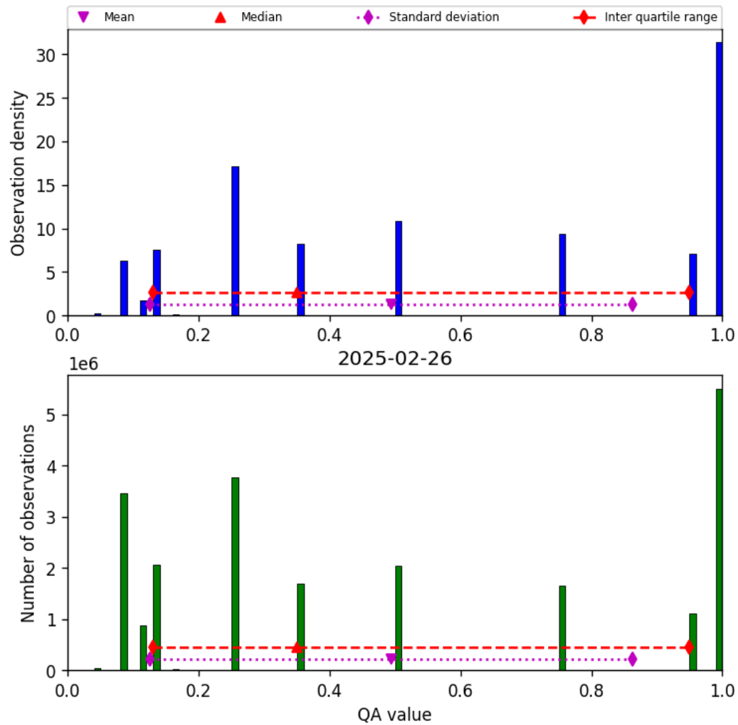
Figure 32: Histogram of “QA value” for 2025-02-26 to 2025-02-27
