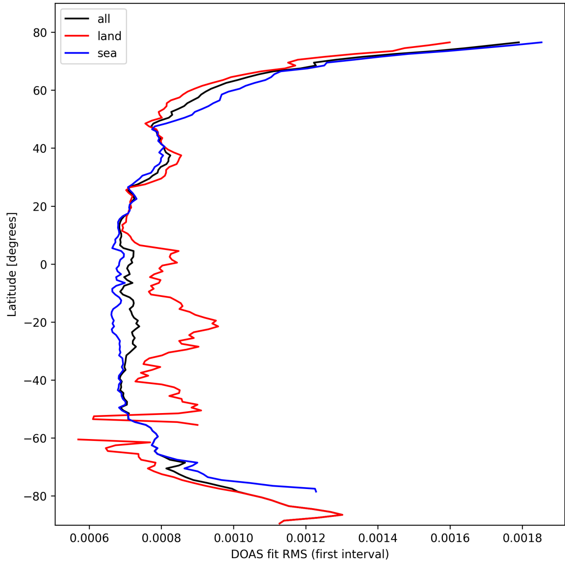
Figure 30: Zonal average of “DOAS fit RMS (first interval)” for 2025-02-26 to 2025-02-27.
