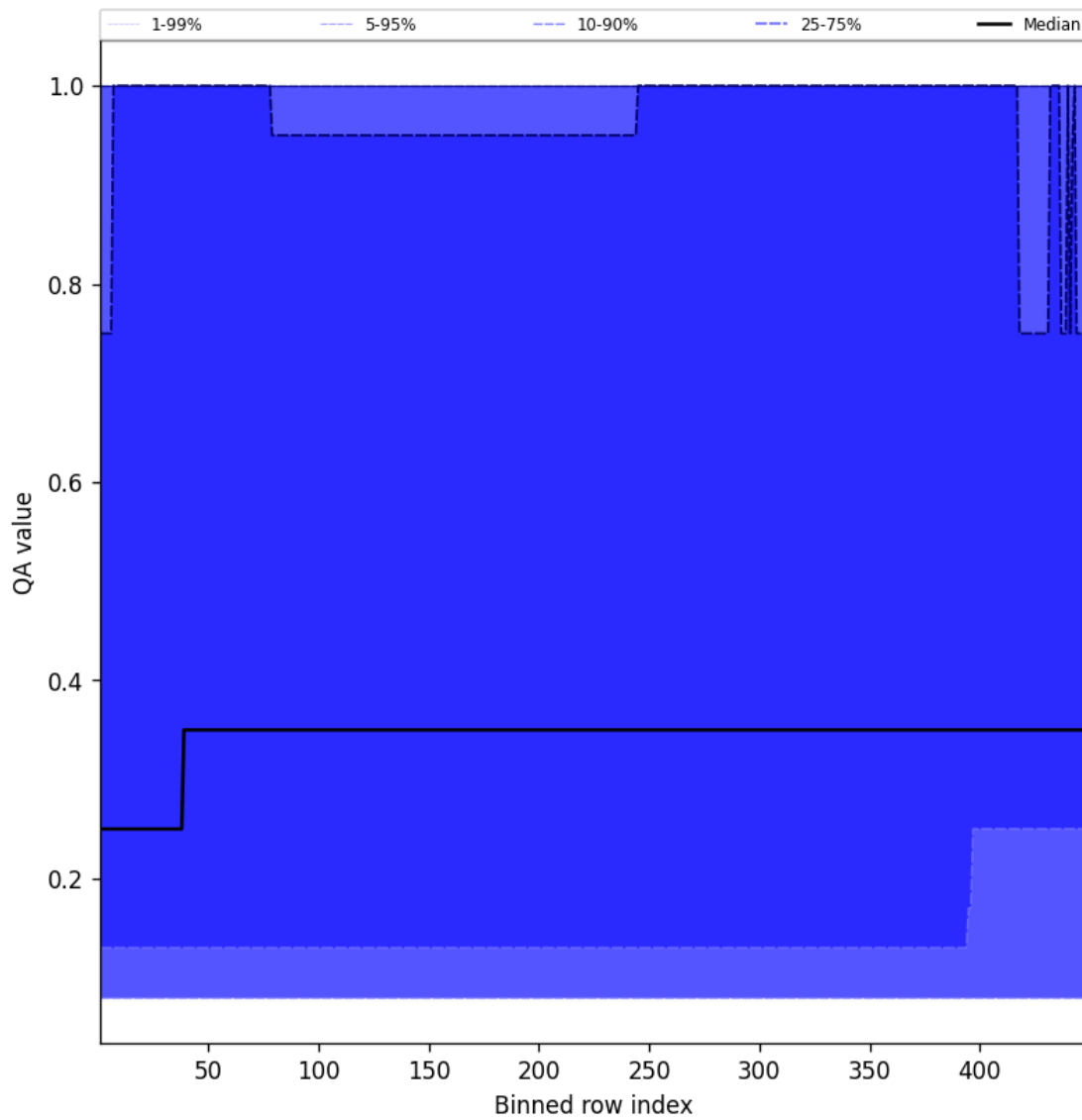
Figure 46: Along track statistics of “QA value” for 2025-02-26 to 2025-02-27
