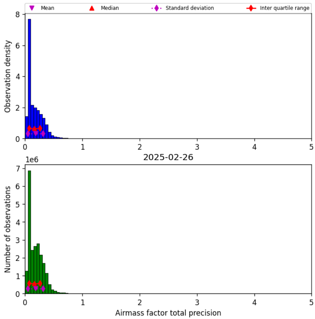
Figure 39: Histogram of “Airmass factor total precision” for 2025-02-26 to 2025-02-27
