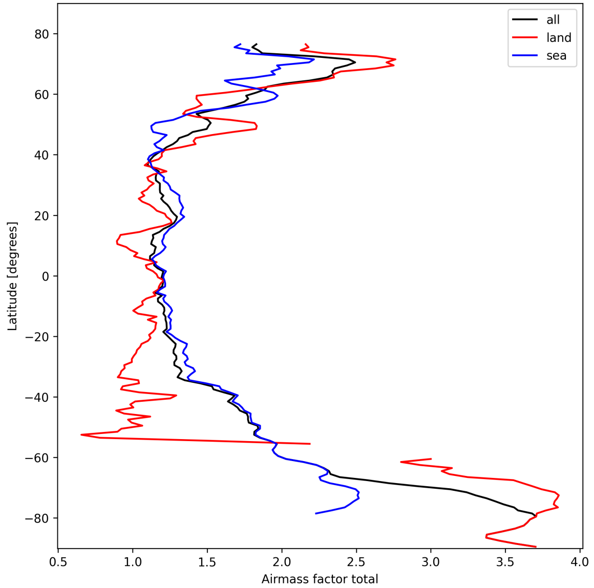
Figure 24: Zonal average of “Airmass factor total” for 2025-02-26 to 2025-02-27.
