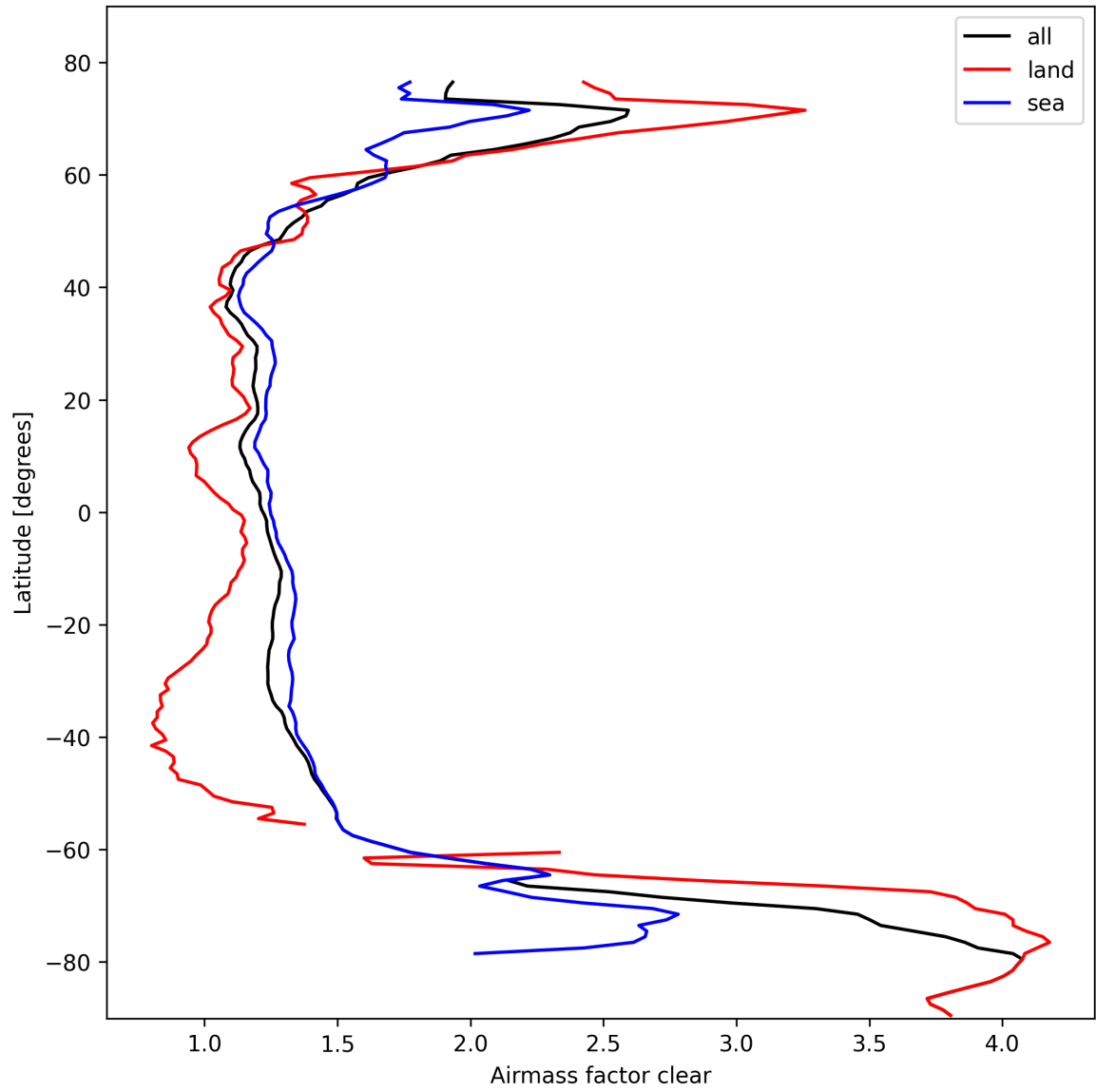
Figure 26: Zonal average of “Airmass factor clear” for 2025-02-26 to 2025-02-27.
