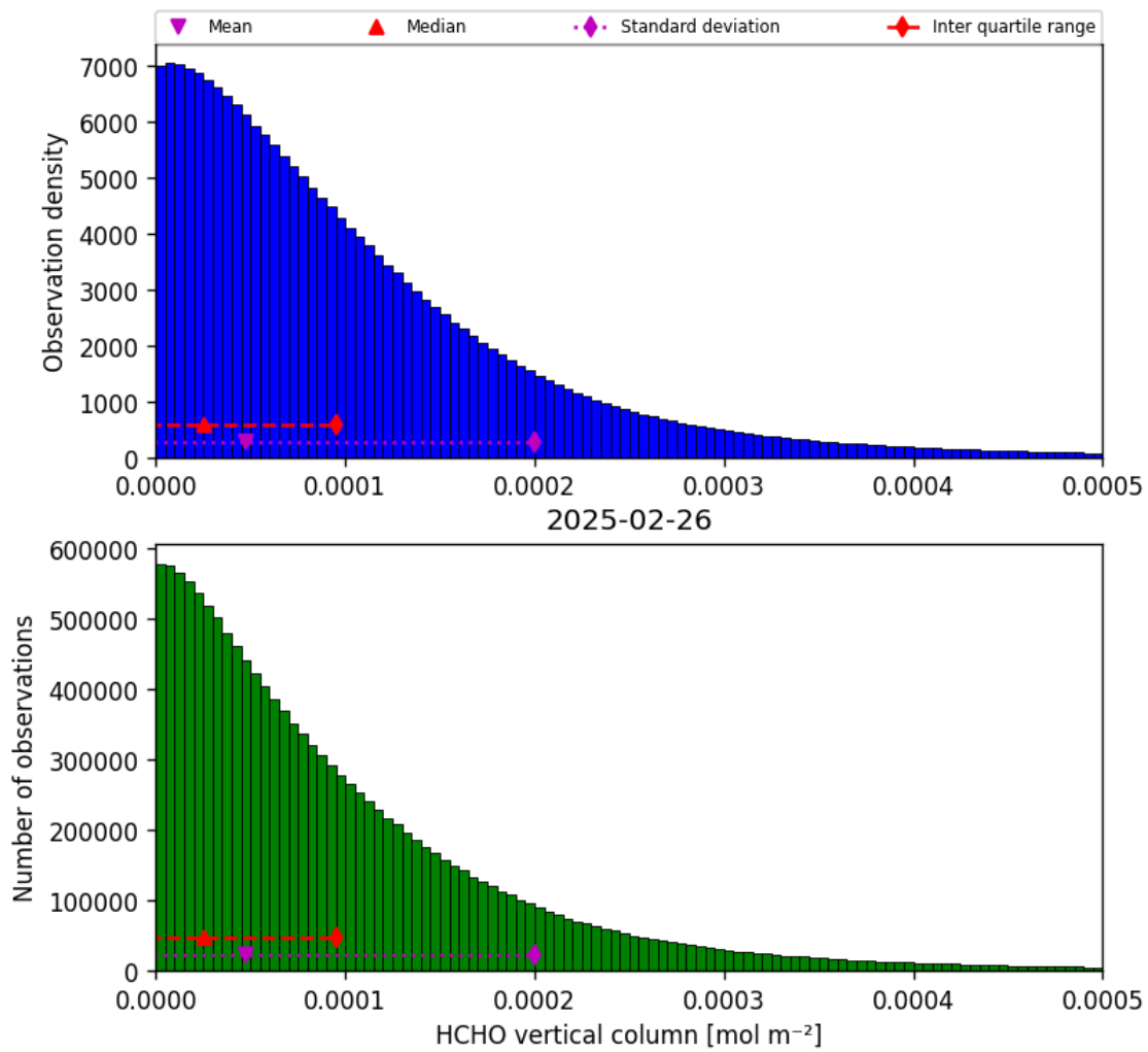
Figure 33: Histogram of “HCHO vertical column” for 2025-02-26 to 2025-02-27
