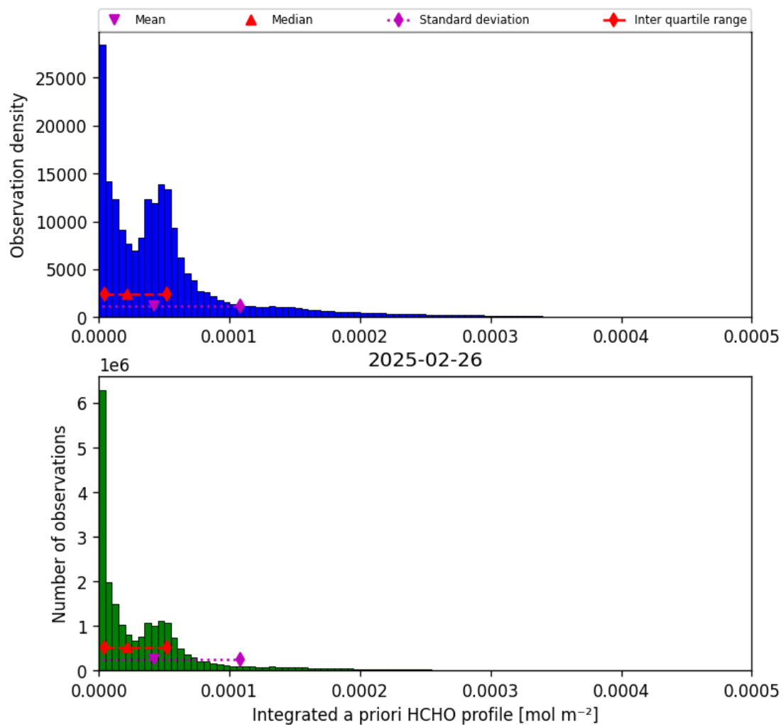
Figure 41: Histogram of “Integrated a priori HCHO profile” for 2025-02-26 to 2025-02-27
