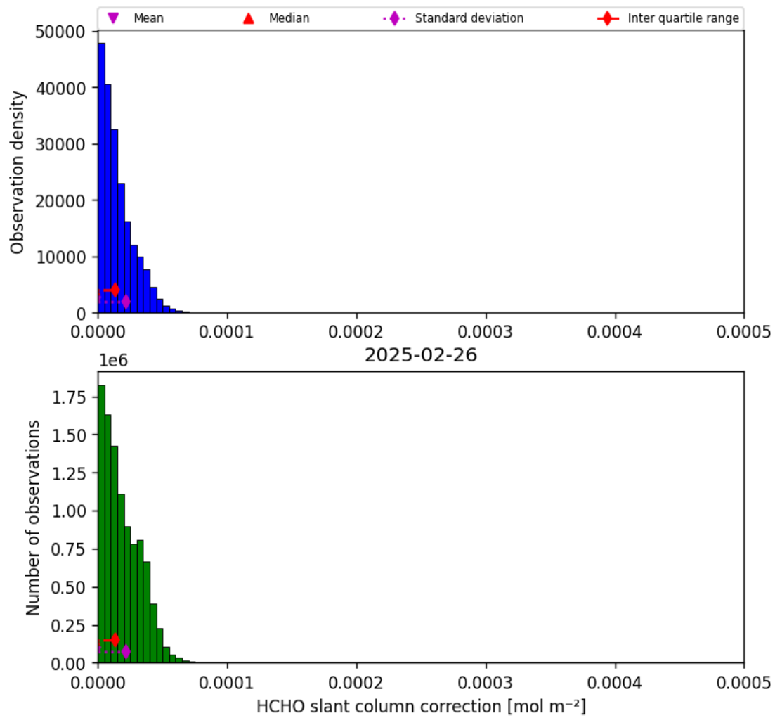
Figure 45: Histogram of “HCHO slant column correction” for 2025-02-26 to 2025-02-27
