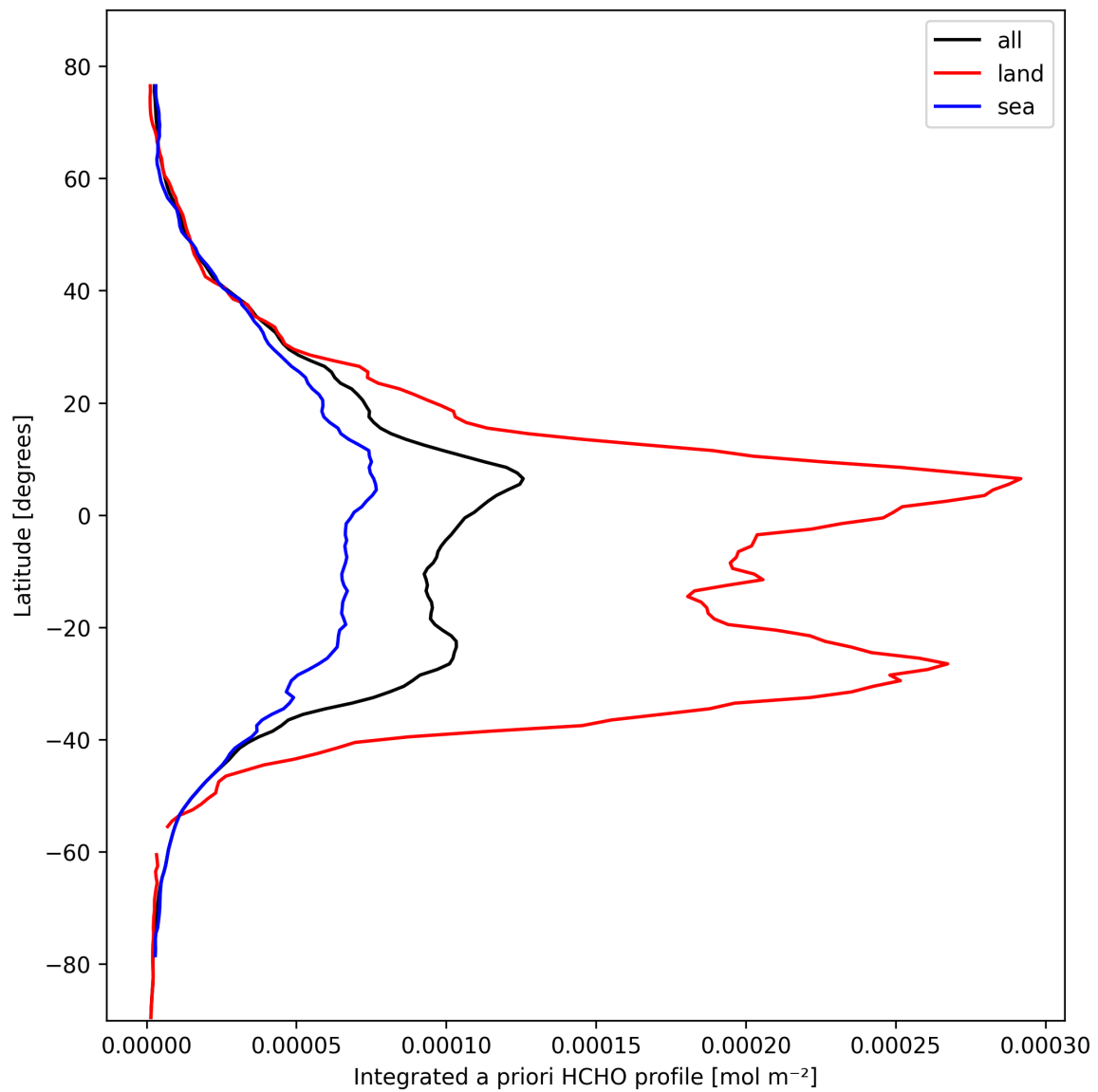
Figure 27: Zonal average of “Integrated a priori HCHO profile” for 2025-02-26 to 2025-02-27.
