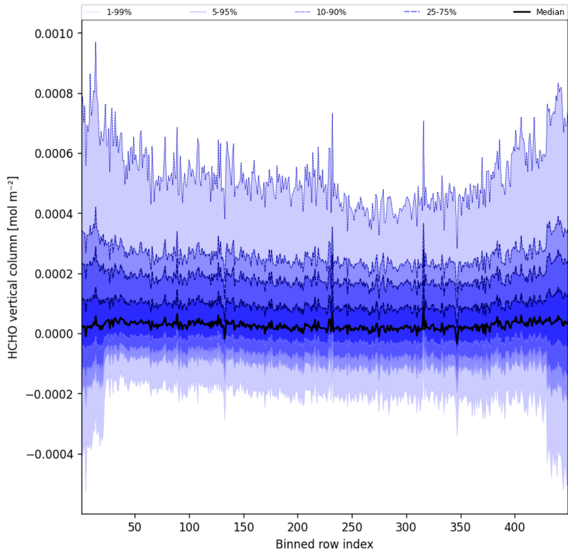
Figure 47: Along track statistics of “HCHO vertical column” for 2025-02-26 to 2025-02-27
