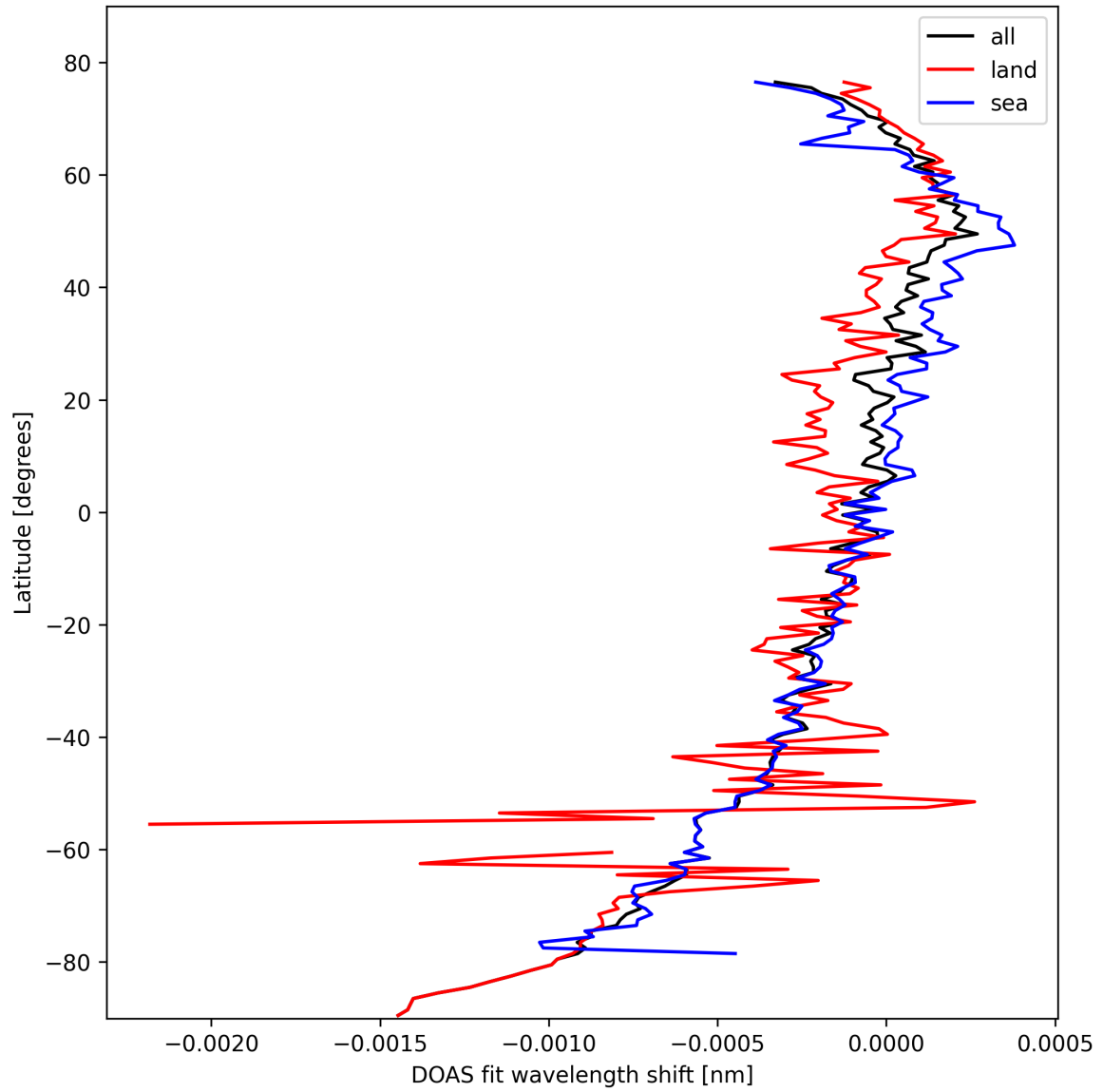
Figure 28: Zonal average of "DOAS fit wavelength shift" for 2025-02-26 to 2025-02-27.
