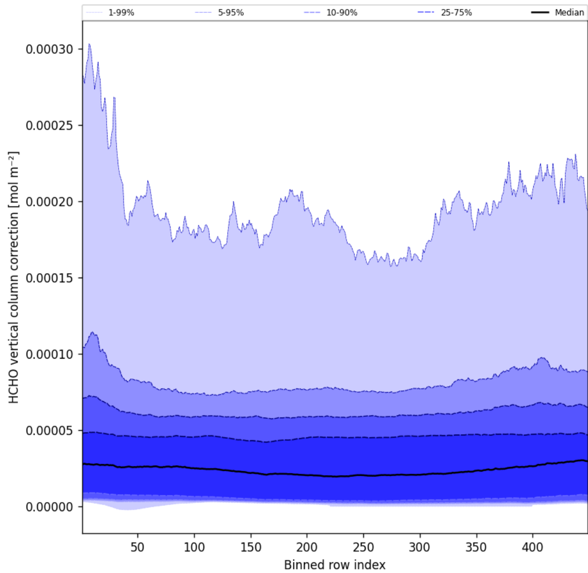
Figure 49: Along track statistics of “HCHO vertical column correction” for 2025-02-26 to 2025-02-27
