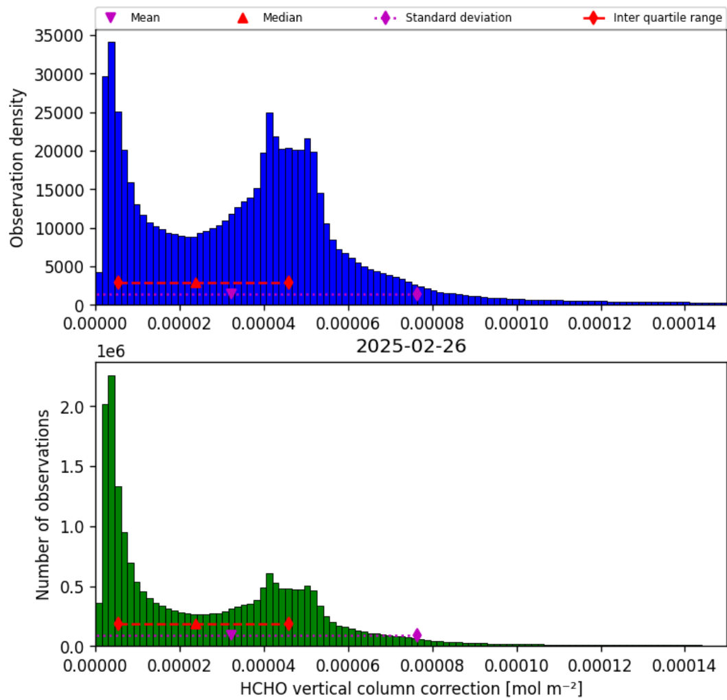
Figure 35: Histogram of “HCHO vertical column correction” for 2025-02-26 to 2025-02-27
