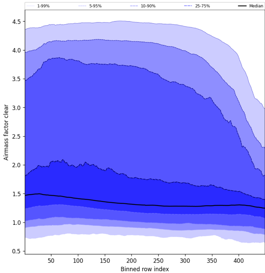
Figure 54: Along track statistics of “Air mass factor clear” for 2025-02-26 to 2025-02-27
