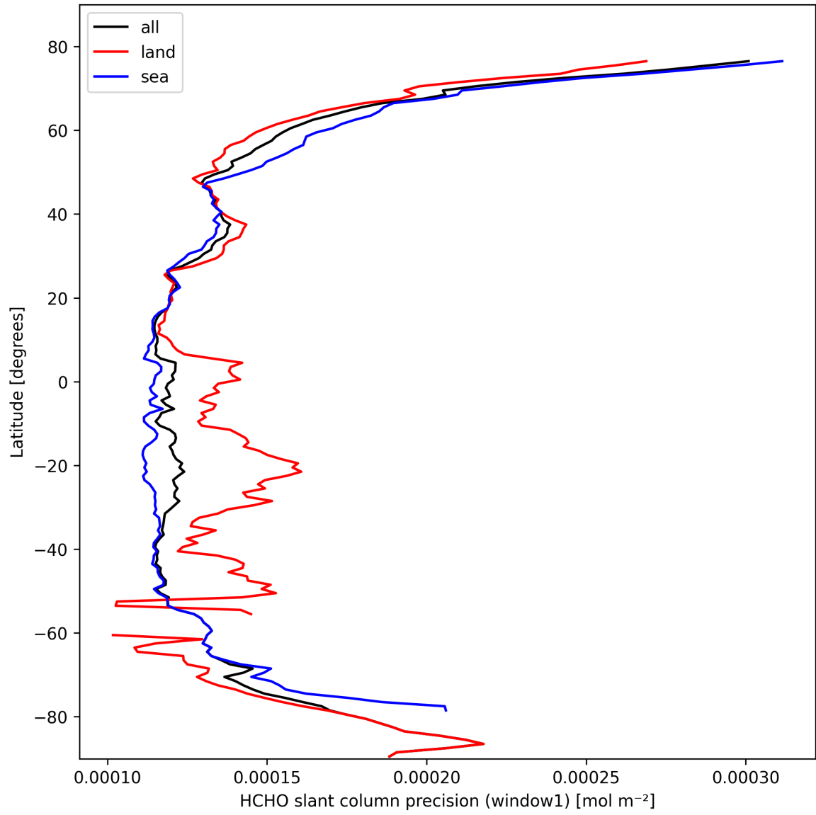
Figure 23: Zonal average of “HCHO slant column precision (window1)” for 2025-02-26 to 2025-02-27.
