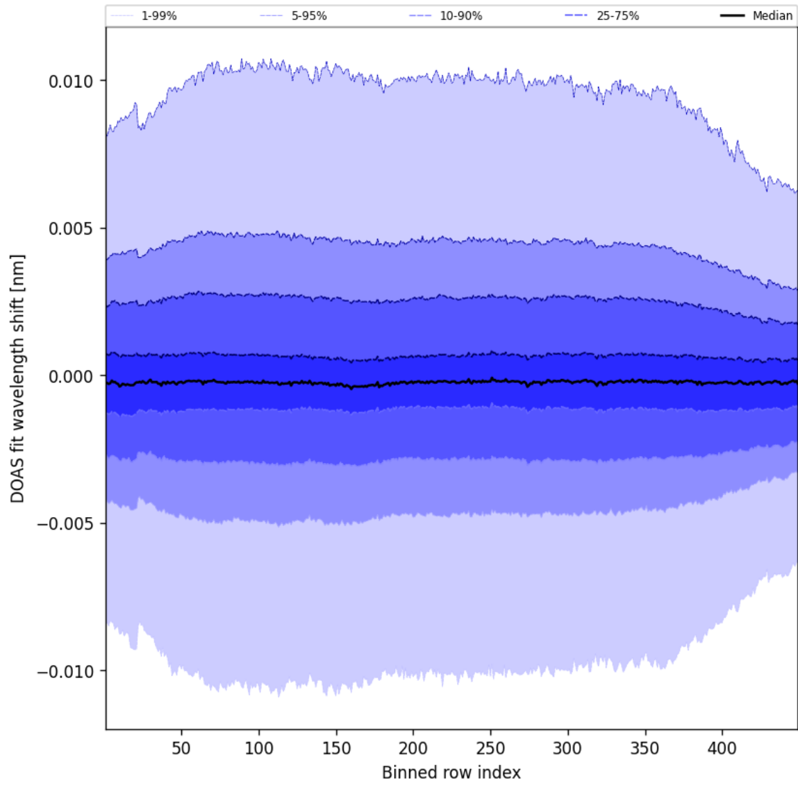
Figure 56: Along track statistics of “DOAS fit wavelength shift” for 2025-02-26 to 2025-02-27
