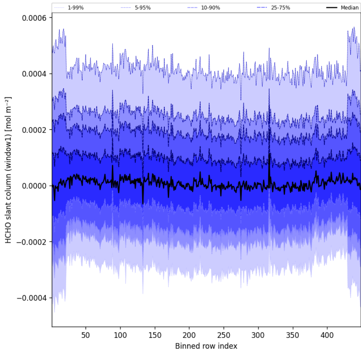
Figure 50: Along track statistics of “HCHO slant column (window1)” for 2025-02-26 to 2025-02-27
