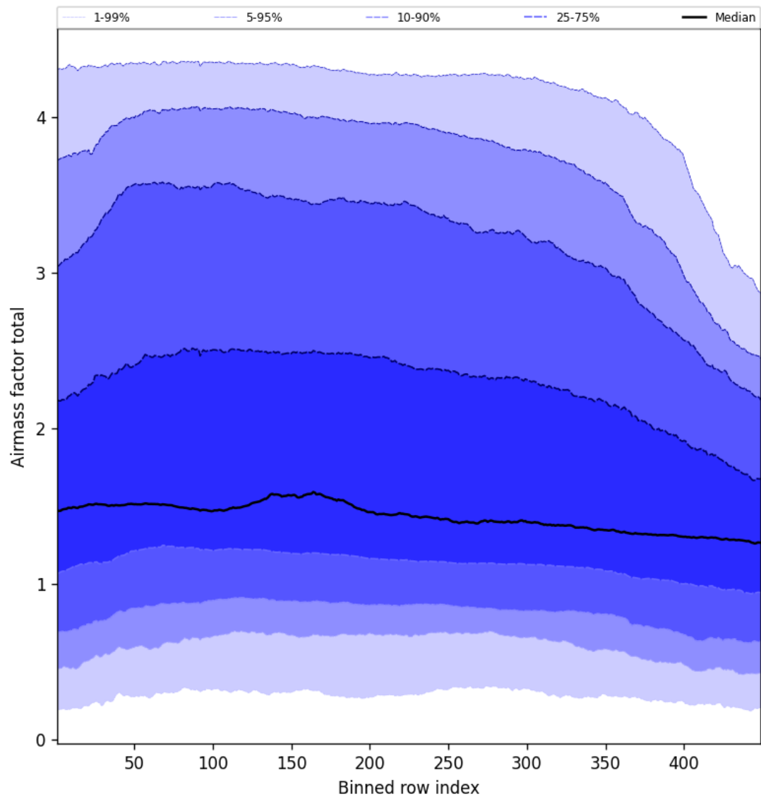
Figure 52: Along track statistics of “Airmass factor total” for 2025-02-26 to 2025-02-27
