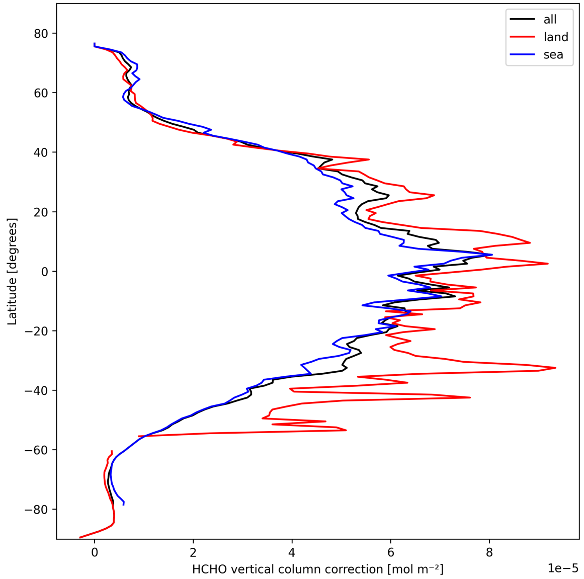
Figure 21: Zonal average of “HCHO vertical column correction” for 2025-02-26 to 2025-02-27.
