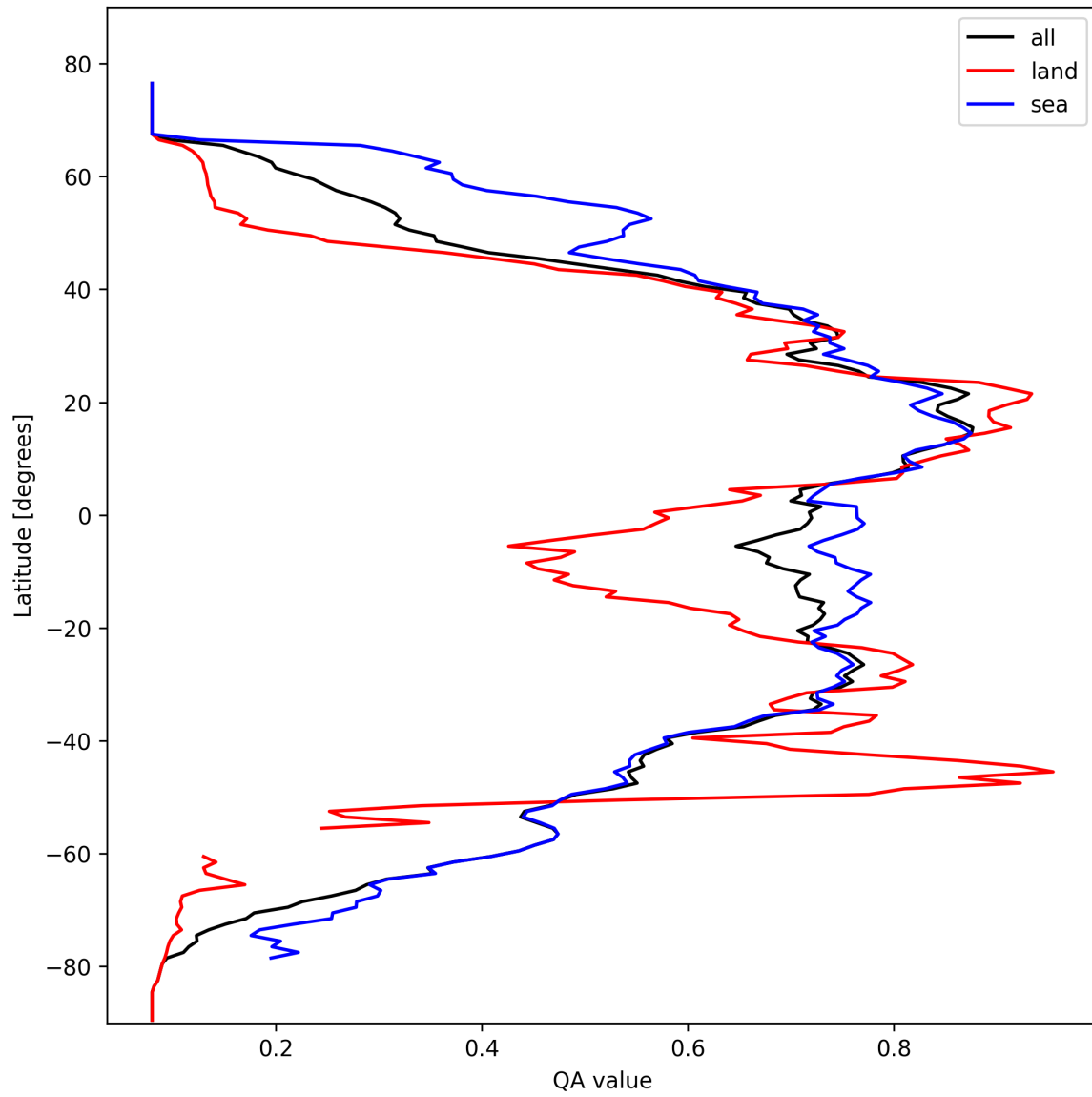
Figure 18: Zonal average of “QA value” for 2025-02-26 to 2025-02-27.
