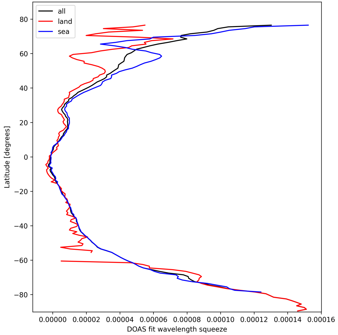
Figure 29: Zonal average of “DOAS fit wavelength squeeze” for 2025-02-26 to 2025-02-27.
