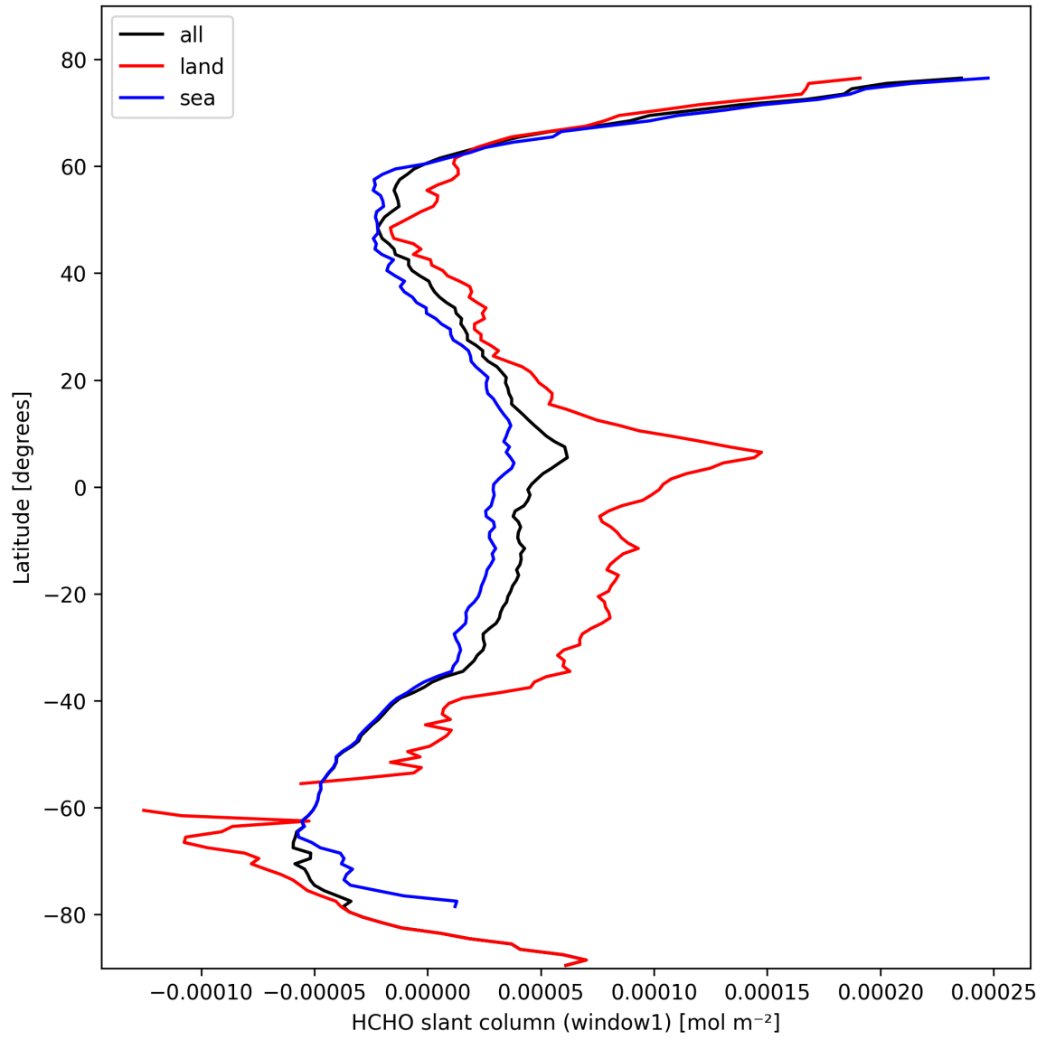
Figure 22: Zonal average of “HCHO slant column (window1)” for 2025-02-26 to 2025-02-27.
