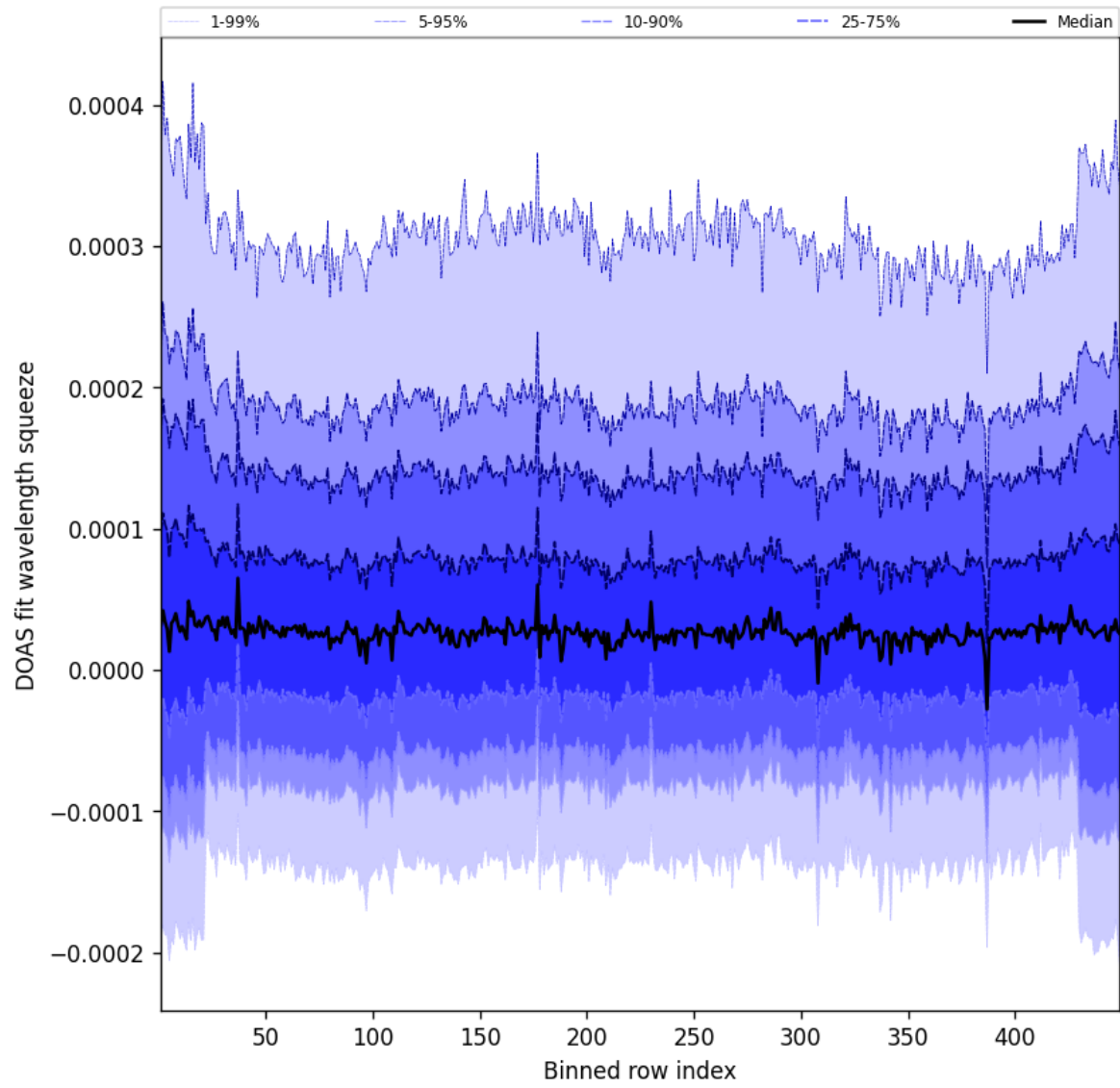
Figure 57: Along track statistics of “DOAS fit wavelength squeeze” for 2025-02-26 to 2025-02-27
