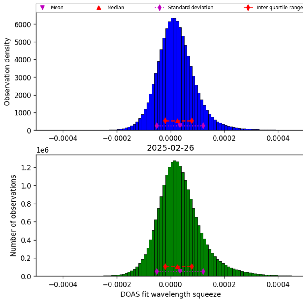
Figure 43: Histogram of “DOAS fit wavelength squeeze” for 2025-02-26 to 2025-02-27
