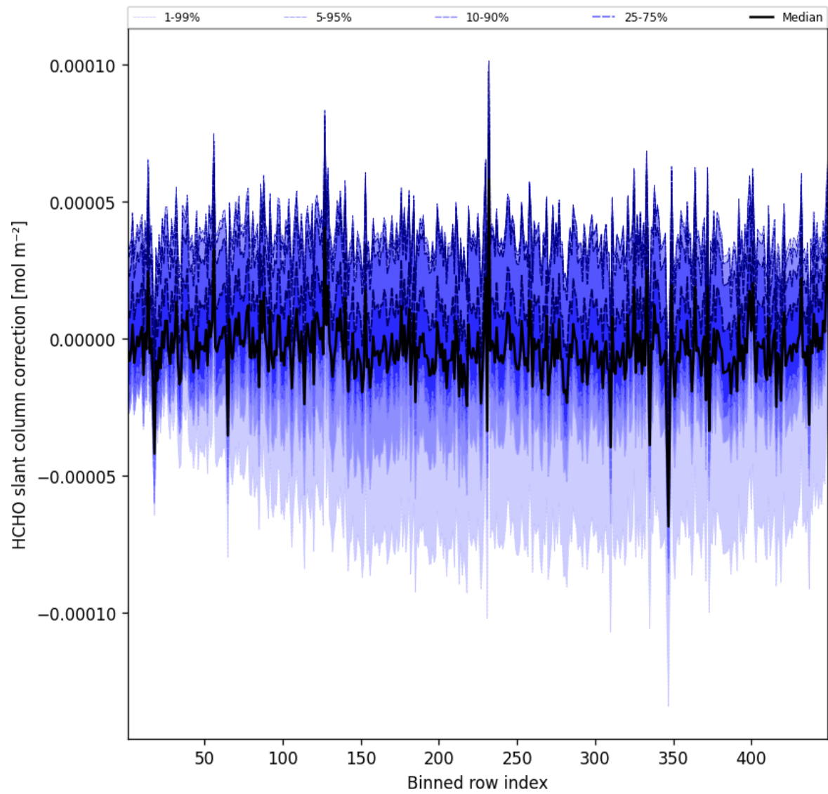
Figure 59: Along track statistics of “HCHO slant column correction” for 2025-02-26 to 2025-02-27
