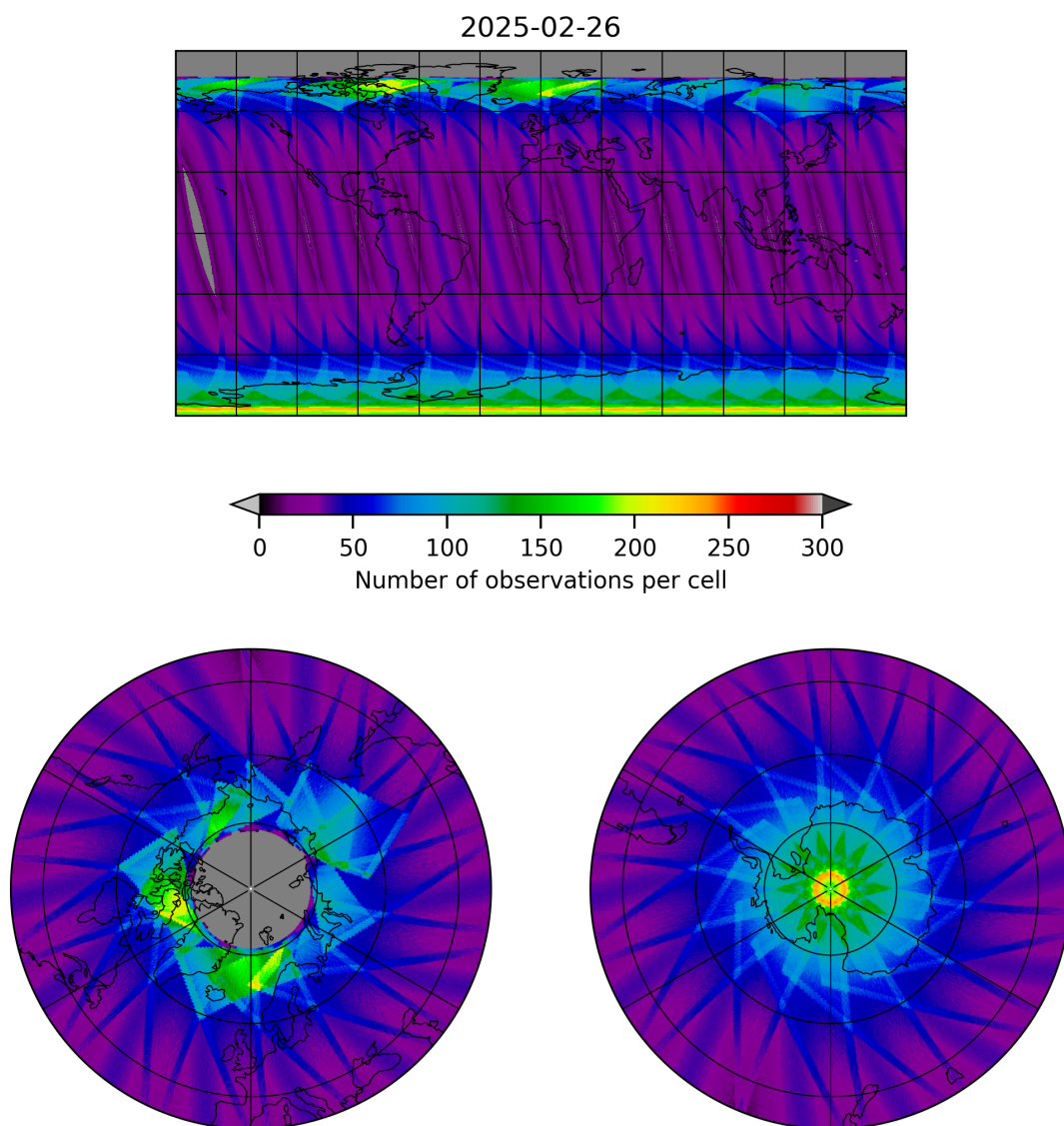
Figure 17: Map of the number of observations for 2025-02-26 to 2025-02-27
