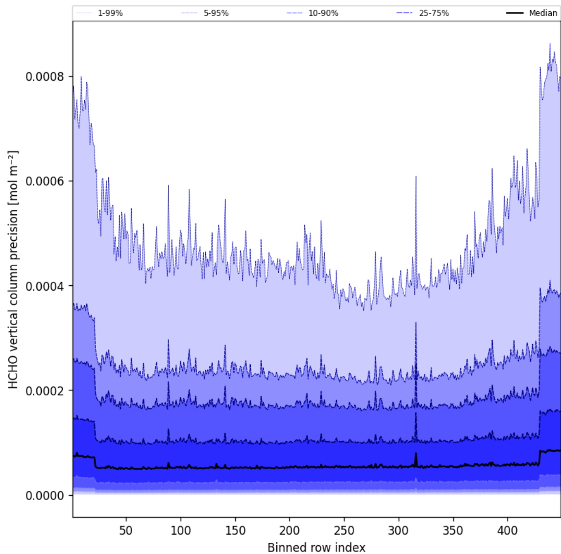
Figure 48: Along track statistics of “HCHO vertical column precision” for 2025-02-26 to 2025-02-27
