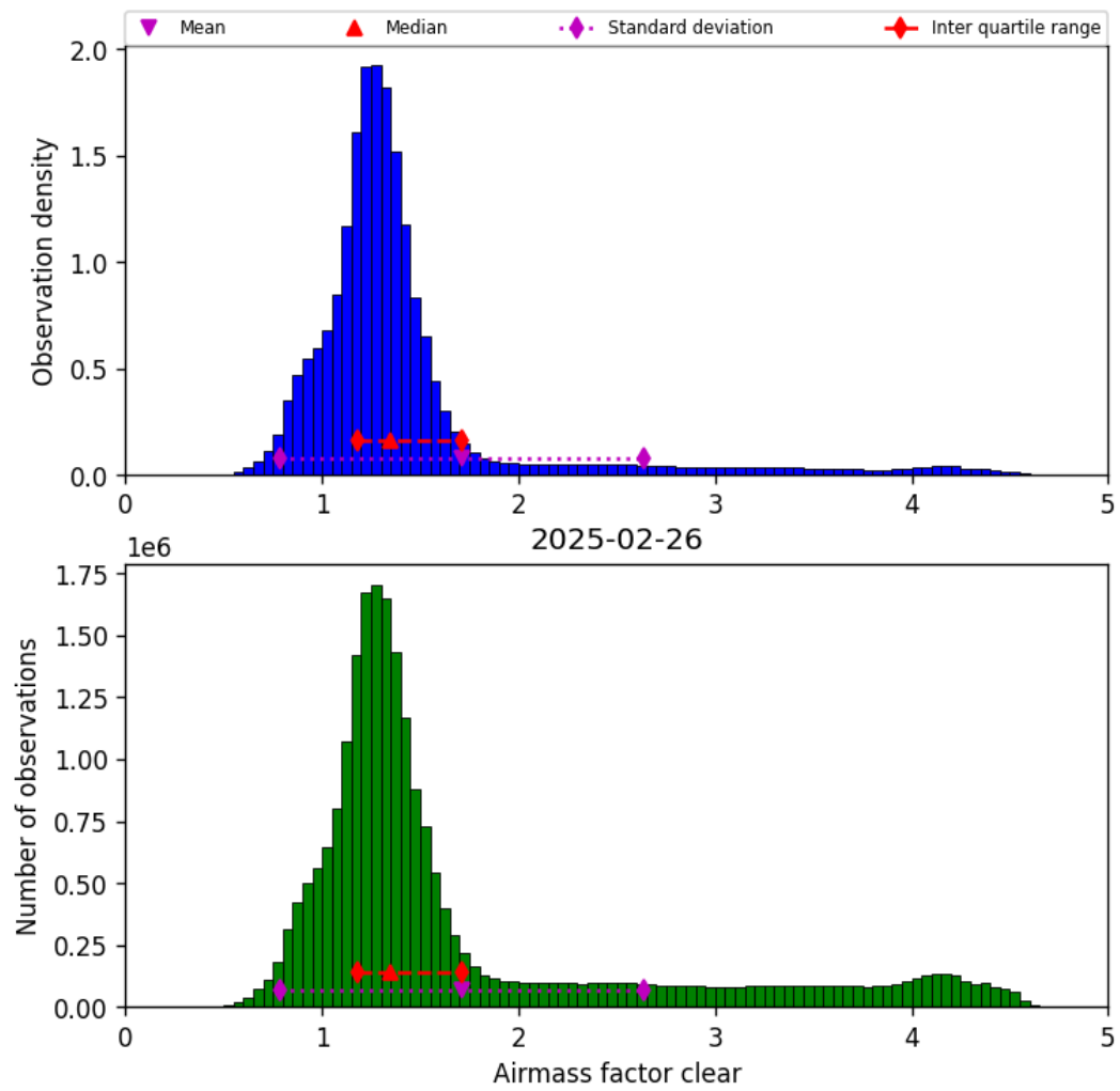
Figure 40: Histogram of “Airmass factor clear” for 2025-02-26 to 2025-02-27
