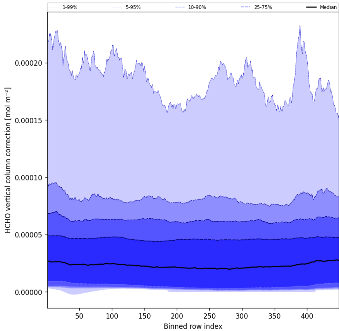
Figure 49: Along track statistics of “HCHO vertical column correction” for 2025-02-27 to 2025-02-27
