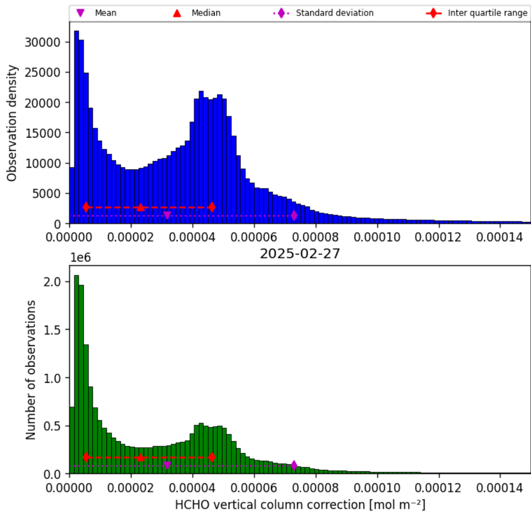
Figure 35: Histogram of “HCHO vertical column correction” for 2025-02-27 to 2025-02-27
