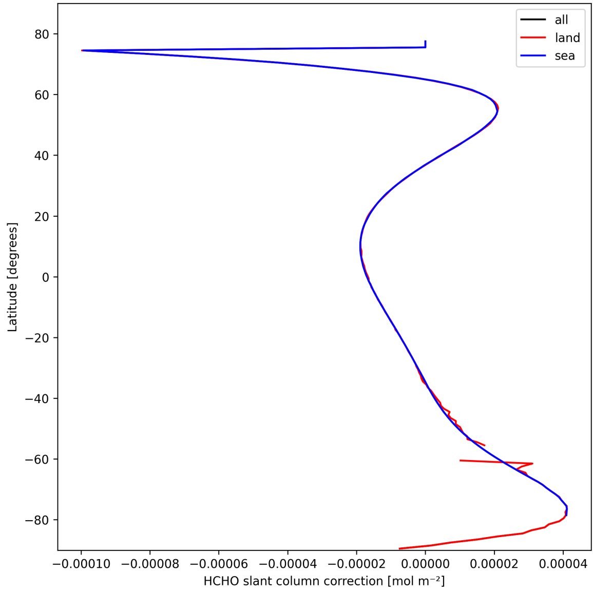
Figure 31: Zonal average of “HCHO slant column correction” for 2025-02-27 to 2025-02-27.
