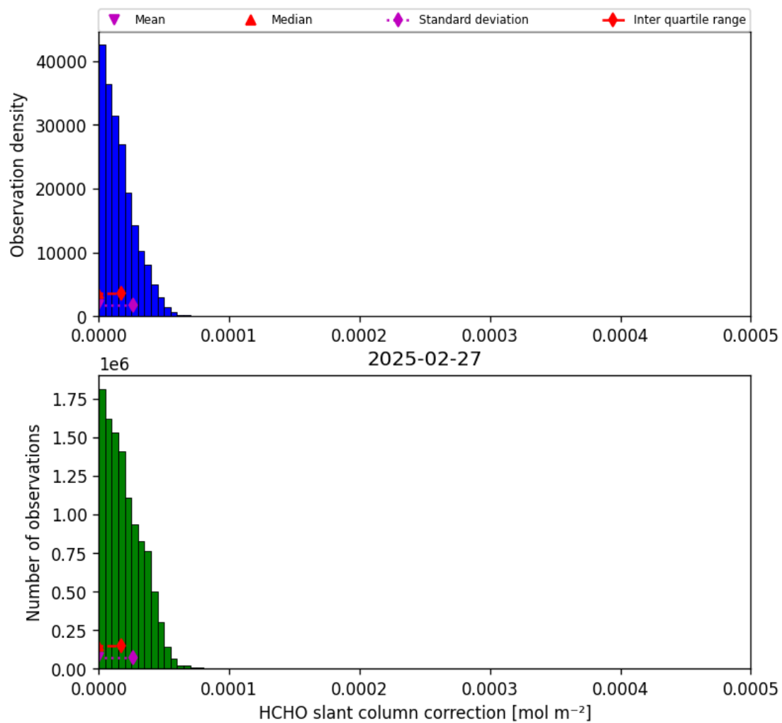
Figure 45: Histogram of “HCHO slant column correction” for 2025-02-27 to 2025-02-27
