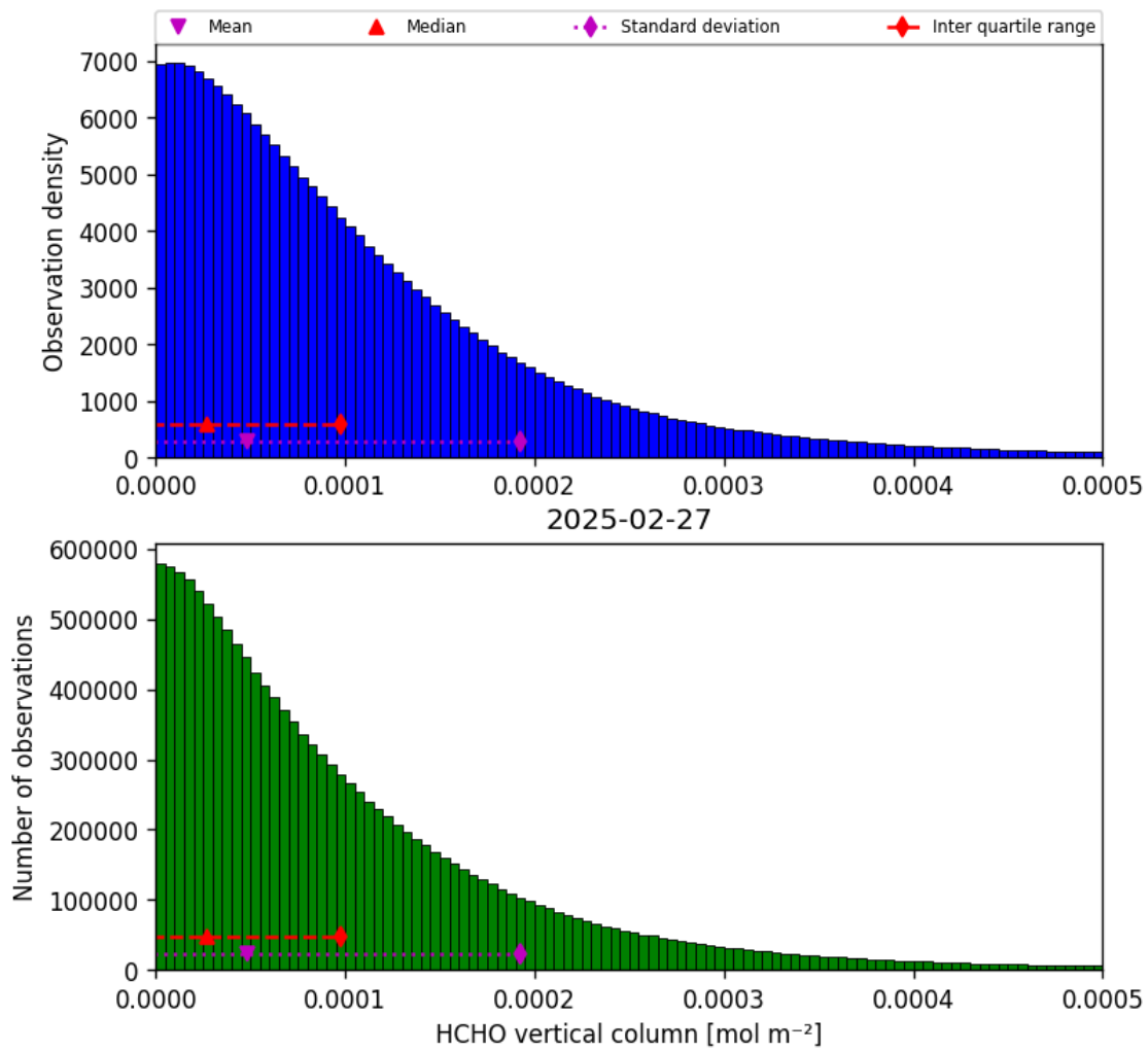
Figure 33: Histogram of “HCHO vertical column” for 2025-02-27 to 2025-02-27
