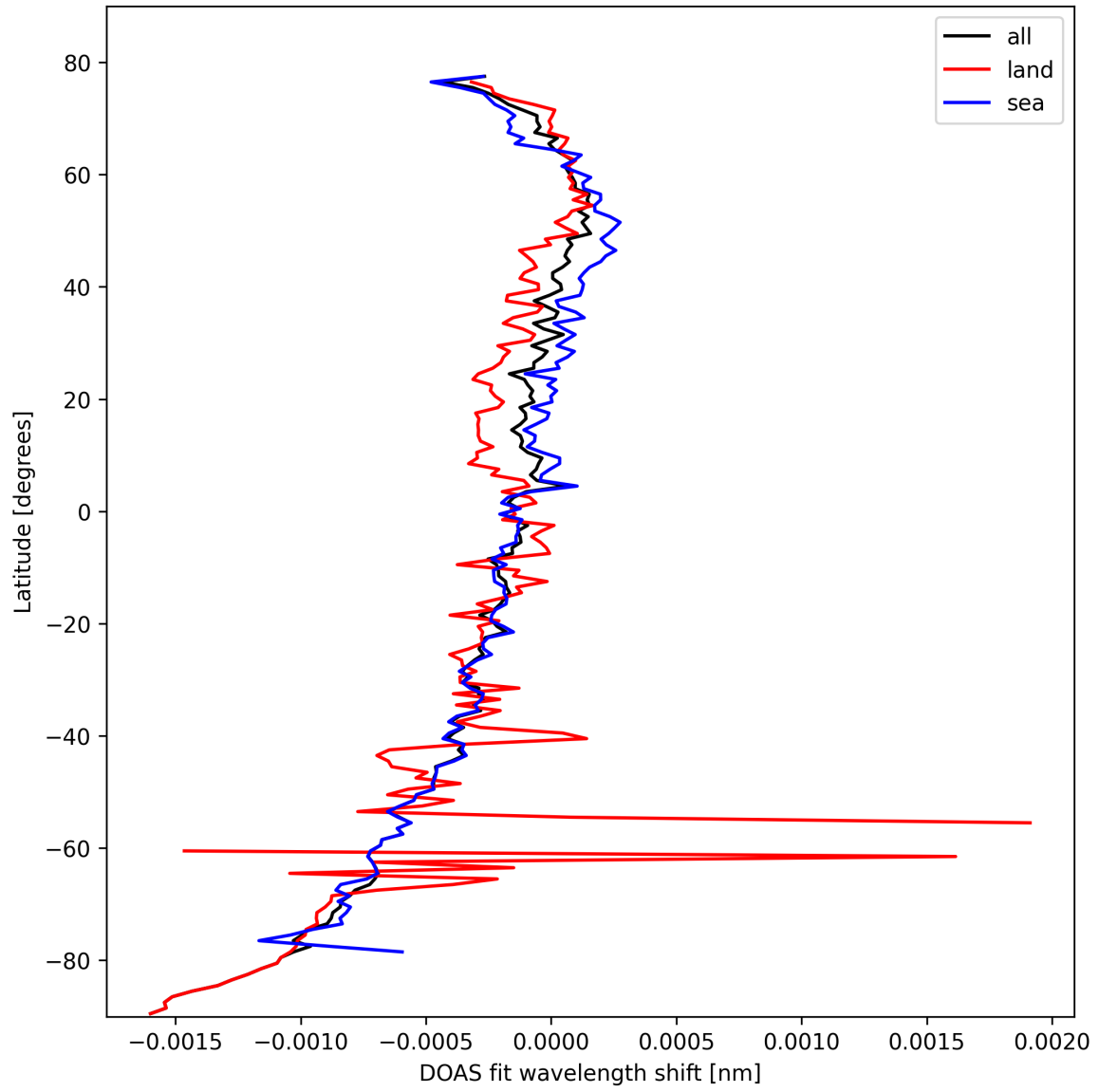
Figure 28: Zonal average of “DOAS fit wavelength shift” for 2025-02-27 to 2025-02-27.
