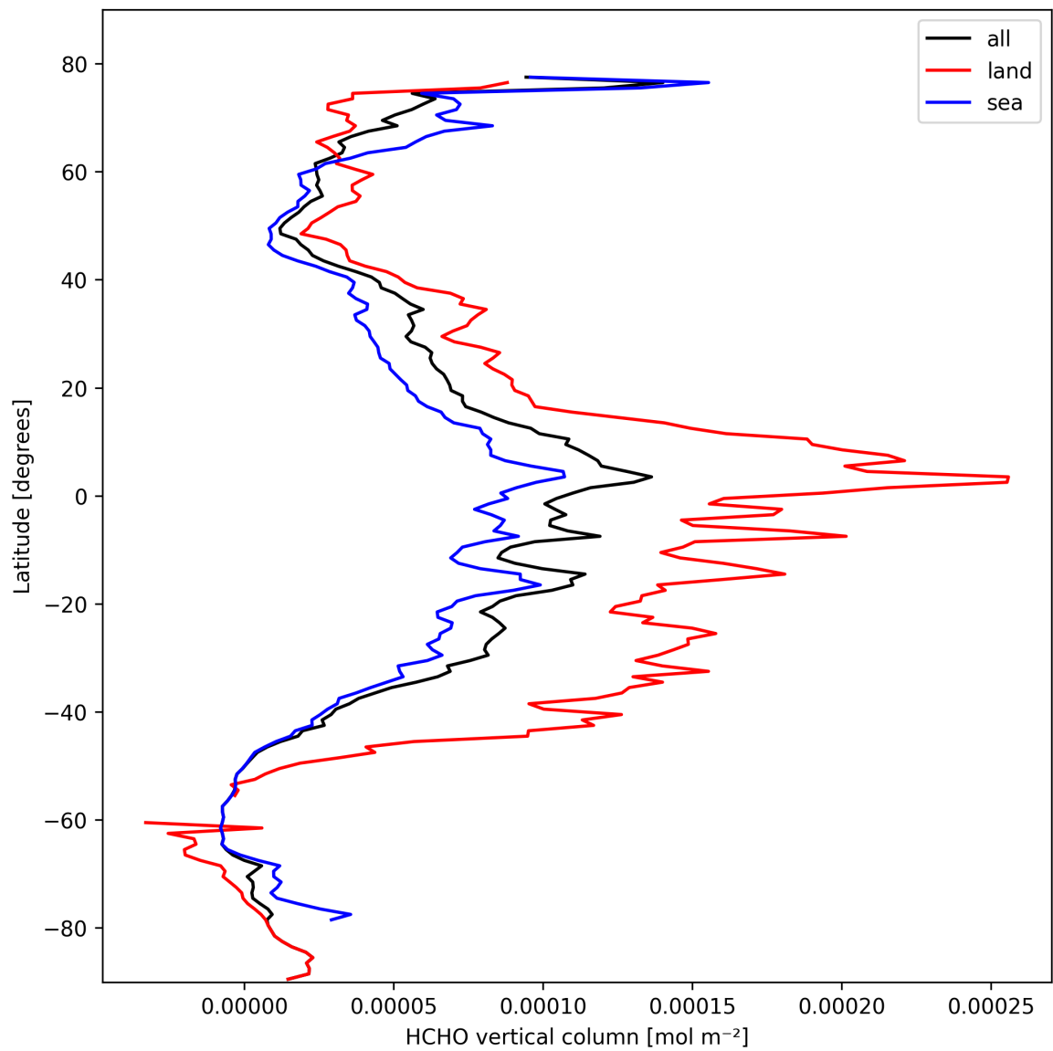
Figure 19: Zonal average of “HCHO vertical column” for 2025-02-27 to 2025-02-27.
