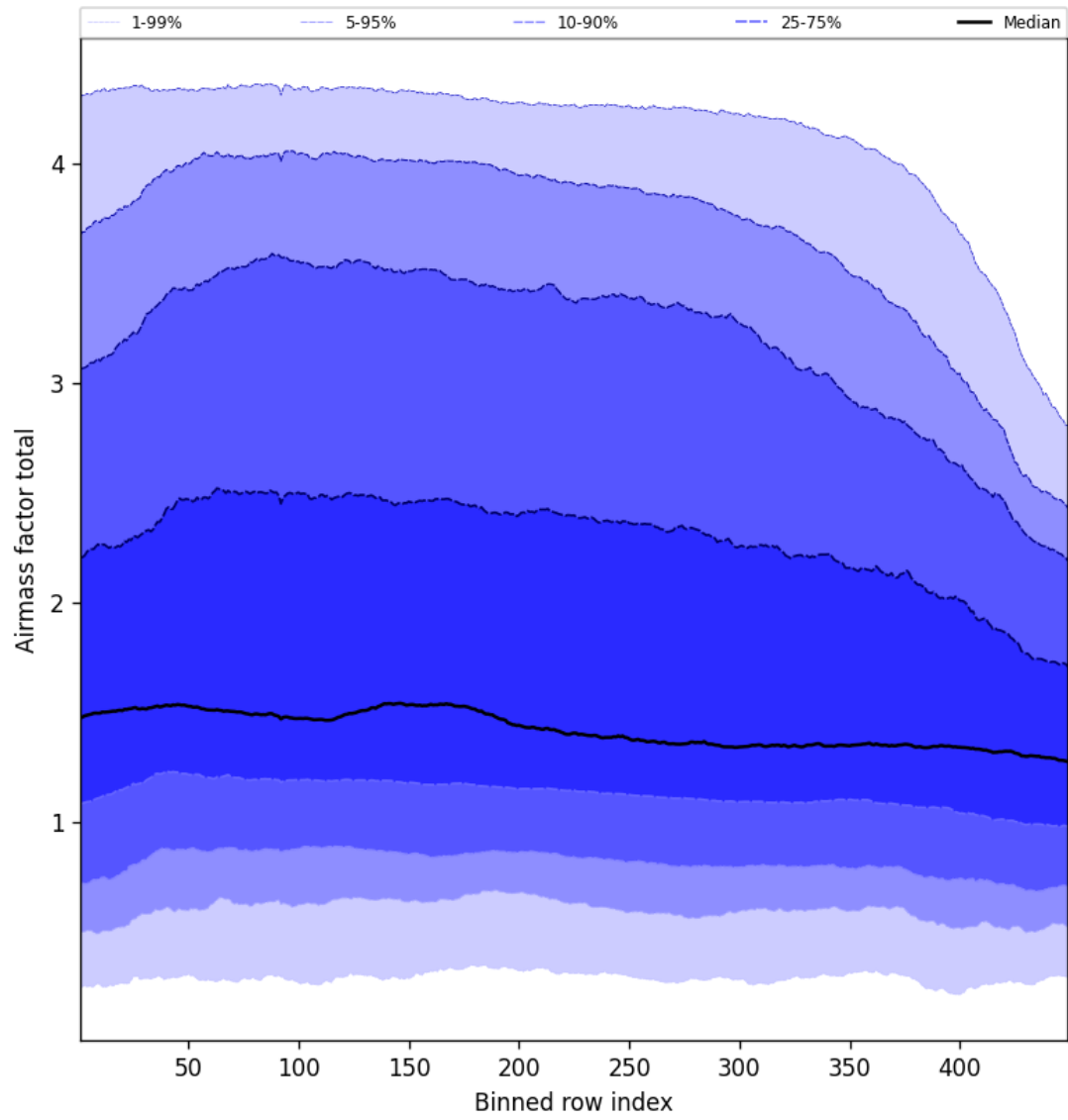
Figure 52: Along track statistics of “Airmass factor total” for 2025-02-27 to 2025-02-27
