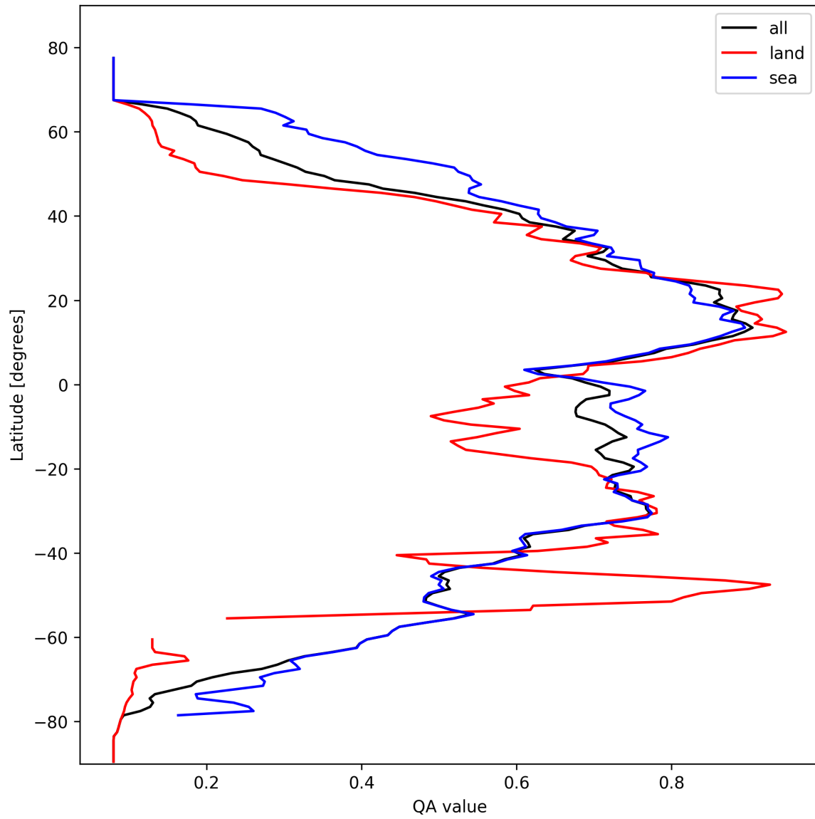
Figure 18: Zonal average of “QA value” for 2025-02-27 to 2025-02-27.
