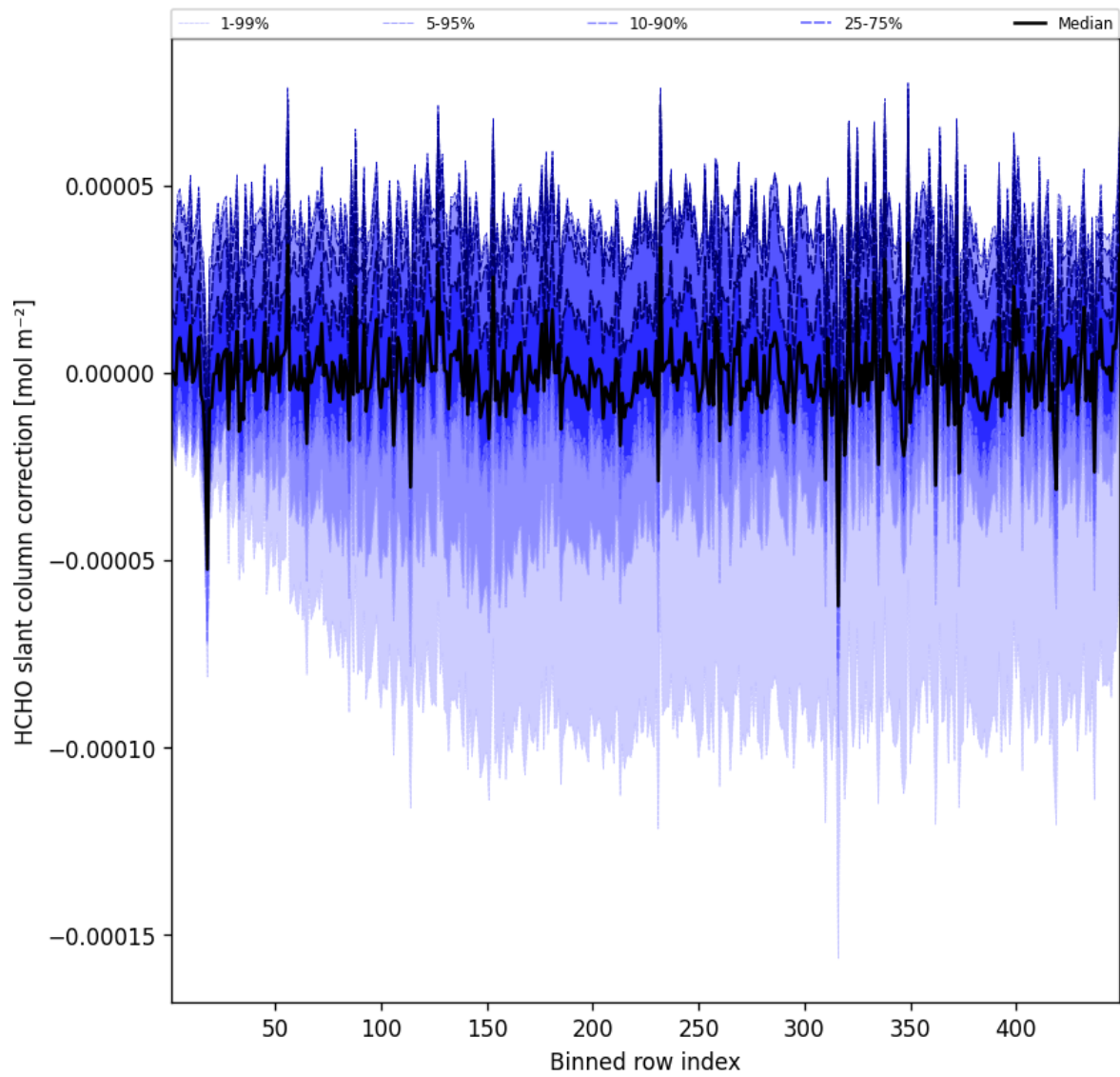
Figure 59: Along track statistics of “HCHO slant column correction” for 2025-02-27 to 2025-02-27
