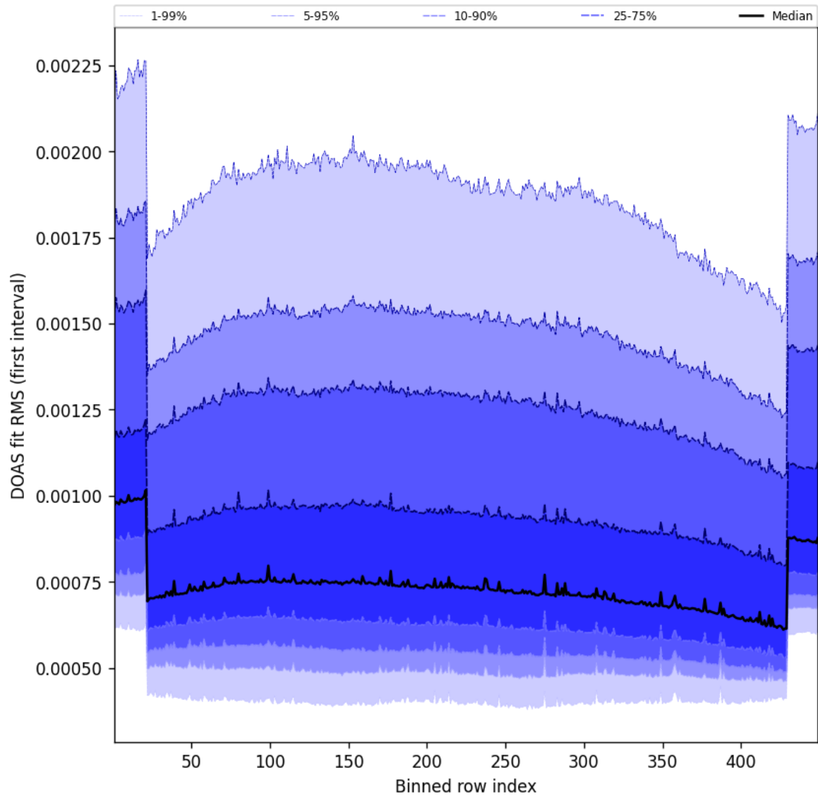
Figure 58: Along track statistics of “DOAS fit RMS (first interval)” for 2025-02-27 to 2025-02-27
