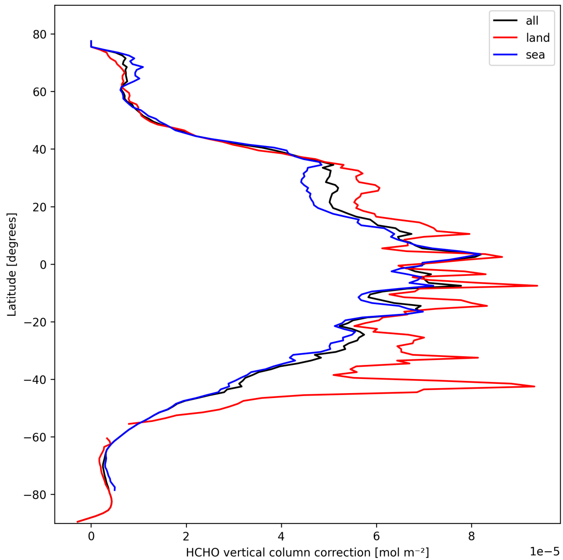
Figure 21: Zonal average of “HCHO vertical column correction” for 2025-02-27 to 2025-02-27.
