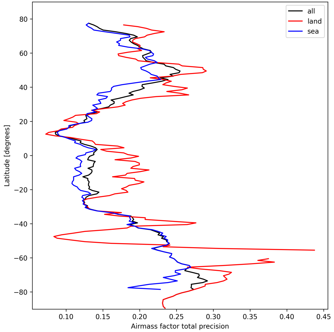
Figure 25: Zonal average of “Airmass factor total precision” for 2025-02-27 to 2025-02-27.
