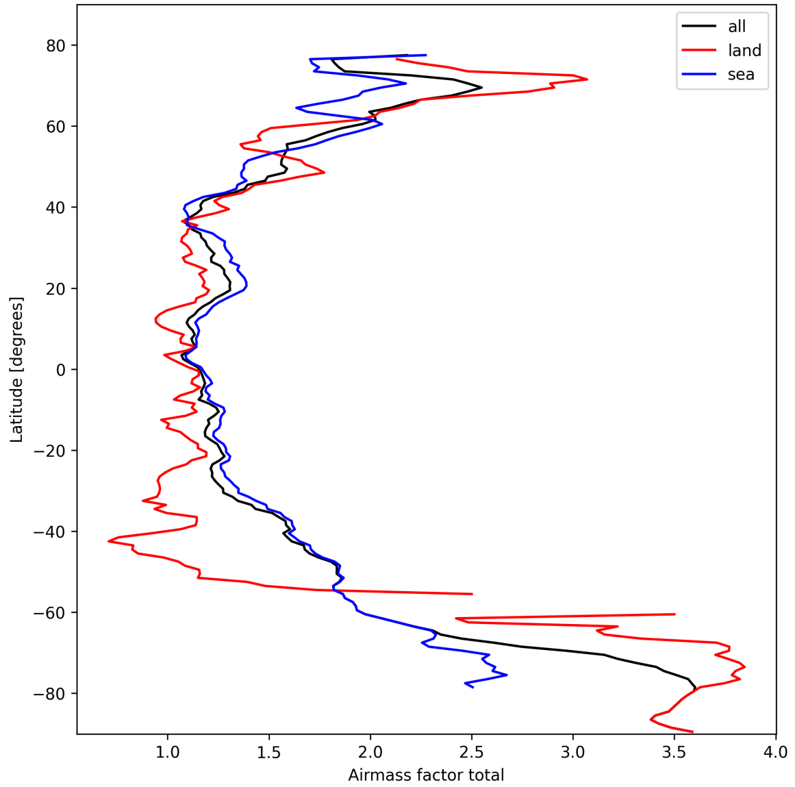
Figure 24: Zonal average of “Airmass factor total” for 2025-02-27 to 2025-02-27.
