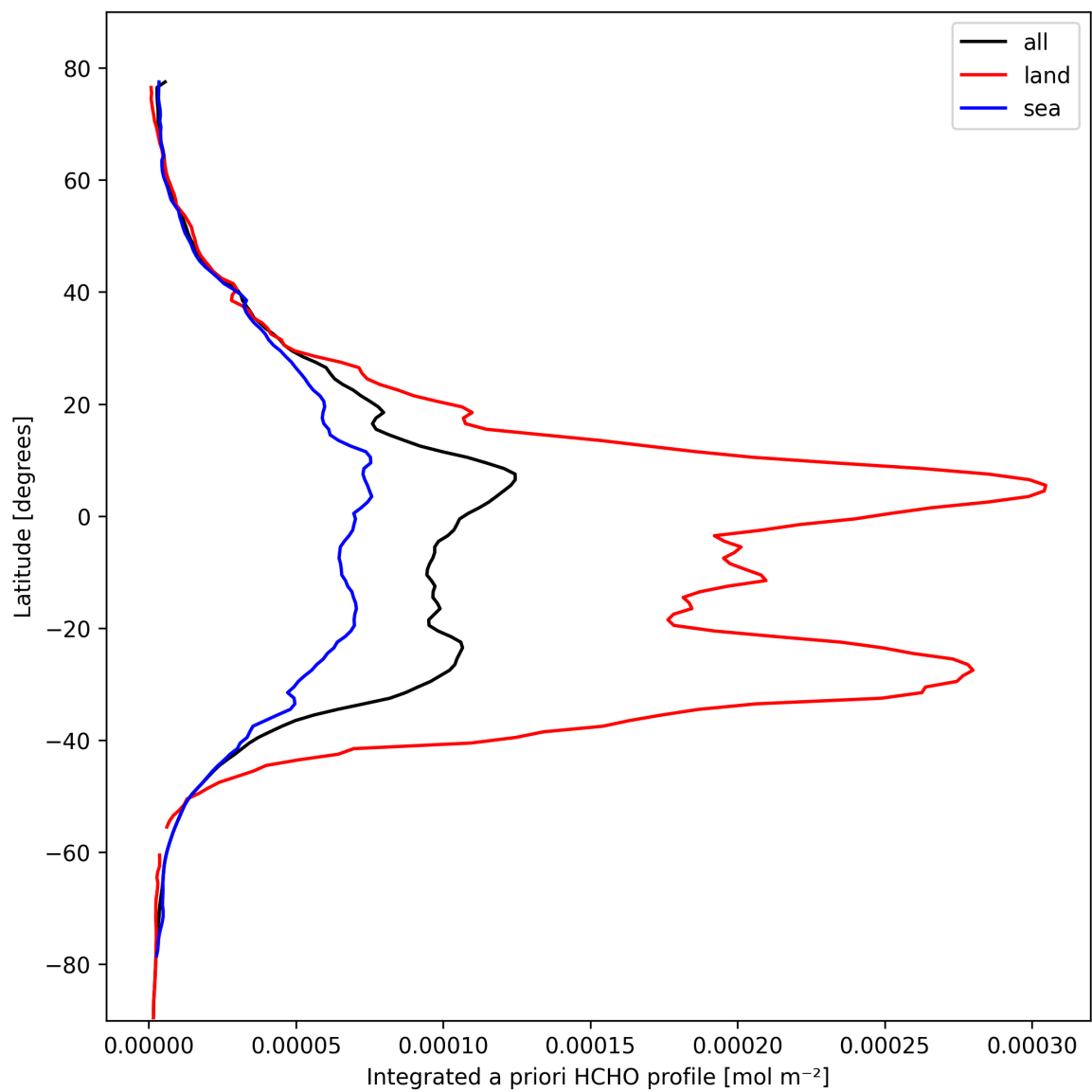
Figure 27: Zonal average of “Integrated a priori HCHO profile” for 2025-02-27 to 2025-02-27.
