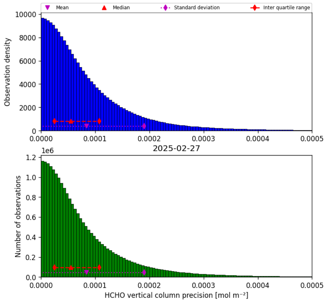
Figure 34: Histogram of “HCHO vertical column precision” for 2025-02-27 to 2025-02-27
