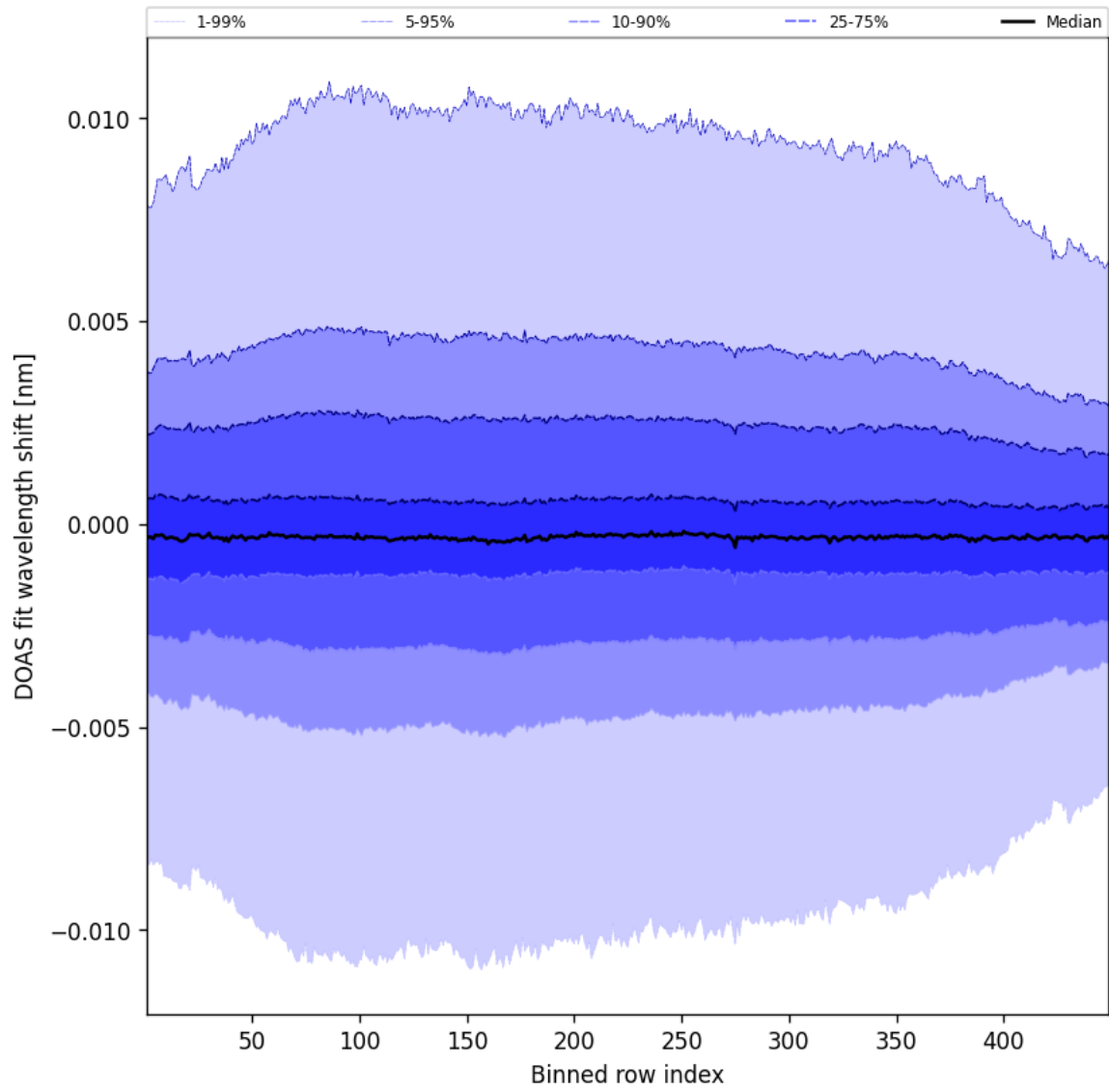
Figure 56: Along track statistics of “DOAS fit wavelength shift” for 2025-02-27 to 2025-02-27
