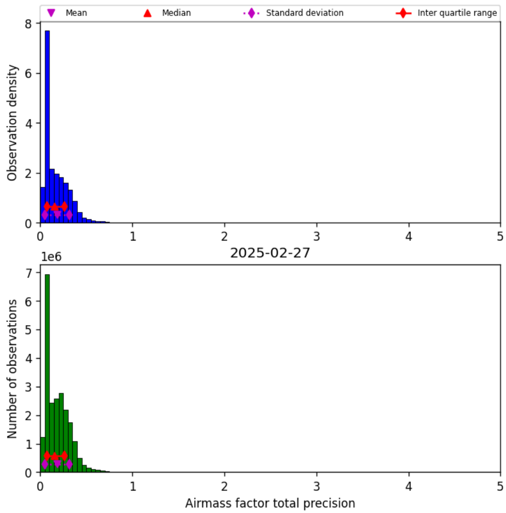
Figure 39: Histogram of “Airmass factor total precision” for 2025-02-27 to 2025-02-27
