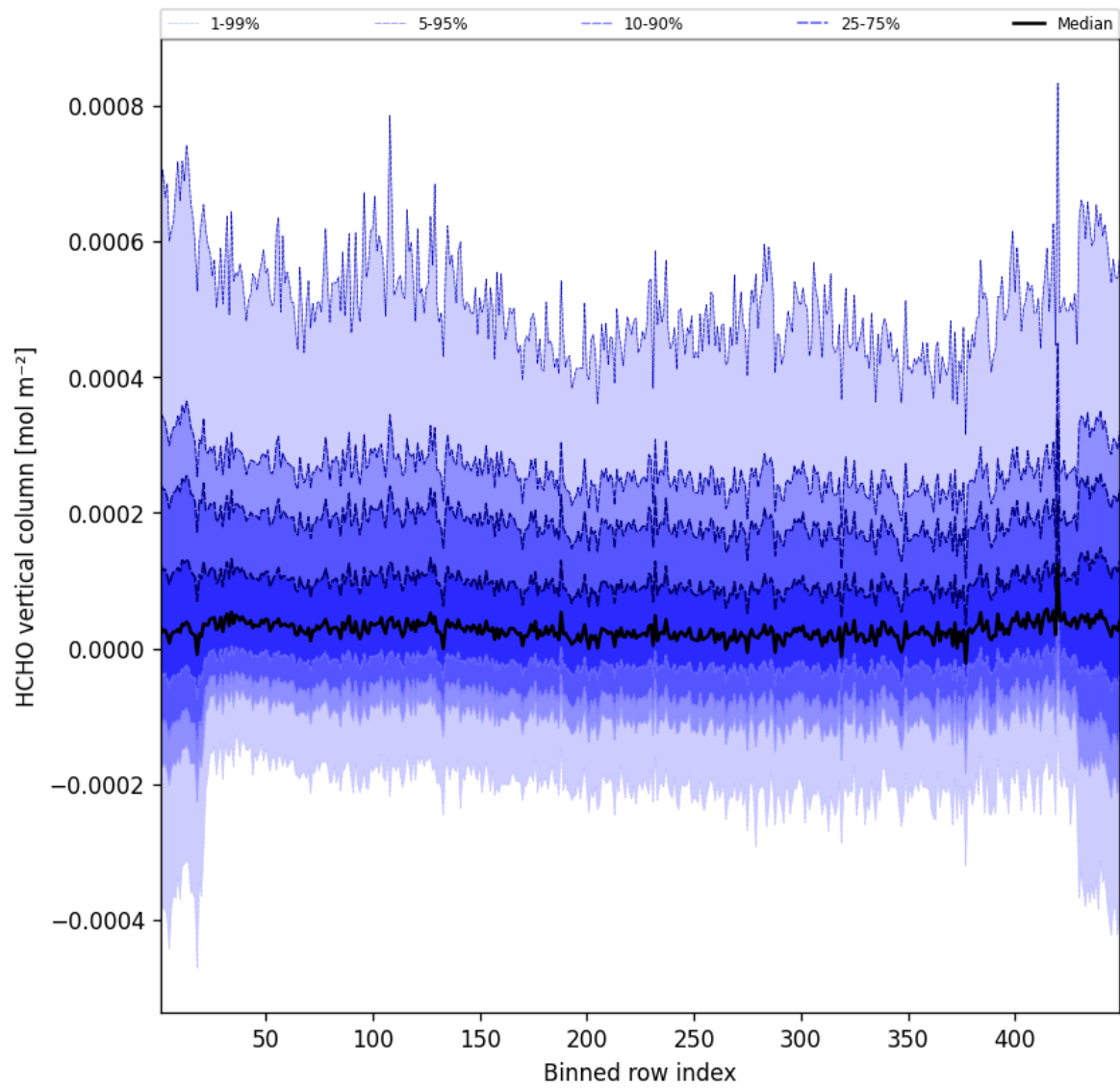
Figure 47: Along track statistics of “HCHO vertical column” for 2025-02-27 to 2025-02-27
