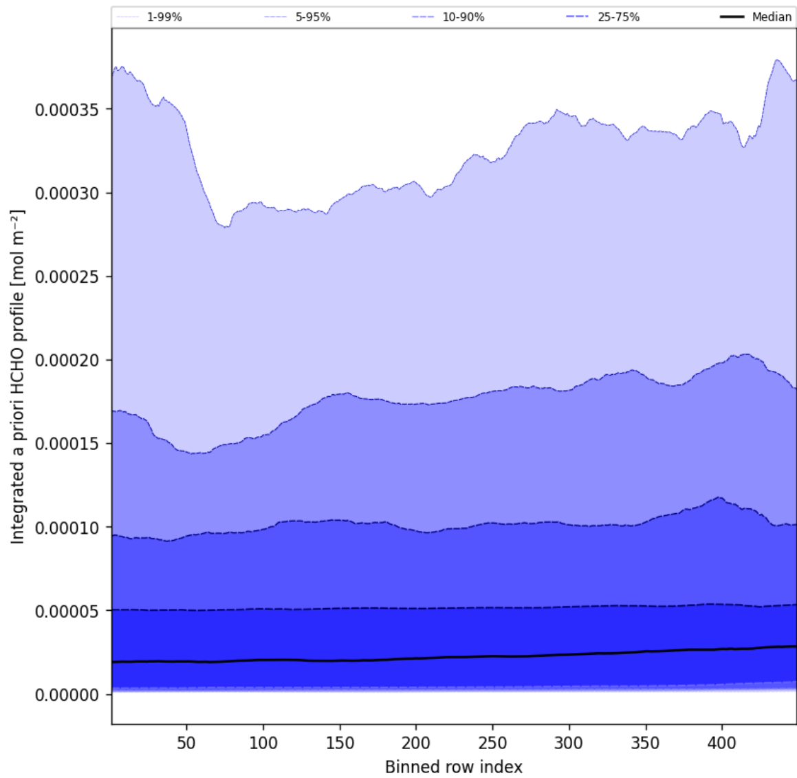
Figure 55: Along track statistics of "Integrated a priori HCHO profile" for 2025-02-27 to 2025-02-27
