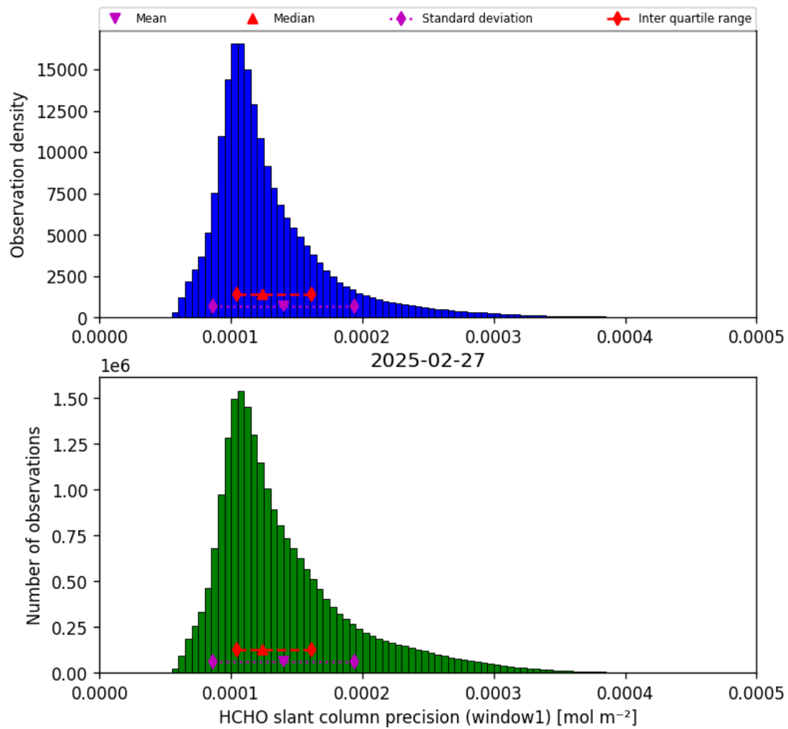
Figure 37: Histogram of “HCHO slant column precision (window1)” for 2025-02-27 to 2025-02-27
