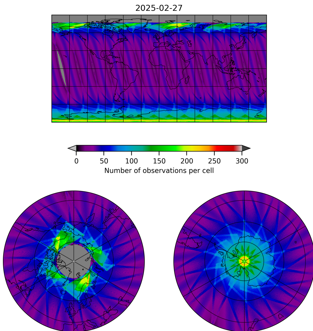
Figure 17: Map of the number of observations for 2025-02-27 to 2025-02-27
