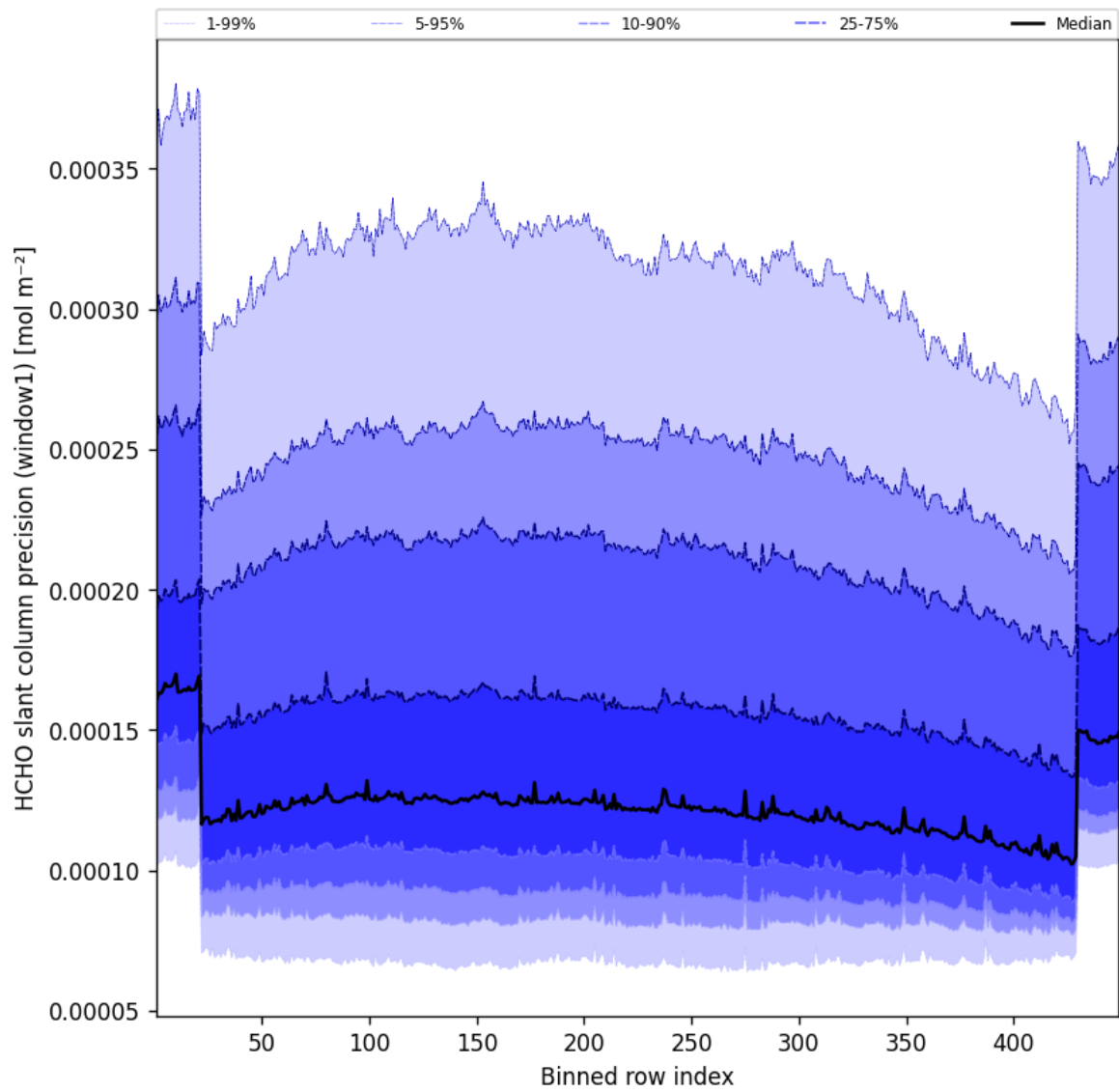
Figure 51: Along track statistics of “HCHO slant column precision (window1)” for 2025-02-27 to 2025-02-27
