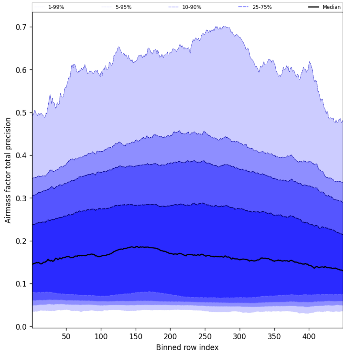
Figure 53: Along track statistics of “Airmass factor total precision” for 2025-02-27 to 2025-02-27
