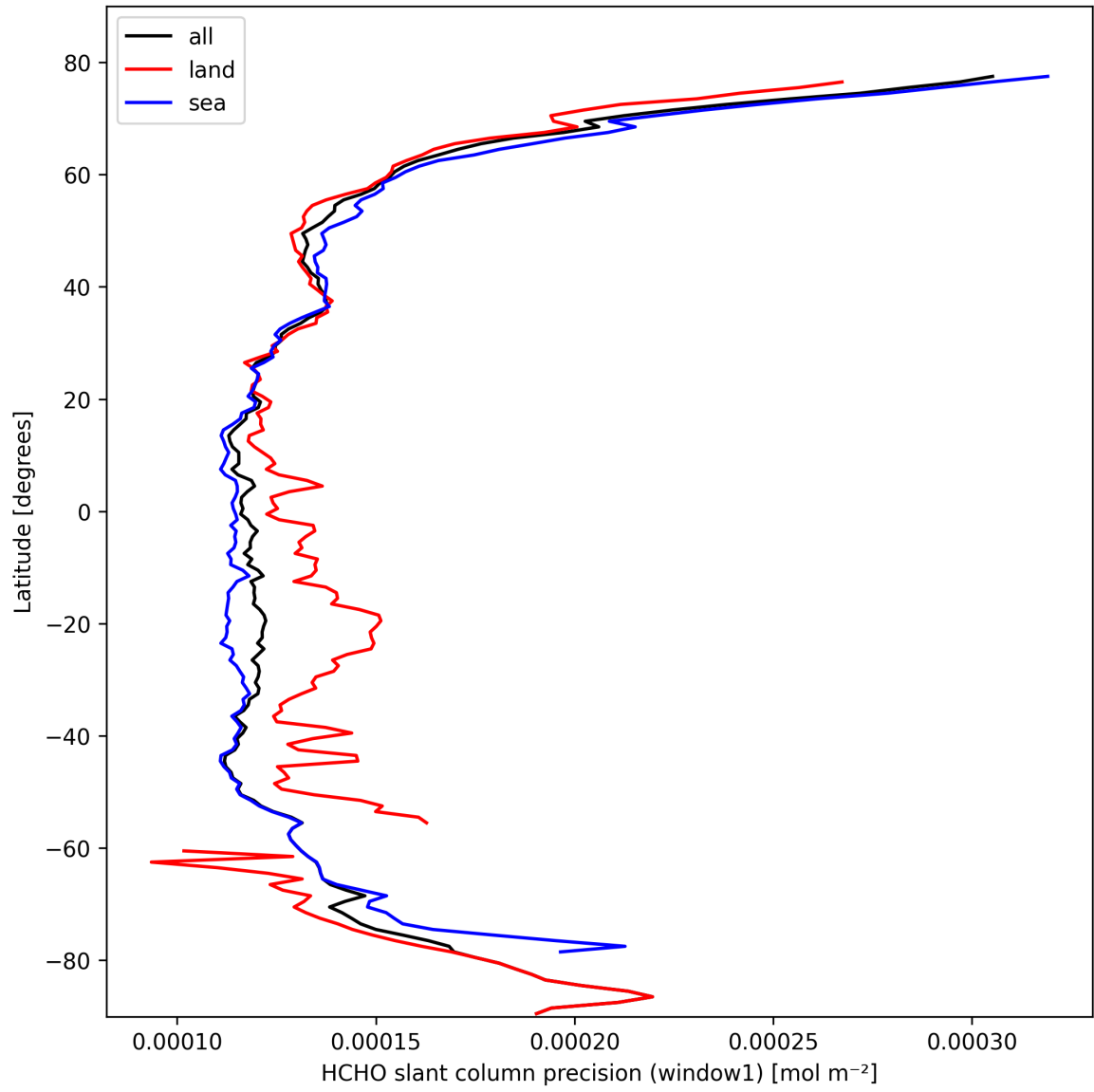
Figure 23: Zonal average of “HCHO slant column precision (window1)” for 2025-02-27 to 2025-02-27.
