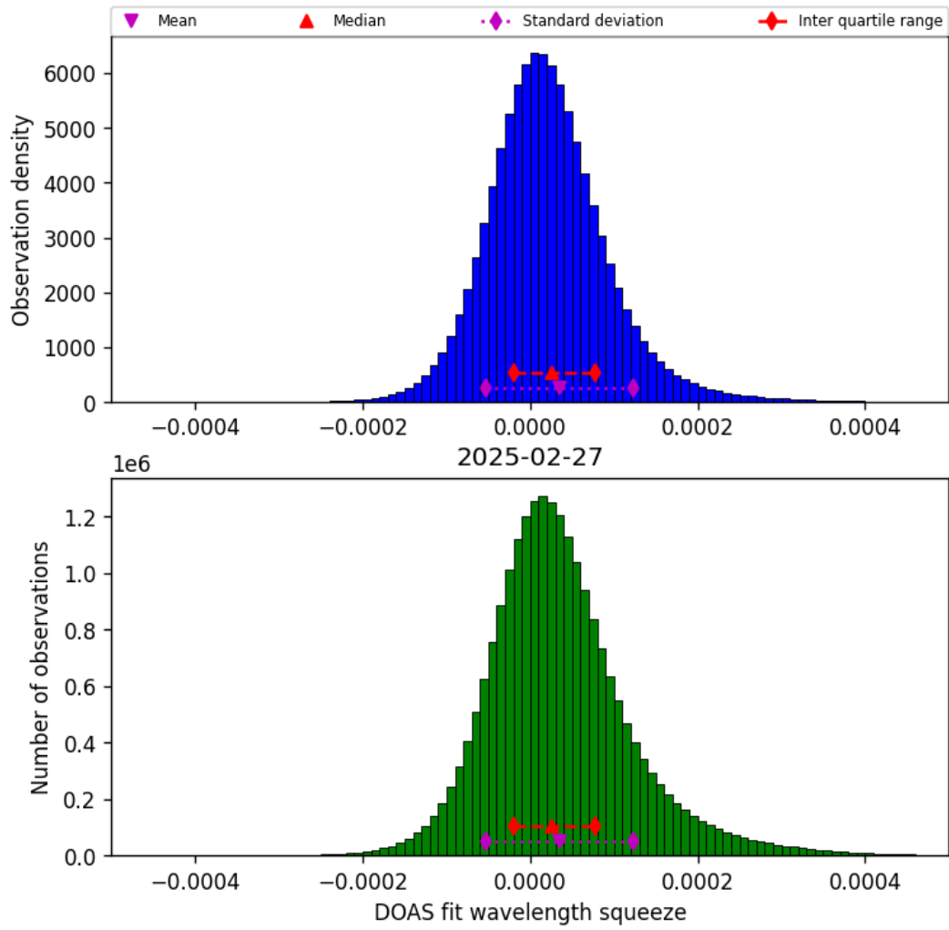
Figure 43: Histogram of “DOAS fit wavelength squeeze” for 2025-02-27 to 2025-02-27
