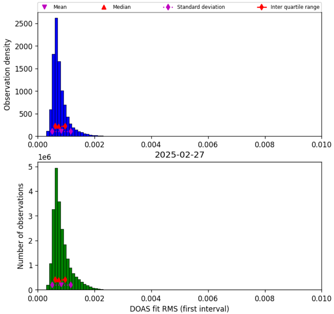
Figure 44: Histogram of “DOAS fit RMS (first interval)” for 2025-02-27 to 2025-02-27
