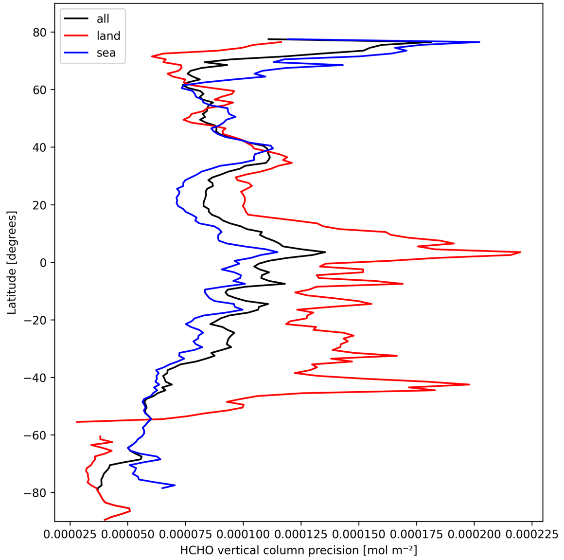
Figure 20: Zonal average of “HCHO vertical column precision” for 2025-02-27 to 2025-02-27.
