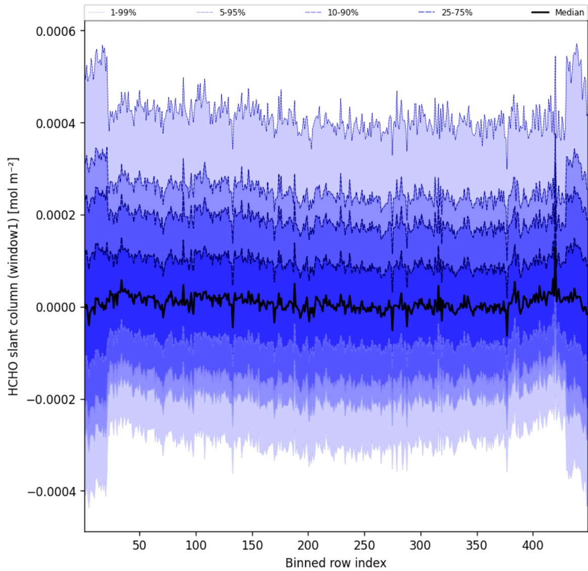
Figure 50: Along track statistics of “HCHO slant column (window1)” for 2025-02-27 to 2025-02-27
