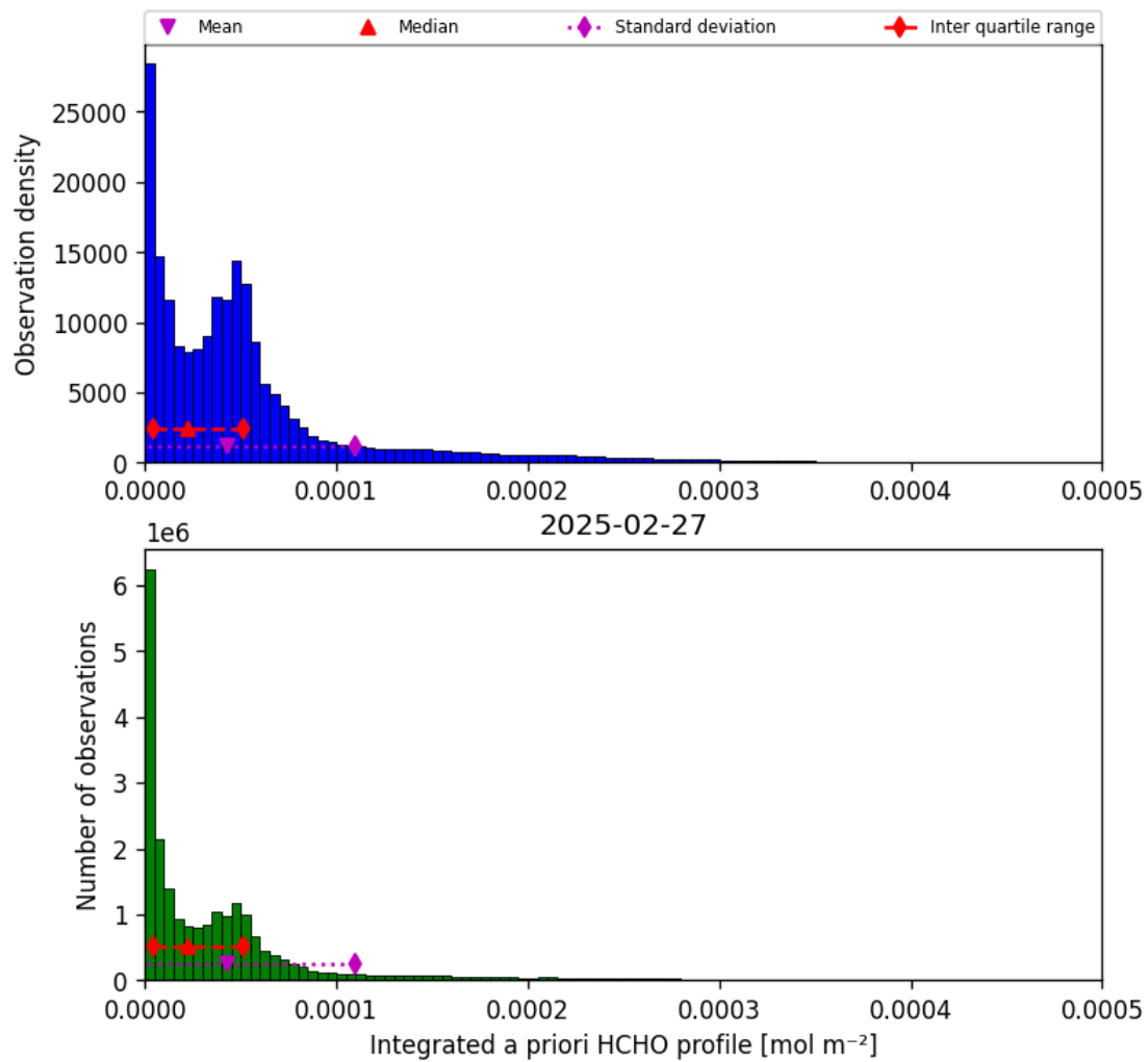
Figure 41: Histogram of “Integrated a priori HCHO profile” for 2025-02-27 to 2025-02-27
