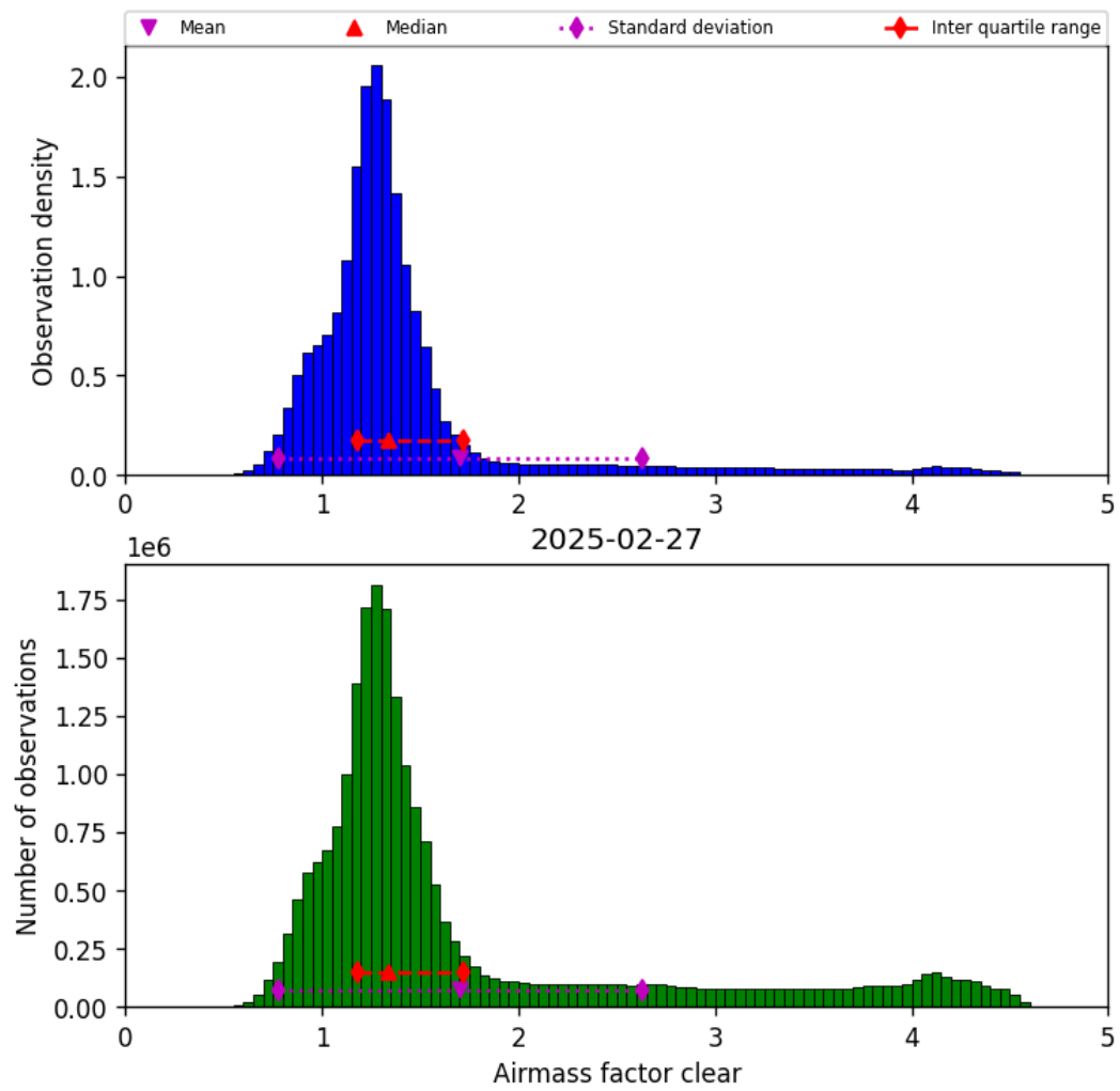
Figure 40: Histogram of “Airmass factor clear” for 2025-02-27 to 2025-02-27
