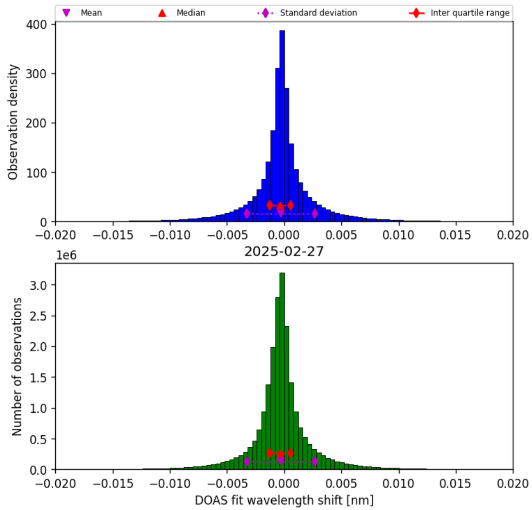
Figure 42: Histogram of “DOAS fit wavelength shift” for 2025-02-27 to 2025-02-27
