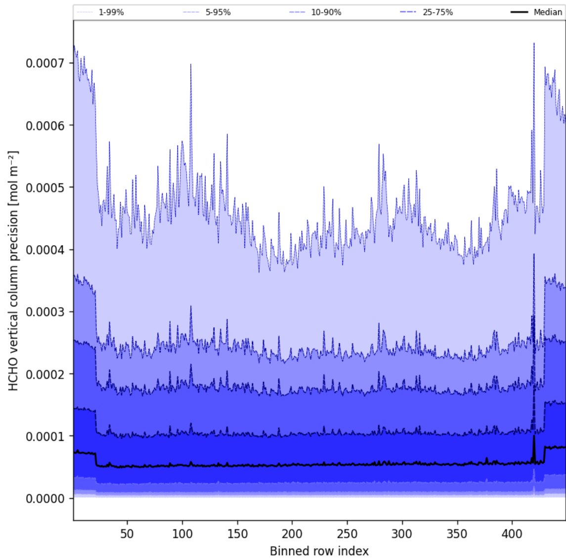
Figure 48: Along track statistics of "HCHO vertical column precision" for 2025-02-27 to 2025-02-27
