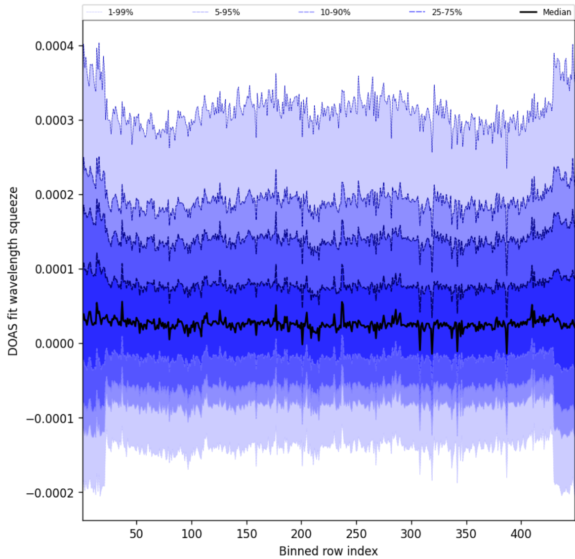
Figure 57: Along track statistics of “DOAS fit wavelength squeeze” for 2025-02-27 to 2025-02-27
