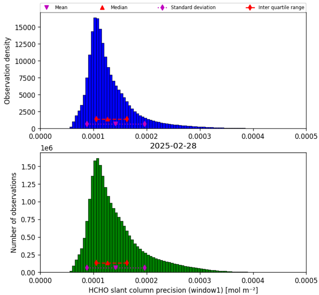
Figure 37: Histogram of “HCHO slant column precision (window1)” for 2025-02-28 to 2025-03-01
