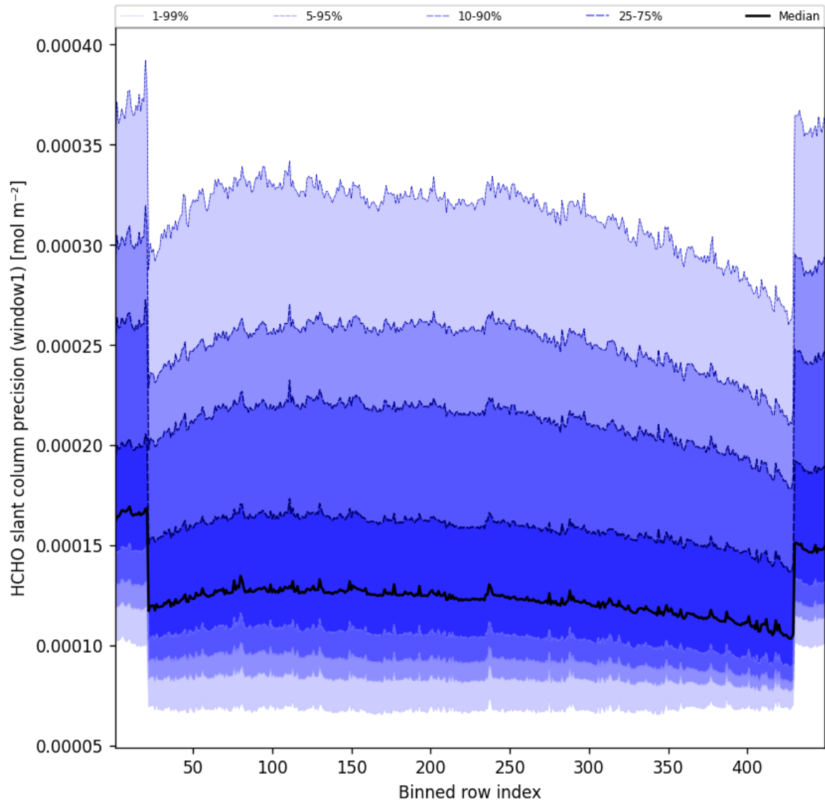
Figure 51: Along track statistics of “HCHO slant column precision (window1)” for 2025-02-28 to 2025-03-01
