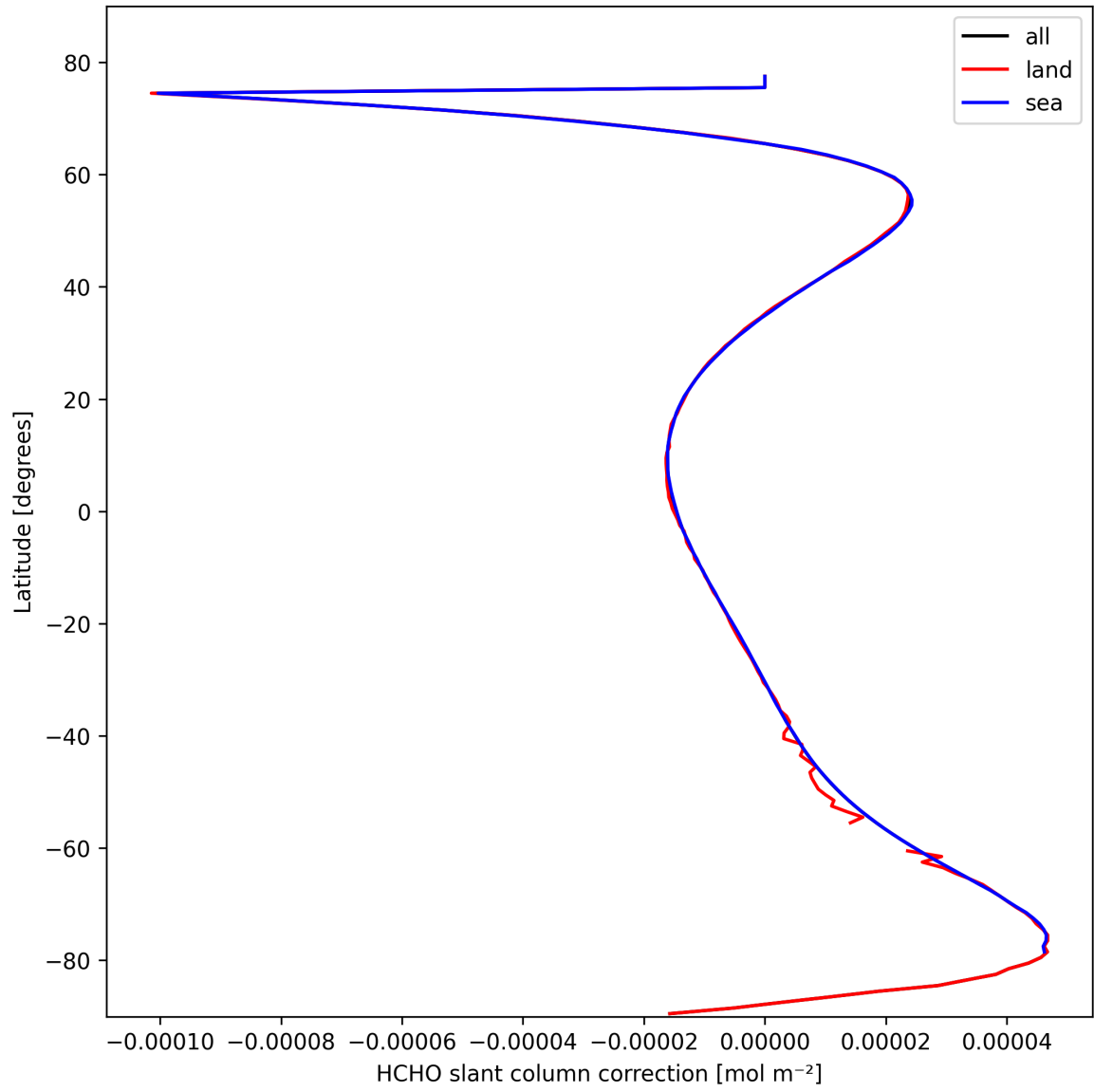
Figure 31: Zonal average of “HCHO slant column correction” for 2025-02-28 to 2025-03-01.
