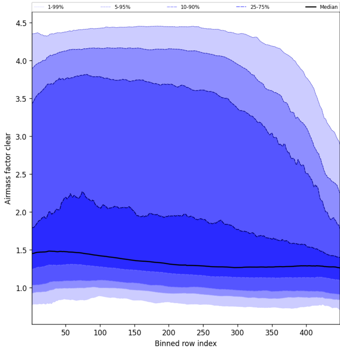
Figure 54: Along track statistics of “Airmass factor clear” for 2025-02-28 to 2025-03-01
