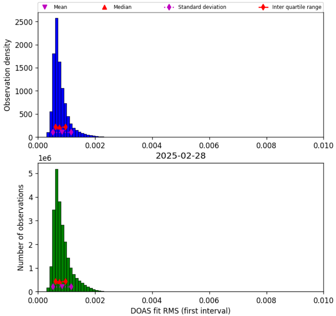
Figure 44: Histogram of “DOAS fit RMS (first interval)” for 2025-02-28 to 2025-03-01
