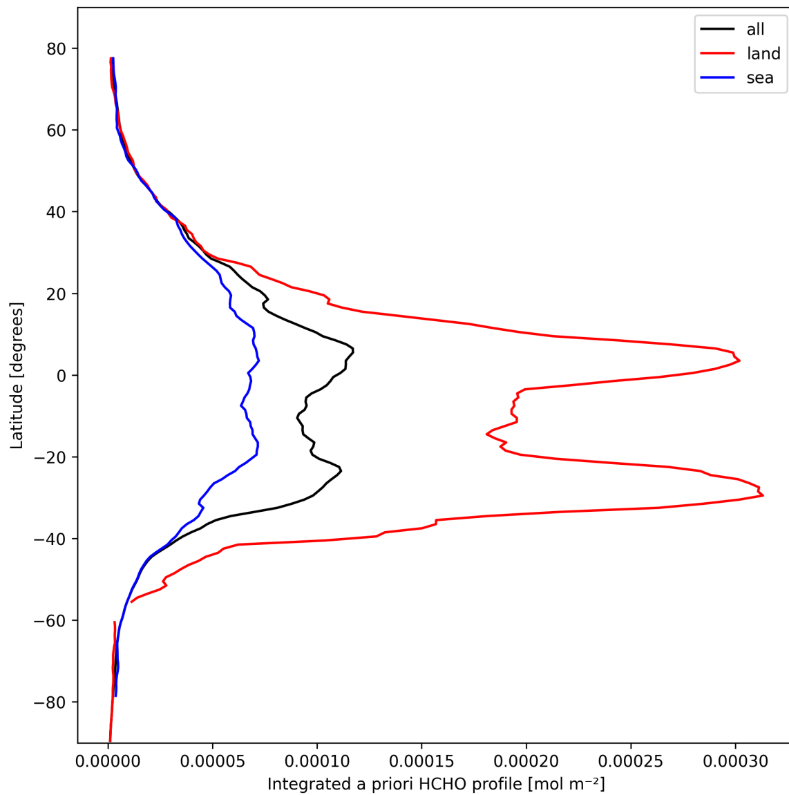
Figure 27: Zonal average of “Integrated a priori HCHO profile” for 2025-02-28 to 2025-03-01.
