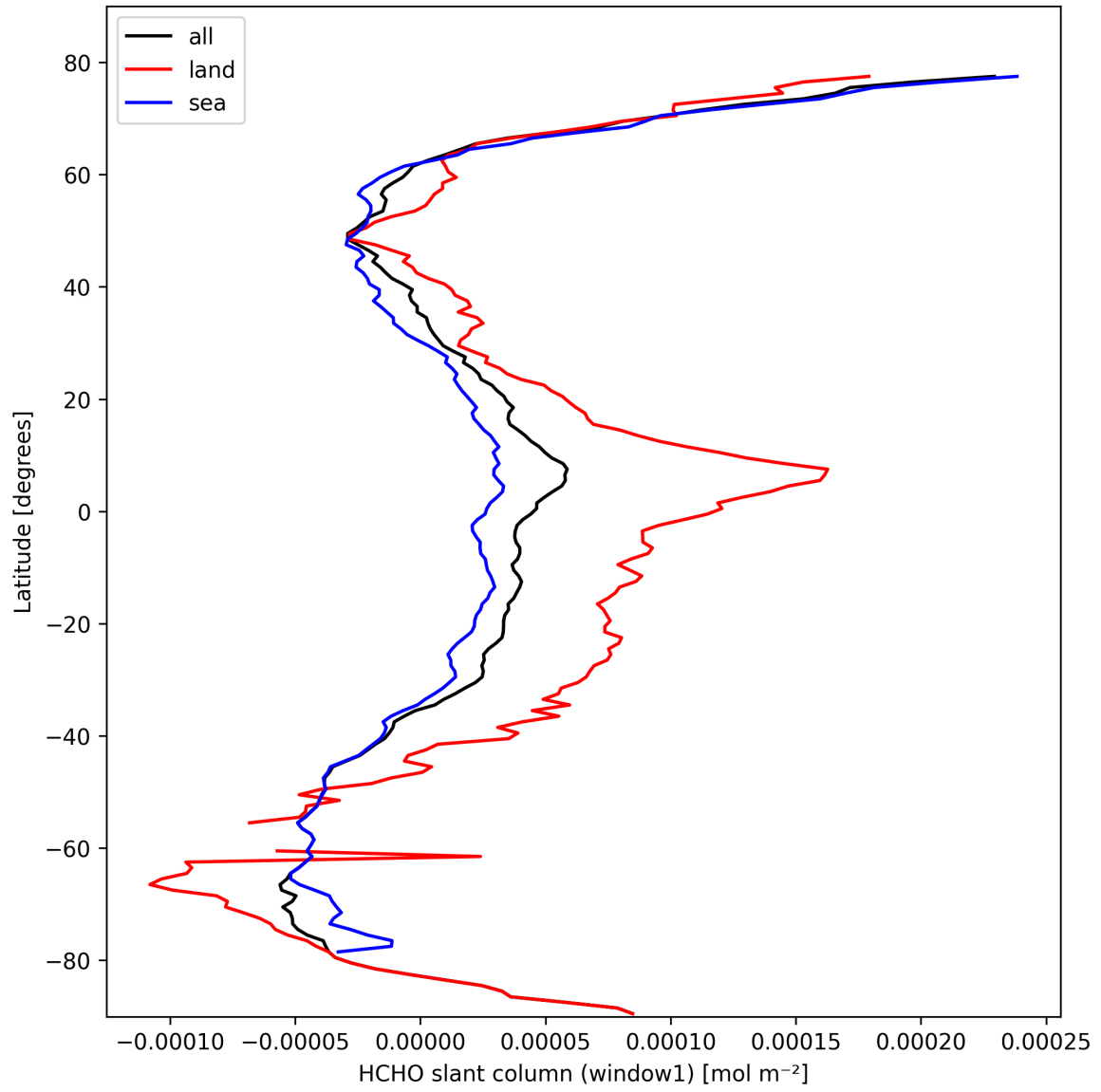
Figure 22: Zonal average of “HCHO slant column (window1)” for 2025-02-28 to 2025-03-01.
