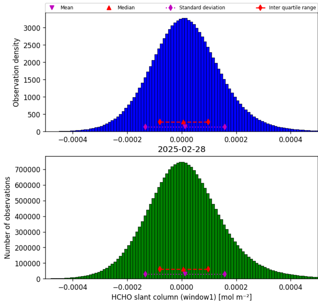
Figure 36: Histogram of “HCHO slant column (window1)” for 2025-02-28 to 2025-03-01
