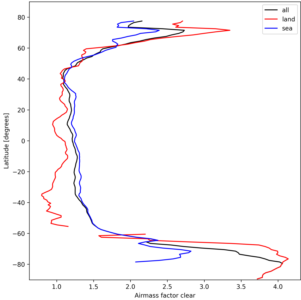
Figure 26: Zonal average of “Airmass factor clear” for 2025-02-28 to 2025-03-01.
