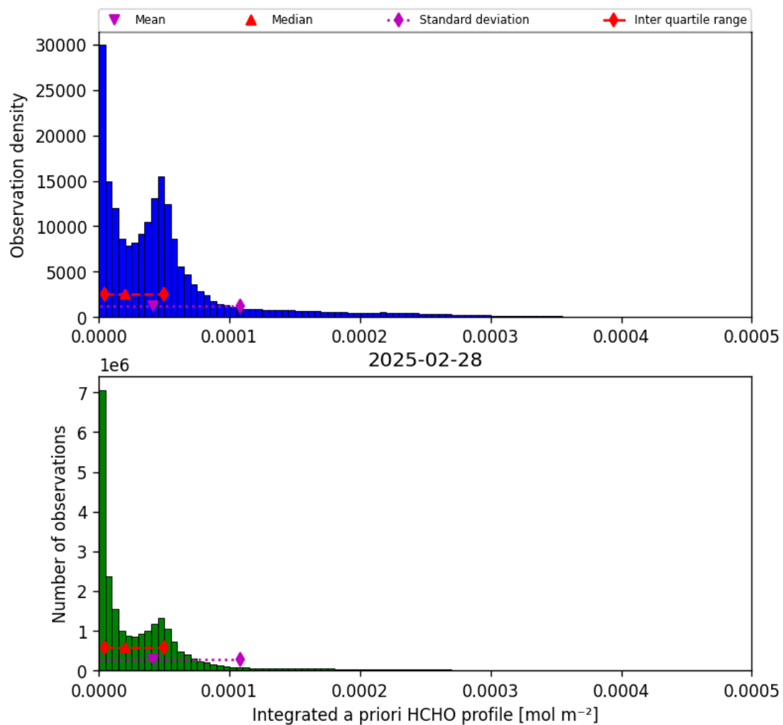
Figure 41: Histogram of “Integrated a priori HCHO profile” for 2025-02-28 to 2025-03-01
