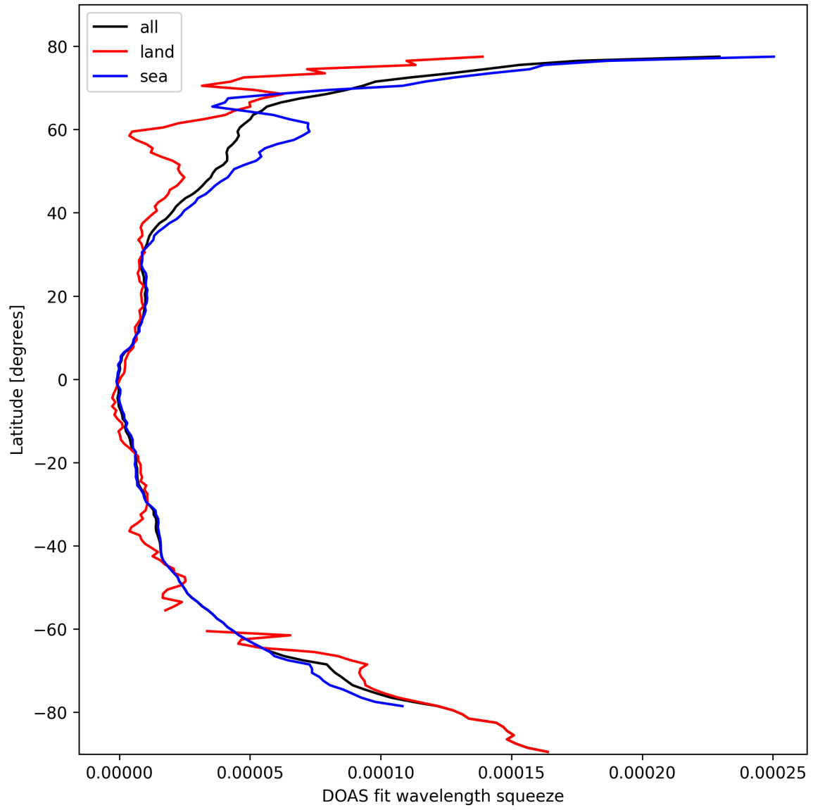
Figure 29: Zonal average of “DOAS fit wavelength squeeze” for 2025-02-28 to 2025-03-01.
