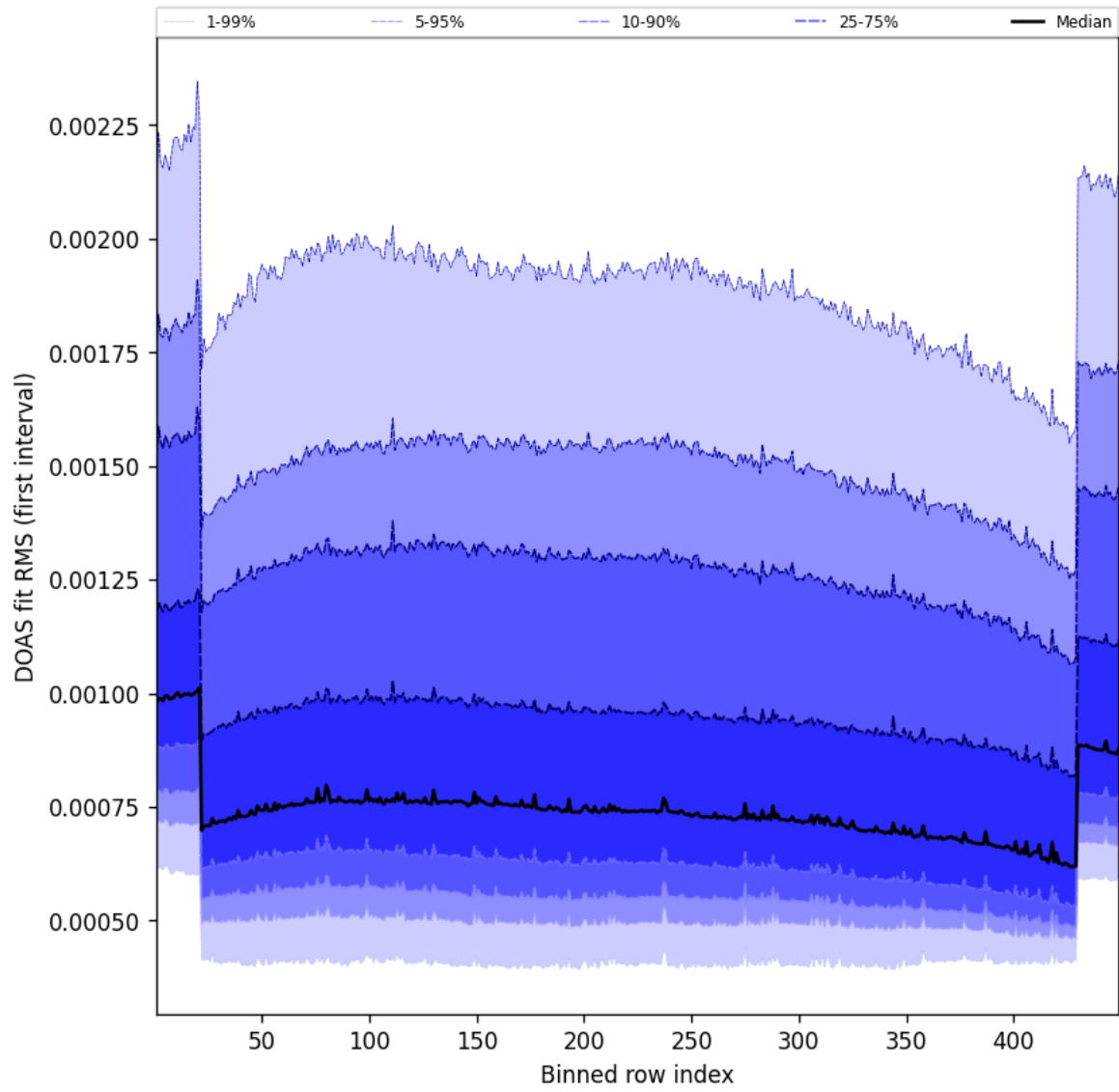
Figure 58: Along track statistics of “DOAS fit RMS (first interval)” for 2025-02-28 to 2025-03-01
