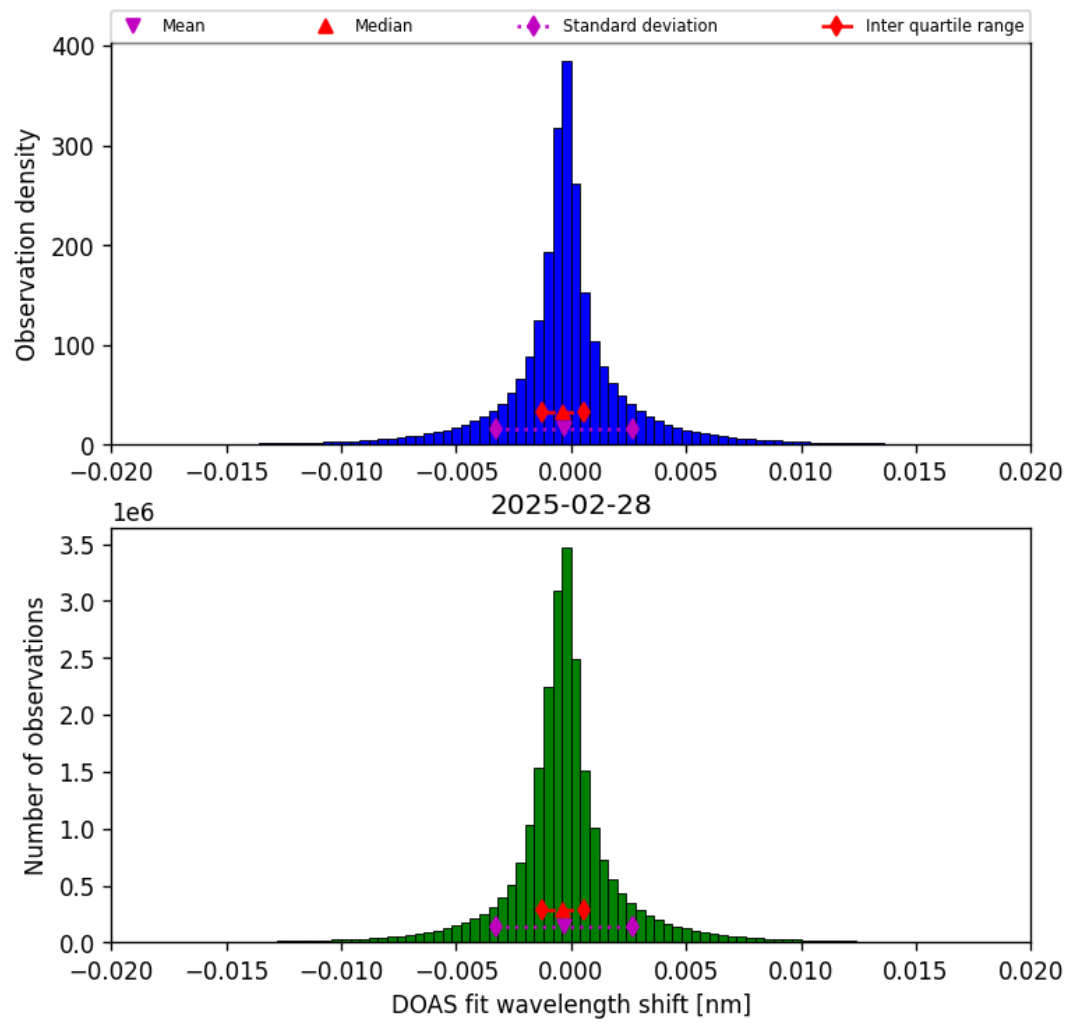
Figure 42: Histogram of “DOAS fit wavelength shift” for 2025-02-28 to 2025-03-01
