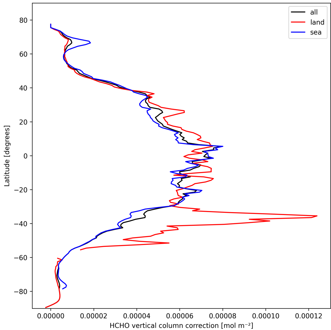
Figure 21: Zonal average of “HCHO vertical column correction” for 2025-02-28 to 2025-03-01.
