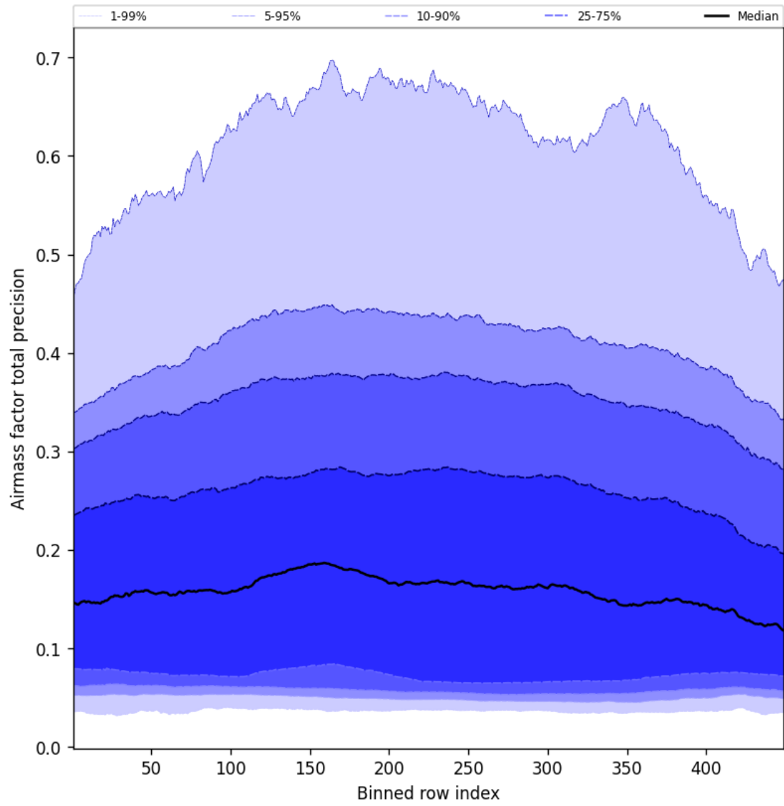
Figure 53: Along track statistics of “Airmass factor total precision” for 2025-02-28 to 2025-03-01
