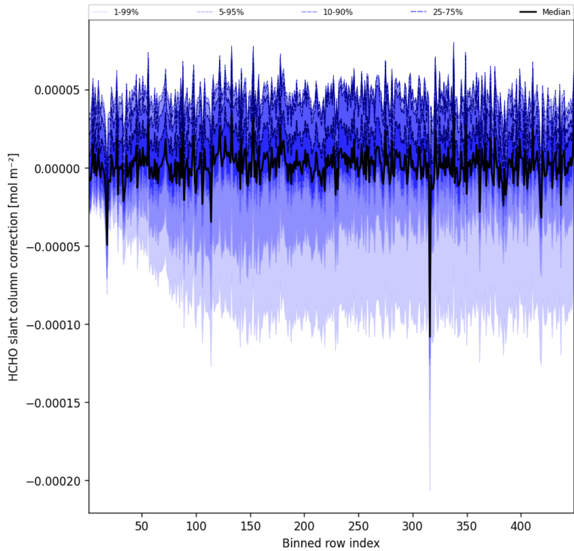
Figure 59: Along track statistics of “HCHO slant column correction” for 2025-02-28 to 2025-03-01
