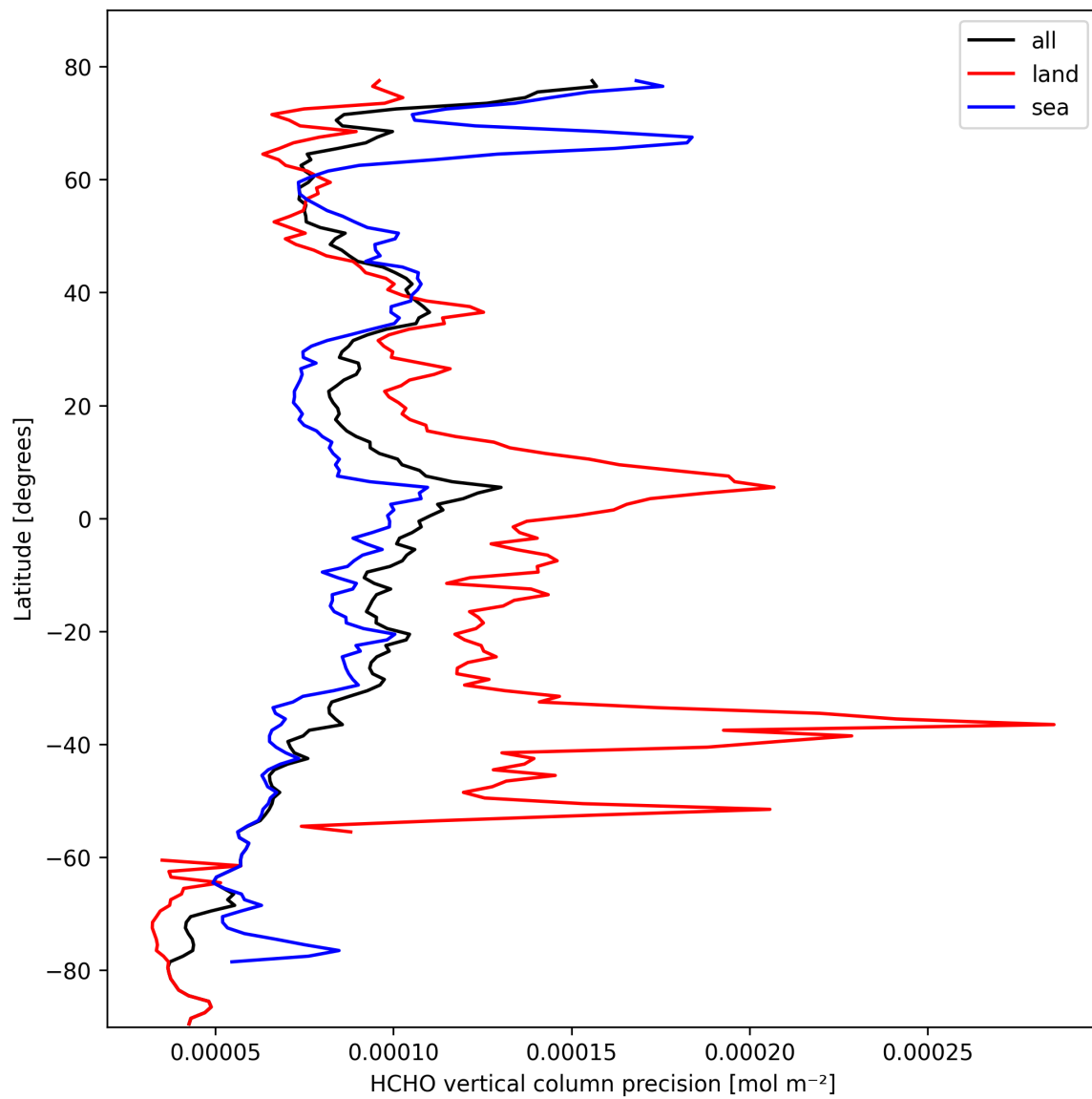
Figure 20: Zonal average of “HCHO vertical column precision” for 2025-02-28 to 2025-03-01.
