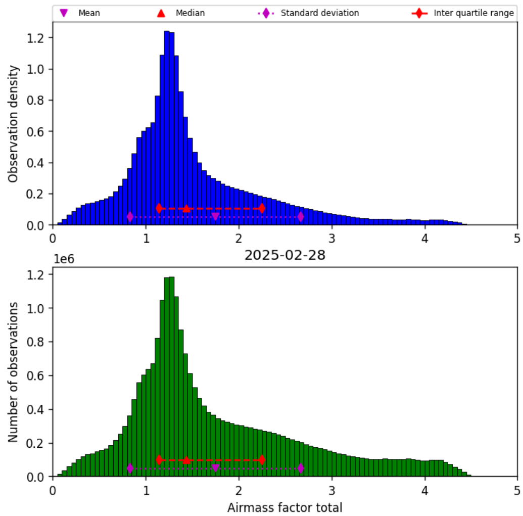
Figure 38: Histogram of “Airmass factor total” for 2025-02-28 to 2025-03-01
