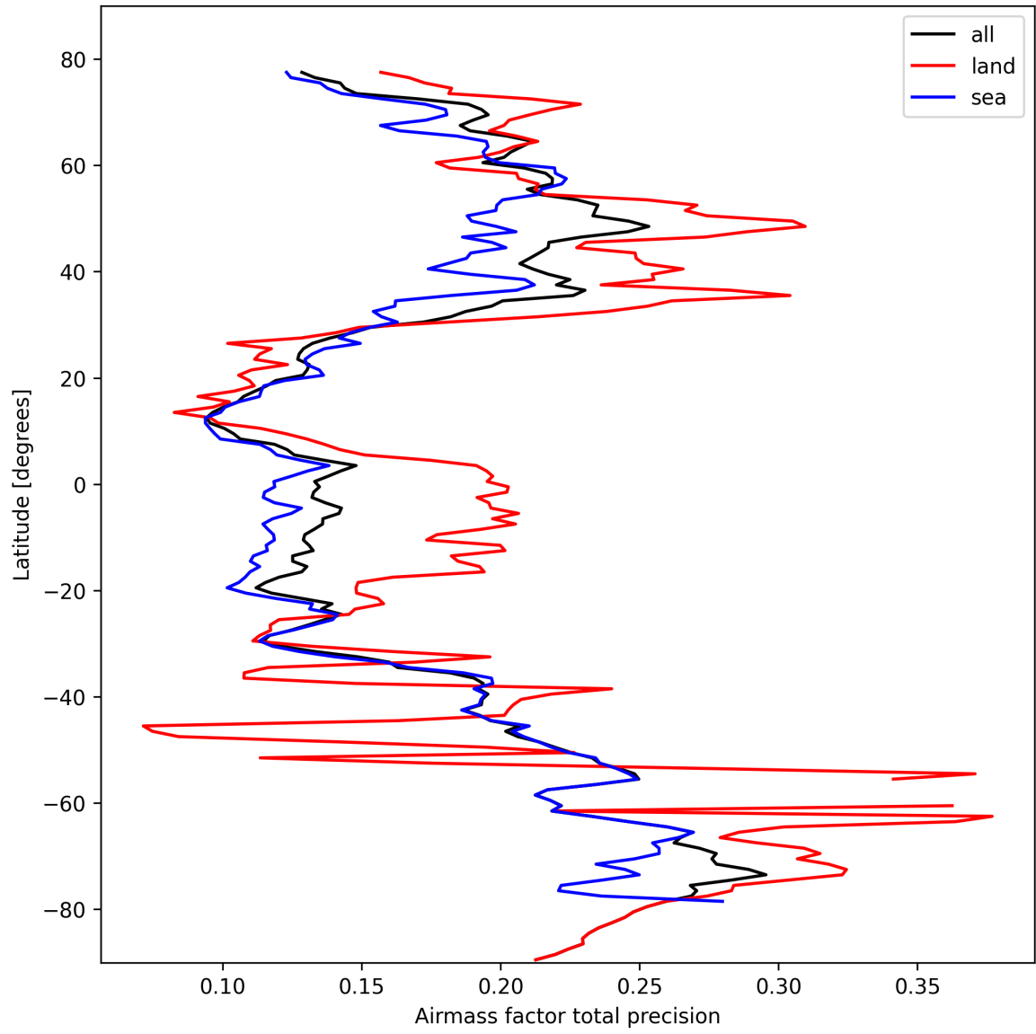
Figure 25: Zonal average of “Airmass factor total precision” for 2025-02-28 to 2025-03-01.
