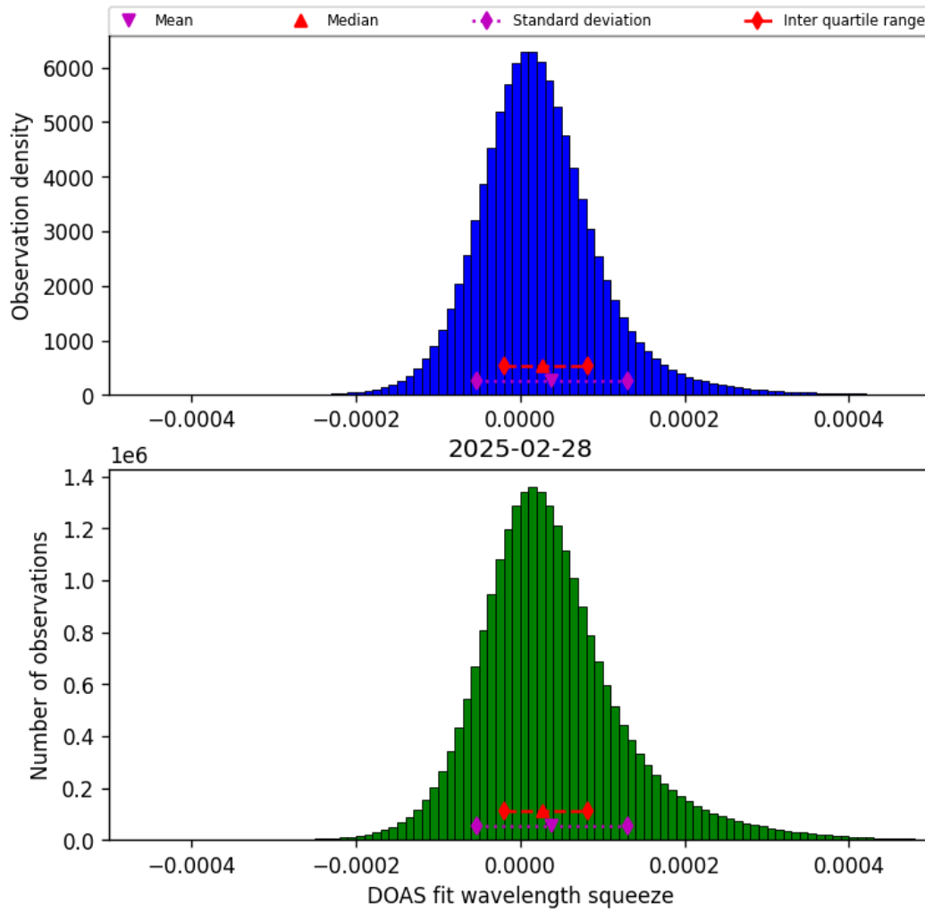
Figure 43: Histogram of “DOAS fit wavelength squeeze” for 2025-02-28 to 2025-03-01
