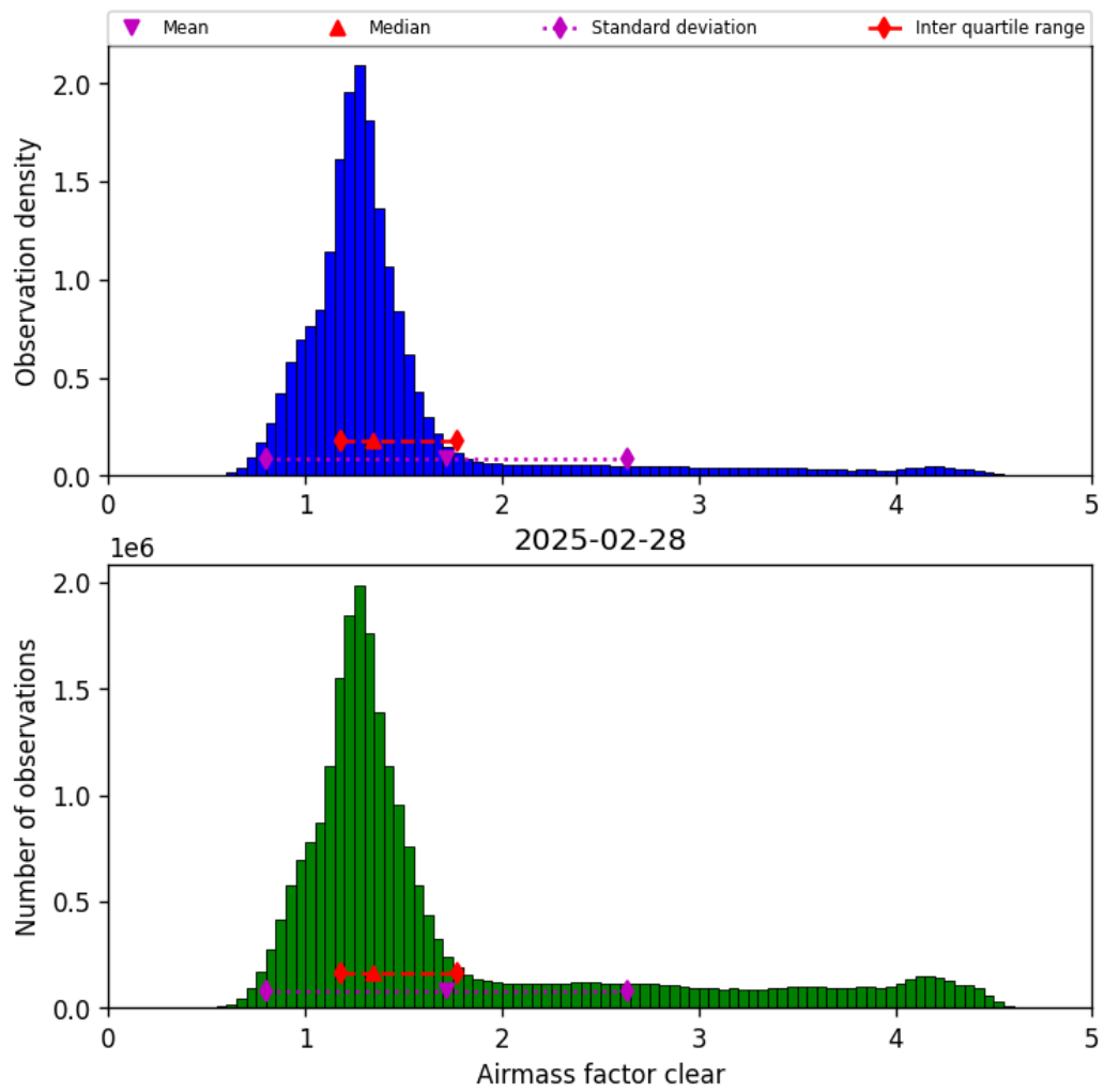
Figure 40: Histogram of “Airmass factor clear” for 2025-02-28 to 2025-03-01
