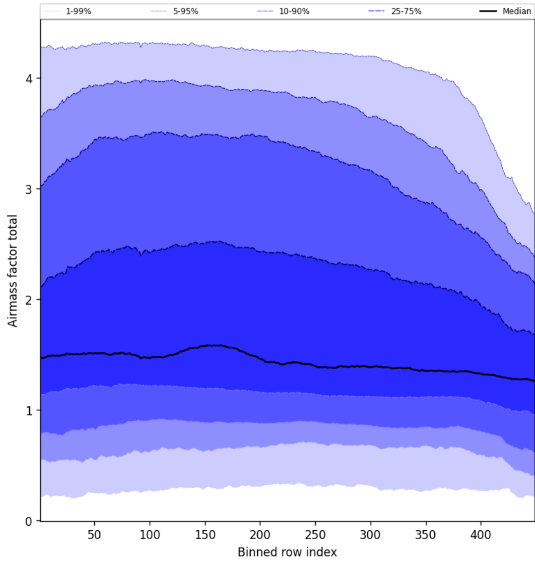
Figure 52: Along track statistics of “Airmass factor total” for 2025-02-28 to 2025-03-01
