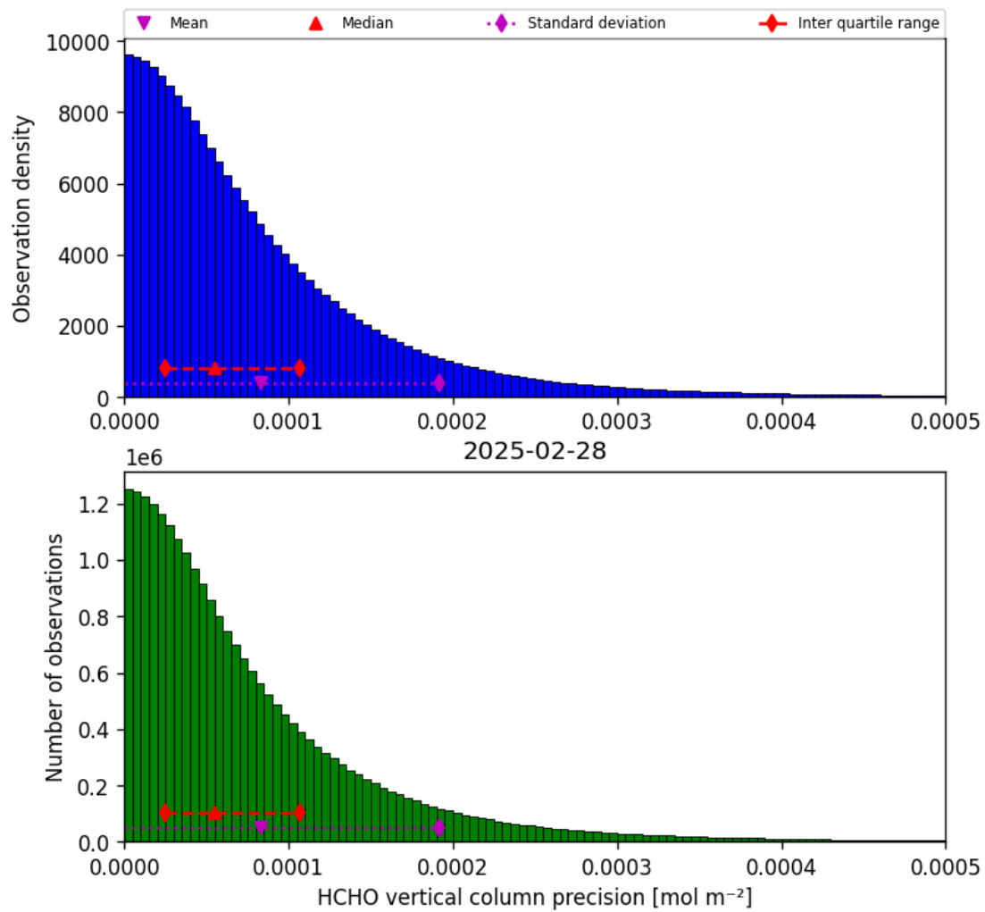
Figure 34: Histogram of “HCHO vertical column precision” for 2025-02-28 to 2025-03-01
