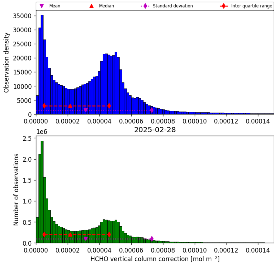
Figure 35: Histogram of “HCHO vertical column correction” for 2025-02-28 to 2025-03-01
