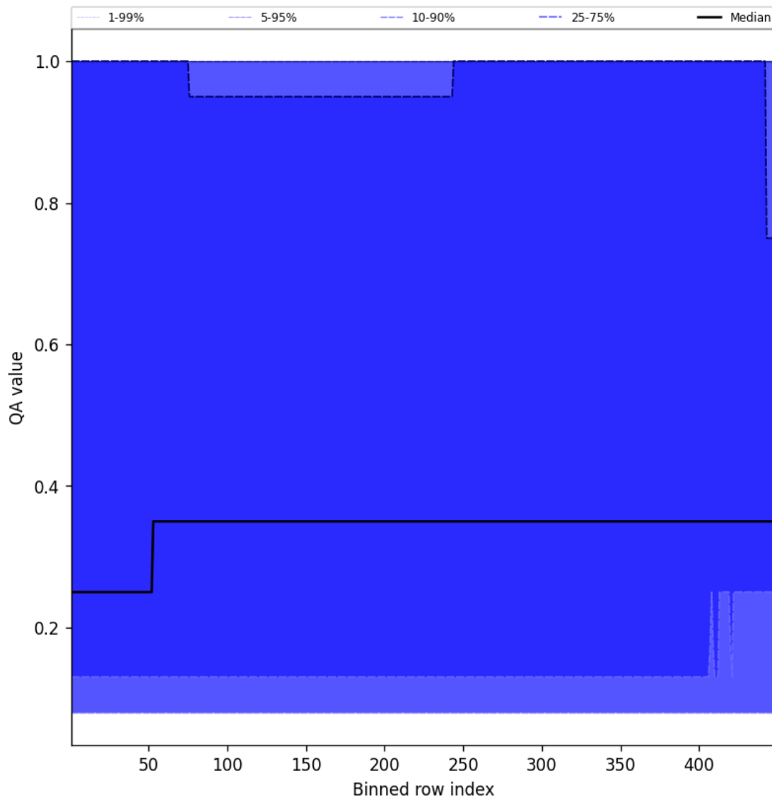
Figure 46: Along track statistics of “QA value” for 2025-02-28 to 2025-03-01
