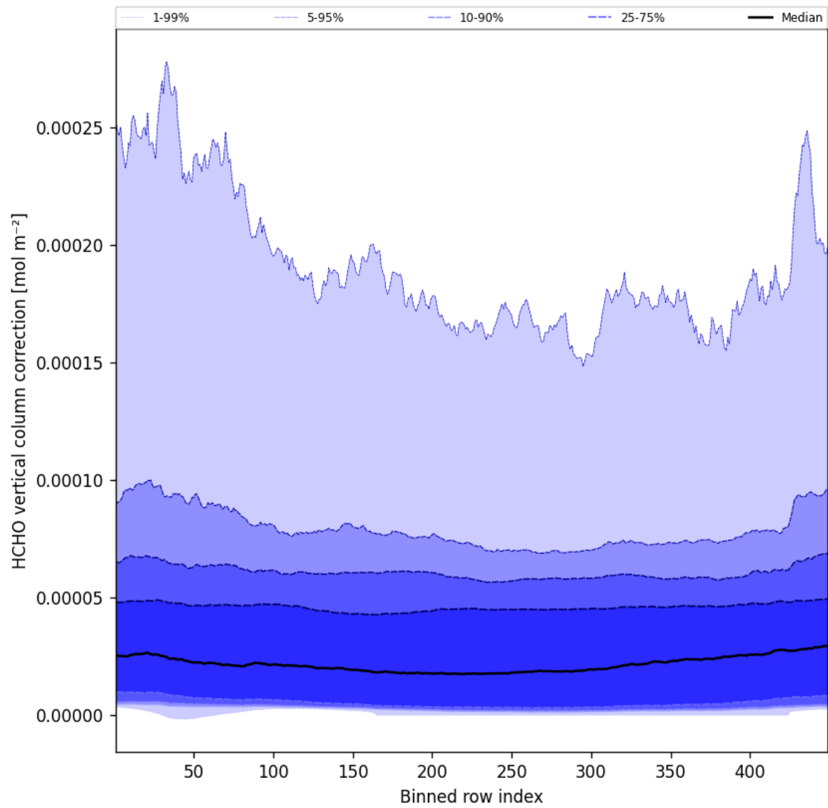
Figure 49: Along track statistics of “HCHO vertical column correction” for 2025-02-28 to 2025-03-01
