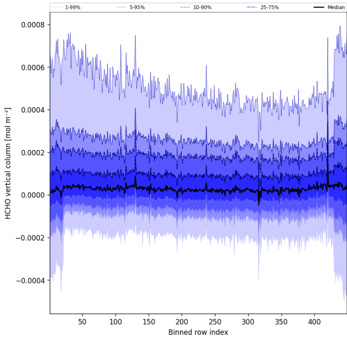
Figure 47: Along track statistics of “HCHO vertical column” for 2025-02-28 to 2025-03-01
