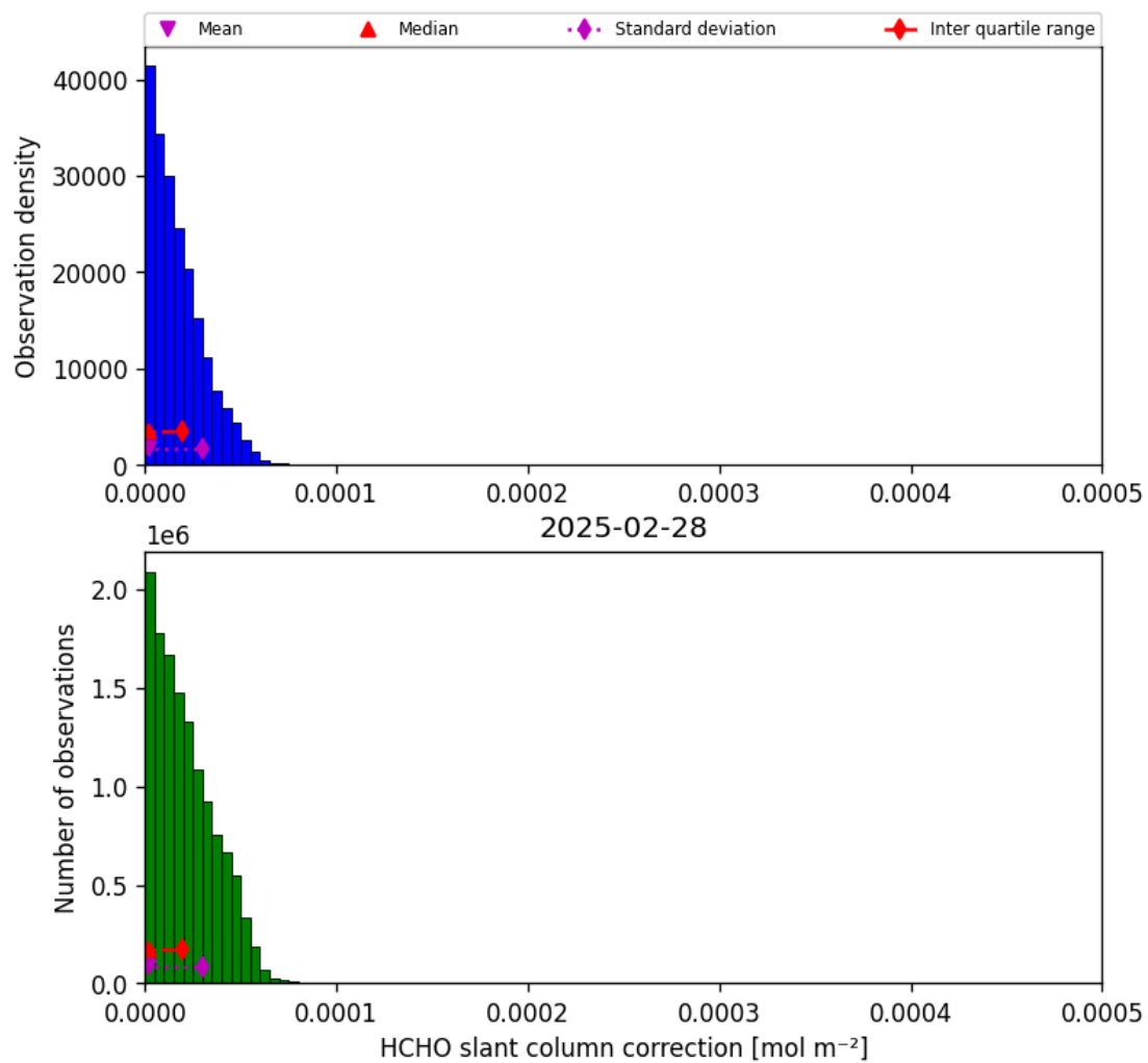
Figure 45: Histogram of “HCHO slant column correction” for 2025-02-28 to 2025-03-01
