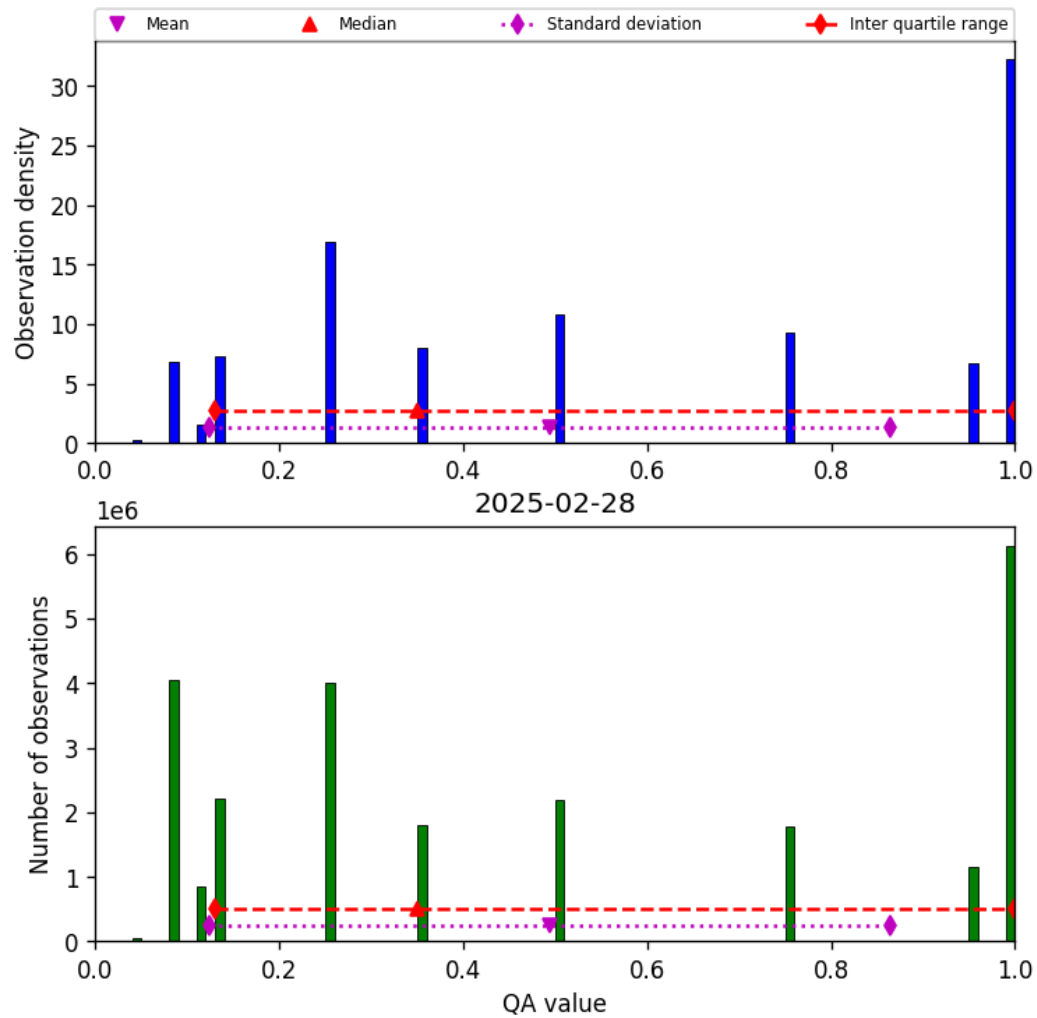
Figure 32: Histogram of “QA value” for 2025-02-28 to 2025-03-01
