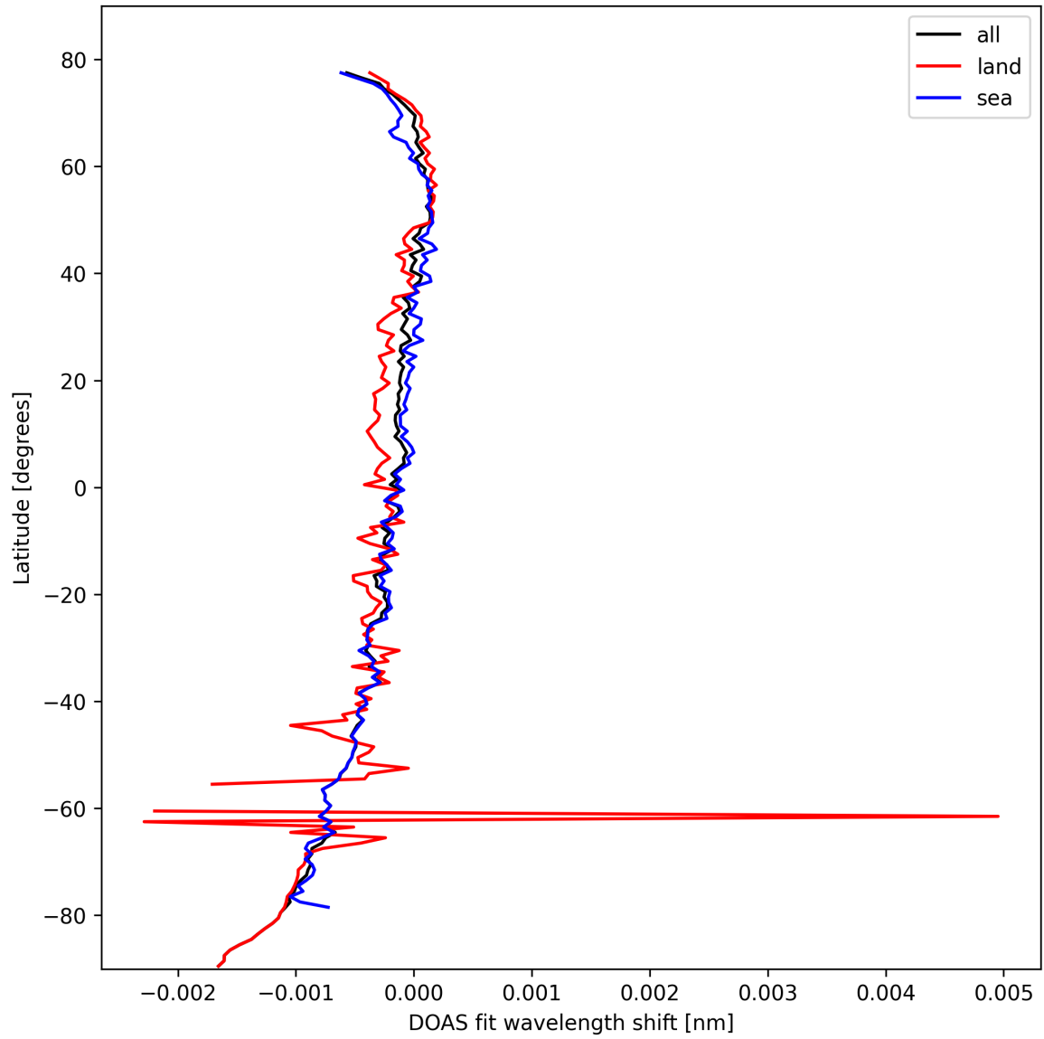
Figure 28: Zonal average of “DOAS fit wavelength shift” for 2025-02-28 to 2025-03-01.
