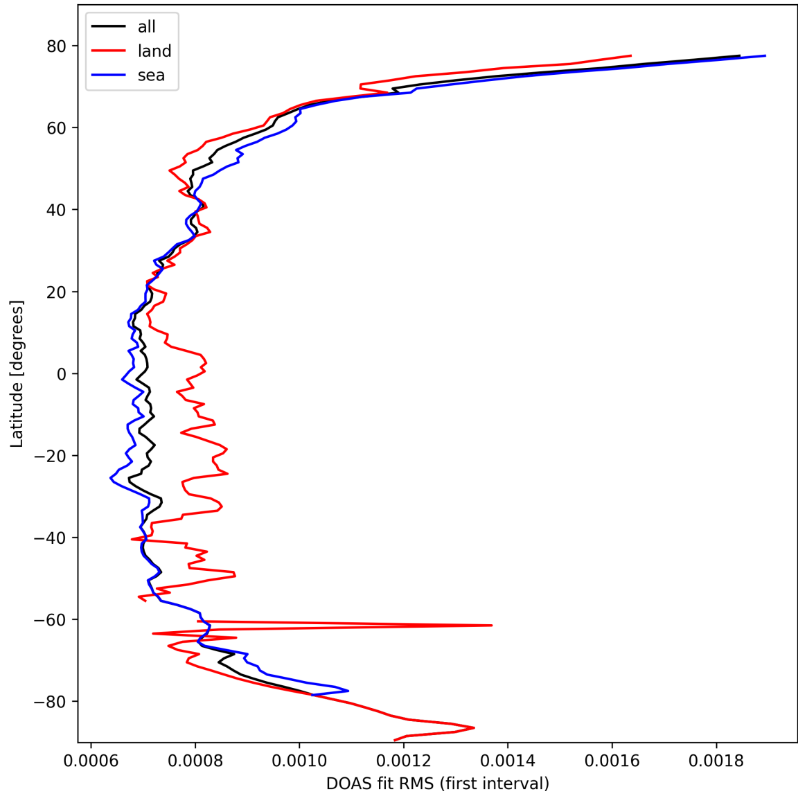
Figure 30: Zonal average of “DOAS fit RMS (first interval)” for 2025-02-28 to 2025-03-01.
