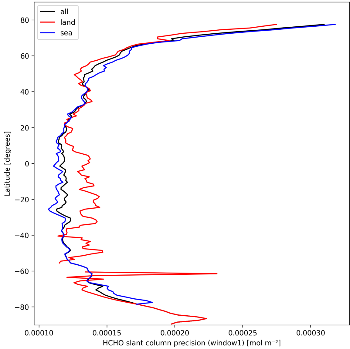
Figure 23: Zonal average of “HCHO slant column precision (window1)” for 2025-02-28 to 2025-03-01.
