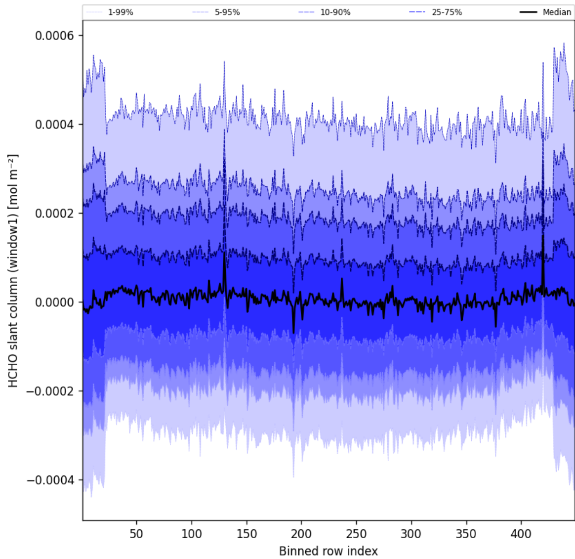
Figure 50: Along track statistics of “HCHO slant column (window1)” for 2025-02-28 to 2025-03-01
