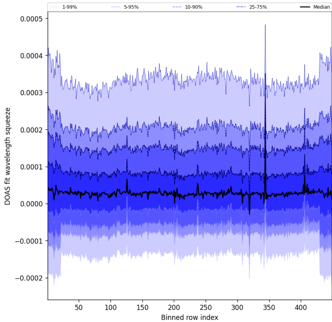
Figure 57: Along track statistics of “DOAS fit wavelength squeeze” for 2025-02-28 to 2025-03-01
