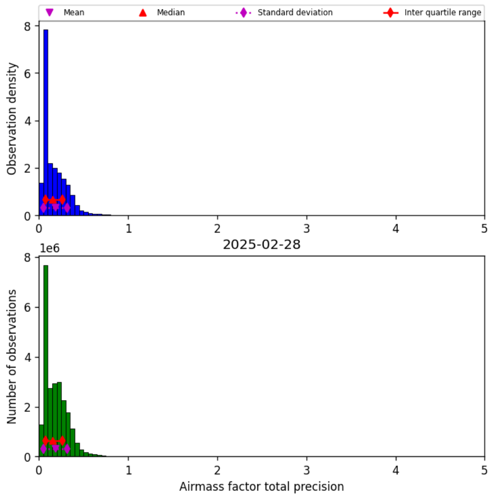
Figure 39: Histogram of “Airmass factor total precision” for 2025-02-28 to 2025-03-01
