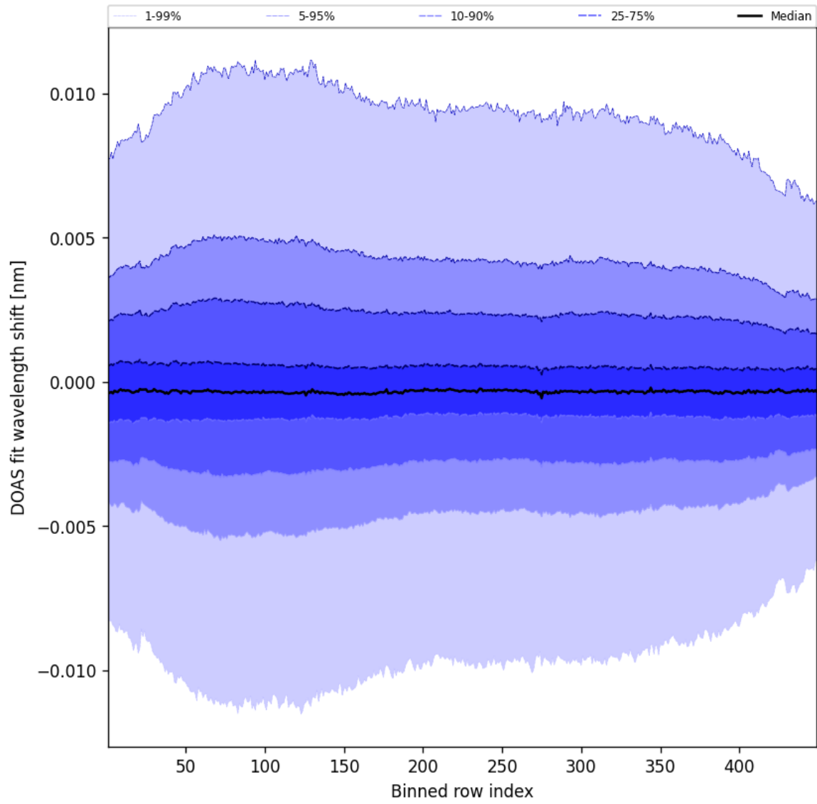
Figure 56: Along track statistics of “DOAS fit wavelength shift” for 2025-02-28 to 2025-03-01
