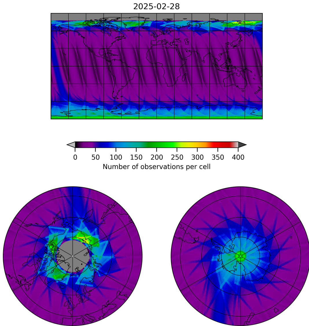
Figure 17: Map of the number of observations for 2025-02-28 to 2025-03-01
