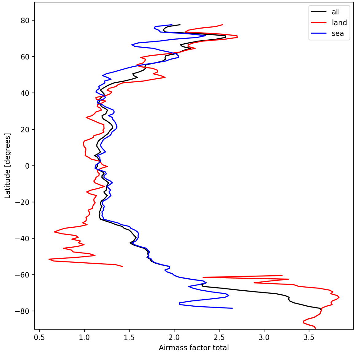
Figure 24: Zonal average of “Airmass factor total” for 2025-02-28 to 2025-03-01.
