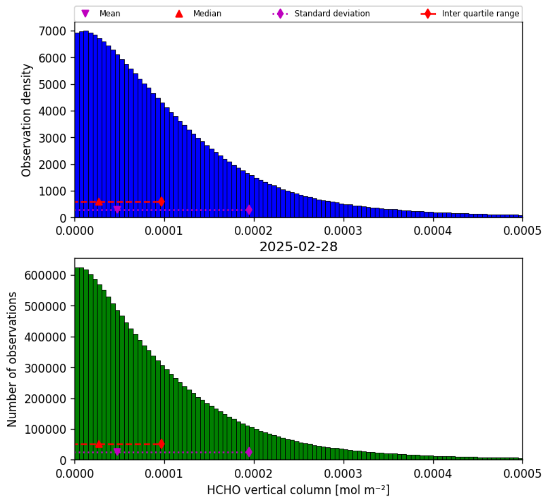
Figure 33: Histogram of “HCHO vertical column” for 2025-02-28 to 2025-03-01
