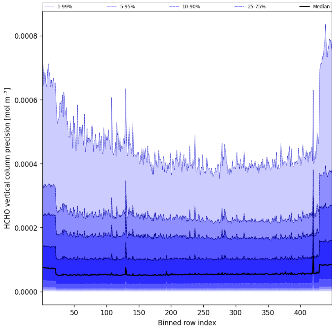
Figure 48: Along track statistics of “HCHO vertical column precision” for 2025-02-28 to 2025-03-01
