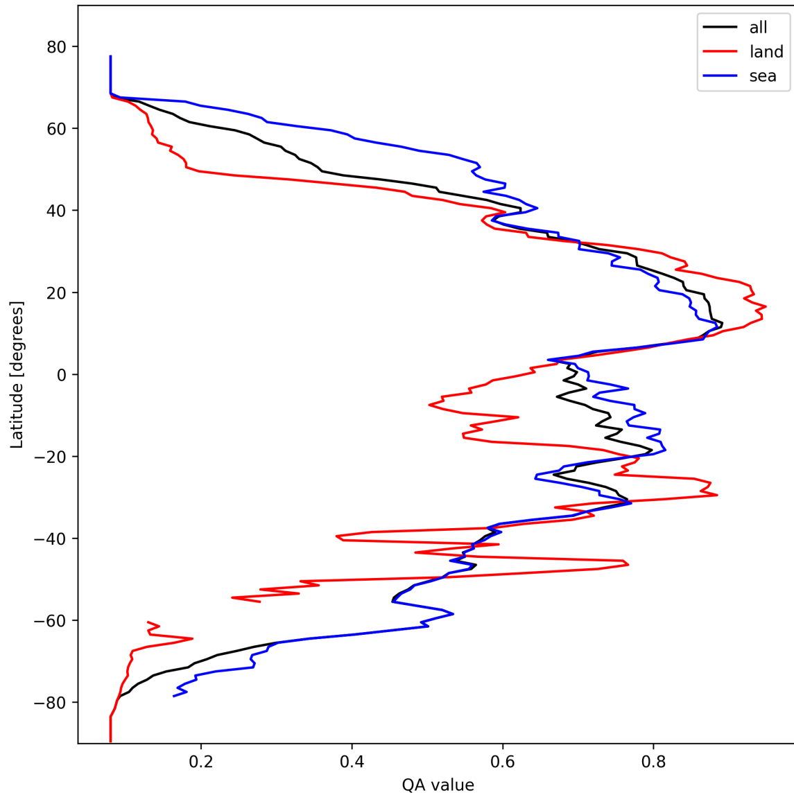
Figure 18: Zonal average of “QA value” for 2025-02-28 to 2025-03-01.
