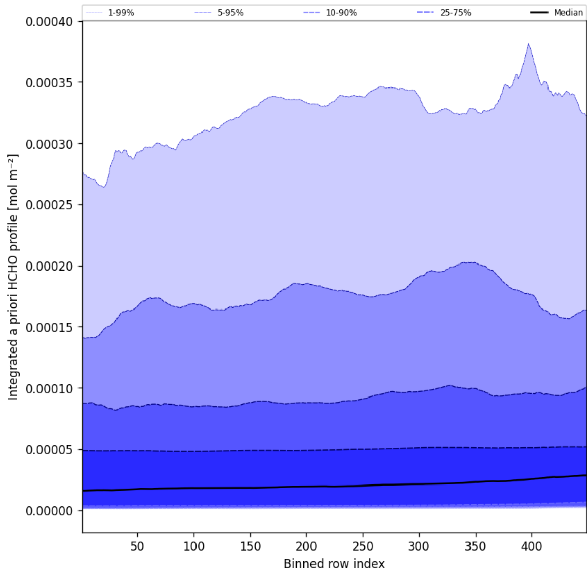
Figure 55: Along track statistics of "Integrated a priori HCHO profile" for 2025-02-28 to 2025-03-01
