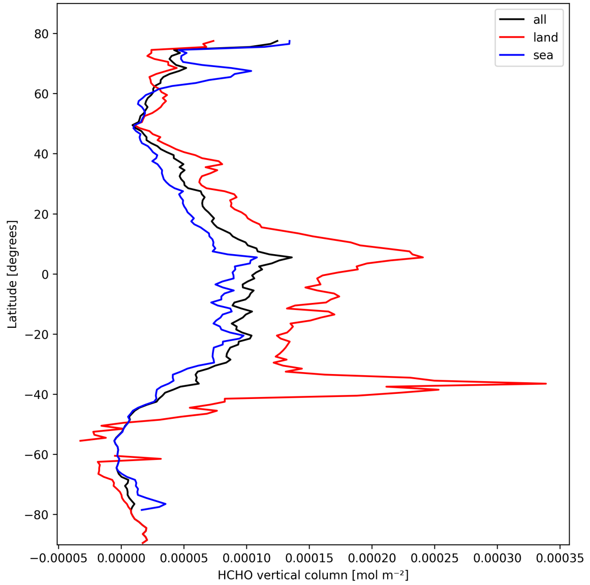
Figure 19: Zonal average of “HCHO vertical column” for 2025-02-28 to 2025-03-01.
