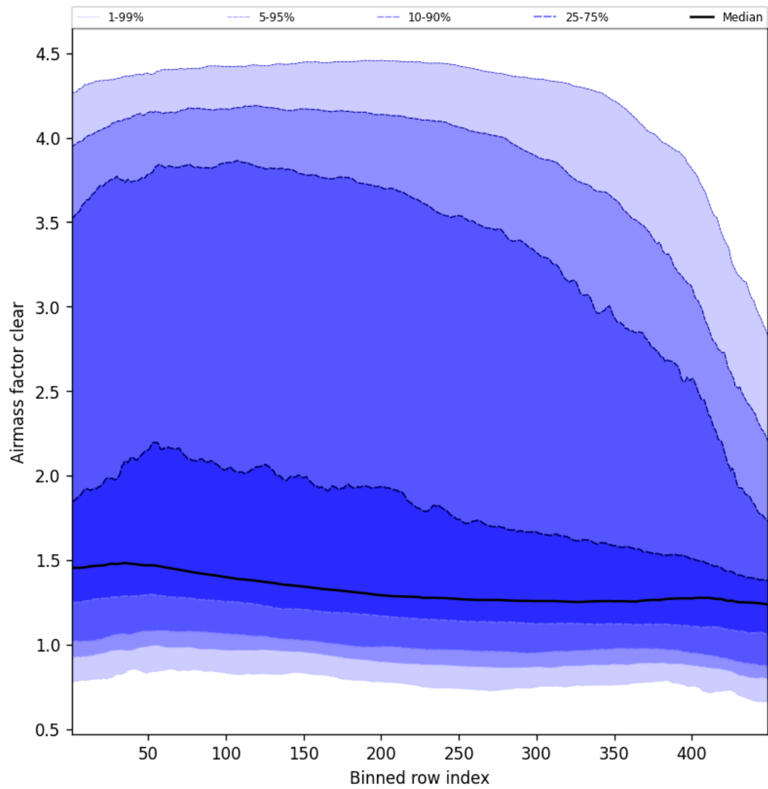
Figure 54: Along track statistics of “Airmass factor clear” for 2025-03-01 to 2025-03-02
