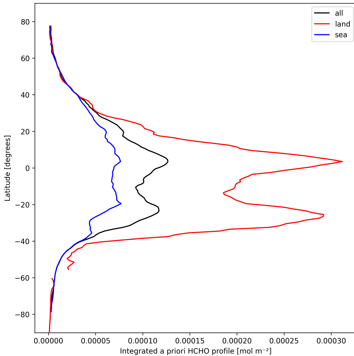
Figure 27: Zonal average of “Integrated a priori HCHO profile” for 2025-03-01 to 2025-03-02.
