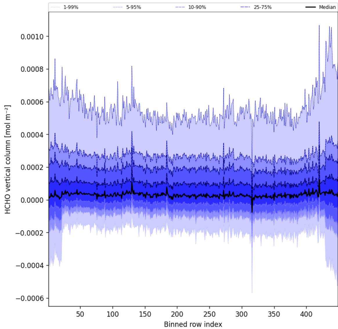
Figure 47: Along track statistics of “HCHO vertical column” for 2025-03-01 to 2025-03-02
