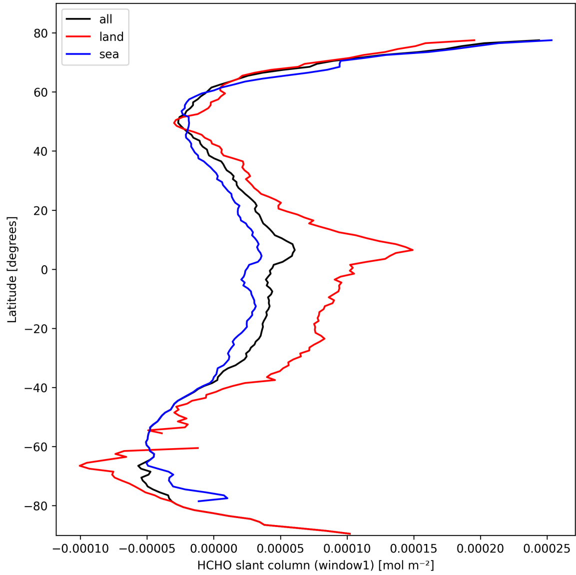
Figure 22: Zonal average of “HCHO slant column (window1)” for 2025-03-01 to 2025-03-02.
