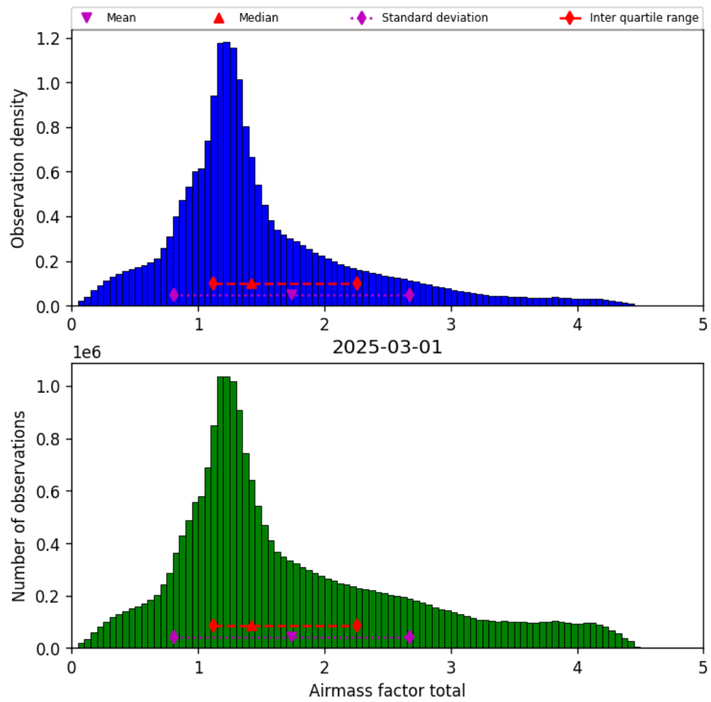
Figure 38: Histogram of “Airmass factor total” for 2025-03-01 to 2025-03-02
