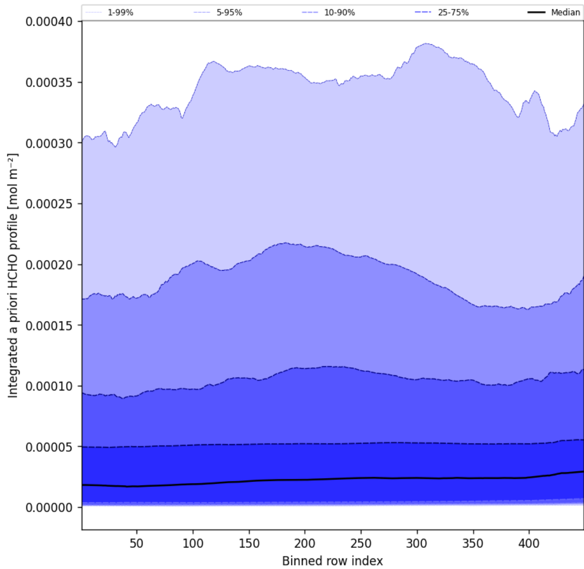
Figure 55: Along track statistics of “Integrated a priori HCHO profile” for 2025-03-01 to 2025-03-02
