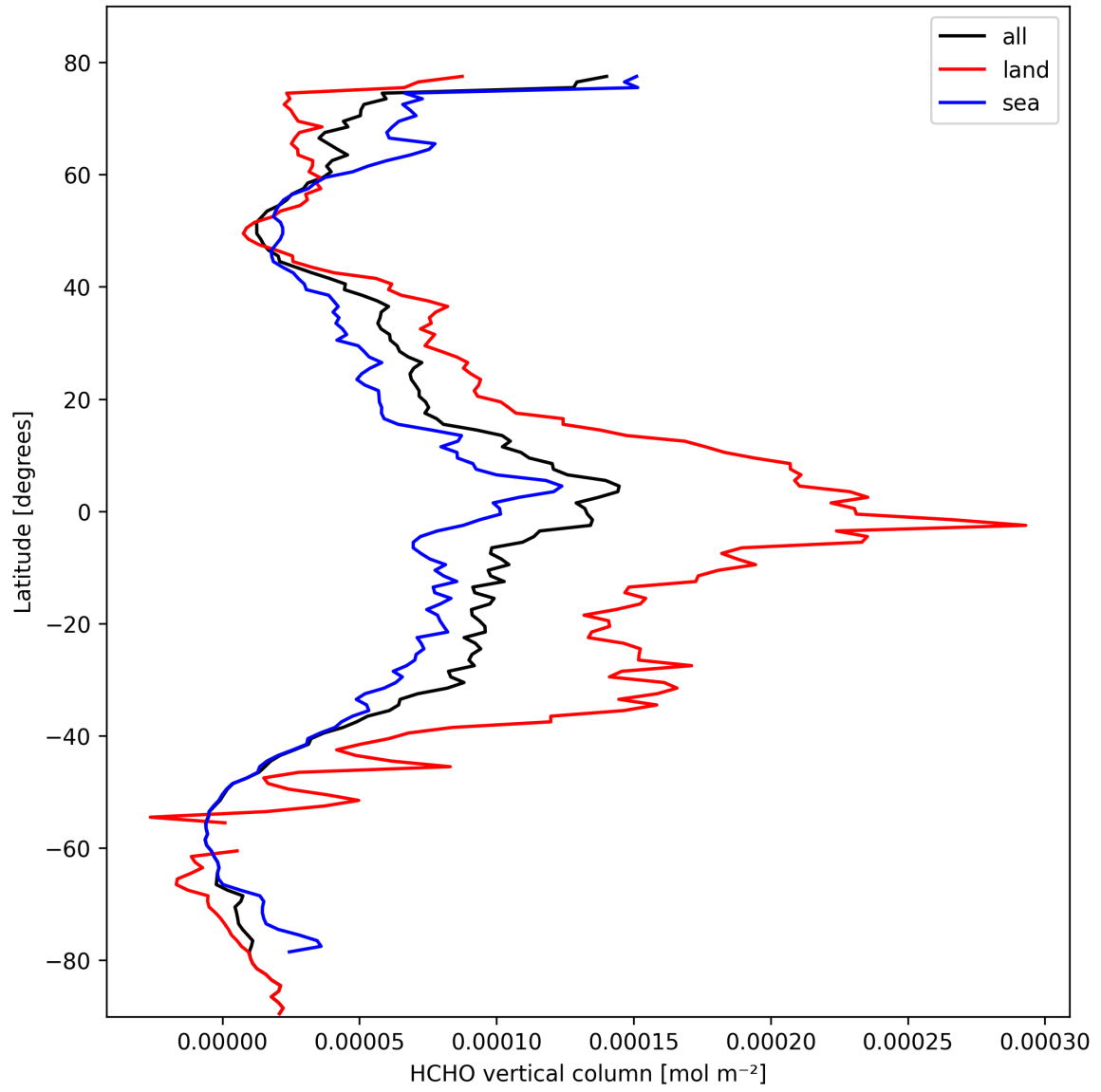
Figure 19: Zonal average of “HCHO vertical column” for 2025-03-01 to 2025-03-02.
