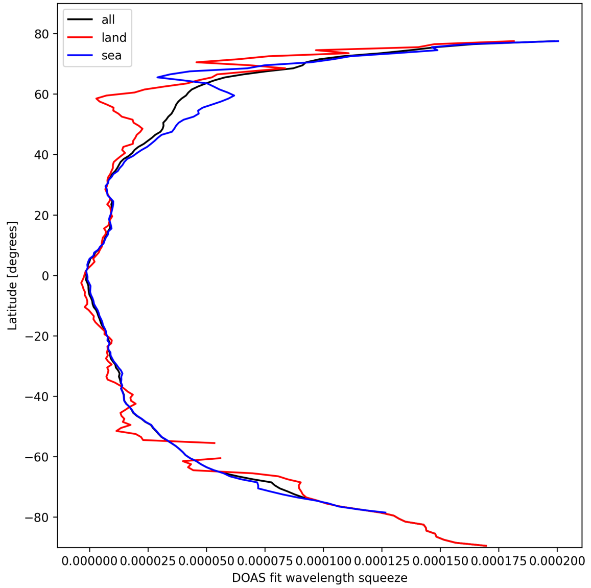
Figure 29: Zonal average of “DOAS fit wavelength squeeze” for 2025-03-01 to 2025-03-02.
