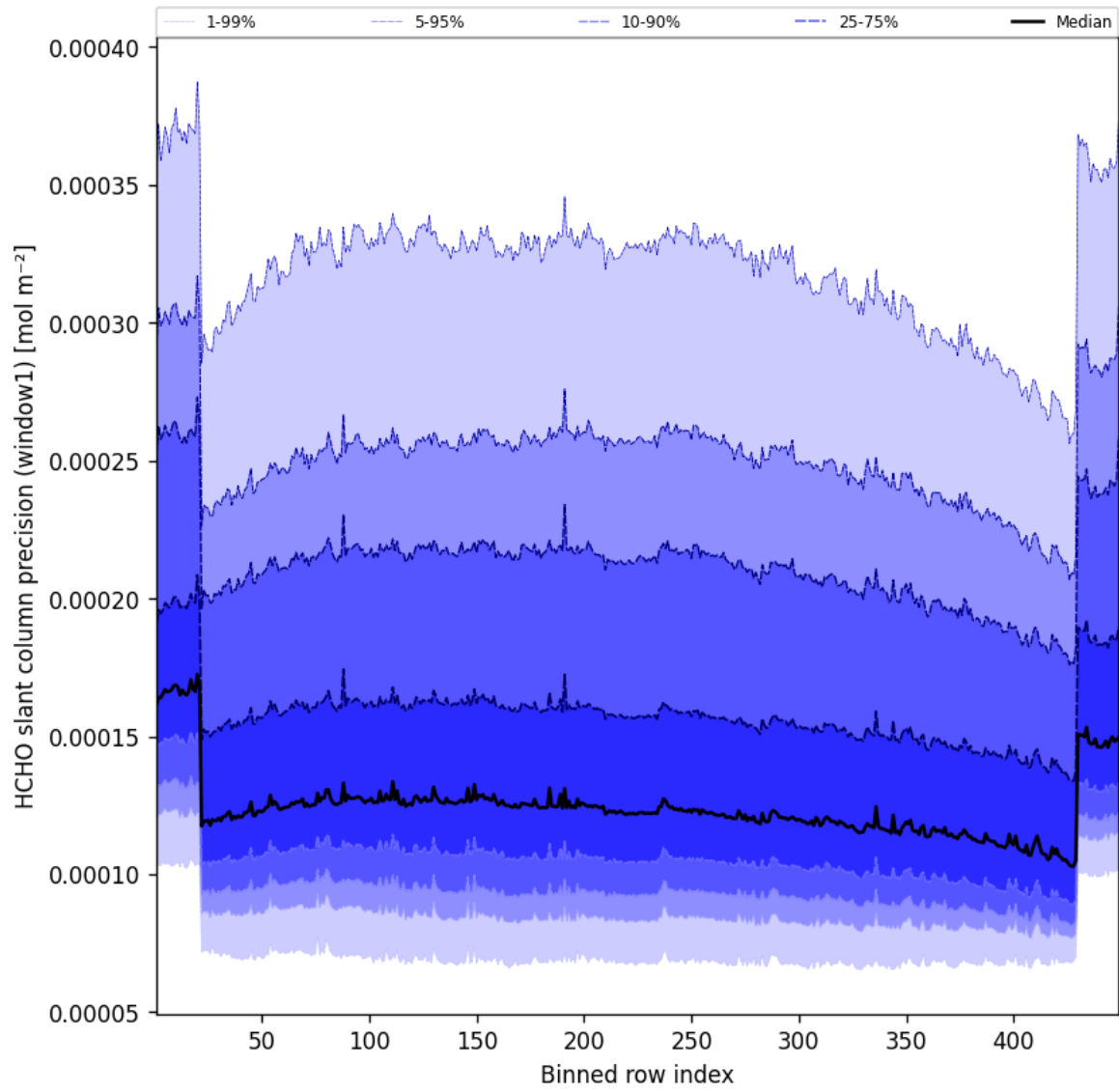
Figure 51: Along track statistics of “HCHO slant column precision (window1)” for 2025-03-01 to 2025-03-02
