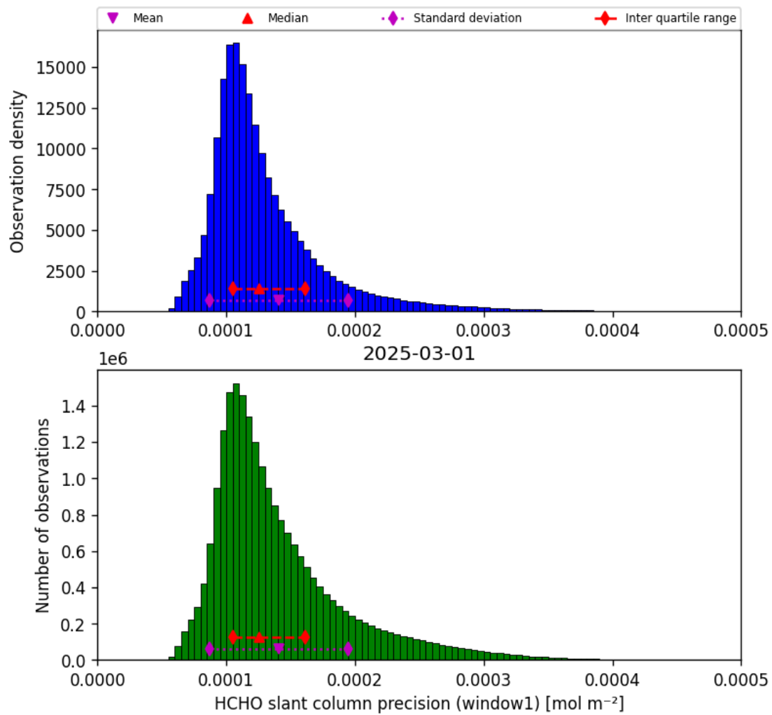
Figure 37: Histogram of “HCHO slant column precision (window1)” for 2025-03-01 to 2025-03-02
