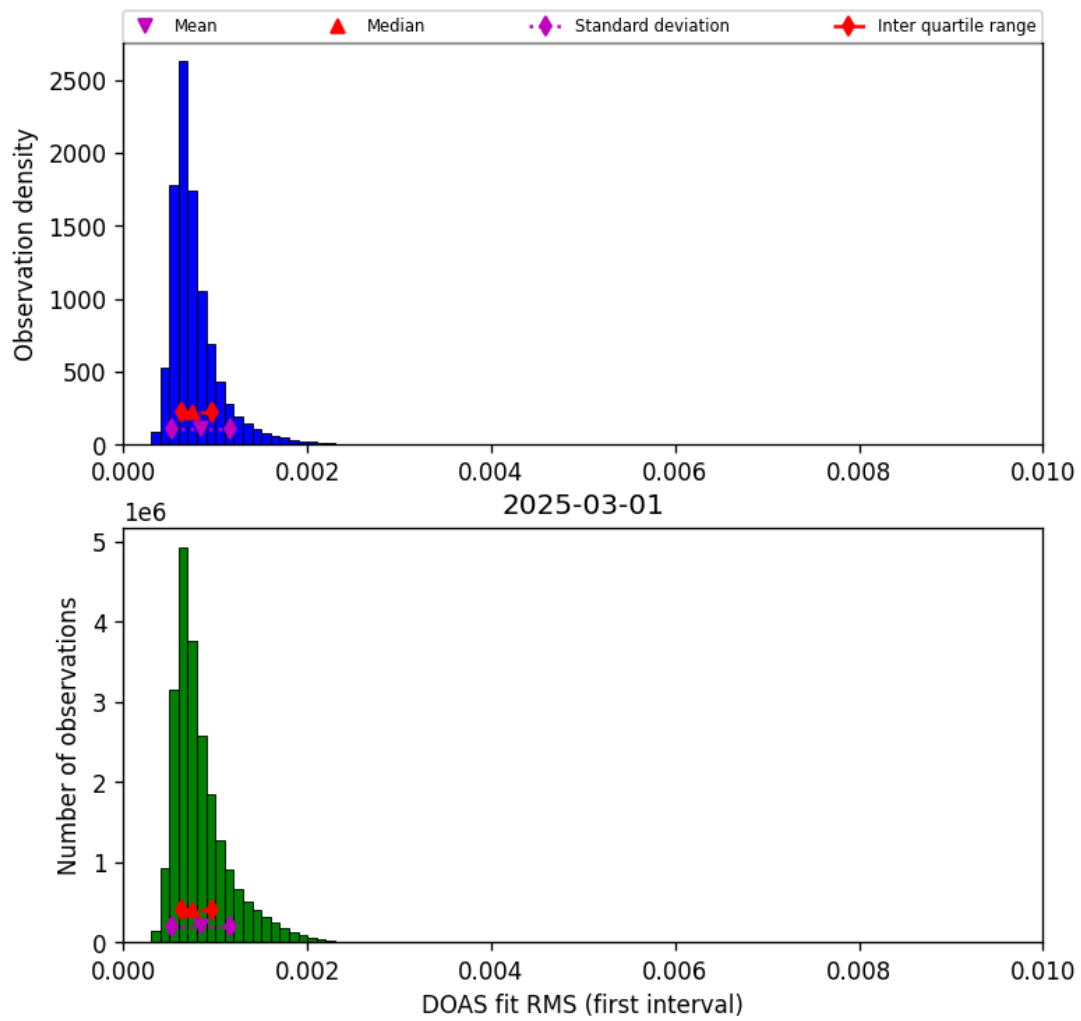
Figure 44: Histogram of “DOAS fit RMS (first interval)” for 2025-03-01 to 2025-03-02
