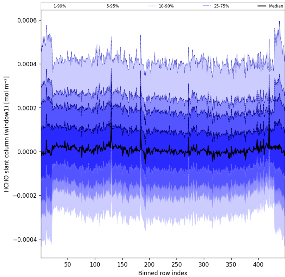
Figure 50: Along track statistics of “HCHO slant column (window1)” for 2025-03-01 to 2025-03-02
