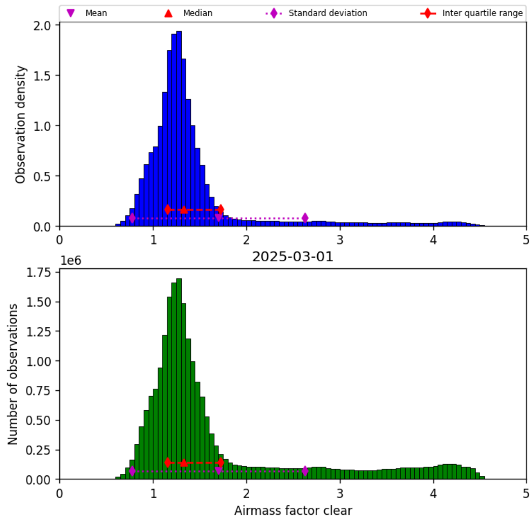
Figure 40: Histogram of “Airmass factor clear” for 2025-03-01 to 2025-03-02
