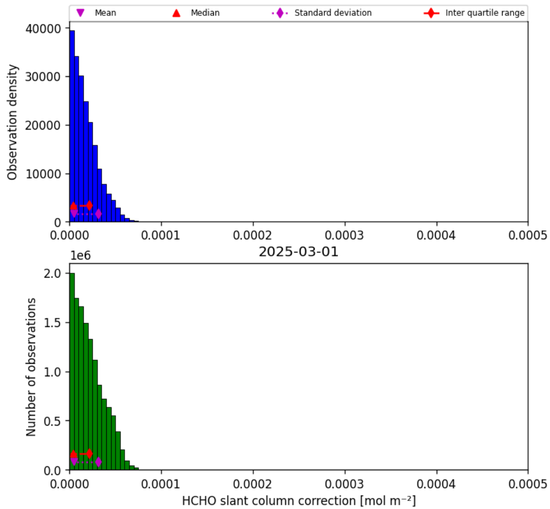
Figure 45: Histogram of “HCHO slant column correction” for 2025-03-01 to 2025-03-02
