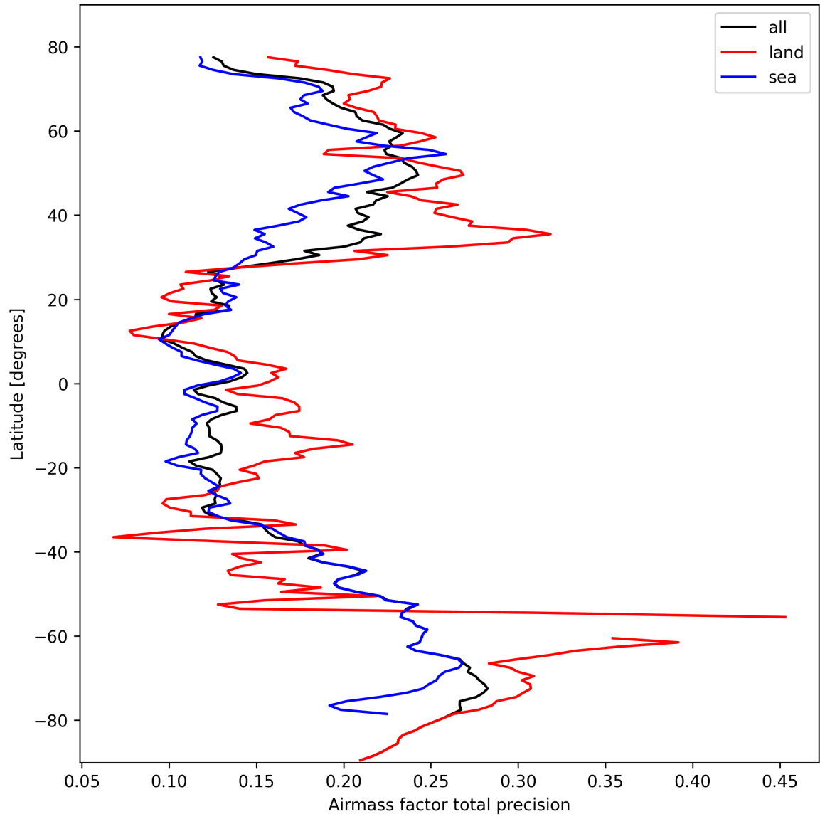
Figure 25: Zonal average of “Airmass factor total precision” for 2025-03-01 to 2025-03-02.
