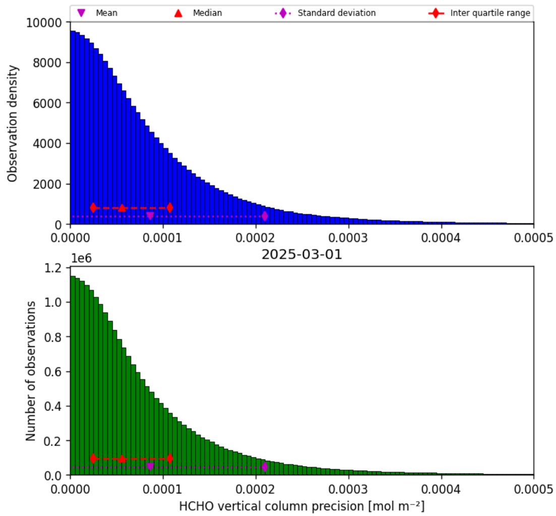
Figure 34: Histogram of "HCHO vertical column precision" for 2025-03-01 to 2025-03-02
