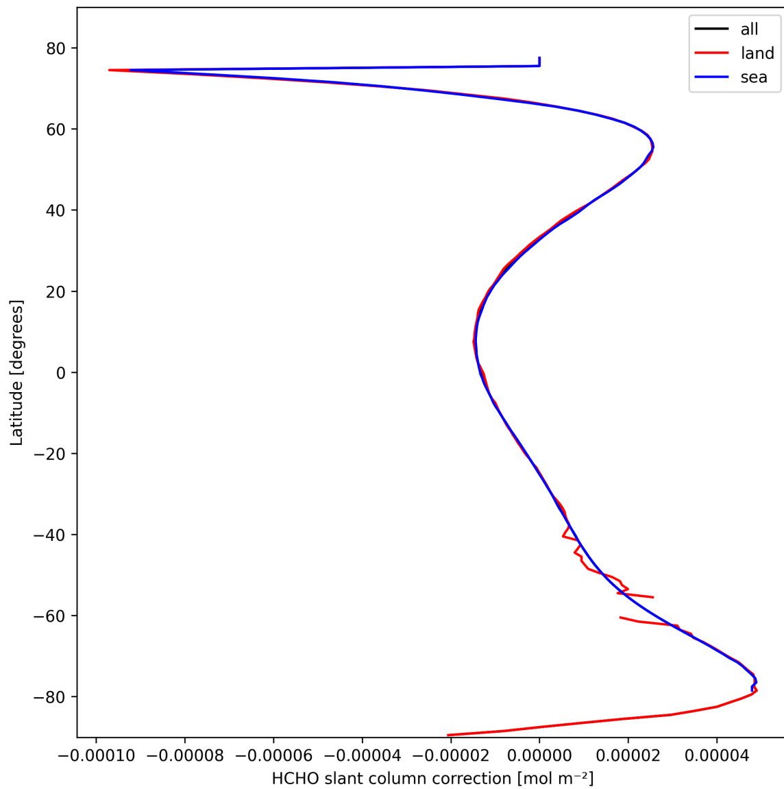
Figure 31: Zonal average of “HCHO slant column correction” for 2025-03-01 to 2025-03-02.
