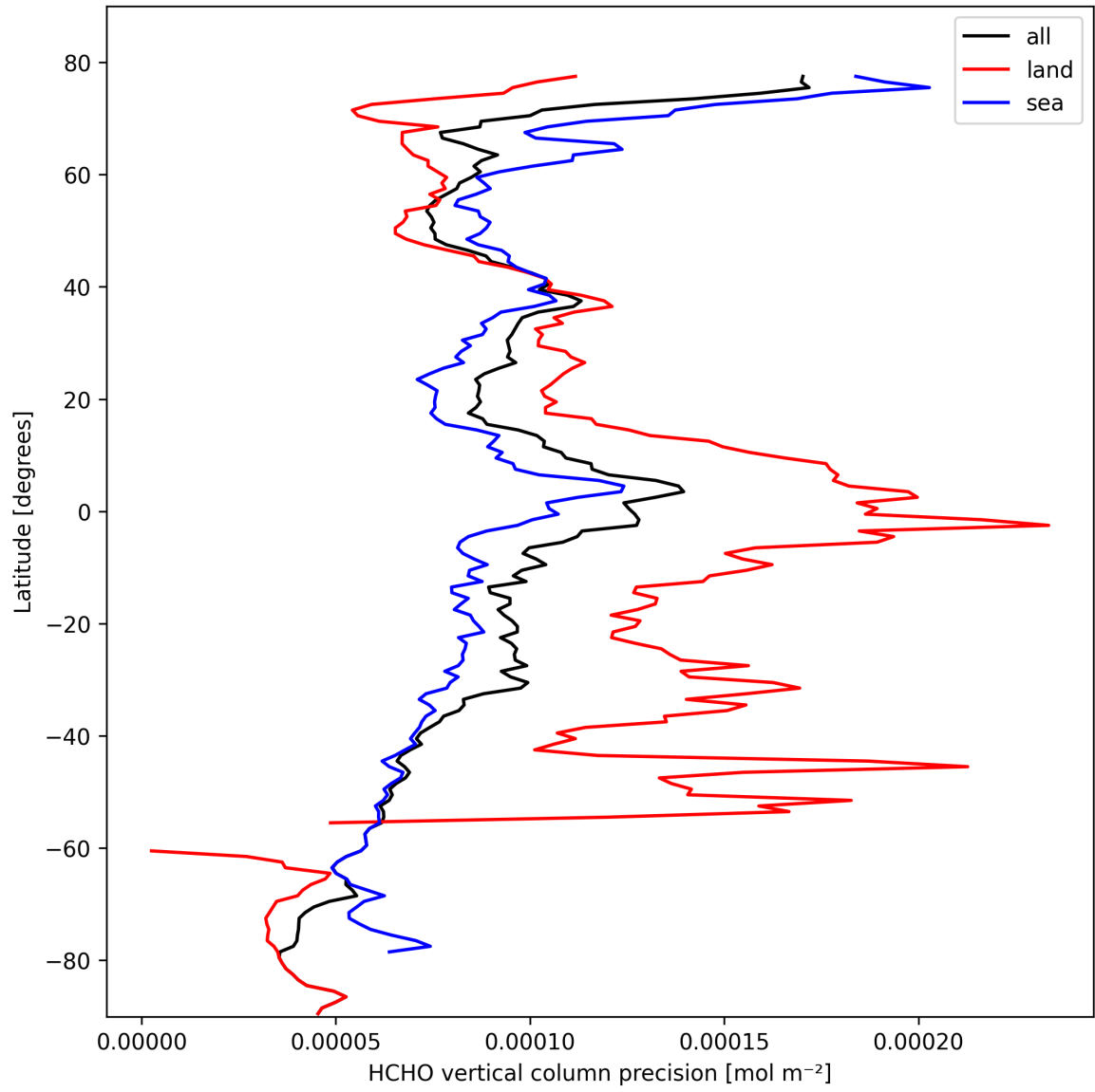
Figure 20: Zonal average of “HCHO vertical column precision” for 2025-03-01 to 2025-03-02.
