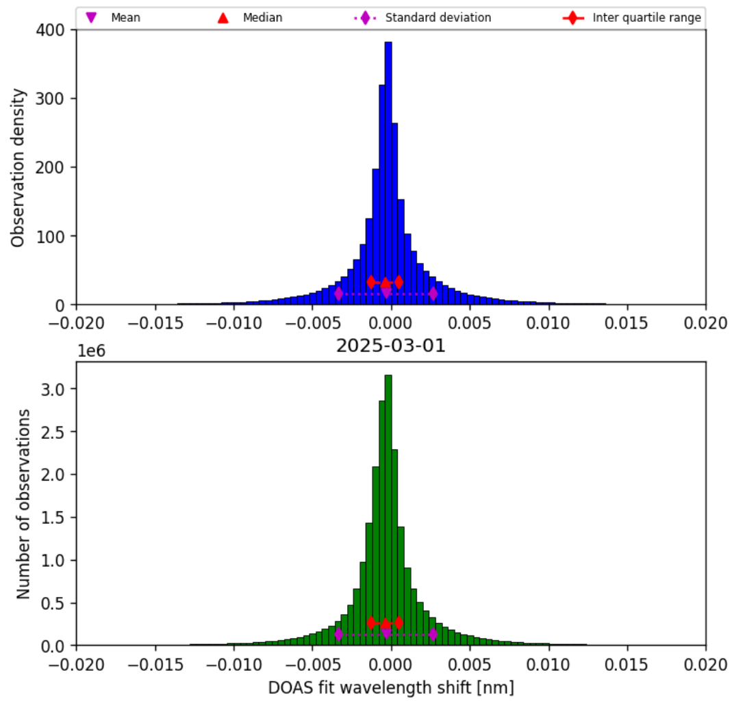
Figure 42: Histogram of “DOAS fit wavelength shift” for 2025-03-01 to 2025-03-02
