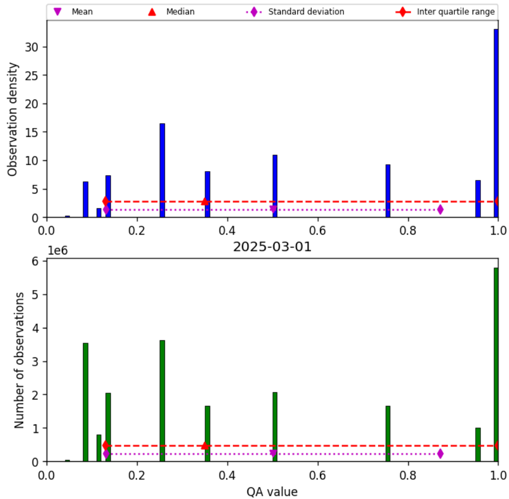
Figure 32: Histogram of “QA value” for 2025-03-01 to 2025-03-02
