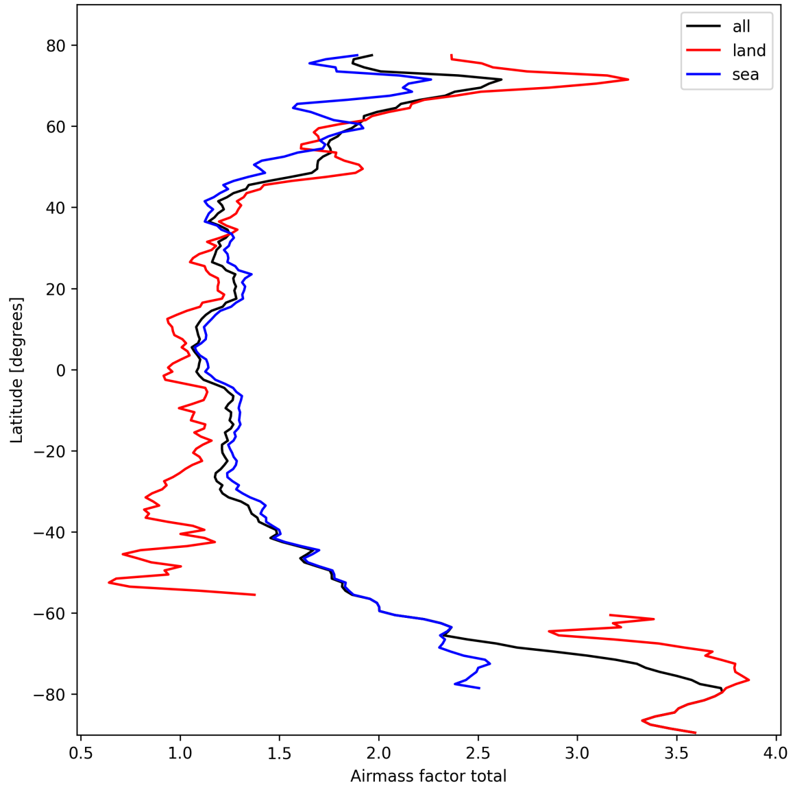
Figure 24: Zonal average of “Airmass factor total” for 2025-03-01 to 2025-03-02.
