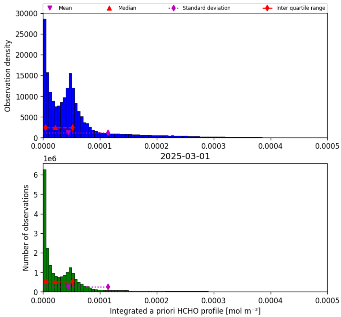
Figure 41: Histogram of “Integrated a priori HCHO profile” for 2025-03-01 to 2025-03-02
