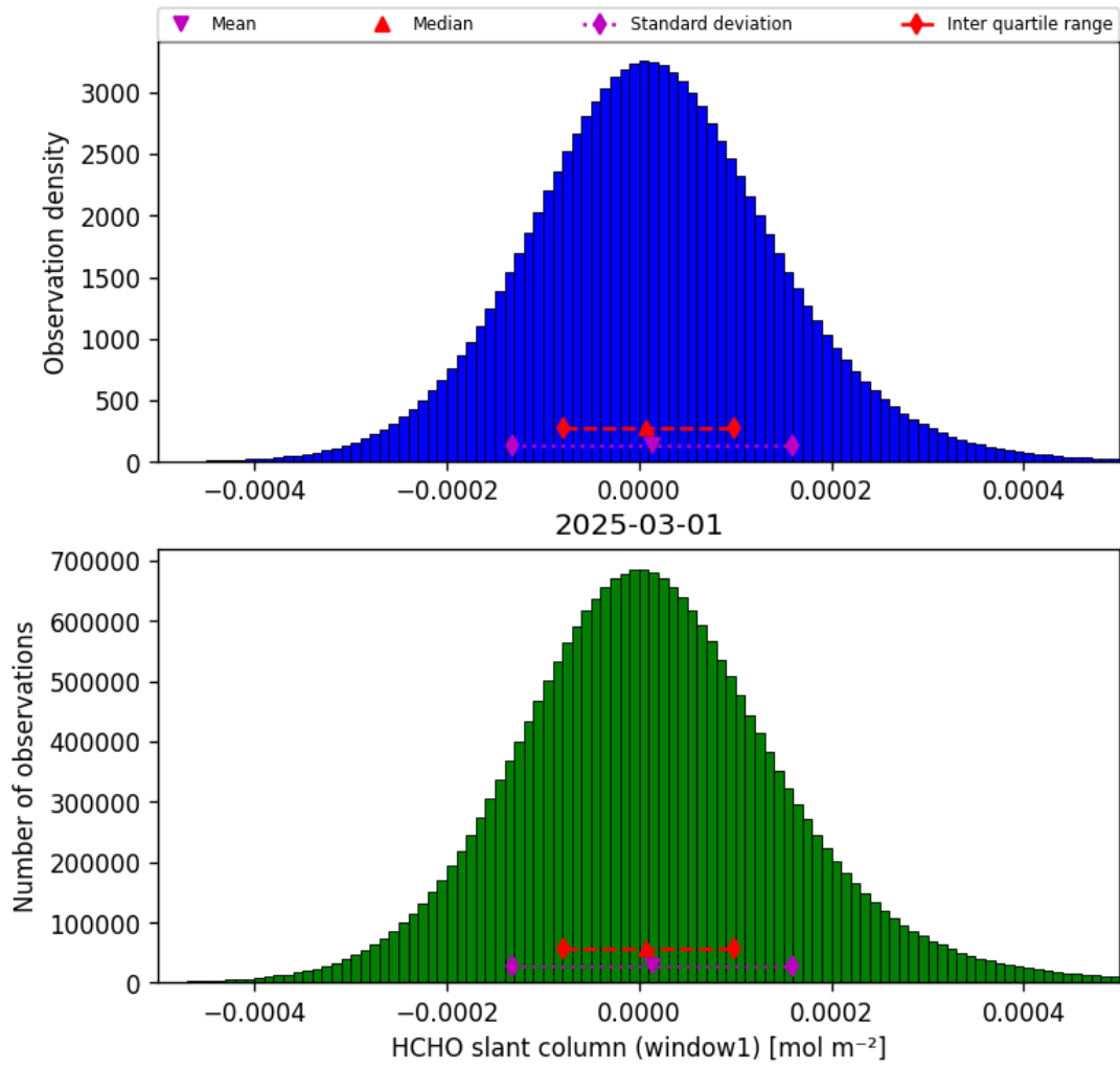
Figure 36: Histogram of “HCHO slant column (window1)” for 2025-03-01 to 2025-03-02
