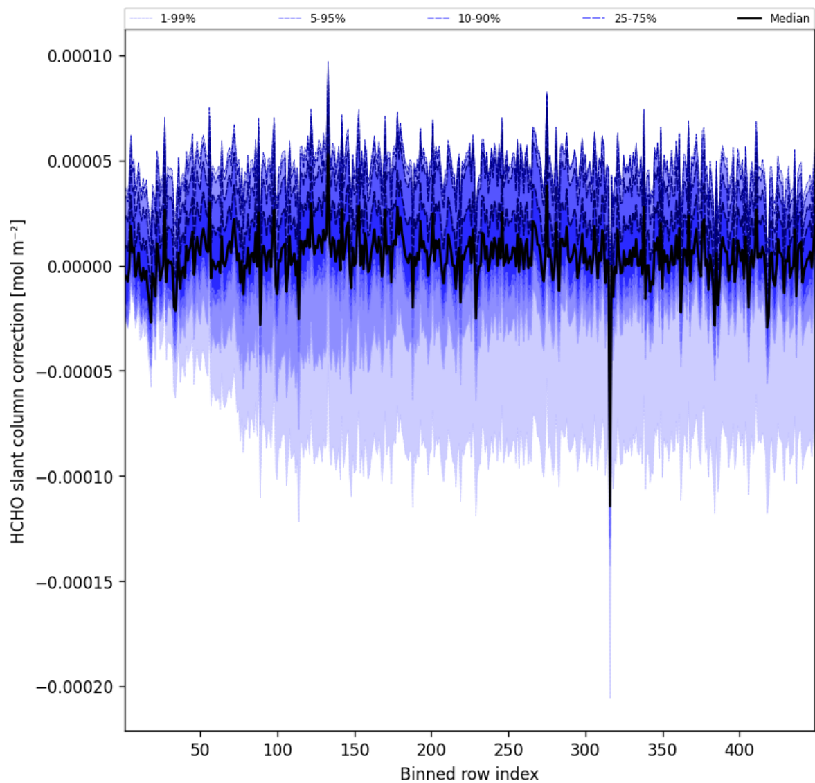
Figure 59: Along track statistics of “HCHO slant column correction” for 2025-03-01 to 2025-03-02
