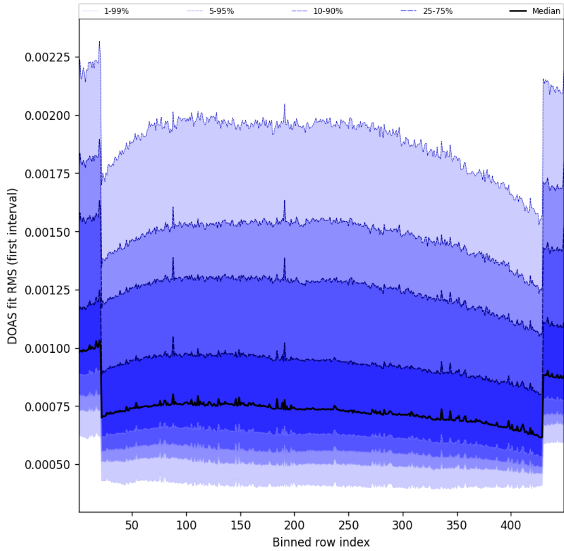
Figure 58: Along track statistics of “DOAS fit RMS (first interval)” for 2025-03-01 to 2025-03-02
