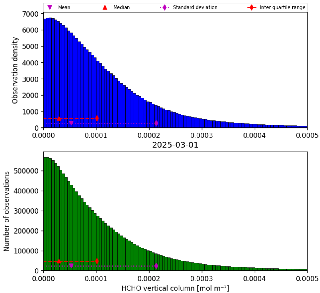
Figure 33: Histogram of “HCHO vertical column” for 2025-03-01 to 2025-03-02
