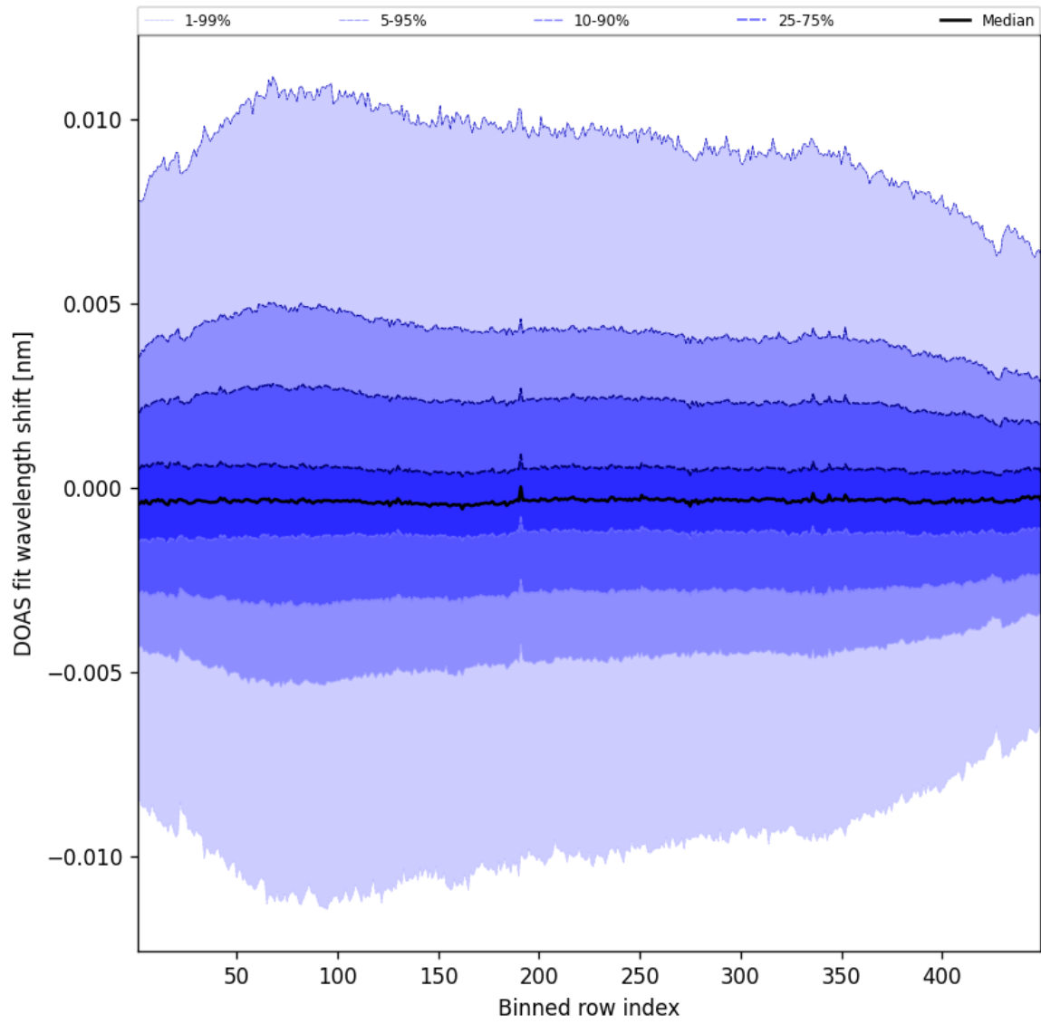
Figure 56: Along track statistics of “DOAS fit wavelength shift” for 2025-03-01 to 2025-03-02
