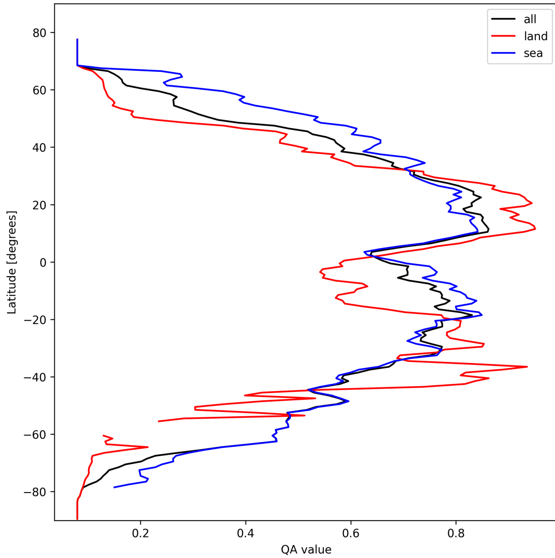
Figure 18: Zonal average of “QA value” for 2025-03-01 to 2025-03-02.
