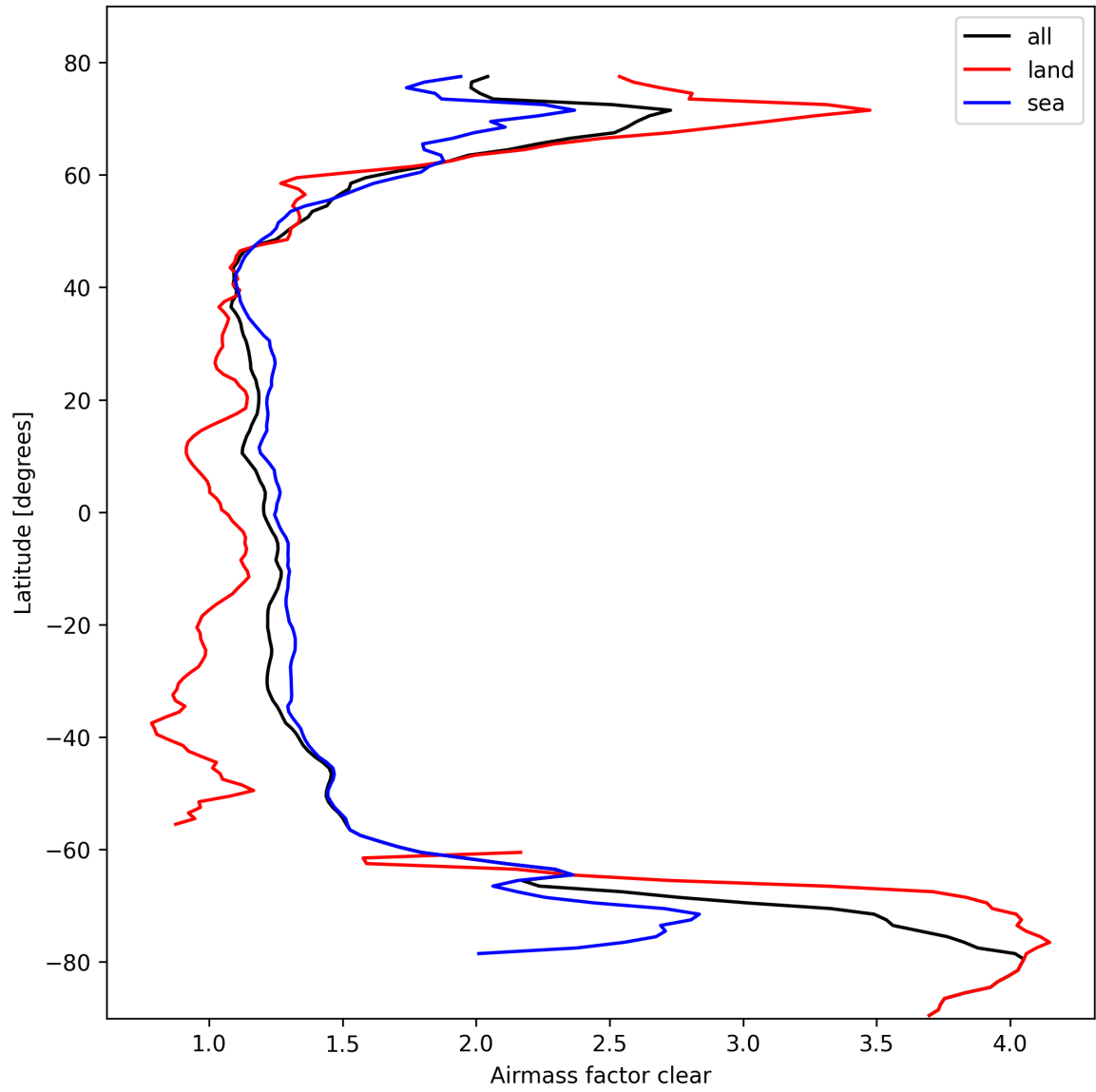
Figure 26: Zonal average of “Airmass factor clear” for 2025-03-01 to 2025-03-02.
