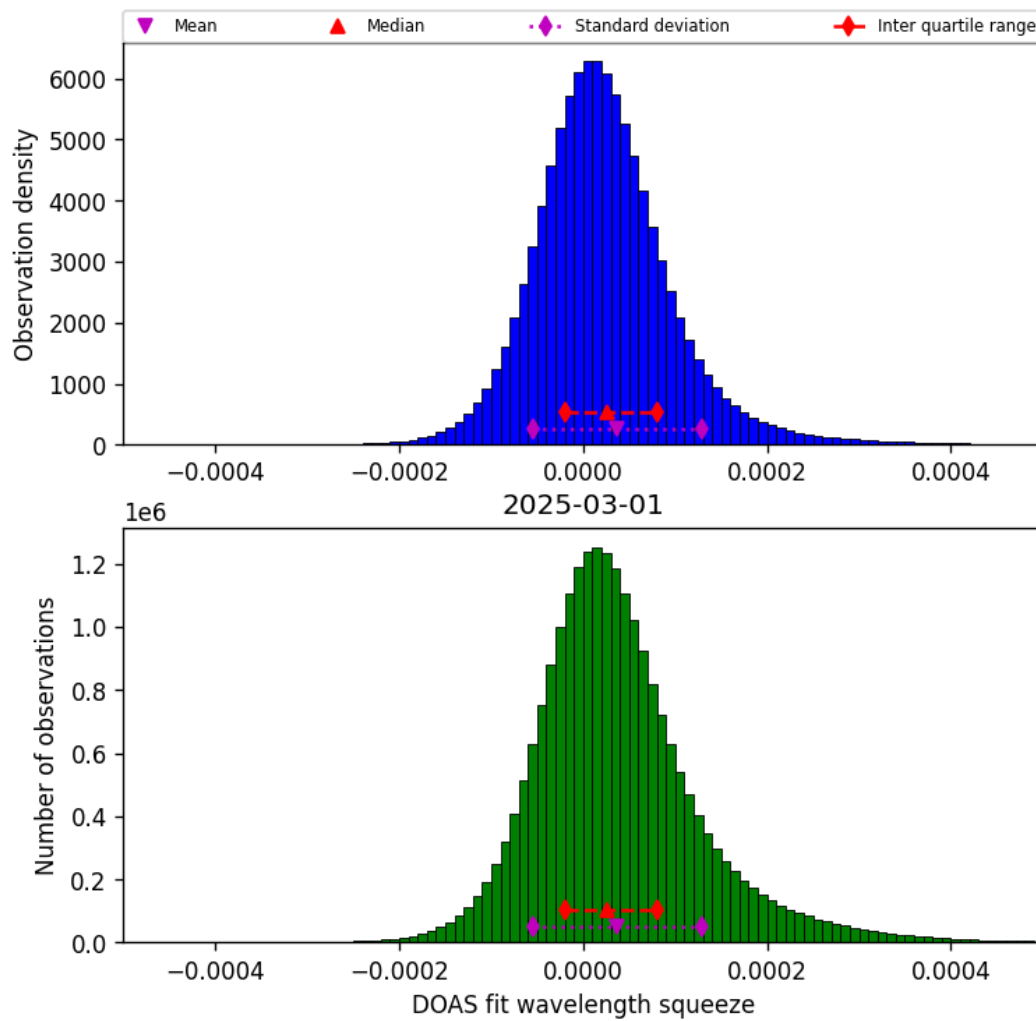
Figure 43: Histogram of “DOAS fit wavelength squeeze” for 2025-03-01 to 2025-03-02
