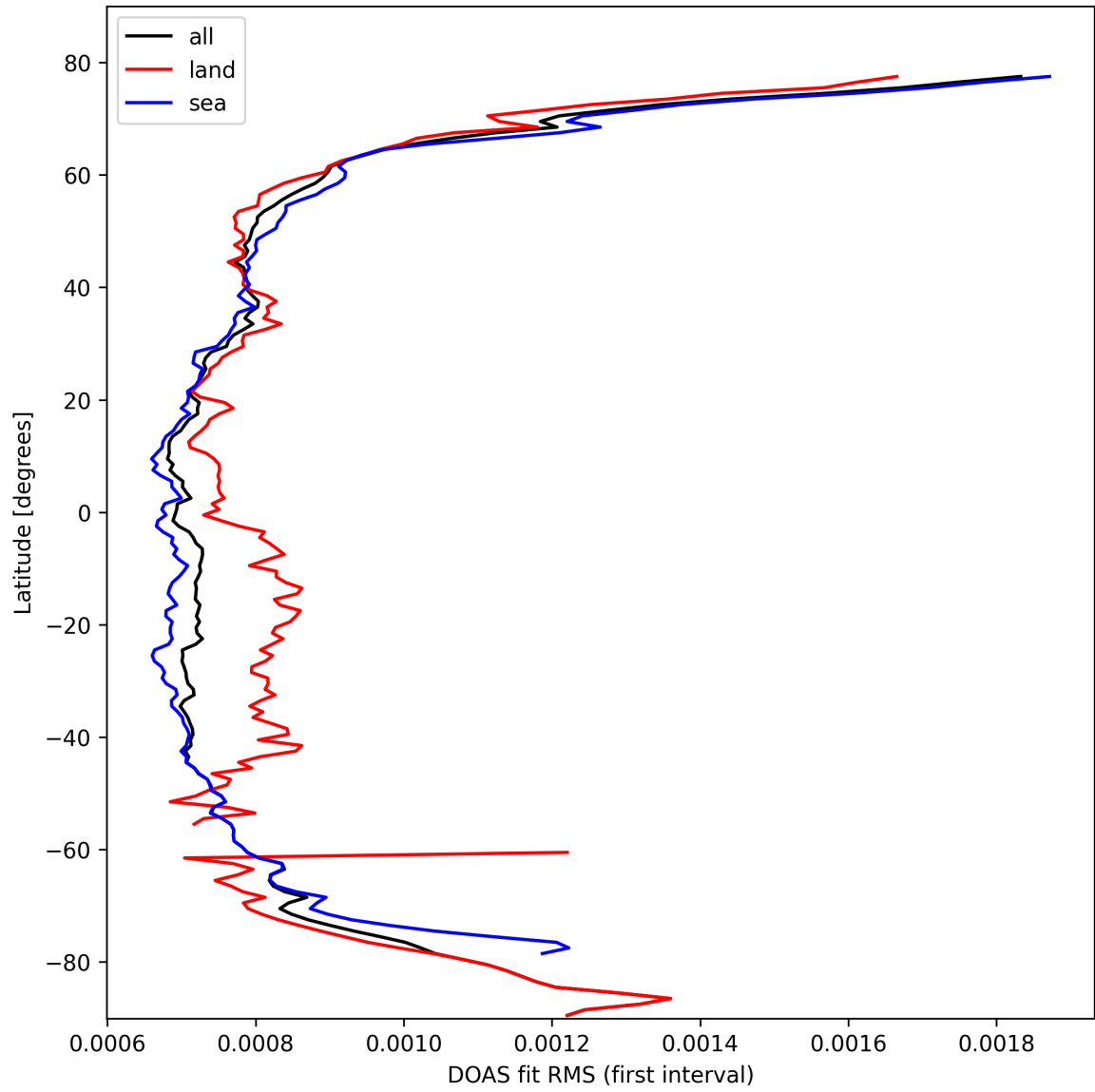
Figure 30: Zonal average of “DOAS fit RMS (first interval)” for 2025-03-01 to 2025-03-02.
