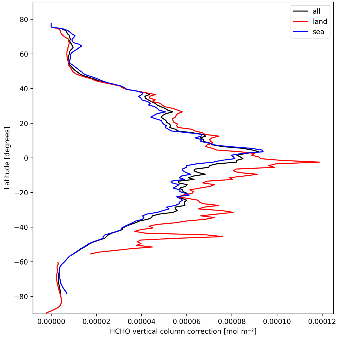
Figure 21: Zonal average of “HCHO vertical column correction” for 2025-03-01 to 2025-03-02.
