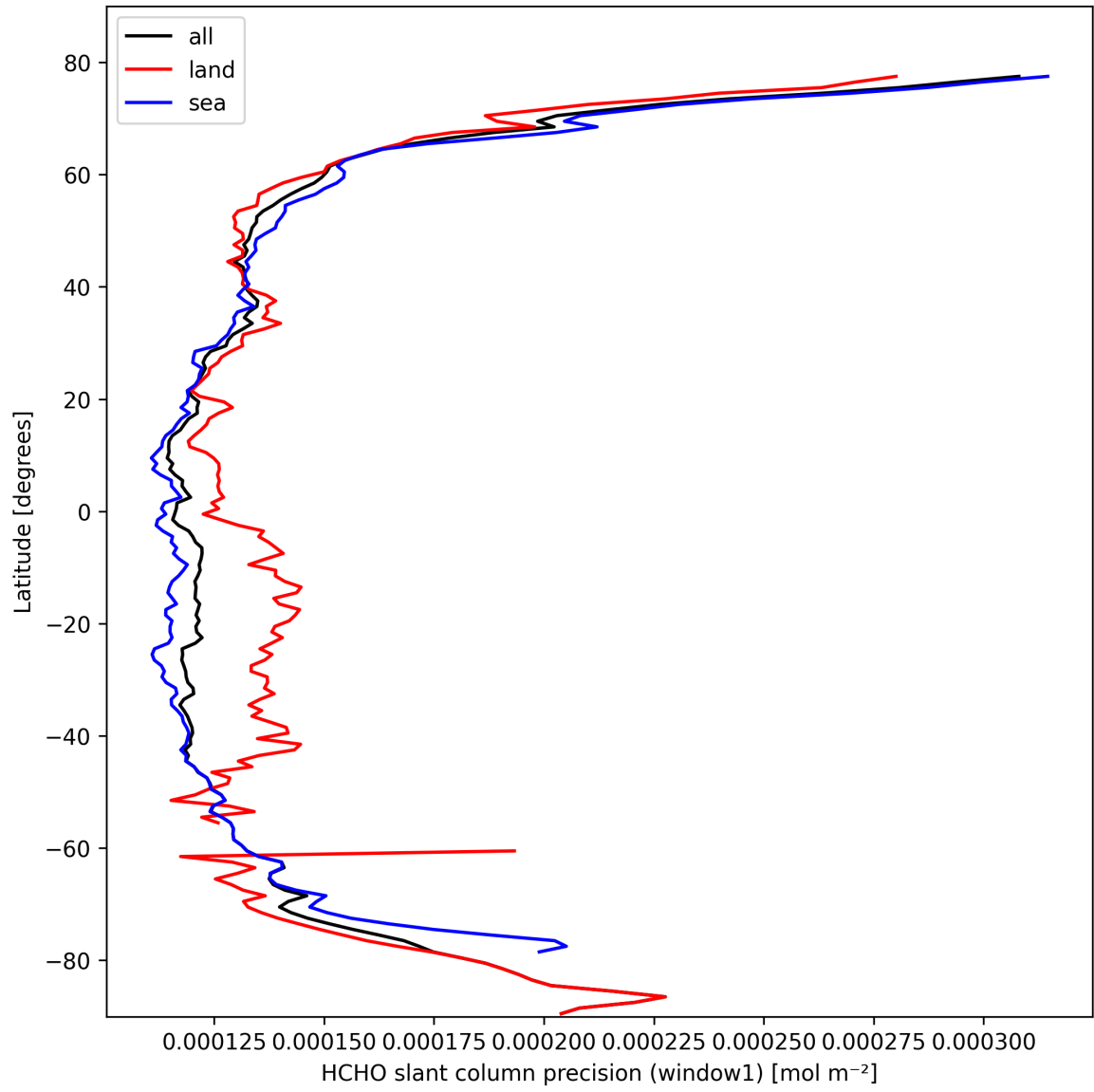
Figure 23: Zonal average of “HCHO slant column precision (window1)” for 2025-03-01 to 2025-03-02.
