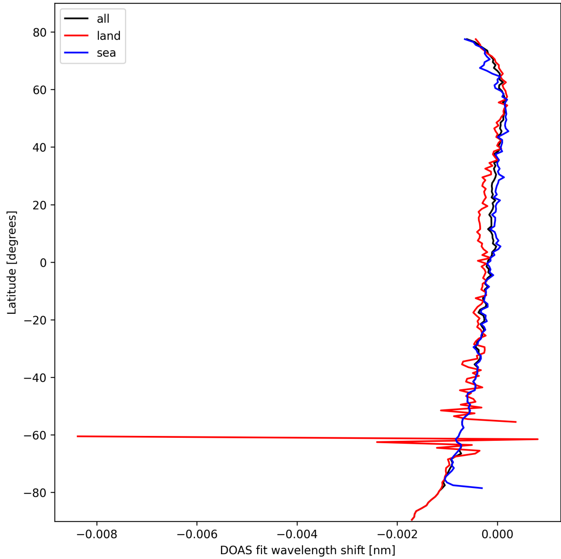
Figure 28: Zonal average of "DOAS fit wavelength shift" for 2025-03-01 to 2025-03-02.
