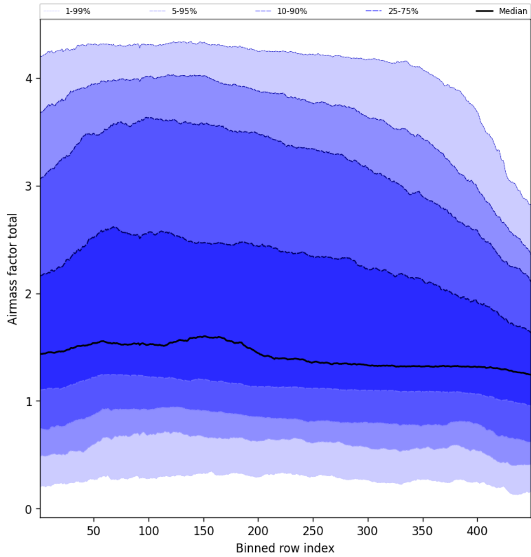
Figure 52: Along track statistics of “Airmass factor total” for 2025-03-01 to 2025-03-02
