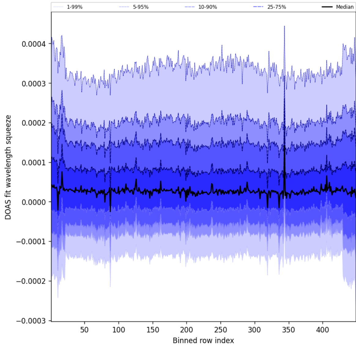
Figure 57: Along track statistics of “DOAS fit wavelength squeeze” for 2025-03-01 to 2025-03-02
