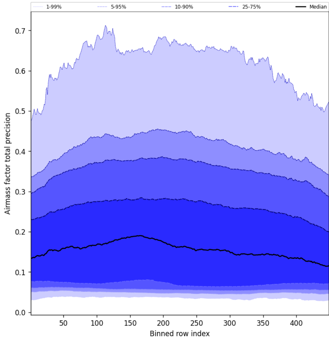
Figure 53: Along track statistics of “Airmass factor total precision” for 2025-03-01 to 2025-03-02
