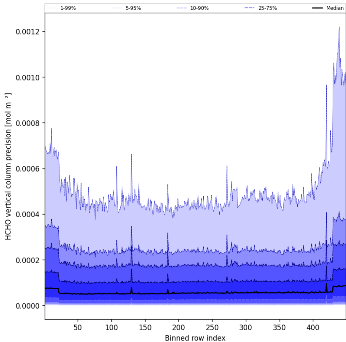
Figure 48: Along track statistics of “HCHO vertical column precision” for 2025-03-01 to 2025-03-02
