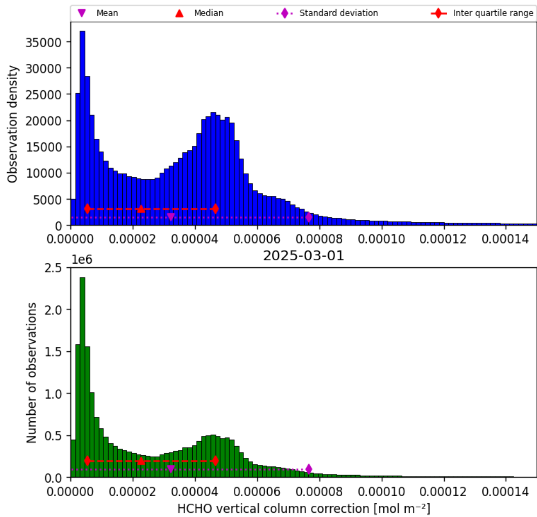
Figure 35: Histogram of “HCHO vertical column correction” for 2025-03-01 to 2025-03-02
