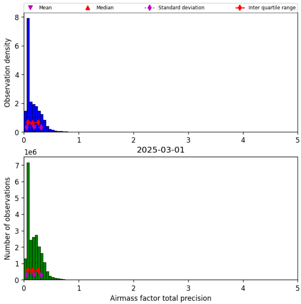
Figure 39: Histogram of “Airmass factor total precision” for 2025-03-01 to 2025-03-02
