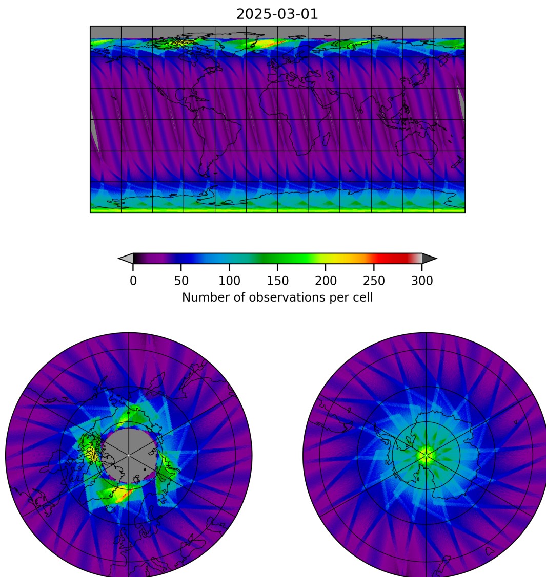
Figure 17: Map of the number of observations for 2025-03-01 to 2025-03-02
