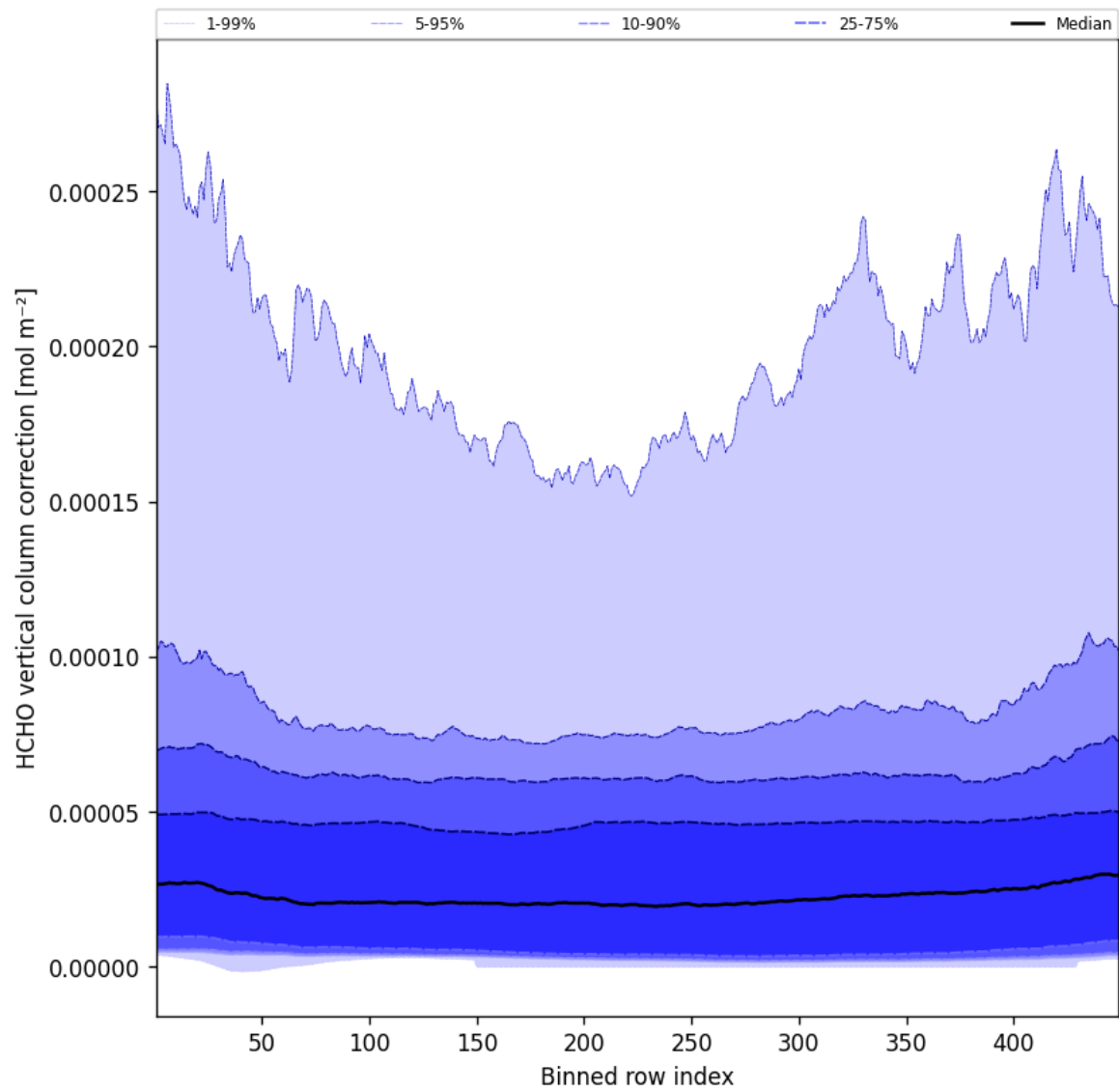
Figure 49: Along track statistics of “HCHO vertical column correction” for 2025-03-01 to 2025-03-02
