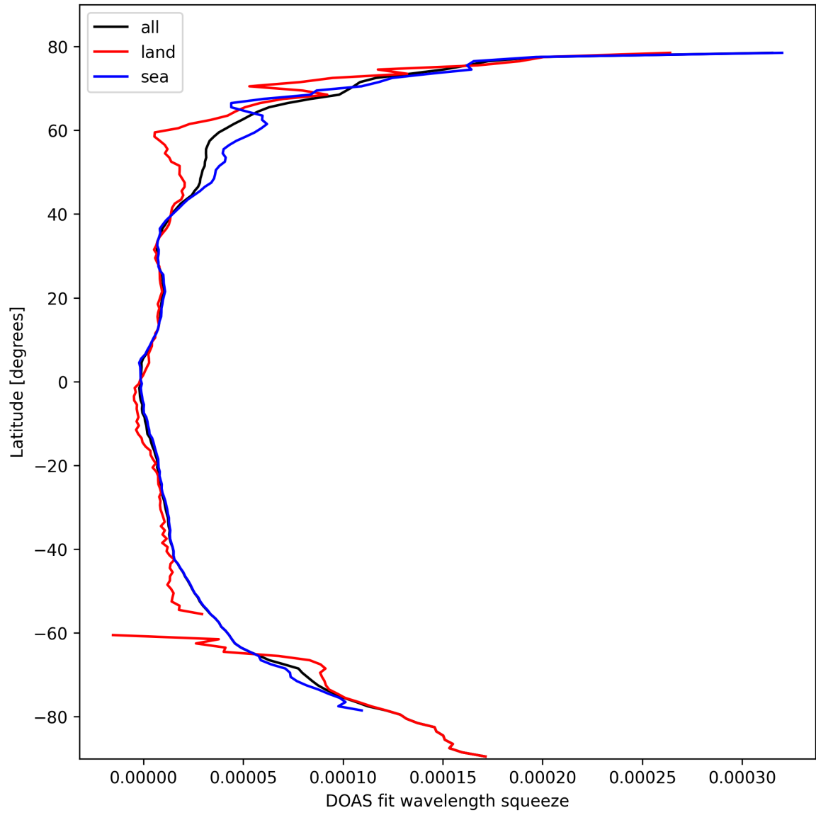
Figure 29: Zonal average of “DOAS fit wavelength squeeze” for 2025-03-02 to 2025-03-03.
