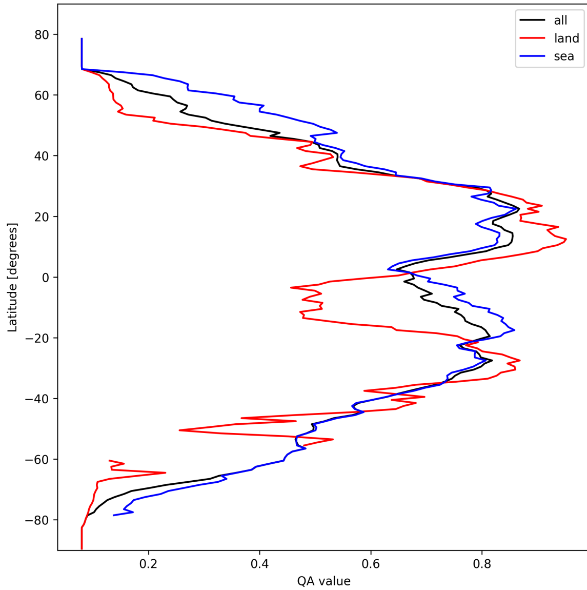
Figure 18: Zonal average of “QA value” for 2025-03-02 to 2025-03-03.
