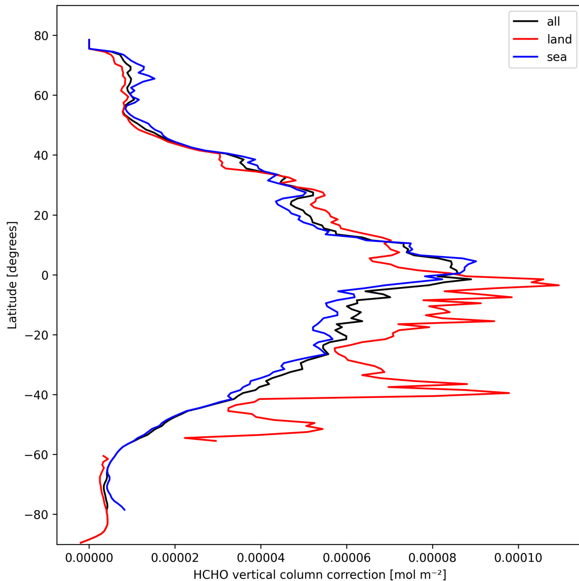
Figure 21: Zonal average of “HCHO vertical column correction” for 2025-03-02 to 2025-03-03.
