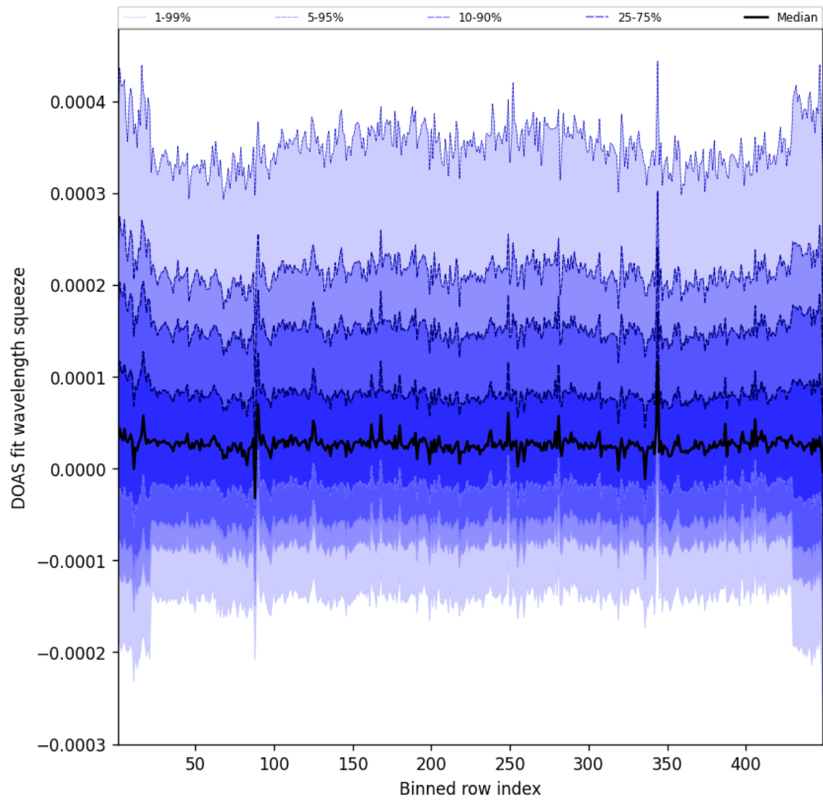
Figure 57: Along track statistics of “DOAS fit wavelength squeeze” for 2025-03-02 to 2025-03-03
