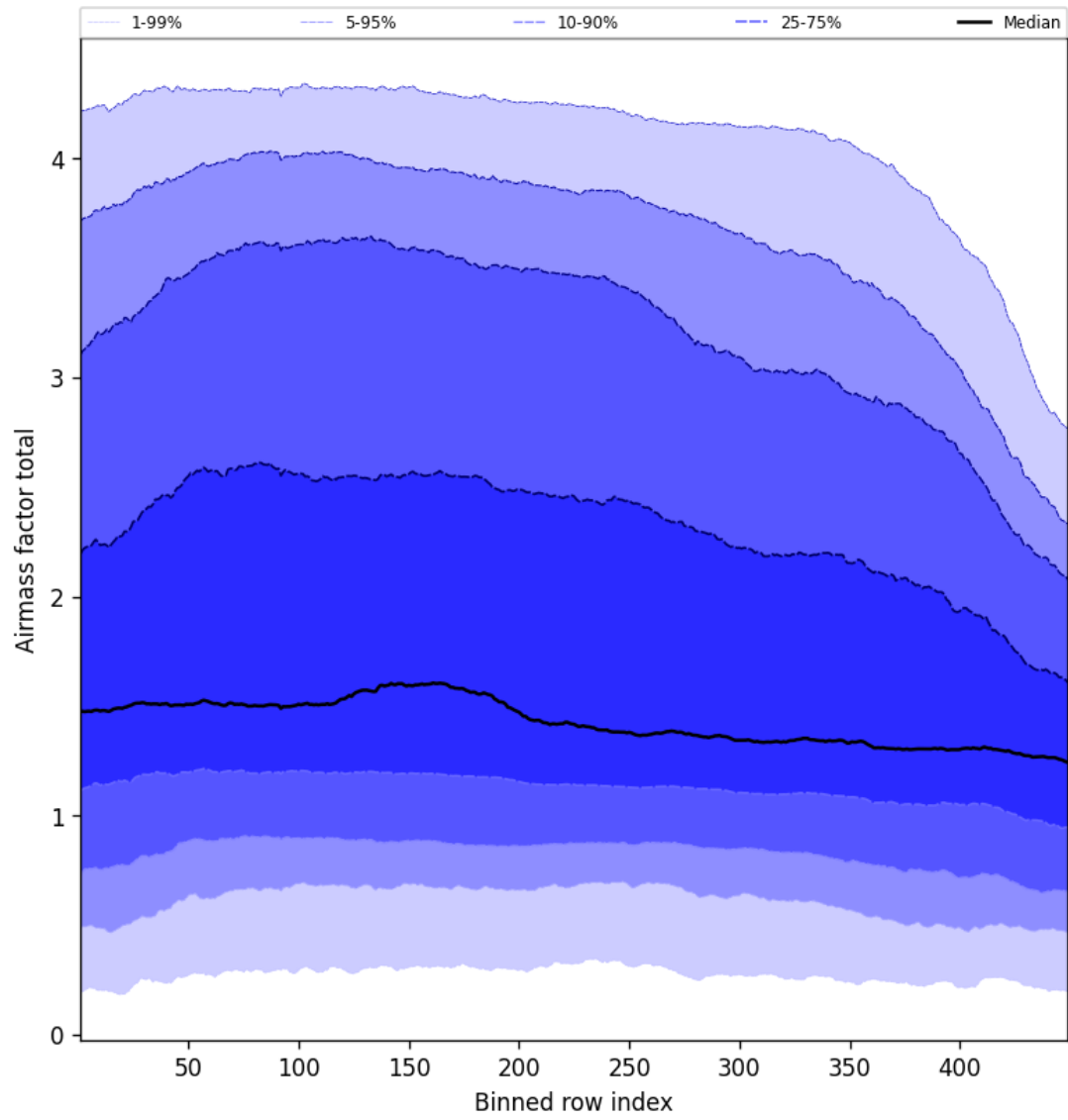
Figure 52: Along track statistics of “Airmass factor total” for 2025-03-02 to 2025-03-03
