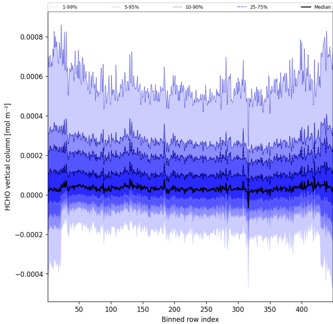
Figure 47: Along track statistics of “HCHO vertical column” for 2025-03-02 to 2025-03-03
