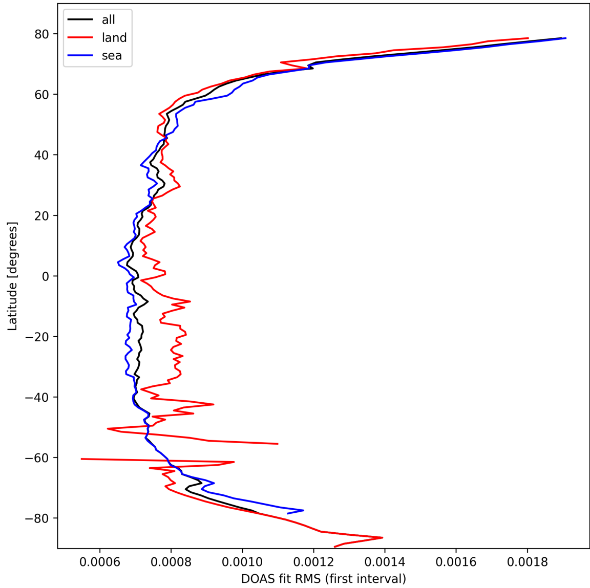
Figure 30: Zonal average of "DOAS fit RMS (first interval)" for 2025-03-02 to 2025-03-03.
