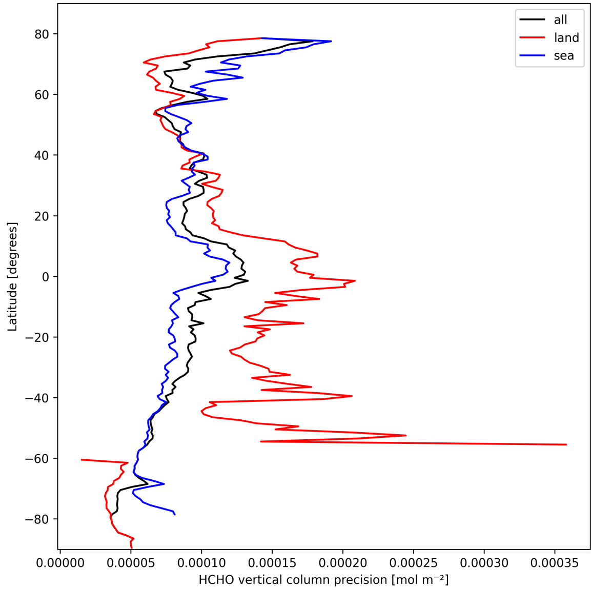
Figure 20: Zonal average of “HCHO vertical column precision” for 2025-03-02 to 2025-03-03.
