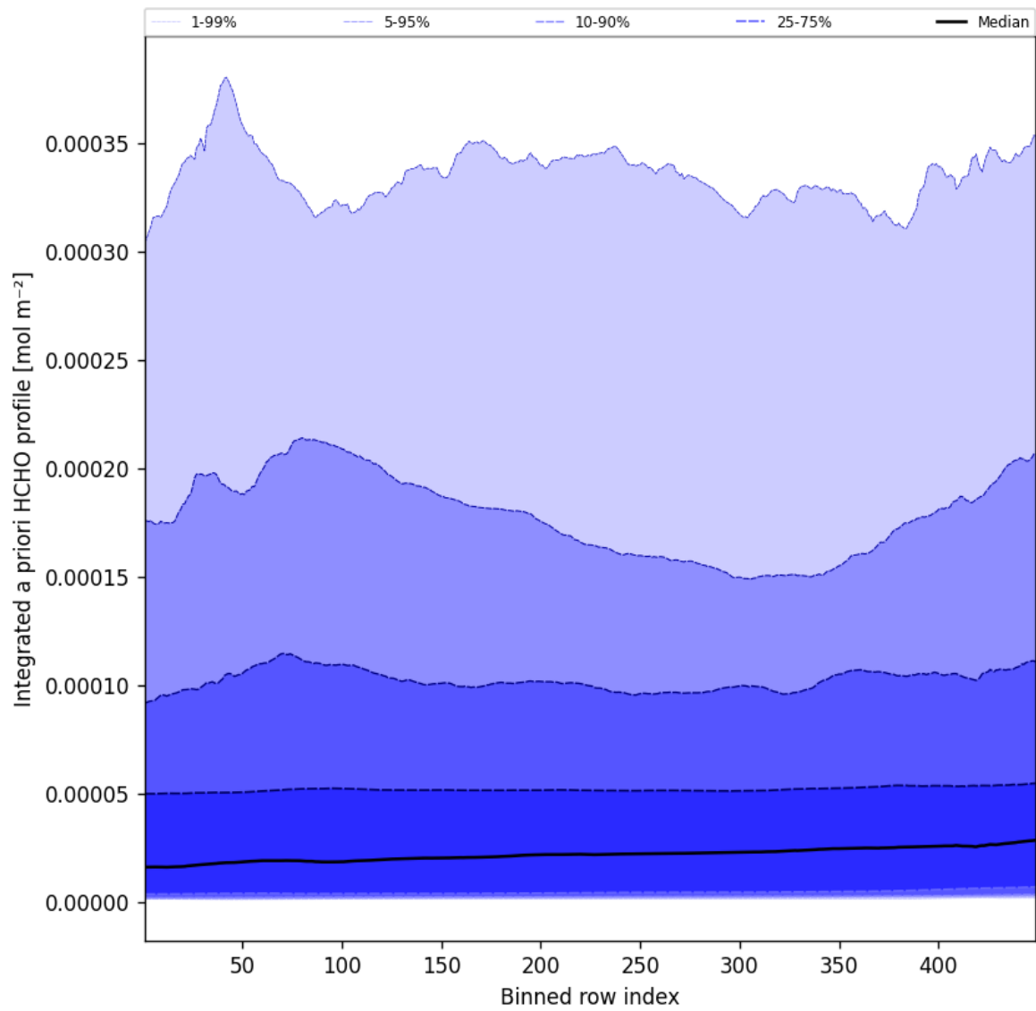
Figure 55: Along track statistics of "Integrated a priori HCHO profile" for 2025-03-02 to 2025-03-03
