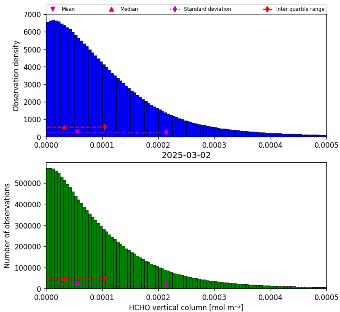
Figure 33: Histogram of “HCHO vertical column” for 2025-03-02 to 2025-03-03
