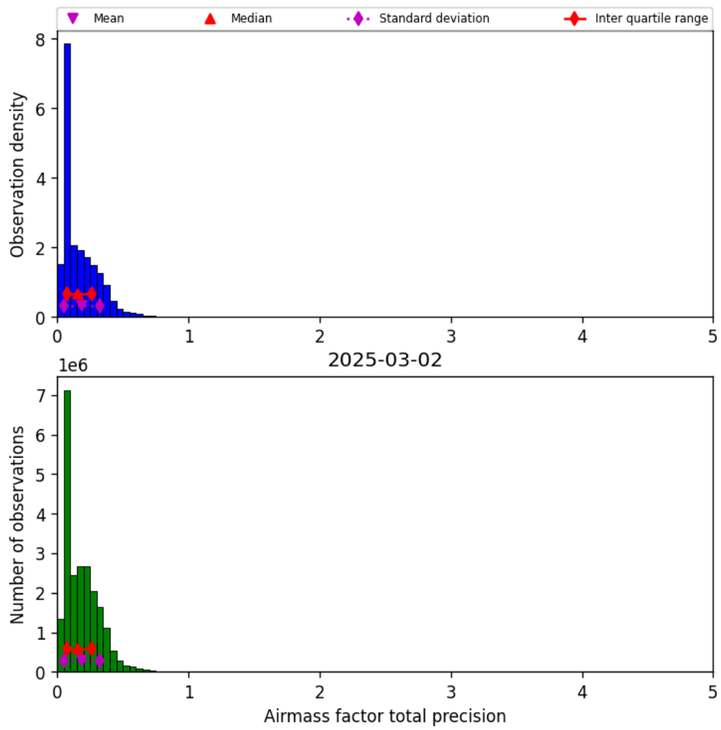
Figure 39: Histogram of “Airmass factor total precision” for 2025-03-02 to 2025-03-03
