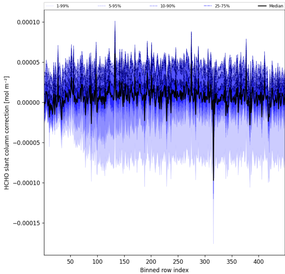
Figure 59: Along track statistics of “HCHO slant column correction” for 2025-03-02 to 2025-03-03
