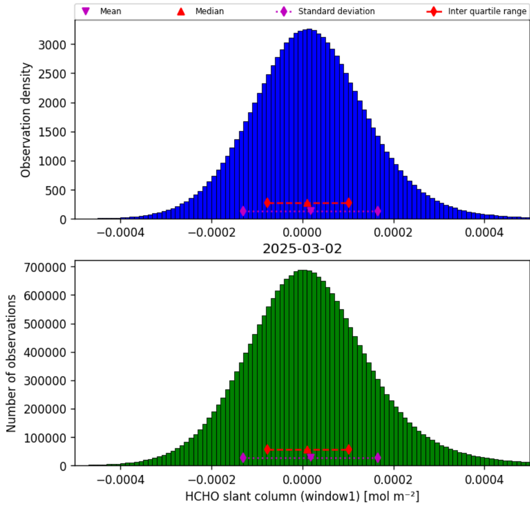
Figure 36: Histogram of “HCHO slant column (window1)” for 2025-03-02 to 2025-03-03
