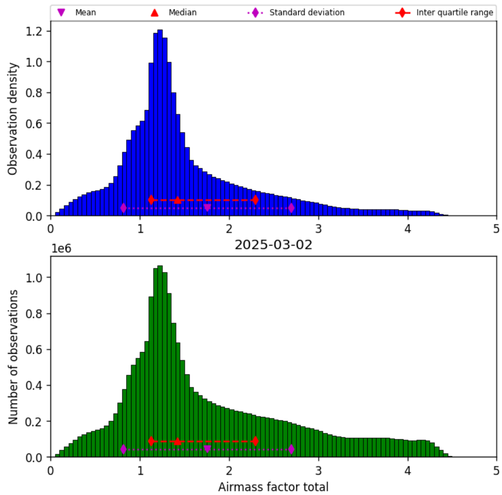
Figure 38: Histogram of “Airmass factor total” for 2025-03-02 to 2025-03-03
