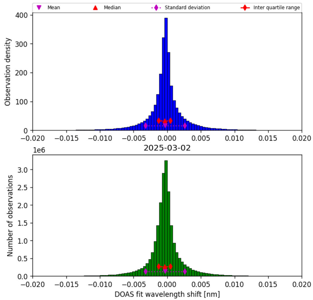
Figure 42: Histogram of “DOAS fit wavelength shift” for 2025-03-02 to 2025-03-03
