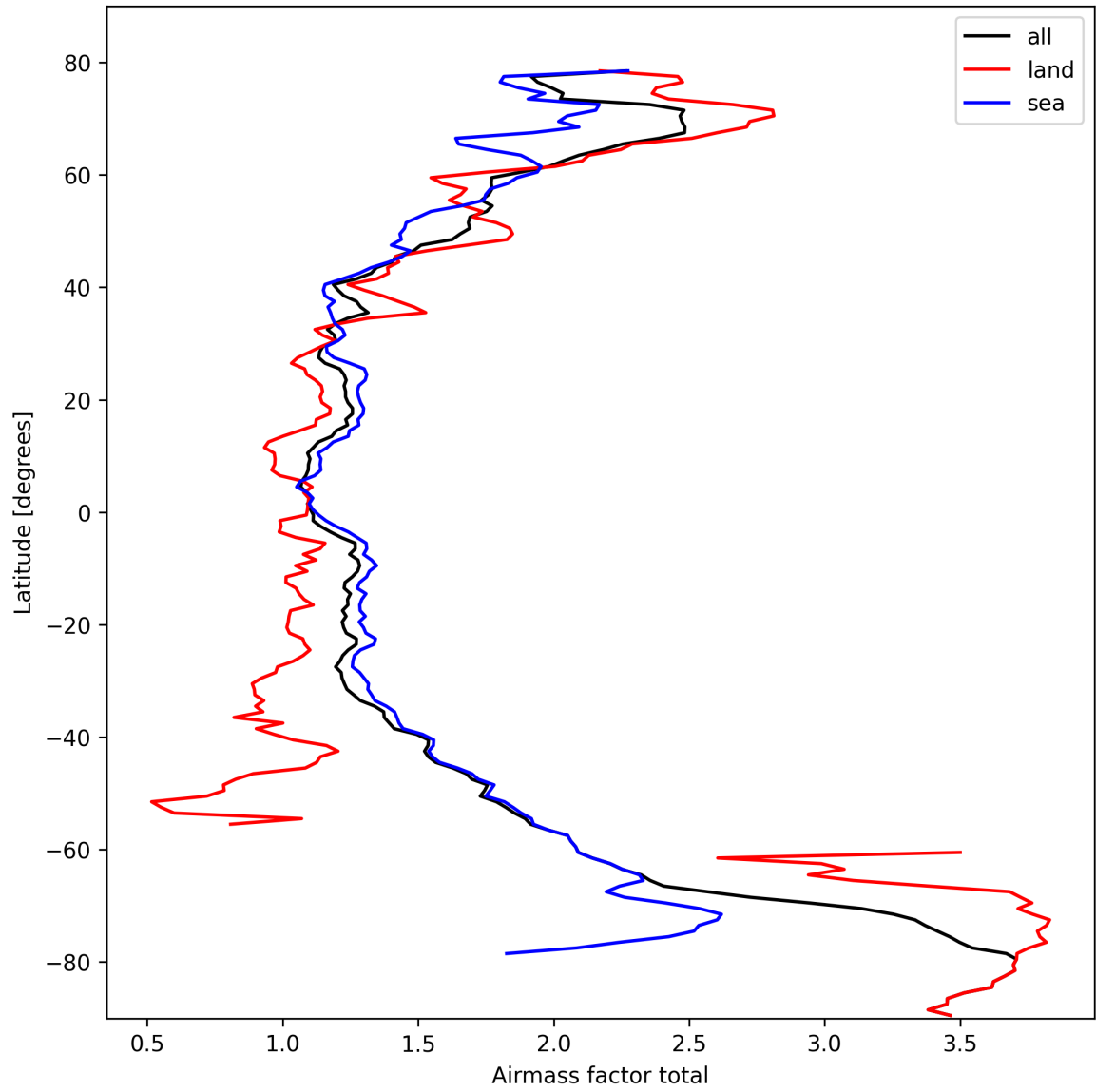
Figure 24: Zonal average of “Airmass factor total” for 2025-03-02 to 2025-03-03.
