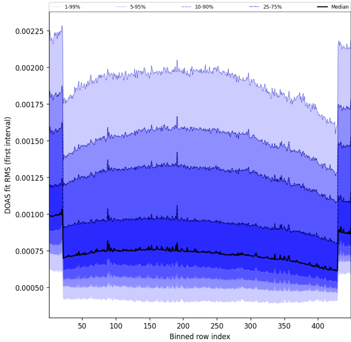
Figure 58: Along track statistics of “DOAS fit RMS (first interval)” for 2025-03-02 to 2025-03-03
