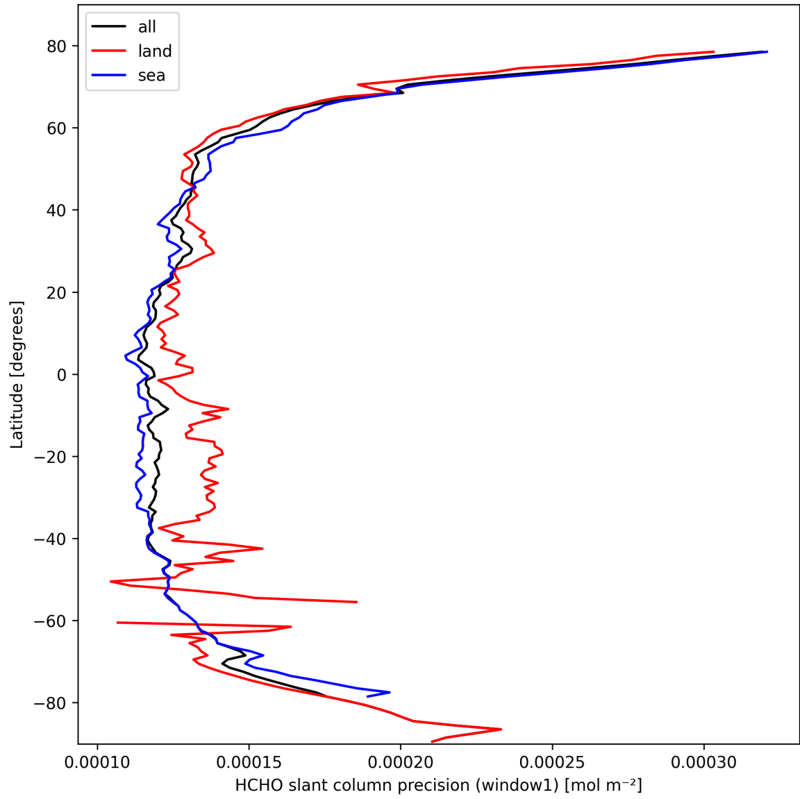
Figure 23: Zonal average of “HCHO slant column precision (window1)” for 2025-03-02 to 2025-03-03.
