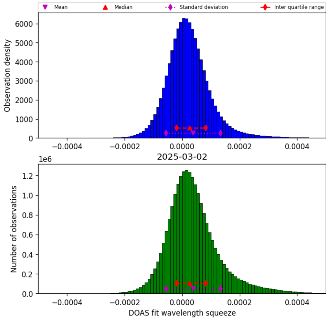
Figure 43: Histogram of “DOAS fit wavelength squeeze” for 2025-03-02 to 2025-03-03
