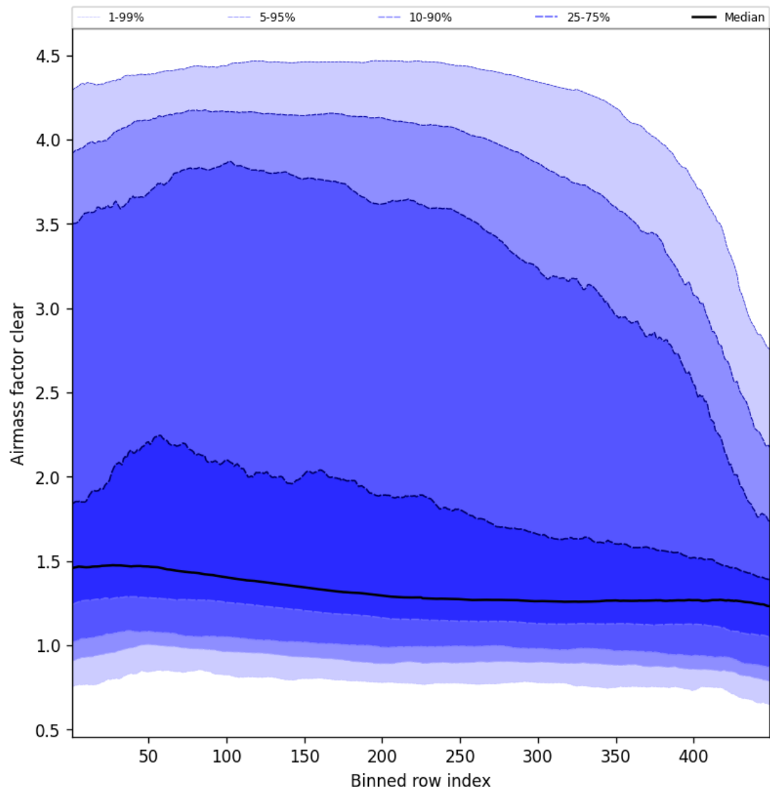
Figure 54: Along track statistics of “Airmass factor clear” for 2025-03-02 to 2025-03-03
