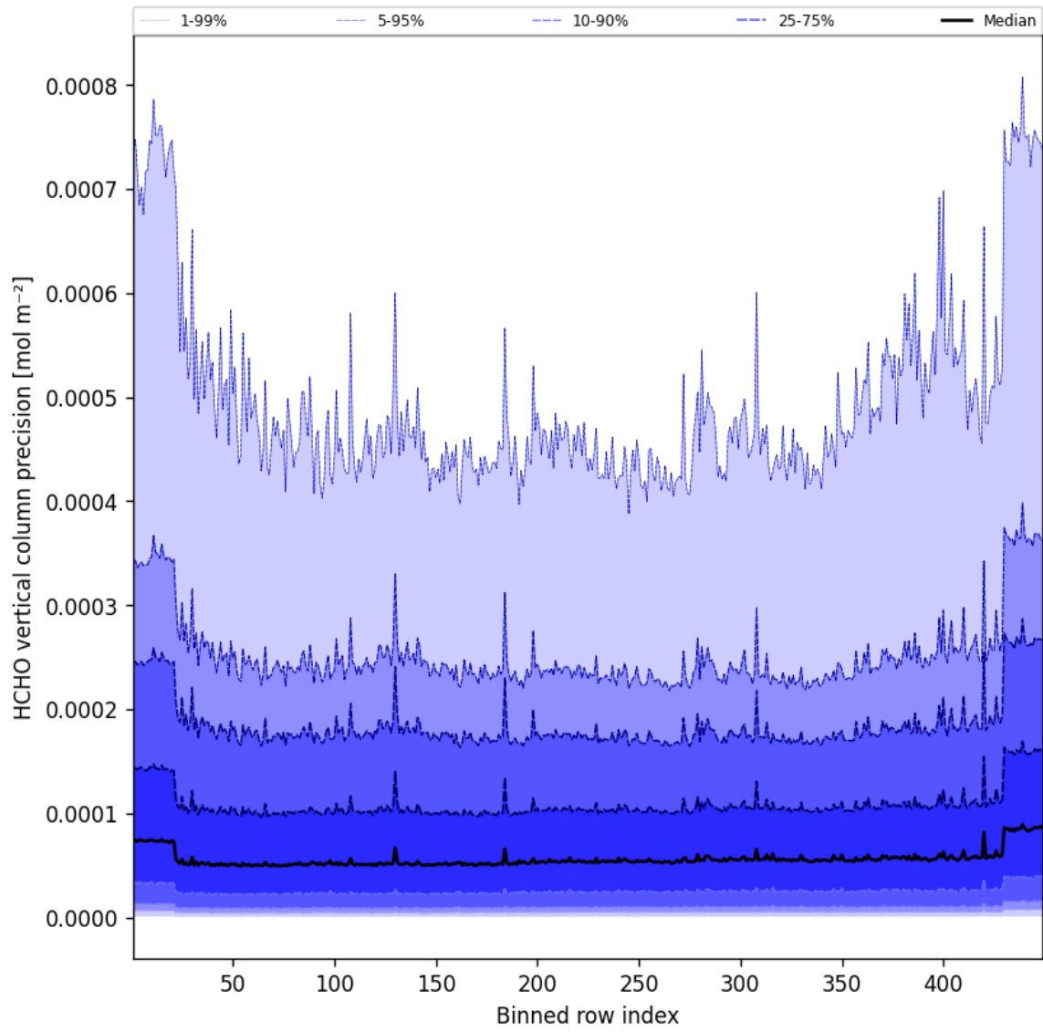
Figure 48: Along track statistics of “HCHO vertical column precision” for 2025-03-02 to 2025-03-03
