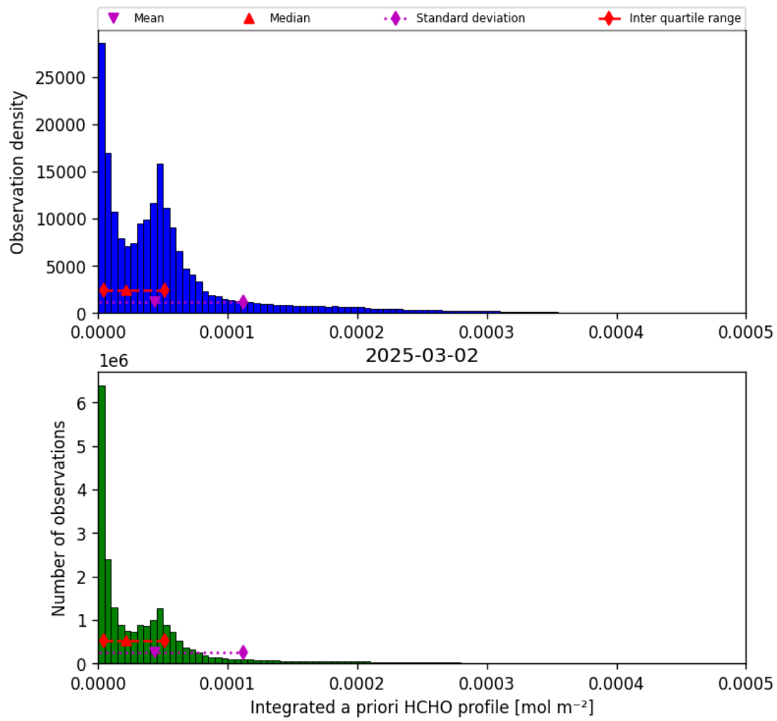
Figure 41: Histogram of “Integrated a priori HCHO profile” for 2025-03-02 to 2025-03-03
