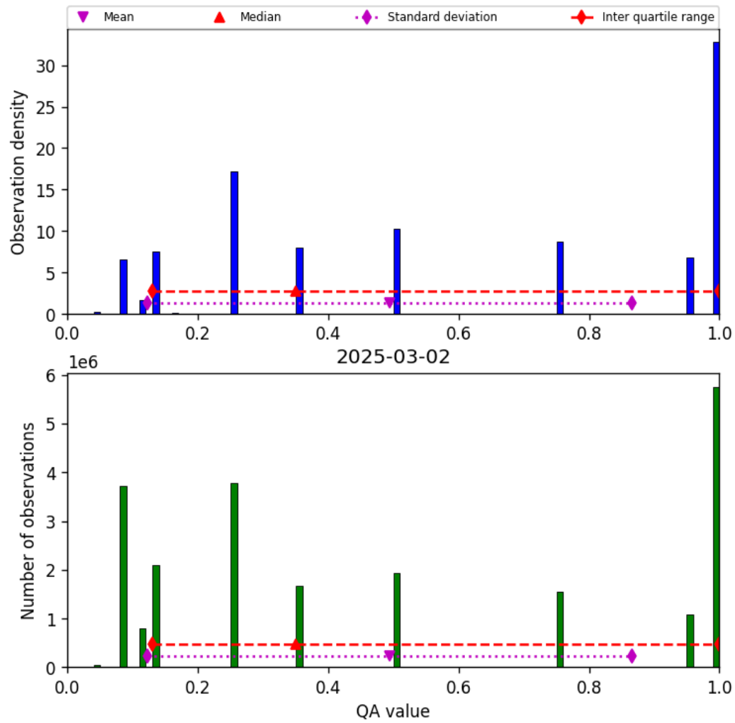
Figure 32: Histogram of “QA value” for 2025-03-02 to 2025-03-03
