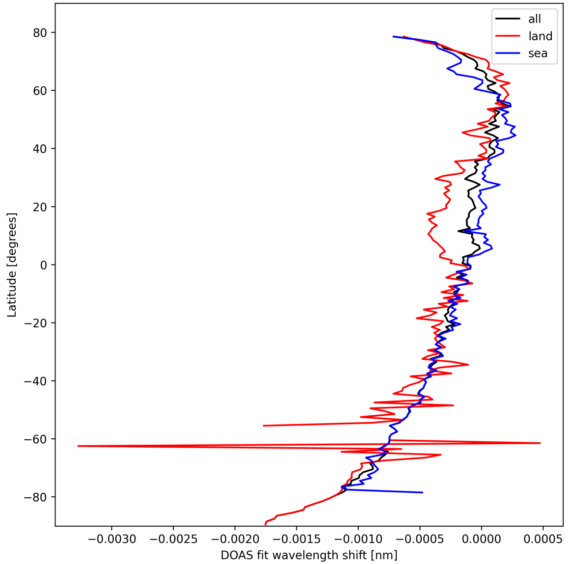
Figure 28: Zonal average of "DOAS fit wavelength shift" for 2025-03-02 to 2025-03-03.
