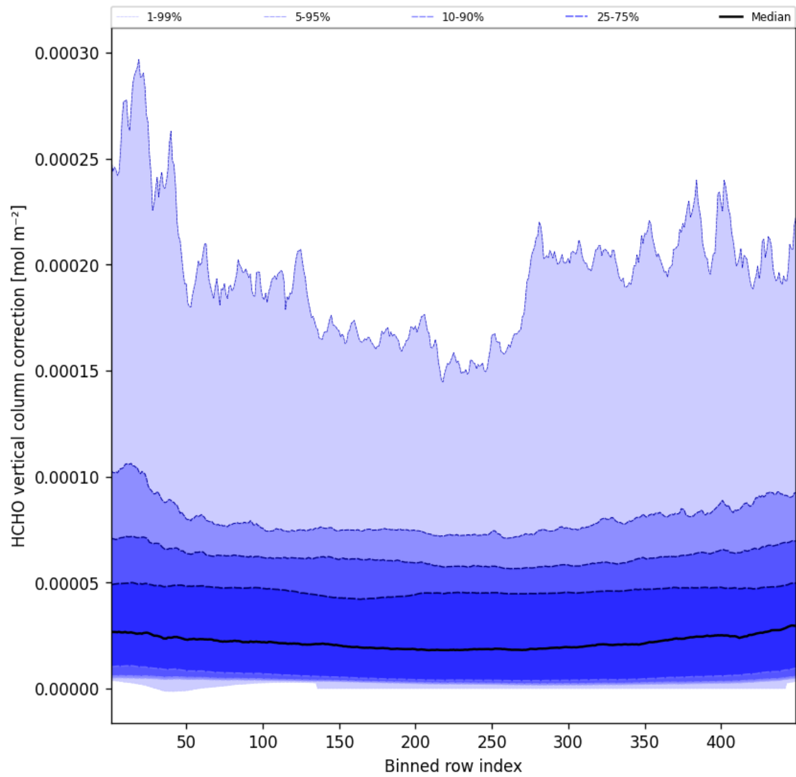
Figure 49: Along track statistics of “HCHO vertical column correction” for 2025-03-02 to 2025-03-03
