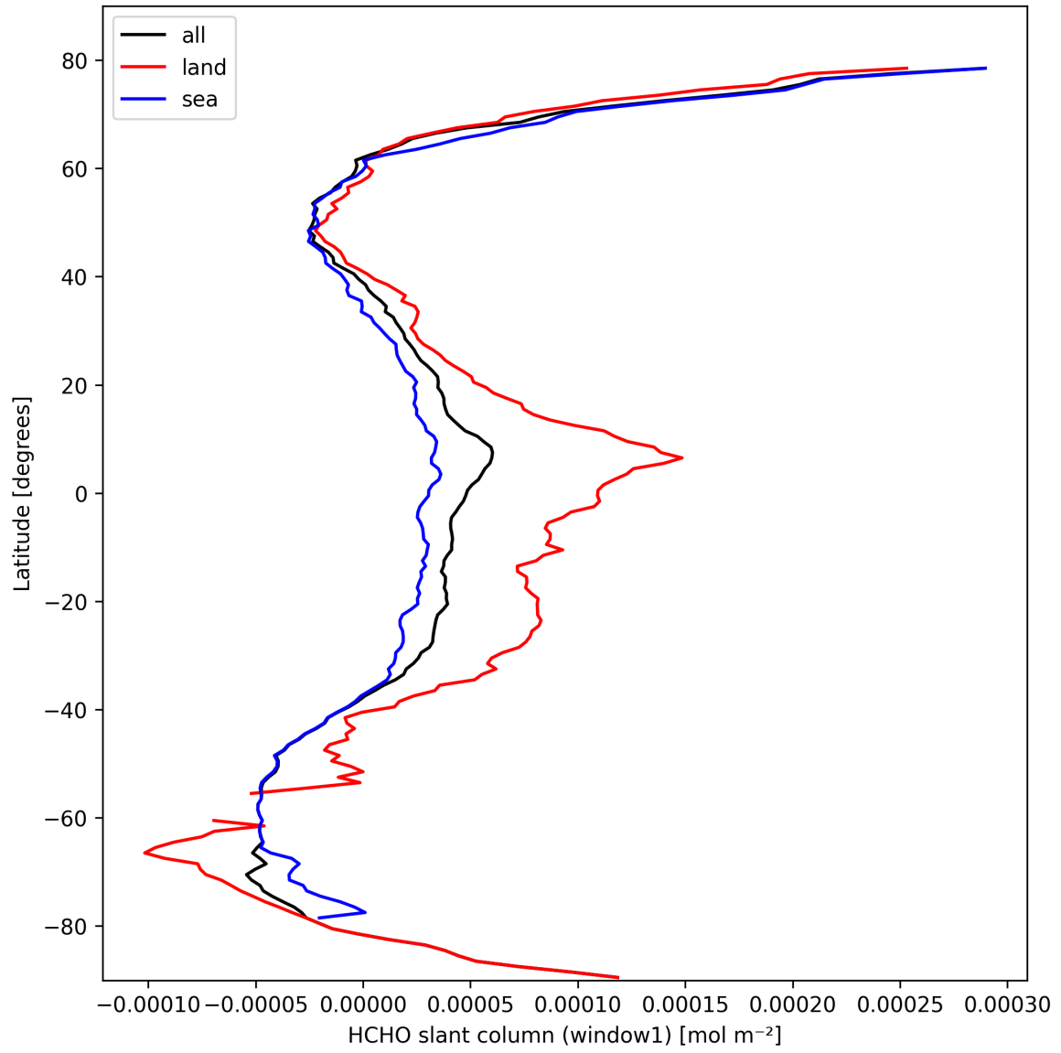
Figure 22: Zonal average of “HCHO slant column (window1)” for 2025-03-02 to 2025-03-03.
