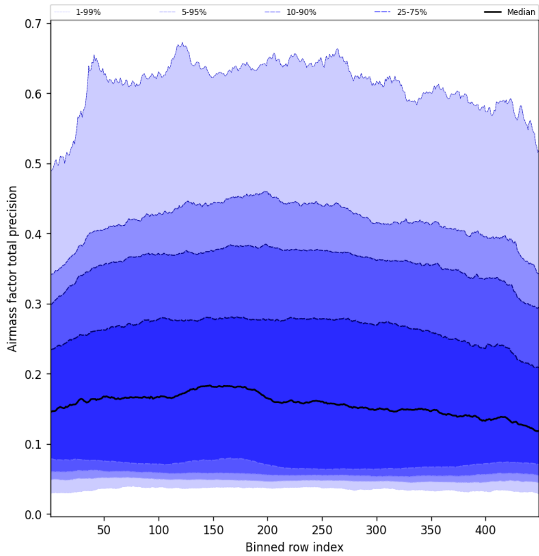
Figure 53: Along track statistics of “Airmass factor total precision” for 2025-03-02 to 2025-03-03
