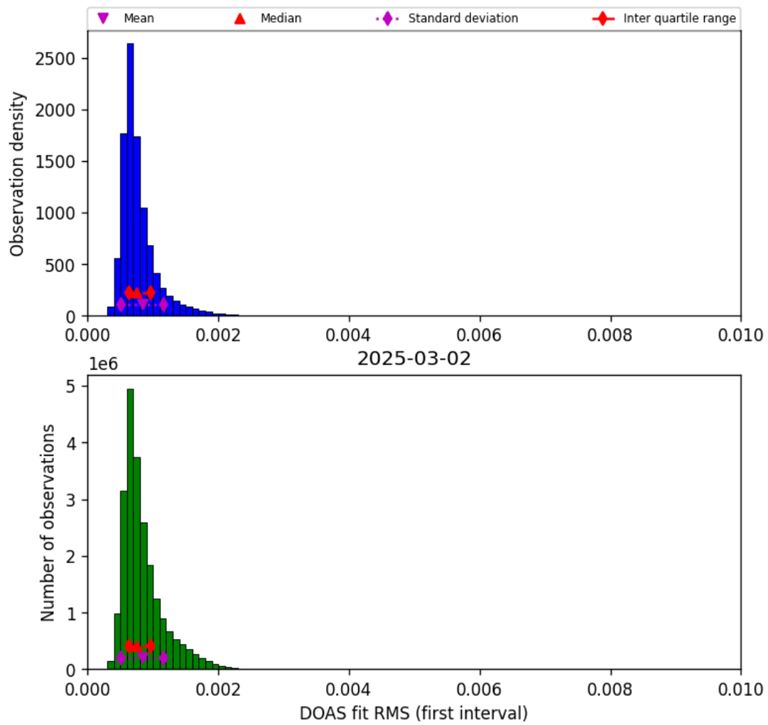
Figure 44: Histogram of “DOAS fit RMS (first interval)” for 2025-03-02 to 2025-03-03
