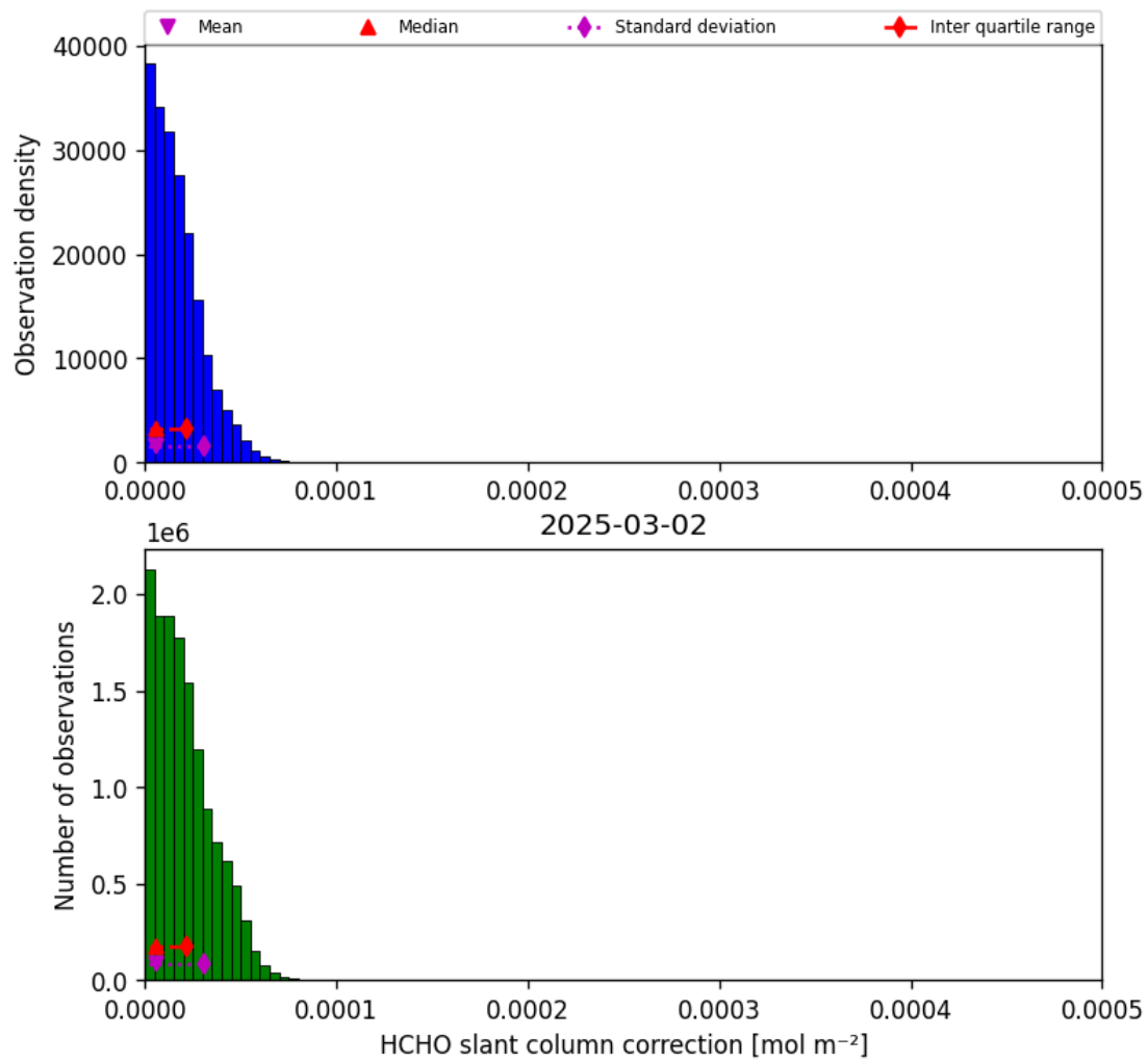
Figure 45: Histogram of “HCHO slant column correction” for 2025-03-02 to 2025-03-03
