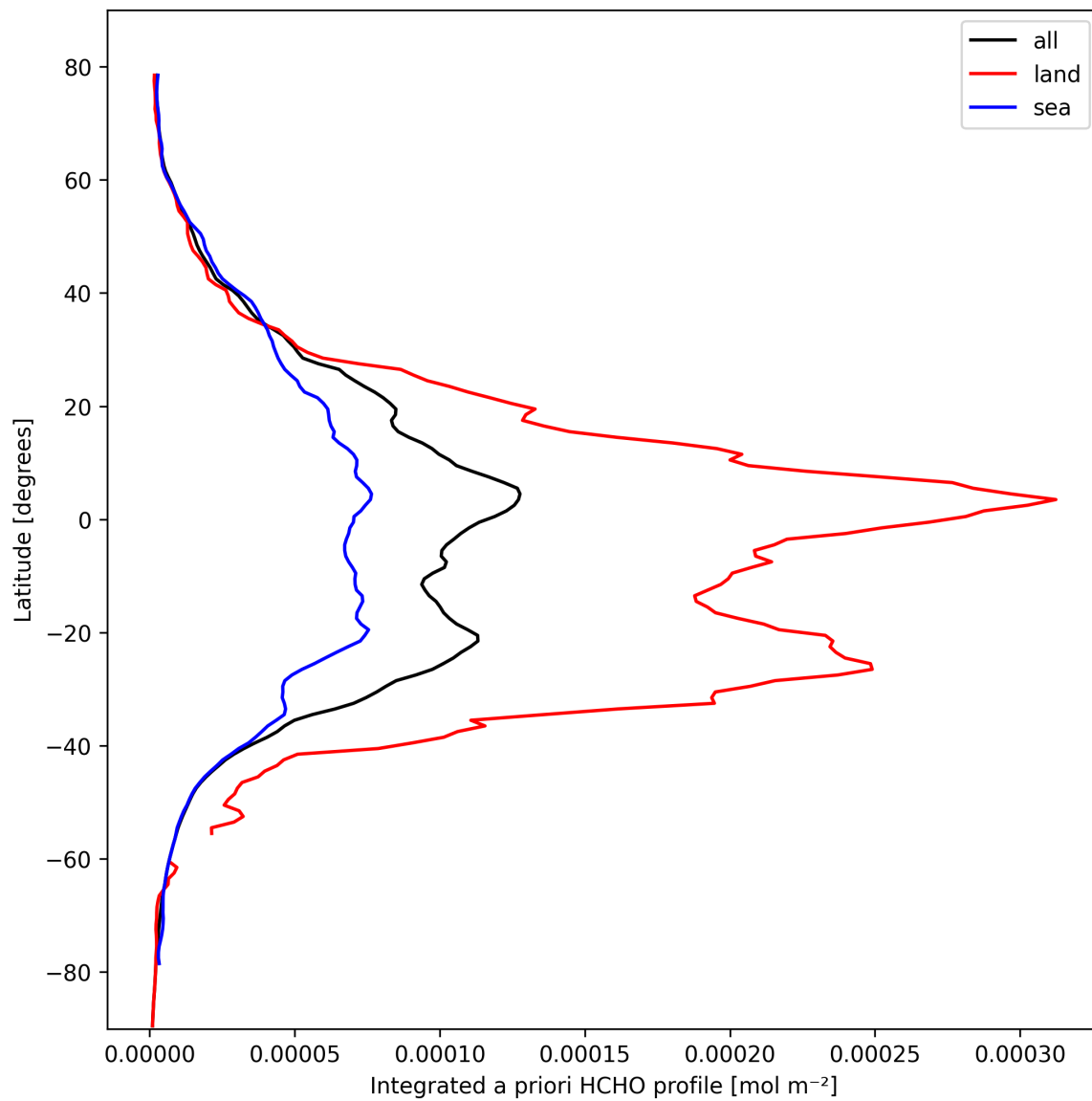
Figure 27: Zonal average of “Integrated a priori HCHO profile” for 2025-03-02 to 2025-03-03.
