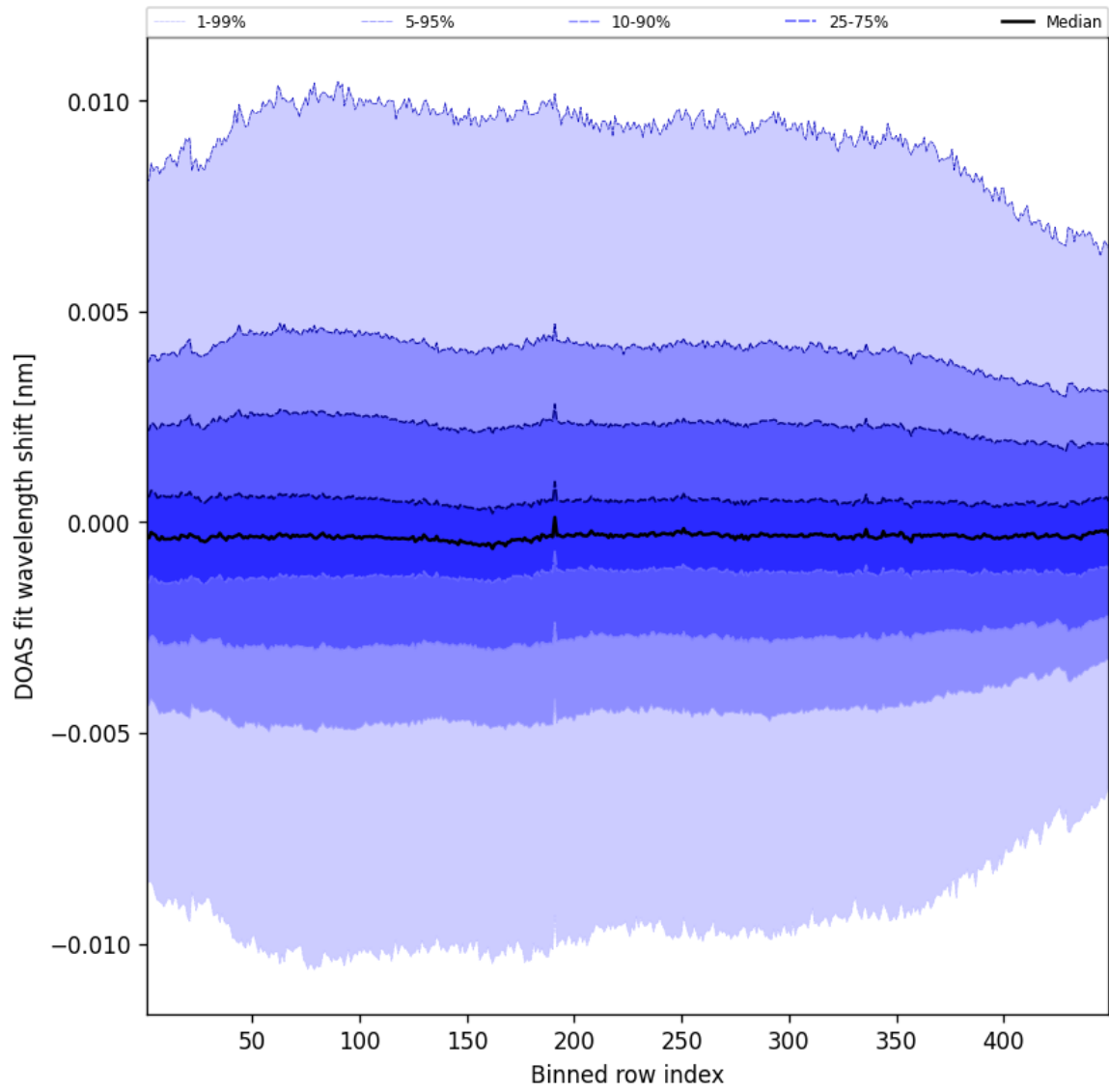
Figure 56: Along track statistics of “DOAS fit wavelength shift” for 2025-03-02 to 2025-03-03
