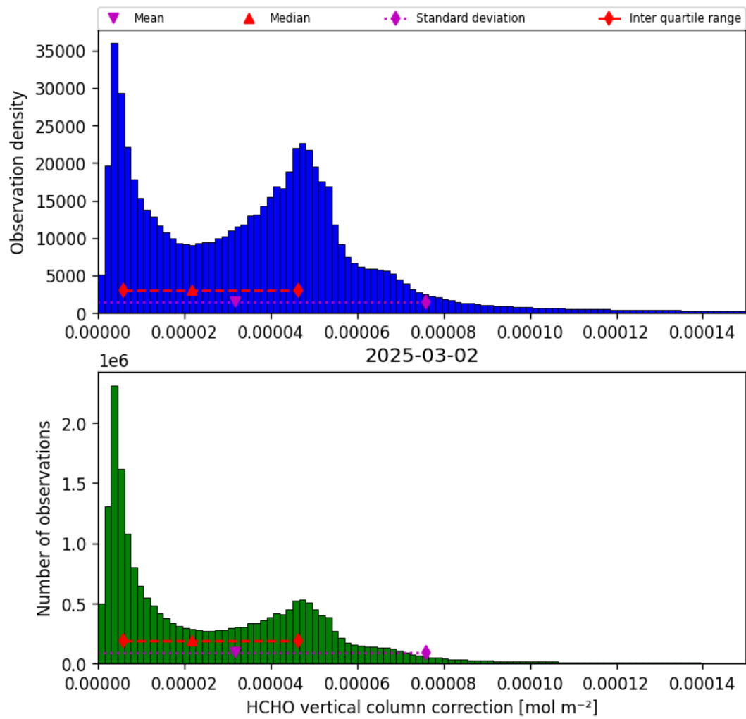
Figure 35: Histogram of “HCHO vertical column correction” for 2025-03-02 to 2025-03-03
