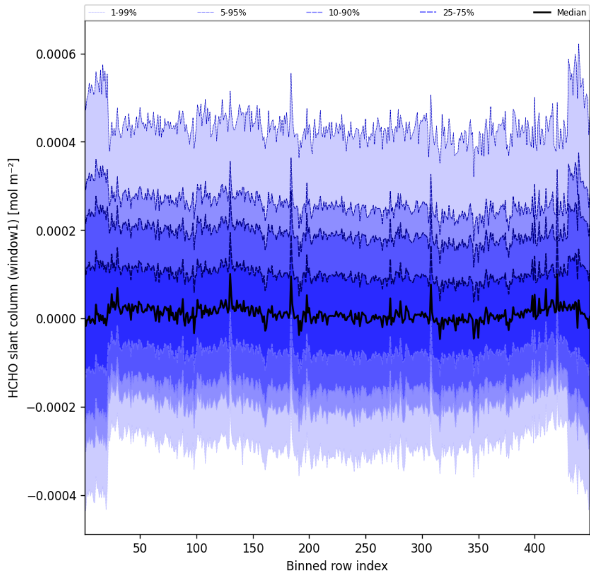
Figure 50: Along track statistics of “HCHO slant column (window1)” for 2025-03-02 to 2025-03-03
