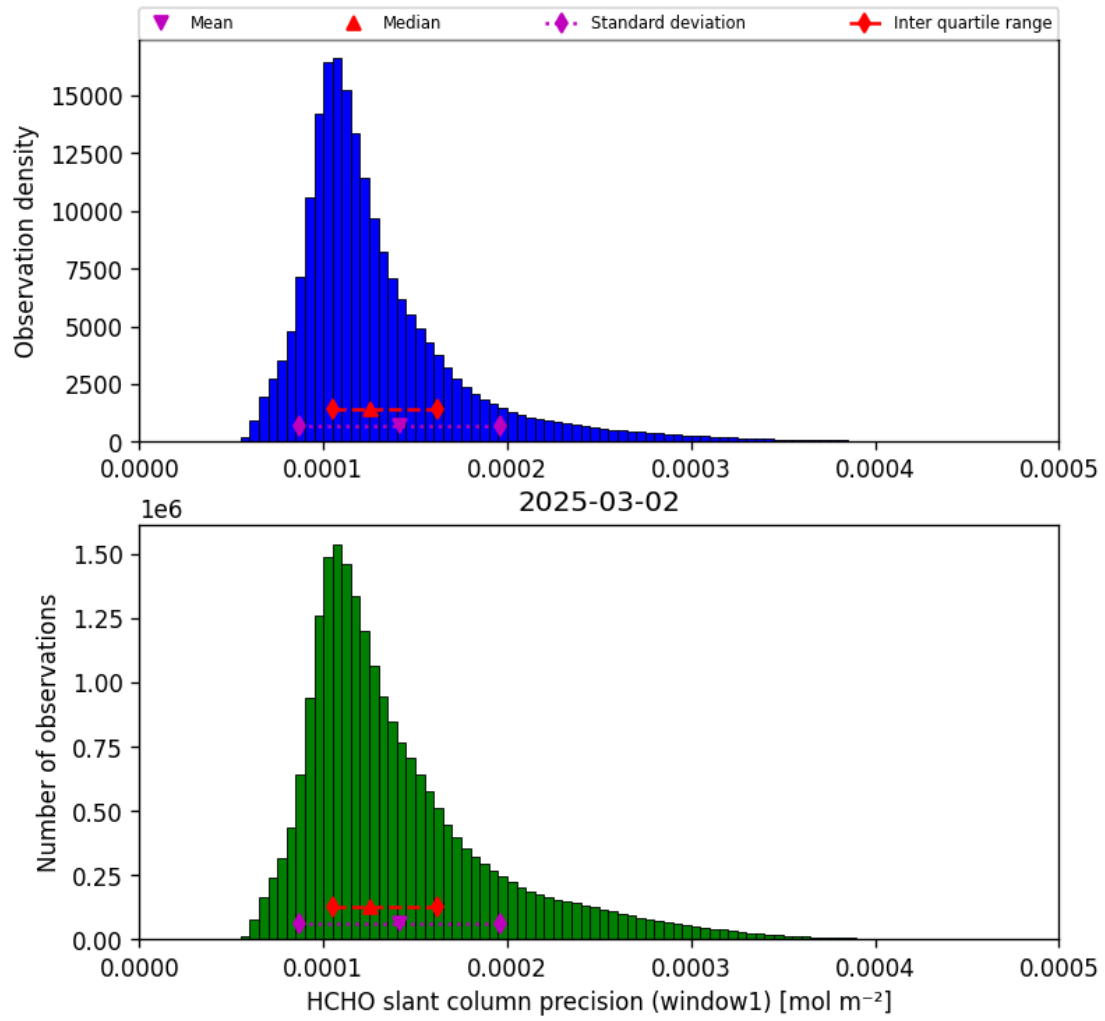
Figure 37: Histogram of “HCHO slant column precision (window1)” for 2025-03-02 to 2025-03-03
