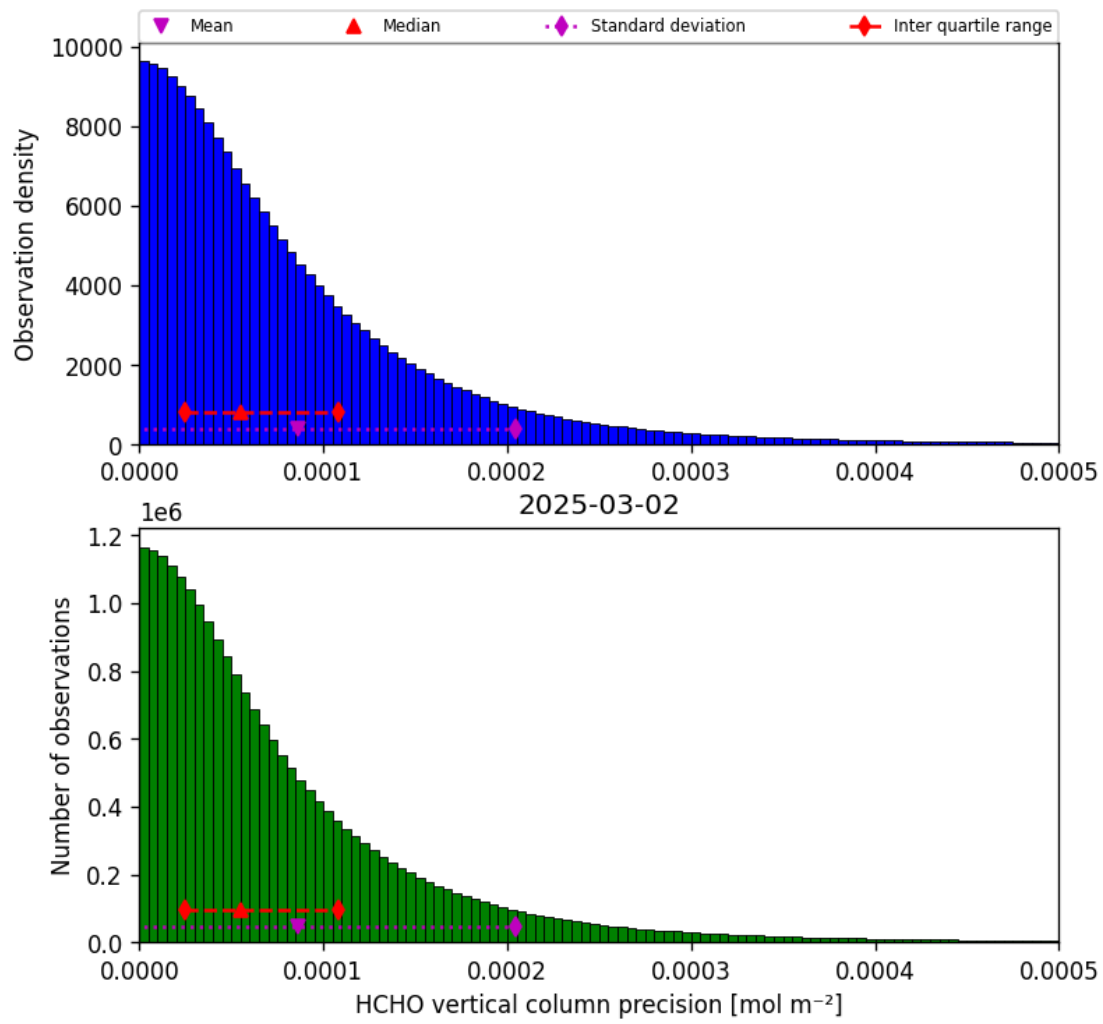
Figure 34: Histogram of “HCHO vertical column precision” for 2025-03-02 to 2025-03-03
