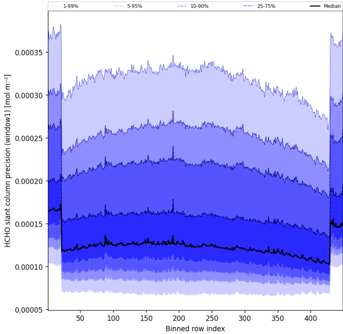
Figure 51: Along track statistics of “HCHO slant column precision (window1)” for 2025-03-02 to 2025-03-03
