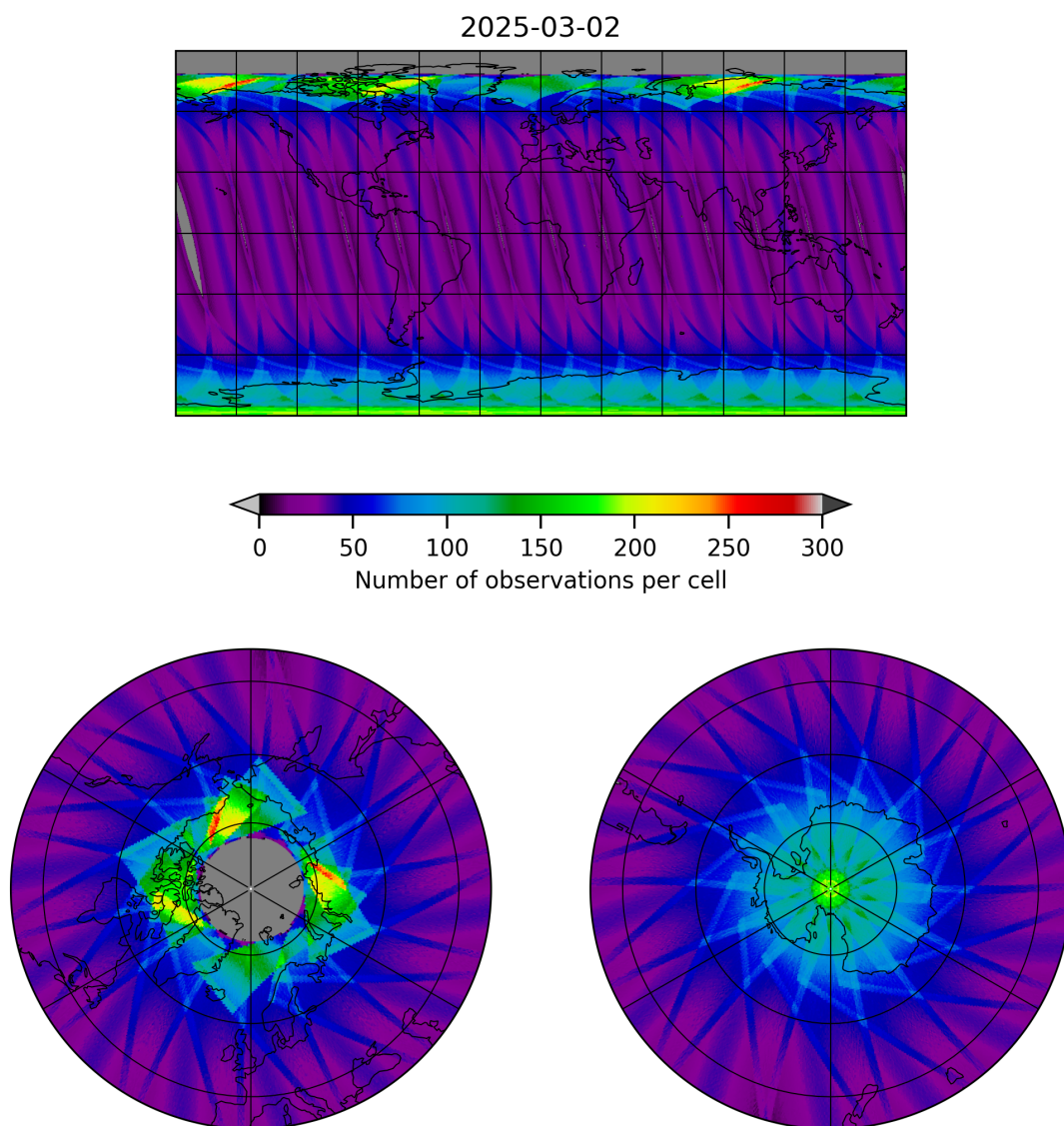
Figure 17: Map of the number of observations for 2025-03-02 to 2025-03-03
