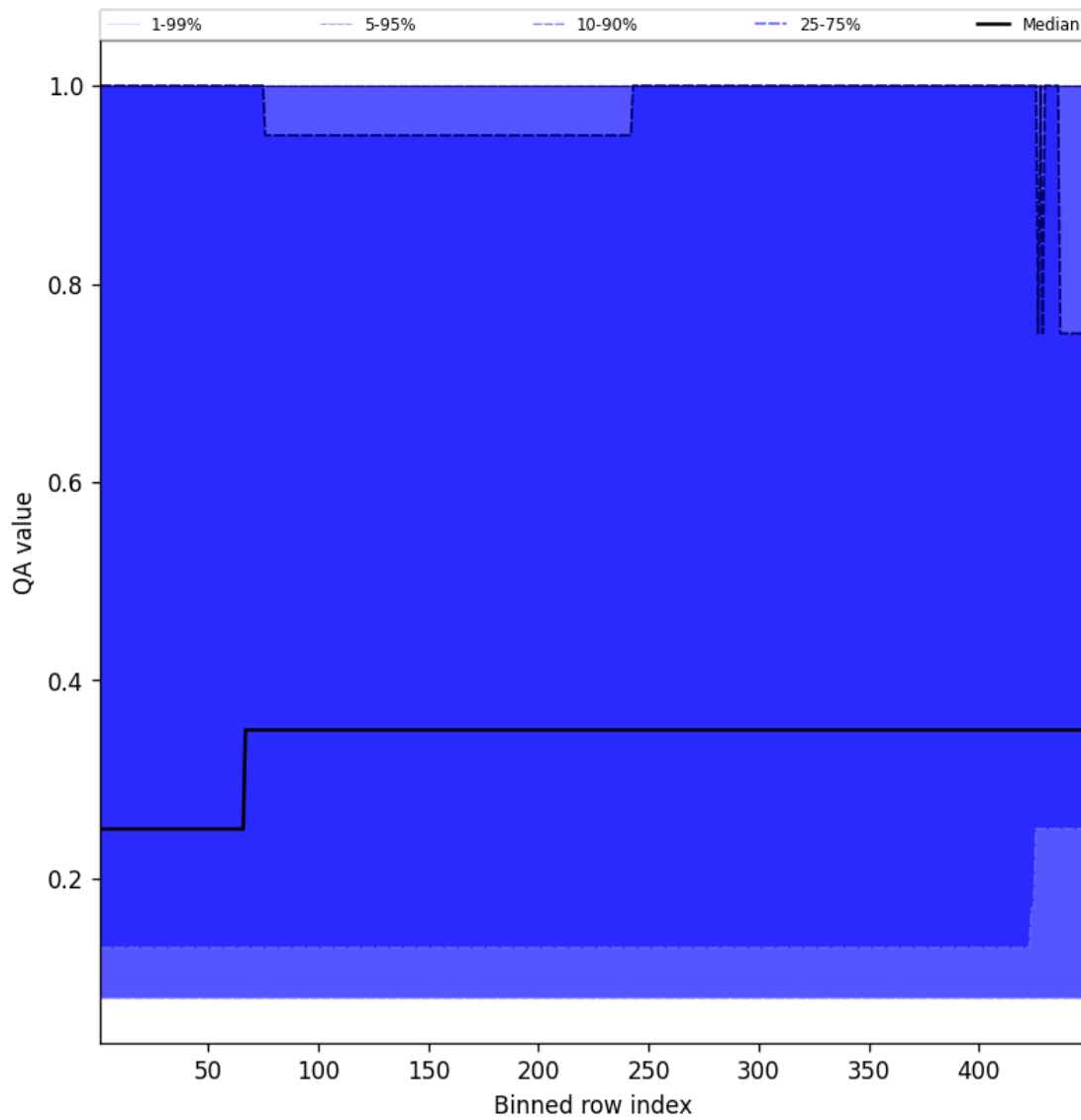
Figure 46: Along track statistics of “QA value” for 2025-03-02 to 2025-03-03
