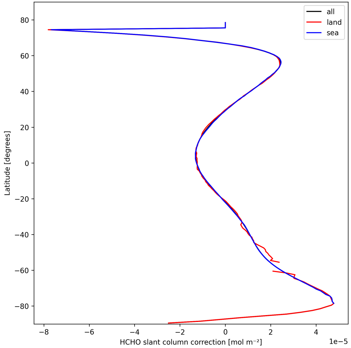
Figure 31: Zonal average of “HCHO slant column correction” for 2025-03-02 to 2025-03-03.
