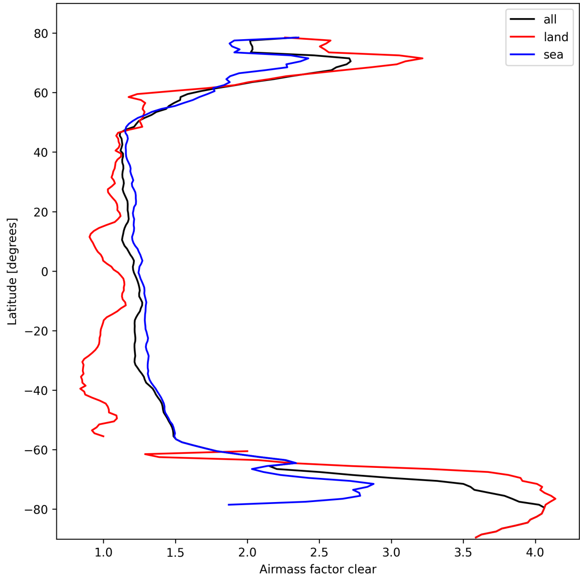
Figure 26: Zonal average of “Airmass factor clear” for 2025-03-02 to 2025-03-03.
