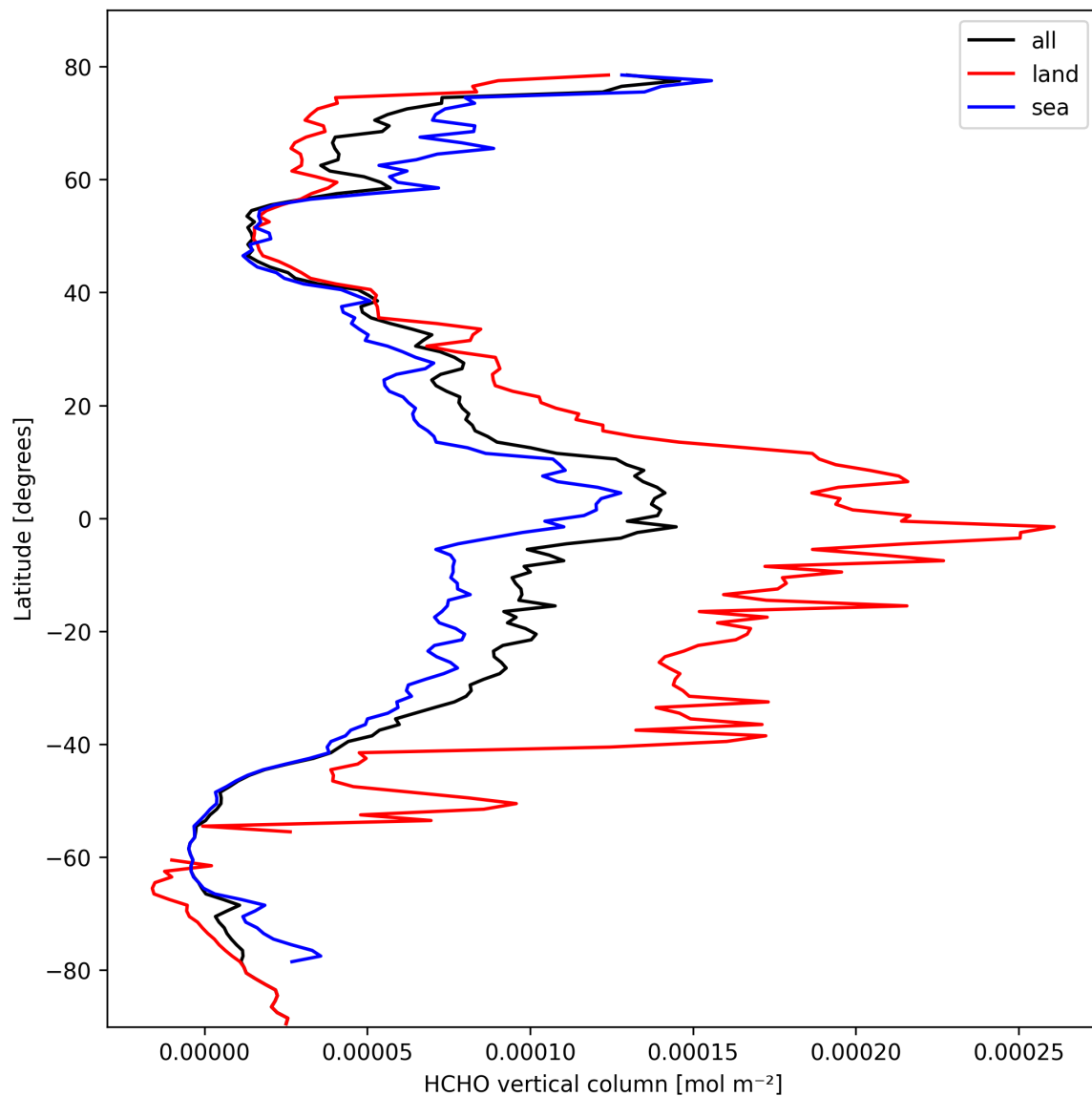
Figure 19: Zonal average of “HCHO vertical column” for 2025-03-02 to 2025-03-03.
