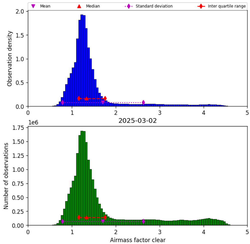
Figure 40: Histogram of “Airmass factor clear” for 2025-03-02 to 2025-03-03
