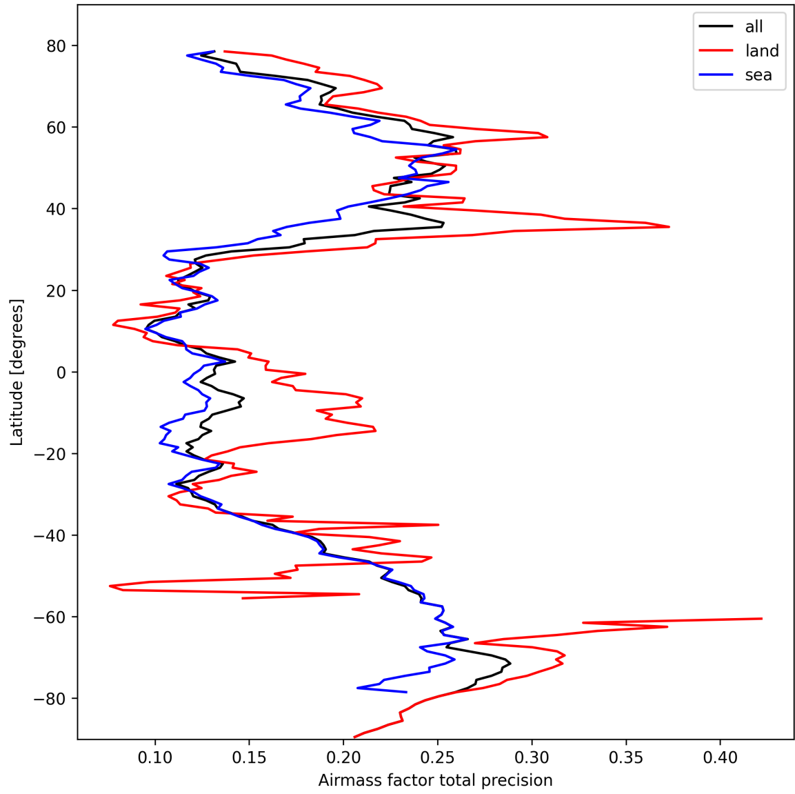
Figure 25: Zonal average of “Airmass factor total precision” for 2025-03-02 to 2025-03-03.
