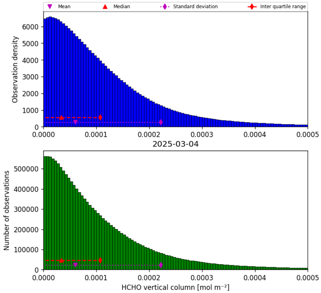
Figure 33: Histogram of “HCHO vertical column” for 2025-03-04 to 2025-03-04
