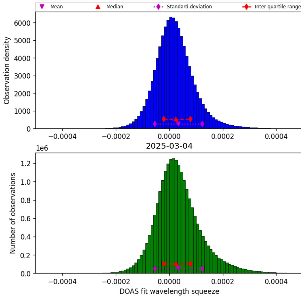
Figure 43: Histogram of “DOAS fit wavelength squeeze” for 2025-03-04 to 2025-03-04
