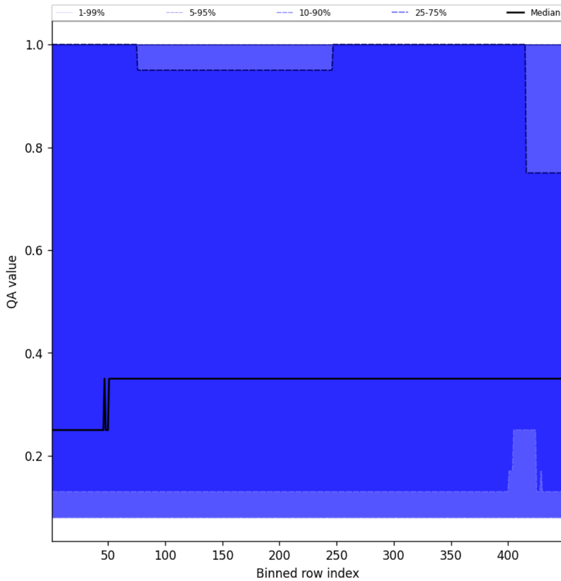
Figure 46: Along track statistics of “QA value” for 2025-03-04 to 2025-03-04
