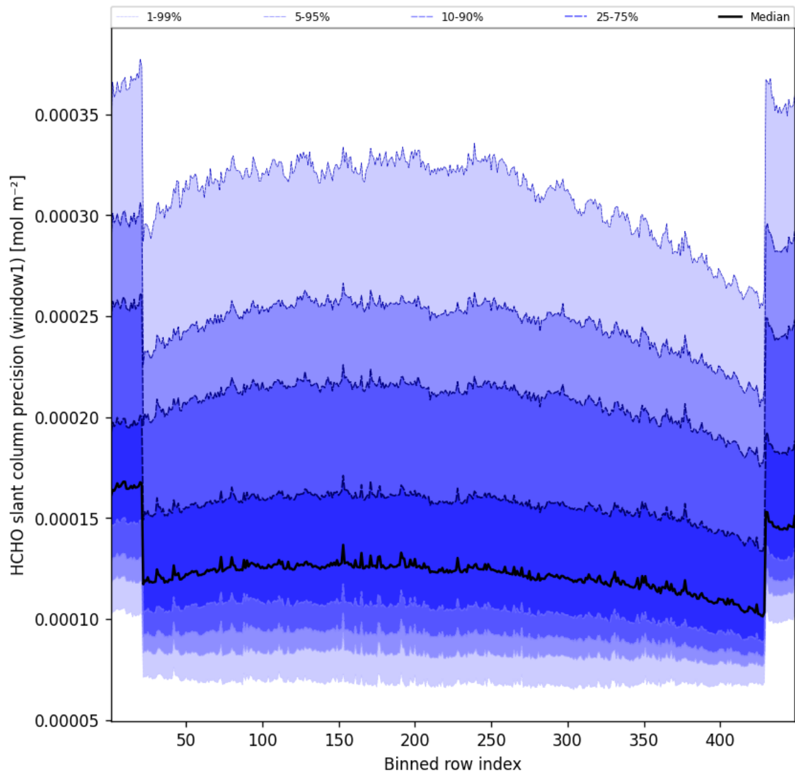
Figure 51: Along track statistics of “HCHO slant column precision (window1)” for 2025-03-04 to 2025-03-04
