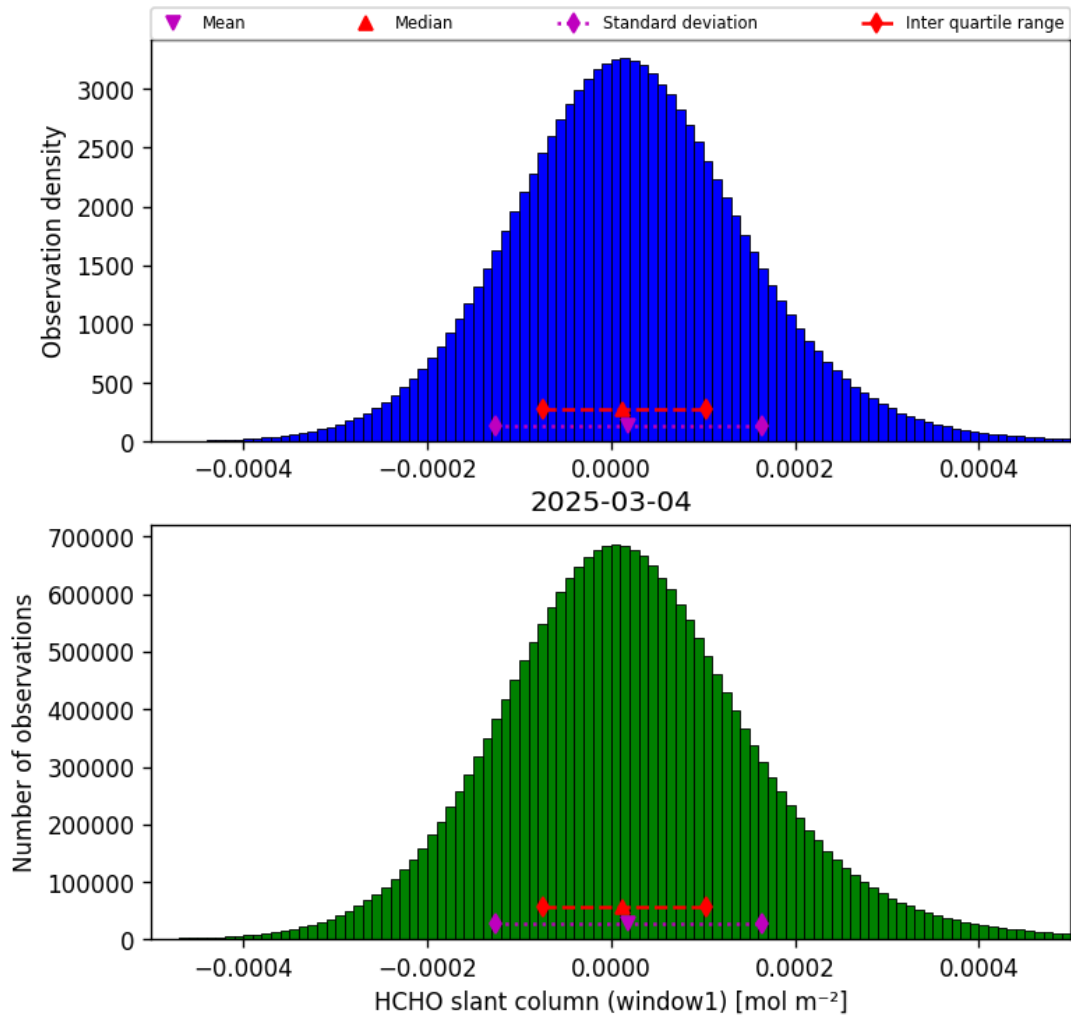
Figure 36: Histogram of “HCHO slant column (window1)” for 2025-03-04 to 2025-03-04
