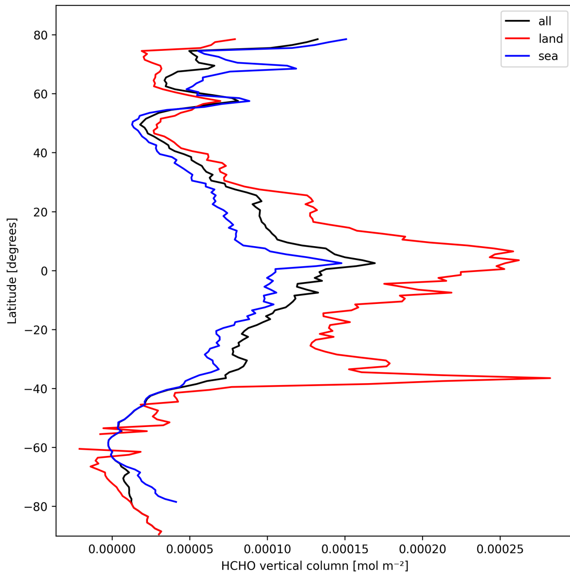
Figure 19: Zonal average of “HCHO vertical column” for 2025-03-04 to 2025-03-04.
