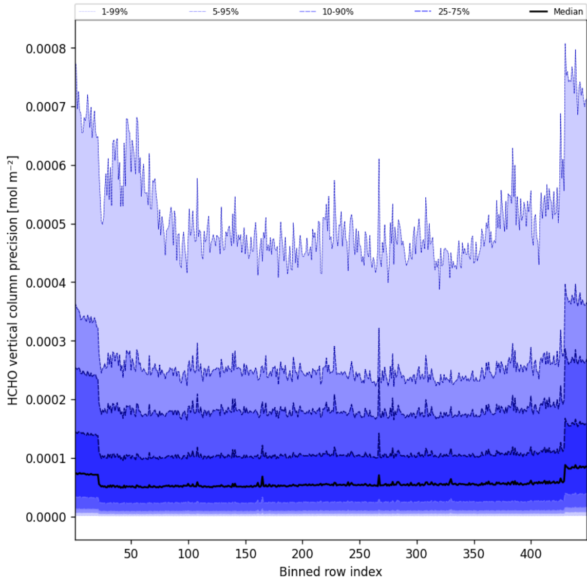
Figure 48: Along track statistics of “HCHO vertical column precision” for 2025-03-04 to 2025-03-04
