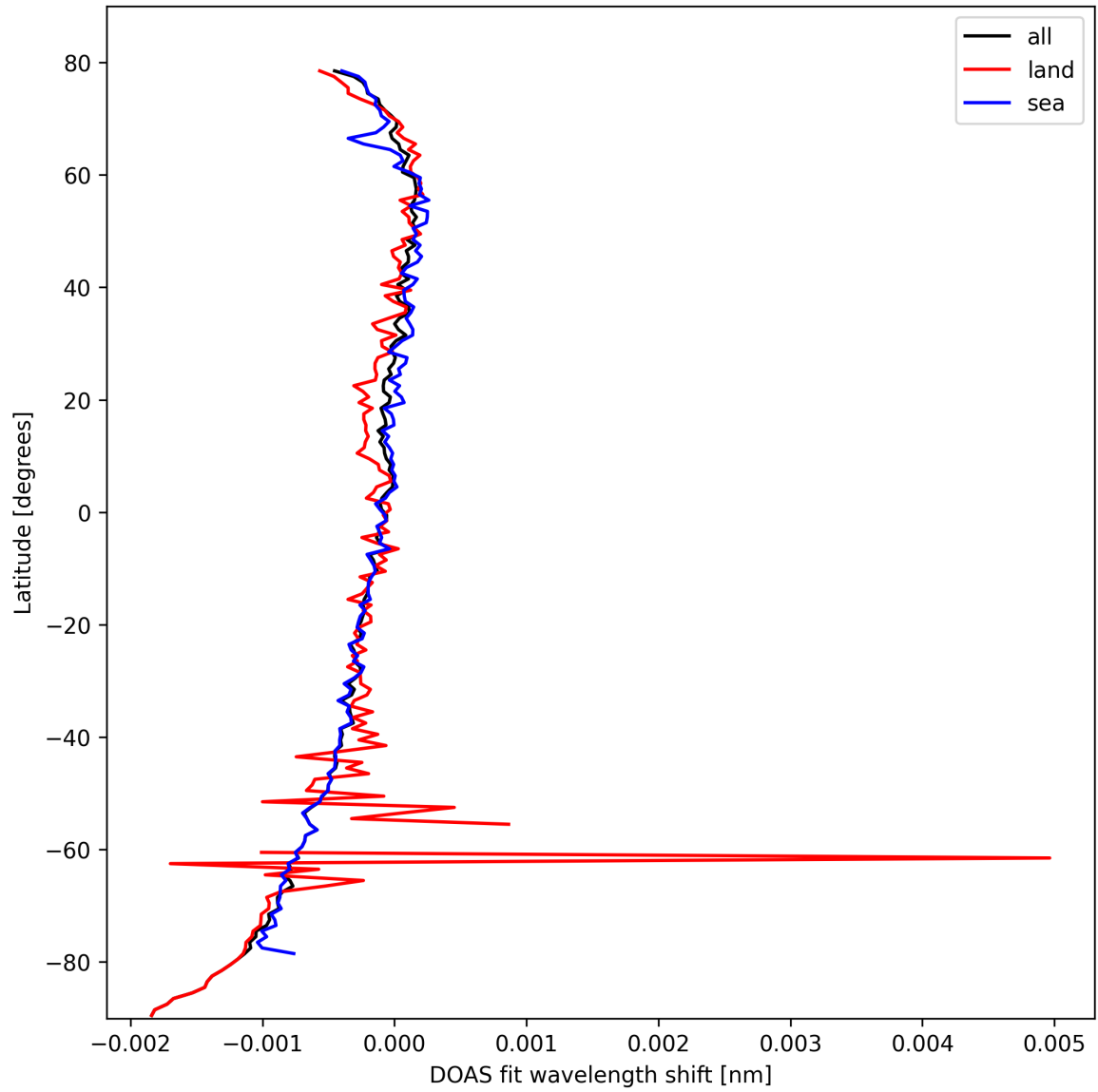
Figure 28: Zonal average of “DOAS fit wavelength shift” for 2025-03-04 to 2025-03-04.
