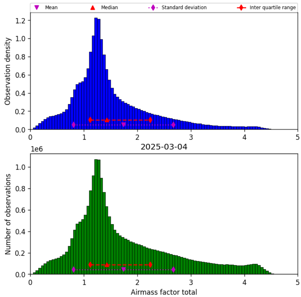
Figure 38: Histogram of “Airmass factor total” for 2025-03-04 to 2025-03-04
