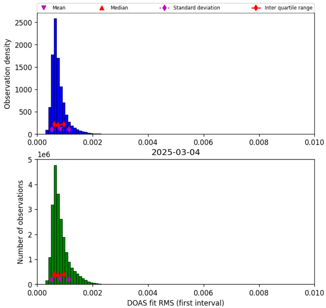
Figure 44: Histogram of “DOAS fit RMS (first interval)” for 2025-03-04 to 2025-03-04
