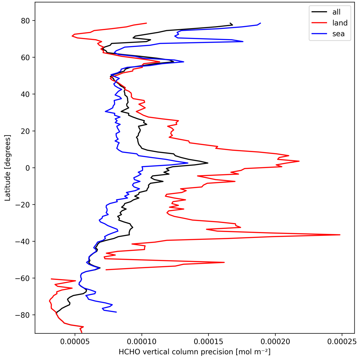
Figure 20: Zonal average of “HCHO vertical column precision” for 2025-03-04 to 2025-03-04.
