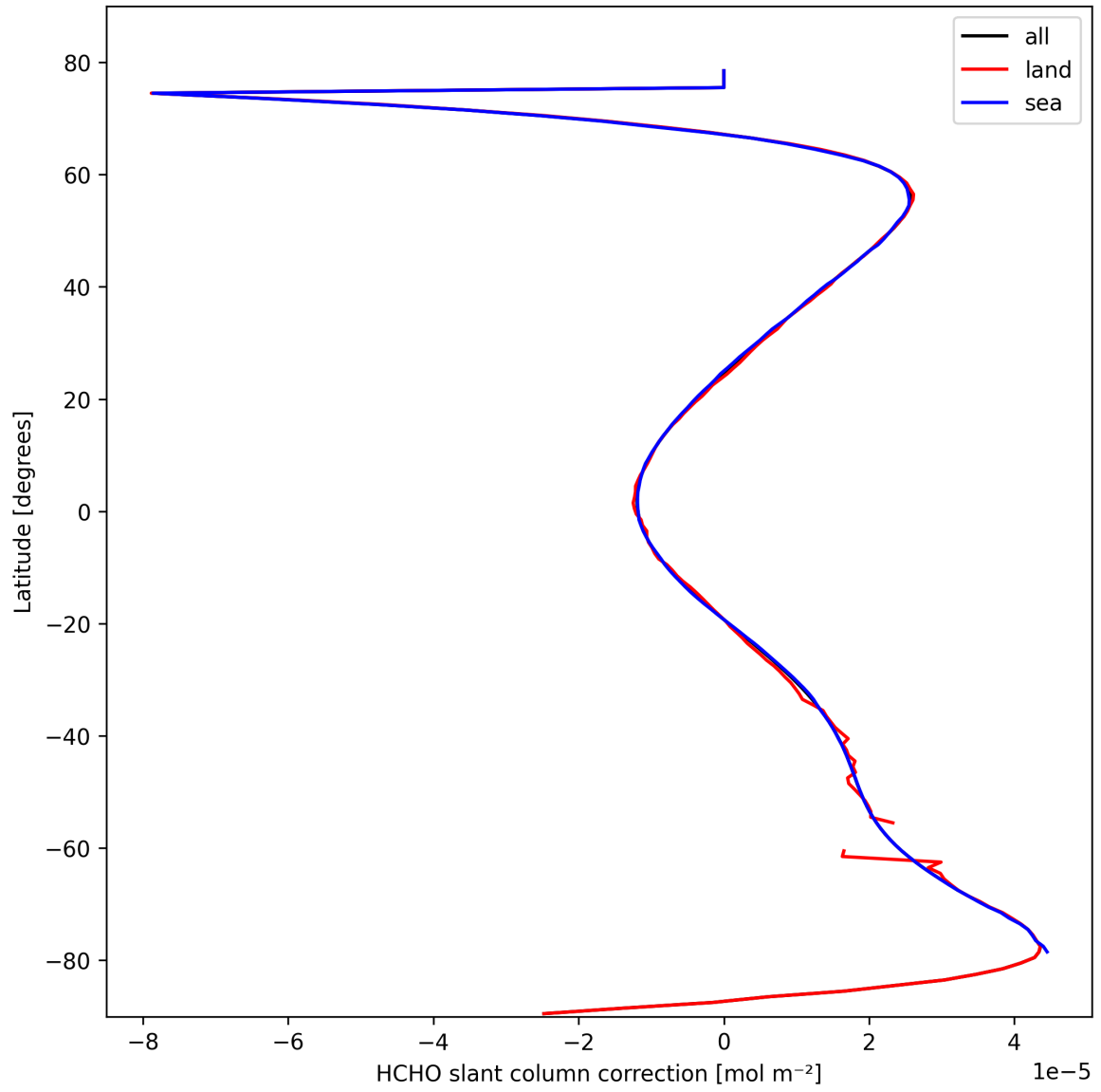
Figure 31: Zonal average of “HCHO slant column correction” for 2025-03-04 to 2025-03-04.
