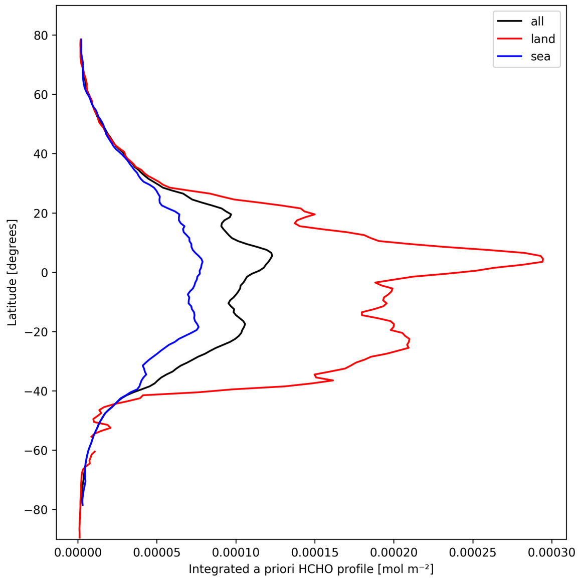
Figure 27: Zonal average of “Integrated a priori HCHO profile” for 2025-03-04 to 2025-03-04.
