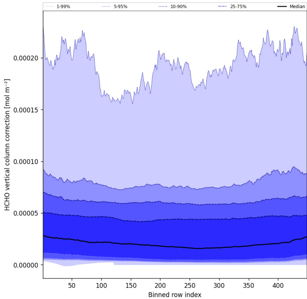
Figure 49: Along track statistics of “HCHO vertical column correction” for 2025-03-04 to 2025-03-04
