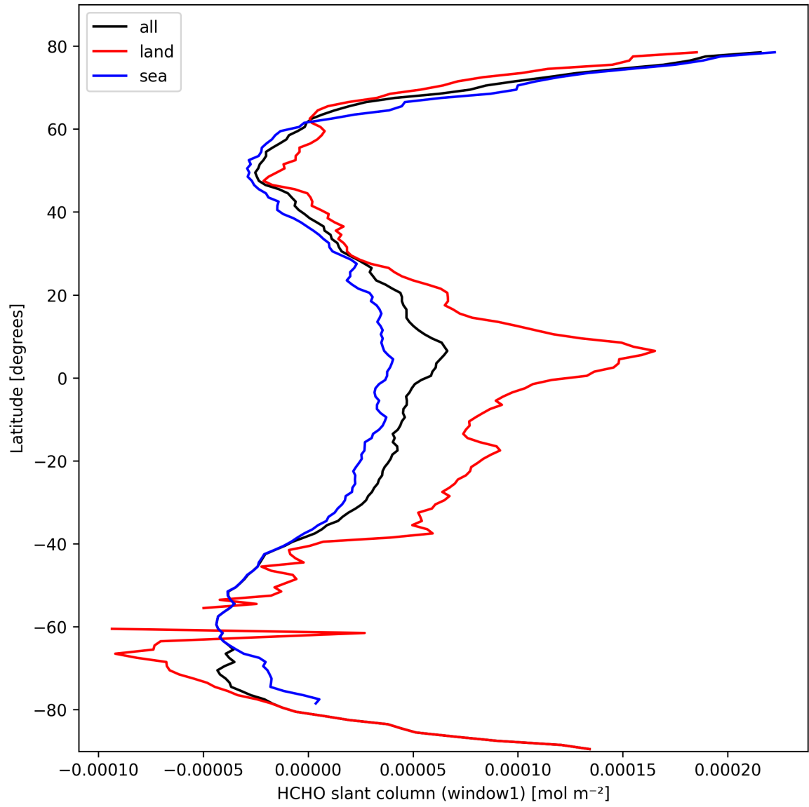
Figure 22: Zonal average of “HCHO slant column (window1)” for 2025-03-04 to 2025-03-04.
