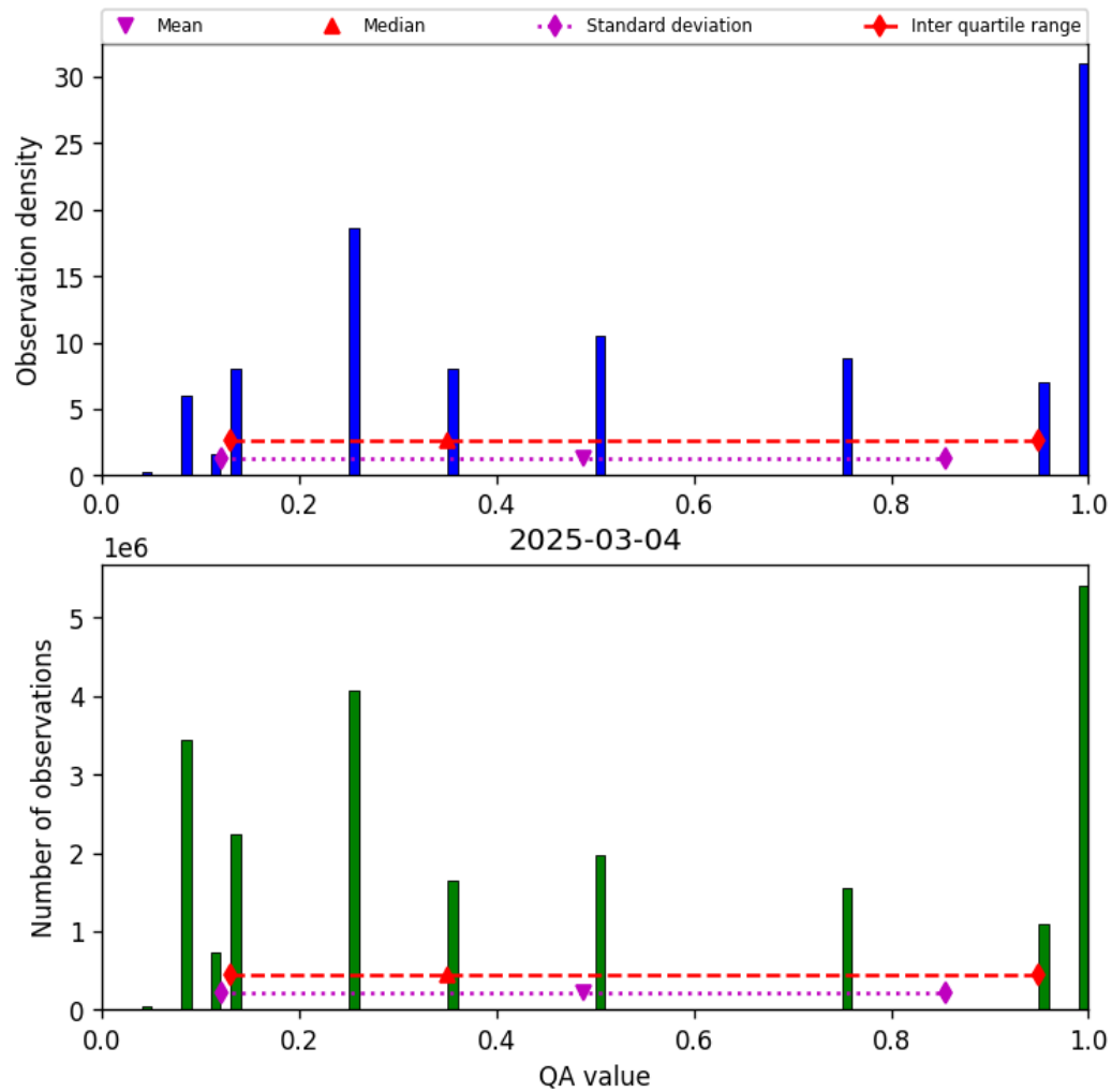
Figure 32: Histogram of “QA value” for 2025-03-04 to 2025-03-04
