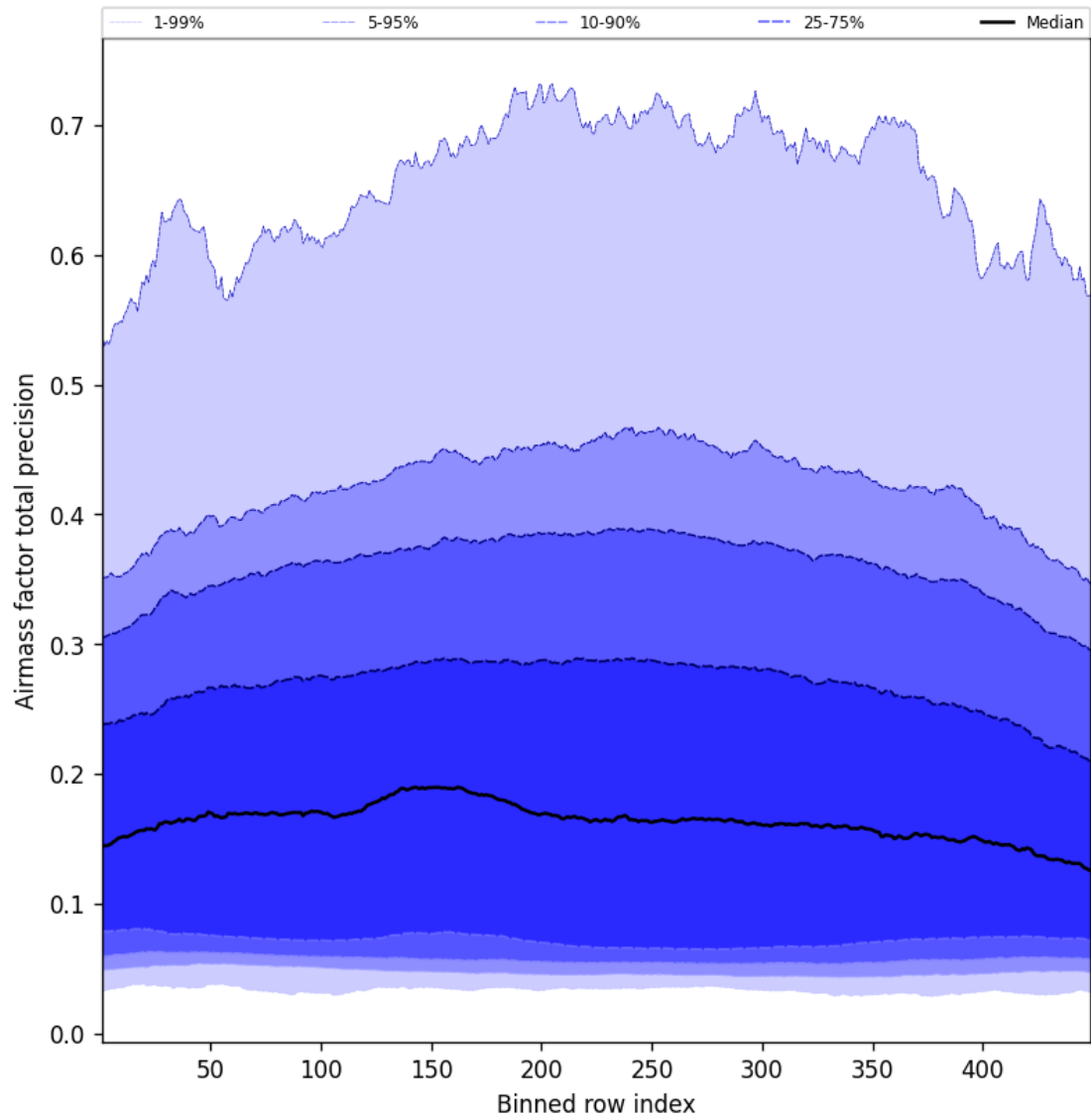
Figure 53: Along track statistics of “Airmass factor total precision” for 2025-03-04 to 2025-03-04
