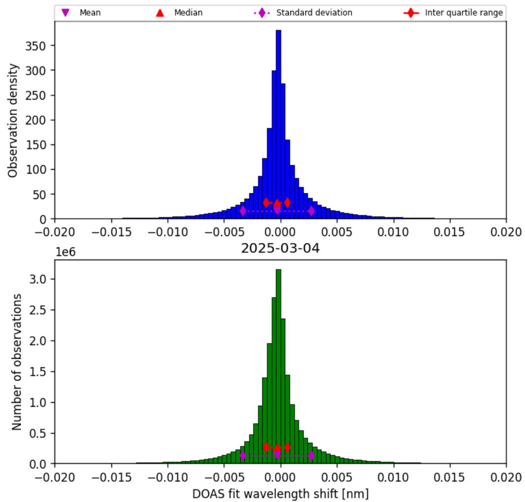
Figure 42: Histogram of “DOAS fit wavelength shift” for 2025-03-04 to 2025-03-04
