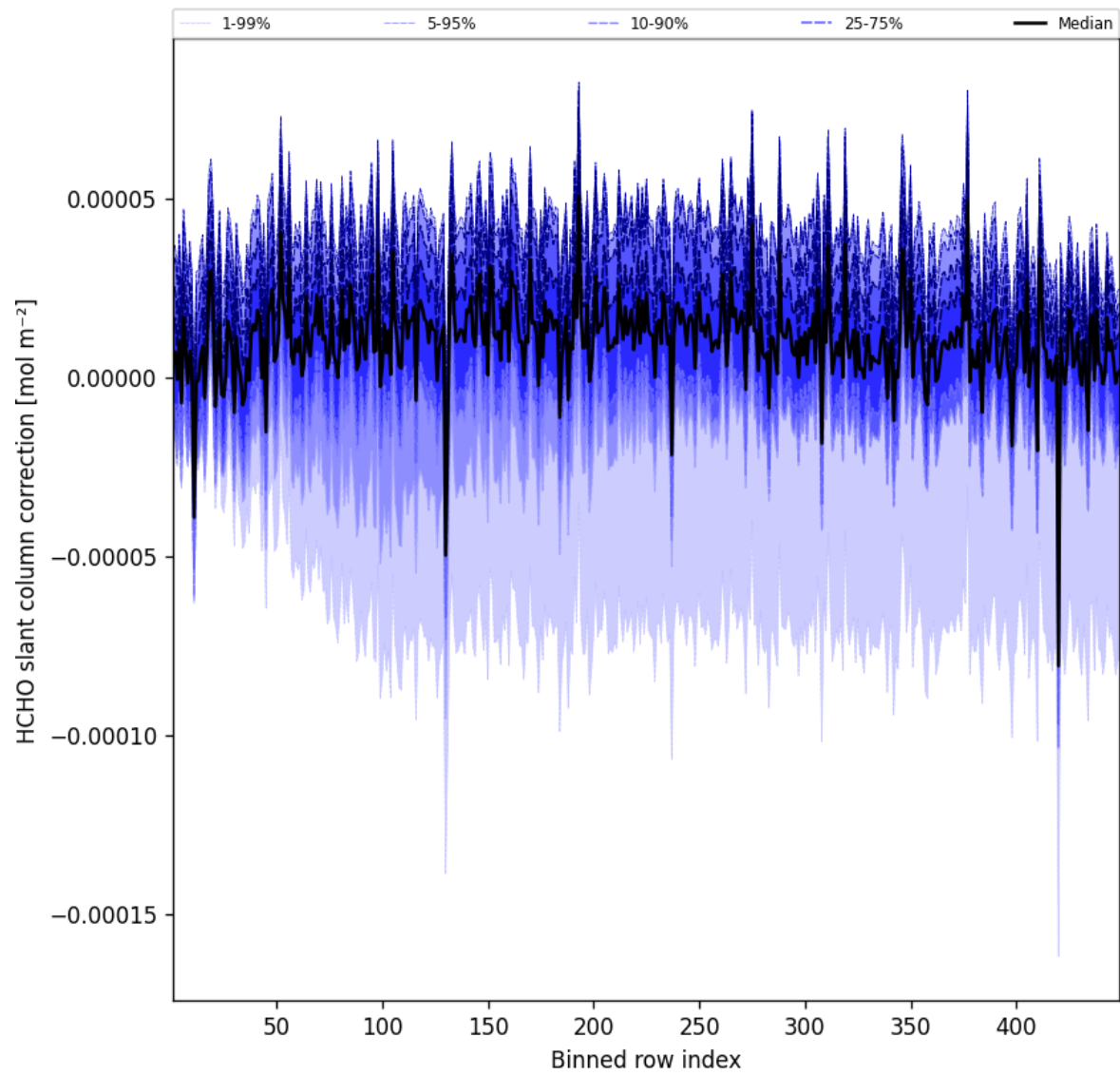
Figure 59: Along track statistics of “HCHO slant column correction” for 2025-03-04 to 2025-03-04
