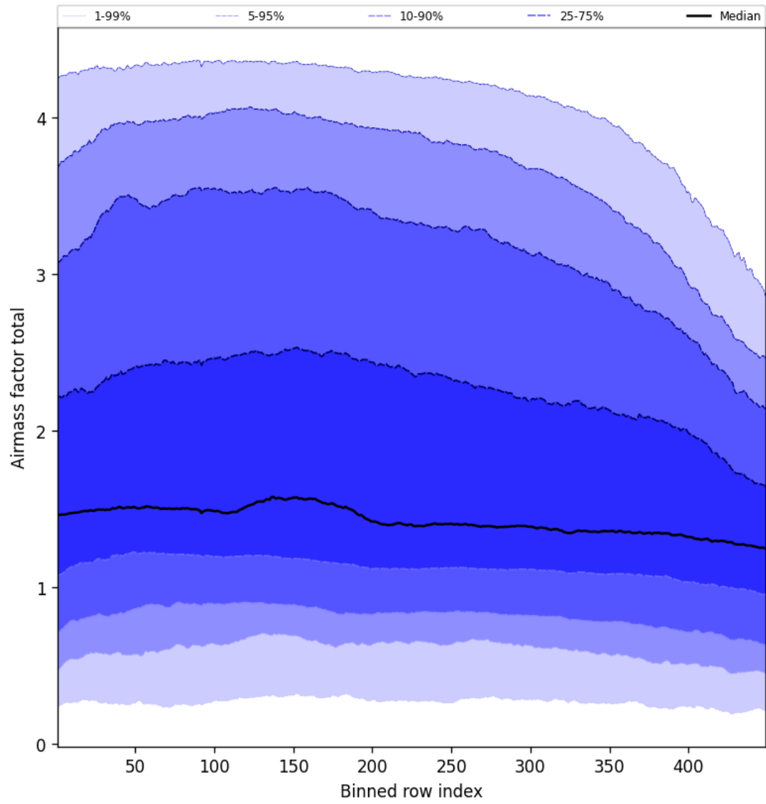
Figure 52: Along track statistics of “Airmass factor total” for 2025-03-04 to 2025-03-04
