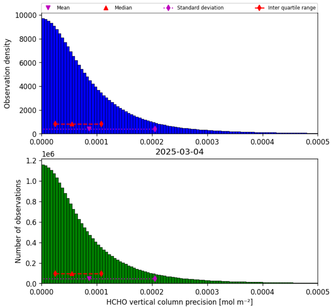
Figure 34: Histogram of “HCHO vertical column precision” for 2025-03-04 to 2025-03-04
