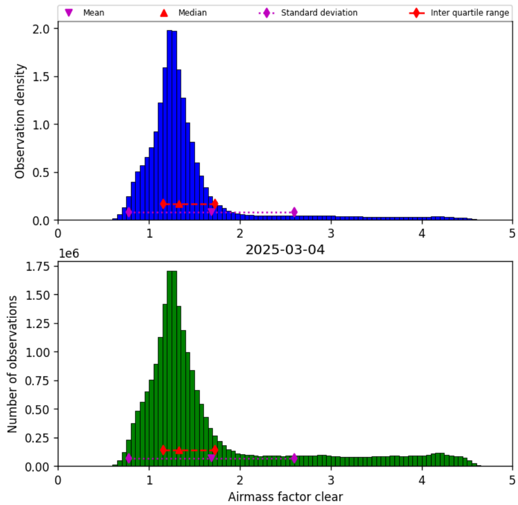
Figure 40: Histogram of “Airmass factor clear” for 2025-03-04 to 2025-03-04
