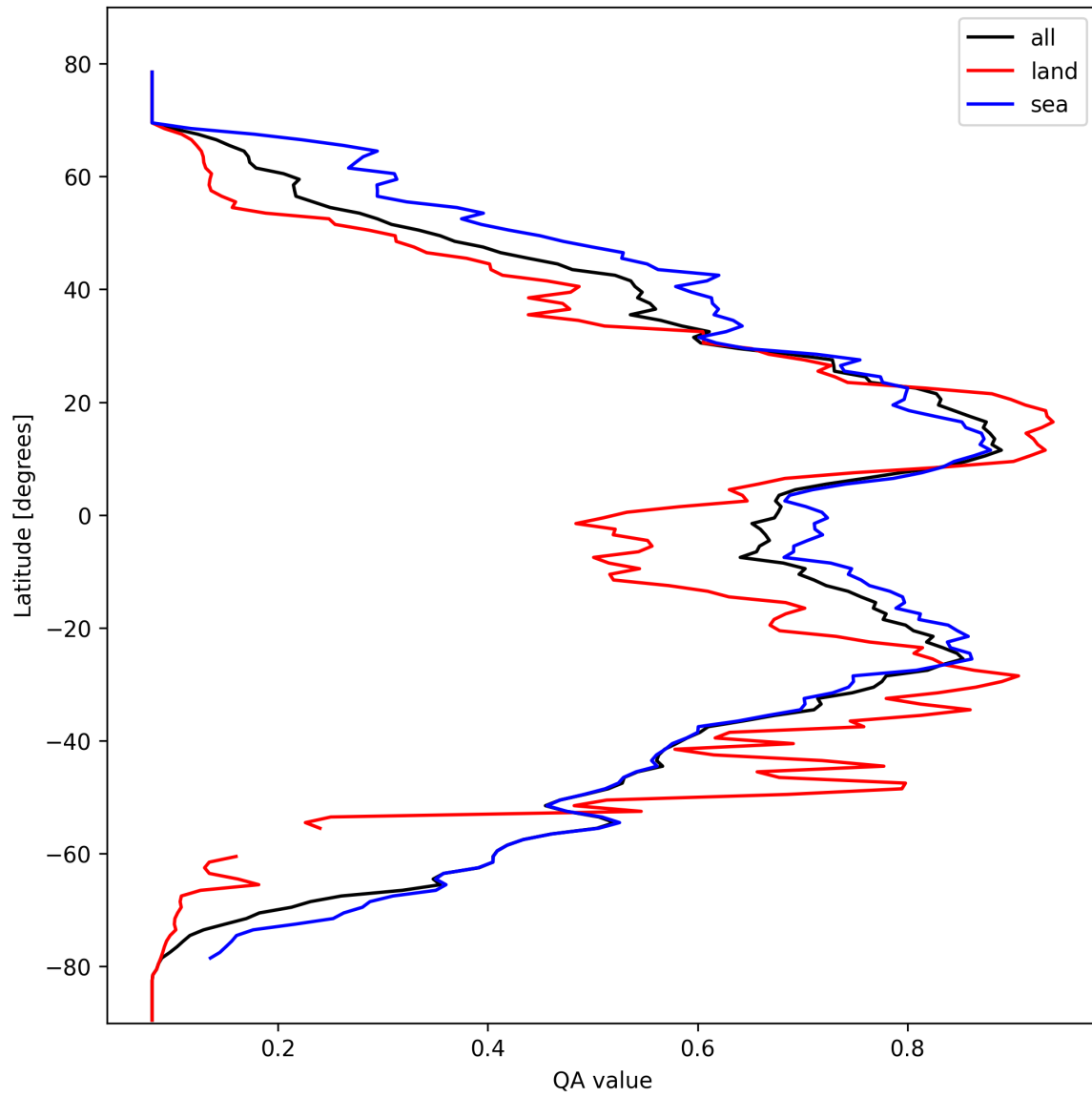
Figure 18: Zonal average of “QA value” for 2025-03-04 to 2025-03-04.
