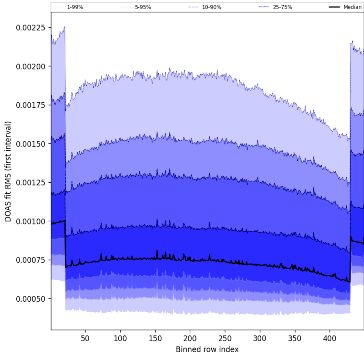
Figure 58: Along track statistics of “DOAS fit RMS (first interval)” for 2025-03-04 to 2025-03-04
