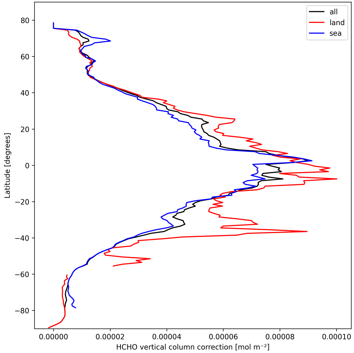
Figure 21: Zonal average of “HCHO vertical column correction” for 2025-03-04 to 2025-03-04.
