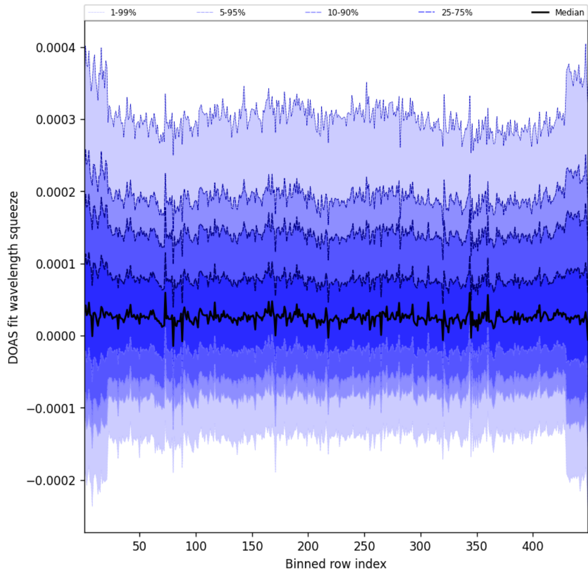
Figure 57: Along track statistics of “DOAS fit wavelength squeeze” for 2025-03-04 to 2025-03-04
