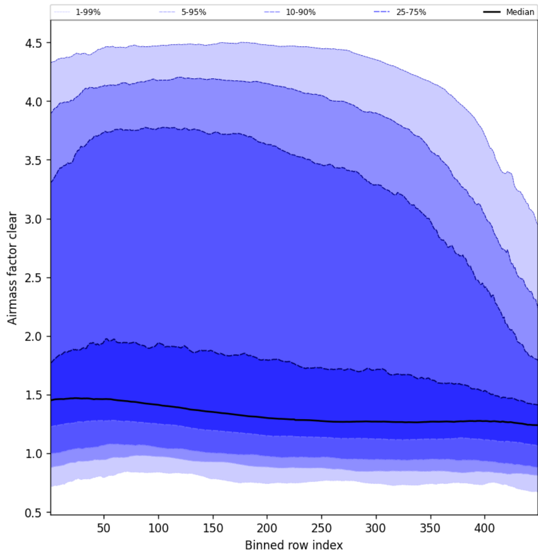
Figure 54: Along track statistics of “Airmass factor clear” for 2025-03-04 to 2025-03-04
