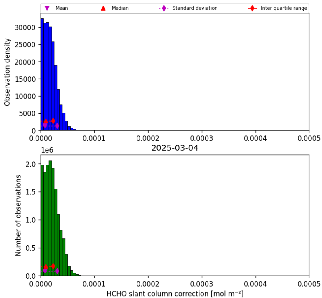
Figure 45: Histogram of “HCHO slant column correction” for 2025-03-04 to 2025-03-04
