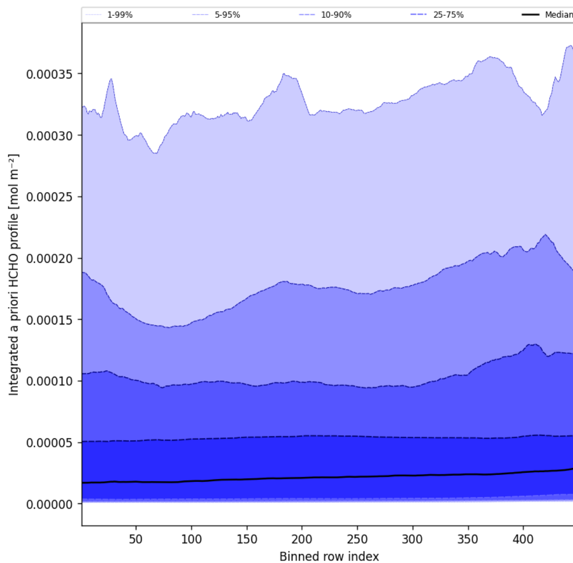
Figure 55: Along track statistics of “Integrated a priori HCHO profile” for 2025-03-04 to 2025-03-04
