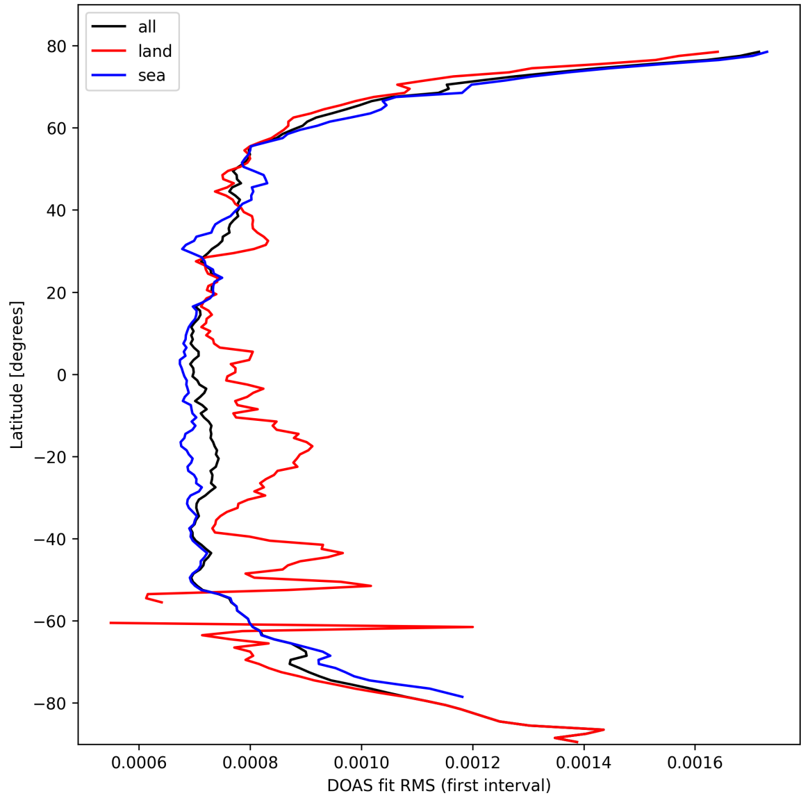
Figure 30: Zonal average of “DOAS fit RMS (first interval)” for 2025-03-04 to 2025-03-04.
