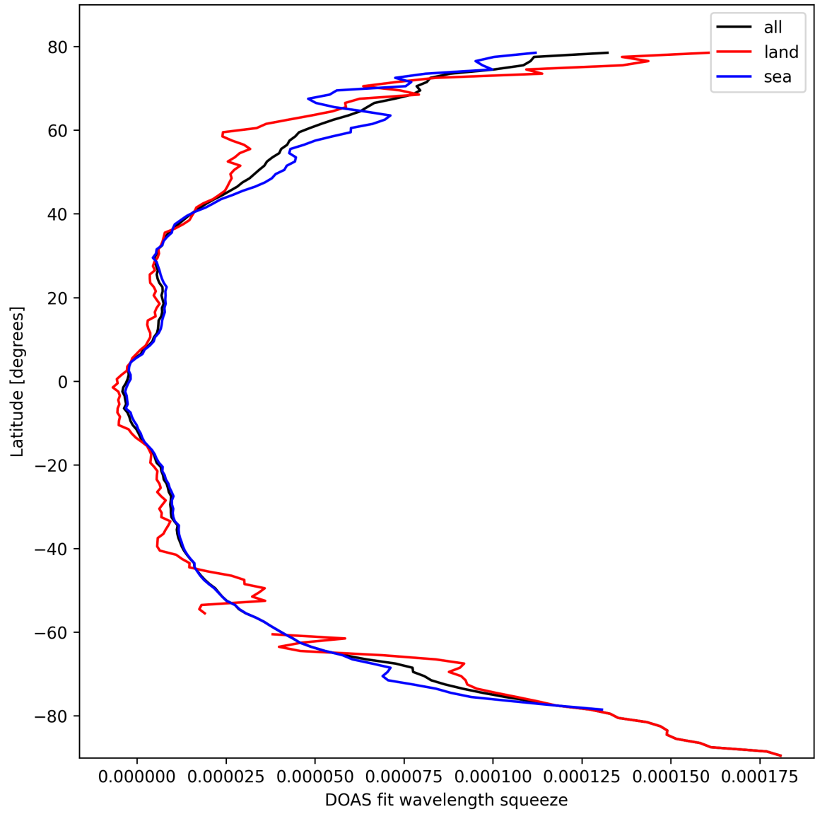
Figure 29: Zonal average of “DOAS fit wavelength squeeze” for 2025-03-04 to 2025-03-04.
