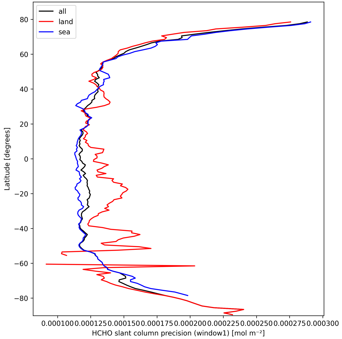
Figure 23: Zonal average of “HCHO slant column precision (window1)” for 2025-03-04 to 2025-03-04.
