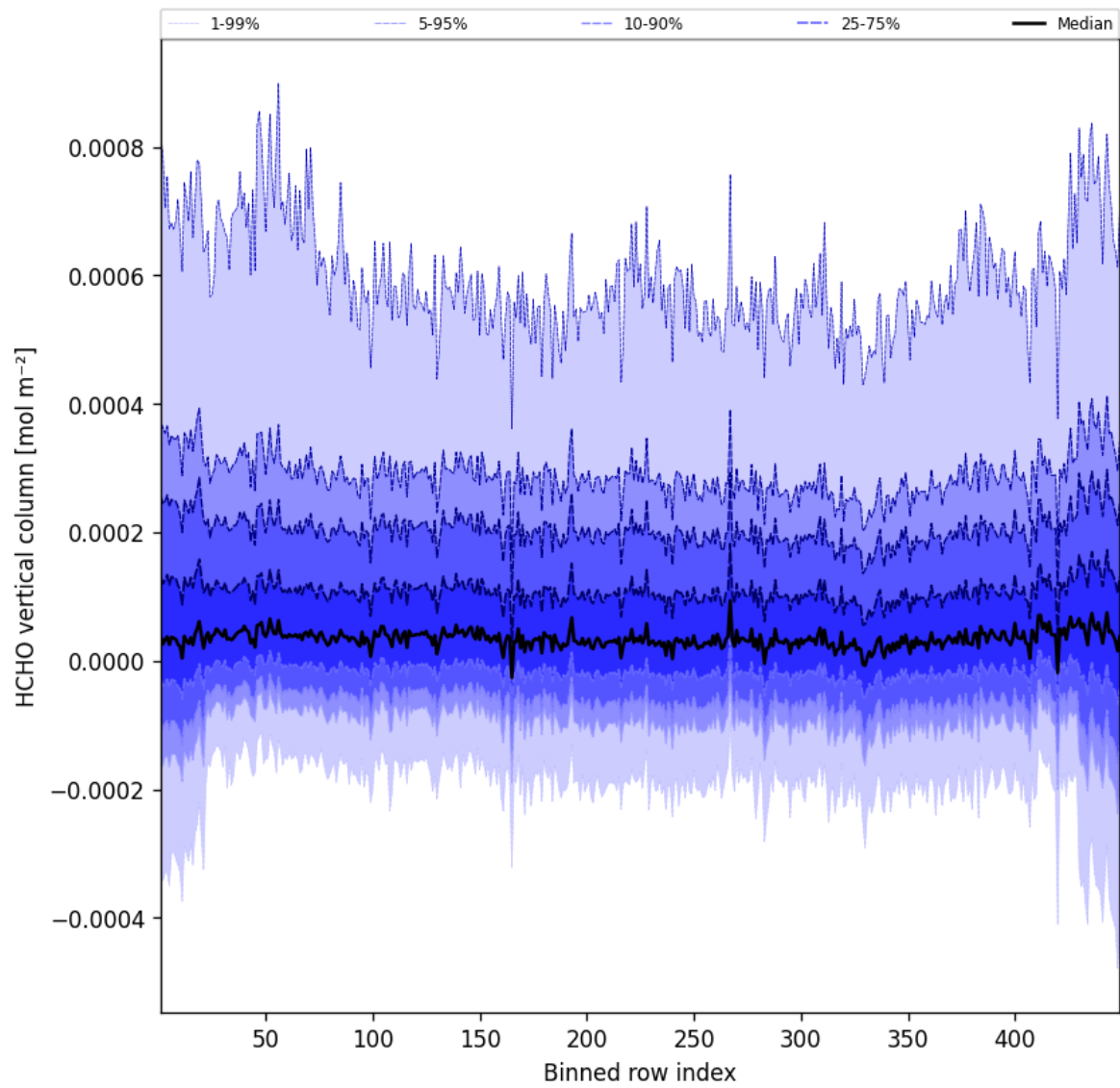
Figure 47: Along track statistics of “HCHO vertical column” for 2025-03-04 to 2025-03-04
