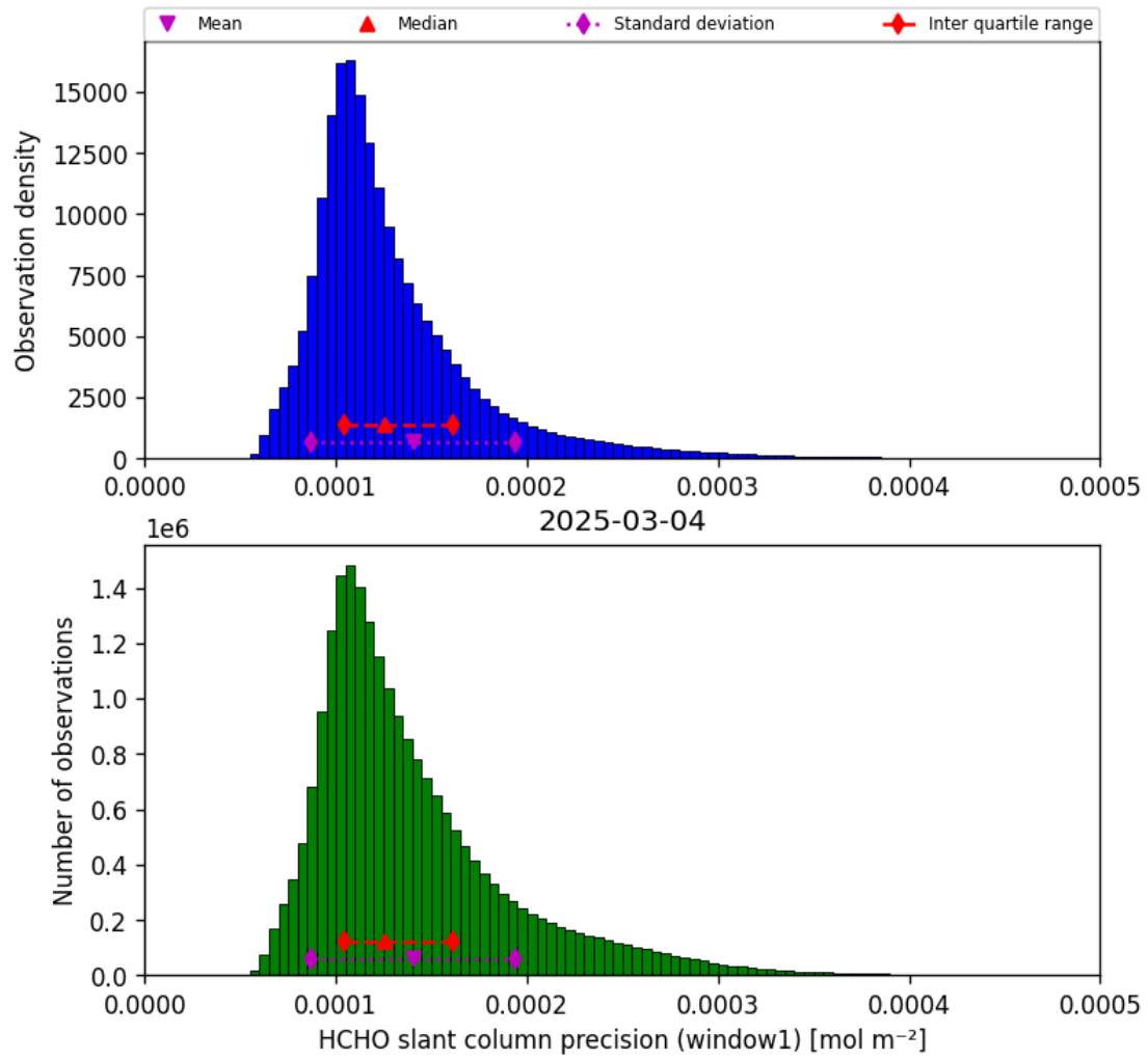
Figure 37: Histogram of “HCHO slant column precision (window1)” for 2025-03-04 to 2025-03-04
