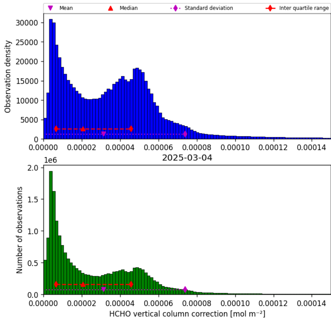
Figure 35: Histogram of “HCHO vertical column correction” for 2025-03-04 to 2025-03-04
