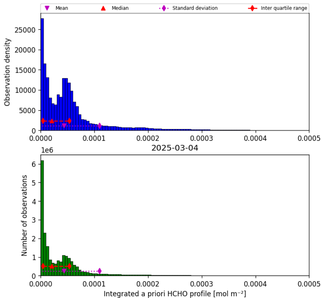
Figure 41: Histogram of “Integrated a priori HCHO profile” for 2025-03-04 to 2025-03-04
