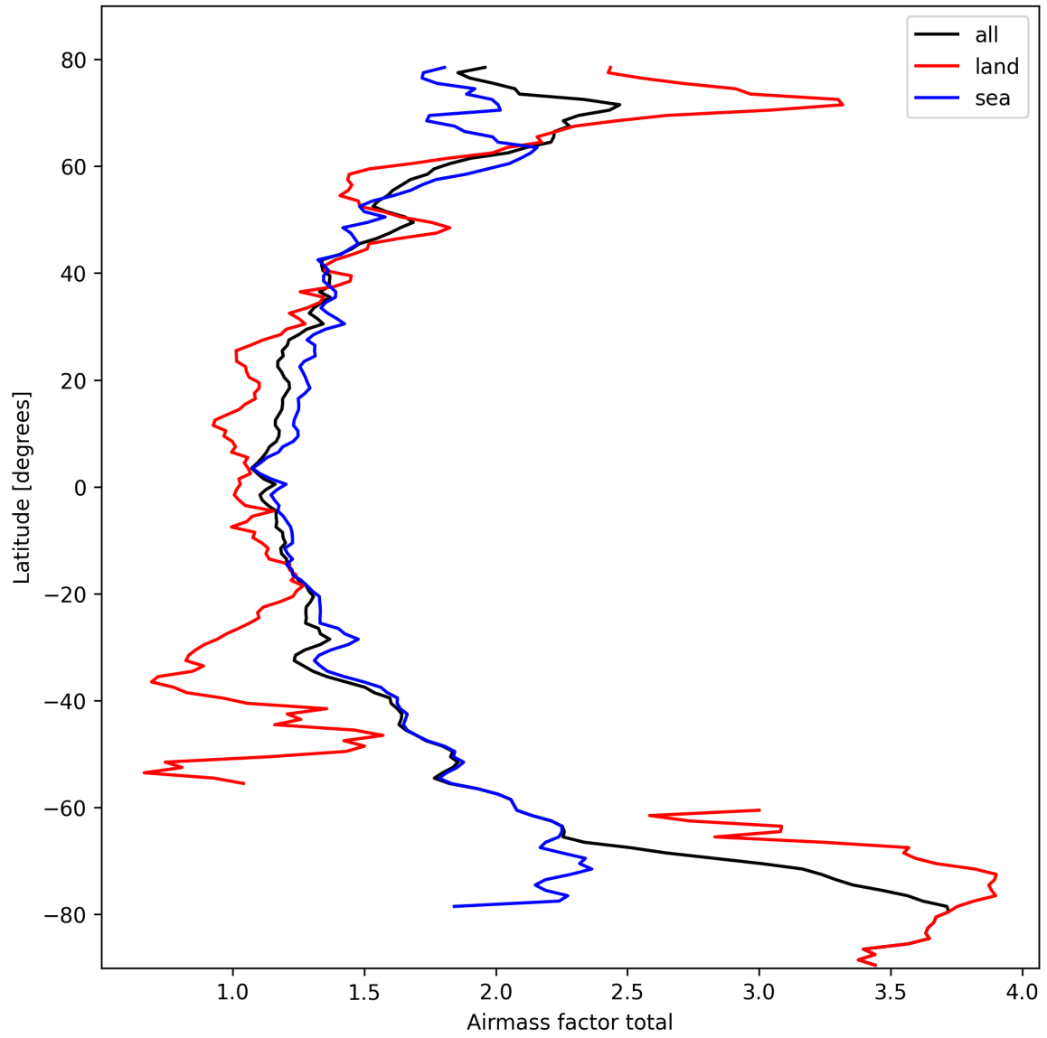
Figure 24: Zonal average of “Airmass factor total” for 2025-03-04 to 2025-03-04.
