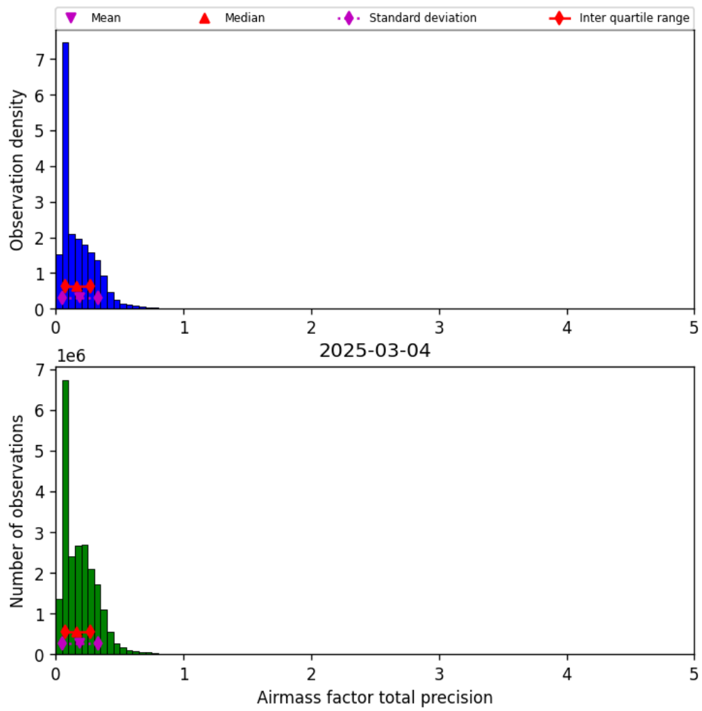
Figure 39: Histogram of “Airmass factor total precision” for 2025-03-04 to 2025-03-04
