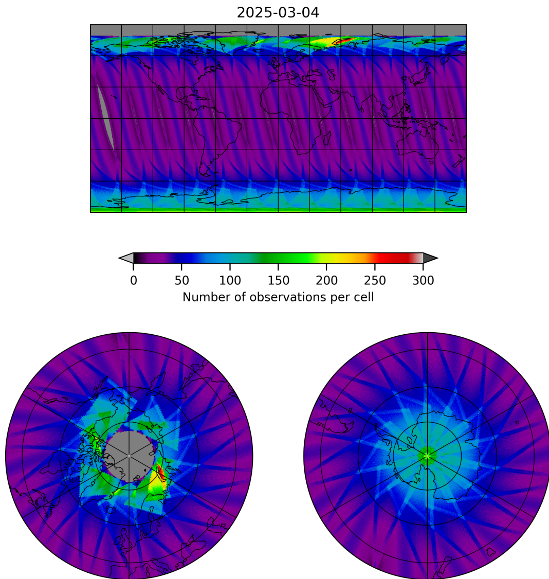
Figure 17: Map of the number of observations for 2025-03-04 to 2025-03-04
