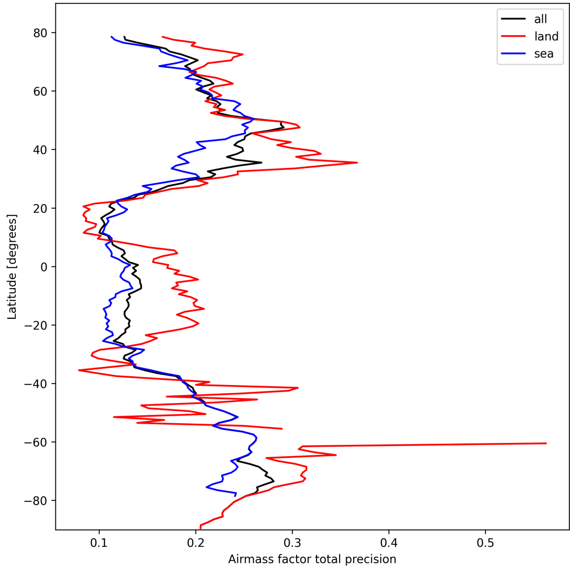
Figure 25: Zonal average of “Airmass factor total precision” for 2025-03-04 to 2025-03-04.
