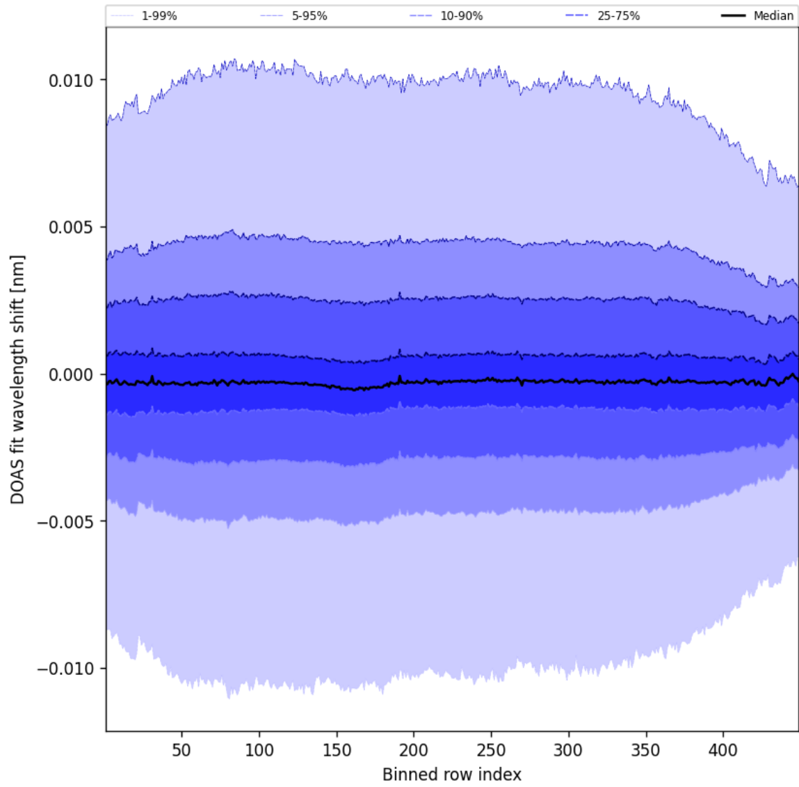
Figure 56: Along track statistics of "DOAS fit wavelength shift" for 2025-03-04 to 2025-03-04
