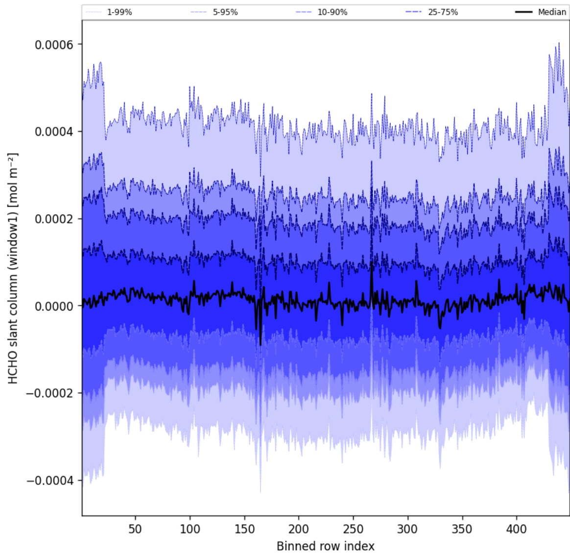
Figure 50: Along track statistics of “HCHO slant column (window1)” for 2025-03-04 to 2025-03-04
