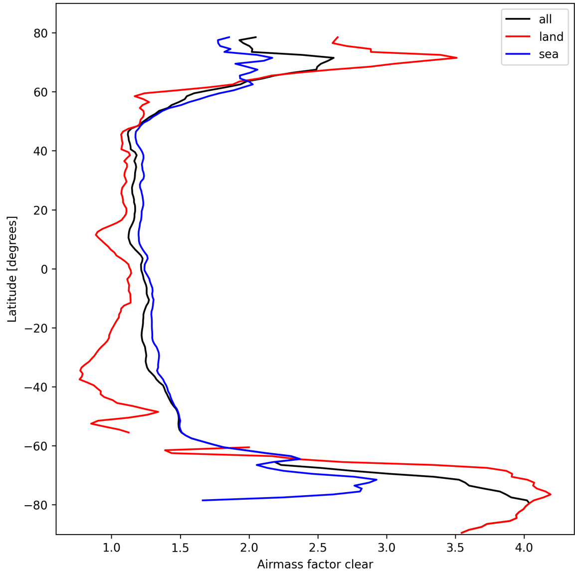
Figure 26: Zonal average of “Airmass factor clear” for 2025-03-04 to 2025-03-04.
