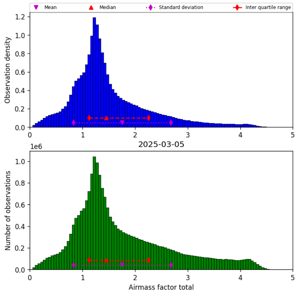
Figure 38: Histogram of “Airmass factor total” for 2025-03-05 to 2025-03-05
