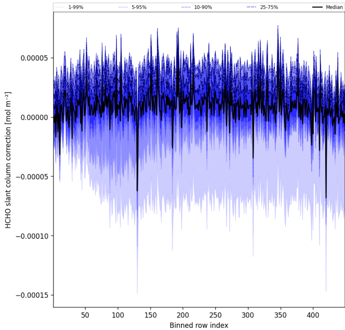
Figure 59: Along track statistics of “HCHO slant column correction” for 2025-03-05 to 2025-03-05
