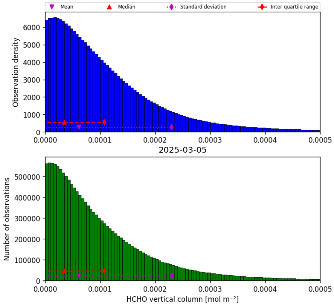
Figure 33: Histogram of “HCHO vertical column” for 2025-03-05 to 2025-03-05
