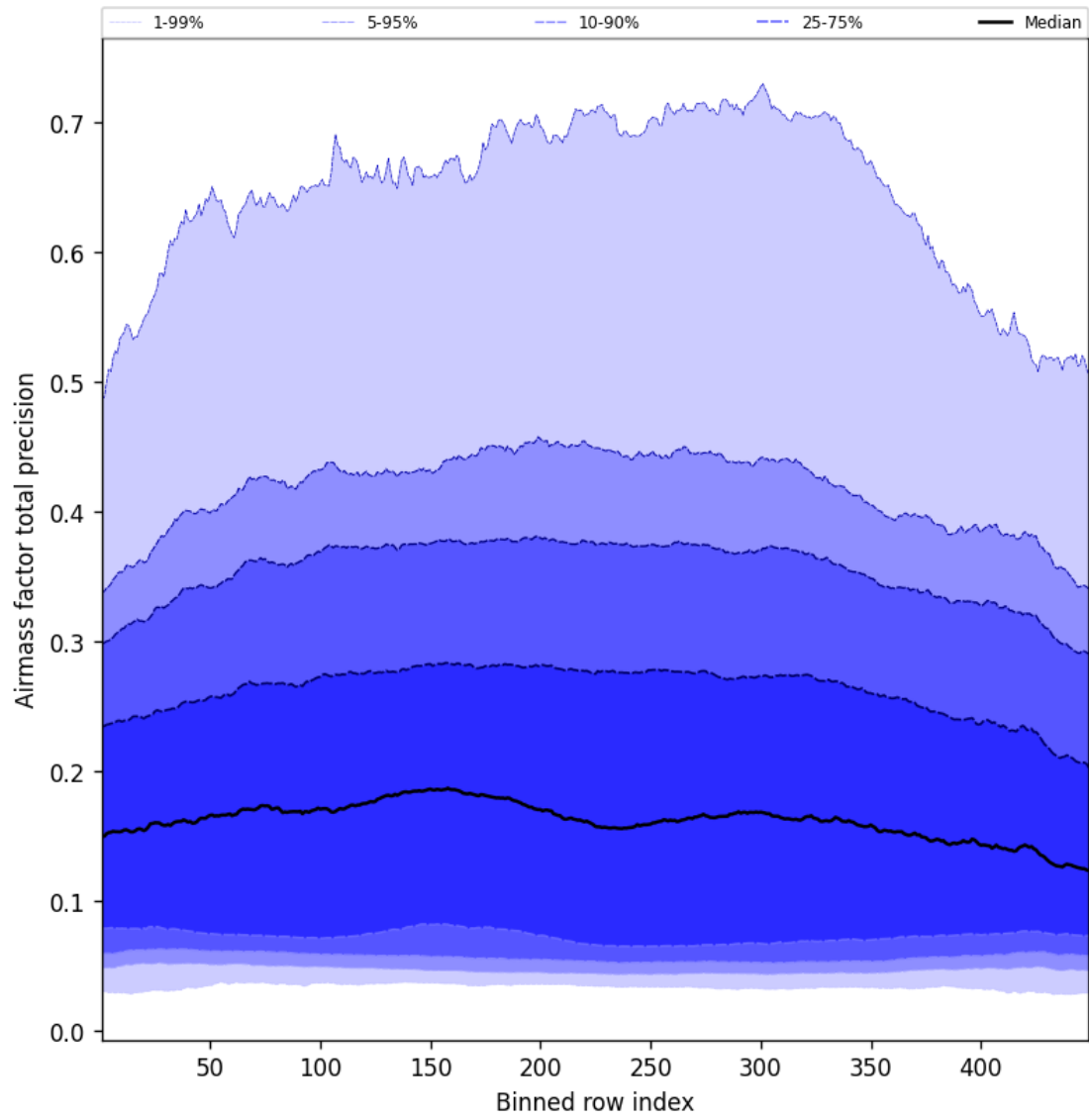
Figure 53: Along track statistics of “Airmass factor total precision” for 2025-03-05 to 2025-03-05
