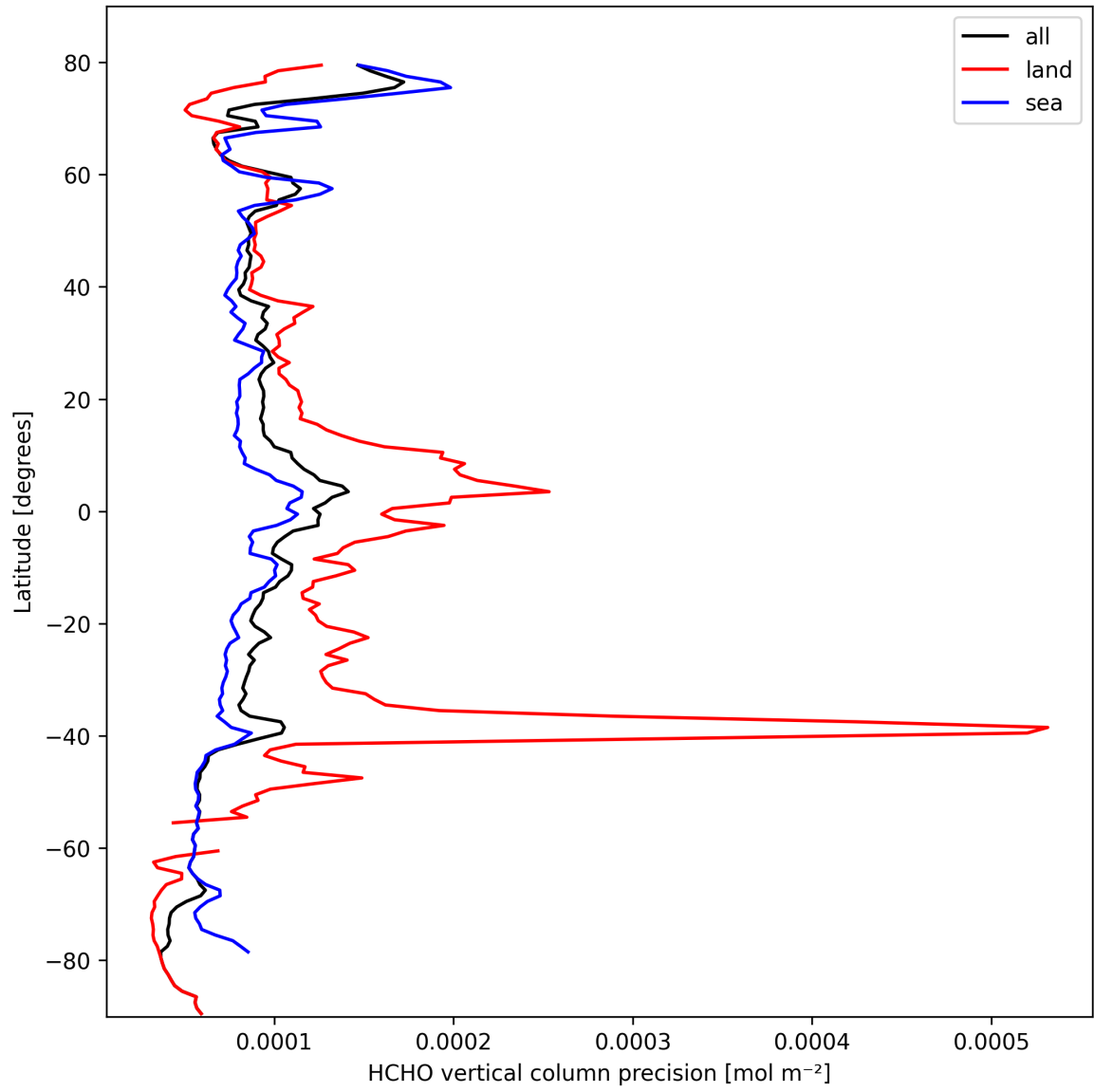
Figure 20: Zonal average of “HCHO vertical column precision” for 2025-03-05 to 2025-03-05.
