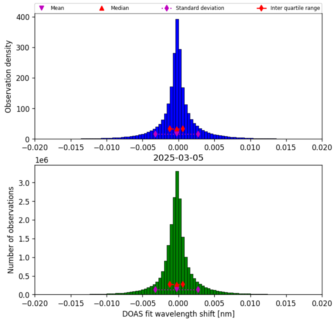
Figure 42: Histogram of “DOAS fit wavelength shift” for 2025-03-05 to 2025-03-05
