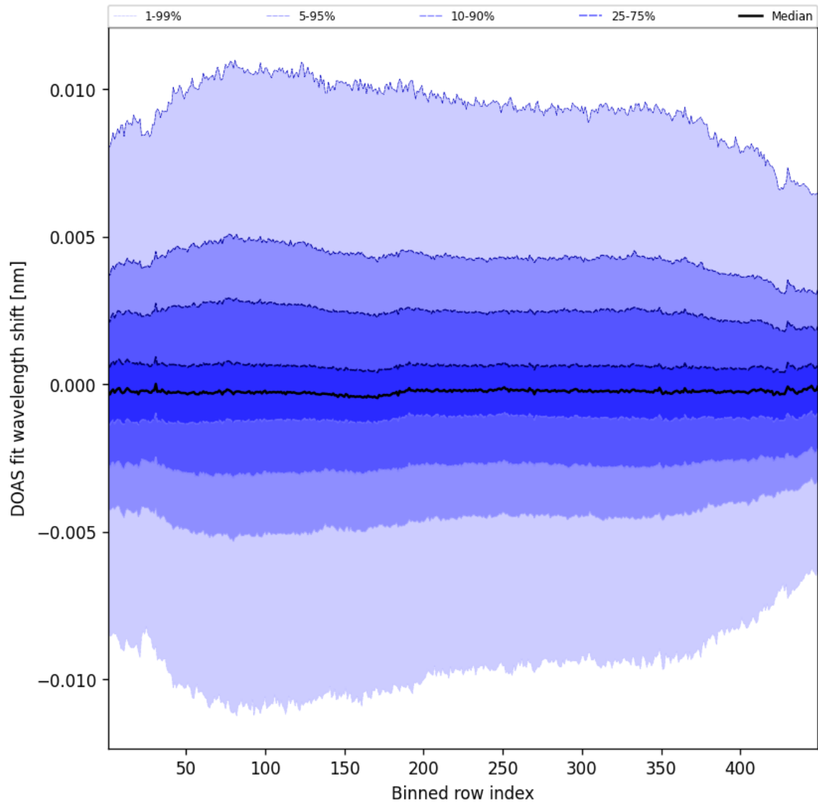
Figure 56: Along track statistics of “DOAS fit wavelength shift” for 2025-03-05 to 2025-03-05
