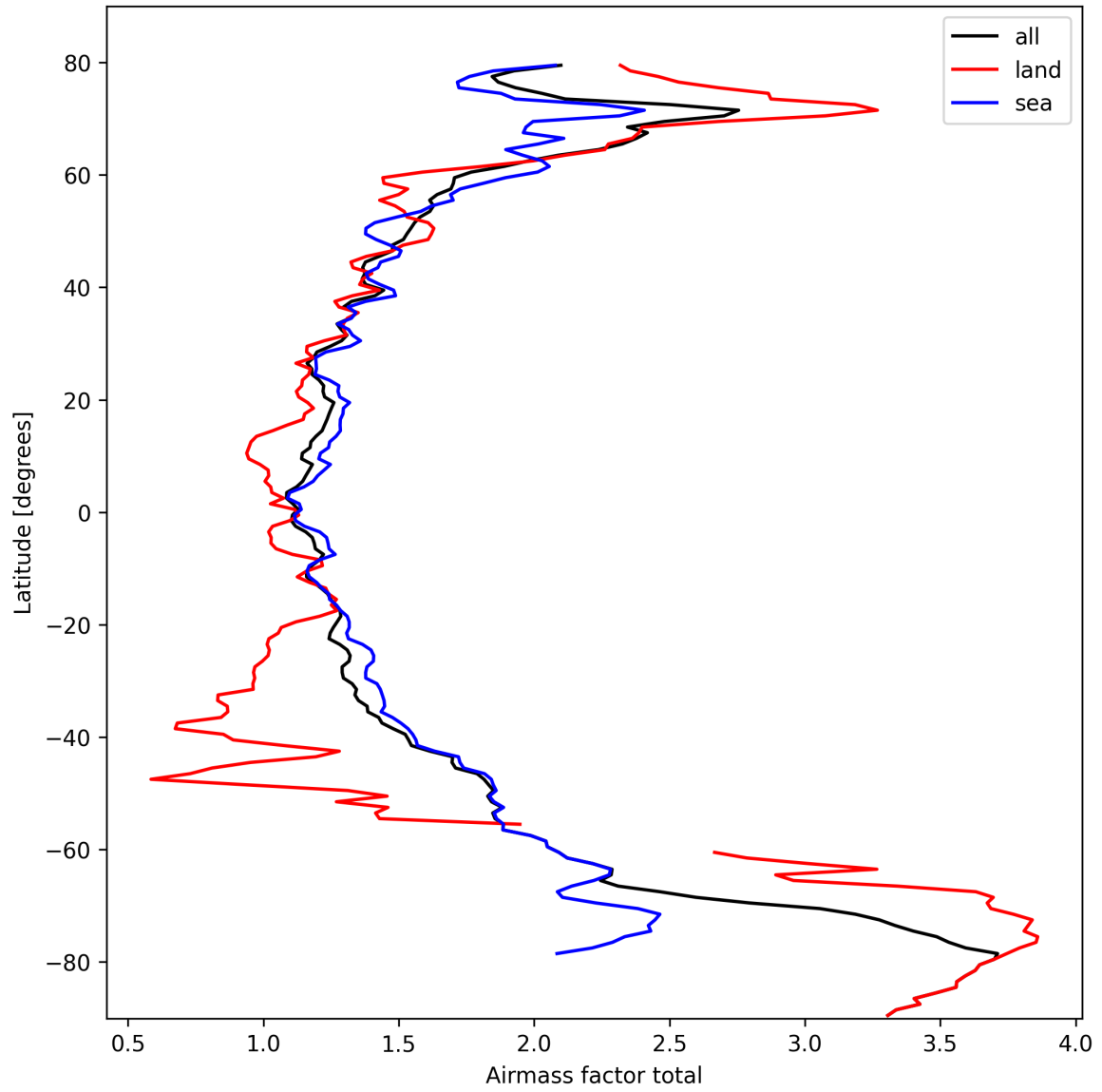
Figure 24: Zonal average of "Airmass factor total" for 2025-03-05 to 2025-03-05.
