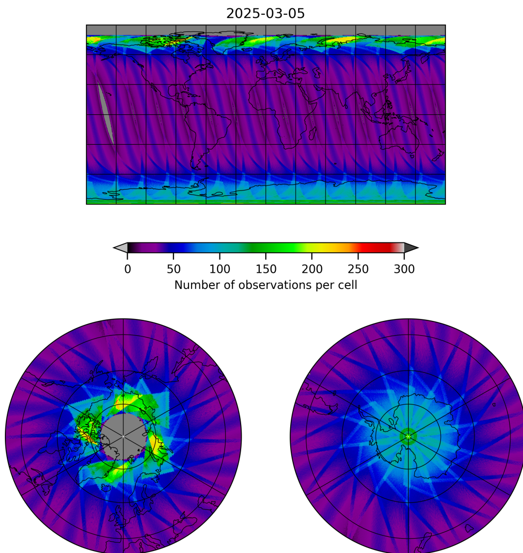
Figure 17: Map of the number of observations for 2025-03-05 to 2025-03-05
