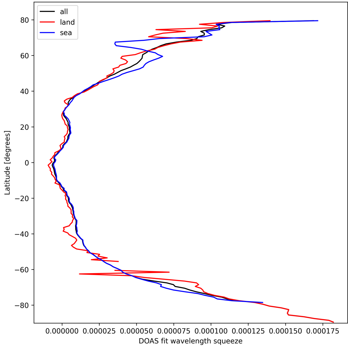
Figure 29: Zonal average of “DOAS fit wavelength squeeze” for 2025-03-05 to 2025-03-05.
