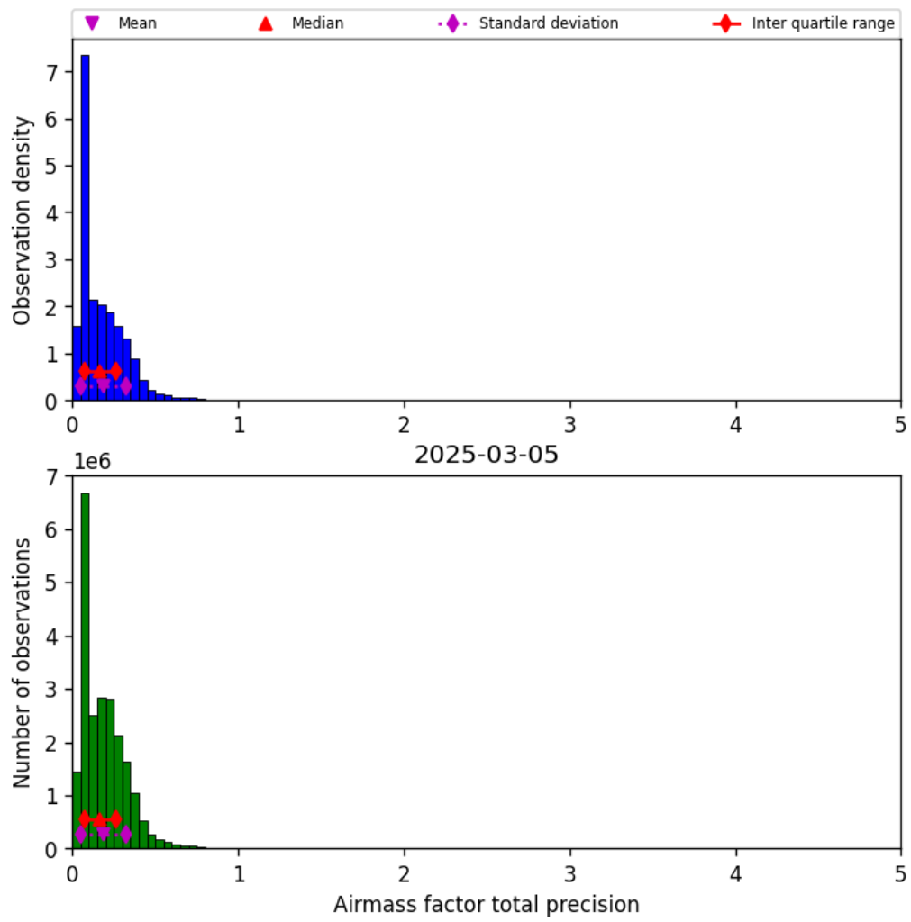
Figure 39: Histogram of “Airmass factor total precision” for 2025-03-05 to 2025-03-05
