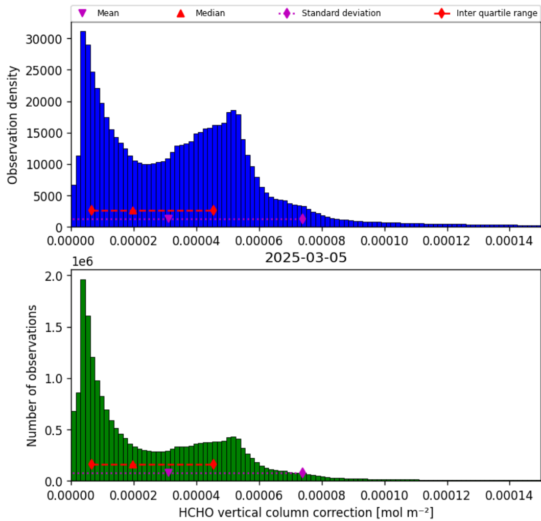
Figure 35: Histogram of “HCHO vertical column correction” for 2025-03-05 to 2025-03-05
