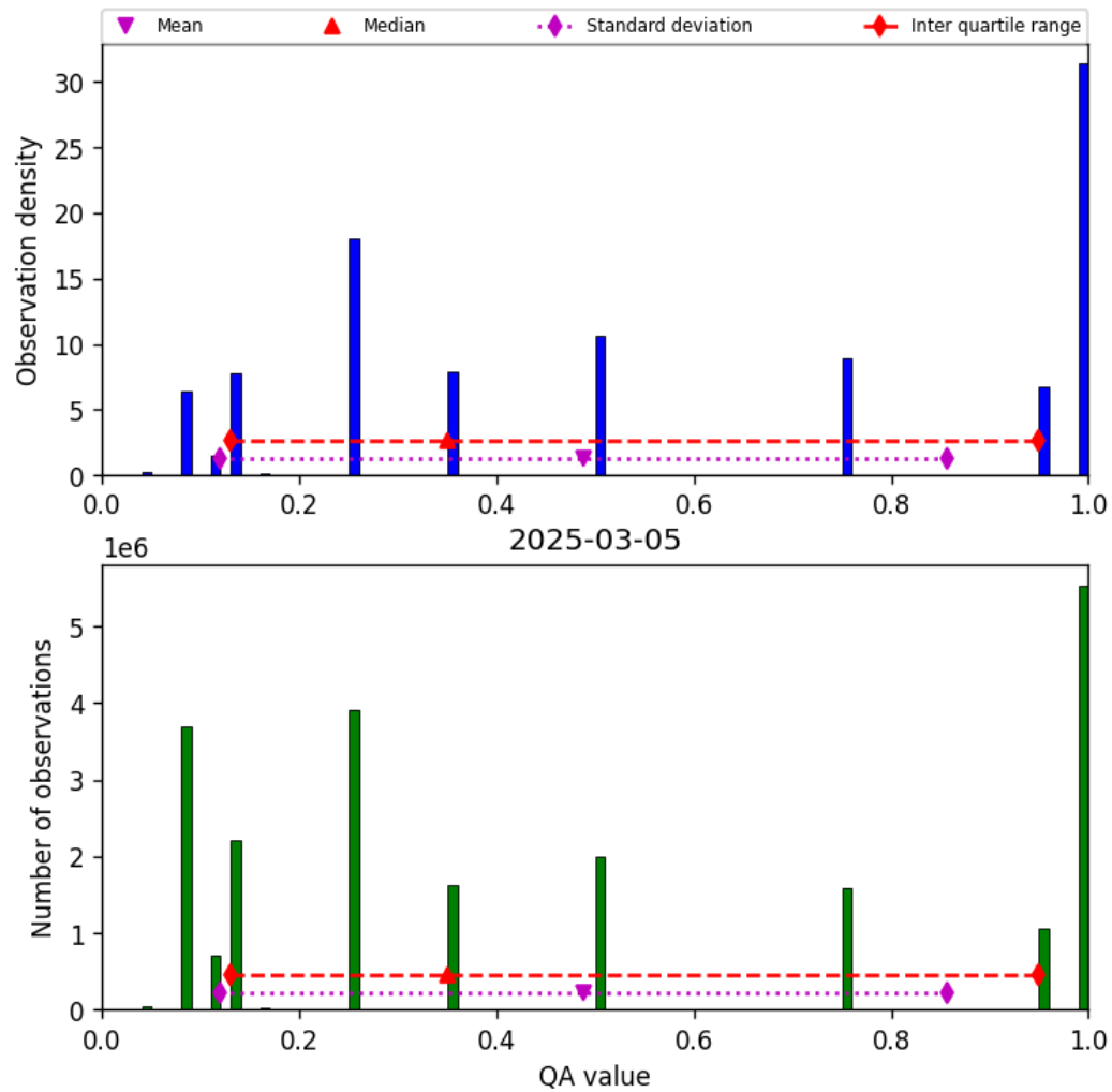
Figure 32: Histogram of “QA value” for 2025-03-05 to 2025-03-05
