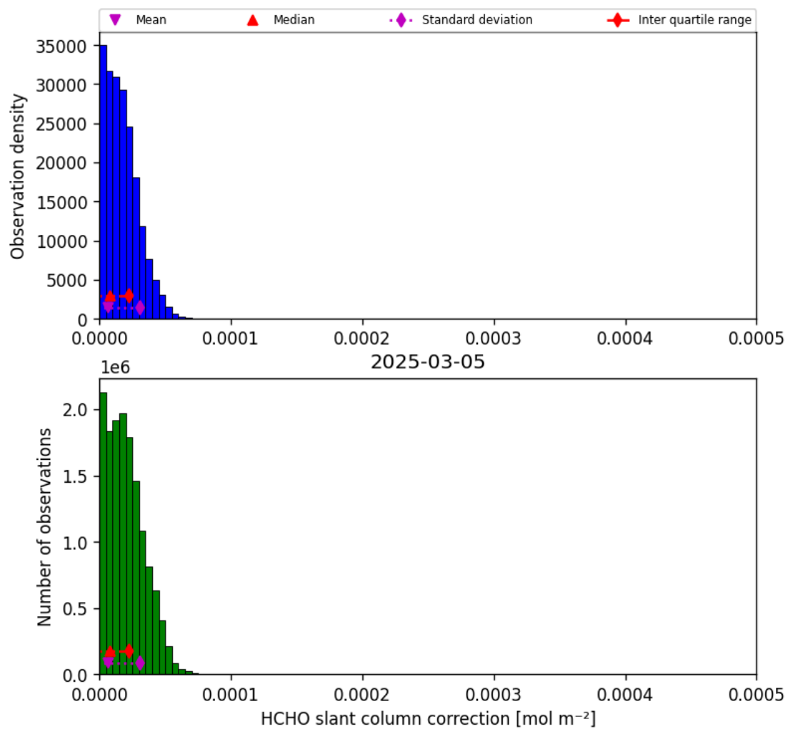
Figure 45: Histogram of “HCHO slant column correction” for 2025-03-05 to 2025-03-05
