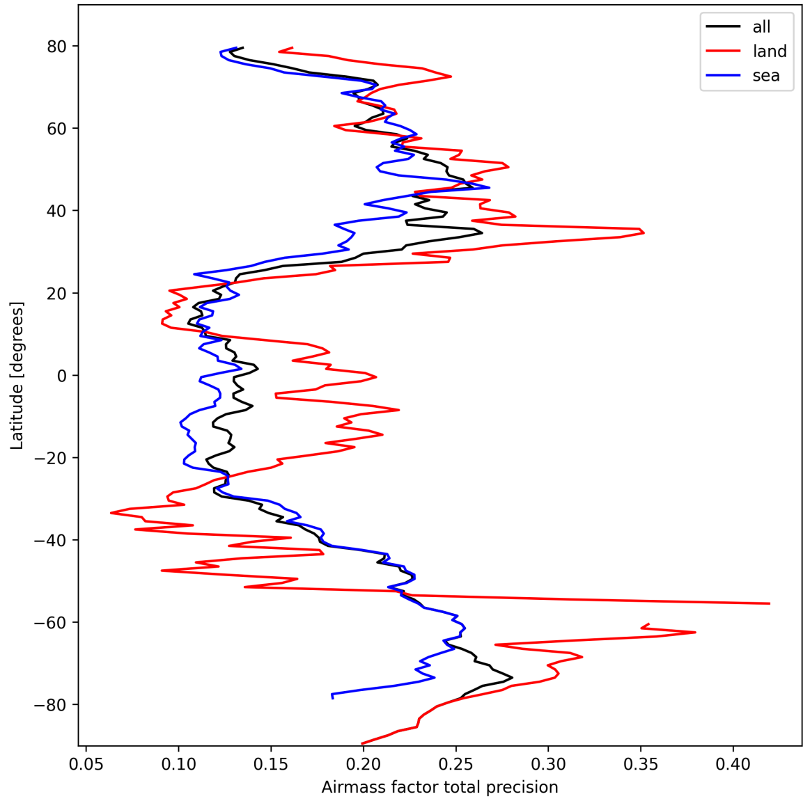
Figure 25: Zonal average of “Airmass factor total precision” for 2025-03-05 to 2025-03-05.
