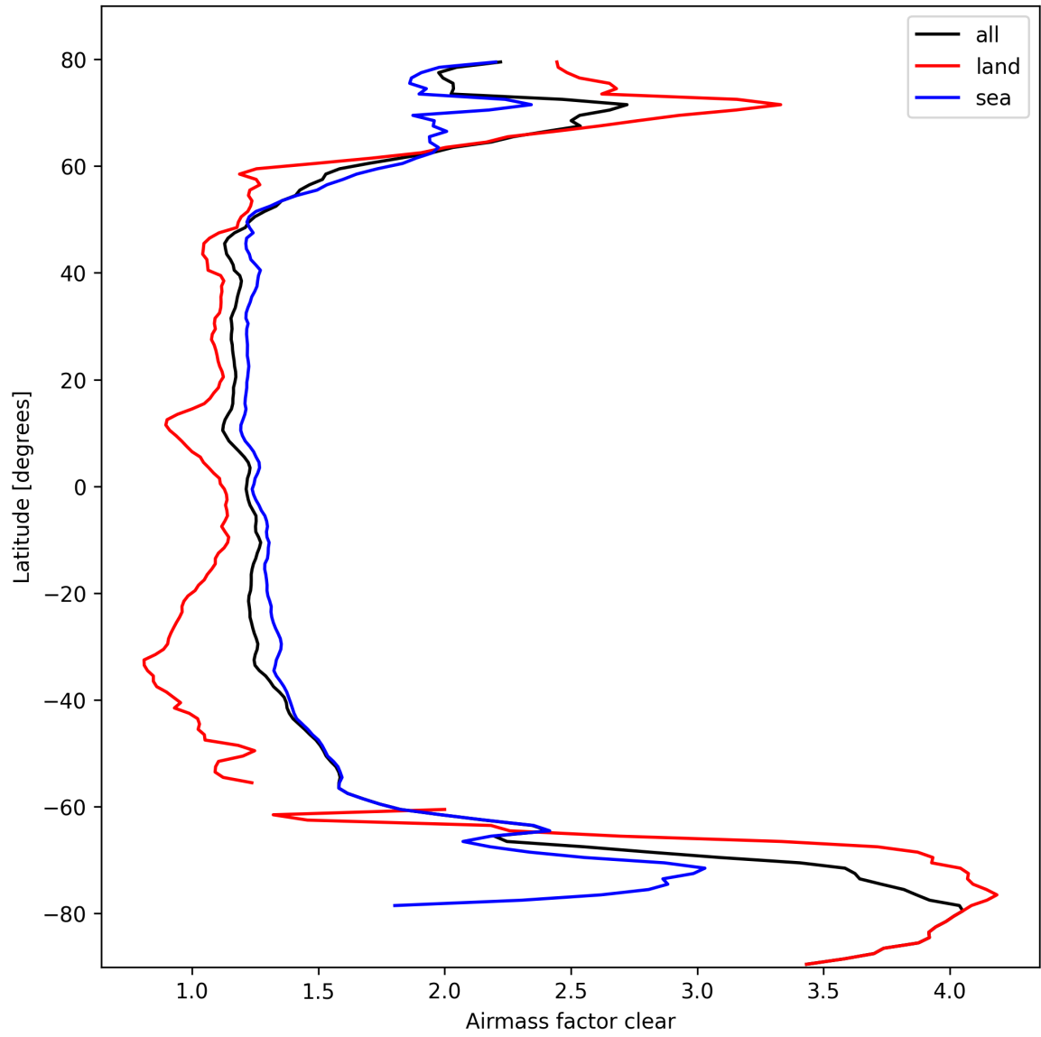
Figure 26: Zonal average of “Airmass factor clear” for 2025-03-05 to 2025-03-05.
