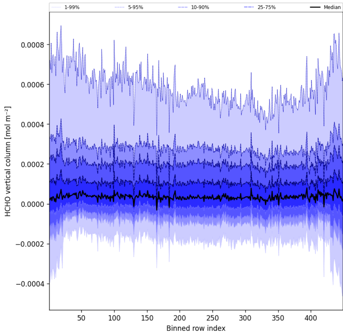
Figure 47: Along track statistics of “HCHO vertical column” for 2025-03-05 to 2025-03-05
