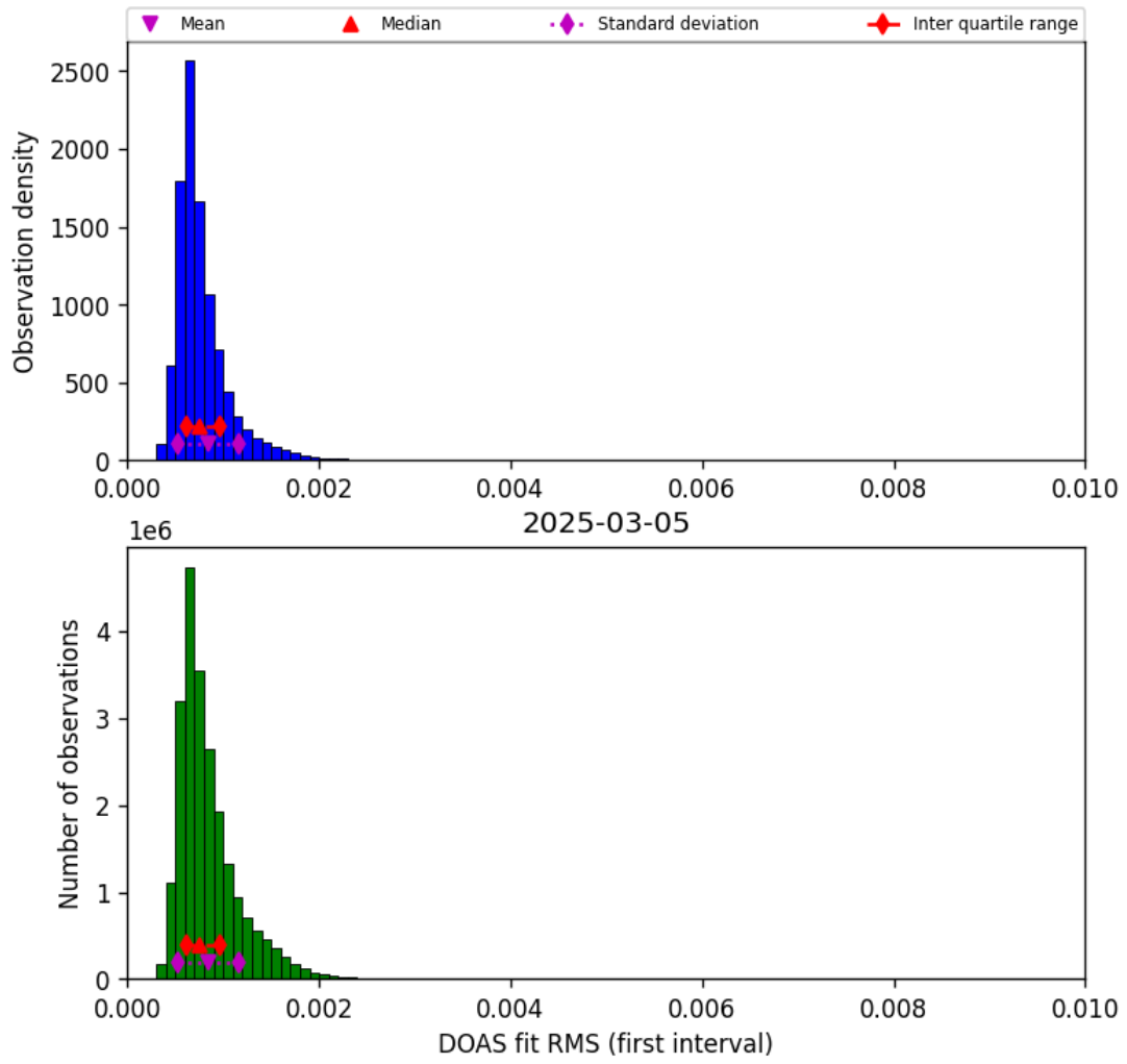
Figure 44: Histogram of “DOAS fit RMS (first interval)” for 2025-03-05 to 2025-03-05
