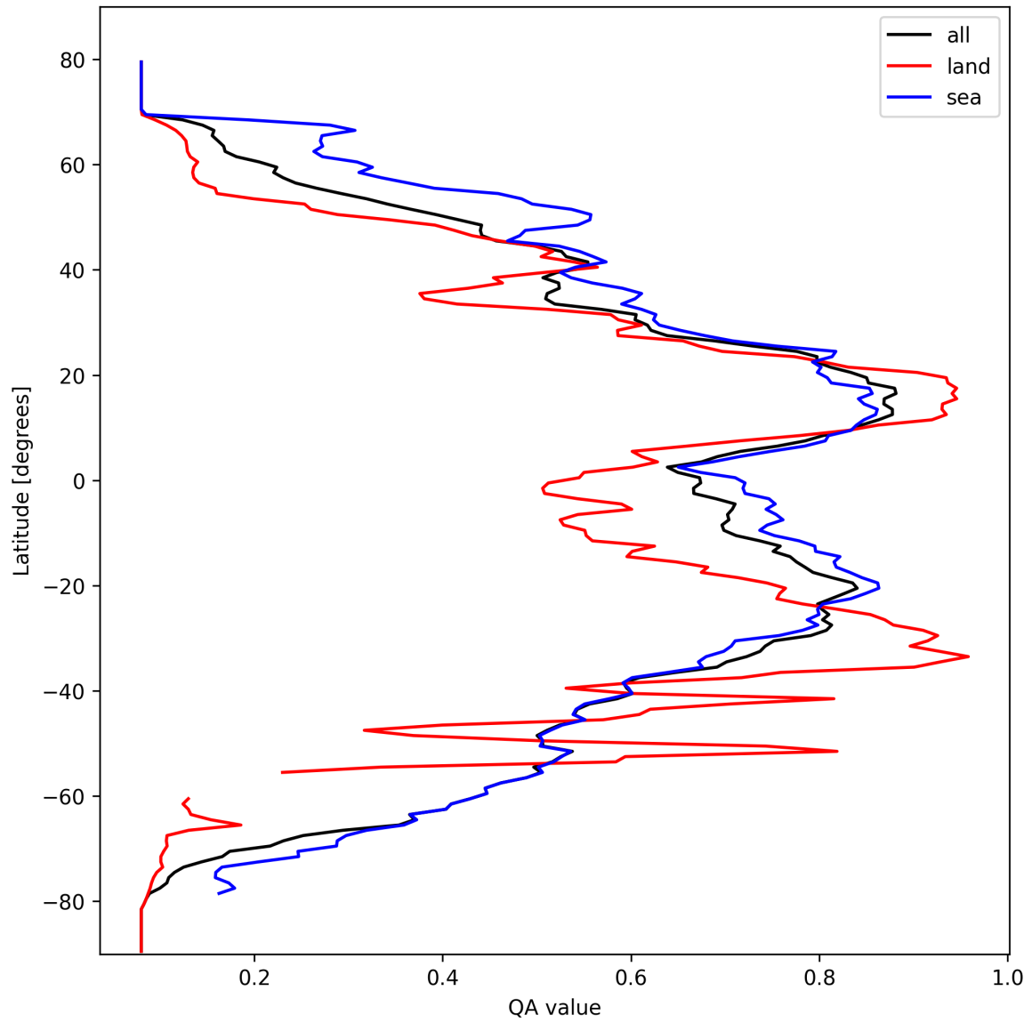
Figure 18: Zonal average of “QA value” for 2025-03-05 to 2025-03-05.
