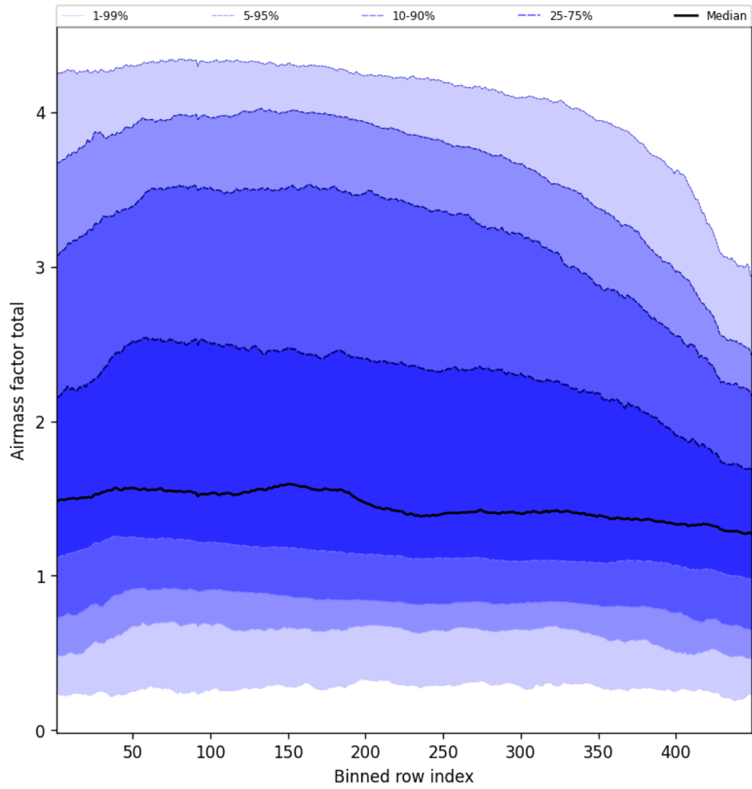
Figure 52: Along track statistics of “Airmass factor total” for 2025-03-05 to 2025-03-05
