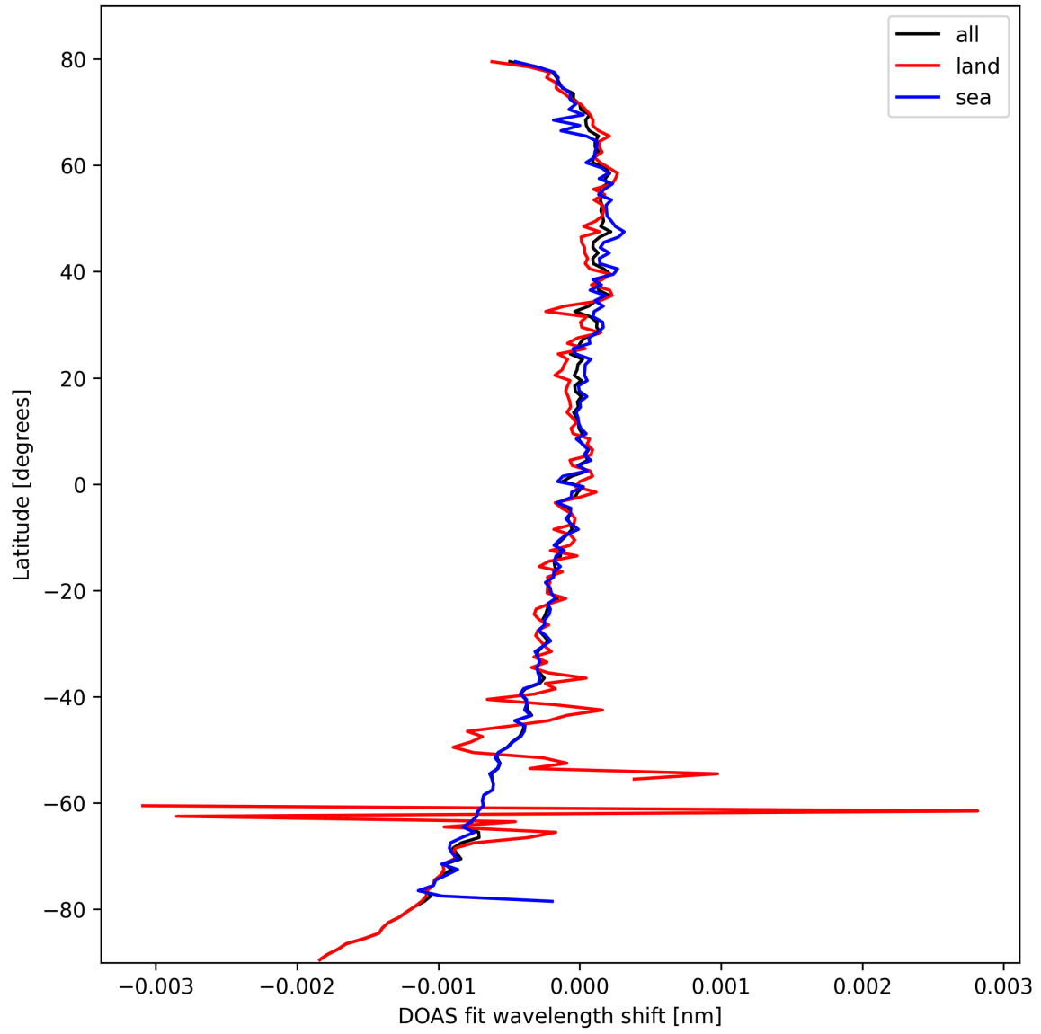
Figure 28: Zonal average of “DOAS fit wavelength shift” for 2025-03-05 to 2025-03-05.
