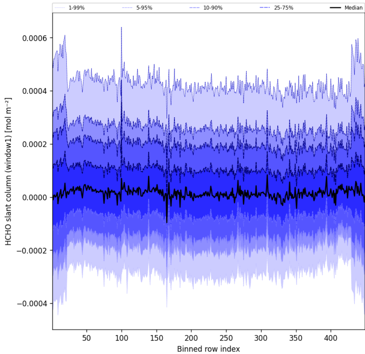
Figure 50: Along track statistics of “HCHO slant column (window1)” for 2025-03-05 to 2025-03-05
