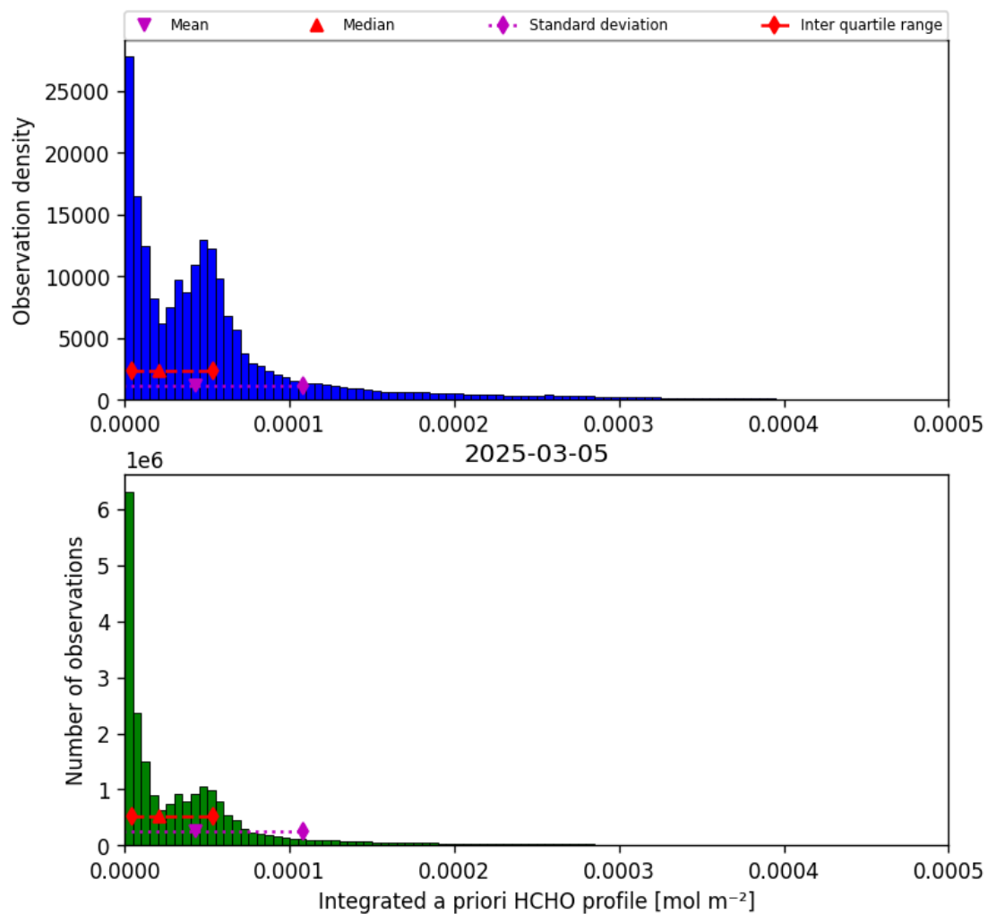
Figure 41: Histogram of “Integrated a priori HCHO profile” for 2025-03-05 to 2025-03-05
