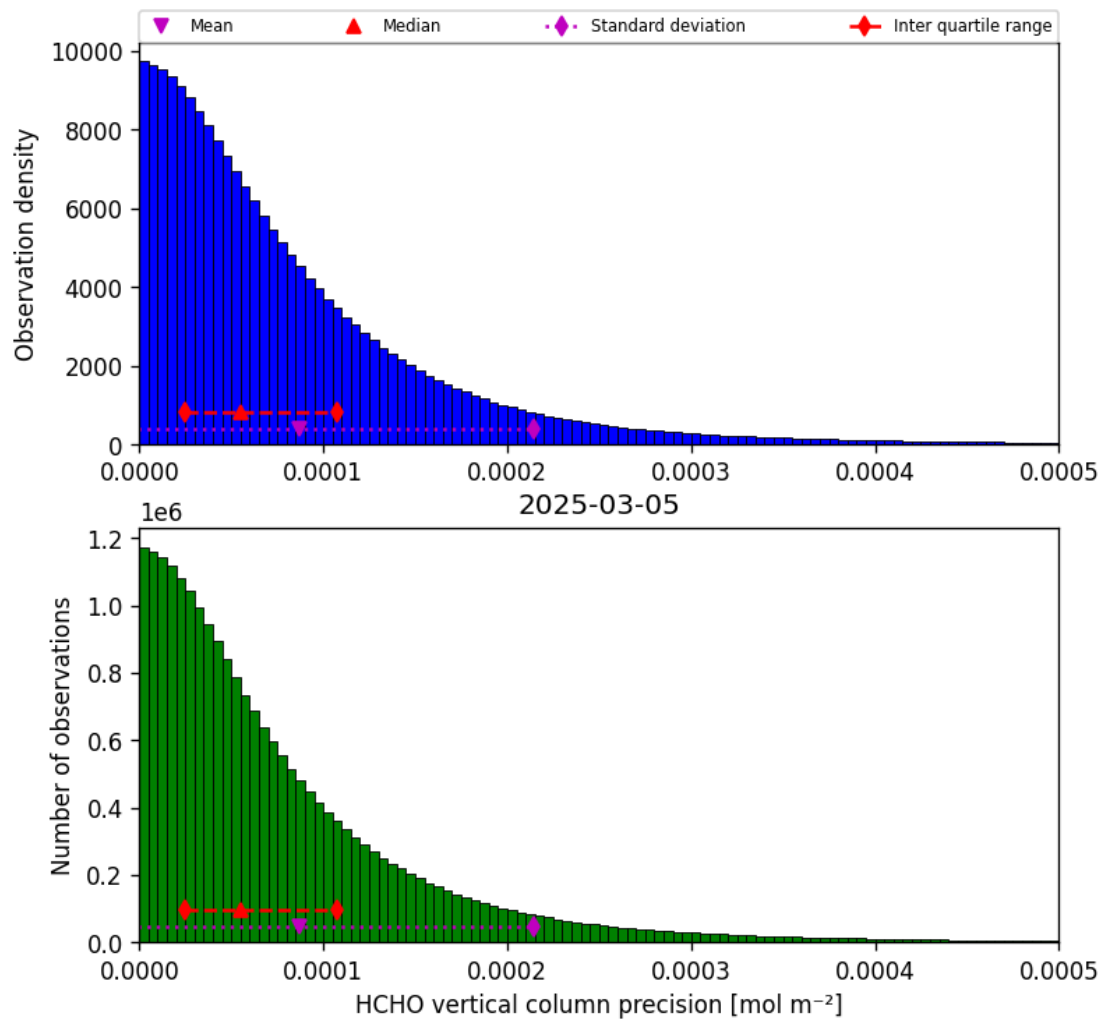
Figure 34: Histogram of “HCHO vertical column precision” for 2025-03-05 to 2025-03-05
