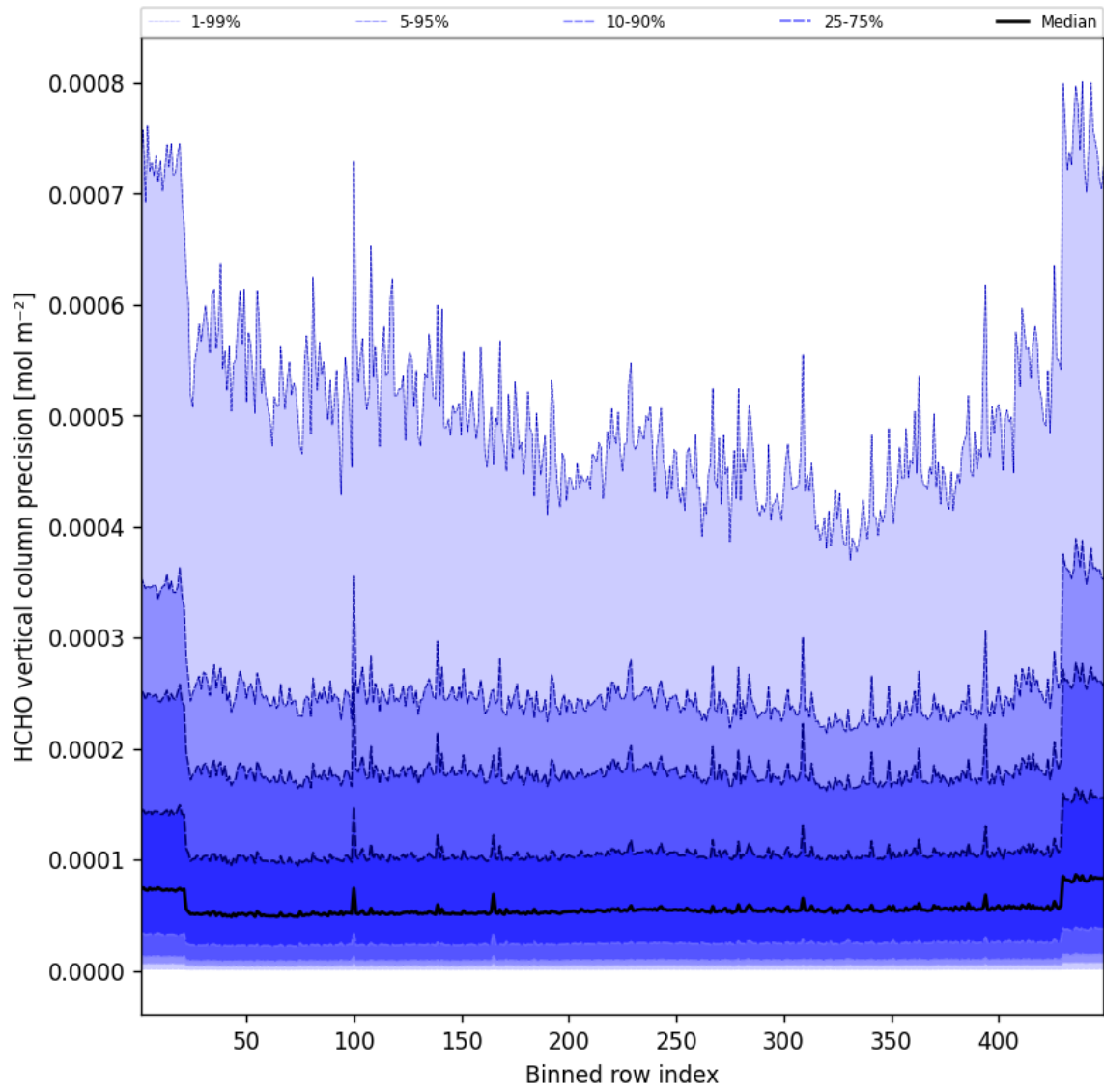
Figure 48: Along track statistics of “HCHO vertical column precision” for 2025-03-05 to 2025-03-05
