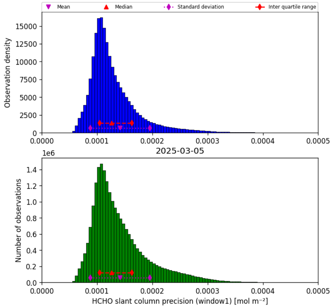
Figure 37: Histogram of “HCHO slant column precision (window1)” for 2025-03-05 to 2025-03-05
