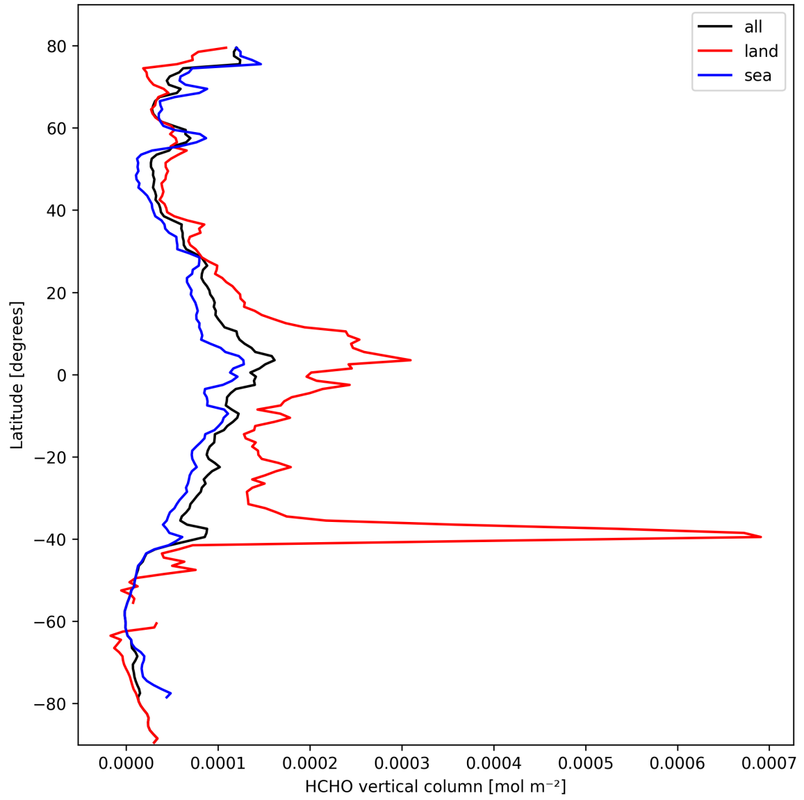
Figure 19: Zonal average of “HCHO vertical column” for 2025-03-05 to 2025-03-05.
