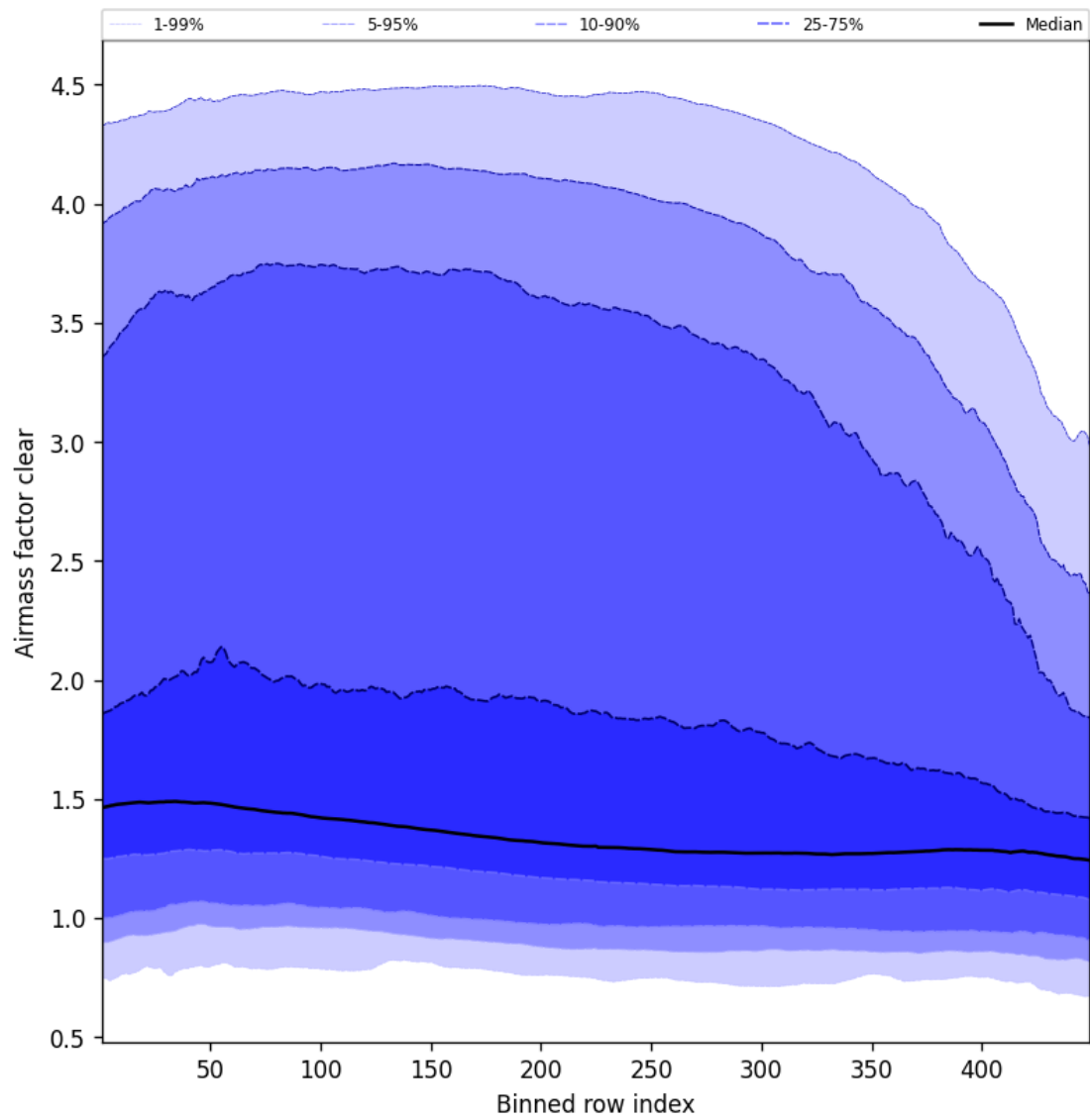
Figure 54: Along track statistics of “Air mass factor clear” for 2025-03-05 to 2025-03-05
