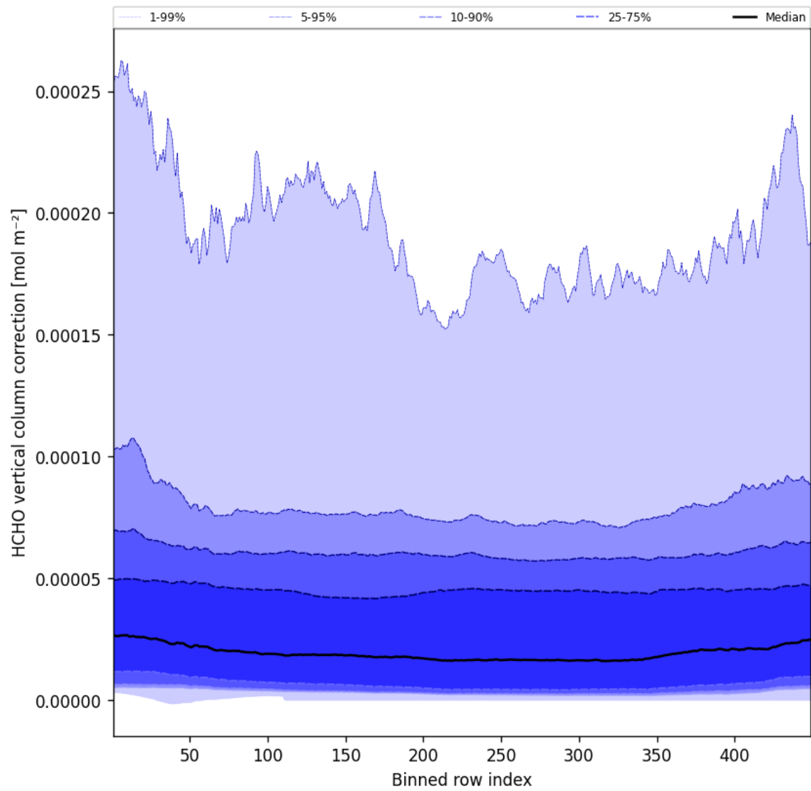
Figure 49: Along track statistics of “HCHO vertical column correction” for 2025-03-05 to 2025-03-05
