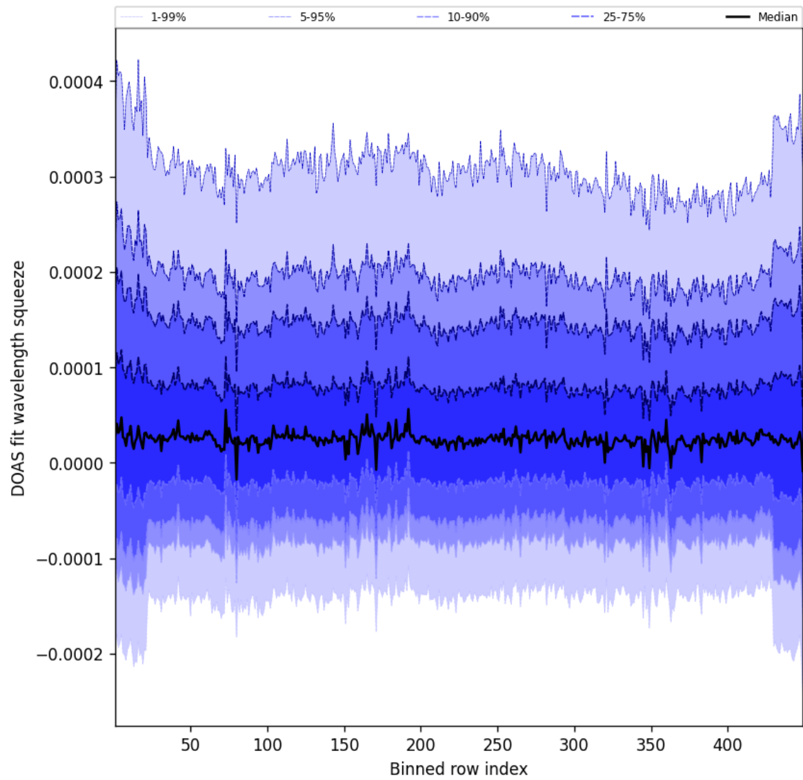
Figure 57: Along track statistics of “DOAS fit wavelength squeeze” for 2025-03-05 to 2025-03-05
