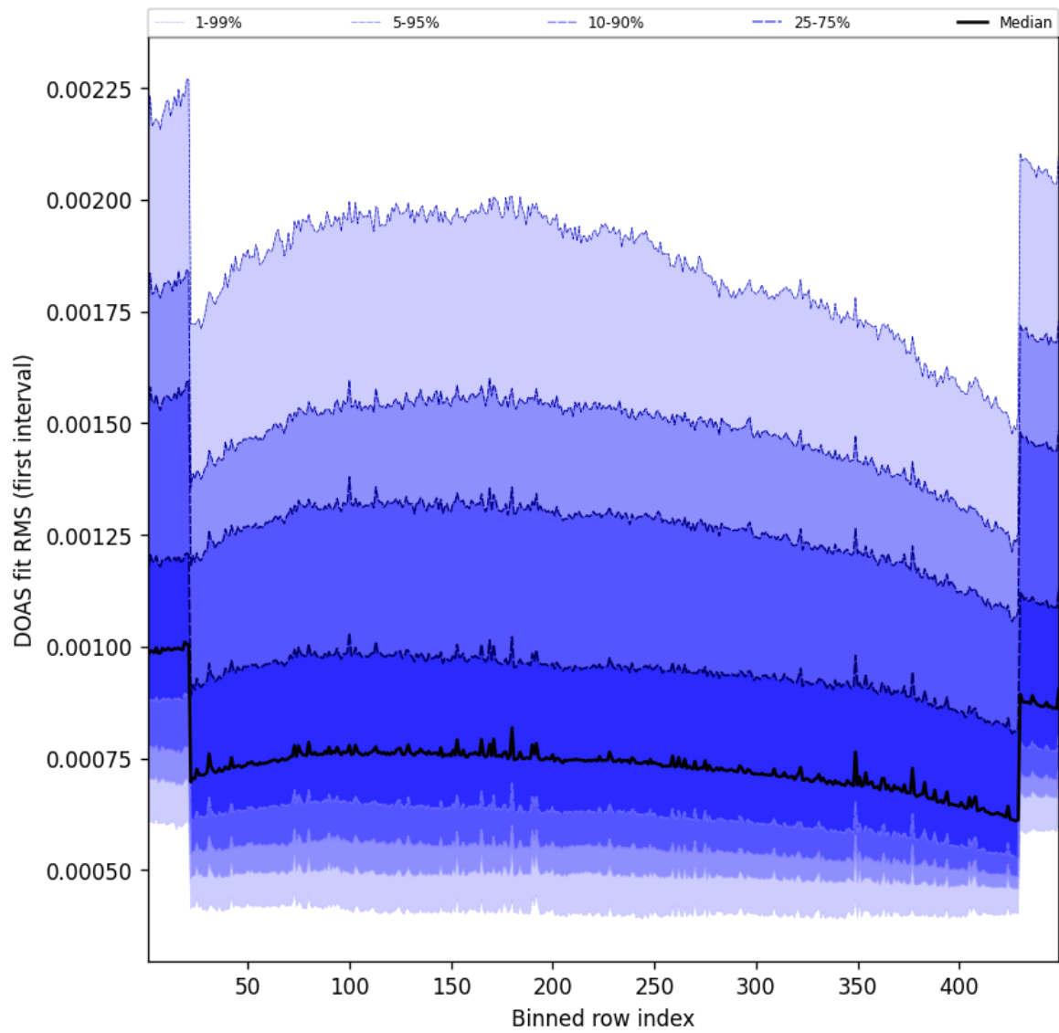
Figure 58: Along track statistics of “DOAS fit RMS (first interval)” for 2025-03-05 to 2025-03-05
