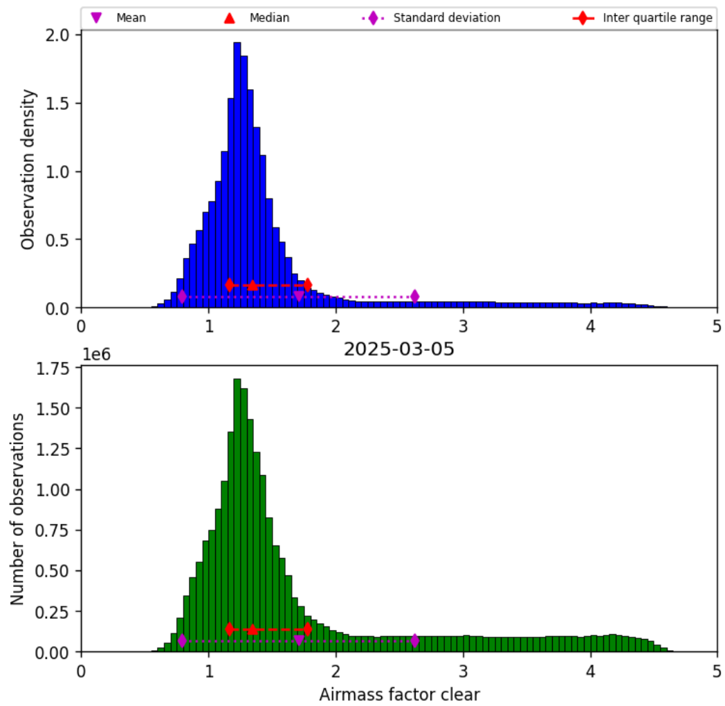
Figure 40: Histogram of “Airmass factor clear” for 2025-03-05 to 2025-03-05
