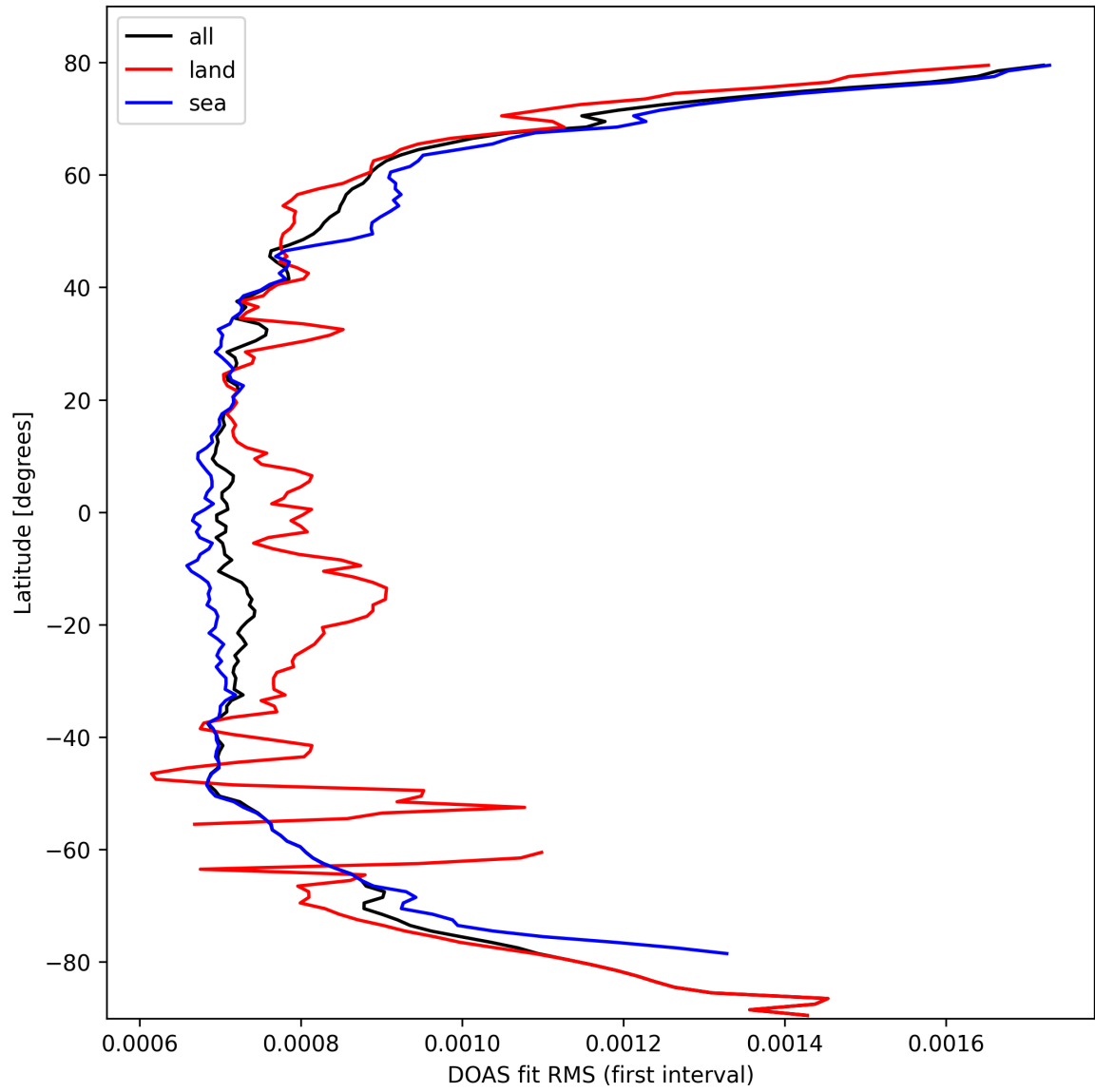
Figure 30: Zonal average of “DOAS fit RMS (first interval)” for 2025-03-05 to 2025-03-05.
