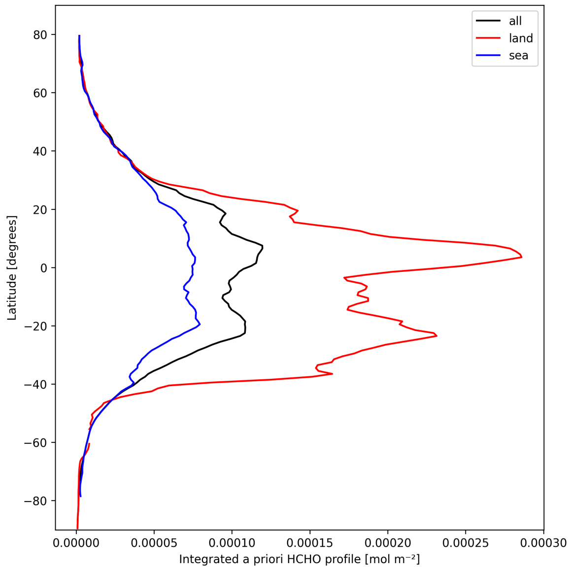
Figure 27: Zonal average of “Integrated a priori HCHO profile” for 2025-03-05 to 2025-03-05.
