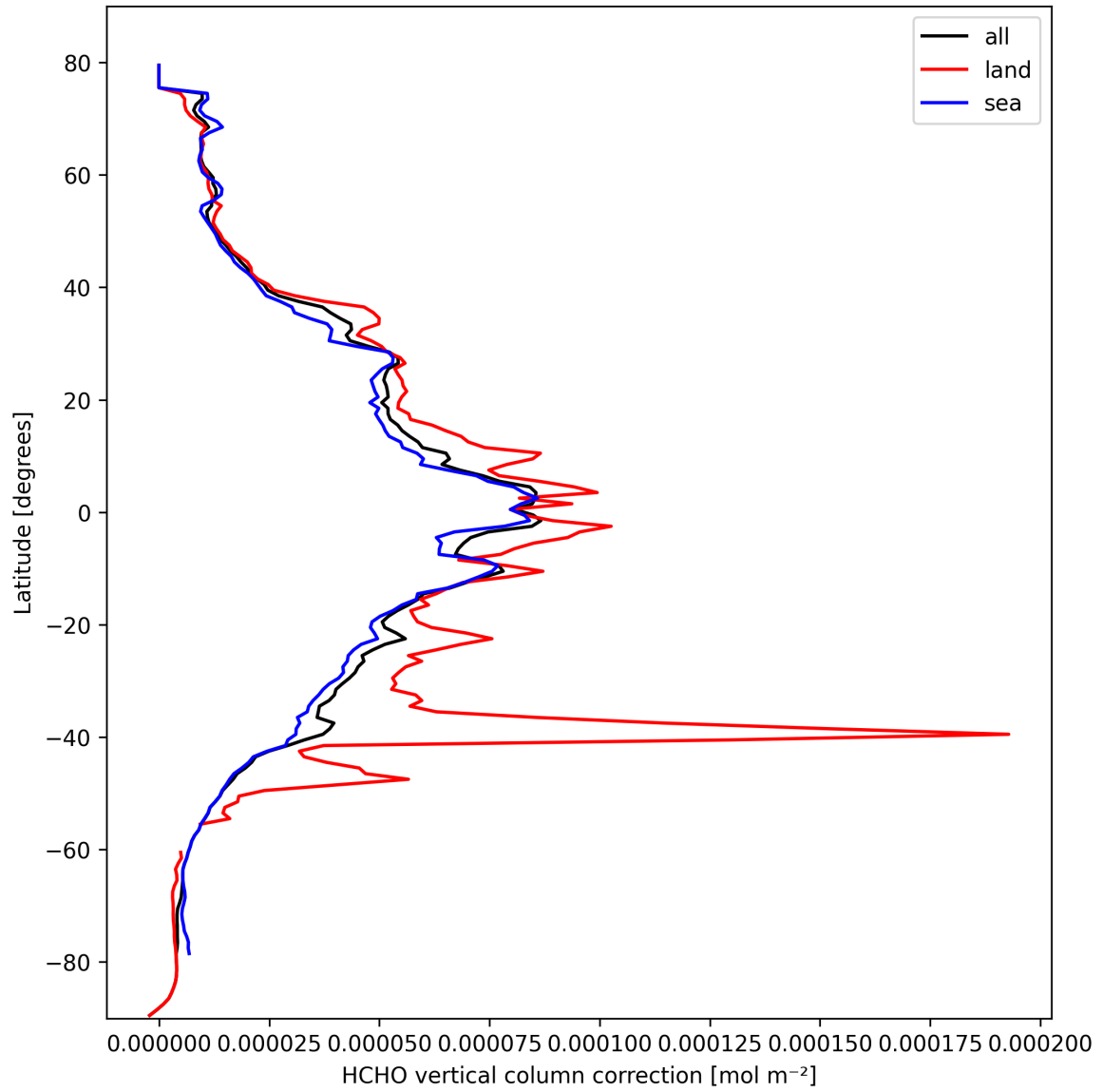
Figure 21: Zonal average of “HCHO vertical column correction” for 2025-03-05 to 2025-03-05.
