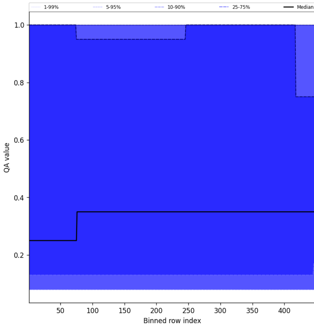
Figure 46: Along track statistics of “QA value” for 2025-03-05 to 2025-03-05
