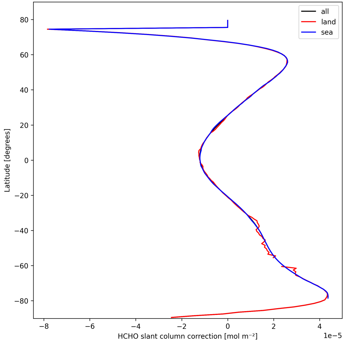
Figure 31: Zonal average of “HCHO slant column correction” for 2025-03-05 to 2025-03-05.
