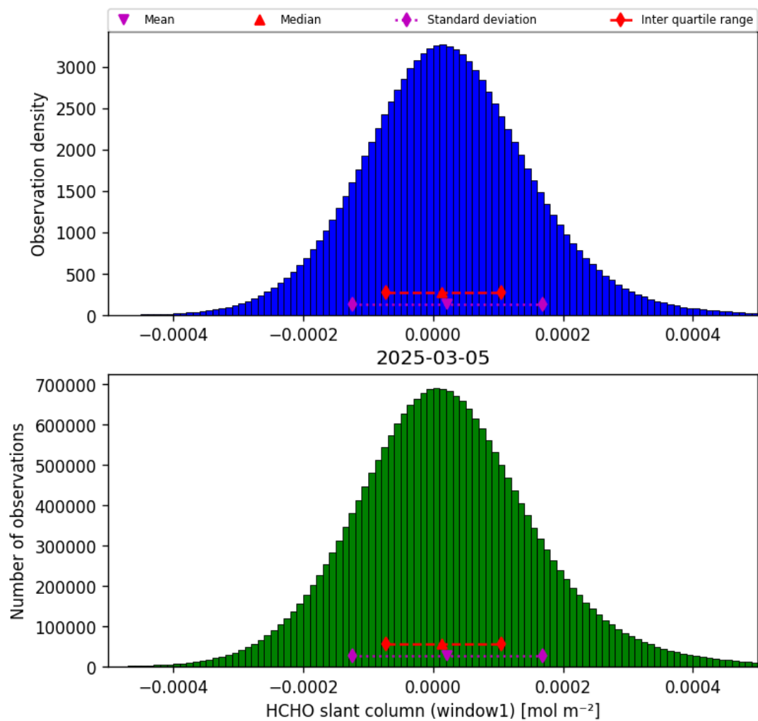
Figure 36: Histogram of “HCHO slant column (window1)” for 2025-03-05 to 2025-03-05
