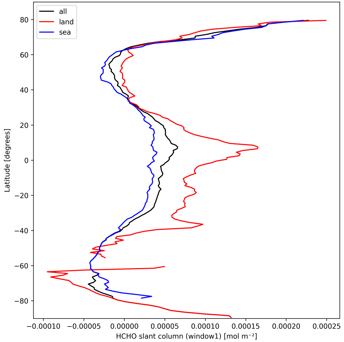
Figure 22: Zonal average of “HCHO slant column (window1)” for 2025-03-05 to 2025-03-05.
