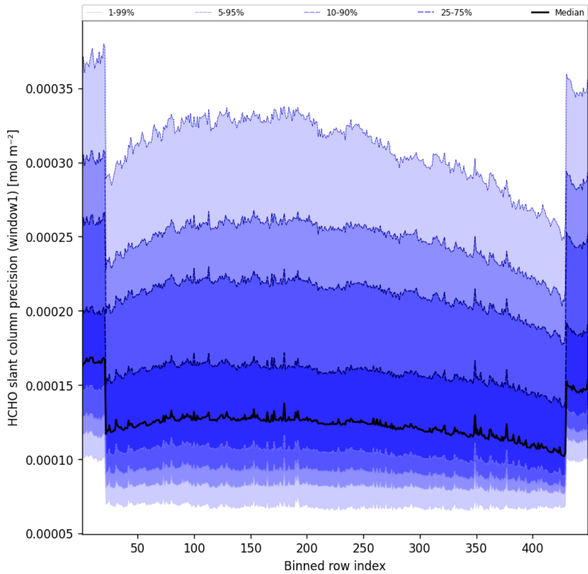
Figure 51: Along track statistics of “HCHO slant column precision (window1)” for 2025-03-05 to 2025-03-05
