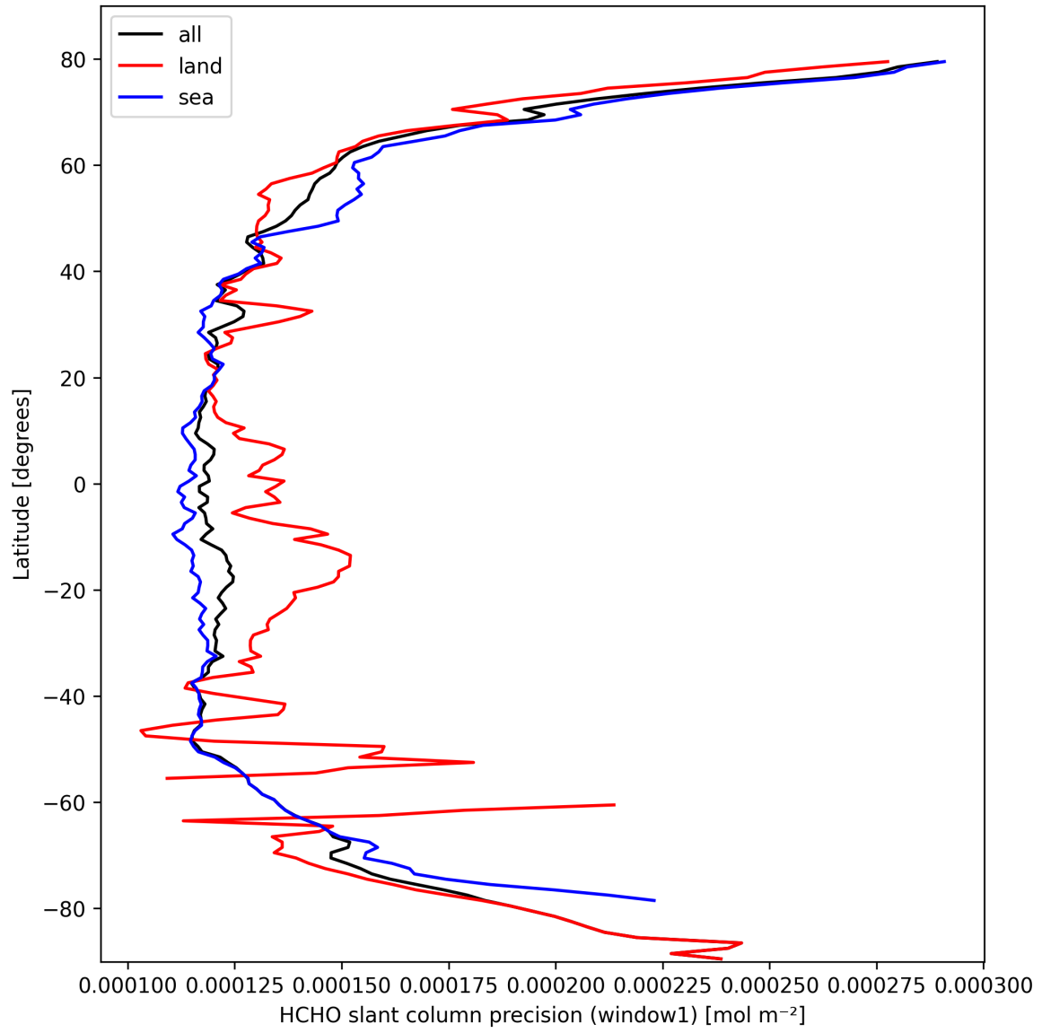
Figure 23: Zonal average of “HCHO slant column precision (window1)” for 2025-03-05 to 2025-03-05.
