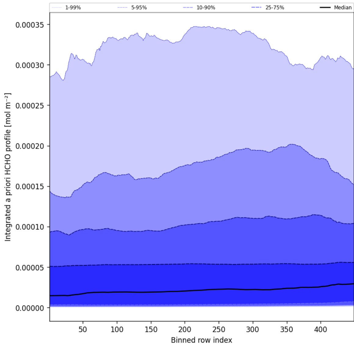
Figure 55: Along track statistics of "Integrated a priori HCHO profile" for 2025-03-05 to 2025-03-05
