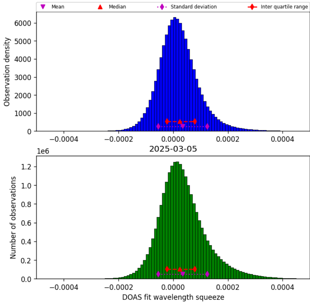
Figure 43: Histogram of “DOAS fit wavelength squeeze” for 2025-03-05 to 2025-03-05
