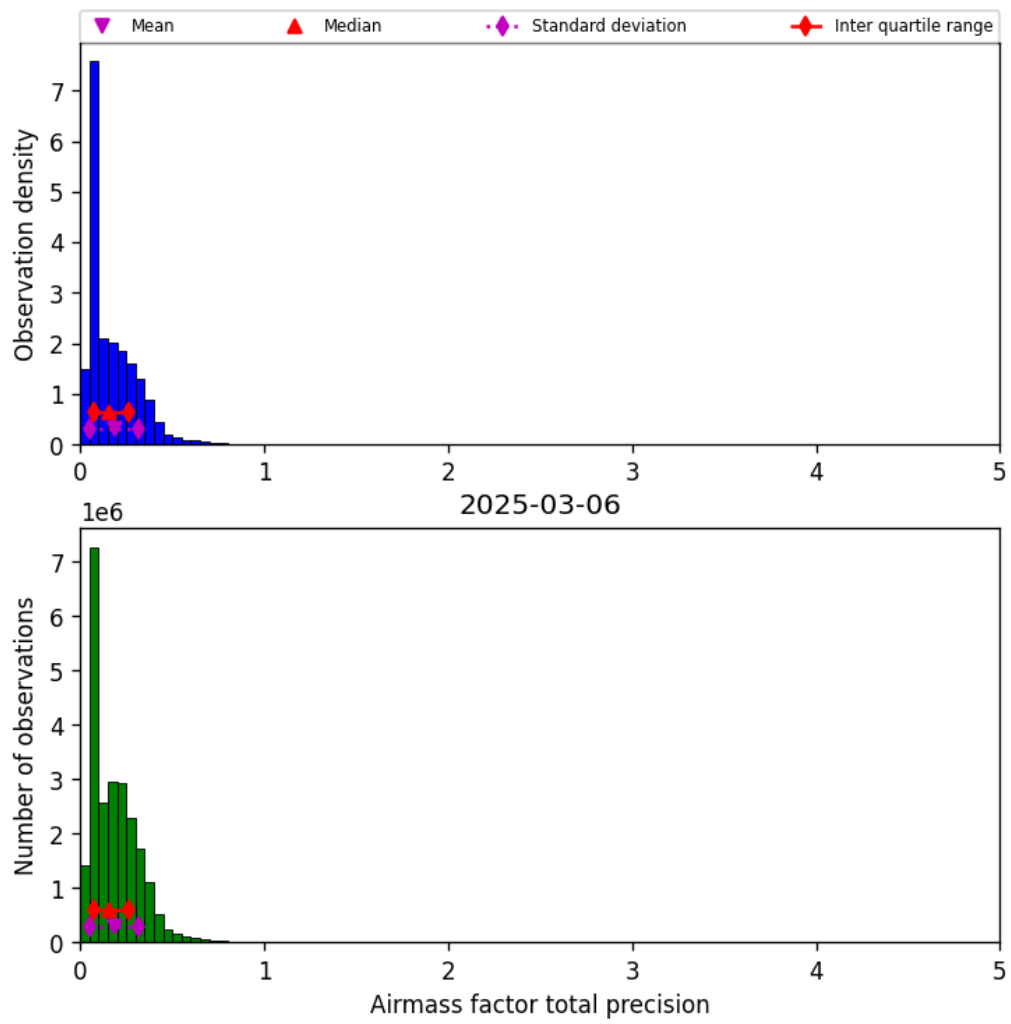
Figure 39: Histogram of “Airmass factor total precision” for 2025-03-06 to 2025-03-07
