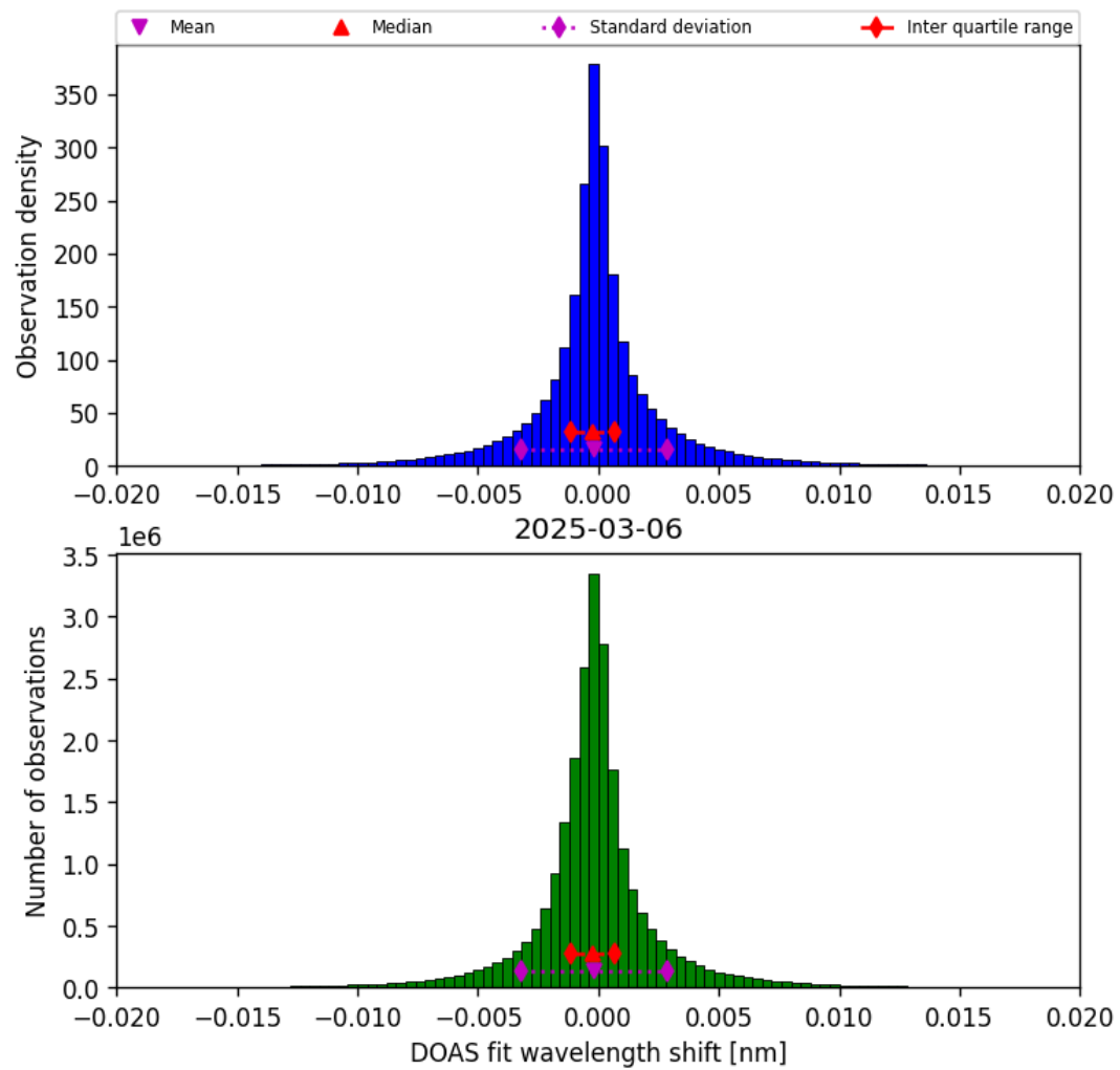
Figure 42: Histogram of “DOAS fit wavelength shift” for 2025-03-06 to 2025-03-07
