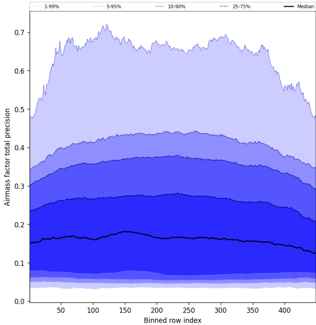
Figure 53: Along track statistics of “Airmass factor total precision” for 2025-03-06 to 2025-03-07
