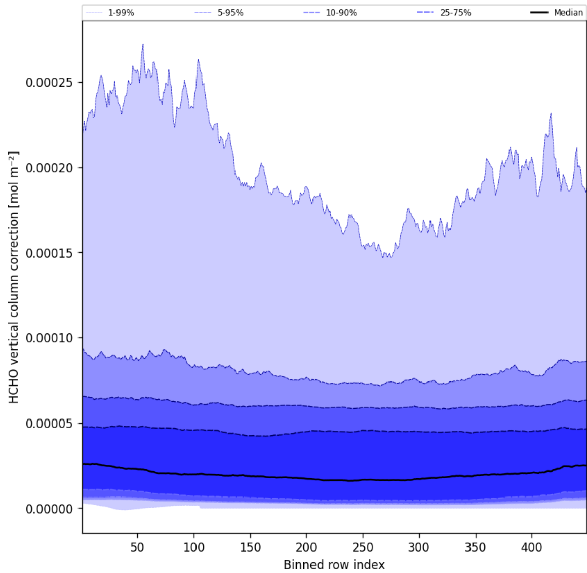
Figure 49: Along track statistics of “HCHO vertical column correction” for 2025-03-06 to 2025-03-07
