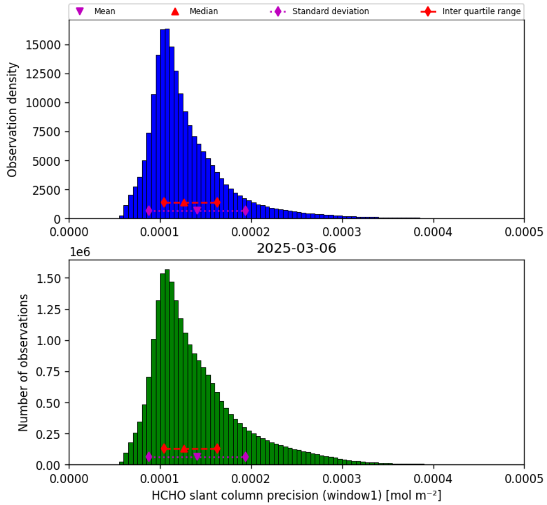
Figure 37: Histogram of “HCHO slant column precision (window1)” for 2025-03-06 to 2025-03-07
