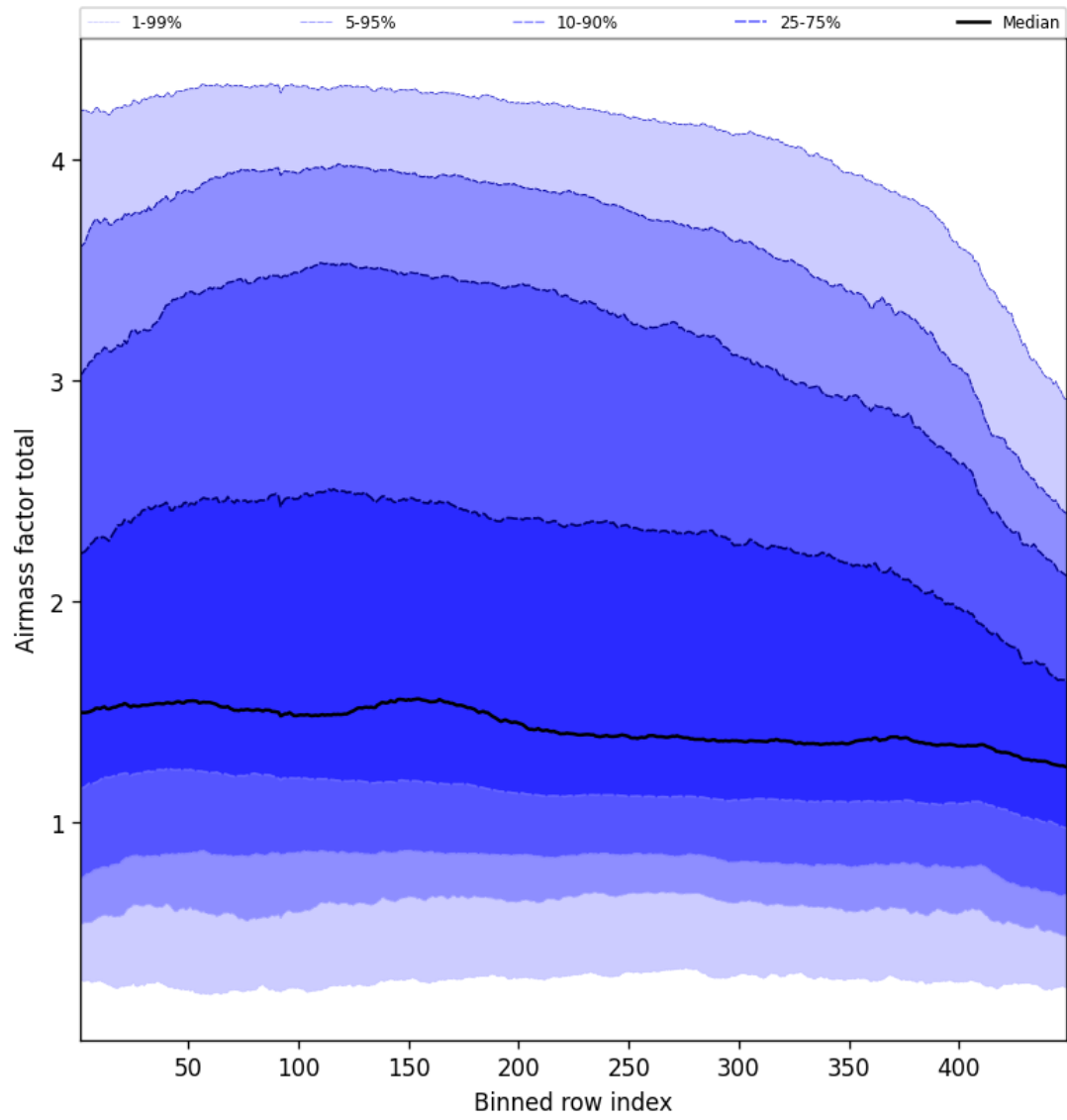
Figure 52: Along track statistics of “Airmass factor total” for 2025-03-06 to 2025-03-07
