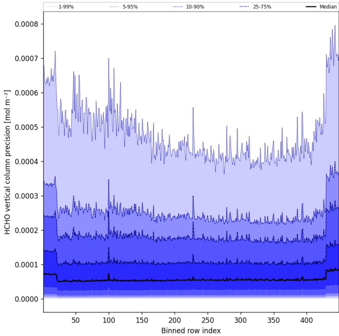
Figure 48: Along track statistics of “HCHO vertical column precision” for 2025-03-06 to 2025-03-07
