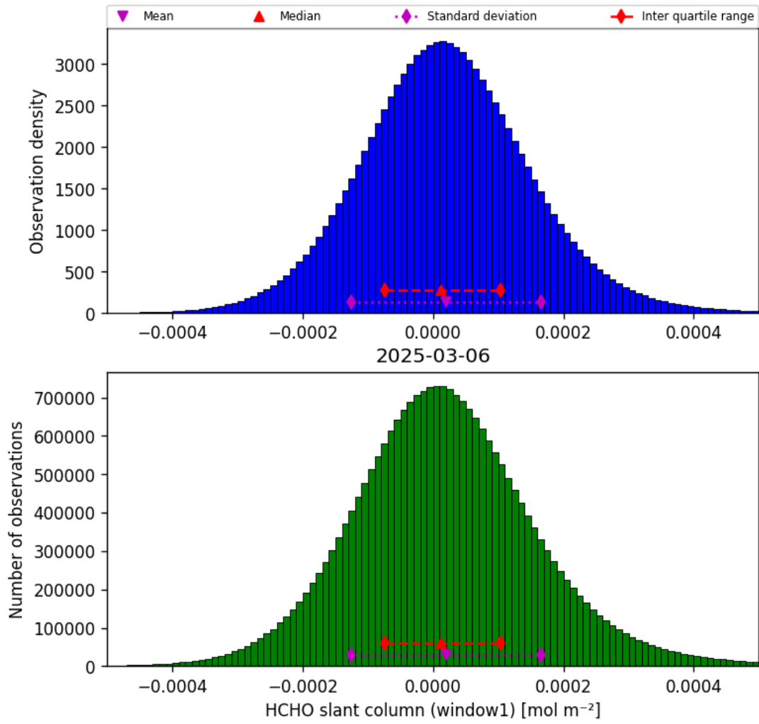
Figure 36: Histogram of “HCHO slant column (window1)” for 2025-03-06 to 2025-03-07
