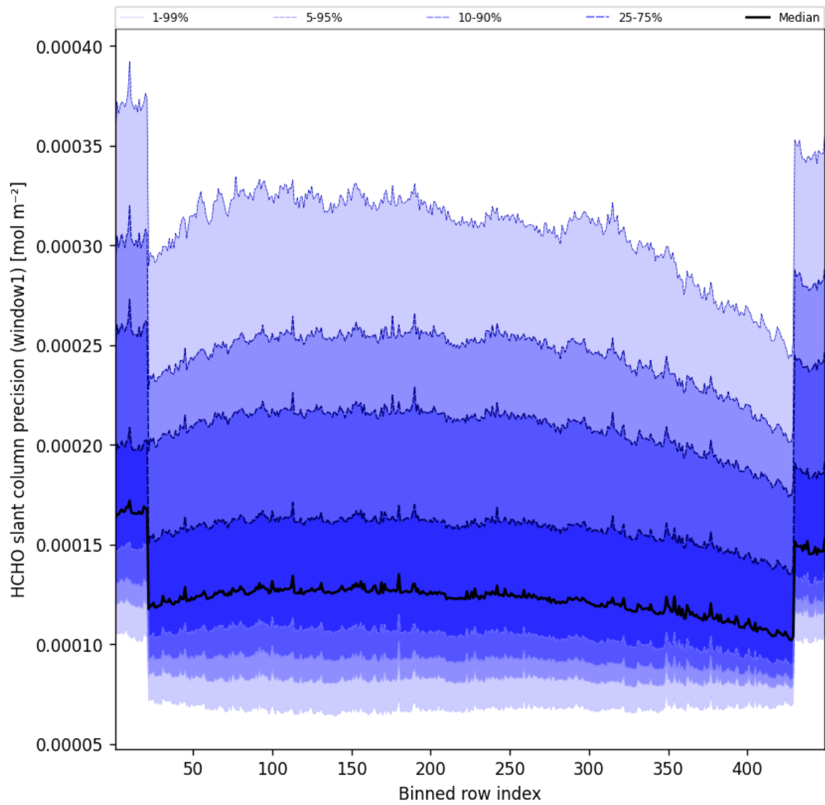
Figure 51: Along track statistics of “HCHO slant column precision (window1)” for 2025-03-06 to 2025-03-07
