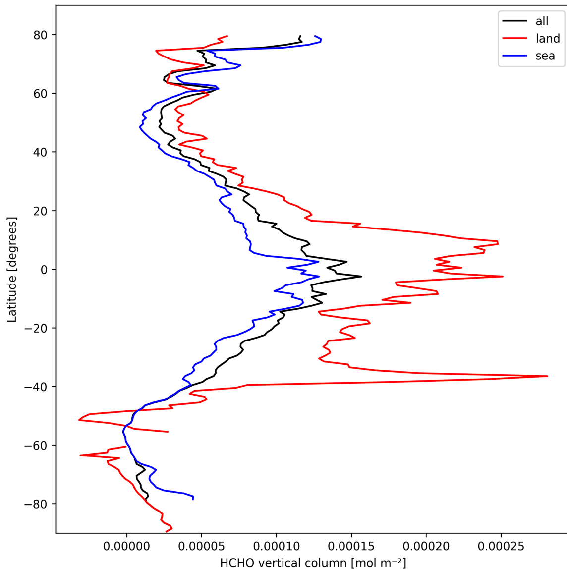
Figure 19: Zonal average of “HCHO vertical column” for 2025-03-06 to 2025-03-07.
