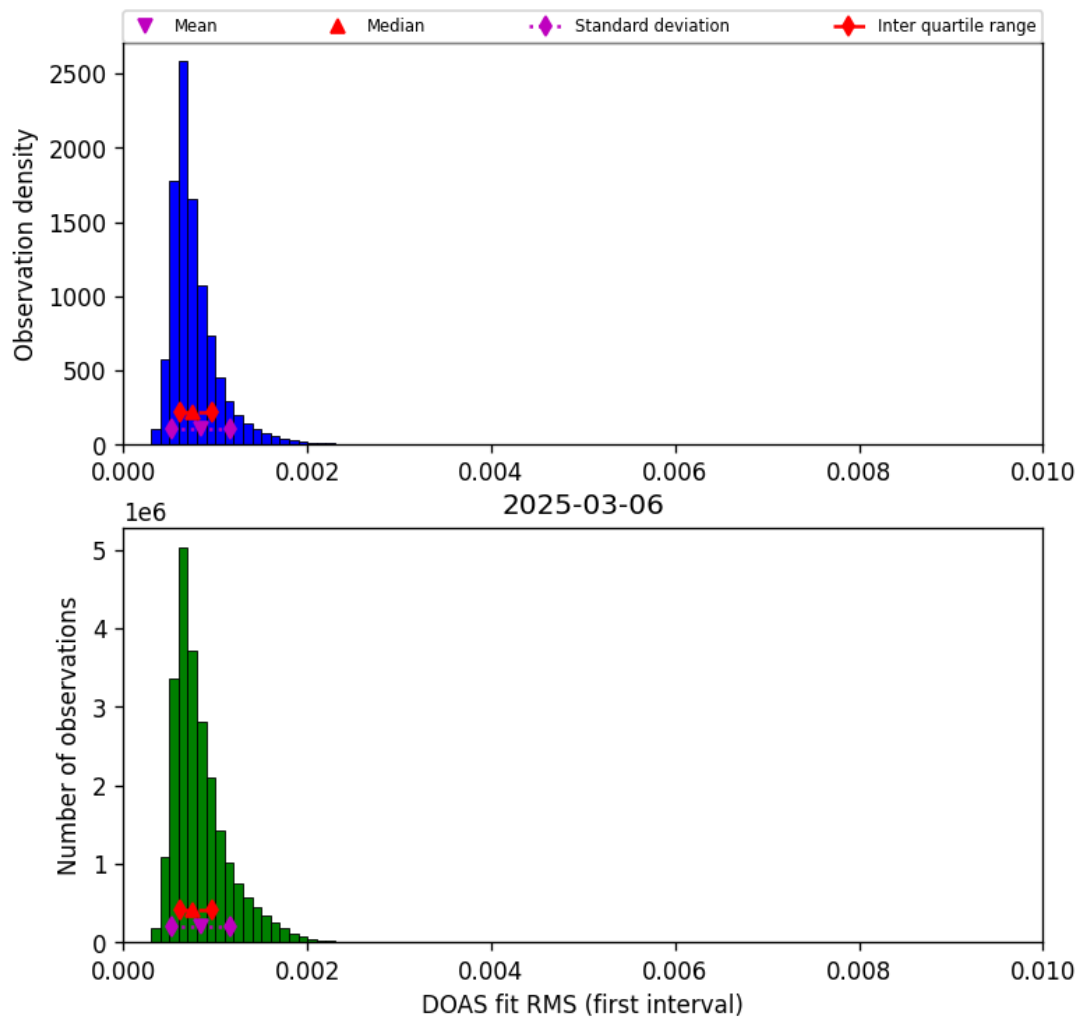
Figure 44: Histogram of “DOAS fit RMS (first interval)” for 2025-03-06 to 2025-03-07
