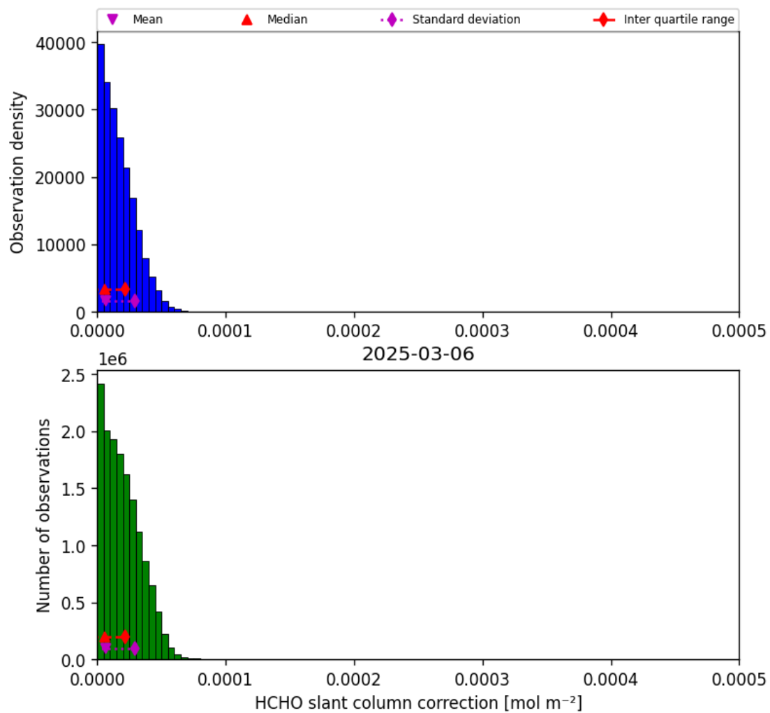
Figure 45: Histogram of “HCHO slant column correction” for 2025-03-06 to 2025-03-07
