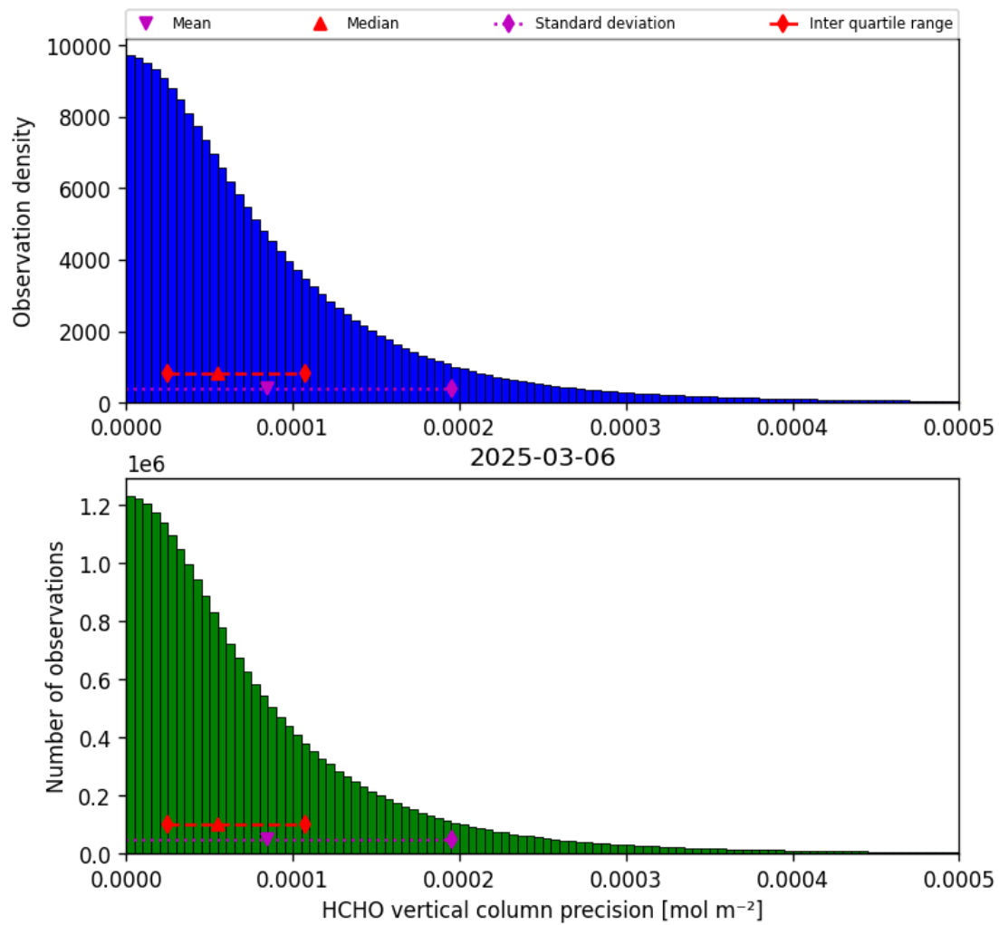
Figure 34: Histogram of “HCHO vertical column precision” for 2025-03-06 to 2025-03-07
