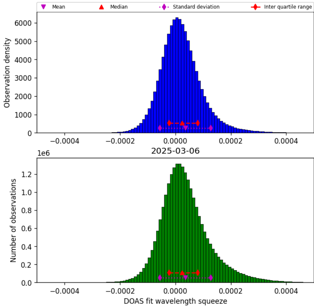
Figure 43: Histogram of “DOAS fit wavelength squeeze” for 2025-03-06 to 2025-03-07
