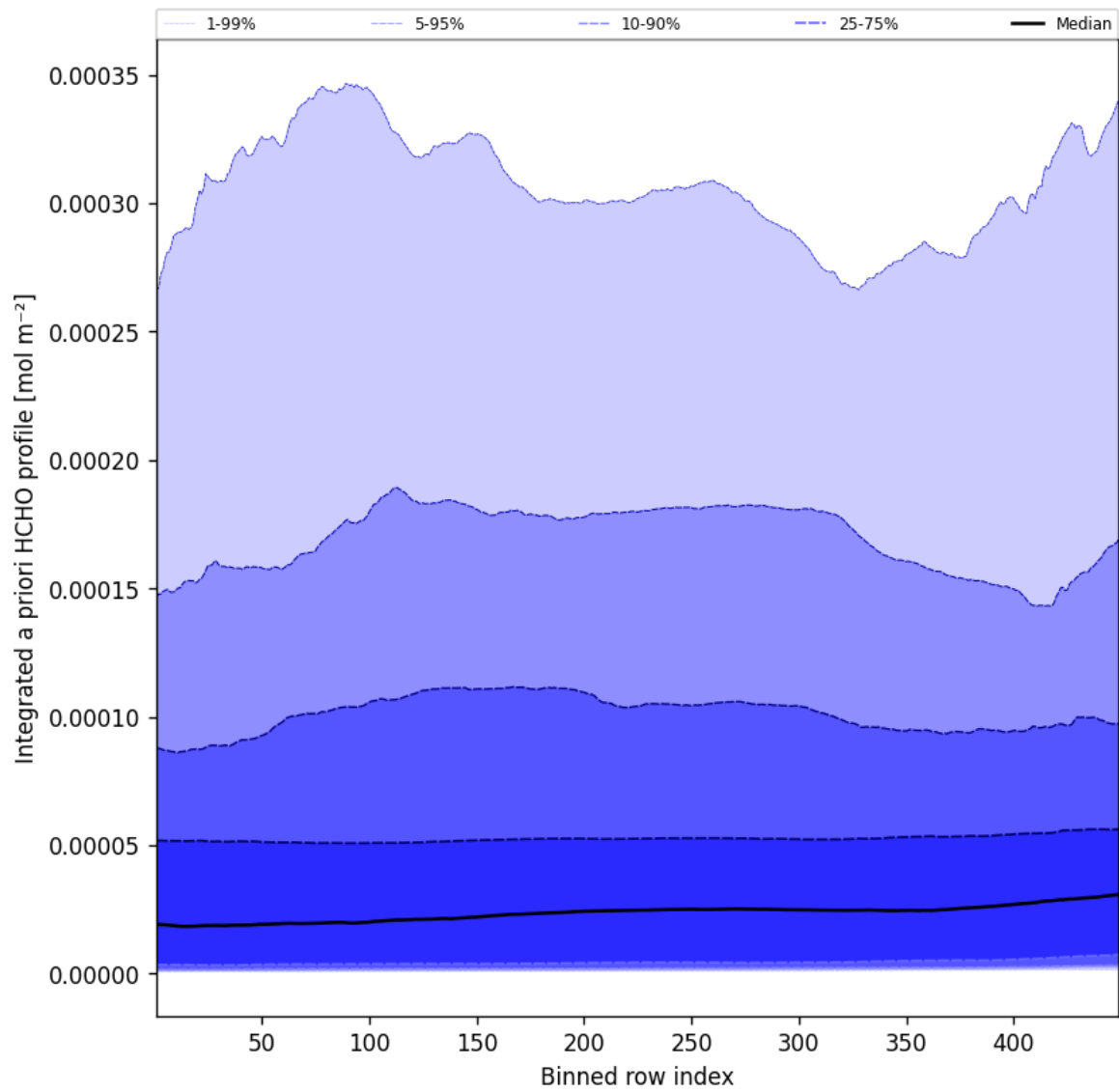
Figure 55: Along track statistics of “Integrated a priori HCHO profile” for 2025-03-06 to 2025-03-07
