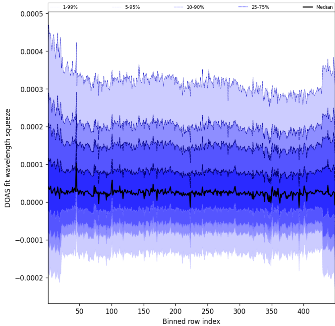
Figure 57: Along track statistics of “DOAS fit wavelength squeeze” for 2025-03-06 to 2025-03-07
