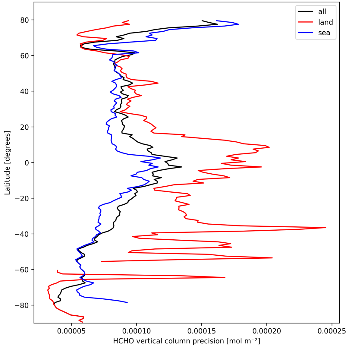
Figure 20: Zonal average of “HCHO vertical column precision” for 2025-03-06 to 2025-03-07.
