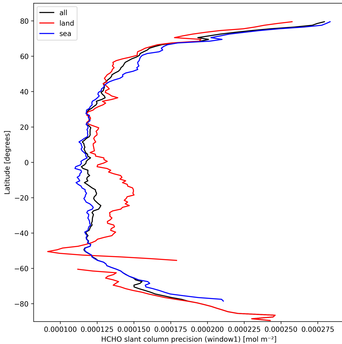
Figure 23: Zonal average of “HCHO slant column precision (window1)” for 2025-03-06 to 2025-03-07.
