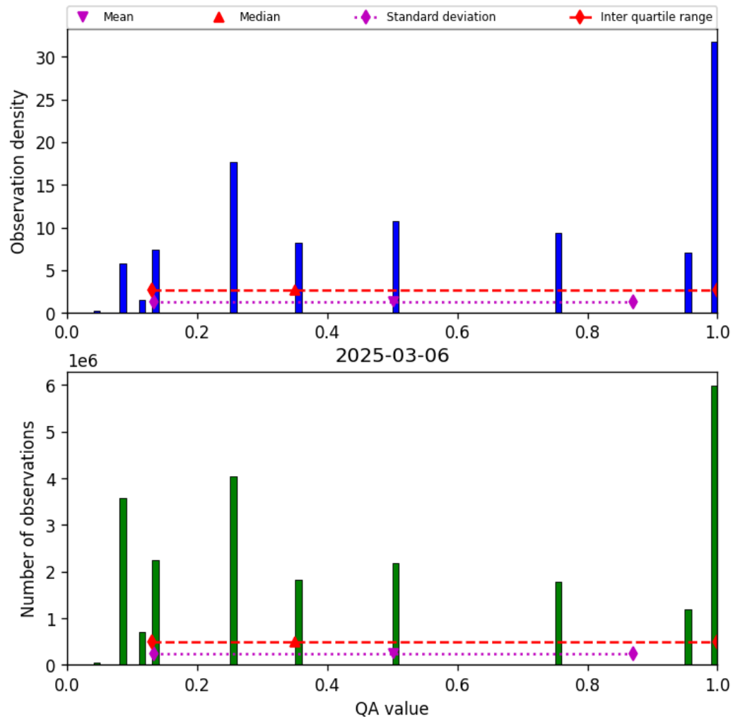
Figure 32: Histogram of “QA value” for 2025-03-06 to 2025-03-07
