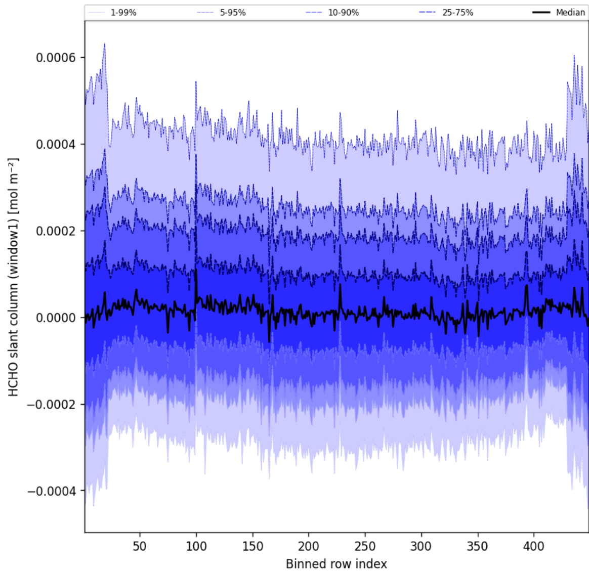
Figure 50: Along track statistics of “HCHO slant column (window1)” for 2025-03-06 to 2025-03-07
