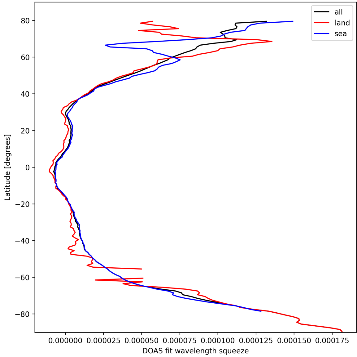
Figure 29: Zonal average of “DOAS fit wavelength squeeze” for 2025-03-06 to 2025-03-07.
