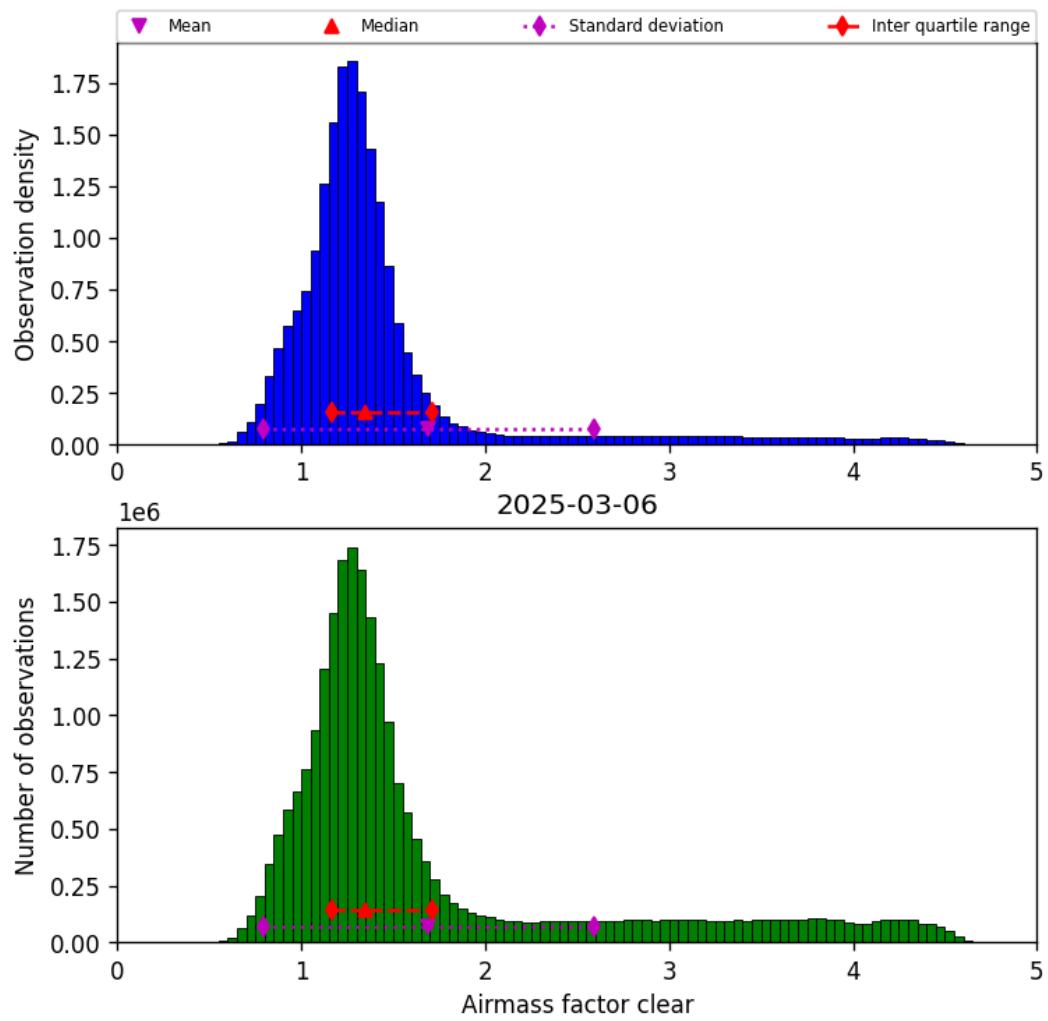
Figure 40: Histogram of “Airmass factor clear” for 2025-03-06 to 2025-03-07
