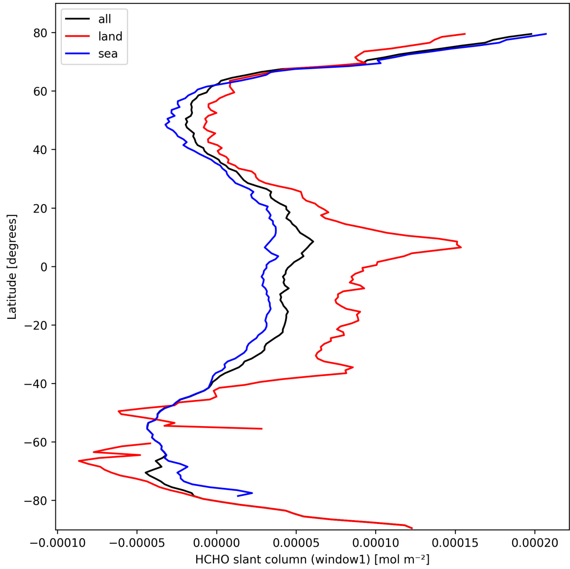
Figure 22: Zonal average of “HCHO slant column (window1)” for 2025-03-06 to 2025-03-07.
