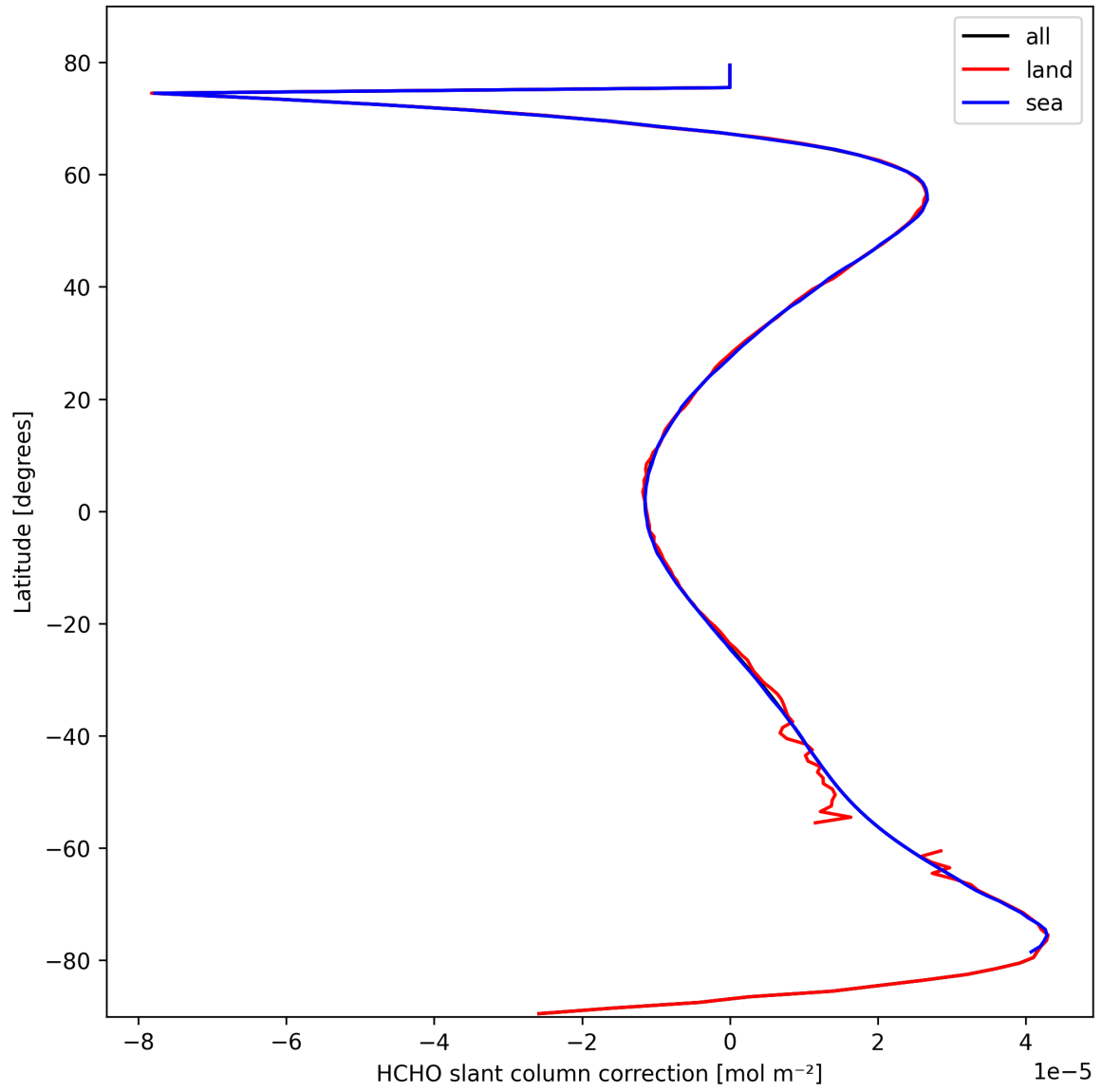
Figure 31: Zonal average of “HCHO slant column correction” for 2025-03-06 to 2025-03-07.
