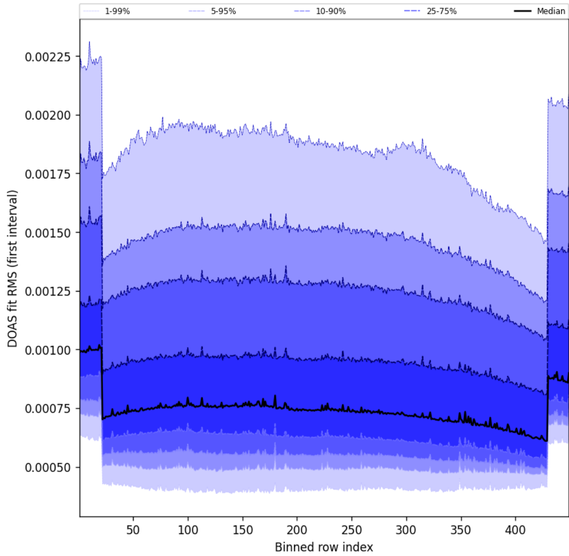
Figure 58: Along track statistics of “DOAS fit RMS (first interval)” for 2025-03-06 to 2025-03-07
