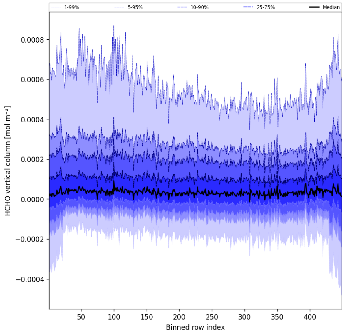
Figure 47: Along track statistics of “HCHO vertical column” for 2025-03-06 to 2025-03-07
