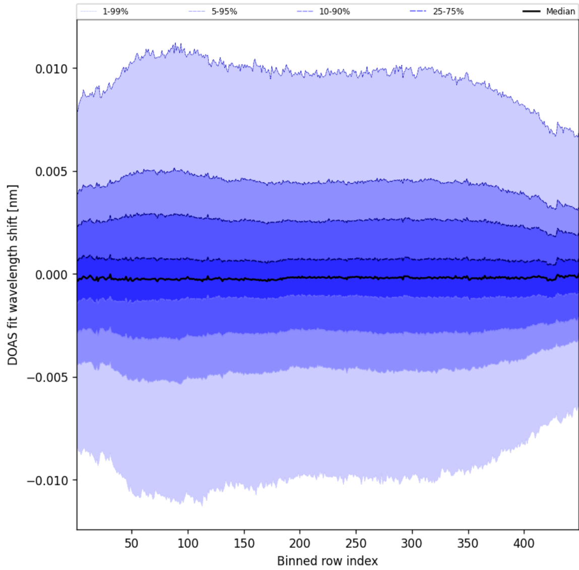
Figure 56: Along track statistics of “DOAS fit wavelength shift” for 2025-03-06 to 2025-03-07
