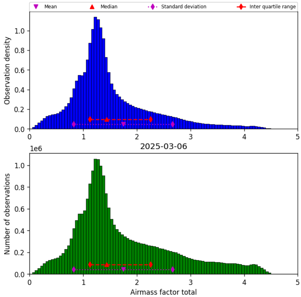
Figure 38: Histogram of “Airmass factor total” for 2025-03-06 to 2025-03-07
