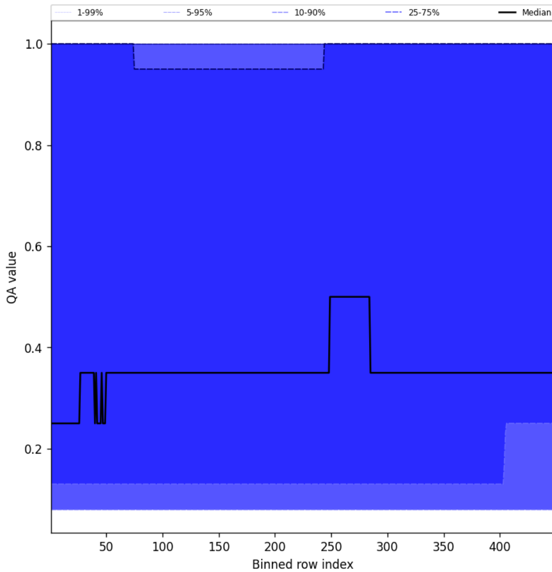
Figure 46: Along track statistics of “QA value” for 2025-03-06 to 2025-03-07
