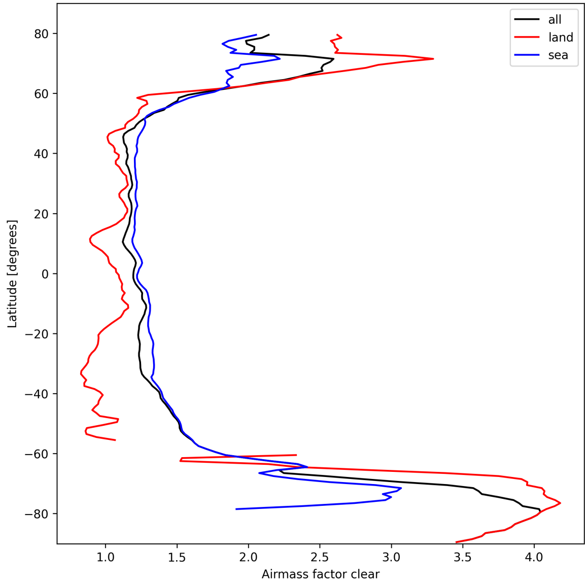
Figure 26: Zonal average of “Airmass factor clear” for 2025-03-06 to 2025-03-07.
