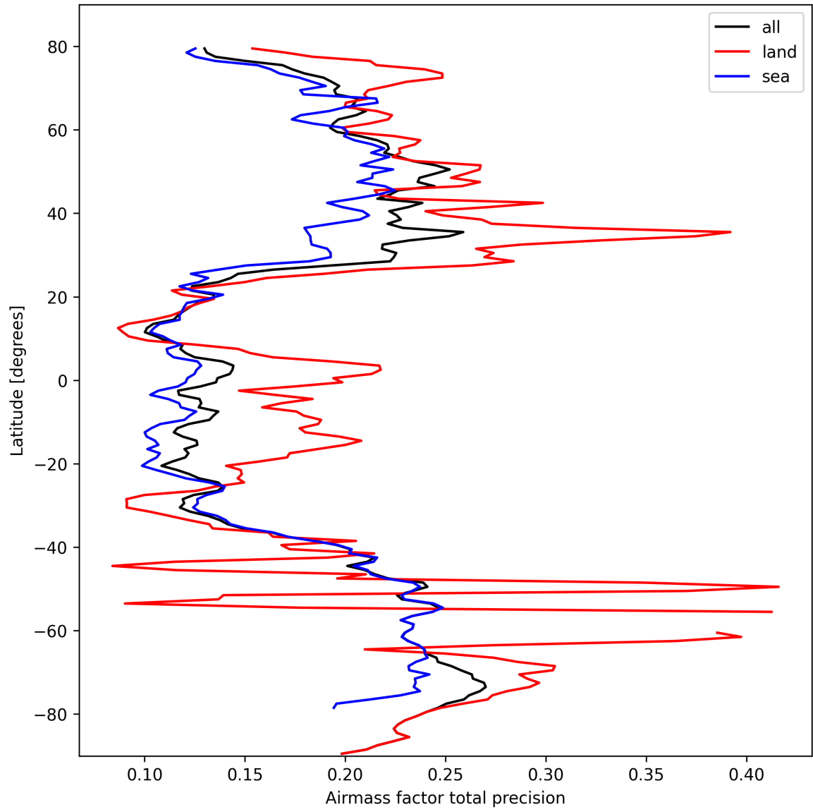
Figure 25: Zonal average of “Airmass factor total precision” for 2025-03-06 to 2025-03-07.
