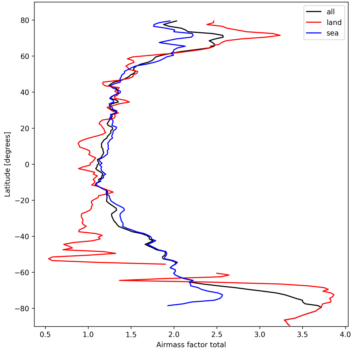
Figure 24: Zonal average of “Airmass factor total” for 2025-03-06 to 2025-03-07.
