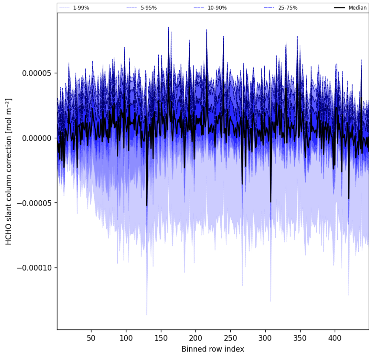
Figure 59: Along track statistics of “HCHO slant column correction” for 2025-03-06 to 2025-03-07
