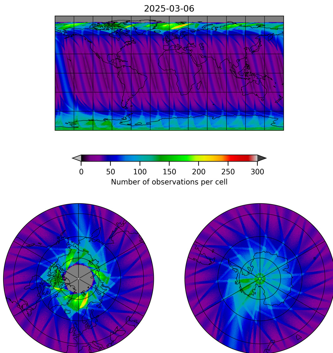
Figure 17: Map of the number of observations for 2025-03-06 to 2025-03-07
