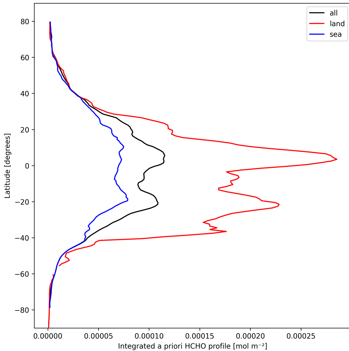
Figure 27: Zonal average of “Integrated a priori HCHO profile” for 2025-03-06 to 2025-03-07.
