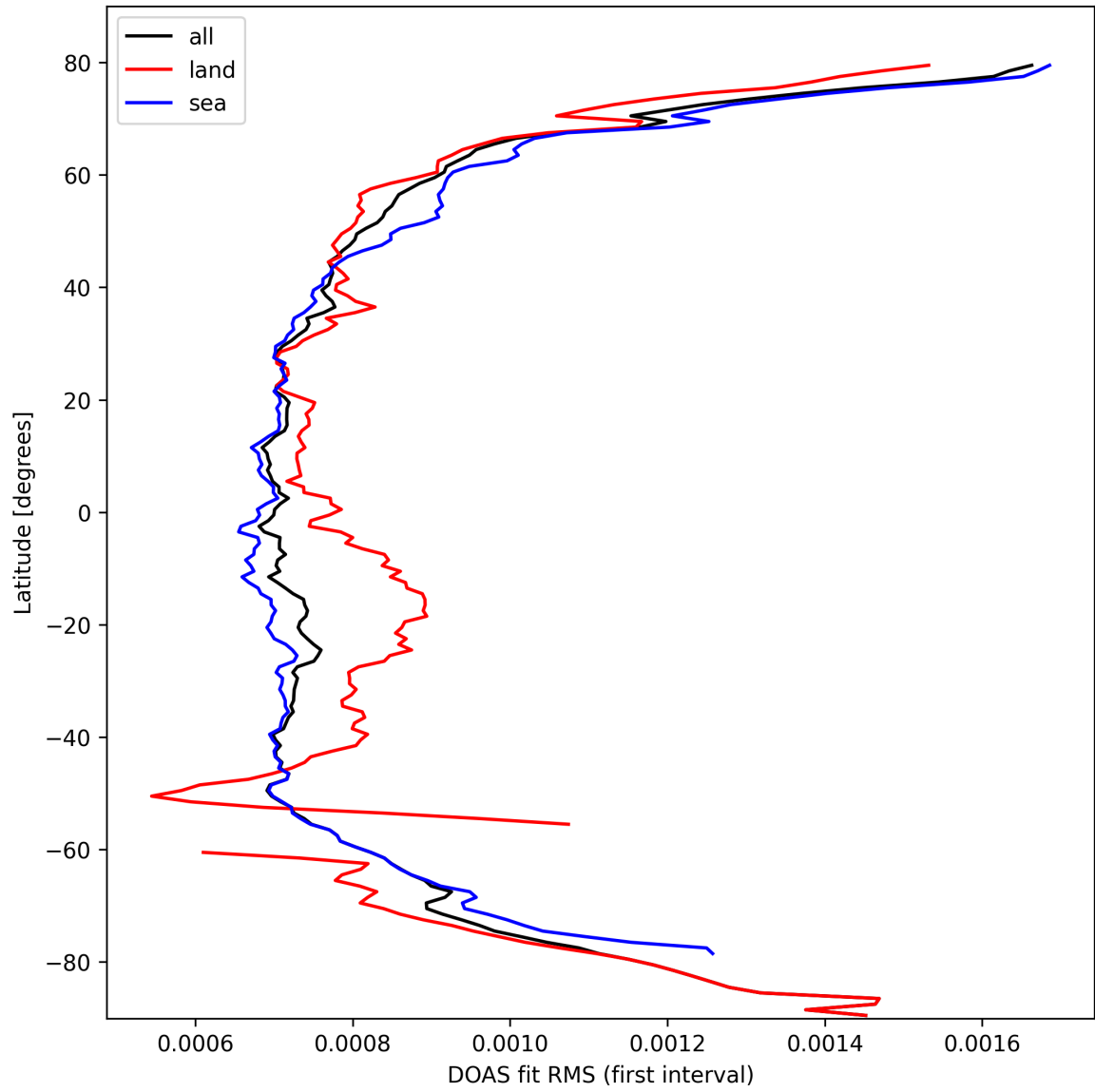
Figure 30: Zonal average of “DOAS fit RMS (first interval)” for 2025-03-06 to 2025-03-07.
