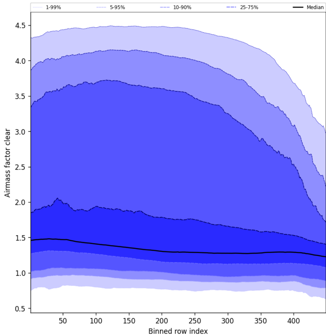
Figure 54: Along track statistics of “Airmass factor clear” for 2025-03-06 to 2025-03-07
