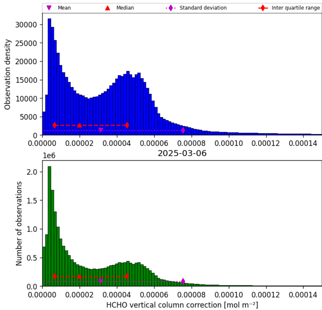
Figure 35: Histogram of “HCHO vertical column correction” for 2025-03-06 to 2025-03-07
