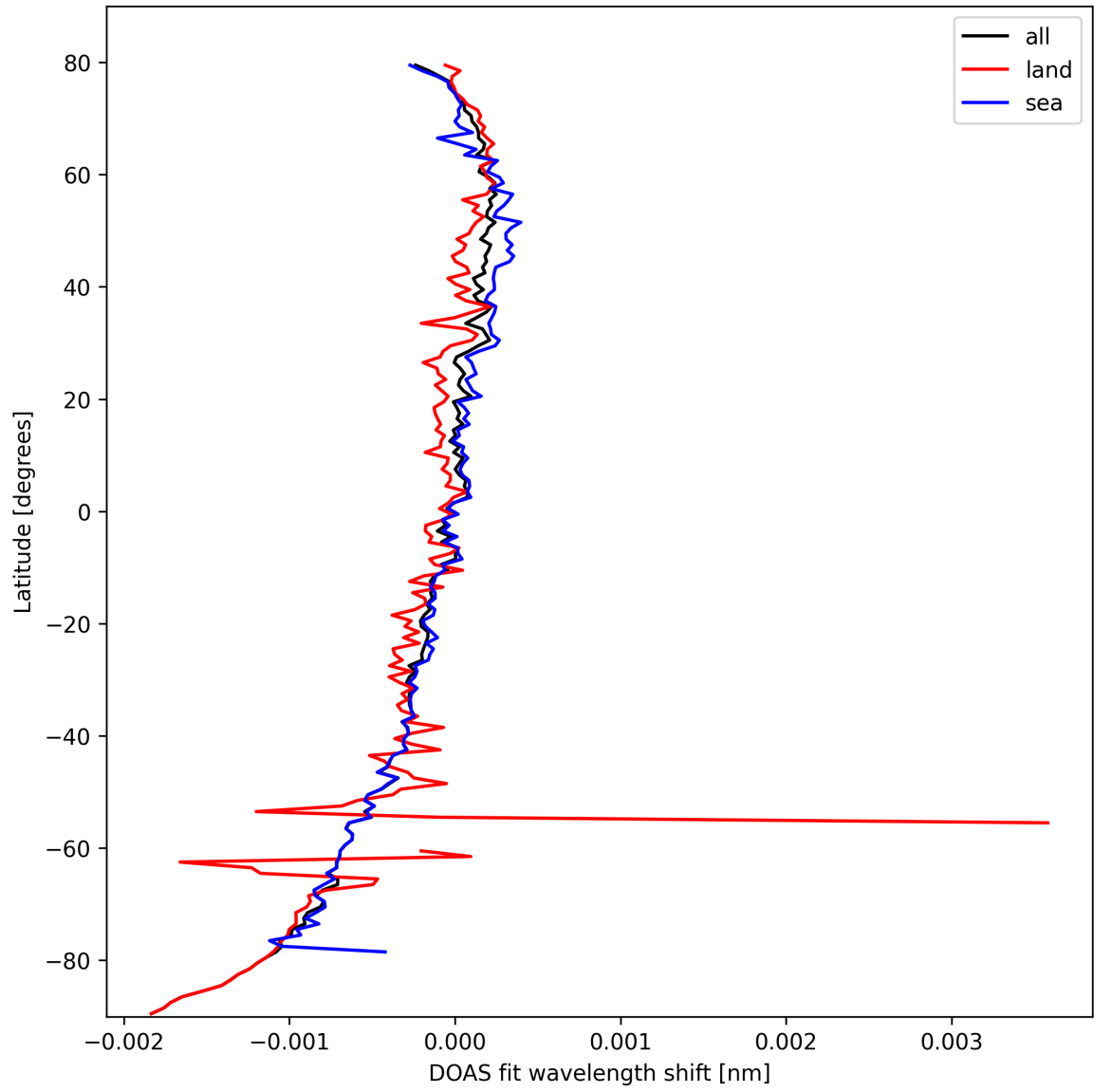
Figure 28: Zonal average of "DOAS fit wavelength shift" for 2025-03-06 to 2025-03-07.
