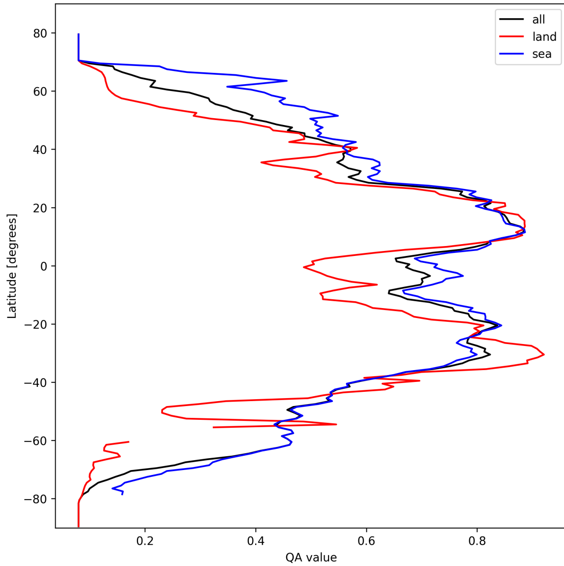
Figure 18: Zonal average of “QA value” for 2025-03-06 to 2025-03-07.
