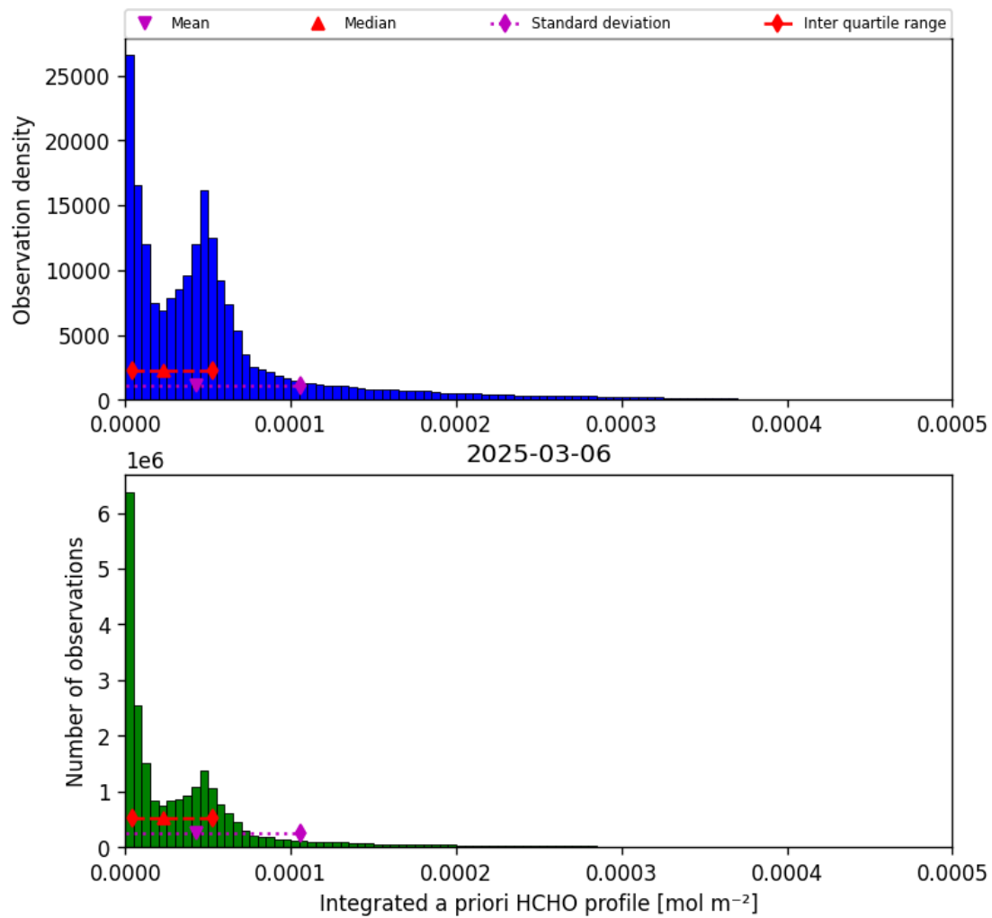
Figure 41: Histogram of “Integrated a priori HCHO profile” for 2025-03-06 to 2025-03-07
