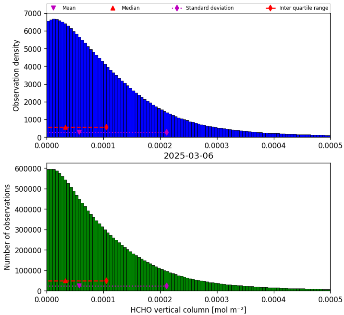
Figure 33: Histogram of “HCHO vertical column” for 2025-03-06 to 2025-03-07
