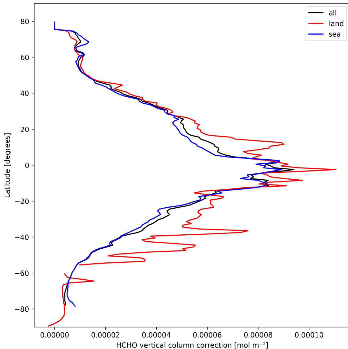
Figure 21: Zonal average of “HCHO vertical column correction” for 2025-03-06 to 2025-03-07.
