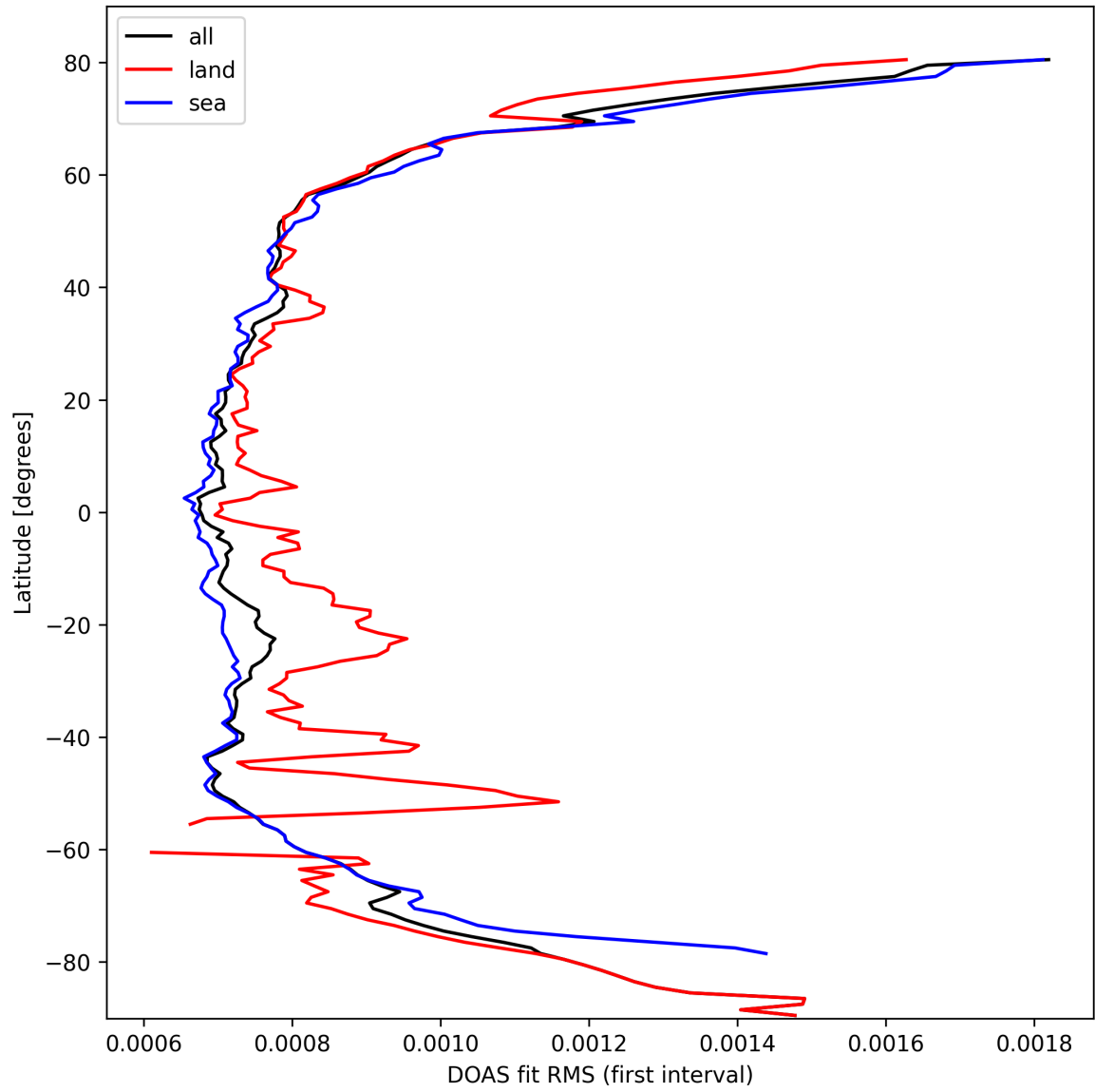
Figure 30: Zonal average of "DOAS fit RMS (first interval)" for 2025-03-07 to 2025-03-08.
