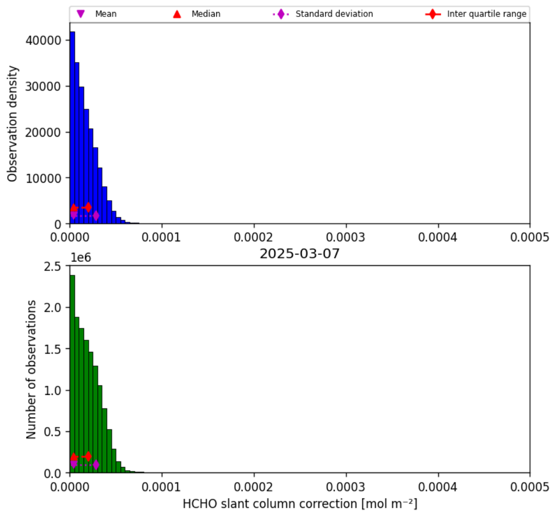
Figure 45: Histogram of “HCHO slant column correction” for 2025-03-07 to 2025-03-08
