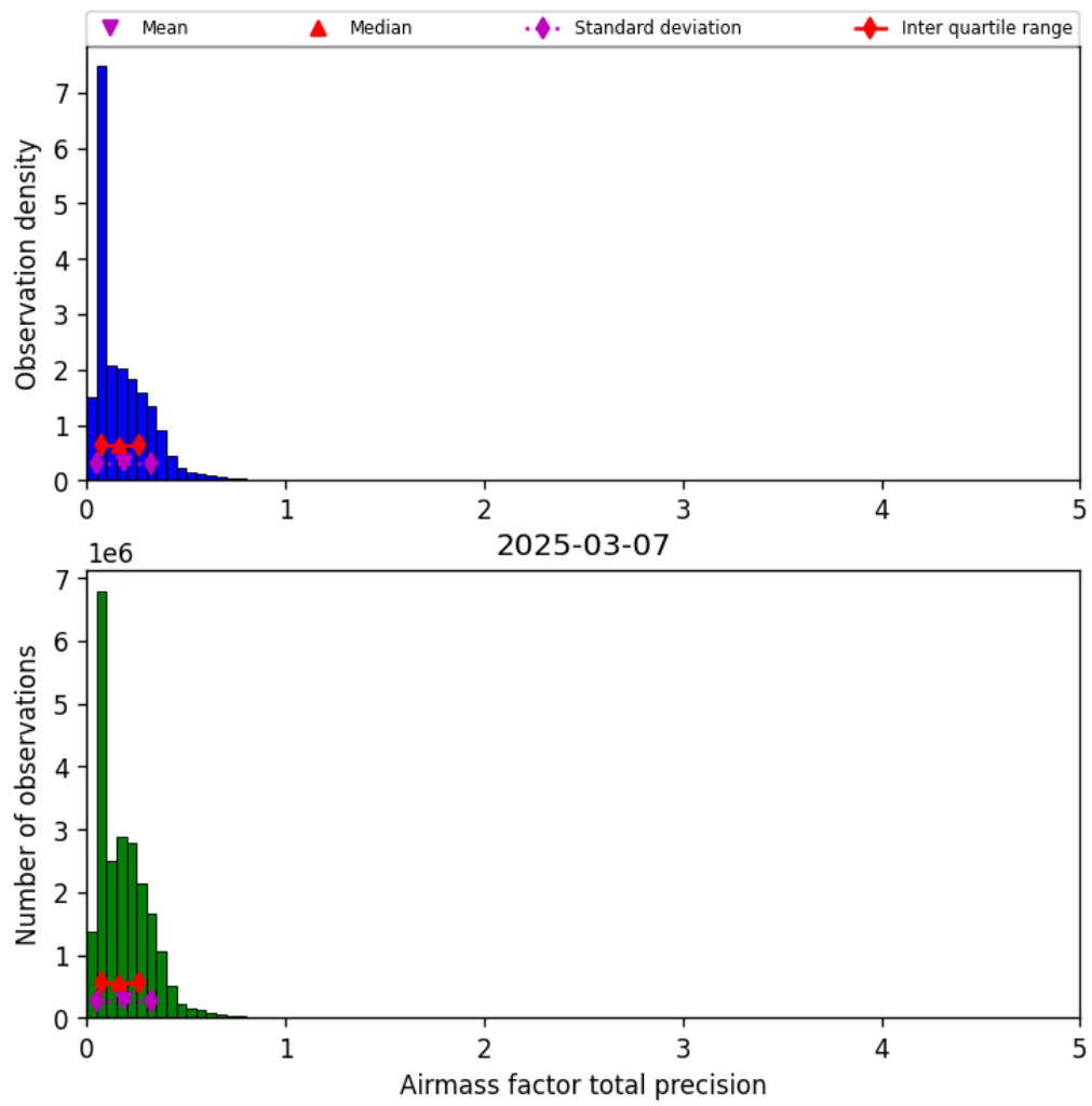
Figure 39: Histogram of “Airmass factor total precision” for 2025-03-07 to 2025-03-08
