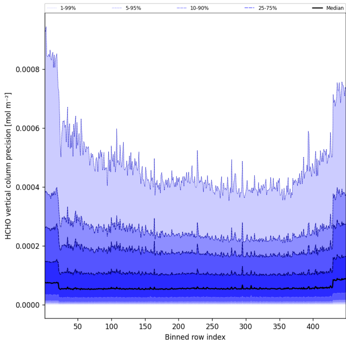
Figure 48: Along track statistics of “HCHO vertical column precision” for 2025-03-07 to 2025-03-08
