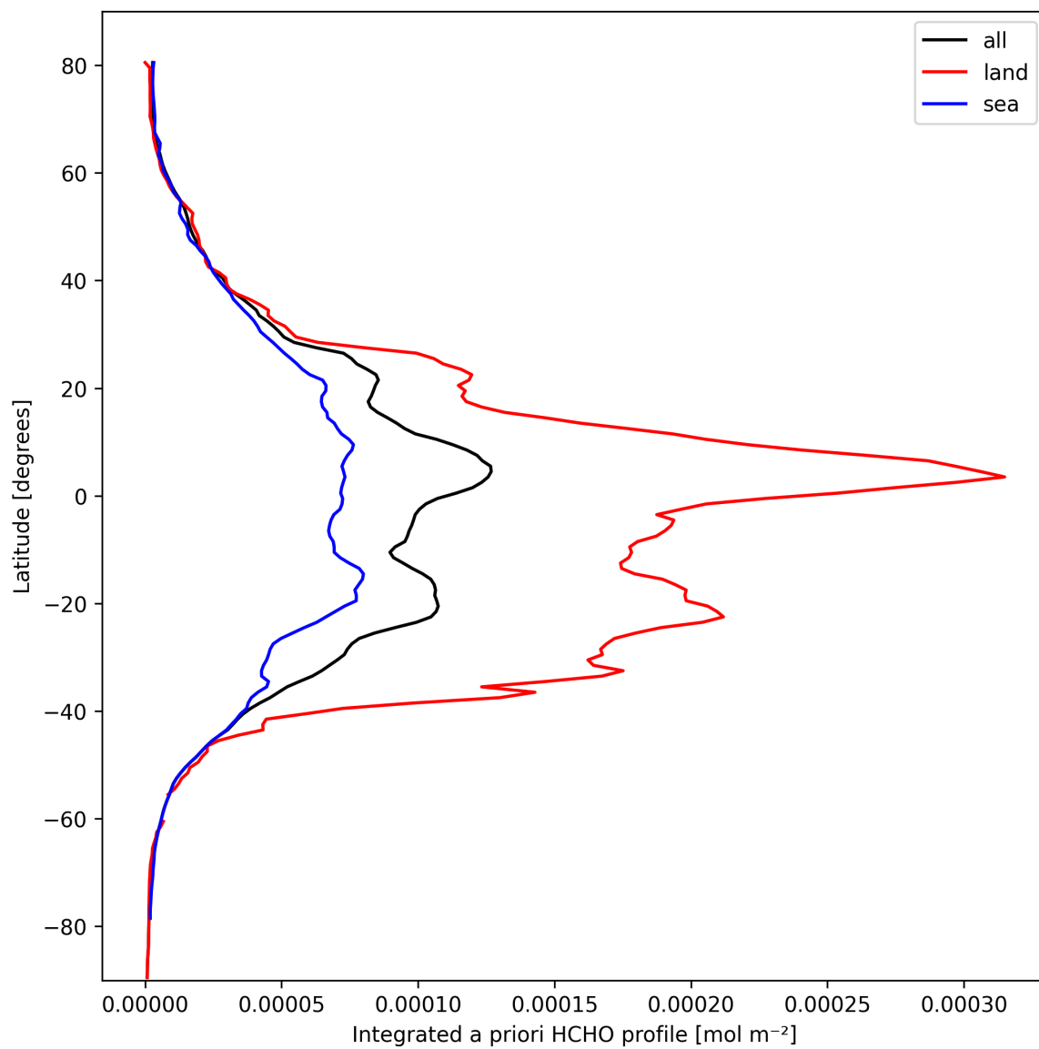
Figure 27: Zonal average of “Integrated a priori HCHO profile” for 2025-03-07 to 2025-03-08.
