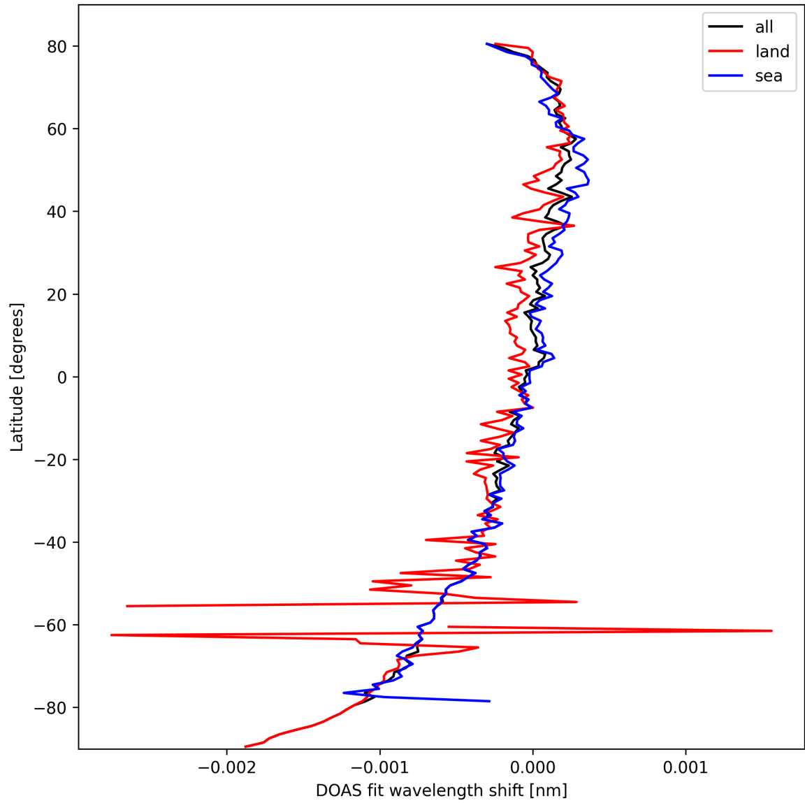
Figure 28: Zonal average of “DOAS fit wavelength shift” for 2025-03-07 to 2025-03-08.
