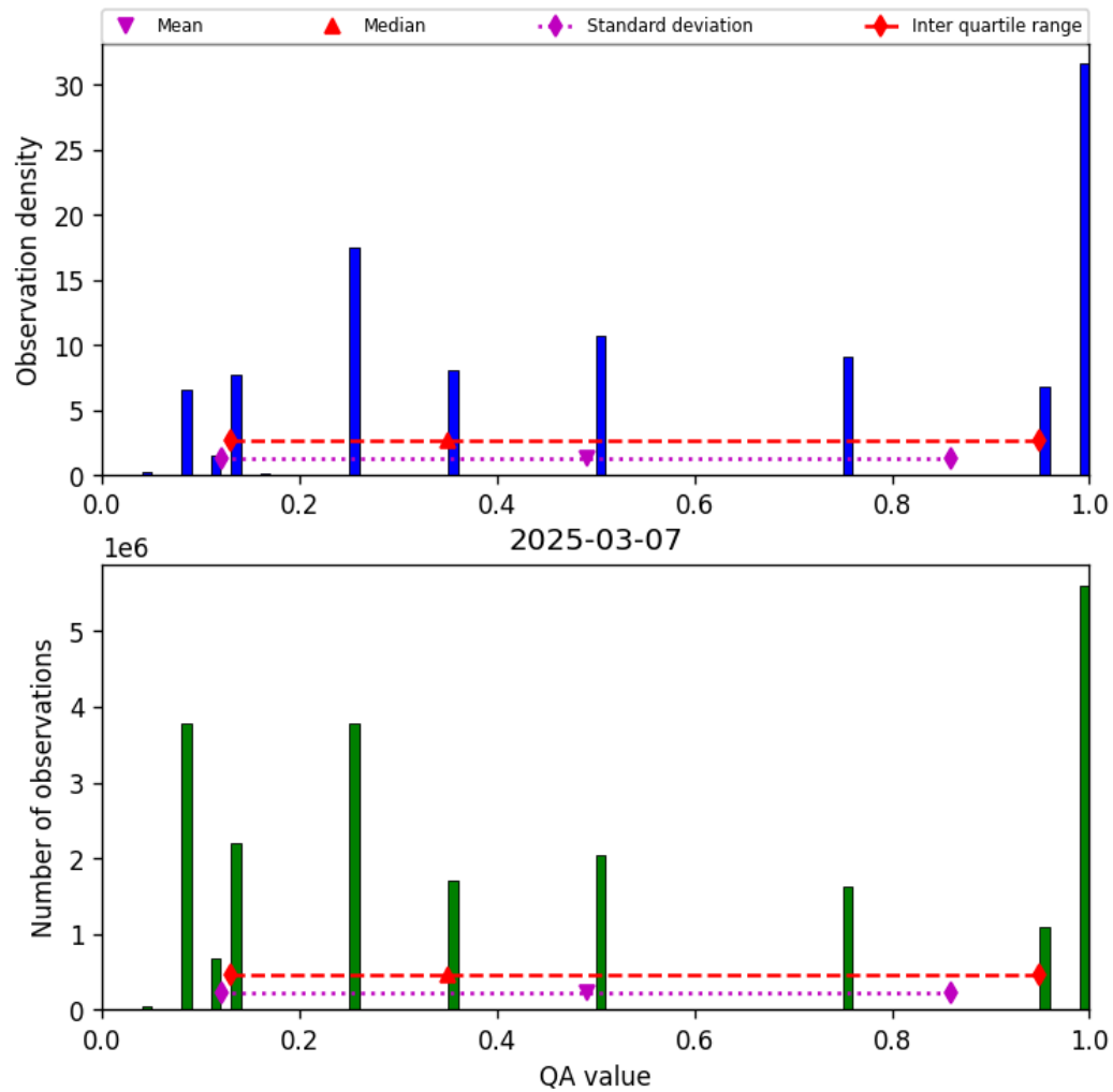
Figure 32: Histogram of “QA value” for 2025-03-07 to 2025-03-08
