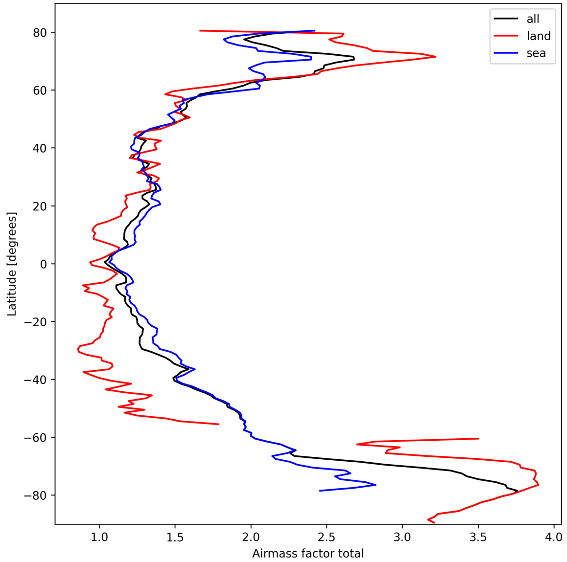
Figure 24: Zonal average of “Airmass factor total” for 2025-03-07 to 2025-03-08.
