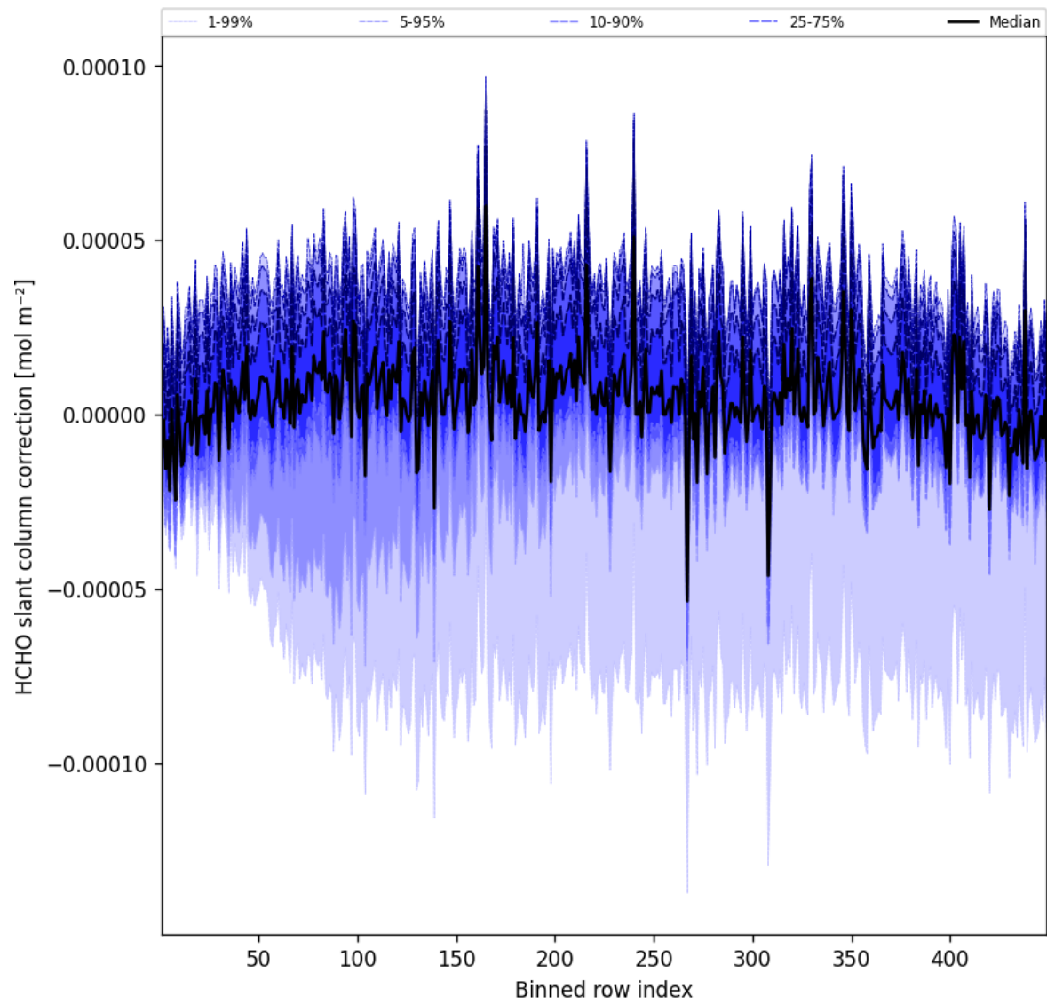
Figure 59: Along track statistics of “HCHO slant column correction” for 2025-03-07 to 2025-03-08
