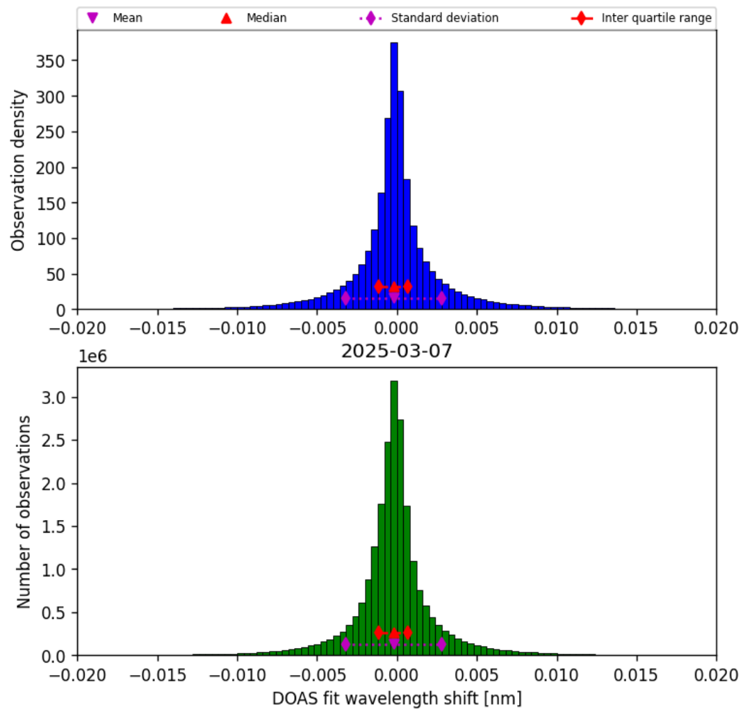
Figure 42: Histogram of “DOAS fit wavelength shift” for 2025-03-07 to 2025-03-08
