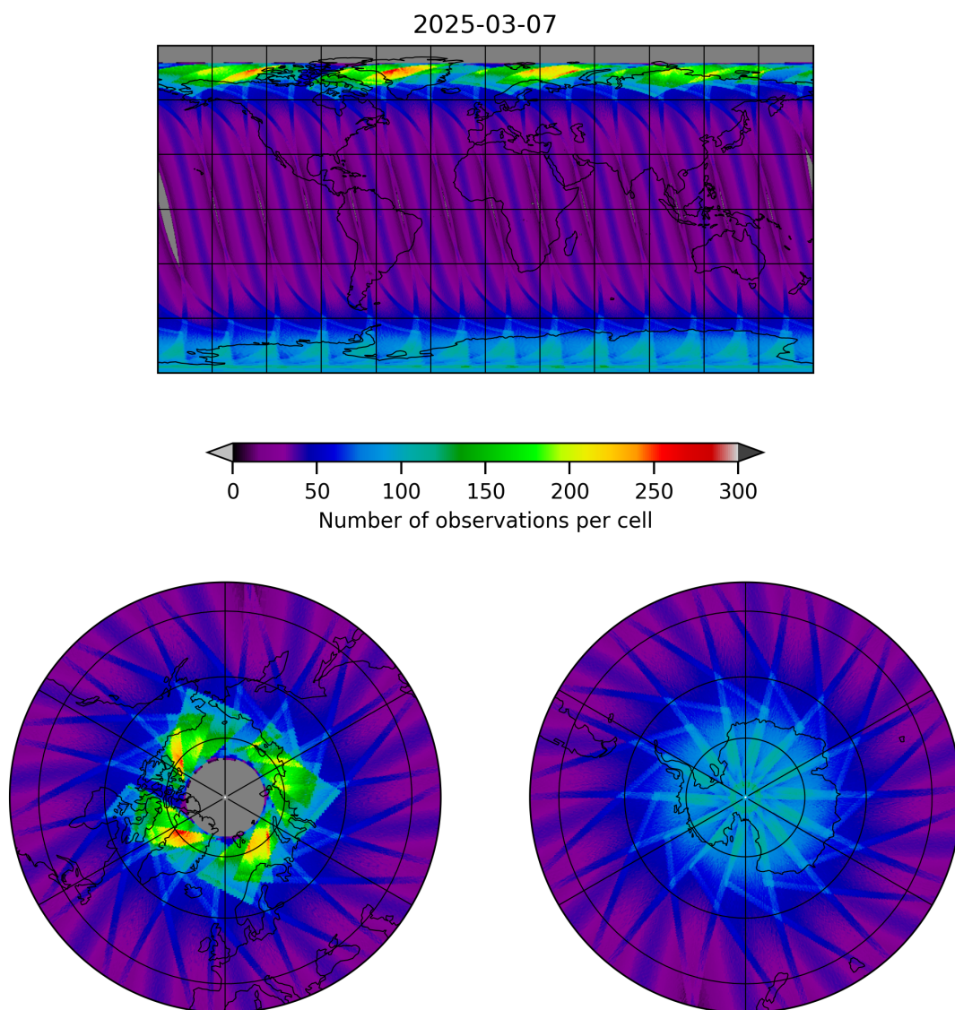
Figure 17: Map of the number of observations for 2025-03-07 to 2025-03-08
