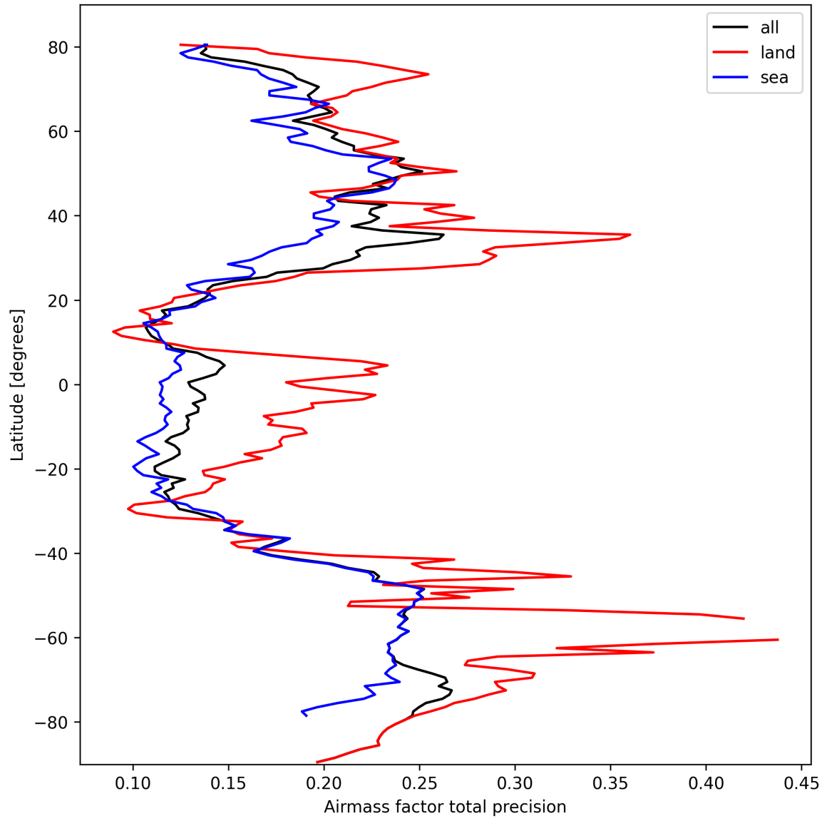
Figure 25: Zonal average of “Airmass factor total precision” for 2025-03-07 to 2025-03-08.
