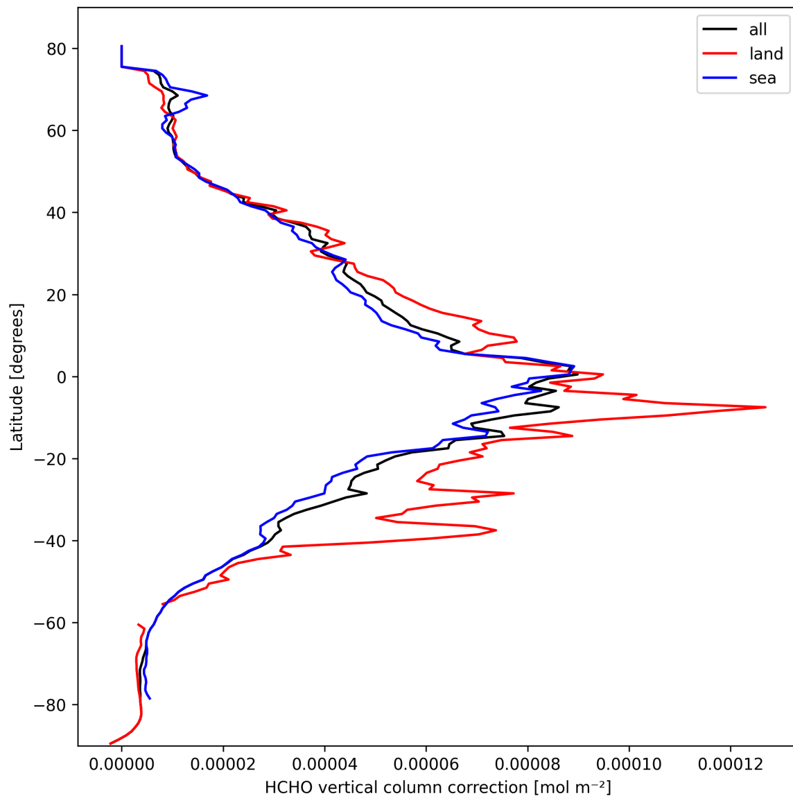
Figure 21: Zonal average of “HCHO vertical column correction” for 2025-03-07 to 2025-03-08.
