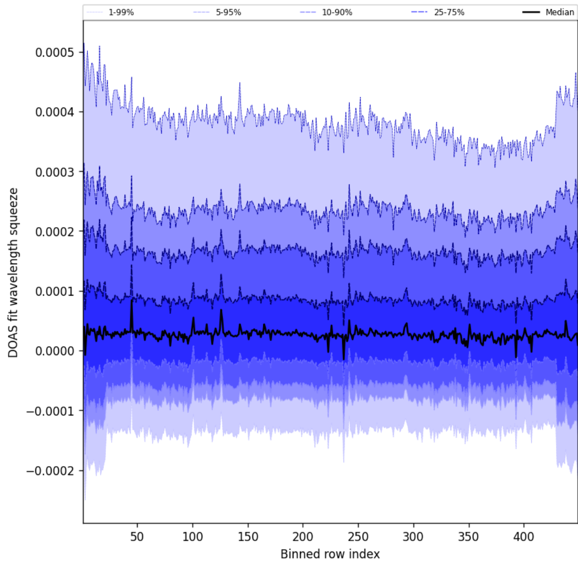
Figure 57: Along track statistics of “DOAS fit wavelength squeeze” for 2025-03-07 to 2025-03-08
