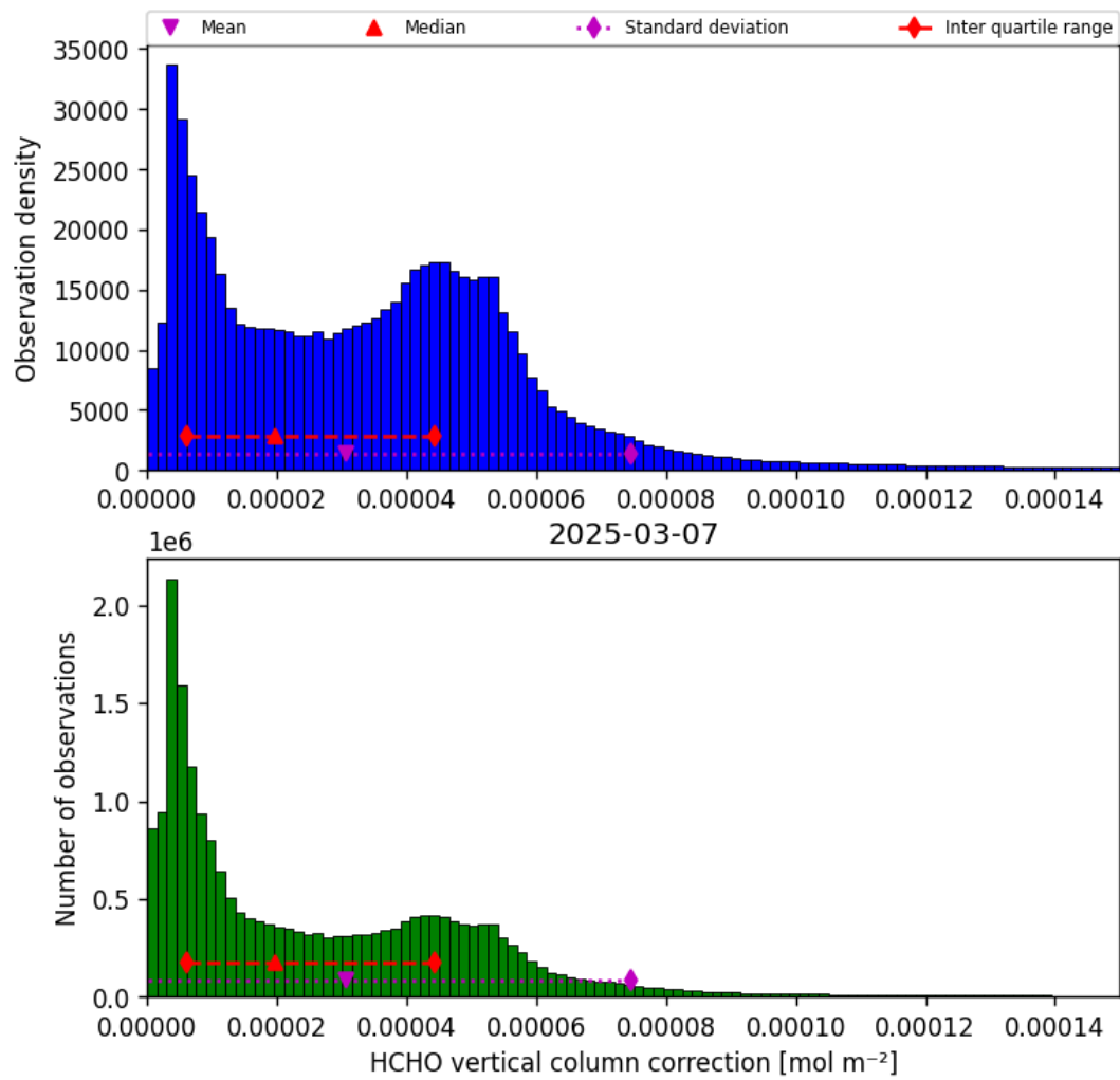
Figure 35: Histogram of “HCHO vertical column correction” for 2025-03-07 to 2025-03-08
