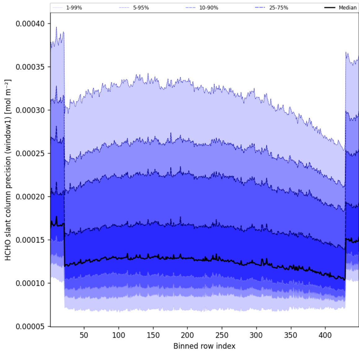
Figure 51: Along track statistics of “HCHO slant column precision (window1)” for 2025-03-07 to 2025-03-08
