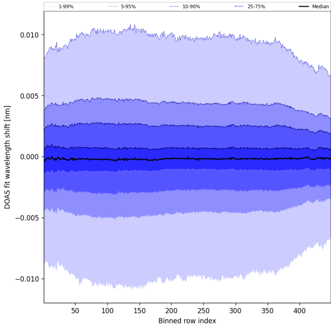
Figure 56: Along track statistics of “DOAS fit wavelength shift” for 2025-03-07 to 2025-03-08
