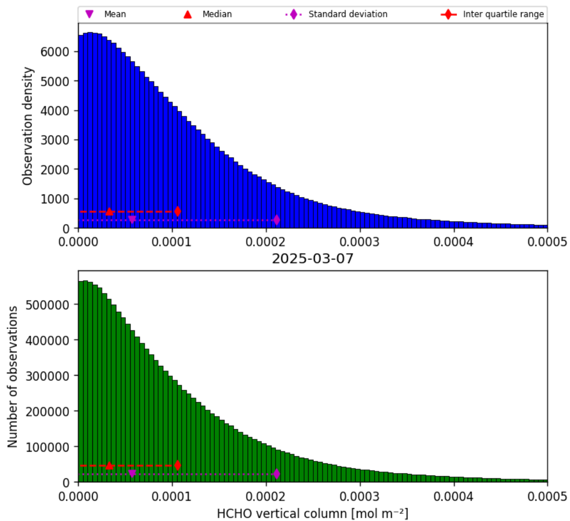
Figure 33: Histogram of “HCHO vertical column” for 2025-03-07 to 2025-03-08
