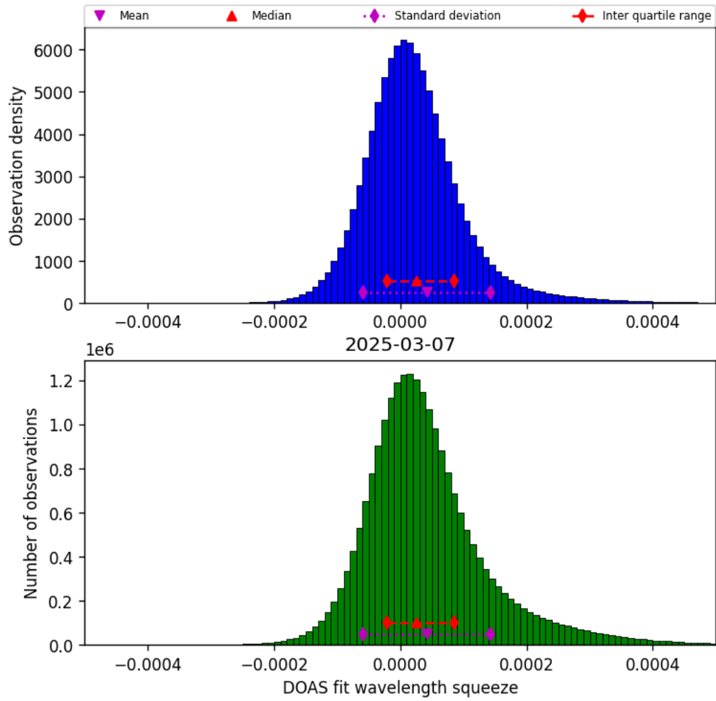
Figure 43: Histogram of “DOAS fit wavelength squeeze” for 2025-03-07 to 2025-03-08
