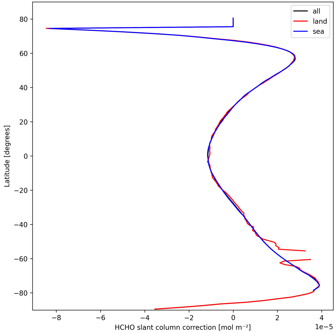
Figure 31: Zonal average of “HCHO slant column correction” for 2025-03-07 to 2025-03-08.
