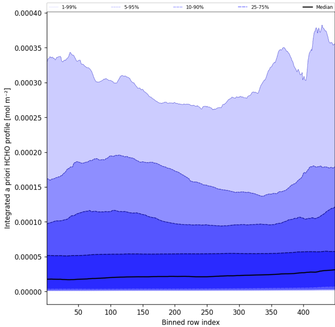
Figure 55: Along track statistics of “Integrated a priori HCHO profile” for 2025-03-07 to 2025-03-08
