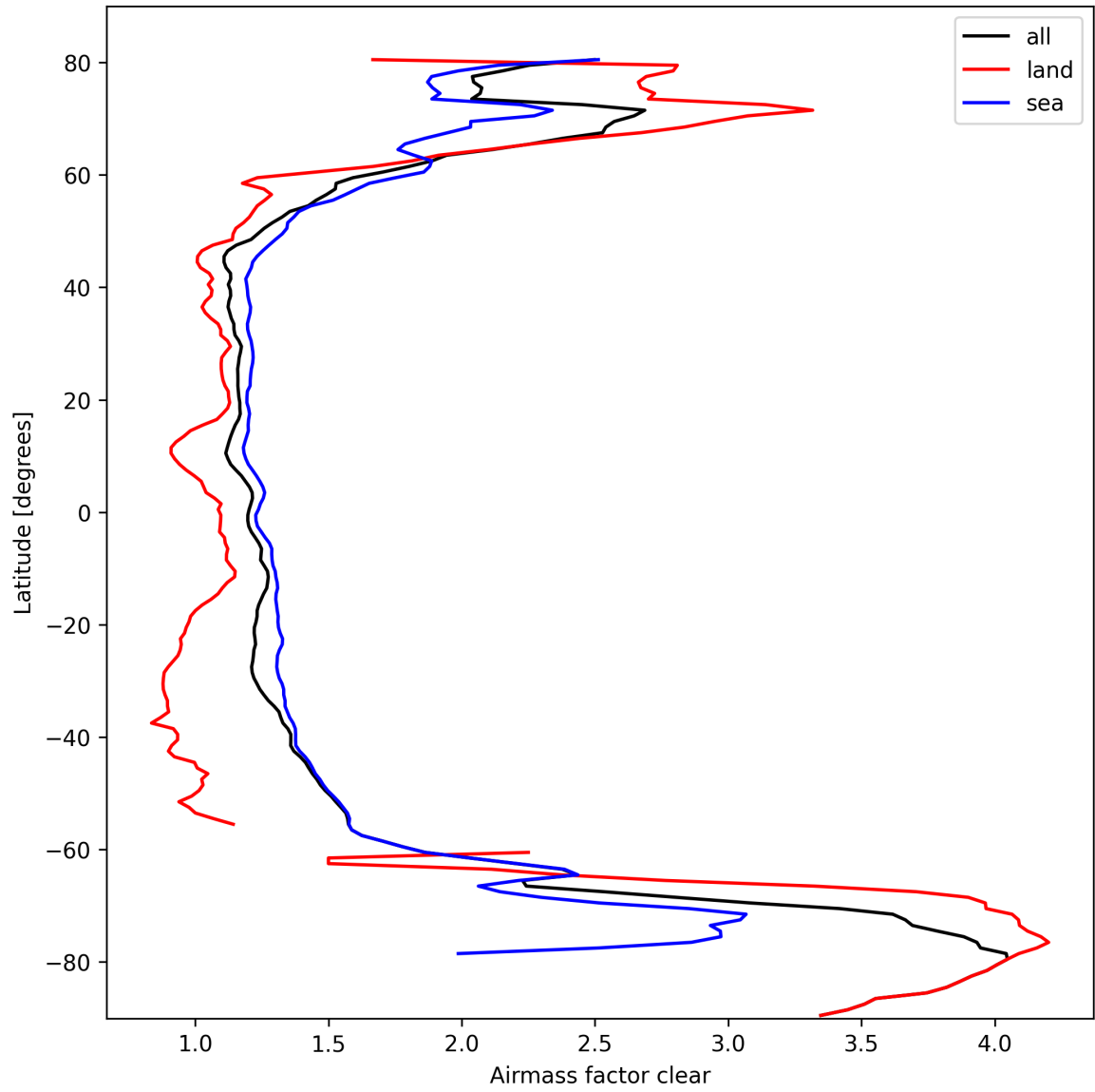
Figure 26: Zonal average of “Airmass factor clear” for 2025-03-07 to 2025-03-08.
