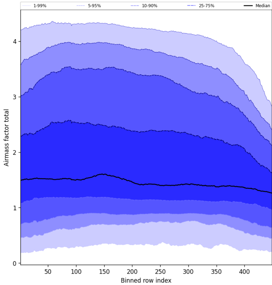
Figure 52: Along track statistics of “Airmass factor total” for 2025-03-07 to 2025-03-08
