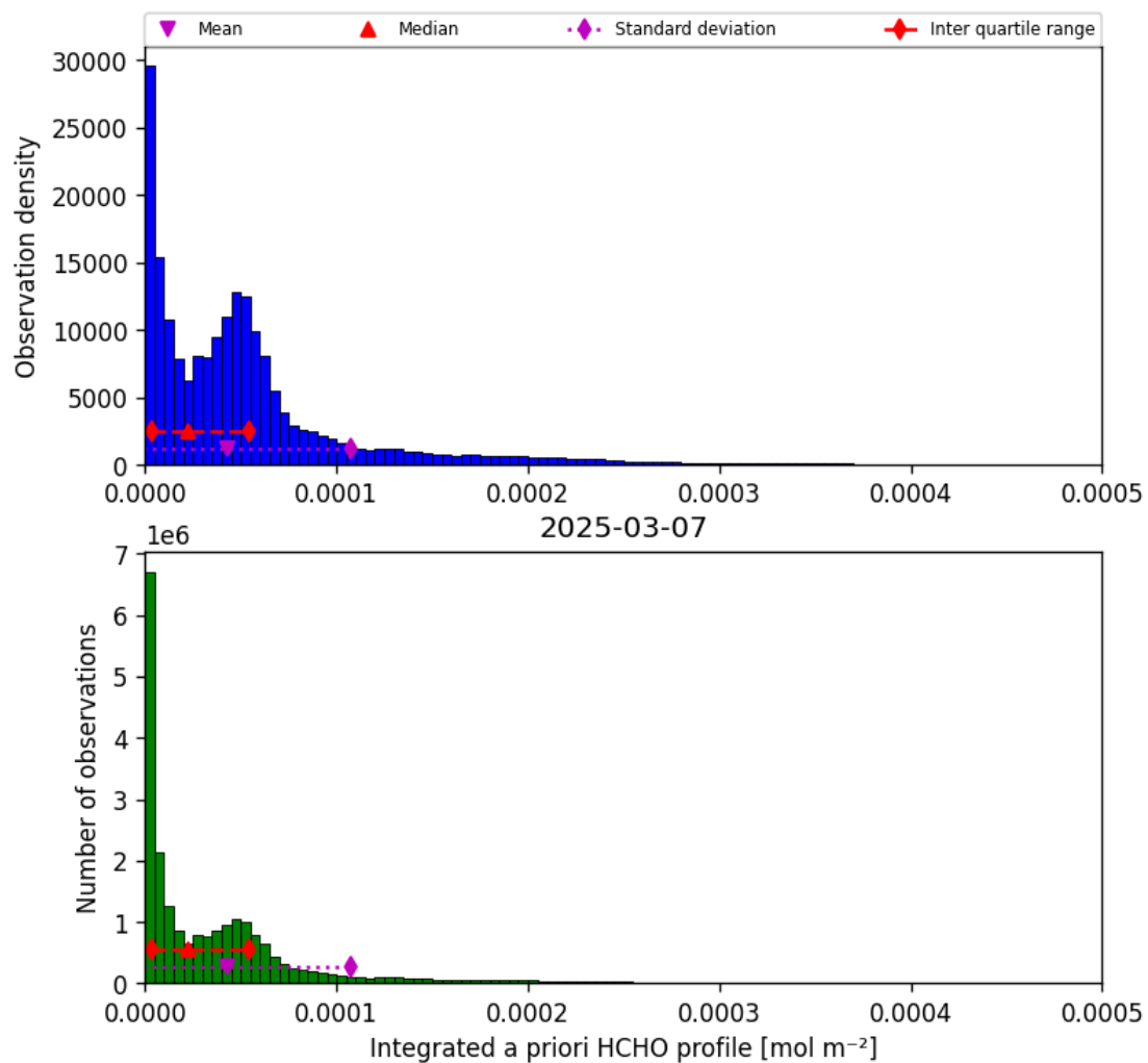
Figure 41: Histogram of “Integrated a priori HCHO profile” for 2025-03-07 to 2025-03-08
