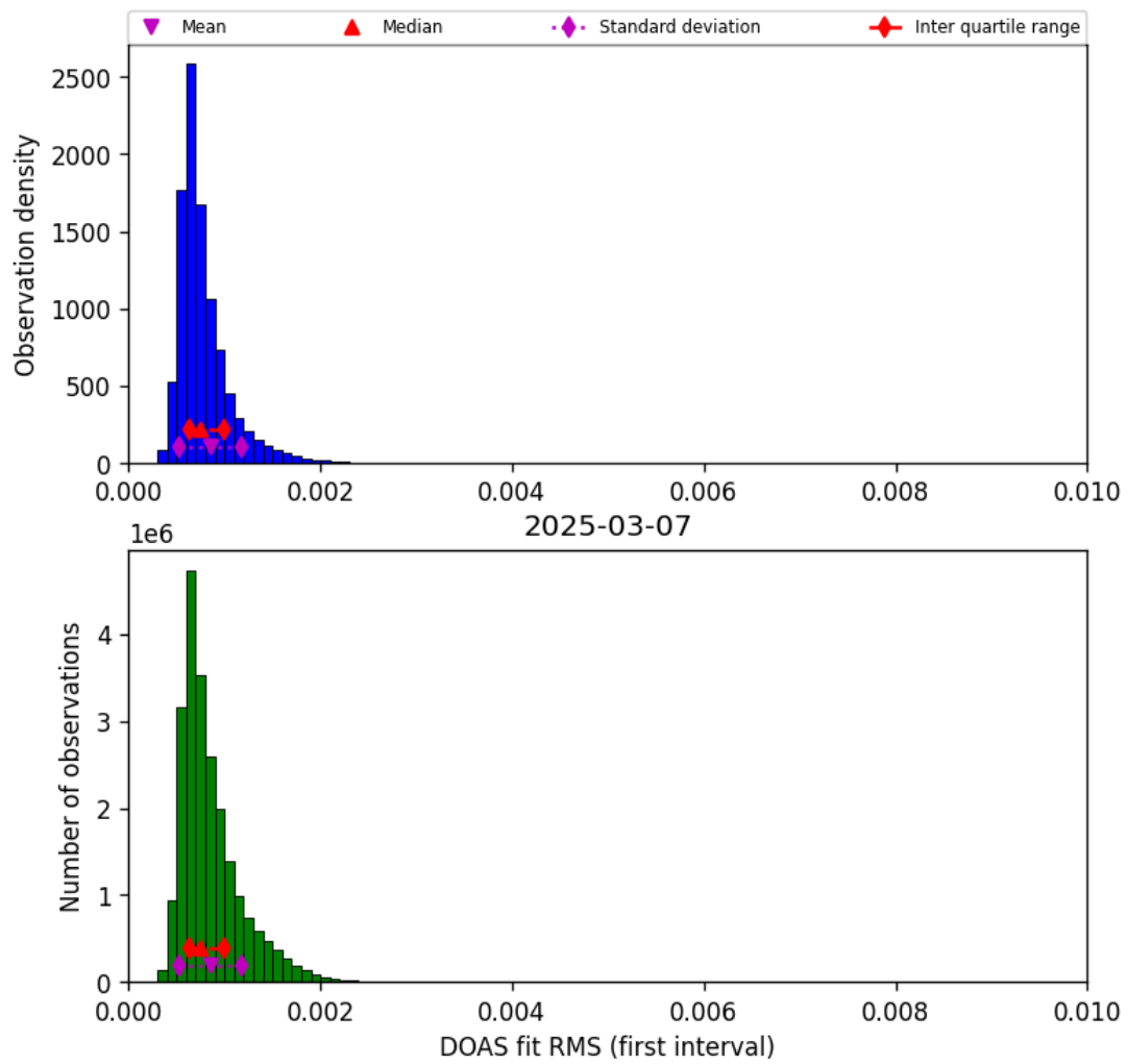
Figure 44: Histogram of “DOAS fit RMS (first interval)” for 2025-03-07 to 2025-03-08
