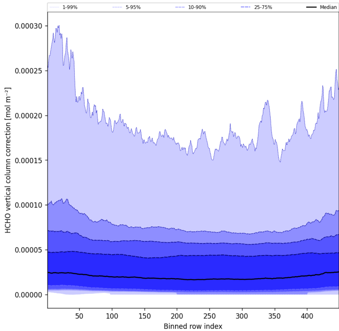
Figure 49: Along track statistics of “HCHO vertical column correction” for 2025-03-07 to 2025-03-08
