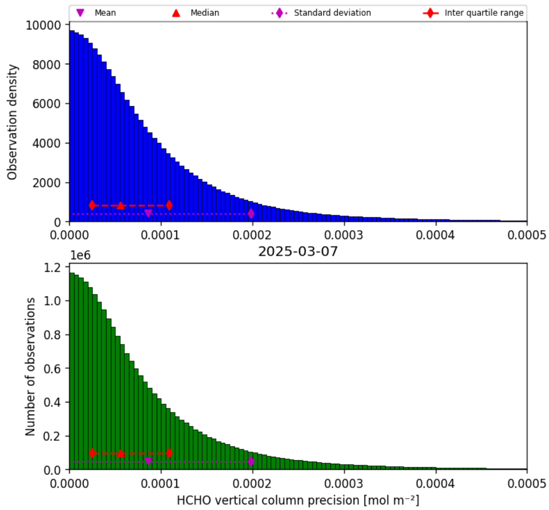
Figure 34: Histogram of “HCHO vertical column precision” for 2025-03-07 to 2025-03-08
