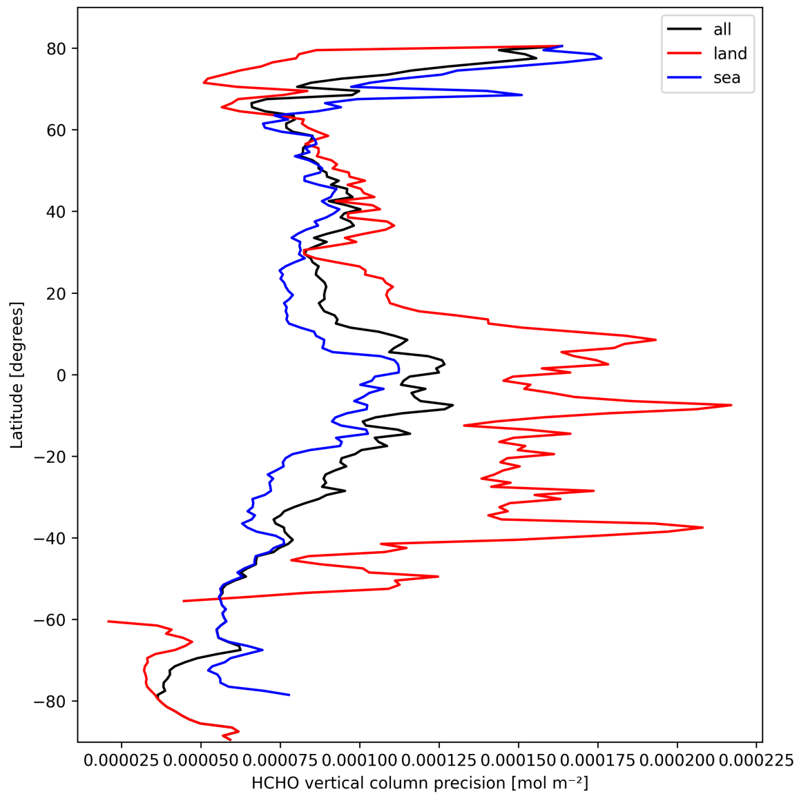
Figure 20: Zonal average of “HCHO vertical column precision” for 2025-03-07 to 2025-03-08.
