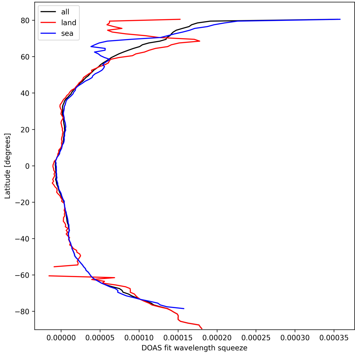
Figure 29: Zonal average of “DOAS fit wavelength squeeze” for 2025-03-07 to 2025-03-08.
