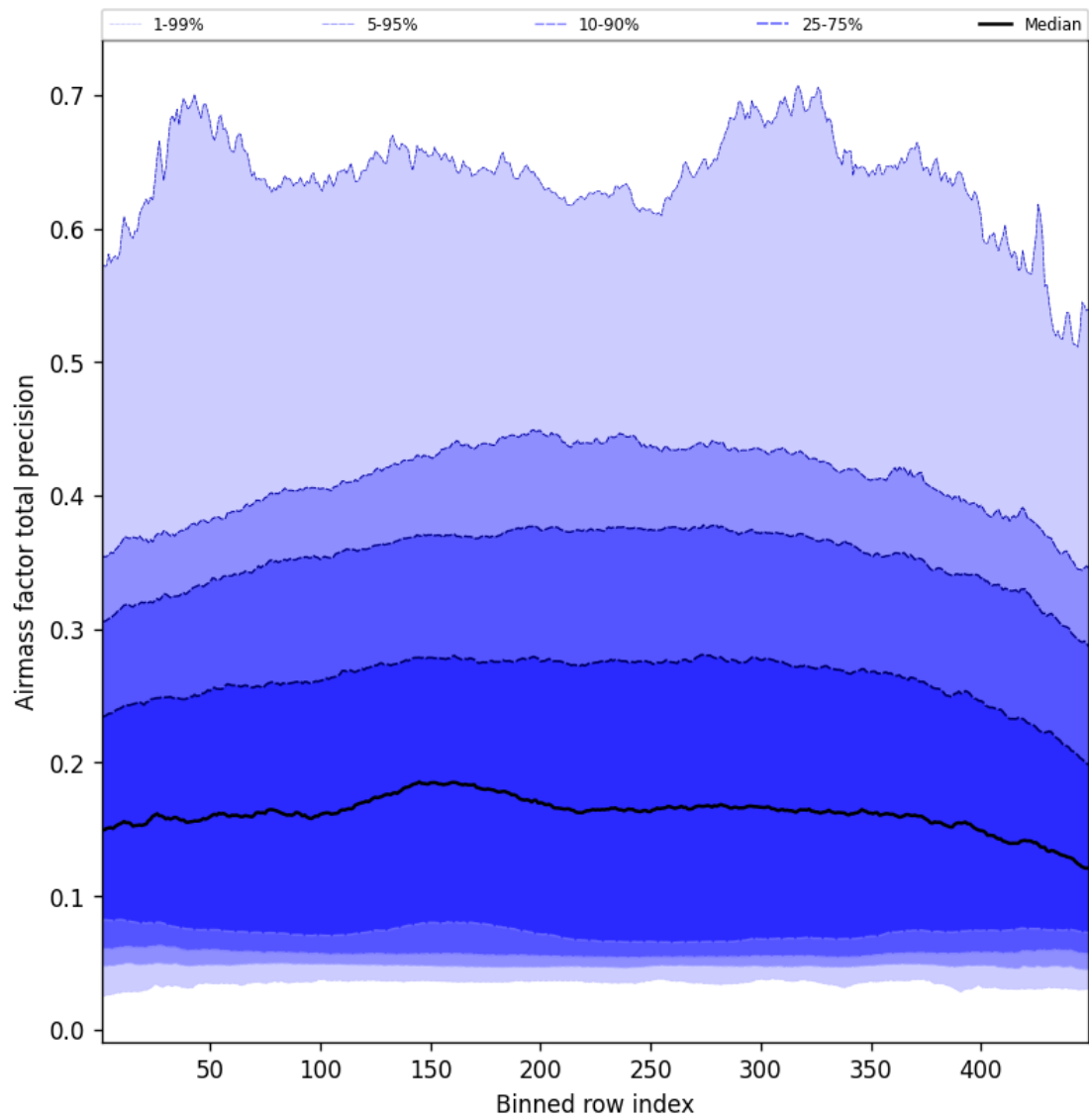
Figure 53: Along track statistics of “Airmass factor total precision” for 2025-03-07 to 2025-03-08
