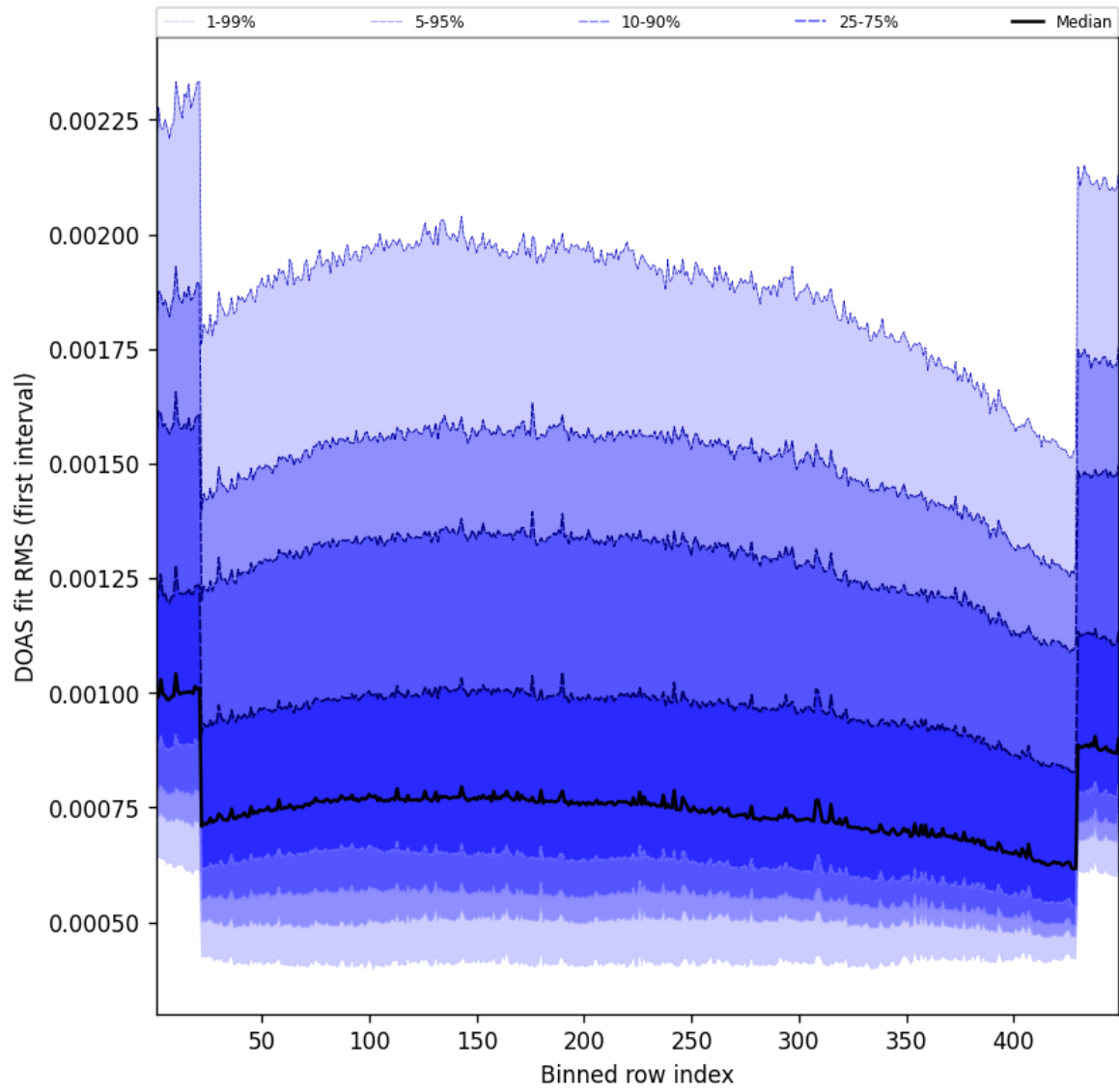
Figure 58: Along track statistics of “DOAS fit RMS (first interval)” for 2025-03-07 to 2025-03-08
