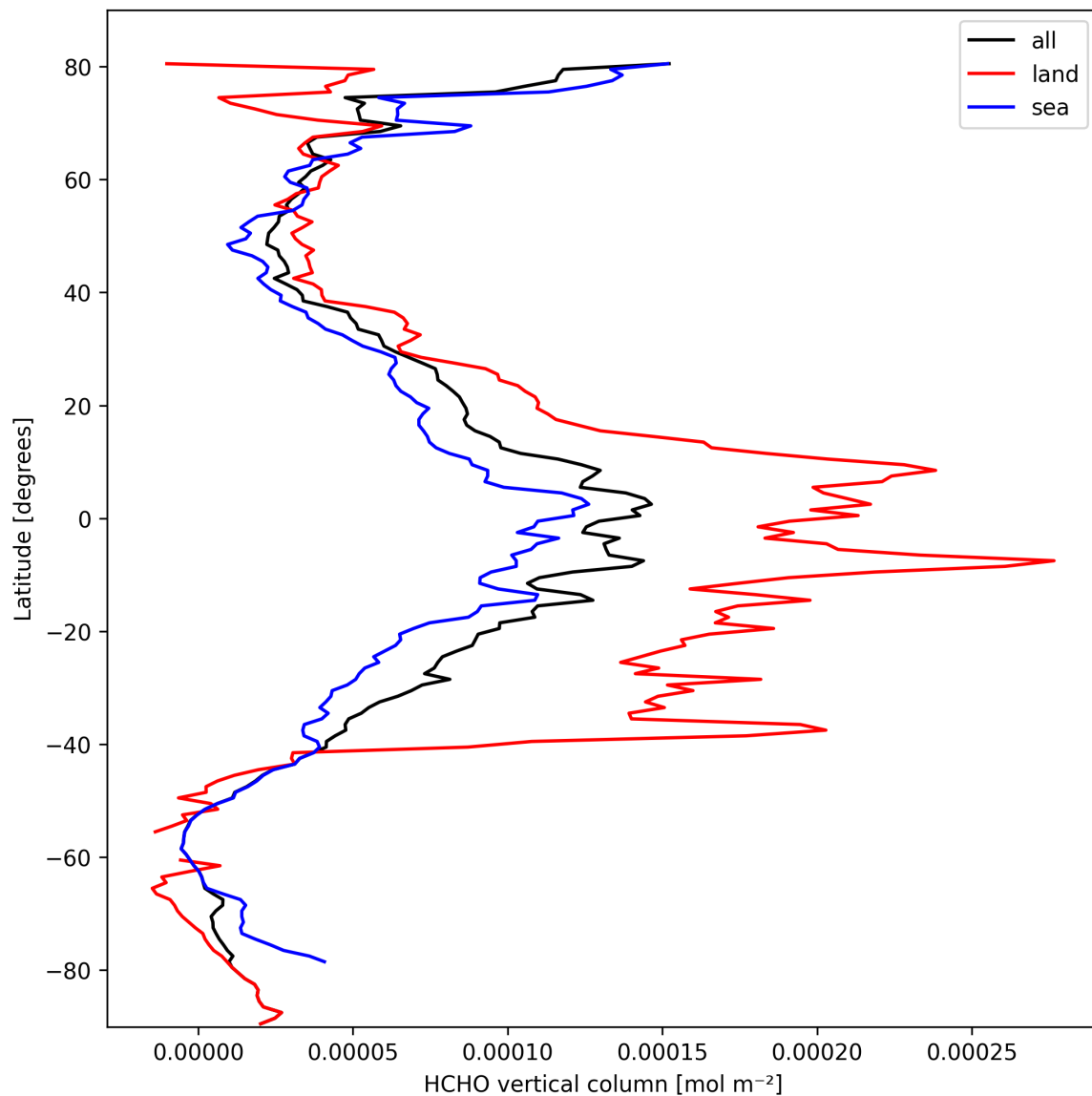
Figure 19: Zonal average of “HCHO vertical column” for 2025-03-07 to 2025-03-08.
