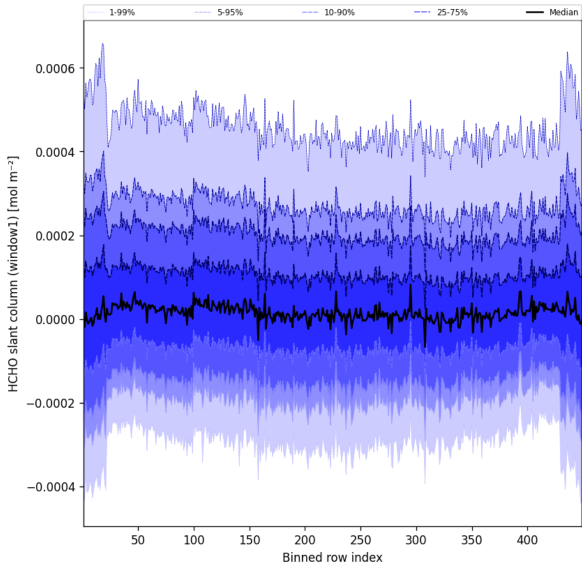
Figure 50: Along track statistics of “HCHO slant column (window1)” for 2025-03-07 to 2025-03-08
