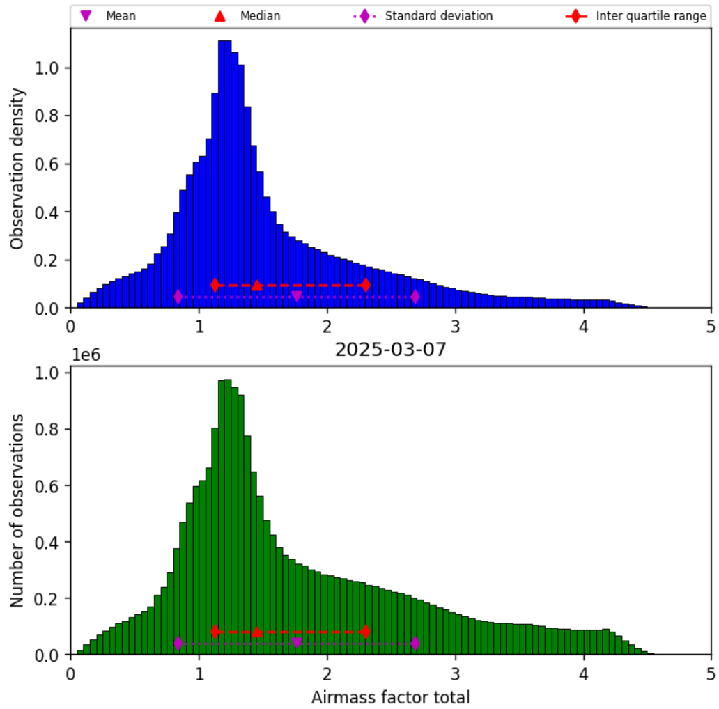
Figure 38: Histogram of “Airmass factor total” for 2025-03-07 to 2025-03-08
