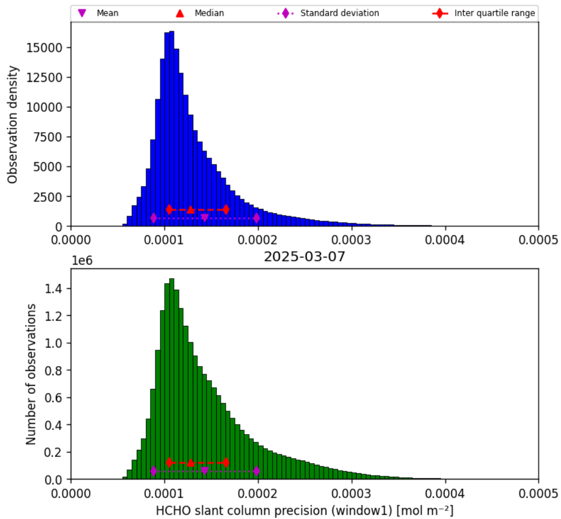
Figure 37: Histogram of “HCHO slant column precision (window1)” for 2025-03-07 to 2025-03-08
