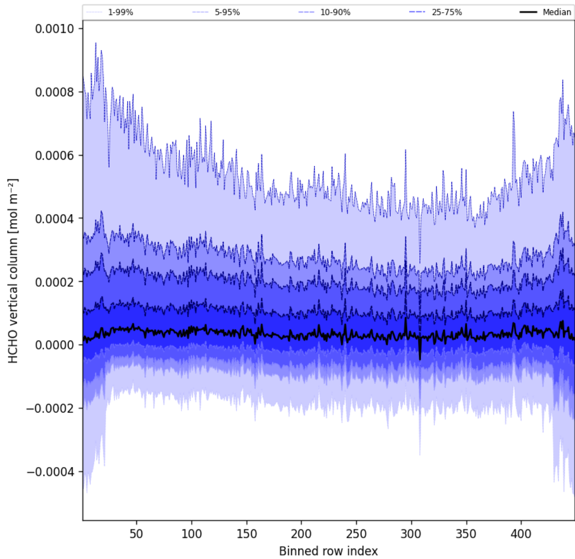
Figure 47: Along track statistics of “HCHO vertical column” for 2025-03-07 to 2025-03-08
