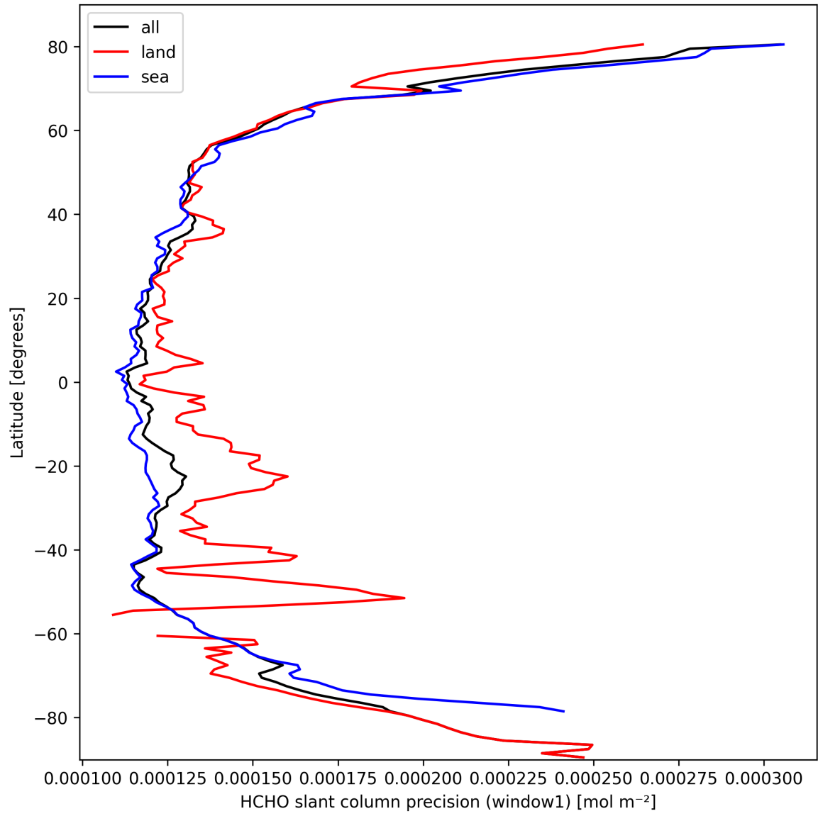
Figure 23: Zonal average of “HCHO slant column precision (window1)” for 2025-03-07 to 2025-03-08.
