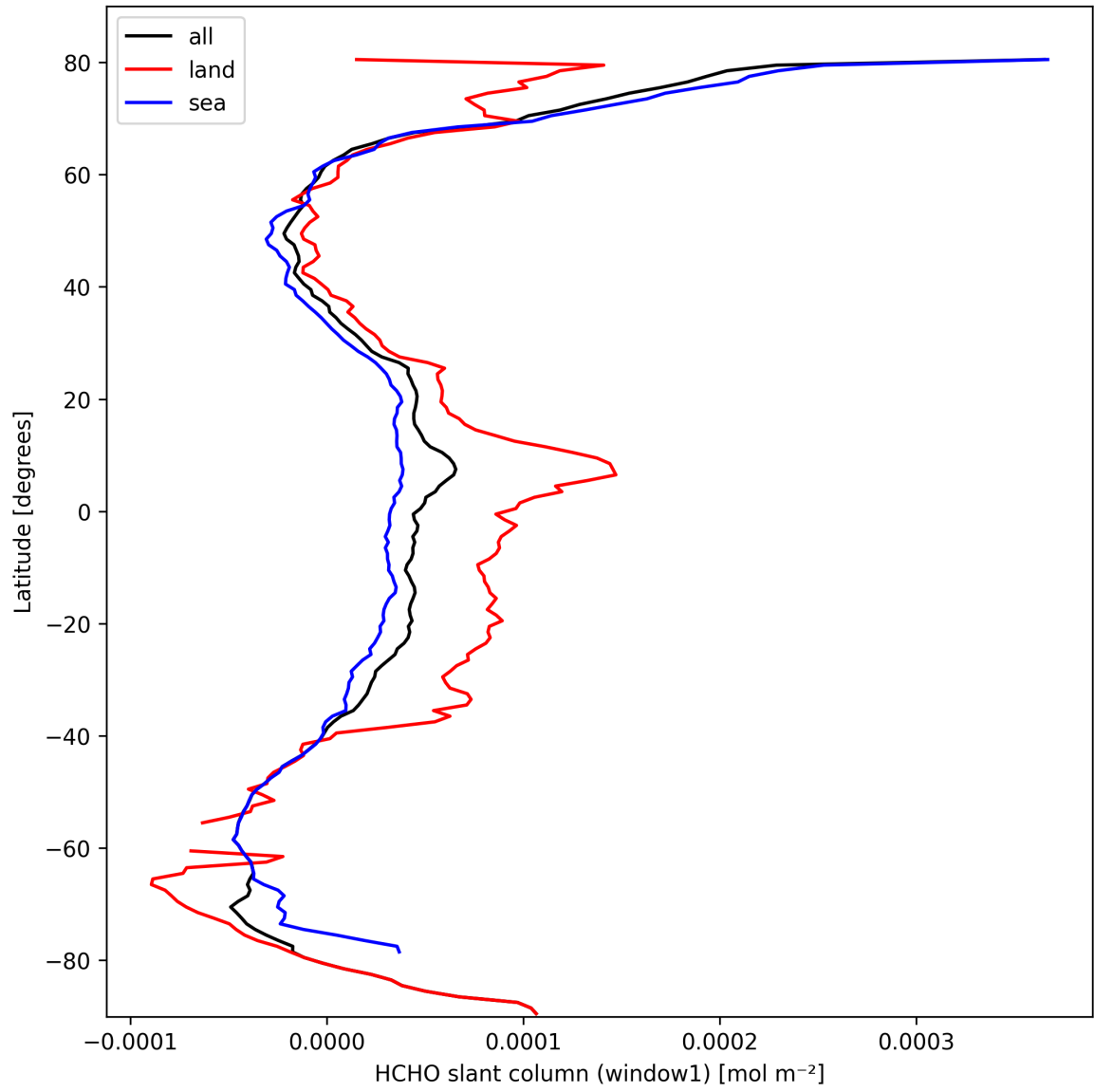
Figure 22: Zonal average of “HCHO slant column (window1)” for 2025-03-07 to 2025-03-08.
