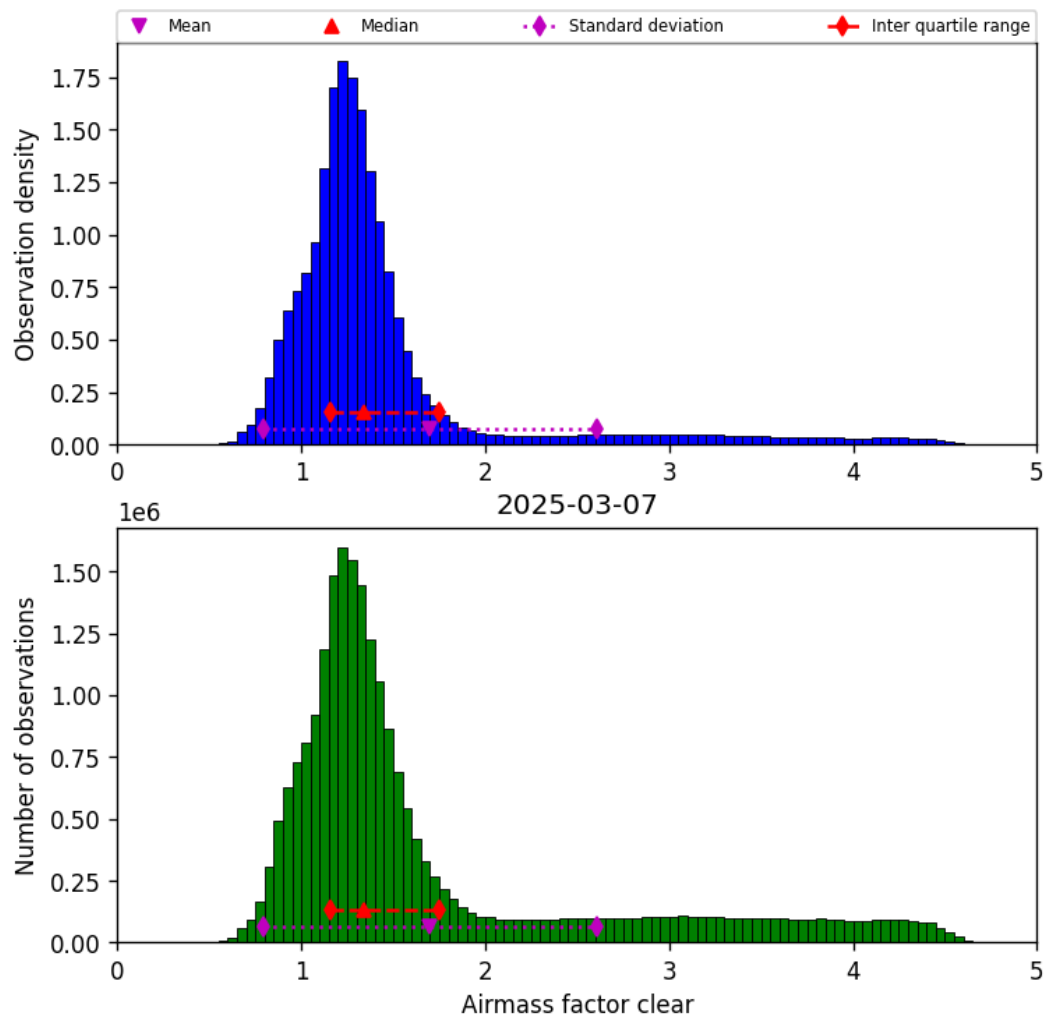
Figure 40: Histogram of “Airmass factor clear” for 2025-03-07 to 2025-03-08
