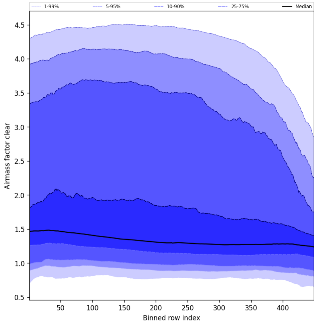
Figure 54: Along track statistics of “Airmass factor clear” for 2025-03-07 to 2025-03-08
