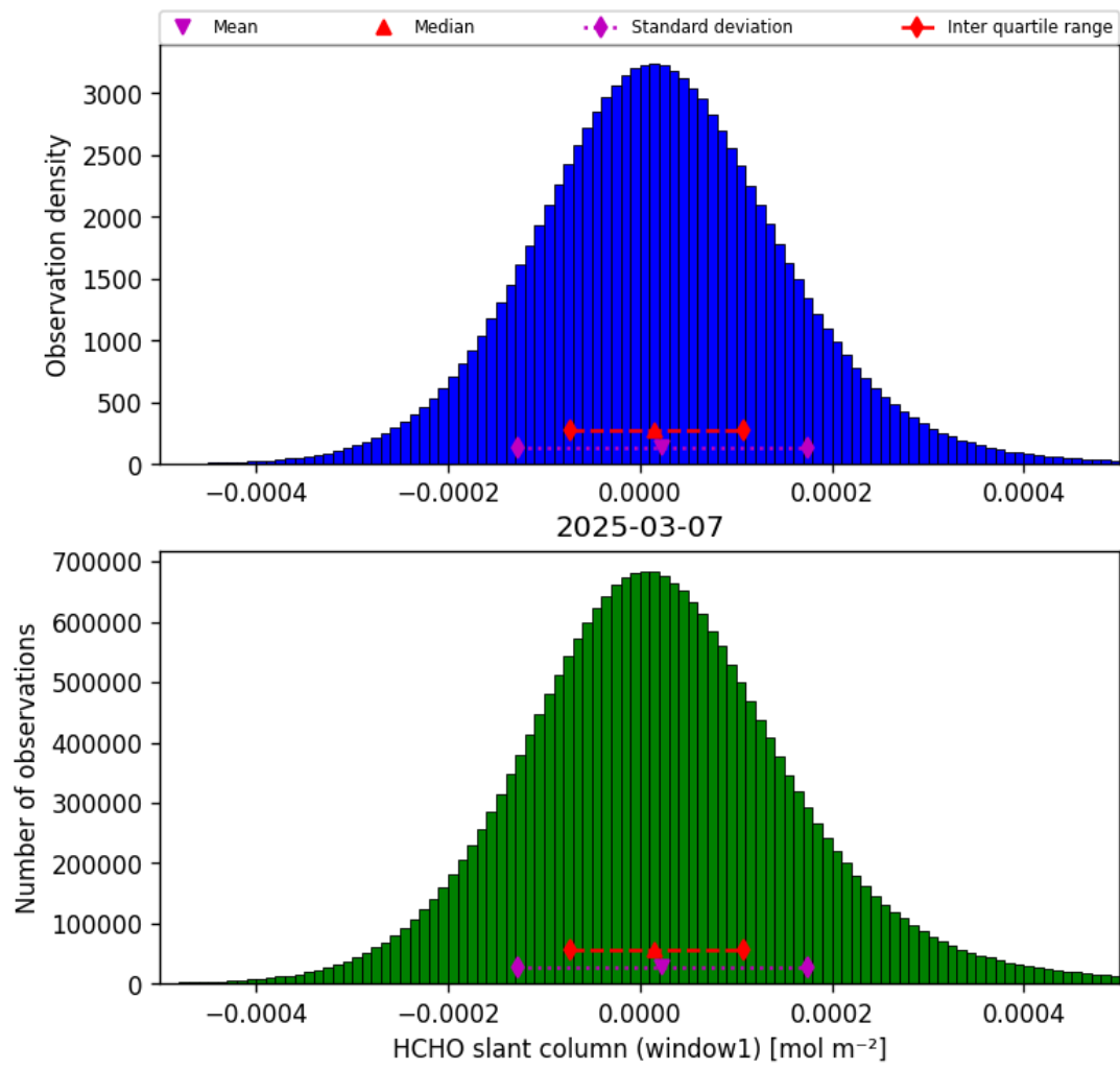
Figure 36: Histogram of “HCHO slant column (window1)” for 2025-03-07 to 2025-03-08
