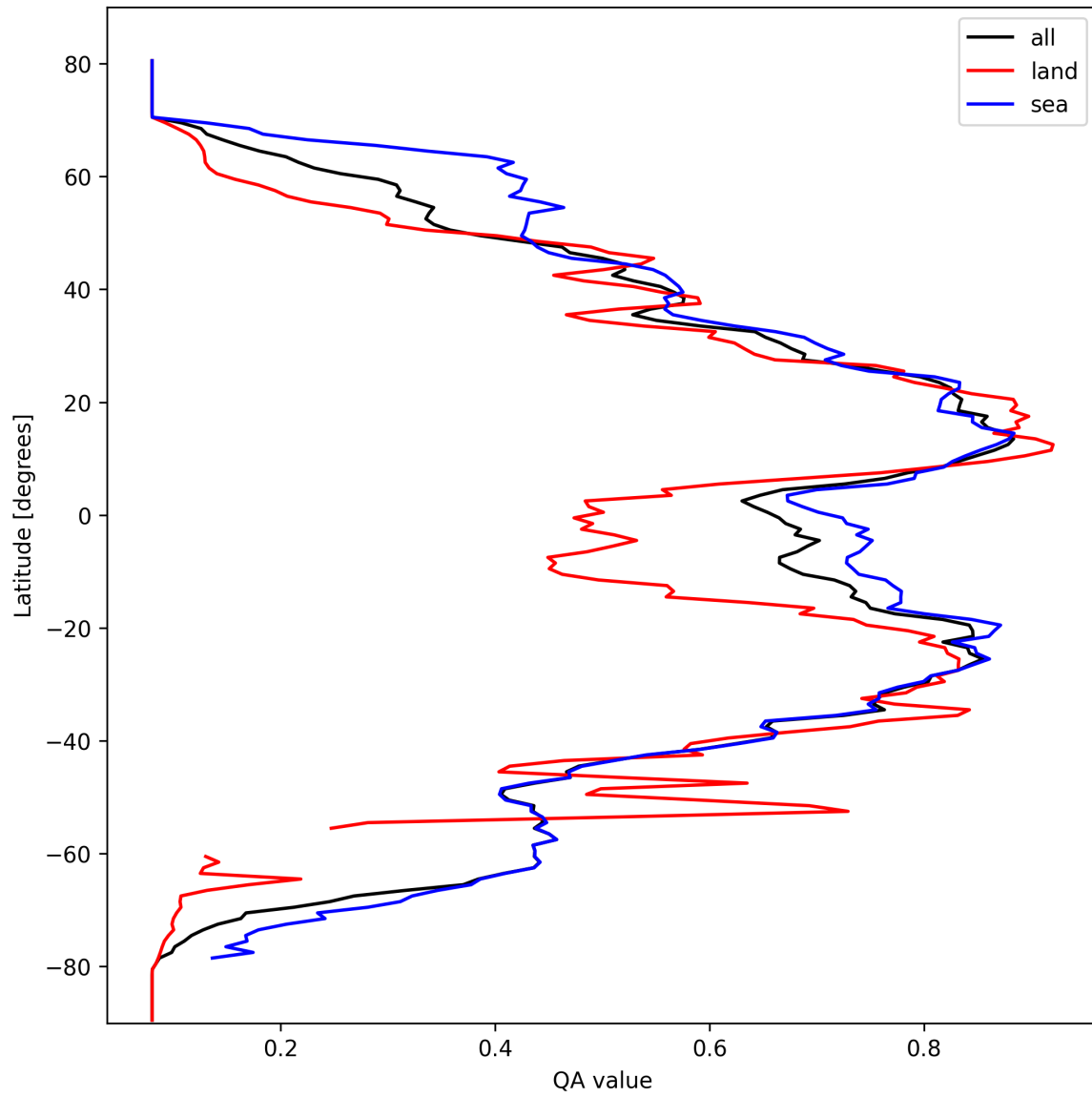
Figure 18: Zonal average of “QA value” for 2025-03-07 to 2025-03-08.
