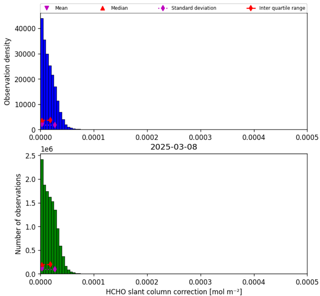
Figure 45: Histogram of “HCHO slant column correction” for 2025-03-08 to 2025-03-09
