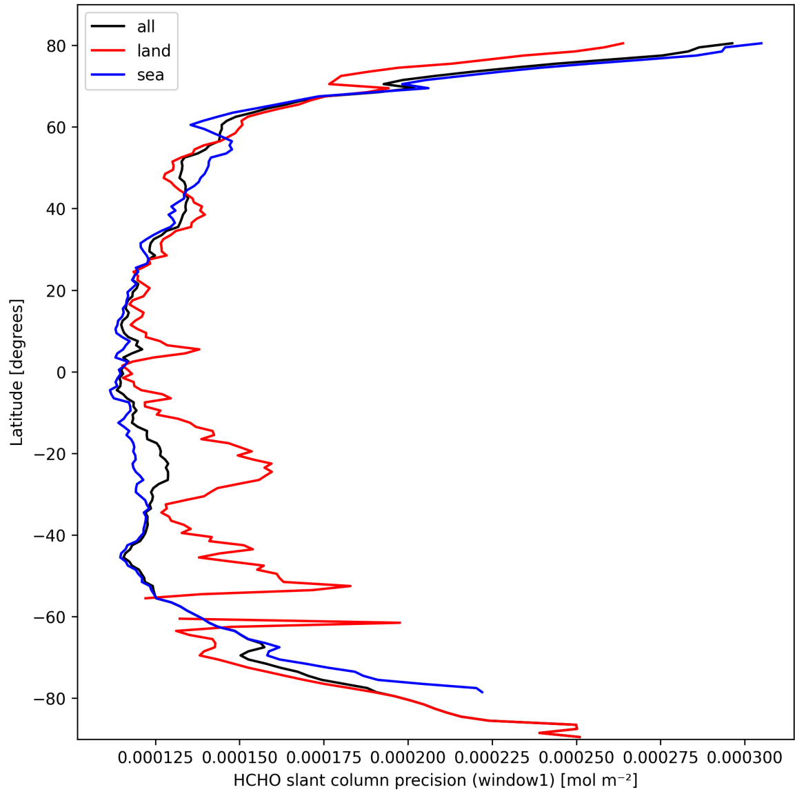
Figure 23: Zonal average of “HCHO slant column precision (window1)” for 2025-03-08 to 2025-03-09.
