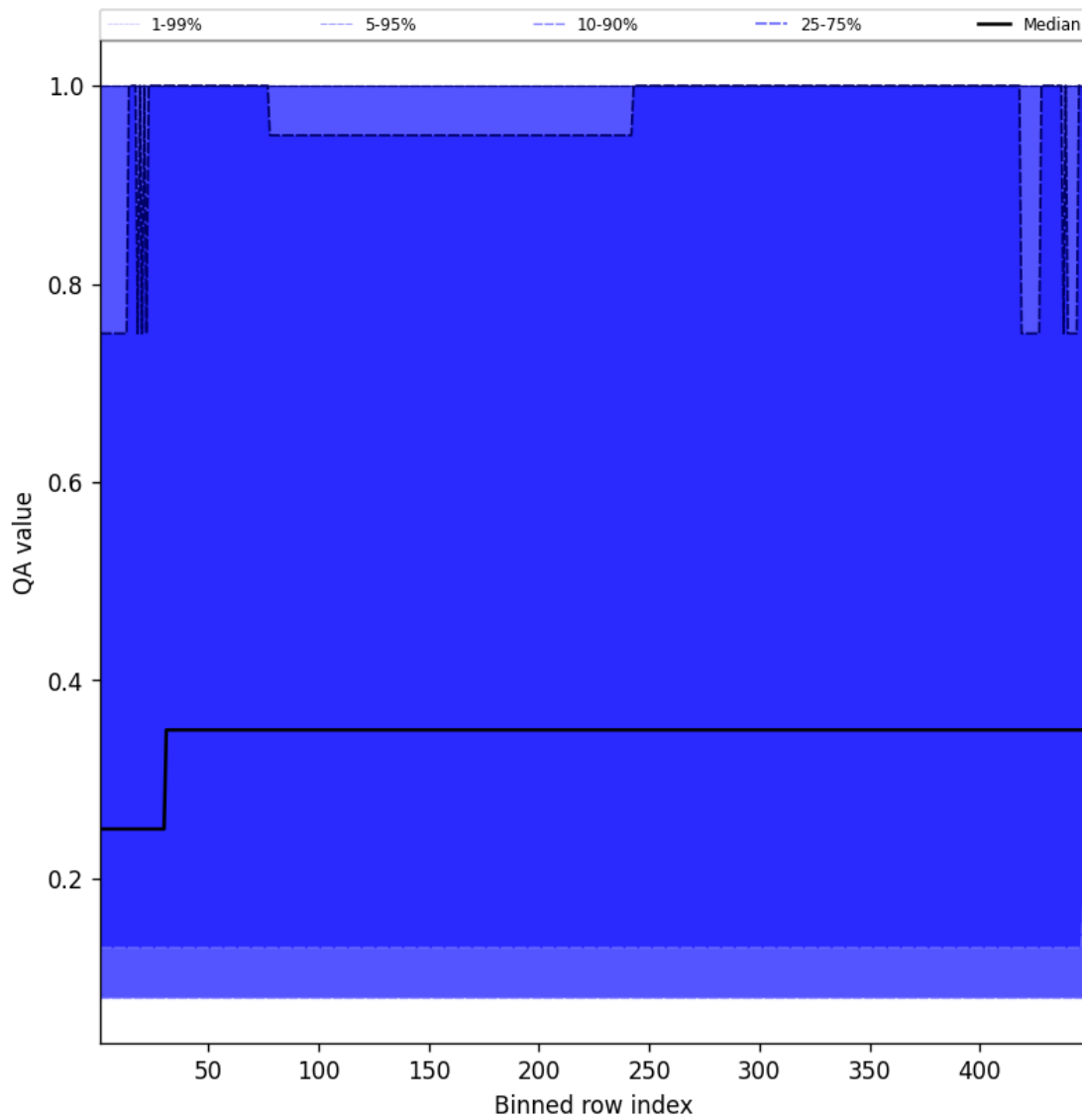
Figure 46: Along track statistics of “QA value” for 2025-03-08 to 2025-03-09
