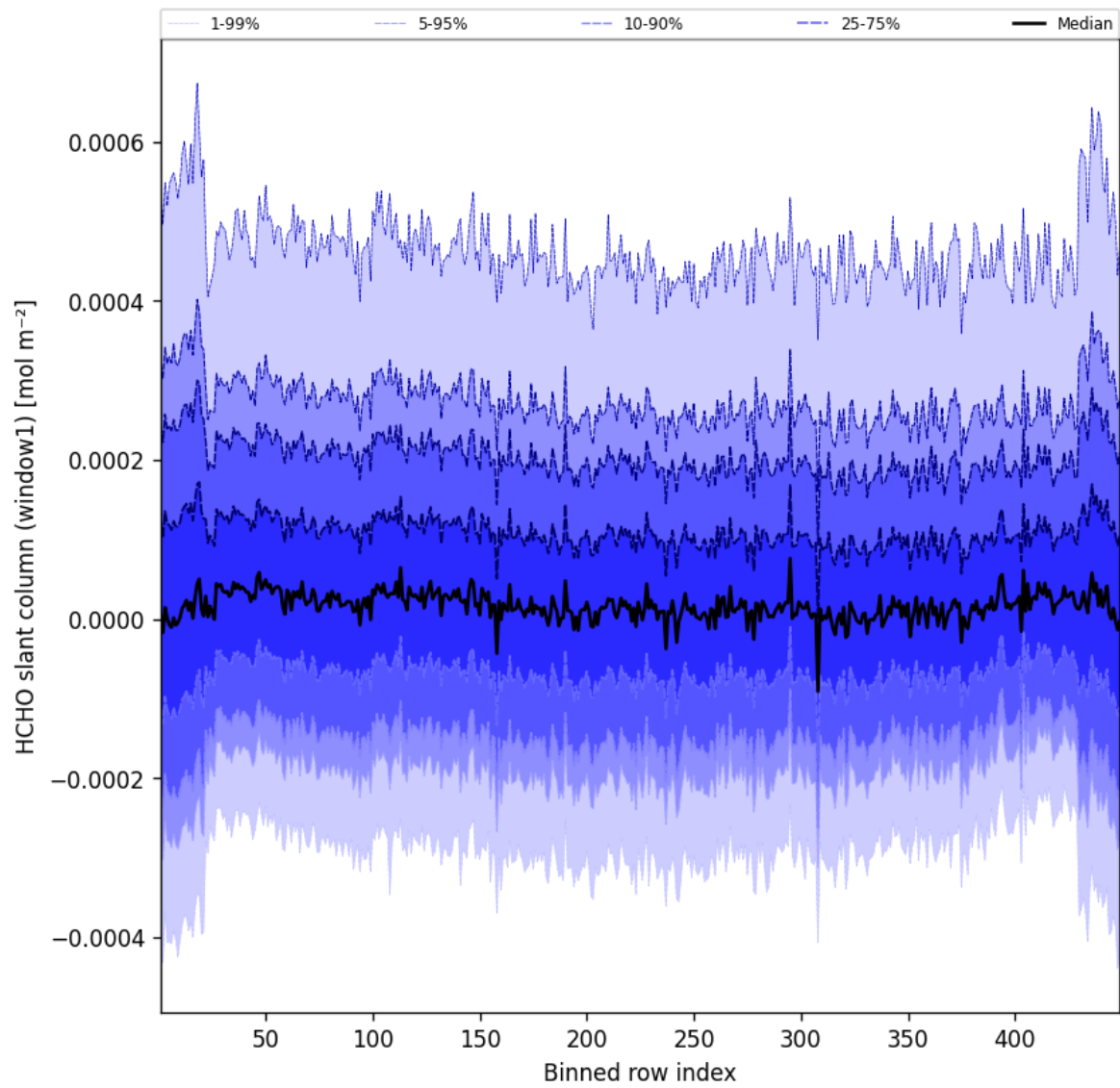
Figure 50: Along track statistics of “HCHO slant column (window1)” for 2025-03-08 to 2025-03-09
