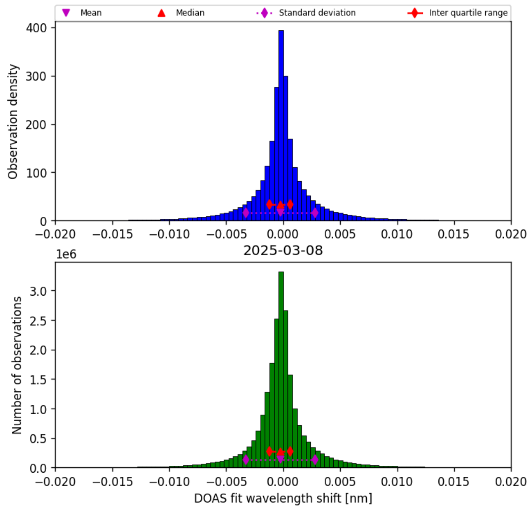
Figure 42: Histogram of “DOAS fit wavelength shift” for 2025-03-08 to 2025-03-09
