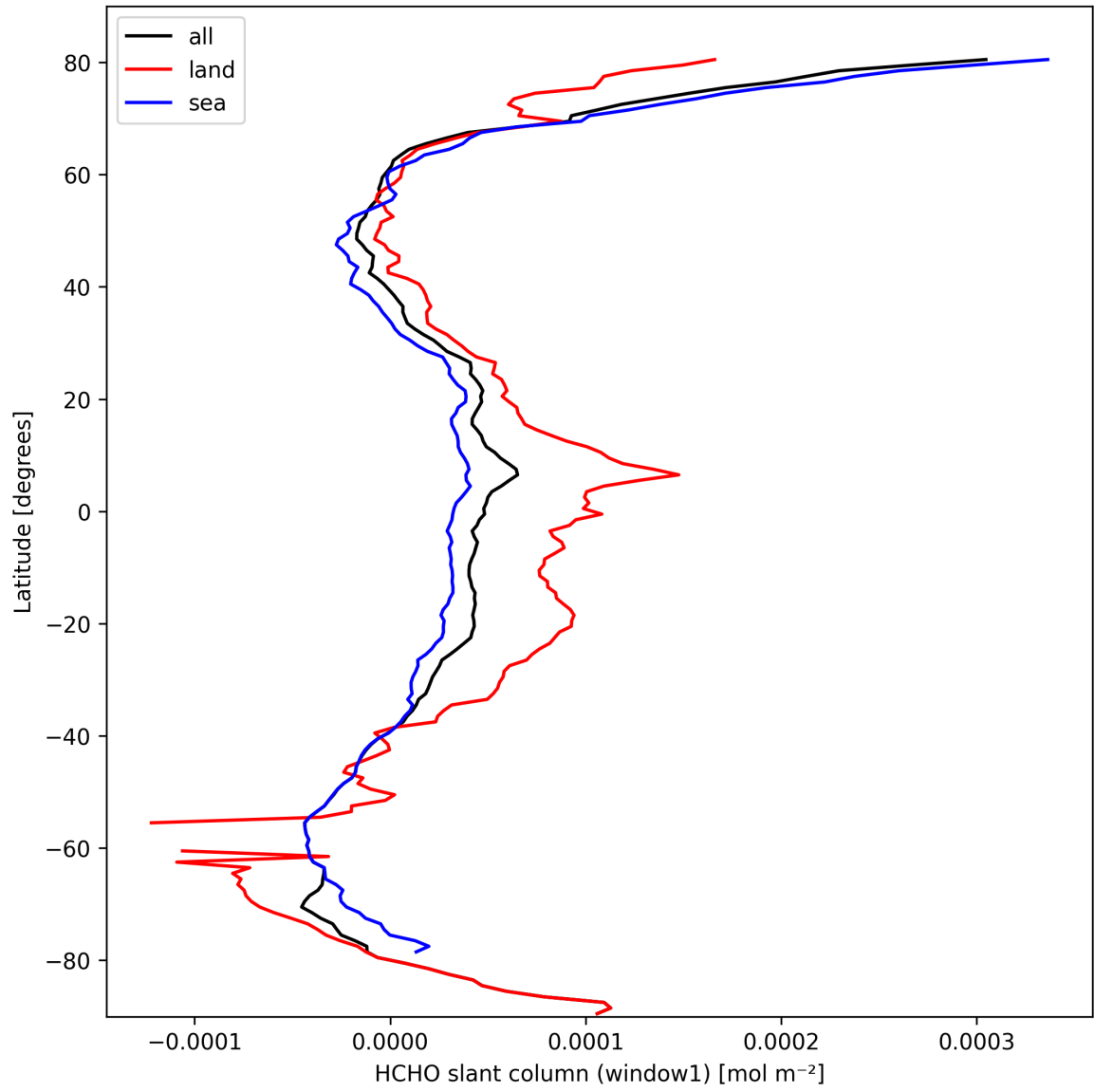
Figure 22: Zonal average of “HCHO slant column (window1)” for 2025-03-08 to 2025-03-09.
