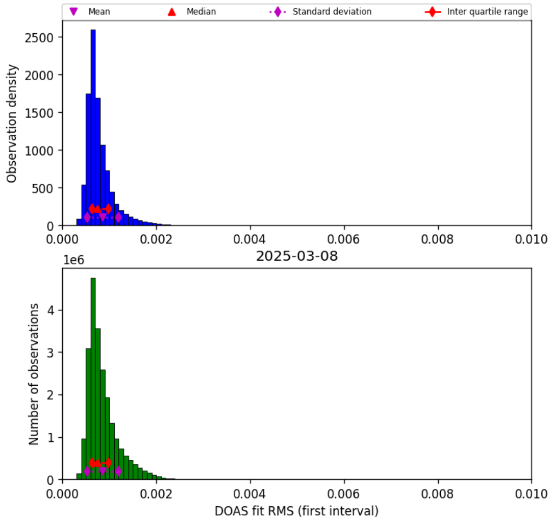
Figure 44: Histogram of “DOAS fit RMS (first interval)” for 2025-03-08 to 2025-03-09
