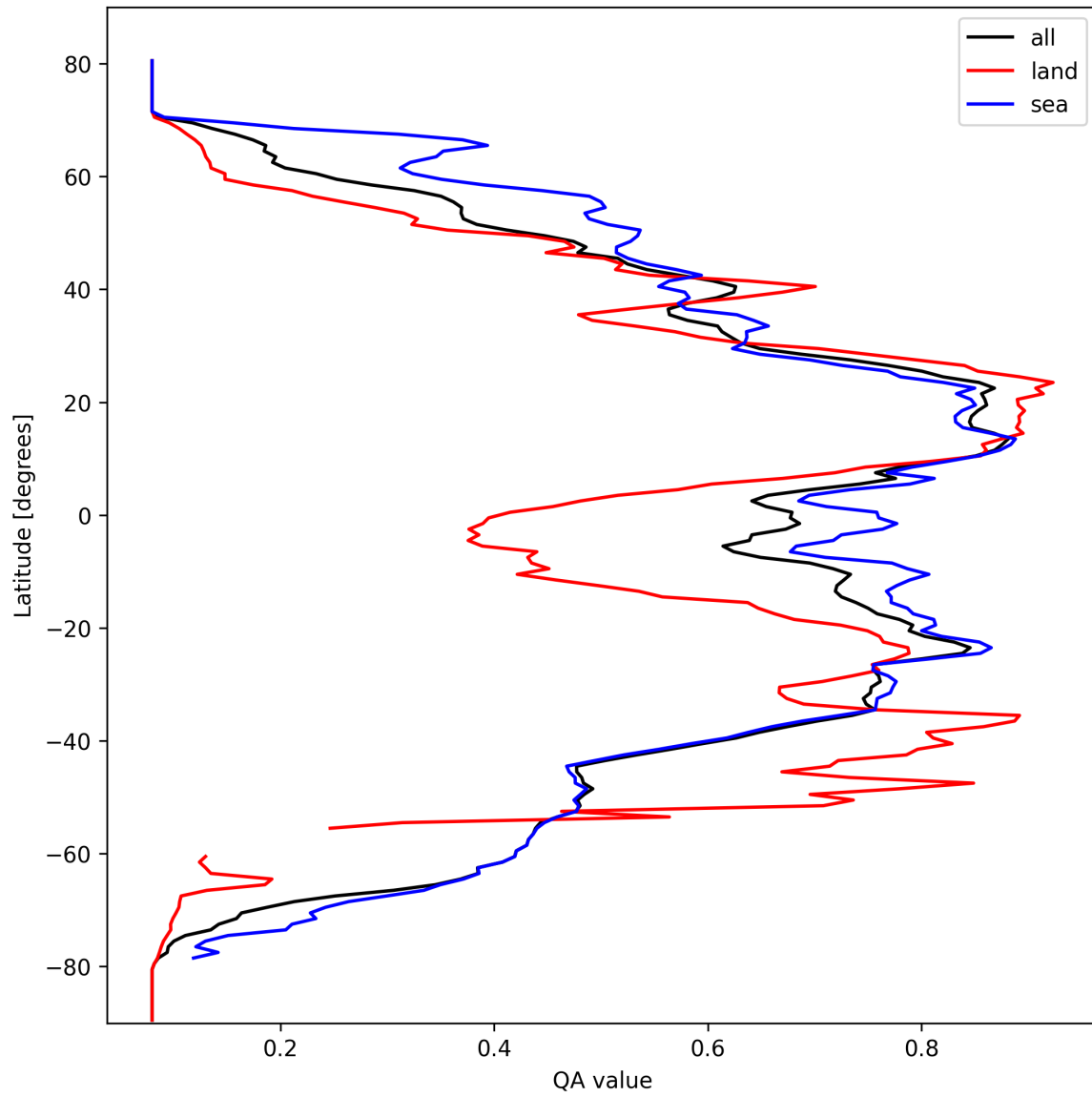
Figure 18: Zonal average of “QA value” for 2025-03-08 to 2025-03-09.
