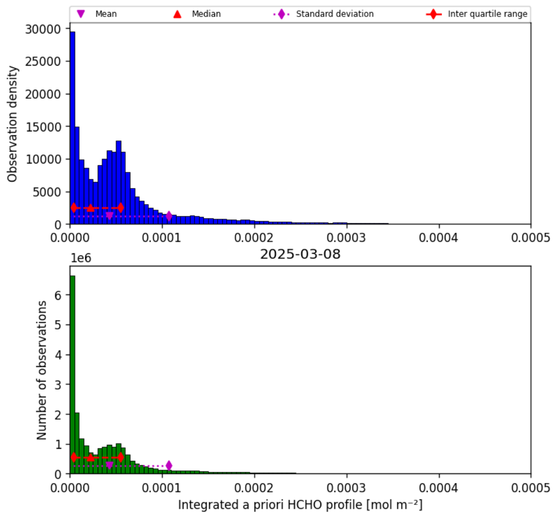
Figure 41: Histogram of “Integrated a priori HCHO profile” for 2025-03-08 to 2025-03-09
