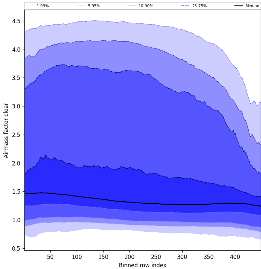
Figure 54: Along track statistics of “Airmass factor clear” for 2025-03-08 to 2025-03-09
