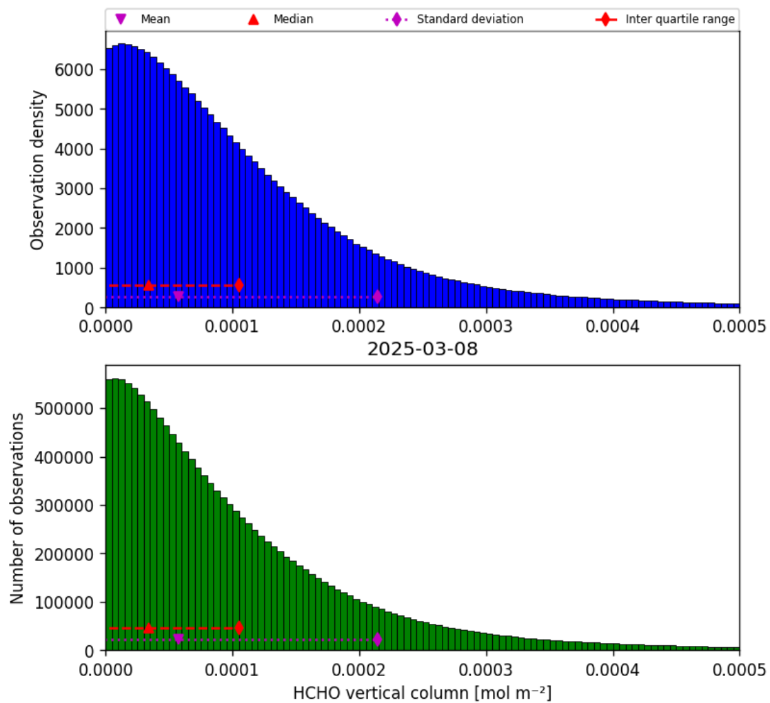
Figure 33: Histogram of “HCHO vertical column” for 2025-03-08 to 2025-03-09
