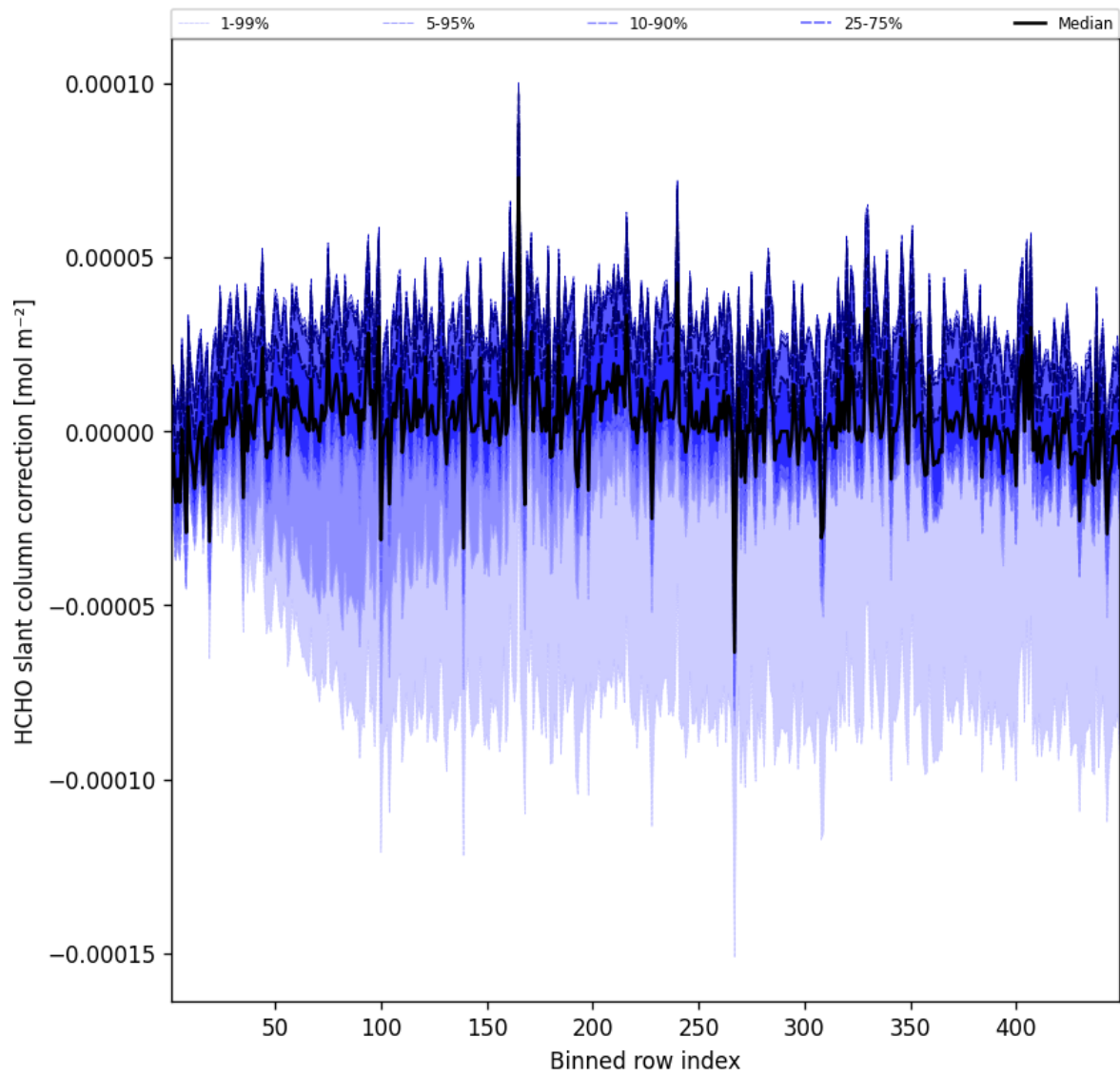
Figure 59: Along track statistics of “HCHO slant column correction” for 2025-03-08 to 2025-03-09
