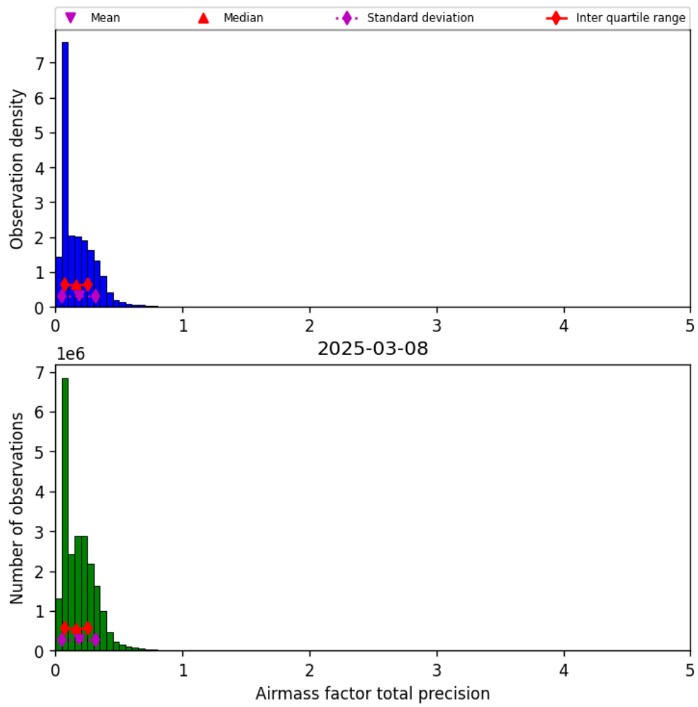
Figure 39: Histogram of “Airmass factor total precision” for 2025-03-08 to 2025-03-09
