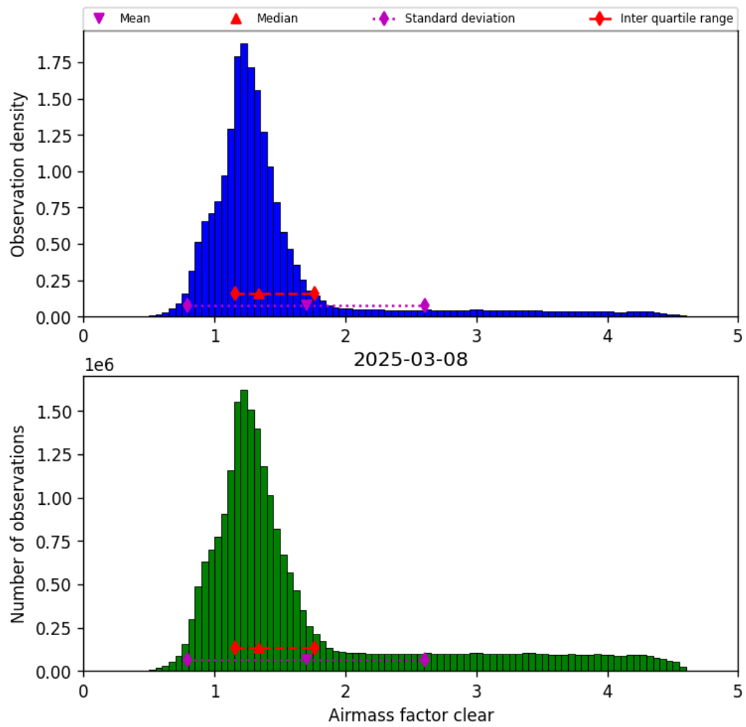
Figure 40: Histogram of “Airmass factor clear” for 2025-03-08 to 2025-03-09
