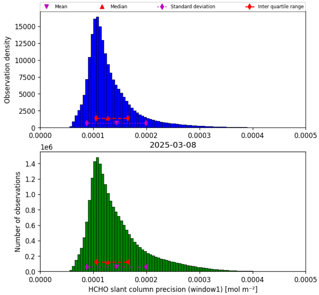
Figure 37: Histogram of “HCHO slant column precision (window1)” for 2025-03-08 to 2025-03-09
