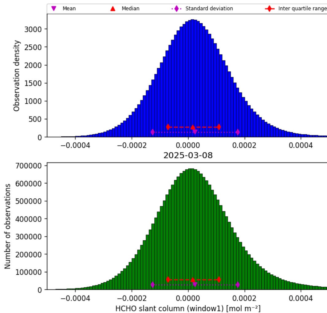
Figure 36: Histogram of “HCHO slant column (window1)” for 2025-03-08 to 2025-03-09
