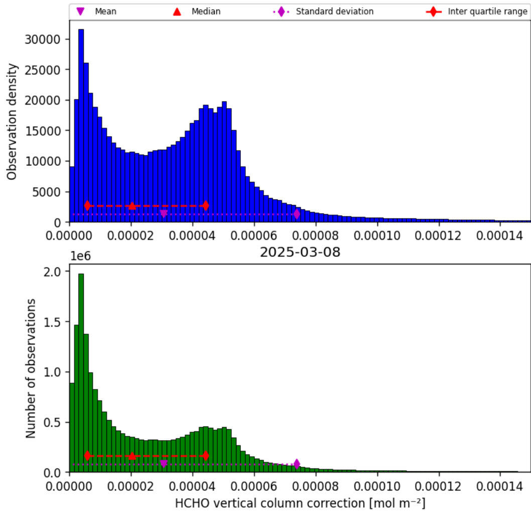
Figure 35: Histogram of “HCHO vertical column correction” for 2025-03-08 to 2025-03-09
