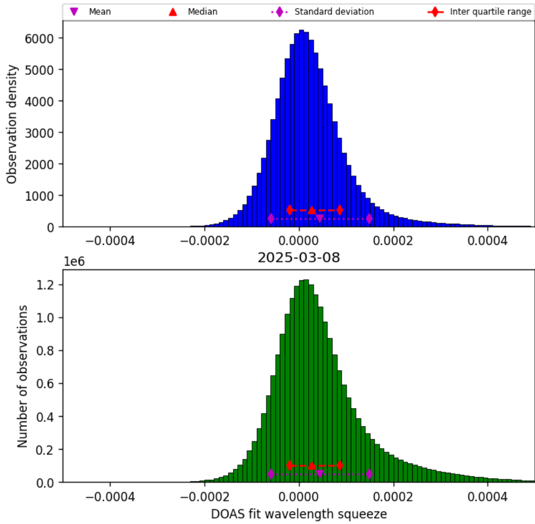
Figure 43: Histogram of “DOAS fit wavelength squeeze” for 2025-03-08 to 2025-03-09
