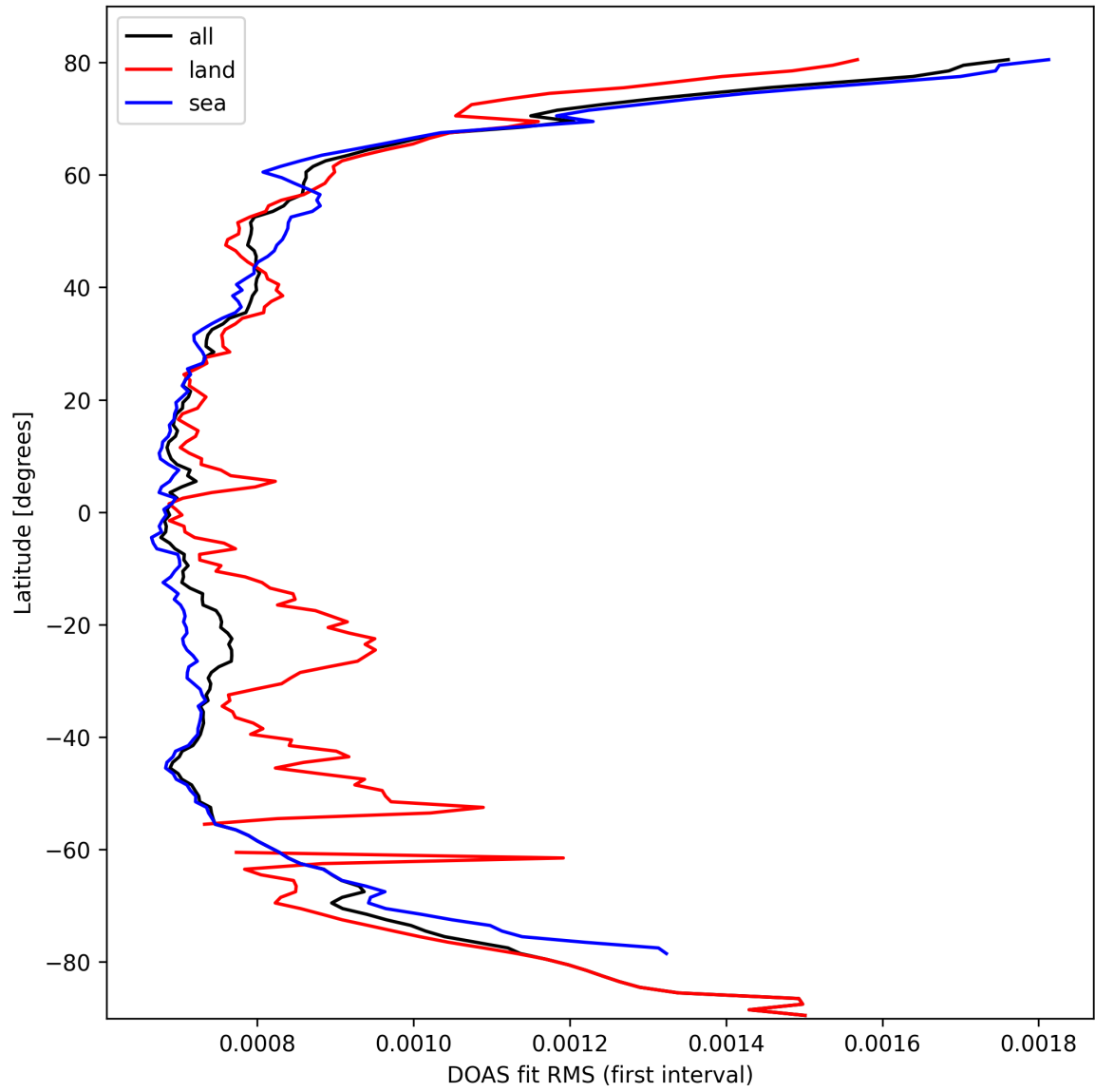
Figure 30: Zonal average of "DOAS fit RMS (first interval)" for 2025-03-08 to 2025-03-09.
