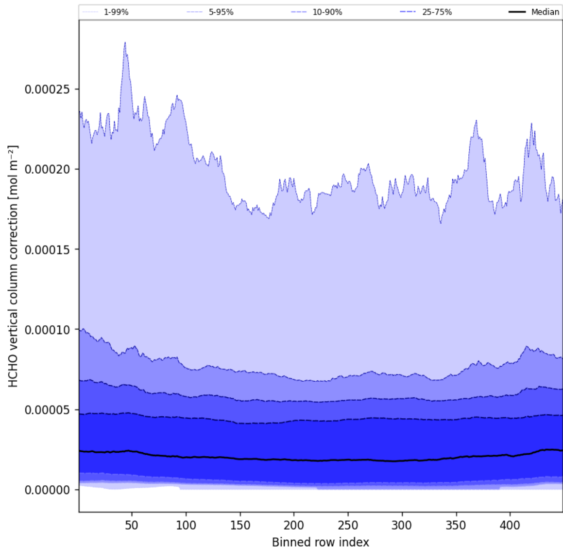
Figure 49: Along track statistics of “HCHO vertical column correction” for 2025-03-08 to 2025-03-09
