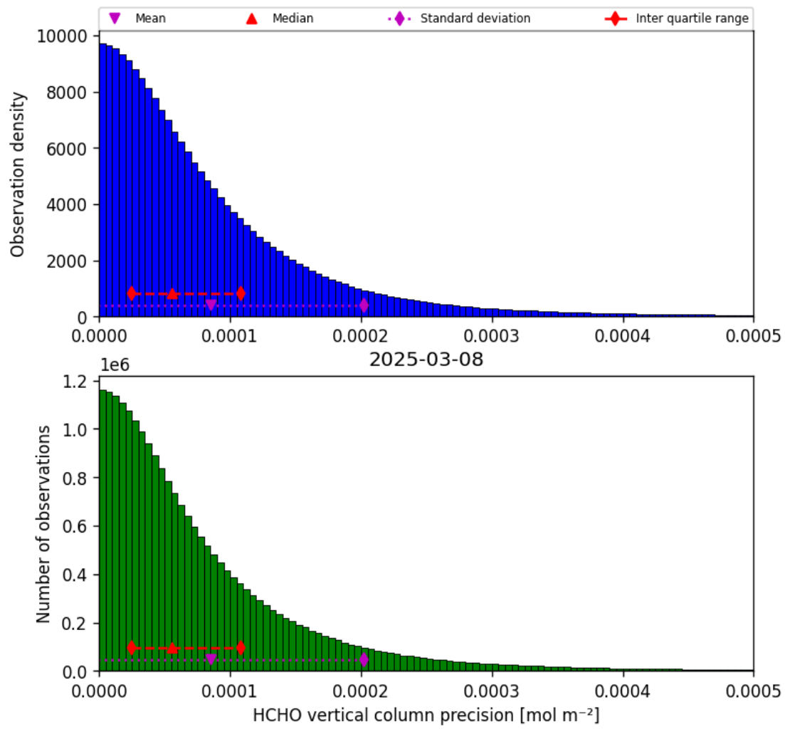
Figure 34: Histogram of “HCHO vertical column precision” for 2025-03-08 to 2025-03-09
