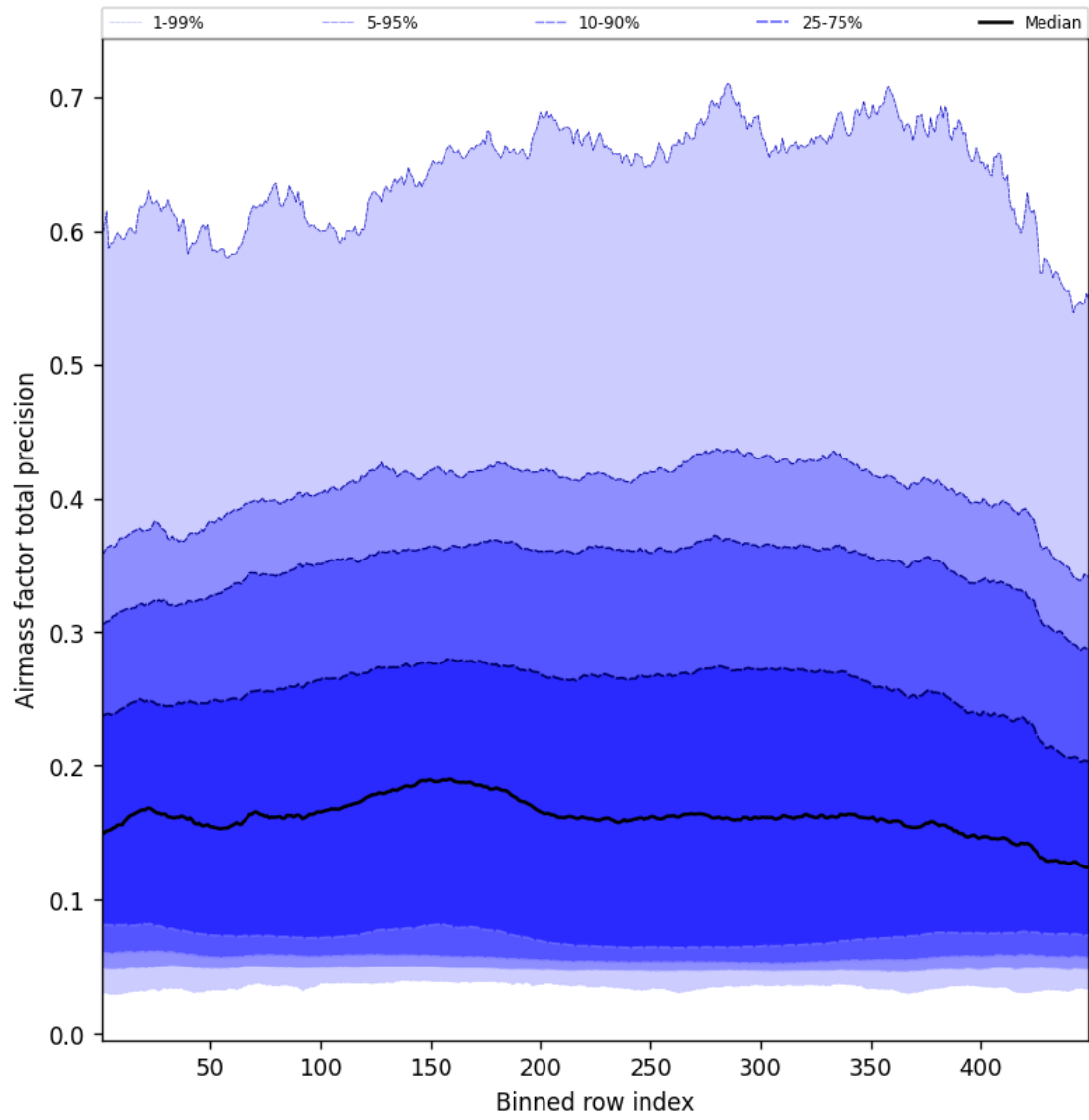
Figure 53: Along track statistics of “Airmass factor total precision” for 2025-03-08 to 2025-03-09
