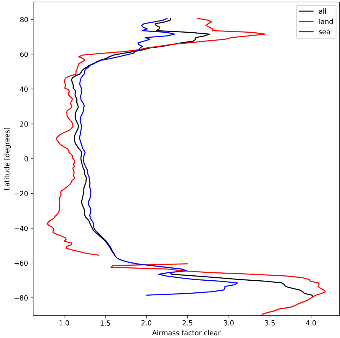
Figure 26: Zonal average of “Airmass factor clear” for 2025-03-08 to 2025-03-09.
