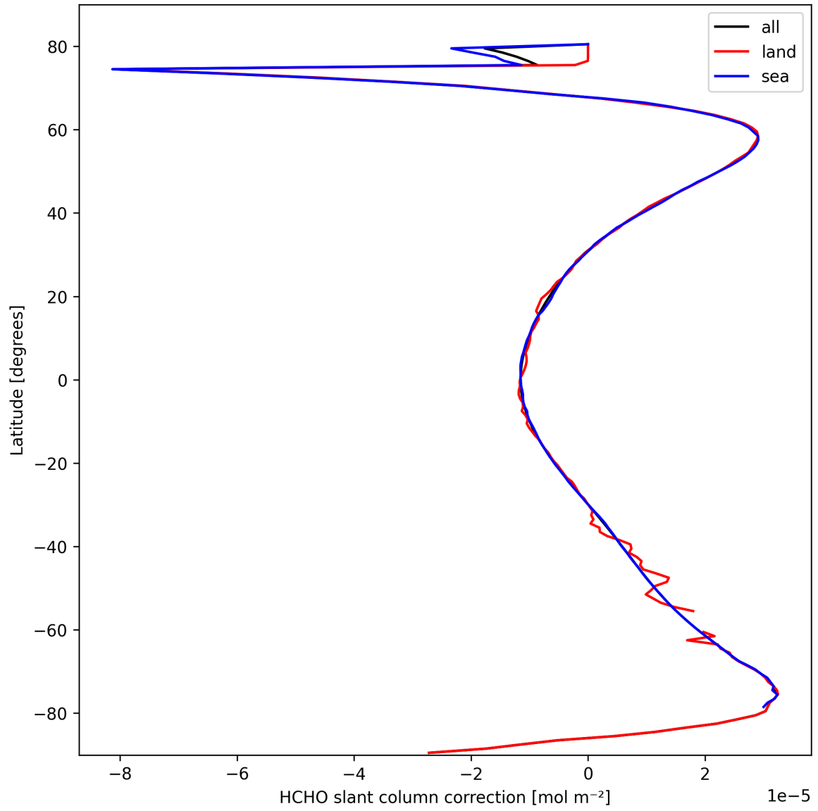
Figure 31: Zonal average of "HCHO slant column correction" for 2025-03-08 to 2025-03-09.
