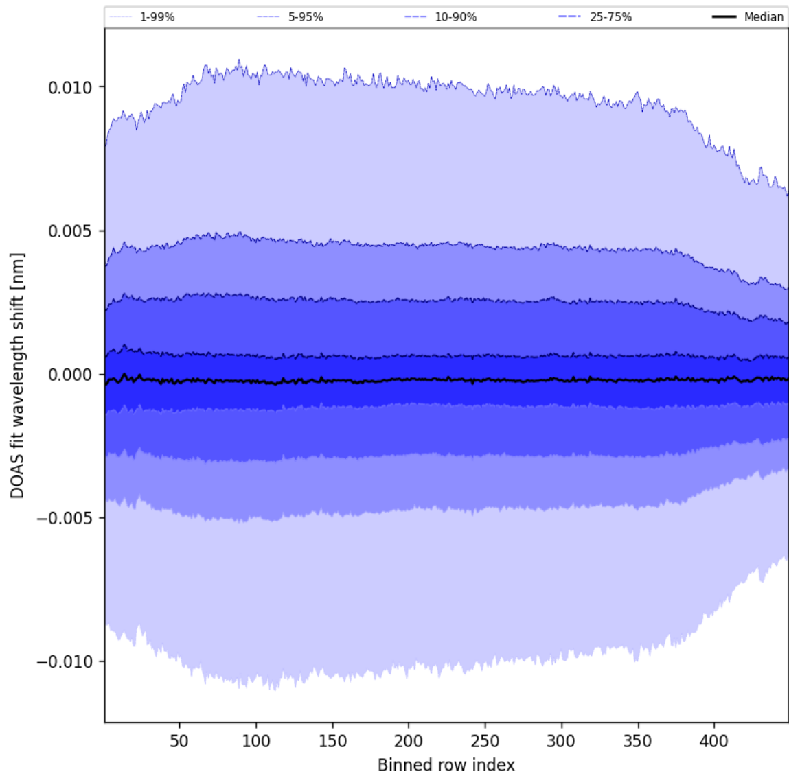
Figure 56: Along track statistics of “DOAS fit wavelength shift” for 2025-03-08 to 2025-03-09
