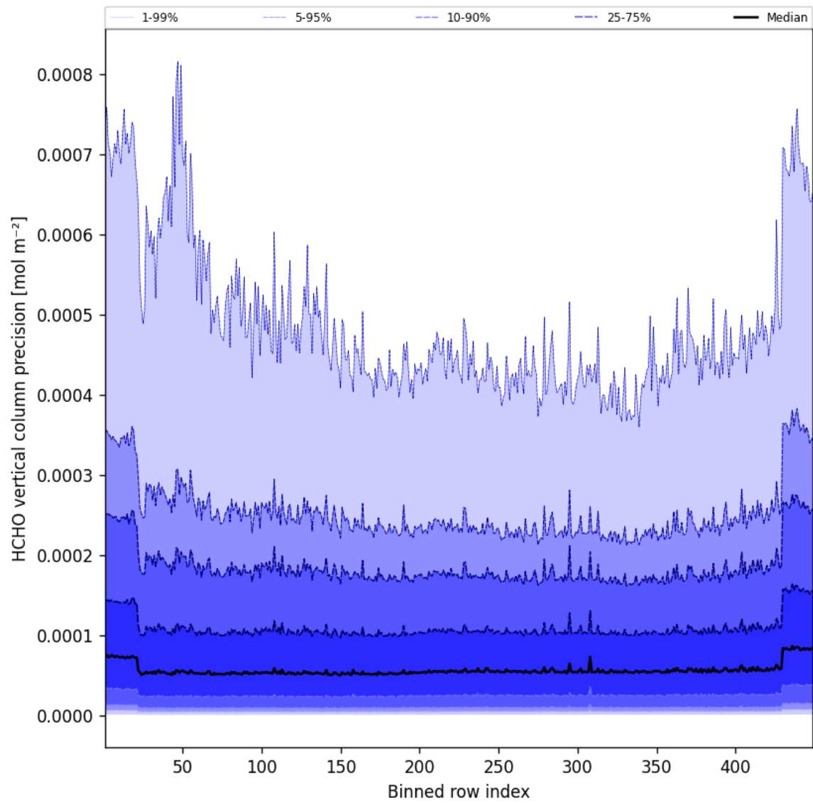
Figure 48: Along track statistics of “HCHO vertical column precision” for 2025-03-08 to 2025-03-09
