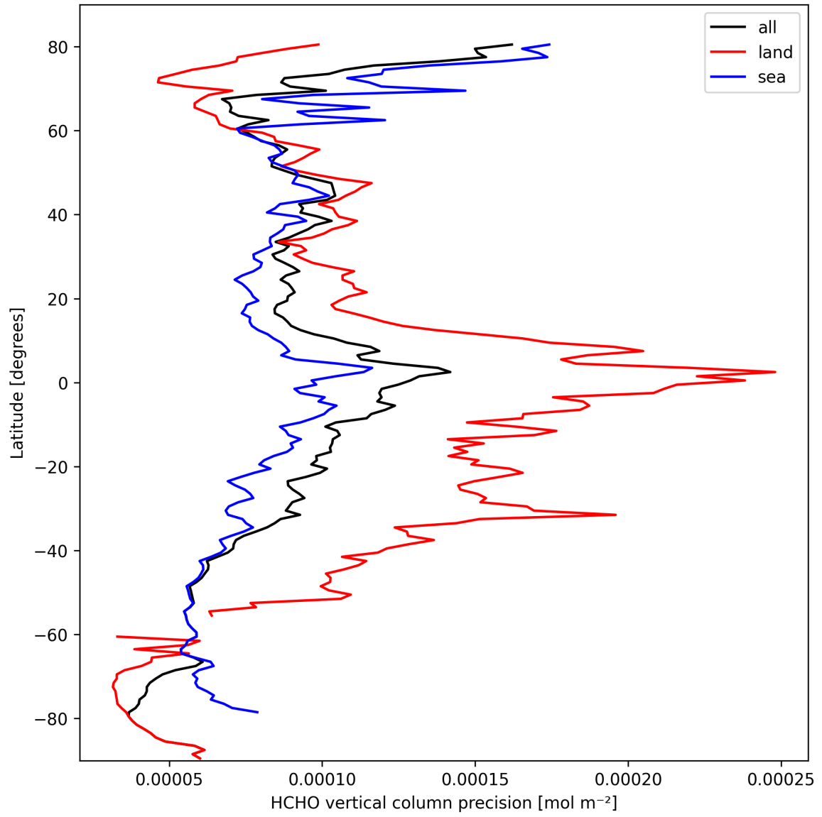
Figure 20: Zonal average of “HCHO vertical column precision” for 2025-03-08 to 2025-03-09.
