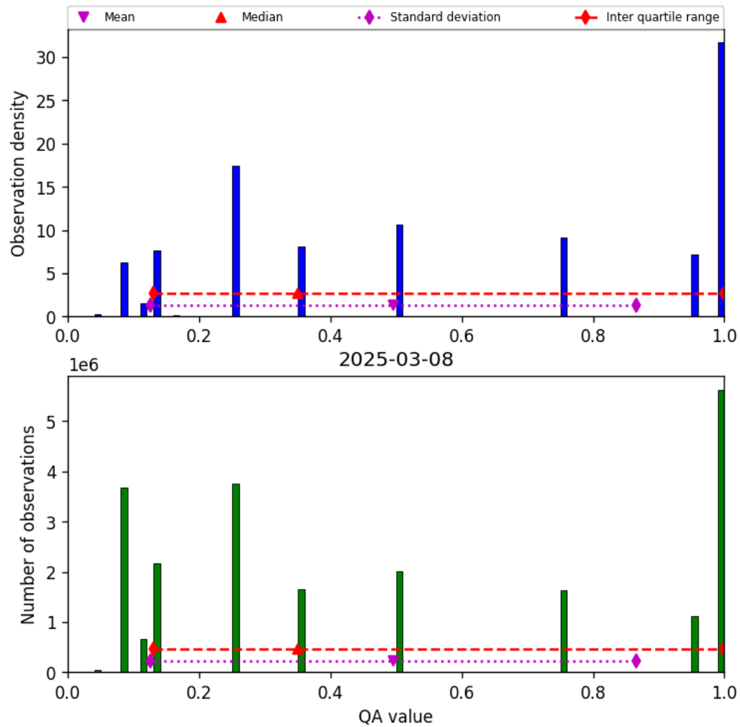
Figure 32: Histogram of “QA value” for 2025-03-08 to 2025-03-09
