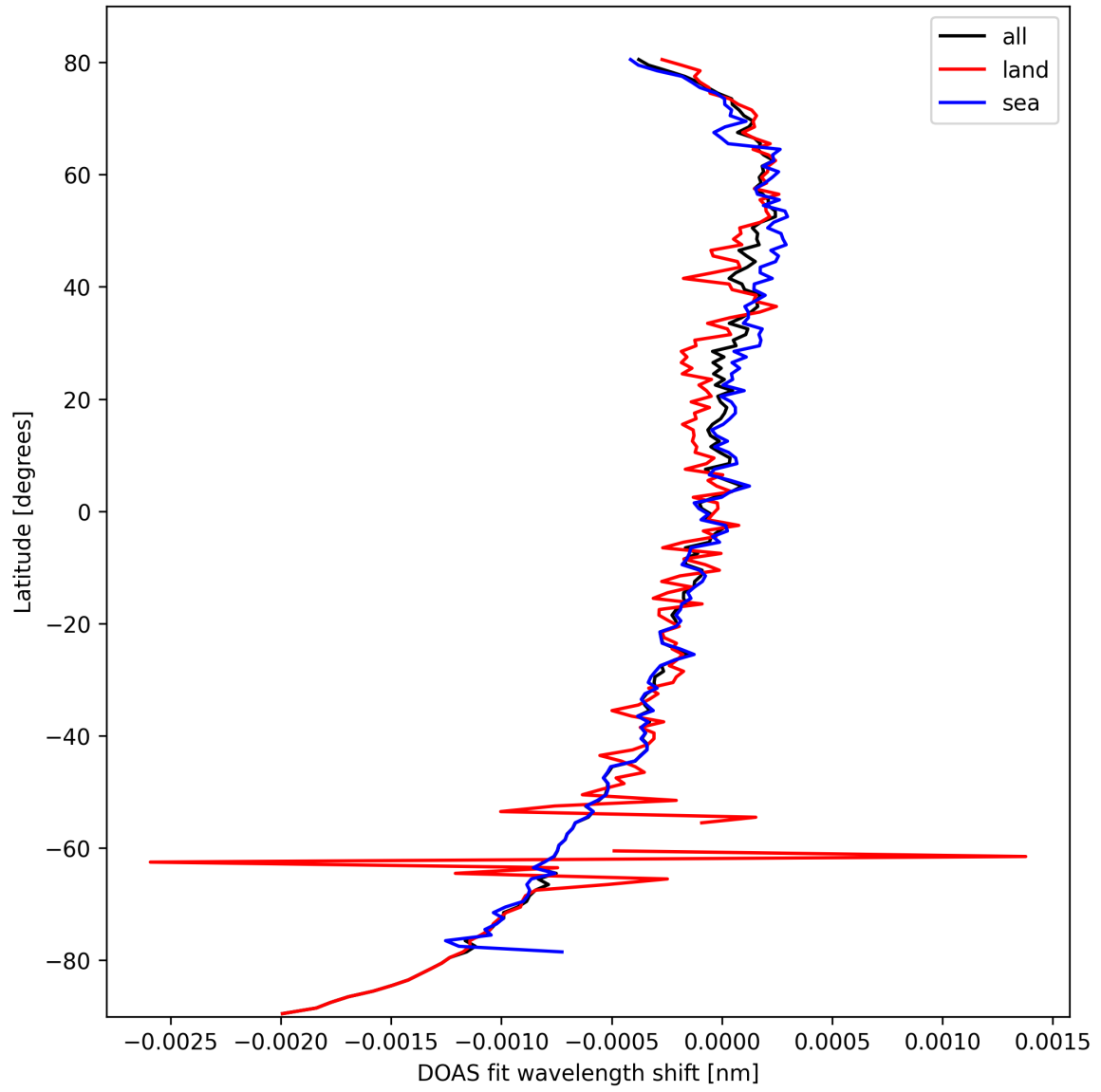
Figure 28: Zonal average of "DOAS fit wavelength shift" for 2025-03-08 to 2025-03-09.
