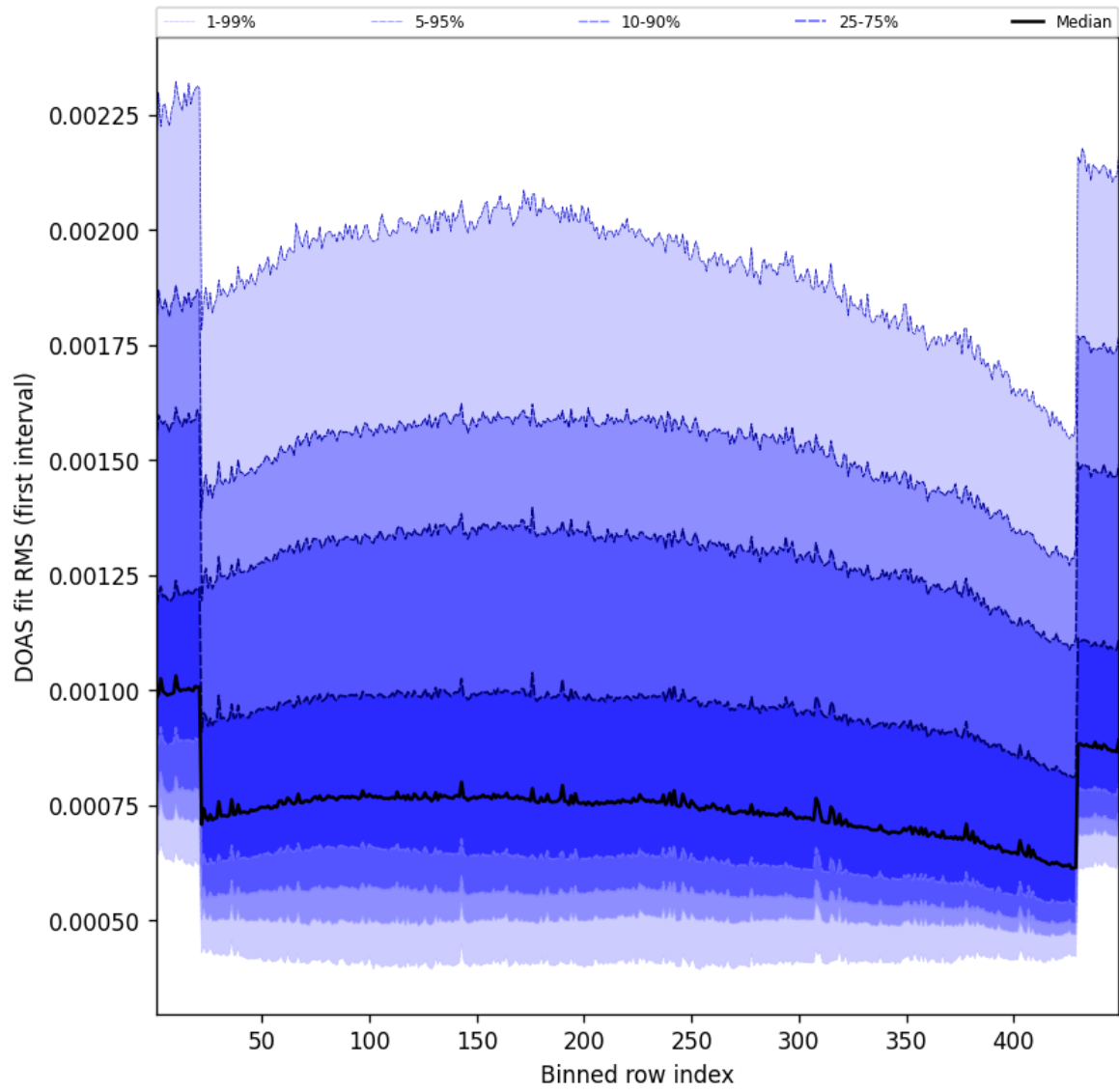
Figure 58: Along track statistics of “DOAS fit RMS (first interval)” for 2025-03-08 to 2025-03-09
