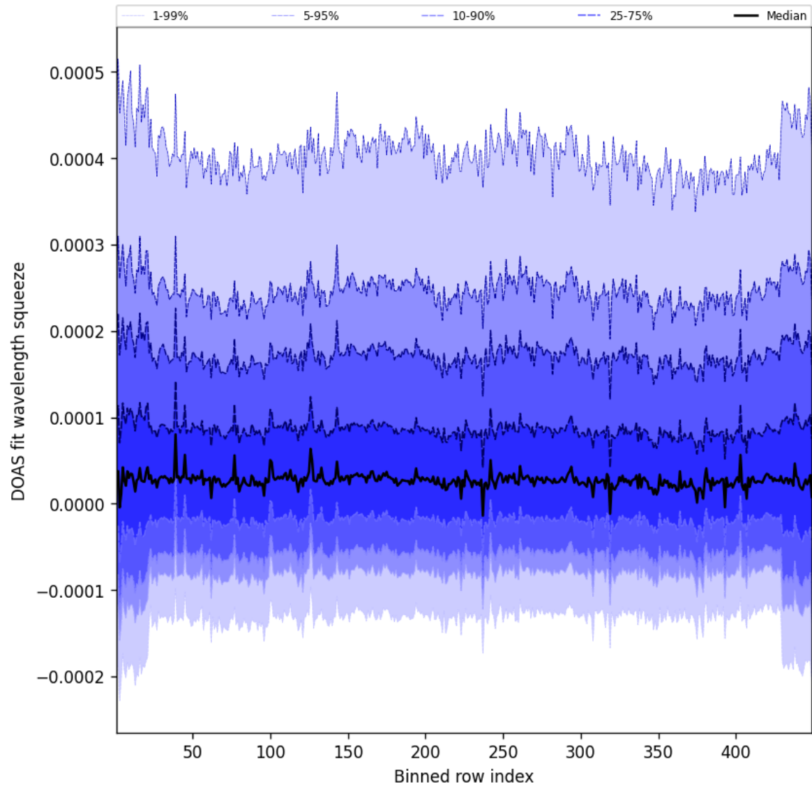
Figure 57: Along track statistics of “DOAS fit wavelength squeeze” for 2025-03-08 to 2025-03-09
