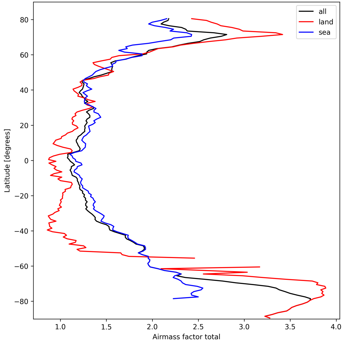
Figure 24: Zonal average of “Airmass factor total” for 2025-03-08 to 2025-03-09.
