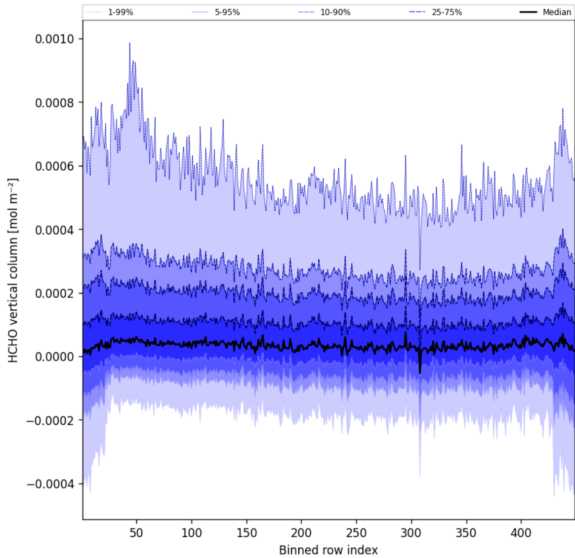
Figure 47: Along track statistics of “HCHO vertical column” for 2025-03-08 to 2025-03-09
