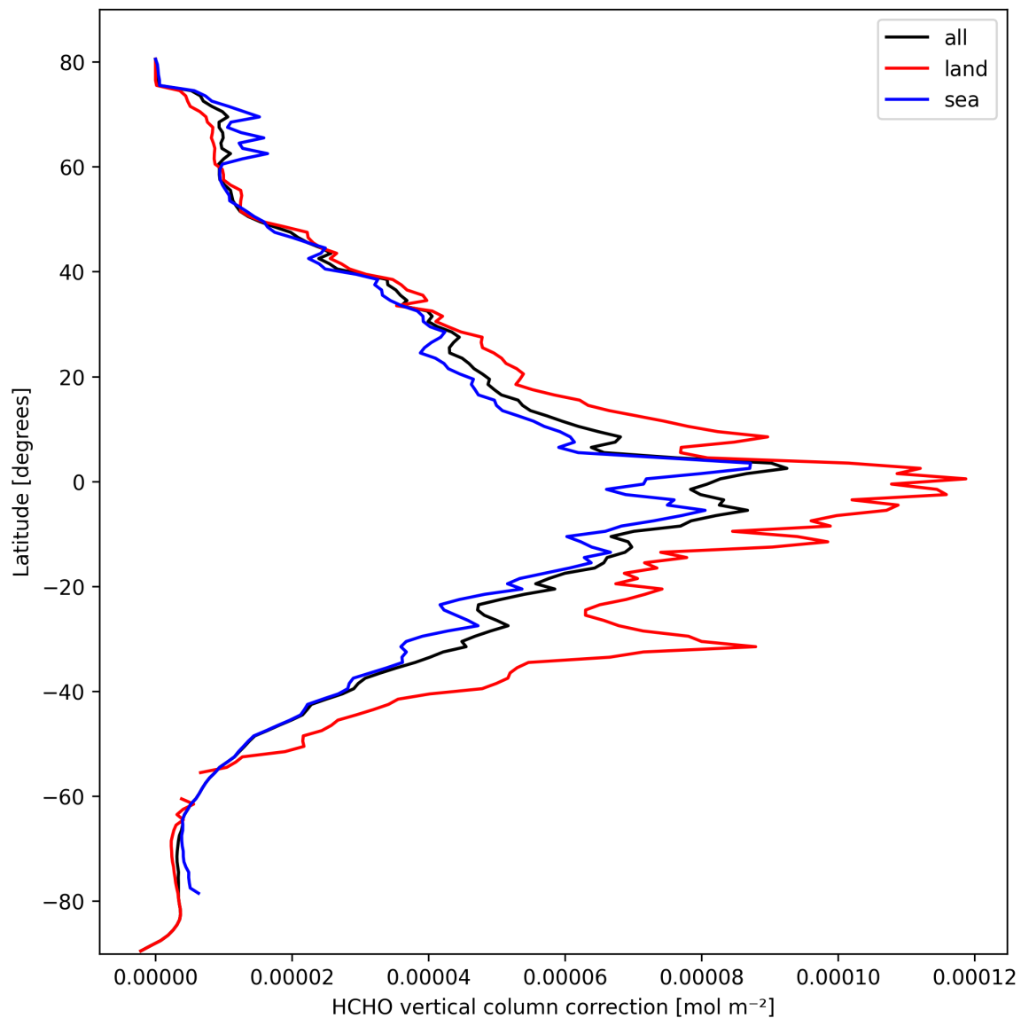
Figure 21: Zonal average of “HCHO vertical column correction” for 2025-03-08 to 2025-03-09.
