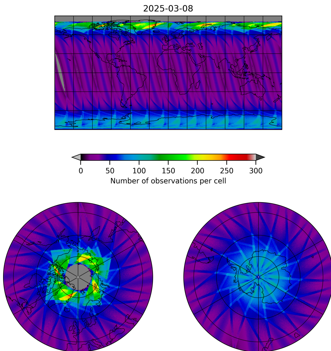
Figure 17: Map of the number of observations for 2025-03-08 to 2025-03-09
