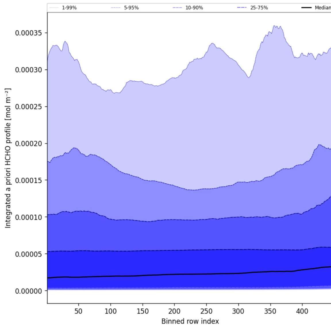
Figure 55: Along track statistics of "Integrated a priori HCHO profile" for 2025-03-08 to 2025-03-09
