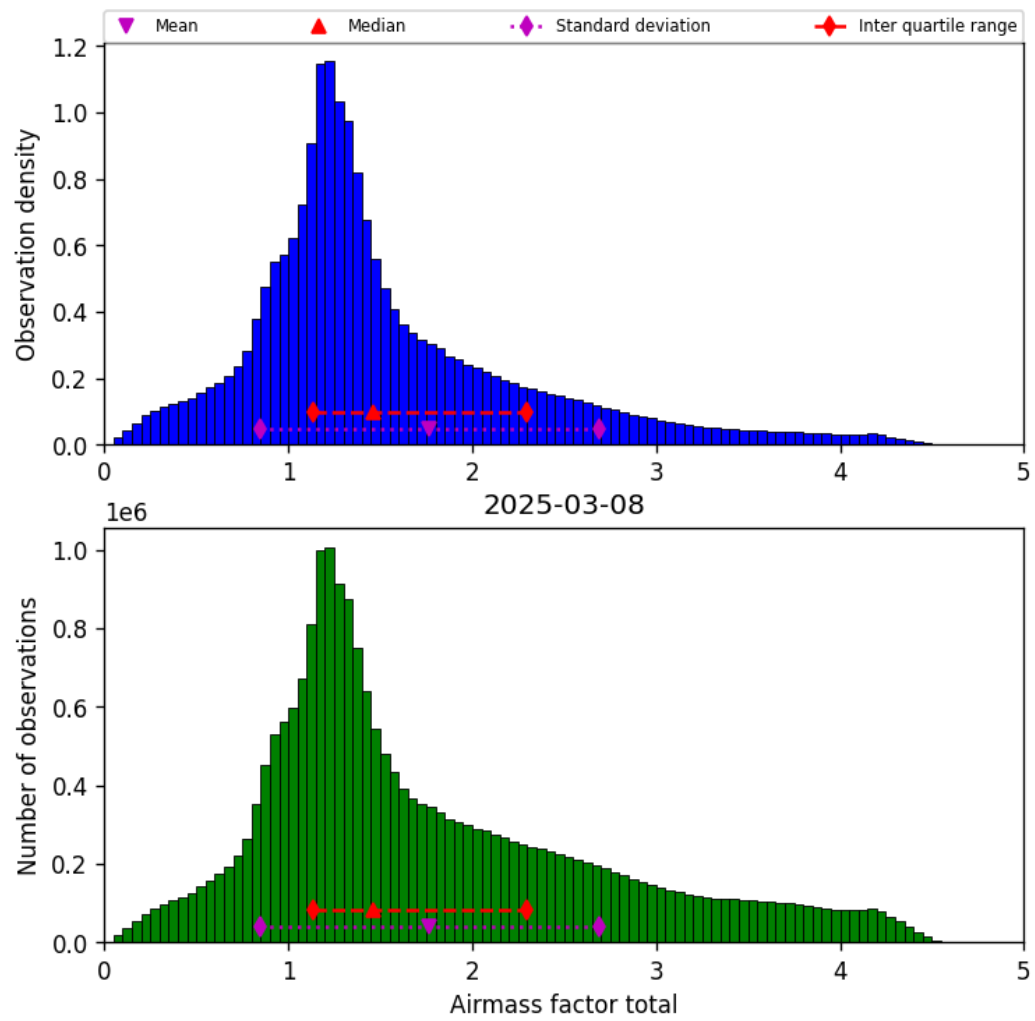
Figure 38: Histogram of “Airmass factor total” for 2025-03-08 to 2025-03-09
