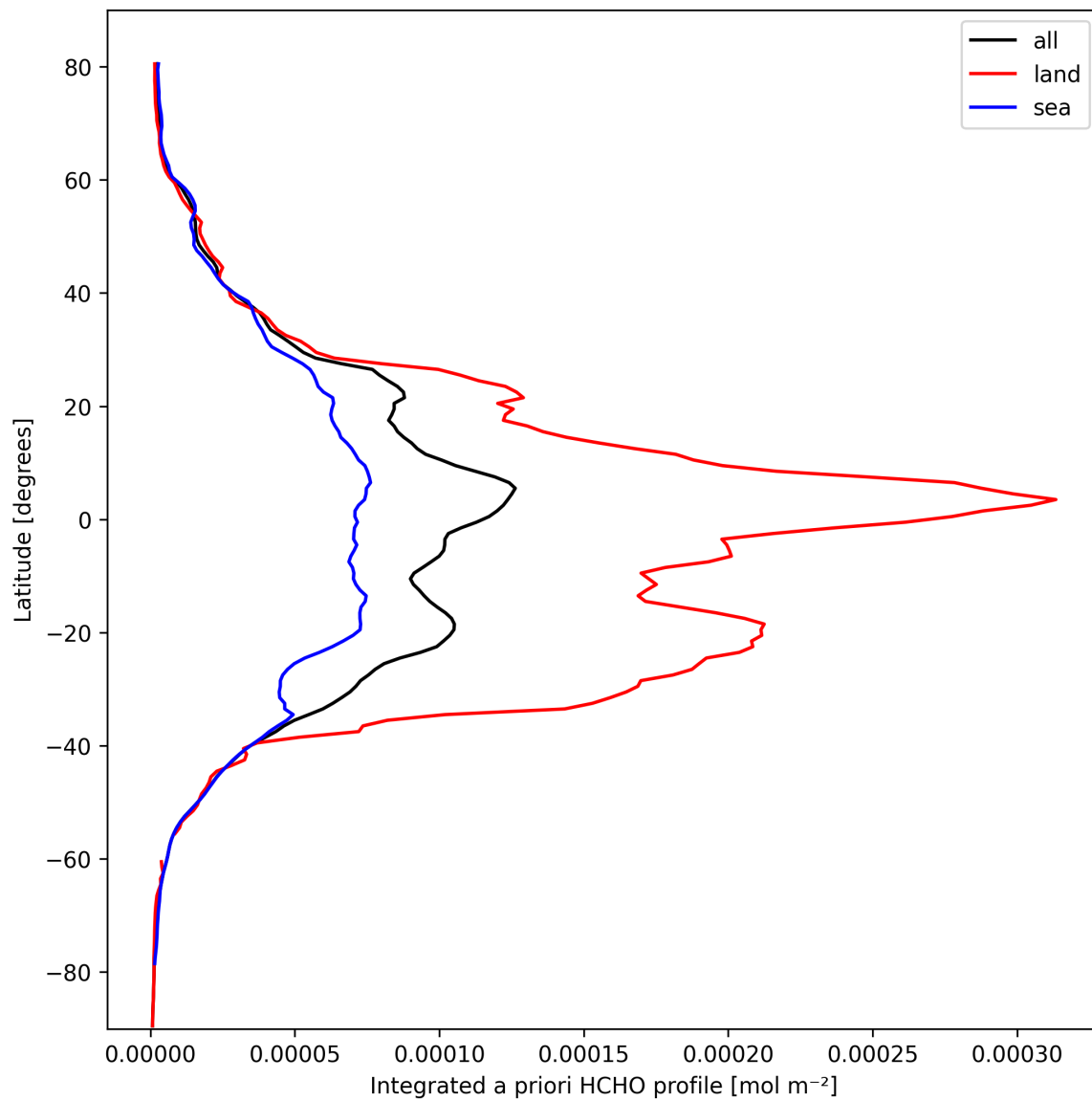
Figure 27: Zonal average of “Integrated a priori HCHO profile” for 2025-03-08 to 2025-03-09.
