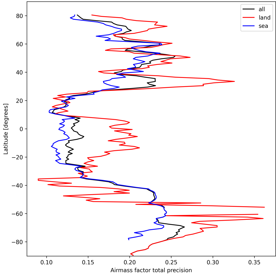
Figure 25: Zonal average of “Airmass factor total precision” for 2025-03-08 to 2025-03-09.
