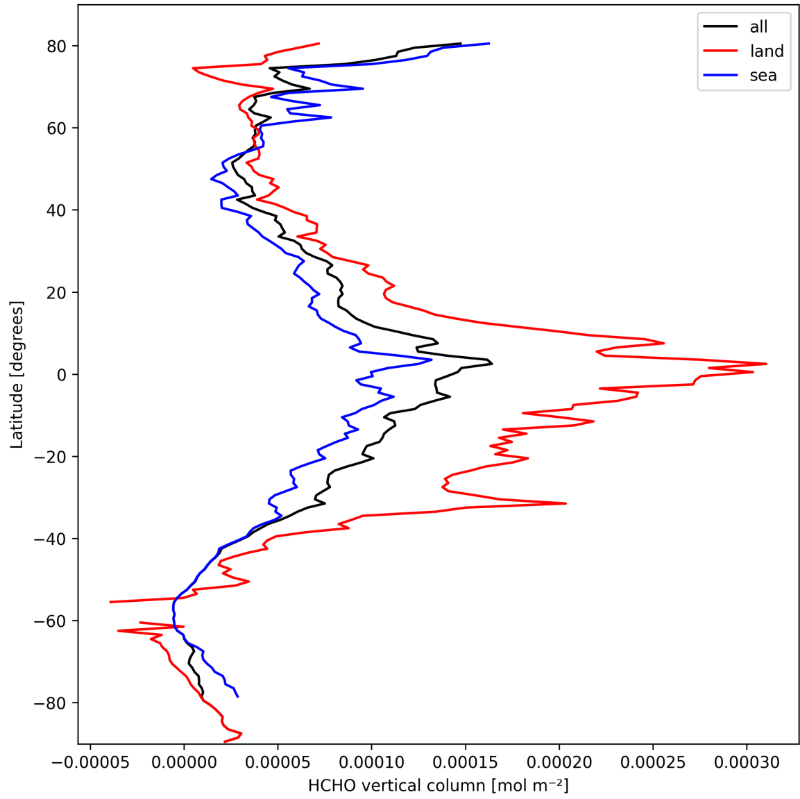
Figure 19: Zonal average of “HCHO vertical column” for 2025-03-08 to 2025-03-09.
