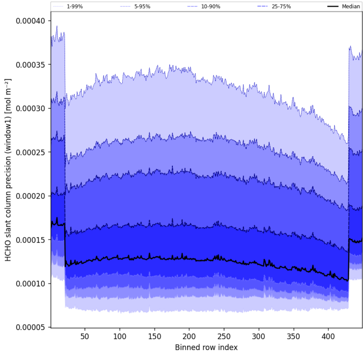
Figure 51: Along track statistics of “HCHO slant column precision (window1)” for 2025-03-08 to 2025-03-09
