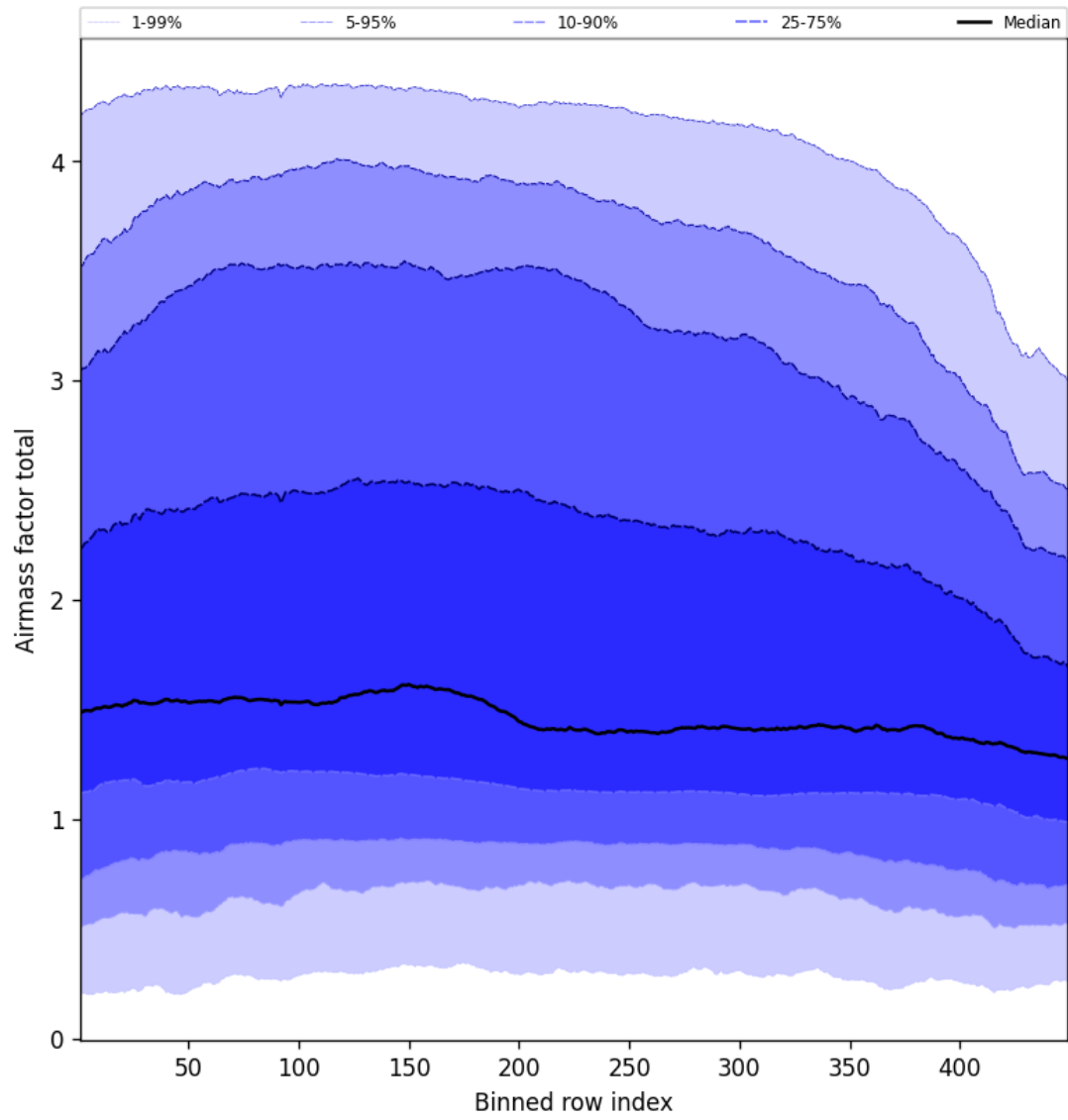
Figure 52: Along track statistics of “Airmass factor total” for 2025-03-08 to 2025-03-09
