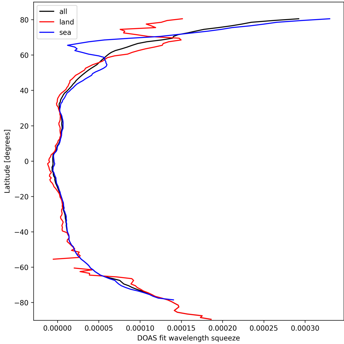
Figure 29: Zonal average of “DOAS fit wavelength squeeze” for 2025-03-08 to 2025-03-09.
