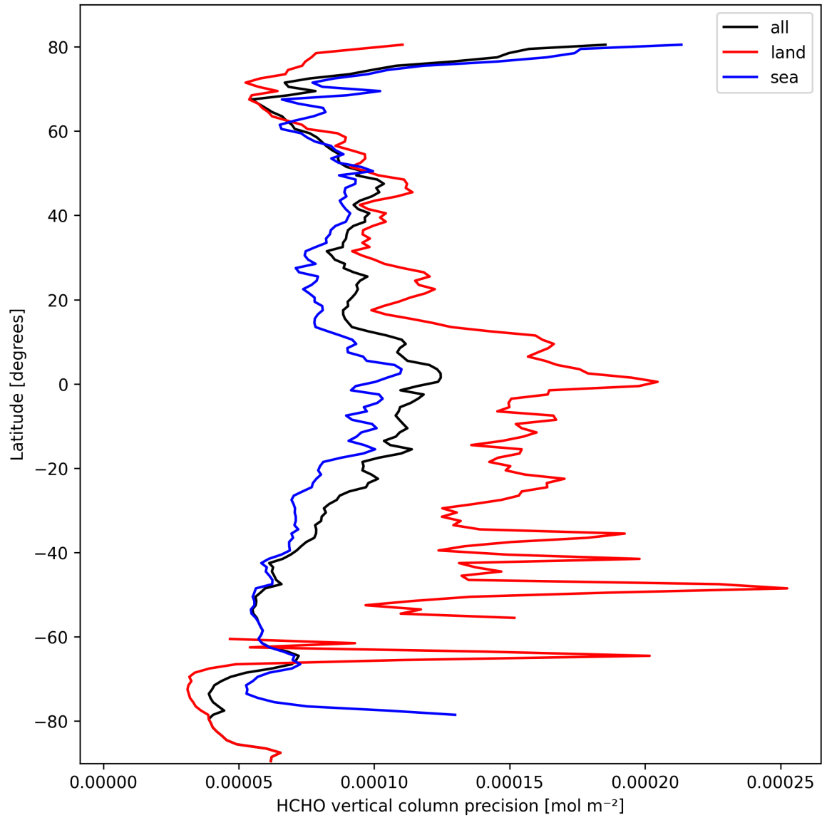
Figure 20: Zonal average of “HCHO vertical column precision” for 2025-03-09 to 2025-03-10.
