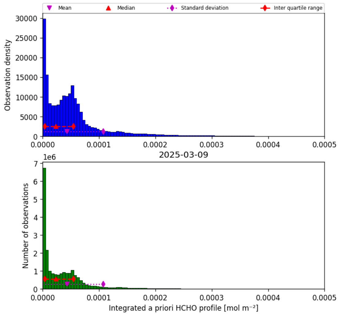
Figure 41: Histogram of “Integrated a priori HCHO profile” for 2025-03-09 to 2025-03-10
