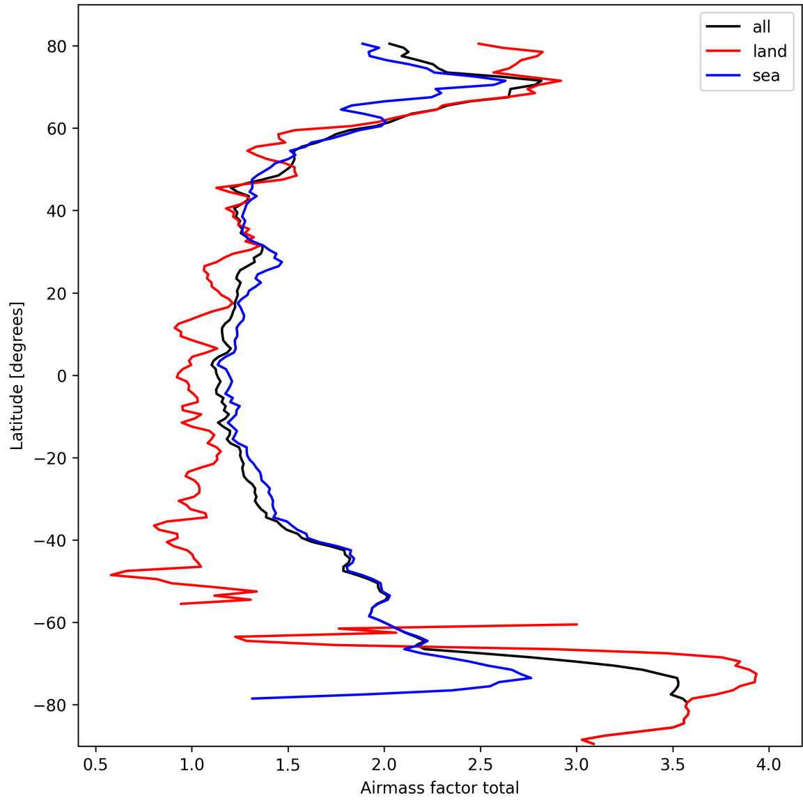
Figure 24: Zonal average of “Airmass factor total” for 2025-03-09 to 2025-03-10.
