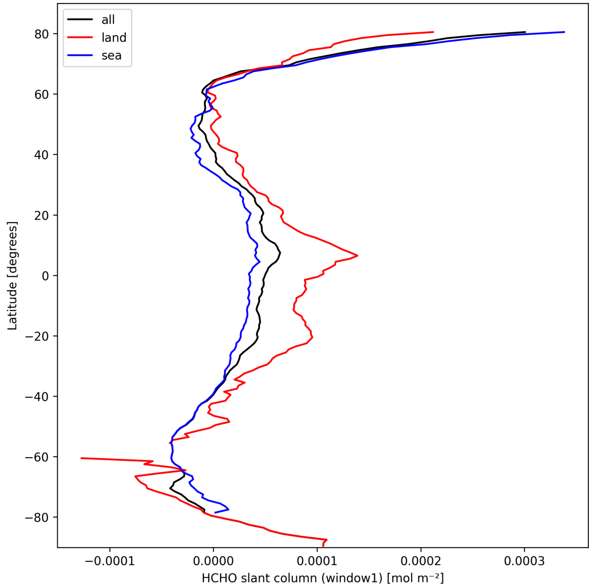
Figure 22: Zonal average of “HCHO slant column (window1)” for 2025-03-09 to 2025-03-10.
