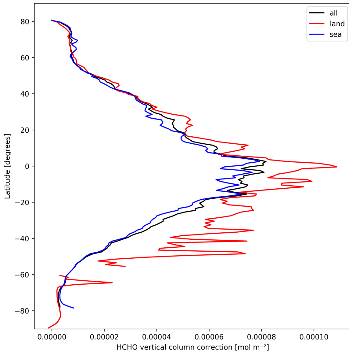
Figure 21: Zonal average of “HCHO vertical column correction” for 2025-03-09 to 2025-03-10.
