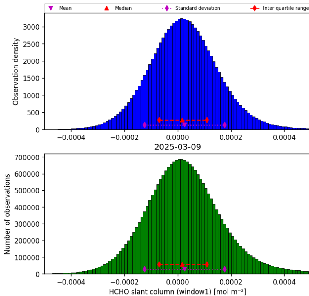
Figure 36: Histogram of “HCHO slant column (window1)” for 2025-03-09 to 2025-03-10
