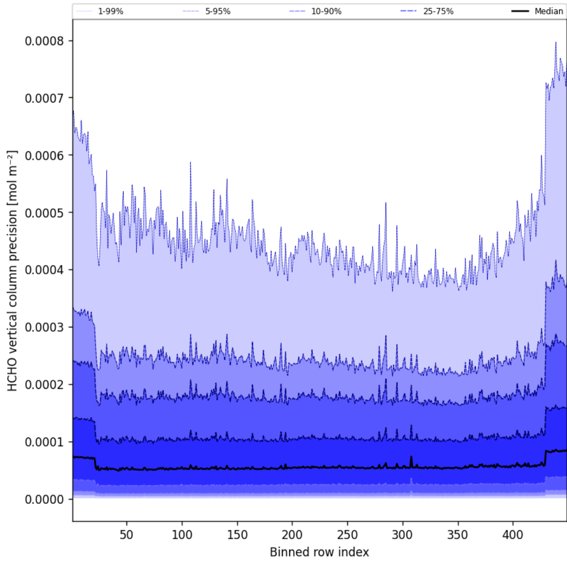
Figure 48: Along track statistics of “HCHO vertical column precision” for 2025-03-09 to 2025-03-10
