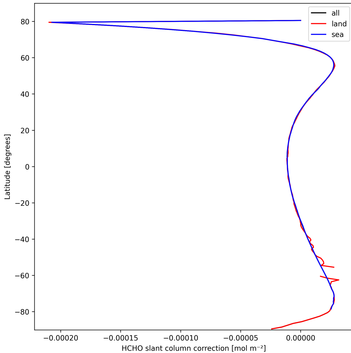
Figure 31: Zonal average of “HCHO slant column correction” for 2025-03-09 to 2025-03-10.
