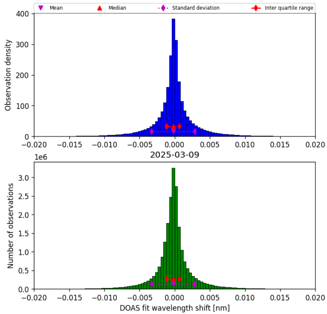
Figure 42: Histogram of “DOAS fit wavelength shift” for 2025-03-09 to 2025-03-10
