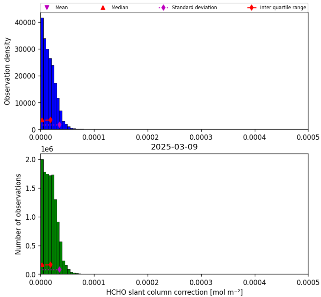
Figure 45: Histogram of “HCHO slant column correction” for 2025-03-09 to 2025-03-10
