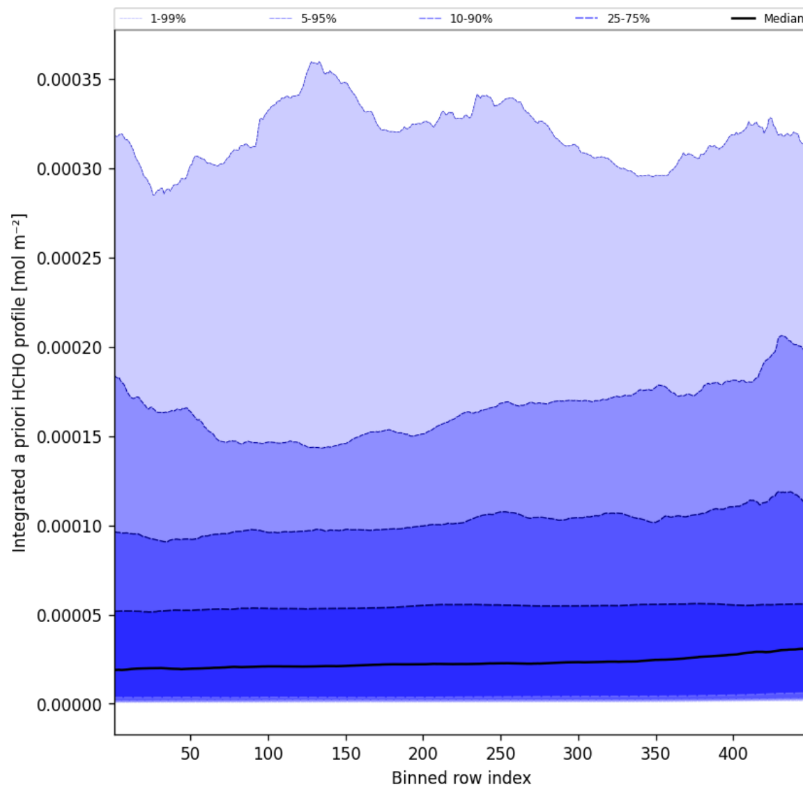
Figure 55: Along track statistics of "Integrated a priori HCHO profile" for 2025-03-09 to 2025-03-10
