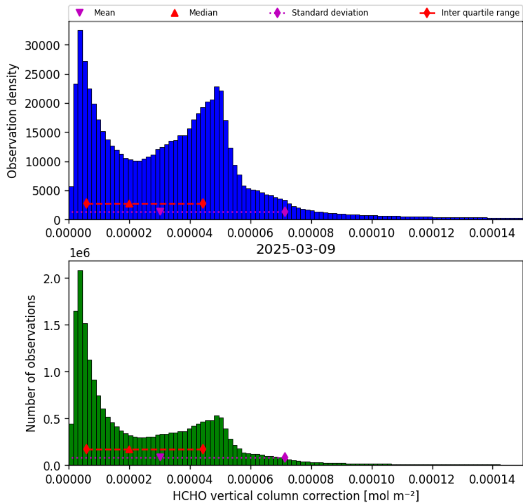
Figure 35: Histogram of “HCHO vertical column correction” for 2025-03-09 to 2025-03-10
