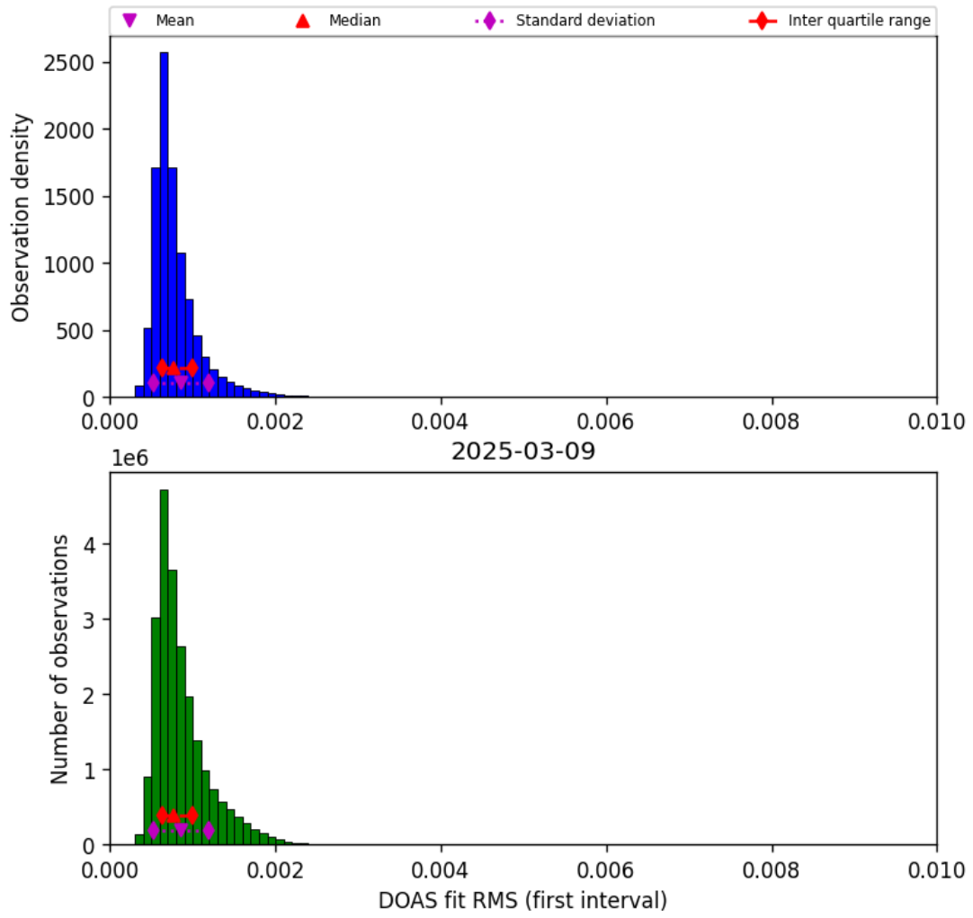
Figure 44: Histogram of “DOAS fit RMS (first interval)” for 2025-03-09 to 2025-03-10
