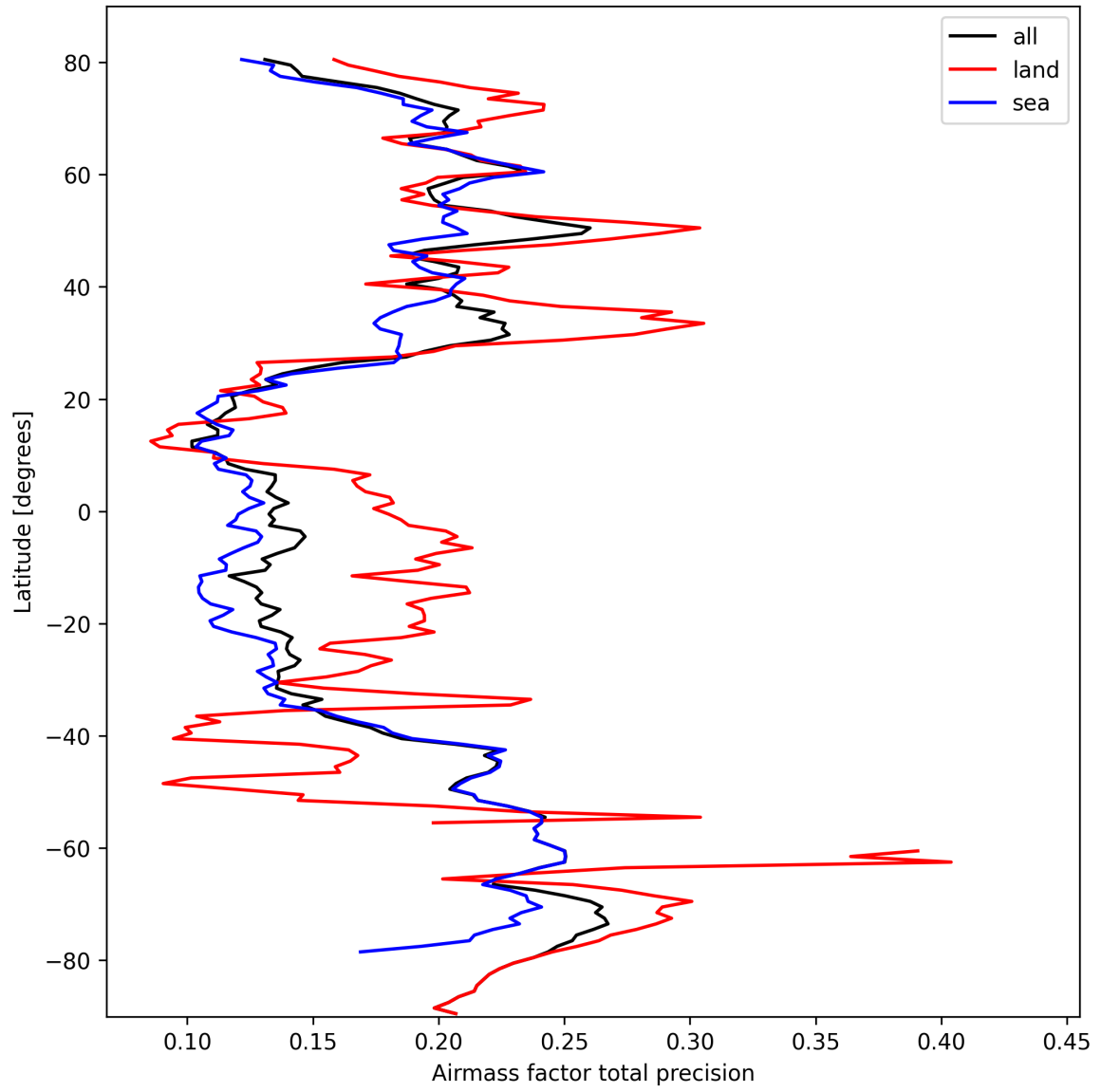
Figure 25: Zonal average of “Airmass factor total precision” for 2025-03-09 to 2025-03-10.
