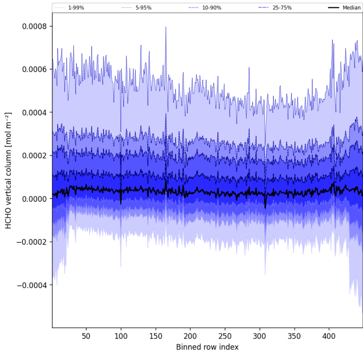
Figure 47: Along track statistics of “HCHO vertical column” for 2025-03-09 to 2025-03-10
