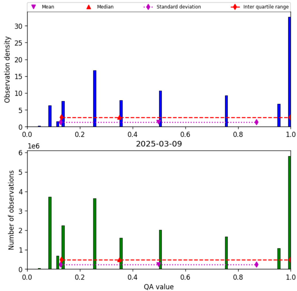
Figure 32: Histogram of “QA value” for 2025-03-09 to 2025-03-10
