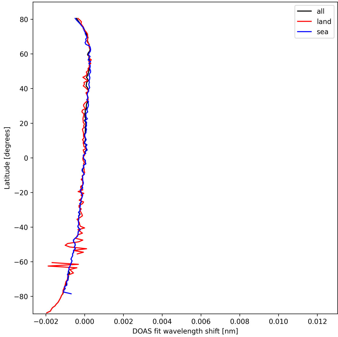
Figure 28: Zonal average of "DOAS fit wavelength shift" for 2025-03-09 to 2025-03-10.
