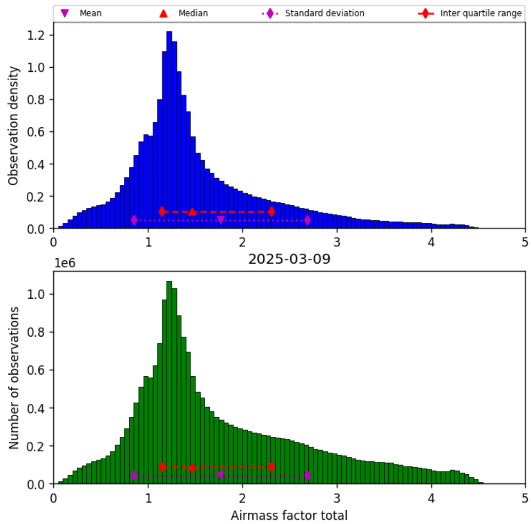
Figure 38: Histogram of “Airmass factor total” for 2025-03-09 to 2025-03-10
