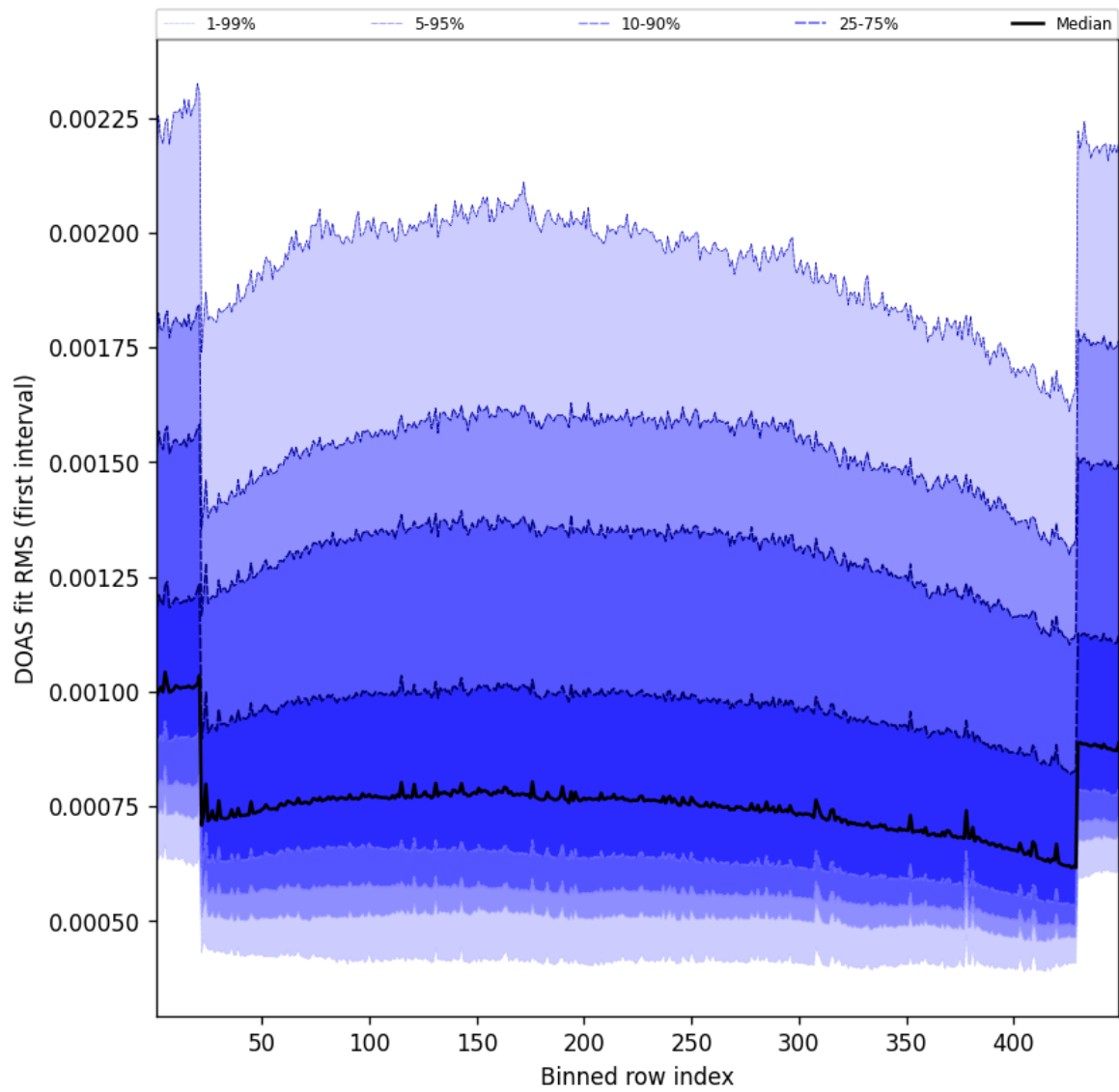
Figure 58: Along track statistics of “DOAS fit RMS (first interval)” for 2025-03-09 to 2025-03-10
