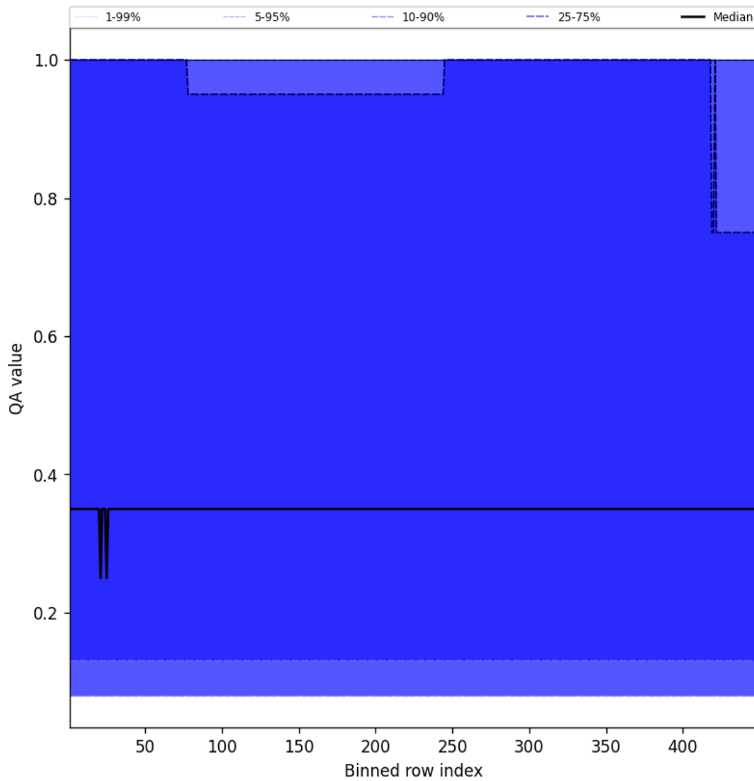
Figure 46: Along track statistics of “QA value” for 2025-03-09 to 2025-03-10
