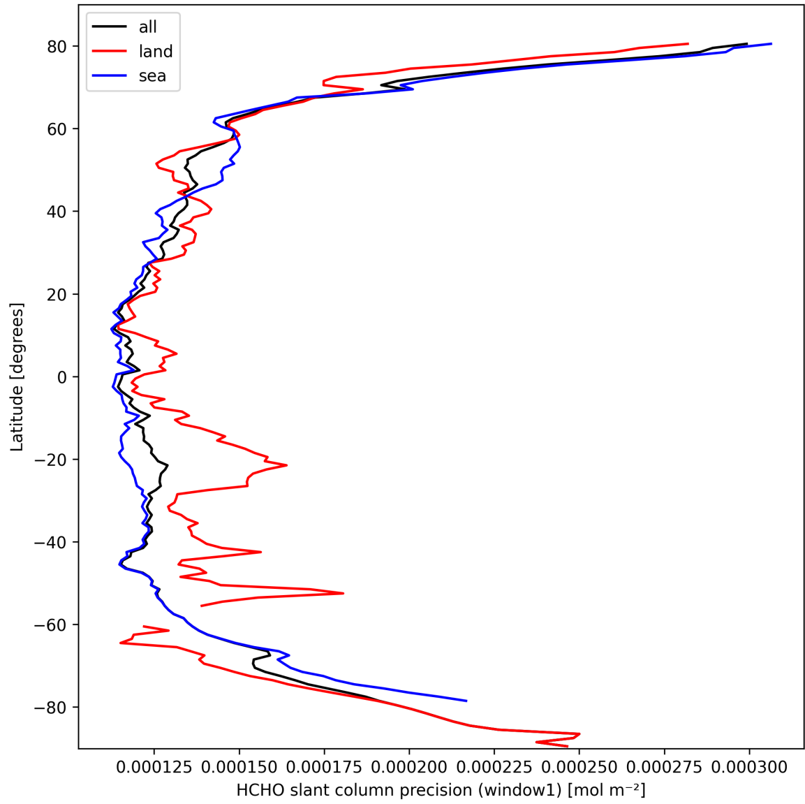
Figure 23: Zonal average of “HCHO slant column precision (window1)” for 2025-03-09 to 2025-03-10.
