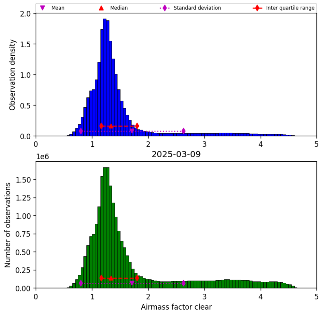
Figure 40: Histogram of “Airmass factor clear” for 2025-03-09 to 2025-03-10
