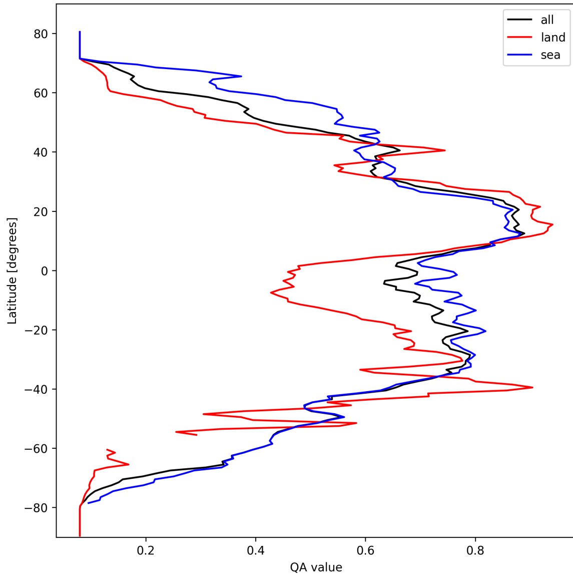
Figure 18: Zonal average of “QA value” for 2025-03-09 to 2025-03-10.
