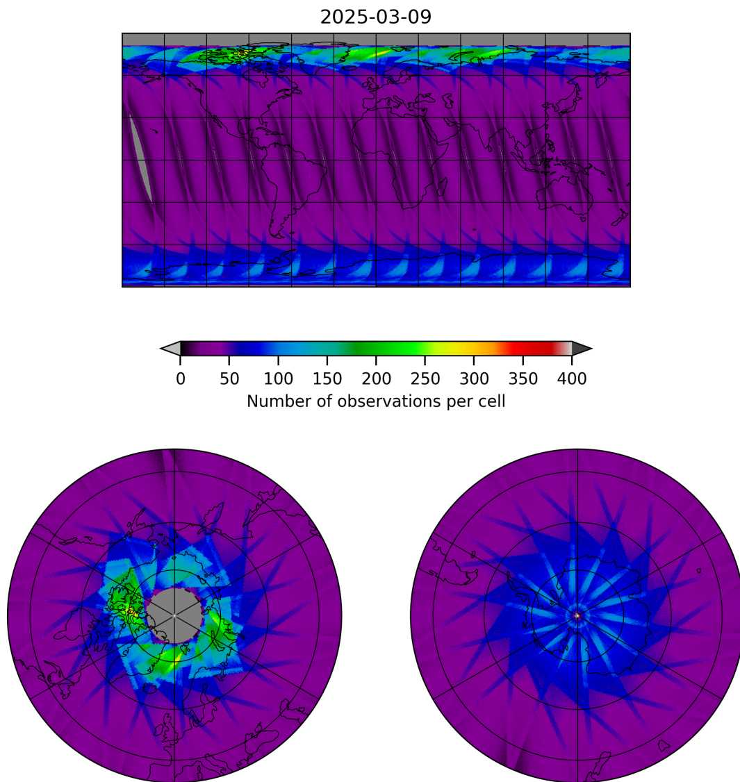
Figure 17: Map of the number of observations for 2025-03-09 to 2025-03-10
