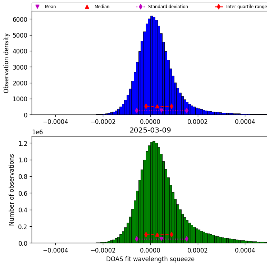
Figure 43: Histogram of “DOAS fit wavelength squeeze” for 2025-03-09 to 2025-03-10
