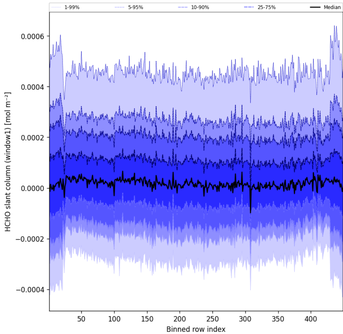
Figure 50: Along track statistics of “HCHO slant column (window1)” for 2025-03-09 to 2025-03-10
