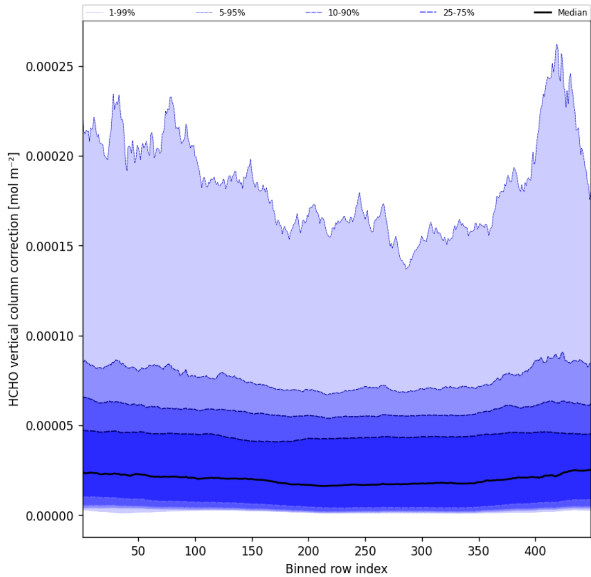
Figure 49: Along track statistics of “HCHO vertical column correction” for 2025-03-09 to 2025-03-10
