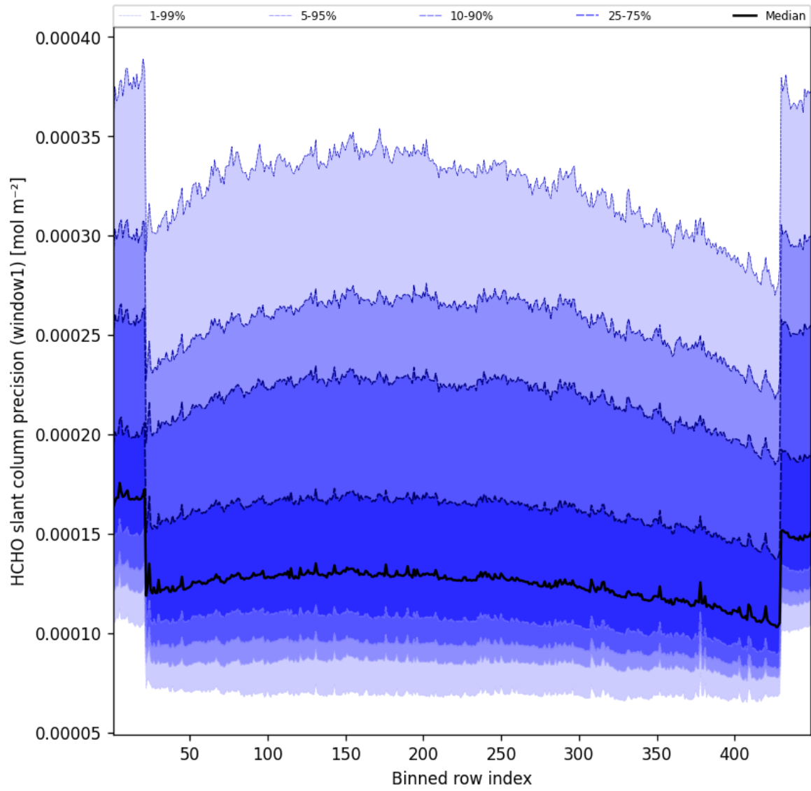
Figure 51: Along track statistics of “HCHO slant column precision (window1)” for 2025-03-09 to 2025-03-10
