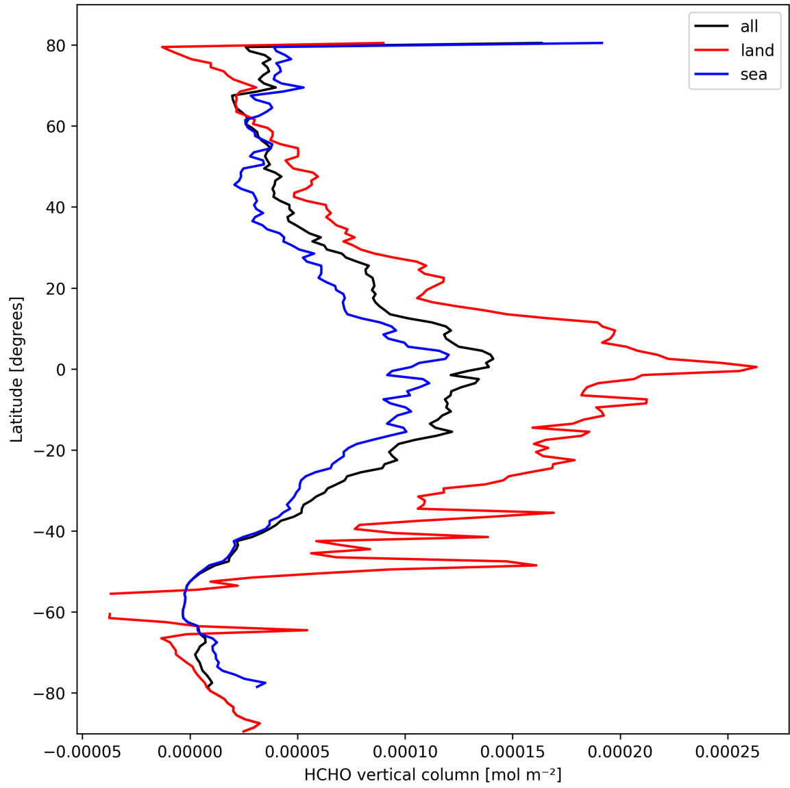
Figure 19: Zonal average of “HCHO vertical column” for 2025-03-09 to 2025-03-10.
