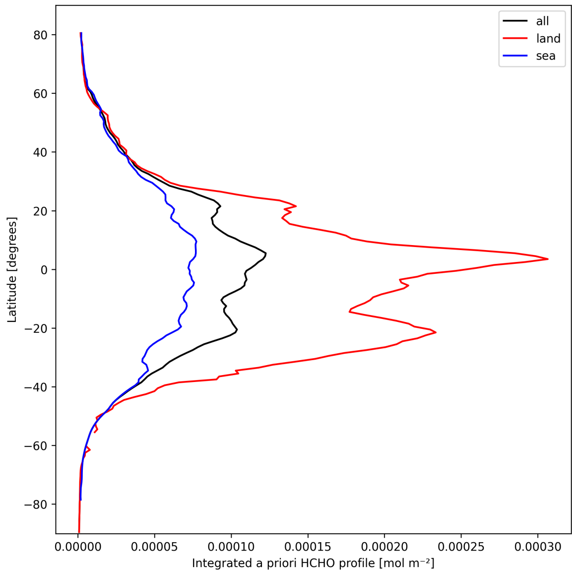
Figure 27: Zonal average of “Integrated a priori HCHO profile” for 2025-03-09 to 2025-03-10.
