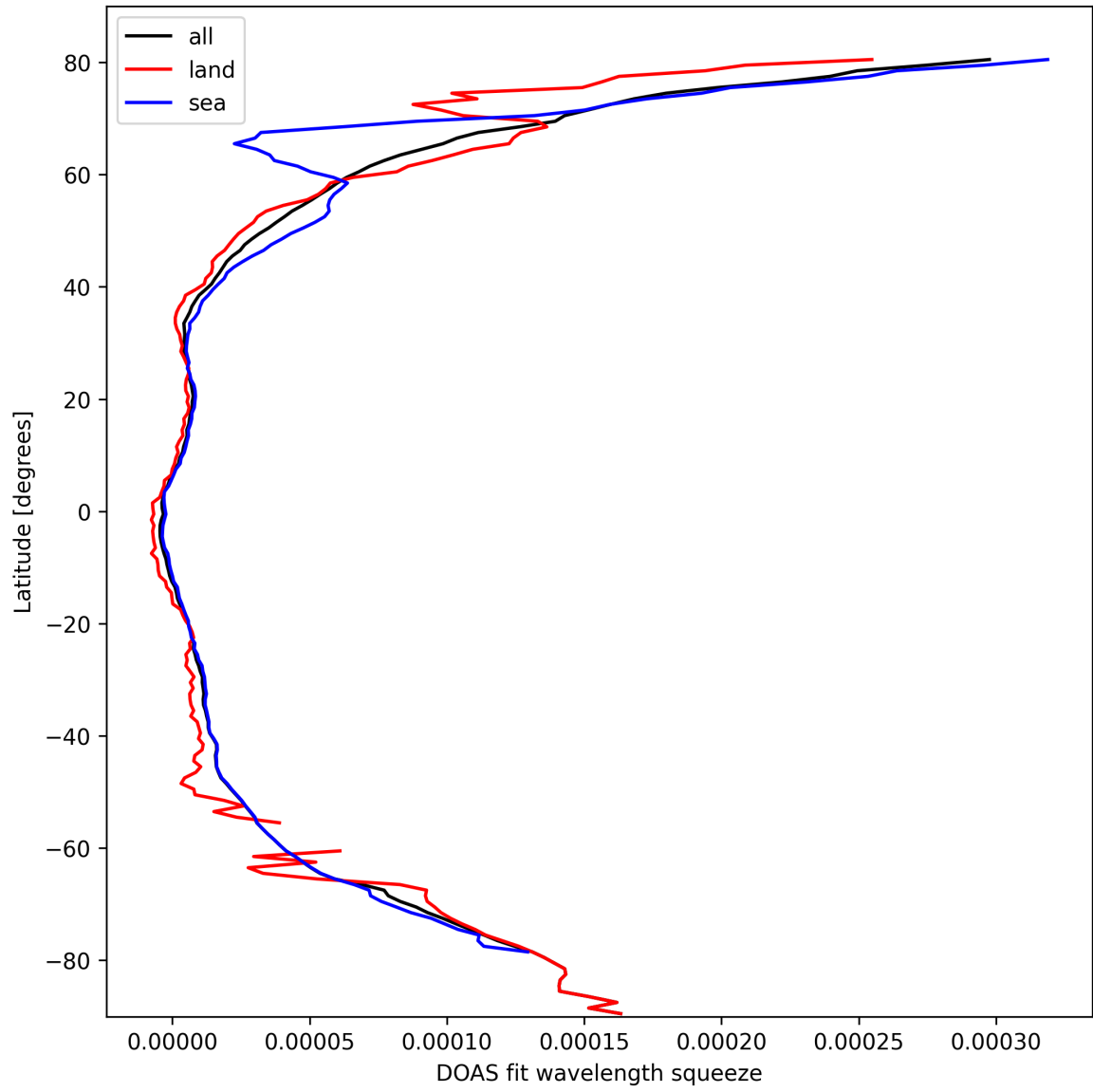
Figure 29: Zonal average of “DOAS fit wavelength squeeze” for 2025-03-09 to 2025-03-10.
