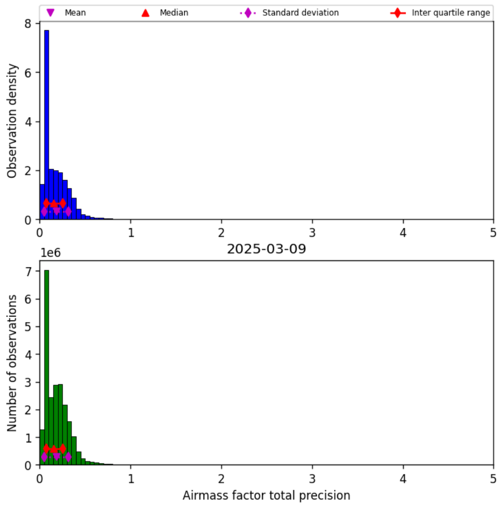
Figure 39: Histogram of “Airmass factor total precision” for 2025-03-09 to 2025-03-10
