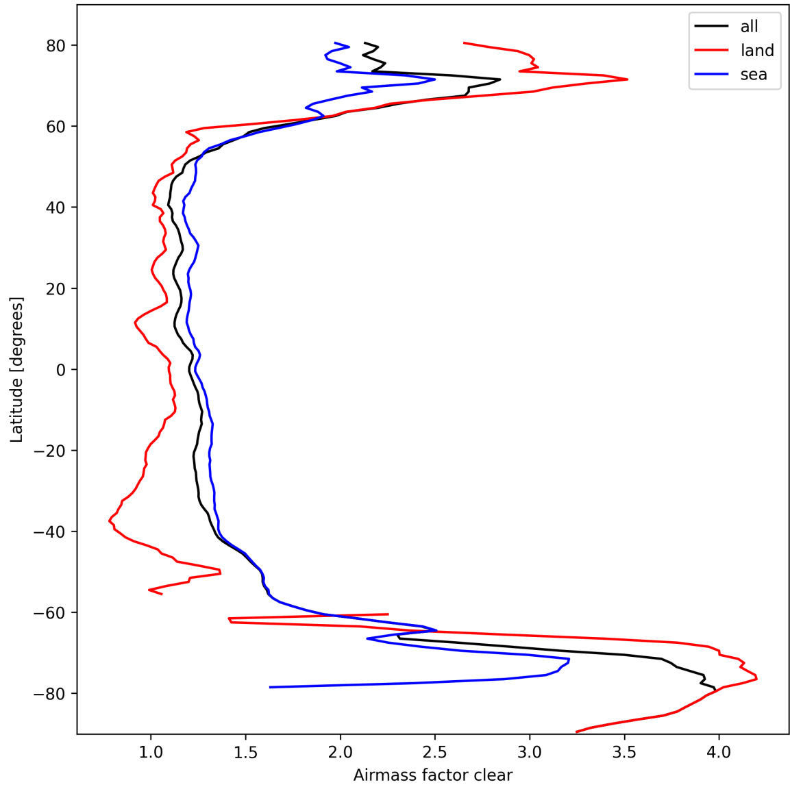
Figure 26: Zonal average of “Airmass factor clear” for 2025-03-09 to 2025-03-10.
