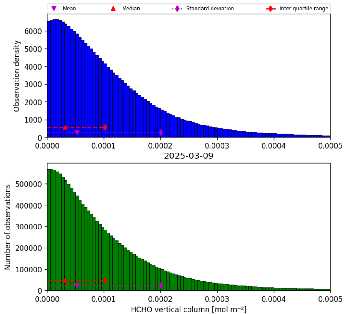
Figure 33: Histogram of “HCHO vertical column” for 2025-03-09 to 2025-03-10
