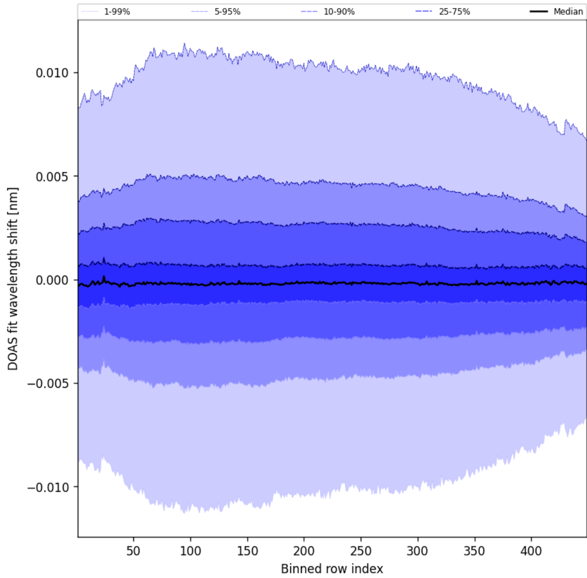
Figure 56: Along track statistics of “DOAS fit wavelength shift” for 2025-03-09 to 2025-03-10
