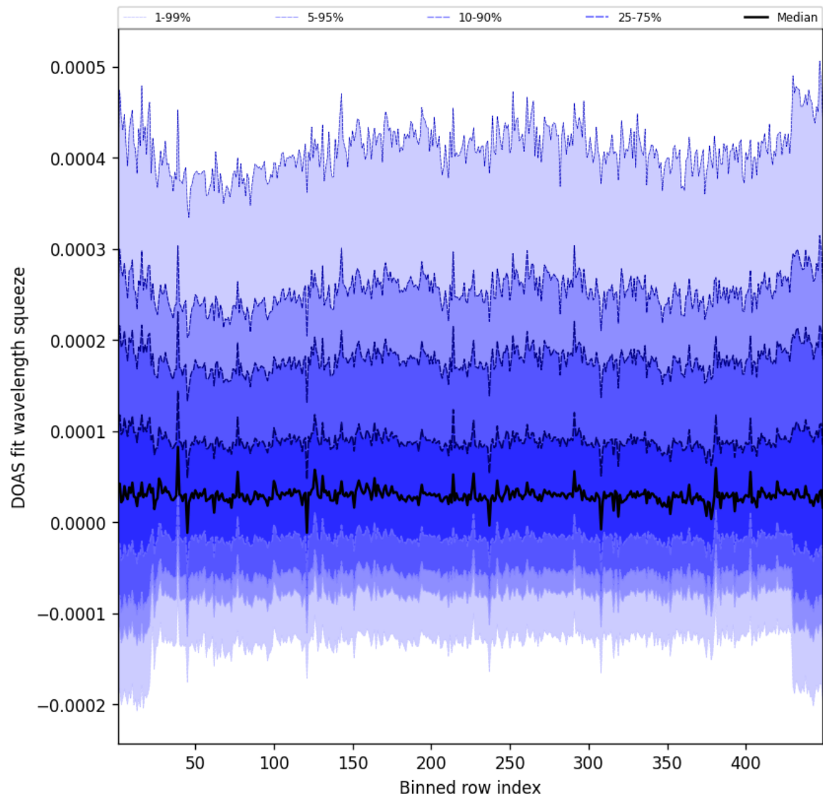
Figure 57: Along track statistics of “DOAS fit wavelength squeeze” for 2025-03-09 to 2025-03-10
