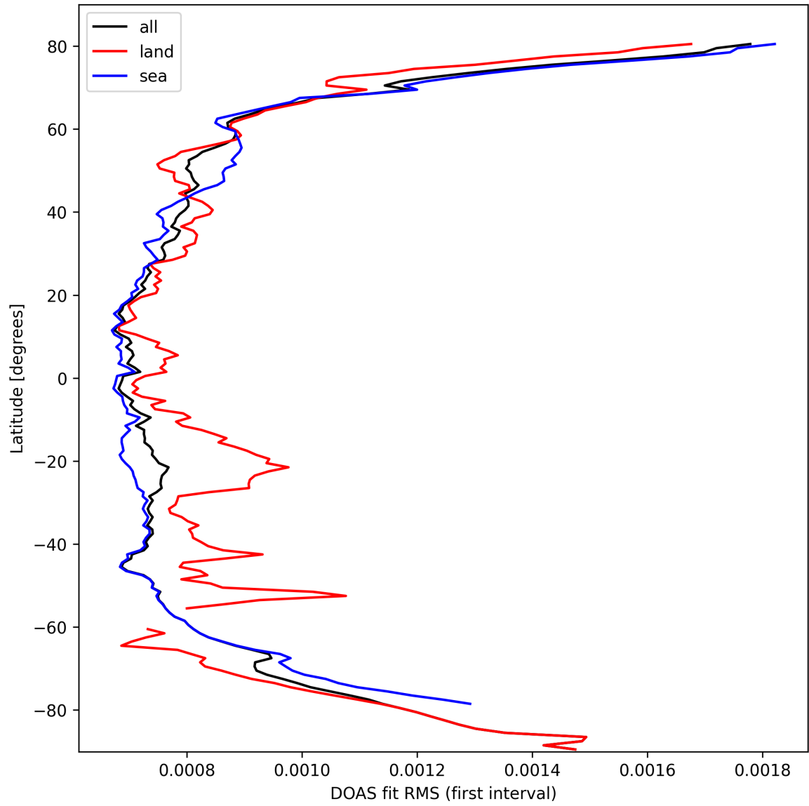
Figure 30: Zonal average of "DOAS fit RMS (first interval)" for 2025-03-09 to 2025-03-10.
