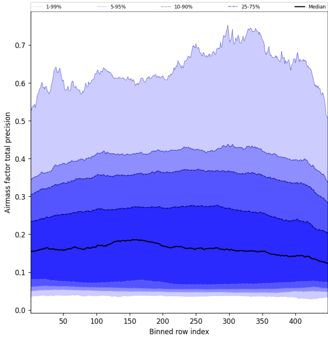
Figure 53: Along track statistics of “Airmass factor total precision” for 2025-03-09 to 2025-03-10
