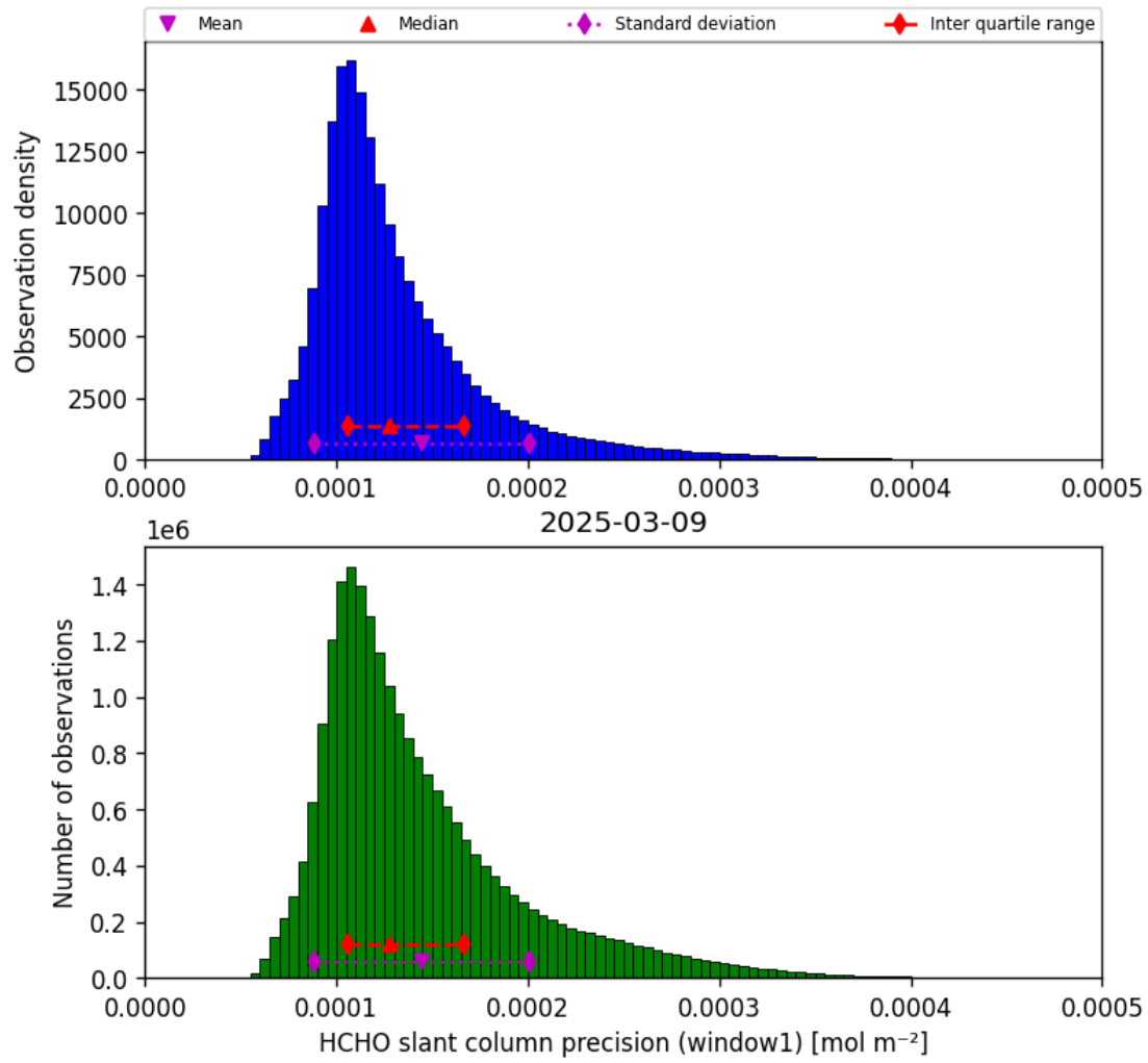
Figure 37: Histogram of “HCHO slant column precision (window1)” for 2025-03-09 to 2025-03-10
