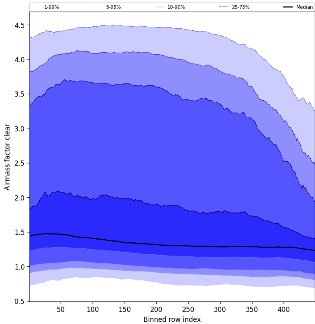
Figure 54: Along track statistics of “Airmass factor clear” for 2025-03-09 to 2025-03-10
