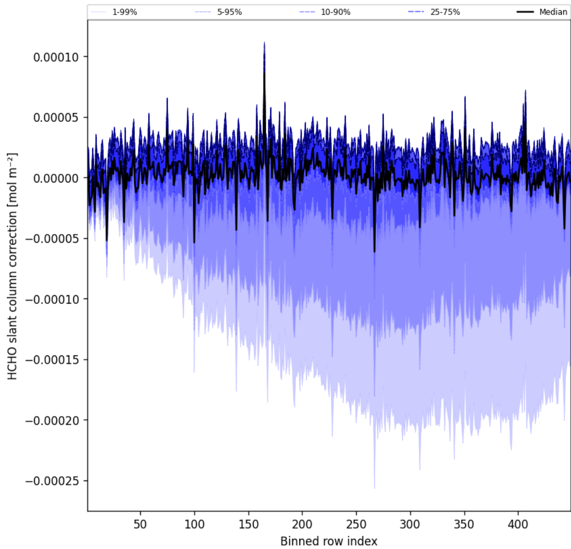
Figure 59: Along track statistics of “HCHO slant column correction” for 2025-03-09 to 2025-03-10
