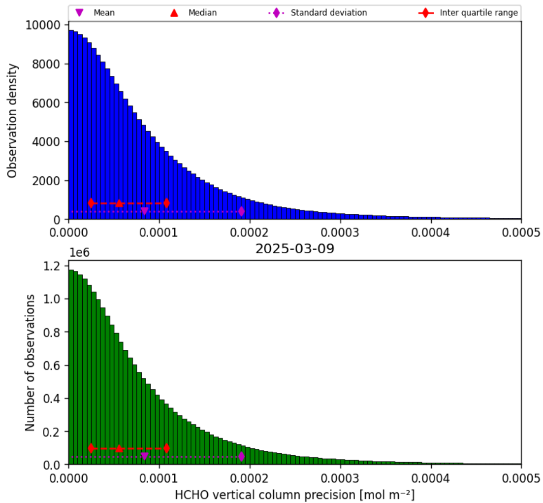
Figure 34: Histogram of “HCHO vertical column precision” for 2025-03-09 to 2025-03-10
