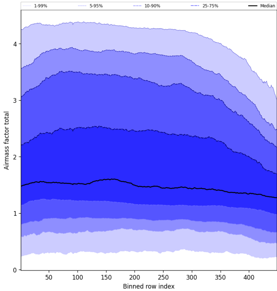
Figure 52: Along track statistics of “Airmass factor total” for 2025-03-09 to 2025-03-10
