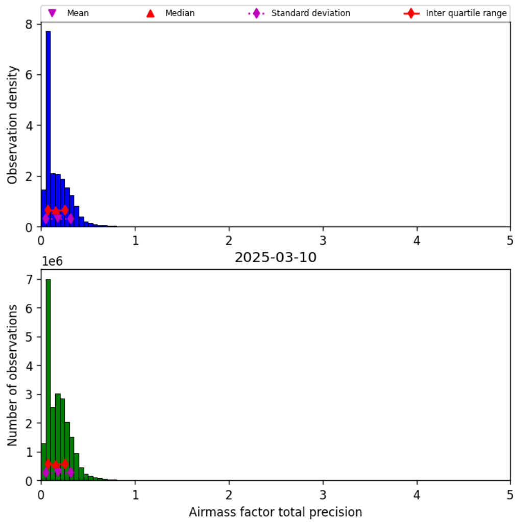
Figure 39: Histogram of “Airmass factor total precision” for 2025-03-10 to 2025-03-10
