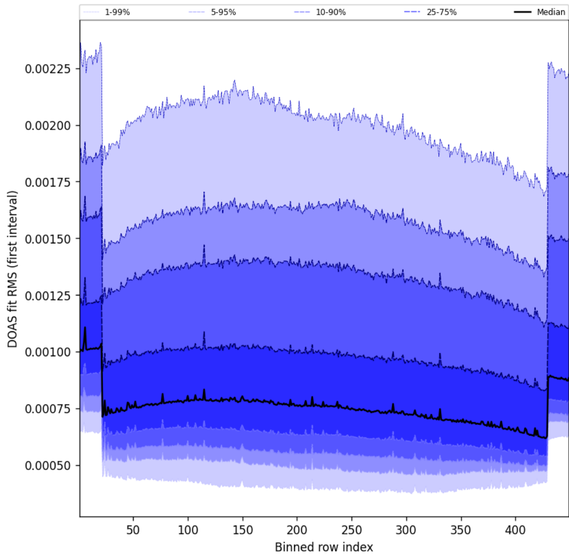
Figure 58: Along track statistics of “DOAS fit RMS (first interval)” for 2025-03-10 to 2025-03-10
