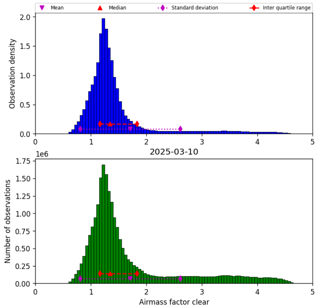
Figure 40: Histogram of “Airmass factor clear” for 2025-03-10 to 2025-03-10
