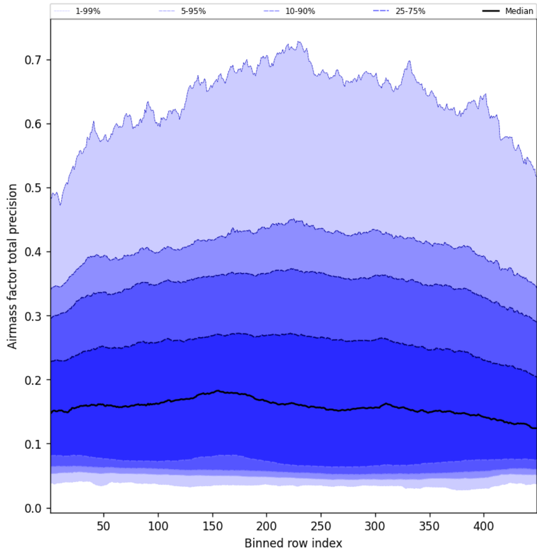
Figure 53: Along track statistics of “Airmass factor total precision” for 2025-03-10 to 2025-03-10
