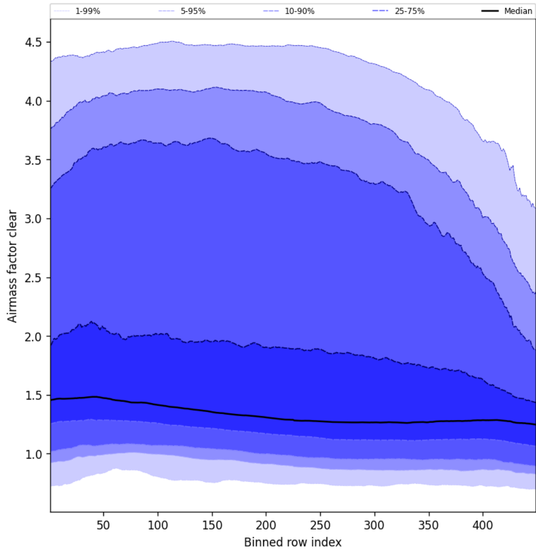
Figure 54: Along track statistics of “Air mass factor clear” for 2025-03-10 to 2025-03-10
