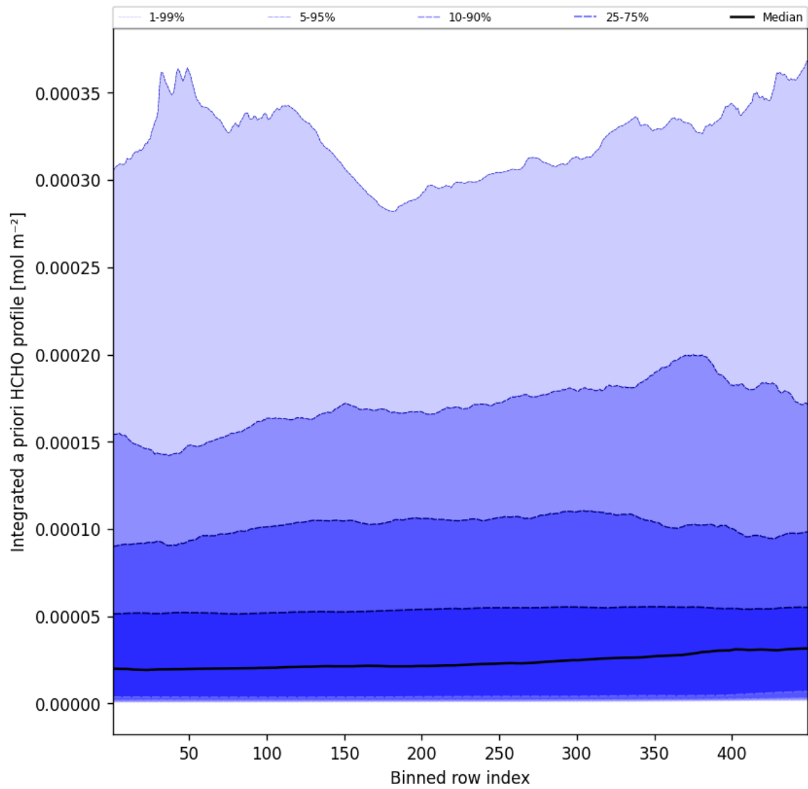
Figure 55: Along track statistics of “Integrated a priori HCHO profile” for 2025-03-10 to 2025-03-10
