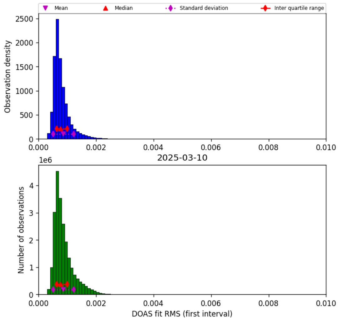
Figure 44: Histogram of “DOAS fit RMS (first interval)” for 2025-03-10 to 2025-03-10
