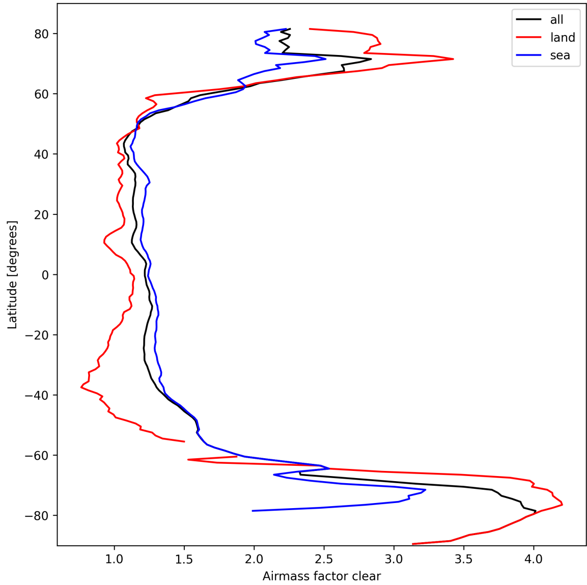
Figure 26: Zonal average of “Airmass factor clear” for 2025-03-10 to 2025-03-10.
