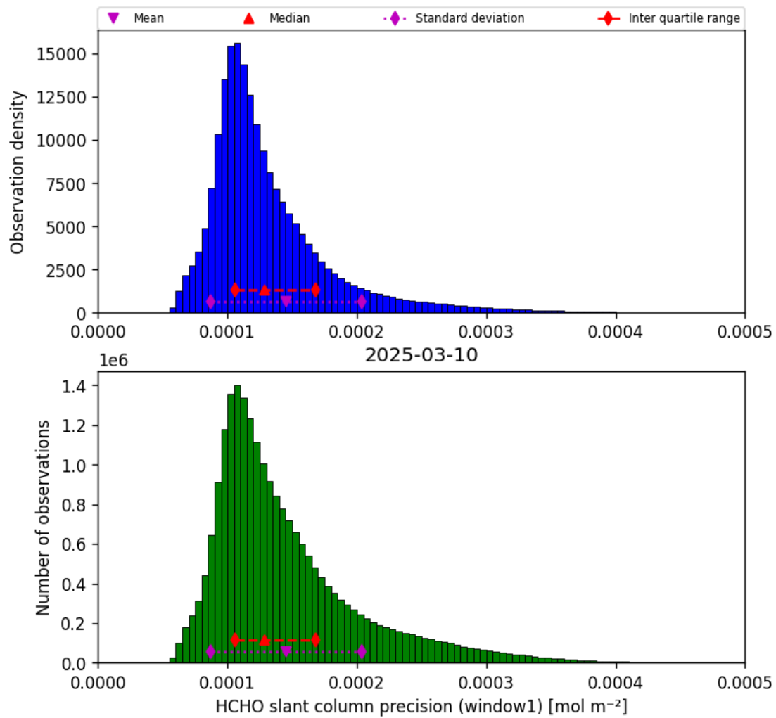
Figure 37: Histogram of “HCHO slant column precision (window1)” for 2025-03-10 to 2025-03-10
