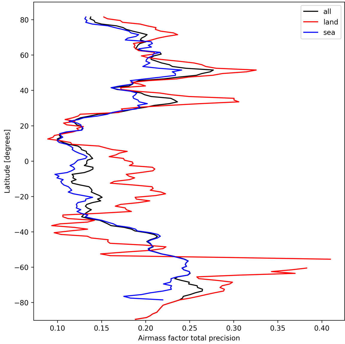
Figure 25: Zonal average of “Airmass factor total precision” for 2025-03-10 to 2025-03-10.
