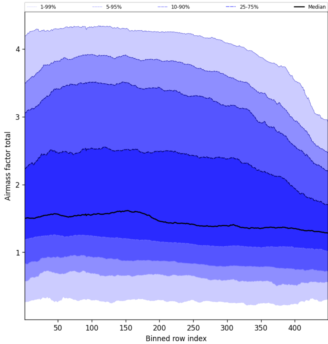
Figure 52: Along track statistics of “Airmass factor total” for 2025-03-10 to 2025-03-10
