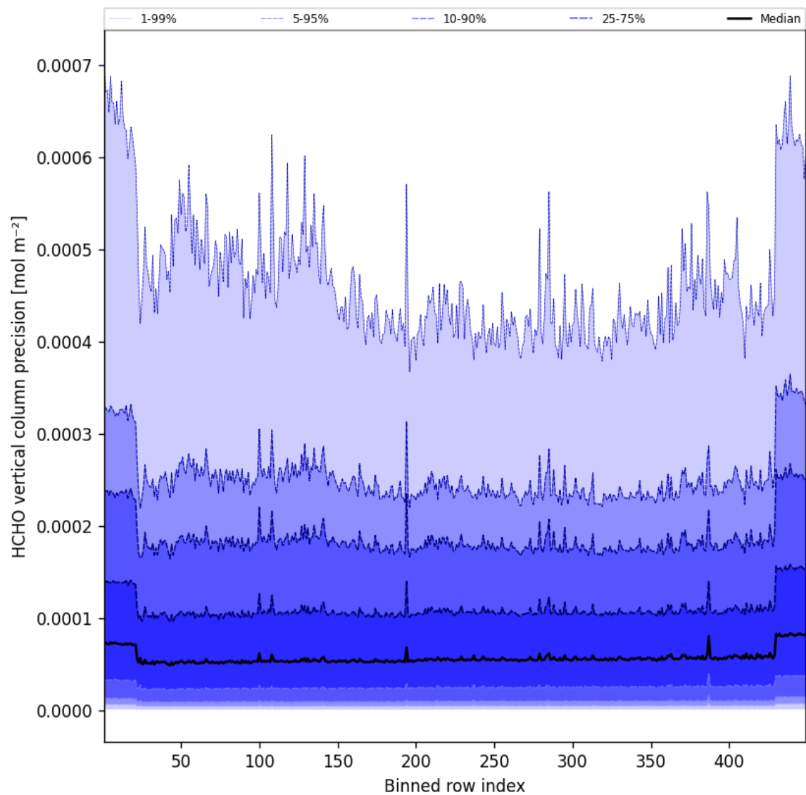
Figure 48: Along track statistics of “HCHO vertical column precision” for 2025-03-10 to 2025-03-10
