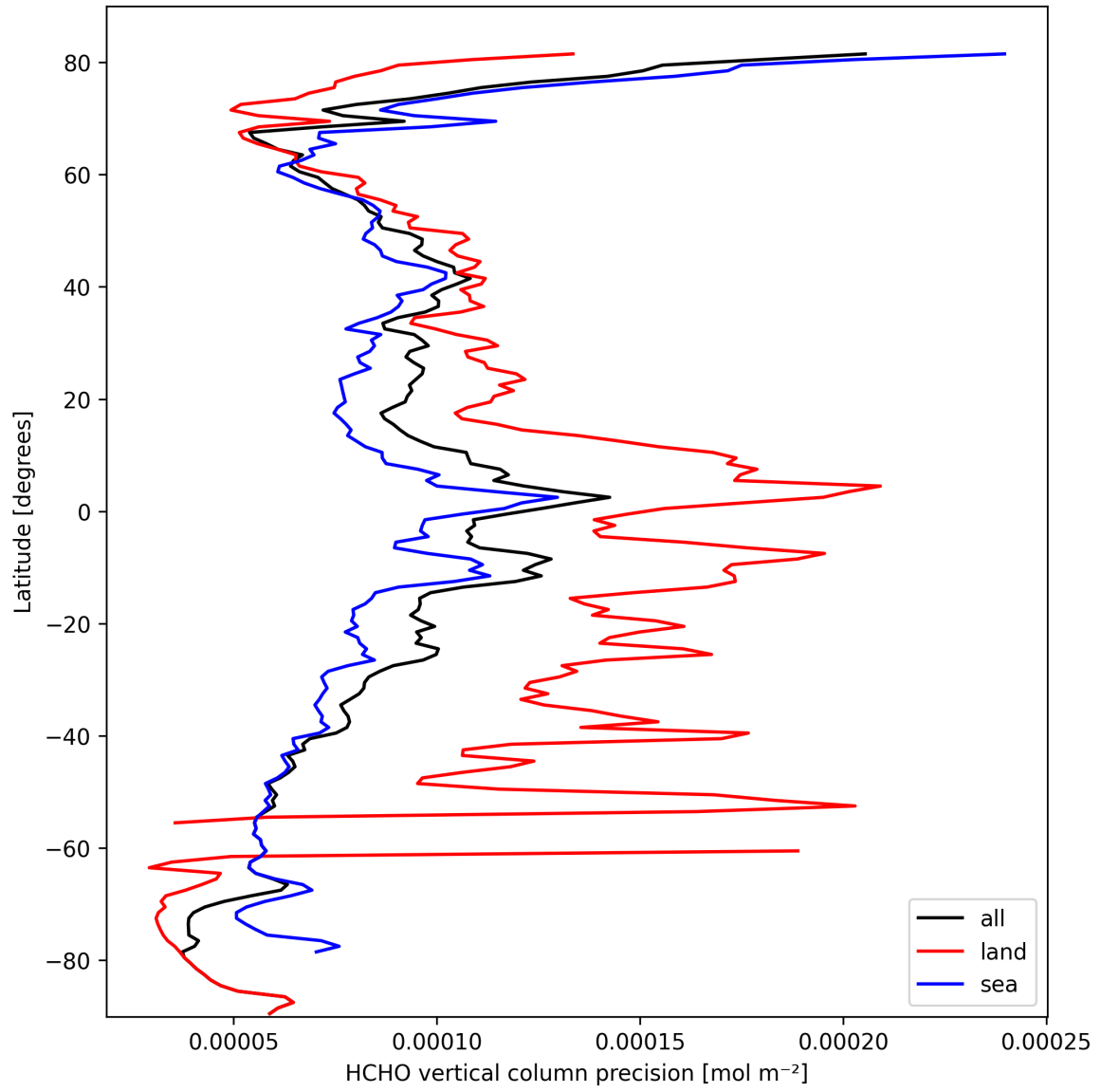
Figure 20: Zonal average of “HCHO vertical column precision” for 2025-03-10 to 2025-03-10.
