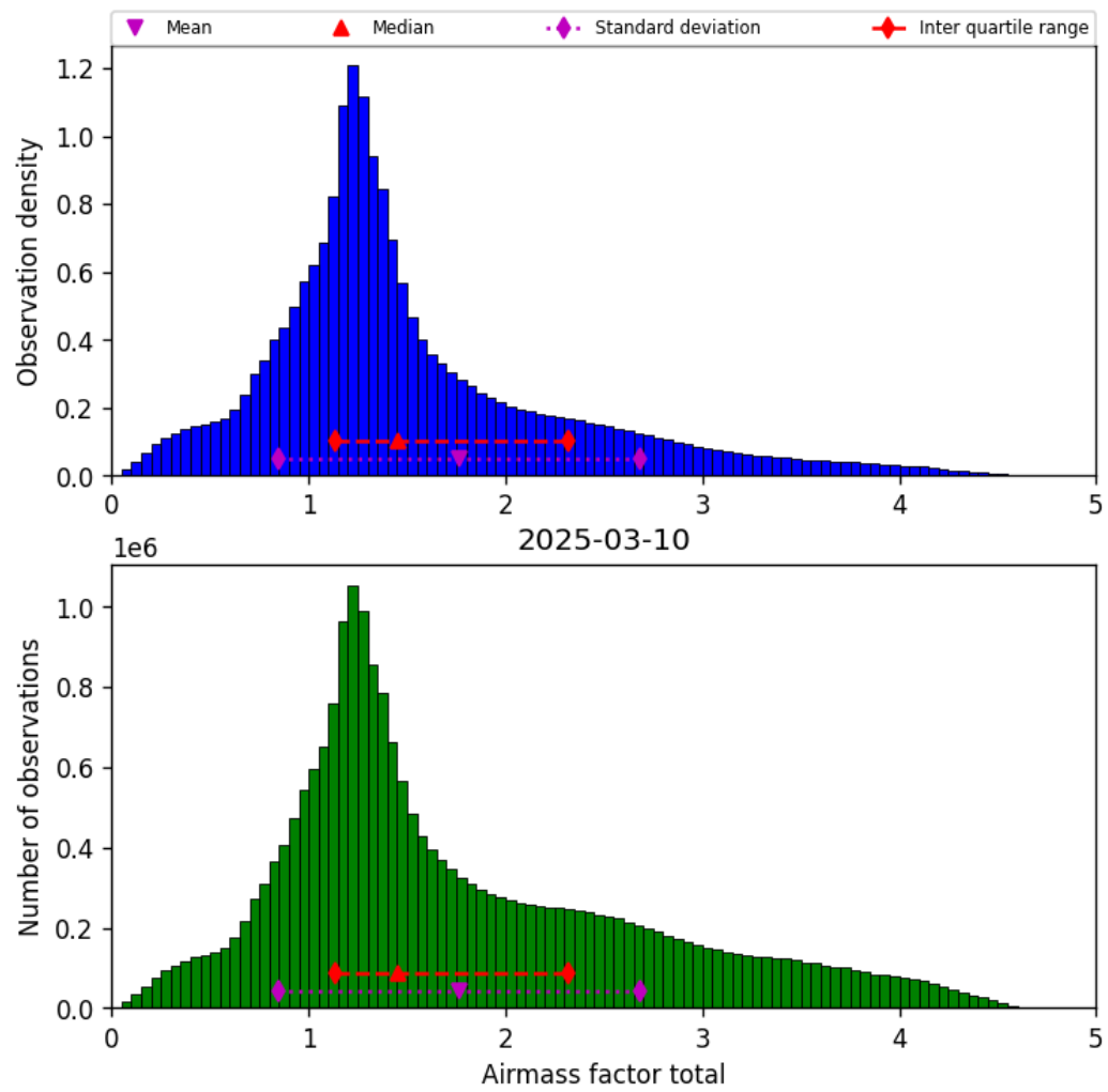
Figure 38: Histogram of “Airmass factor total” for 2025-03-10 to 2025-03-10
