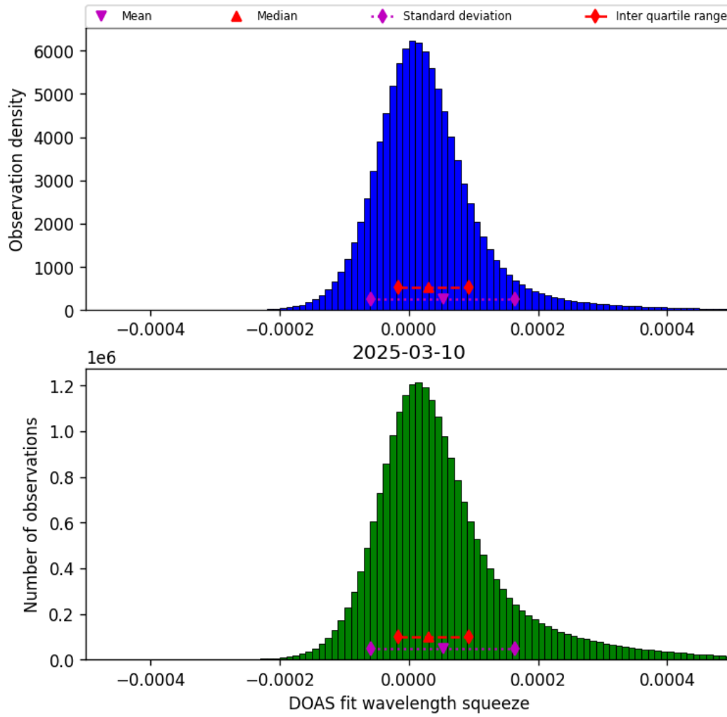
Figure 43: Histogram of “DOAS fit wavelength squeeze” for 2025-03-10 to 2025-03-10
