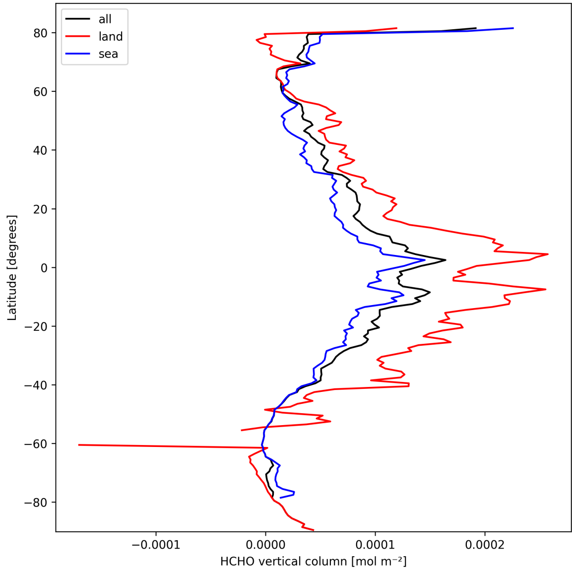
Figure 19: Zonal average of “HCHO vertical column” for 2025-03-10 to 2025-03-10.
