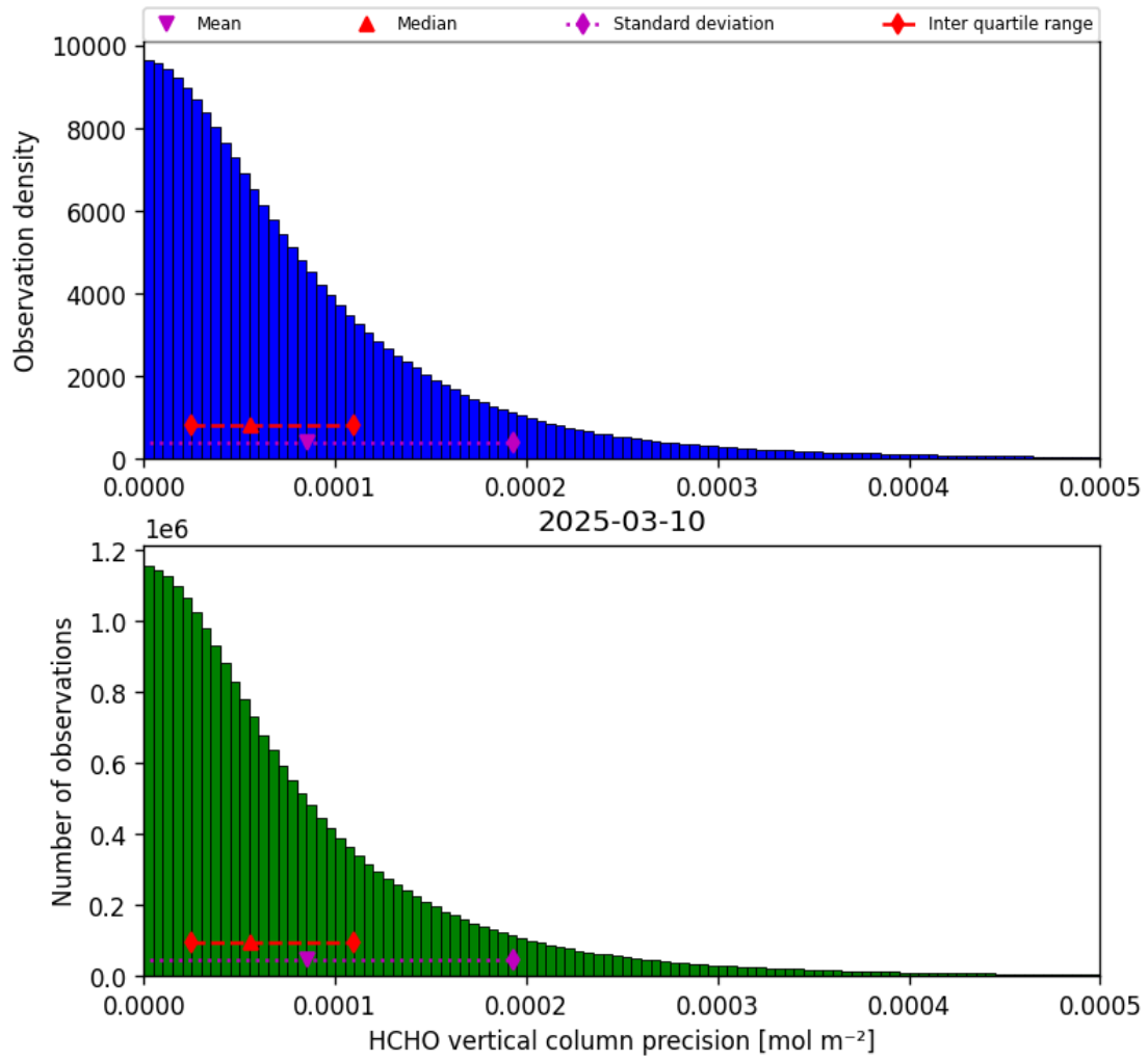
Figure 34: Histogram of "HCHO vertical column precision" for 2025-03-10 to 2025-03-10
