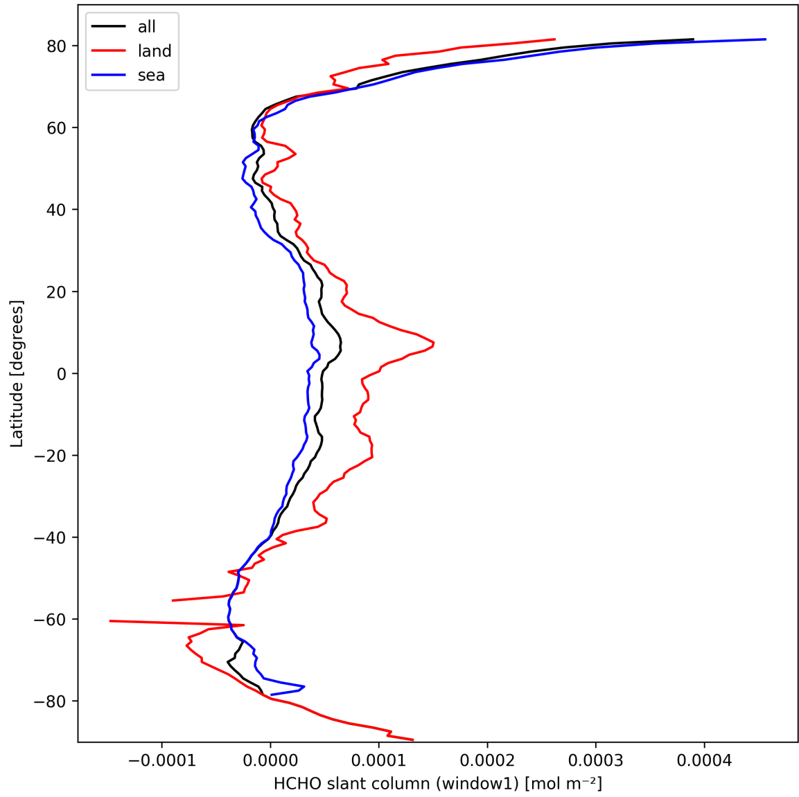
Figure 22: Zonal average of “HCHO slant column (window1)” for 2025-03-10 to 2025-03-10.
