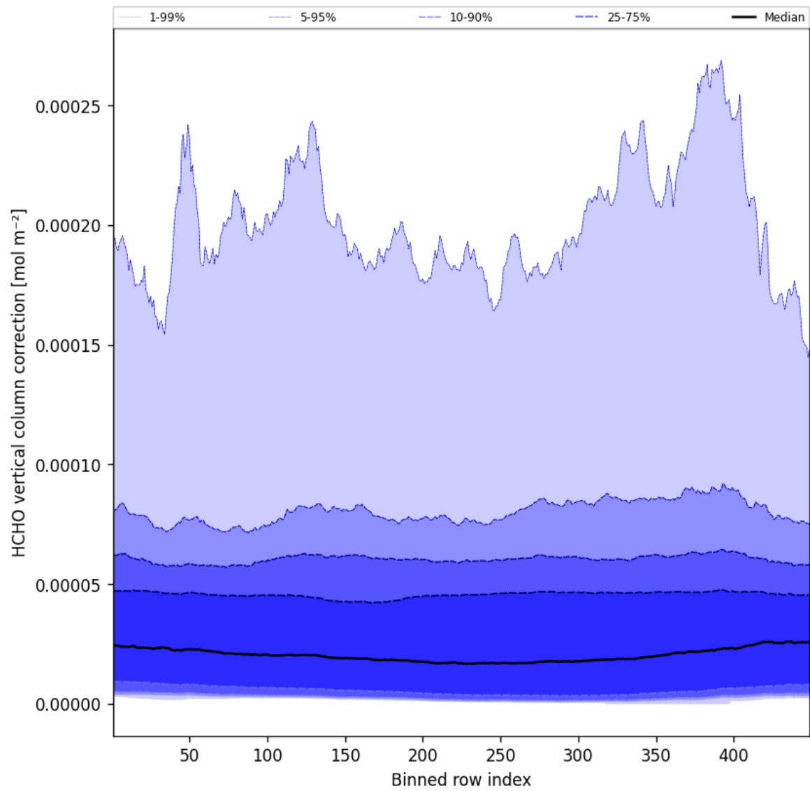
Figure 49: Along track statistics of "HCHO vertical column correction" for 2025-03-10 to 2025-03-10
