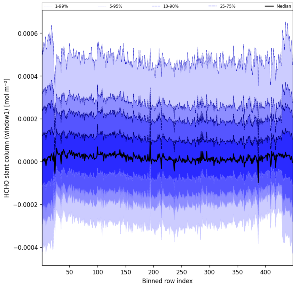
Figure 50: Along track statistics of “HCHO slant column (window1)” for 2025-03-10 to 2025-03-10
