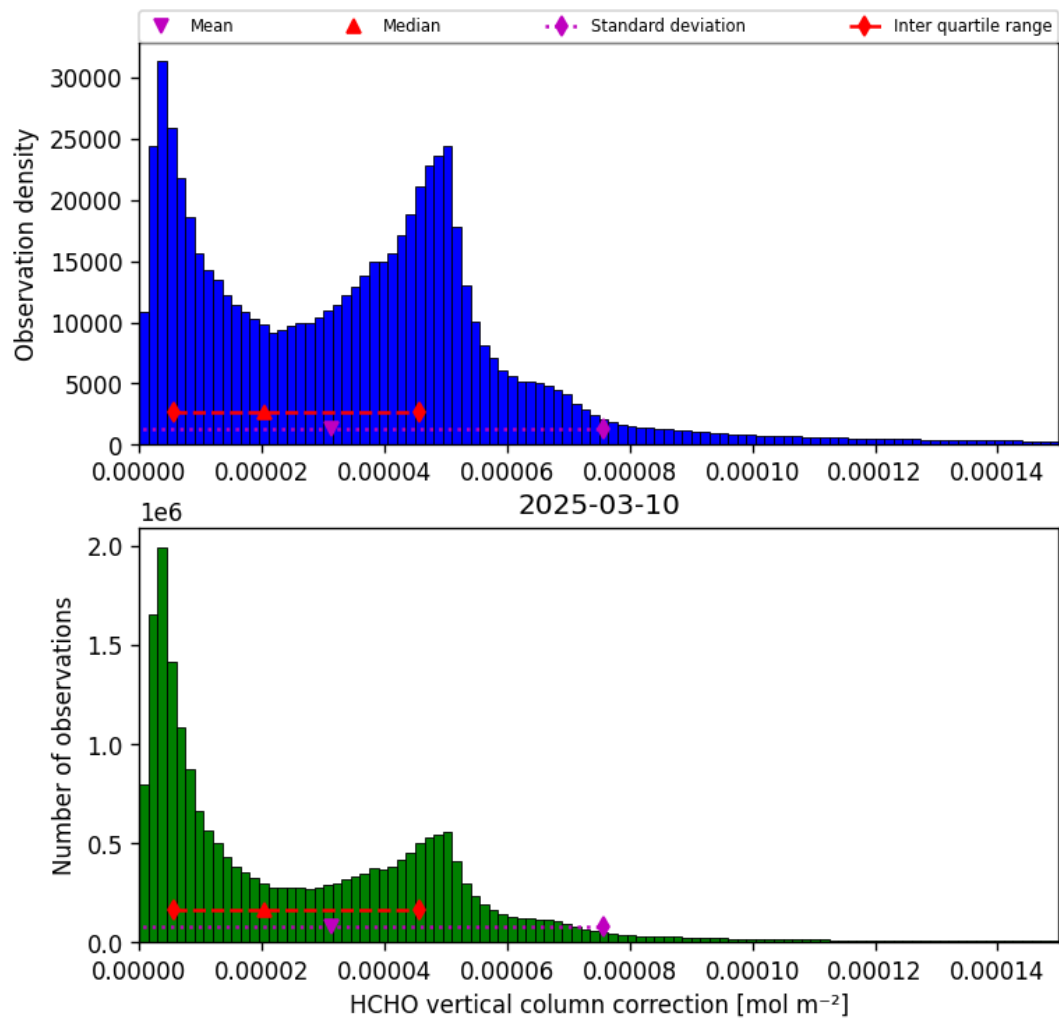
Figure 35: Histogram of “HCHO vertical column correction” for 2025-03-10 to 2025-03-10
