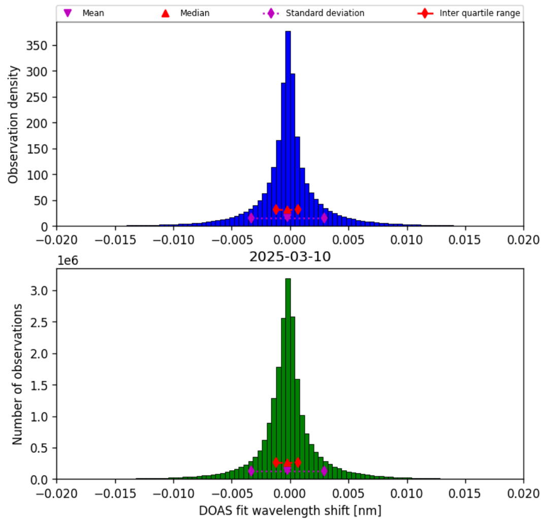
Figure 42: Histogram of “DOAS fit wavelength shift” for 2025-03-10 to 2025-03-10
