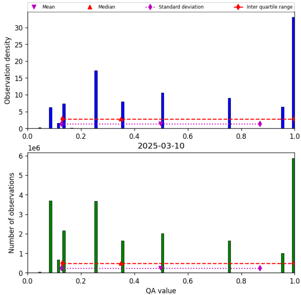
Figure 32: Histogram of “QA value” for 2025-03-10 to 2025-03-10
