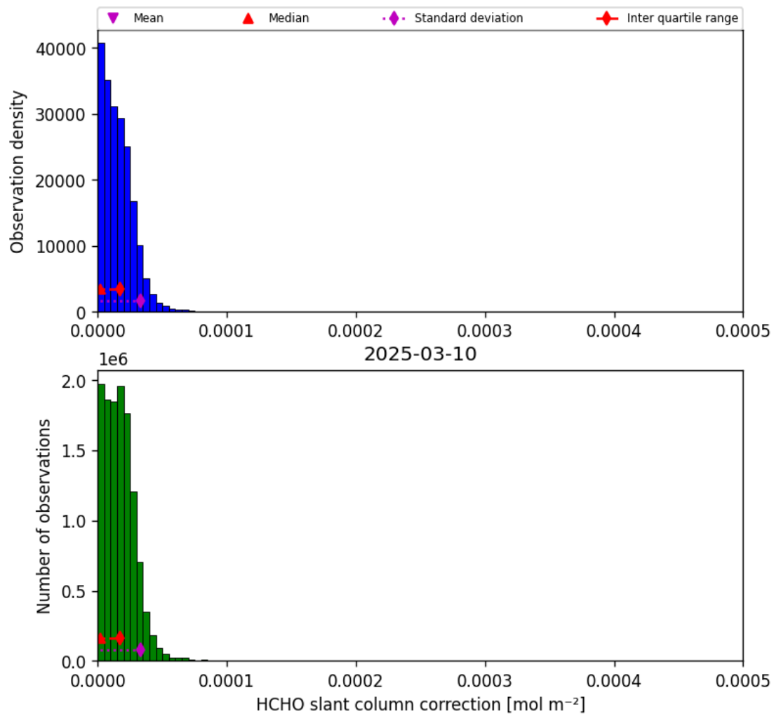
Figure 45: Histogram of “HCHO slant column correction” for 2025-03-10 to 2025-03-10
