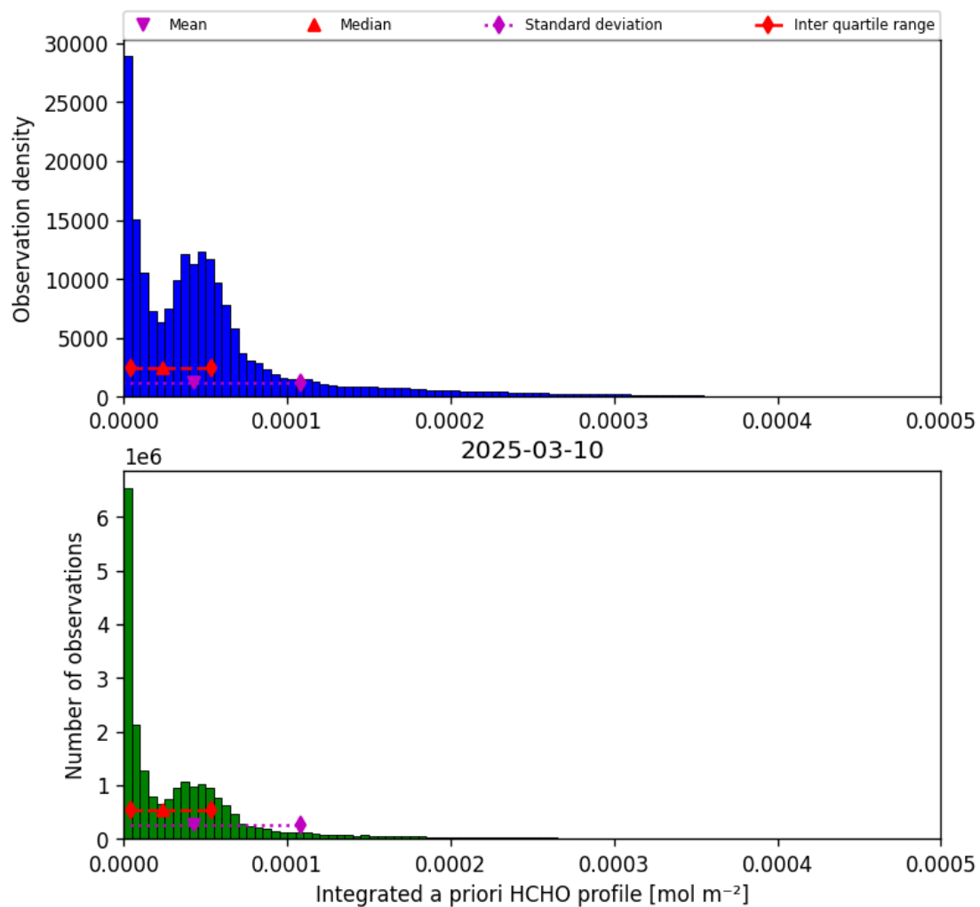
Figure 41: Histogram of “Integrated a priori HCHO profile” for 2025-03-10 to 2025-03-10
