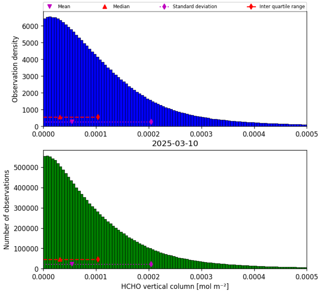
Figure 33: Histogram of “HCHO vertical column” for 2025-03-10 to 2025-03-10
