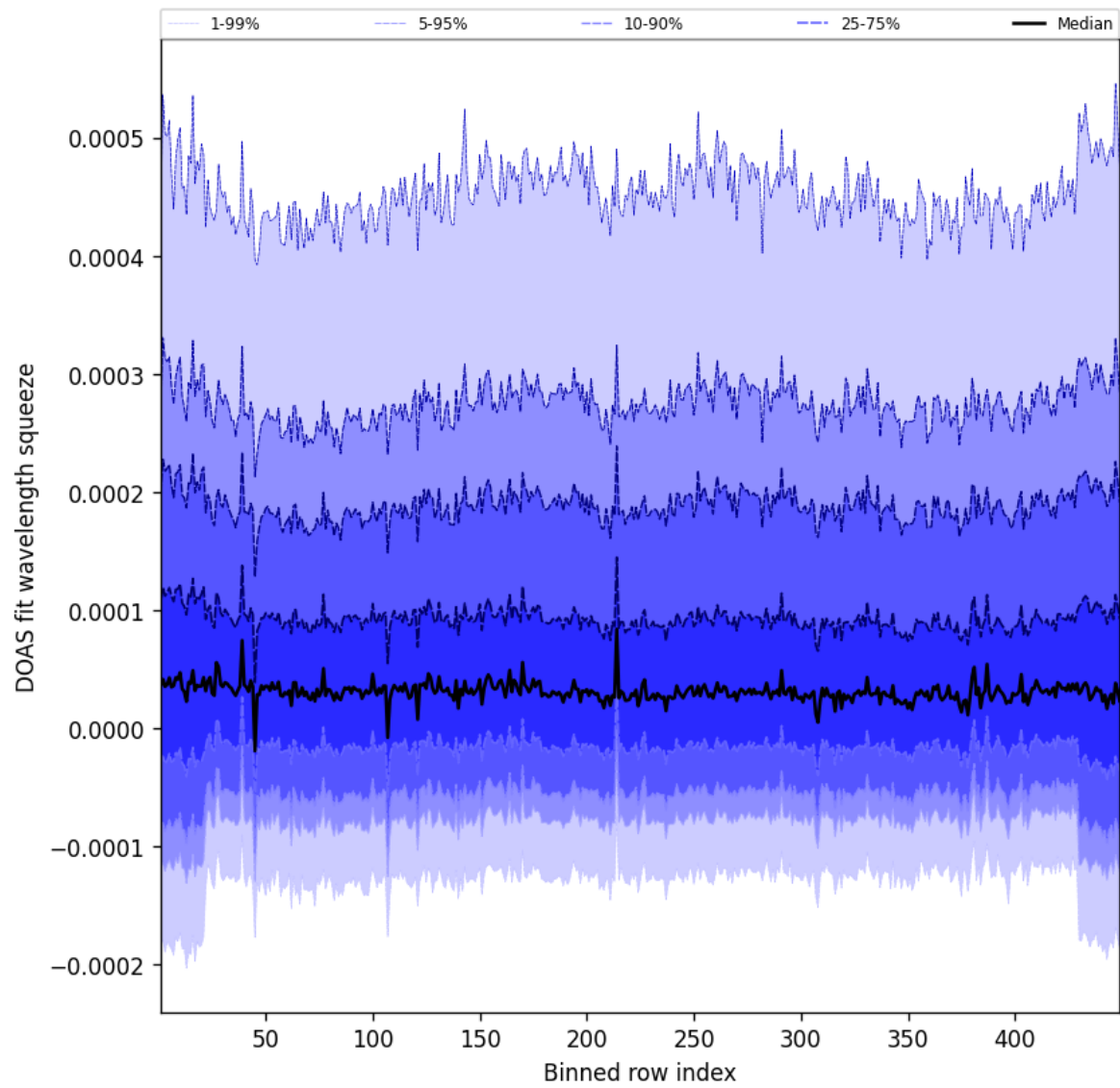
Figure 57: Along track statistics of “DOAS fit wavelength squeeze” for 2025-03-10 to 2025-03-10
