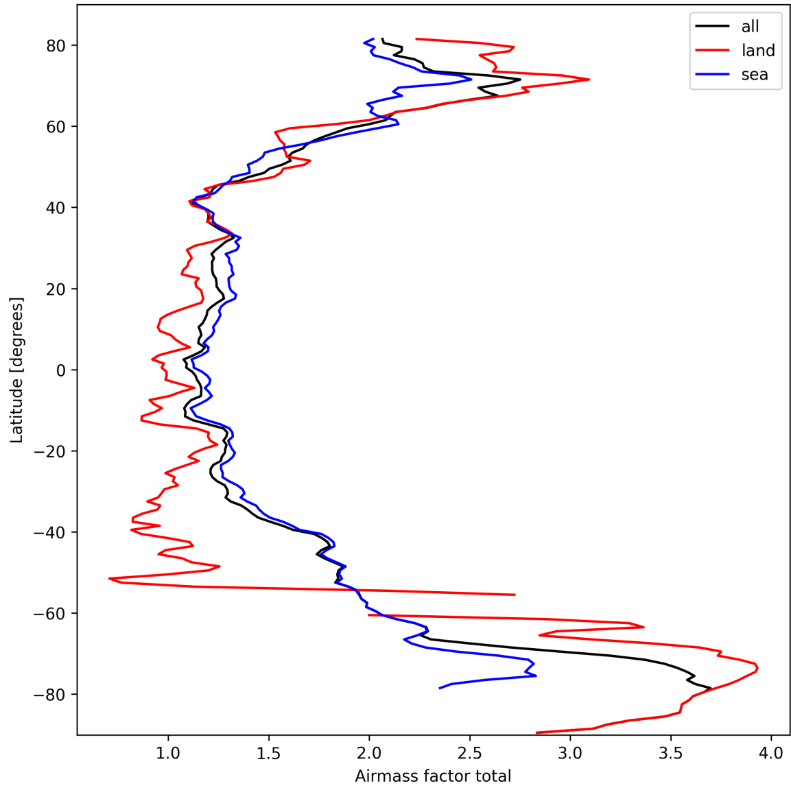
Figure 24: Zonal average of “Airmass factor total” for 2025-03-10 to 2025-03-10.
