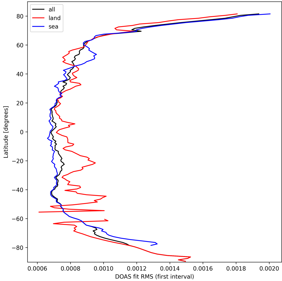
Figure 30: Zonal average of “DOAS fit RMS (first interval)” for 2025-03-10 to 2025-03-10.
