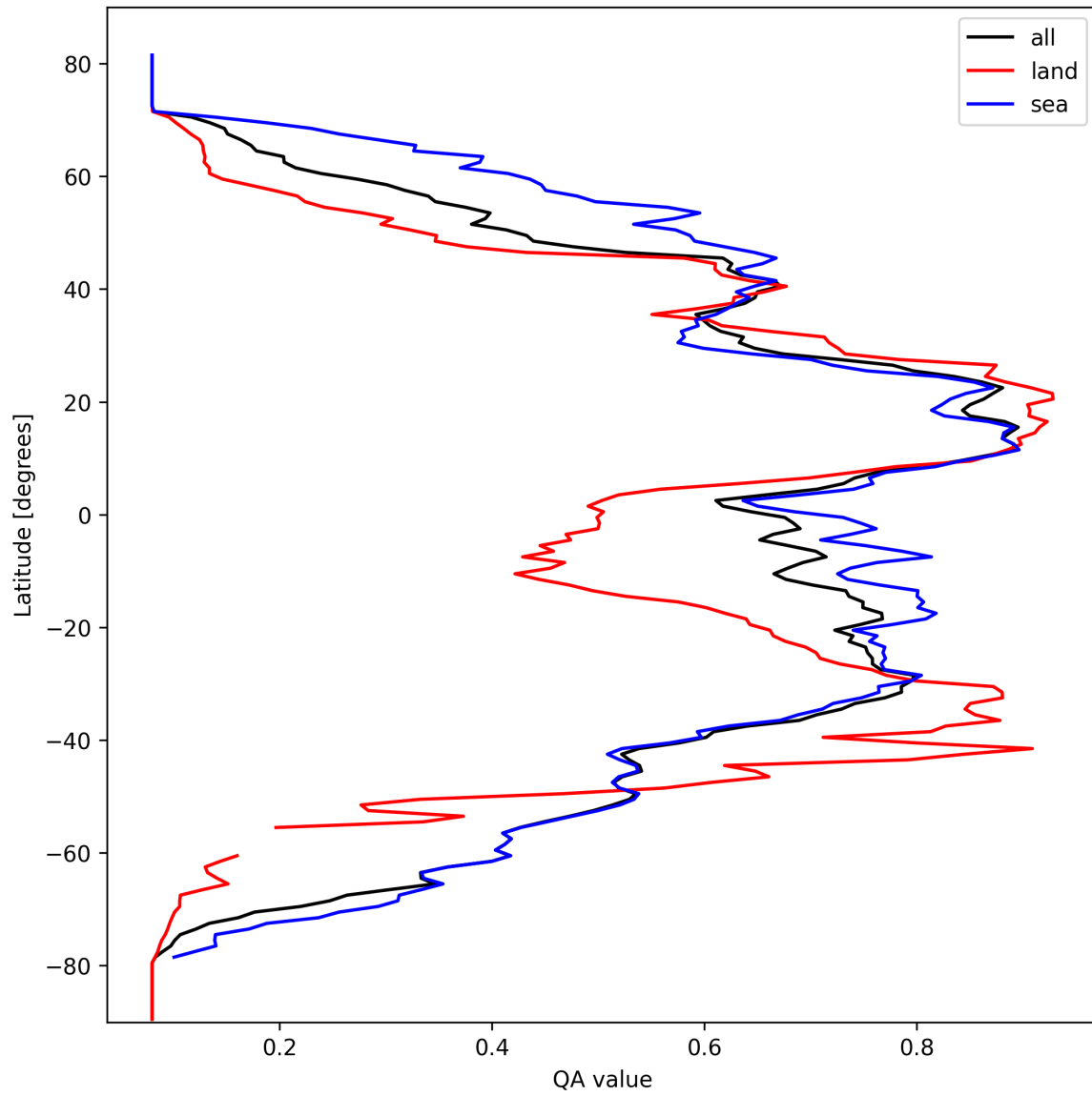
Figure 18: Zonal average of “QA value” for 2025-03-10 to 2025-03-10.
