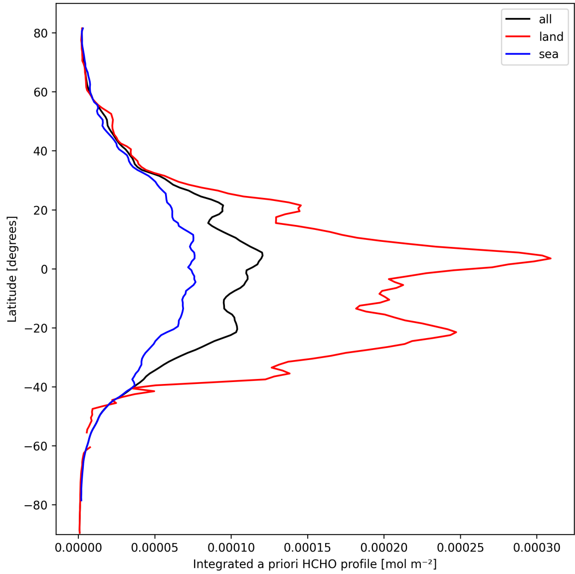
Figure 27: Zonal average of “Integrated a priori HCHO profile” for 2025-03-10 to 2025-03-10.
