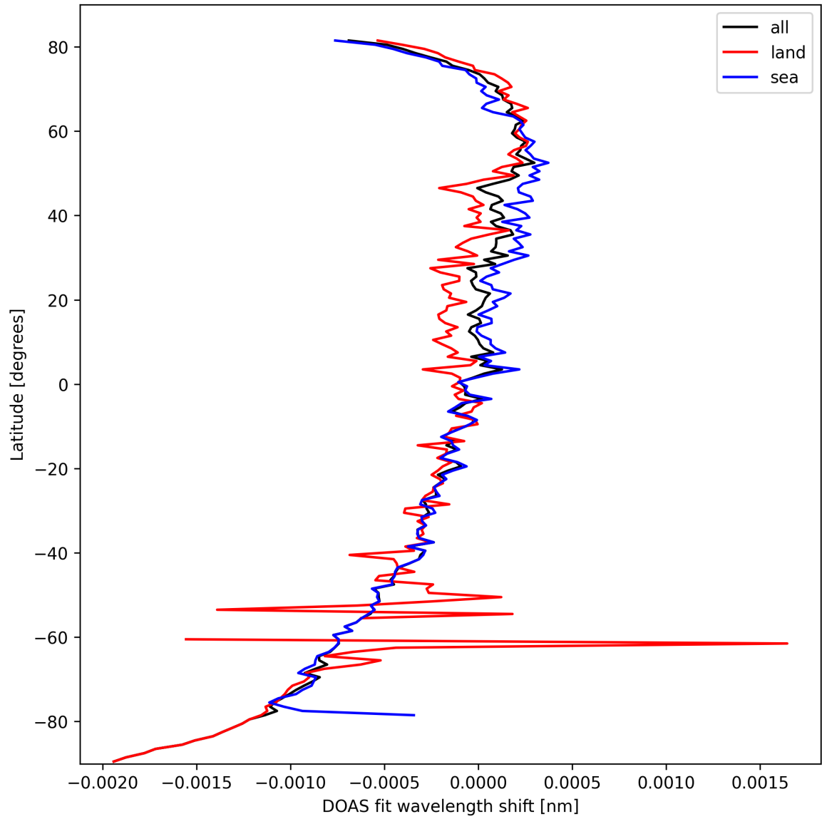
Figure 28: Zonal average of “DOAS fit wavelength shift” for 2025-03-10 to 2025-03-10.
