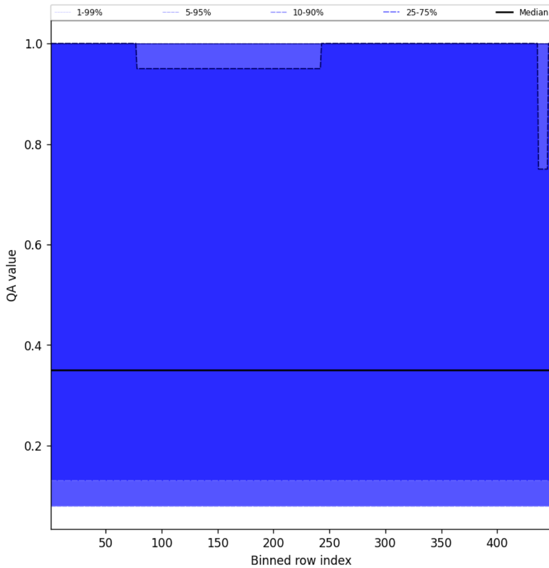
Figure 46: Along track statistics of “QA value” for 2025-03-10 to 2025-03-10
