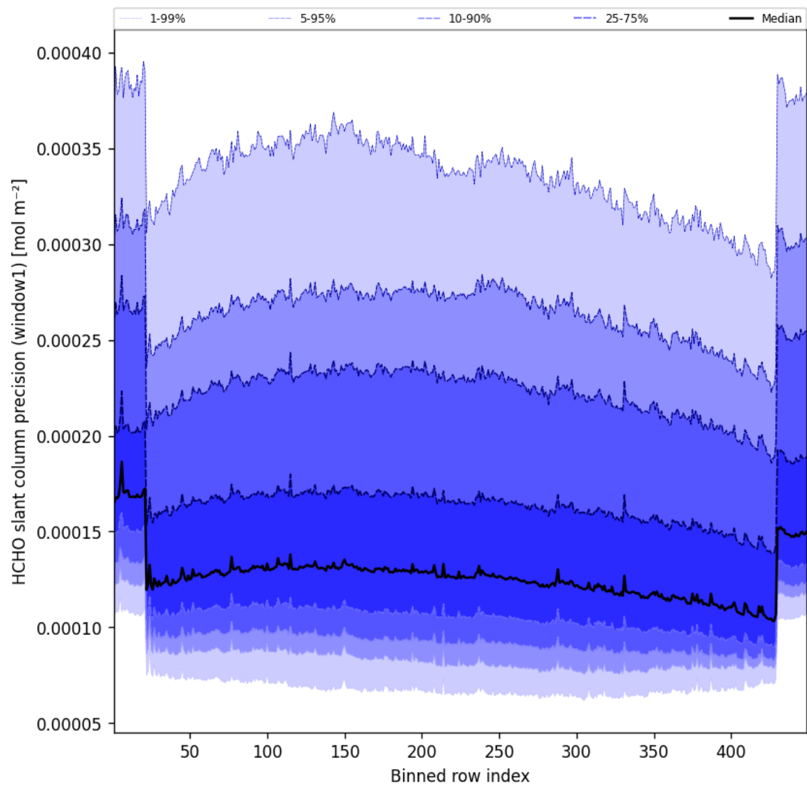
Figure 51: Along track statistics of “HCHO slant column precision (window1)” for 2025-03-10 to 2025-03-10
