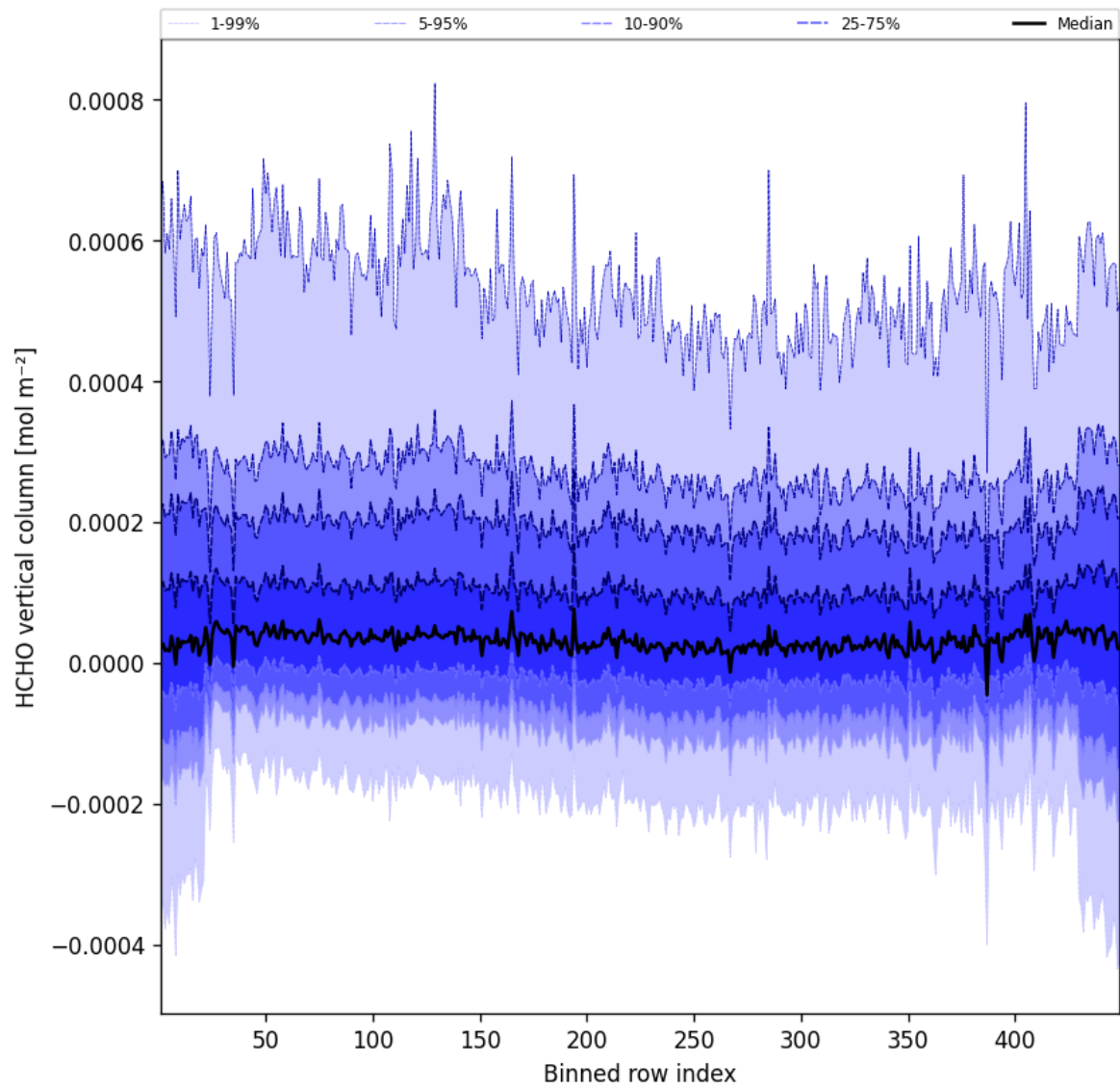
Figure 47: Along track statistics of “HCHO vertical column” for 2025-03-10 to 2025-03-10
