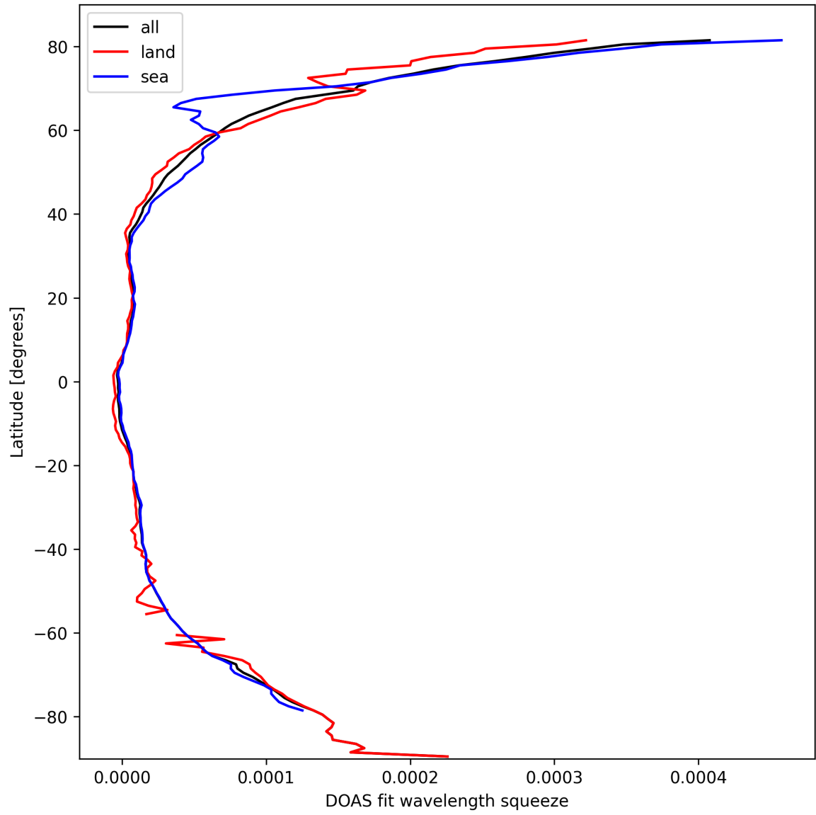
Figure 29: Zonal average of “DOAS fit wavelength squeeze” for 2025-03-10 to 2025-03-10.
