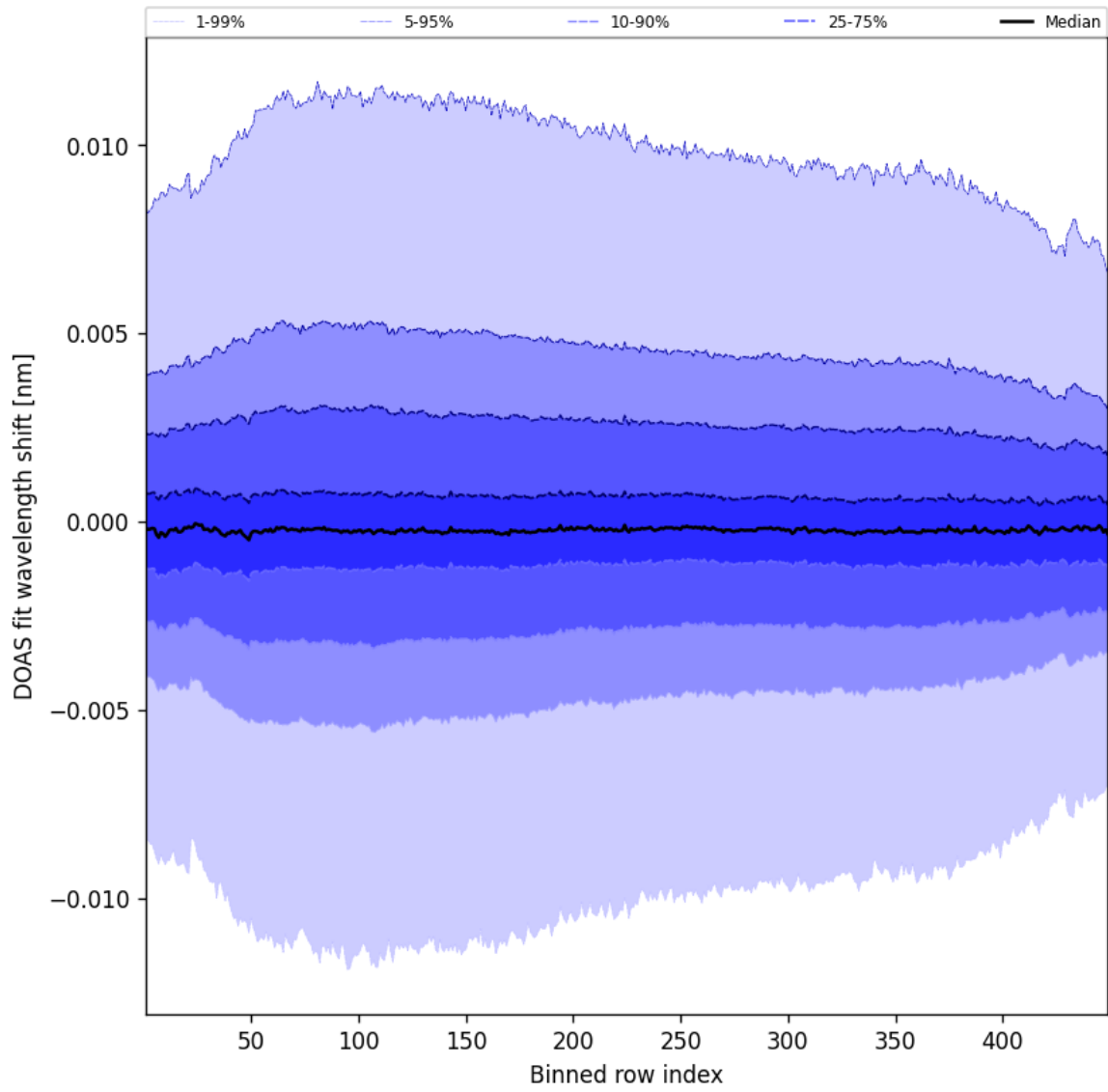
Figure 56: Along track statistics of “DOAS fit wavelength shift” for 2025-03-10 to 2025-03-10
