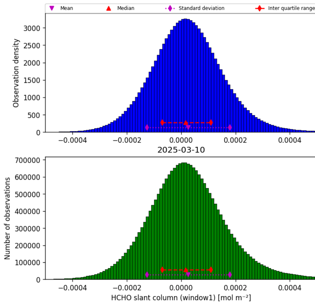
Figure 36: Histogram of “HCHO slant column (window1)” for 2025-03-10 to 2025-03-10
