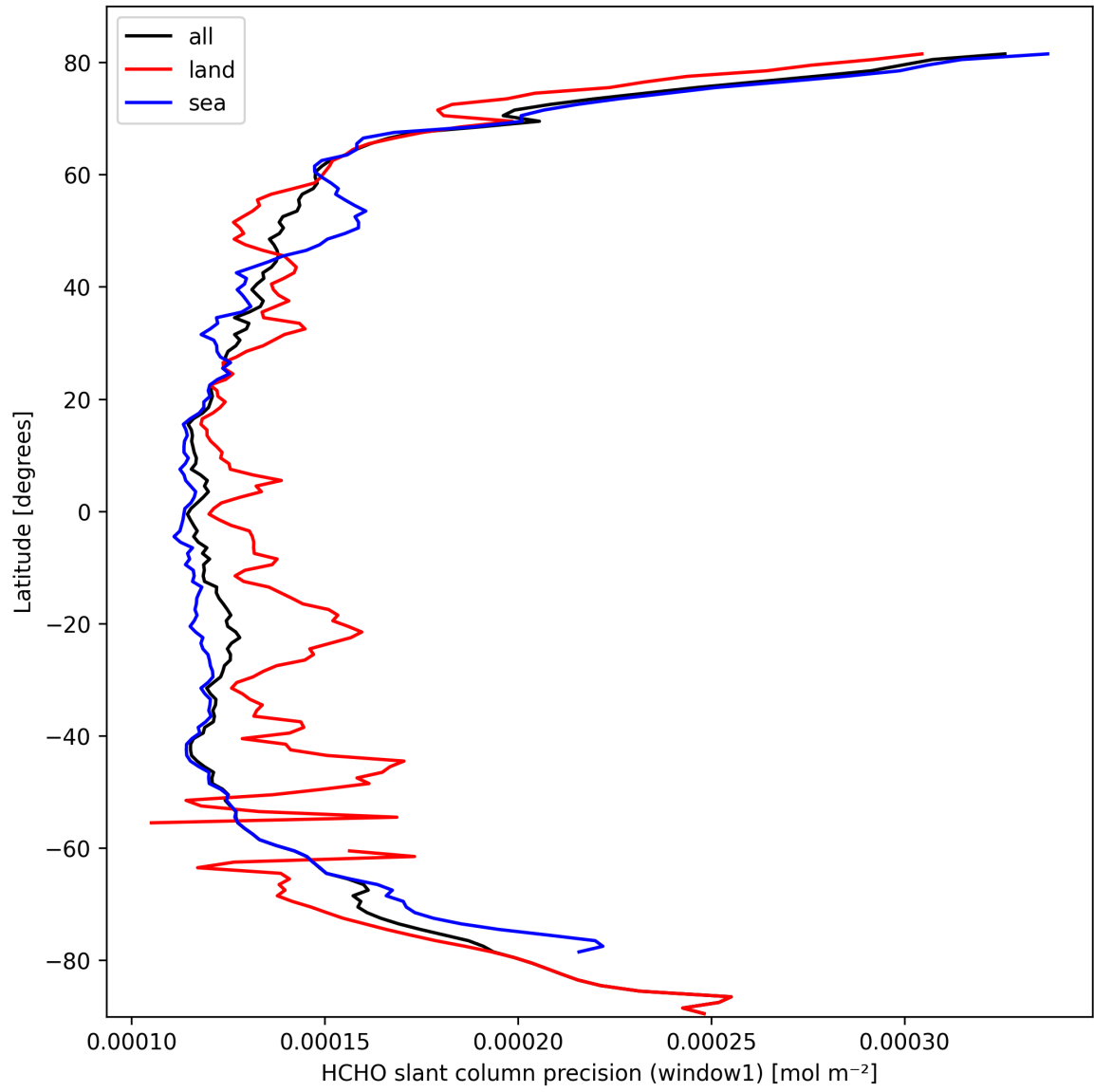
Figure 23: Zonal average of “HCHO slant column precision (window1)” for 2025-03-10 to 2025-03-10.
