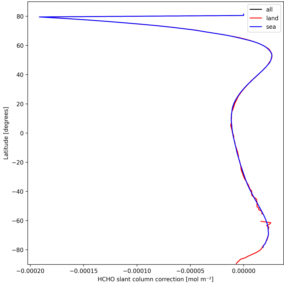
Figure 31: Zonal average of “HCHO slant column correction” for 2025-03-10 to 2025-03-10.
