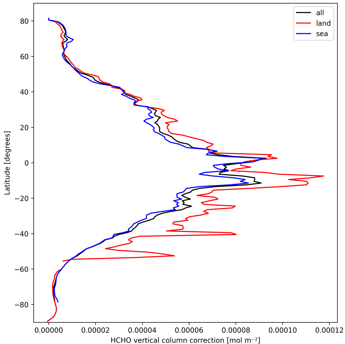
Figure 21: Zonal average of “HCHO vertical column correction” for 2025-03-10 to 2025-03-10.
