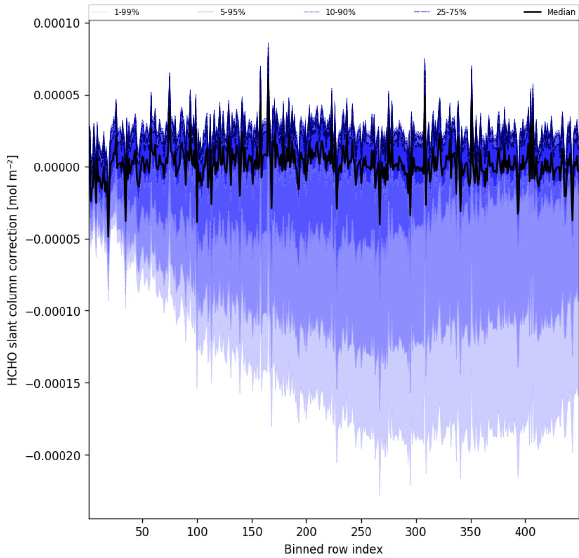
Figure 59: Along track statistics of “HCHO slant column correction” for 2025-03-10 to 2025-03-10
