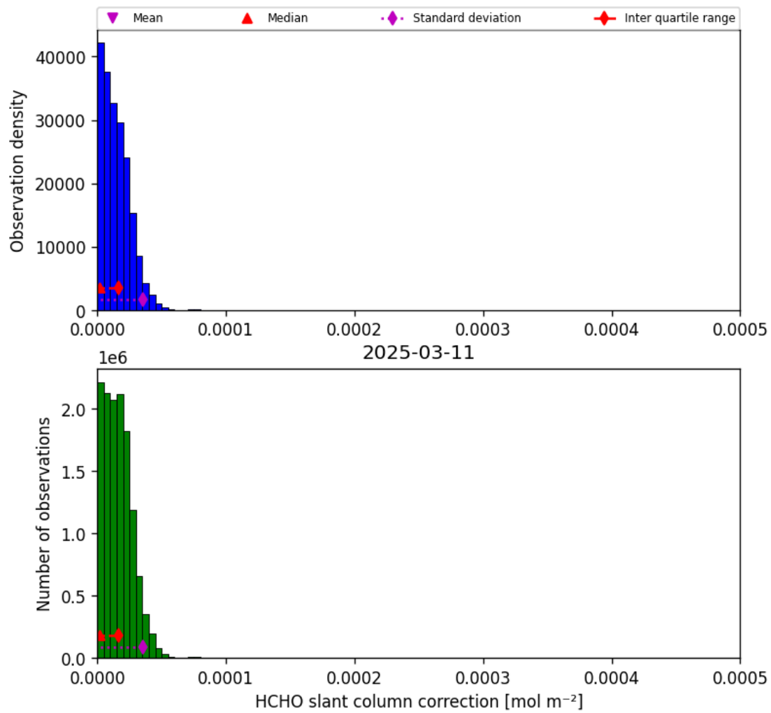
Figure 45: Histogram of “HCHO slant column correction” for 2025-03-11 to 2025-03-12
