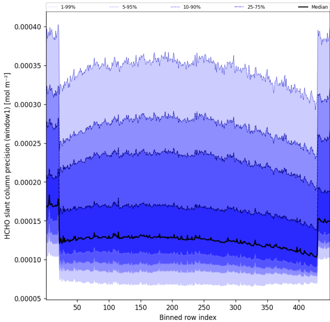
Figure 51: Along track statistics of “HCHO slant column precision (window1)” for 2025-03-11 to 2025-03-12
