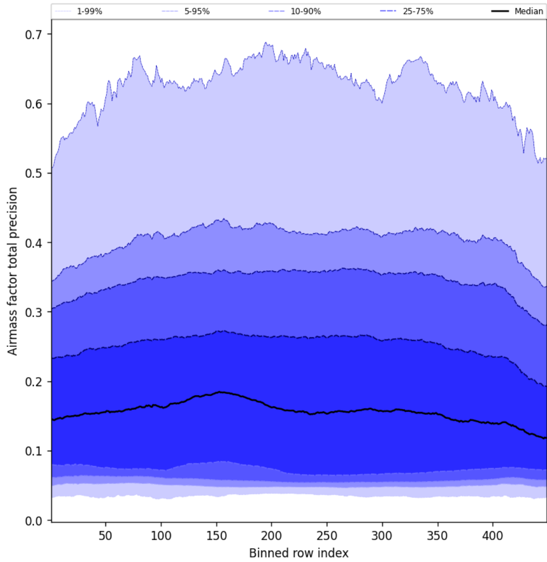
Figure 53: Along track statistics of “Airmass factor total precision” for 2025-03-11 to 2025-03-12
