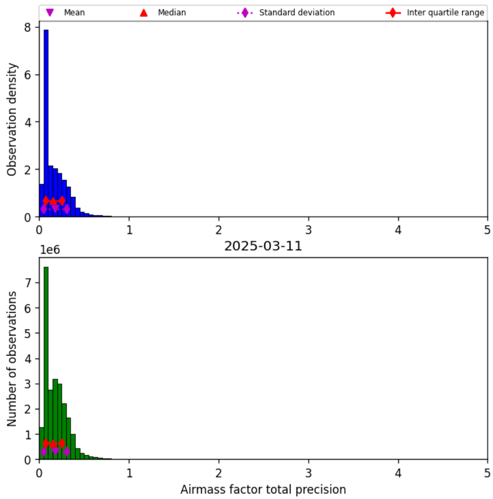
Figure 39: Histogram of “Airmass factor total precision” for 2025-03-11 to 2025-03-12
