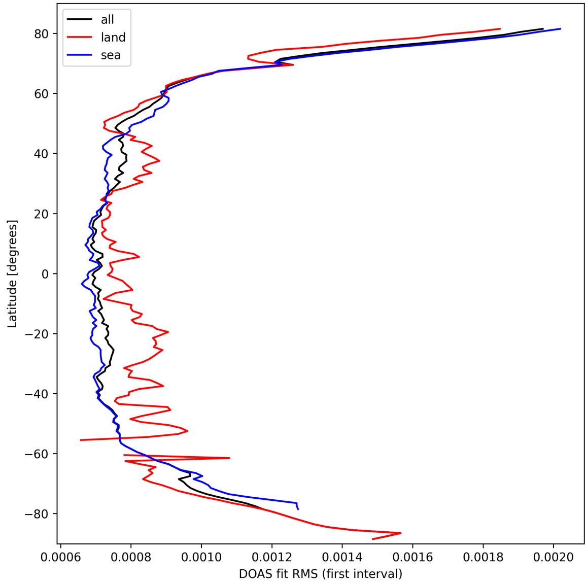
Figure 30: Zonal average of "DOAS fit RMS (first interval)" for 2025-03-11 to 2025-03-12.
