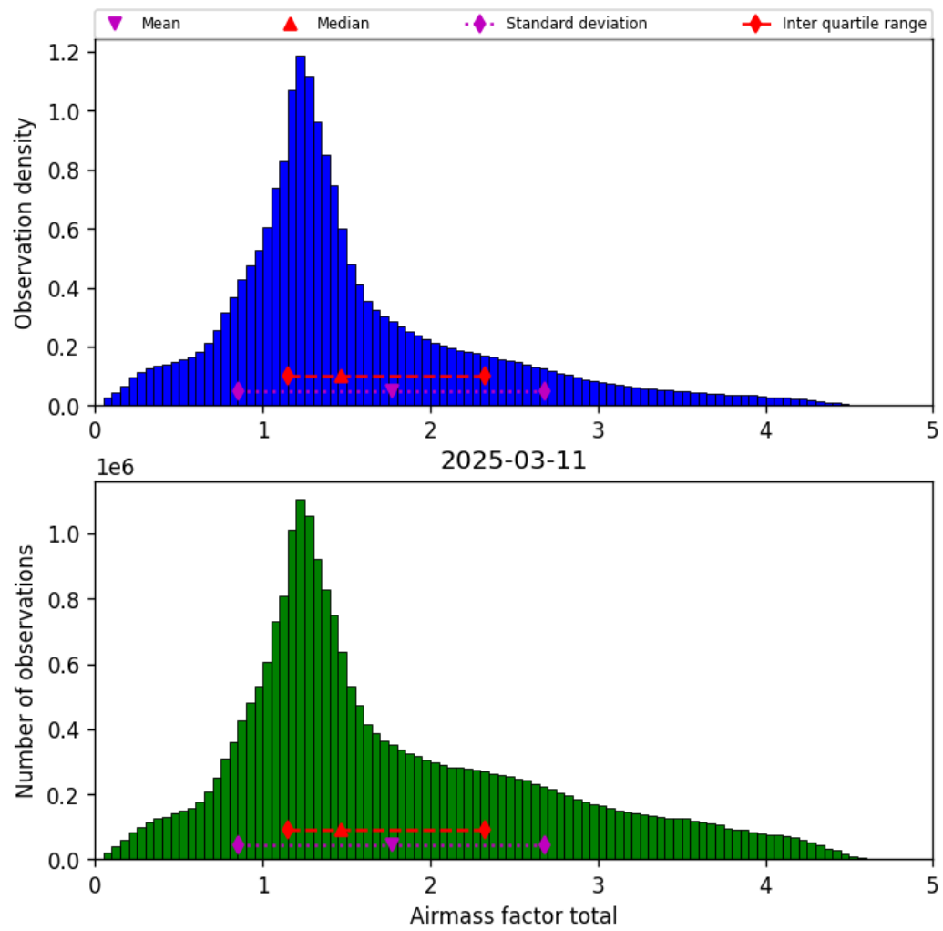
Figure 38: Histogram of “Airmass factor total” for 2025-03-11 to 2025-03-12
