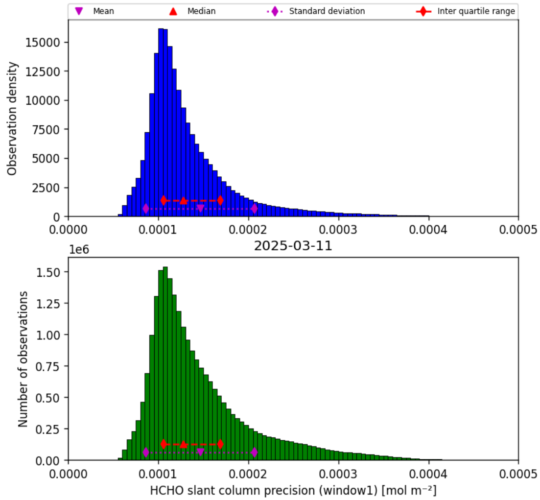
Figure 37: Histogram of “HCHO slant column precision (window1)” for 2025-03-11 to 2025-03-12
