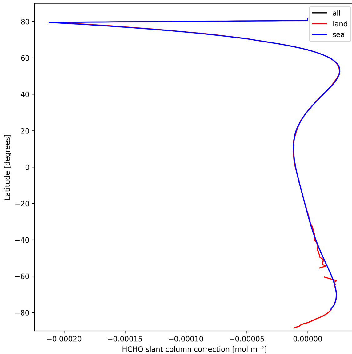
Figure 31: Zonal average of “HCHO slant column correction” for 2025-03-11 to 2025-03-12.
