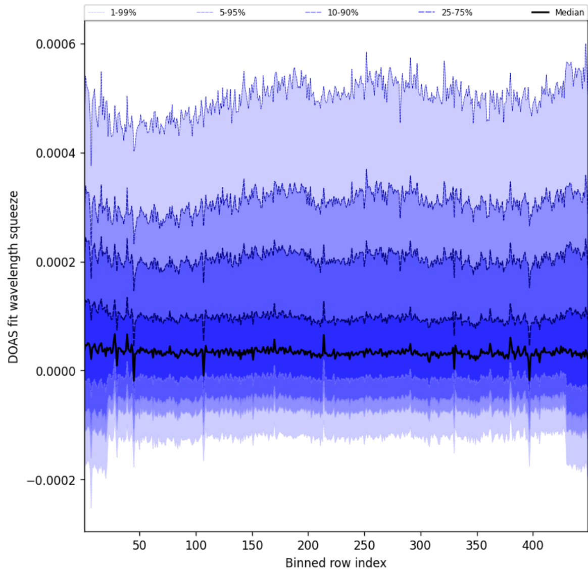
Figure 57: Along track statistics of “DOAS fit wavelength squeeze” for 2025-03-11 to 2025-03-12
