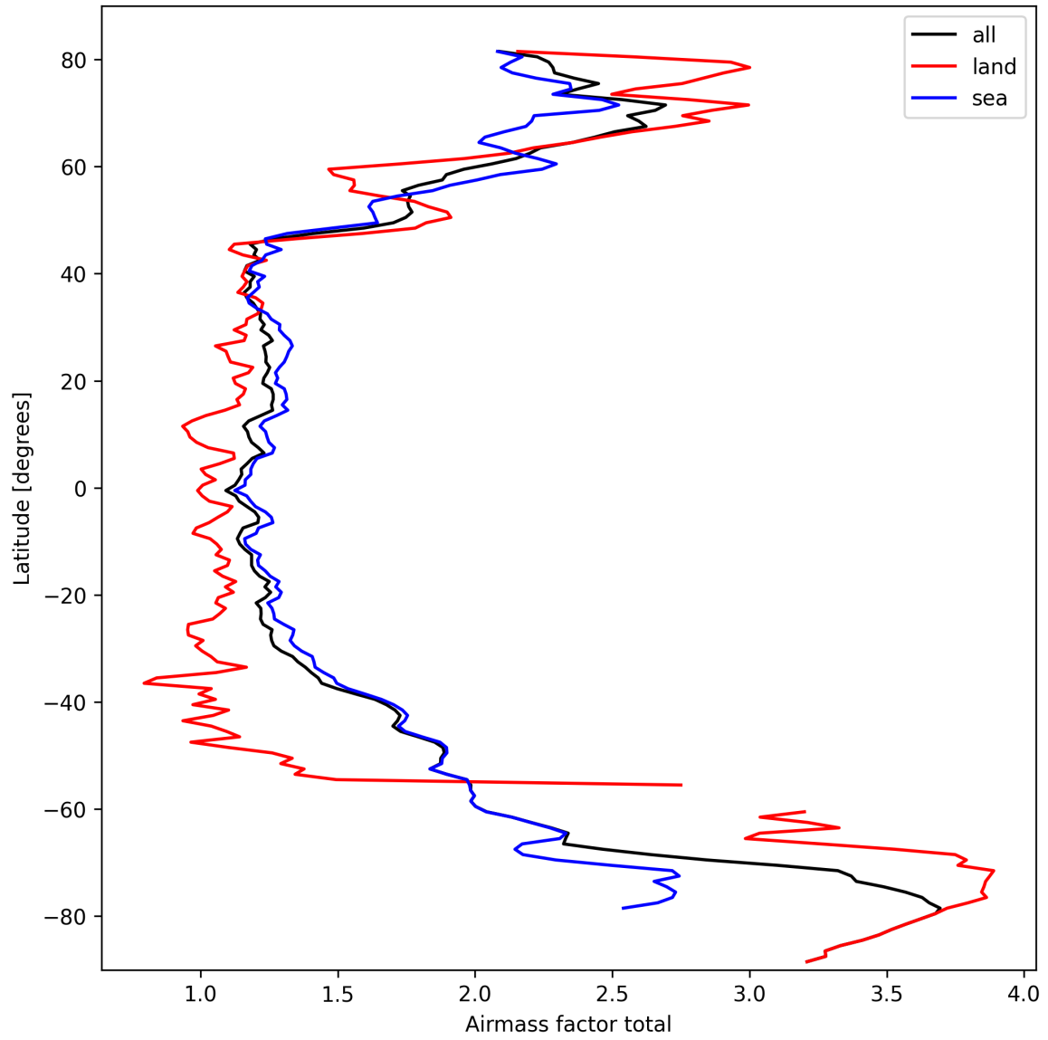
Figure 24: Zonal average of “Airmass factor total” for 2025-03-11 to 2025-03-12.
