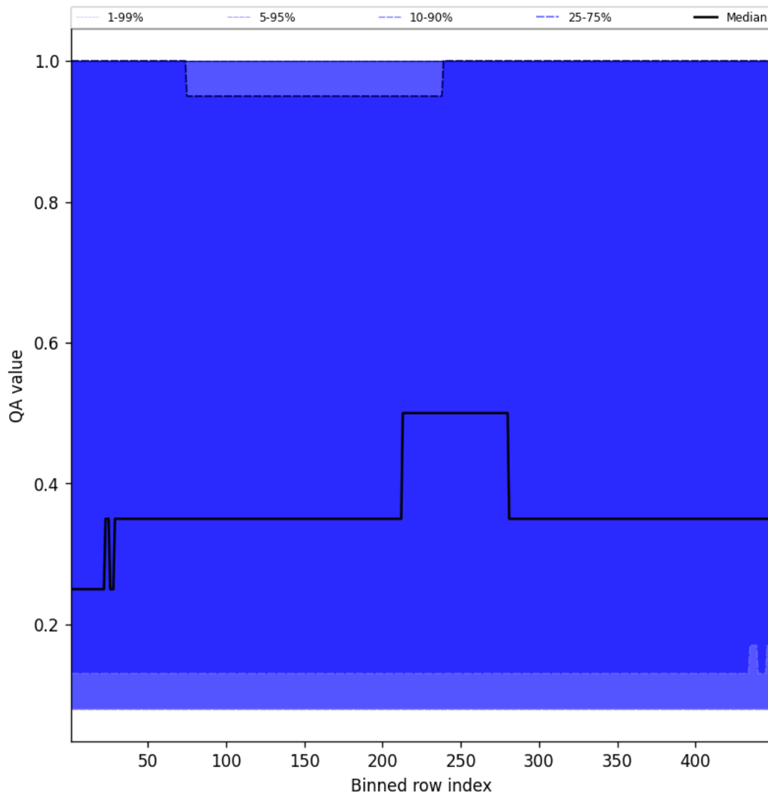
Figure 46: Along track statistics of “QA value” for 2025-03-11 to 2025-03-12
