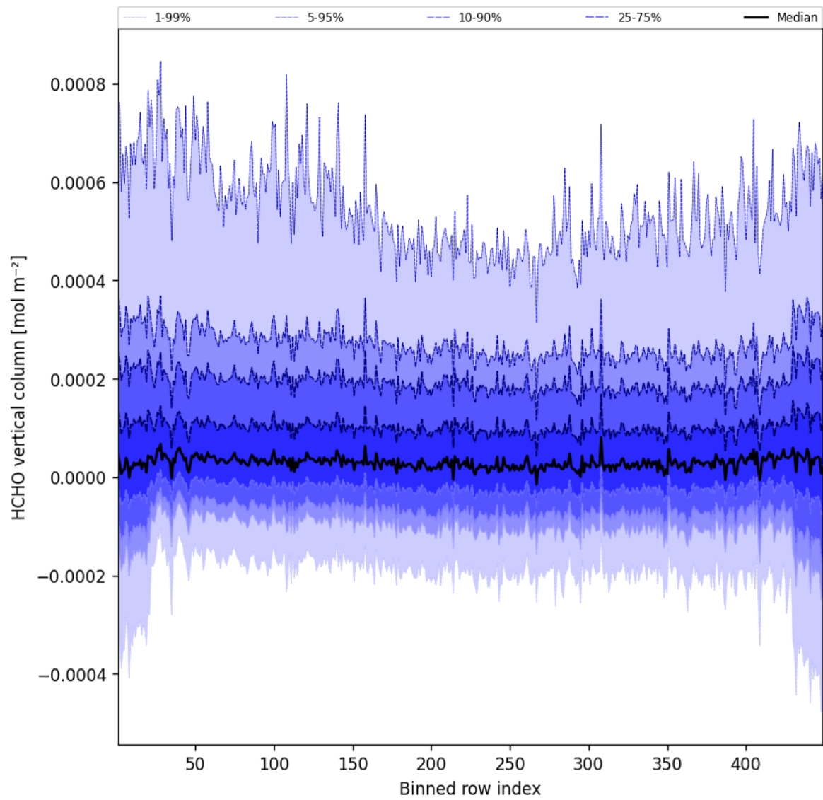
Figure 47: Along track statistics of “HCHO vertical column” for 2025-03-11 to 2025-03-12
