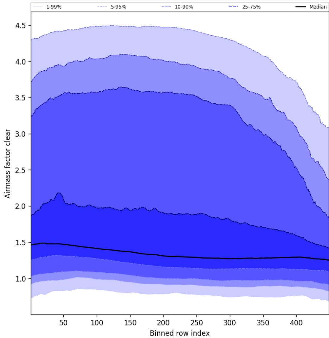
Figure 54: Along track statistics of “Airmass factor clear” for 2025-03-11 to 2025-03-12
