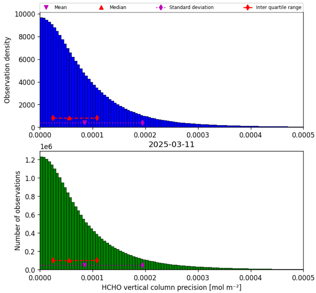
Figure 34: Histogram of “HCHO vertical column precision” for 2025-03-11 to 2025-03-12
