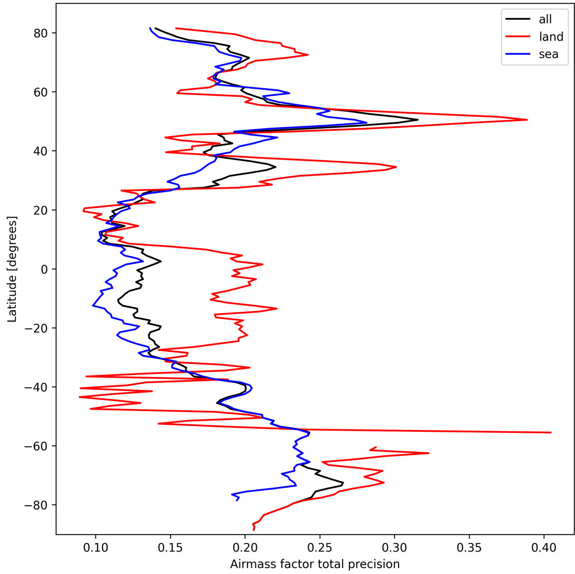
Figure 25: Zonal average of “Airmass factor total precision” for 2025-03-11 to 2025-03-12.
