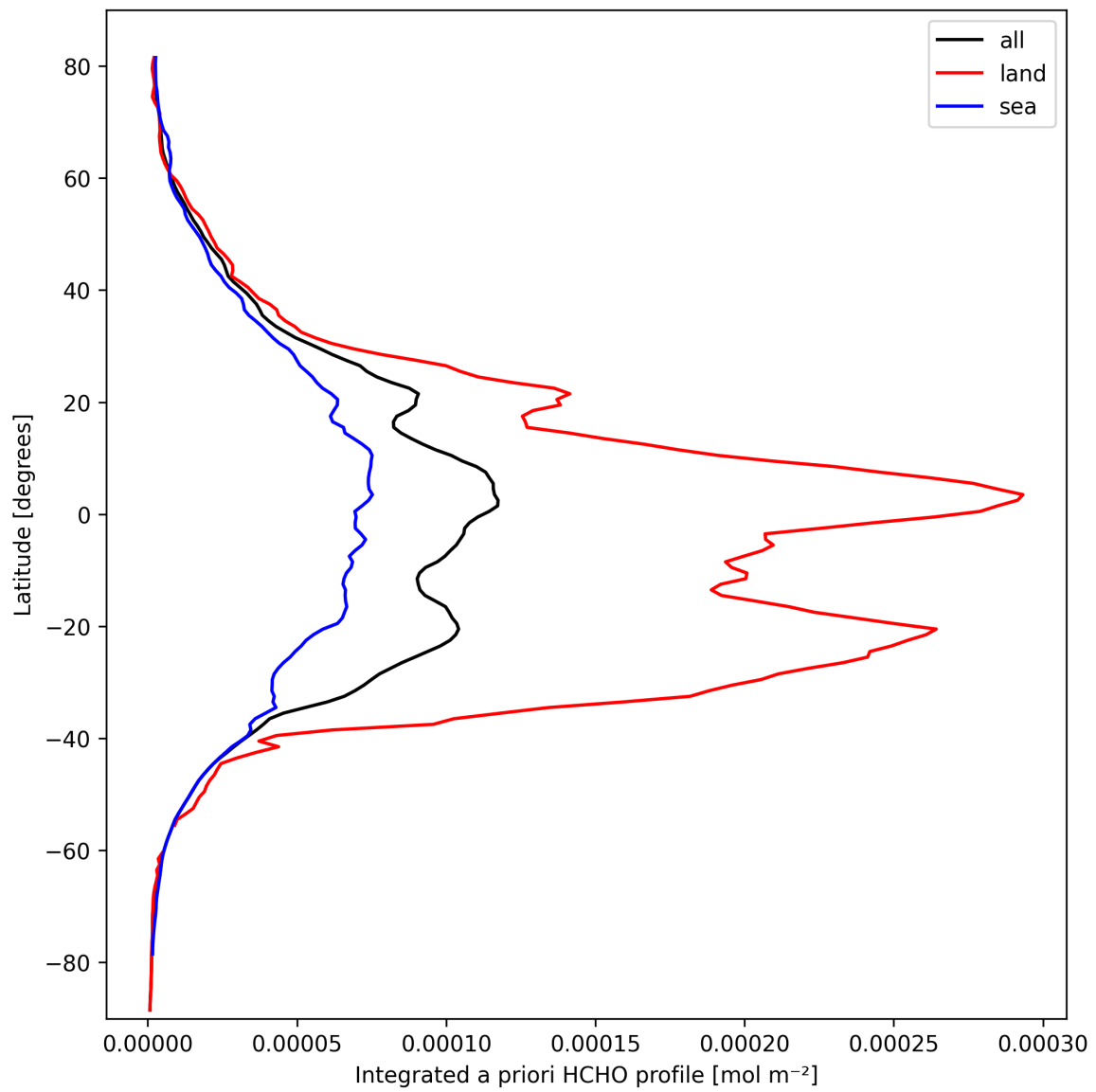
Figure 27: Zonal average of “Integrated a priori HCHO profile” for 2025-03-11 to 2025-03-12.
