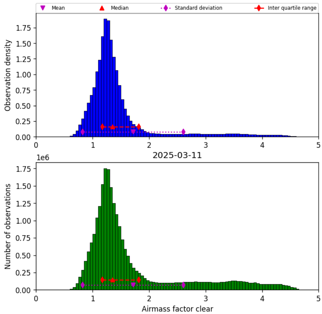
Figure 40: Histogram of “Airmass factor clear” for 2025-03-11 to 2025-03-12
