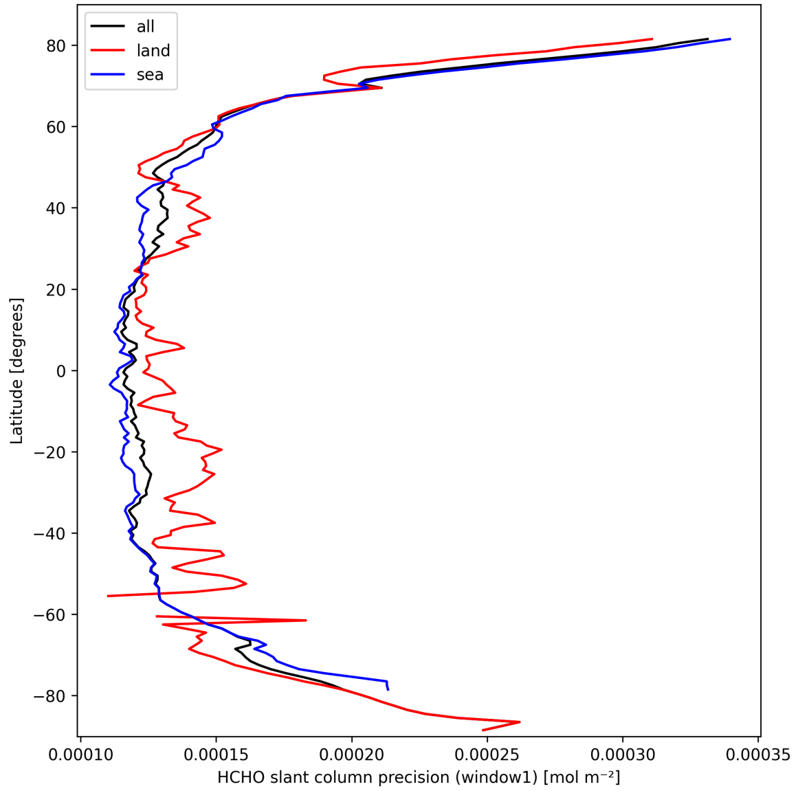
Figure 23: Zonal average of “HCHO slant column precision (window1)” for 2025-03-11 to 2025-03-12.
