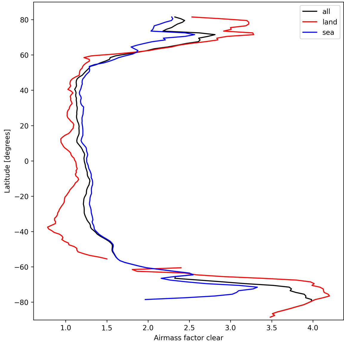
Figure 26: Zonal average of “Airmass factor clear” for 2025-03-11 to 2025-03-12.
