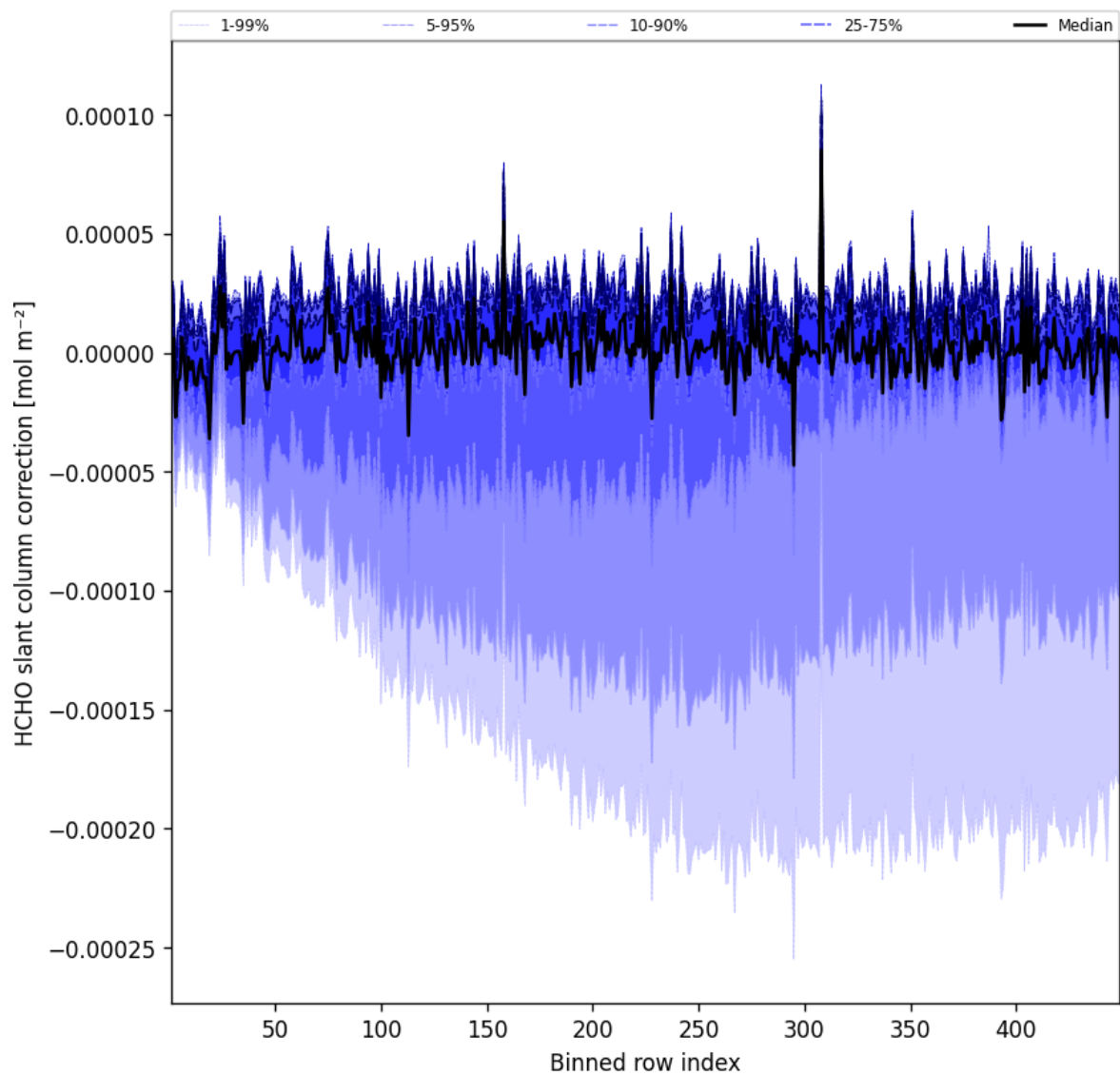
Figure 59: Along track statistics of “HCHO slant column correction” for 2025-03-11 to 2025-03-12
