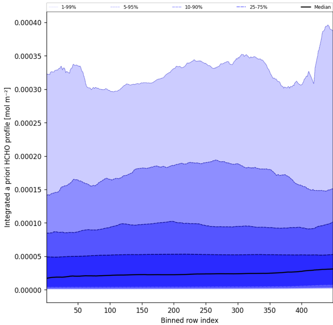
Figure 55: Along track statistics of “Integrated a priori HCHO profile” for 2025-03-11 to 2025-03-12
