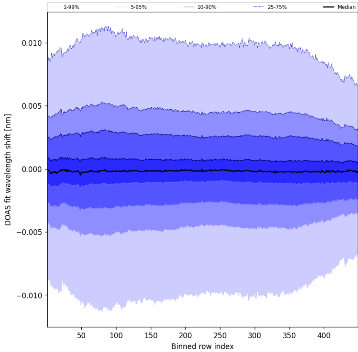
Figure 56: Along track statistics of “DOAS fit wavelength shift” for 2025-03-11 to 2025-03-12
