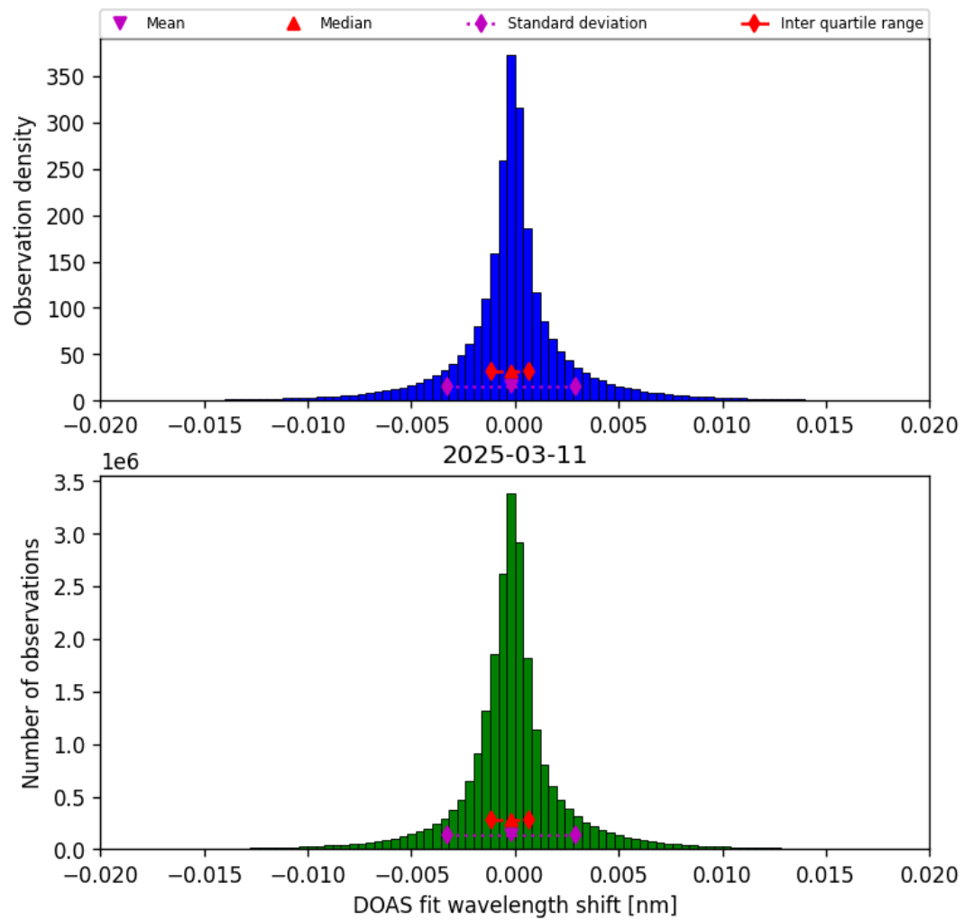
Figure 42: Histogram of “DOAS fit wavelength shift” for 2025-03-11 to 2025-03-12
