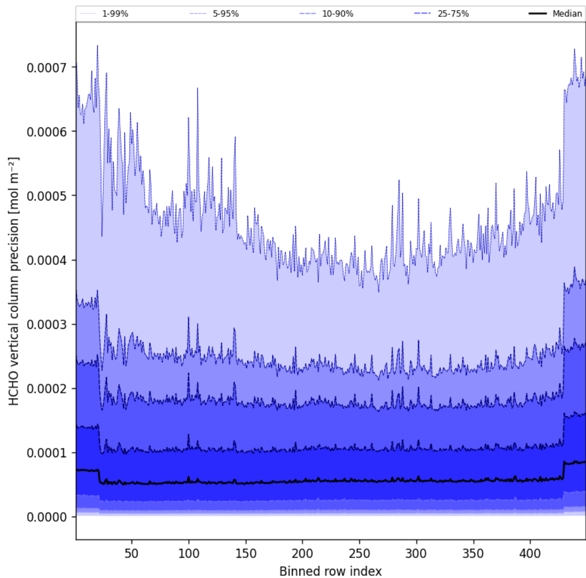
Figure 48: Along track statistics of “HCHO vertical column precision” for 2025-03-11 to 2025-03-12
