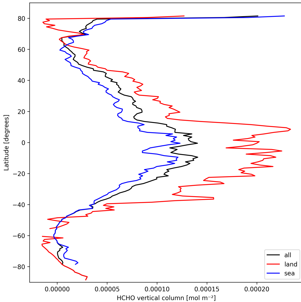
Figure 19: Zonal average of “HCHO vertical column” for 2025-03-11 to 2025-03-12.
