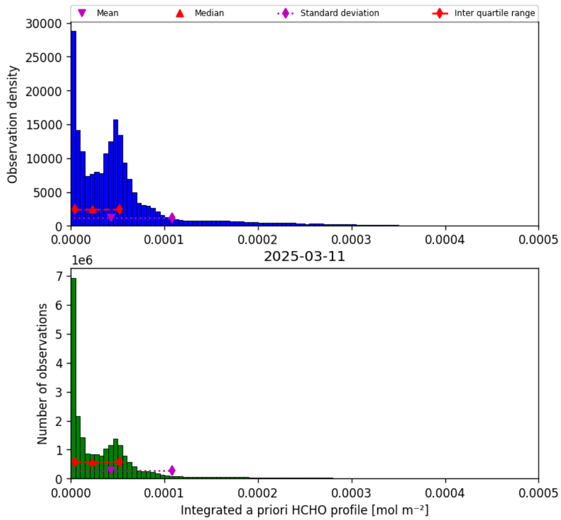
Figure 41: Histogram of “Integrated a priori HCHO profile” for 2025-03-11 to 2025-03-12
