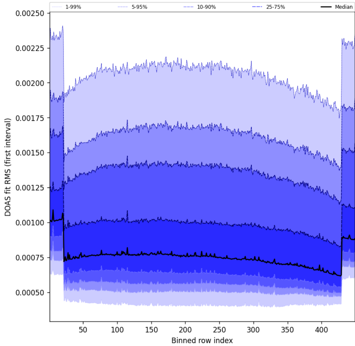
Figure 58: Along track statistics of “DOAS fit RMS (first interval)” for 2025-03-11 to 2025-03-12
