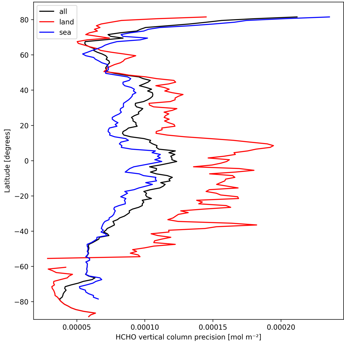
Figure 20: Zonal average of “HCHO vertical column precision” for 2025-03-11 to 2025-03-12.
