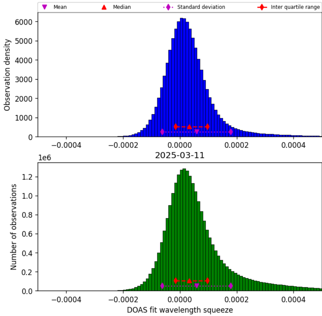
Figure 43: Histogram of “DOAS fit wavelength squeeze” for 2025-03-11 to 2025-03-12
