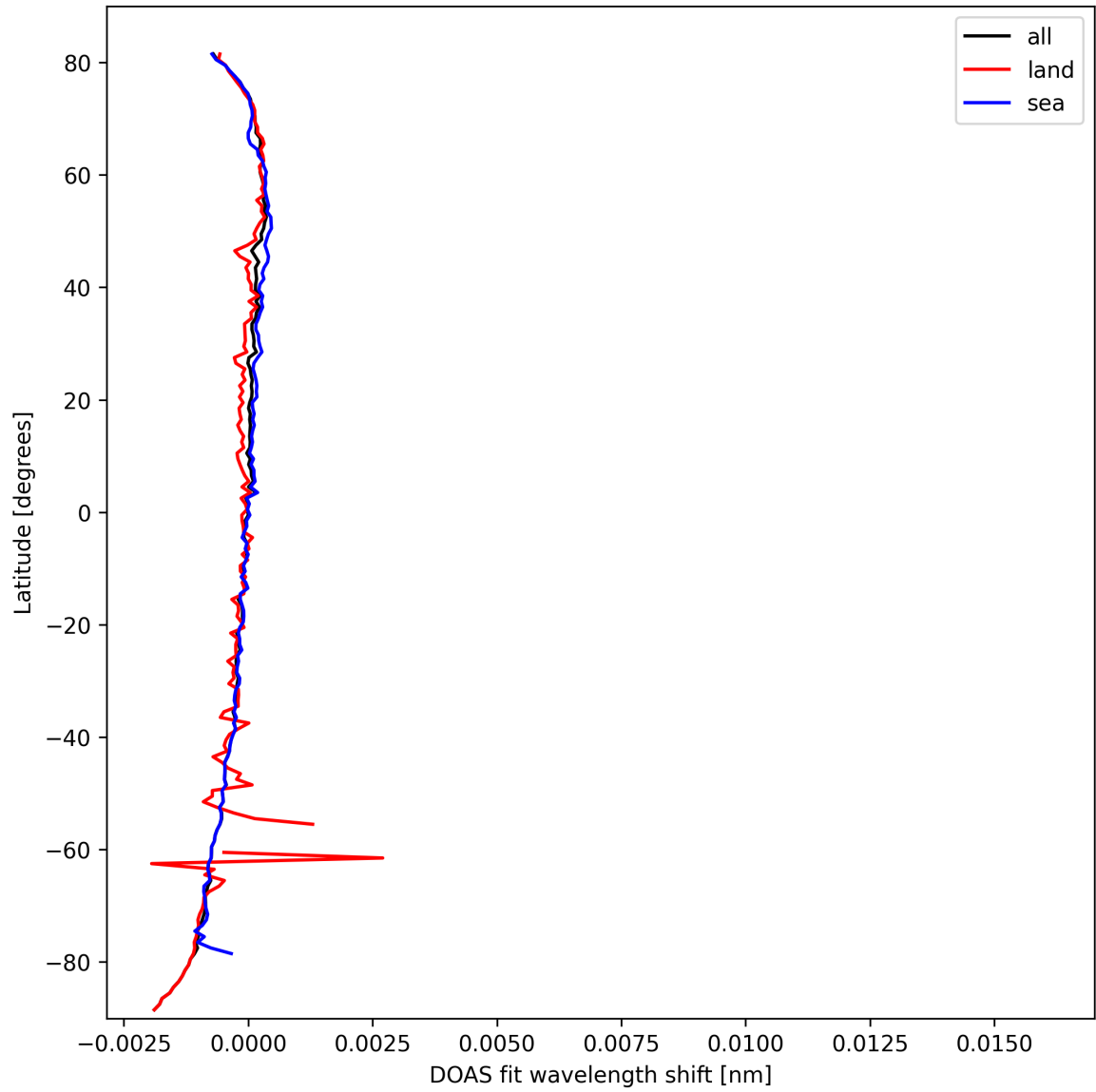
Figure 28: Zonal average of "DOAS fit wavelength shift" for 2025-03-11 to 2025-03-12.
