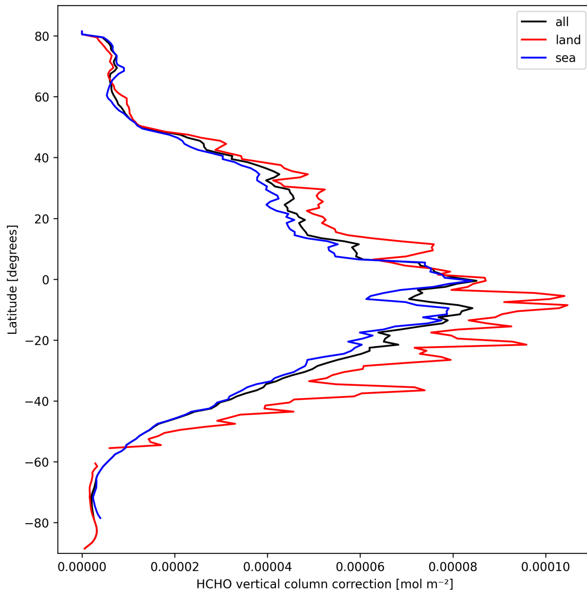
Figure 21: Zonal average of “HCHO vertical column correction” for 2025-03-11 to 2025-03-12.
