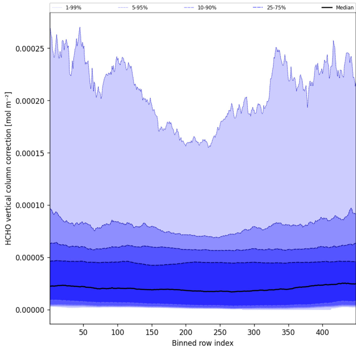
Figure 49: Along track statistics of “HCHO vertical column correction” for 2025-03-11 to 2025-03-12
