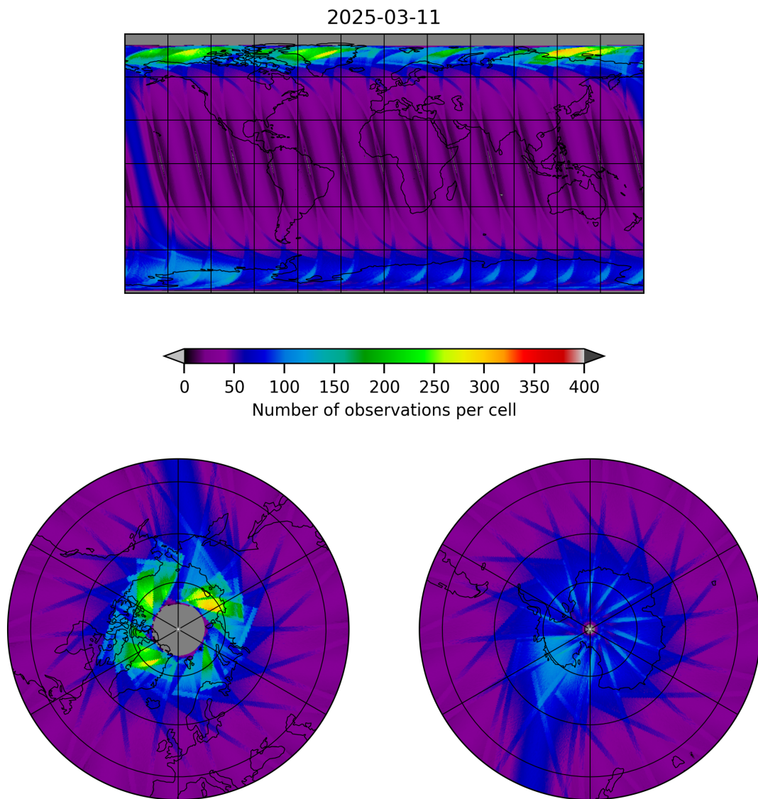
Figure 17: Map of the number of observations for 2025-03-11 to 2025-03-12
