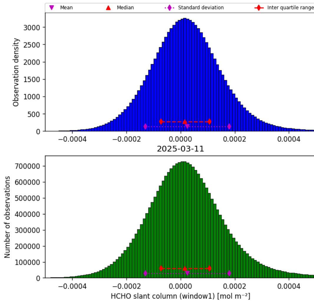
Figure 36: Histogram of “HCHO slant column (window1)” for 2025-03-11 to 2025-03-12
