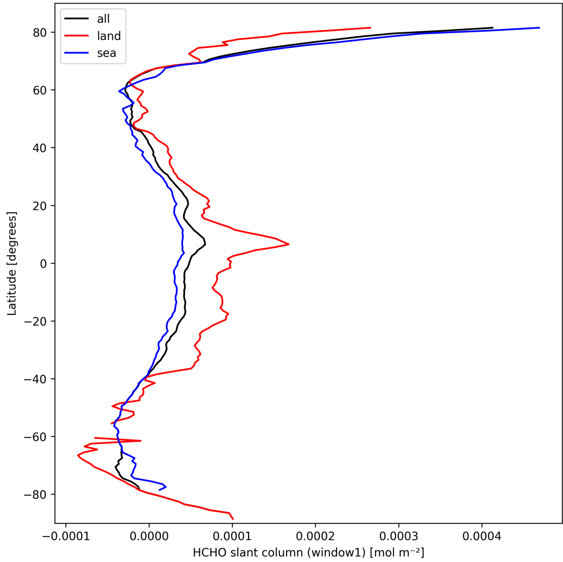
Figure 22: Zonal average of “HCHO slant column (window1)” for 2025-03-11 to 2025-03-12.
