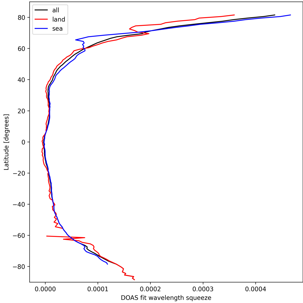
Figure 29: Zonal average of “DOAS fit wavelength squeeze” for 2025-03-11 to 2025-03-12.
