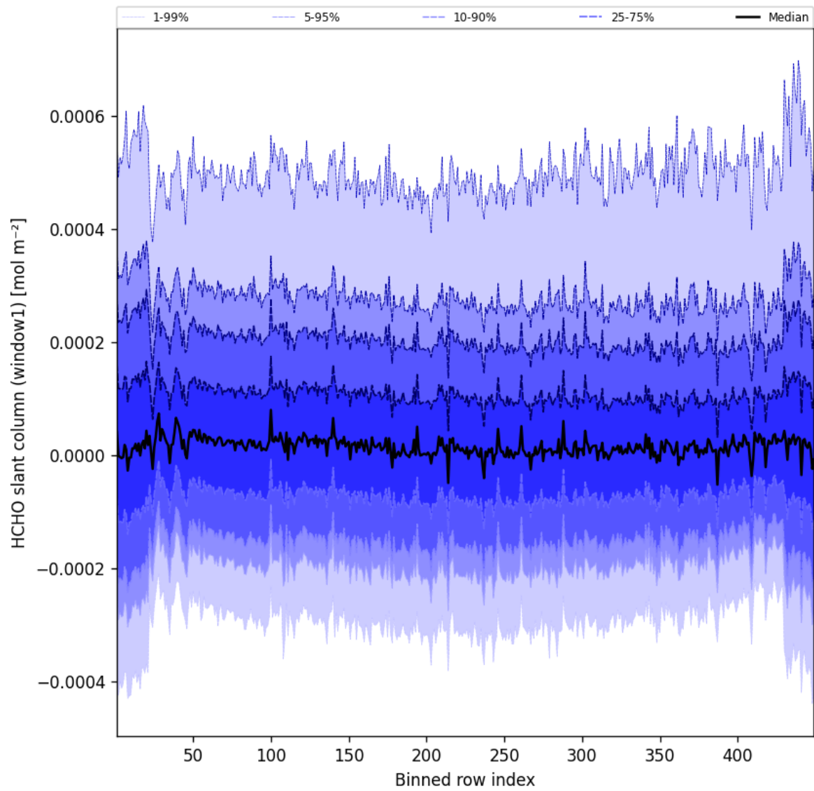
Figure 50: Along track statistics of “HCHO slant column (window1)” for 2025-03-11 to 2025-03-12
