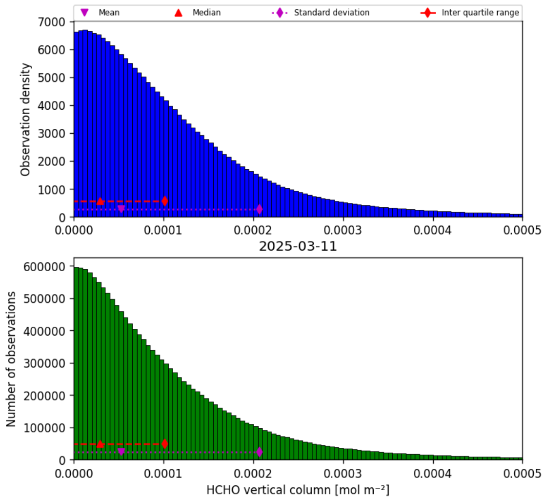
Figure 33: Histogram of “HCHO vertical column” for 2025-03-11 to 2025-03-12
