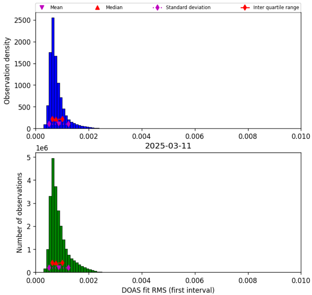
Figure 44: Histogram of "DOAS fit RMS (first interval)" for 2025-03-11 to 2025-03-12
