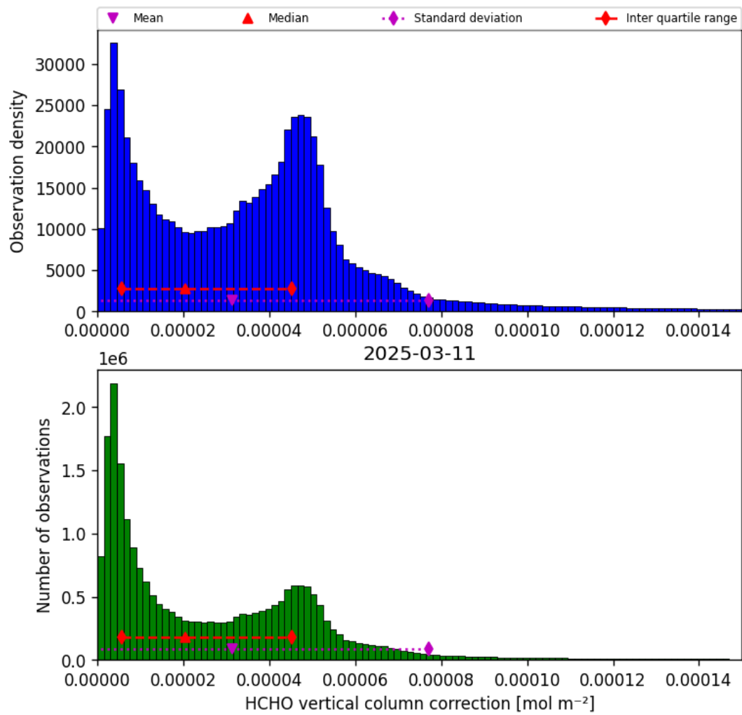
Figure 35: Histogram of “HCHO vertical column correction” for 2025-03-11 to 2025-03-12
