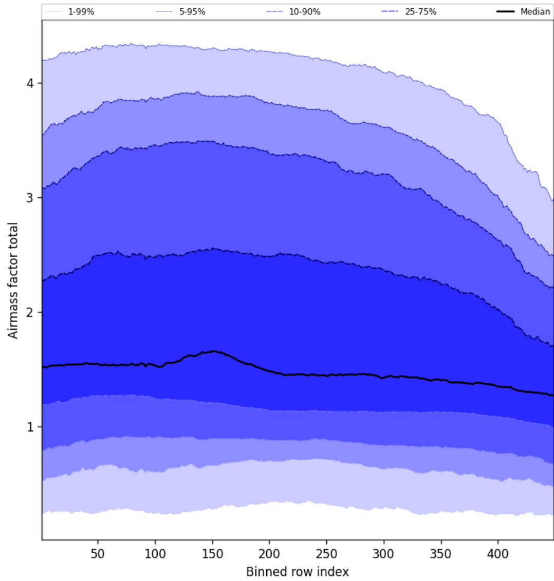
Figure 52: Along track statistics of “Airmass factor total” for 2025-03-11 to 2025-03-12
