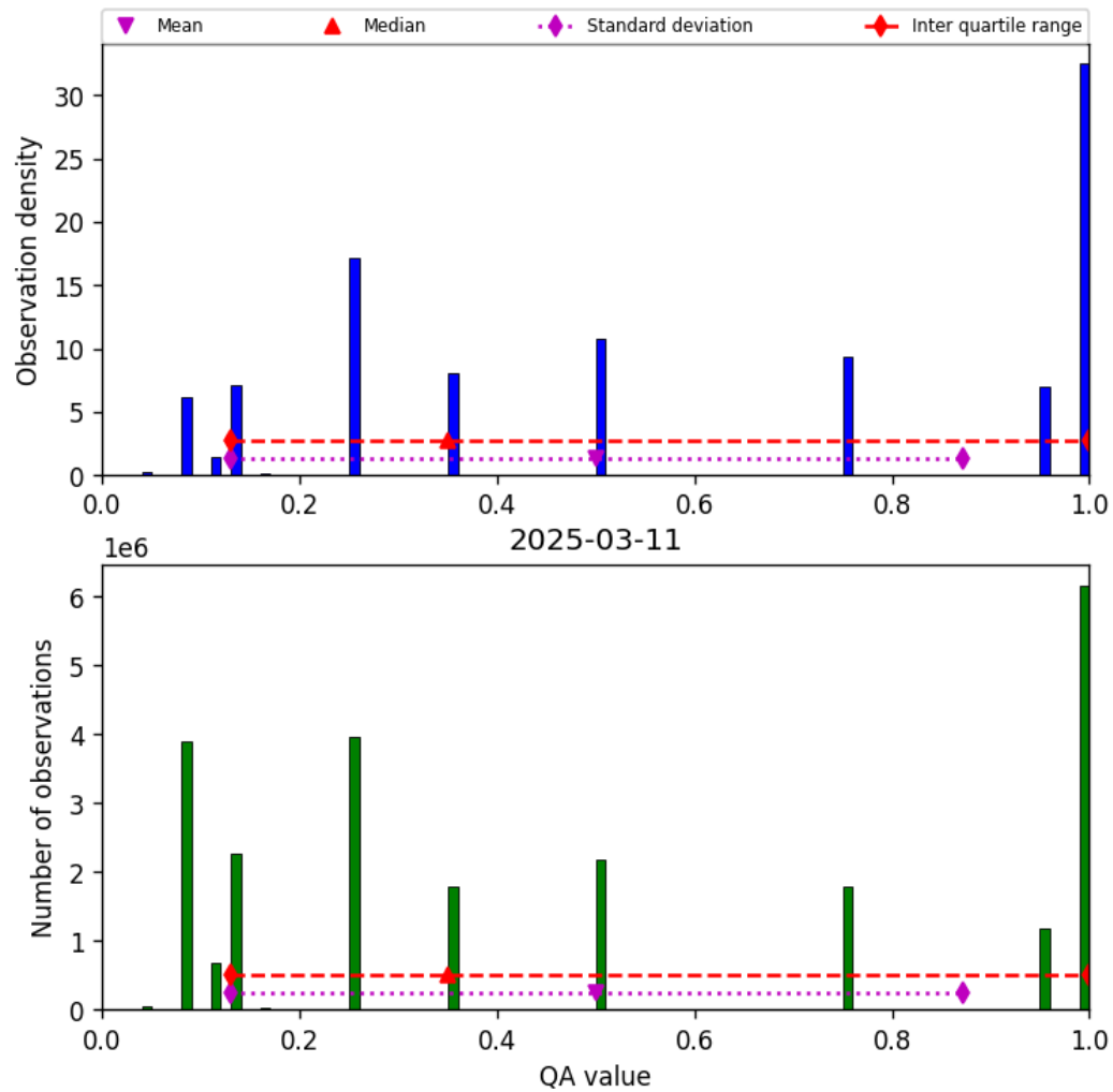
Figure 32: Histogram of “QA value” for 2025-03-11 to 2025-03-12
