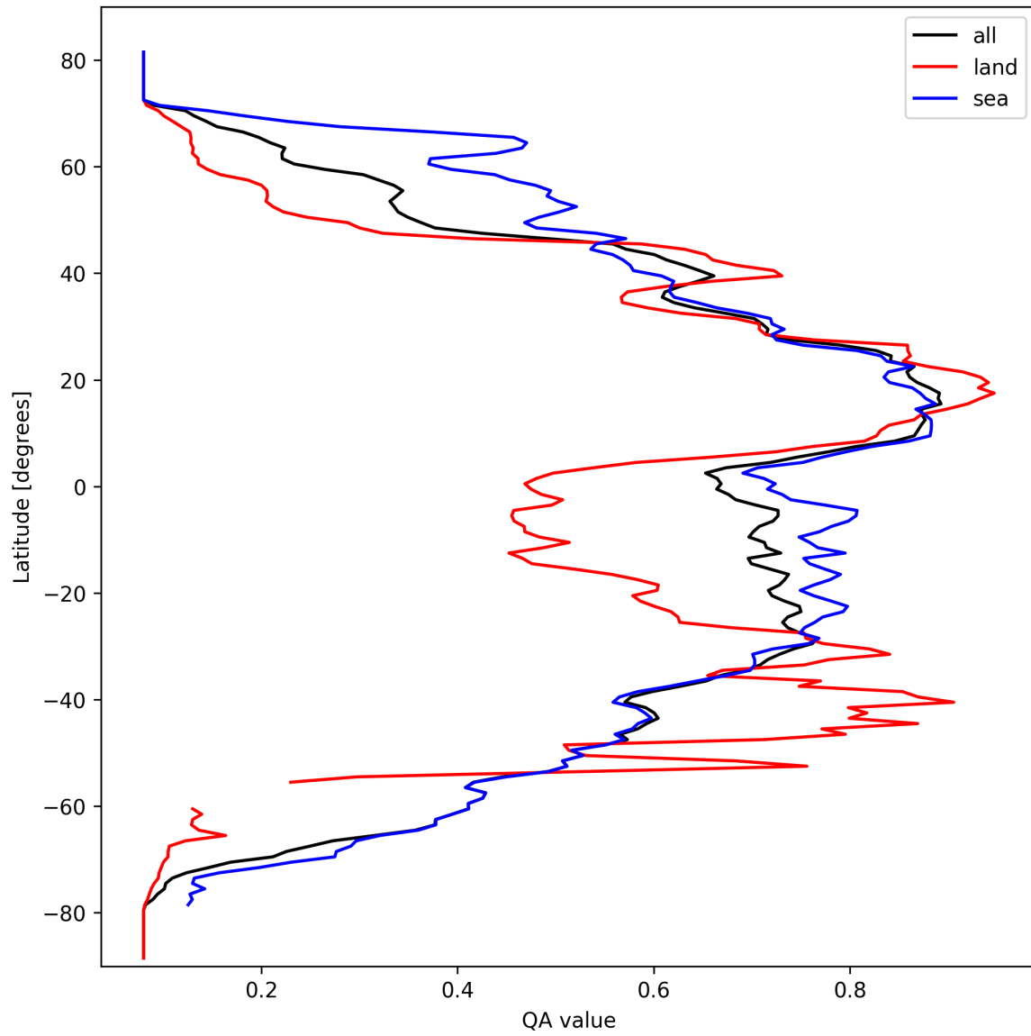
Figure 18: Zonal average of “QA value” for 2025-03-11 to 2025-03-12.
