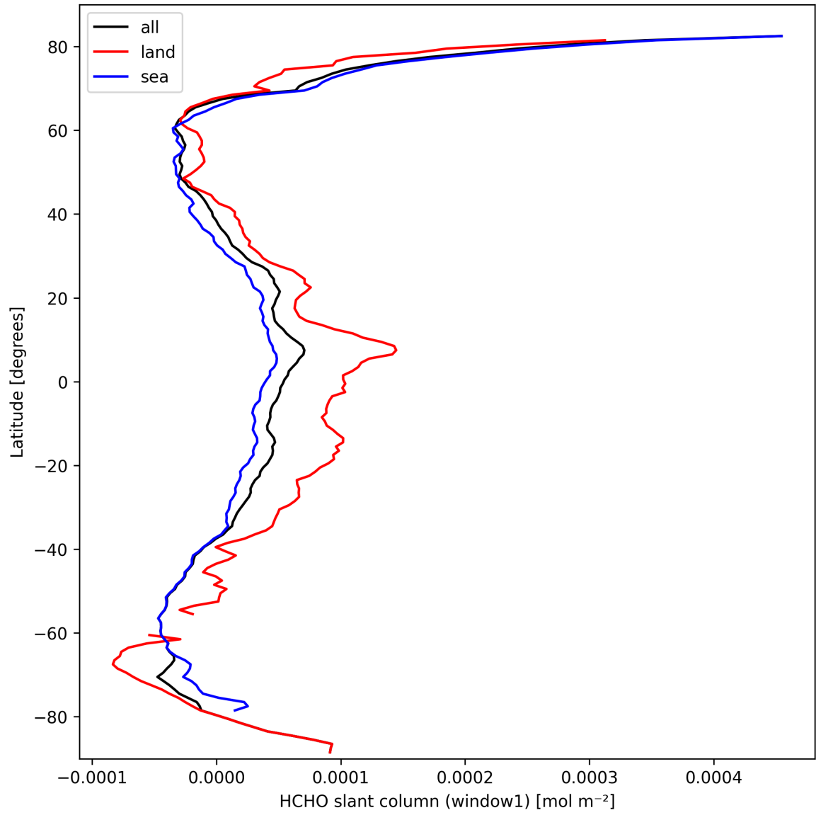
Figure 22: Zonal average of “HCHO slant column (window1)” for 2025-03-12 to 2025-03-13.
