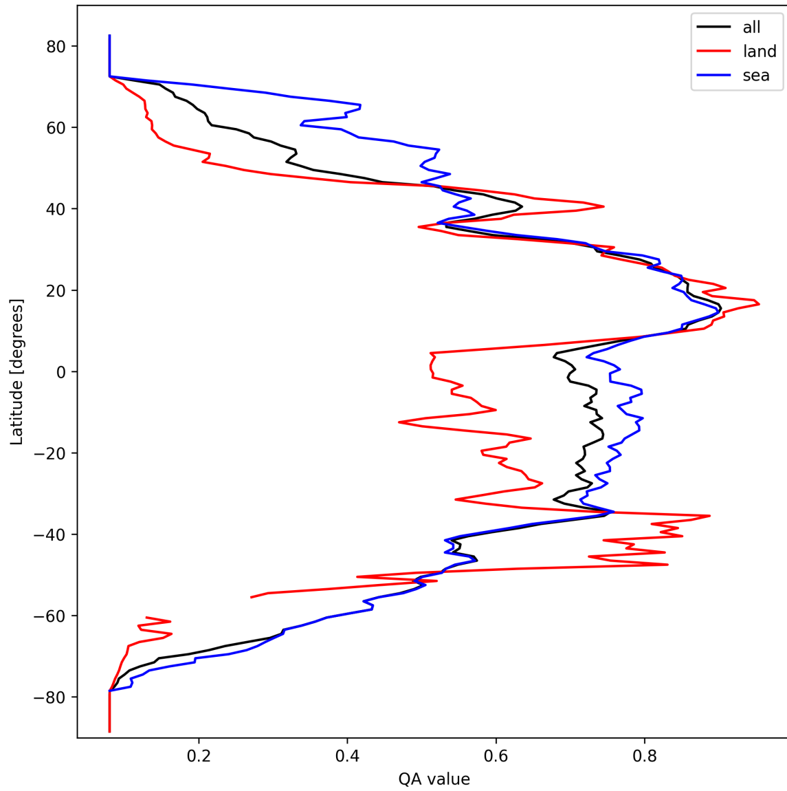
Figure 18: Zonal average of “QA value” for 2025-03-12 to 2025-03-13.
