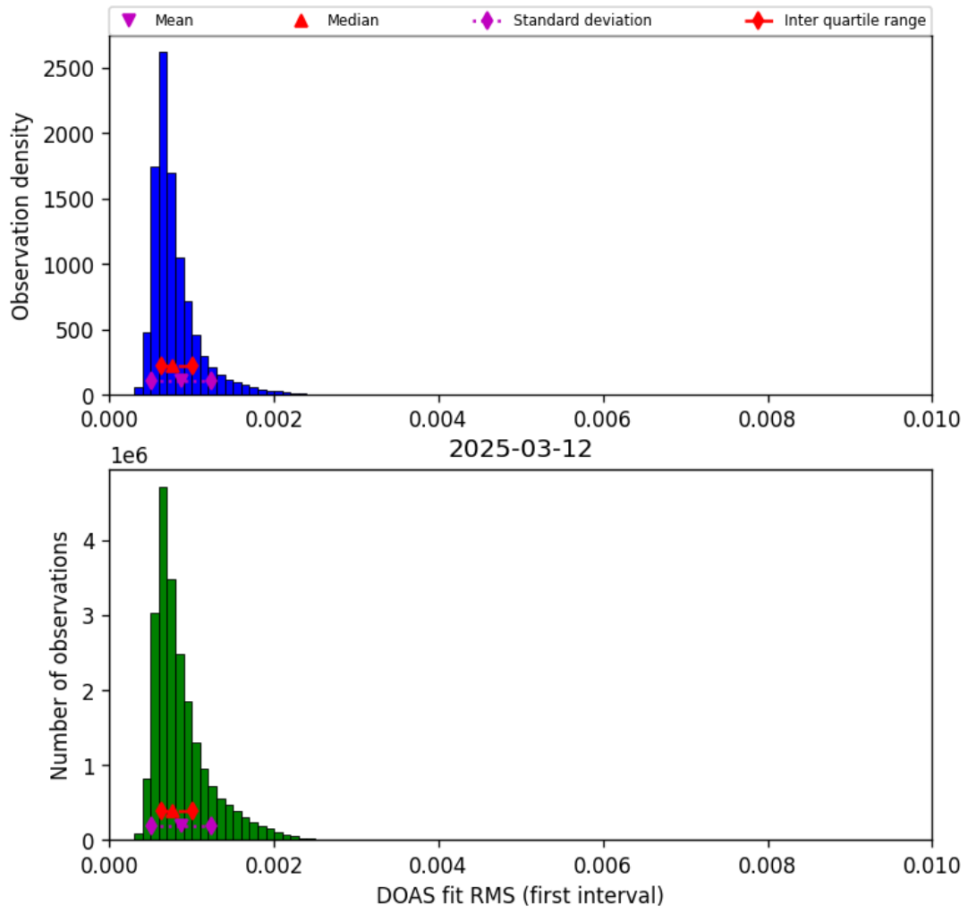
Figure 44: Histogram of “DOAS fit RMS (first interval)” for 2025-03-12 to 2025-03-13
