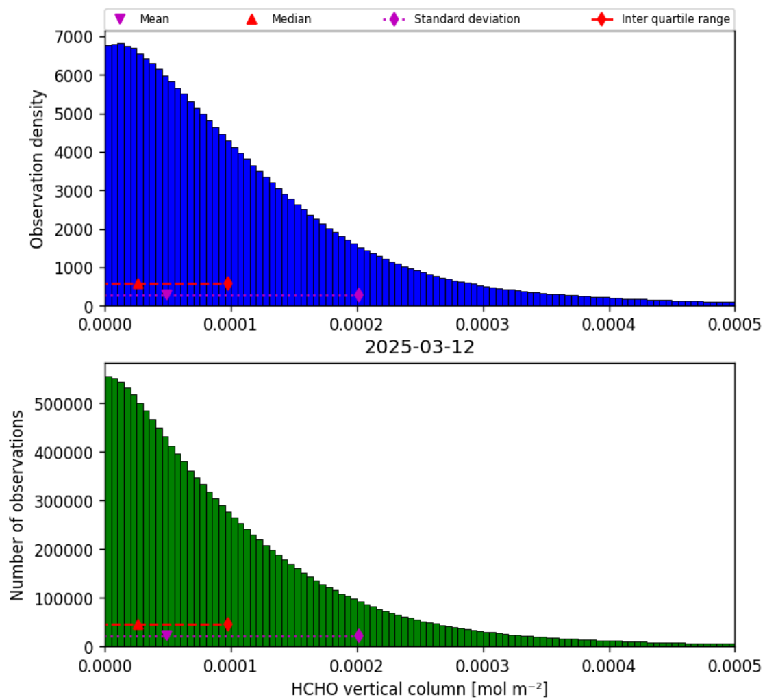
Figure 33: Histogram of “HCHO vertical column” for 2025-03-12 to 2025-03-13
