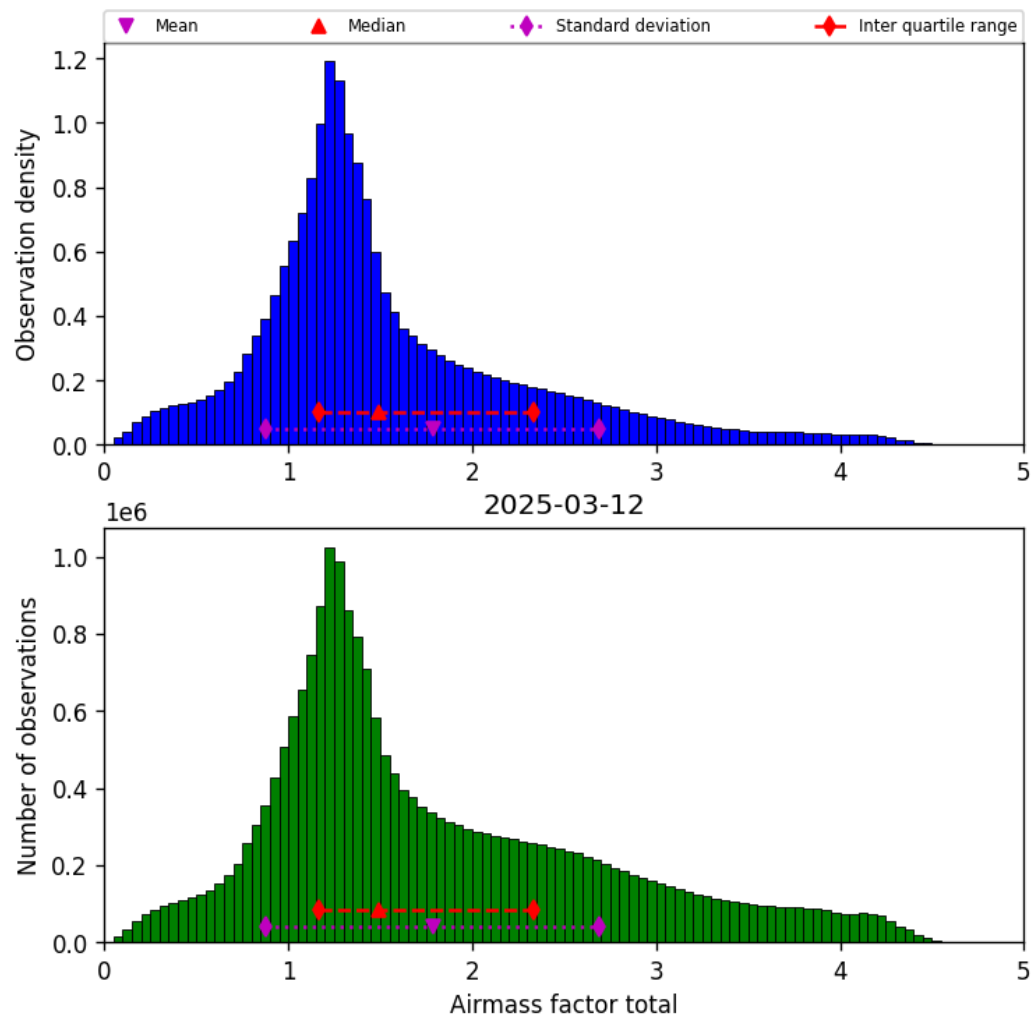
Figure 38: Histogram of “Airmass factor total” for 2025-03-12 to 2025-03-13
