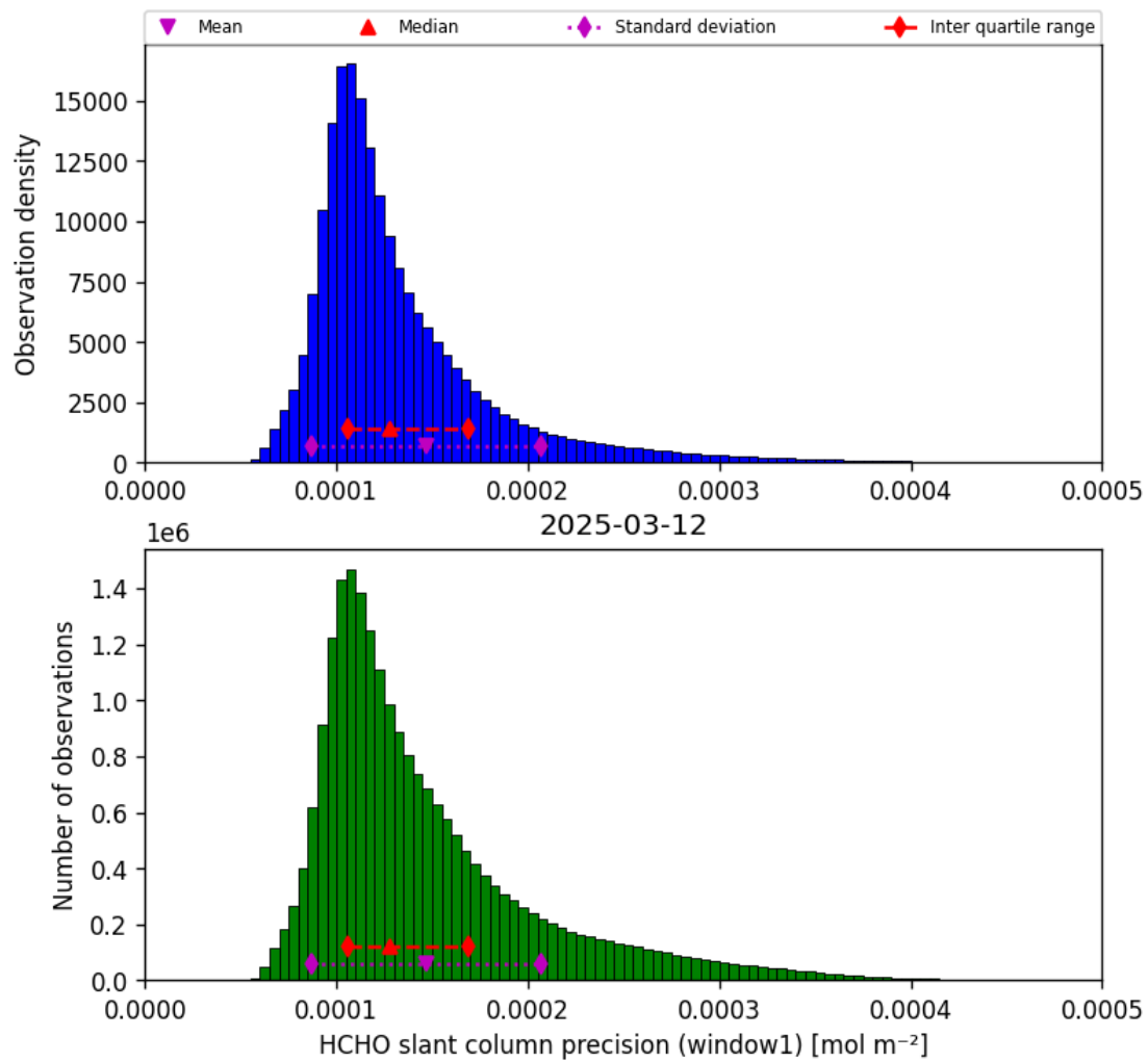
Figure 37: Histogram of “HCHO slant column precision (window1)” for 2025-03-12 to 2025-03-13
