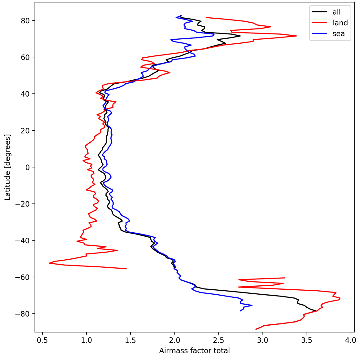
Figure 24: Zonal average of “Airmass factor total” for 2025-03-12 to 2025-03-13.
