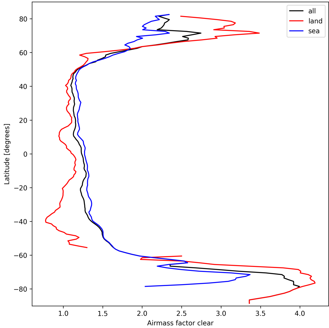
Figure 26: Zonal average of “Airmass factor clear” for 2025-03-12 to 2025-03-13.
