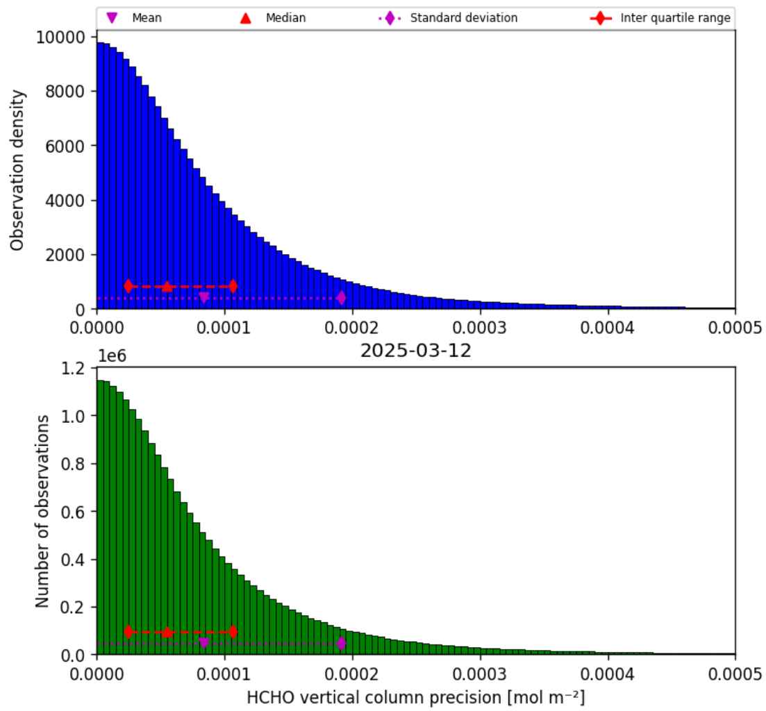
Figure 34: Histogram of “HCHO vertical column precision” for 2025-03-12 to 2025-03-13
