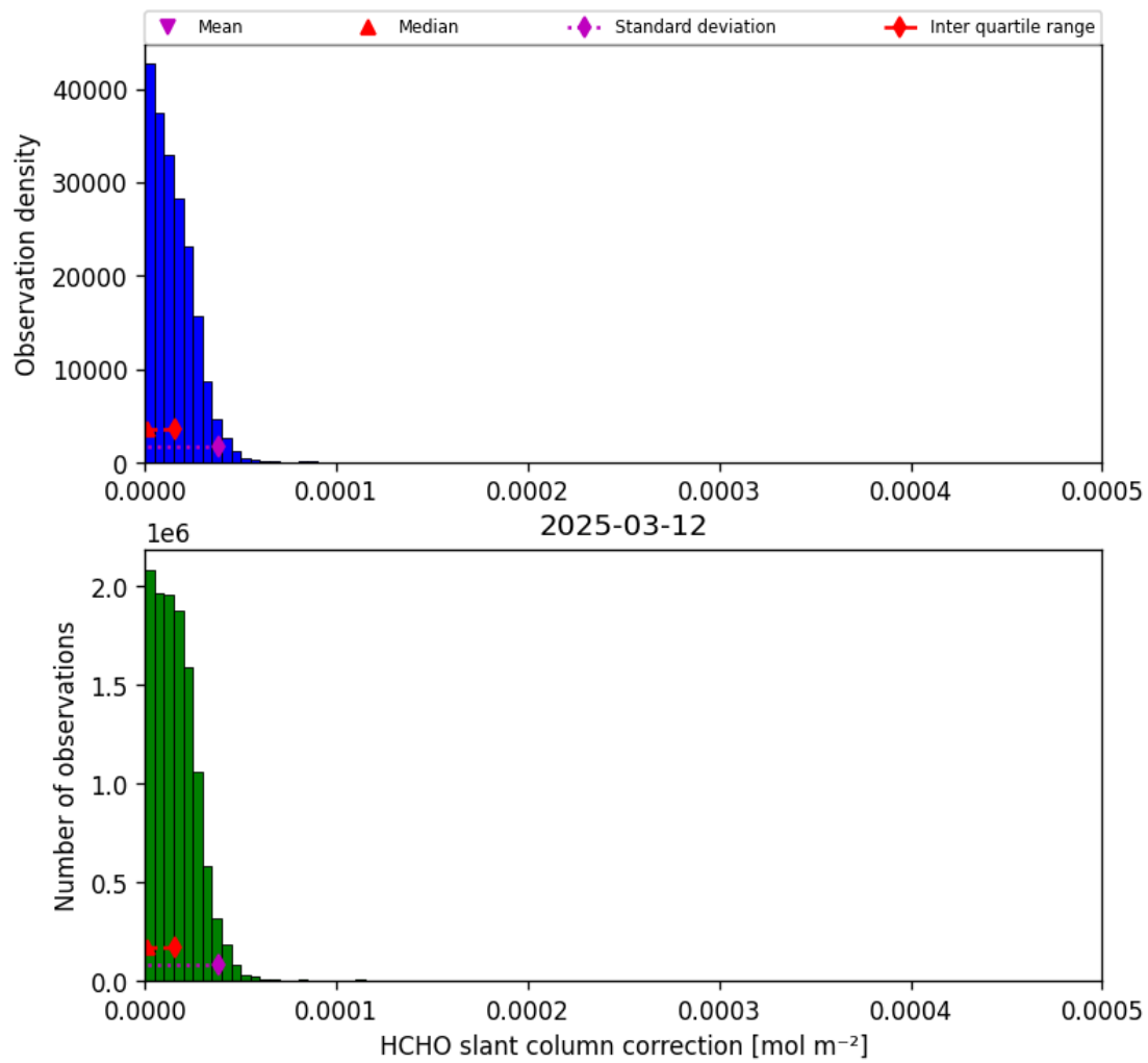
Figure 45: Histogram of “HCHO slant column correction” for 2025-03-12 to 2025-03-13
