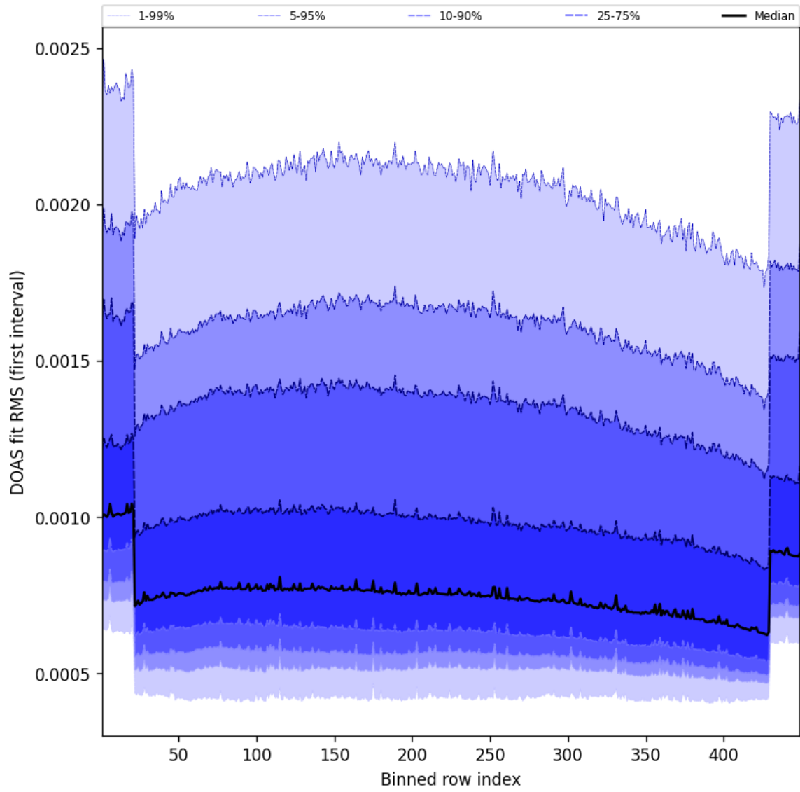
Figure 58: Along track statistics of “DOAS fit RMS (first interval)” for 2025-03-12 to 2025-03-13
