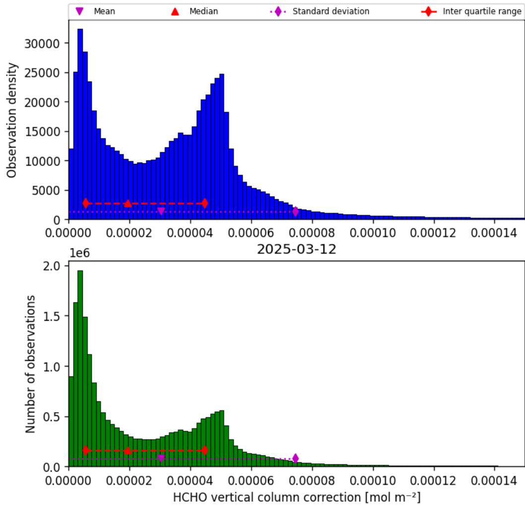
Figure 35: Histogram of “HCHO vertical column correction” for 2025-03-12 to 2025-03-13
