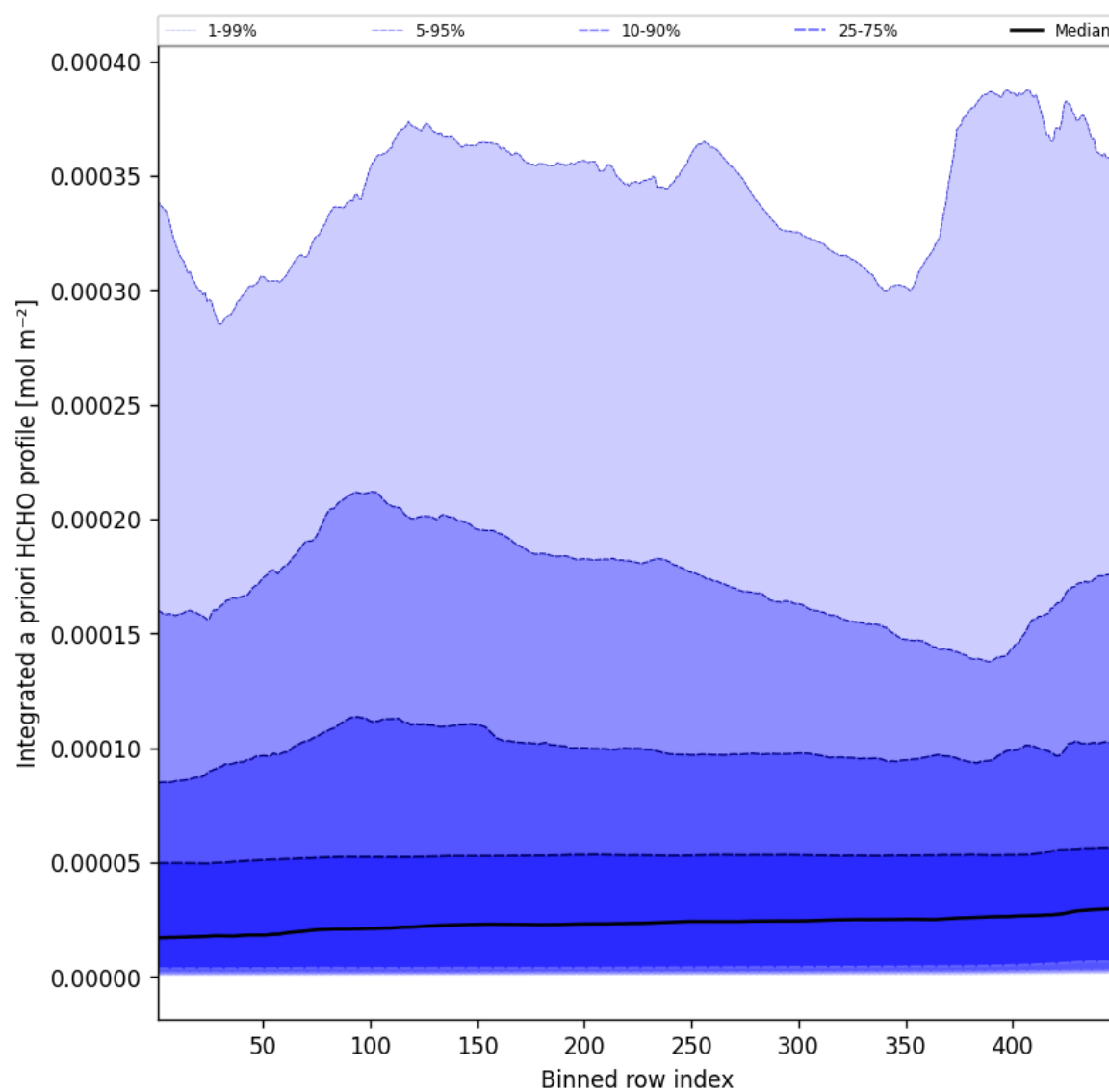
Figure 55: Along track statistics of “Integrated a priori HCHO profile” for 2025-03-12 to 2025-03-13
