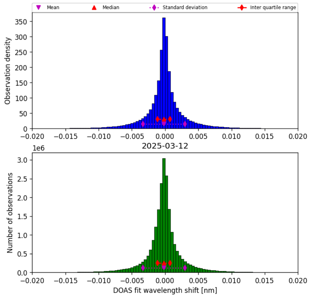
Figure 42: Histogram of “DOAS fit wavelength shift” for 2025-03-12 to 2025-03-13
