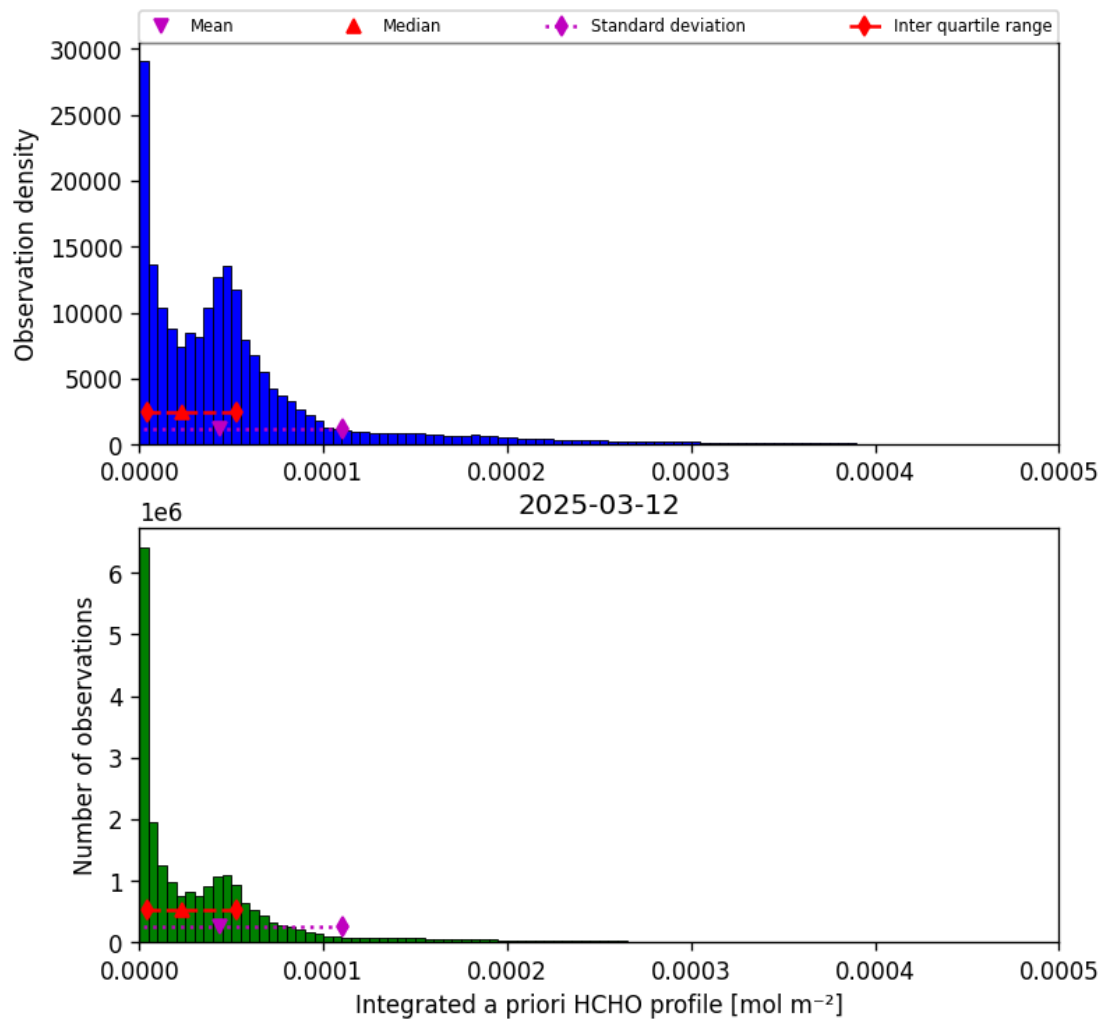
Figure 41: Histogram of “Integrated a priori HCHO profile” for 2025-03-12 to 2025-03-13
