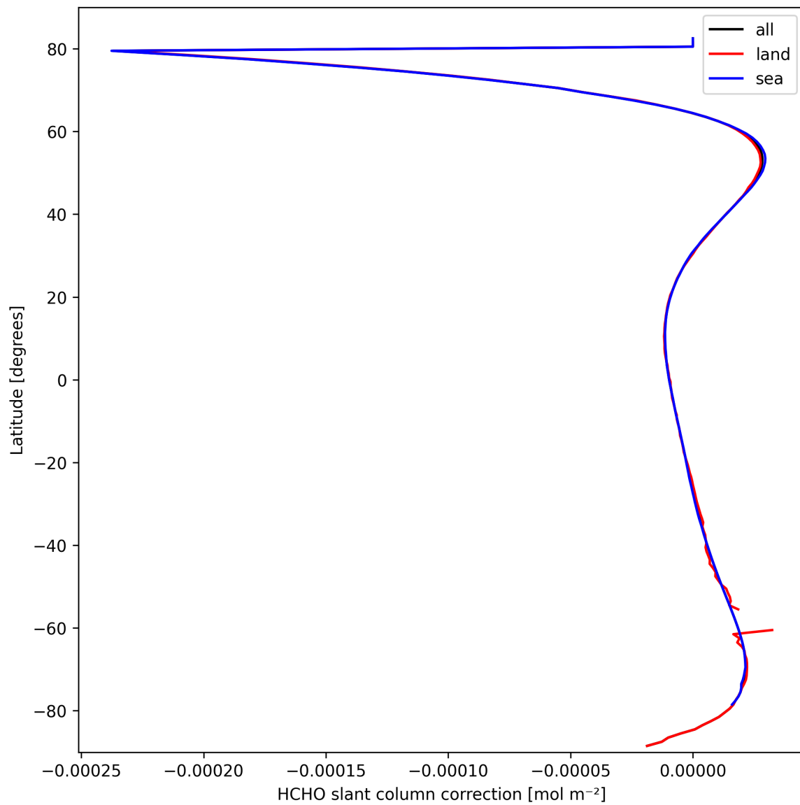
Figure 31: Zonal average of “HCHO slant column correction” for 2025-03-12 to 2025-03-13.
