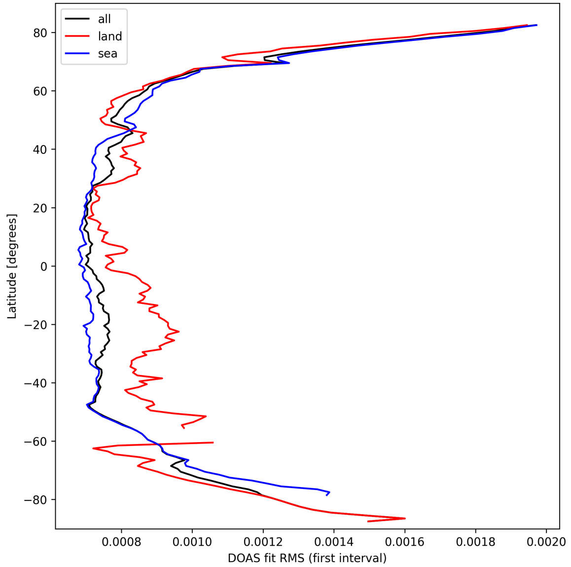
Figure 30: Zonal average of “DOAS fit RMS (first interval)” for 2025-03-13 to 2025-03-14.
