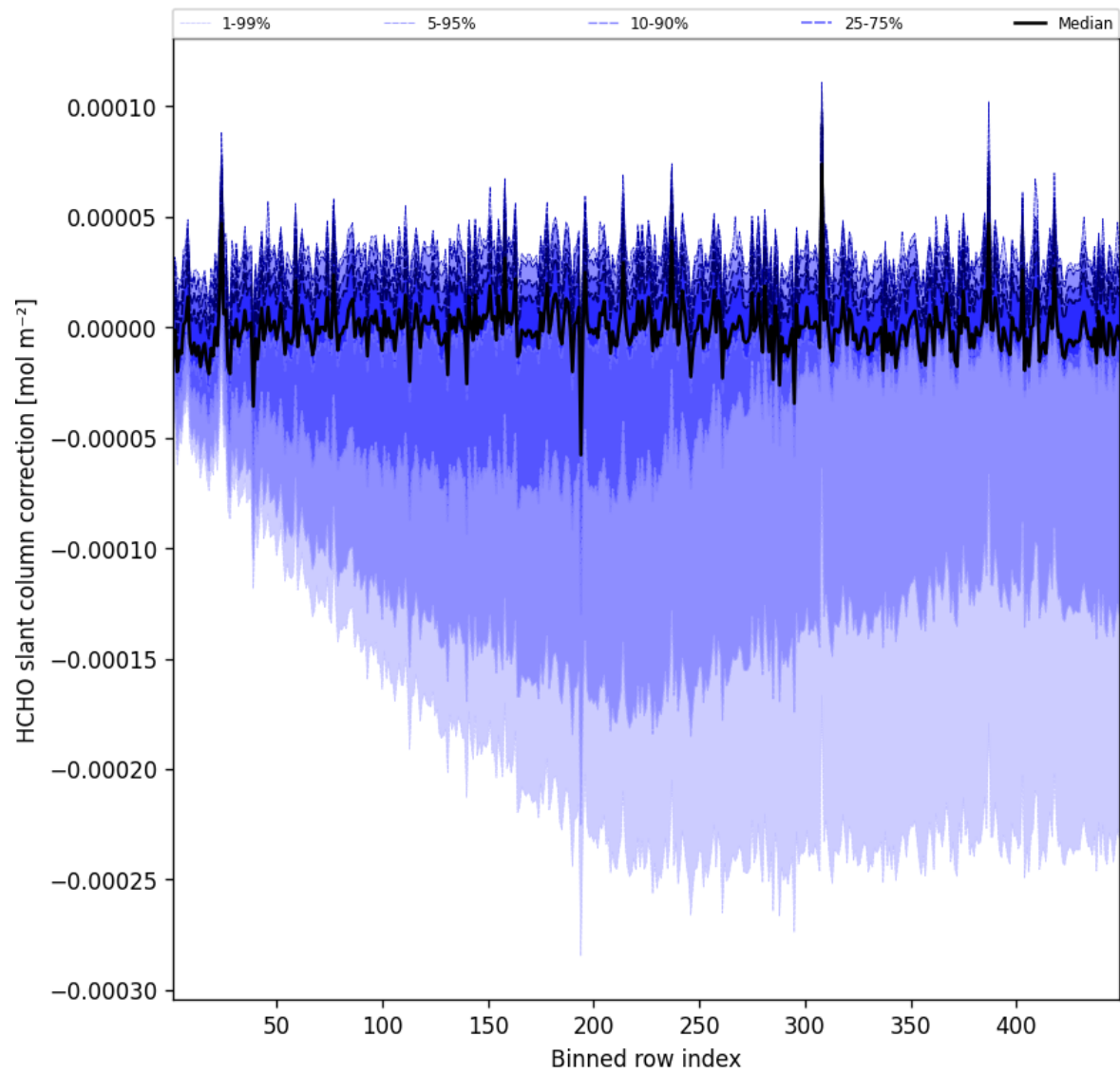
Figure 59: Along track statistics of “HCHO slant column correction” for 2025-03-13 to 2025-03-14
