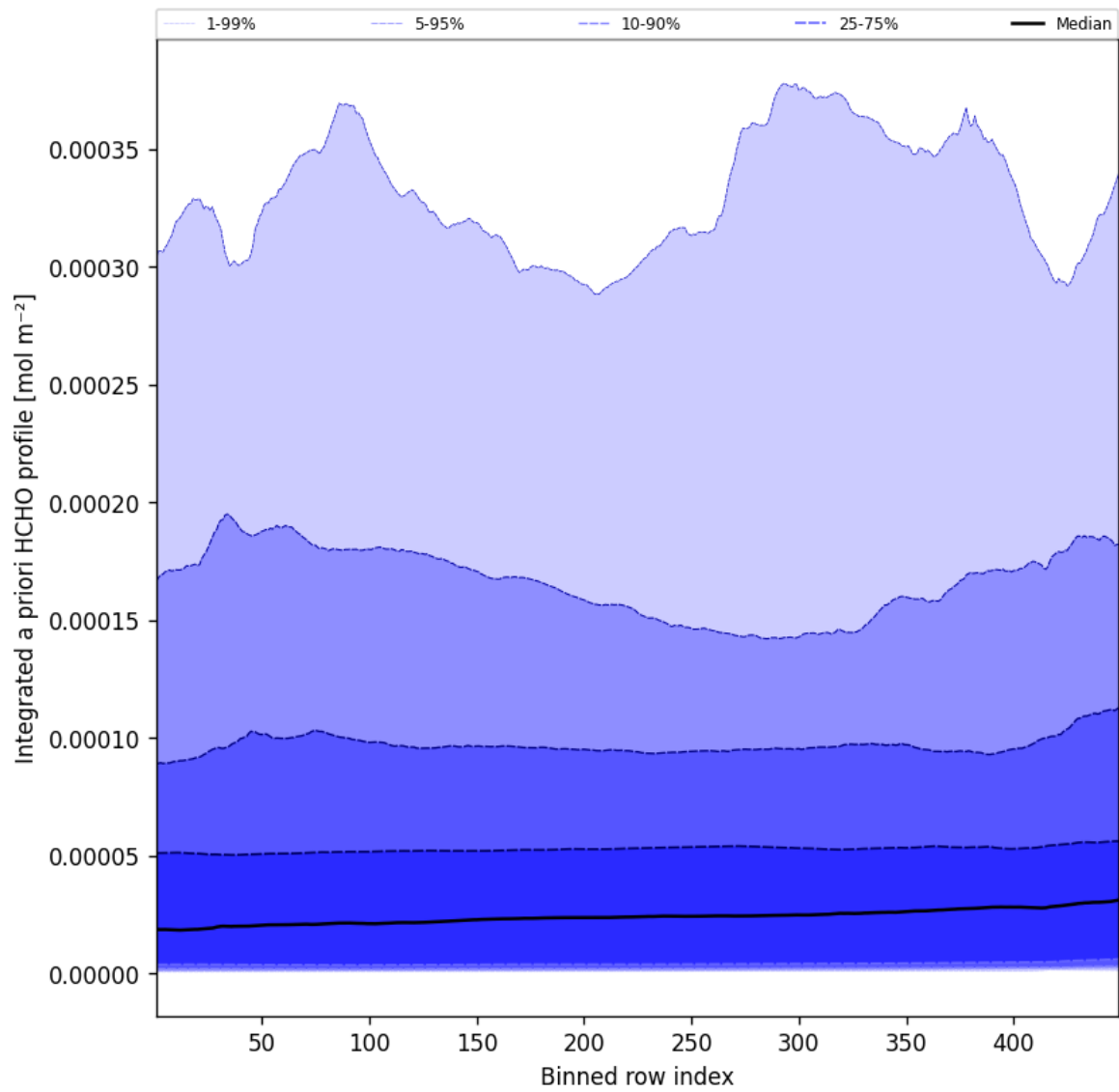
Figure 55: Along track statistics of "Integrated a priori HCHO profile" for 2025-03-13 to 2025-03-14
