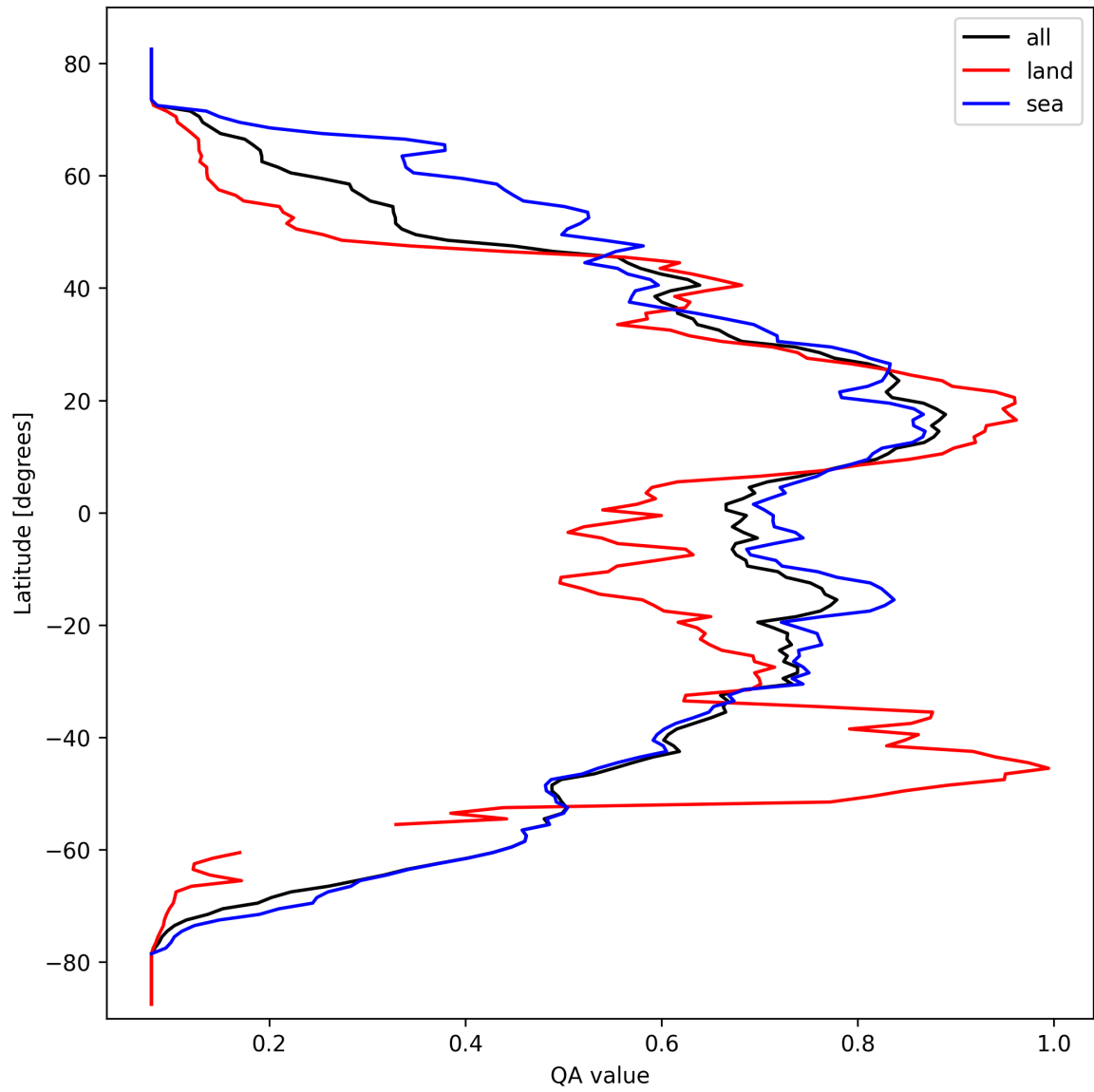
Figure 18: Zonal average of “QA value” for 2025-03-13 to 2025-03-14.
