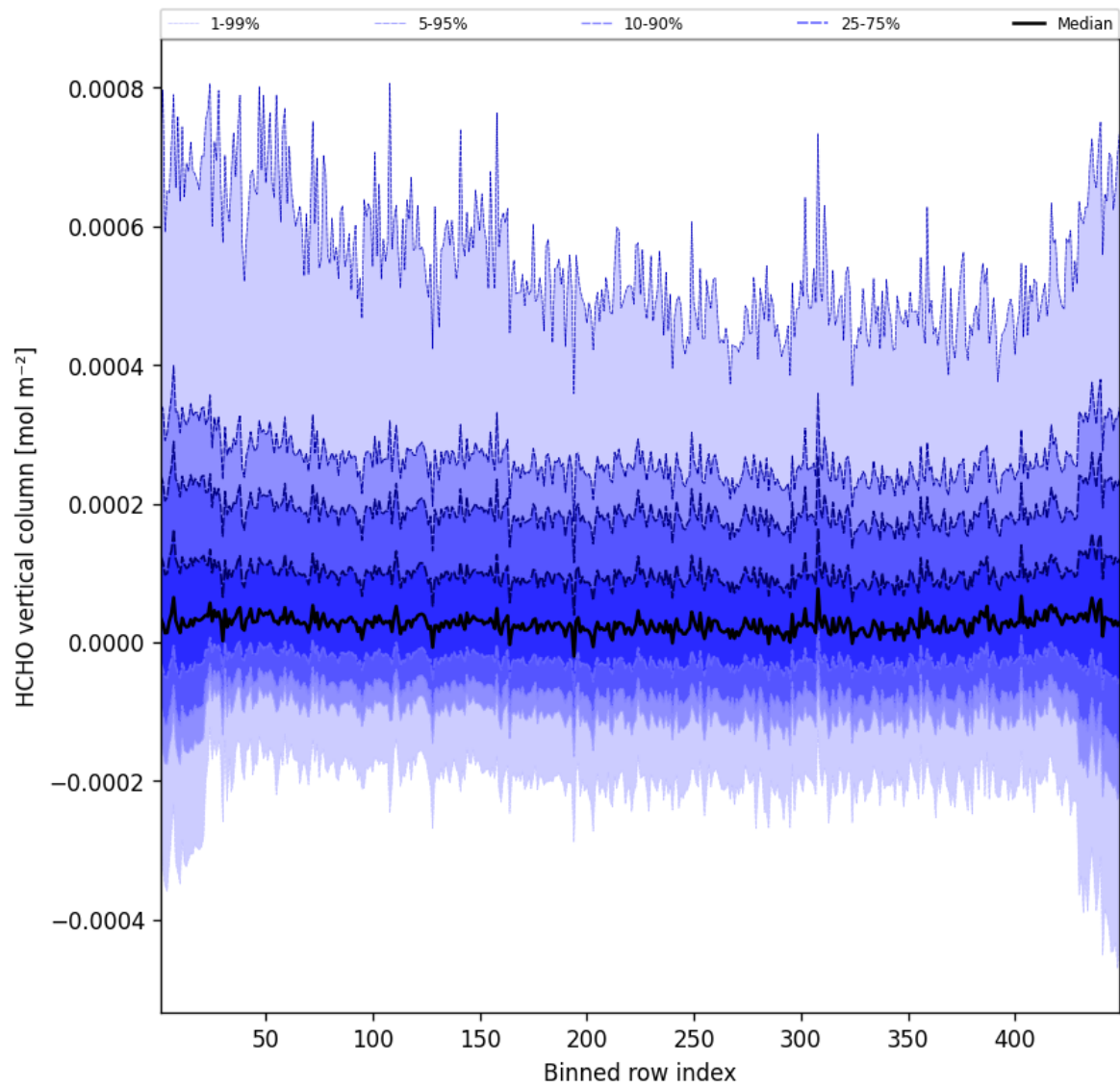
Figure 47: Along track statistics of “HCHO vertical column” for 2025-03-13 to 2025-03-14
