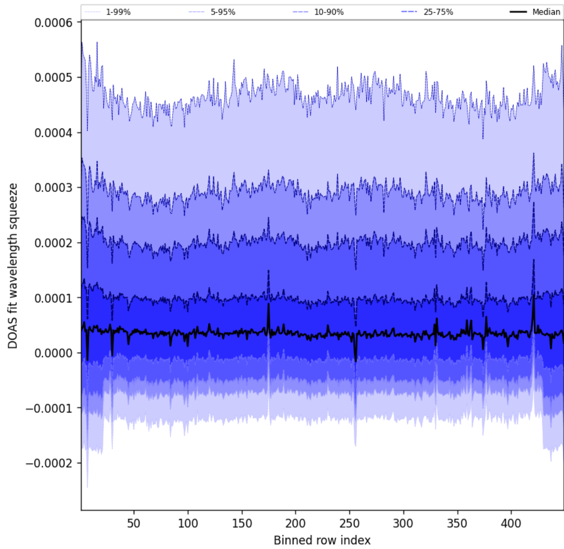
Figure 57: Along track statistics of “DOAS fit wavelength squeeze” for 2025-03-13 to 2025-03-14
