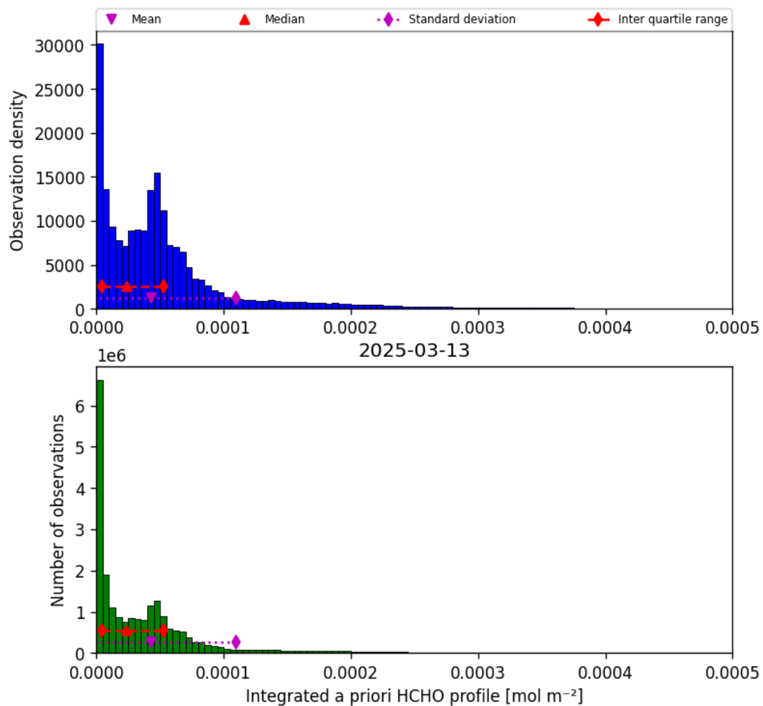
Figure 41: Histogram of “Integrated a priori HCHO profile” for 2025-03-13 to 2025-03-14
