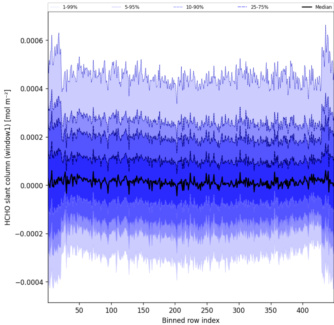
Figure 50: Along track statistics of “HCHO slant column (window1)” for 2025-03-13 to 2025-03-14
