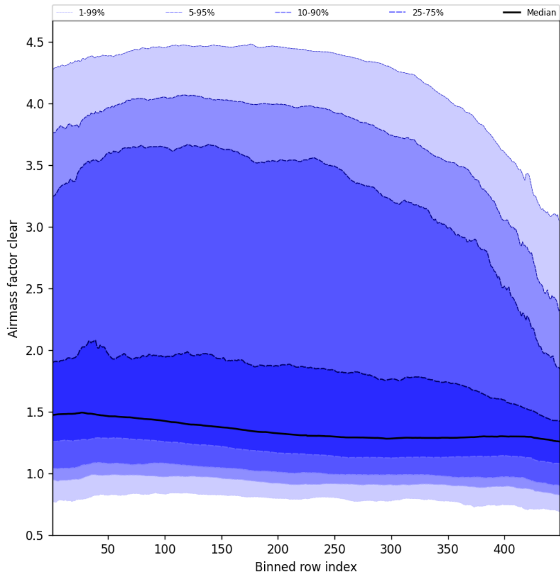
Figure 54: Along track statistics of “Airmass factor clear” for 2025-03-13 to 2025-03-14
