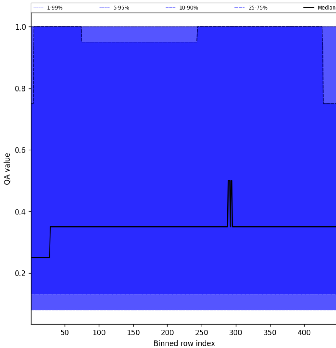
Figure 46: Along track statistics of “QA value” for 2025-03-13 to 2025-03-14
