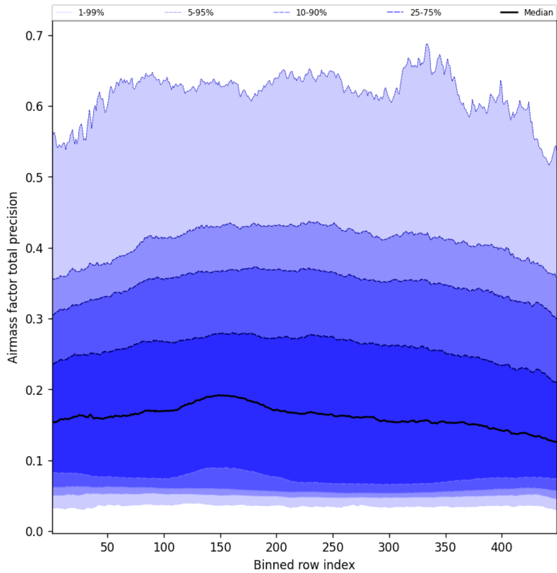
Figure 53: Along track statistics of “Airmass factor total precision” for 2025-03-13 to 2025-03-14
