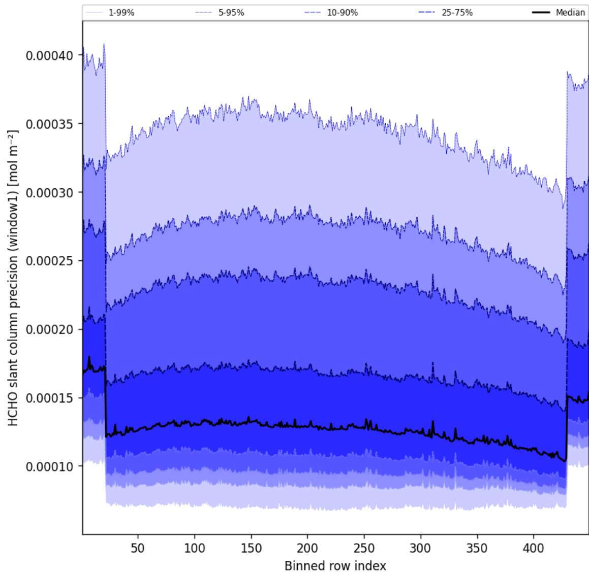
Figure 51: Along track statistics of “HCHO slant column precision (window1)” for 2025-03-13 to 2025-03-14
