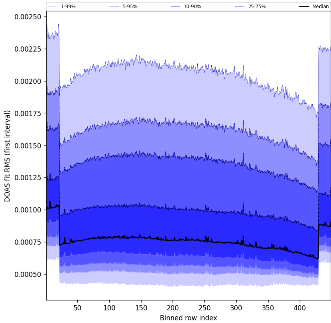
Figure 58: Along track statistics of “DOAS fit RMS (first interval)” for 2025-03-13 to 2025-03-14
