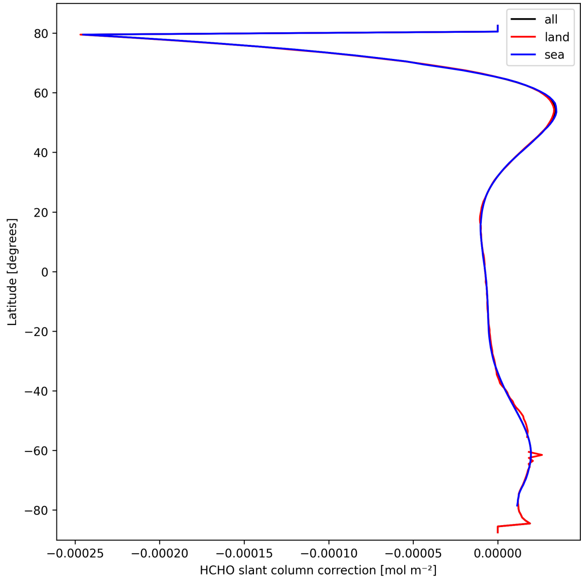
Figure 31: Zonal average of “HCHO slant column correction” for 2025-03-13 to 2025-03-14.
