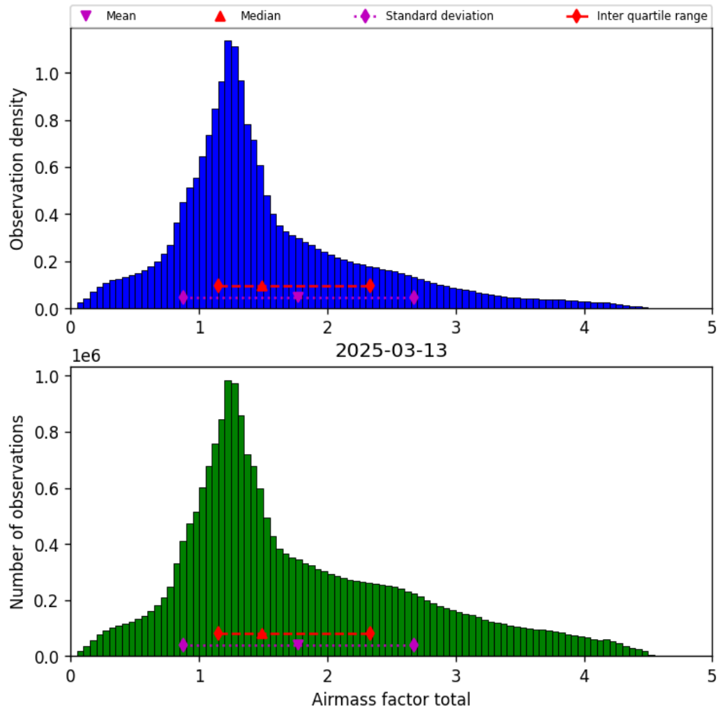
Figure 38: Histogram of “Airmass factor total” for 2025-03-13 to 2025-03-14
