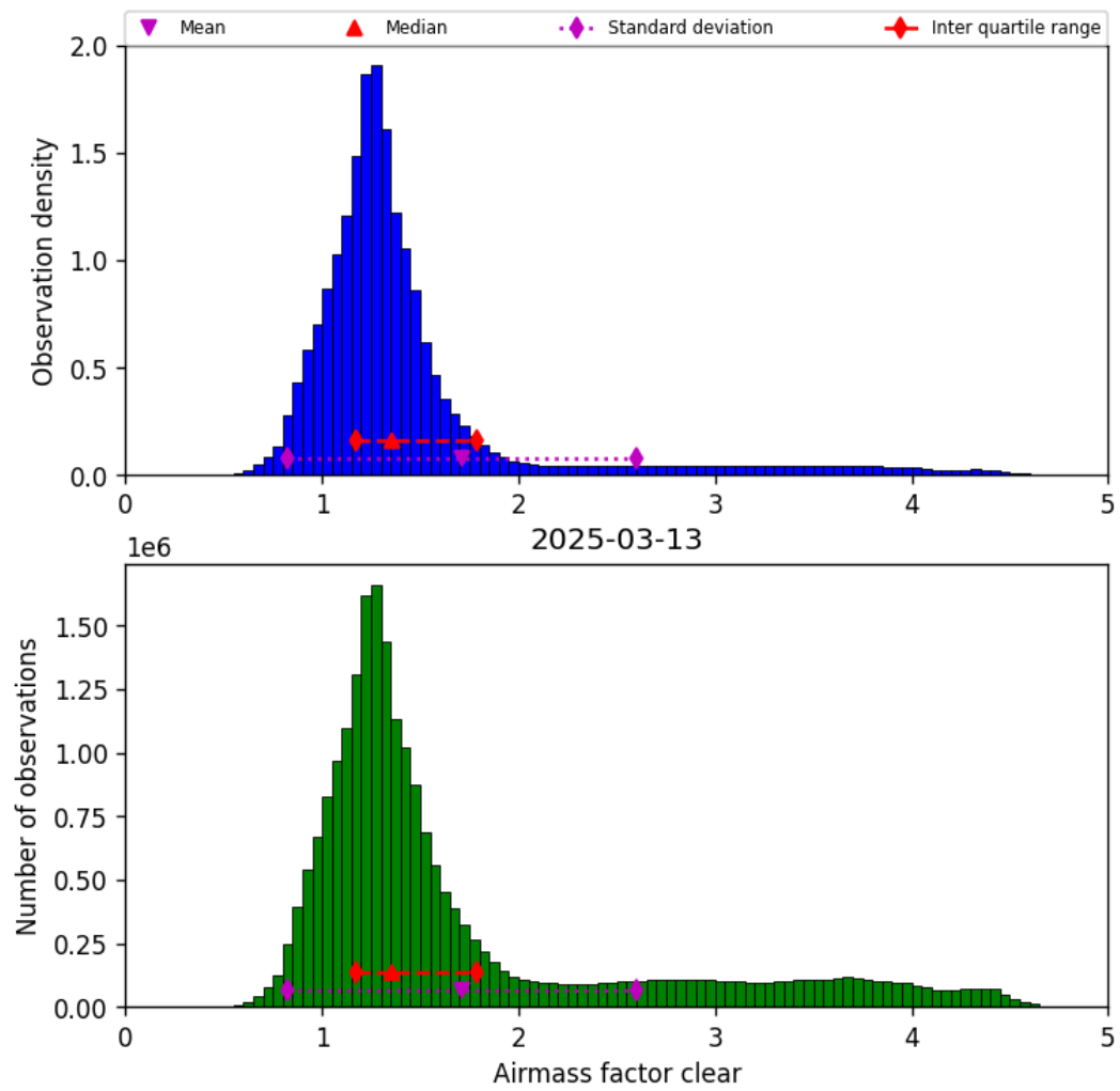
Figure 40: Histogram of “Airmass factor clear” for 2025-03-13 to 2025-03-14
