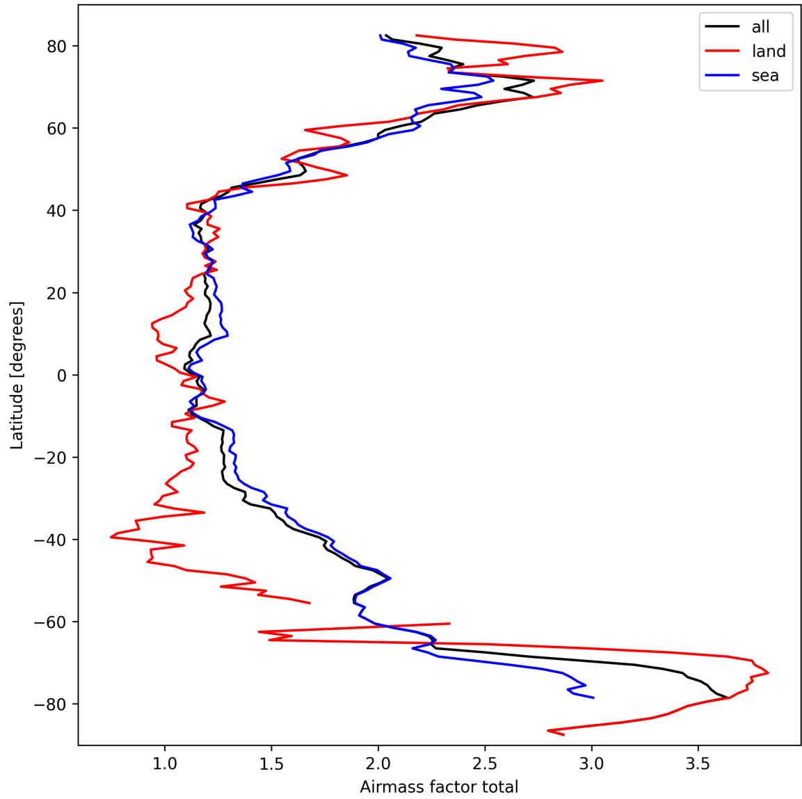
Figure 24: Zonal average of “Airmass factor total” for 2025-03-13 to 2025-03-14.
