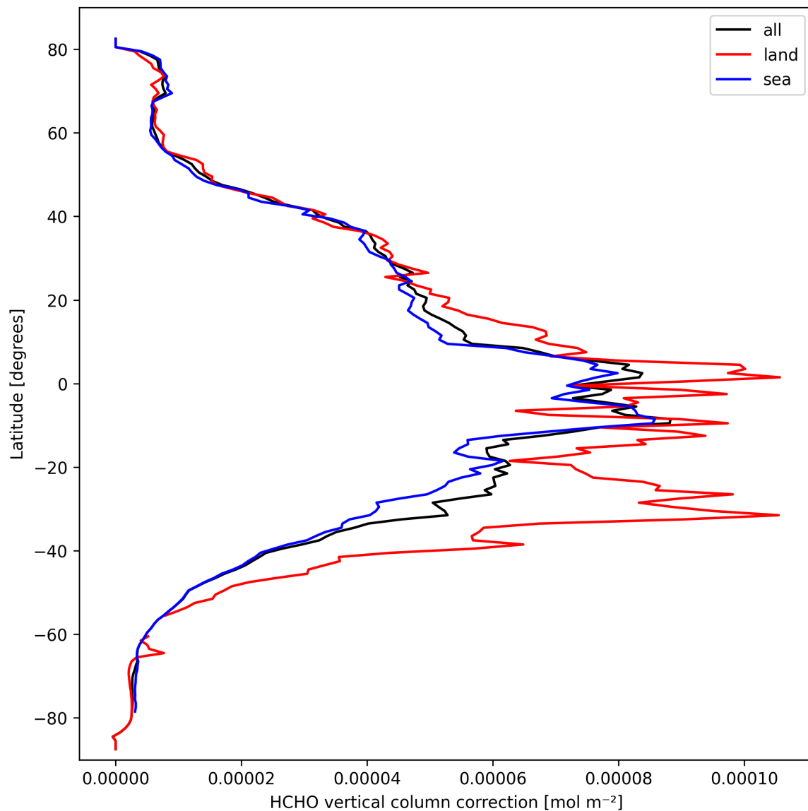
Figure 21: Zonal average of “HCHO vertical column correction” for 2025-03-13 to 2025-03-14.
