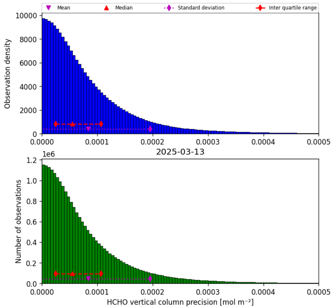
Figure 34: Histogram of “HCHO vertical column precision” for 2025-03-13 to 2025-03-14
