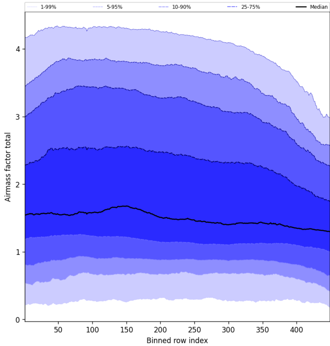
Figure 52: Along track statistics of “Airmass factor total” for 2025-03-13 to 2025-03-14
