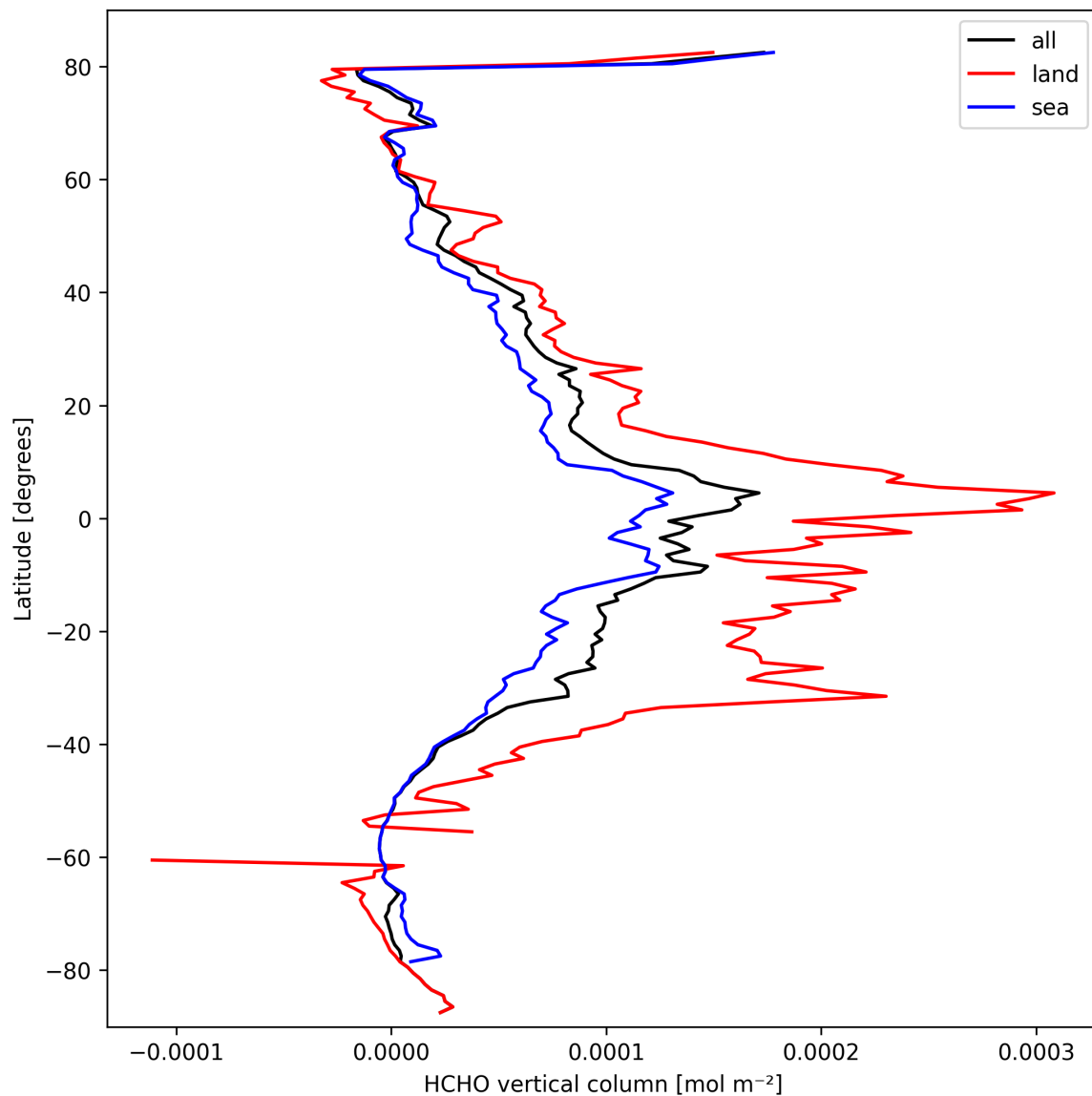
Figure 19: Zonal average of “HCHO vertical column” for 2025-03-13 to 2025-03-14.
