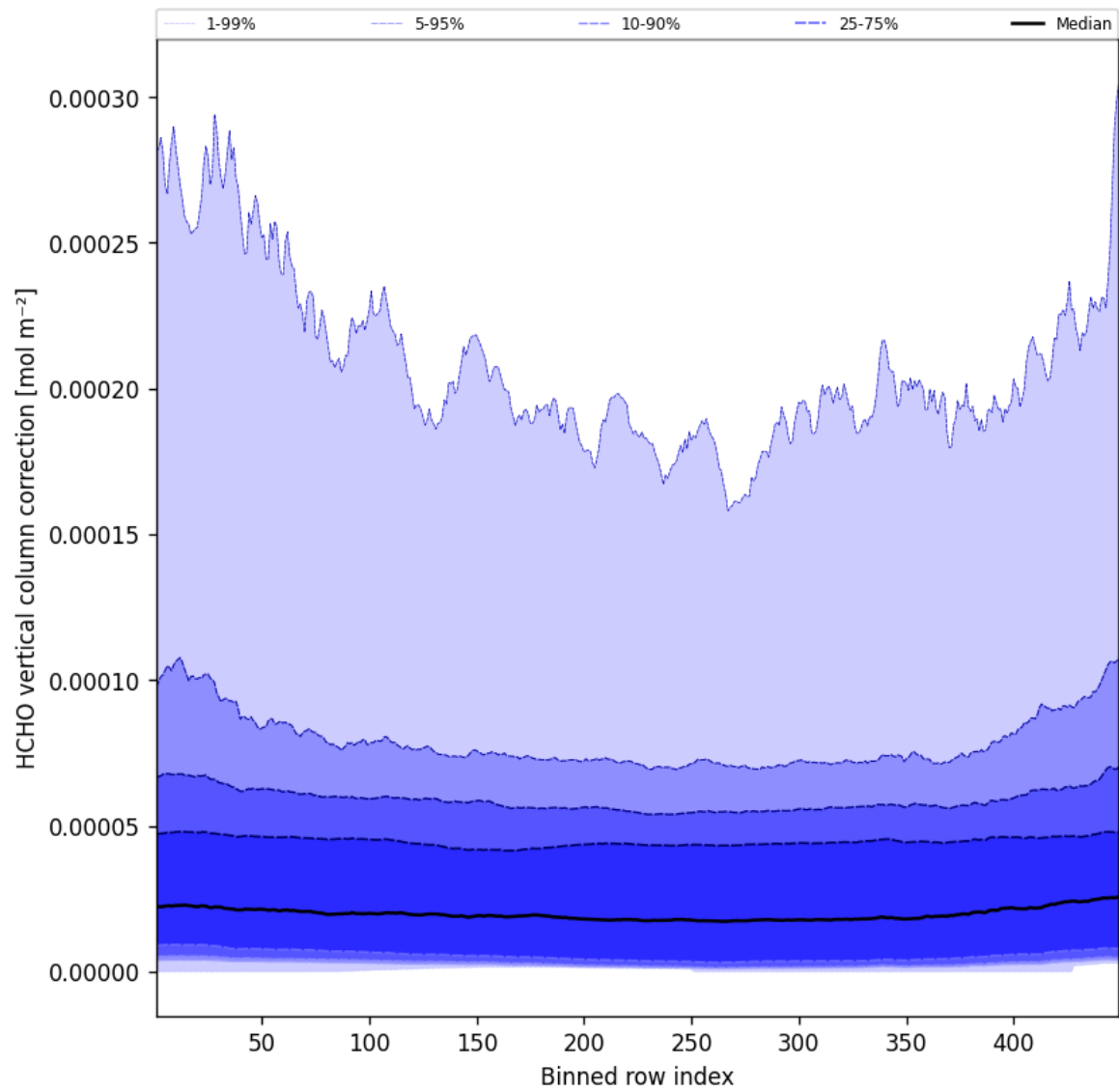
Figure 49: Along track statistics of “HCHO vertical column correction” for 2025-03-13 to 2025-03-14
