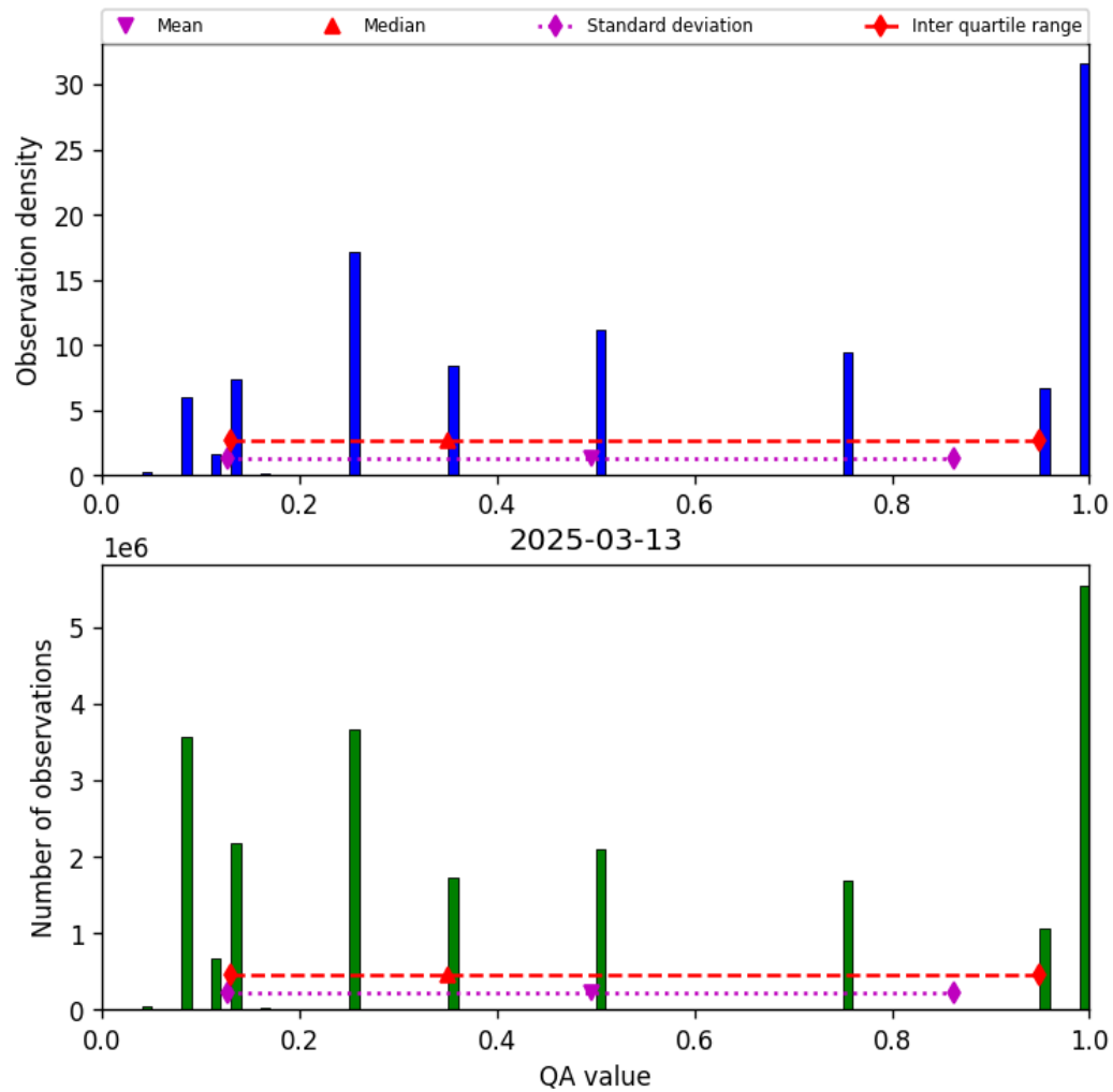
Figure 32: Histogram of “QA value” for 2025-03-13 to 2025-03-14
