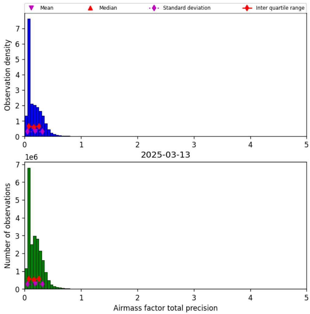
Figure 39: Histogram of “Airmass factor total precision” for 2025-03-13 to 2025-03-14
