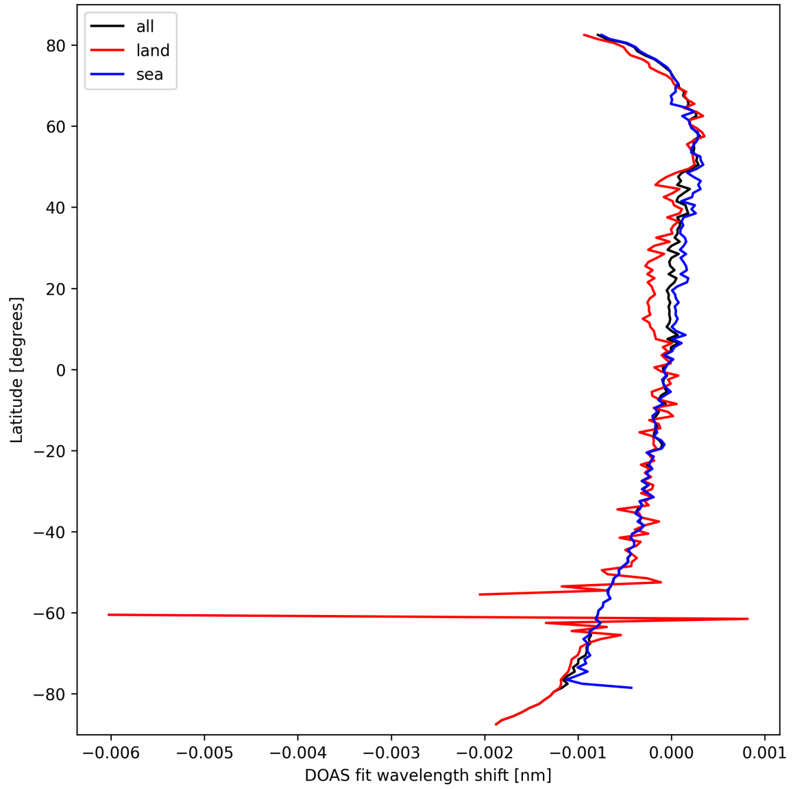
Figure 28: Zonal average of “DOAS fit wavelength shift” for 2025-03-13 to 2025-03-14.
