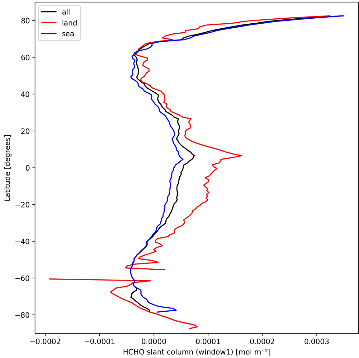
Figure 22: Zonal average of “HCHO slant column (window1)” for 2025-03-13 to 2025-03-14.
