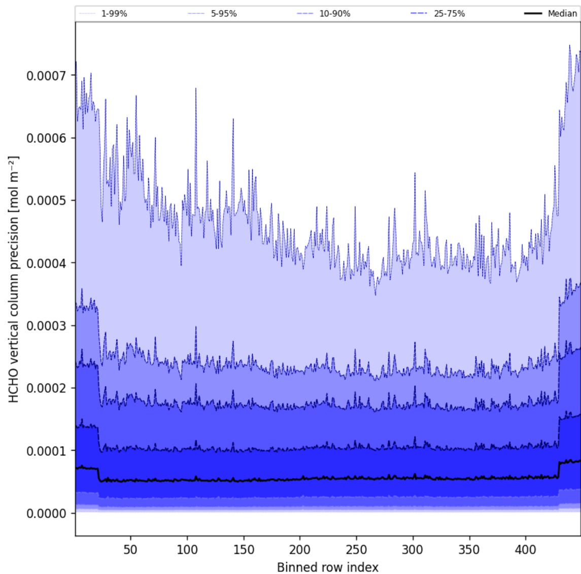
Figure 48: Along track statistics of “HCHO vertical column precision” for 2025-03-13 to 2025-03-14
