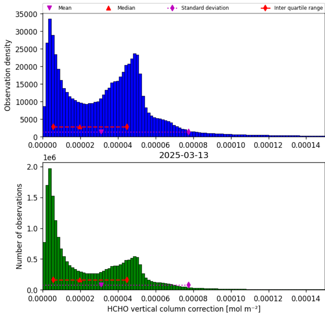
Figure 35: Histogram of “HCHO vertical column correction” for 2025-03-13 to 2025-03-14
