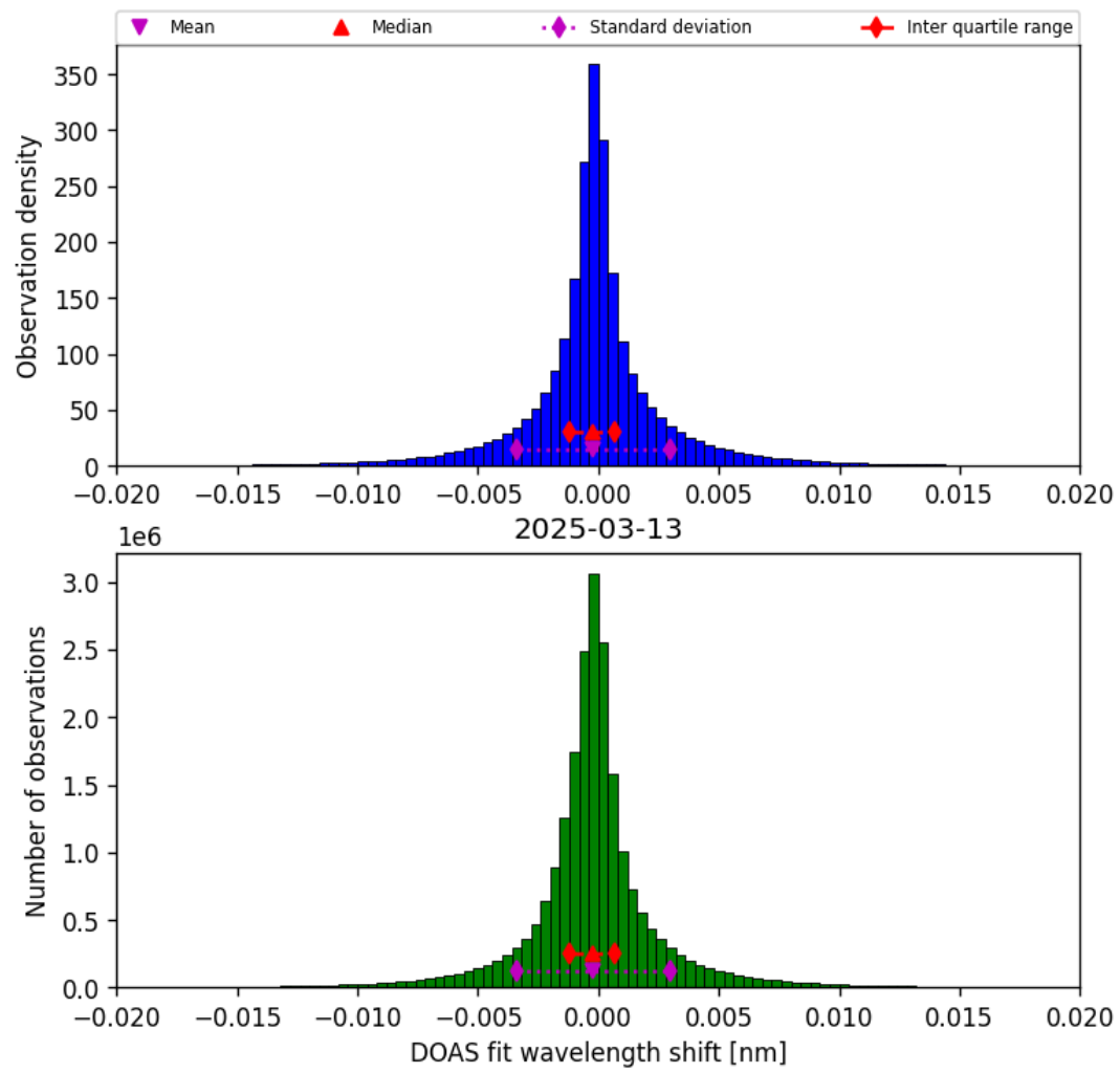
Figure 42: Histogram of “DOAS fit wavelength shift” for 2025-03-13 to 2025-03-14
