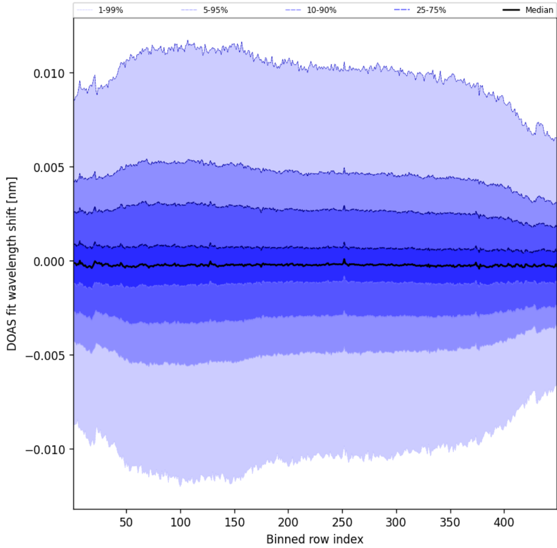
Figure 56: Along track statistics of “DOAS fit wavelength shift” for 2025-03-13 to 2025-03-14
