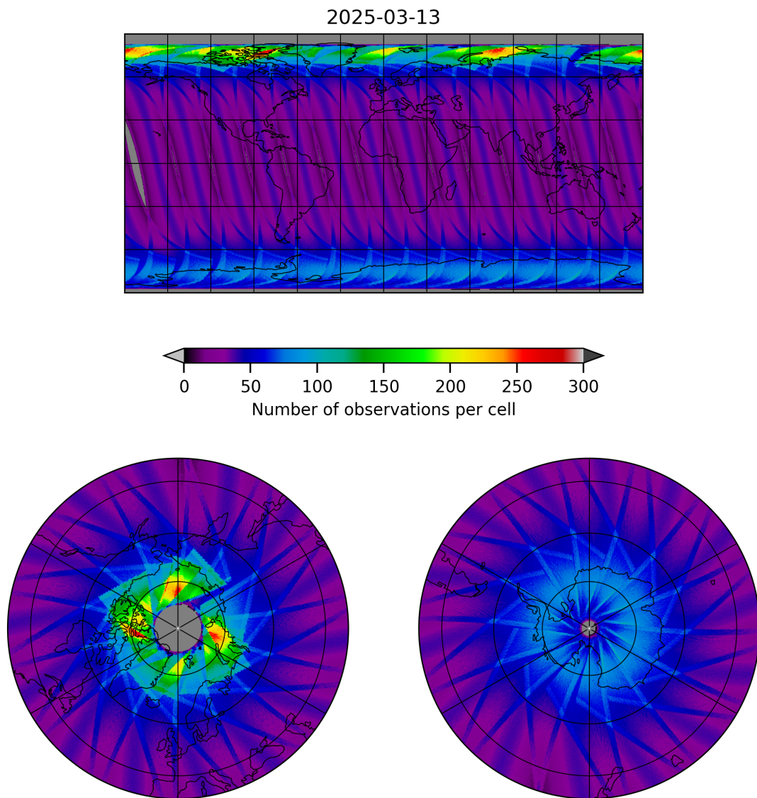
Figure 17: Map of the number of observations for 2025-03-13 to 2025-03-14
