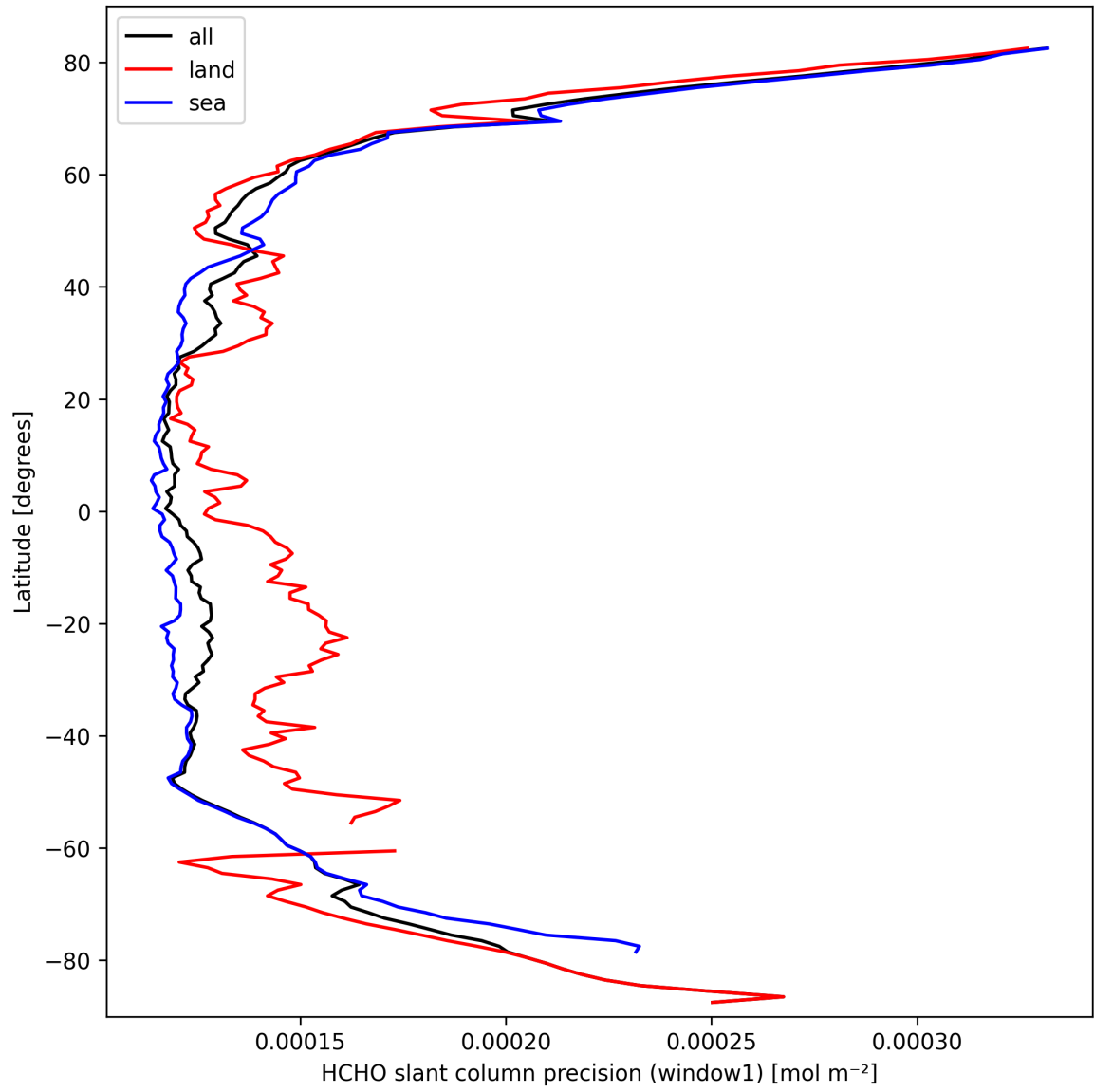
Figure 23: Zonal average of “HCHO slant column precision (window1)” for 2025-03-13 to 2025-03-14.
