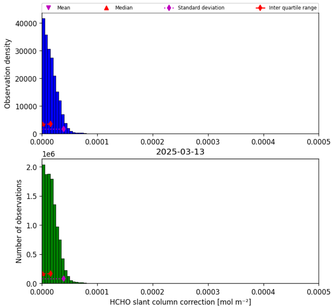
Figure 45: Histogram of “HCHO slant column correction” for 2025-03-13 to 2025-03-14
