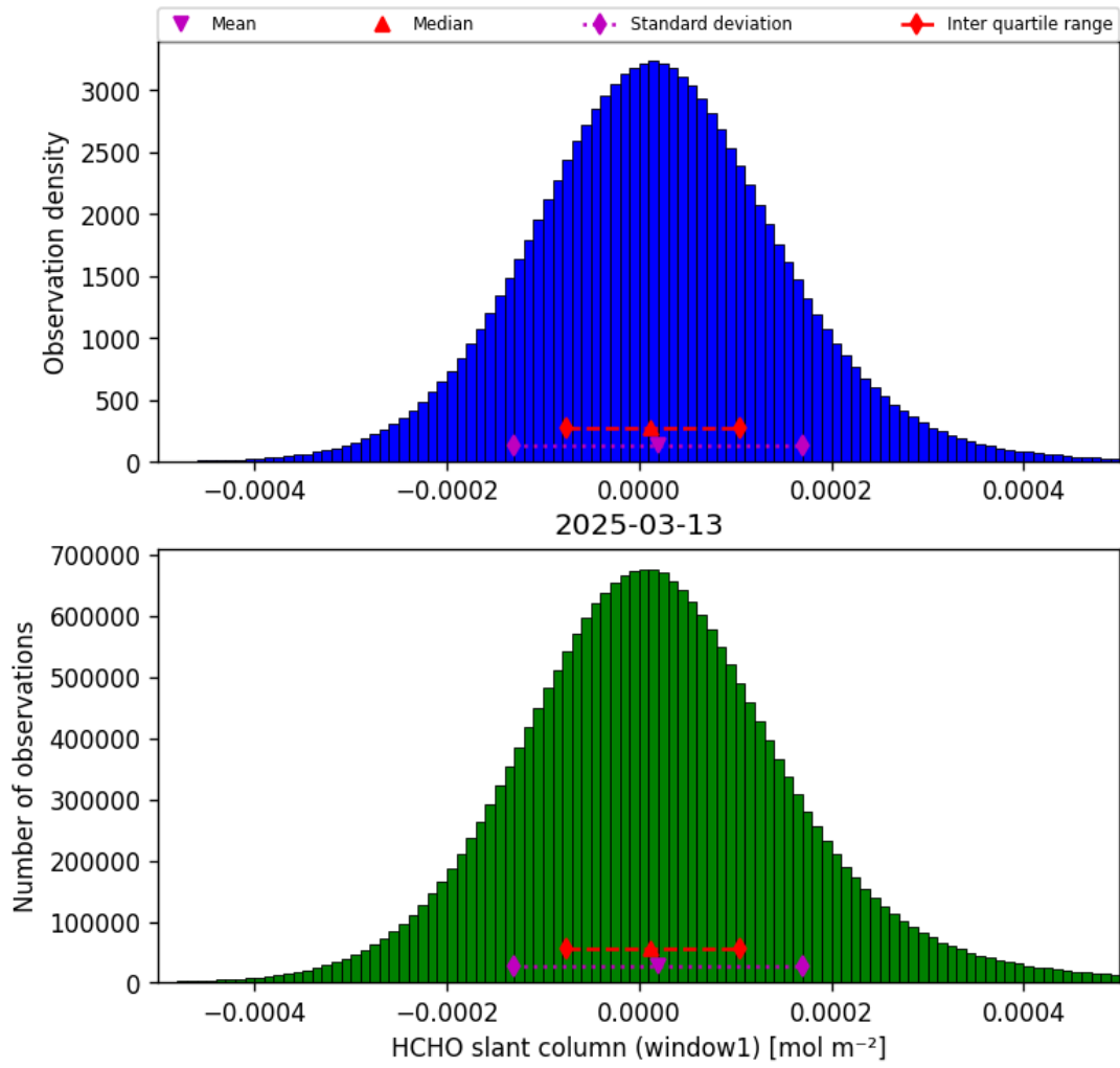
Figure 36: Histogram of “HCHO slant column (window1)” for 2025-03-13 to 2025-03-14
