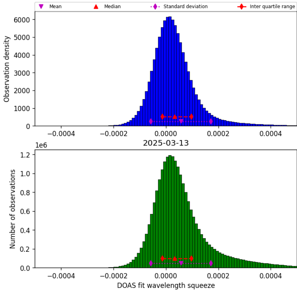
Figure 43: Histogram of “DOAS fit wavelength squeeze” for 2025-03-13 to 2025-03-14
