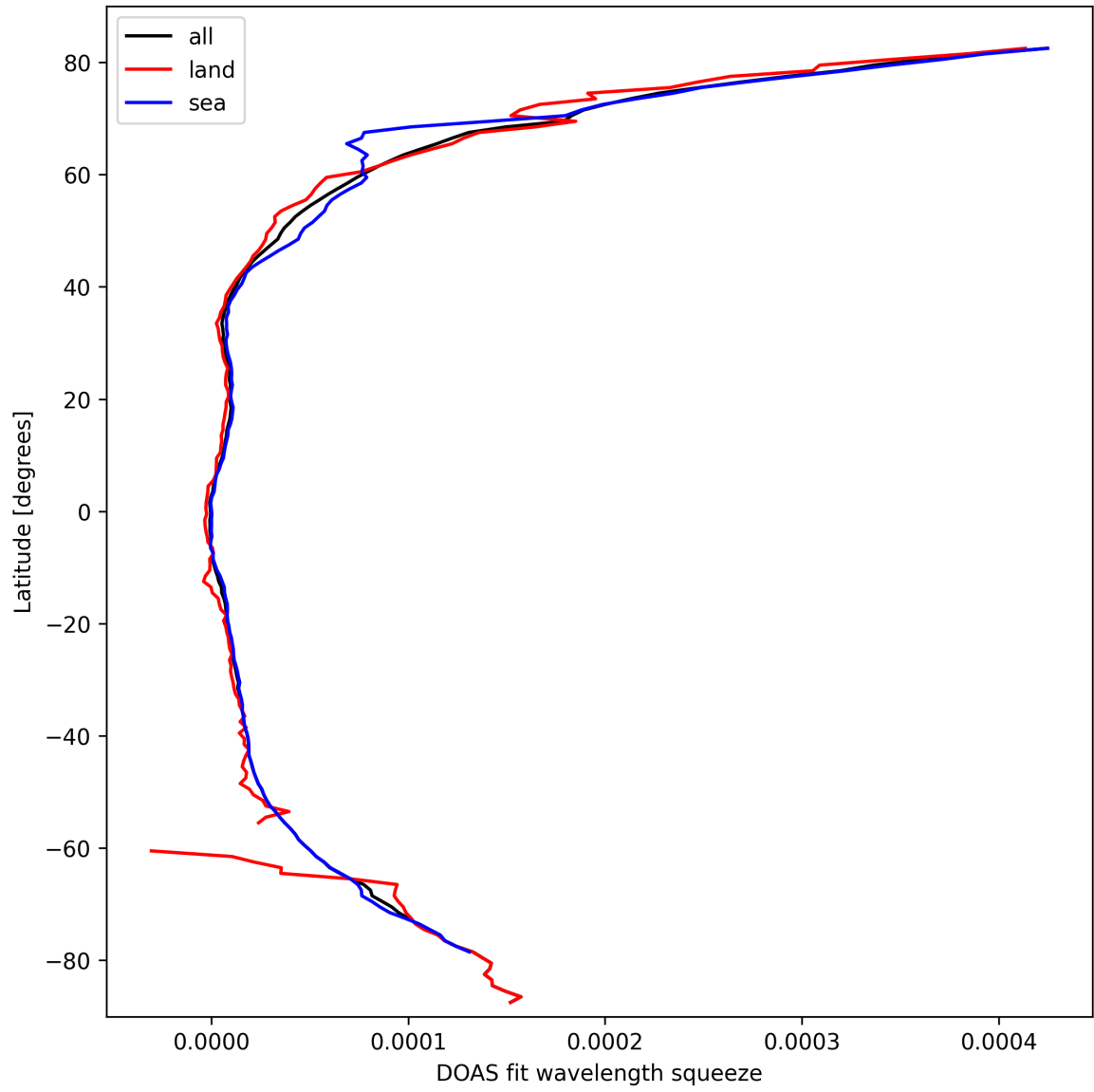
Figure 29: Zonal average of “DOAS fit wavelength squeeze” for 2025-03-13 to 2025-03-14.
