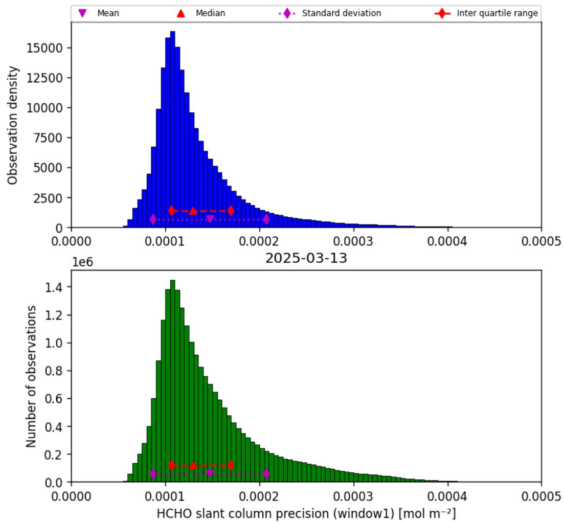
Figure 37: Histogram of “HCHO slant column precision (window1)” for 2025-03-13 to 2025-03-14
