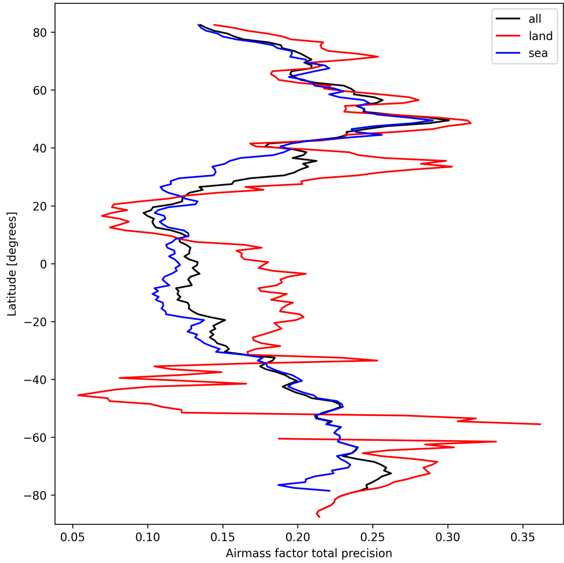
Figure 25: Zonal average of “Airmass factor total precision” for 2025-03-13 to 2025-03-14.
