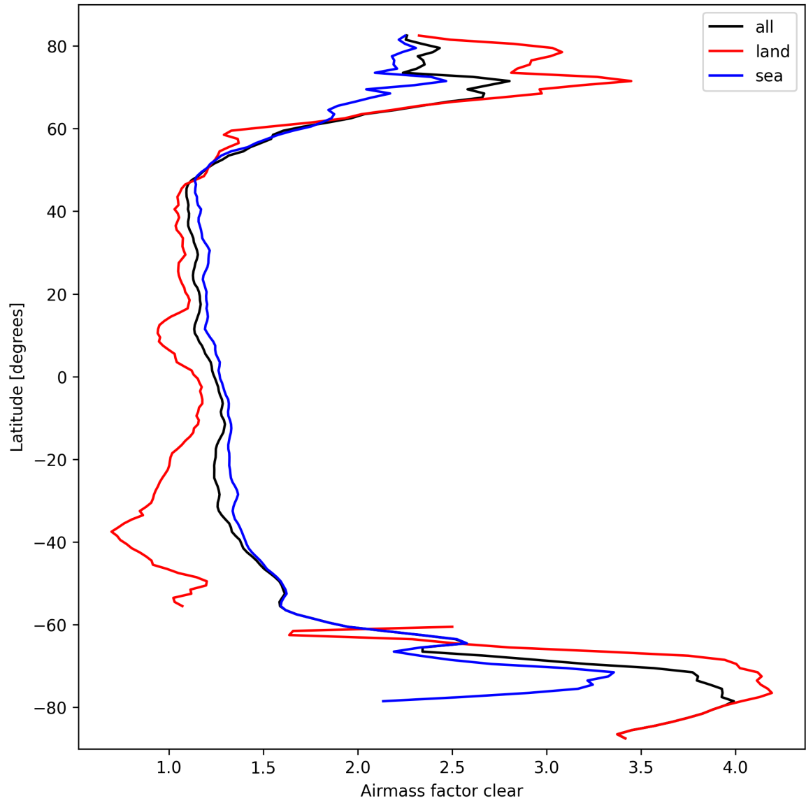
Figure 26: Zonal average of “Airmass factor clear” for 2025-03-13 to 2025-03-14.
