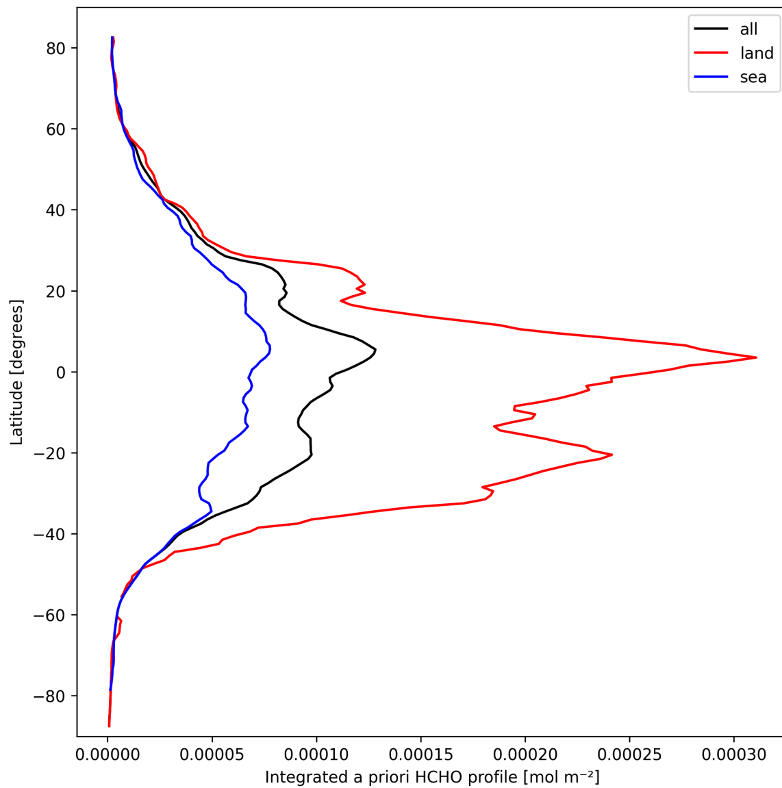
Figure 27: Zonal average of “Integrated a priori HCHO profile” for 2025-03-13 to 2025-03-14.
