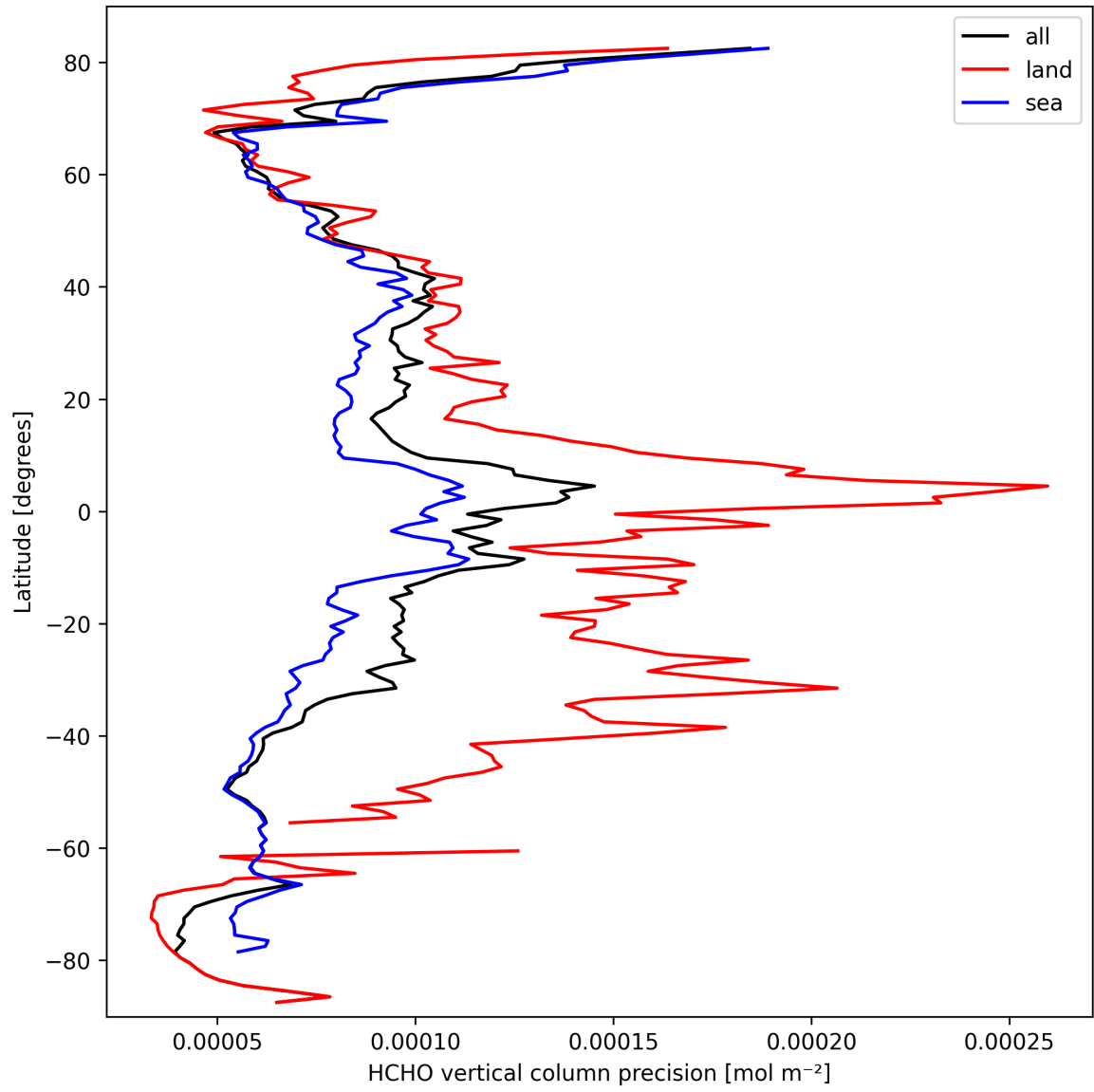
Figure 20: Zonal average of “HCHO vertical column precision” for 2025-03-13 to 2025-03-14.
