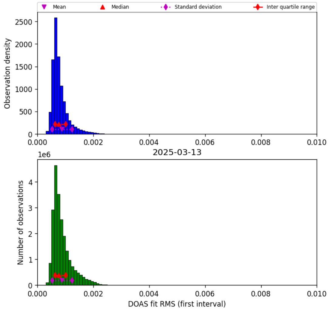
Figure 44: Histogram of “DOAS fit RMS (first interval)” for 2025-03-13 to 2025-03-14
