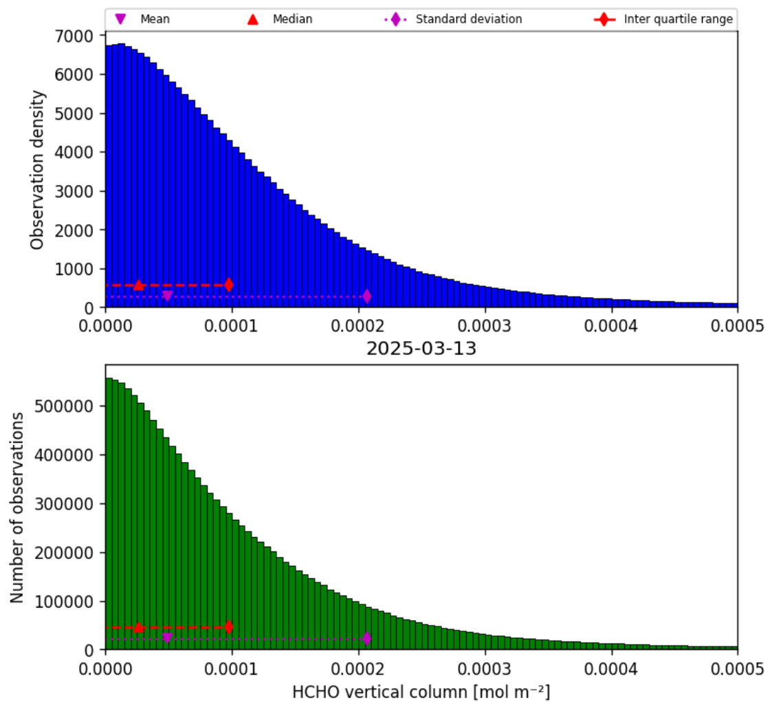
Figure 33: Histogram of “HCHO vertical column” for 2025-03-13 to 2025-03-14
