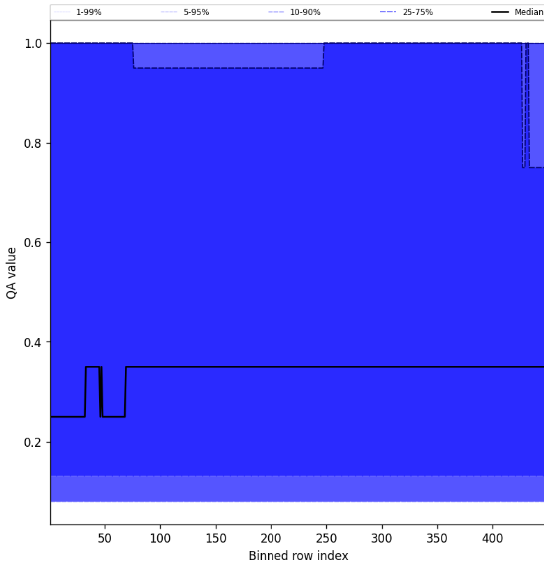
Figure 46: Along track statistics of “QA value” for 2025-03-15 to 2025-03-15
