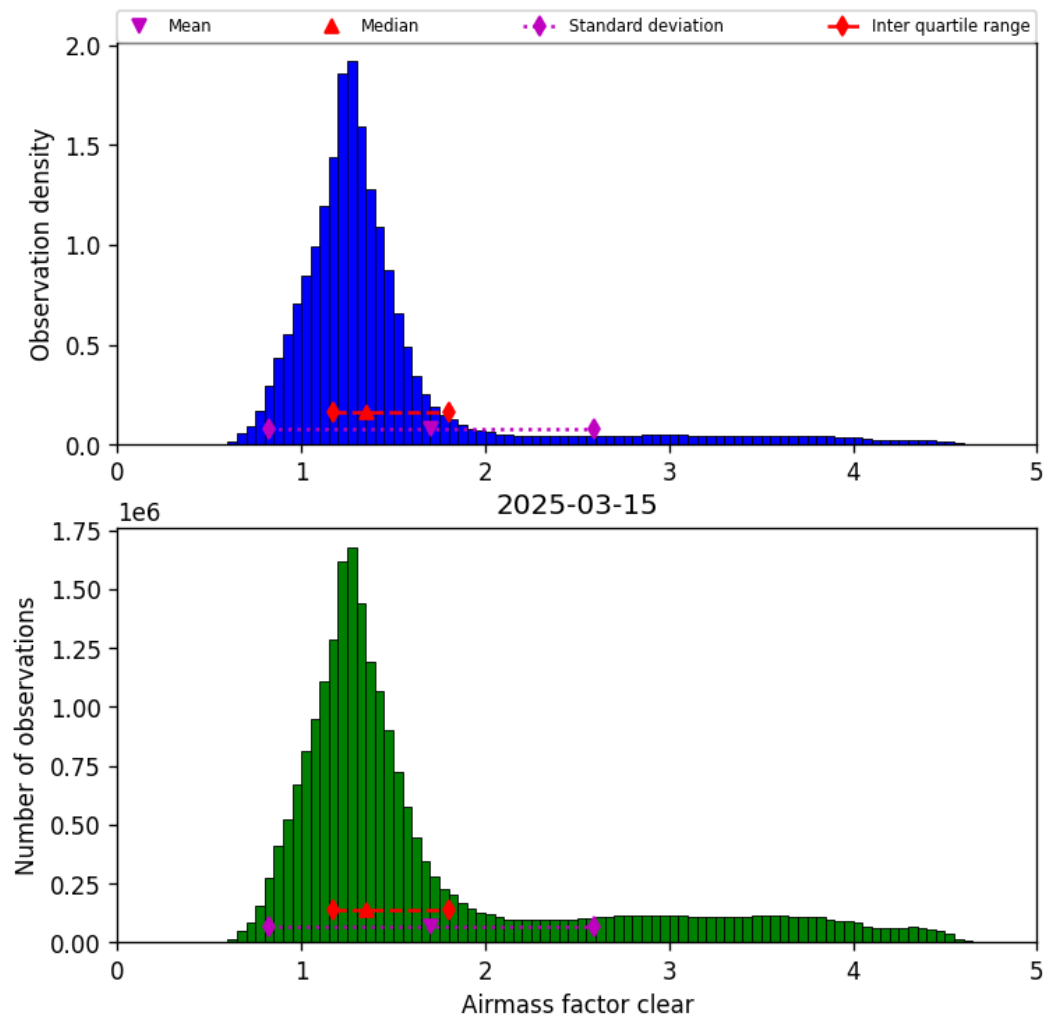
Figure 40: Histogram of “Airmass factor clear” for 2025-03-15 to 2025-03-15
