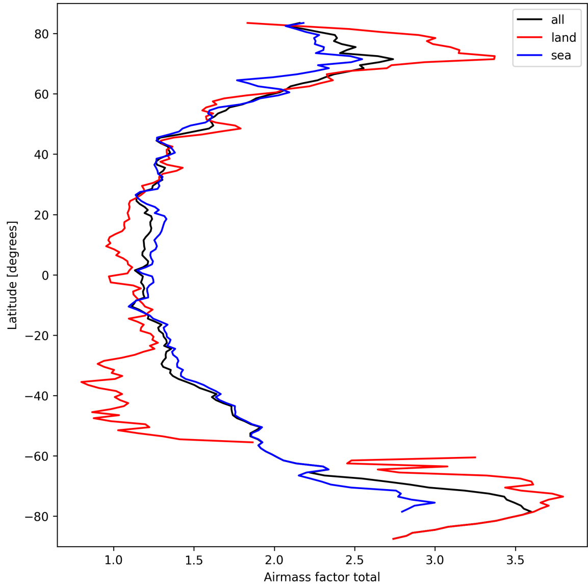
Figure 24: Zonal average of “Airmass factor total” for 2025-03-15 to 2025-03-15.
