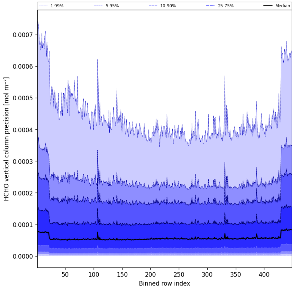
Figure 48: Along track statistics of “HCHO vertical column precision” for 2025-03-15 to 2025-03-15
