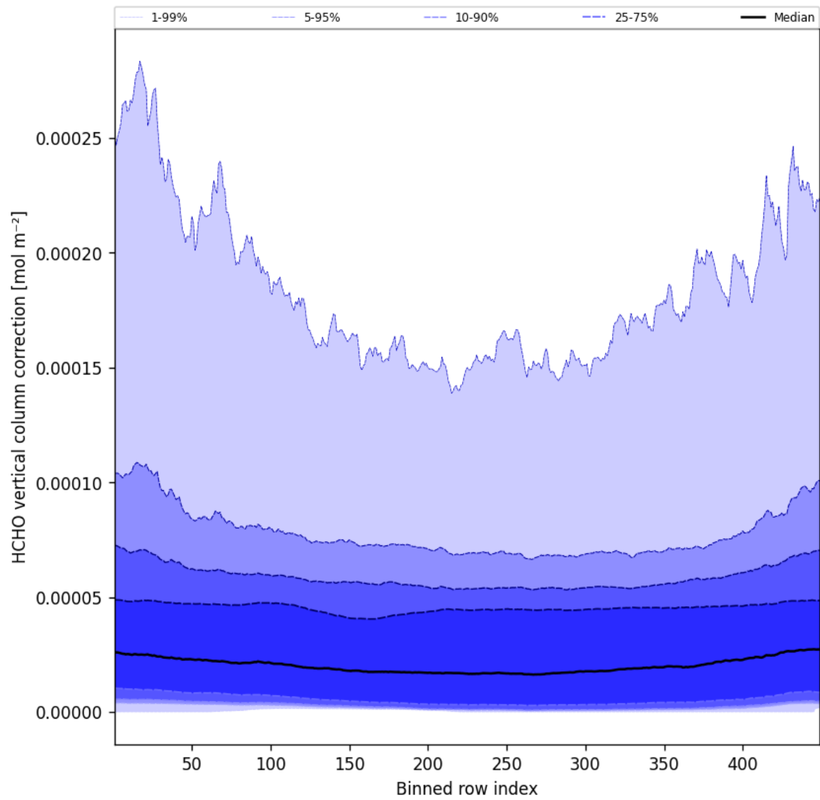
Figure 49: Along track statistics of “HCHO vertical column correction” for 2025-03-15 to 2025-03-15
