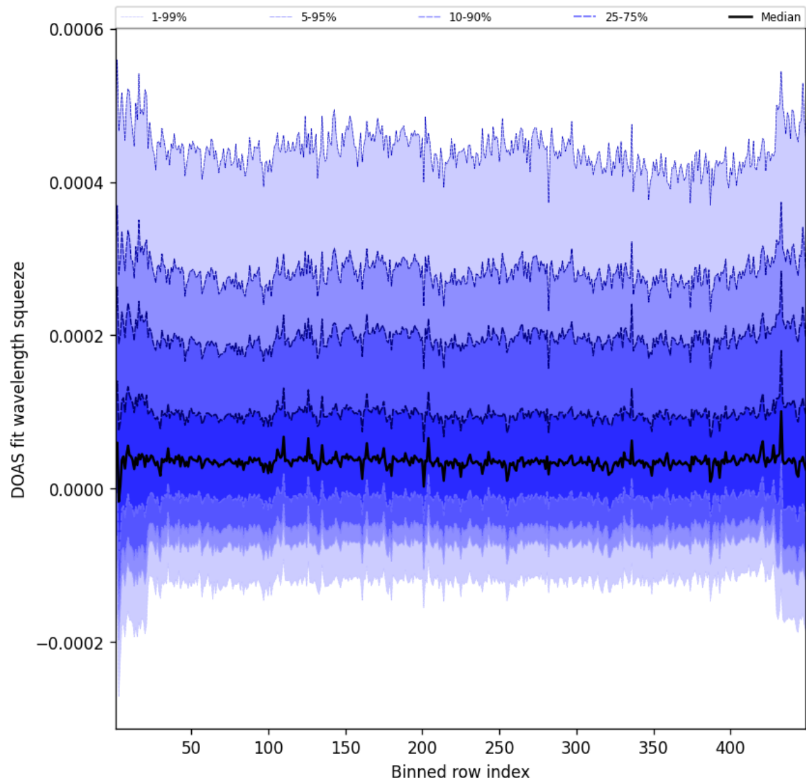
Figure 57: Along track statistics of “DOAS fit wavelength squeeze” for 2025-03-15 to 2025-03-15
