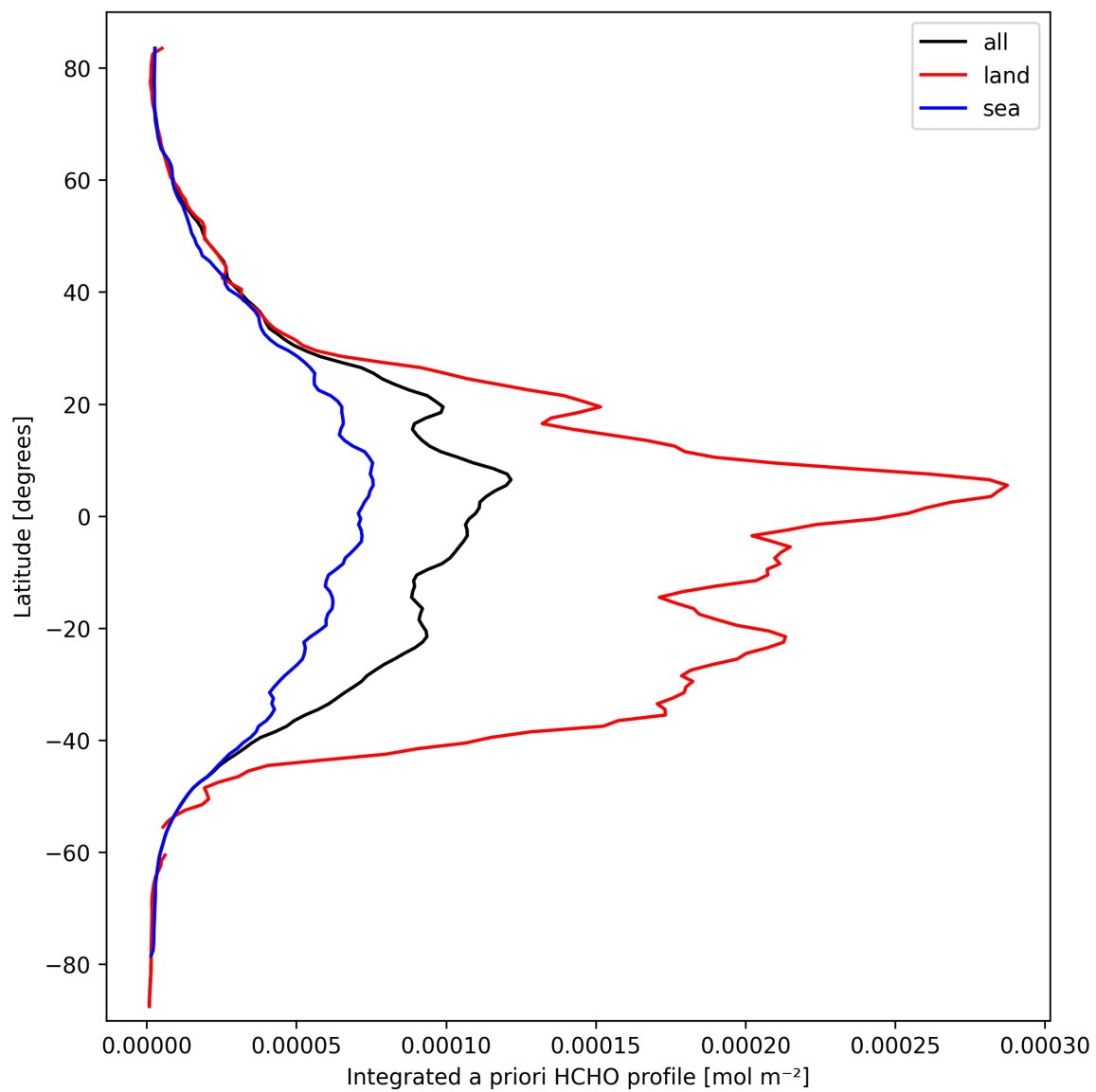
Figure 27: Zonal average of “Integrated a priori HCHO profile” for 2025-03-15 to 2025-03-15.
