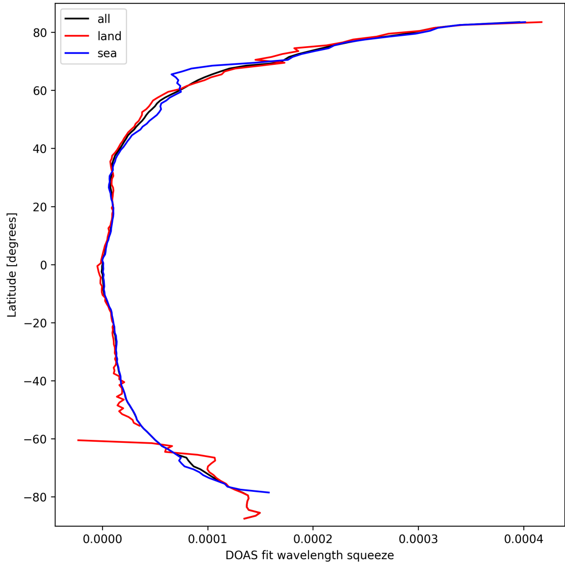
Figure 29: Zonal average of “DOAS fit wavelength squeeze” for 2025-03-15 to 2025-03-15.
