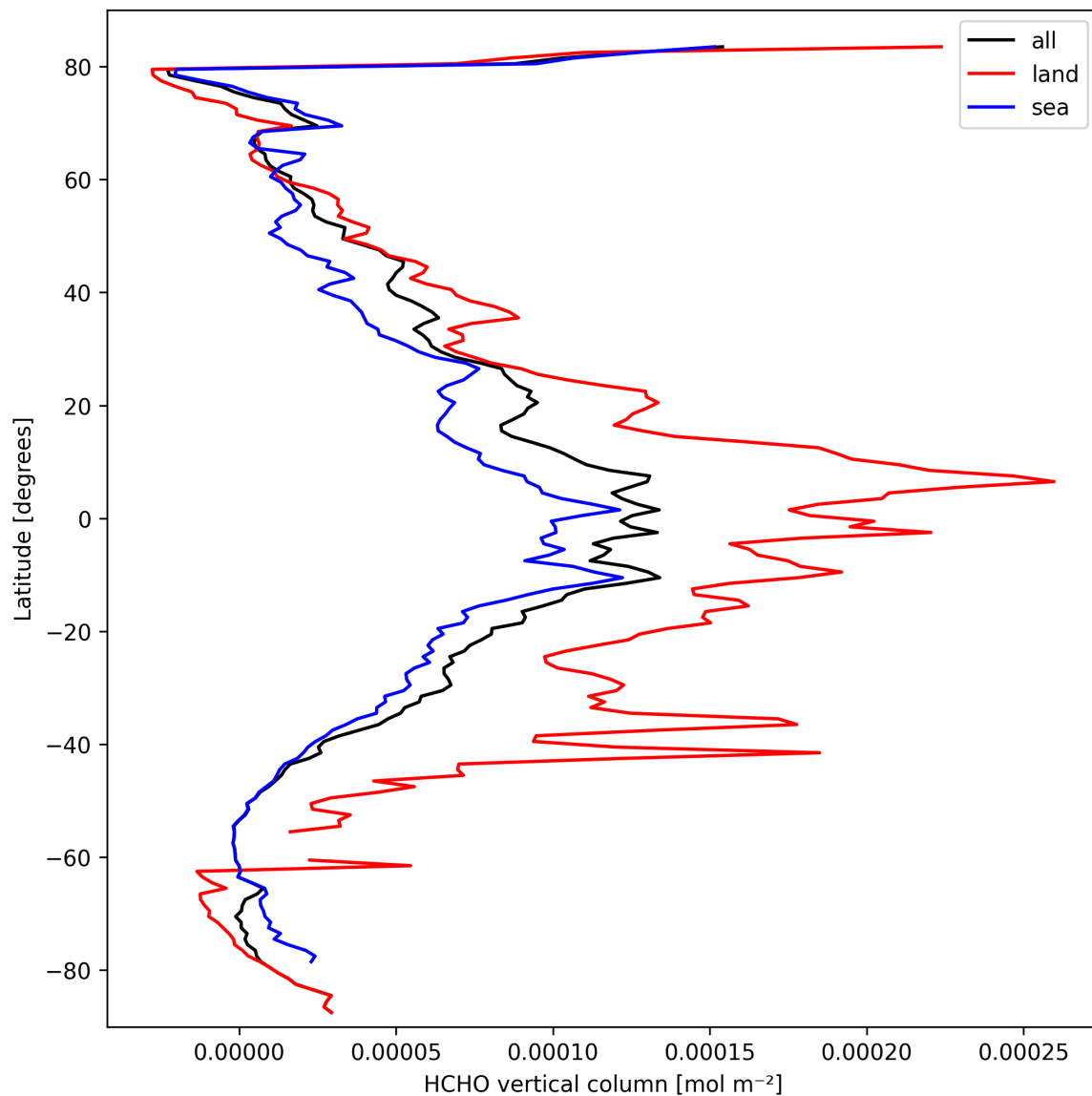
Figure 19: Zonal average of “HCHO vertical column” for 2025-03-15 to 2025-03-15.
