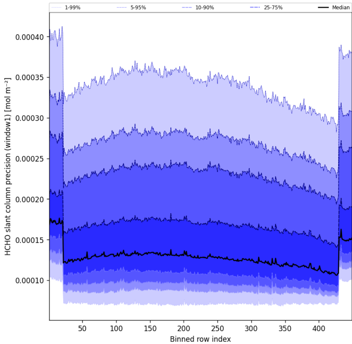
Figure 51: Along track statistics of “HCHO slant column precision (window1)” for 2025-03-15 to 2025-03-15
