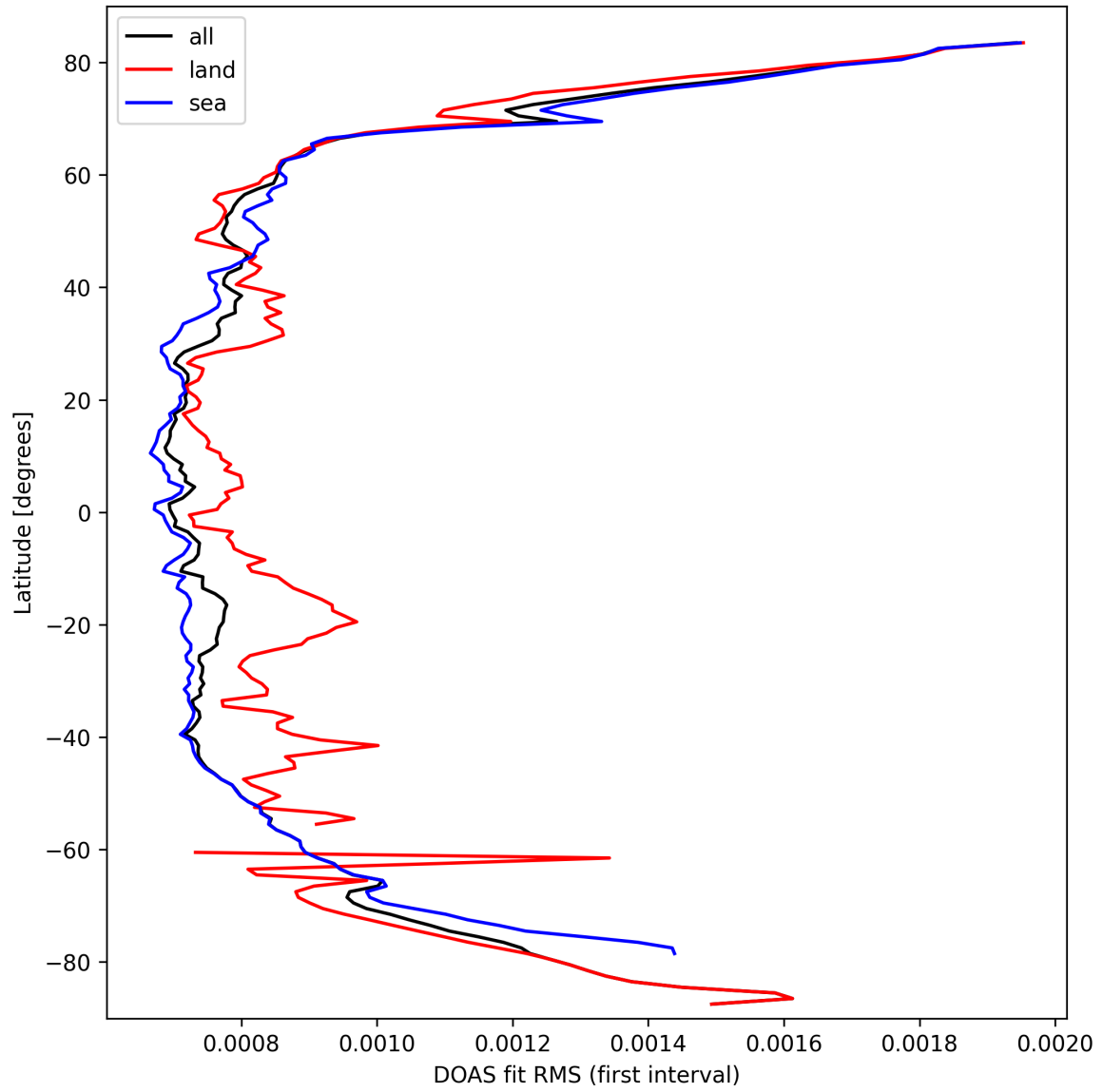
Figure 30: Zonal average of "DOAS fit RMS (first interval)" for 2025-03-15 to 2025-03-15.
