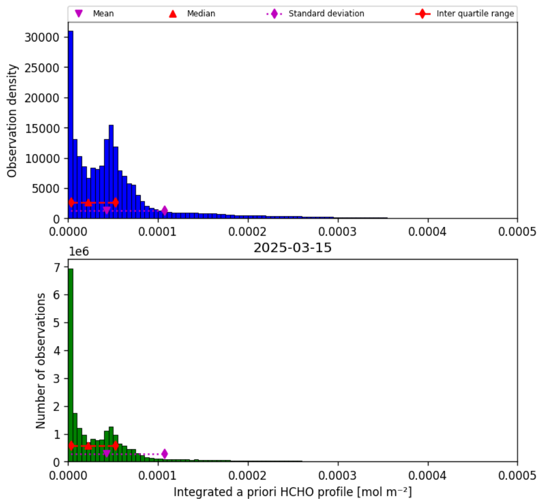
Figure 41: Histogram of “Integrated a priori HCHO profile” for 2025-03-15 to 2025-03-15
