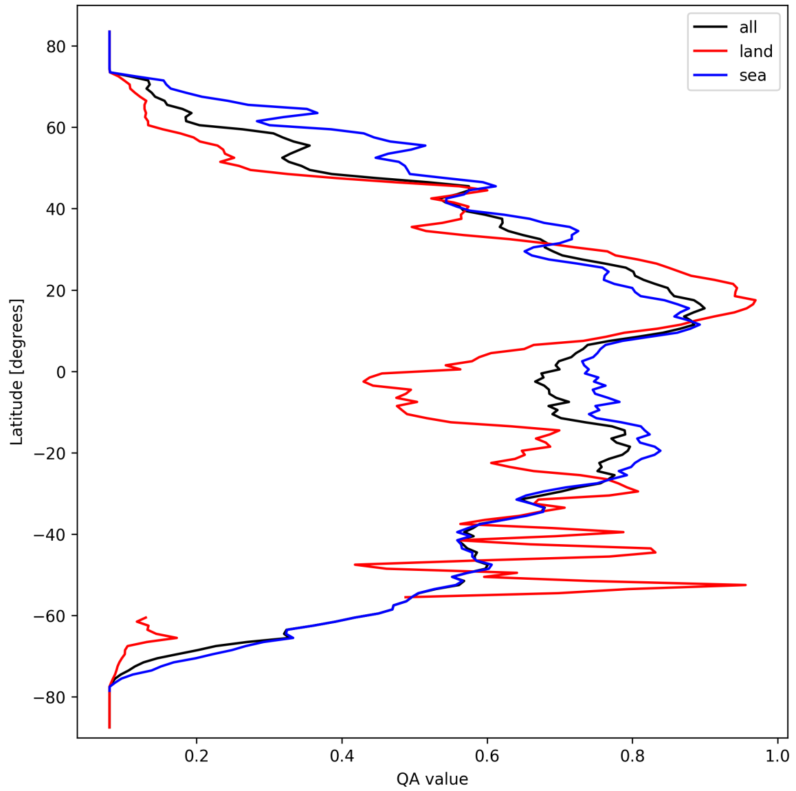
Figure 18: Zonal average of “QA value” for 2025-03-15 to 2025-03-15.
