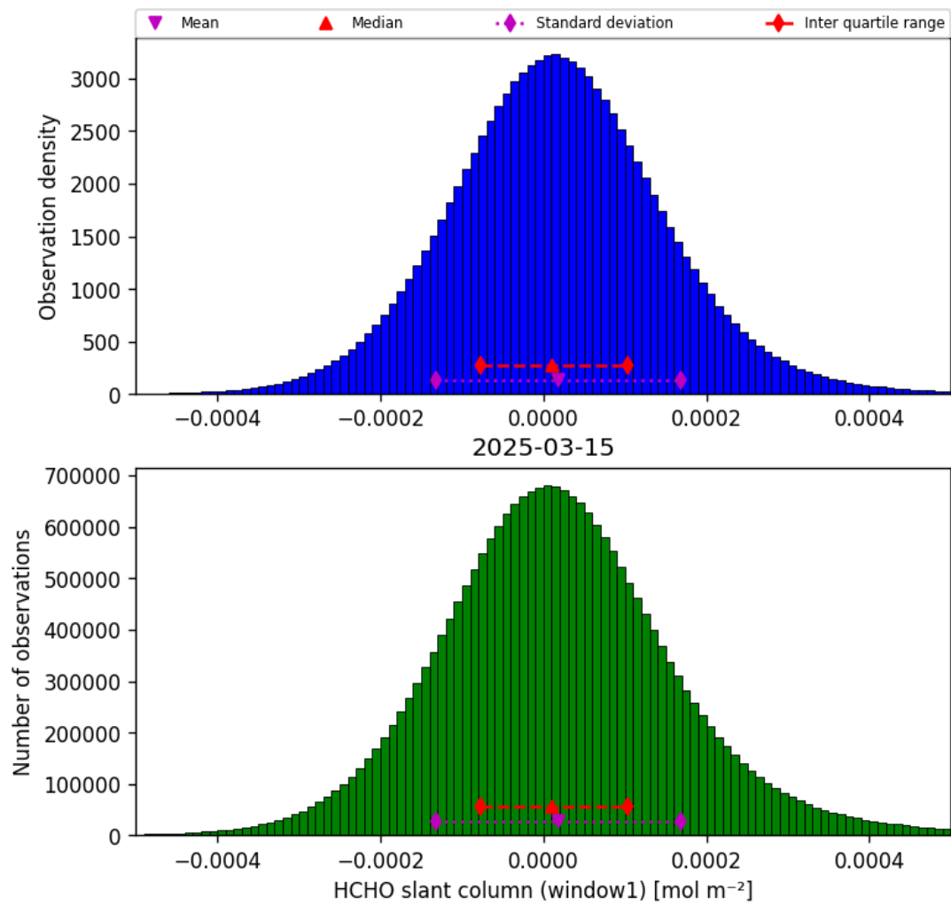
Figure 36: Histogram of “HCHO slant column (window1)” for 2025-03-15 to 2025-03-15
