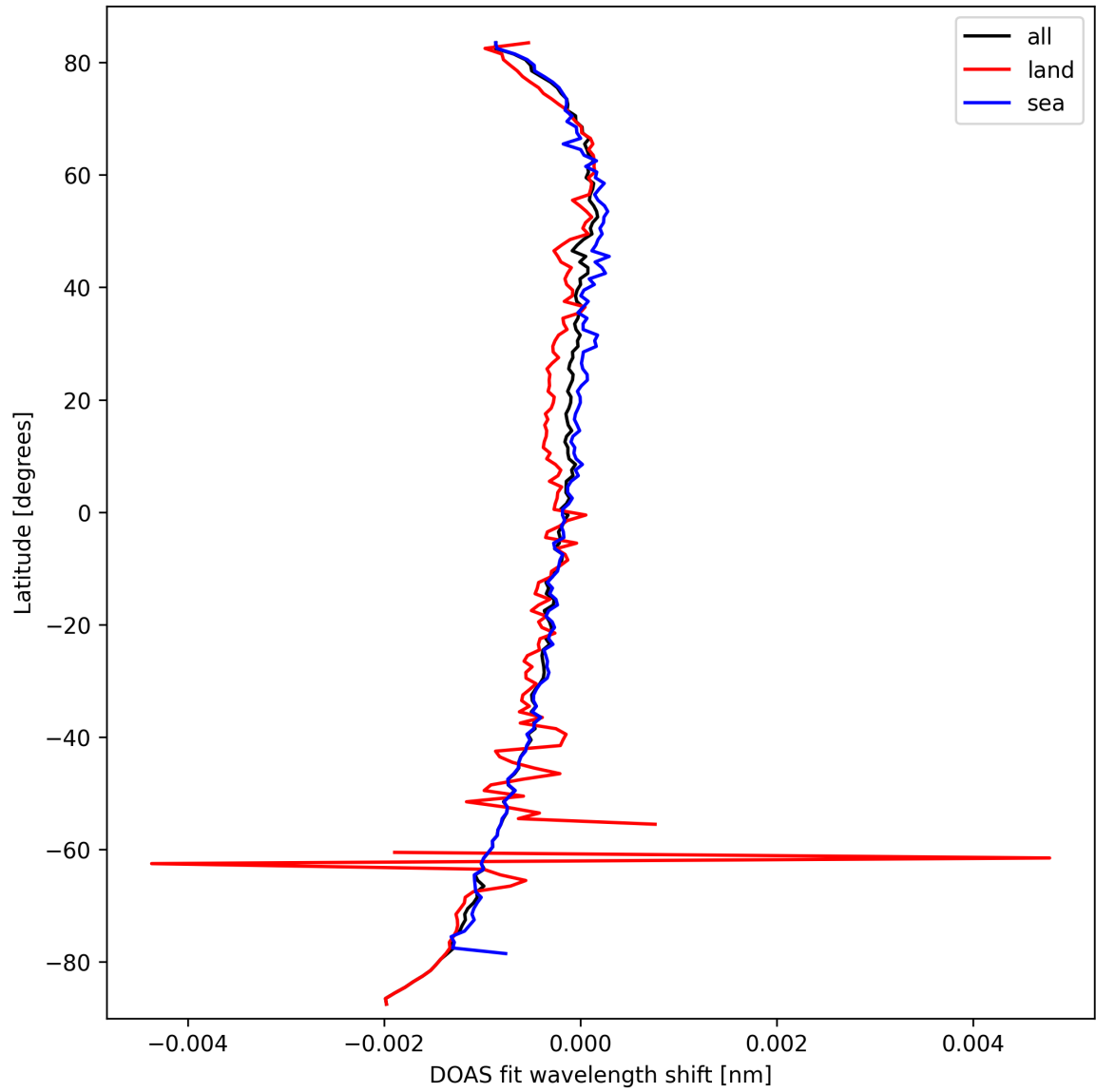
Figure 28: Zonal average of “DOAS fit wavelength shift” for 2025-03-15 to 2025-03-15.
