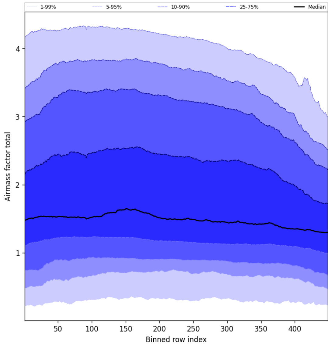
Figure 52: Along track statistics of “Airmass factor total” for 2025-03-15 to 2025-03-15
