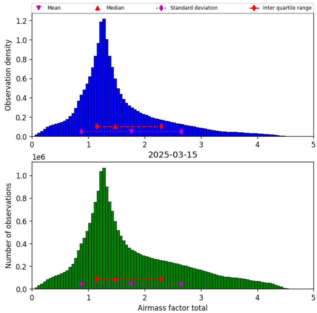
Figure 38: Histogram of “Airmass factor total” for 2025-03-15 to 2025-03-15
