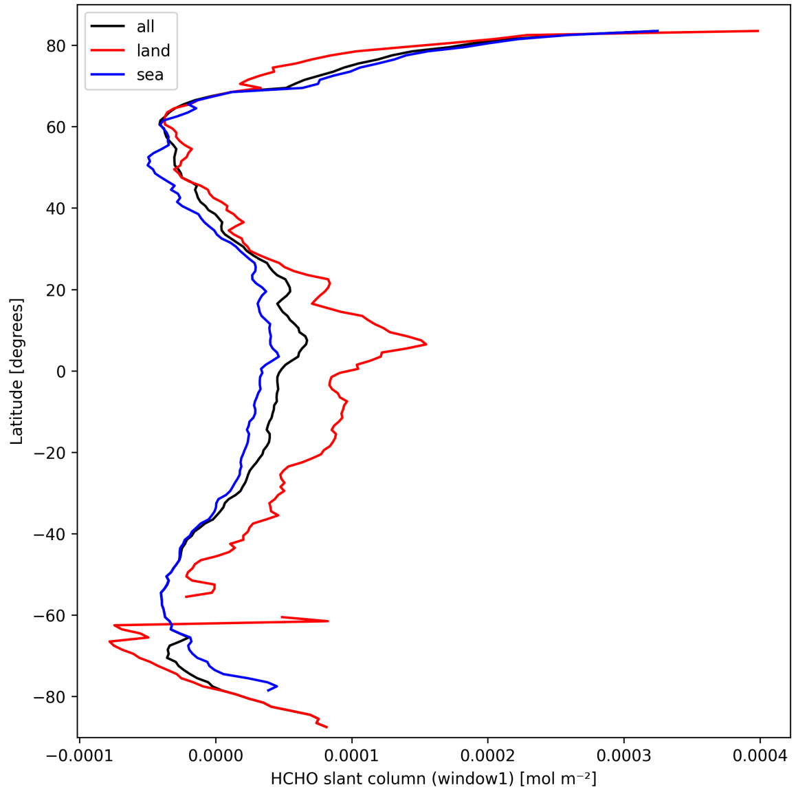
Figure 22: Zonal average of “HCHO slant column (window1)” for 2025-03-15 to 2025-03-15.
