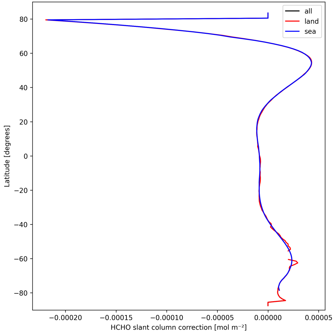
Figure 31: Zonal average of “HCHO slant column correction” for 2025-03-15 to 2025-03-15.
