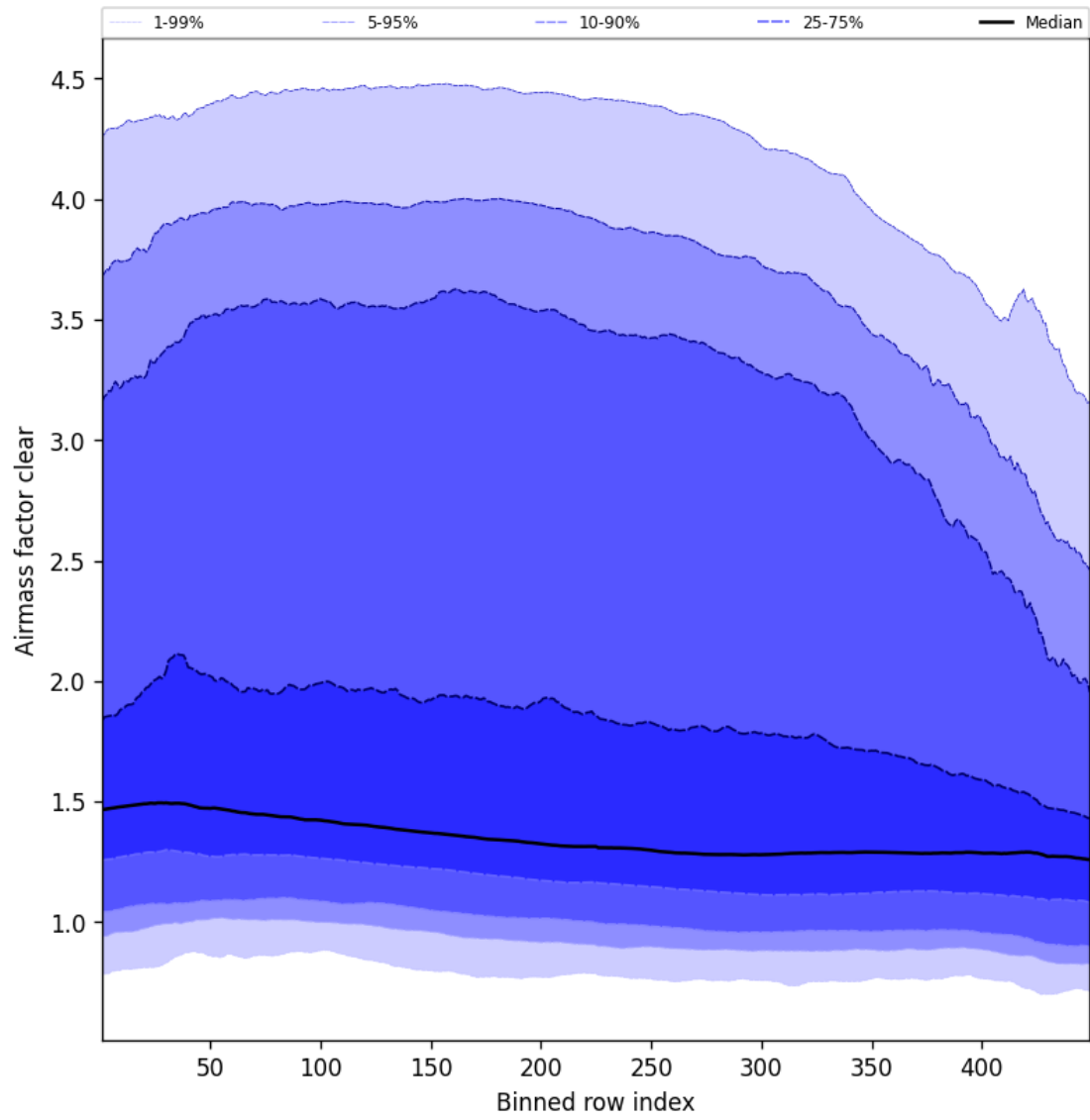
Figure 54: Along track statistics of “Airmass factor clear” for 2025-03-15 to 2025-03-15
