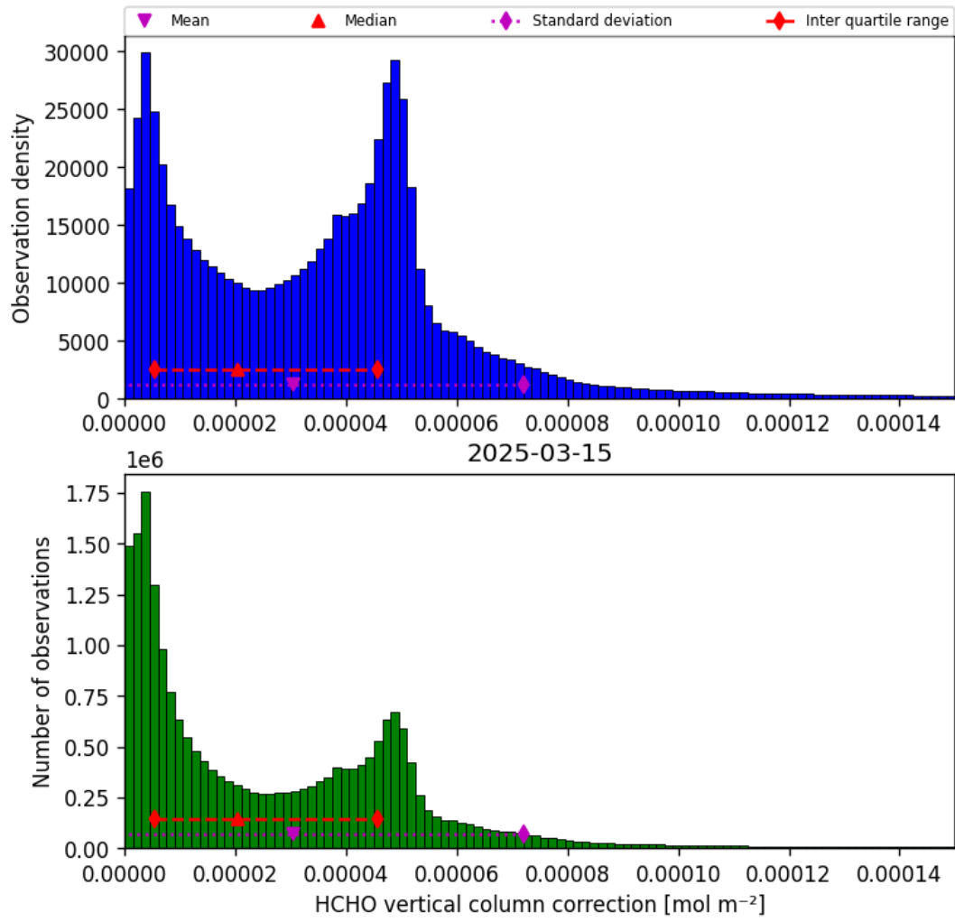
Figure 35: Histogram of “HCHO vertical column correction” for 2025-03-15 to 2025-03-15
