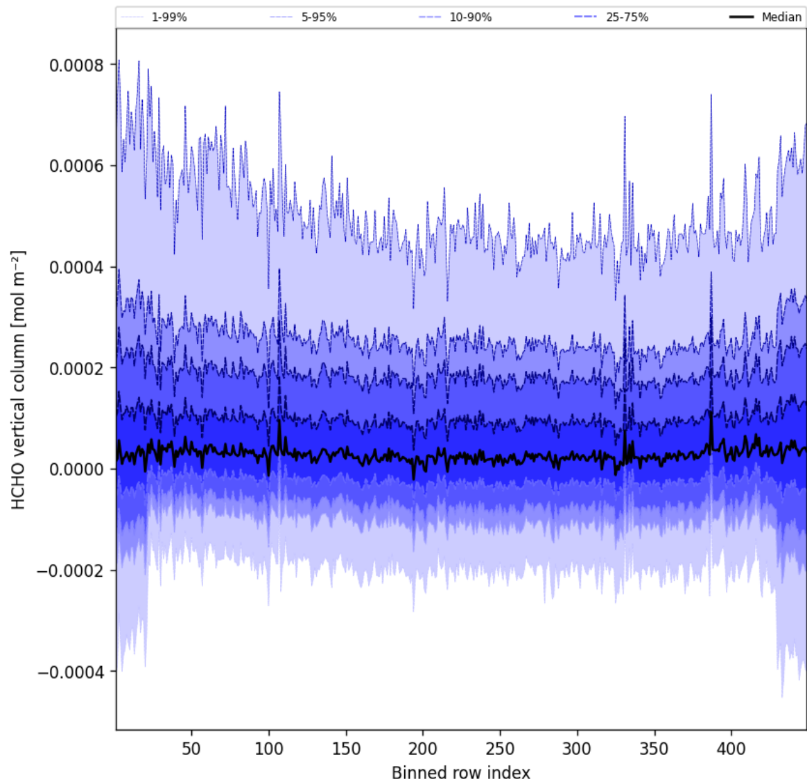
Figure 47: Along track statistics of “HCHO vertical column” for 2025-03-15 to 2025-03-15
