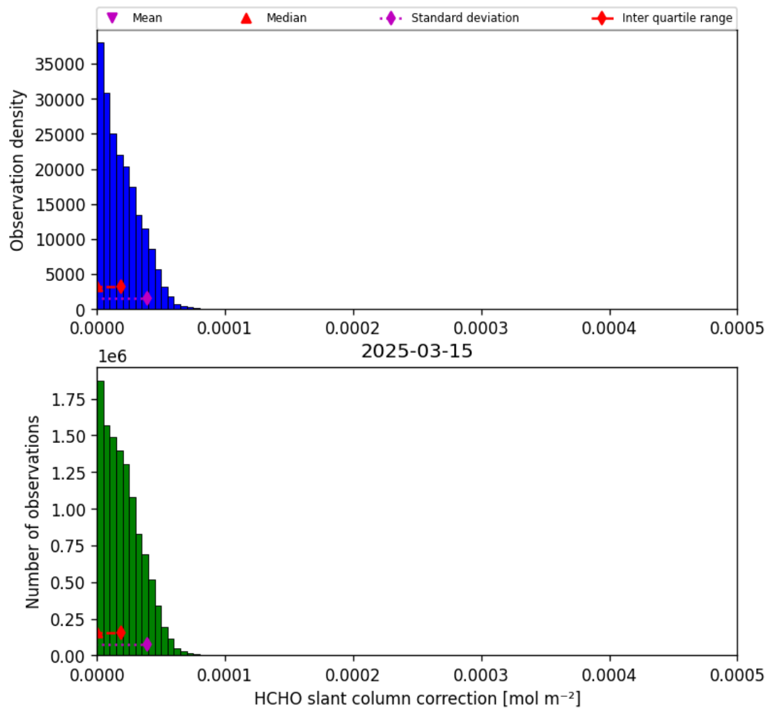
Figure 45: Histogram of “HCHO slant column correction” for 2025-03-15 to 2025-03-15
