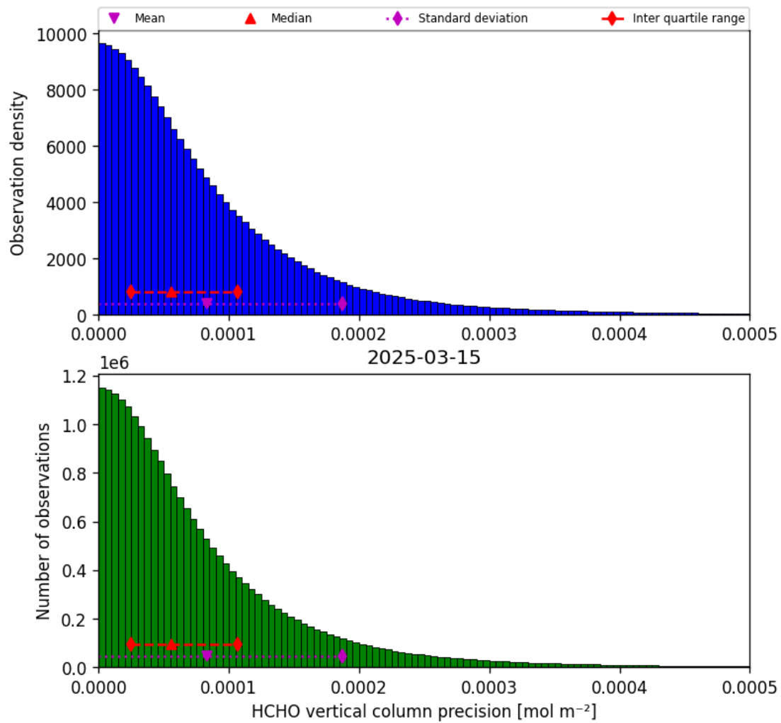
Figure 34: Histogram of “HCHO vertical column precision” for 2025-03-15 to 2025-03-15
