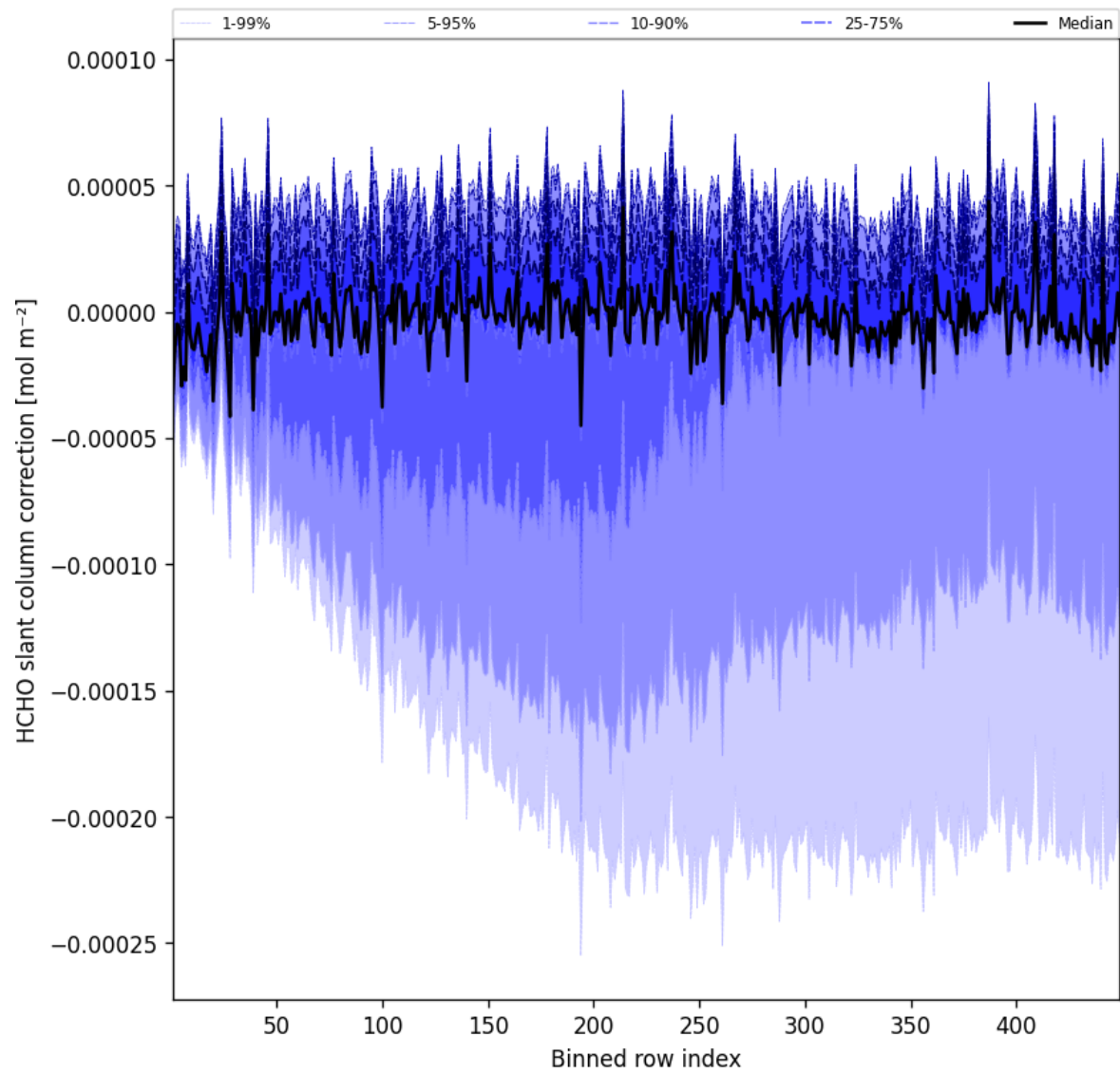
Figure 59: Along track statistics of “HCHO slant column correction” for 2025-03-15 to 2025-03-15
