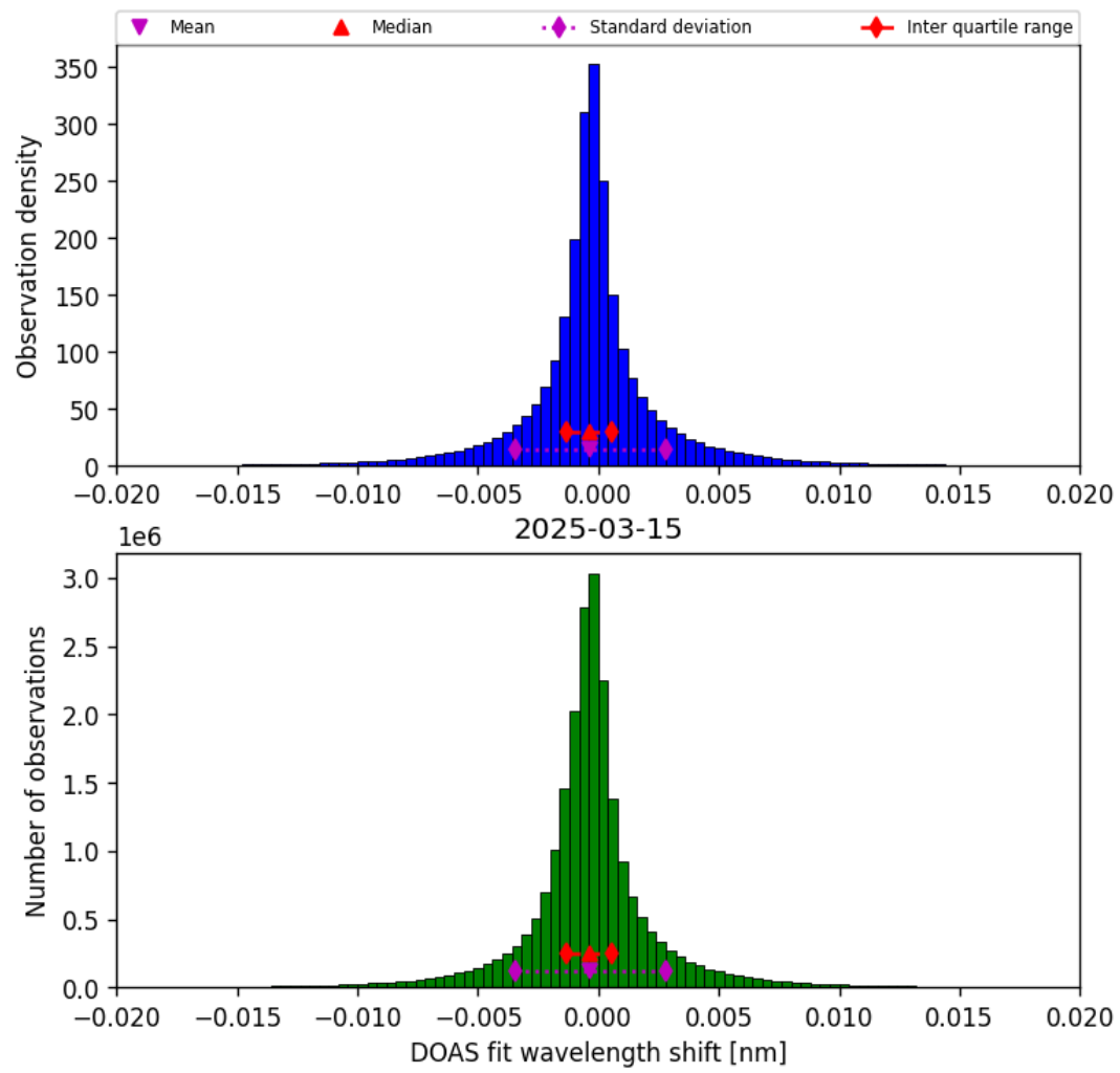
Figure 42: Histogram of “DOAS fit wavelength shift” for 2025-03-15 to 2025-03-15
