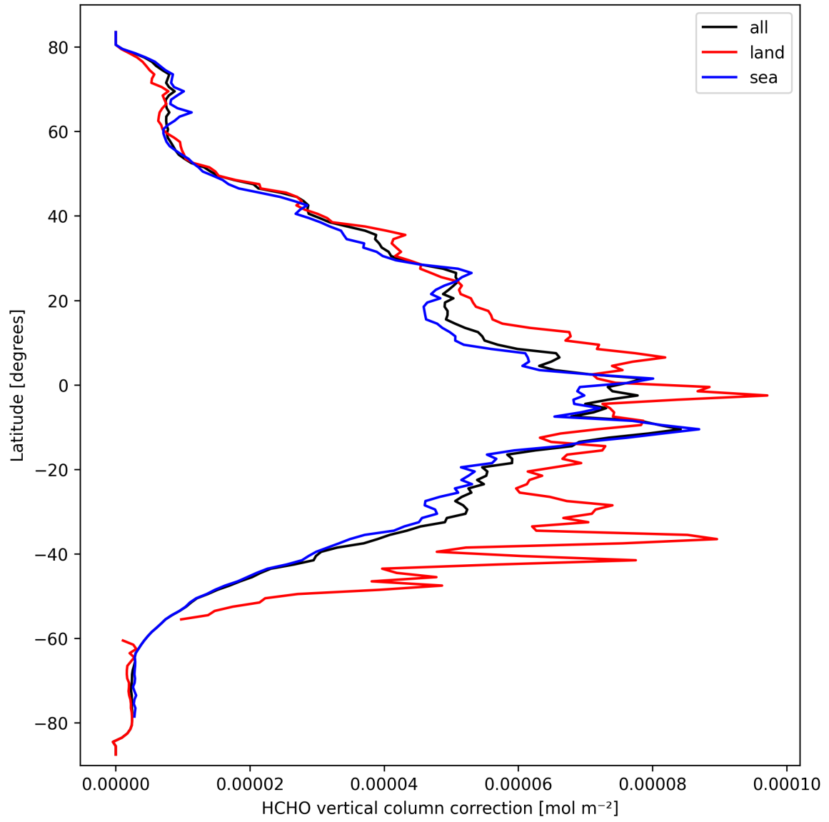
Figure 21: Zonal average of “HCHO vertical column correction” for 2025-03-15 to 2025-03-15.
