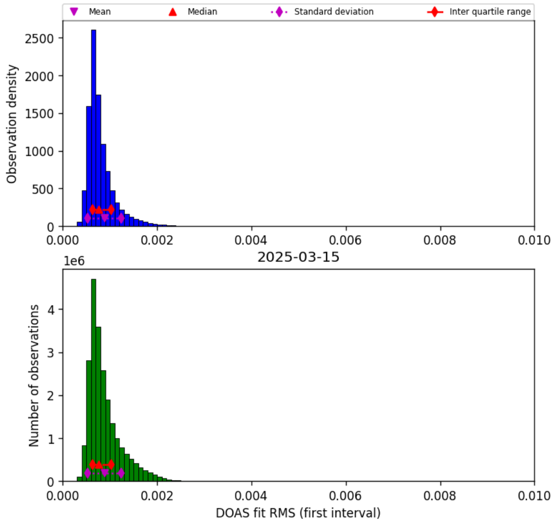
Figure 44: Histogram of “DOAS fit RMS (first interval)” for 2025-03-15 to 2025-03-15
