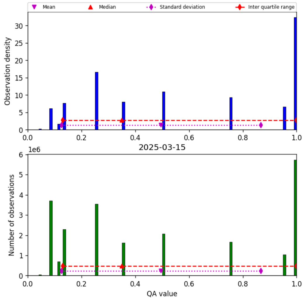
Figure 32: Histogram of “QA value” for 2025-03-15 to 2025-03-15
