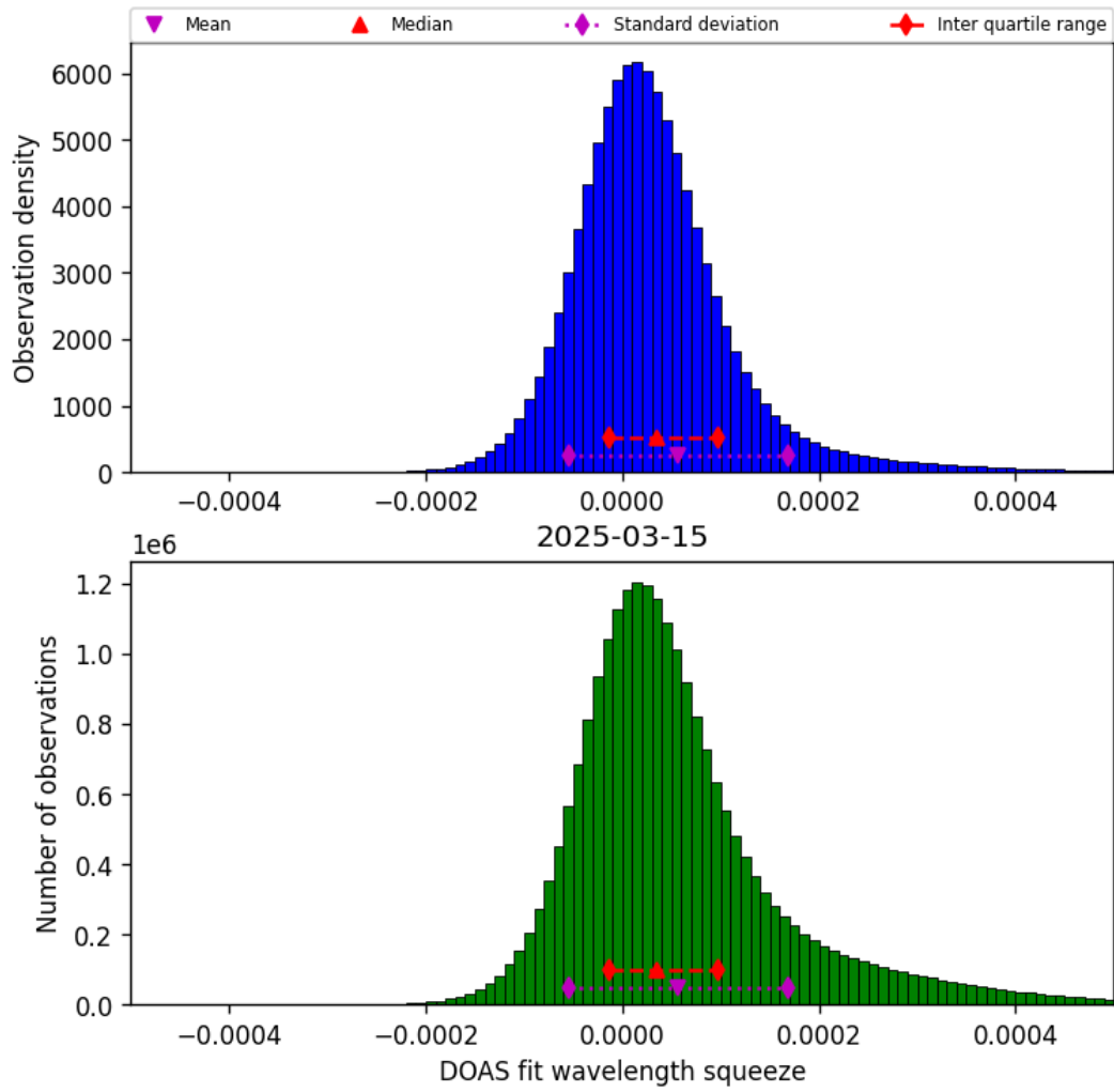
Figure 43: Histogram of “DOAS fit wavelength squeeze” for 2025-03-15 to 2025-03-15
