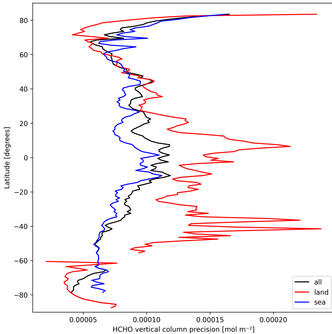
Figure 20: Zonal average of “HCHO vertical column precision” for 2025-03-15 to 2025-03-15.
