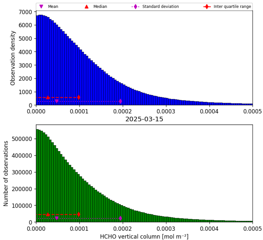
Figure 33: Histogram of “HCHO vertical column” for 2025-03-15 to 2025-03-15
