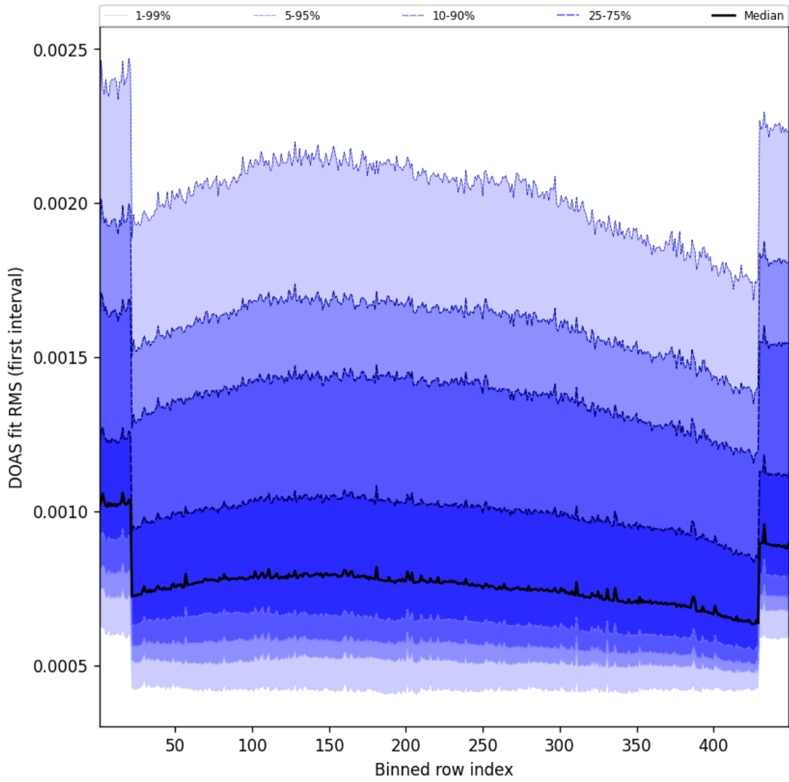
Figure 58: Along track statistics of “DOAS fit RMS (first interval)” for 2025-03-15 to 2025-03-15
