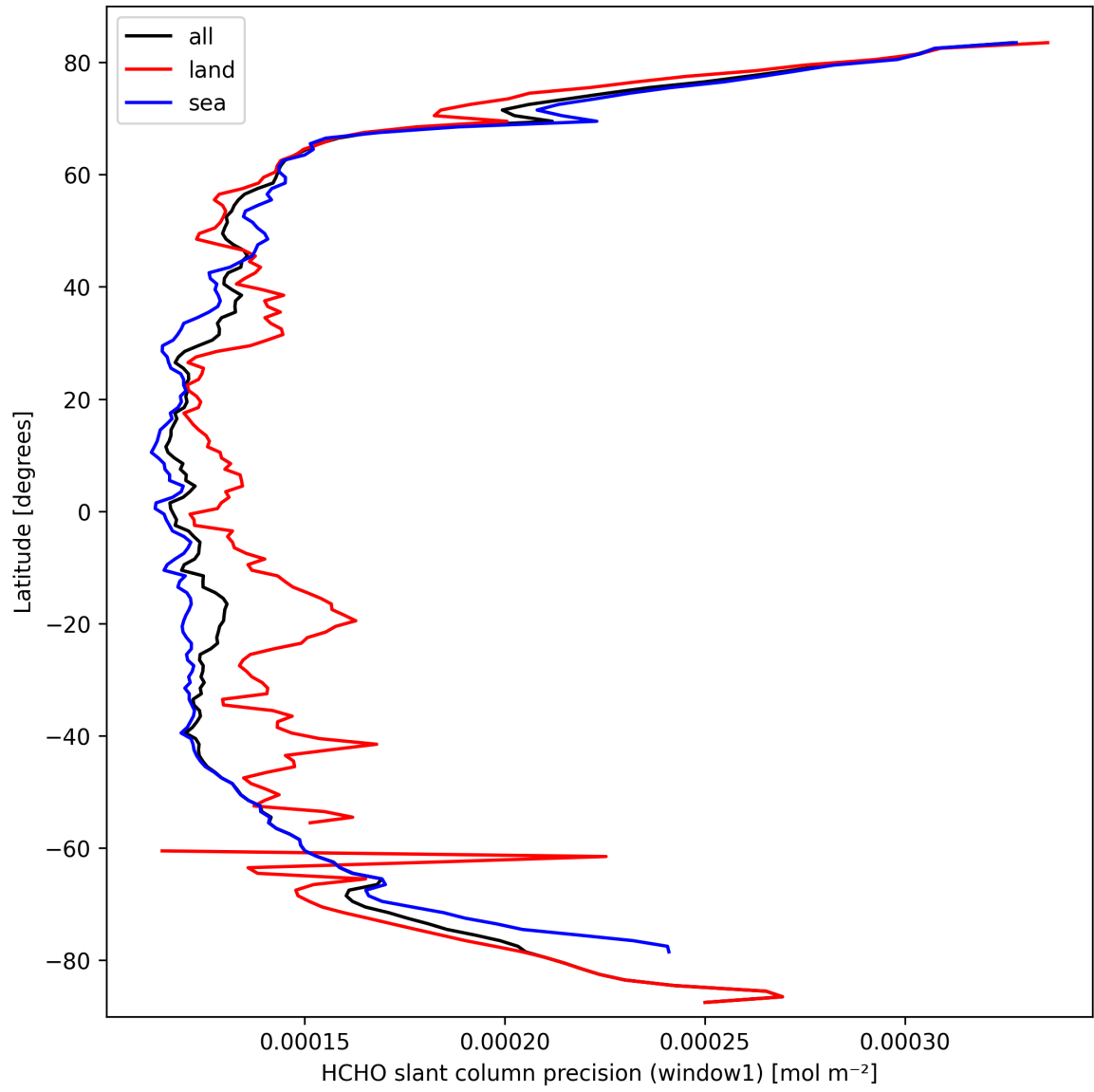
Figure 23: Zonal average of "HCHO slant column precision (window1)" for 2025-03-15 to 2025-03-15.
