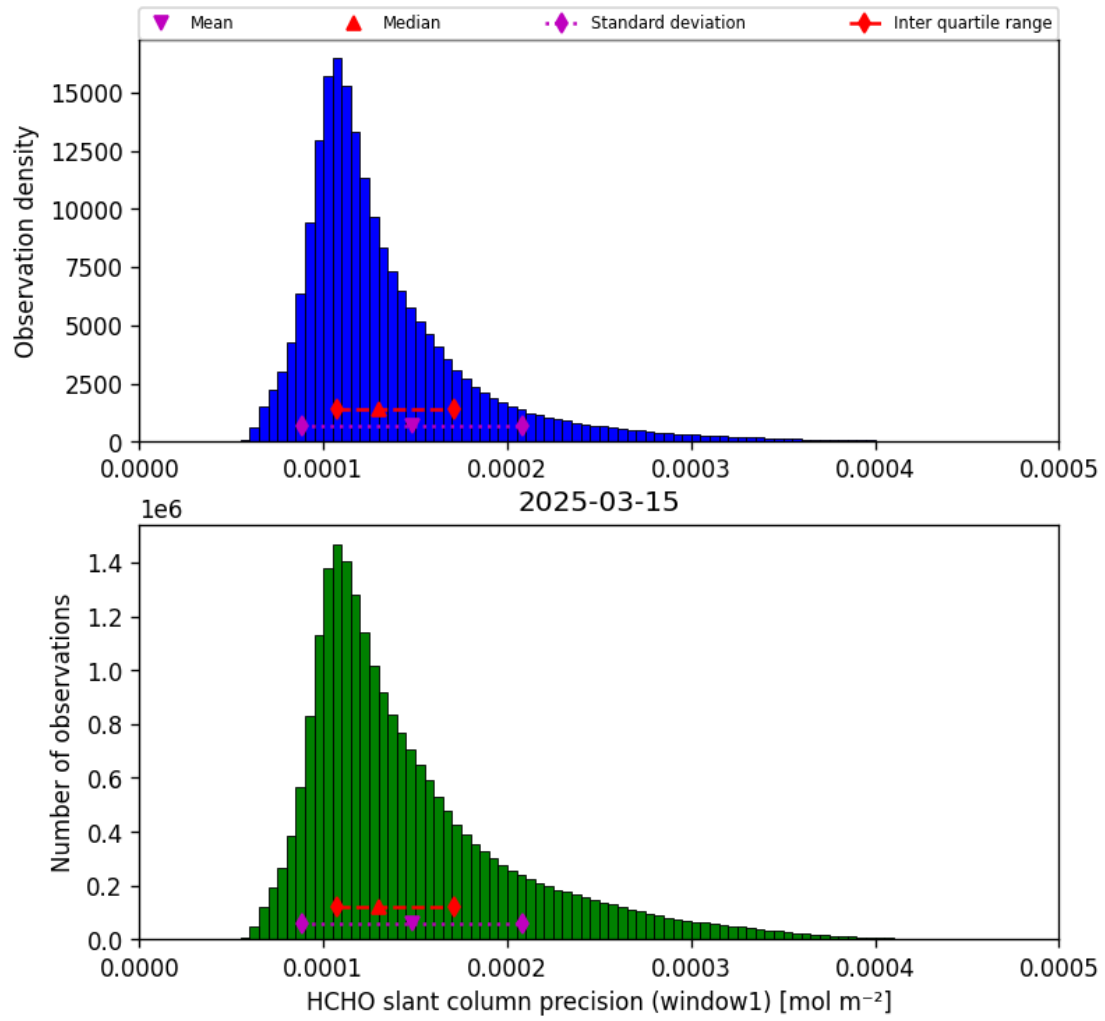
Figure 37: Histogram of “HCHO slant column precision (window1)” for 2025-03-15 to 2025-03-15
