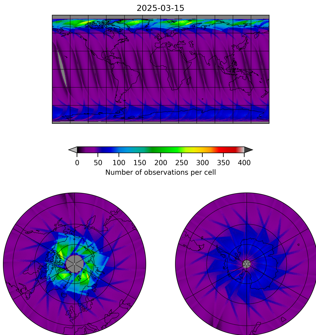
Figure 17: Map of the number of observations for 2025-03-15 to 2025-03-15
