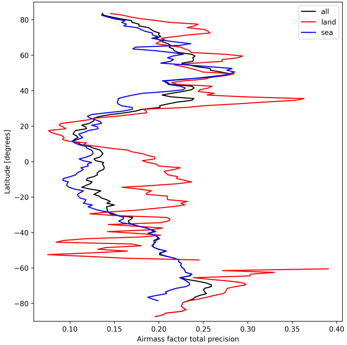
Figure 25: Zonal average of “Airmass factor total precision” for 2025-03-15 to 2025-03-15.
