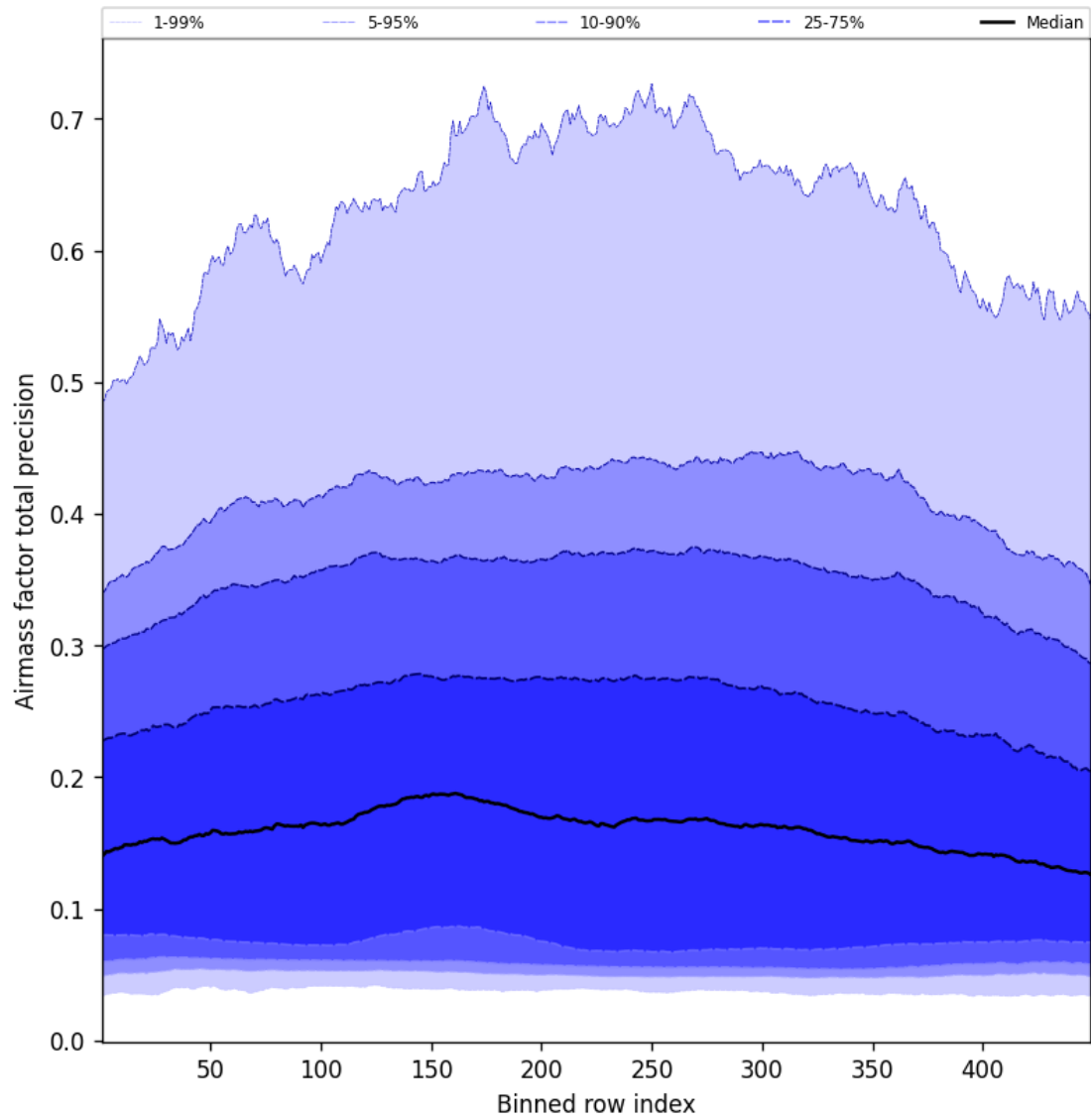
Figure 53: Along track statistics of “Airmass factor total precision” for 2025-03-15 to 2025-03-15
