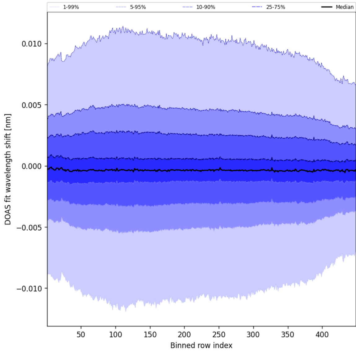
Figure 56: Along track statistics of "DOAS fit wavelength shift" for 2025-03-15 to 2025-03-15
