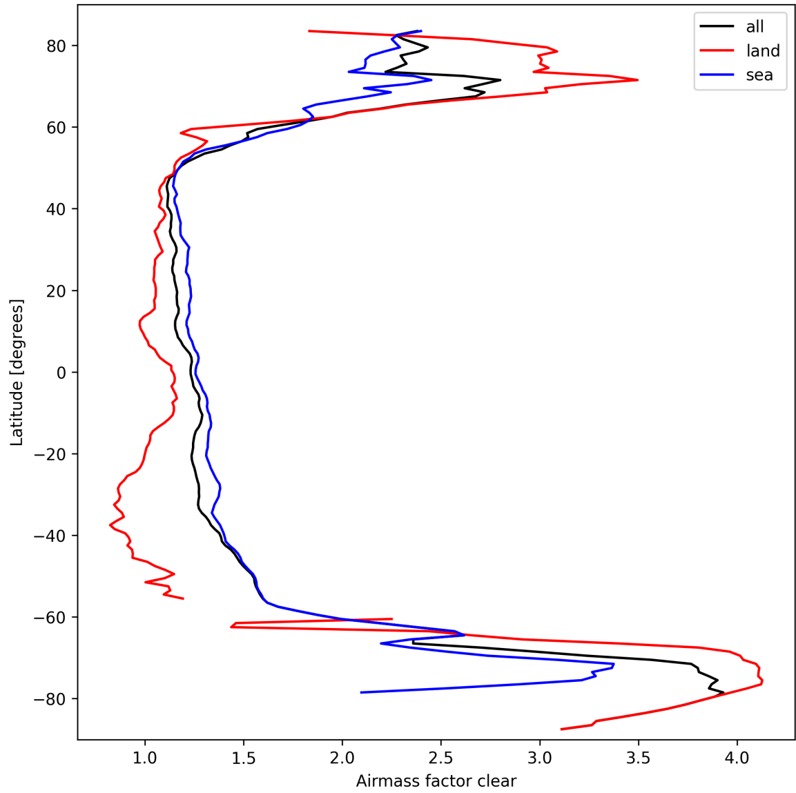
Figure 26: Zonal average of “Airmass factor clear” for 2025-03-15 to 2025-03-15.
