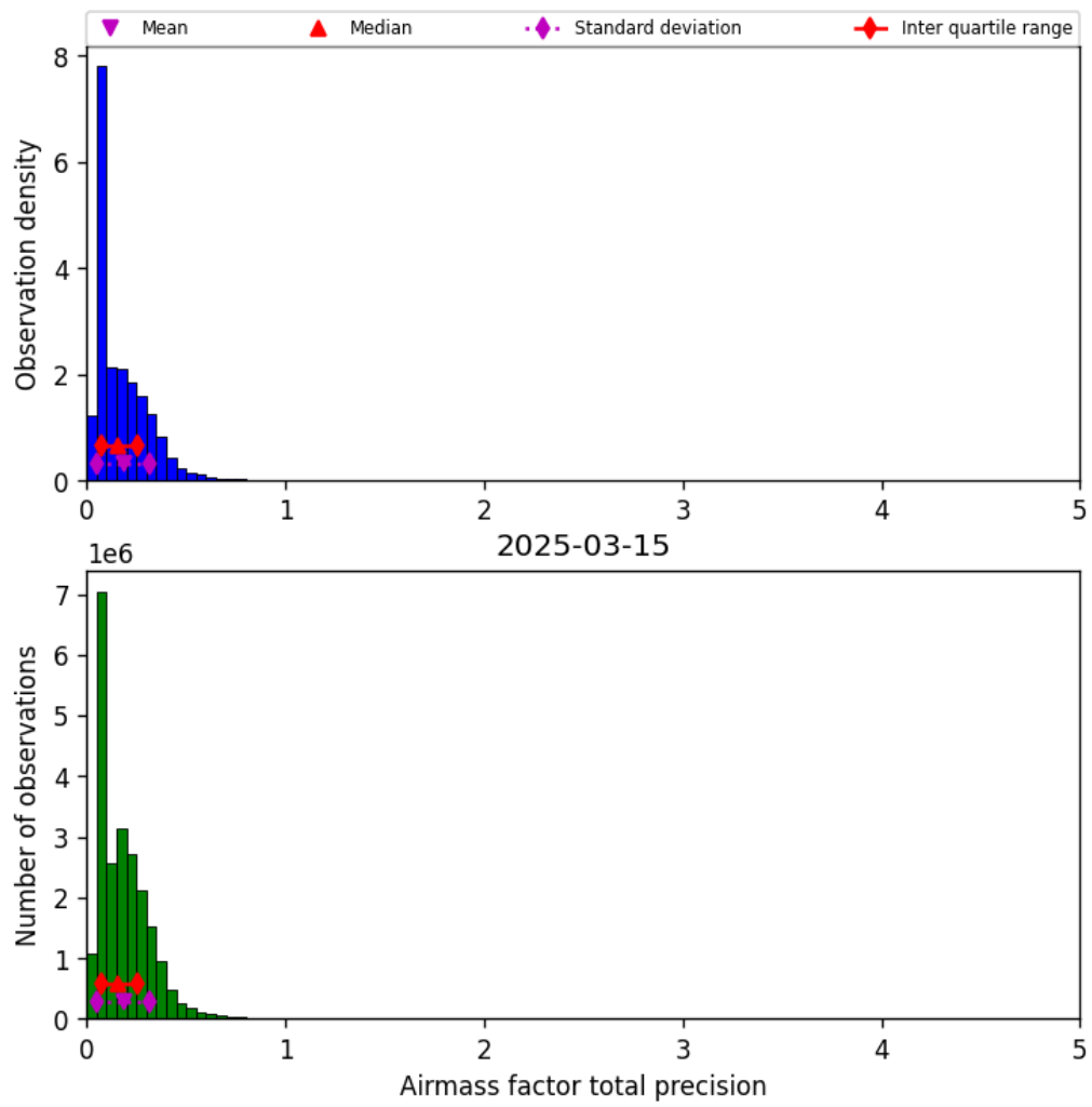
Figure 39: Histogram of “Airmass factor total precision” for 2025-03-15 to 2025-03-15
