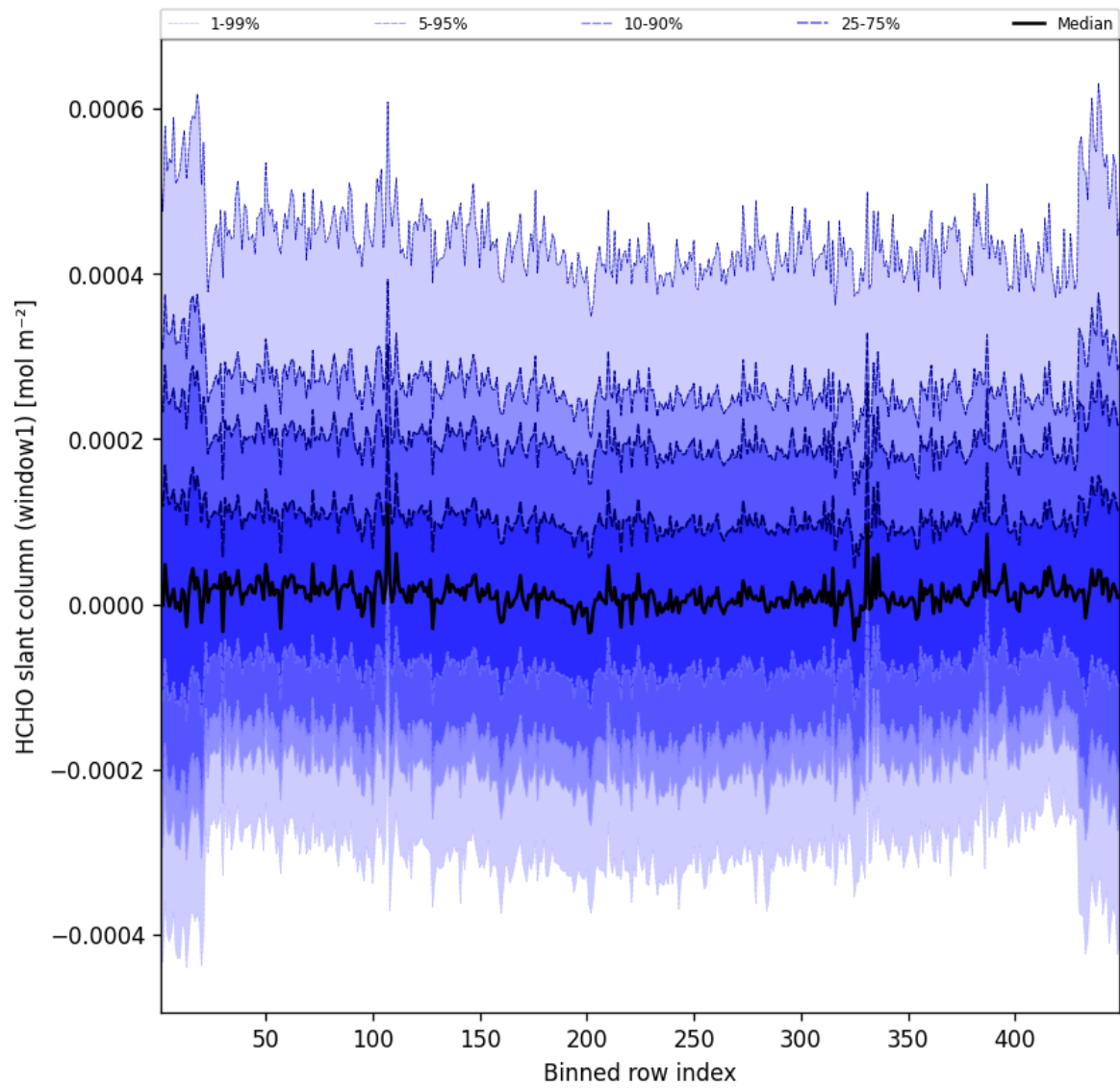
Figure 50: Along track statistics of “HCHO slant column (window1)” for 2025-03-15 to 2025-03-15
