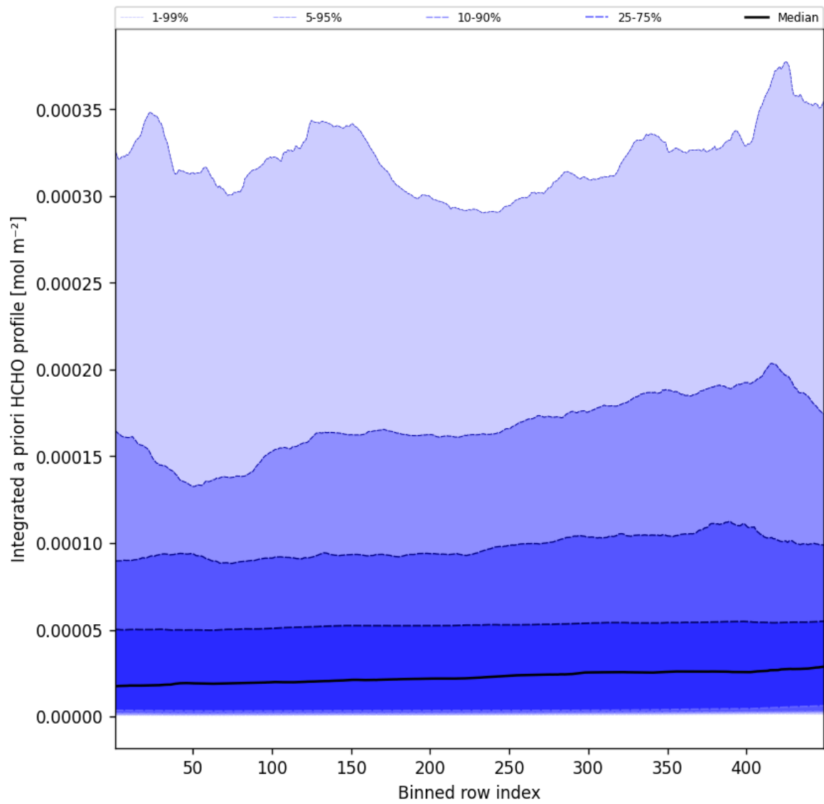
Figure 55: Along track statistics of “Integrated a priori HCHO profile” for 2025-03-15 to 2025-03-15
