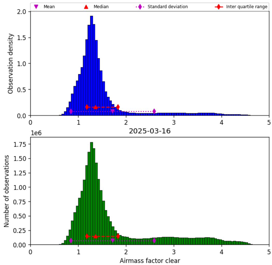
Figure 40: Histogram of “Airmass factor clear” for 2025-03-16 to 2025-03-17
