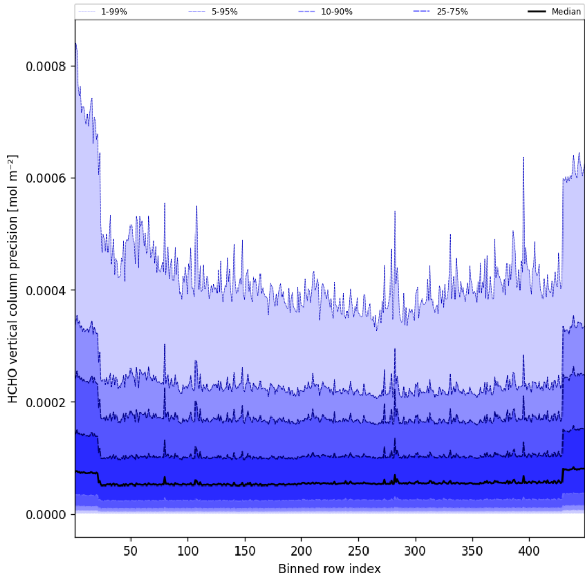
Figure 48: Along track statistics of “HCHO vertical column precision” for 2025-03-16 to 2025-03-17
