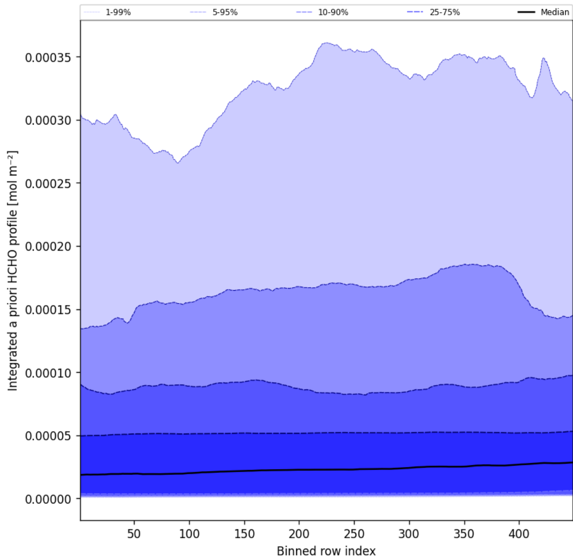
Figure 55: Along track statistics of “Integrated a priori HCHO profile” for 2025-03-16 to 2025-03-17
