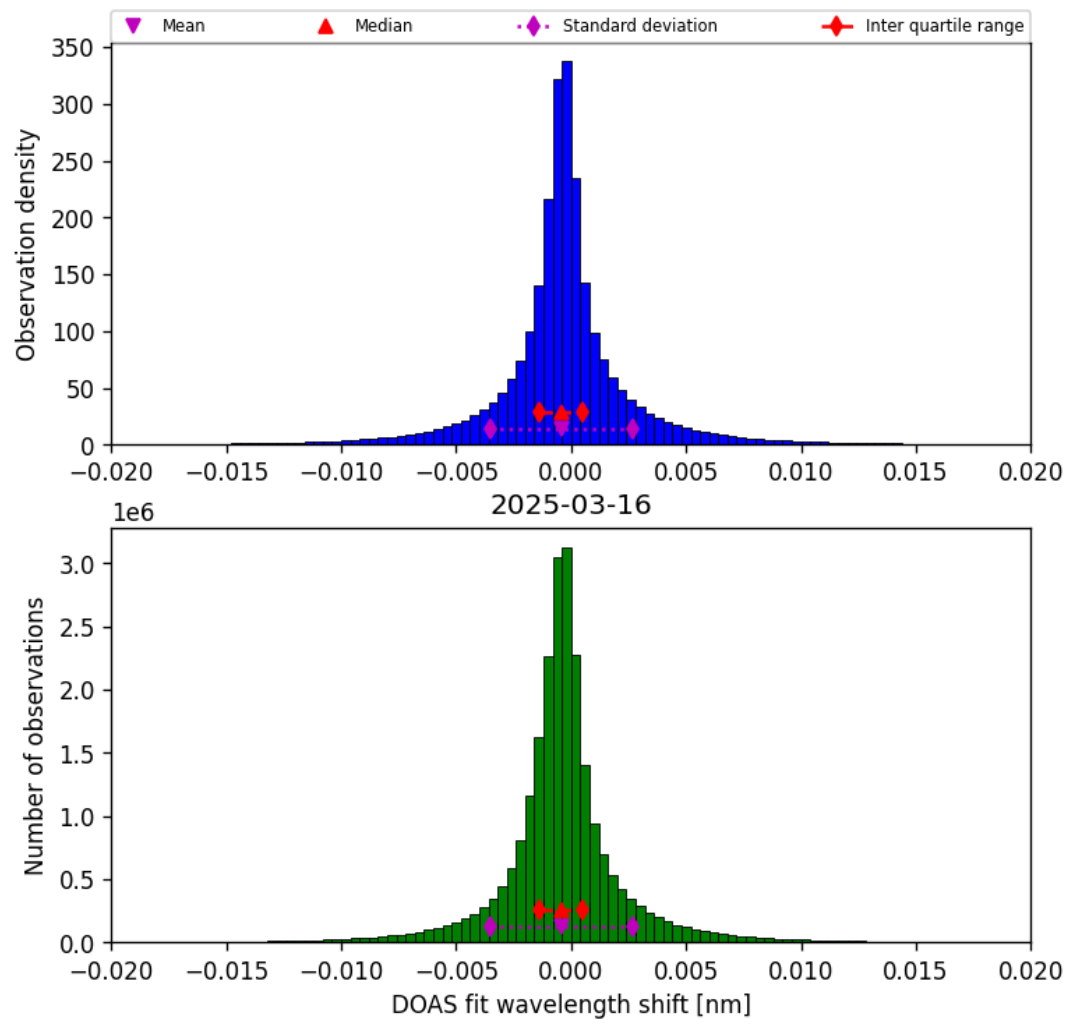
Figure 42: Histogram of “DOAS fit wavelength shift” for 2025-03-16 to 2025-03-17
