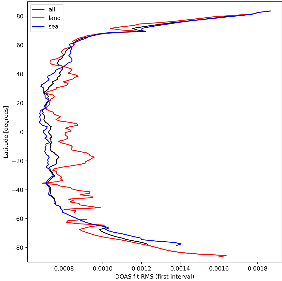
Figure 30: Zonal average of “DOAS fit RMS (first interval)” for 2025-03-16 to 2025-03-17.
