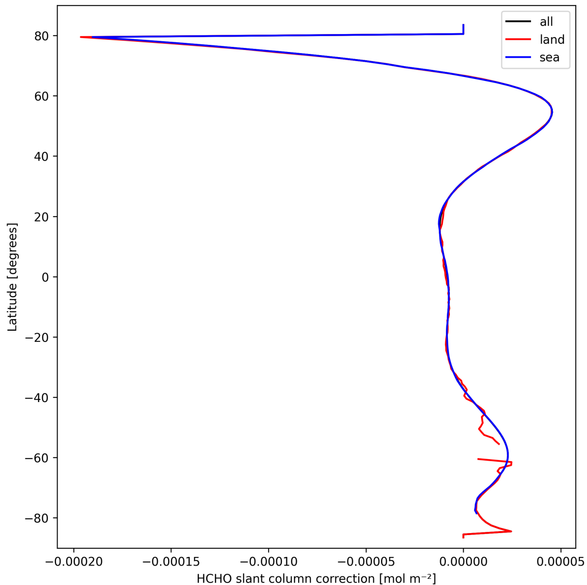
Figure 31: Zonal average of “HCHO slant column correction” for 2025-03-16 to 2025-03-17.
