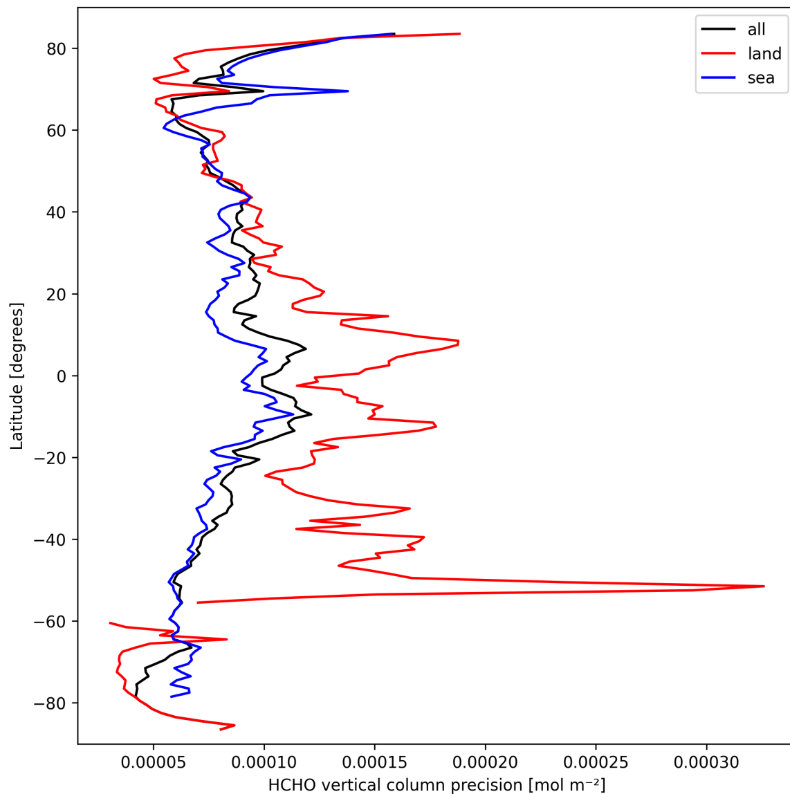
Figure 20: Zonal average of “HCHO vertical column precision” for 2025-03-16 to 2025-03-17.
