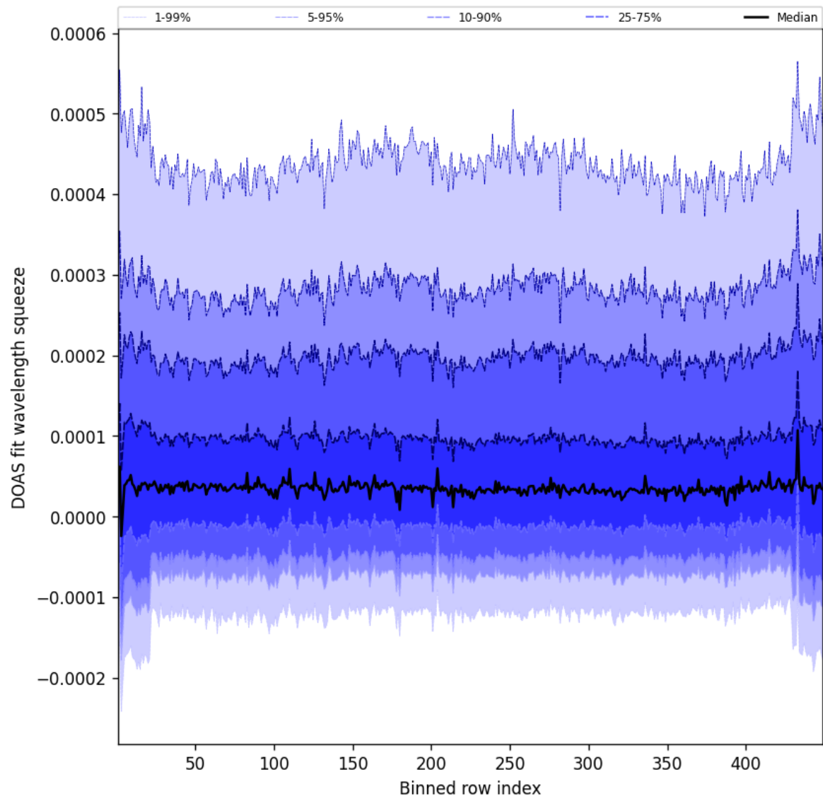
Figure 57: Along track statistics of “DOAS fit wavelength squeeze” for 2025-03-16 to 2025-03-17
