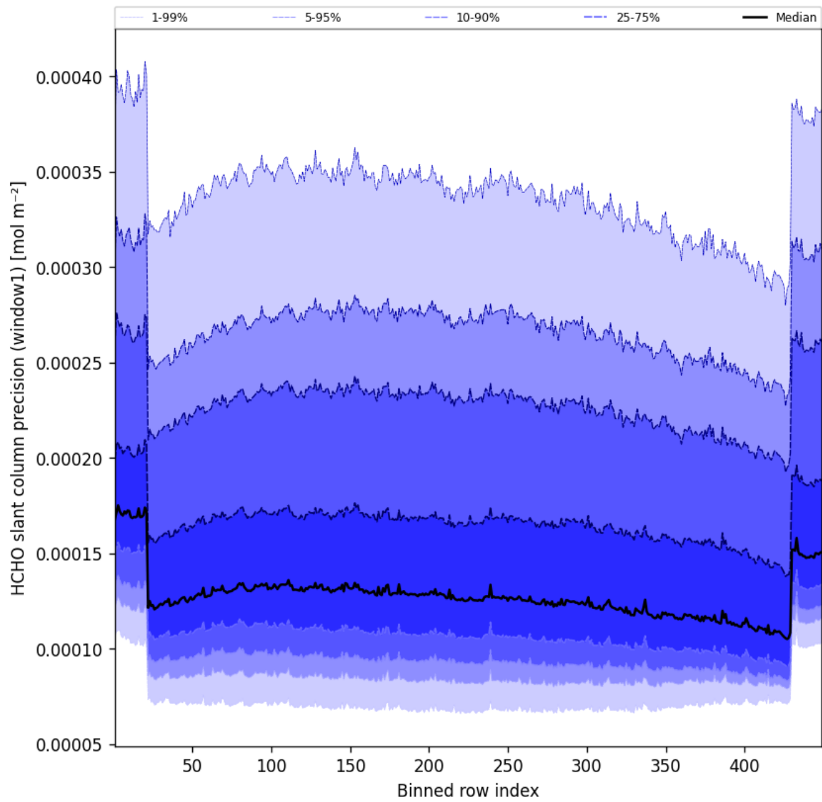
Figure 51: Along track statistics of “HCHO slant column precision (window1)” for 2025-03-16 to 2025-03-17
