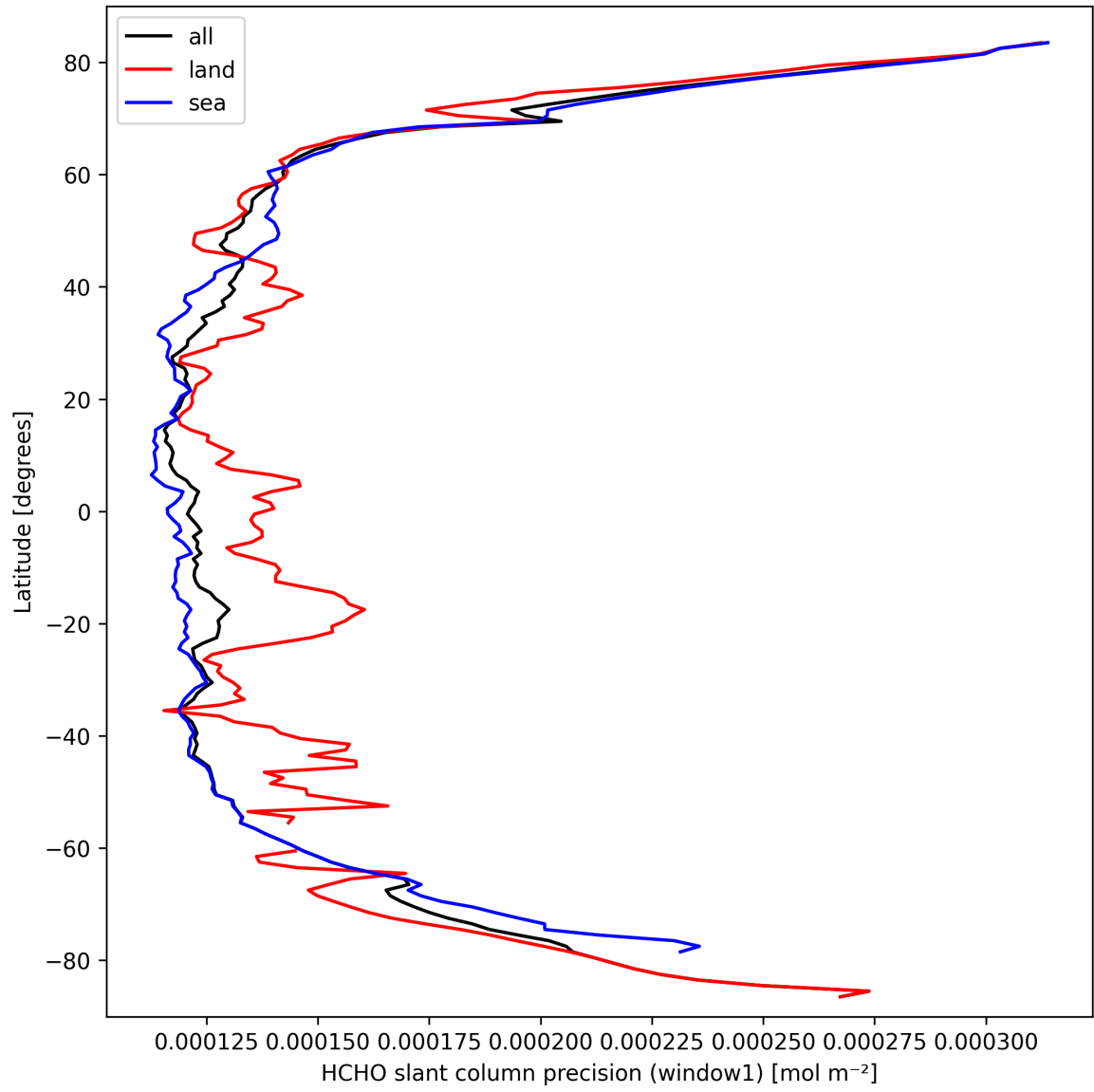
Figure 23: Zonal average of “HCHO slant column precision (window1)” for 2025-03-16 to 2025-03-17.
