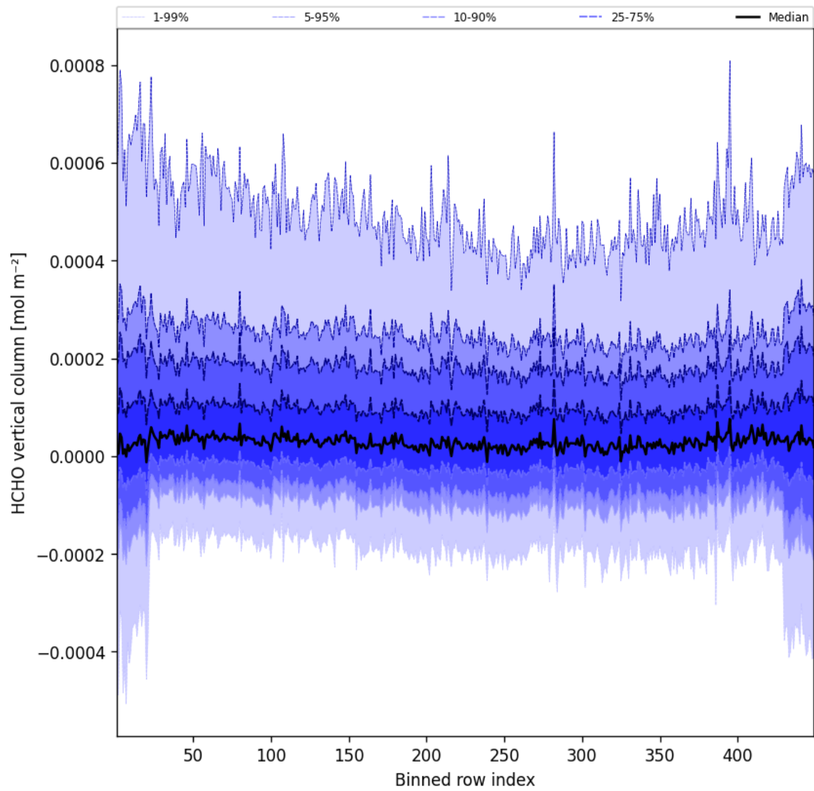
Figure 47: Along track statistics of “HCHO vertical column” for 2025-03-16 to 2025-03-17
