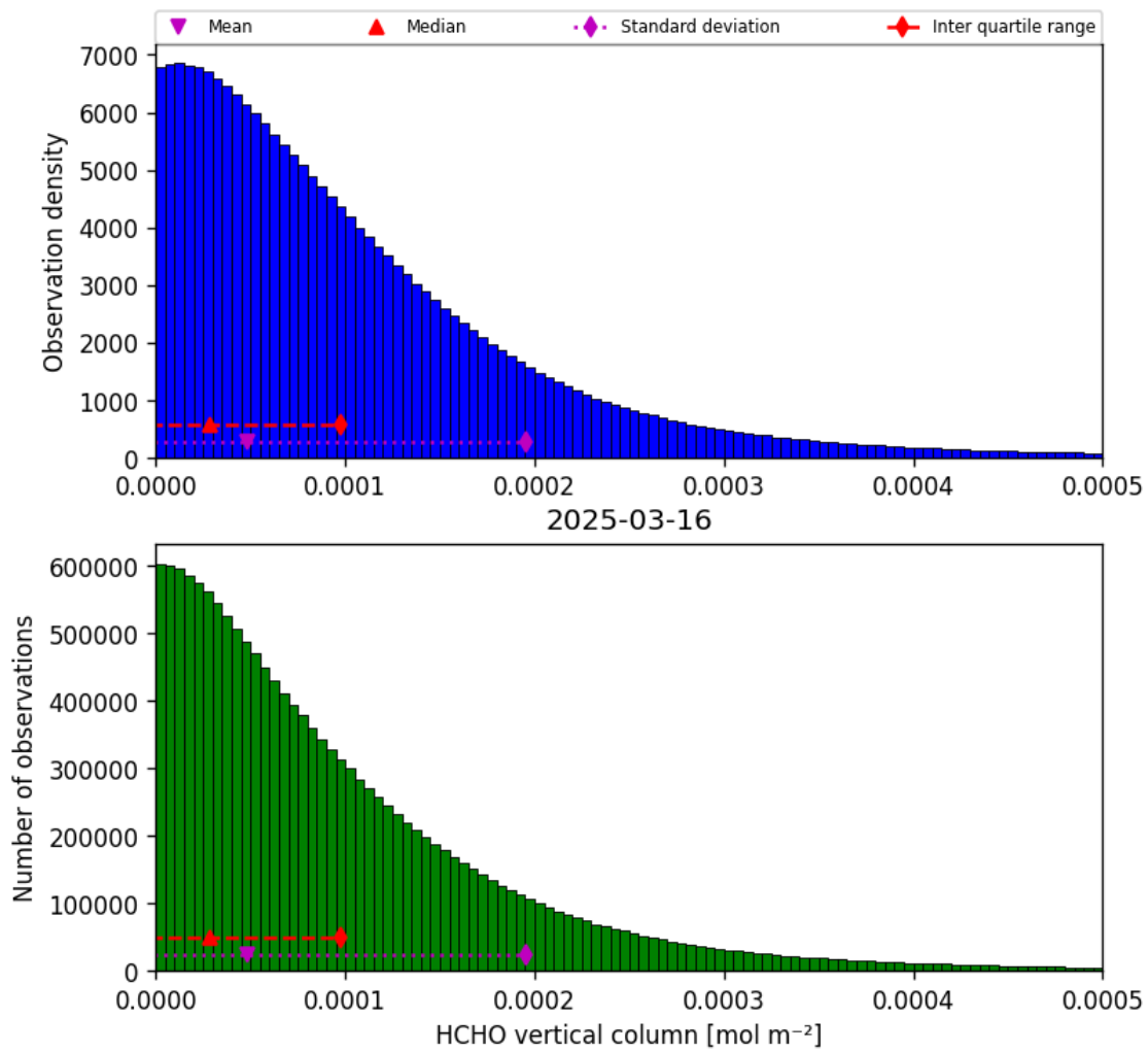
Figure 33: Histogram of “HCHO vertical column” for 2025-03-16 to 2025-03-17
