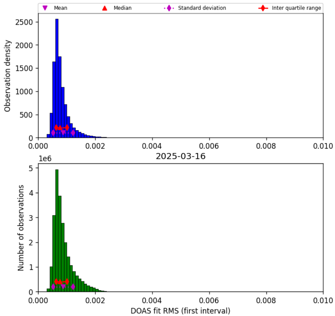
Figure 44: Histogram of “DOAS fit RMS (first interval)” for 2025-03-16 to 2025-03-17
