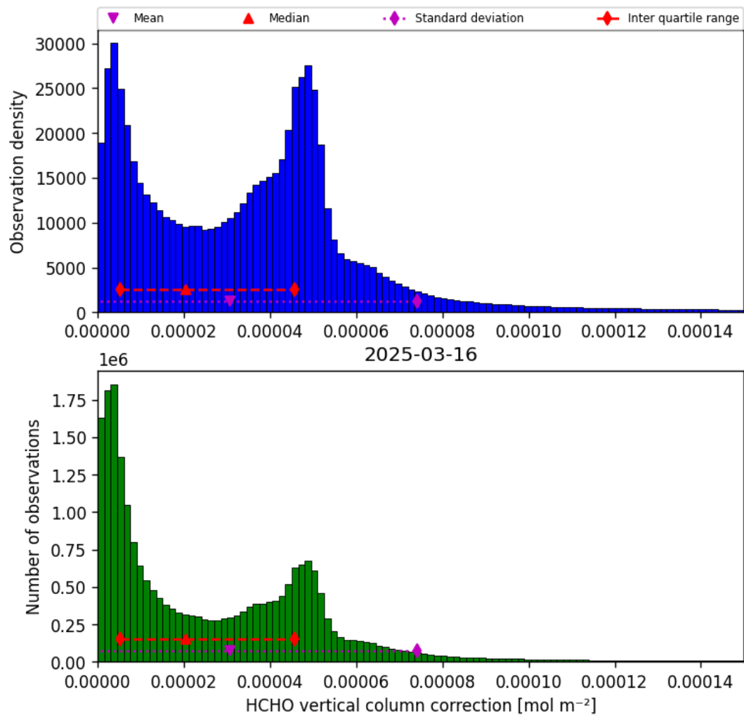
Figure 35: Histogram of “HCHO vertical column correction” for 2025-03-16 to 2025-03-17
