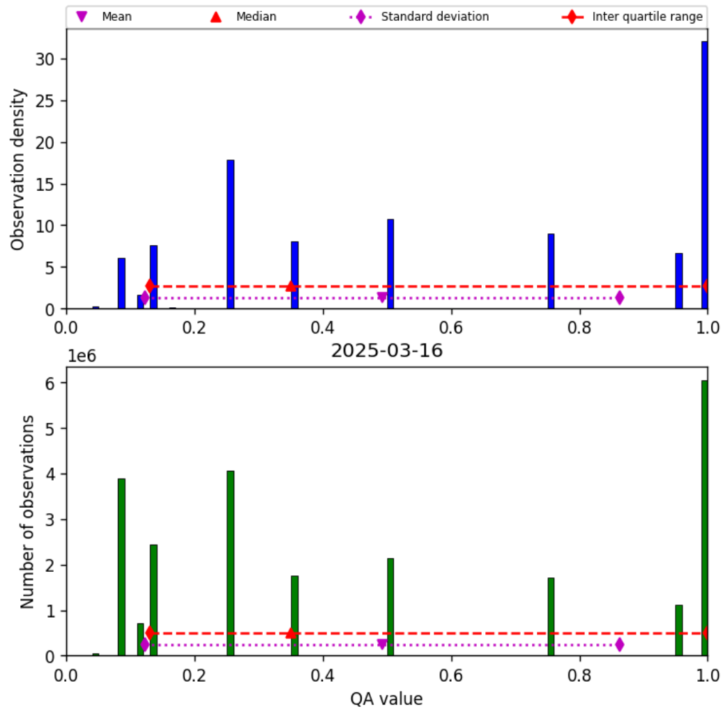
Figure 32: Histogram of “QA value” for 2025-03-16 to 2025-03-17
