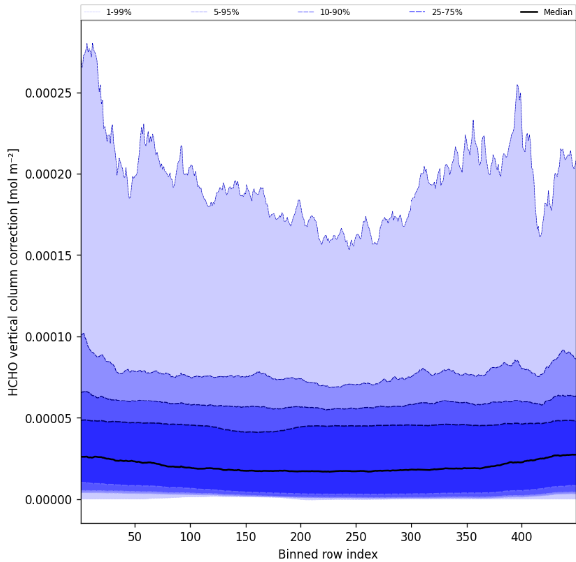
Figure 49: Along track statistics of “HCHO vertical column correction” for 2025-03-16 to 2025-03-17
