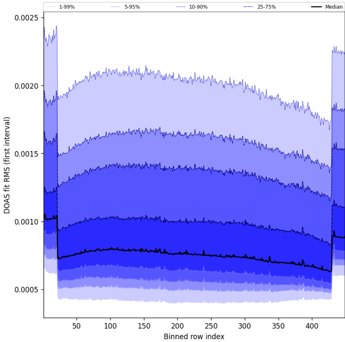
Figure 58: Along track statistics of “DOAS fit RMS (first interval)” for 2025-03-16 to 2025-03-17
