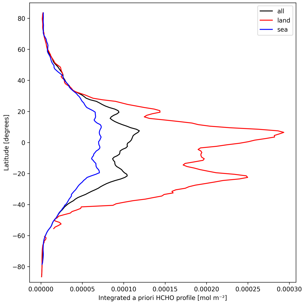
Figure 27: Zonal average of “Integrated a priori HCHO profile” for 2025-03-16 to 2025-03-17.
