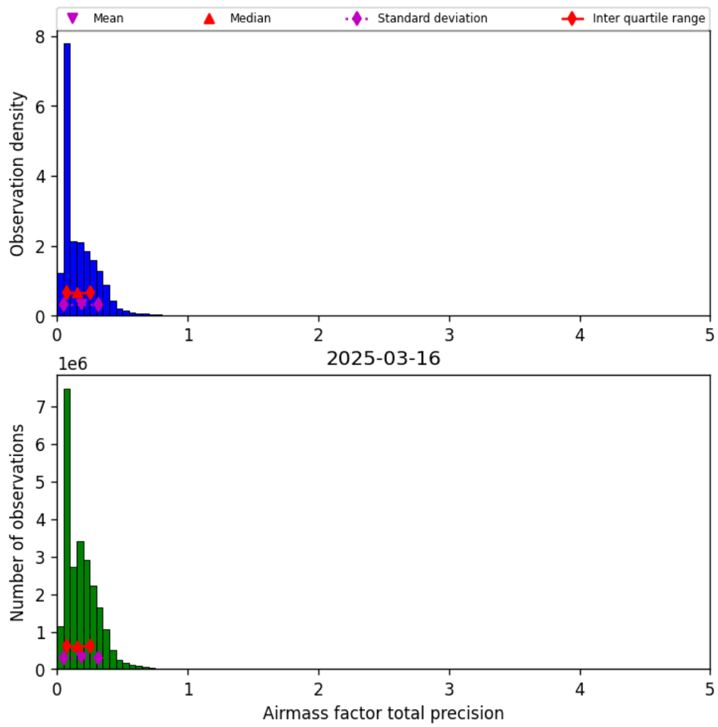
Figure 39: Histogram of “Airmass factor total precision” for 2025-03-16 to 2025-03-17
