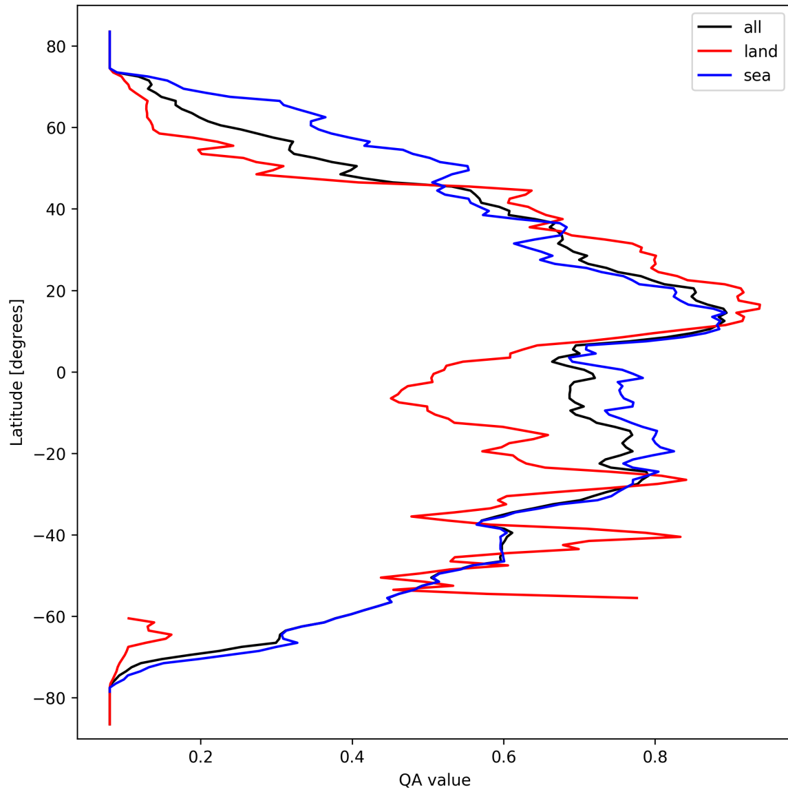
Figure 18: Zonal average of “QA value” for 2025-03-16 to 2025-03-17.
