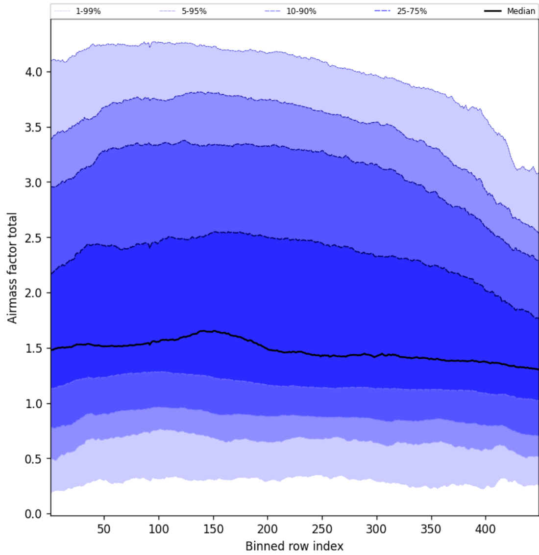
Figure 52: Along track statistics of “Airmass factor total” for 2025-03-16 to 2025-03-17
