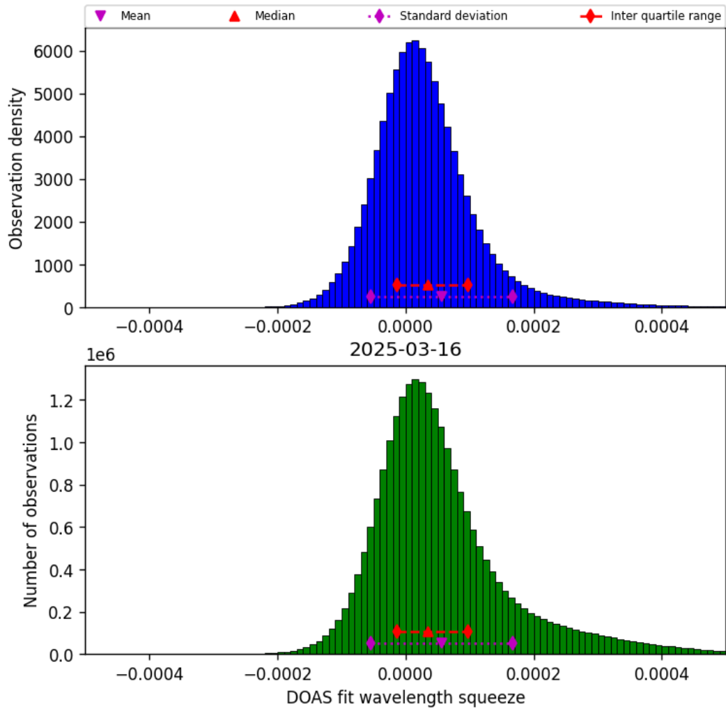
Figure 43: Histogram of “DOAS fit wavelength squeeze” for 2025-03-16 to 2025-03-17
