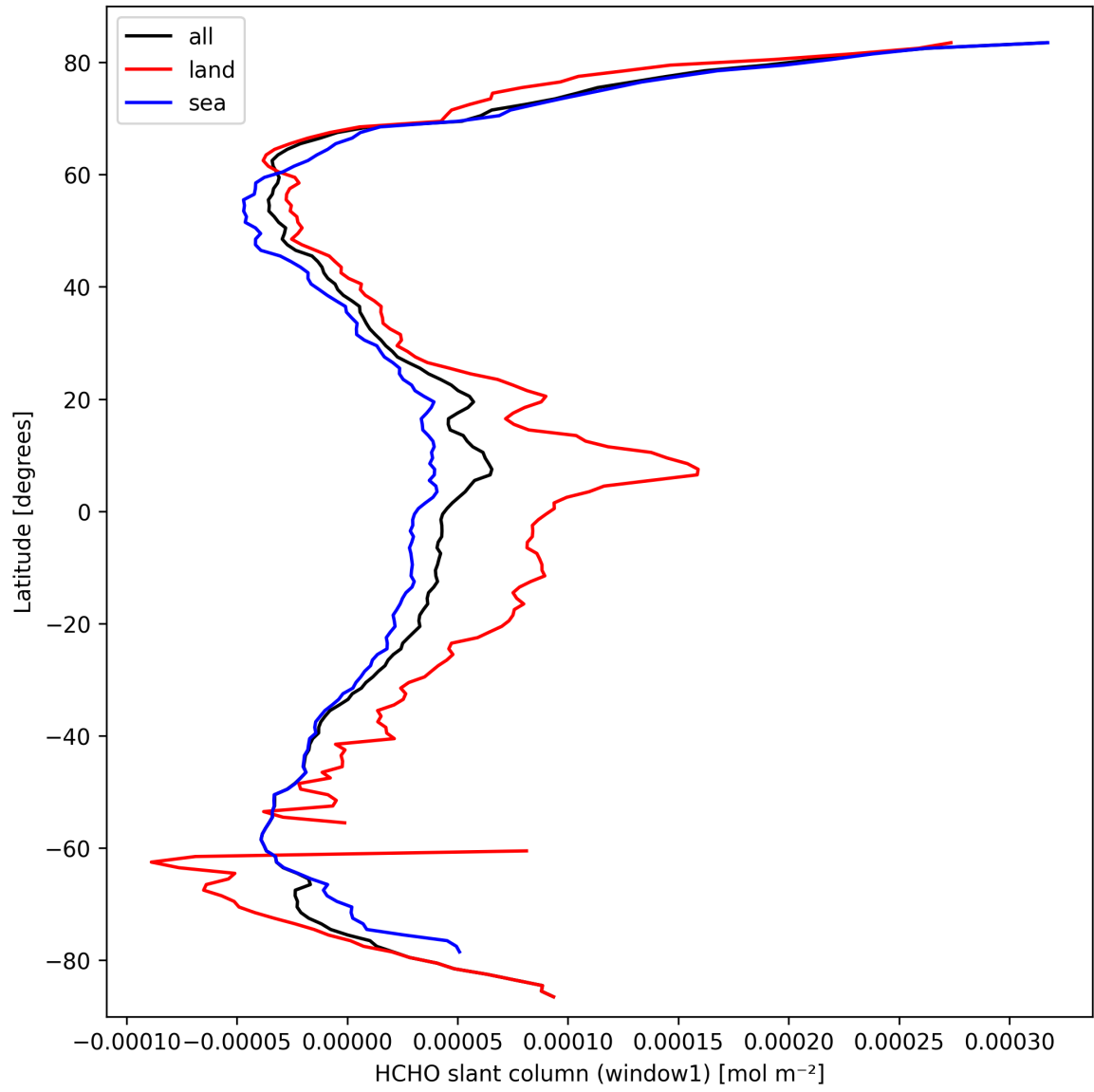
Figure 22: Zonal average of “HCHO slant column (window1)” for 2025-03-16 to 2025-03-17.
