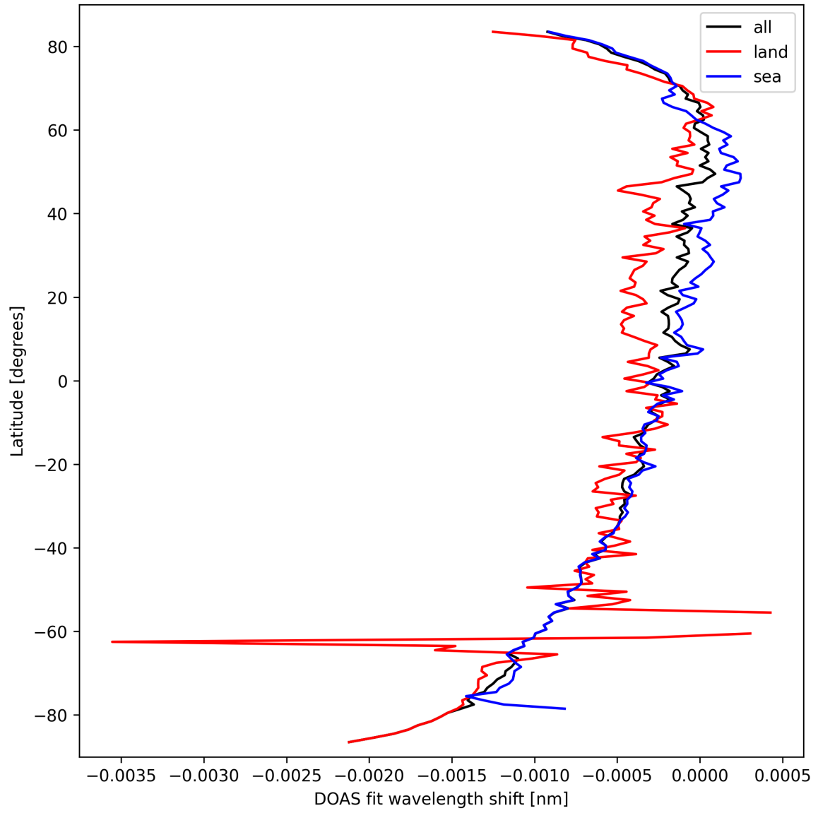
Figure 28: Zonal average of “DOAS fit wavelength shift” for 2025-03-16 to 2025-03-17.
