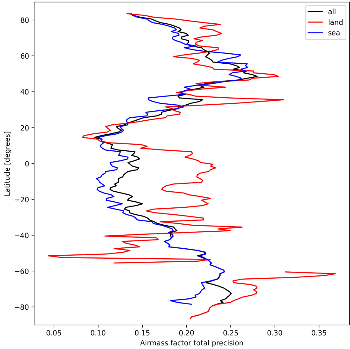
Figure 25: Zonal average of “Airmass factor total precision” for 2025-03-16 to 2025-03-17.
