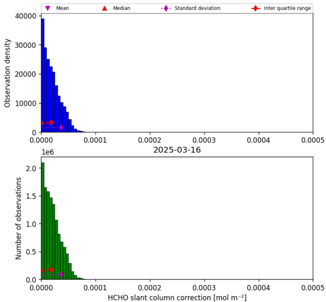
Figure 45: Histogram of “HCHO slant column correction” for 2025-03-16 to 2025-03-17
