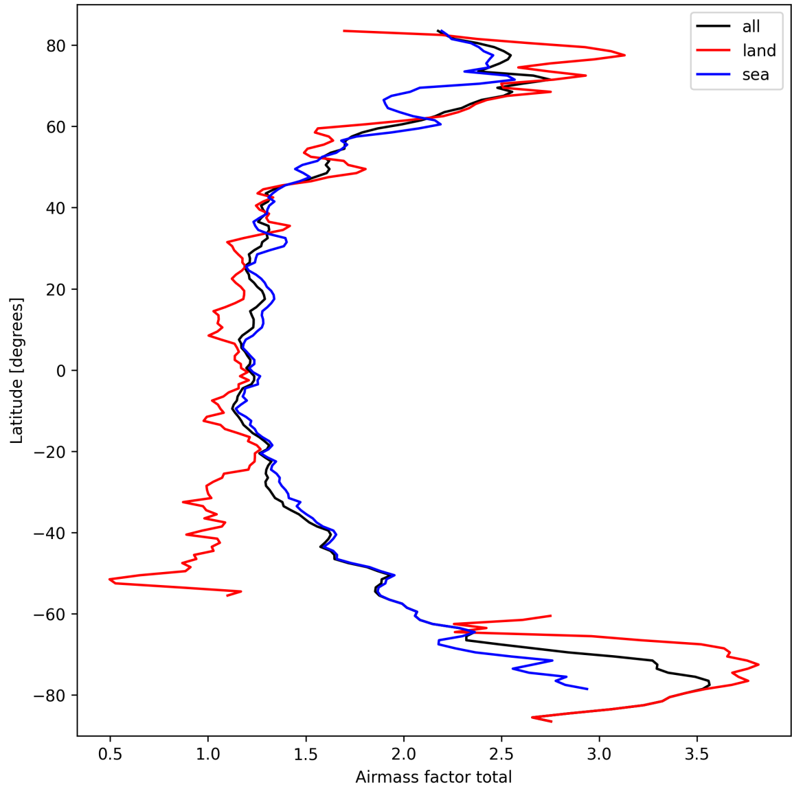
Figure 24: Zonal average of “Airmass factor total” for 2025-03-16 to 2025-03-17.
