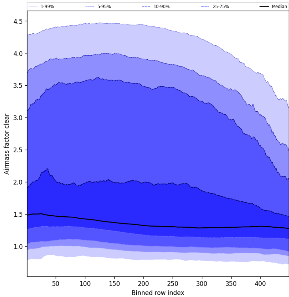
Figure 54: Along track statistics of “Airmass factor clear” for 2025-03-16 to 2025-03-17
