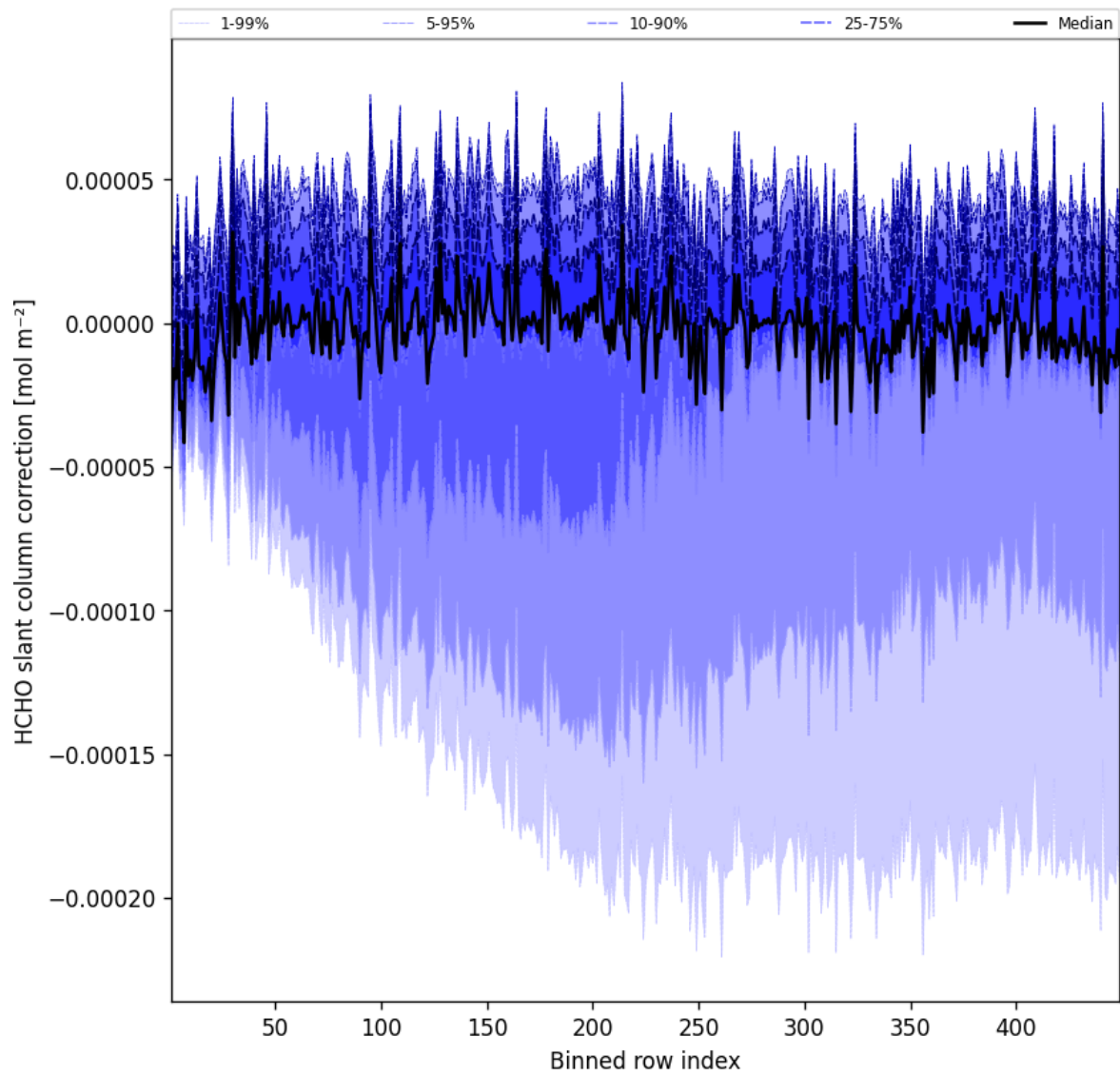
Figure 59: Along track statistics of “HCHO slant column correction” for 2025-03-16 to 2025-03-17
