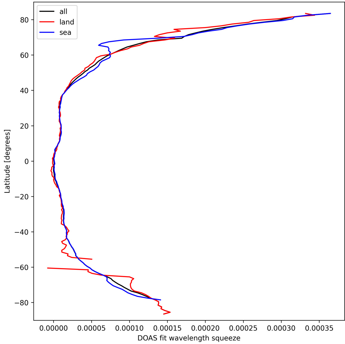
Figure 29: Zonal average of “DOAS fit wavelength squeeze” for 2025-03-16 to 2025-03-17.
