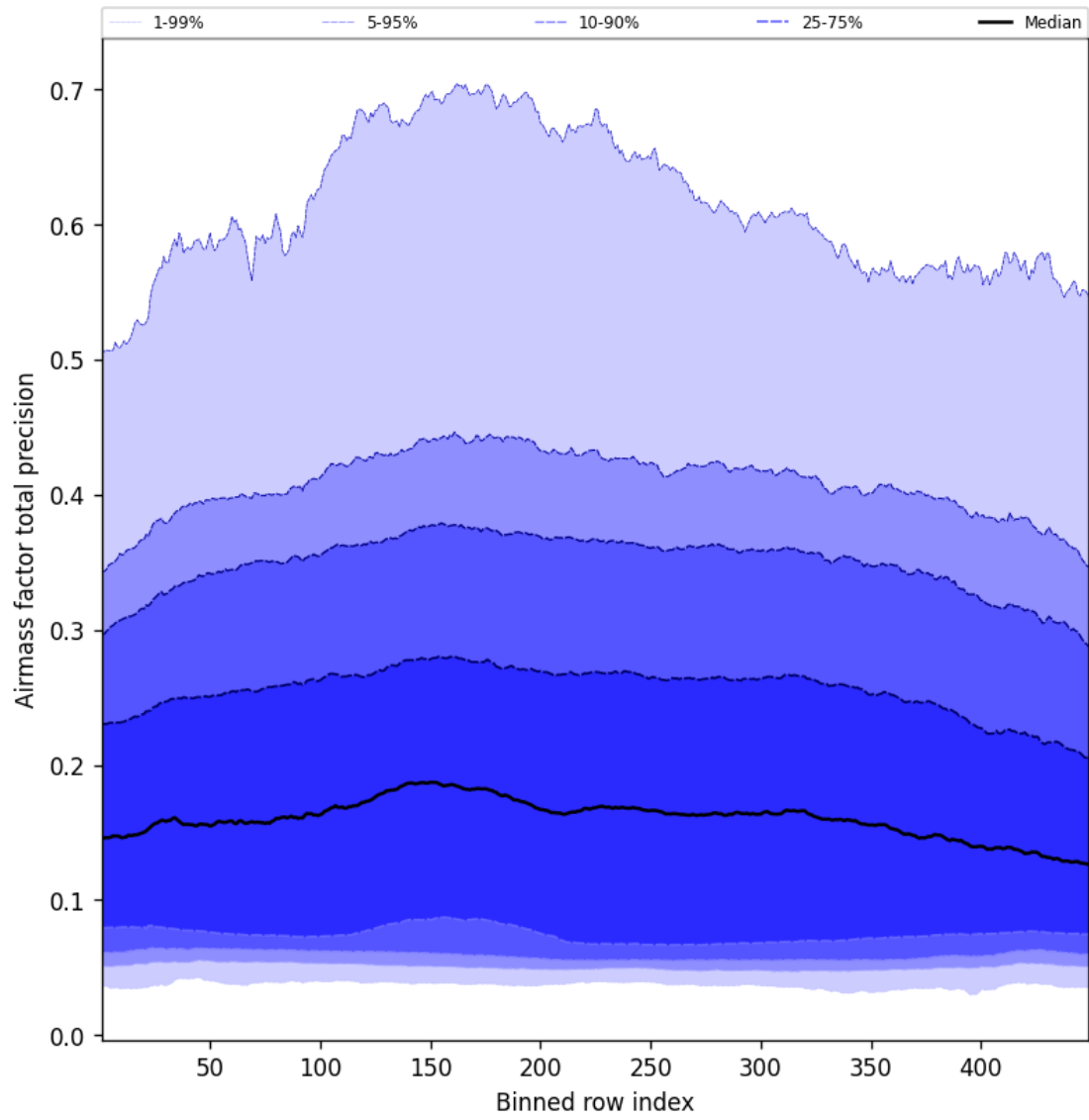
Figure 53: Along track statistics of “Airmass factor total precision” for 2025-03-16 to 2025-03-17
