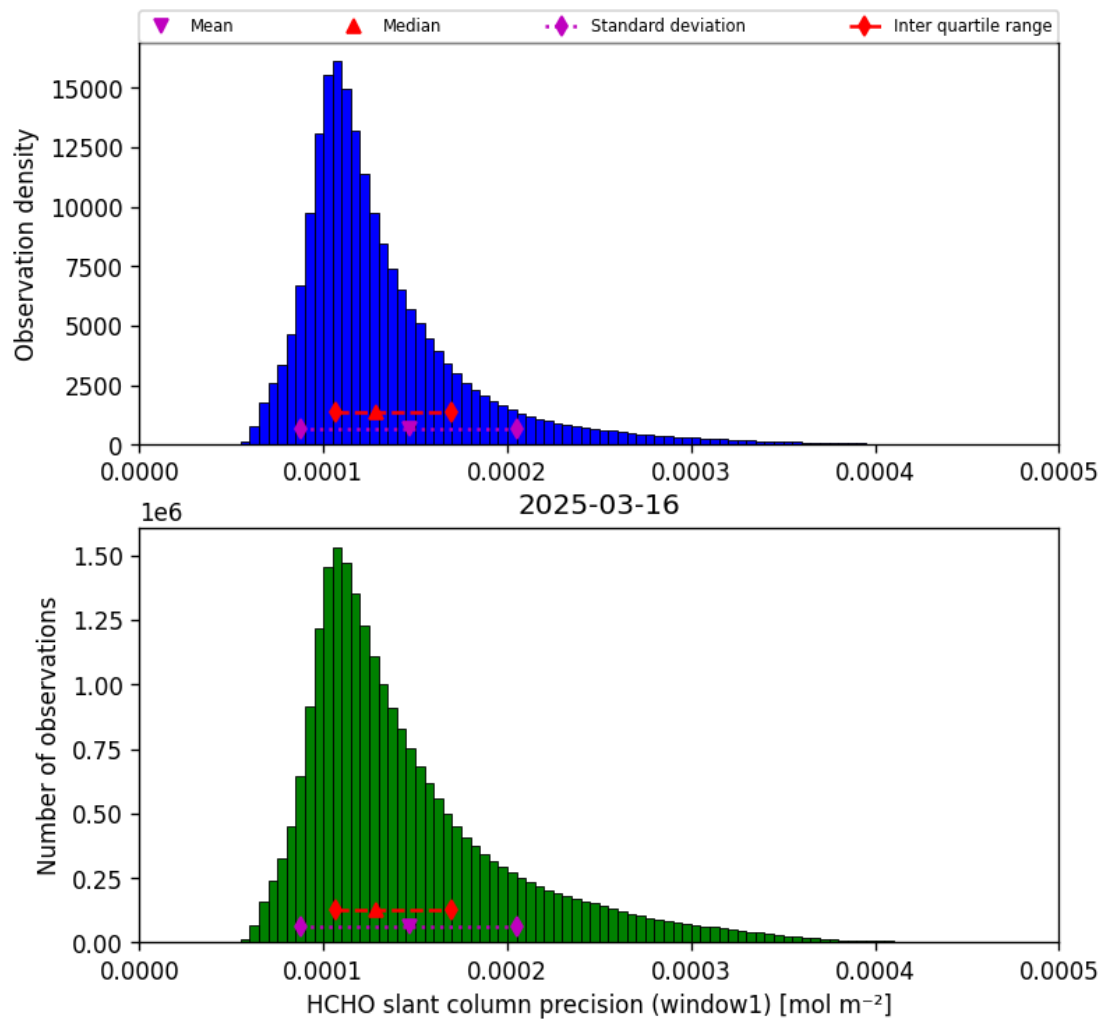
Figure 37: Histogram of “HCHO slant column precision (window1)” for 2025-03-16 to 2025-03-17
