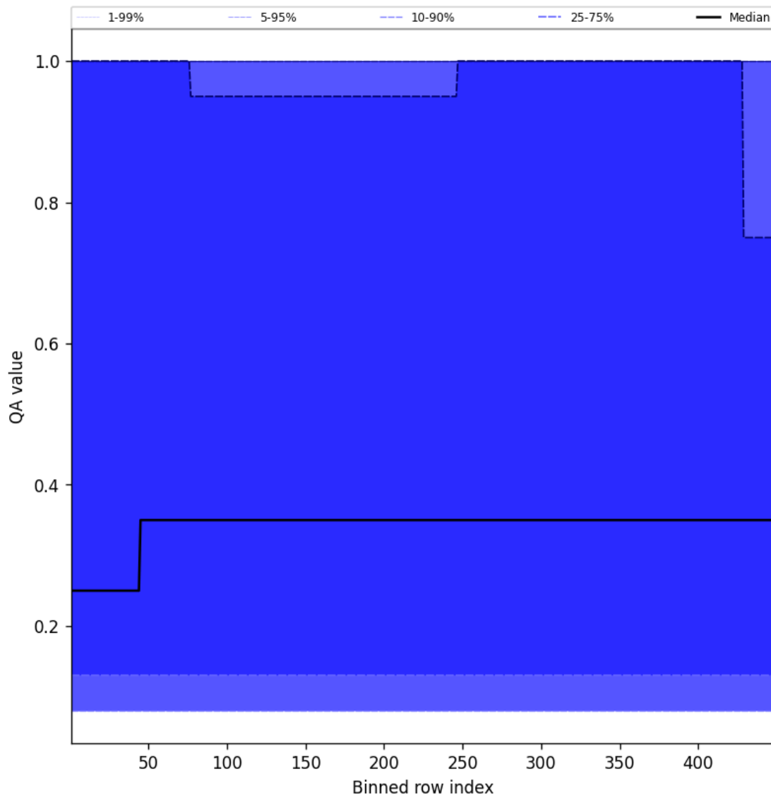
Figure 46: Along track statistics of “QA value” for 2025-03-16 to 2025-03-17
