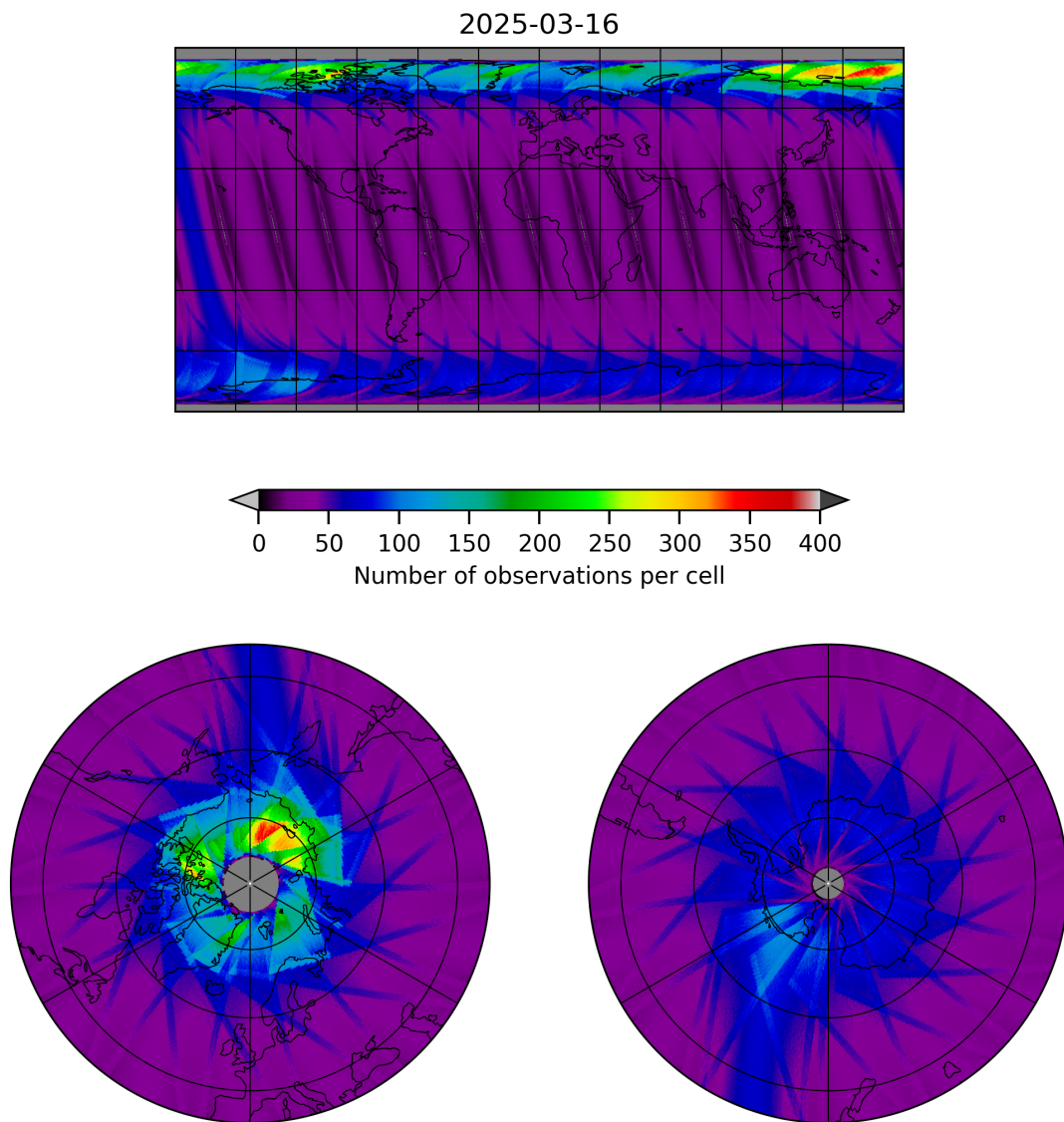
Figure 17: Map of the number of observations for 2025-03-16 to 2025-03-17
