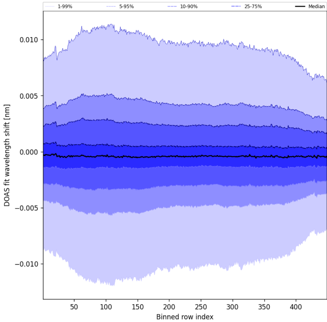
Figure 56: Along track statistics of “DOAS fit wavelength shift” for 2025-03-16 to 2025-03-17
