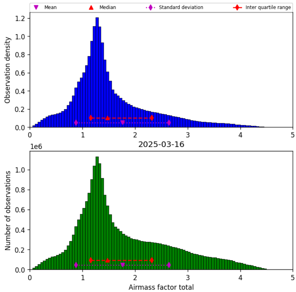
Figure 38: Histogram of “Airmass factor total” for 2025-03-16 to 2025-03-17
