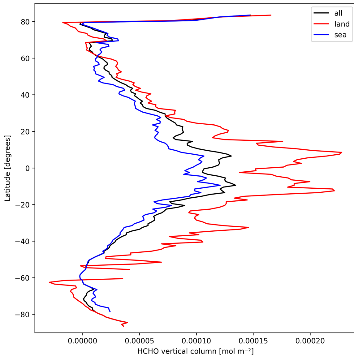
Figure 19: Zonal average of “HCHO vertical column” for 2025-03-16 to 2025-03-17.
