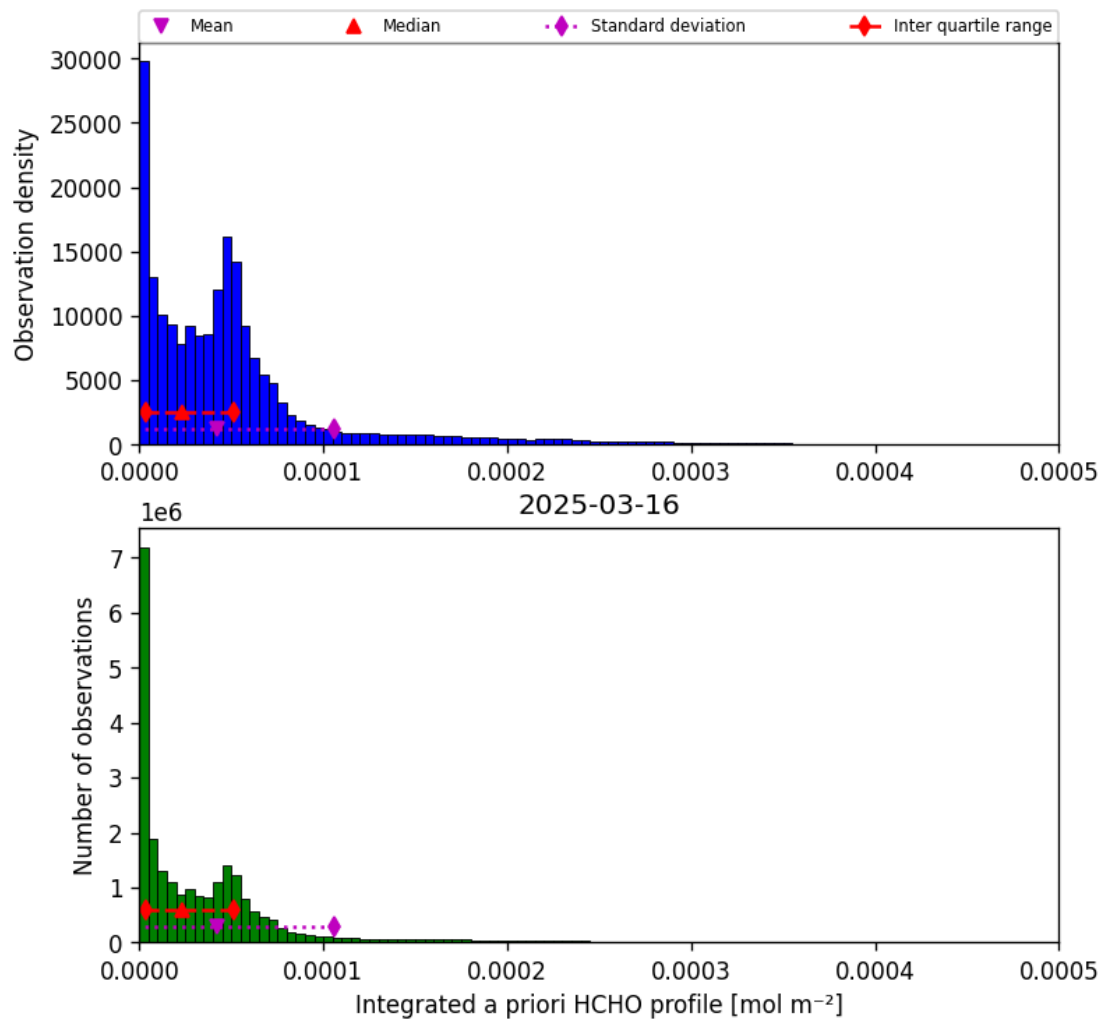
Figure 41: Histogram of “Integrated a priori HCHO profile” for 2025-03-16 to 2025-03-17
