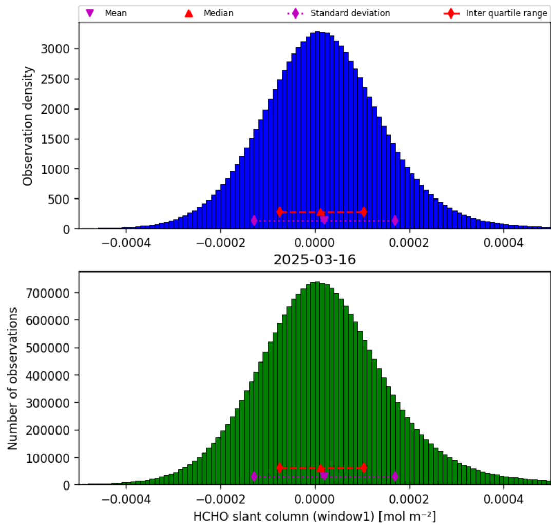
Figure 36: Histogram of “HCHO slant column (window1)” for 2025-03-16 to 2025-03-17
