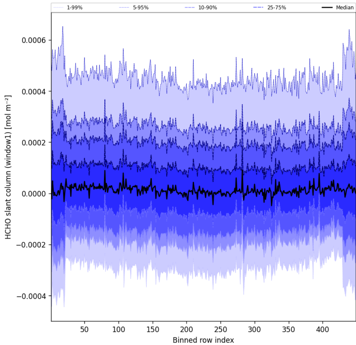
Figure 50: Along track statistics of “HCHO slant column (window1)” for 2025-03-16 to 2025-03-17
