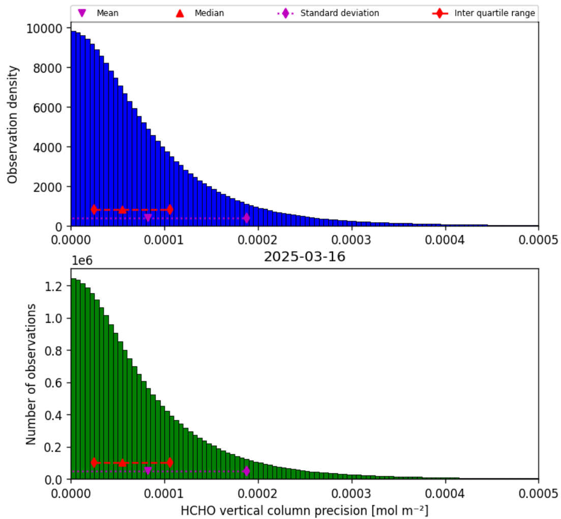
Figure 34: Histogram of “HCHO vertical column precision” for 2025-03-16 to 2025-03-17
