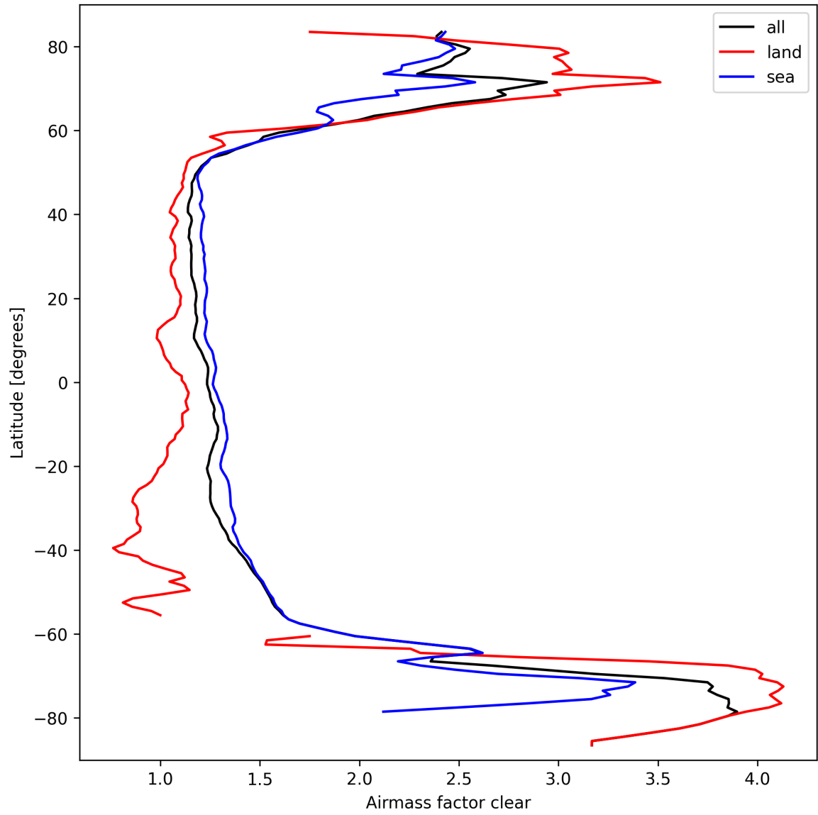
Figure 26: Zonal average of “Airmass factor clear” for 2025-03-16 to 2025-03-17.
