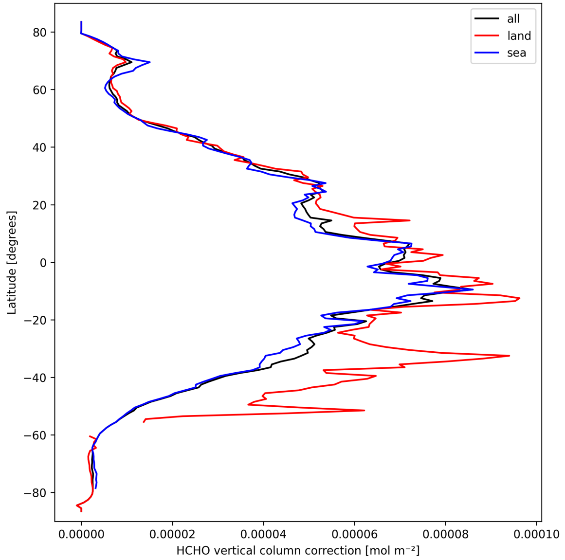
Figure 21: Zonal average of “HCHO vertical column correction” for 2025-03-16 to 2025-03-17.
