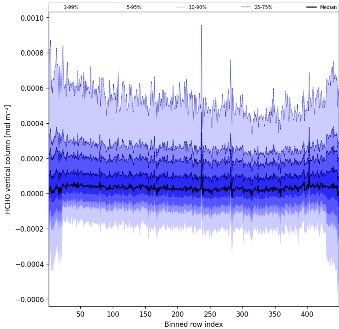
Figure 47: Along track statistics of “HCHO vertical column” for 2025-03-17 to 2025-03-18
