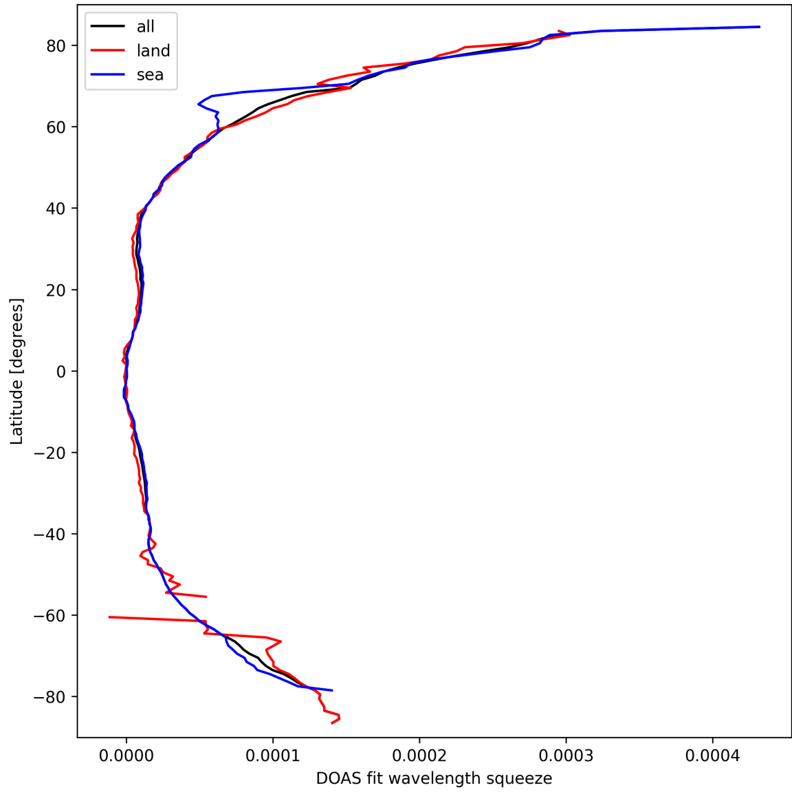
Figure 29: Zonal average of “DOAS fit wavelength squeeze” for 2025-03-17 to 2025-03-18.
