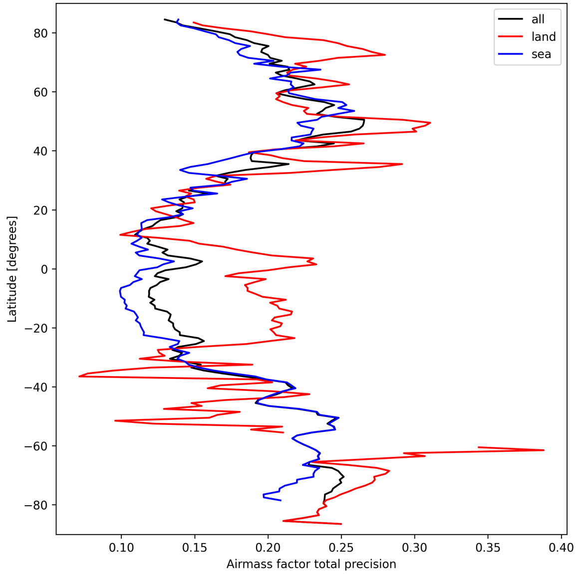
Figure 25: Zonal average of “Airmass factor total precision” for 2025-03-17 to 2025-03-18.
