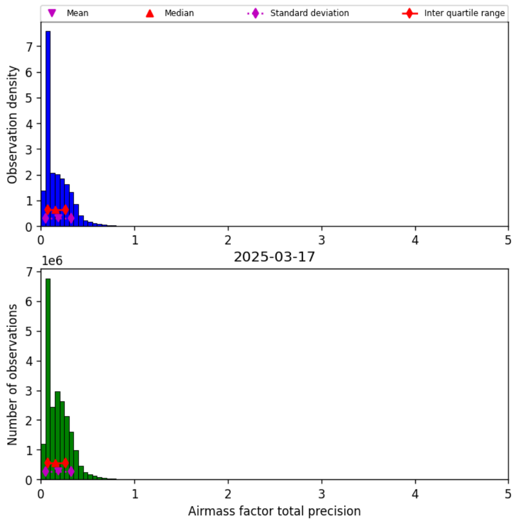
Figure 39: Histogram of “Airmass factor total precision” for 2025-03-17 to 2025-03-18
