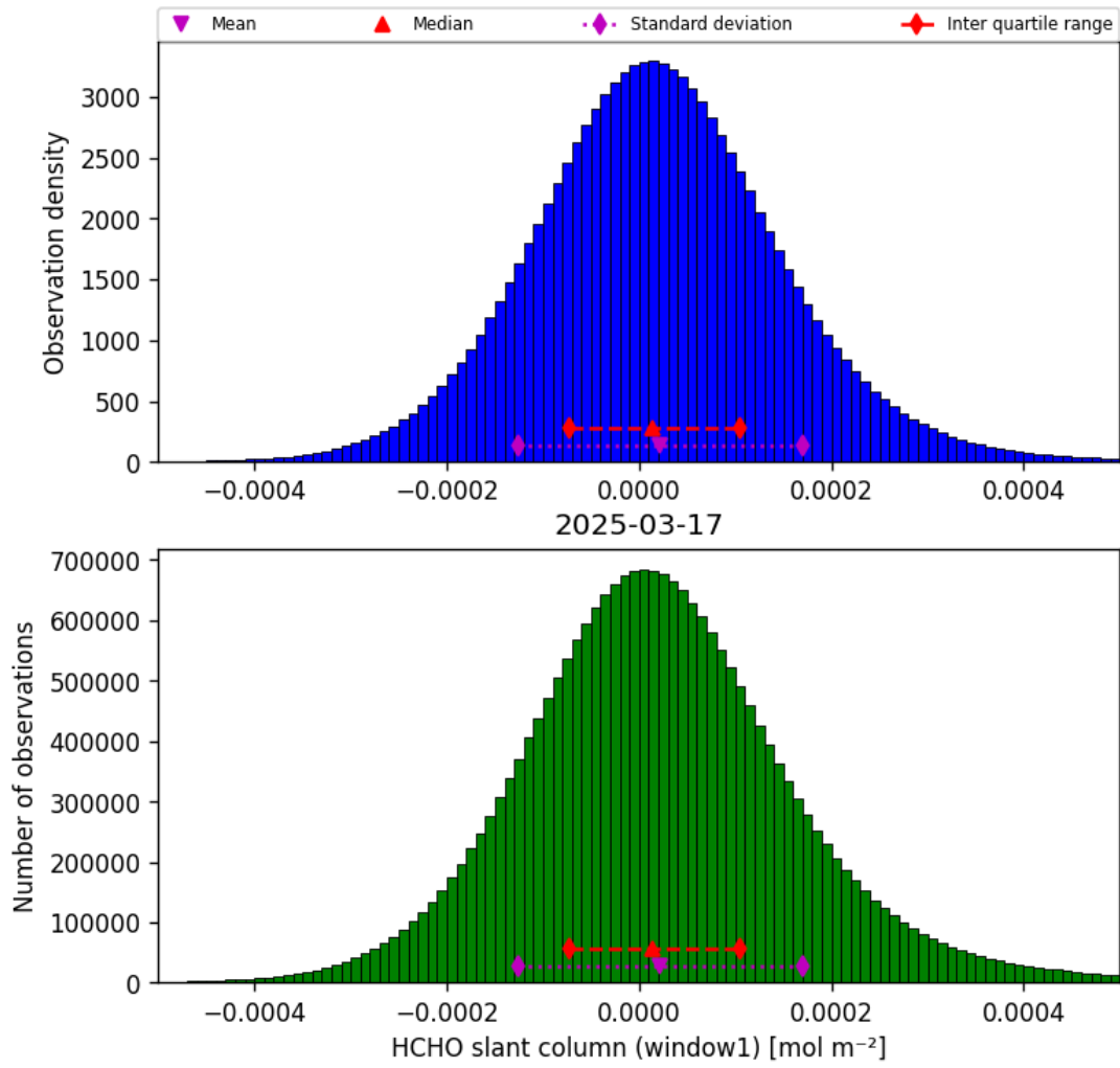
Figure 36: Histogram of “HCHO slant column (window1)” for 2025-03-17 to 2025-03-18
