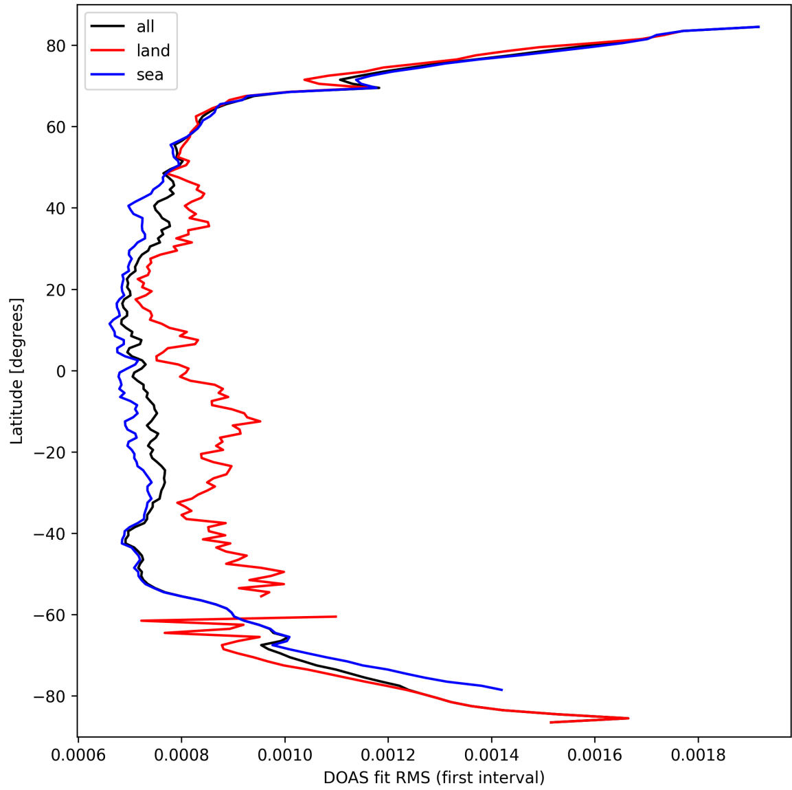
Figure 30: Zonal average of "DOAS fit RMS (first interval)" for 2025-03-17 to 2025-03-18.
