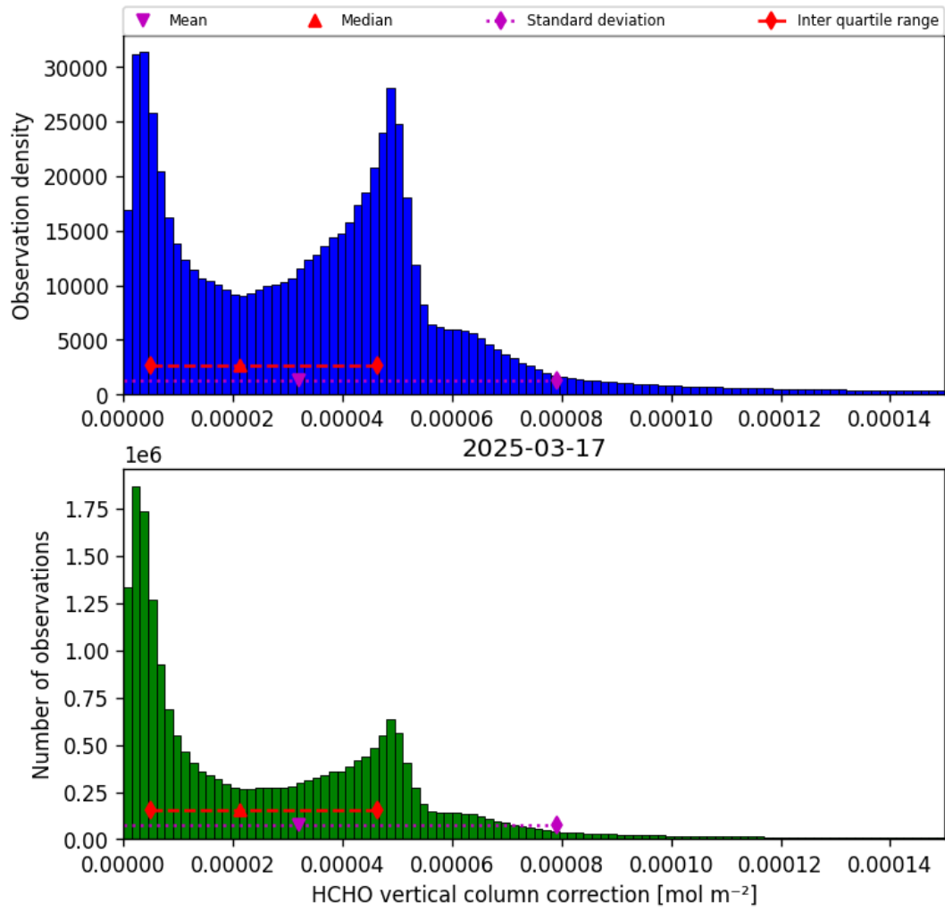
Figure 35: Histogram of “HCHO vertical column correction” for 2025-03-17 to 2025-03-18
