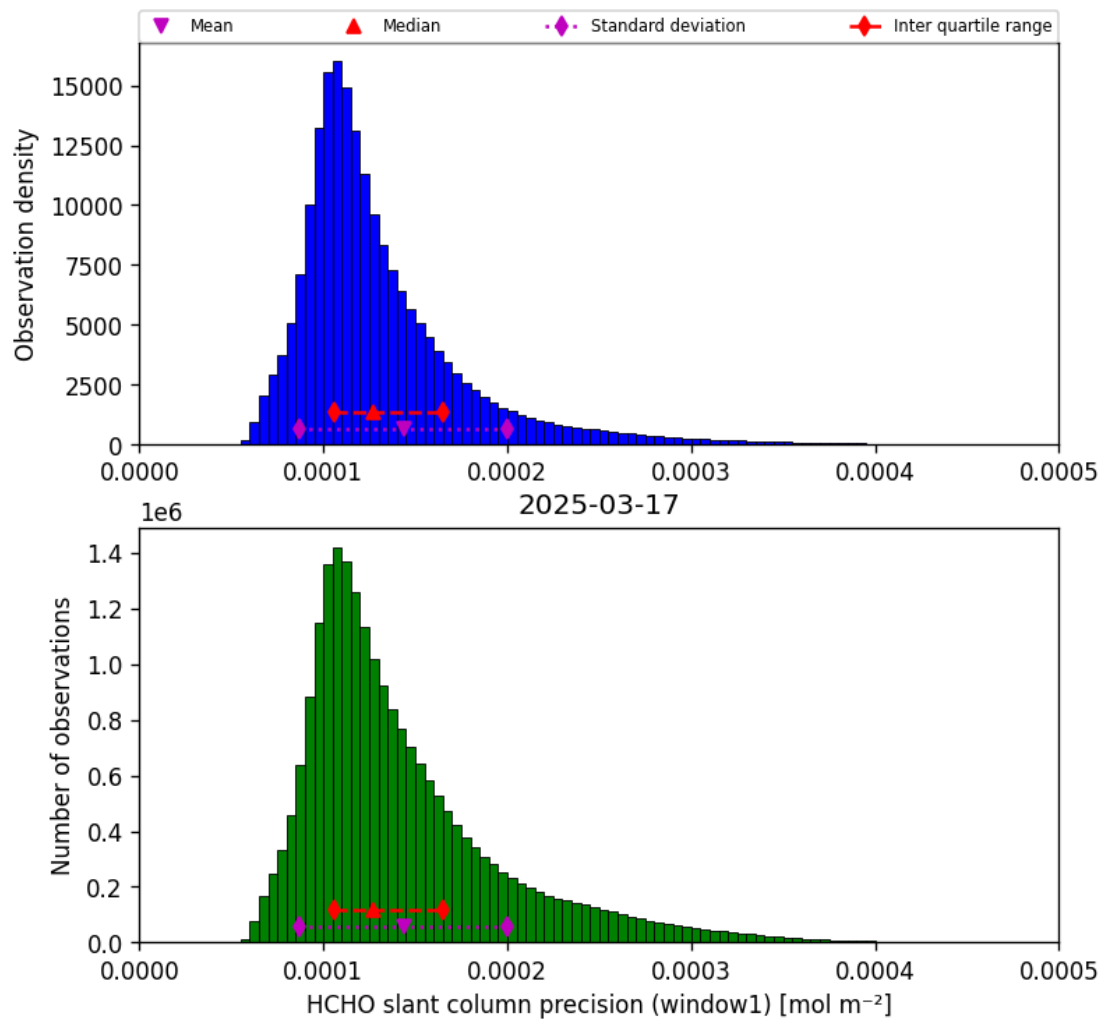
Figure 37: Histogram of “HCHO slant column precision (window1)” for 2025-03-17 to 2025-03-18
