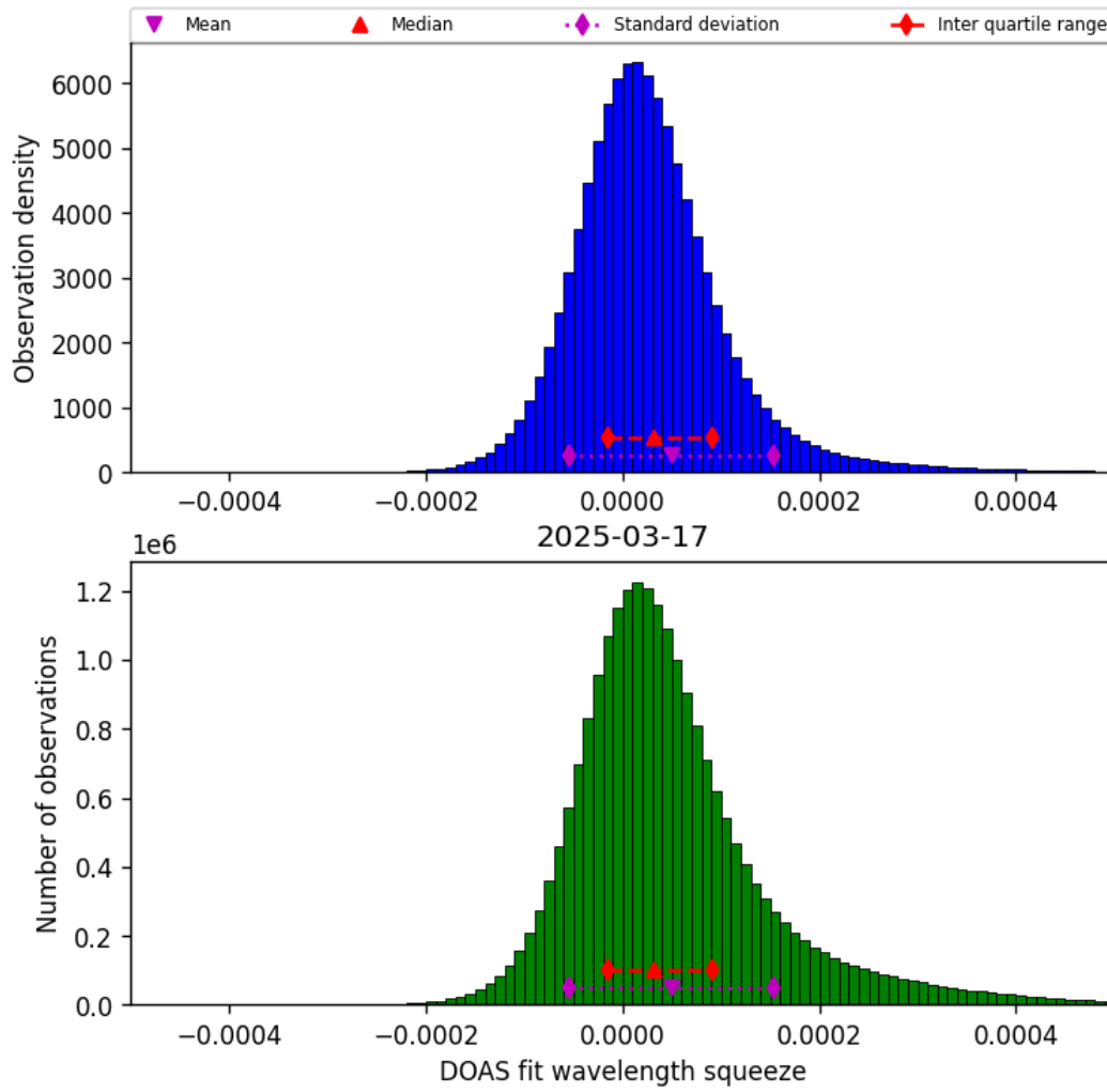
Figure 43: Histogram of “DOAS fit wavelength squeeze” for 2025-03-17 to 2025-03-18
