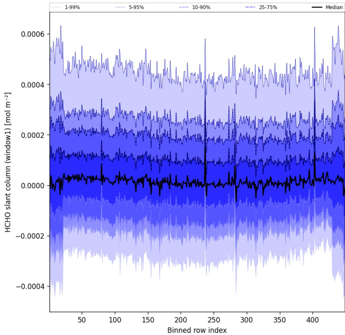
Figure 50: Along track statistics of “HCHO slant column (window1)” for 2025-03-17 to 2025-03-18
