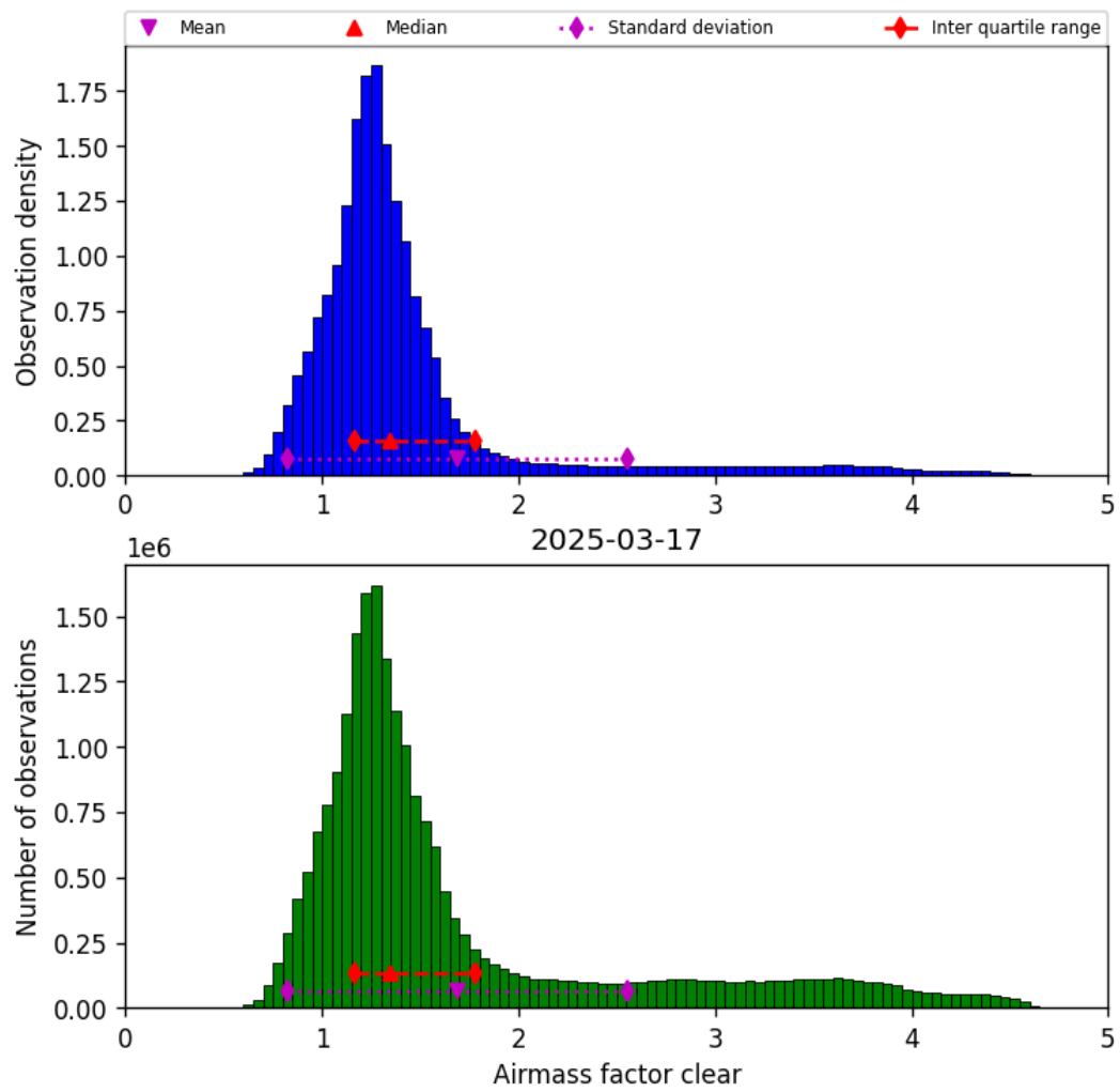
Figure 40: Histogram of “Airmass factor clear” for 2025-03-17 to 2025-03-18
