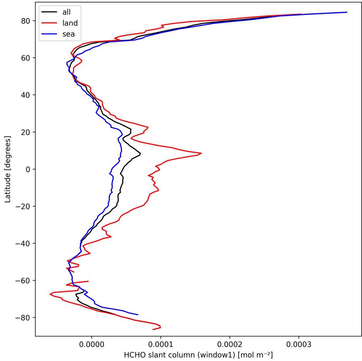
Figure 22: Zonal average of “HCHO slant column (window1)” for 2025-03-17 to 2025-03-18.
