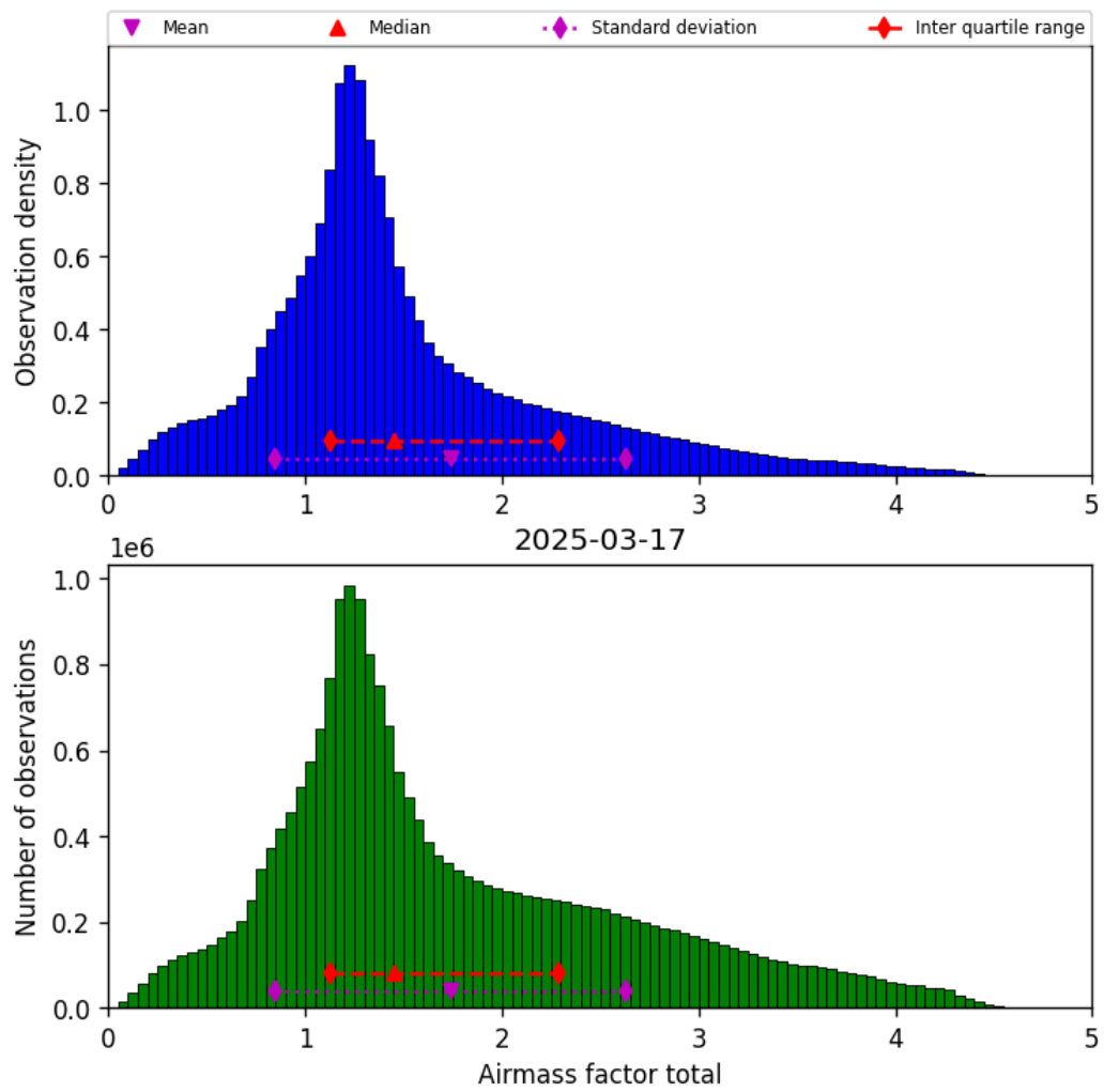
Figure 38: Histogram of “Airmass factor total” for 2025-03-17 to 2025-03-18
