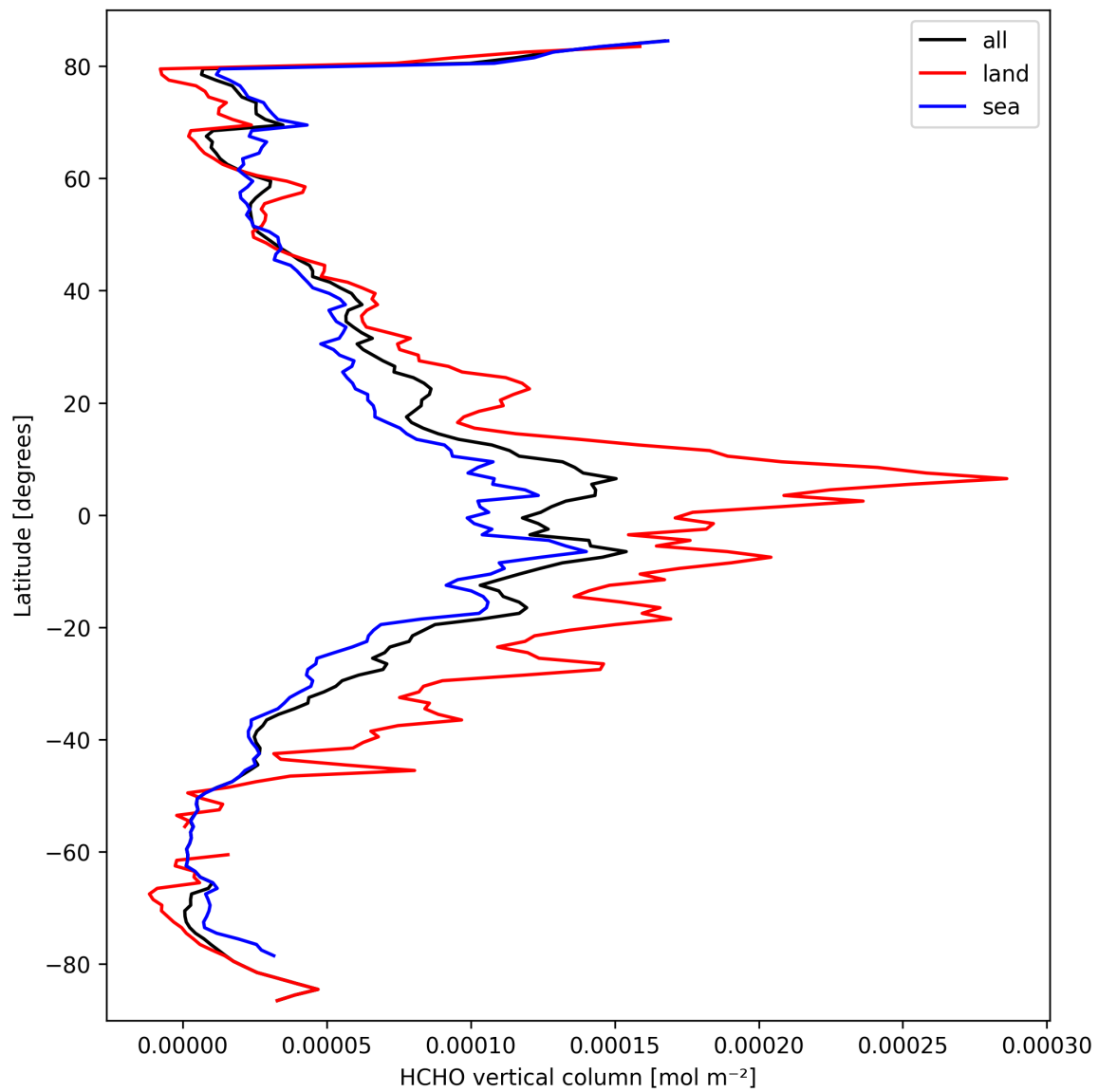
Figure 19: Zonal average of “HCHO vertical column” for 2025-03-17 to 2025-03-18.
