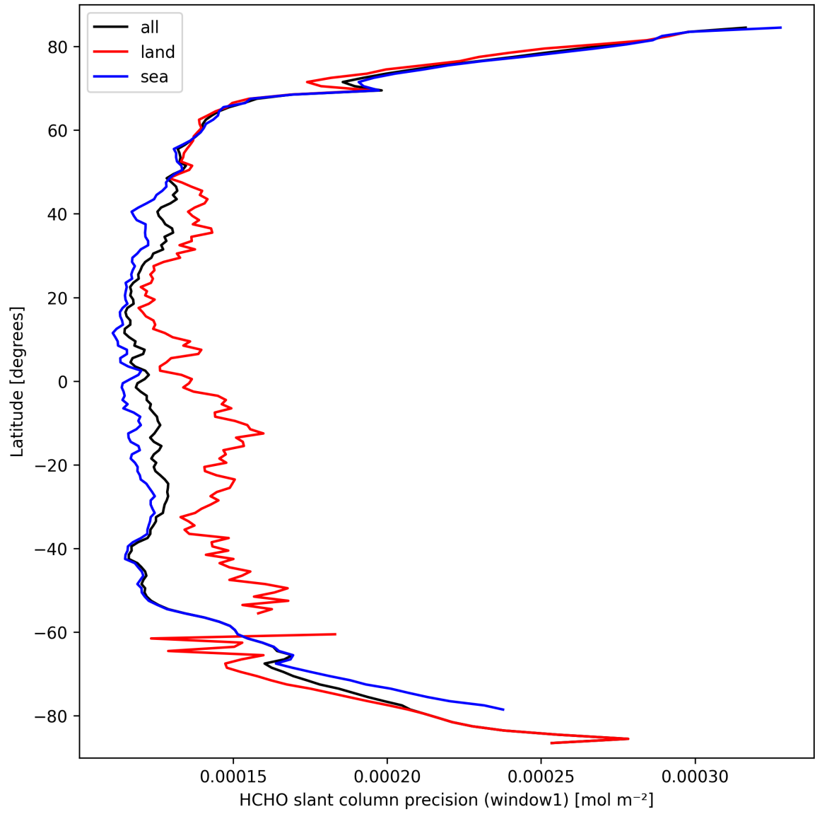
Figure 23: Zonal average of “HCHO slant column precision (window1)” for 2025-03-17 to 2025-03-18.
