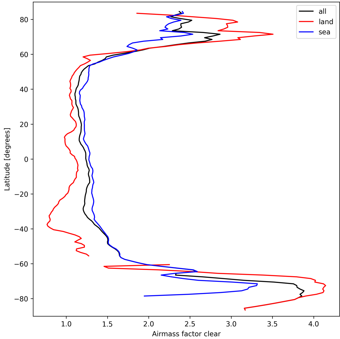
Figure 26: Zonal average of “Airmass factor clear” for 2025-03-17 to 2025-03-18.
