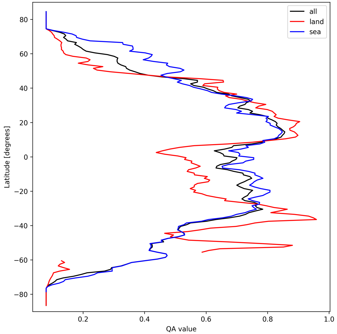
Figure 18: Zonal average of “QA value” for 2025-03-17 to 2025-03-18.
