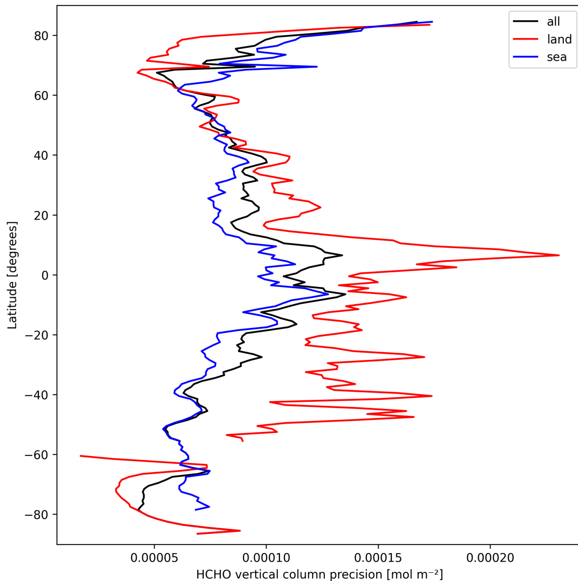
Figure 20: Zonal average of “HCHO vertical column precision” for 2025-03-17 to 2025-03-18.
