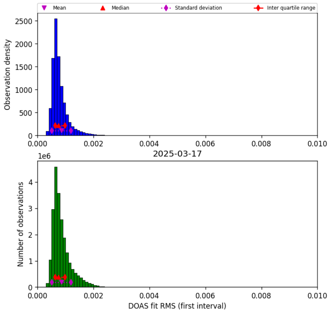
Figure 44: Histogram of “DOAS fit RMS (first interval)” for 2025-03-17 to 2025-03-18
