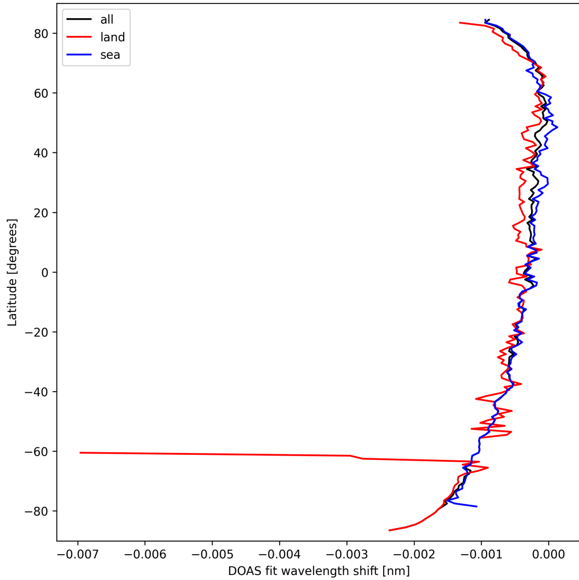
Figure 28: Zonal average of “DOAS fit wavelength shift” for 2025-03-17 to 2025-03-18.
