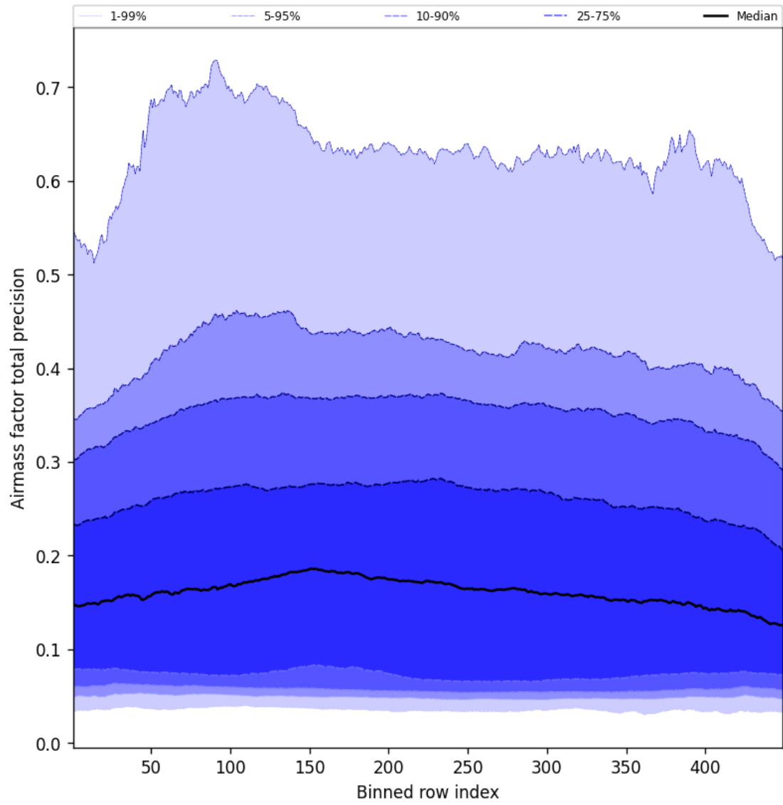
Figure 53: Along track statistics of “Airmass factor total precision” for 2025-03-17 to 2025-03-18
