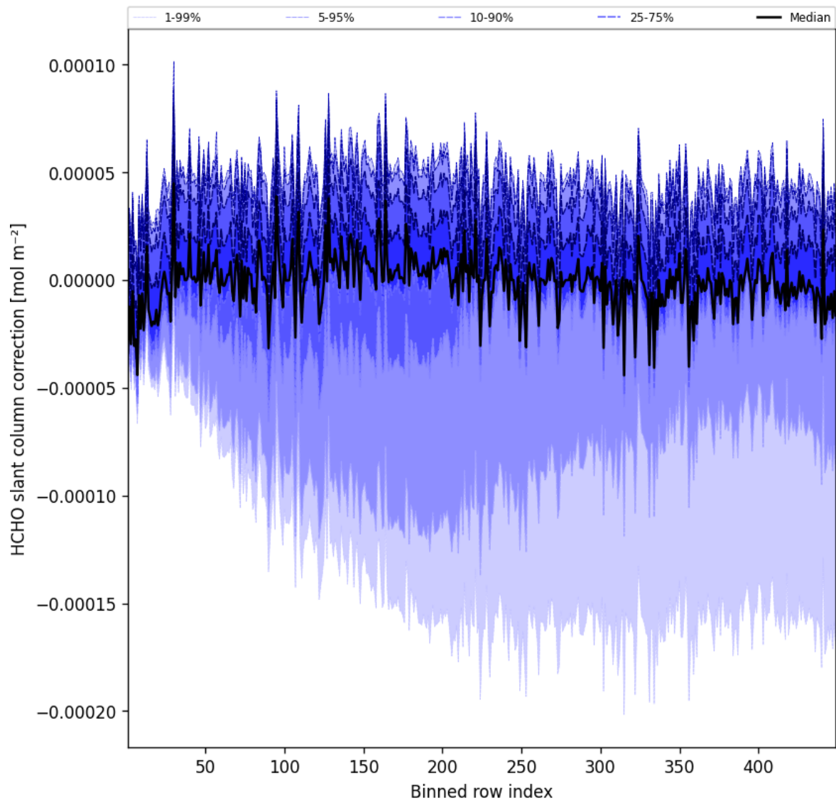
Figure 59: Along track statistics of “HCHO slant column correction” for 2025-03-17 to 2025-03-18
