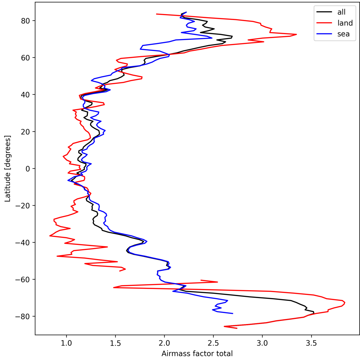
Figure 24: Zonal average of “Airmass factor total” for 2025-03-17 to 2025-03-18.
