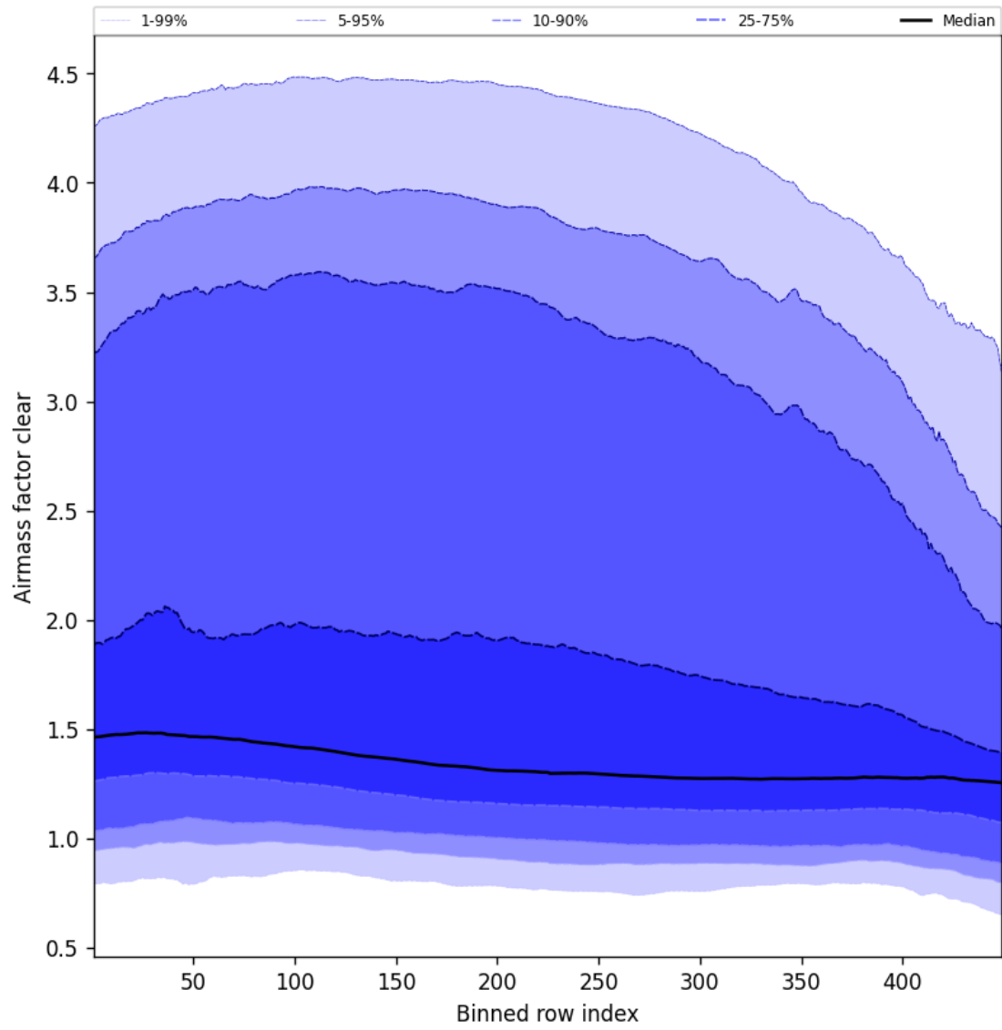
Figure 54: Along track statistics of “Airmass factor clear” for 2025-03-17 to 2025-03-18
