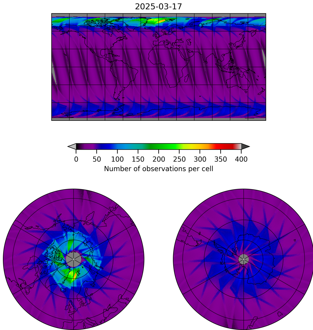
Figure 17: Map of the number of observations for 2025-03-17 to 2025-03-18
