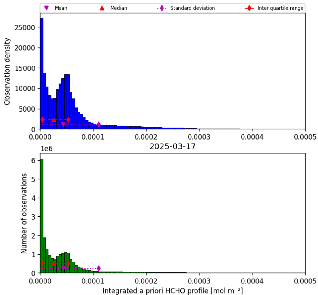
Figure 41: Histogram of “Integrated a priori HCHO profile” for 2025-03-17 to 2025-03-18
