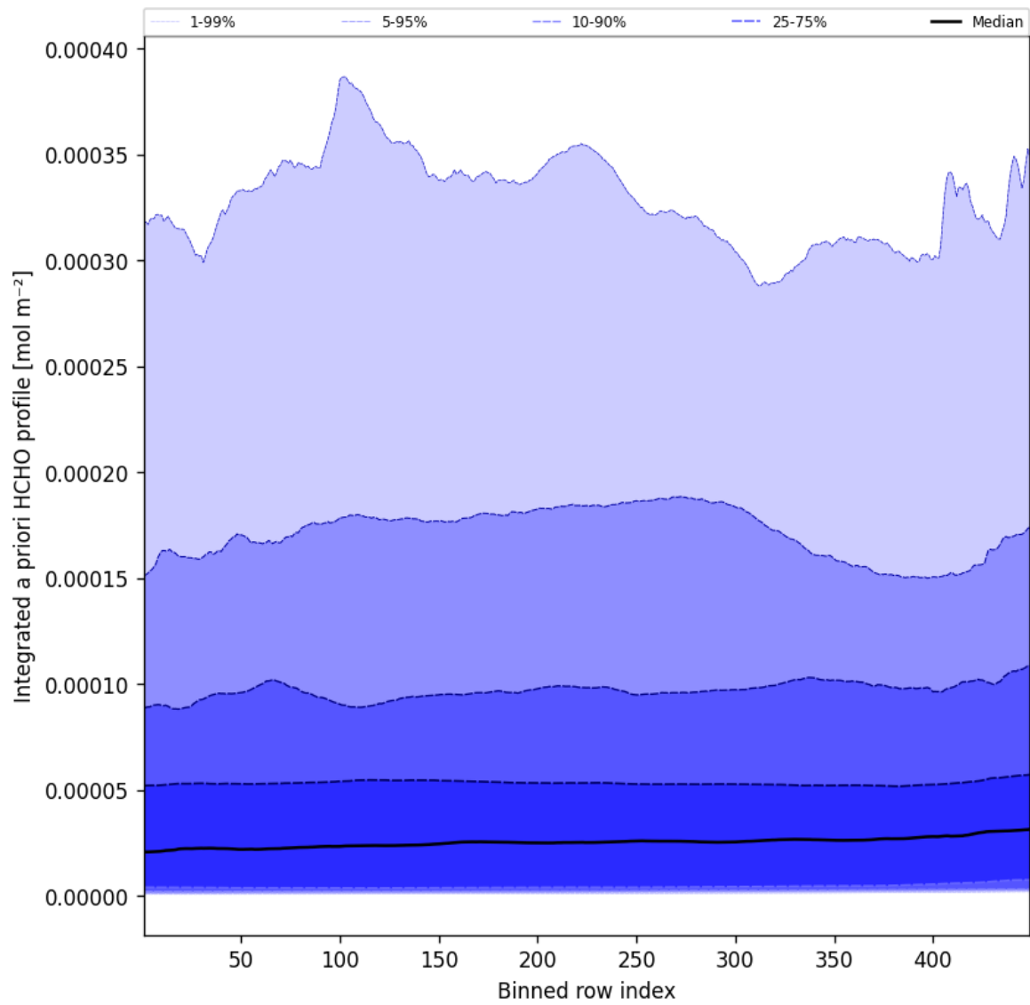
Figure 55: Along track statistics of “Integrated a priori HCHO profile” for 2025-03-17 to 2025-03-18
