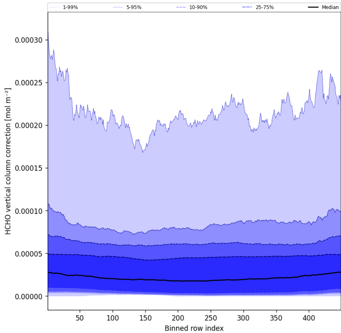
Figure 49: Along track statistics of “HCHO vertical column correction” for 2025-03-17 to 2025-03-18
