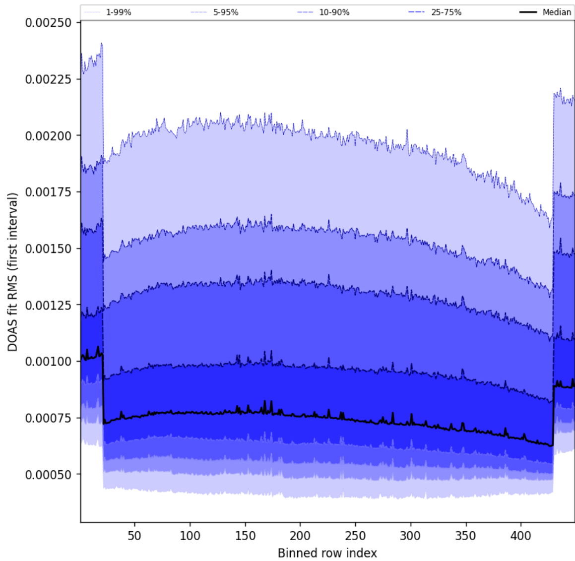
Figure 58: Along track statistics of “DOAS fit RMS (first interval)” for 2025-03-17 to 2025-03-18
