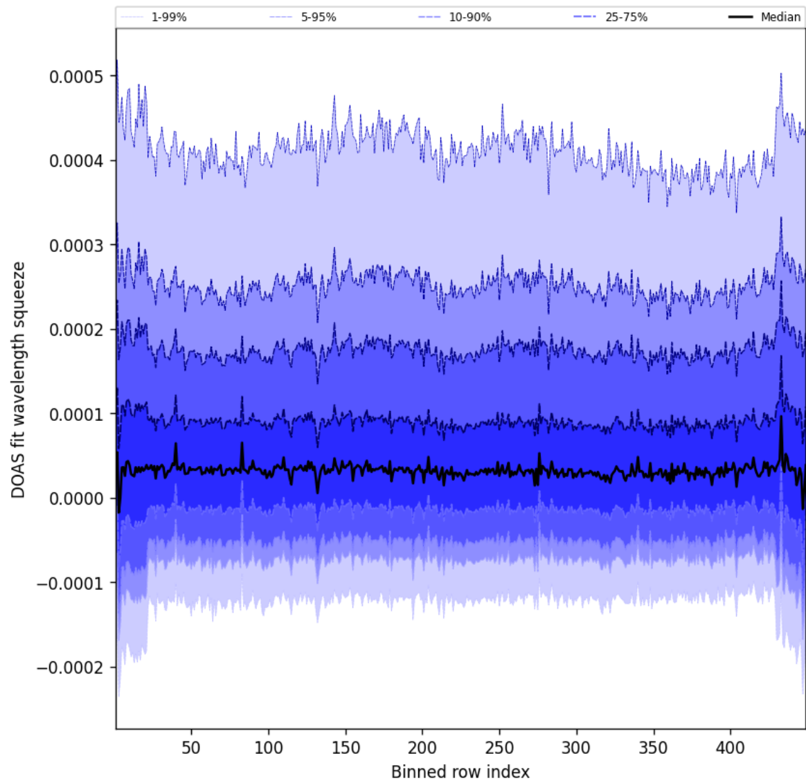
Figure 57: Along track statistics of “DOAS fit wavelength squeeze” for 2025-03-17 to 2025-03-18
