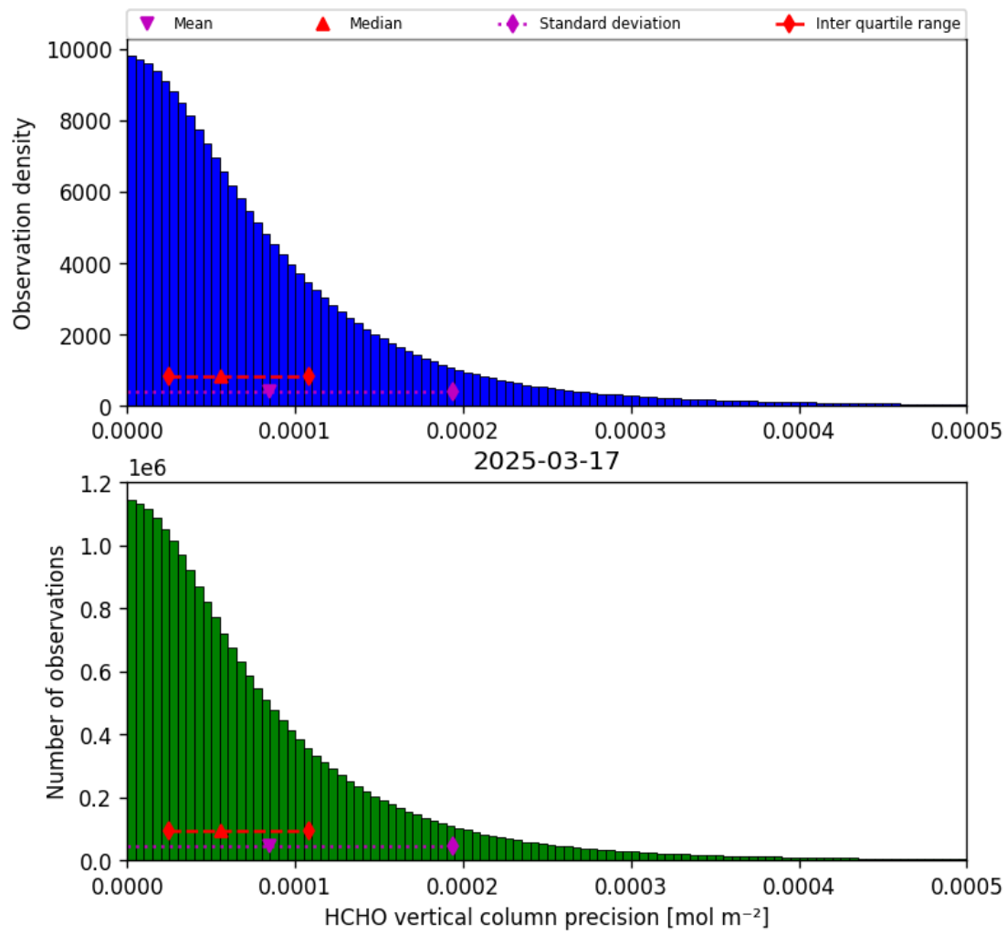
Figure 34: Histogram of “HCHO vertical column precision” for 2025-03-17 to 2025-03-18
