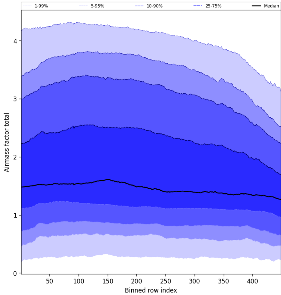
Figure 52: Along track statistics of “Airmass factor total” for 2025-03-17 to 2025-03-18
