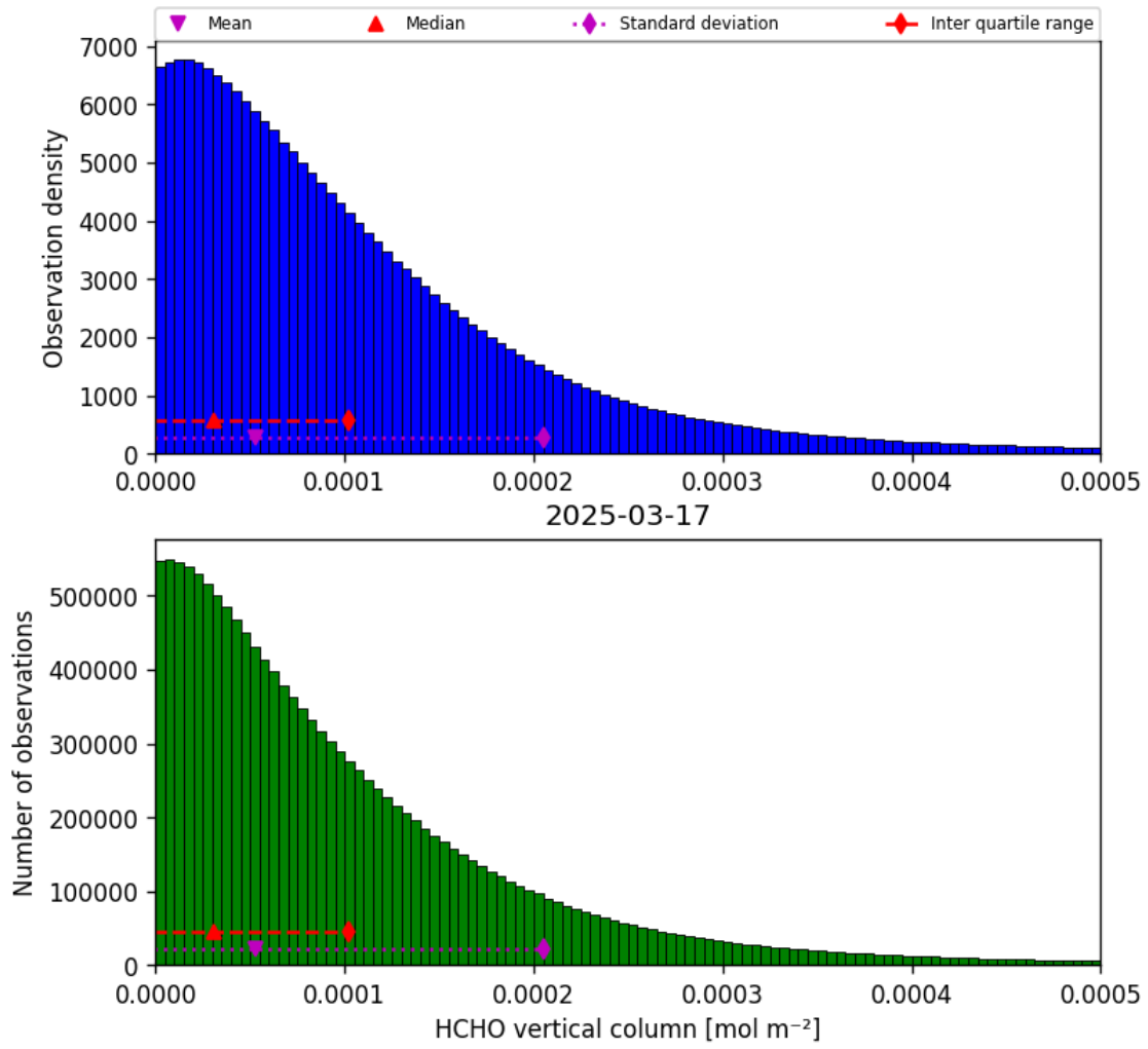
Figure 33: Histogram of “HCHO vertical column” for 2025-03-17 to 2025-03-18
