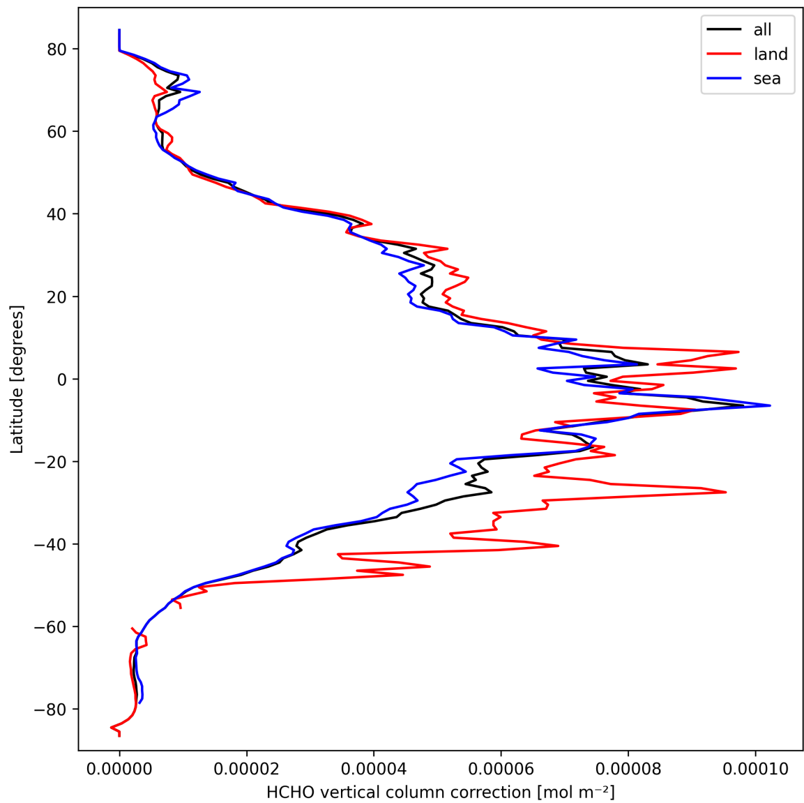
Figure 21: Zonal average of “HCHO vertical column correction” for 2025-03-17 to 2025-03-18.
