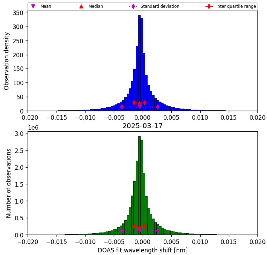
Figure 42: Histogram of “DOAS fit wavelength shift” for 2025-03-17 to 2025-03-18
