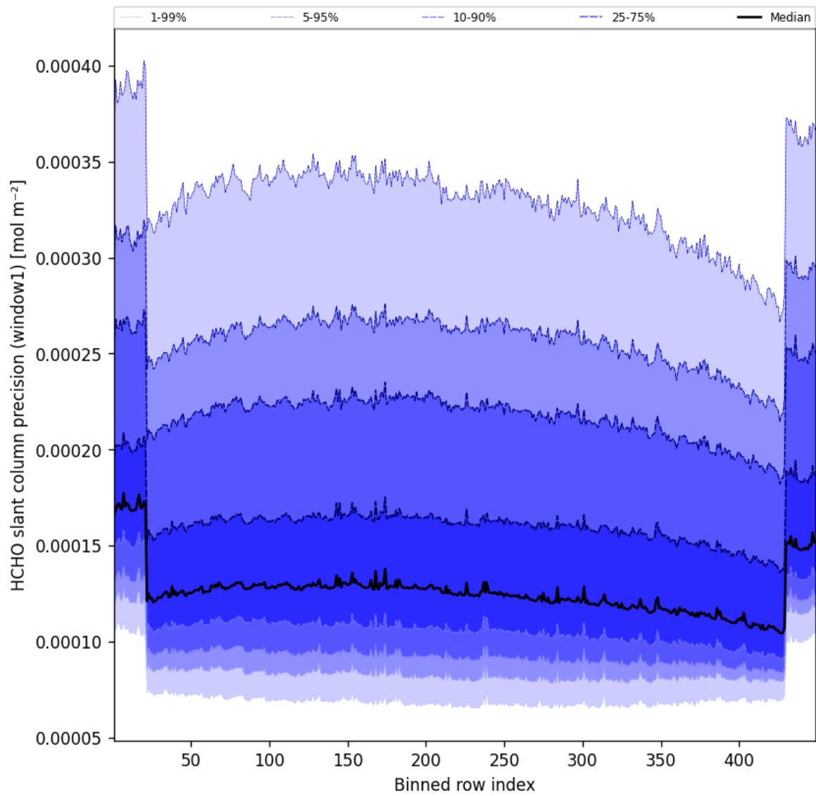
Figure 51: Along track statistics of “HCHO slant column precision (window1)” for 2025-03-17 to 2025-03-18
