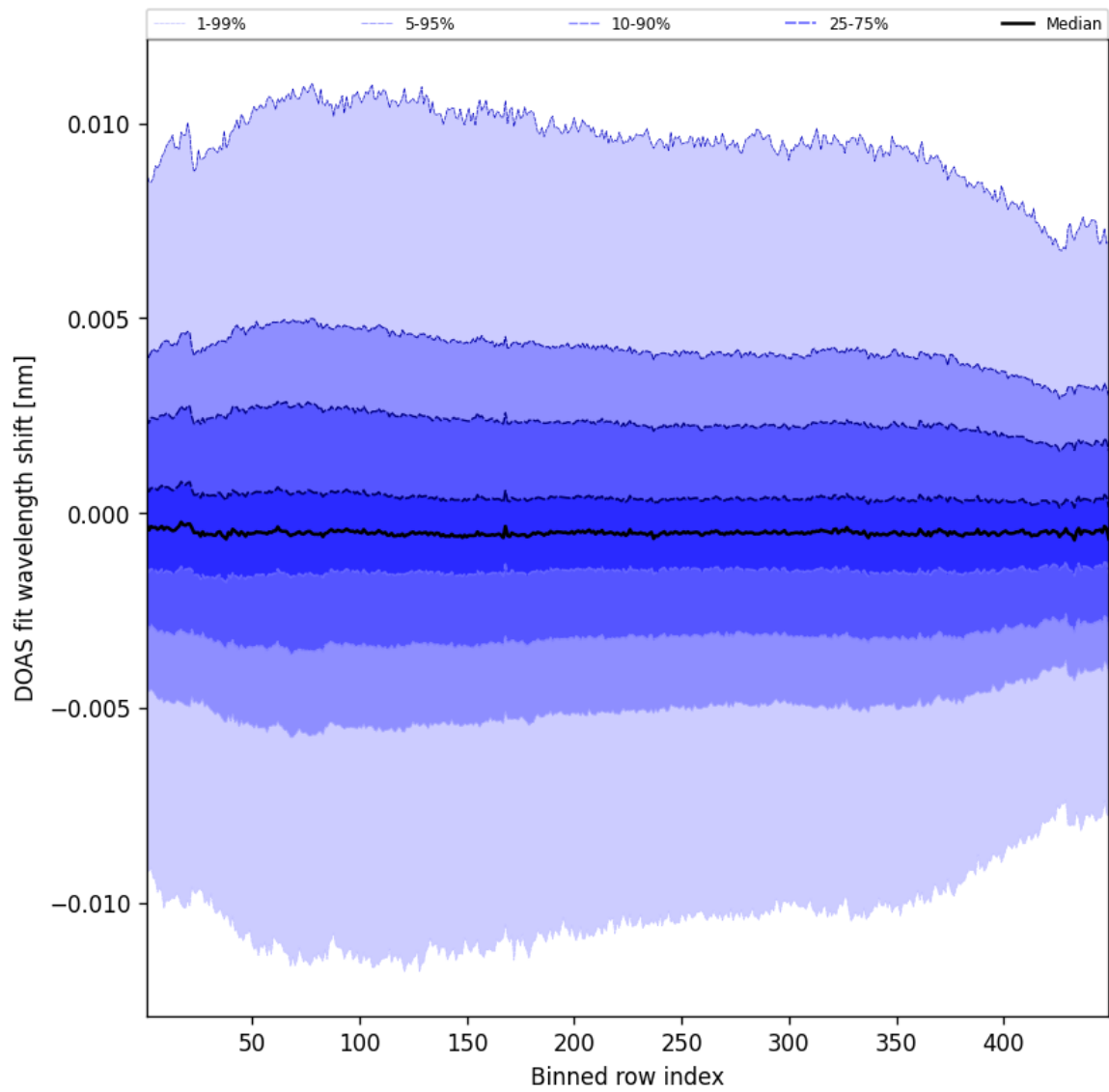
Figure 56: Along track statistics of “DOAS fit wavelength shift” for 2025-03-17 to 2025-03-18
