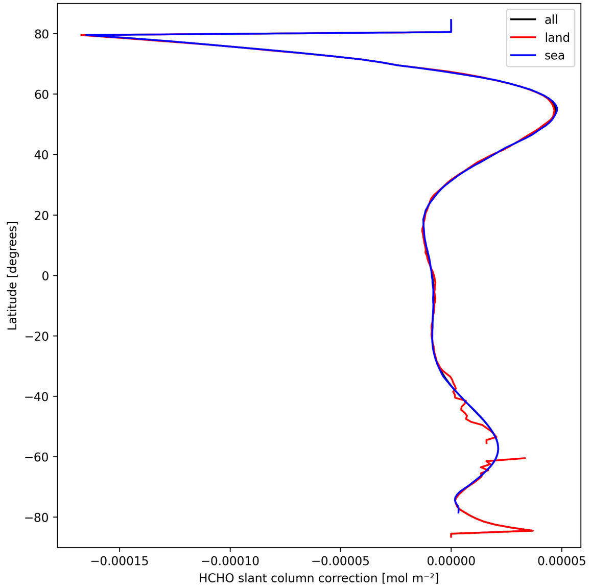
Figure 31: Zonal average of “HCHO slant column correction” for 2025-03-17 to 2025-03-18.
