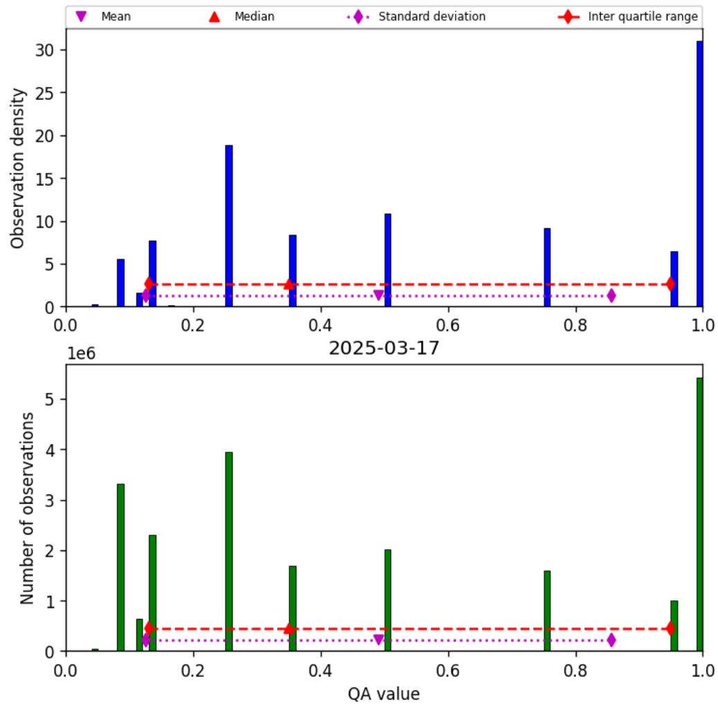
Figure 32: Histogram of “QA value” for 2025-03-17 to 2025-03-18
