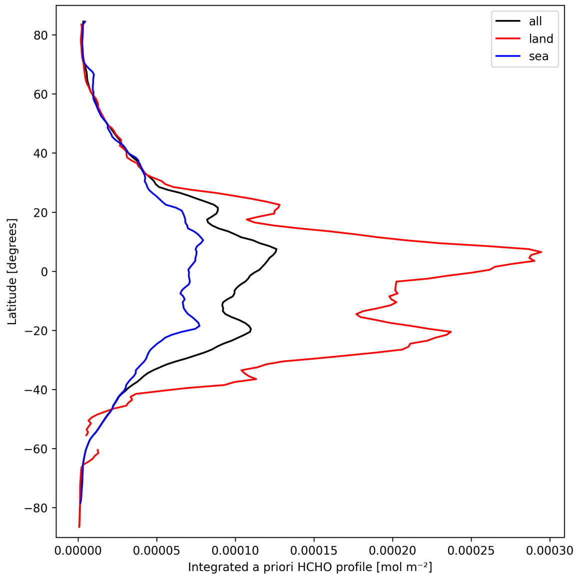
Figure 27: Zonal average of “Integrated a priori HCHO profile” for 2025-03-17 to 2025-03-18.
