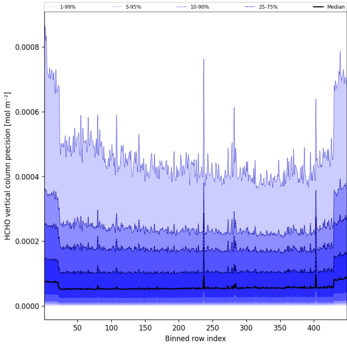
Figure 48: Along track statistics of “HCHO vertical column precision” for 2025-03-17 to 2025-03-18
