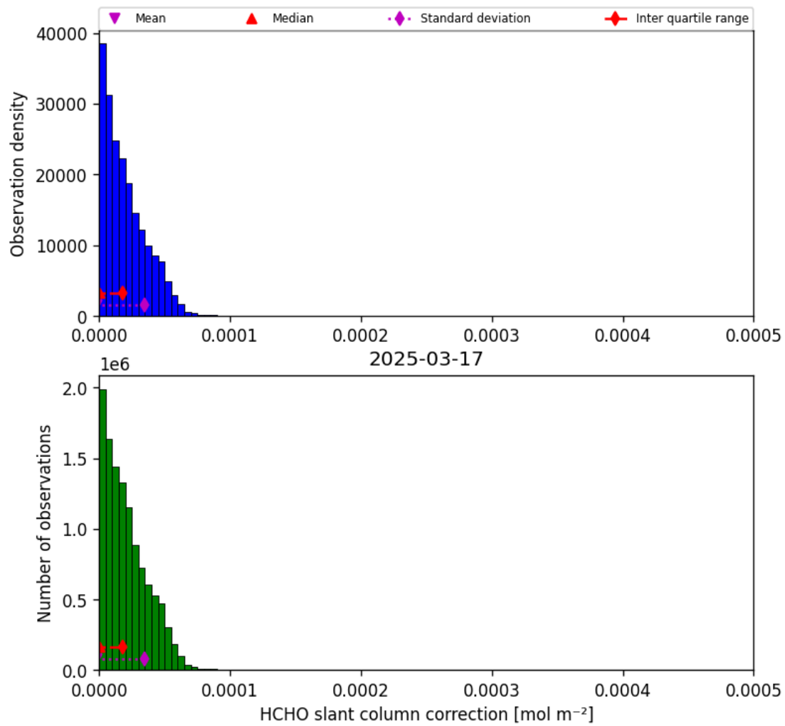
Figure 45: Histogram of “HCHO slant column correction” for 2025-03-17 to 2025-03-18
