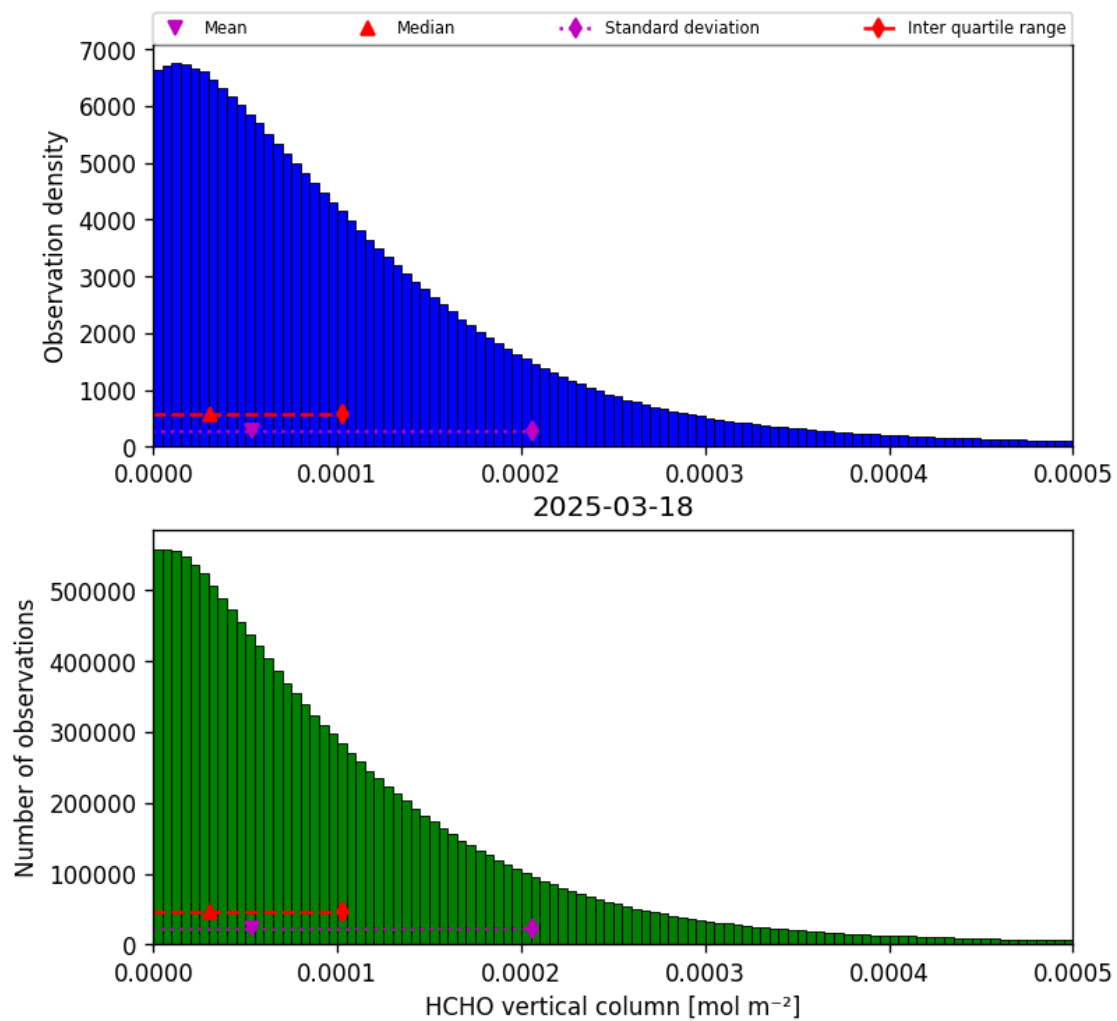
Figure 33: Histogram of “HCHO vertical column” for 2025-03-18 to 2025-03-19
