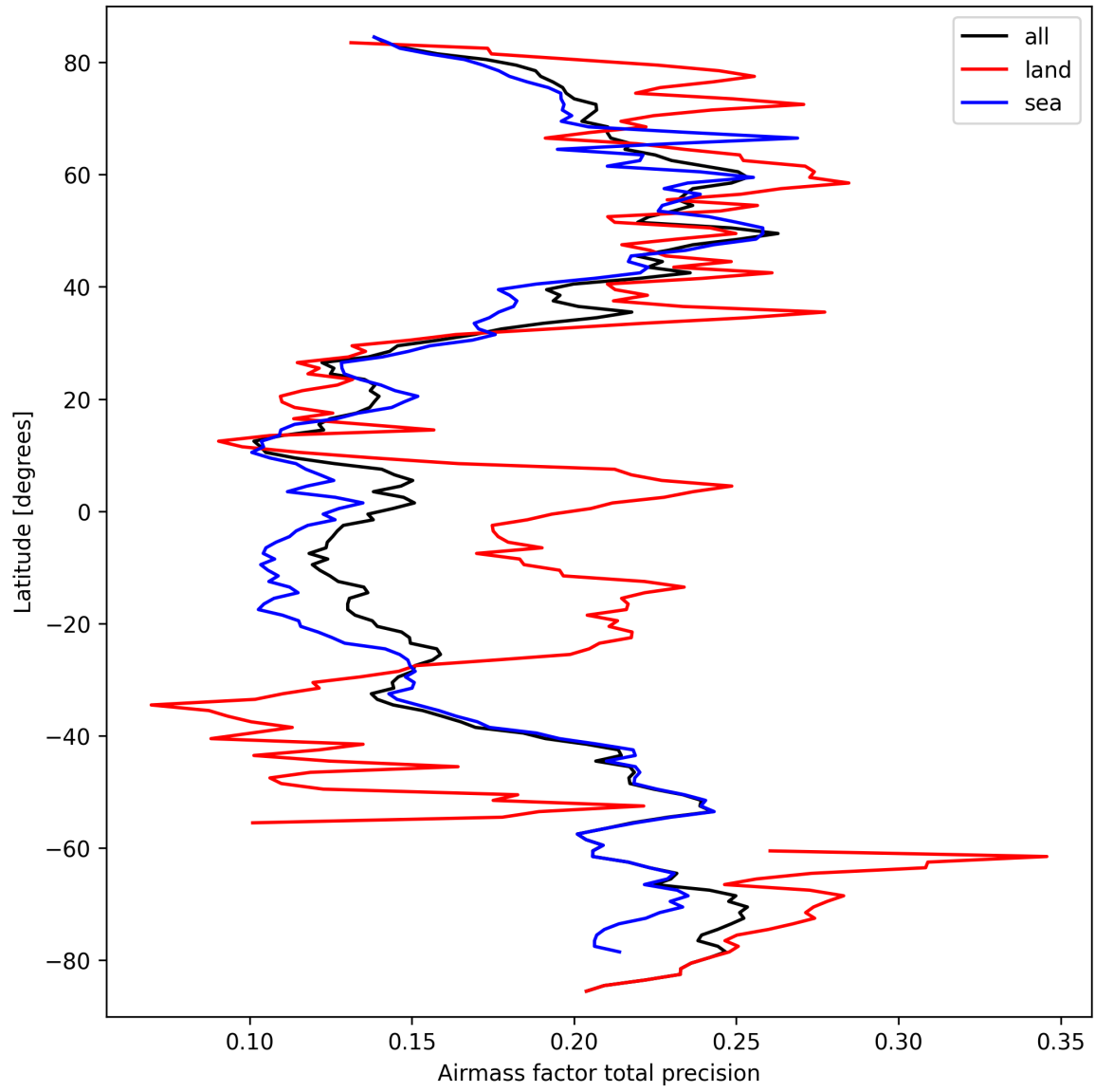
Figure 25: Zonal average of “Airmass factor total precision” for 2025-03-18 to 2025-03-19.
