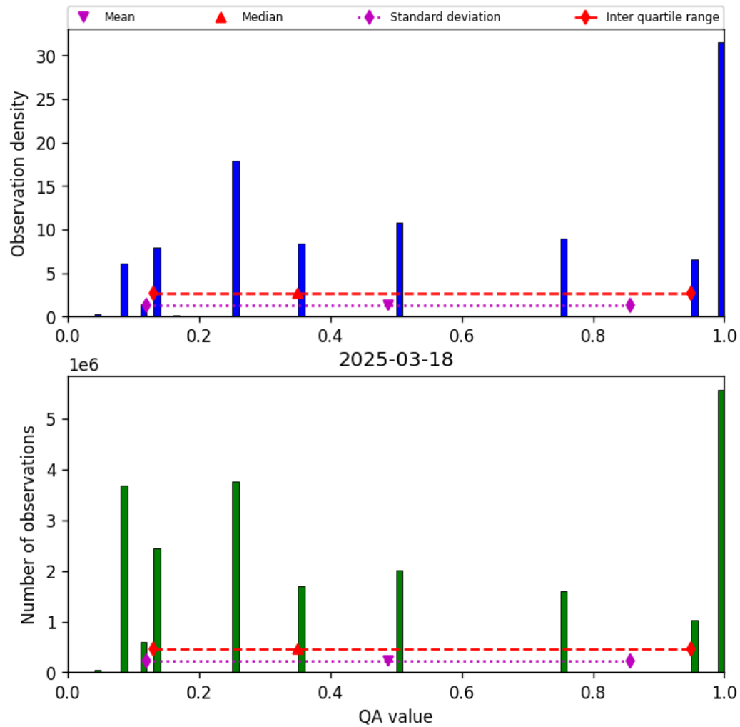
Figure 32: Histogram of “QA value” for 2025-03-18 to 2025-03-19
