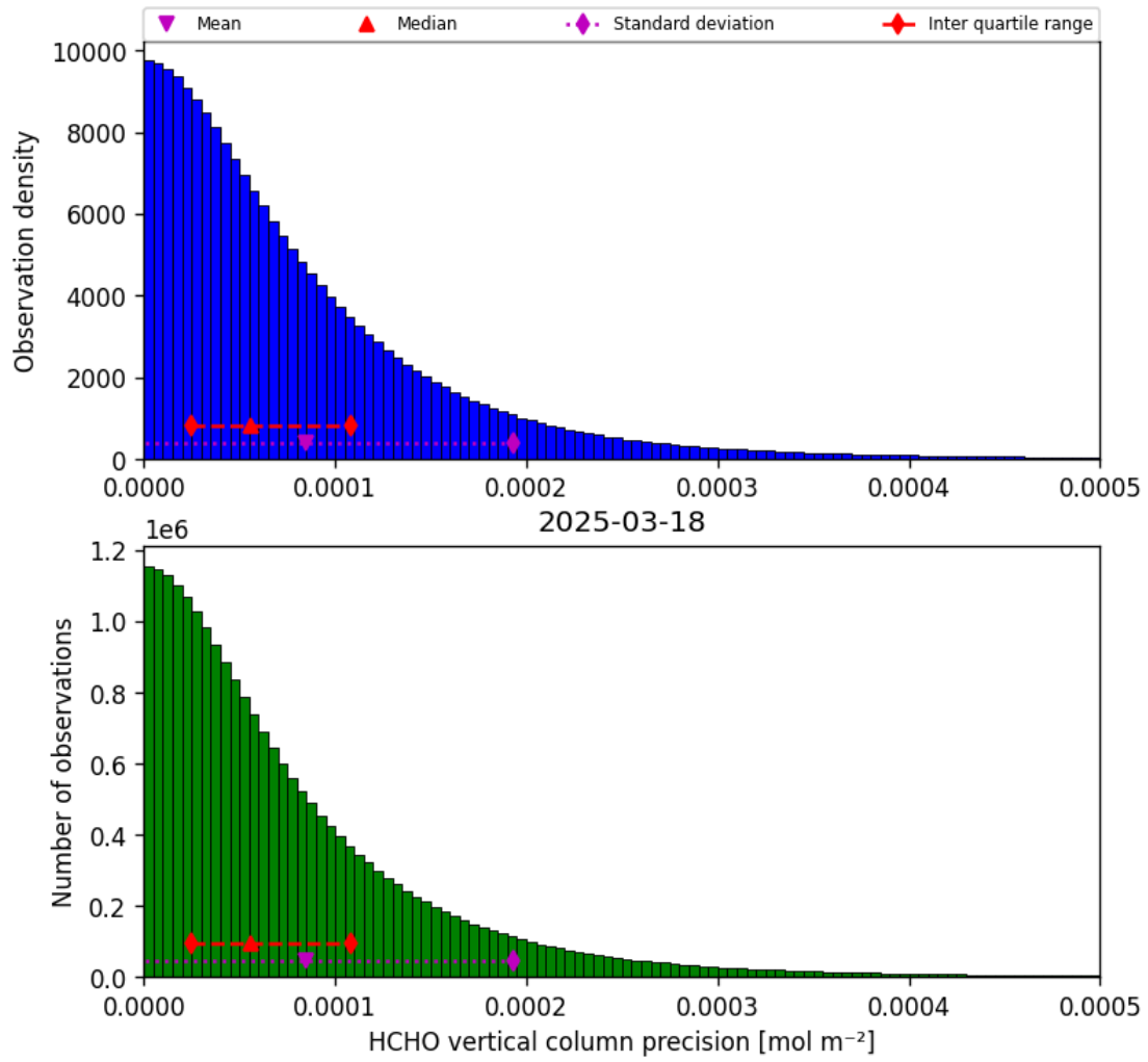
Figure 34: Histogram of “HCHO vertical column precision” for 2025-03-18 to 2025-03-19
