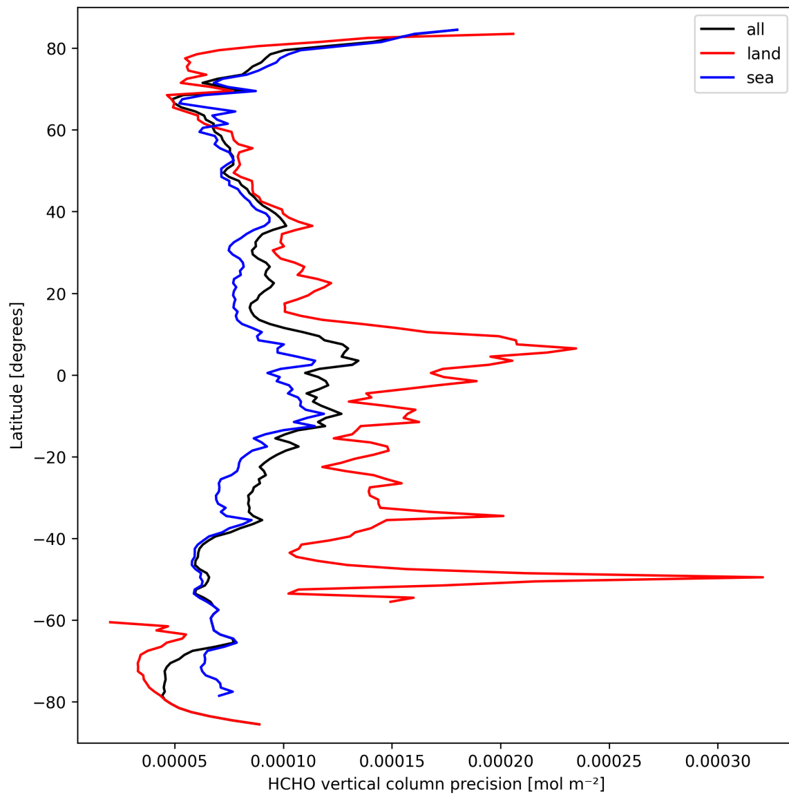
Figure 20: Zonal average of “HCHO vertical column precision” for 2025-03-18 to 2025-03-19.
