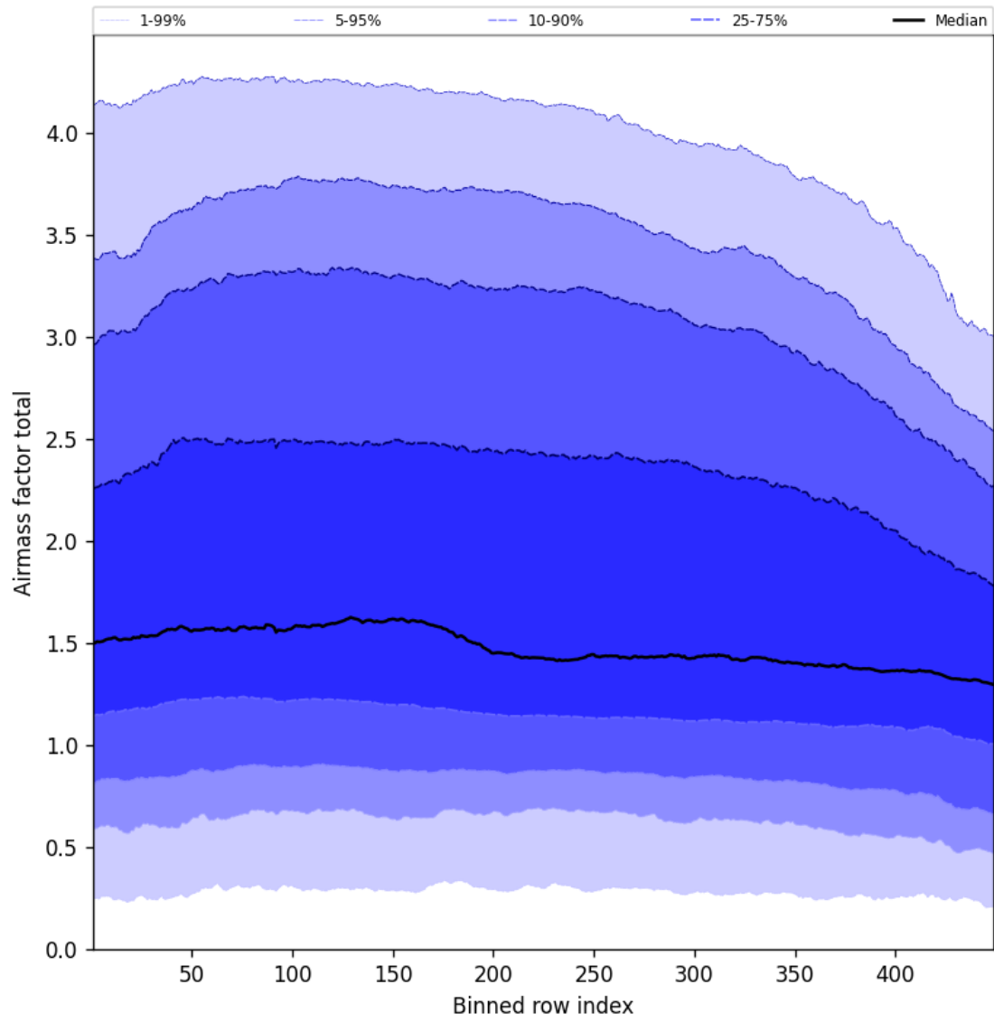
Figure 52: Along track statistics of “Airmass factor total” for 2025-03-18 to 2025-03-19
