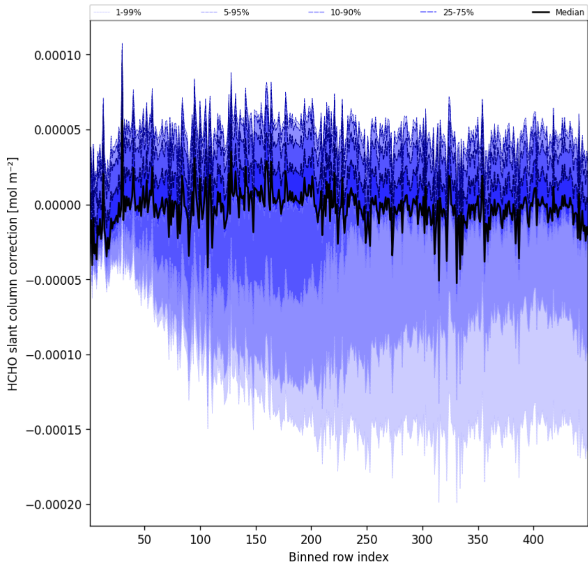
Figure 59: Along track statistics of “HCHO slant column correction” for 2025-03-18 to 2025-03-19
