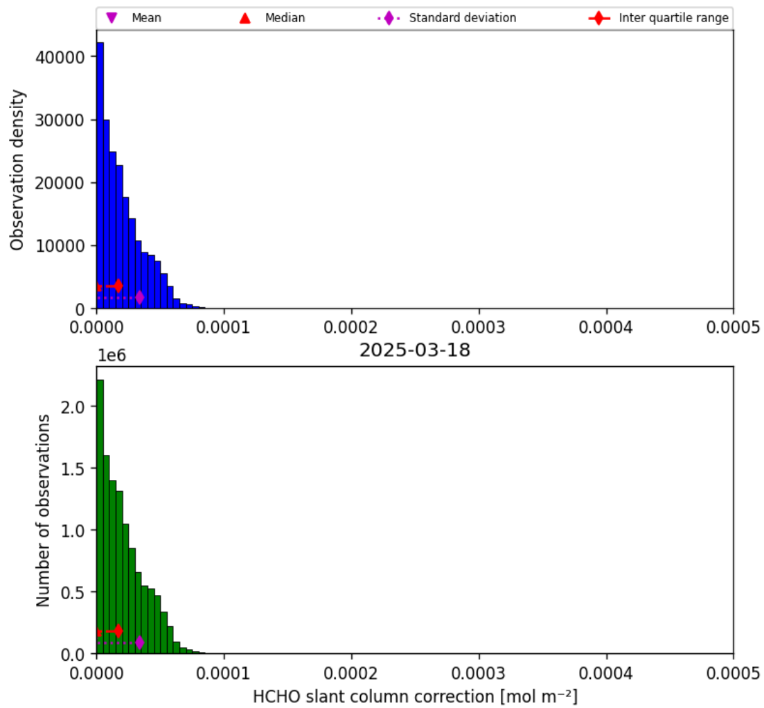
Figure 45: Histogram of “HCHO slant column correction” for 2025-03-18 to 2025-03-19
