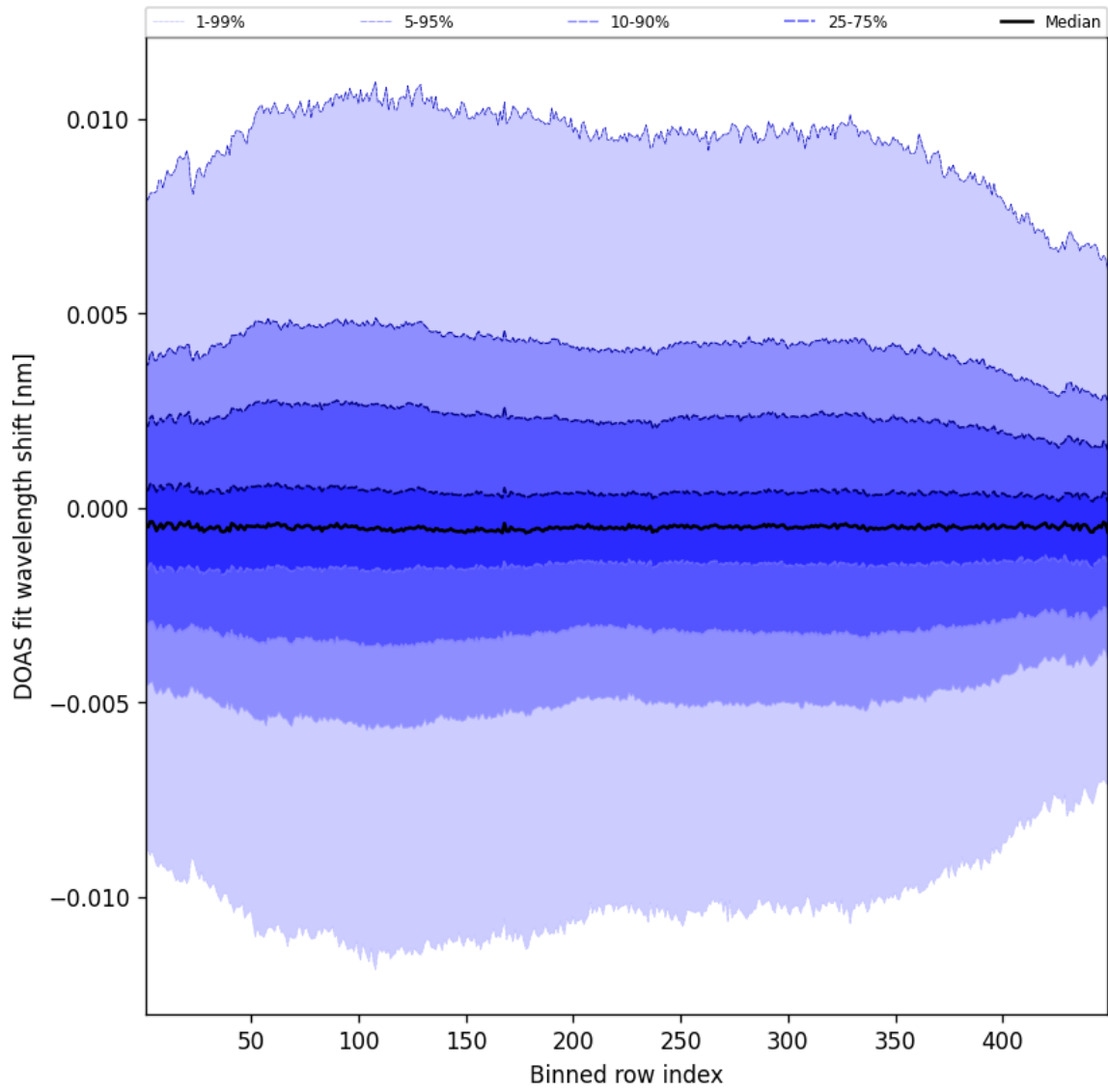
Figure 56: Along track statistics of “DOAS fit wavelength shift” for 2025-03-18 to 2025-03-19
