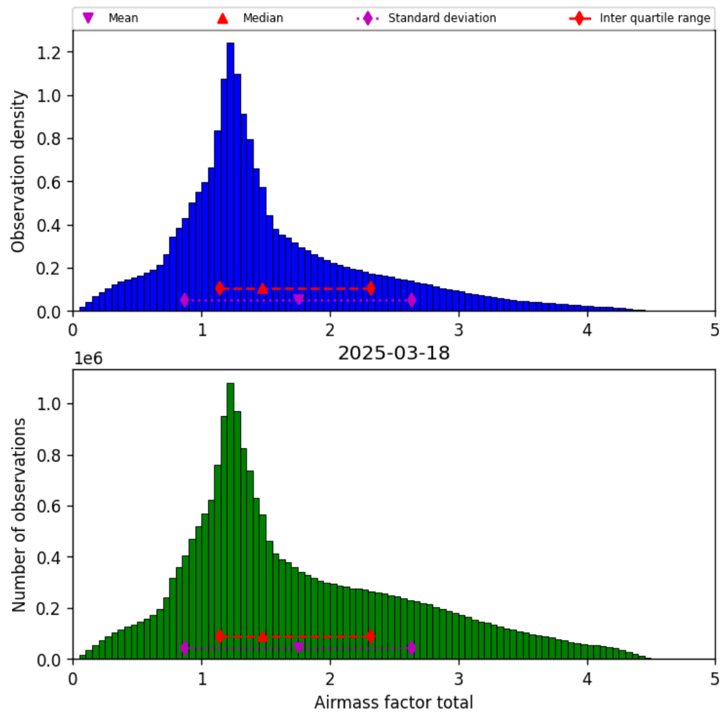
Figure 38: Histogram of “Airmass factor total” for 2025-03-18 to 2025-03-19
