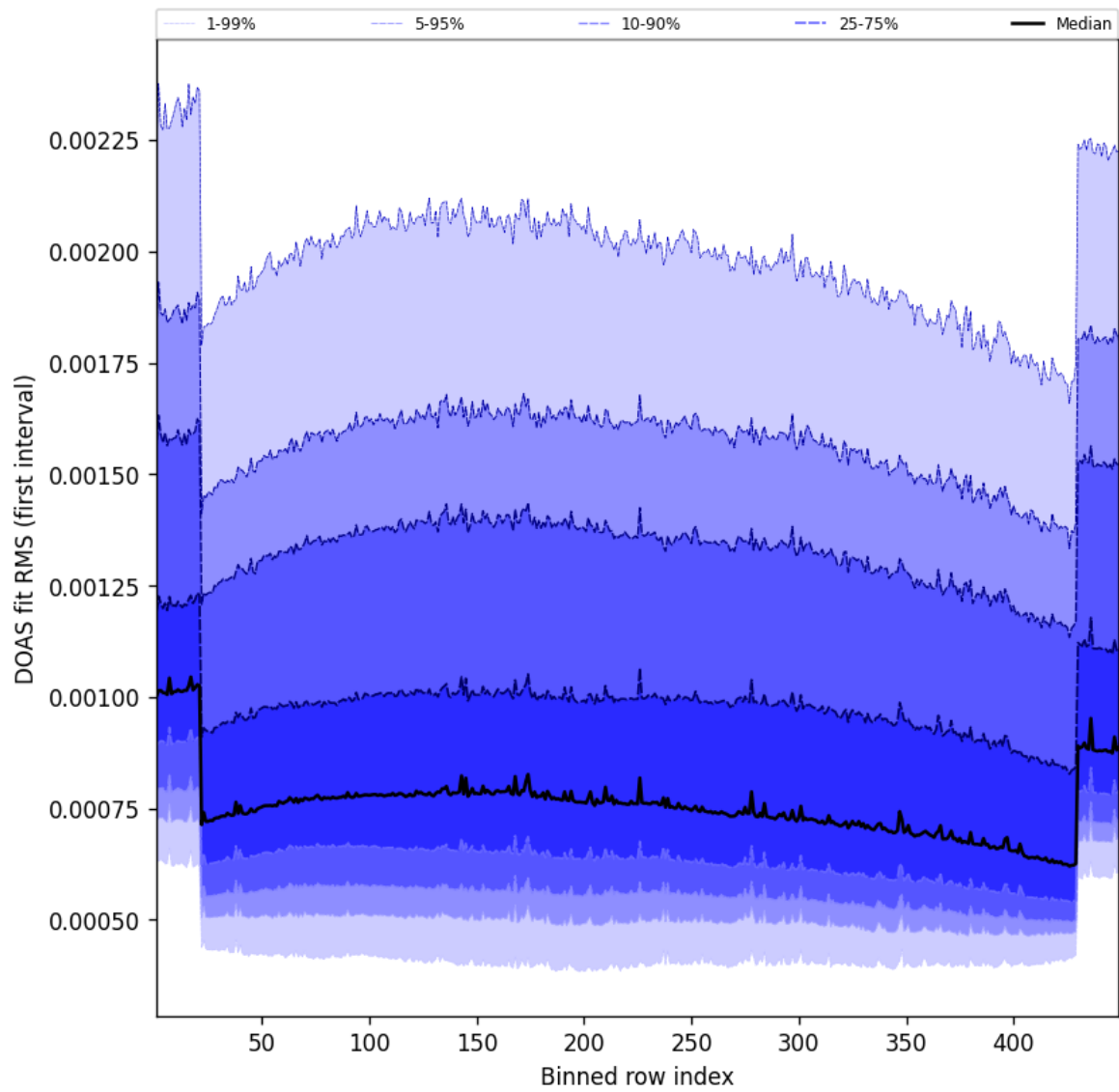
Figure 58: Along track statistics of “DOAS fit RMS (first interval)” for 2025-03-18 to 2025-03-19
