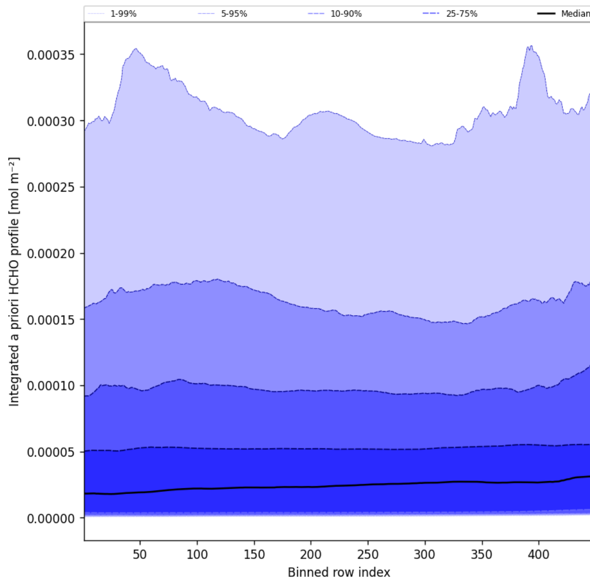
Figure 55: Along track statistics of "Integrated a priori HCHO profile" for 2025-03-18 to 2025-03-19
