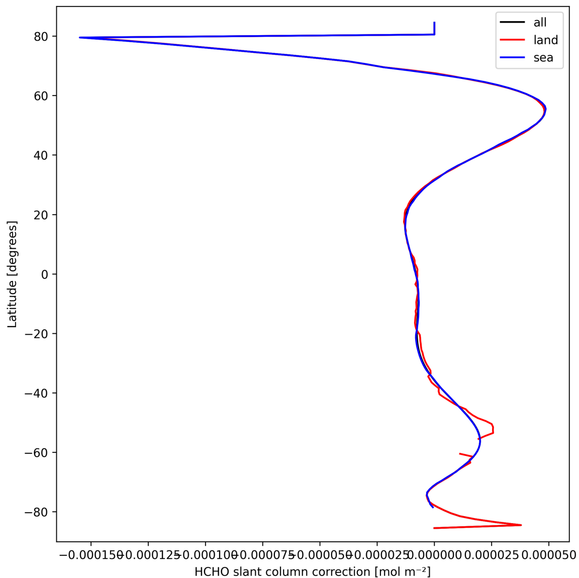
Figure 31: Zonal average of “HCHO slant column correction” for 2025-03-18 to 2025-03-19.
