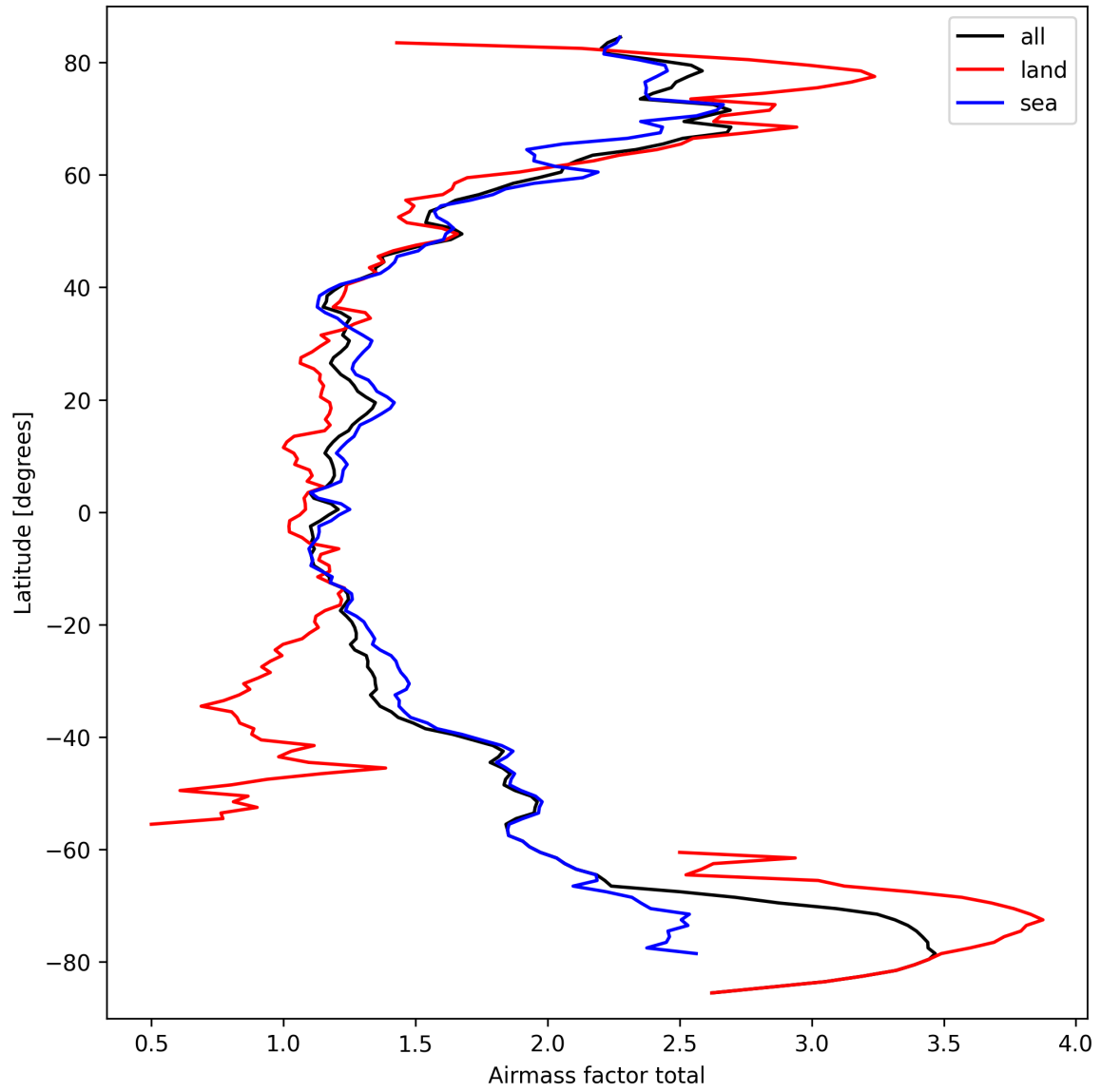
Figure 24: Zonal average of “Airmass factor total” for 2025-03-18 to 2025-03-19.
