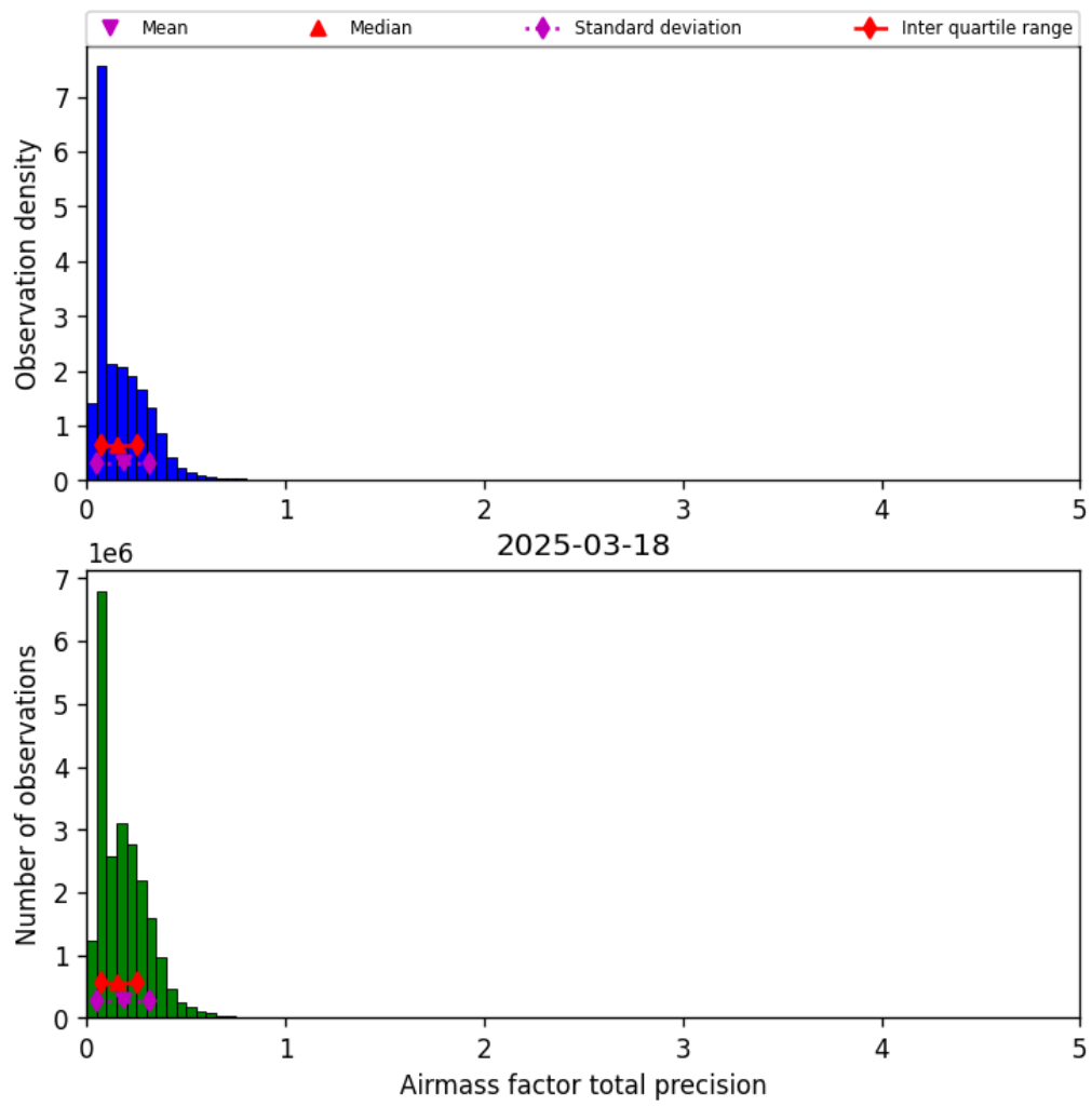
Figure 39: Histogram of “Airmass factor total precision” for 2025-03-18 to 2025-03-19
