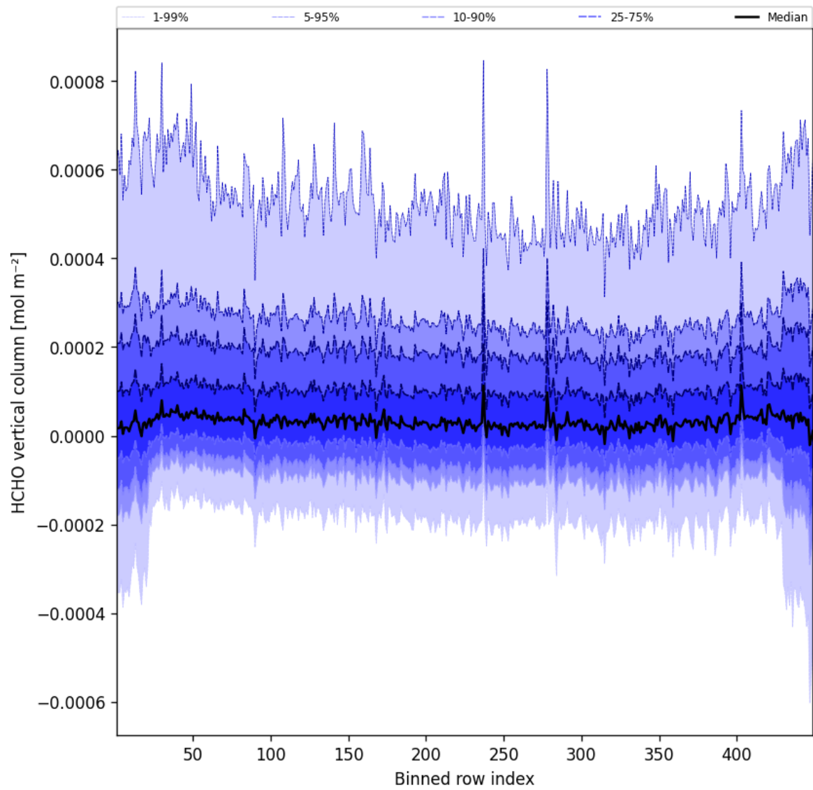
Figure 47: Along track statistics of “HCHO vertical column” for 2025-03-18 to 2025-03-19
