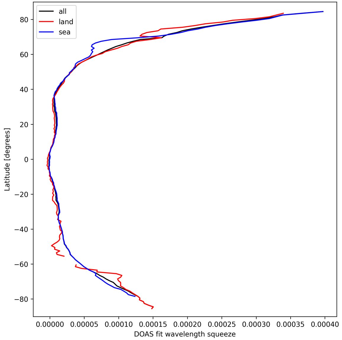
Figure 29: Zonal average of “DOAS fit wavelength squeeze” for 2025-03-18 to 2025-03-19.
