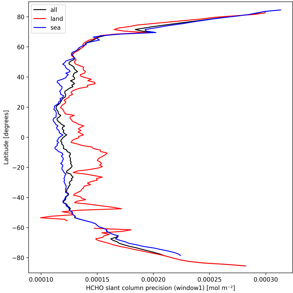
Figure 23: Zonal average of “HCHO slant column precision (window1)” for 2025-03-18 to 2025-03-19.
