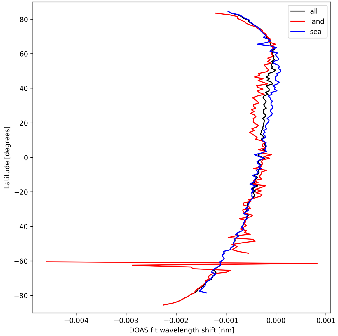
Figure 28: Zonal average of “DOAS fit wavelength shift” for 2025-03-18 to 2025-03-19.
