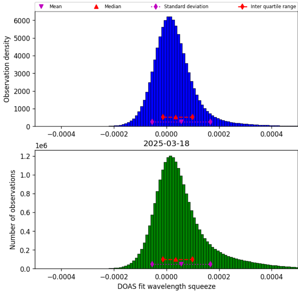
Figure 43: Histogram of “DOAS fit wavelength squeeze” for 2025-03-18 to 2025-03-19
