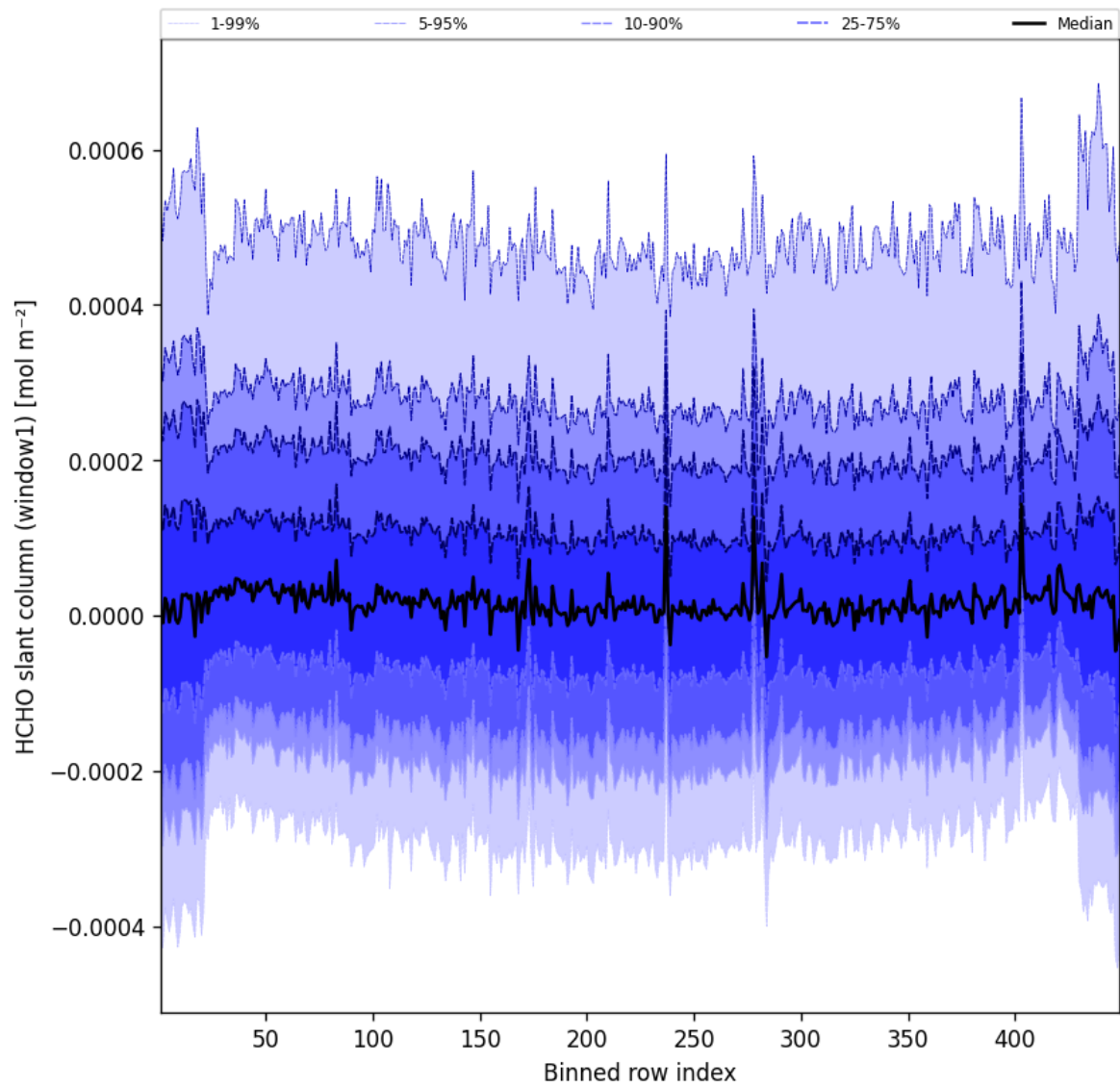
Figure 50: Along track statistics of “HCHO slant column (window1)” for 2025-03-18 to 2025-03-19
