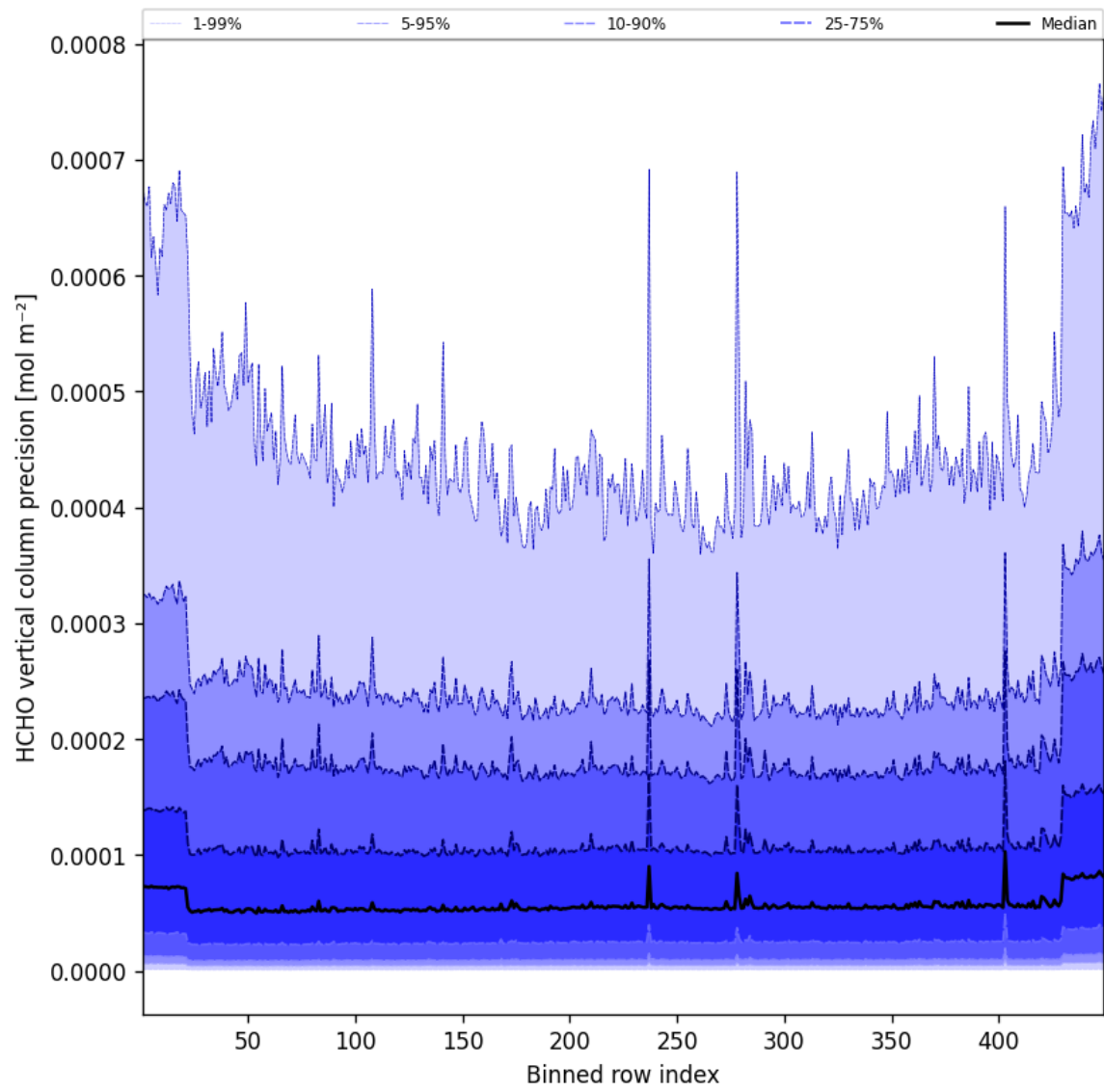
Figure 48: Along track statistics of “HCHO vertical column precision” for 2025-03-18 to 2025-03-19
