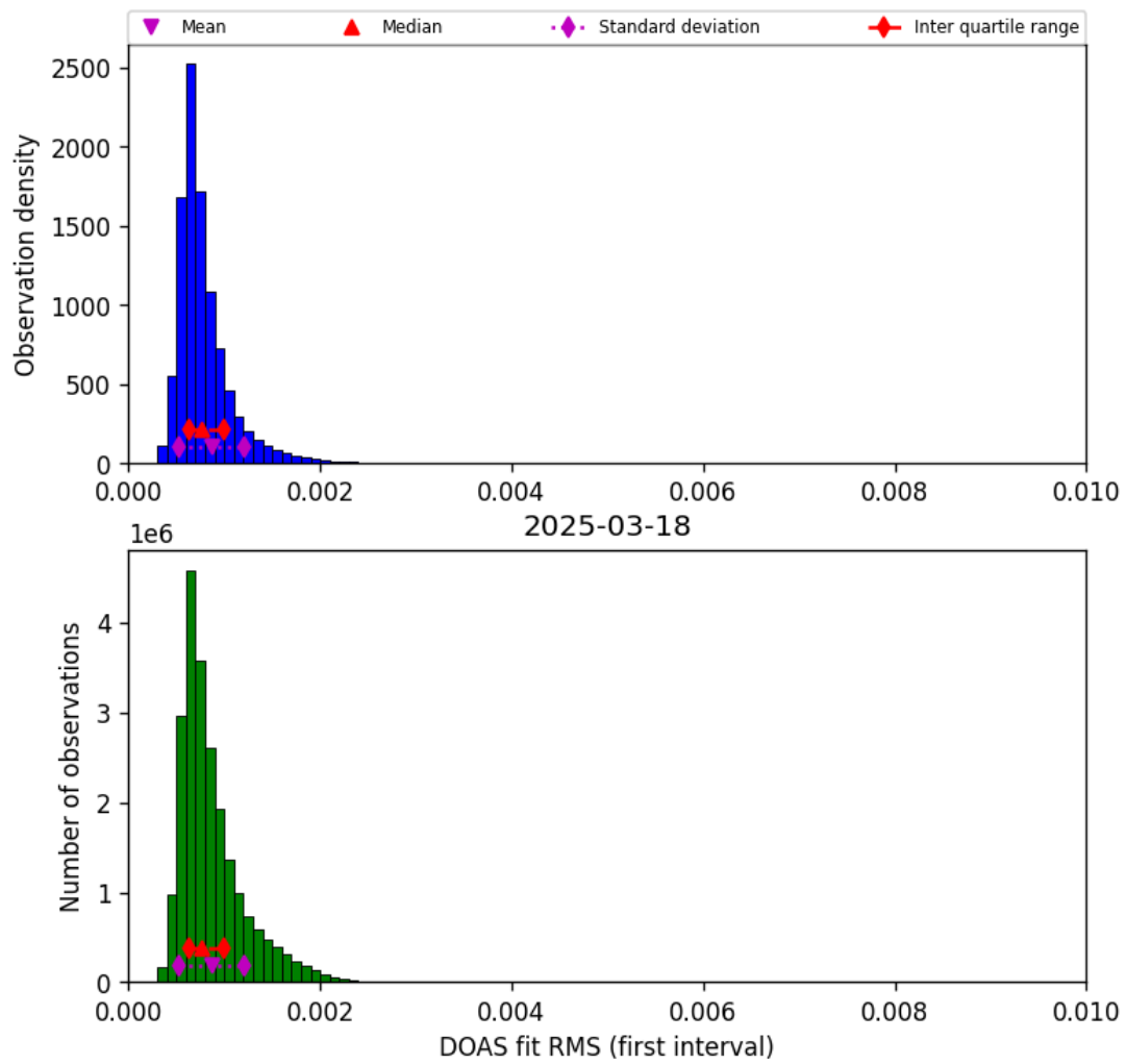
Figure 44: Histogram of "DOAS fit RMS (first interval)" for 2025-03-18 to 2025-03-19
