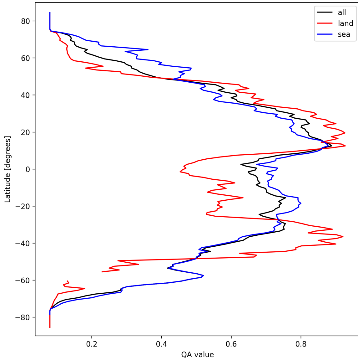
Figure 18: Zonal average of “QA value” for 2025-03-18 to 2025-03-19.
