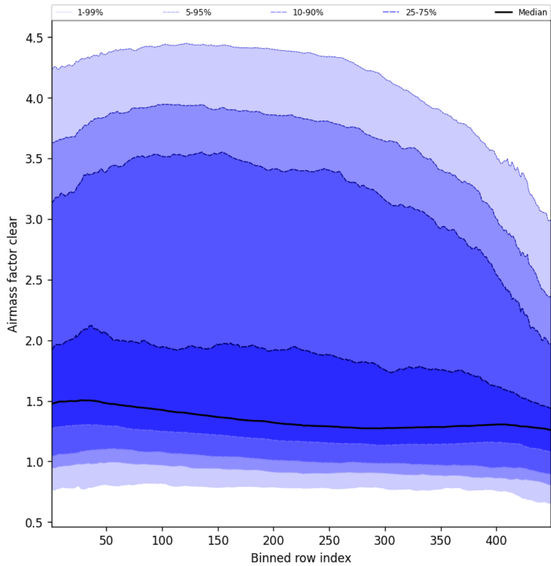
Figure 54: Along track statistics of “Airmass factor clear” for 2025-03-18 to 2025-03-19
