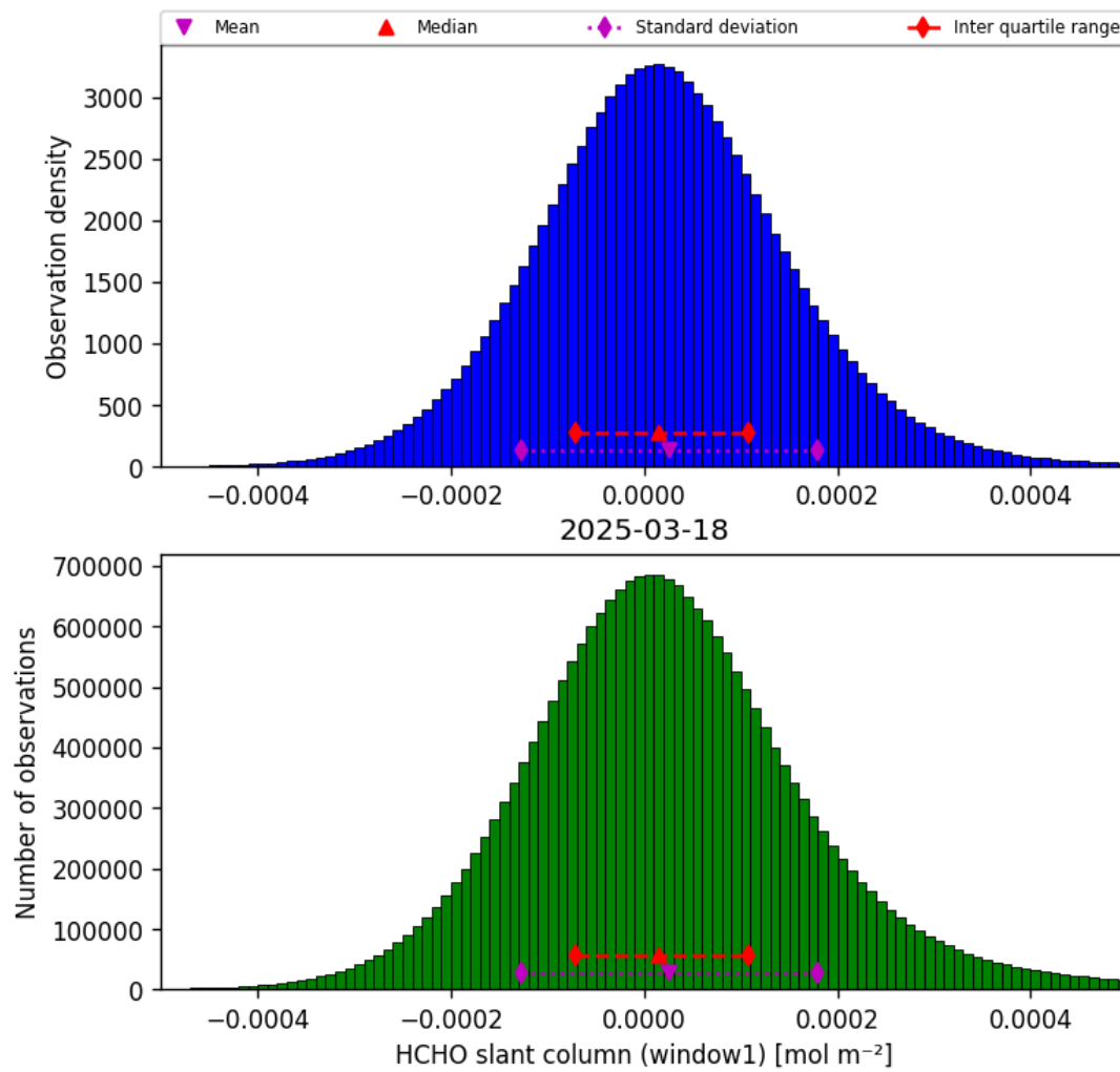
Figure 36: Histogram of “HCHO slant column (window1)” for 2025-03-18 to 2025-03-19
