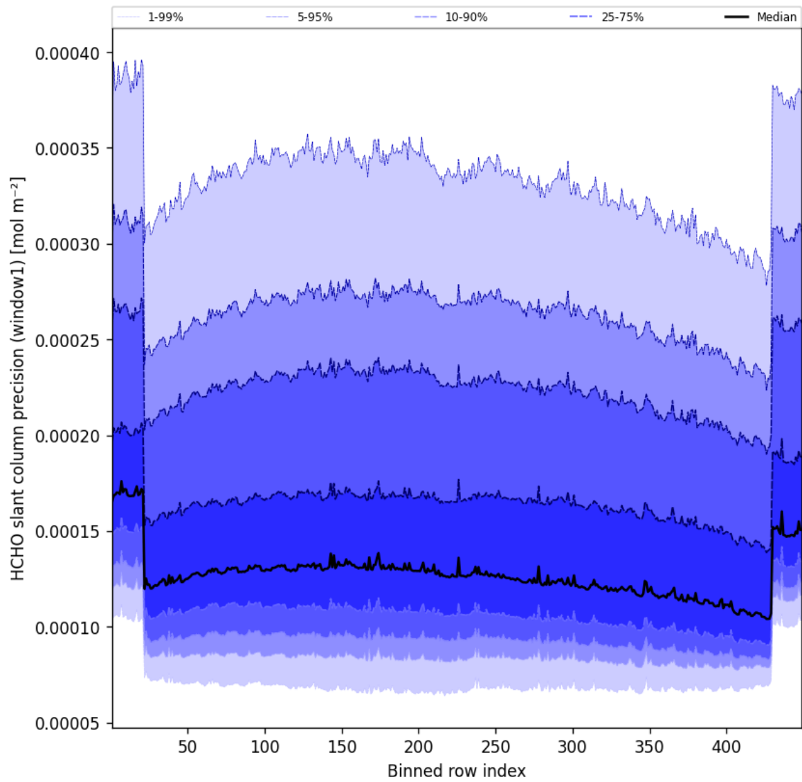
Figure 51: Along track statistics of “HCHO slant column precision (window1)” for 2025-03-18 to 2025-03-19
