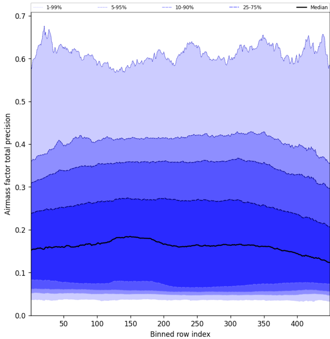
Figure 53: Along track statistics of “Airmass factor total precision” for 2025-03-18 to 2025-03-19
