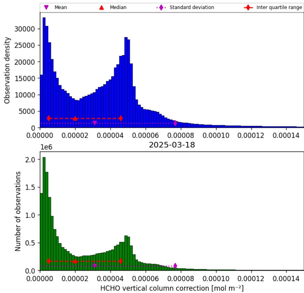
Figure 35: Histogram of “HCHO vertical column correction” for 2025-03-18 to 2025-03-19
