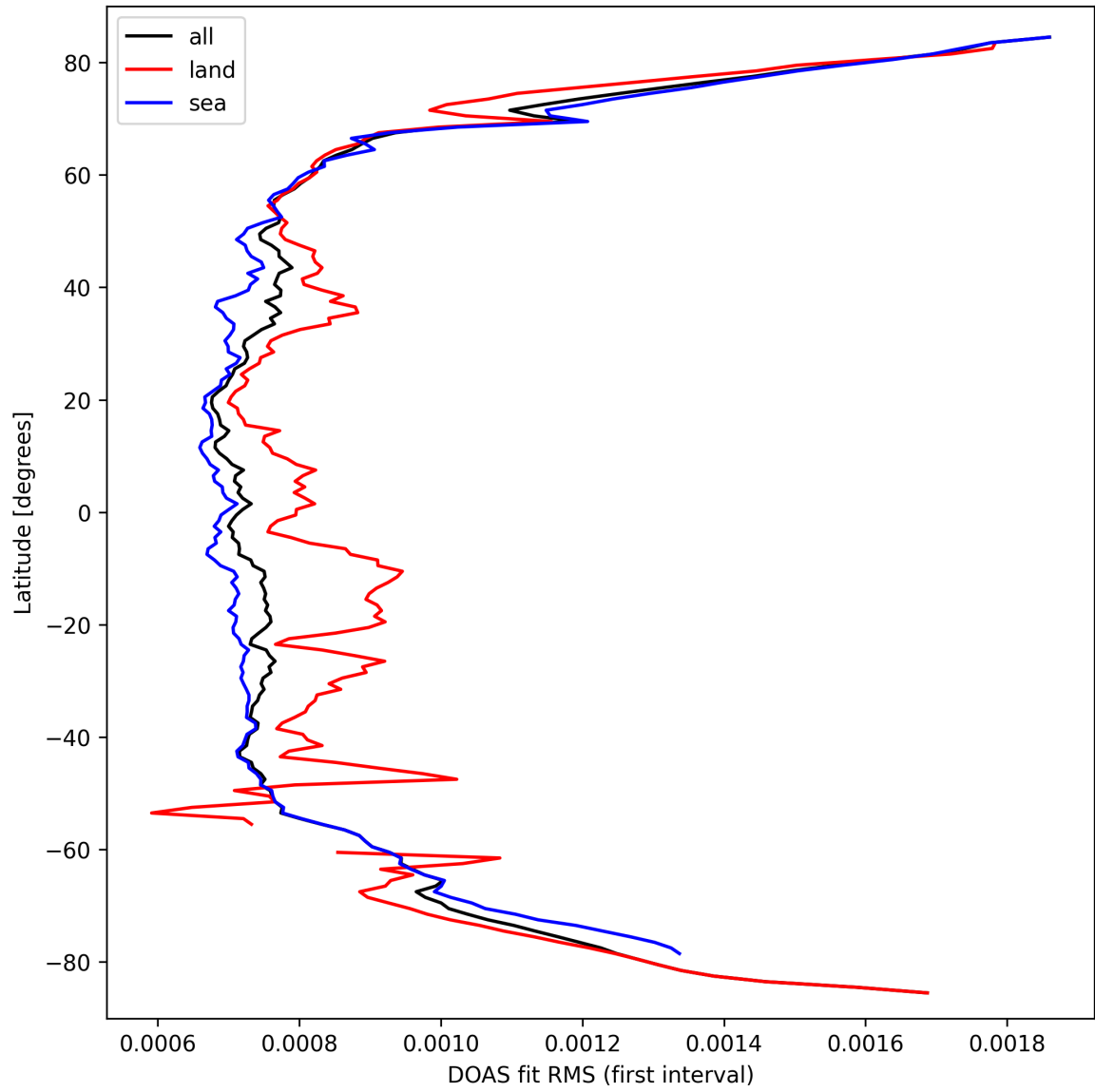
Figure 30: Zonal average of "DOAS fit RMS (first interval)" for 2025-03-18 to 2025-03-19.
