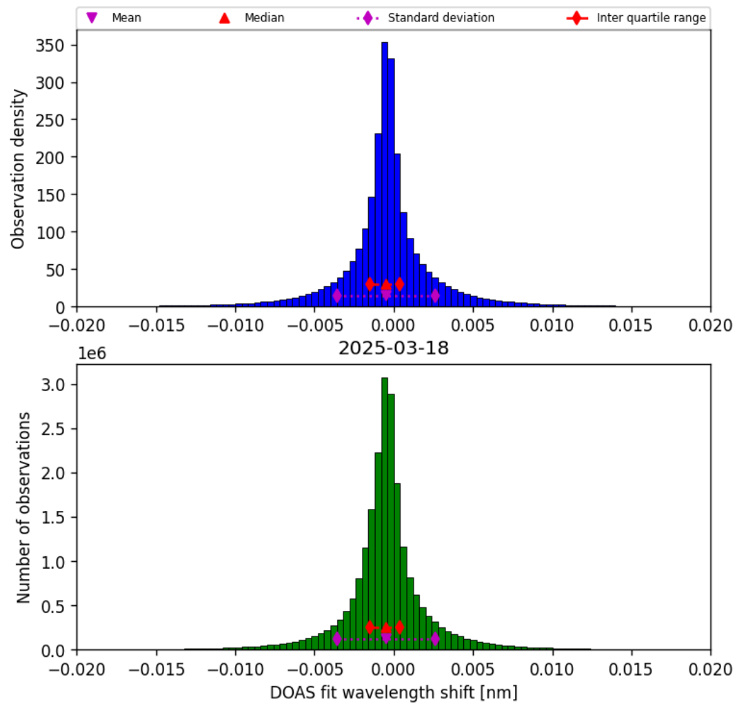
Figure 42: Histogram of “DOAS fit wavelength shift” for 2025-03-18 to 2025-03-19
