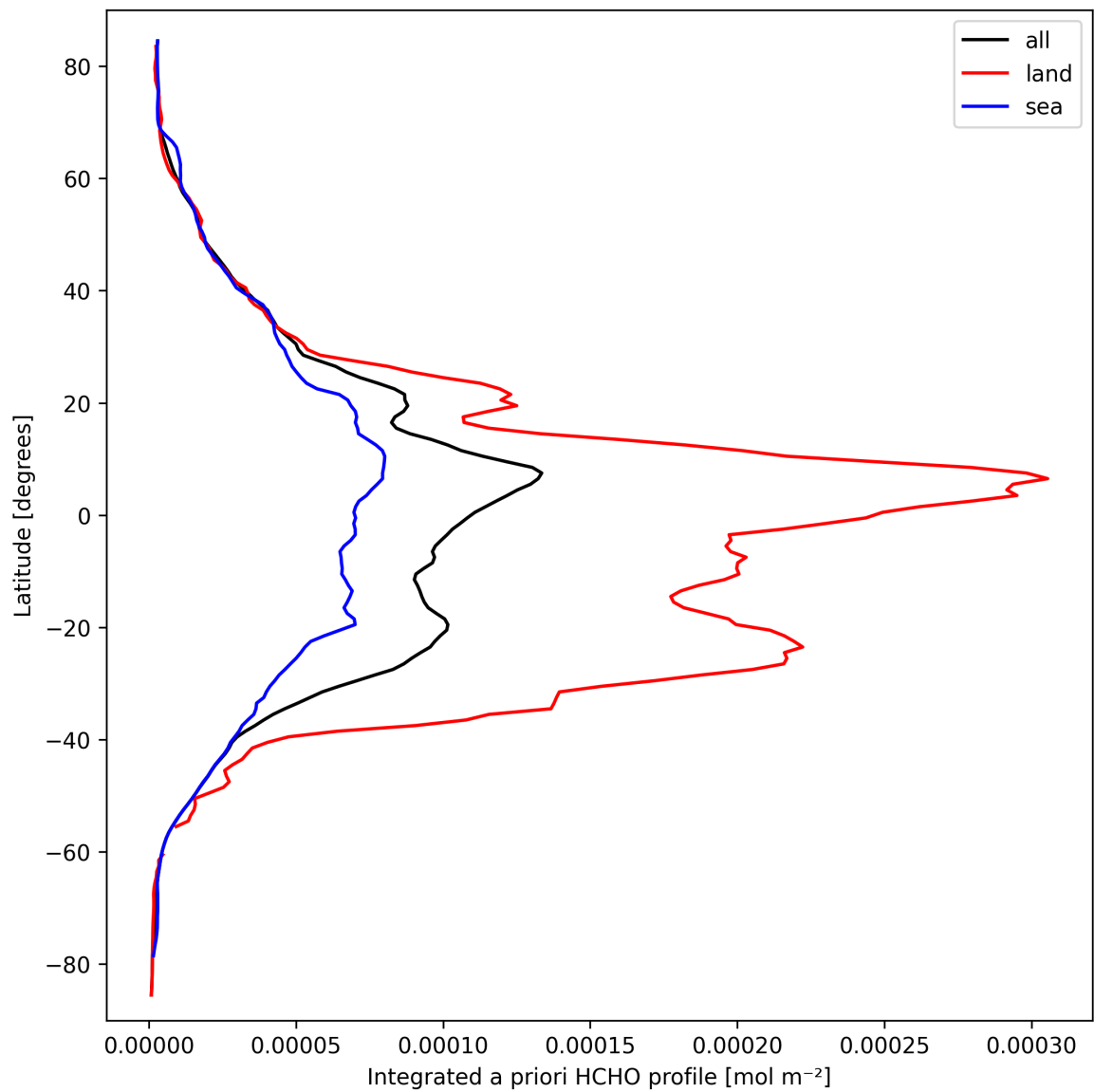
Figure 27: Zonal average of “Integrated a priori HCHO profile” for 2025-03-18 to 2025-03-19.
