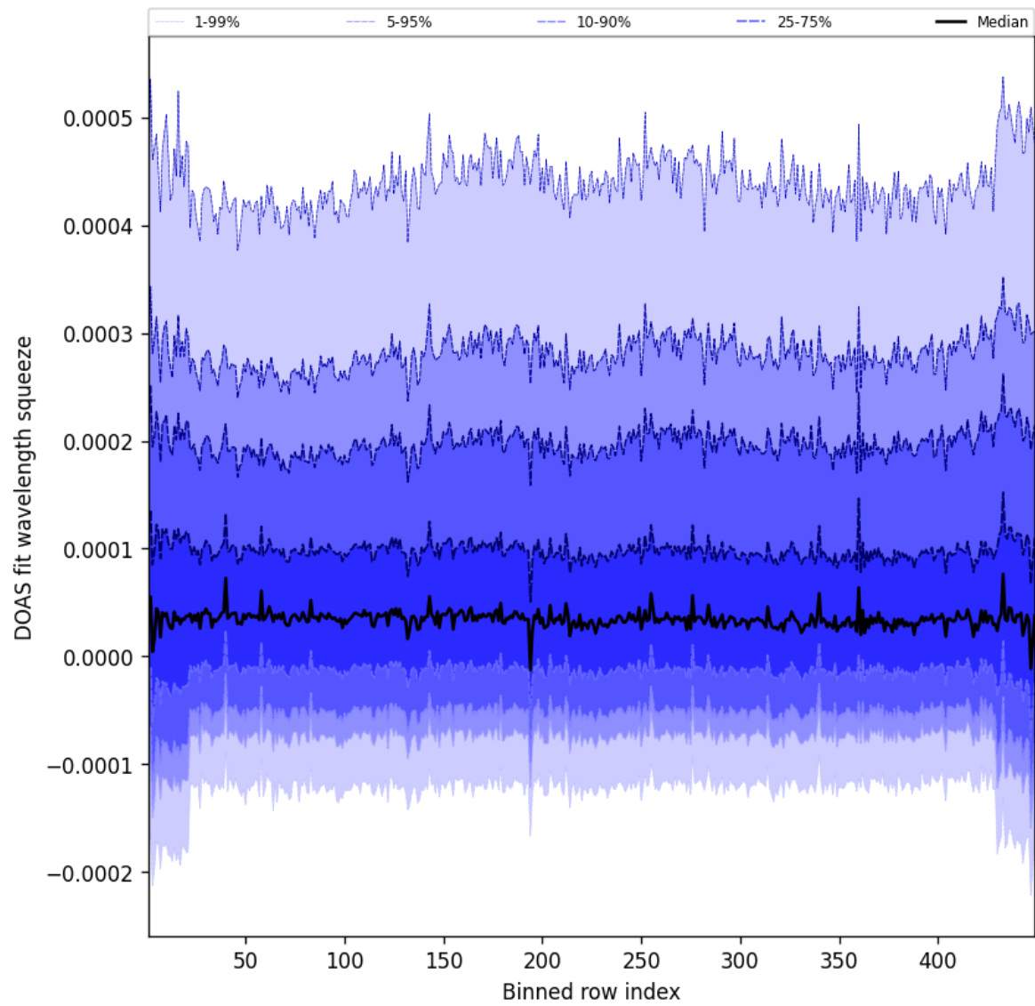
Figure 57: Along track statistics of “DOAS fit wavelength squeeze” for 2025-03-18 to 2025-03-19
