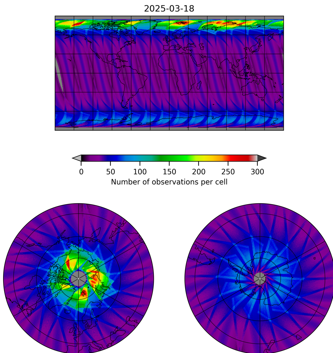
Figure 17: Map of the number of observations for 2025-03-18 to 2025-03-19
