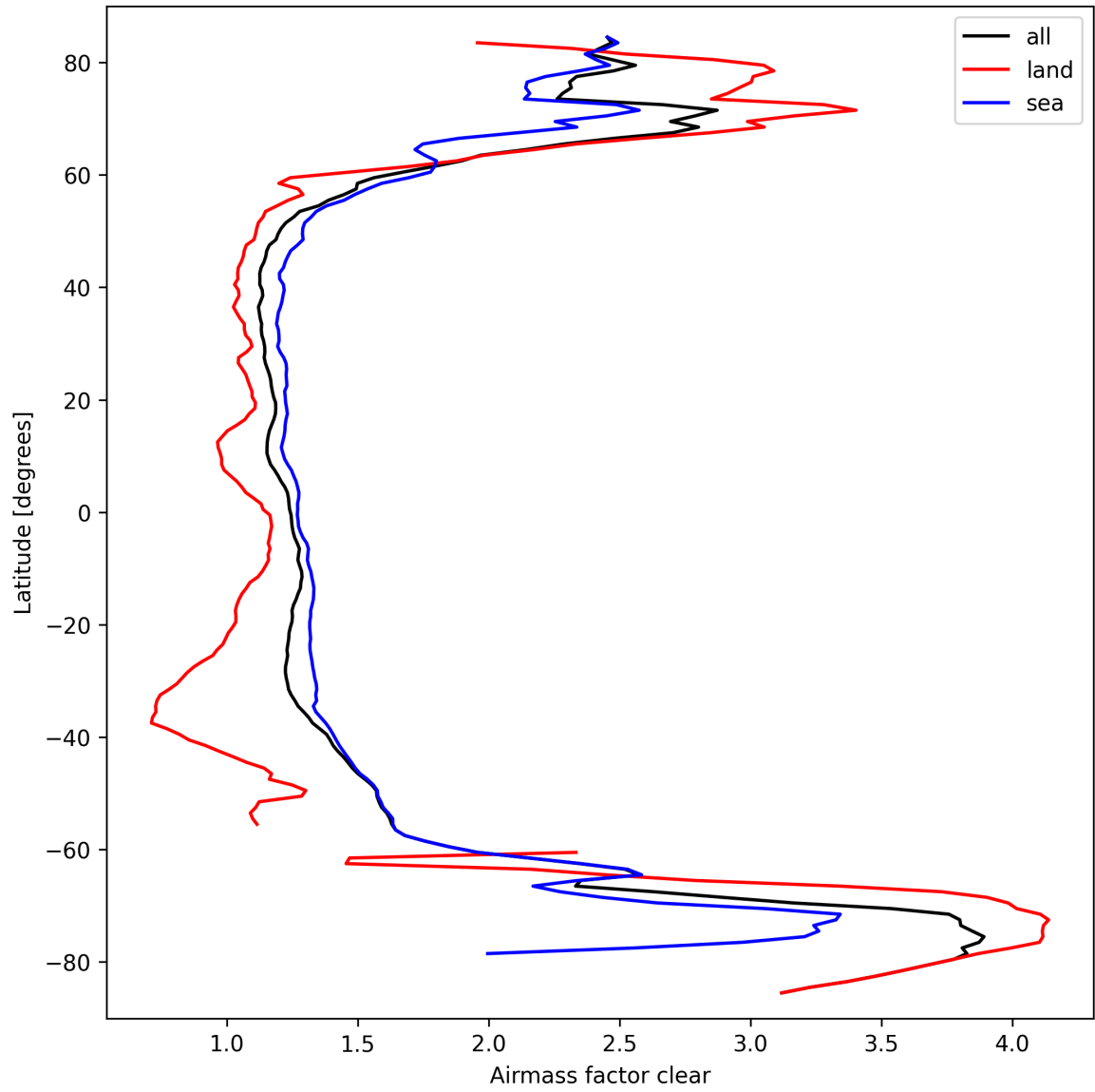
Figure 26: Zonal average of “Airmass factor clear” for 2025-03-18 to 2025-03-19.
