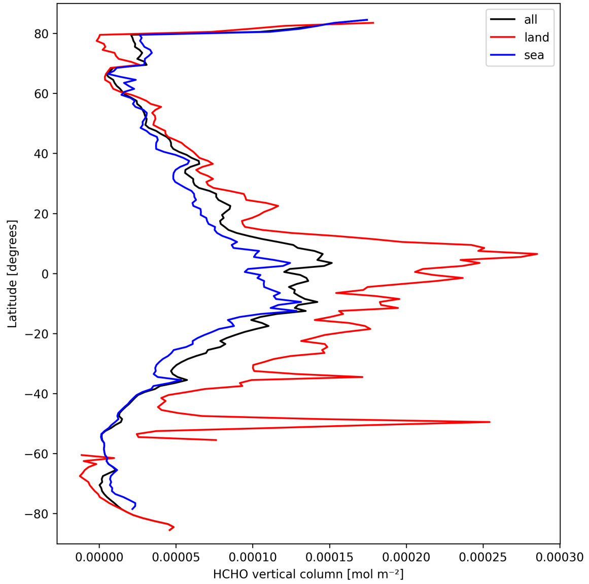
Figure 19: Zonal average of “HCHO vertical column” for 2025-03-18 to 2025-03-19.
