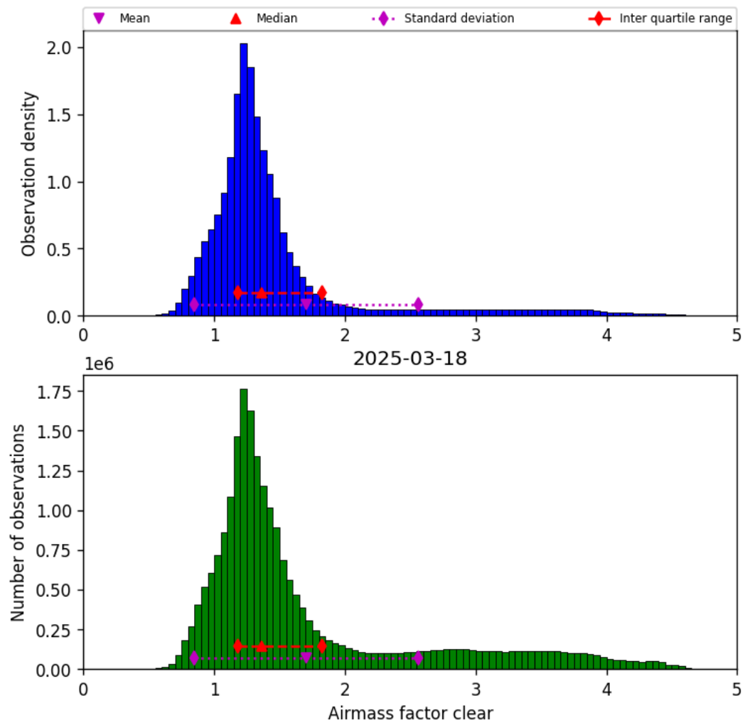
Figure 40: Histogram of “Airmass factor clear” for 2025-03-18 to 2025-03-19
