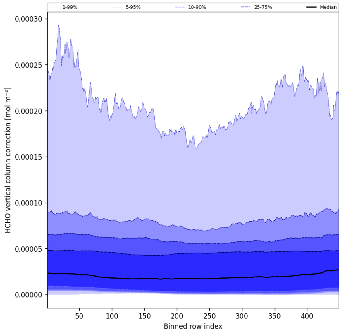
Figure 49: Along track statistics of “HCHO vertical column correction” for 2025-03-18 to 2025-03-19
