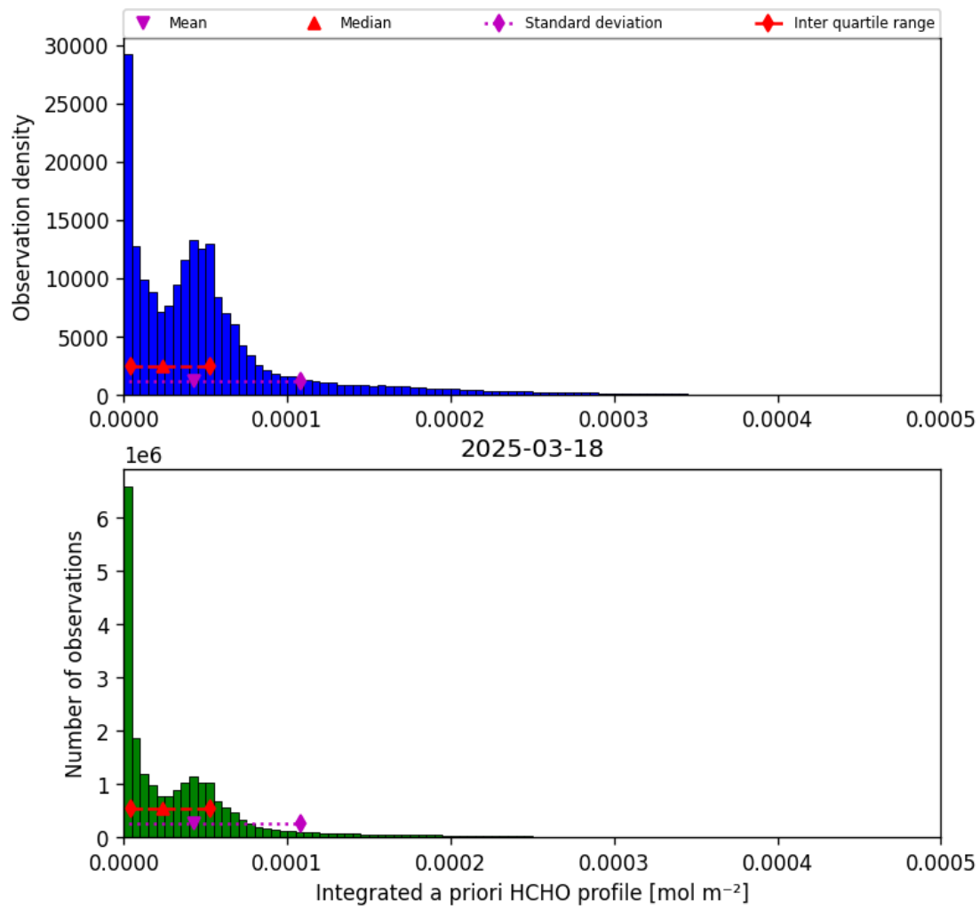
Figure 41: Histogram of “Integrated a priori HCHO profile” for 2025-03-18 to 2025-03-19
