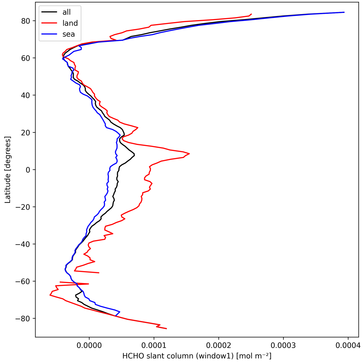
Figure 22: Zonal average of “HCHO slant column (window1)” for 2025-03-18 to 2025-03-19.
