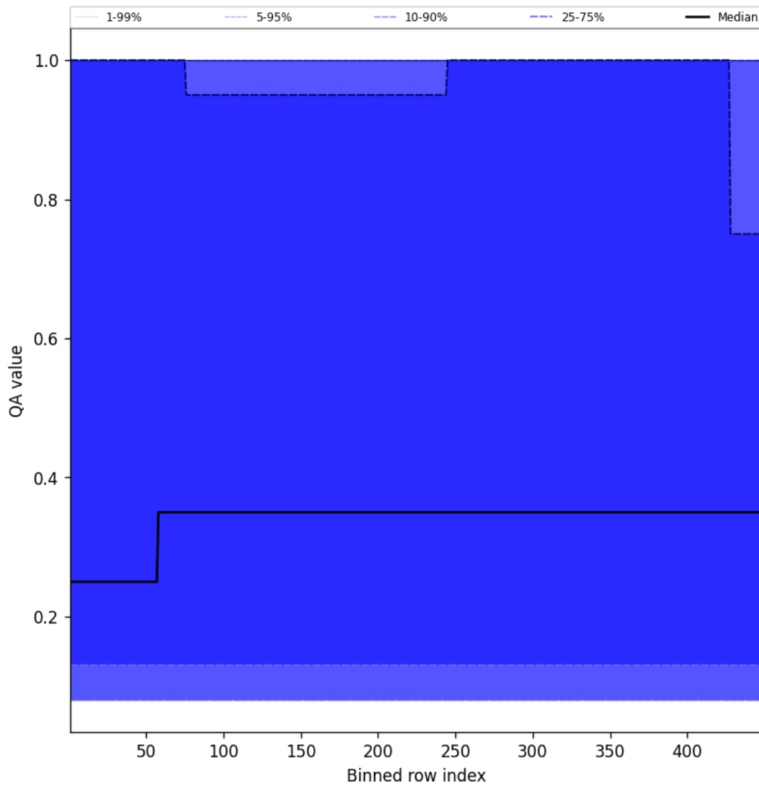
Figure 46: Along track statistics of “QA value” for 2025-03-18 to 2025-03-19
