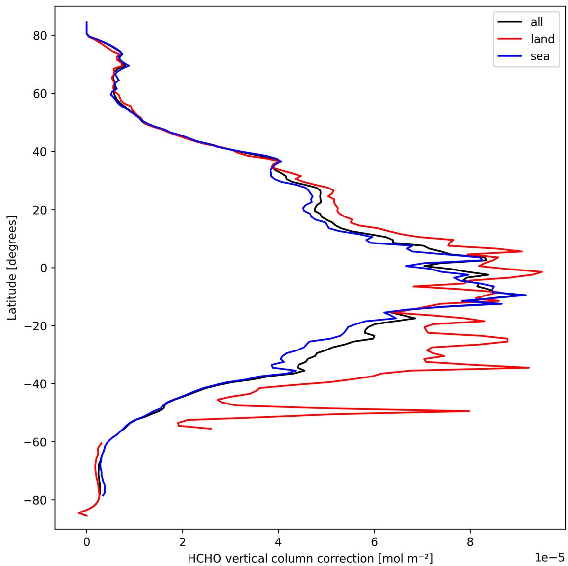
Figure 21: Zonal average of “HCHO vertical column correction” for 2025-03-18 to 2025-03-19.
