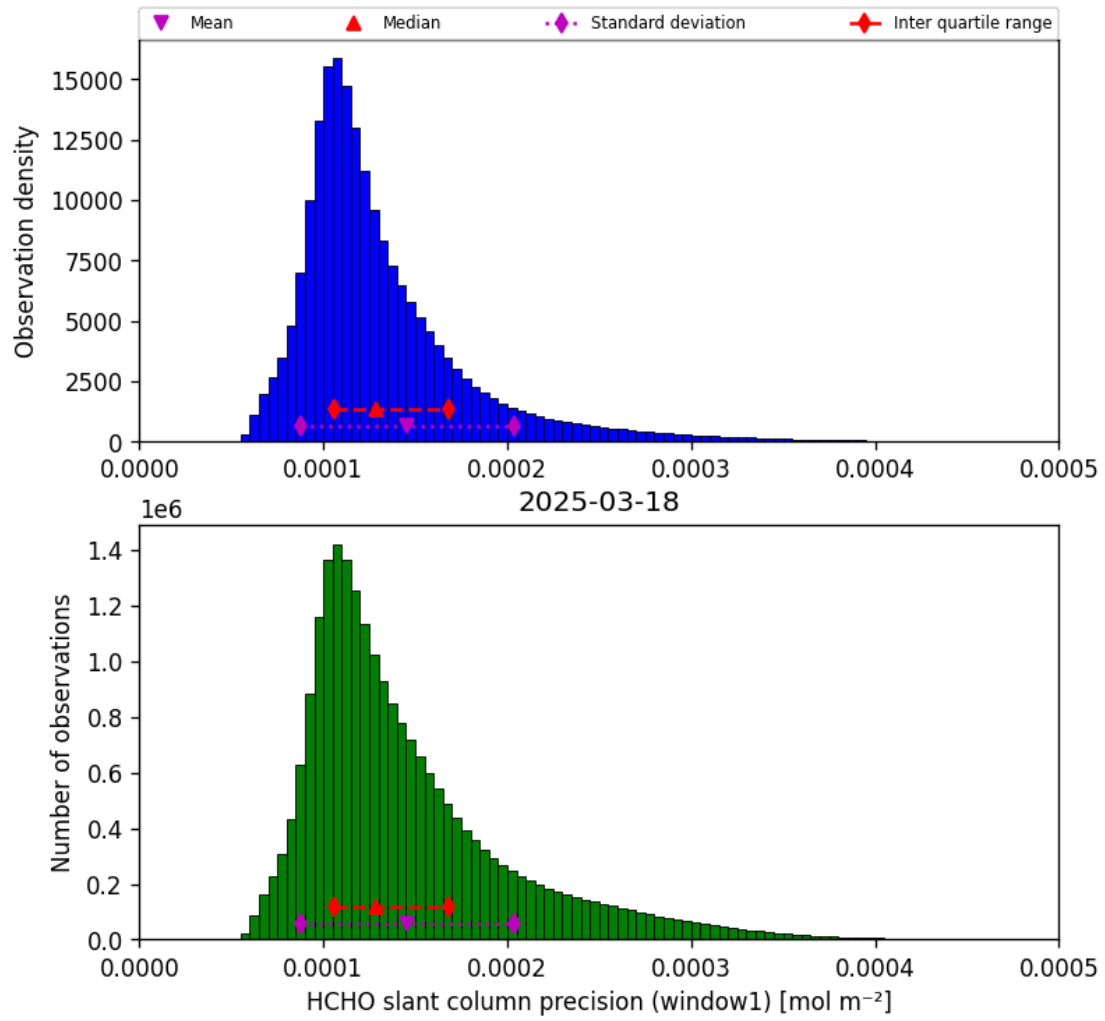
Figure 37: Histogram of “HCHO slant column precision (window1)” for 2025-03-18 to 2025-03-19
