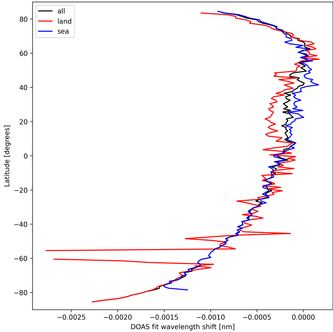
Figure 28: Zonal average of “DOAS fit wavelength shift” for 2025-03-19 to 2025-03-20.
