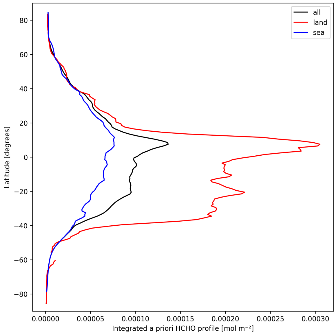
Figure 27: Zonal average of “Integrated a priori HCHO profile” for 2025-03-19 to 2025-03-20.
