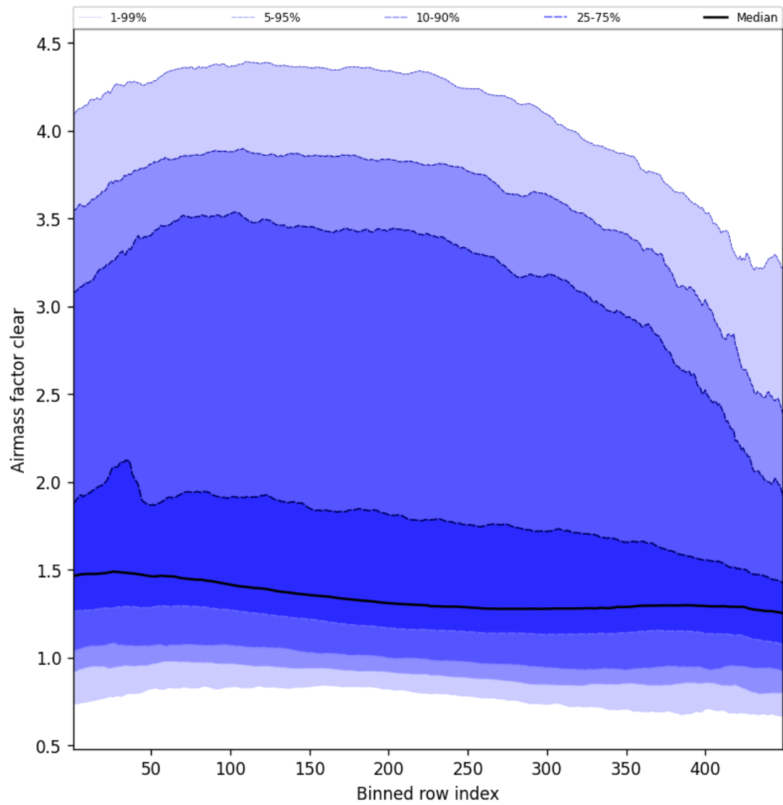
Figure 54: Along track statistics of “Airmass factor clear” for 2025-03-19 to 2025-03-20
