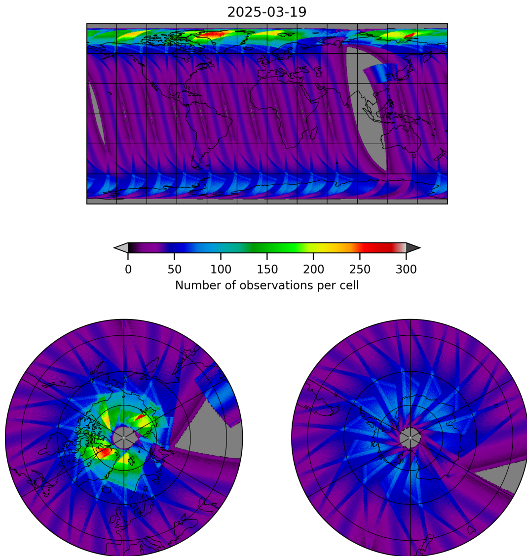
Figure 17: Map of the number of observations for 2025-03-19 to 2025-03-20
