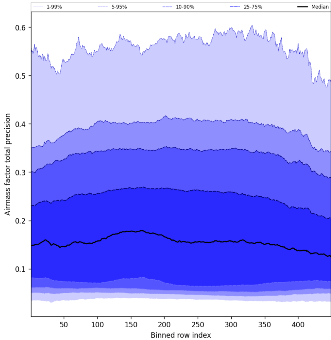
Figure 53: Along track statistics of “Airmass factor total precision” for 2025-03-19 to 2025-03-20
