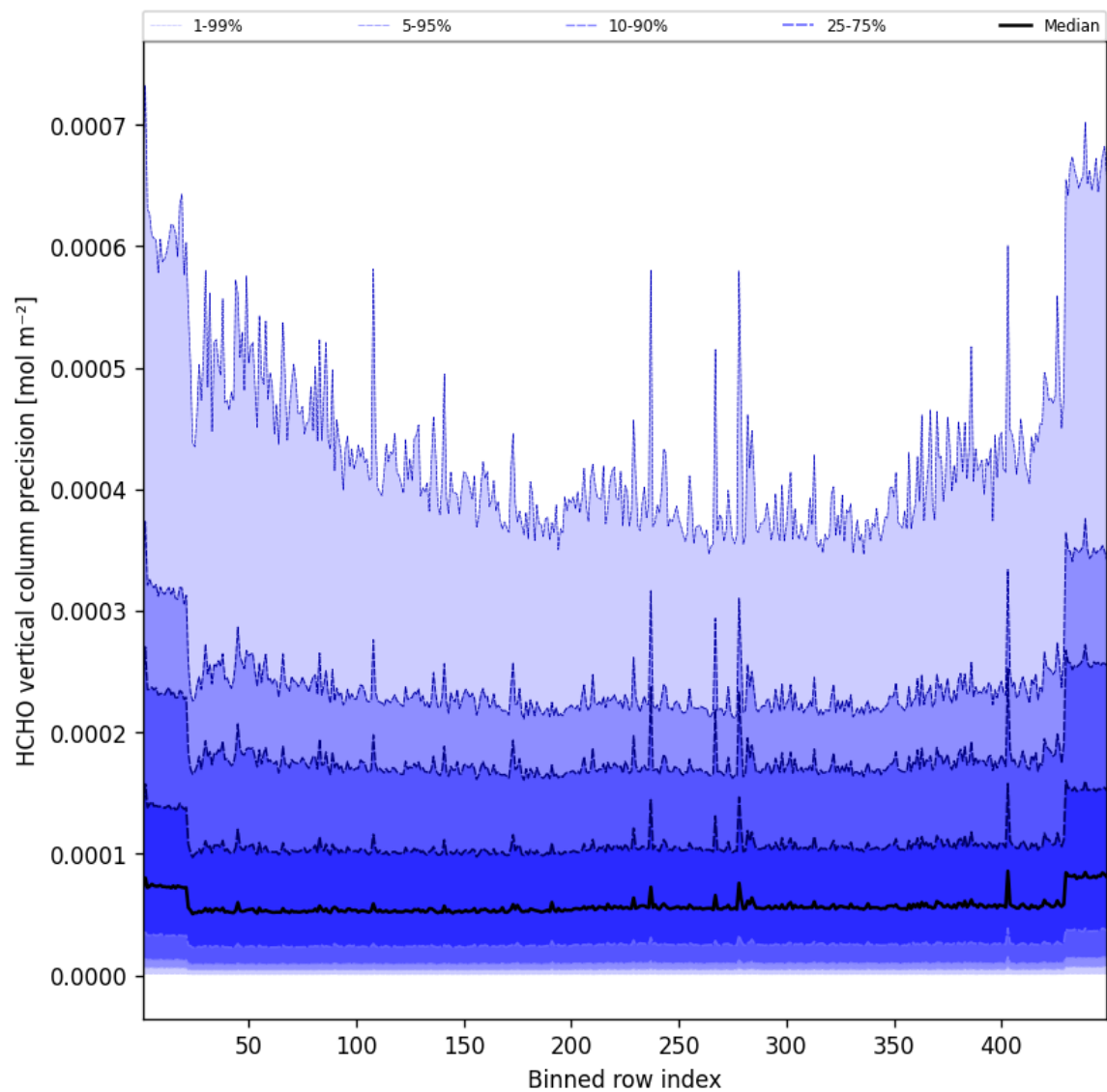
Figure 48: Along track statistics of "HCHO vertical column precision" for 2025-03-19 to 2025-03-20
