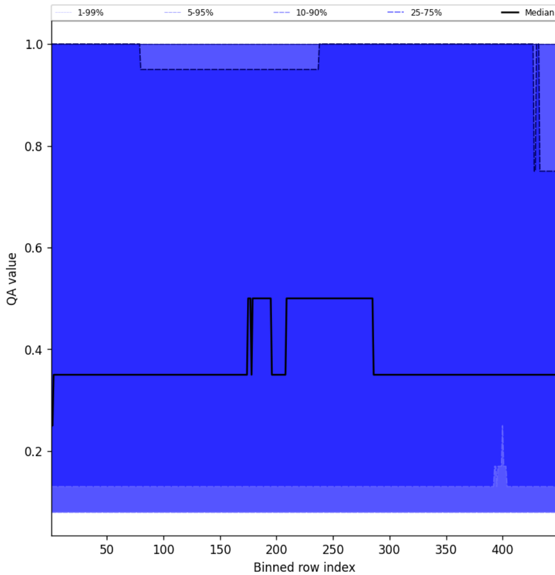
Figure 46: Along track statistics of “QA value” for 2025-03-19 to 2025-03-20
