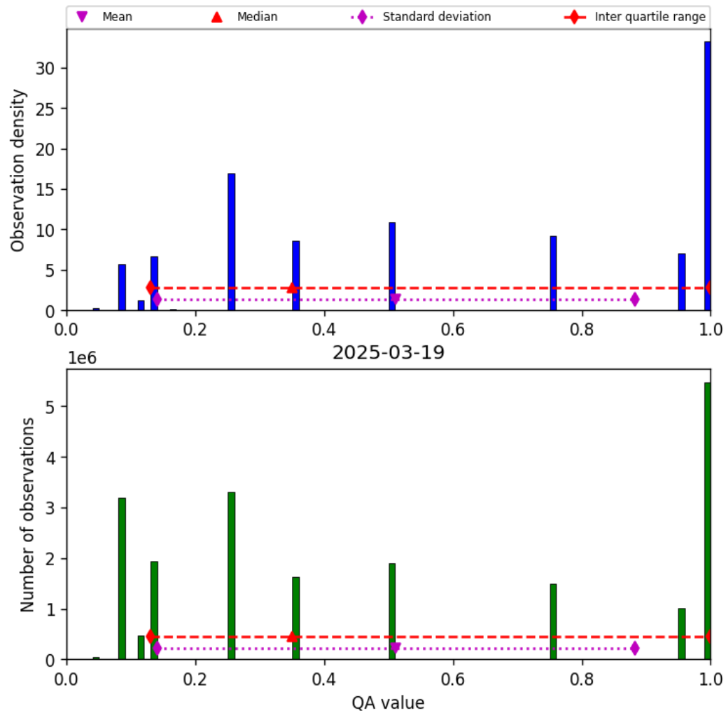
Figure 32: Histogram of “QA value” for 2025-03-19 to 2025-03-20
