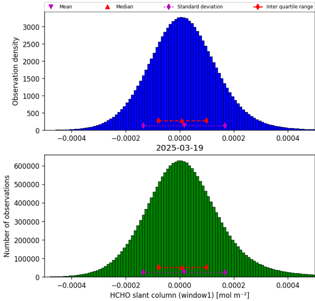
Figure 36: Histogram of “HCHO slant column (window1)” for 2025-03-19 to 2025-03-20
