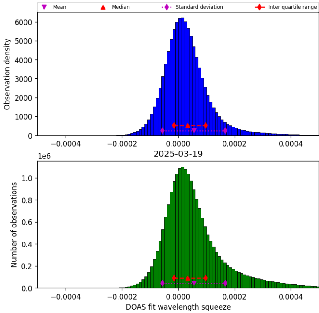
Figure 43: Histogram of “DOAS fit wavelength squeeze” for 2025-03-19 to 2025-03-20
