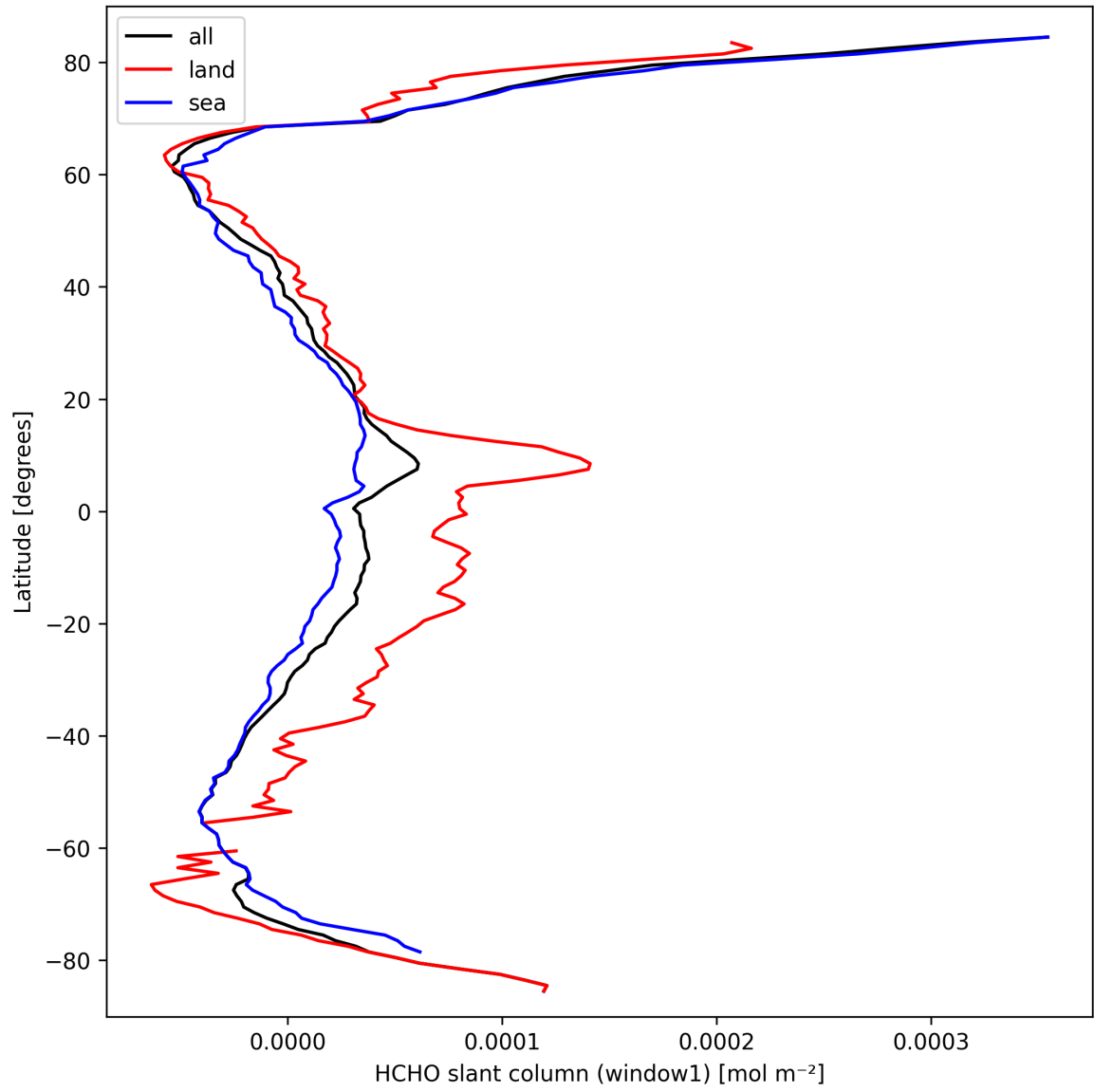
Figure 22: Zonal average of “HCHO slant column (window1)” for 2025-03-19 to 2025-03-20.
