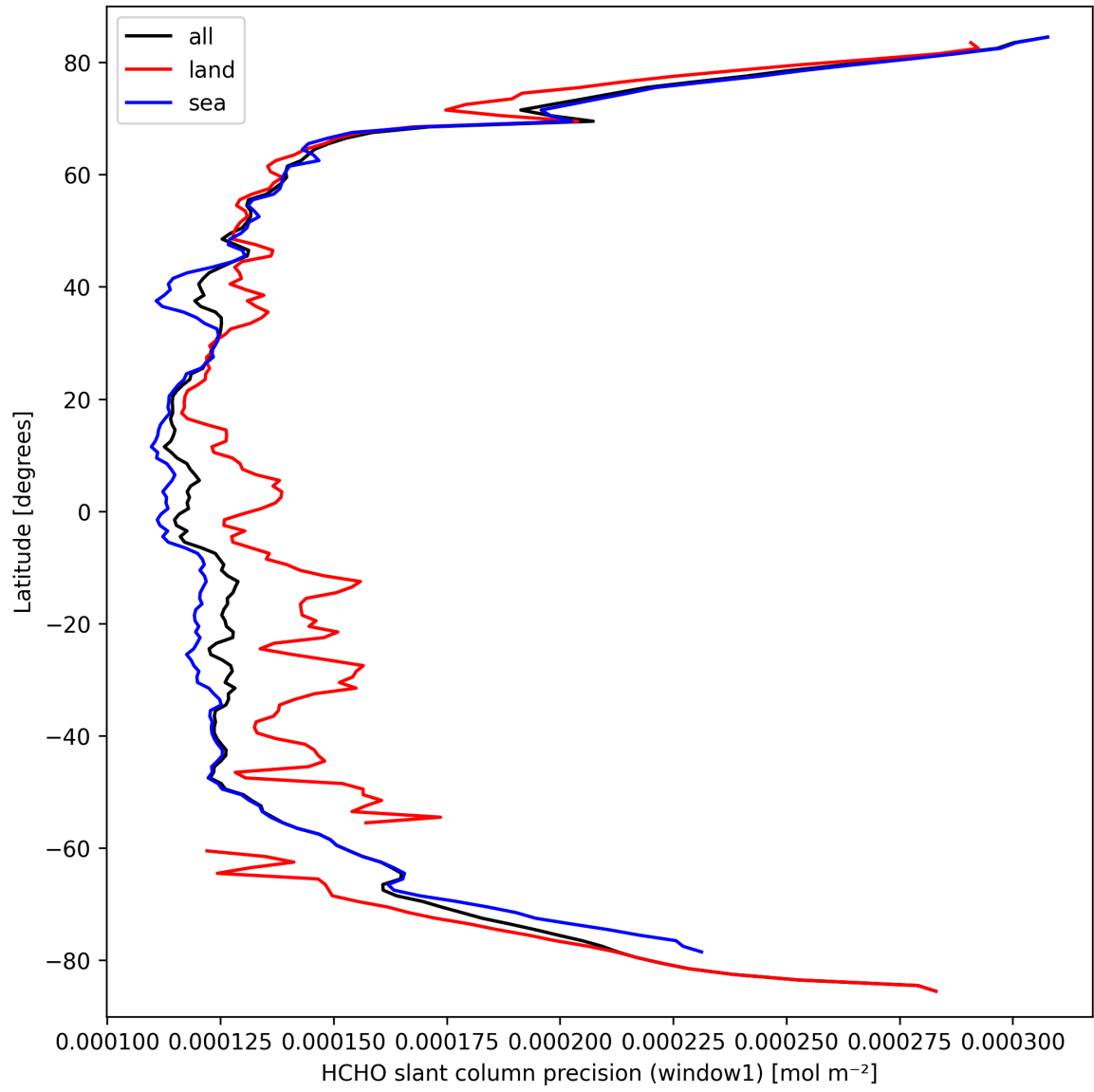
Figure 23: Zonal average of “HCHO slant column precision (window1)” for 2025-03-19 to 2025-03-20.
