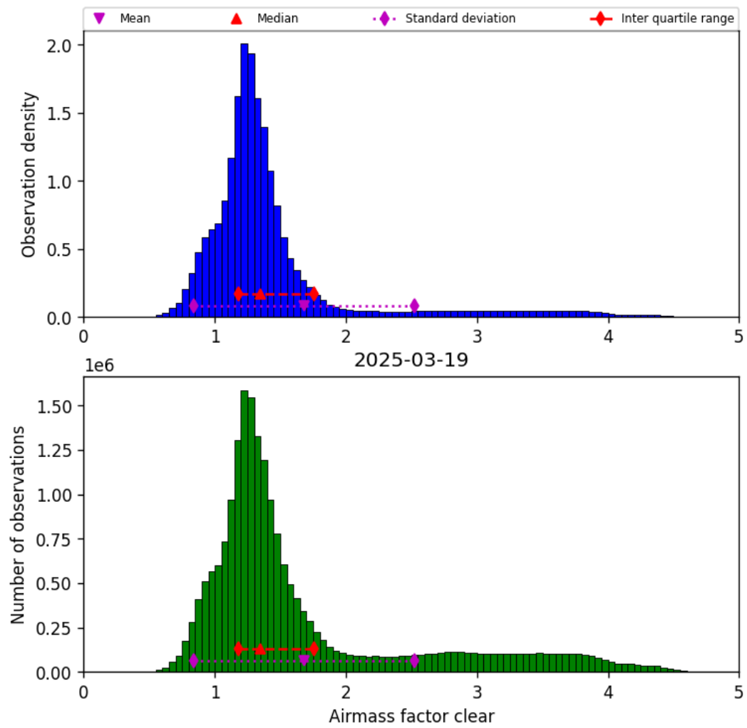
Figure 40: Histogram of “Airmass factor clear” for 2025-03-19 to 2025-03-20
