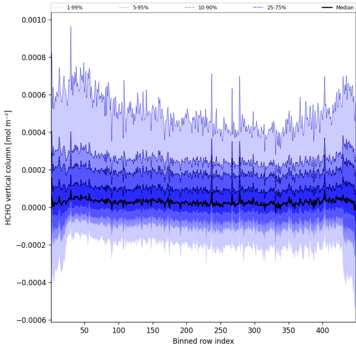
Figure 47: Along track statistics of “HCHO vertical column” for 2025-03-19 to 2025-03-20
