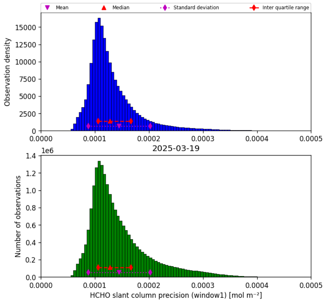
Figure 37: Histogram of “HCHO slant column precision (window1)” for 2025-03-19 to 2025-03-20
