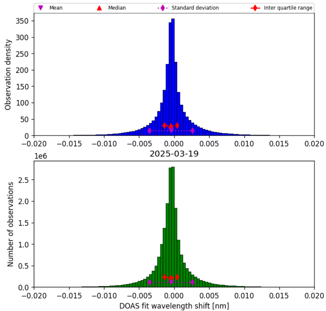
Figure 42: Histogram of “DOAS fit wavelength shift” for 2025-03-19 to 2025-03-20
