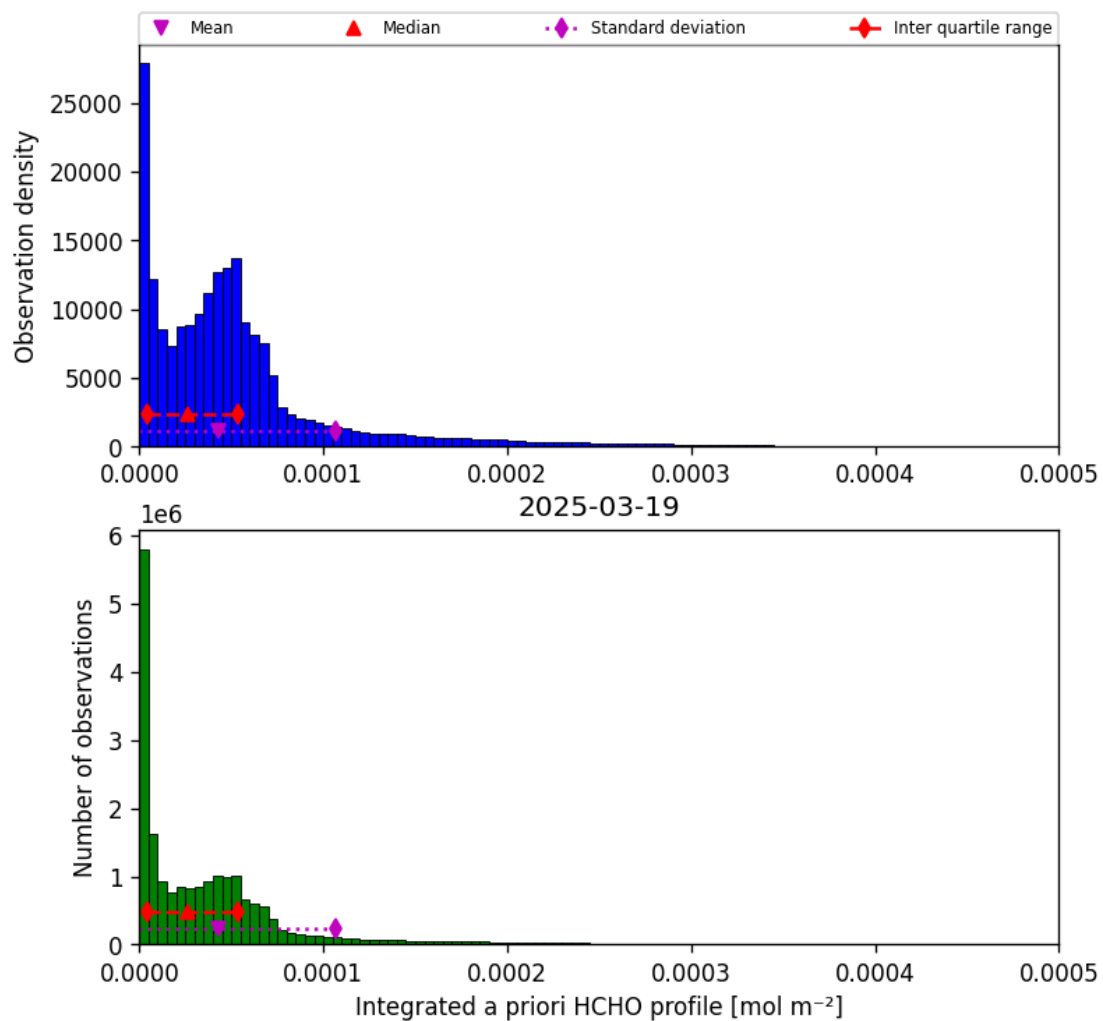
Figure 41: Histogram of “Integrated a priori HCHO profile” for 2025-03-19 to 2025-03-20
