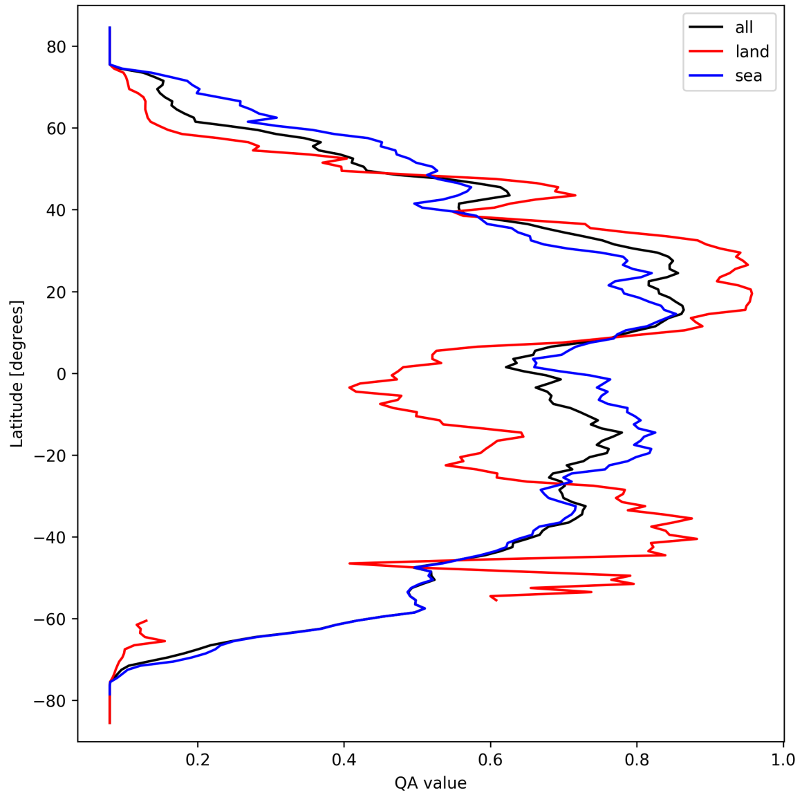
Figure 18: Zonal average of “QA value” for 2025-03-19 to 2025-03-20.
