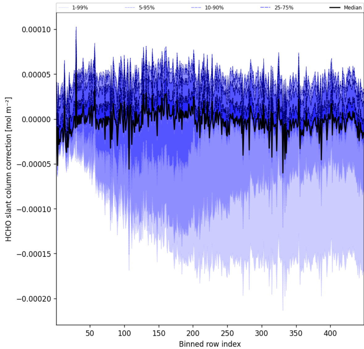
Figure 59: Along track statistics of “HCHO slant column correction” for 2025-03-19 to 2025-03-20
