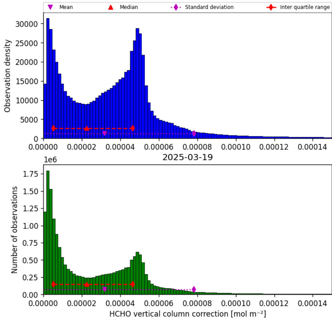
Figure 35: Histogram of “HCHO vertical column correction” for 2025-03-19 to 2025-03-20
