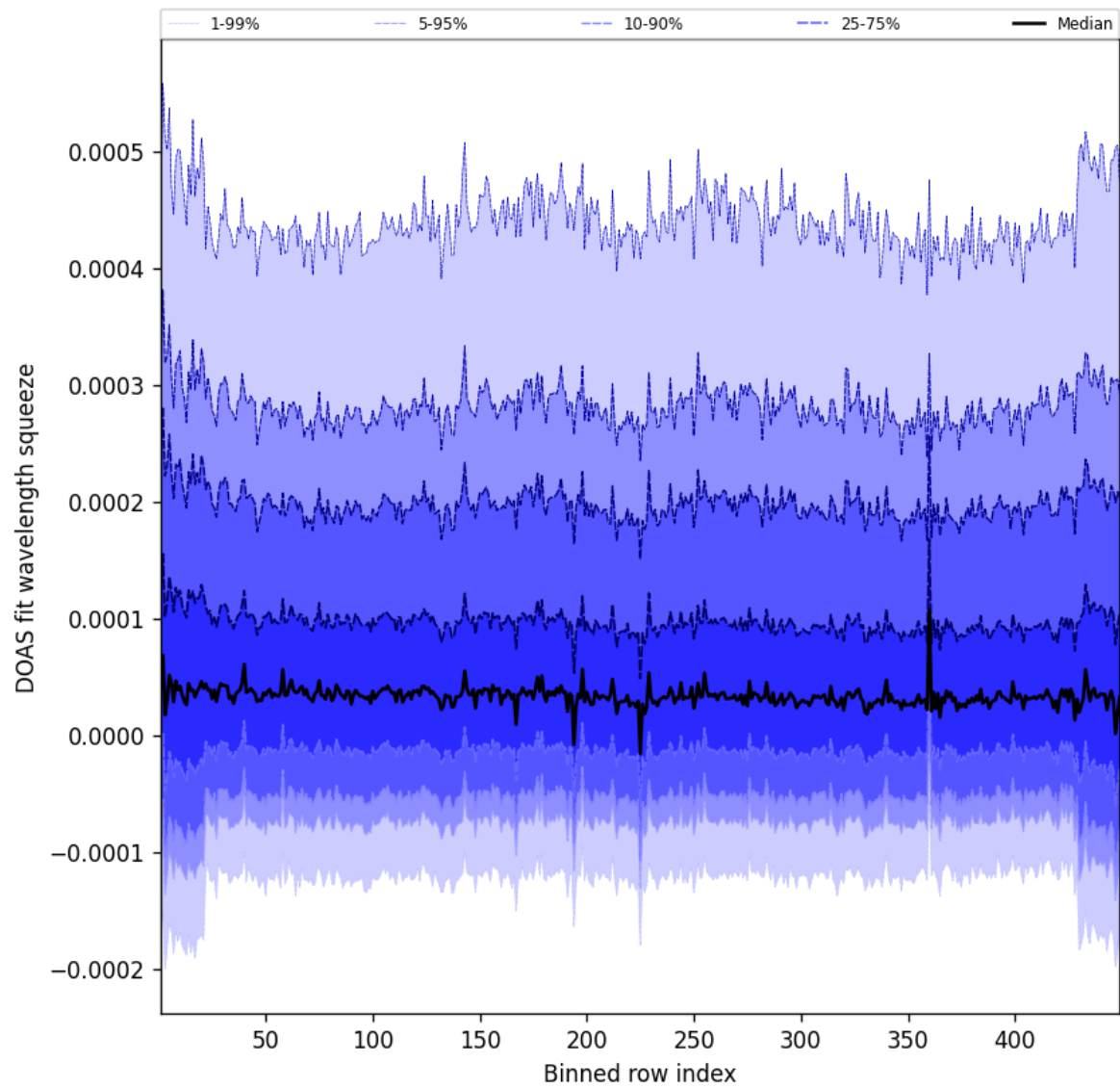
Figure 57: Along track statistics of “DOAS fit wavelength squeeze” for 2025-03-19 to 2025-03-20
