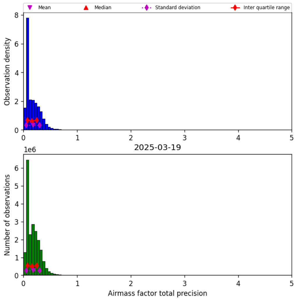
Figure 39: Histogram of “Airmass factor total precision” for 2025-03-19 to 2025-03-20
