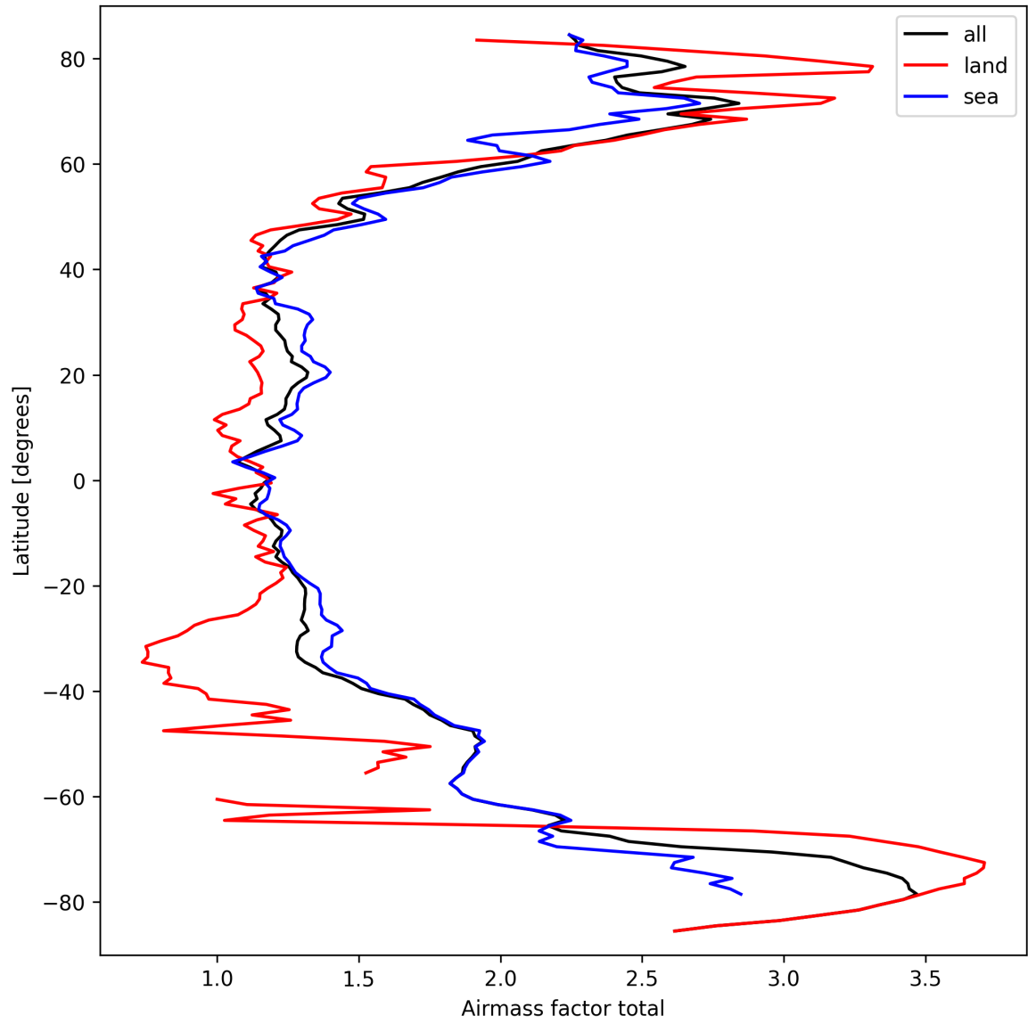
Figure 24: Zonal average of “Airmass factor total” for 2025-03-19 to 2025-03-20.
