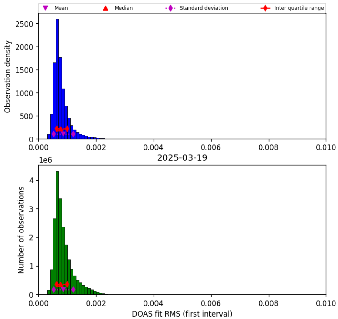
Figure 44: Histogram of “DOAS fit RMS (first interval)” for 2025-03-19 to 2025-03-20
