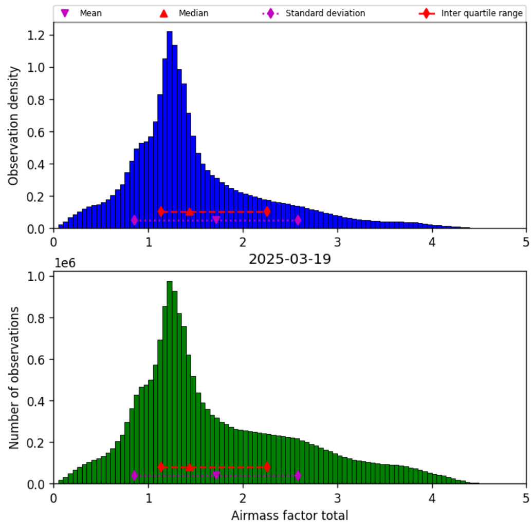
Figure 38: Histogram of “Airmass factor total” for 2025-03-19 to 2025-03-20
