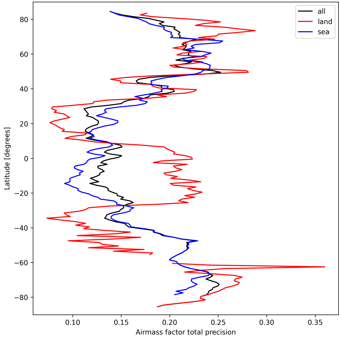
Figure 25: Zonal average of “Airmass factor total precision” for 2025-03-19 to 2025-03-20.
