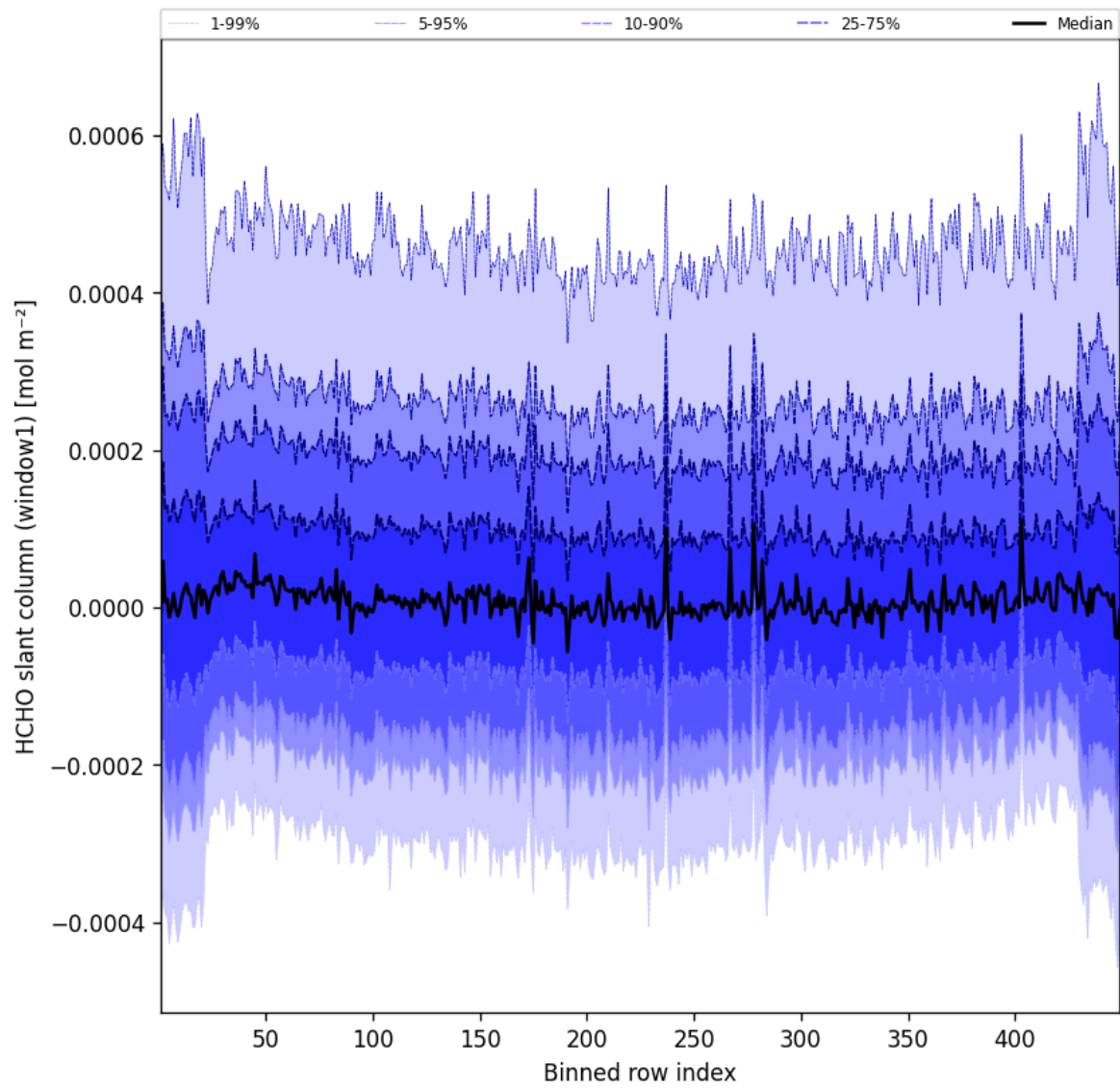
Figure 50: Along track statistics of “HCHO slant column (window1)” for 2025-03-19 to 2025-03-20
