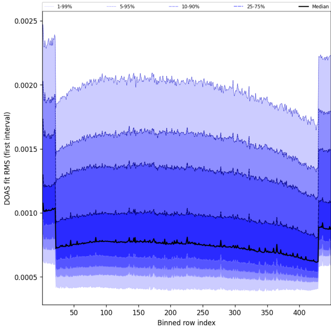
Figure 58: Along track statistics of “DOAS fit RMS (first interval)” for 2025-03-19 to 2025-03-20
