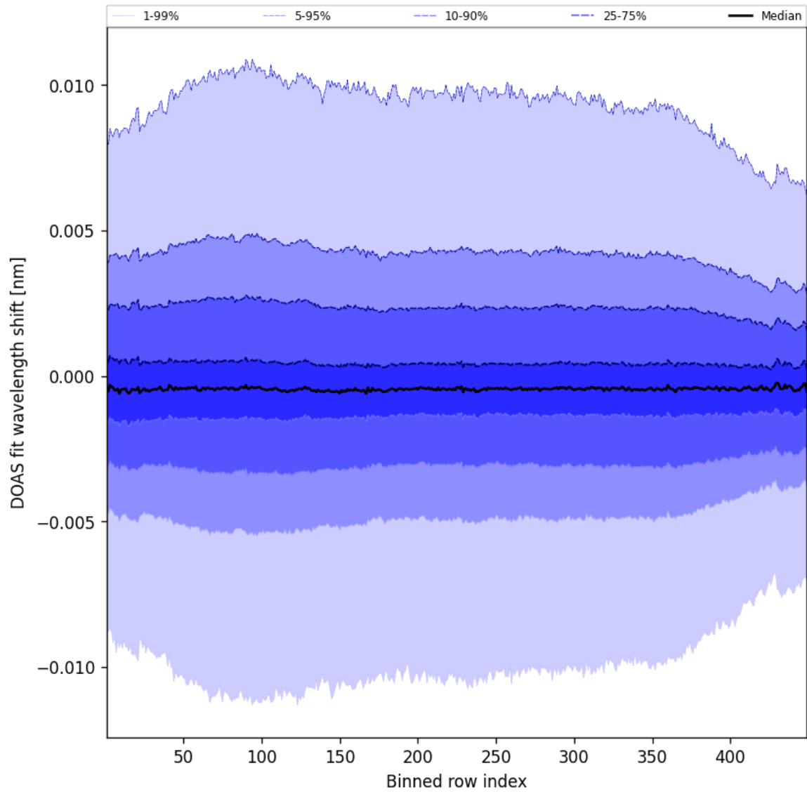
Figure 56: Along track statistics of “DOAS fit wavelength shift” for 2025-03-19 to 2025-03-20
