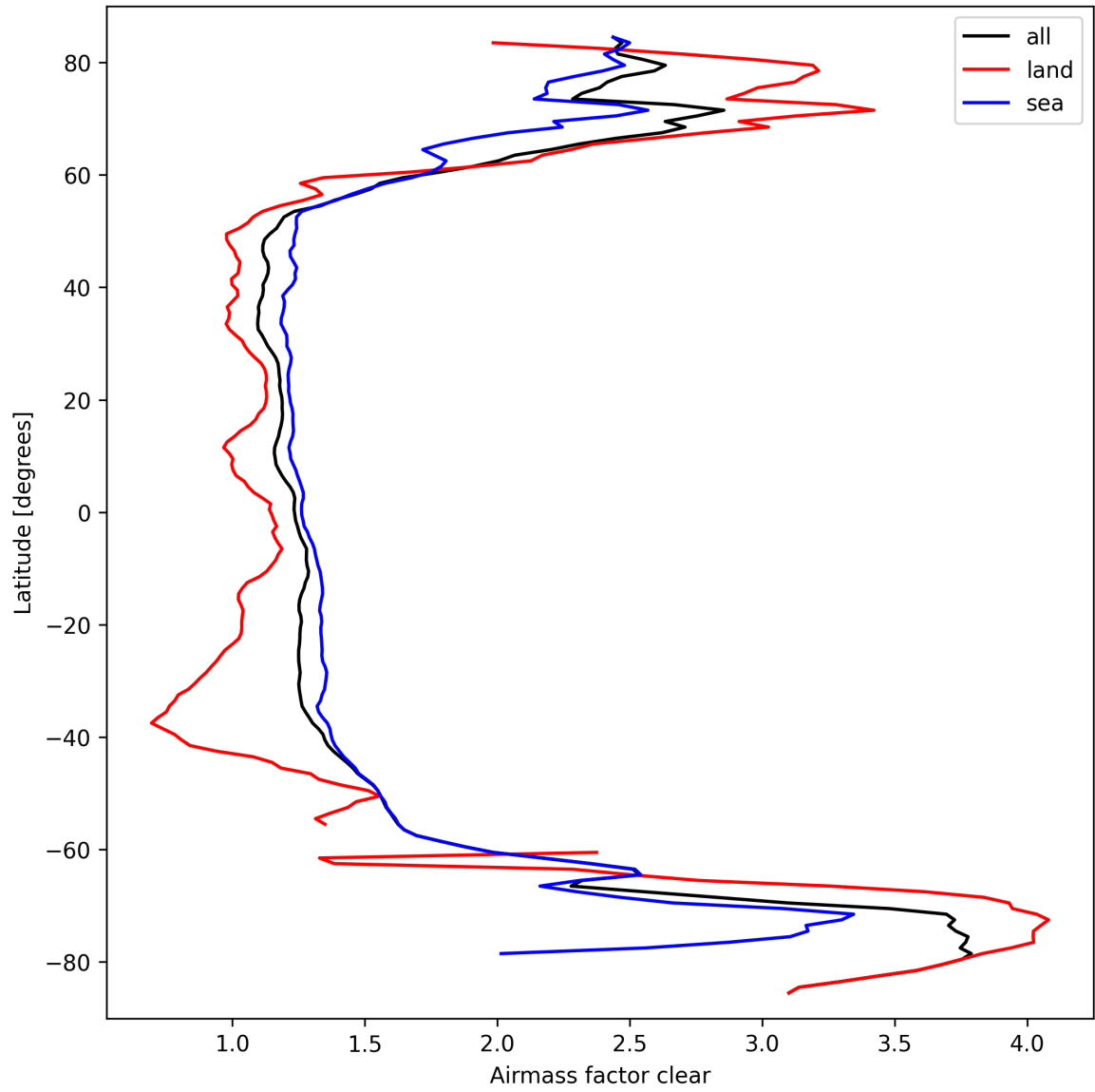
Figure 26: Zonal average of “Airmass factor clear” for 2025-03-19 to 2025-03-20.
