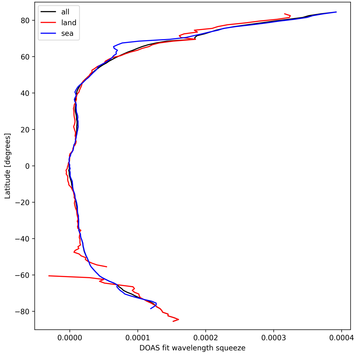
Figure 29: Zonal average of “DOAS fit wavelength squeeze” for 2025-03-19 to 2025-03-20.
