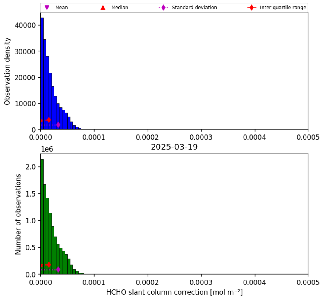
Figure 45: Histogram of “HCHO slant column correction” for 2025-03-19 to 2025-03-20
