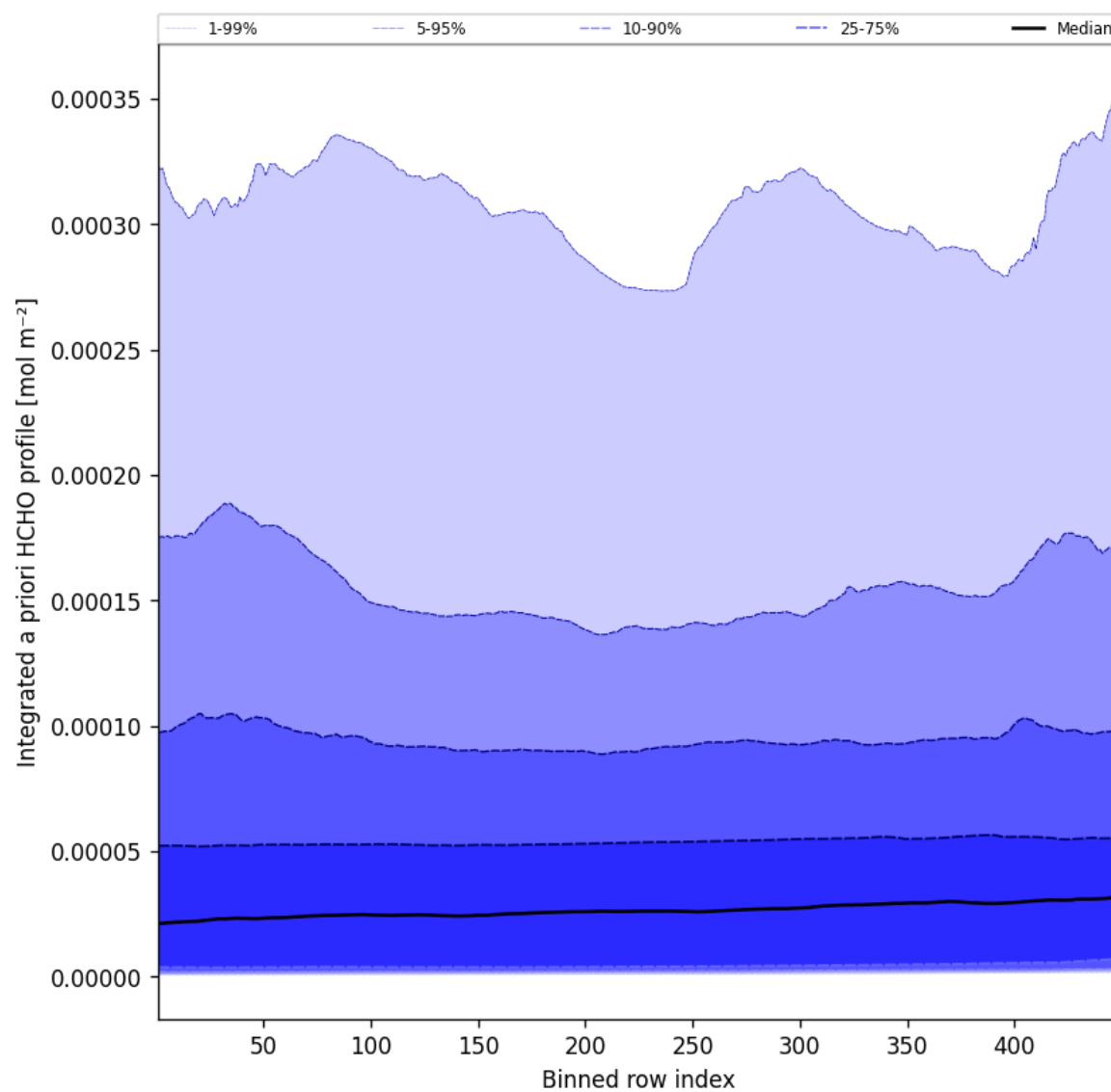
Figure 55: Along track statistics of "Integrated a priori HCHO profile" for 2025-03-19 to 2025-03-20
