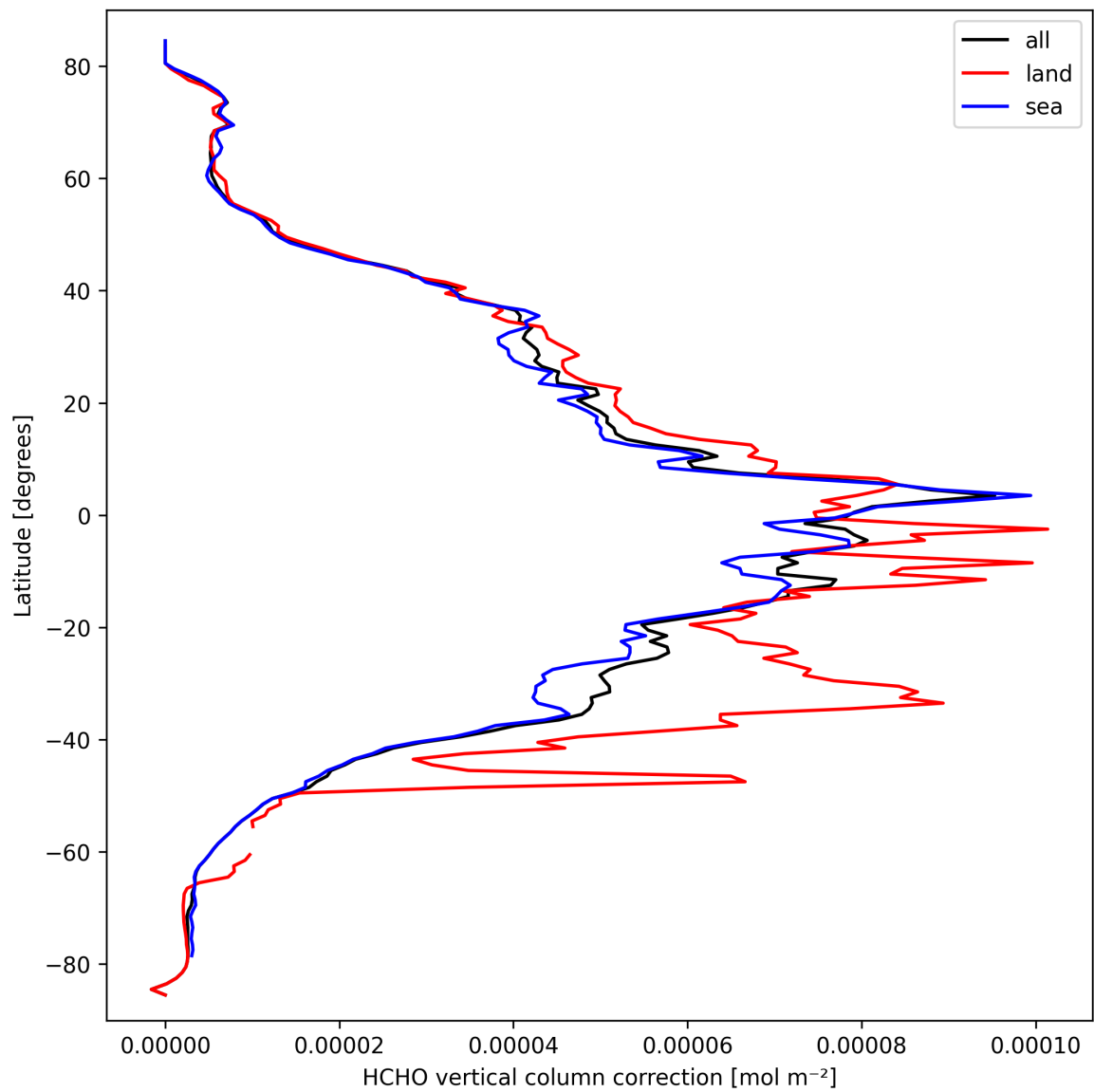
Figure 21: Zonal average of “HCHO vertical column correction” for 2025-03-19 to 2025-03-20.
