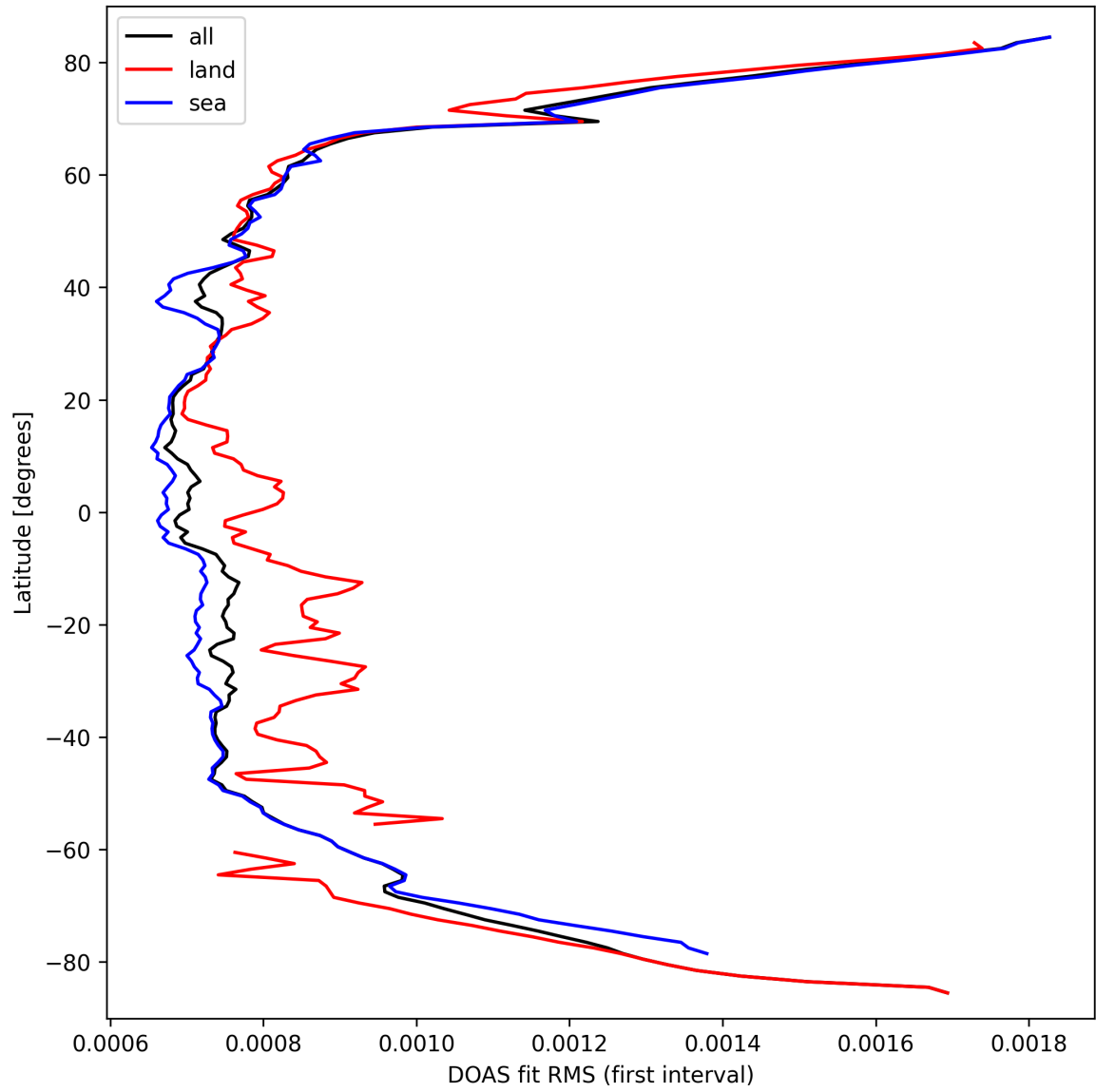
Figure 30: Zonal average of “DOAS fit RMS (first interval)” for 2025-03-19 to 2025-03-20.
