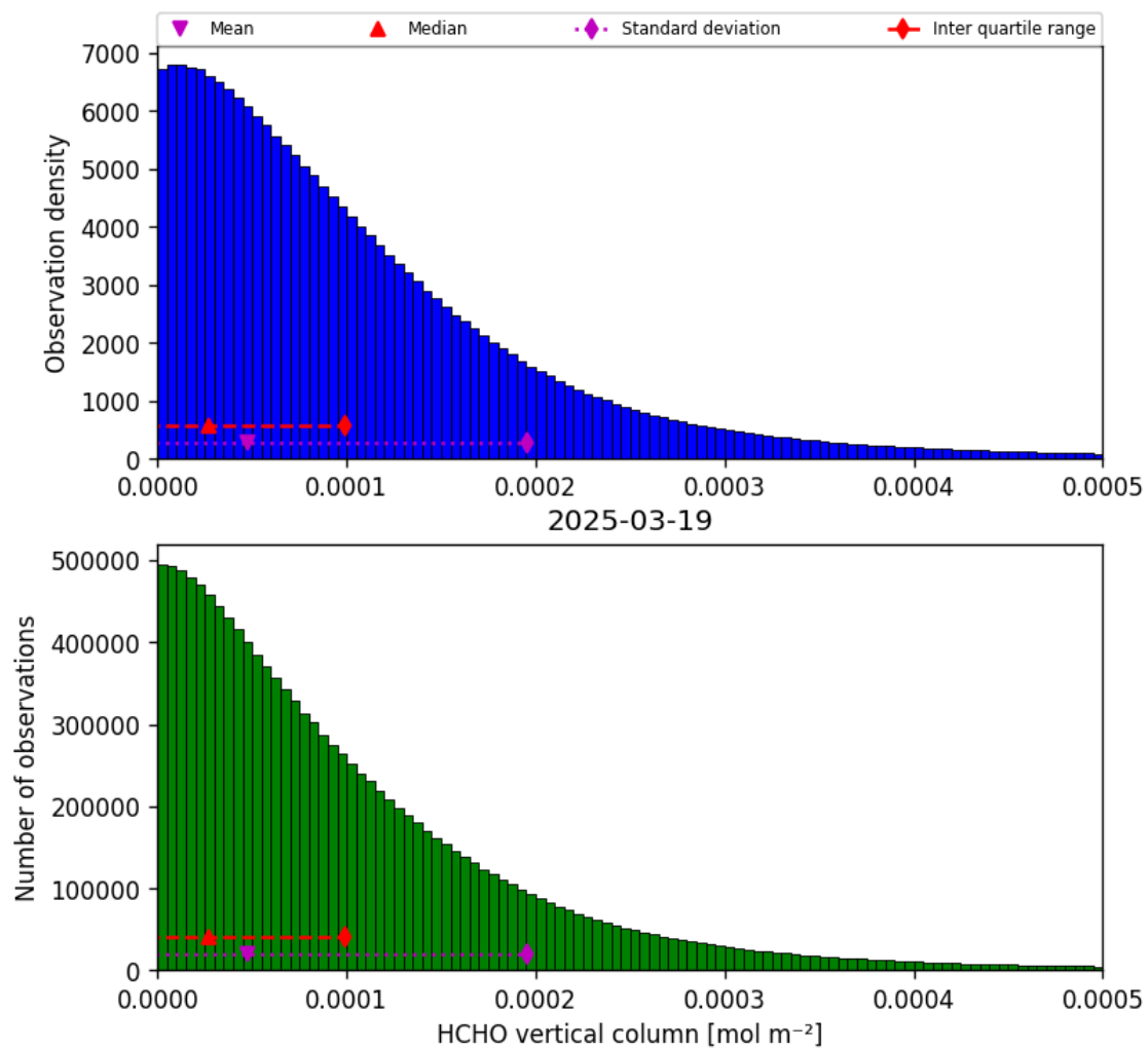
Figure 33: Histogram of “HCHO vertical column” for 2025-03-19 to 2025-03-20
