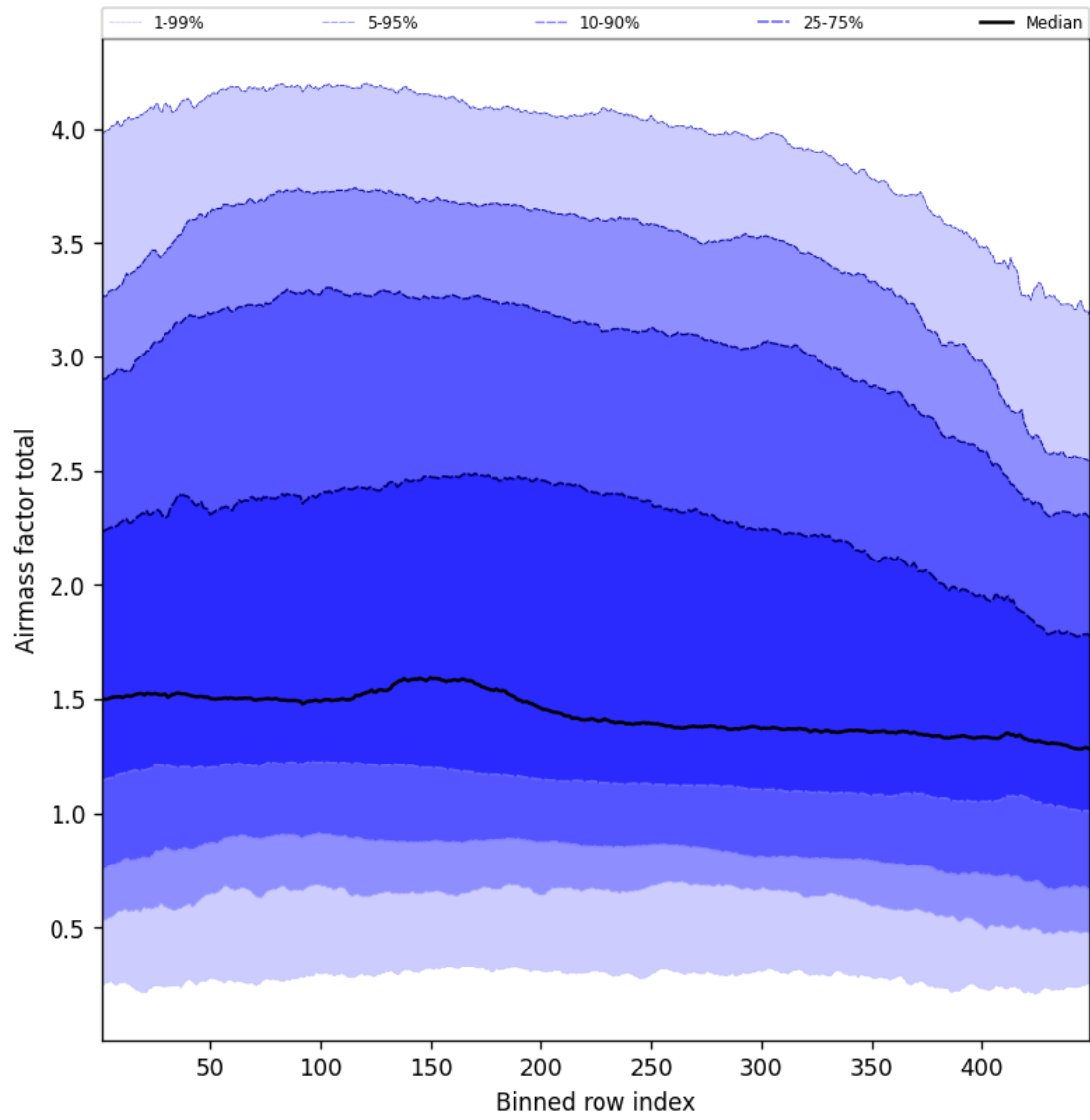
Figure 52: Along track statistics of “Airmass factor total” for 2025-03-19 to 2025-03-20
