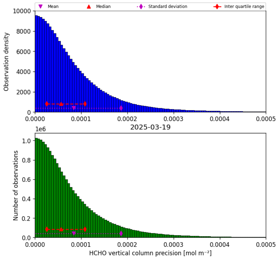
Figure 34: Histogram of “HCHO vertical column precision” for 2025-03-19 to 2025-03-20
