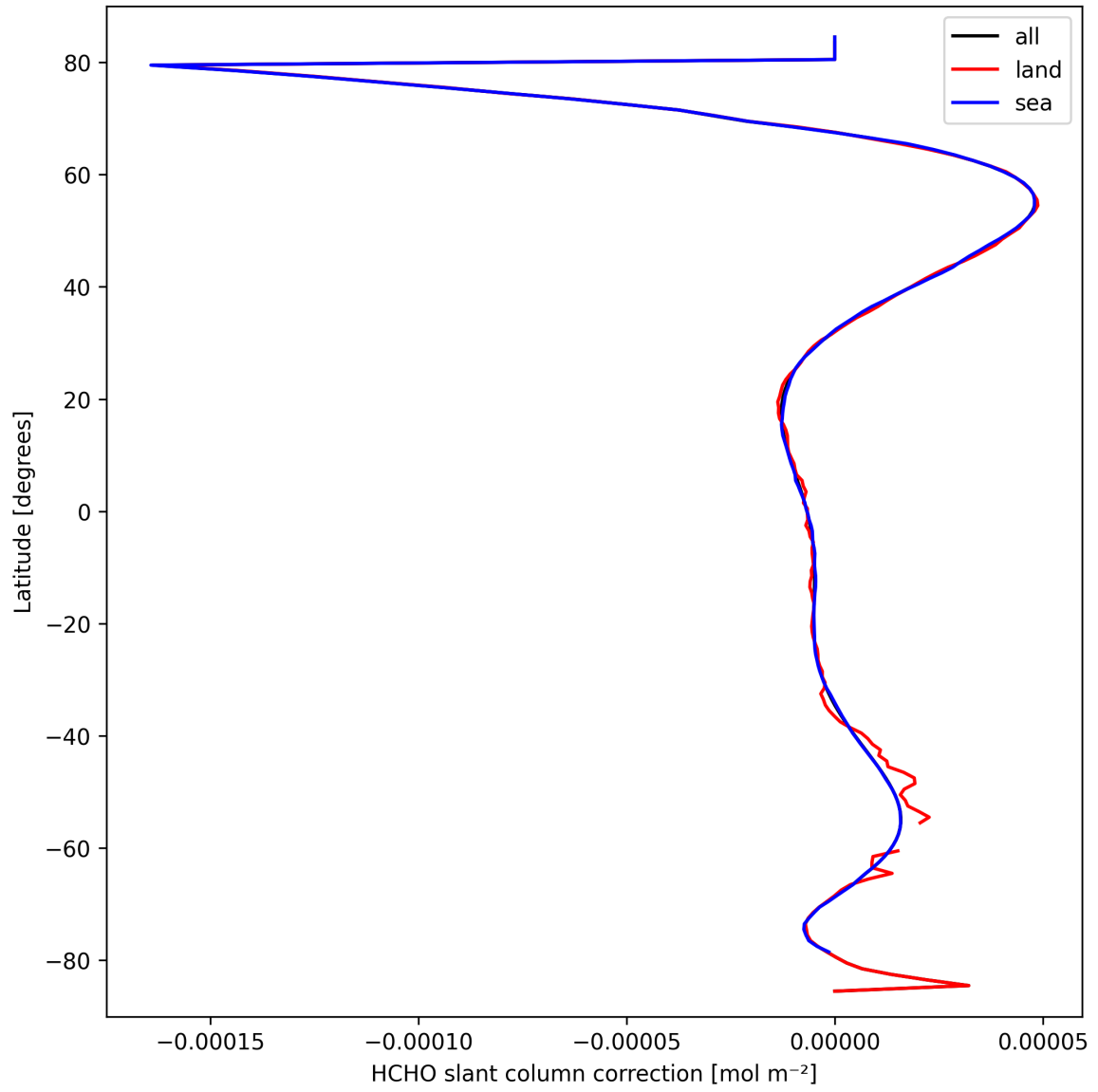
Figure 31: Zonal average of “HCHO slant column correction” for 2025-03-19 to 2025-03-20.
