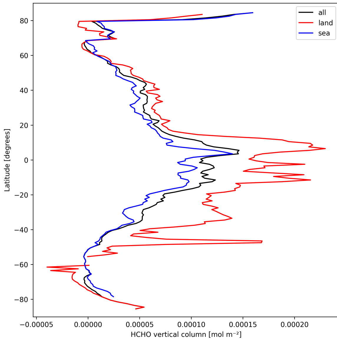
Figure 19: Zonal average of “HCHO vertical column” for 2025-03-19 to 2025-03-20.
