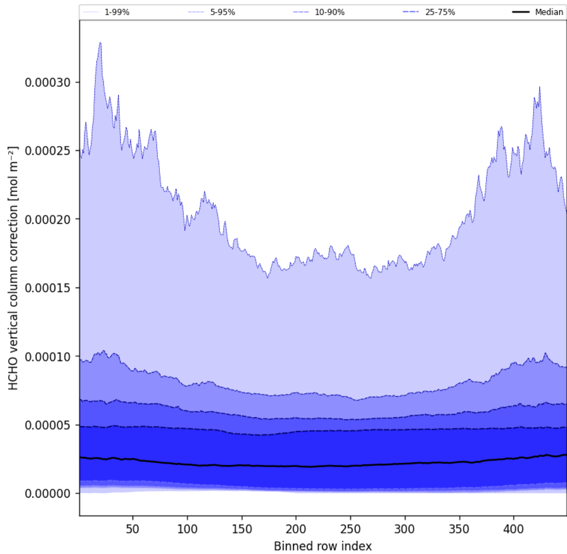
Figure 49: Along track statistics of “HCHO vertical column correction” for 2025-03-19 to 2025-03-20
