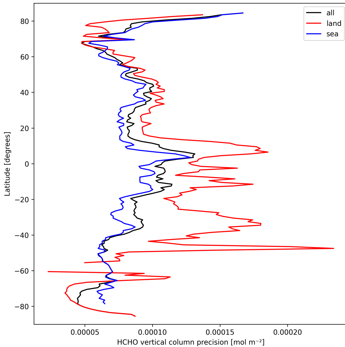
Figure 20: Zonal average of “HCHO vertical column precision” for 2025-03-19 to 2025-03-20.
