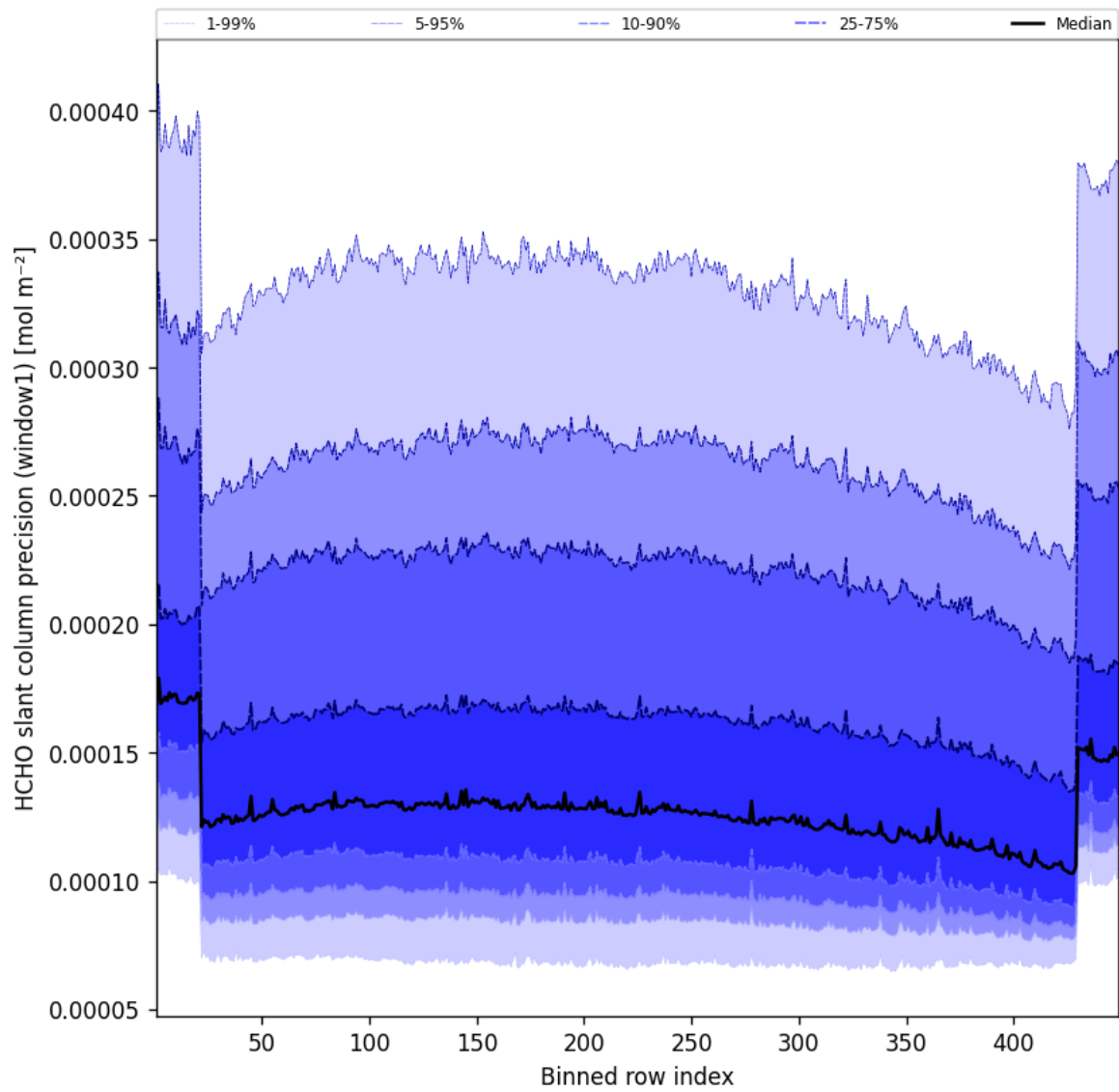
Figure 51: Along track statistics of “HCHO slant column precision (window1)” for 2025-03-19 to 2025-03-20
