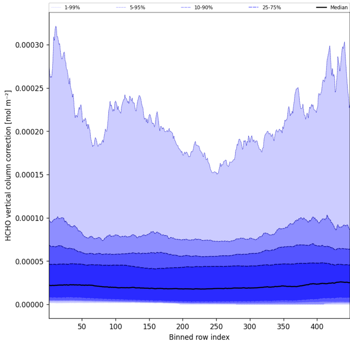
Figure 49: Along track statistics of "HCHO vertical column correction" for 2025-03-20 to 2025-03-21
