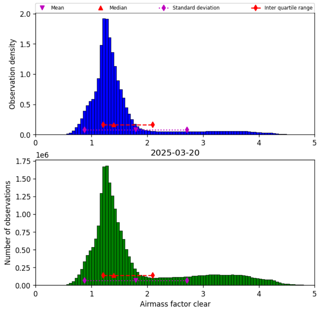
Figure 40: Histogram of “Airmass factor clear” for 2025-03-20 to 2025-03-21
