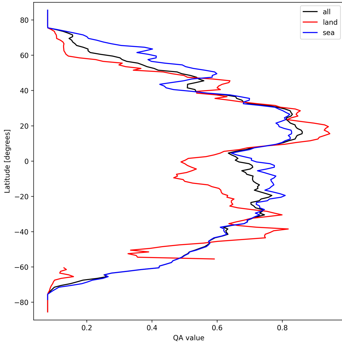
Figure 18: Zonal average of “QA value” for 2025-03-20 to 2025-03-21.
