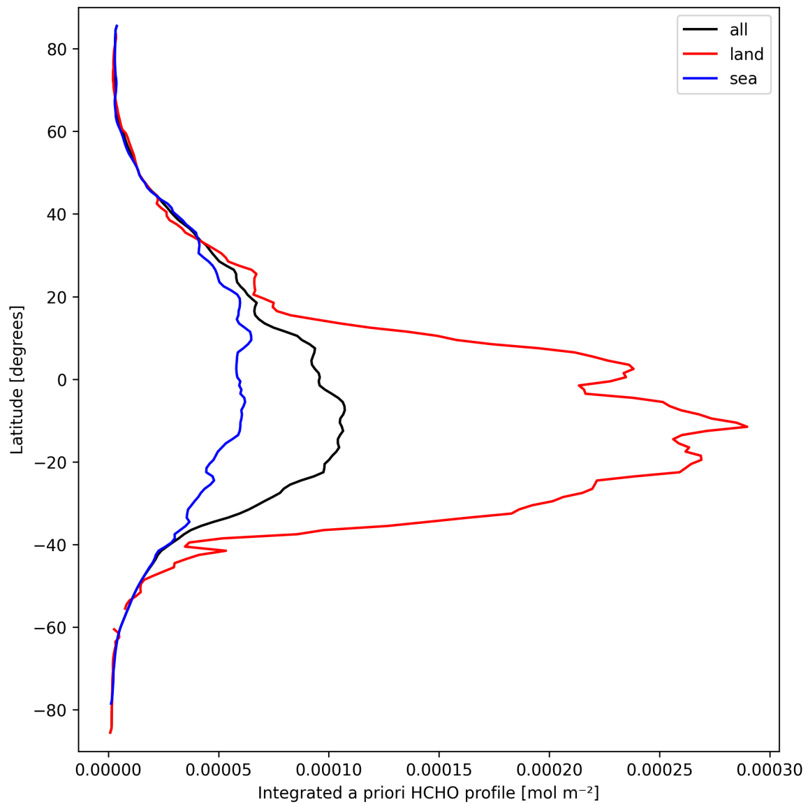
Figure 27: Zonal average of “Integrated a priori HCHO profile” for 2025-03-20 to 2025-03-21.
