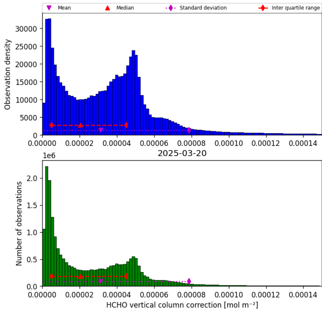
Figure 35: Histogram of “HCHO vertical column correction” for 2025-03-20 to 2025-03-21
