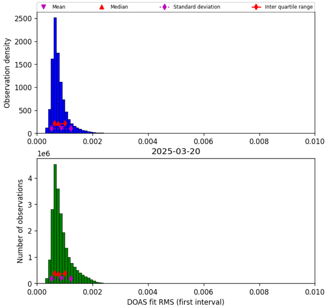
Figure 44: Histogram of “DOAS fit RMS (first interval)” for 2025-03-20 to 2025-03-21
