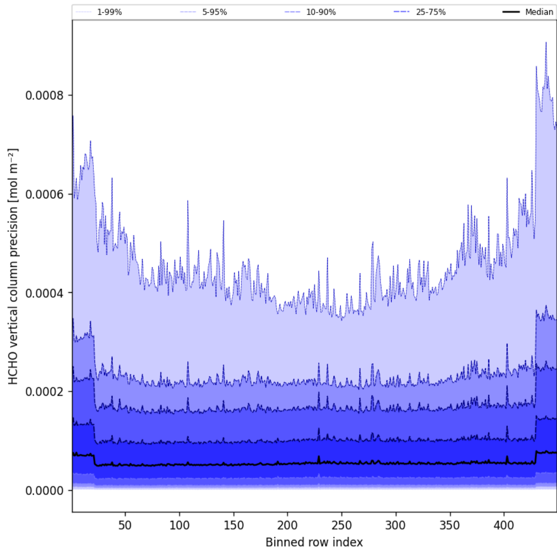
Figure 48: Along track statistics of “HCHO vertical column precision” for 2025-03-20 to 2025-03-21
