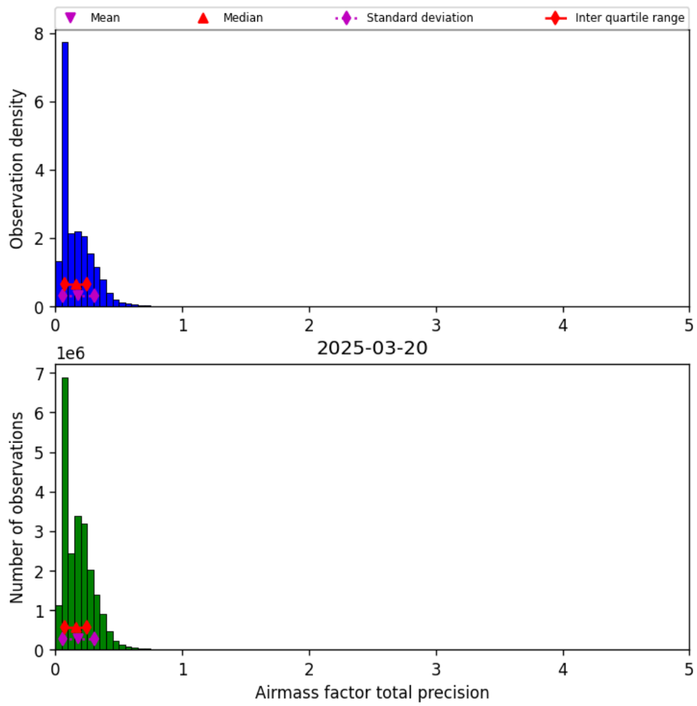
Figure 39: Histogram of “Airmass factor total precision” for 2025-03-20 to 2025-03-21
