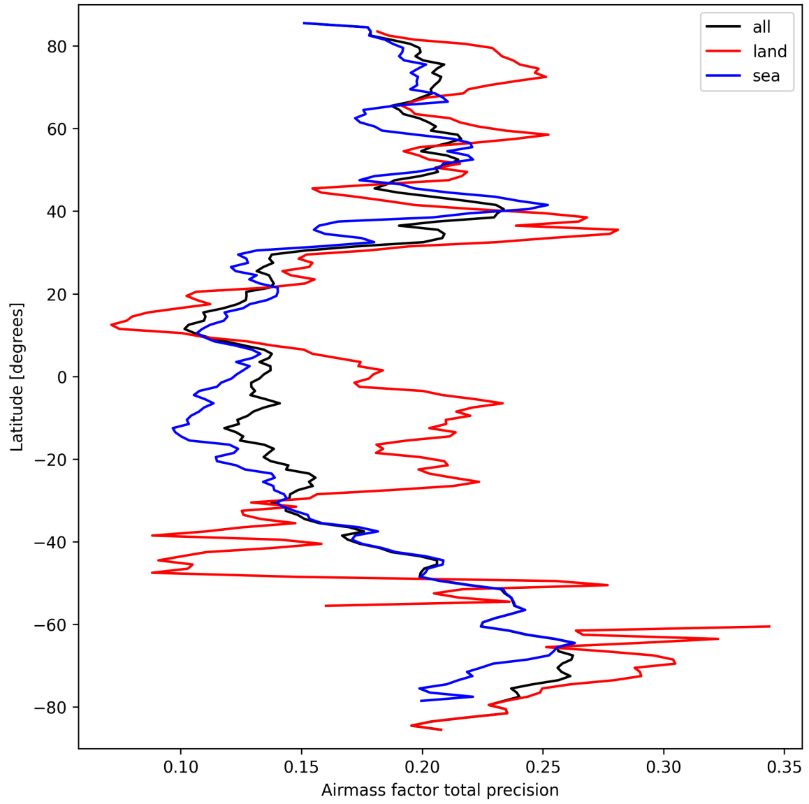
Figure 25: Zonal average of “Airmass factor total precision” for 2025-03-20 to 2025-03-21.
