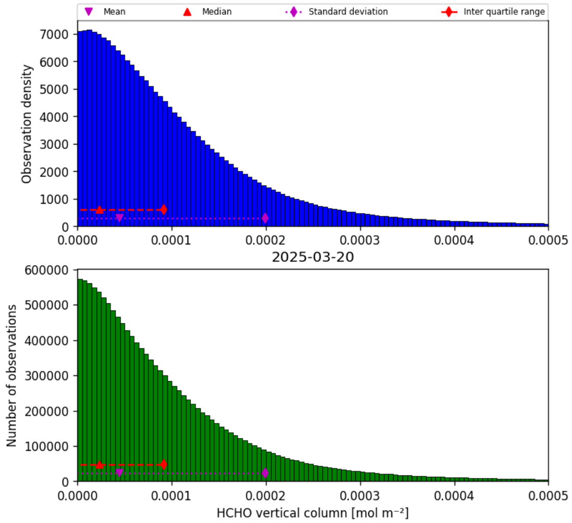
Figure 33: Histogram of “HCHO vertical column” for 2025-03-20 to 2025-03-21
