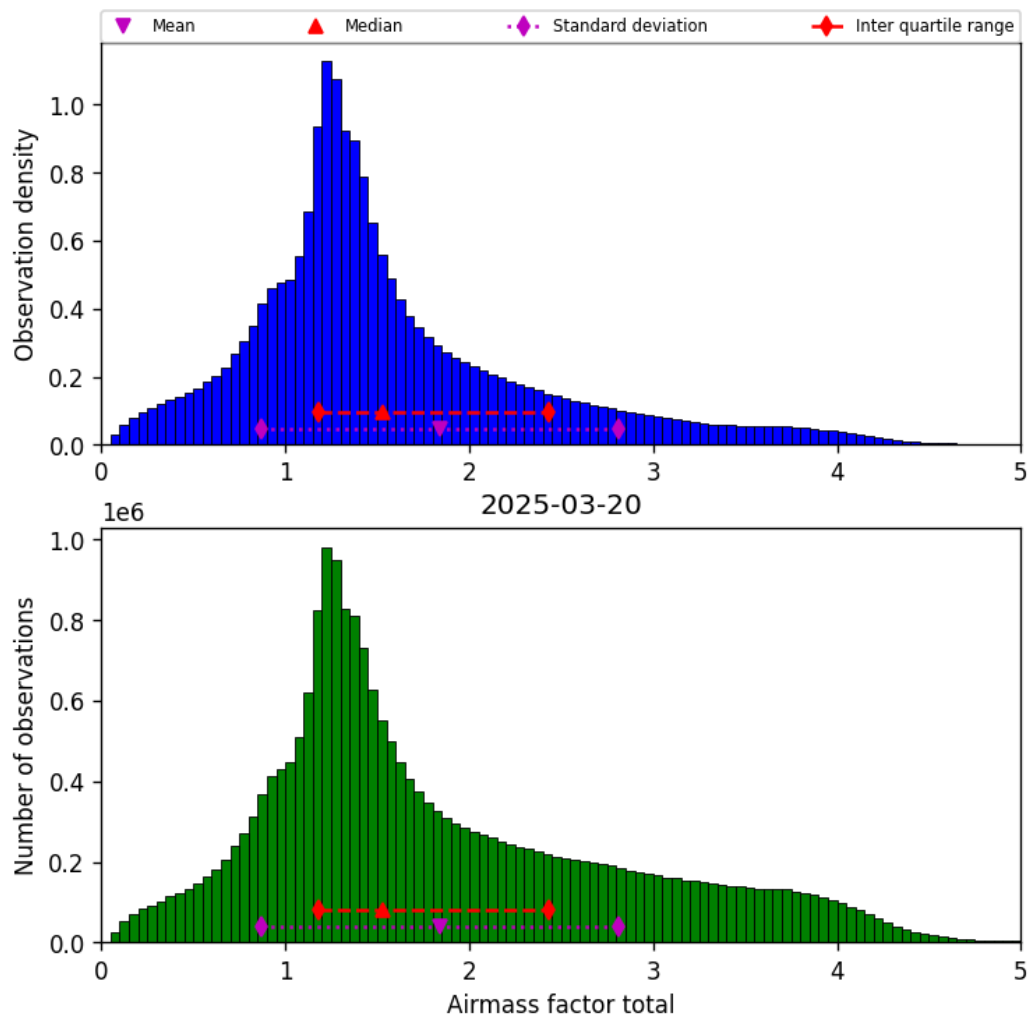
Figure 38: Histogram of “Airmass factor total” for 2025-03-20 to 2025-03-21
