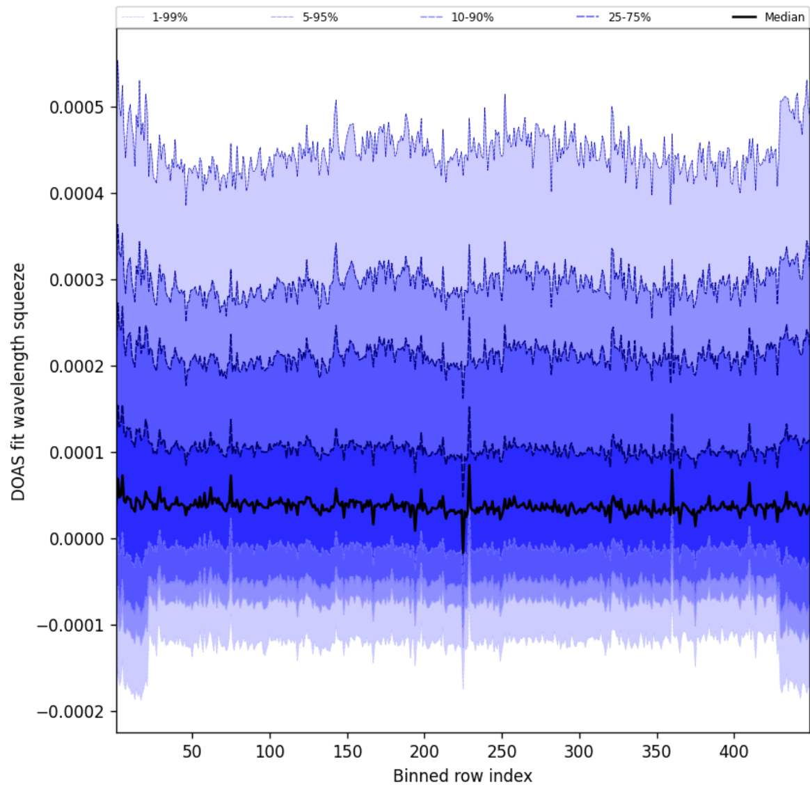
Figure 57: Along track statistics of “DOAS fit wavelength squeeze” for 2025-03-20 to 2025-03-21
