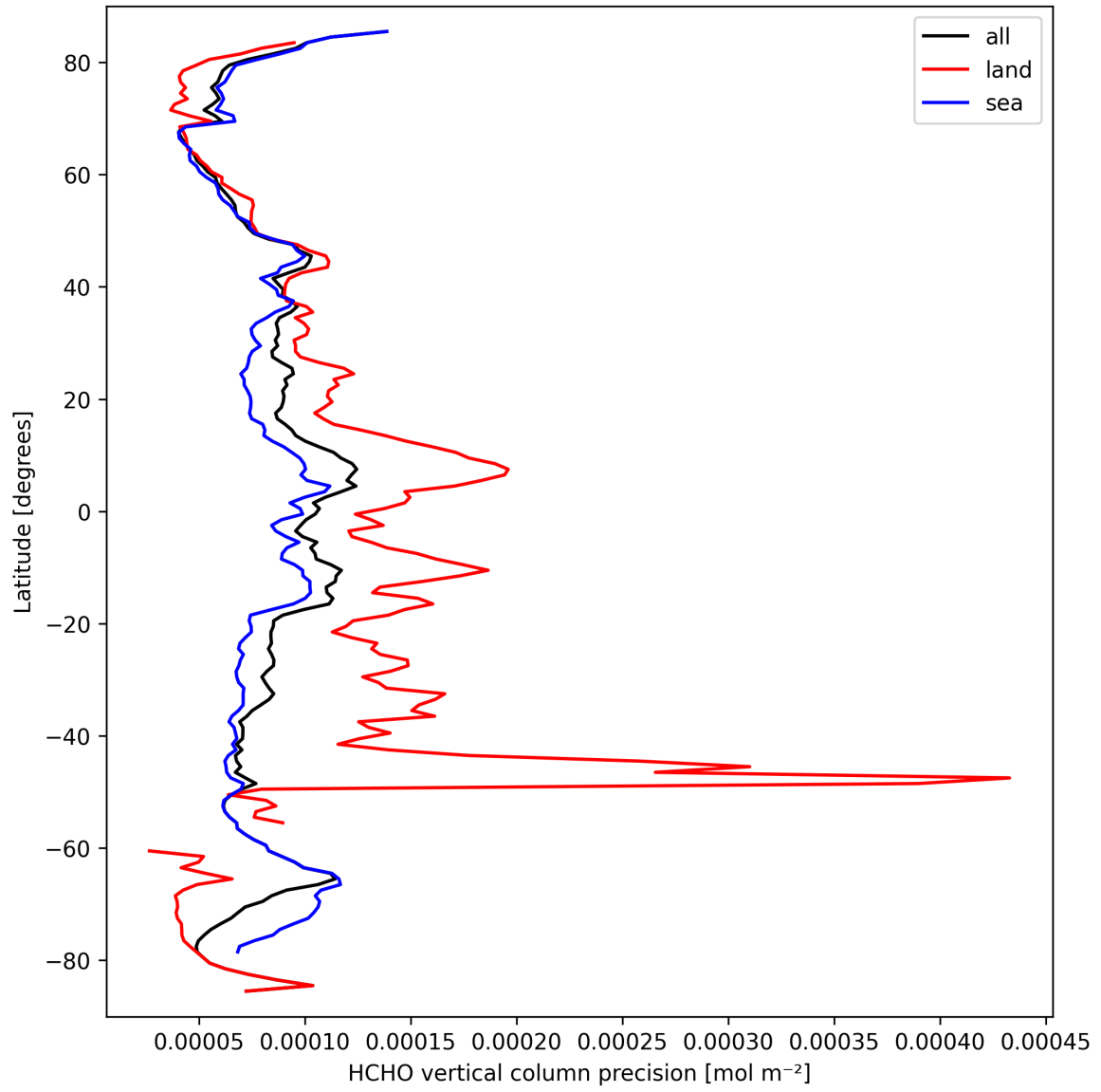
Figure 20: Zonal average of “HCHO vertical column precision” for 2025-03-20 to 2025-03-21.
