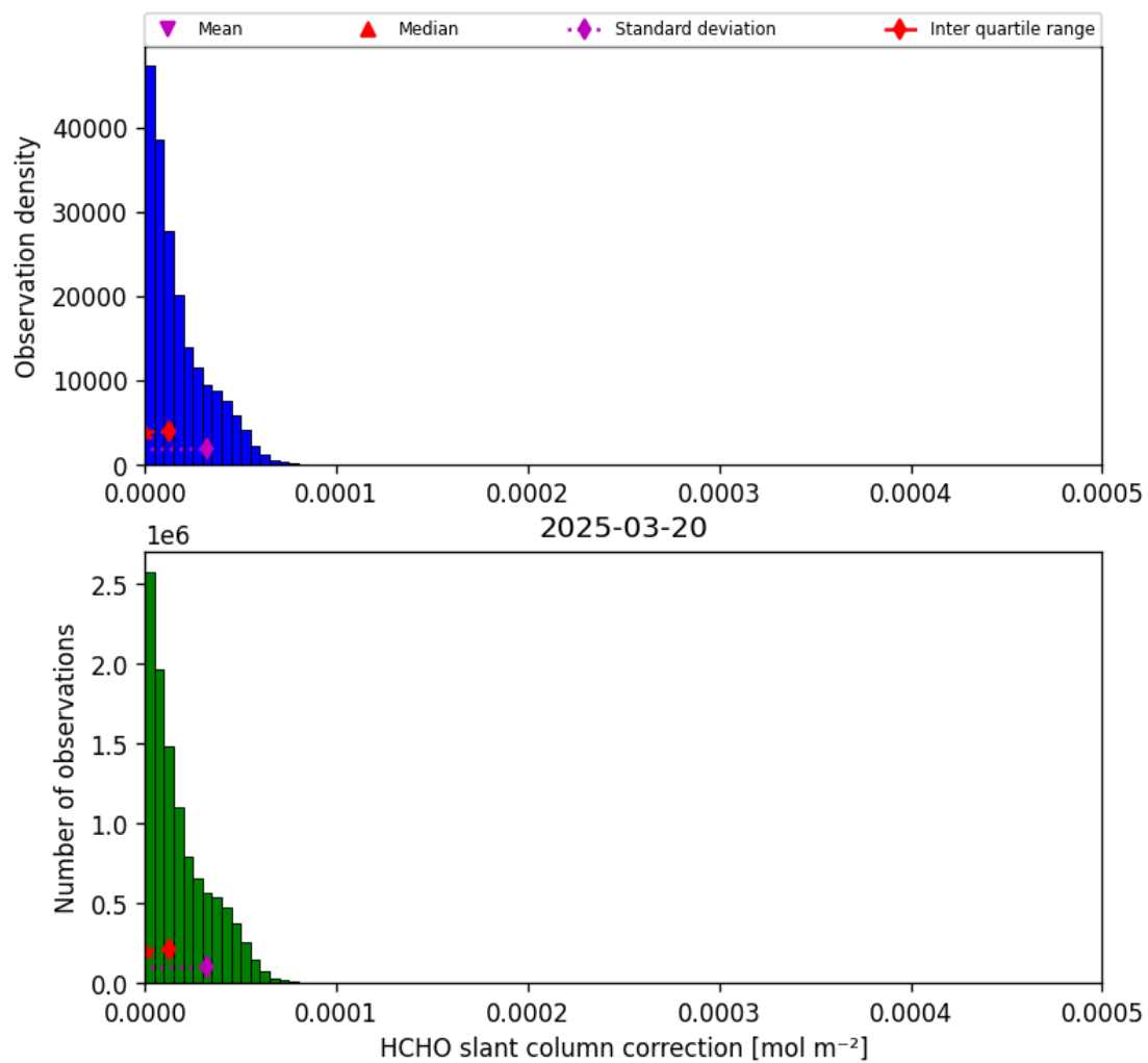
Figure 45: Histogram of “HCHO slant column correction” for 2025-03-20 to 2025-03-21
