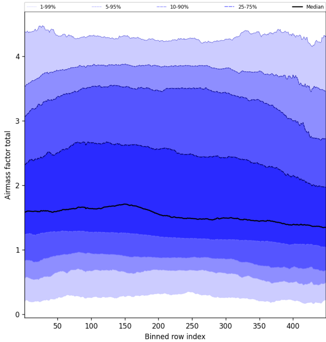
Figure 52: Along track statistics of “Airmass factor total” for 2025-03-20 to 2025-03-21
