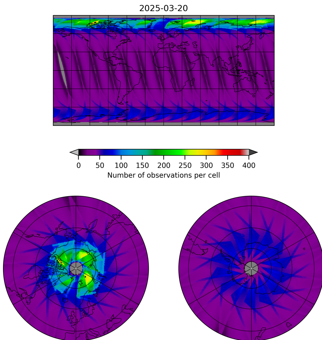
Figure 17: Map of the number of observations for 2025-03-20 to 2025-03-21
