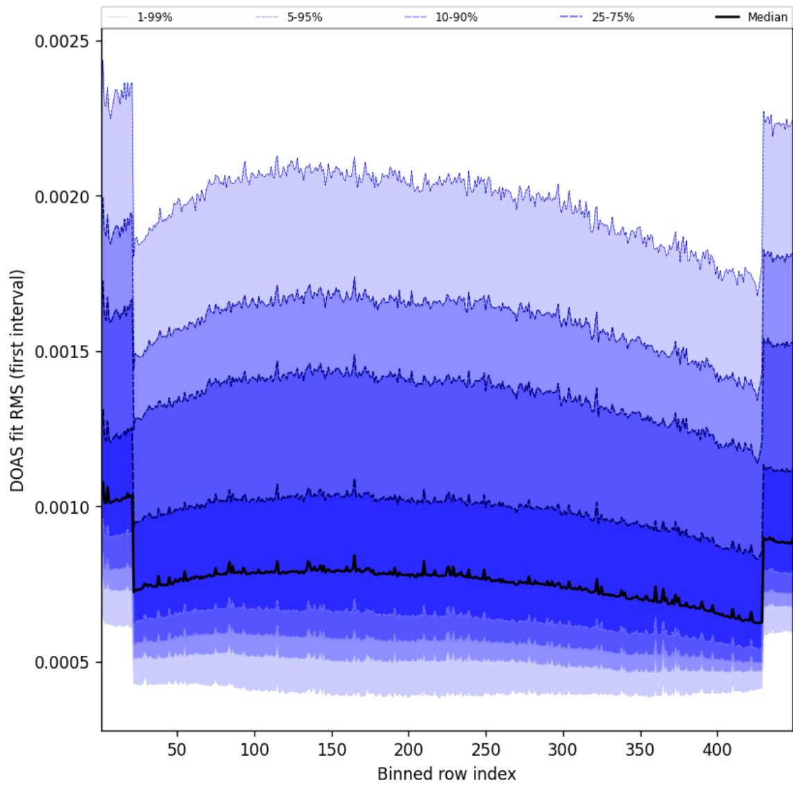
Figure 58: Along track statistics of “DOAS fit RMS (first interval)” for 2025-03-20 to 2025-03-21
