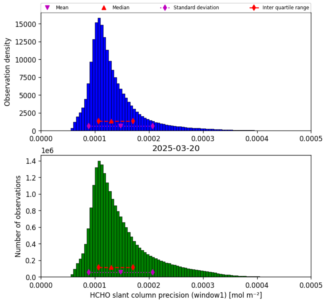
Figure 37: Histogram of “HCHO slant column precision (window1)” for 2025-03-20 to 2025-03-21
