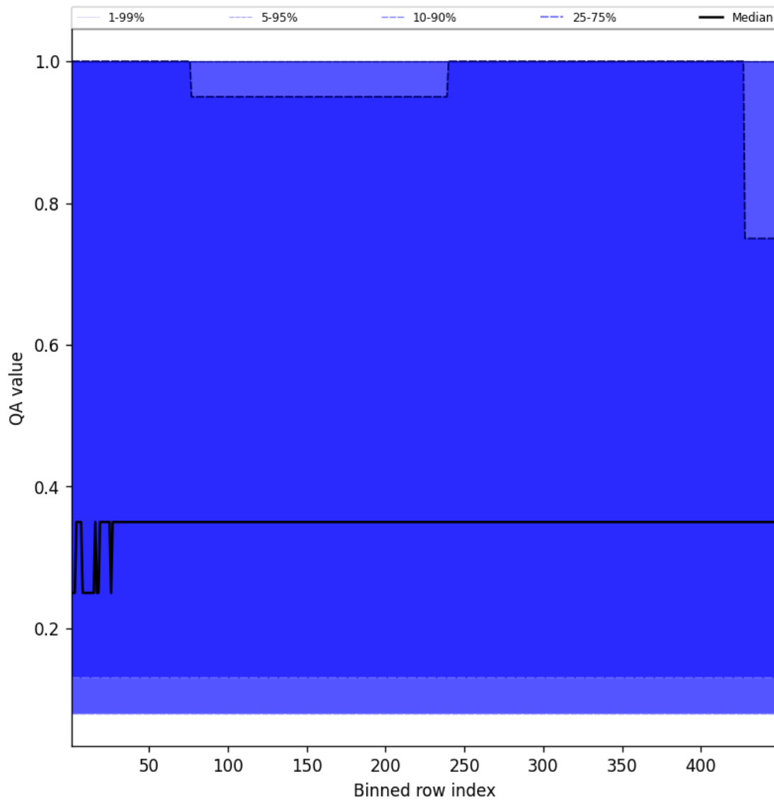
Figure 46: Along track statistics of “QA value” for 2025-03-20 to 2025-03-21
