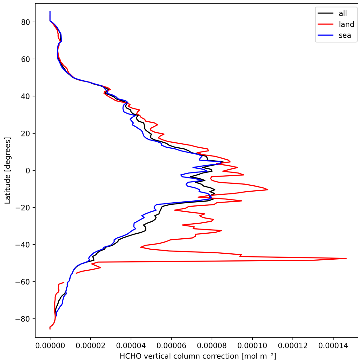
Figure 21: Zonal average of “HCHO vertical column correction” for 2025-03-20 to 2025-03-21.
