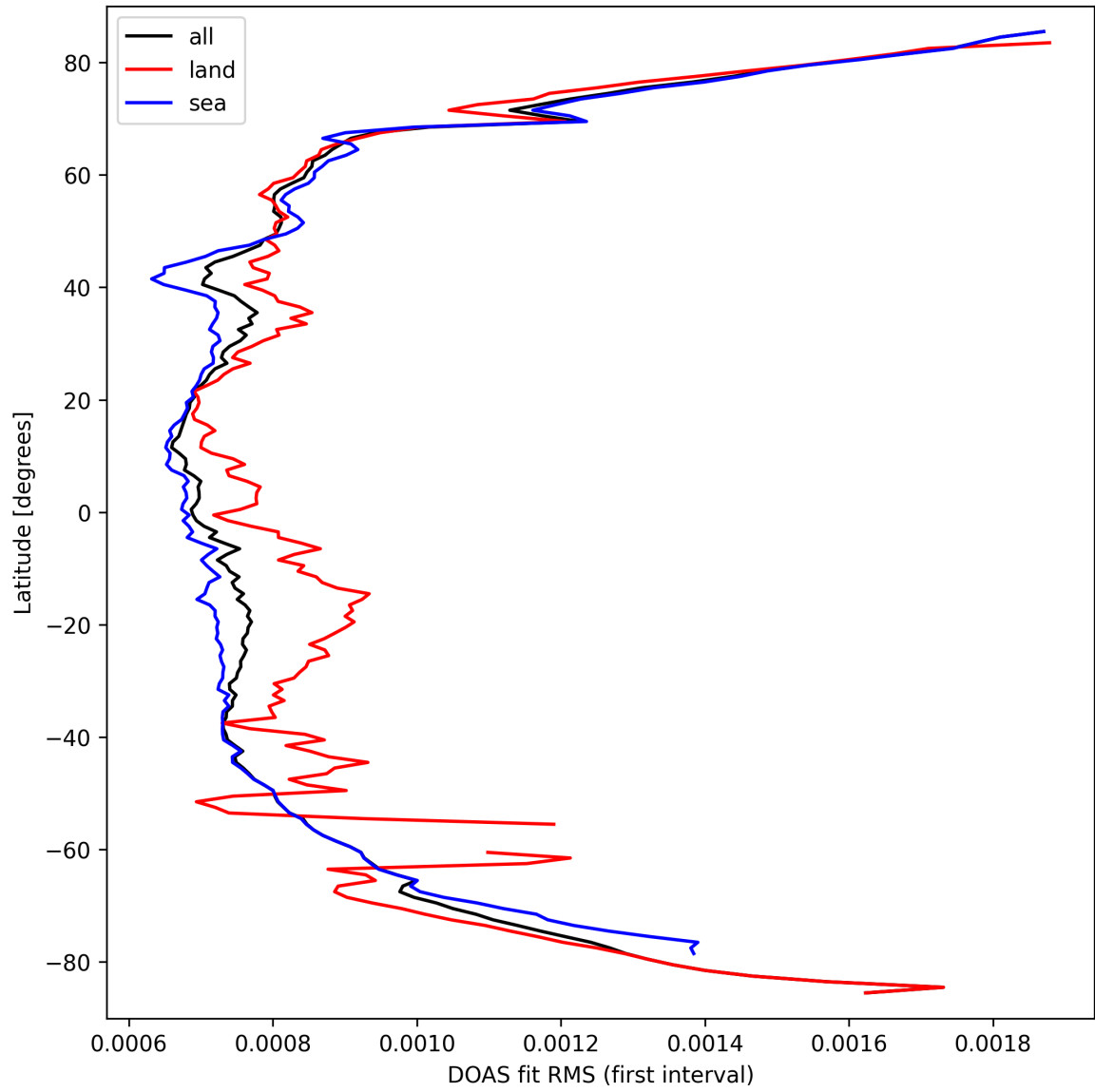
Figure 30: Zonal average of "DOAS fit RMS (first interval)" for 2025-03-20 to 2025-03-21.
