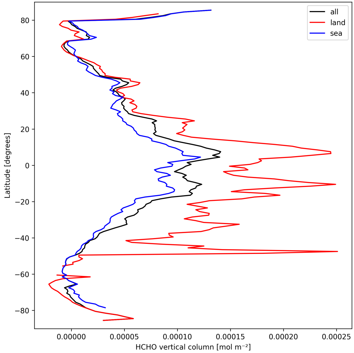
Figure 19: Zonal average of “HCHO vertical column” for 2025-03-20 to 2025-03-21.
