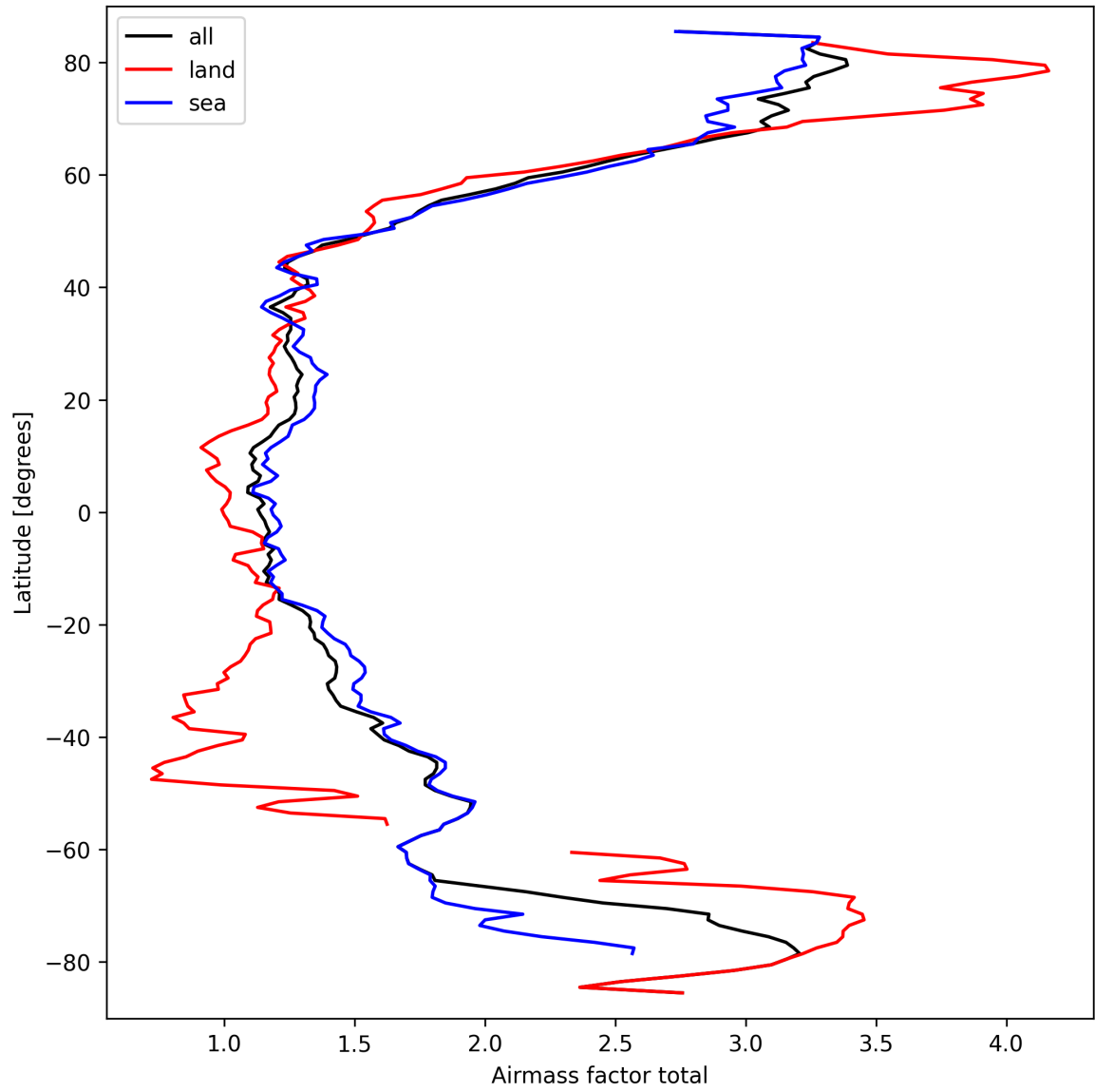
Figure 24: Zonal average of “Airmass factor total” for 2025-03-20 to 2025-03-21.
