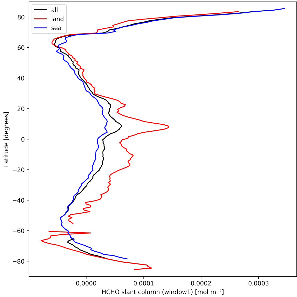
Figure 22: Zonal average of “HCHO slant column (window1)” for 2025-03-20 to 2025-03-21.
