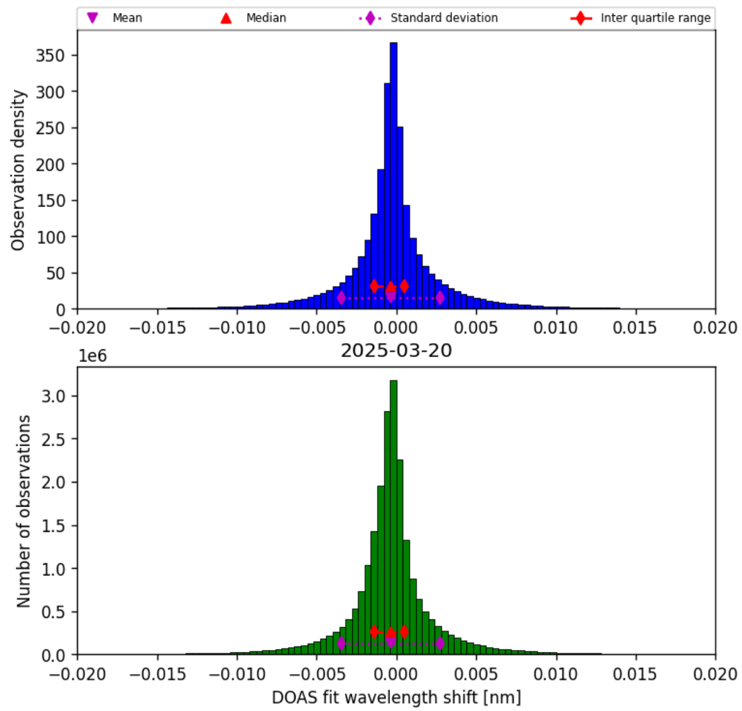
Figure 42: Histogram of “DOAS fit wavelength shift” for 2025-03-20 to 2025-03-21
