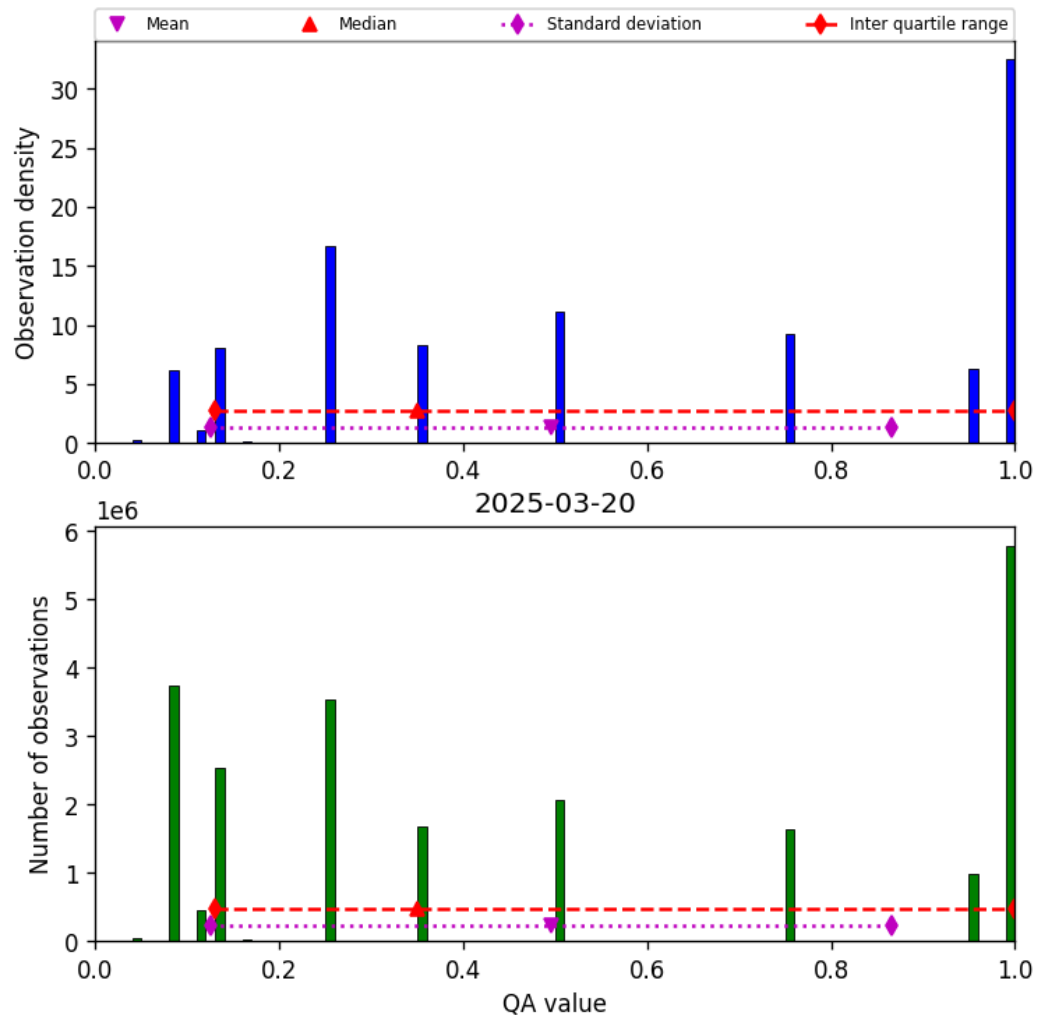
Figure 32: Histogram of “QA value” for 2025-03-20 to 2025-03-21
