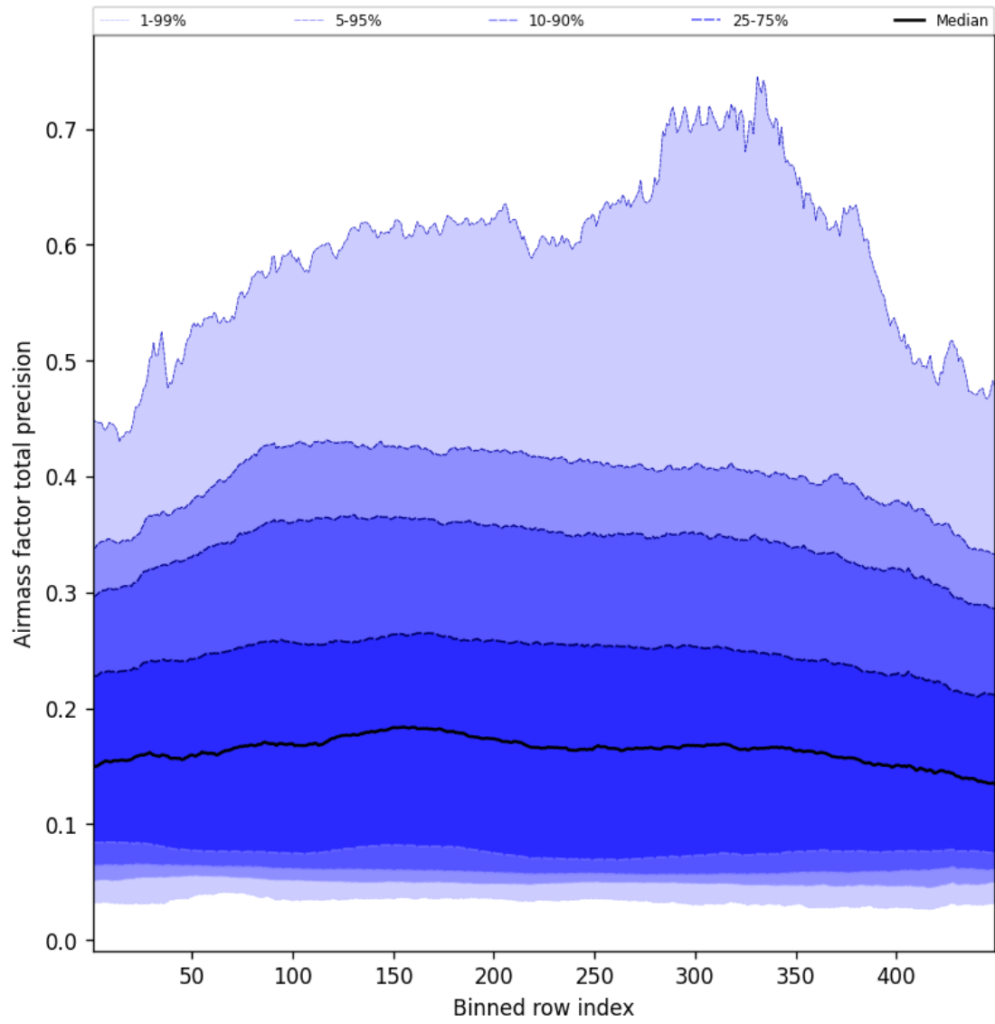
Figure 53: Along track statistics of “Airmass factor total precision” for 2025-03-20 to 2025-03-21
