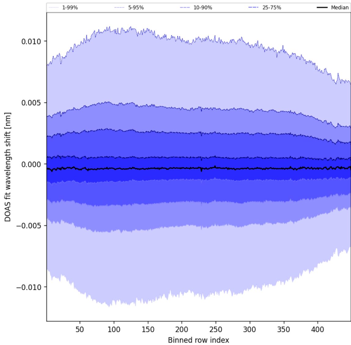
Figure 56: Along track statistics of “DOAS fit wavelength shift” for 2025-03-20 to 2025-03-21
