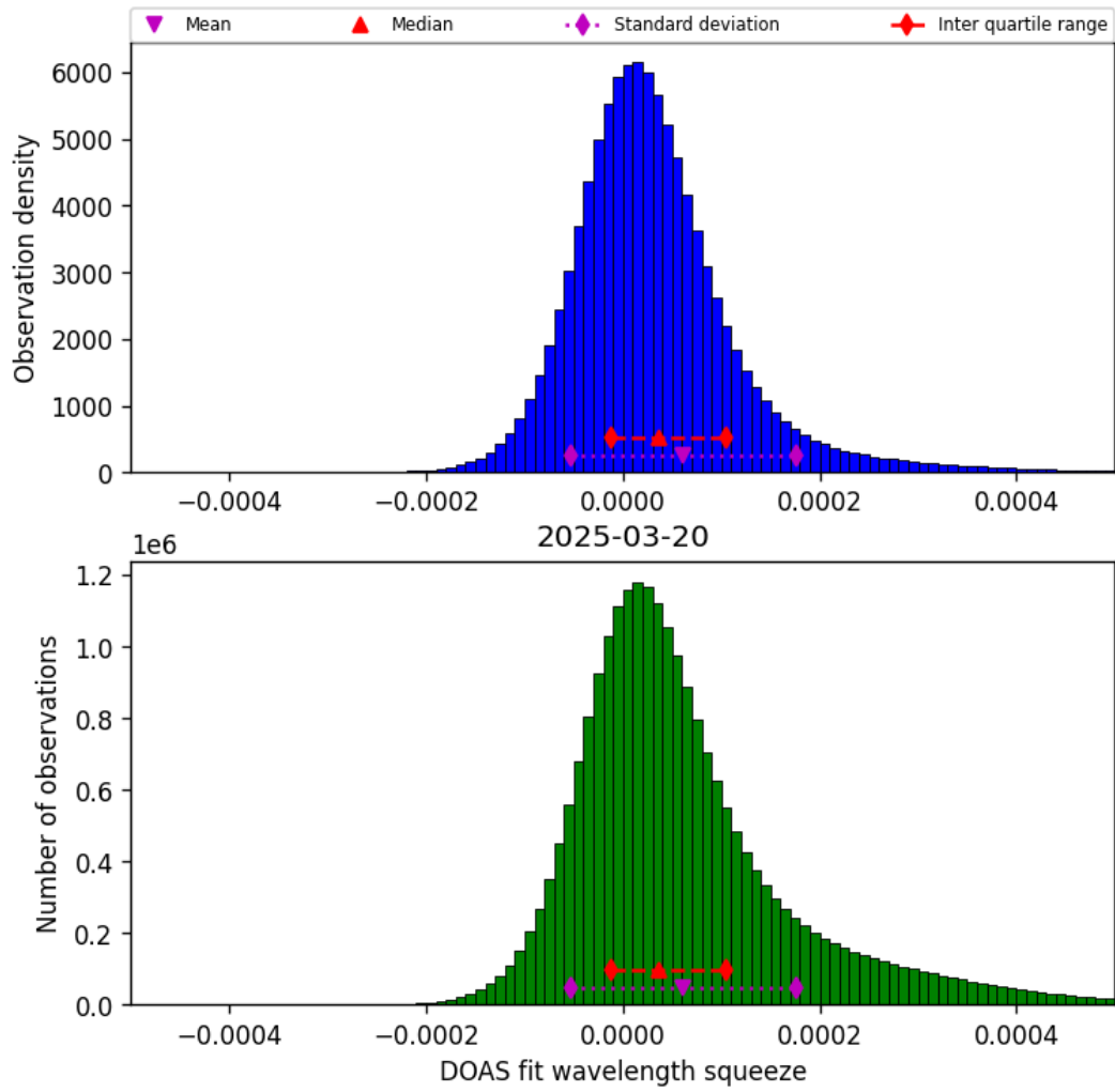
Figure 43: Histogram of “DOAS fit wavelength squeeze” for 2025-03-20 to 2025-03-21
