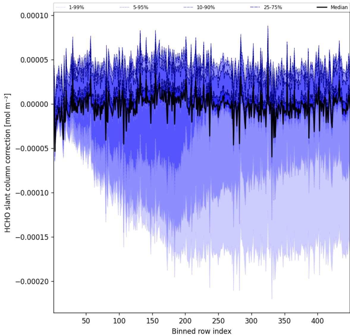
Figure 59: Along track statistics of “HCHO slant column correction” for 2025-03-20 to 2025-03-21
