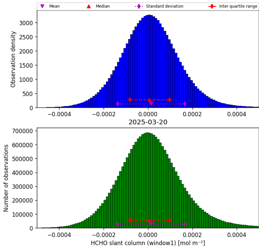
Figure 36: Histogram of “HCHO slant column (window1)” for 2025-03-20 to 2025-03-21
