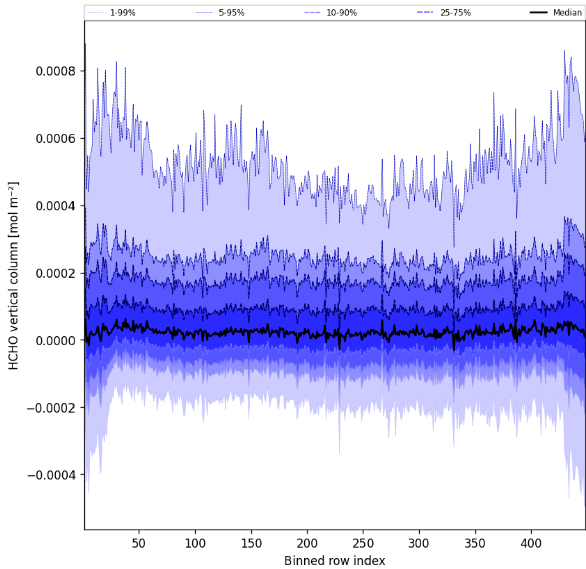
Figure 47: Along track statistics of “HCHO vertical column” for 2025-03-20 to 2025-03-21
