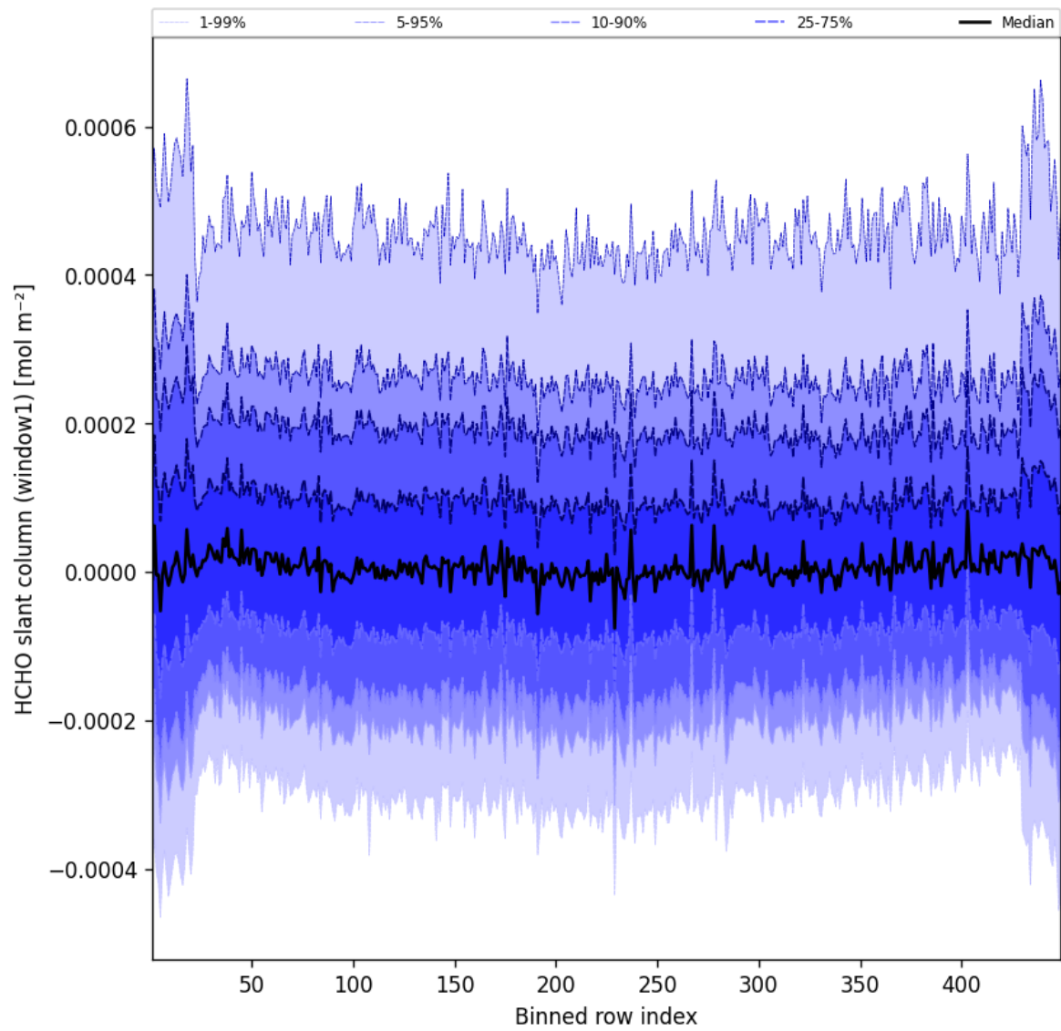
Figure 50: Along track statistics of “HCHO slant column (window1)” for 2025-03-20 to 2025-03-21
