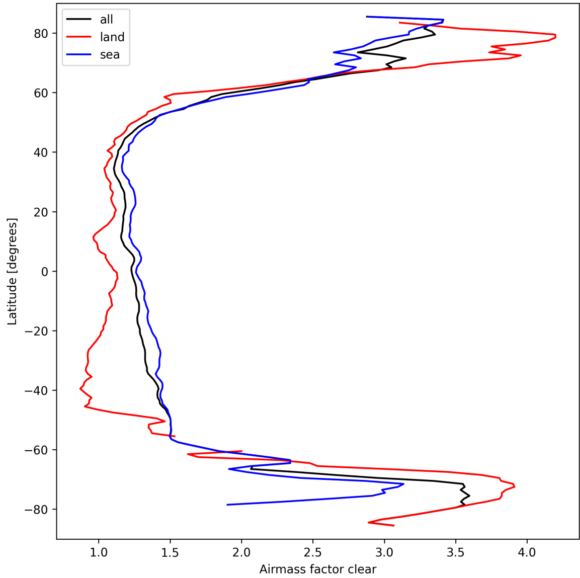
Figure 26: Zonal average of “Airmass factor clear” for 2025-03-20 to 2025-03-21.
