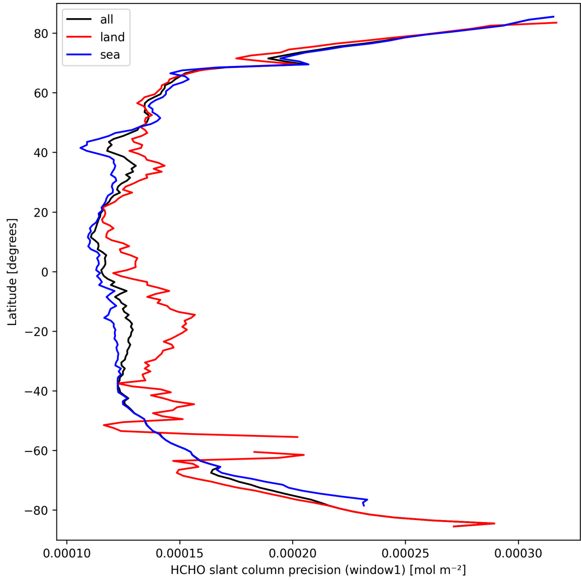
Figure 23: Zonal average of “HCHO slant column precision (window1)” for 2025-03-20 to 2025-03-21.
