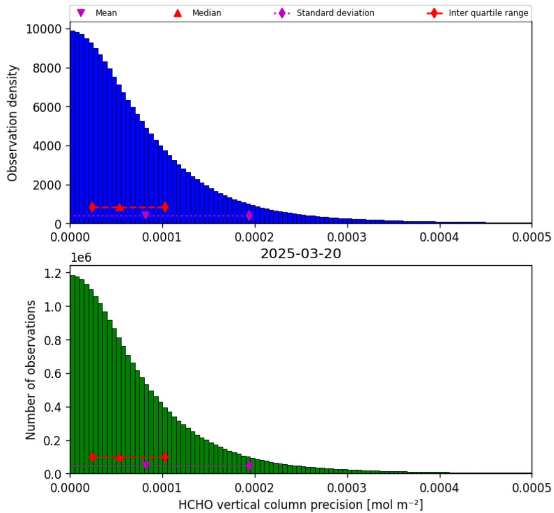
Figure 34: Histogram of “HCHO vertical column precision” for 2025-03-20 to 2025-03-21
