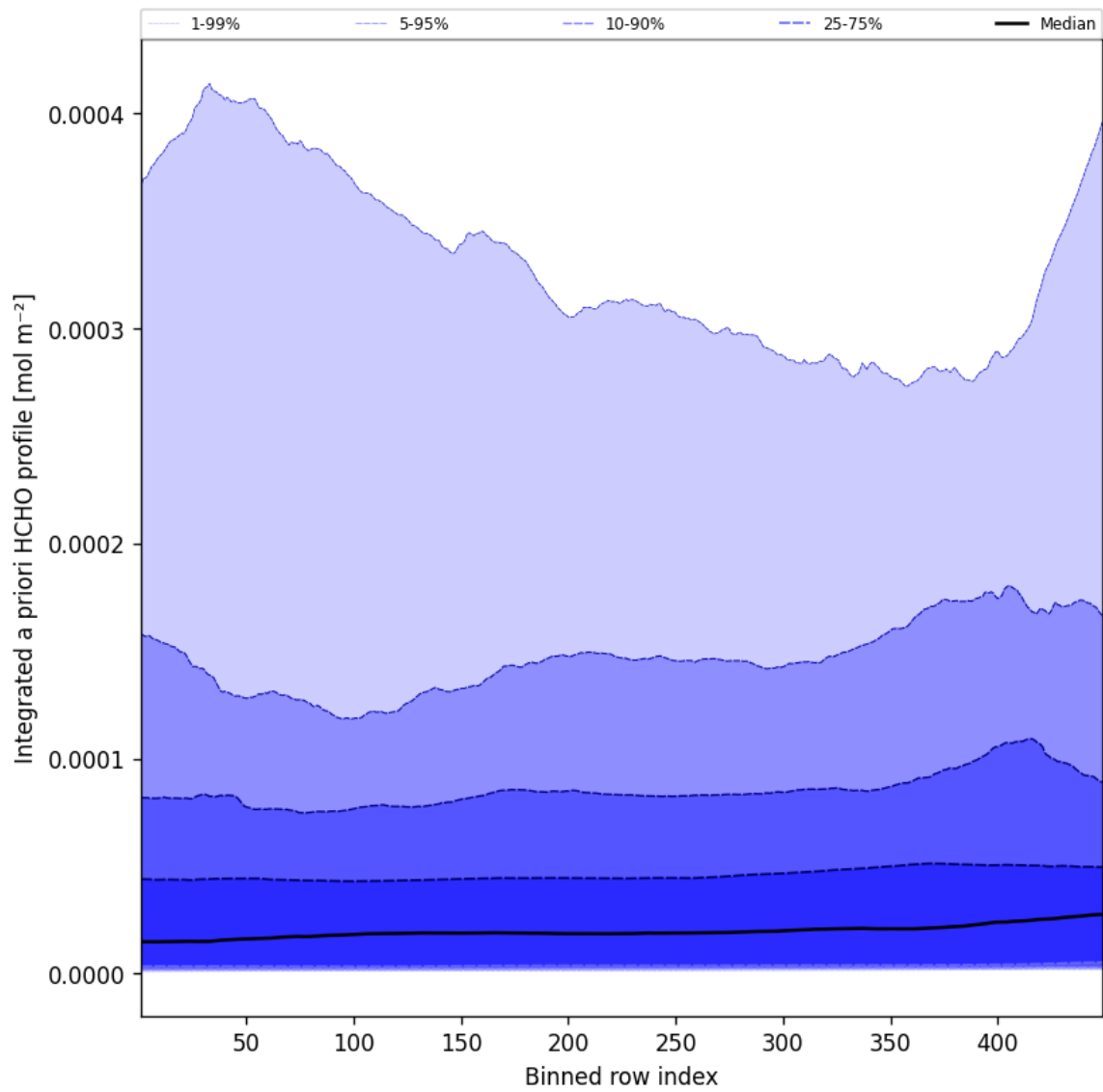
Figure 55: Along track statistics of “Integrated a priori HCHO profile” for 2025-03-20 to 2025-03-21
