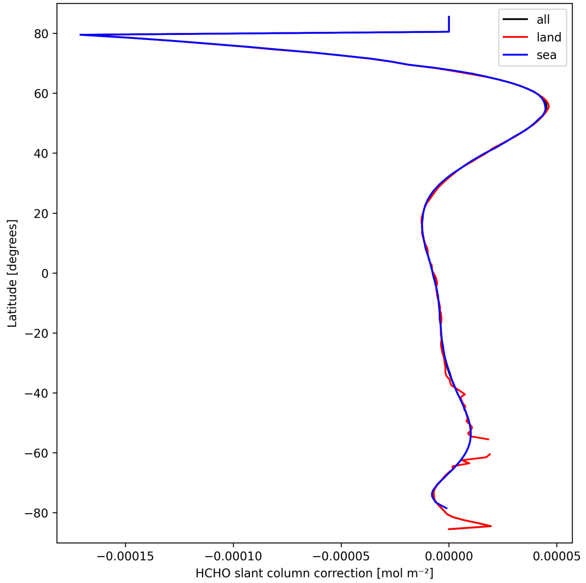
Figure 31: Zonal average of "HCHO slant column correction" for 2025-03-20 to 2025-03-21.
