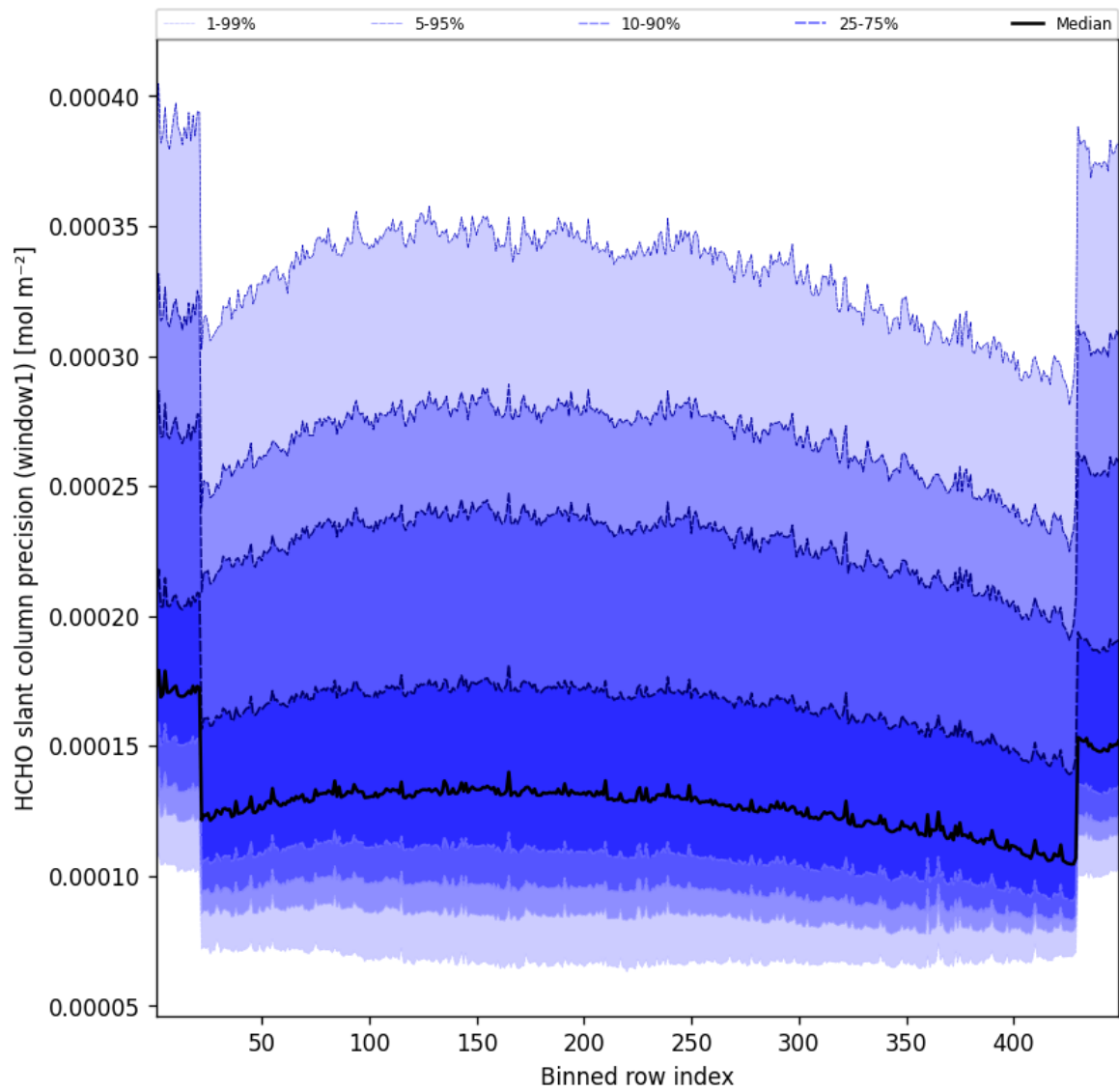
Figure 51: Along track statistics of “HCHO slant column precision (window1)” for 2025-03-20 to 2025-03-21
