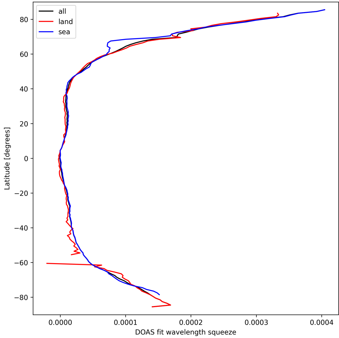
Figure 29: Zonal average of “DOAS fit wavelength squeeze” for 2025-03-20 to 2025-03-21.
