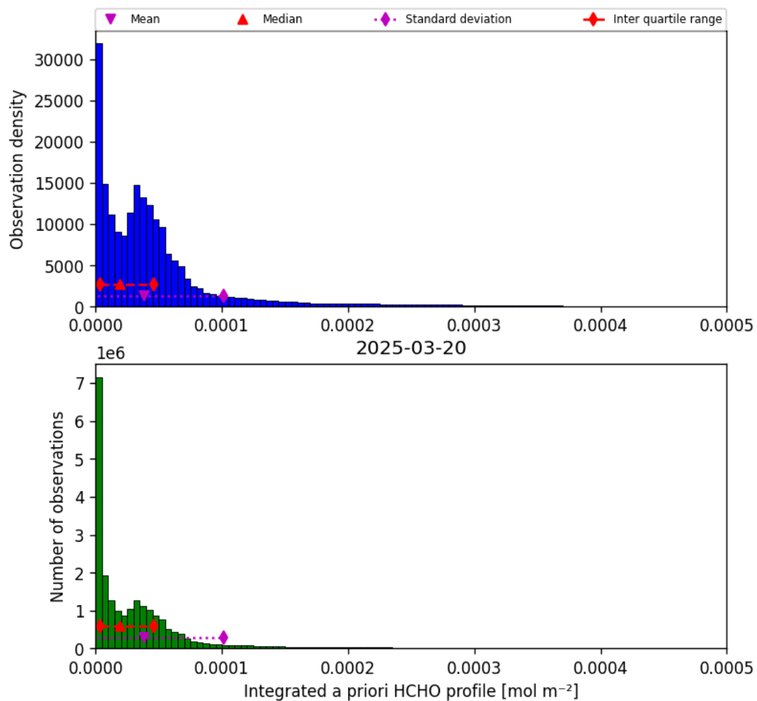
Figure 41: Histogram of “Integrated a priori HCHO profile” for 2025-03-20 to 2025-03-21
