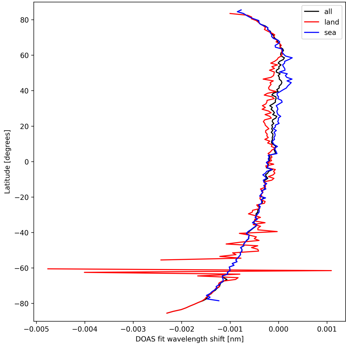
Figure 28: Zonal average of “DOAS fit wavelength shift” for 2025-03-20 to 2025-03-21.
