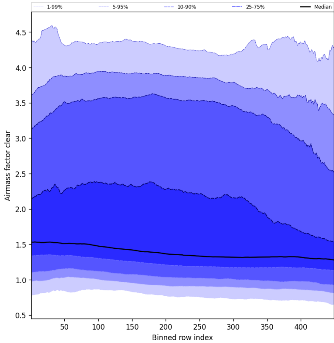
Figure 54: Along track statistics of “Airmass factor clear” for 2025-03-20 to 2025-03-21
