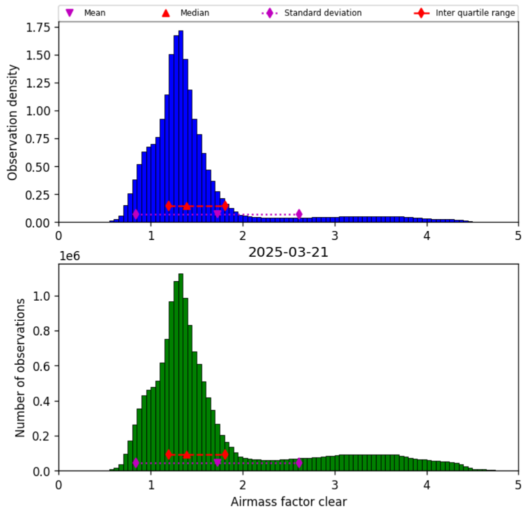
Figure 40: Histogram of “Airmass factor clear” for 2025-03-21 to 2025-03-21
