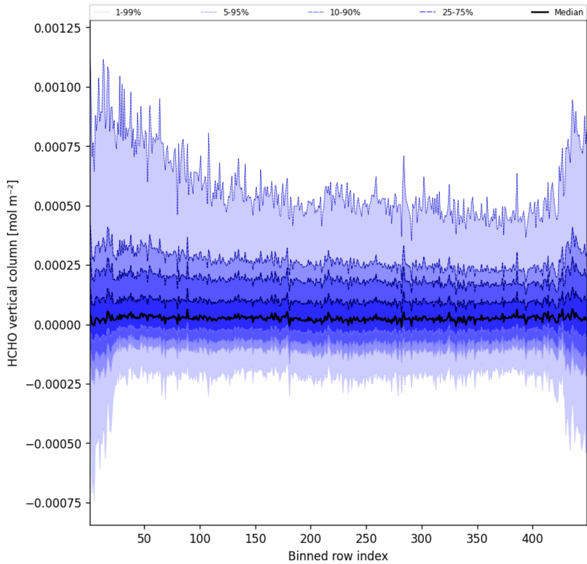
Figure 47: Along track statistics of “HCHO vertical column” for 2025-03-21 to 2025-03-21
