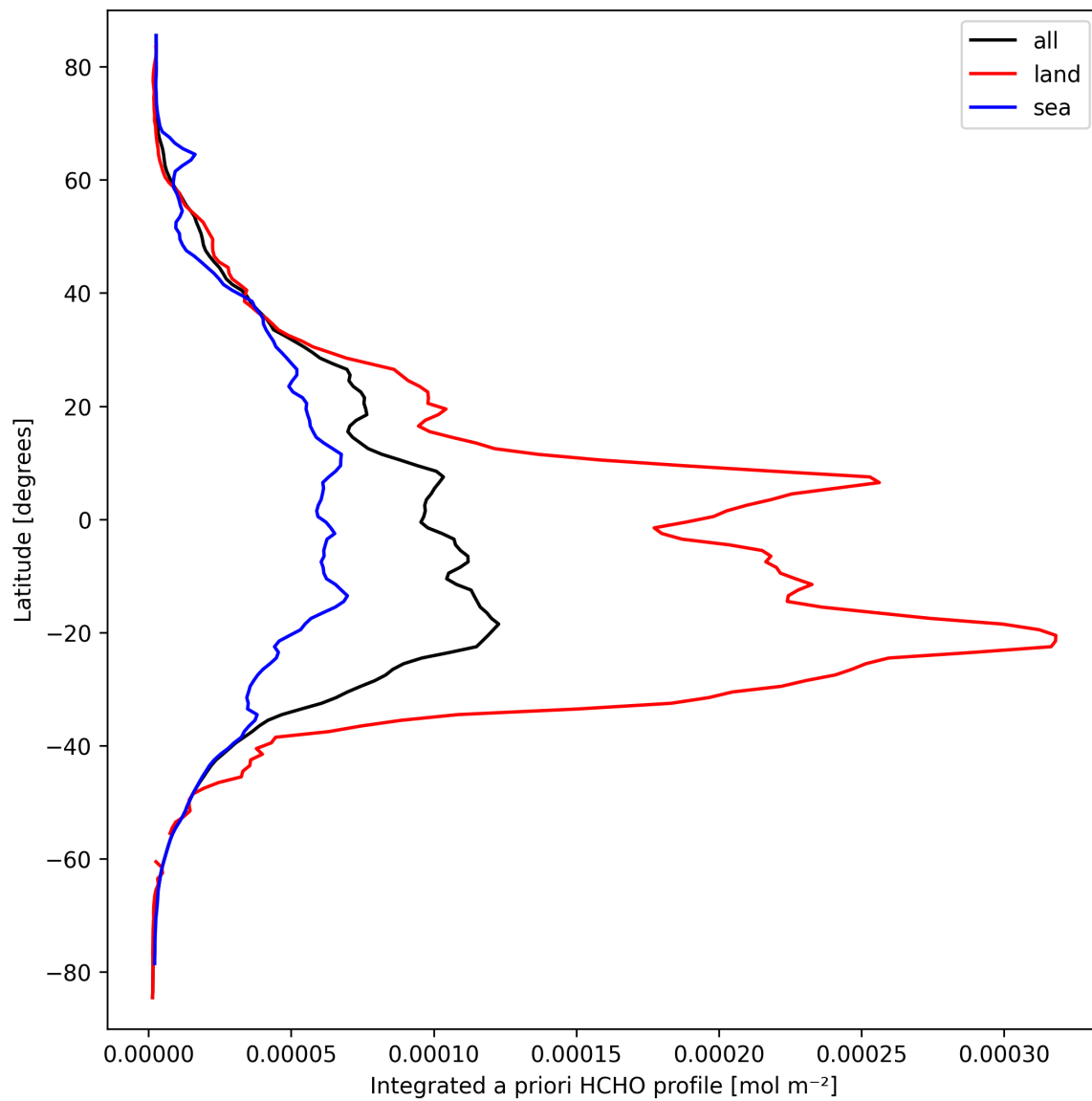
Figure 27: Zonal average of “Integrated a priori HCHO profile” for 2025-03-21 to 2025-03-21.
