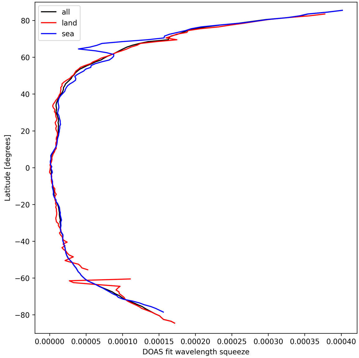
Figure 29: Zonal average of “DOAS fit wavelength squeeze” for 2025-03-21 to 2025-03-21.
