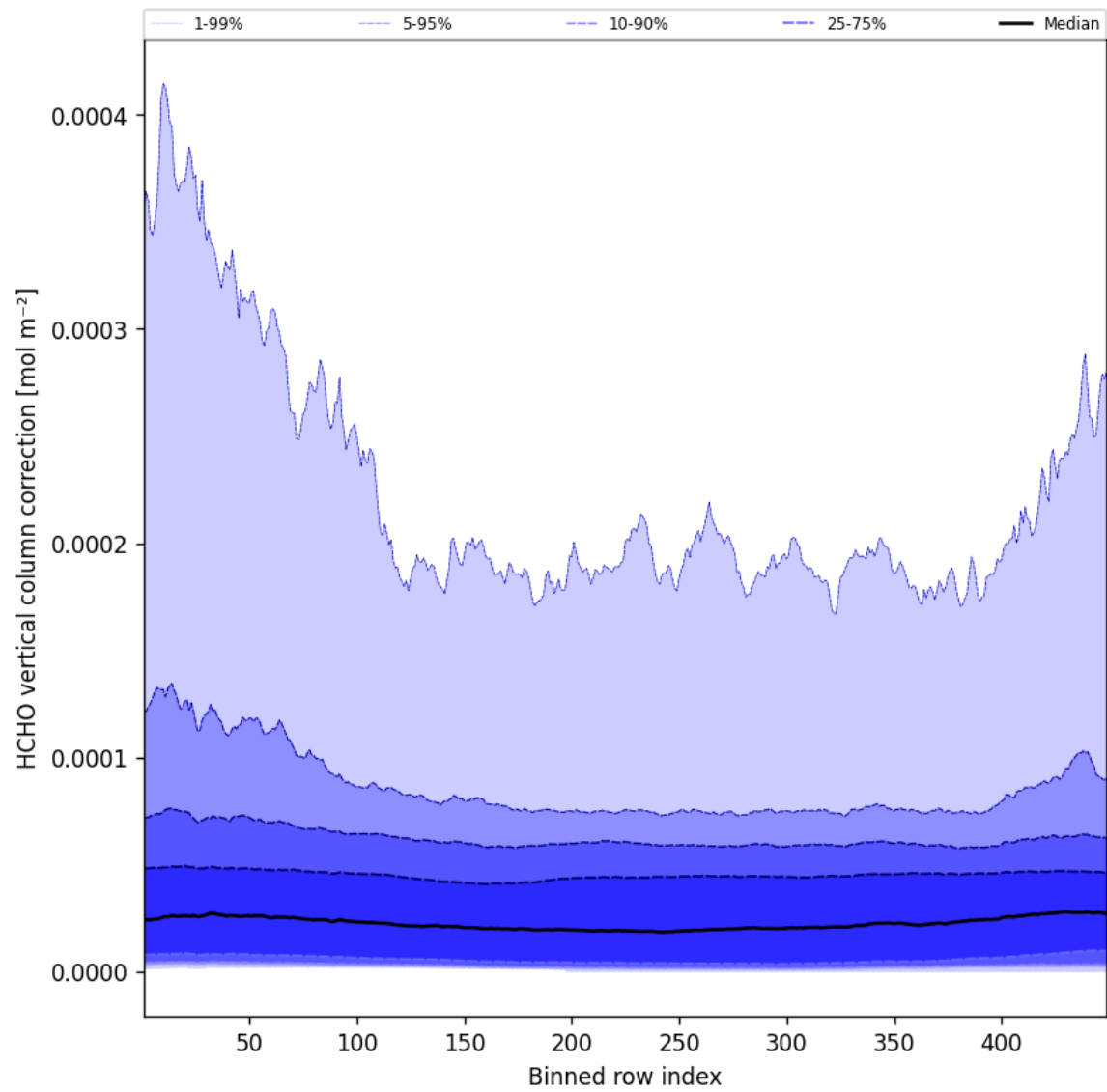
Figure 49: Along track statistics of “HCHO vertical column correction” for 2025-03-21 to 2025-03-21
