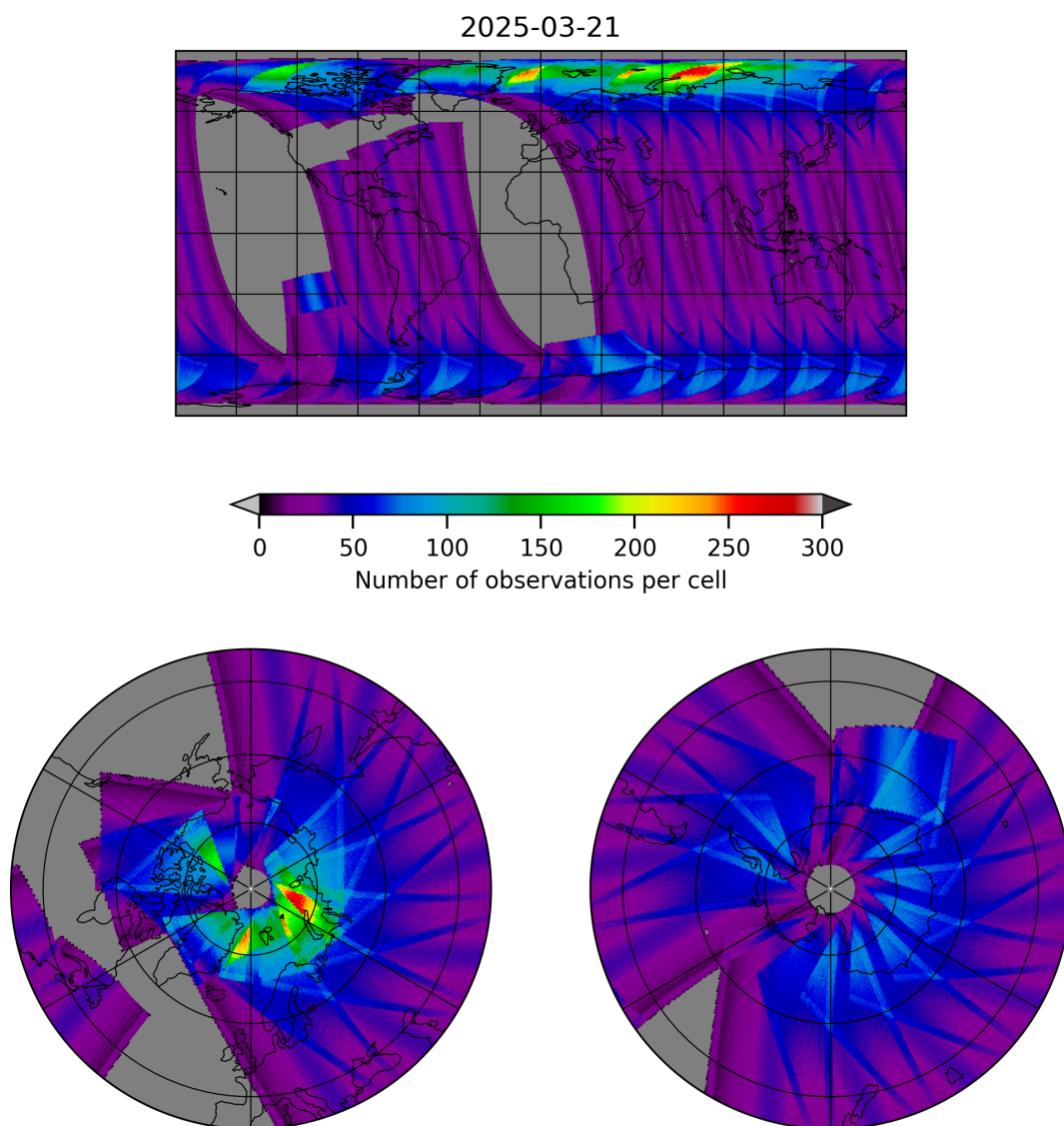
Figure 17: Map of the number of observations for 2025-03-21 to 2025-03-21
