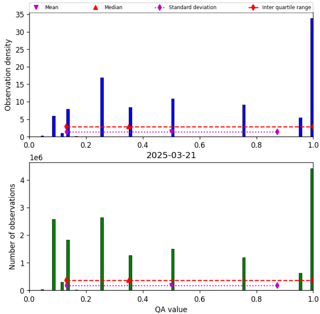
Figure 32: Histogram of “QA value” for 2025-03-21 to 2025-03-21
