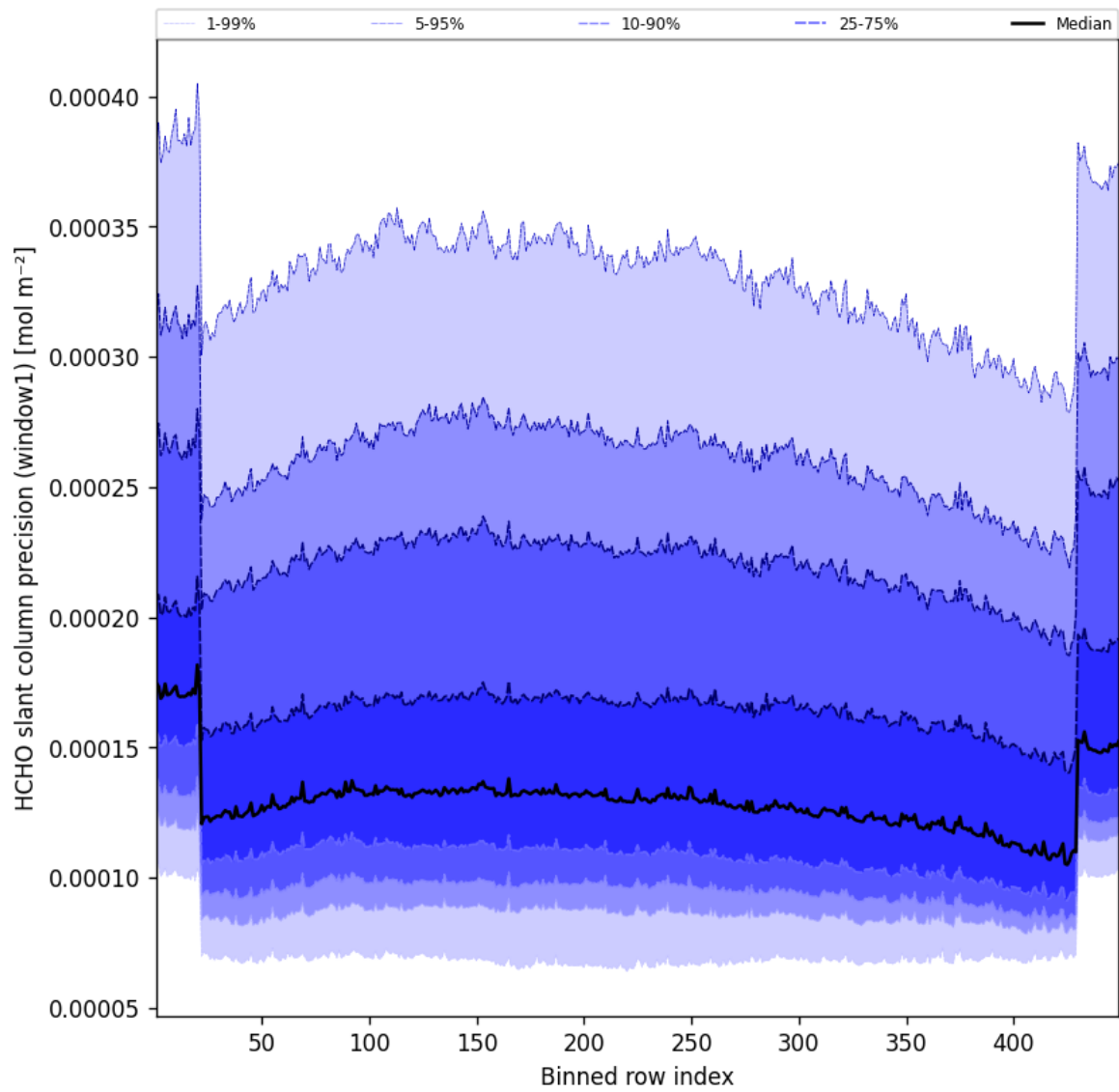
Figure 51: Along track statistics of “HCHO slant column precision (window1)” for 2025-03-21 to 2025-03-21
