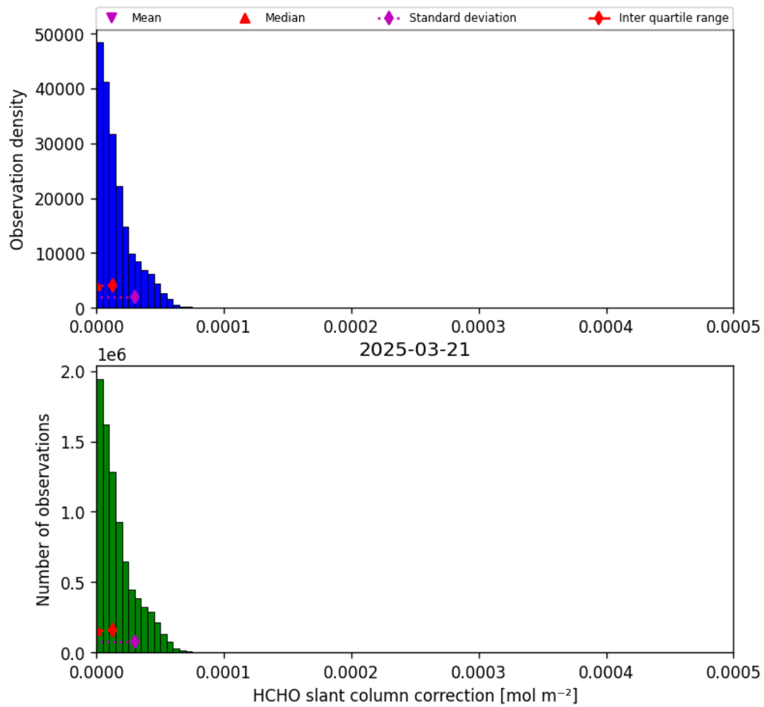
Figure 45: Histogram of “HCHO slant column correction” for 2025-03-21 to 2025-03-21
