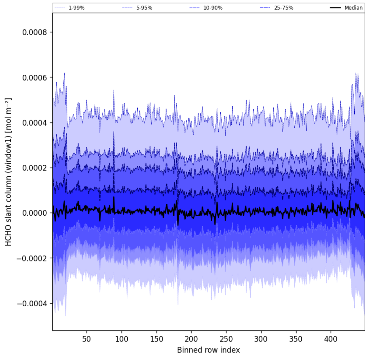
Figure 50: Along track statistics of “HCHO slant column (window1)” for 2025-03-21 to 2025-03-21
