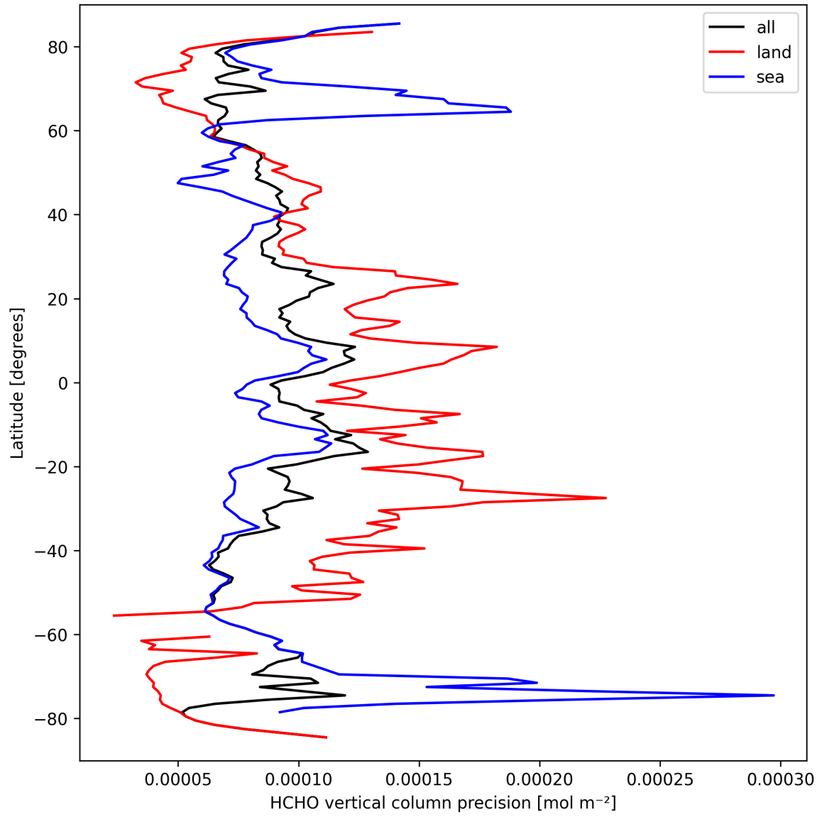
Figure 20: Zonal average of “HCHO vertical column precision” for 2025-03-21 to 2025-03-21.
