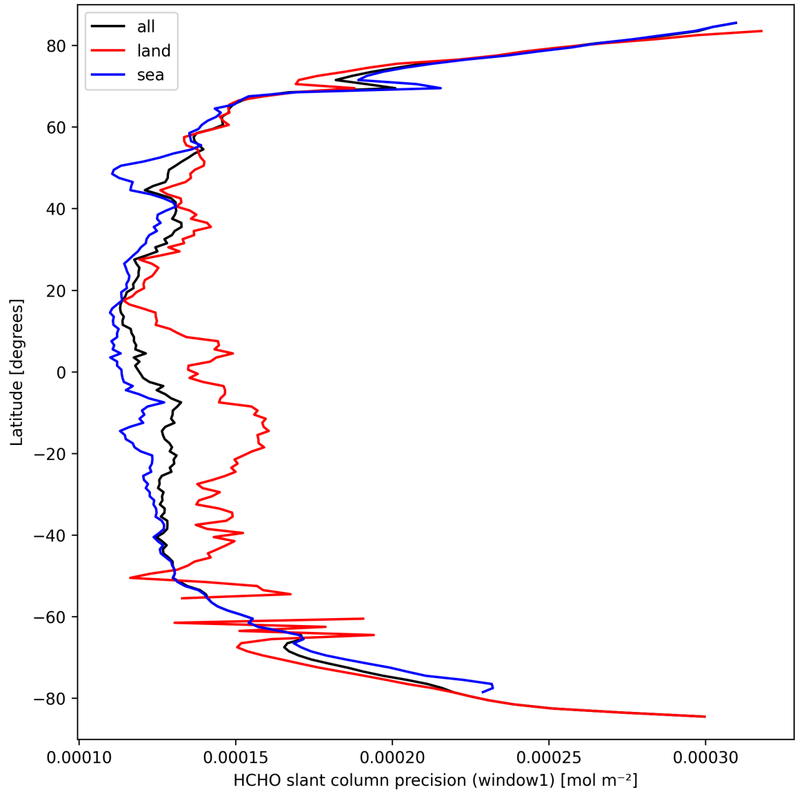
Figure 23: Zonal average of “HCHO slant column precision (window1)” for 2025-03-21 to 2025-03-21.
