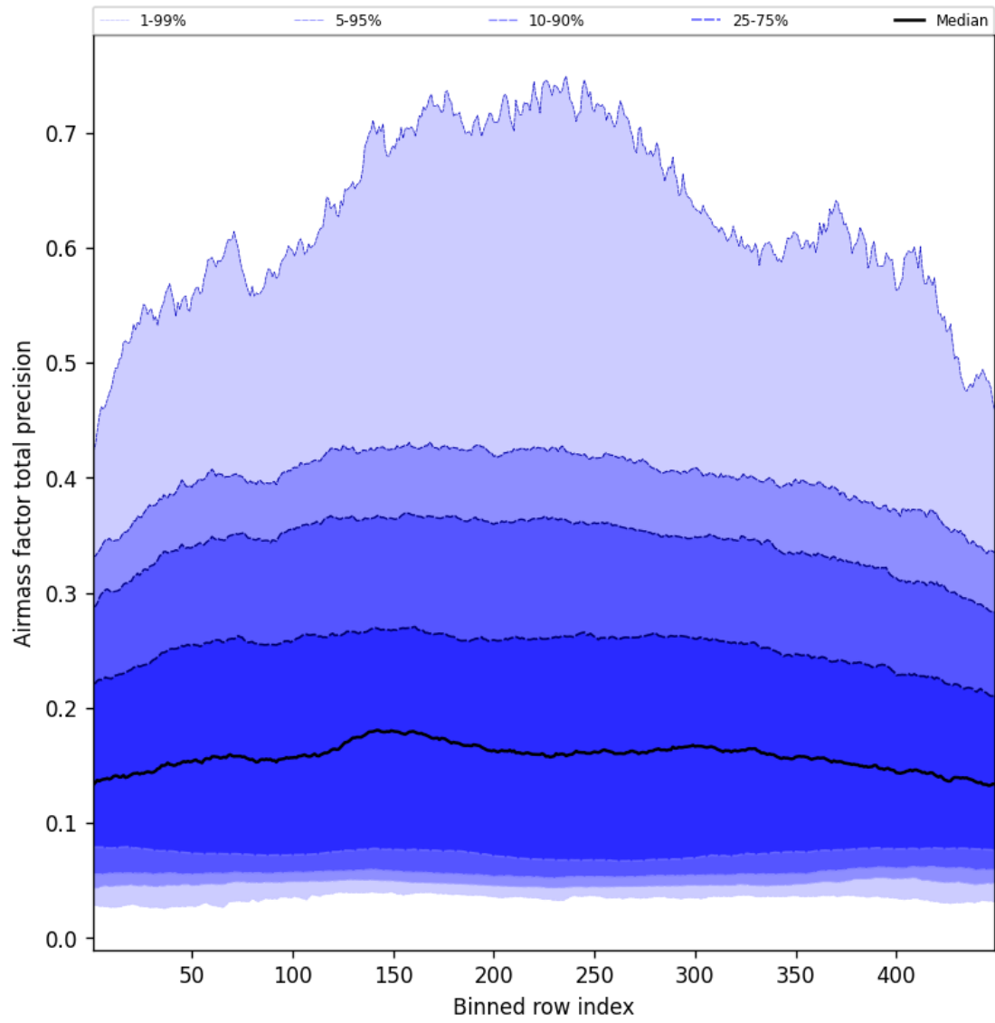
Figure 53: Along track statistics of “Airmass factor total precision” for 2025-03-21 to 2025-03-21
