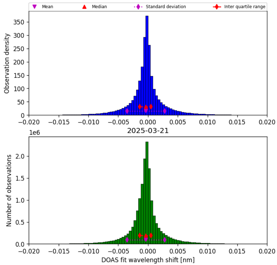
Figure 42: Histogram of “DOAS fit wavelength shift” for 2025-03-21 to 2025-03-21
