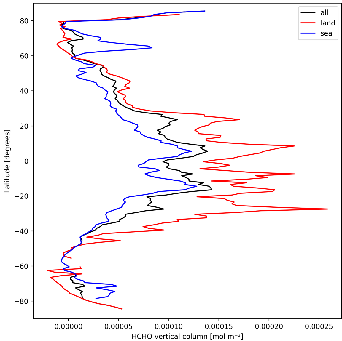
Figure 19: Zonal average of “HCHO vertical column” for 2025-03-21 to 2025-03-21.
