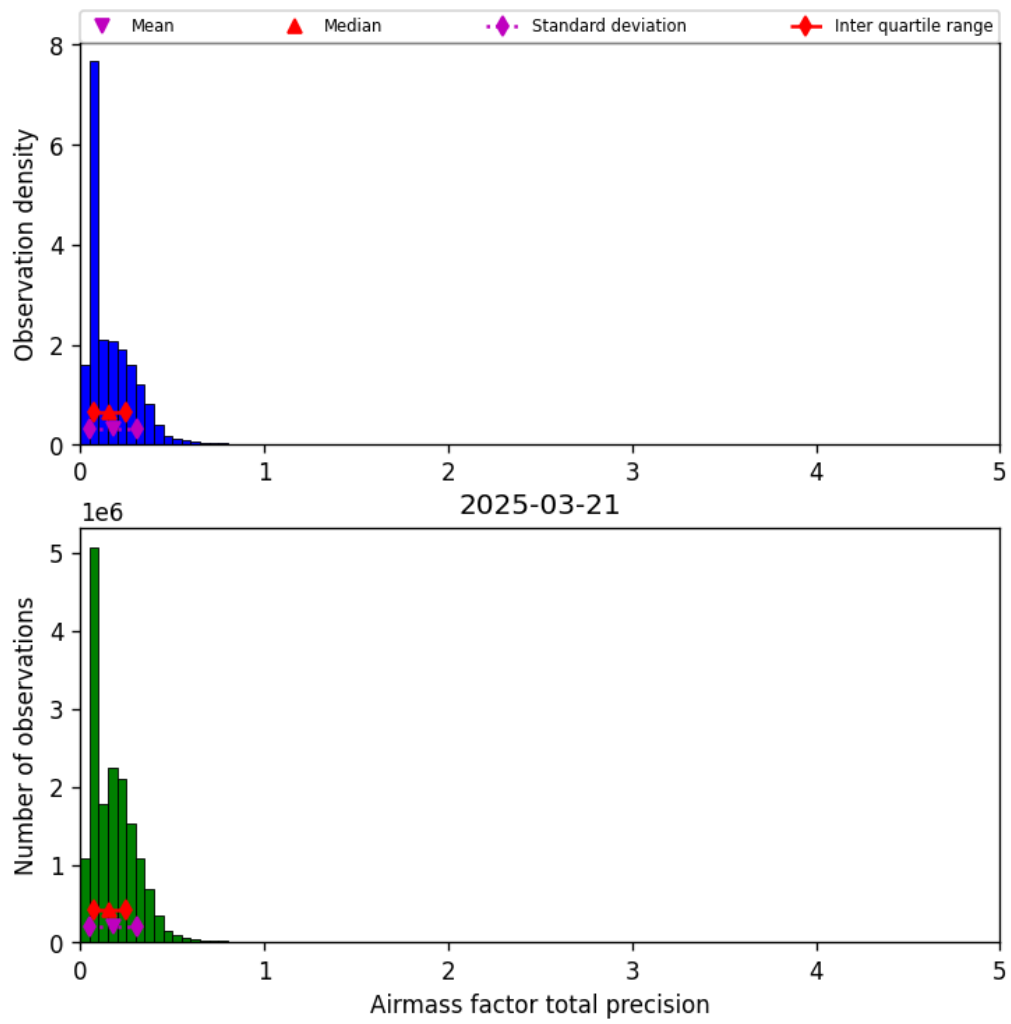
Figure 39: Histogram of “Airmass factor total precision” for 2025-03-21 to 2025-03-21
