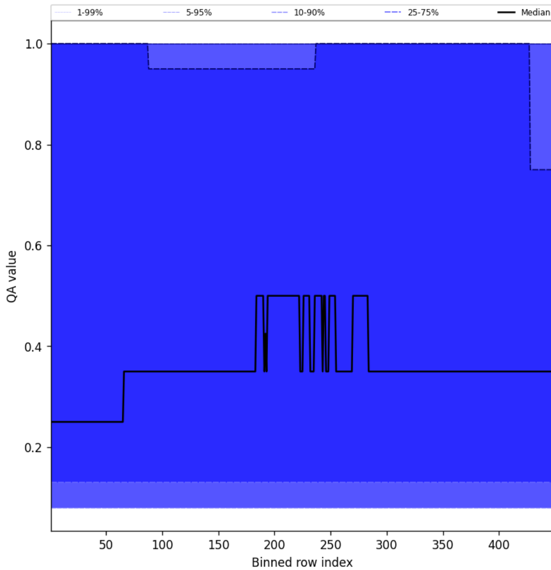
Figure 46: Along track statistics of “QA value” for 2025-03-21 to 2025-03-21
