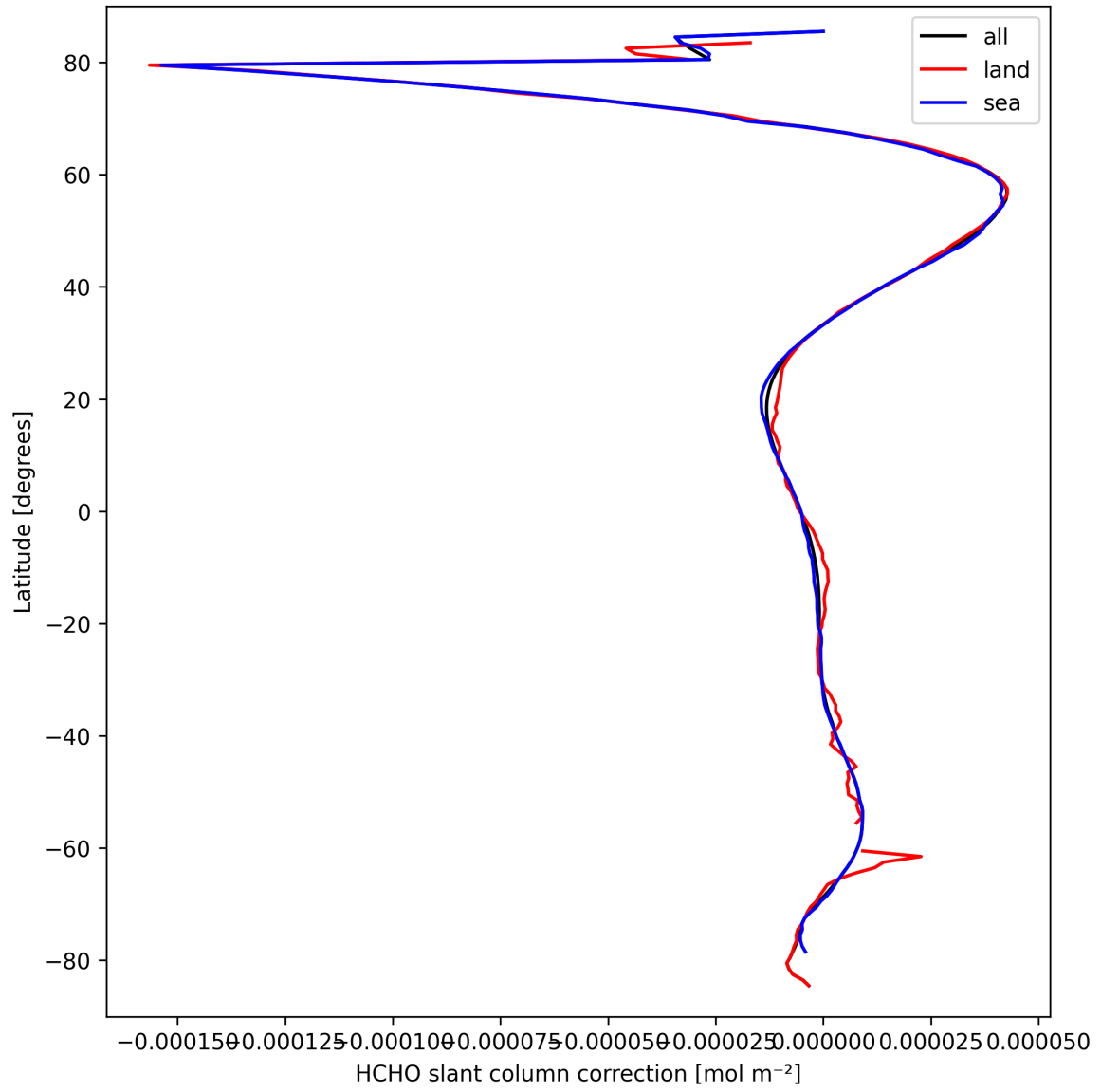
Figure 31: Zonal average of “HCHO slant column correction” for 2025-03-21 to 2025-03-21.
