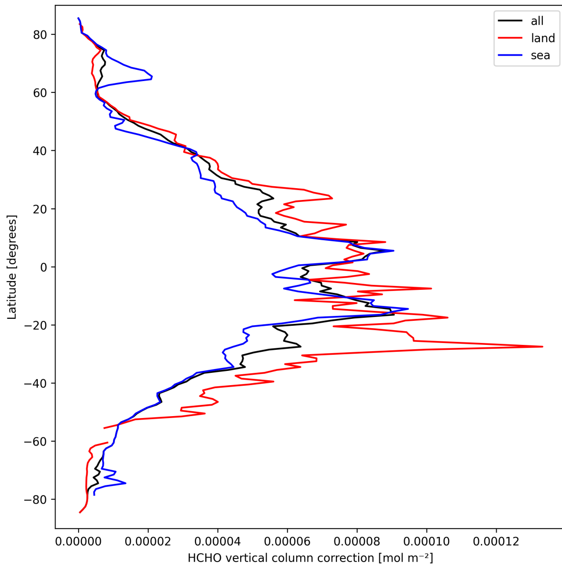
Figure 21: Zonal average of “HCHO vertical column correction” for 2025-03-21 to 2025-03-21.
