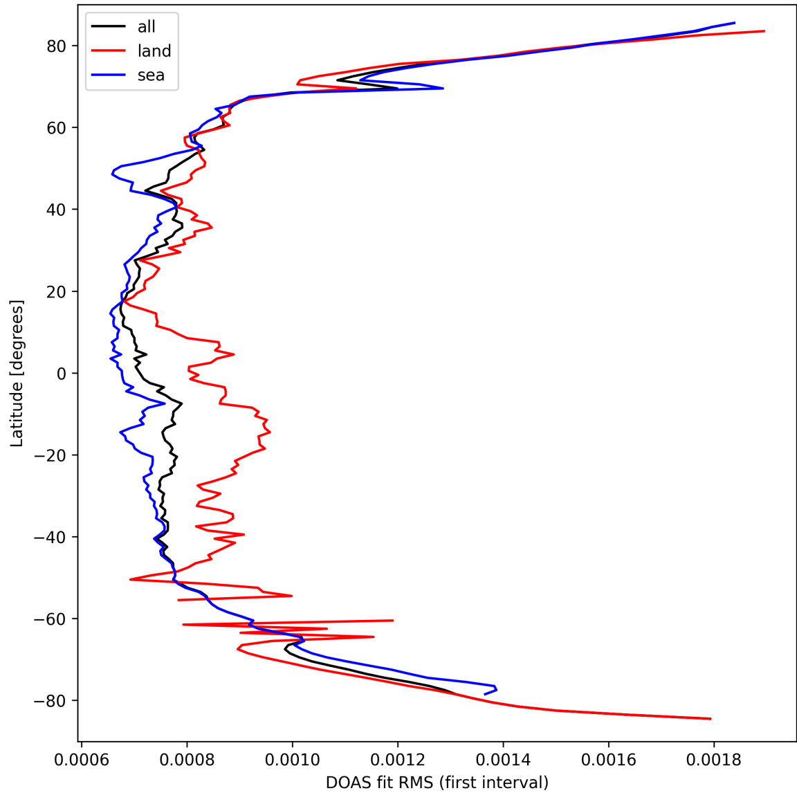
Figure 30: Zonal average of “DOAS fit RMS (first interval)” for 2025-03-21 to 2025-03-21.
