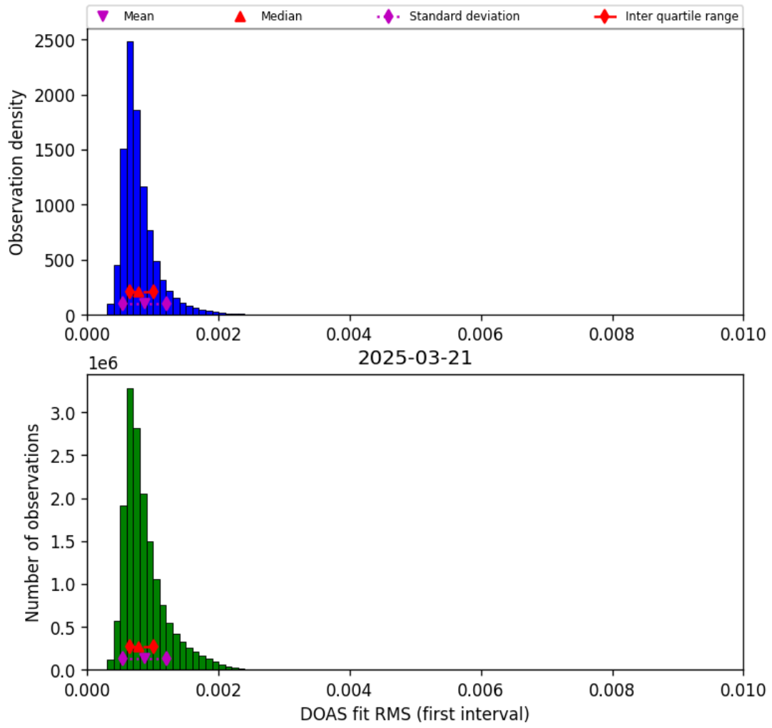
Figure 44: Histogram of “DOAS fit RMS (first interval)” for 2025-03-21 to 2025-03-21
