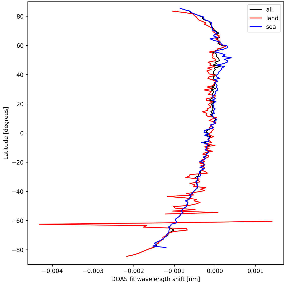
Figure 28: Zonal average of “DOAS fit wavelength shift” for 2025-03-21 to 2025-03-21.
