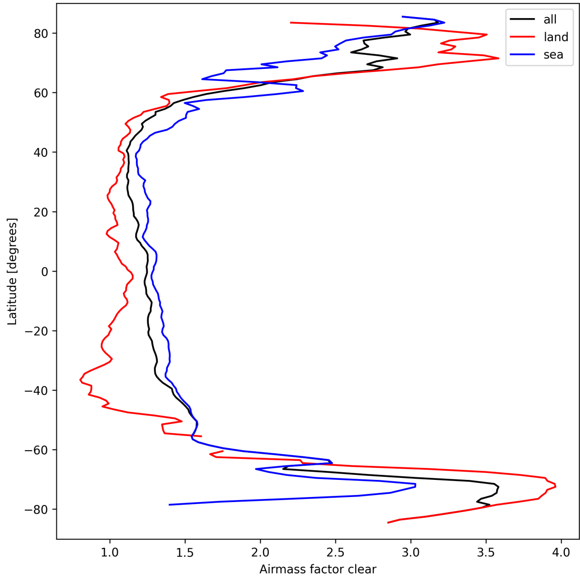
Figure 26: Zonal average of “Airmass factor clear” for 2025-03-21 to 2025-03-21.
