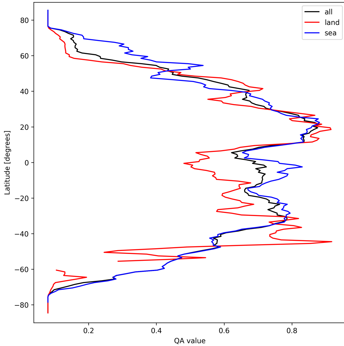
Figure 18: Zonal average of “QA value” for 2025-03-21 to 2025-03-21.
