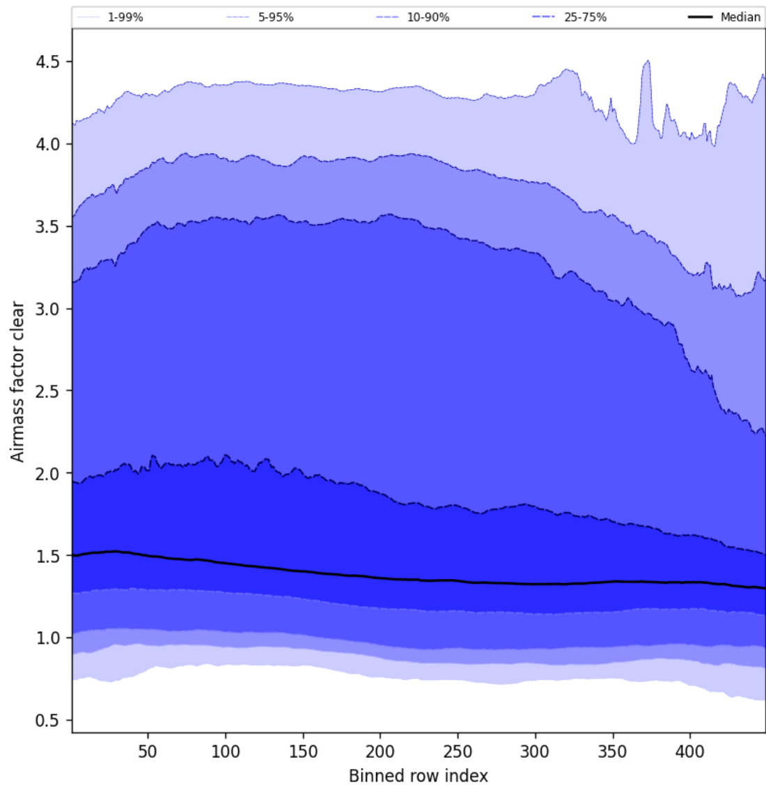
Figure 54: Along track statistics of “Airmass factor clear” for 2025-03-21 to 2025-03-21
