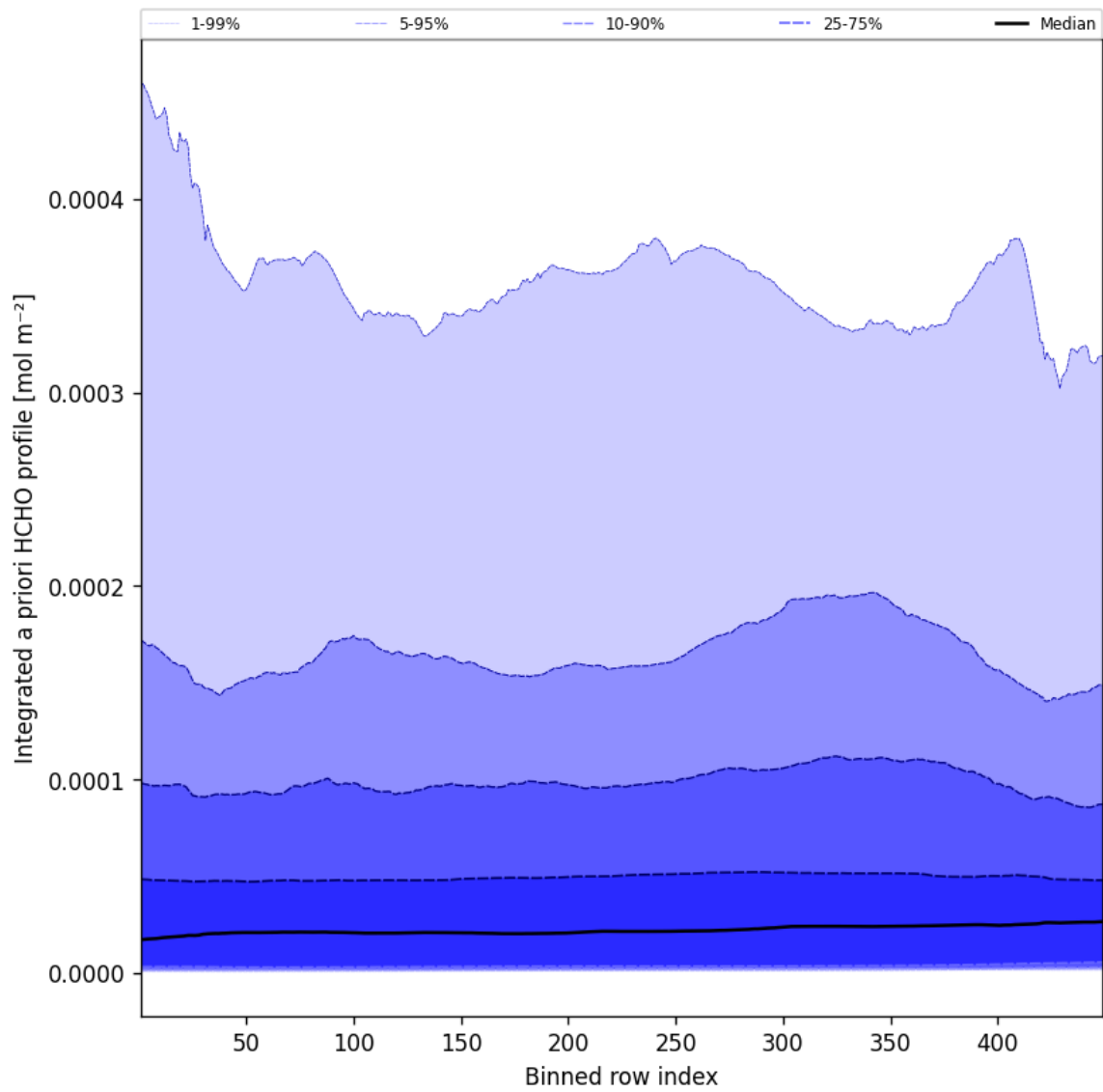
Figure 55: Along track statistics of “Integrated a priori HCHO profile” for 2025-03-21 to 2025-03-21
