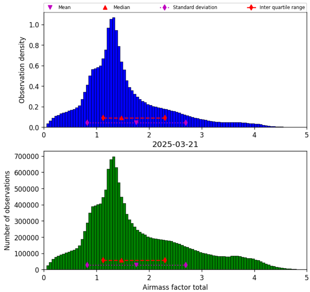
Figure 38: Histogram of “Airmass factor total” for 2025-03-21 to 2025-03-21
