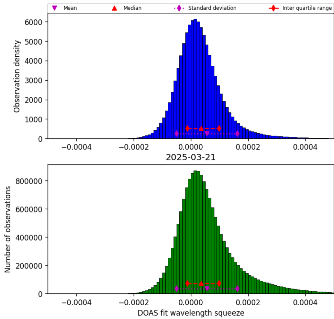
Figure 43: Histogram of “DOAS fit wavelength squeeze” for 2025-03-21 to 2025-03-21
