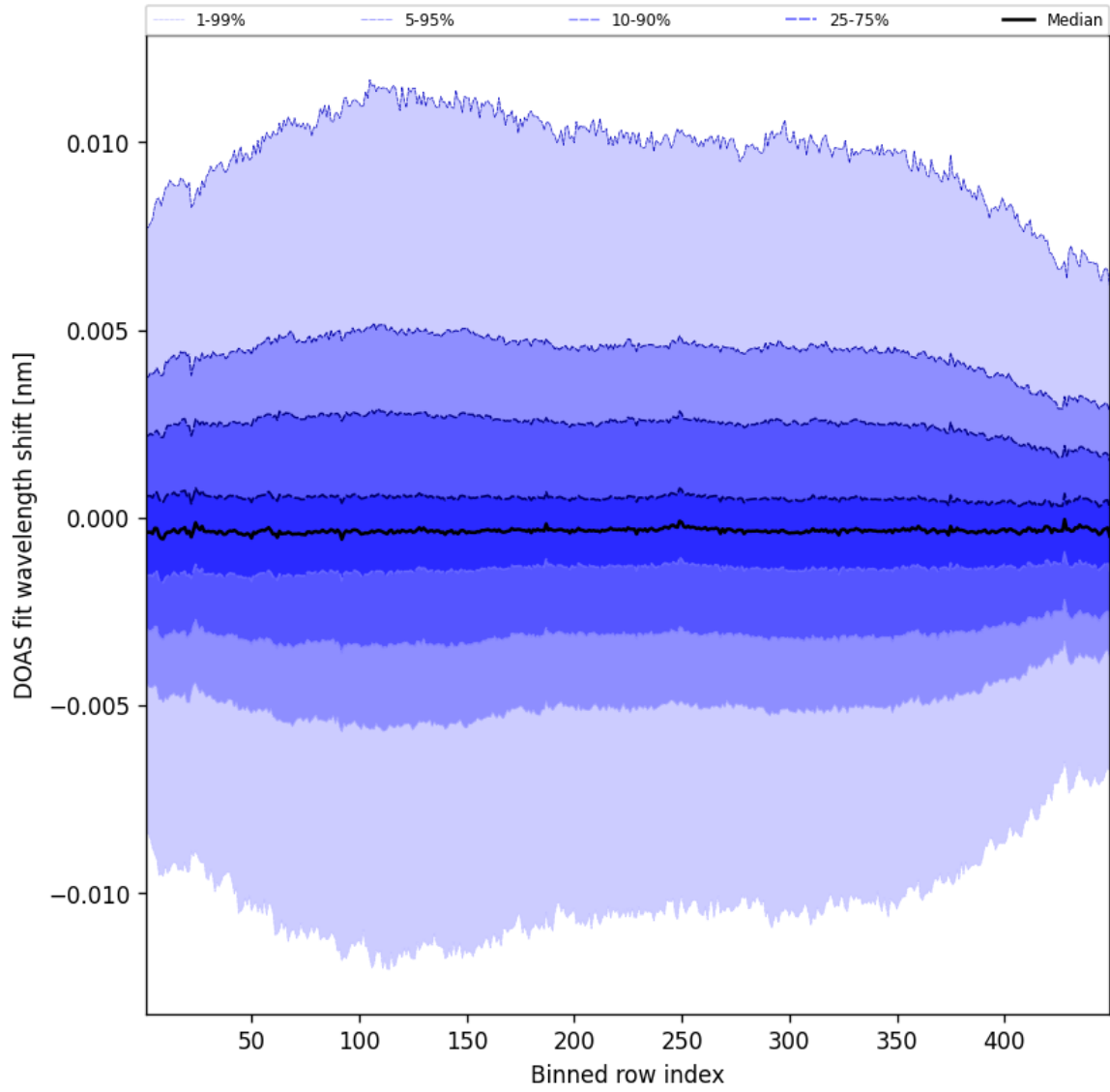
Figure 56: Along track statistics of “DOAS fit wavelength shift” for 2025-03-21 to 2025-03-21
