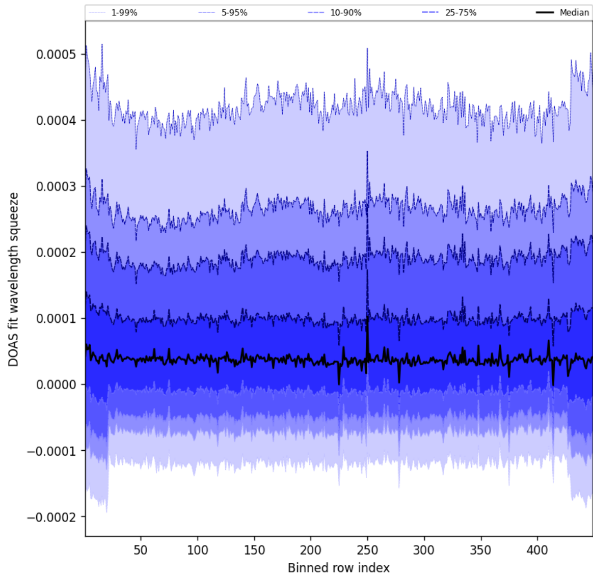
Figure 57: Along track statistics of “DOAS fit wavelength squeeze” for 2025-03-21 to 2025-03-21
