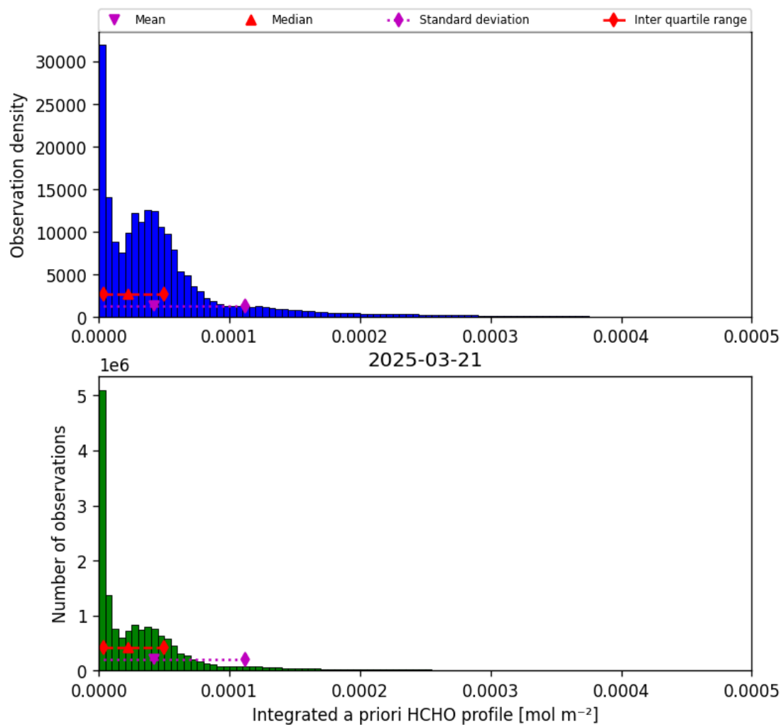
Figure 41: Histogram of “Integrated a priori HCHO profile” for 2025-03-21 to 2025-03-21
