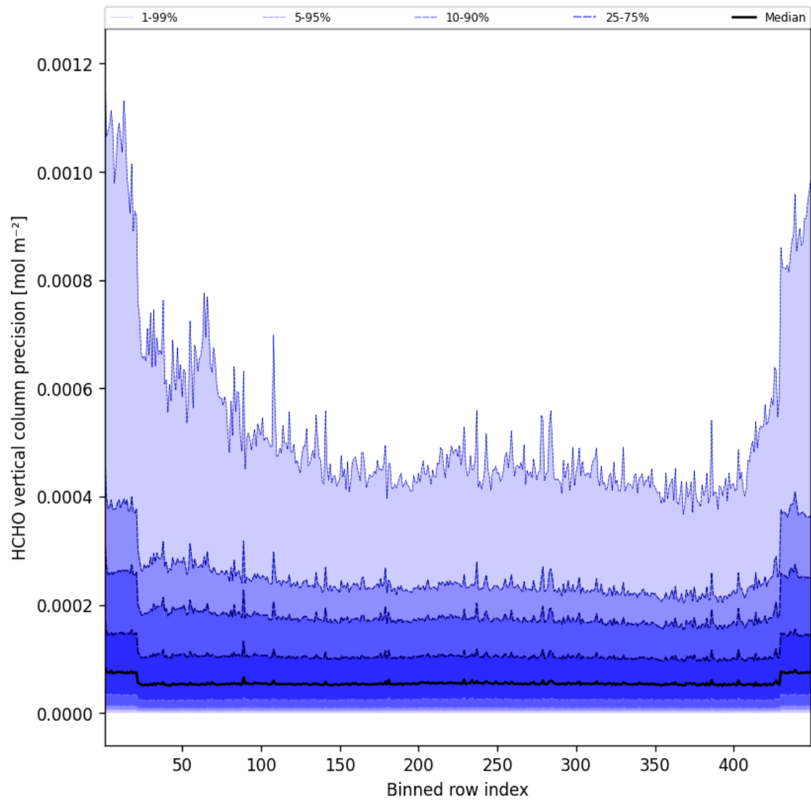
Figure 48: Along track statistics of “HCHO vertical column precision” for 2025-03-21 to 2025-03-21
