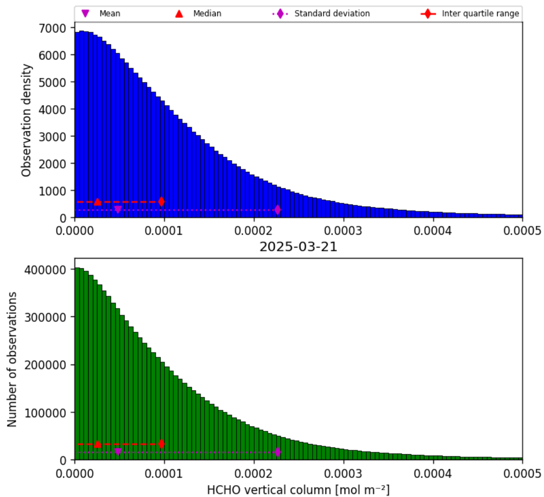
Figure 33: Histogram of “HCHO vertical column” for 2025-03-21 to 2025-03-21
