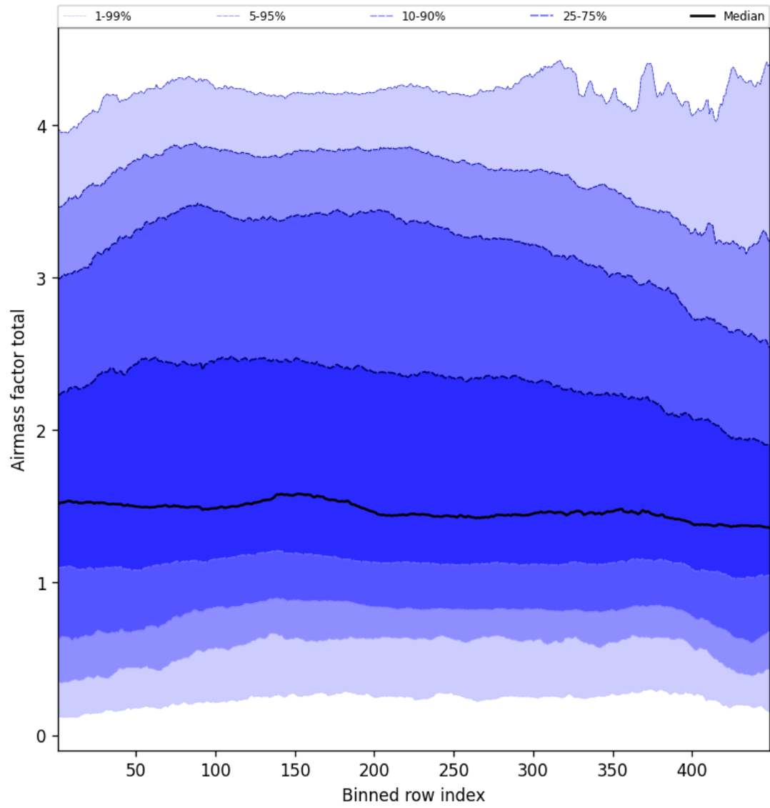
Figure 52: Along track statistics of “Airmass factor total” for 2025-03-21 to 2025-03-21
