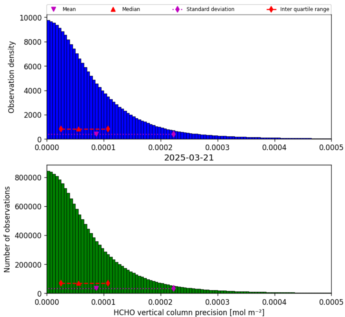
Figure 34: Histogram of “HCHO vertical column precision” for 2025-03-21 to 2025-03-21
