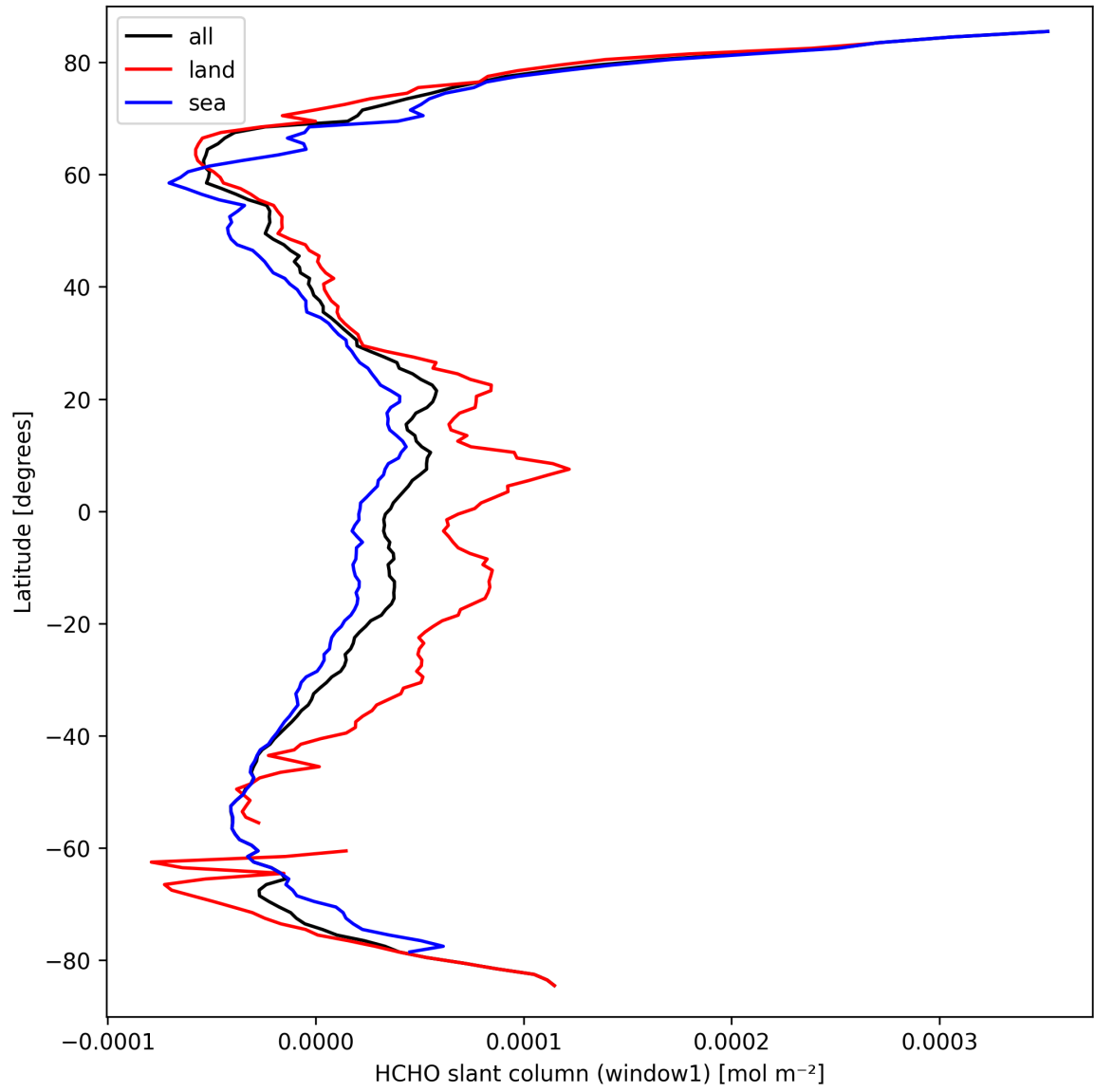
Figure 22: Zonal average of “HCHO slant column (window1)” for 2025-03-21 to 2025-03-21.
