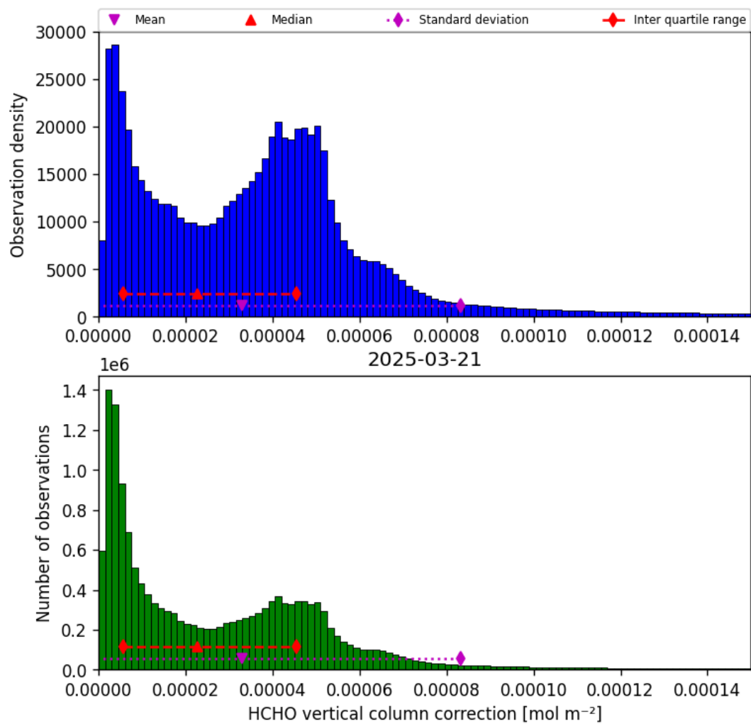
Figure 35: Histogram of “HCHO vertical column correction” for 2025-03-21 to 2025-03-21
