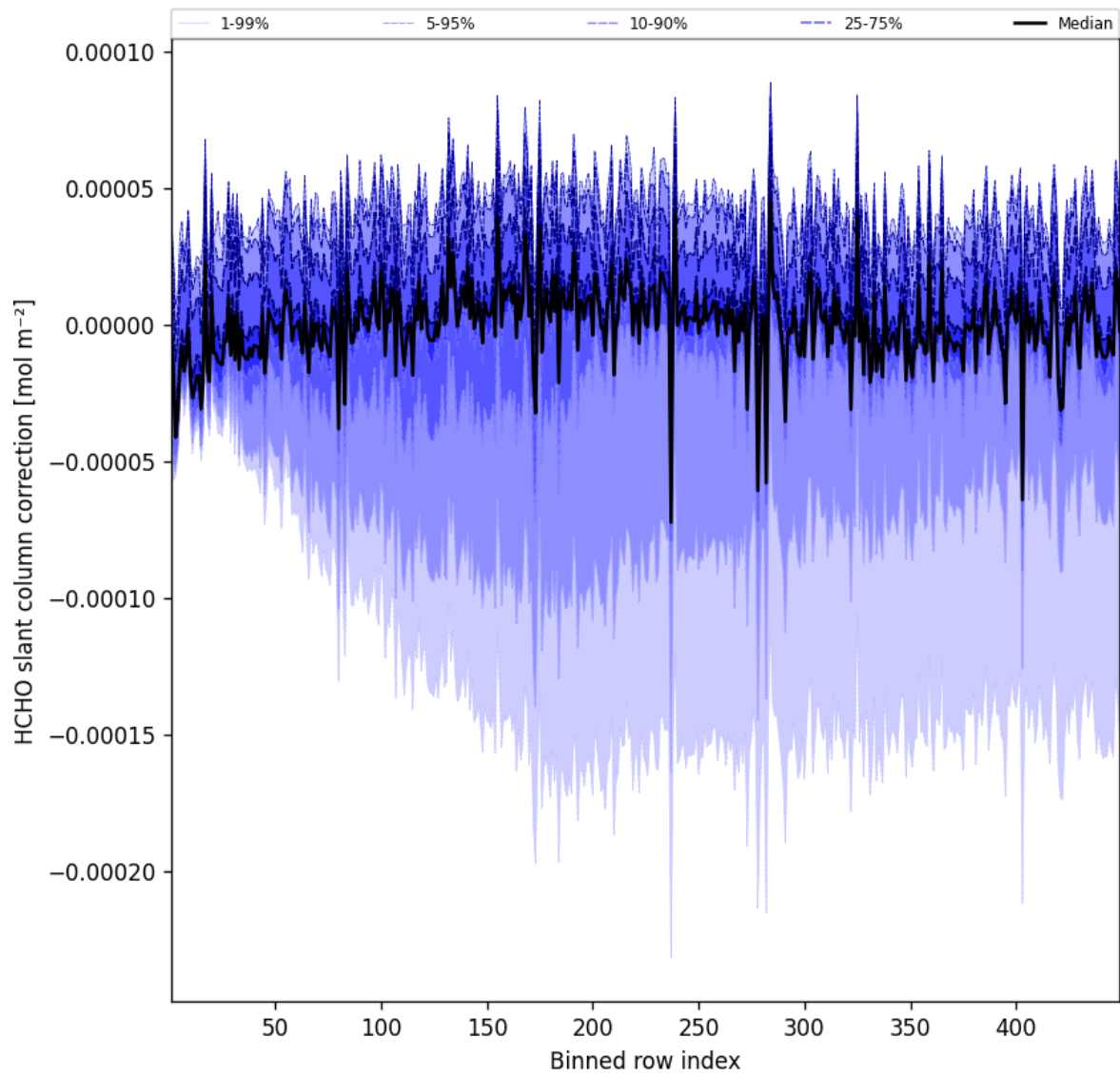
Figure 59: Along track statistics of “HCHO slant column correction” for 2025-03-21 to 2025-03-21
