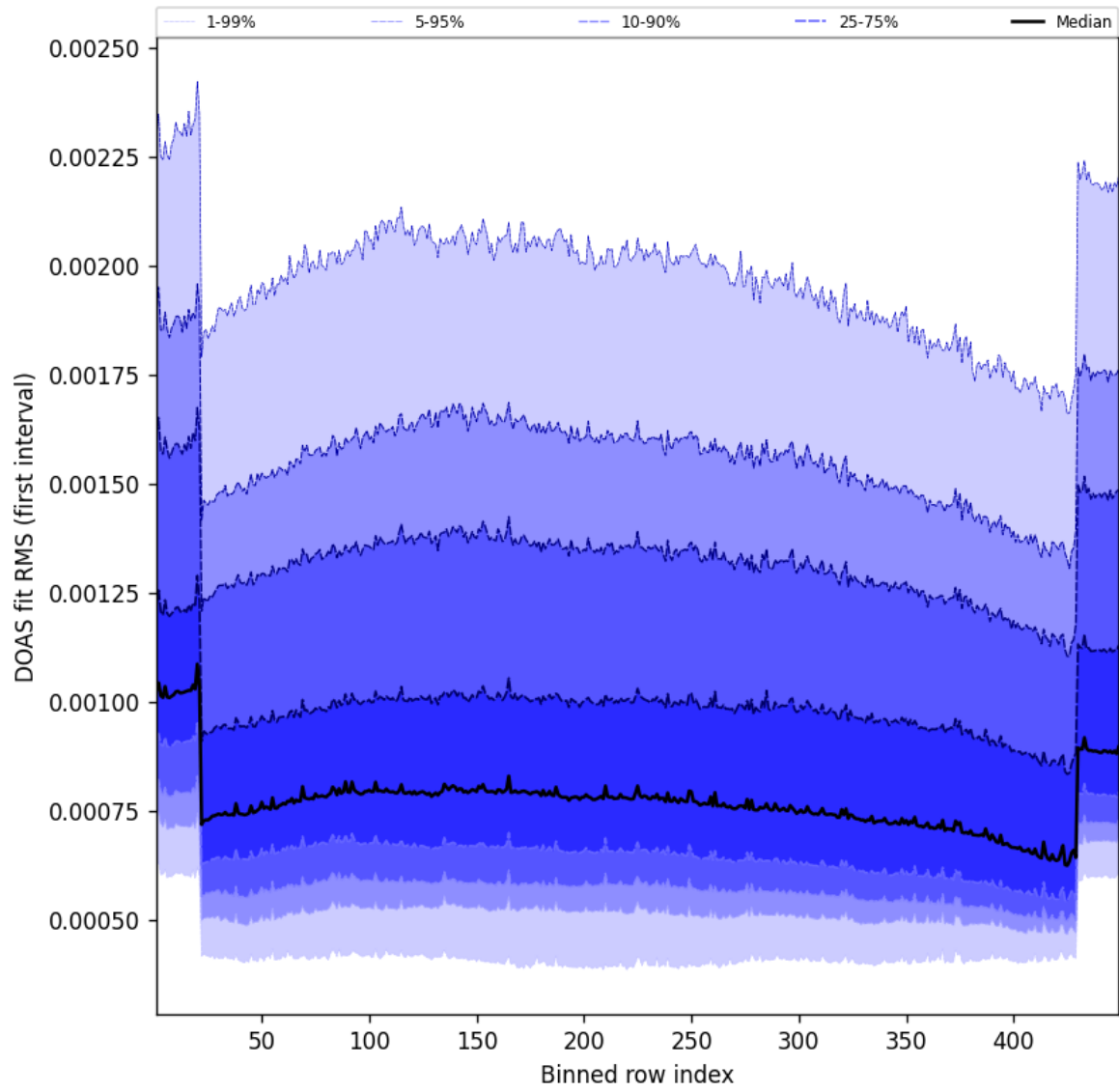
Figure 58: Along track statistics of “DOAS fit RMS (first interval)” for 2025-03-21 to 2025-03-21
