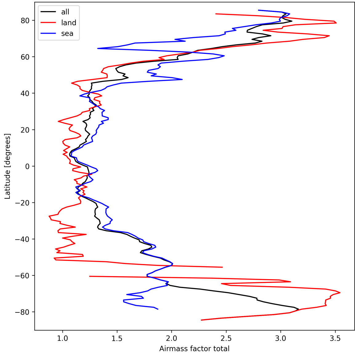
Figure 24: Zonal average of “Airmass factor total” for 2025-03-21 to 2025-03-21.
