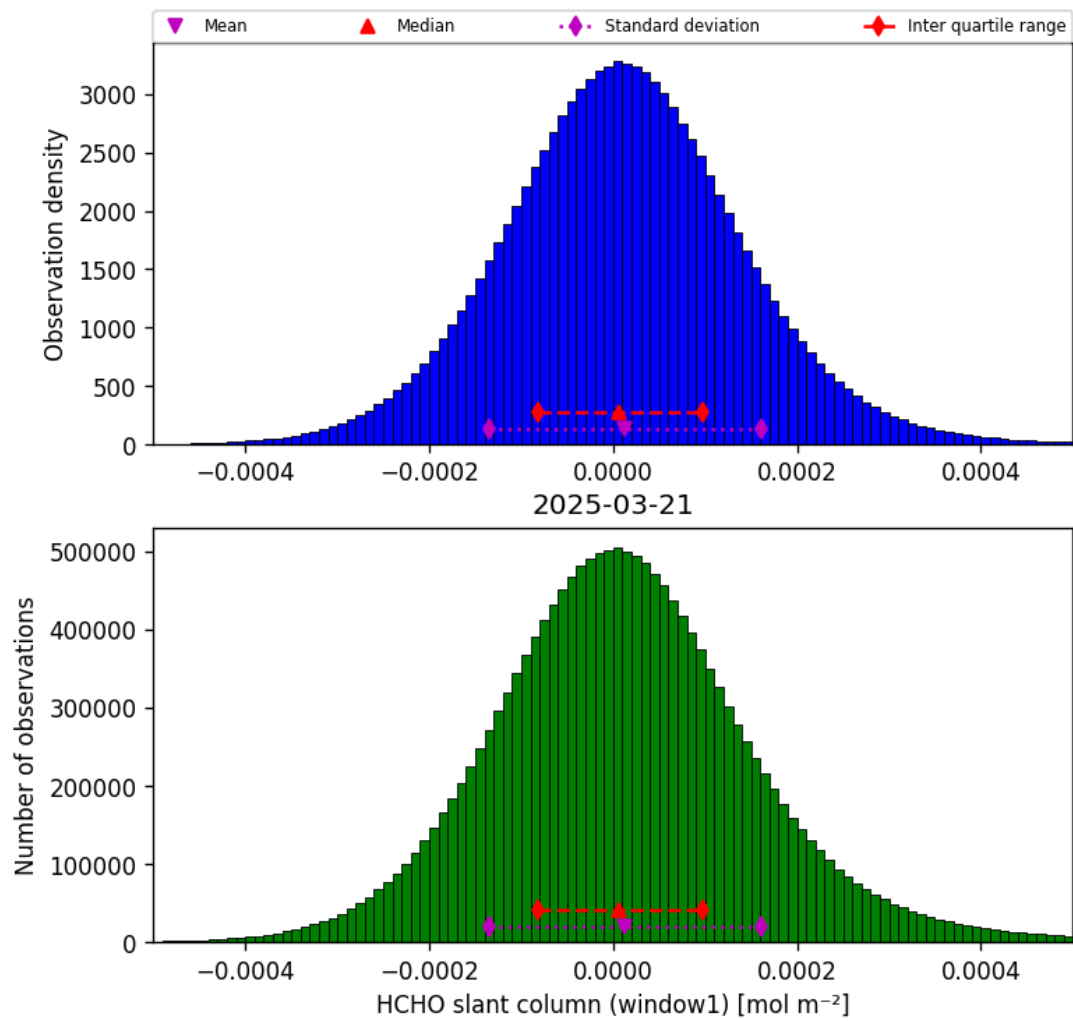
Figure 36: Histogram of “HCHO slant column (window1)” for 2025-03-21 to 2025-03-21
