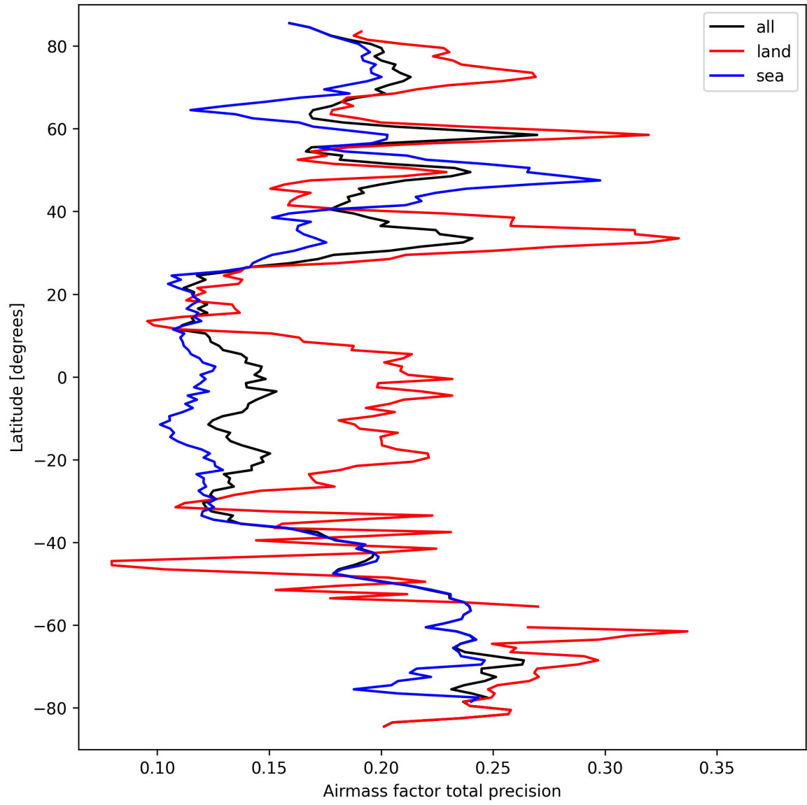
Figure 25: Zonal average of “Airmass factor total precision” for 2025-03-21 to 2025-03-21.
