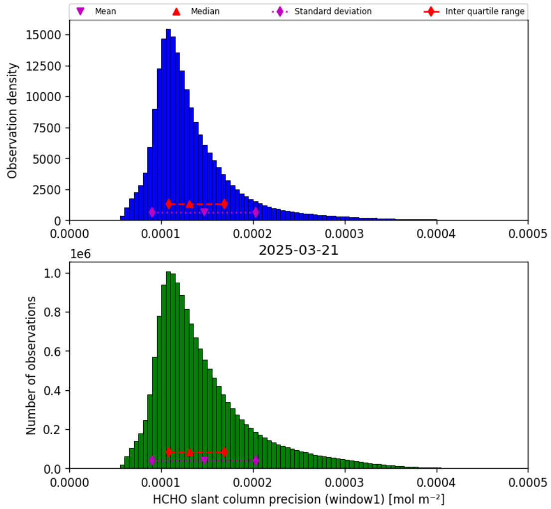
Figure 37: Histogram of “HCHO slant column precision (window1)” for 2025-03-21 to 2025-03-21
