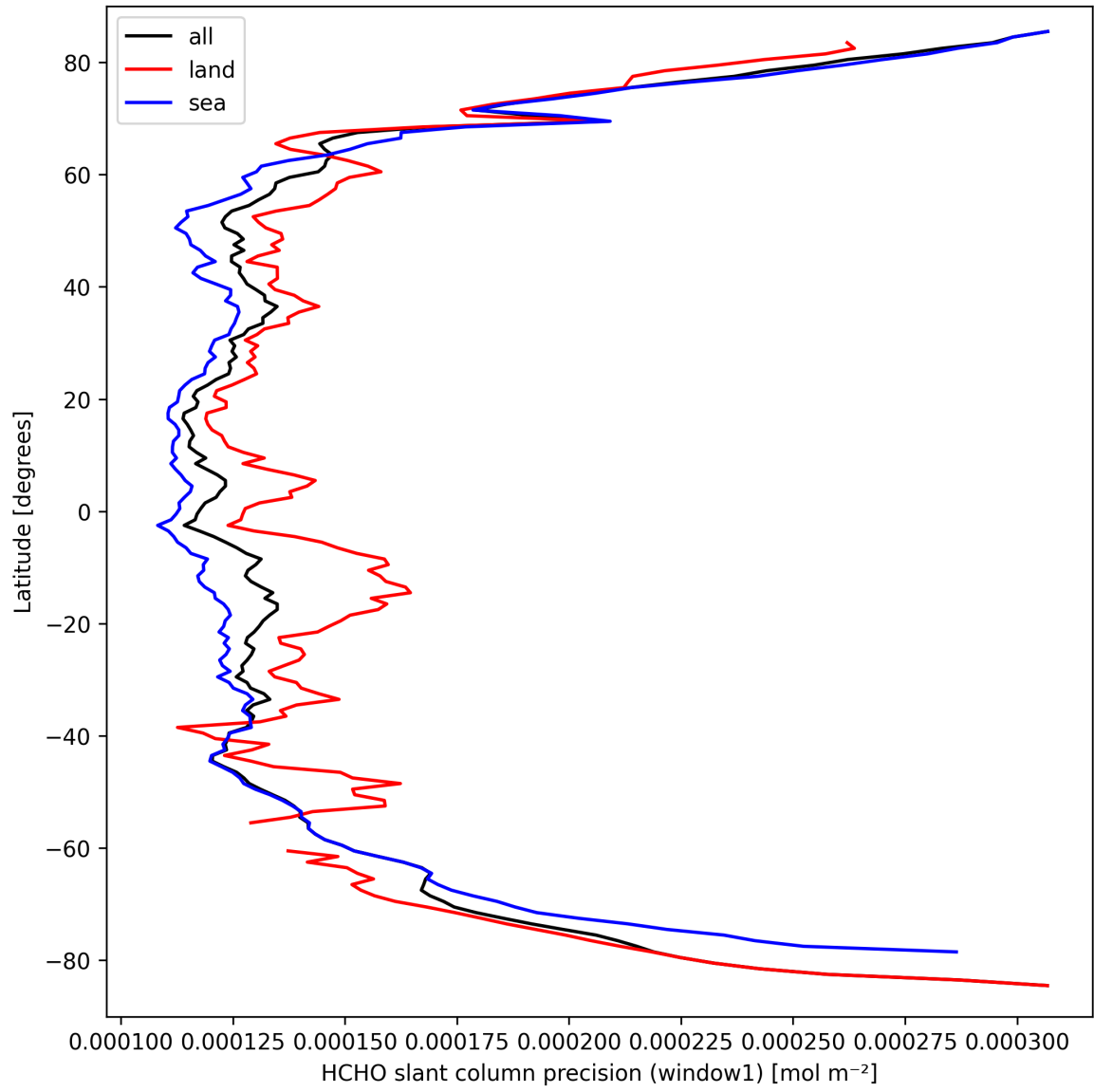
Figure 23: Zonal average of “HCHO slant column precision (window1)” for 2025-03-22 to 2025-03-22.
