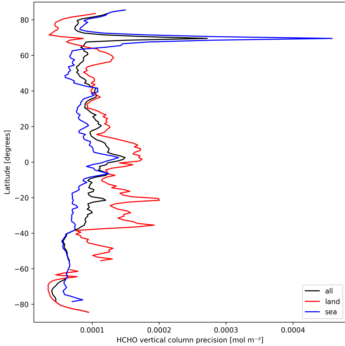
Figure 20: Zonal average of “HCHO vertical column precision” for 2025-03-22 to 2025-03-22.
