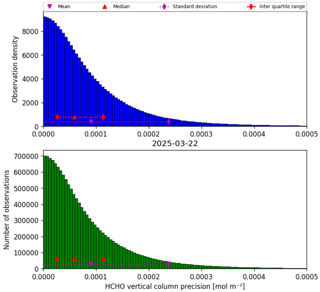
Figure 34: Histogram of “HCHO vertical column precision” for 2025-03-22 to 2025-03-22
