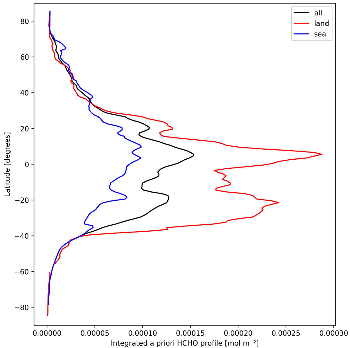
Figure 27: Zonal average of “Integrated a priori HCHO profile” for 2025-03-22 to 2025-03-22.
