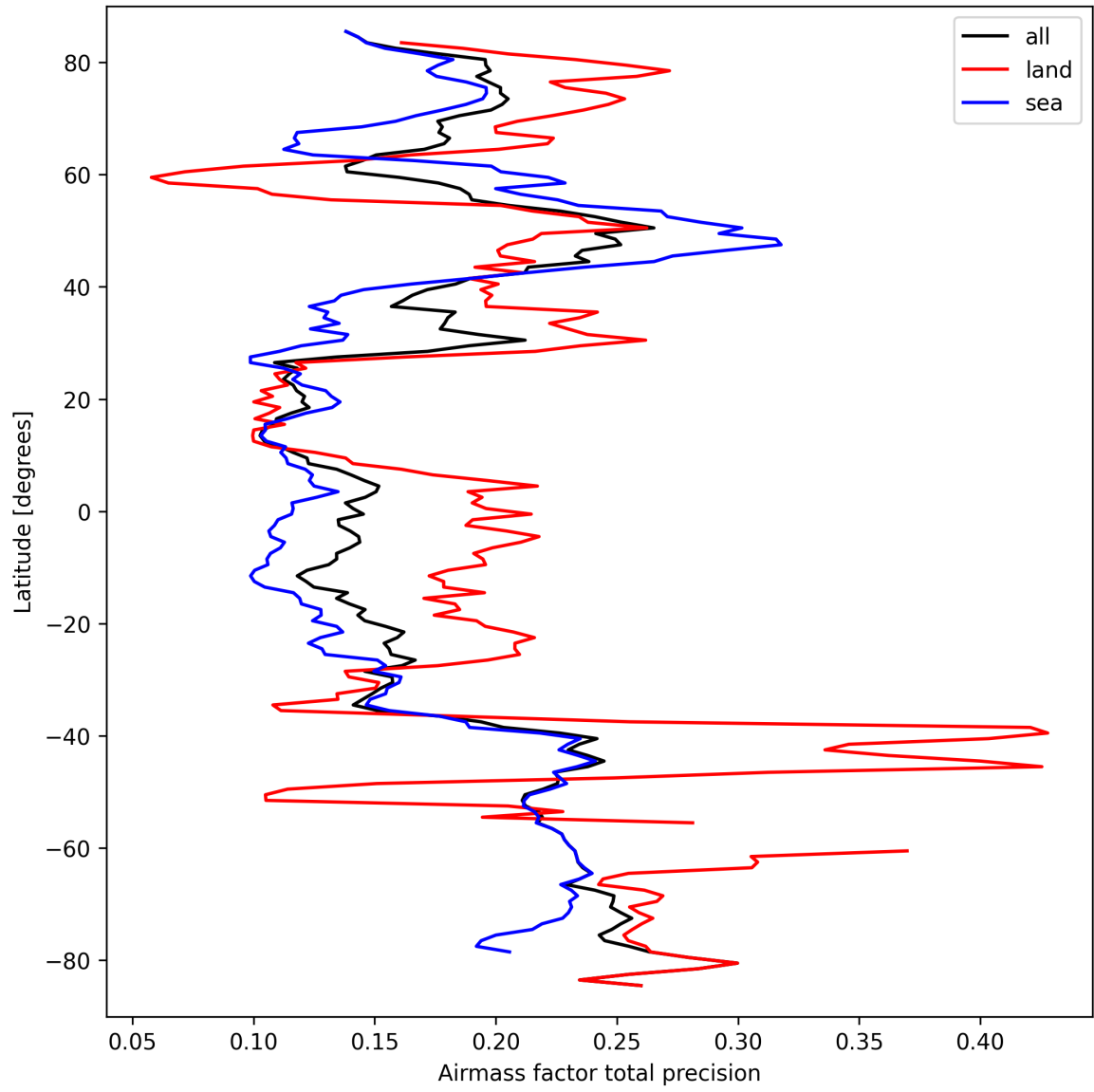
Figure 25: Zonal average of “Airmass factor total precision” for 2025-03-22 to 2025-03-22.
