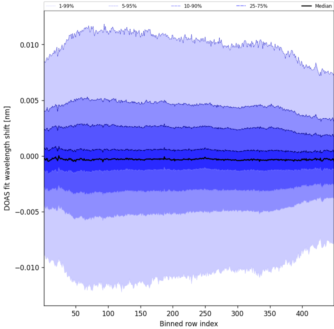
Figure 56: Along track statistics of “DOAS fit wavelength shift” for 2025-03-22 to 2025-03-22
