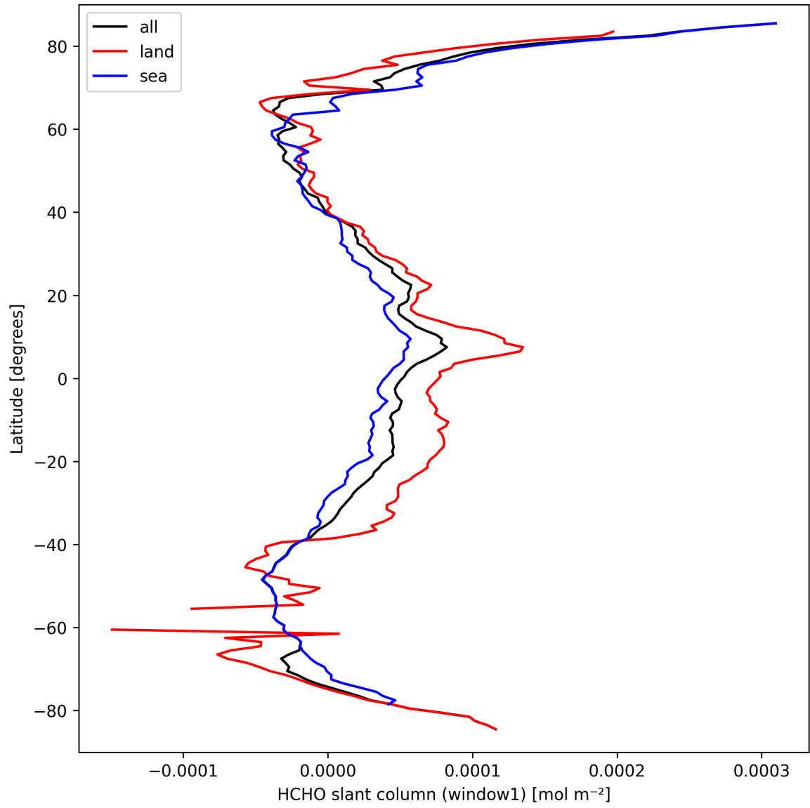
Figure 22: Zonal average of “HCHO slant column (window1)” for 2025-03-22 to 2025-03-22.
