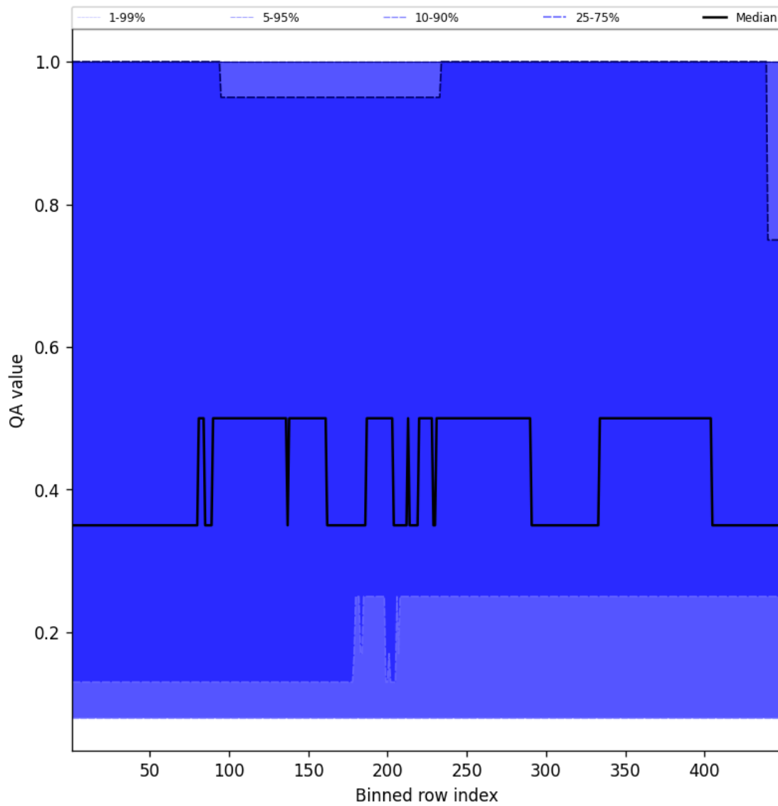
Figure 46: Along track statistics of “QA value” for 2025-03-22 to 2025-03-22
