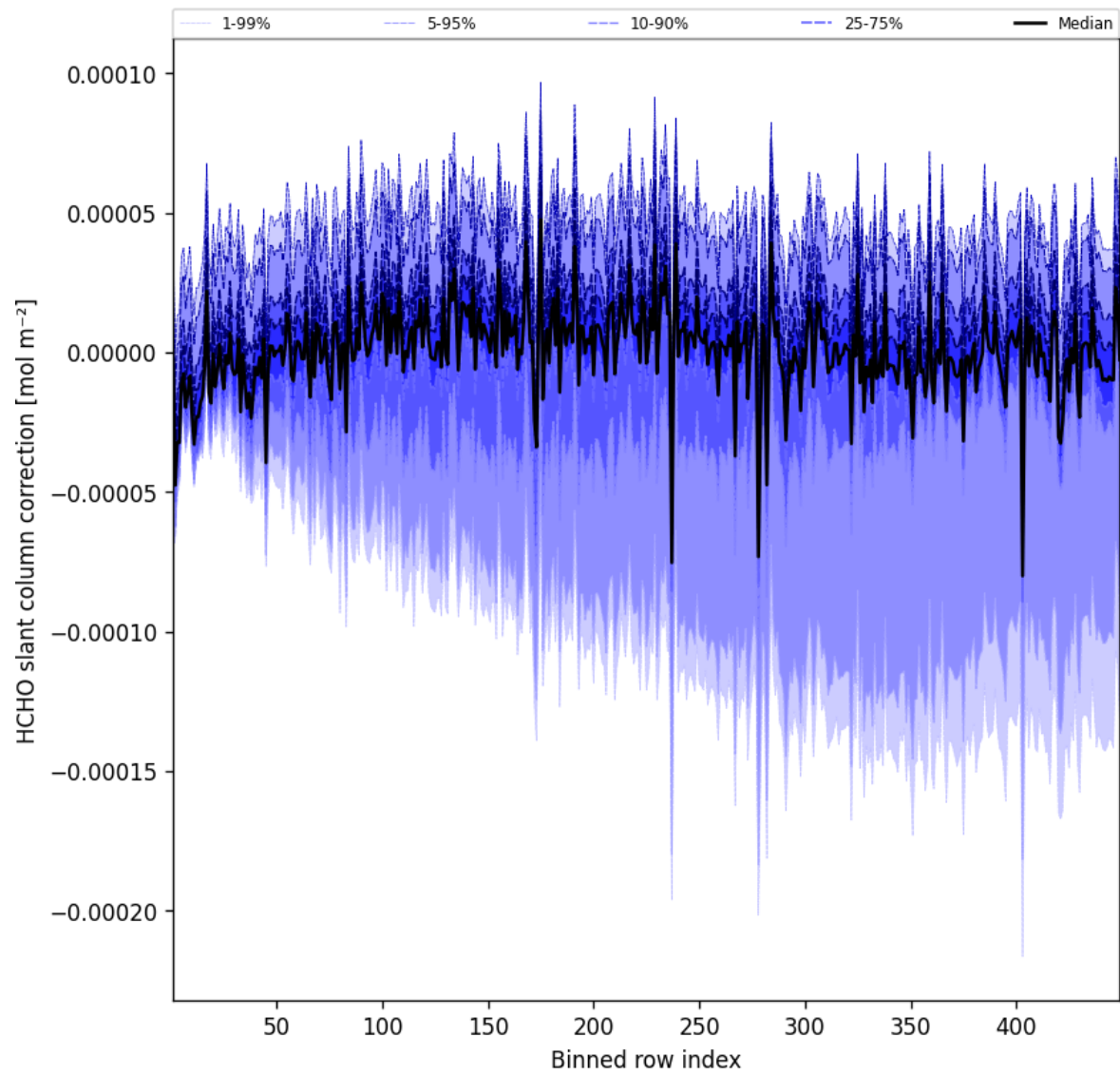
Figure 59: Along track statistics of “HCHO slant column correction” for 2025-03-22 to 2025-03-22
