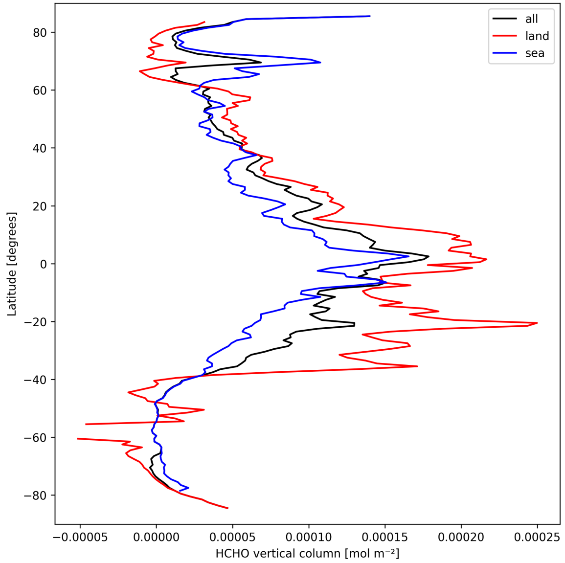
Figure 19: Zonal average of “HCHO vertical column” for 2025-03-22 to 2025-03-22.
