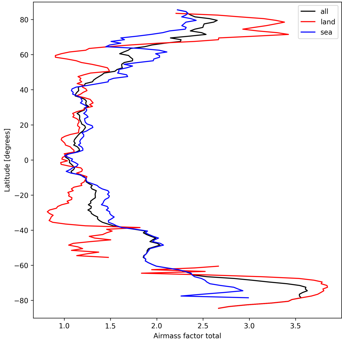
Figure 24: Zonal average of “Airmass factor total” for 2025-03-22 to 2025-03-22.
