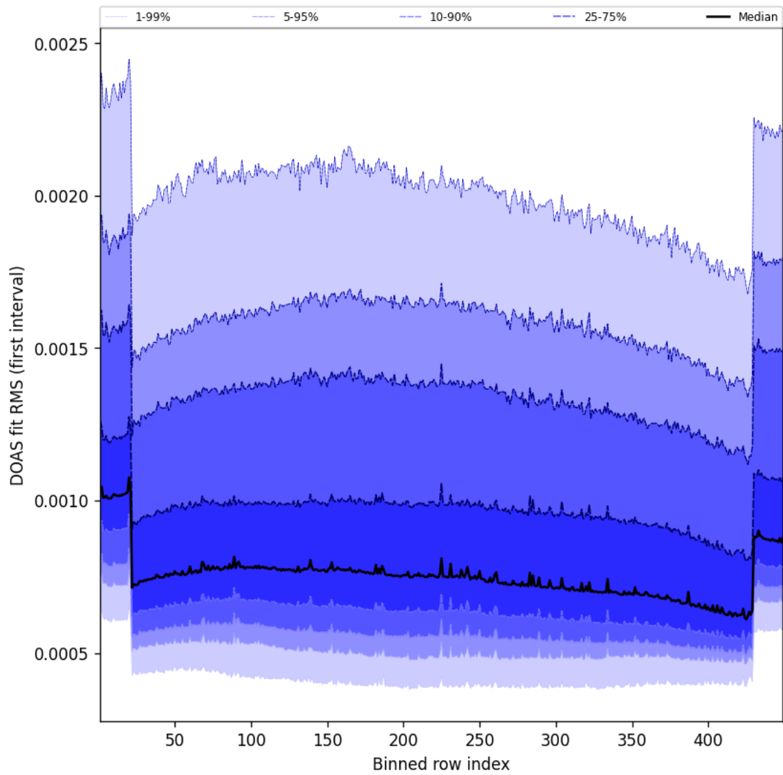
Figure 58: Along track statistics of “DOAS fit RMS (first interval)” for 2025-03-22 to 2025-03-22
