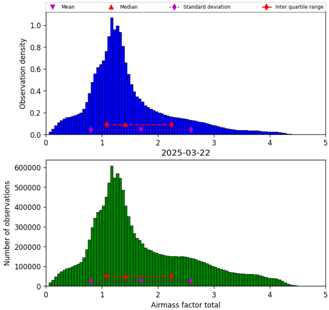
Figure 38: Histogram of “Airmass factor total” for 2025-03-22 to 2025-03-22
