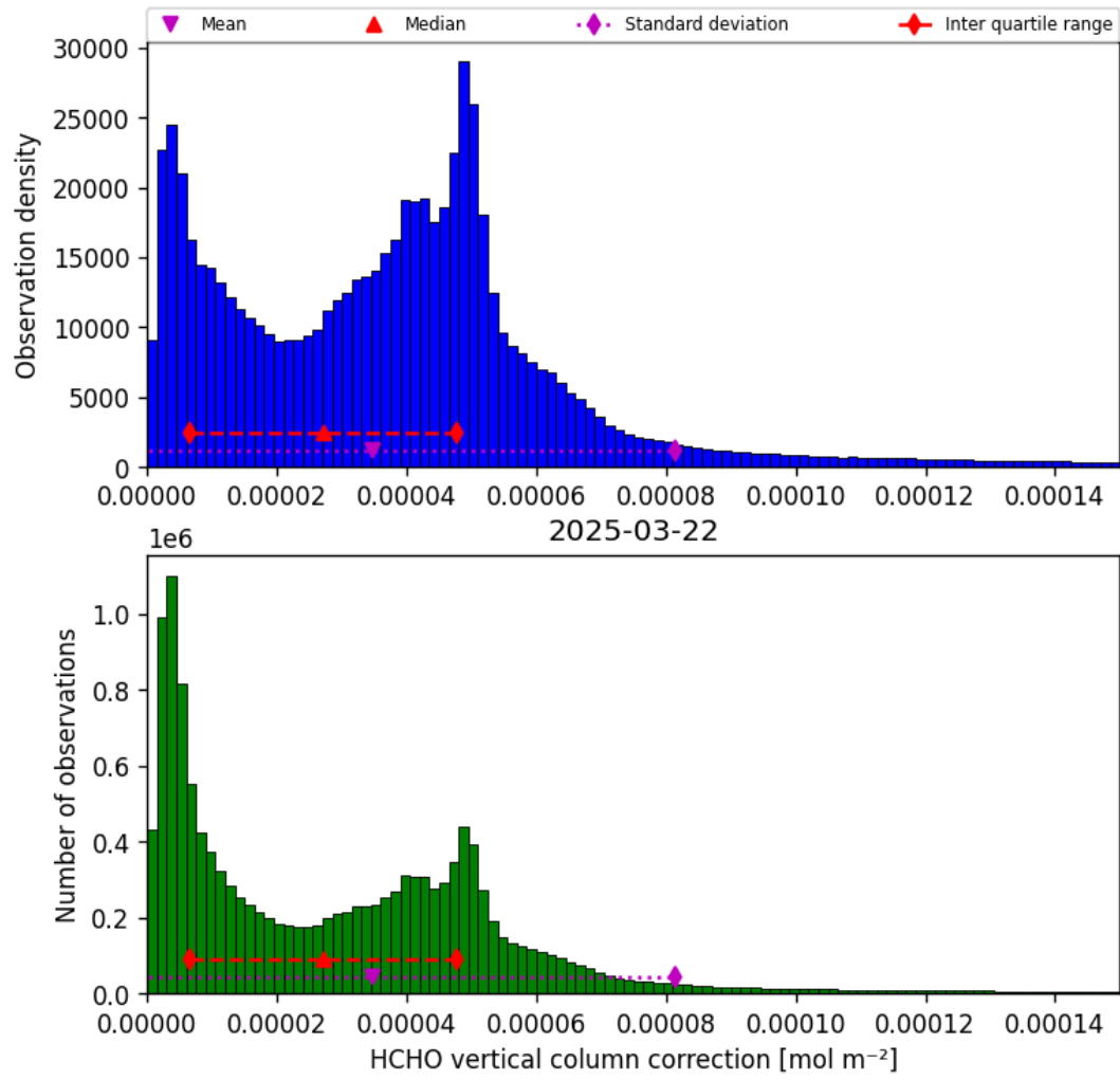
Figure 35: Histogram of “HCHO vertical column correction” for 2025-03-22 to 2025-03-22
