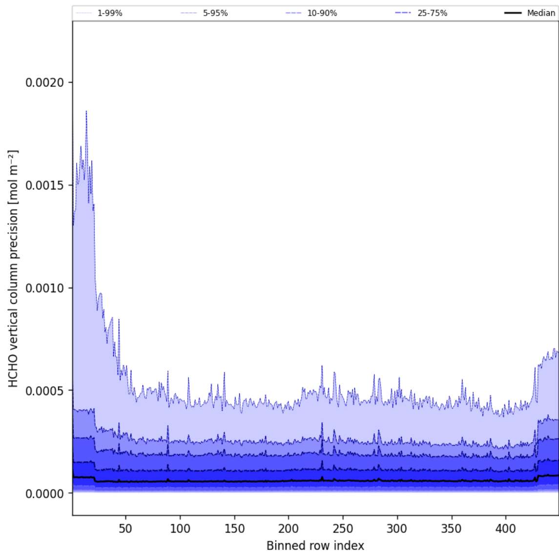
Figure 48: Along track statistics of “HCHO vertical column precision” for 2025-03-22 to 2025-03-22
