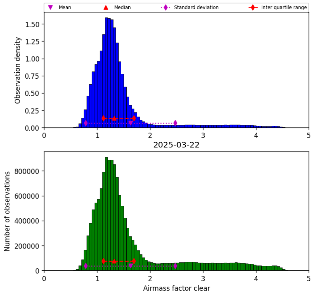
Figure 40: Histogram of “Airmass factor clear” for 2025-03-22 to 2025-03-22
