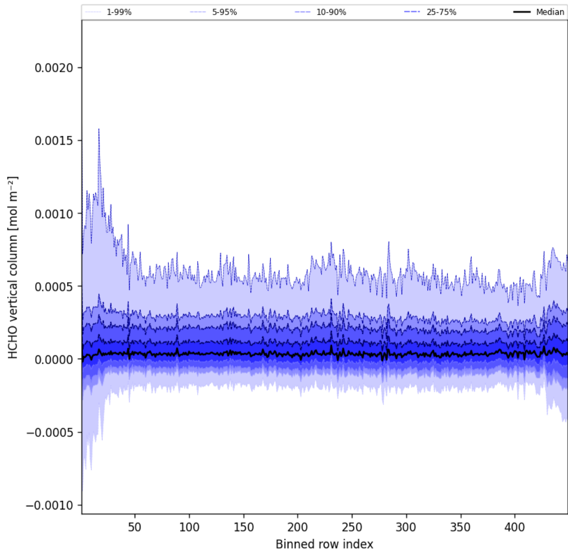
Figure 47: Along track statistics of “HCHO vertical column” for 2025-03-22 to 2025-03-22
