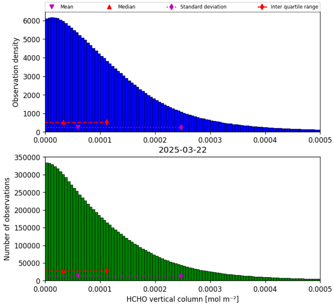
Figure 33: Histogram of “HCHO vertical column” for 2025-03-22 to 2025-03-22
