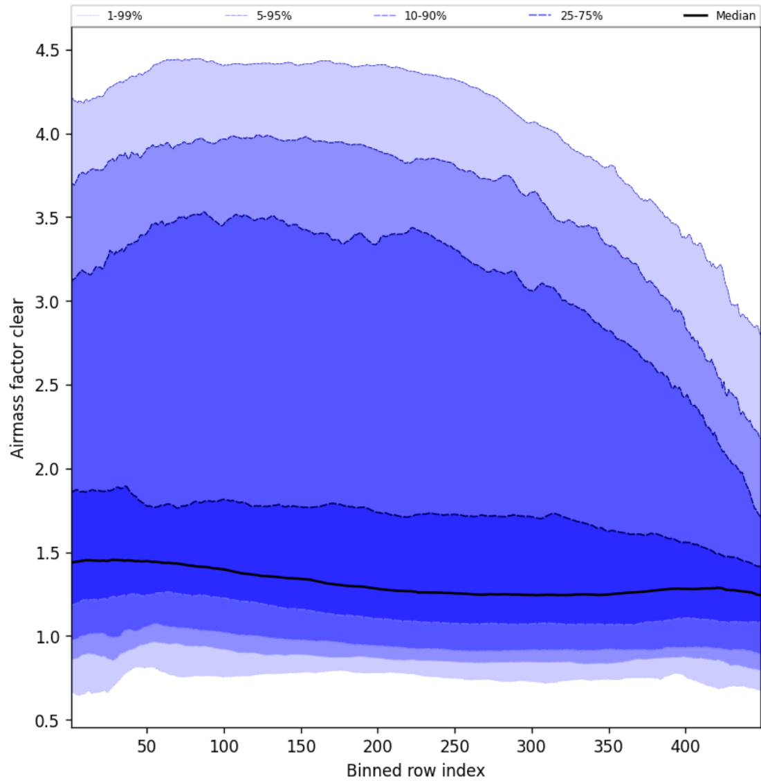
Figure 54: Along track statistics of “Airmass factor clear” for 2025-03-22 to 2025-03-22
