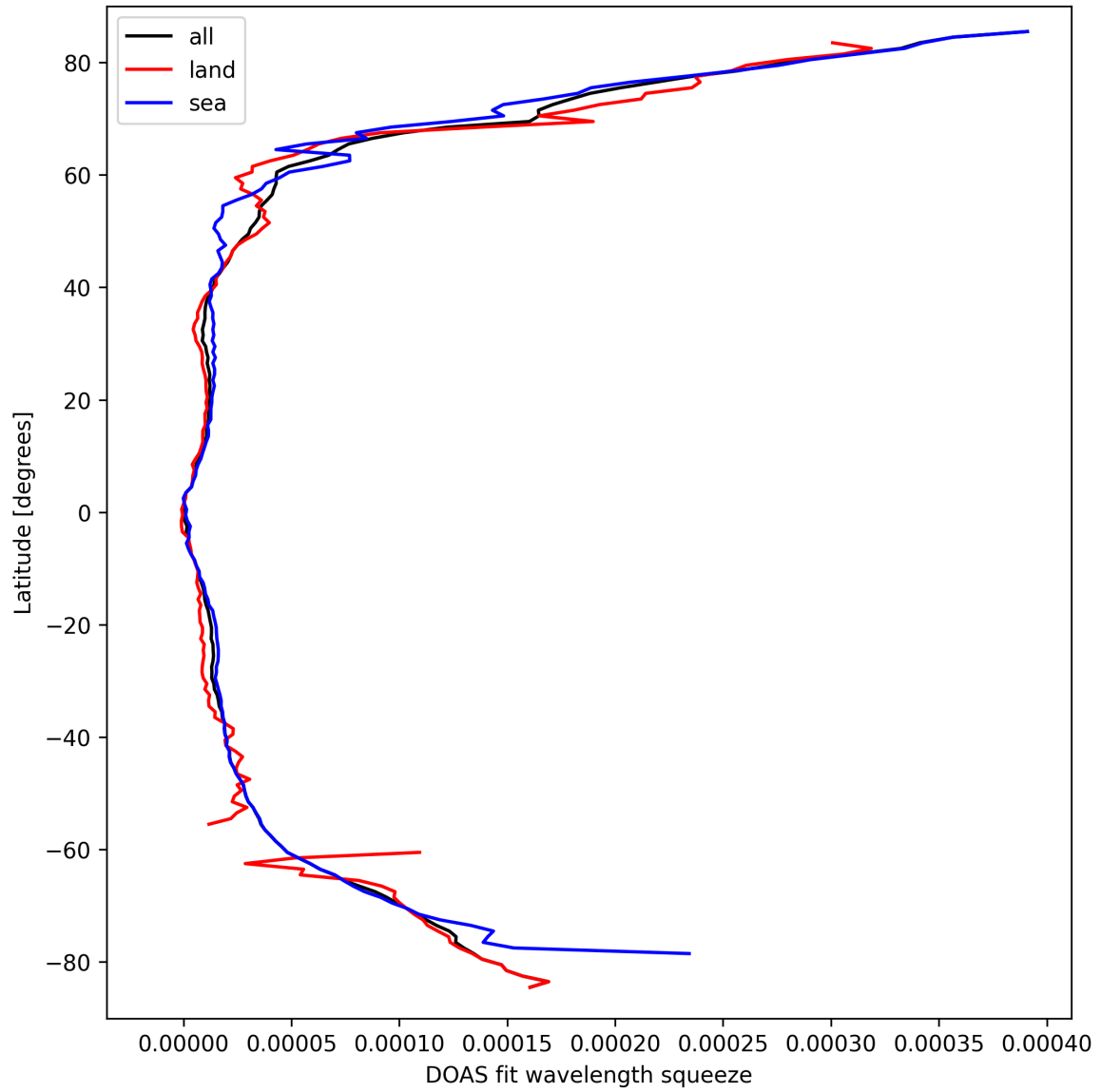
Figure 29: Zonal average of “DOAS fit wavelength squeeze” for 2025-03-22 to 2025-03-22.
