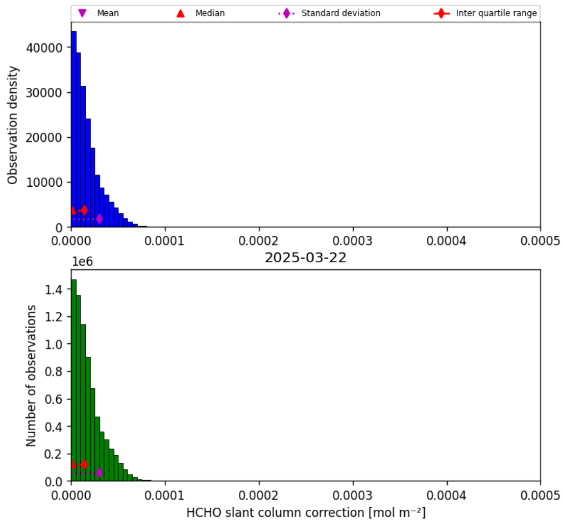
Figure 45: Histogram of “HCHO slant column correction” for 2025-03-22 to 2025-03-22
