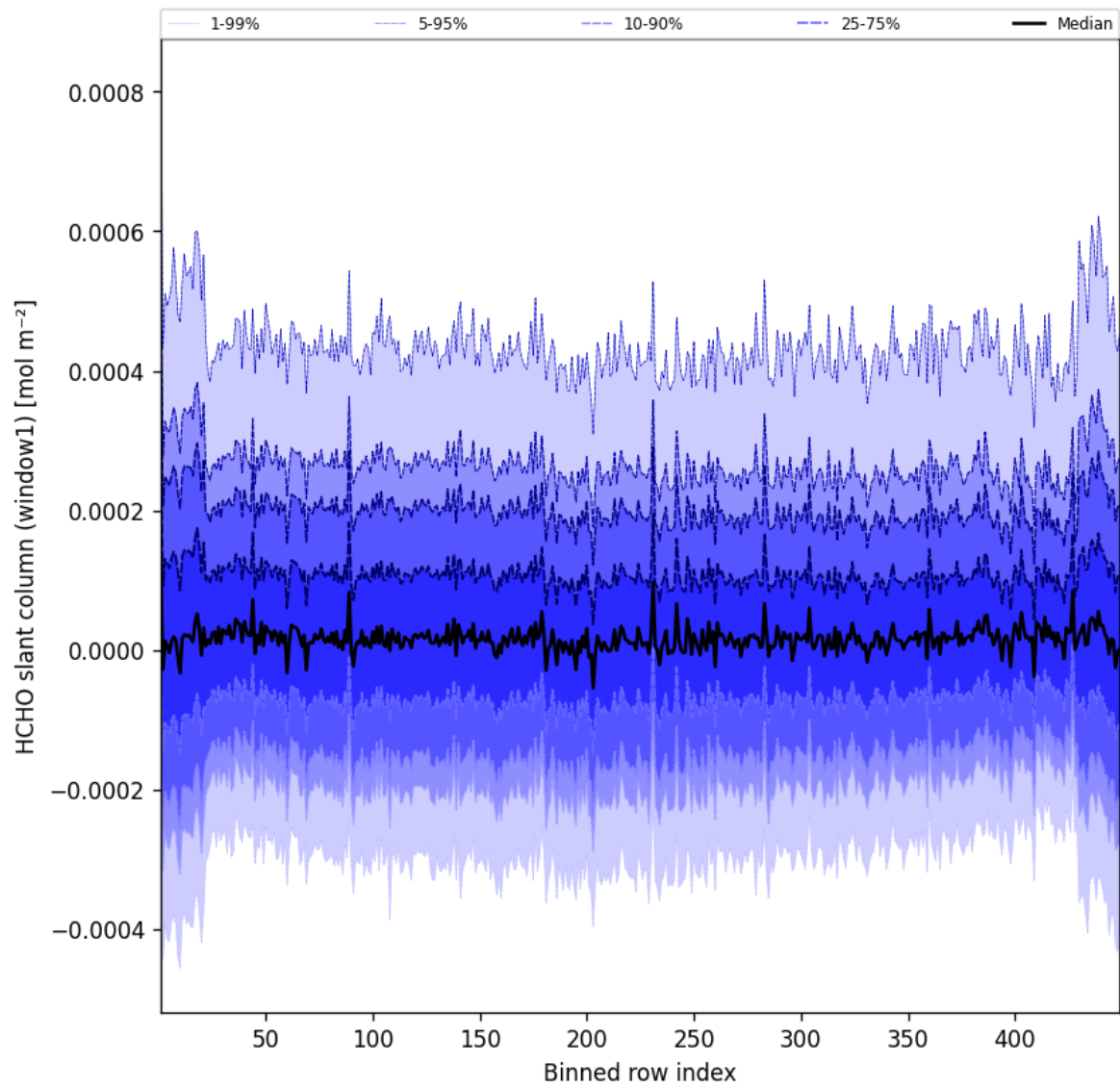
Figure 50: Along track statistics of “HCHO slant column (window1)” for 2025-03-22 to 2025-03-22
