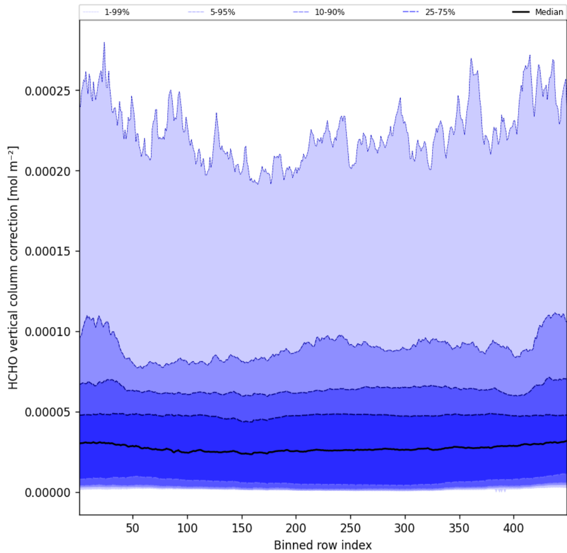
Figure 49: Along track statistics of “HCHO vertical column correction” for 2025-03-22 to 2025-03-22
