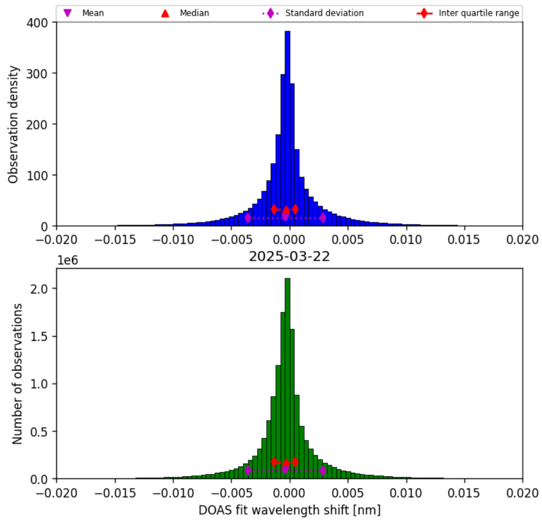
Figure 42: Histogram of “DOAS fit wavelength shift” for 2025-03-22 to 2025-03-22
