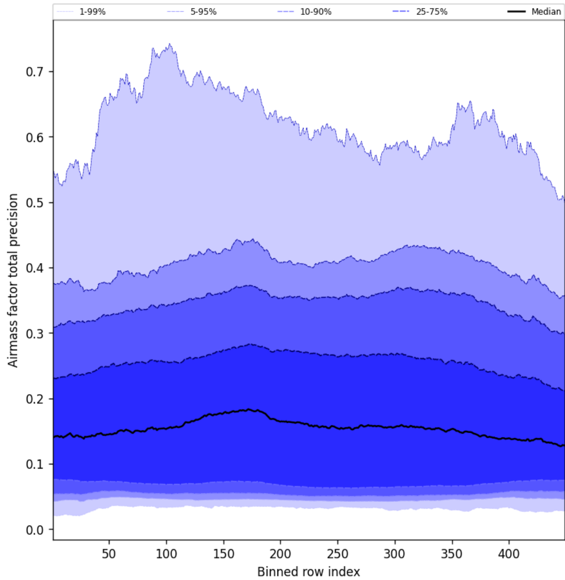
Figure 53: Along track statistics of “Airmass factor total precision” for 2025-03-22 to 2025-03-22
