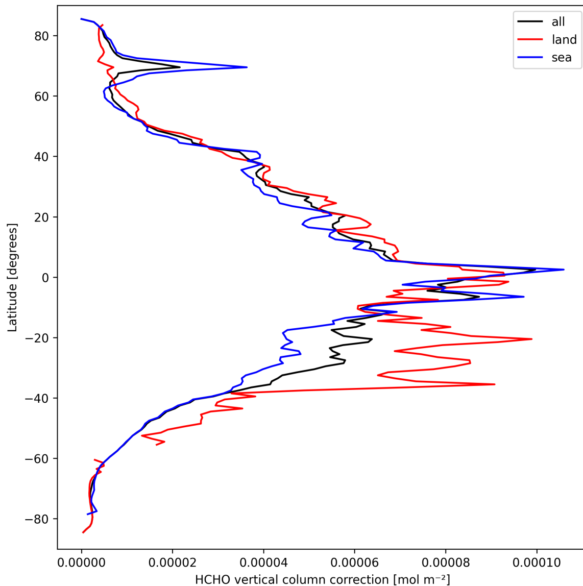
Figure 21: Zonal average of “HCHO vertical column correction” for 2025-03-22 to 2025-03-22.
