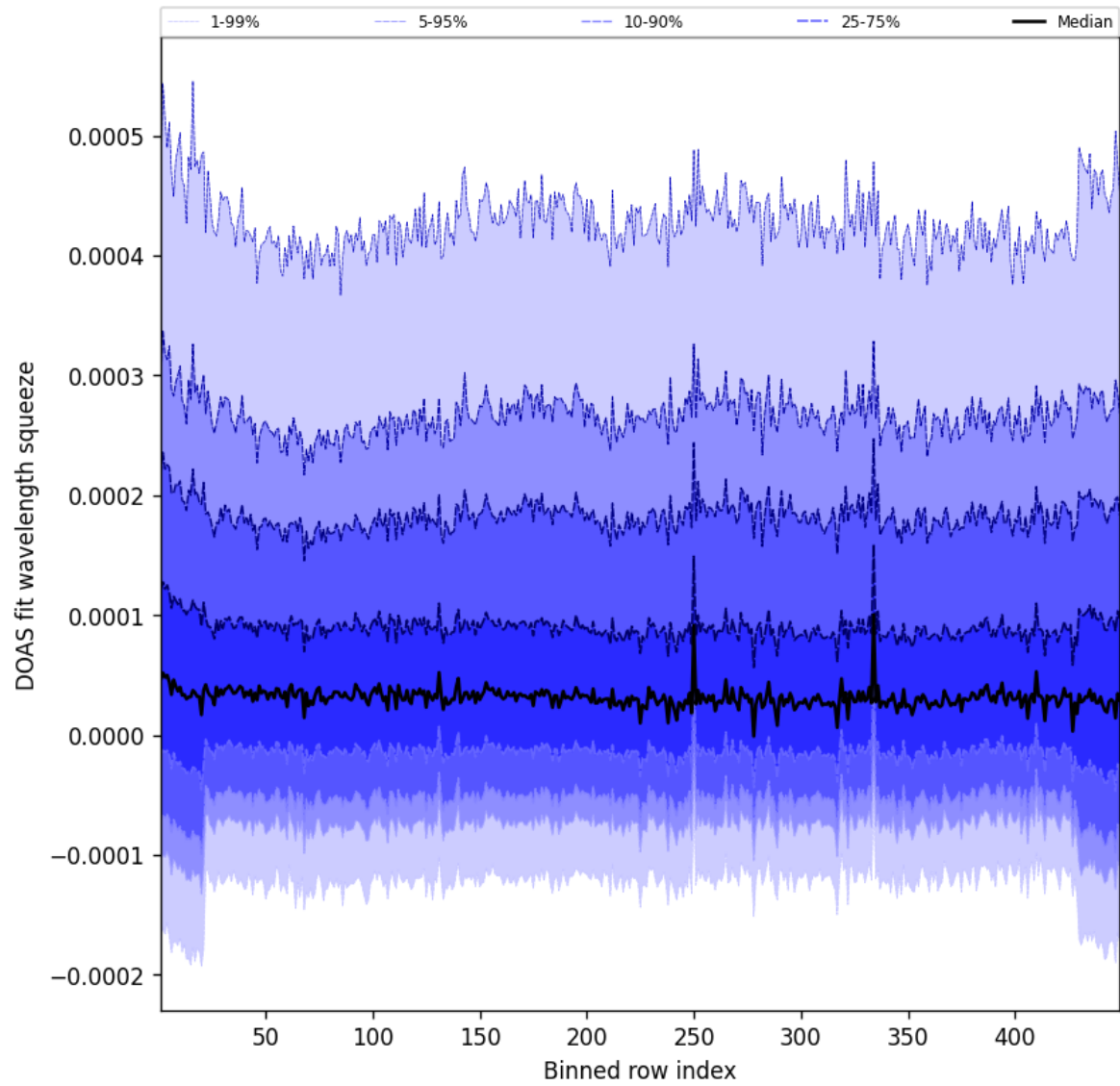
Figure 57: Along track statistics of “DOAS fit wavelength squeeze” for 2025-03-22 to 2025-03-22
