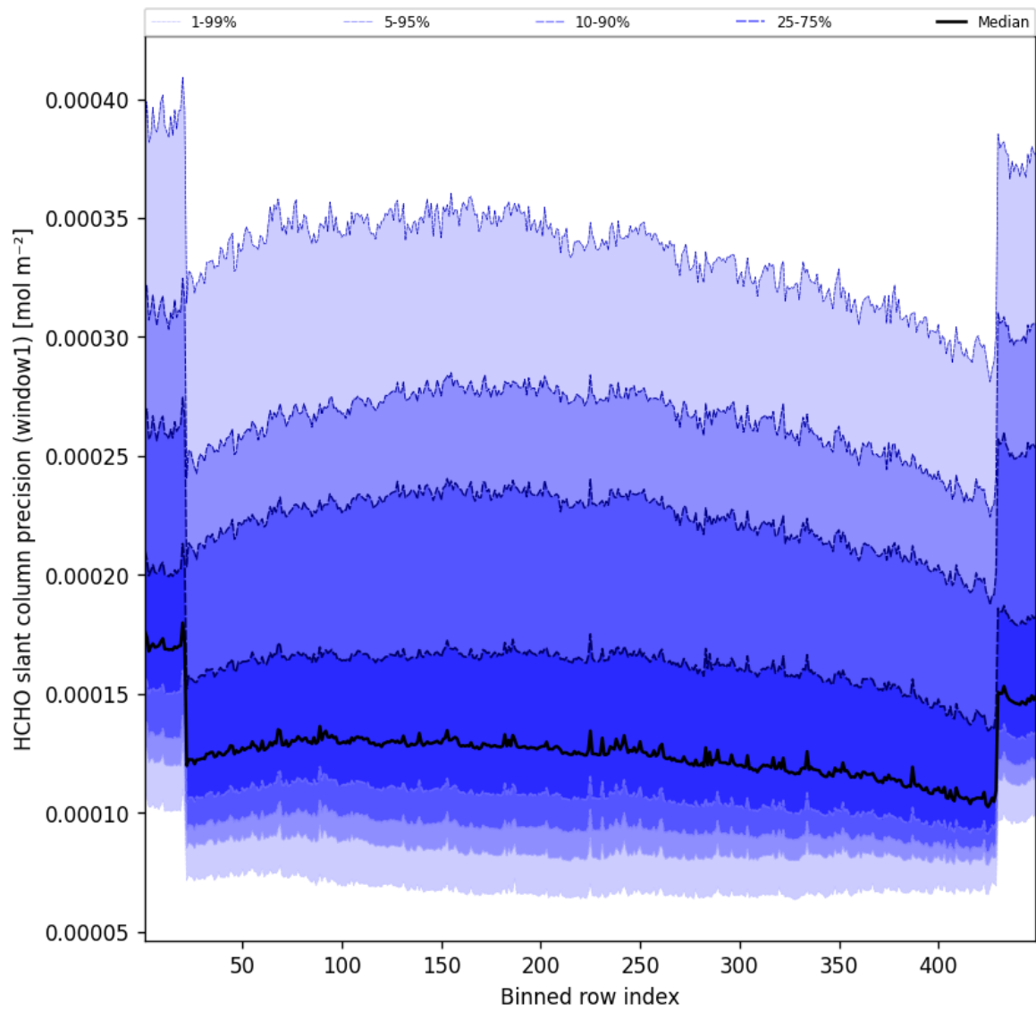
Figure 51: Along track statistics of “HCHO slant column precision (window1)” for 2025-03-22 to 2025-03-22
