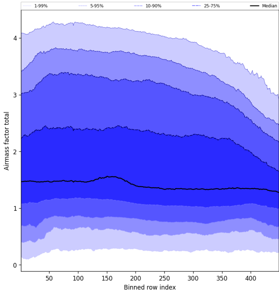
Figure 52: Along track statistics of “Airmass factor total” for 2025-03-22 to 2025-03-22
