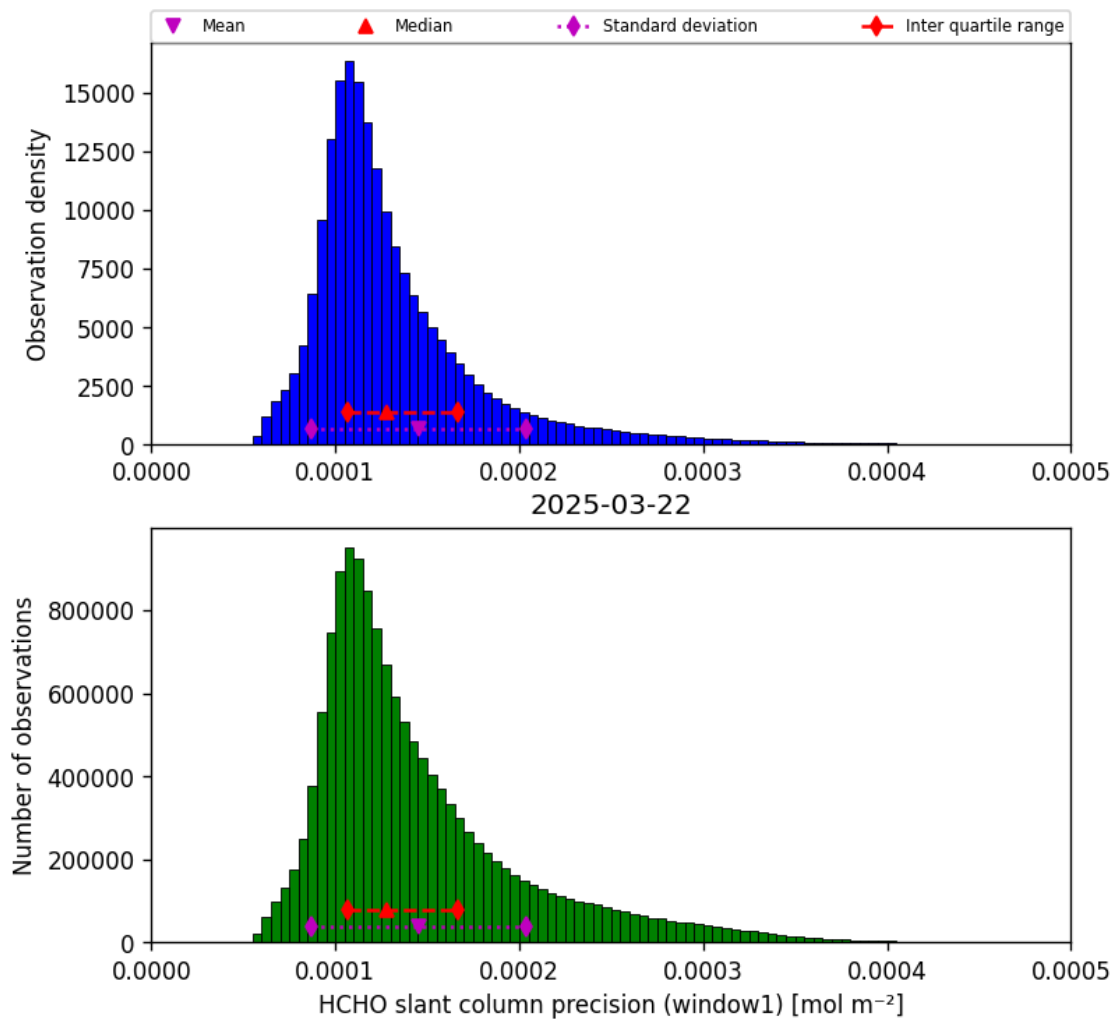
Figure 37: Histogram of “HCHO slant column precision (window1)” for 2025-03-22 to 2025-03-22
