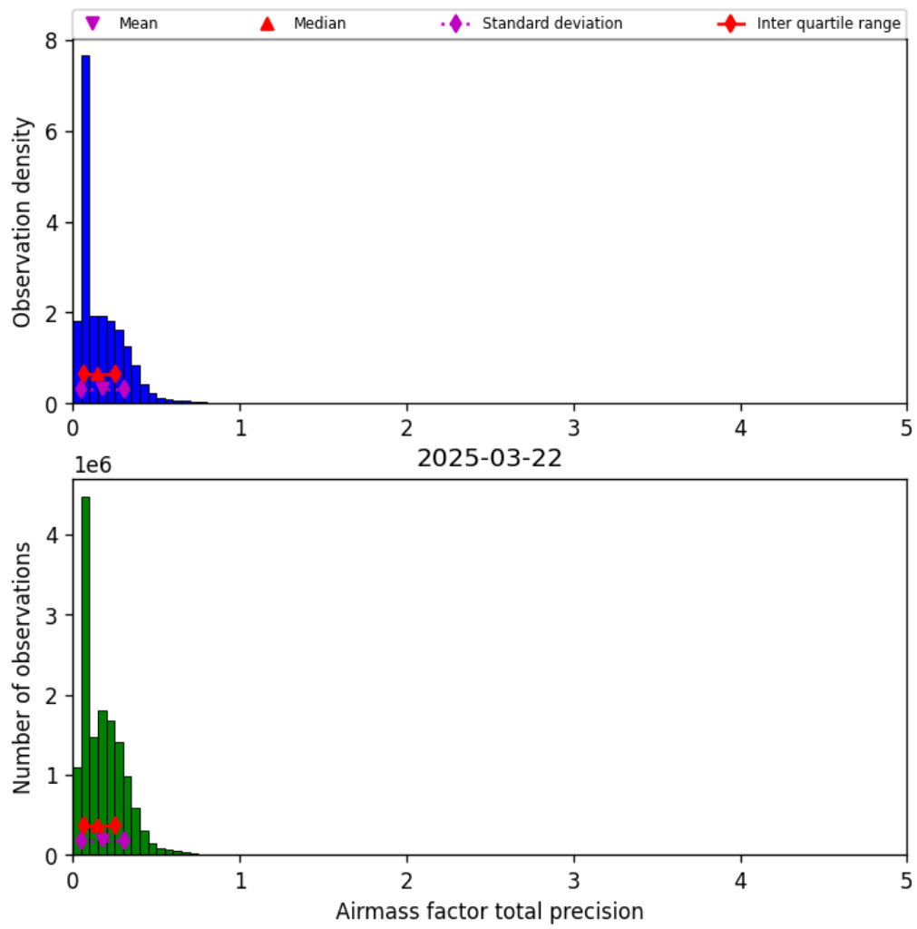
Figure 39: Histogram of “Airmass factor total precision” for 2025-03-22 to 2025-03-22
