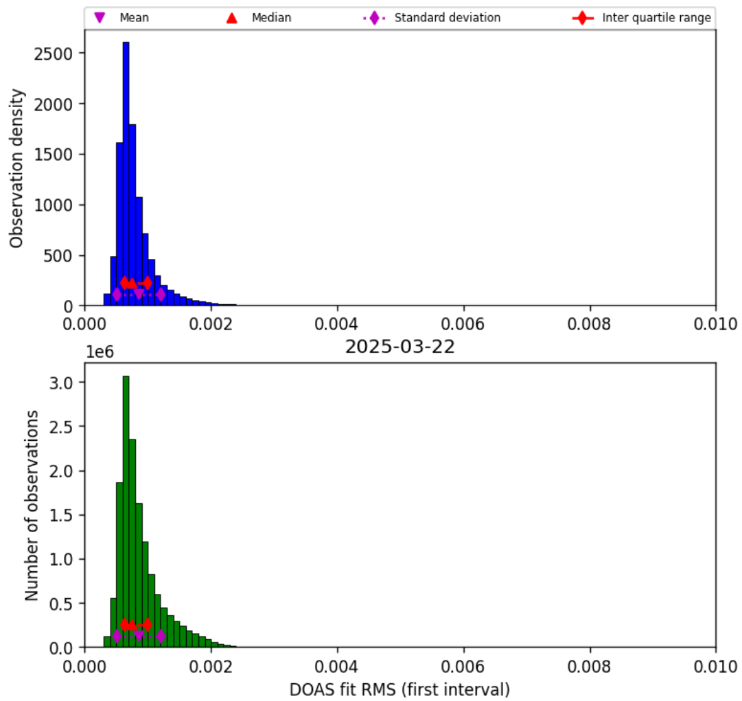
Figure 44: Histogram of “DOAS fit RMS (first interval)” for 2025-03-22 to 2025-03-22
