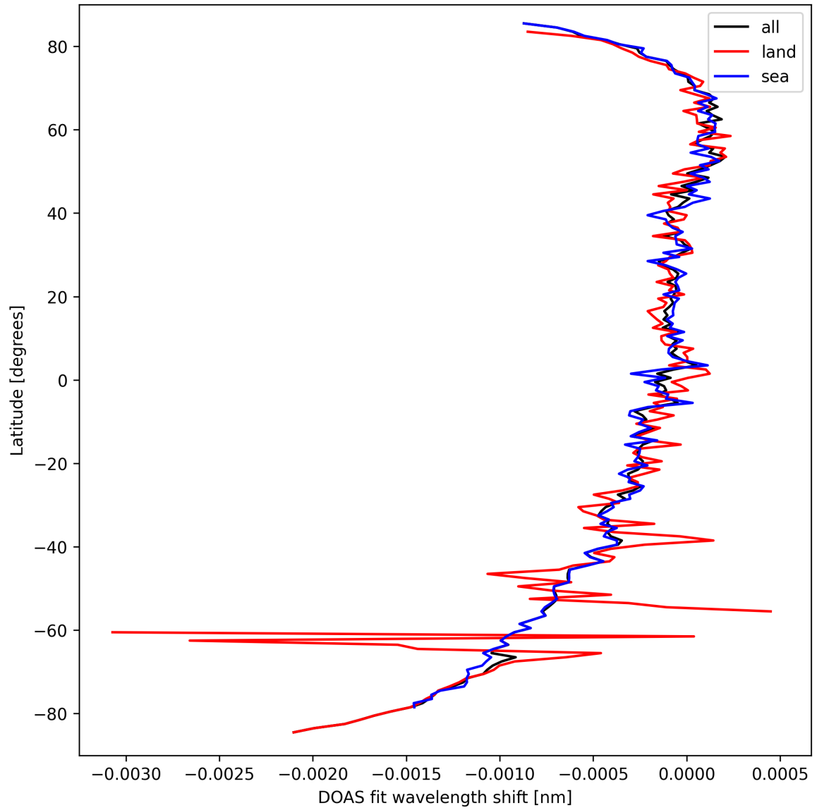
Figure 28: Zonal average of “DOAS fit wavelength shift” for 2025-03-22 to 2025-03-22.
