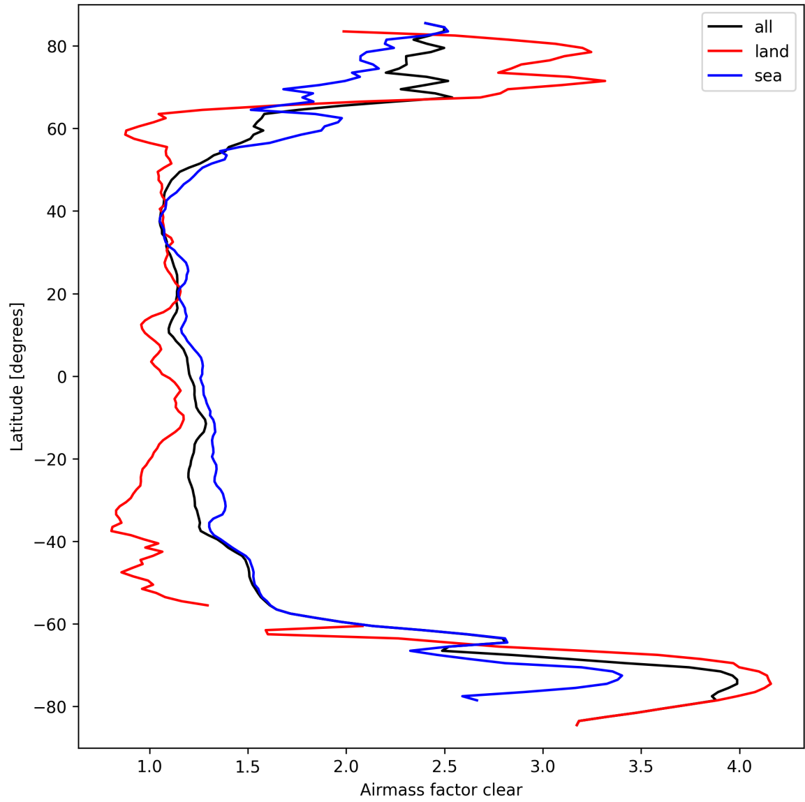
Figure 26: Zonal average of “Airmass factor clear” for 2025-03-22 to 2025-03-22.
