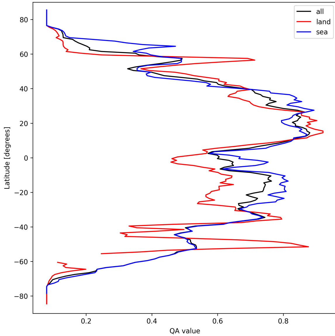
Figure 18: Zonal average of “QA value” for 2025-03-22 to 2025-03-22.
