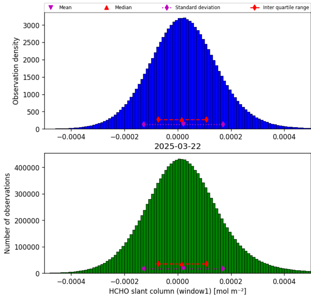
Figure 36: Histogram of “HCHO slant column (window1)” for 2025-03-22 to 2025-03-22
