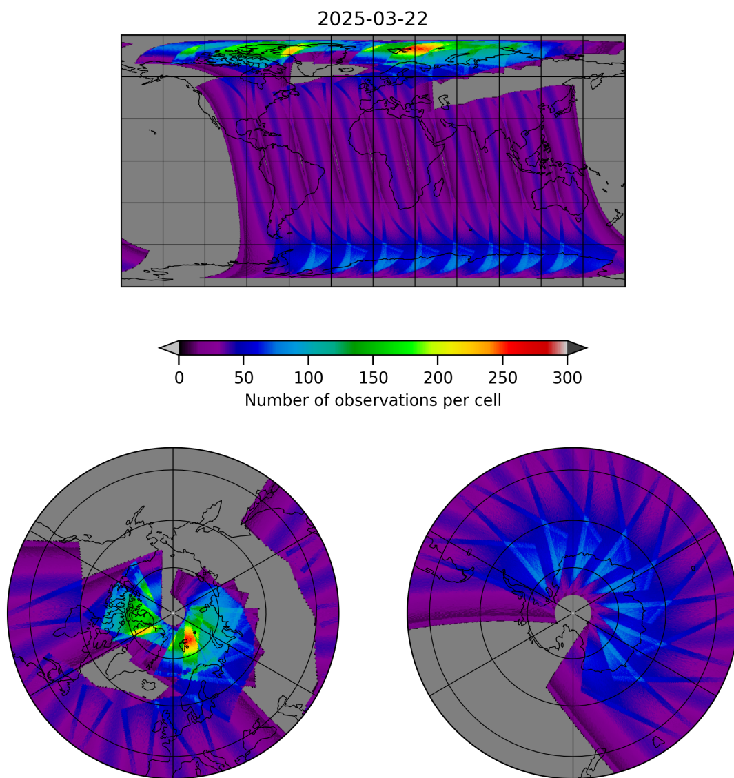
Figure 17: Map of the number of observations for 2025-03-22 to 2025-03-22
