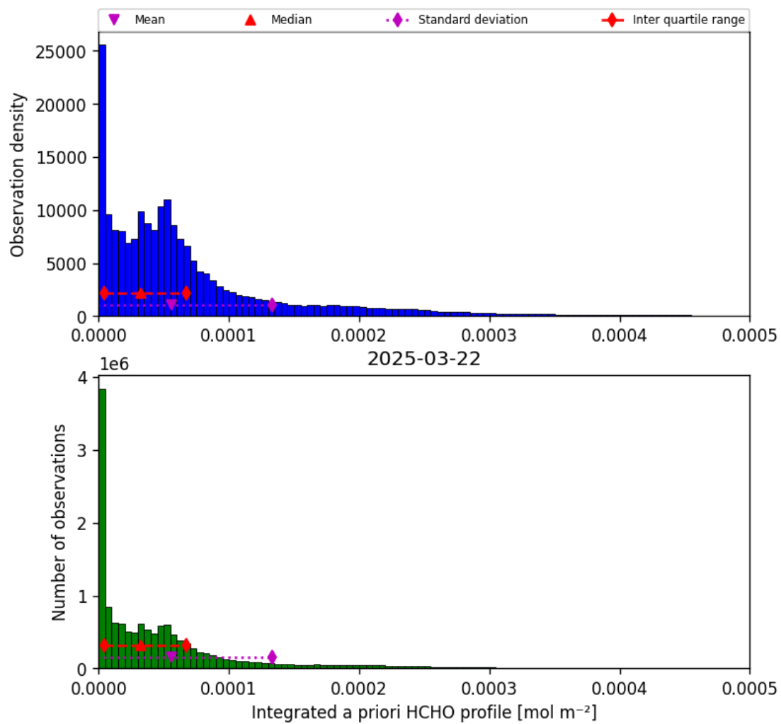
Figure 41: Histogram of "Integrated a priori HCHO profile" for 2025-03-22 to 2025-03-22
