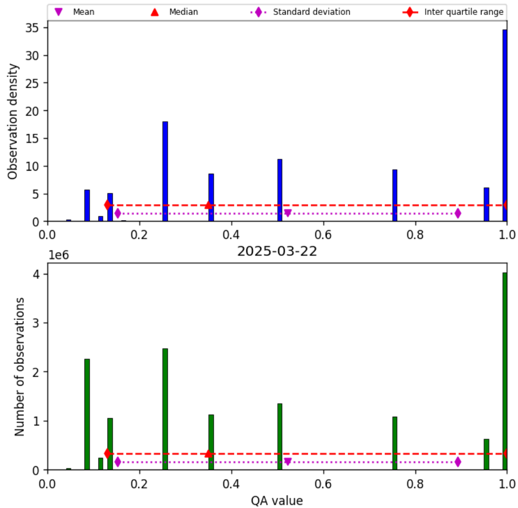
Figure 32: Histogram of “QA value” for 2025-03-22 to 2025-03-22
