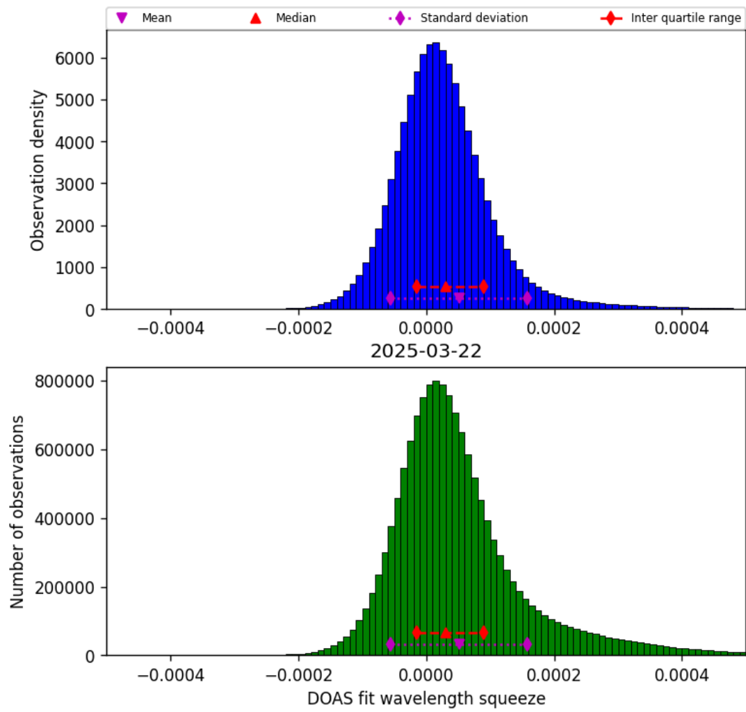
Figure 43: Histogram of “DOAS fit wavelength squeeze” for 2025-03-22 to 2025-03-22
