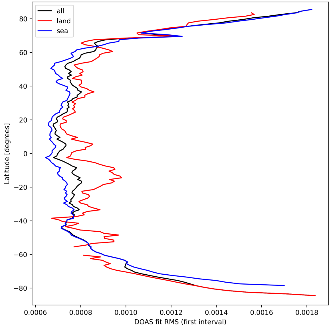
Figure 30: Zonal average of “DOAS fit RMS (first interval)” for 2025-03-22 to 2025-03-22.
