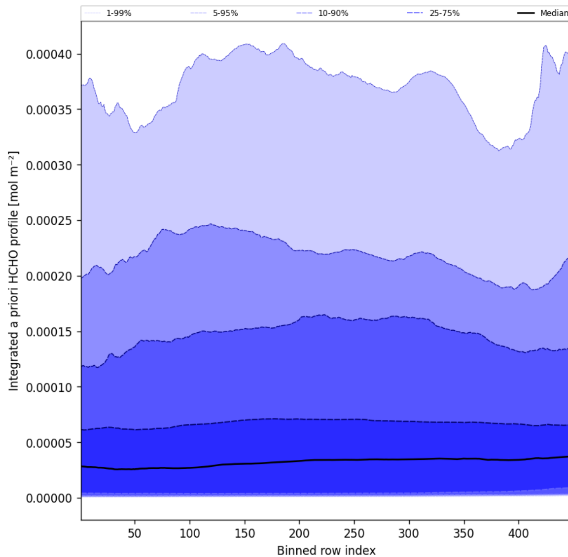
Figure 55: Along track statistics of “Integrated a priori HCHO profile” for 2025-03-22 to 2025-03-22
