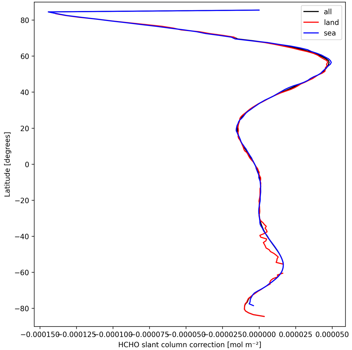
Figure 31: Zonal average of “HCHO slant column correction” for 2025-03-22 to 2025-03-22.
