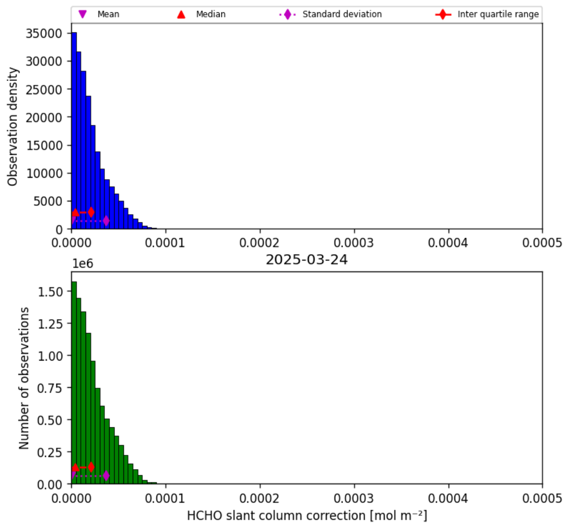
Figure 45: Histogram of “HCHO slant column correction” for 2025-03-24 to 2025-03-25
