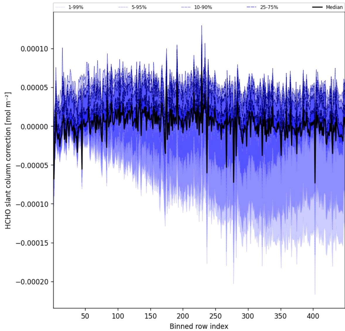
Figure 59: Along track statistics of “HCHO slant column correction” for 2025-03-24 to 2025-03-25
