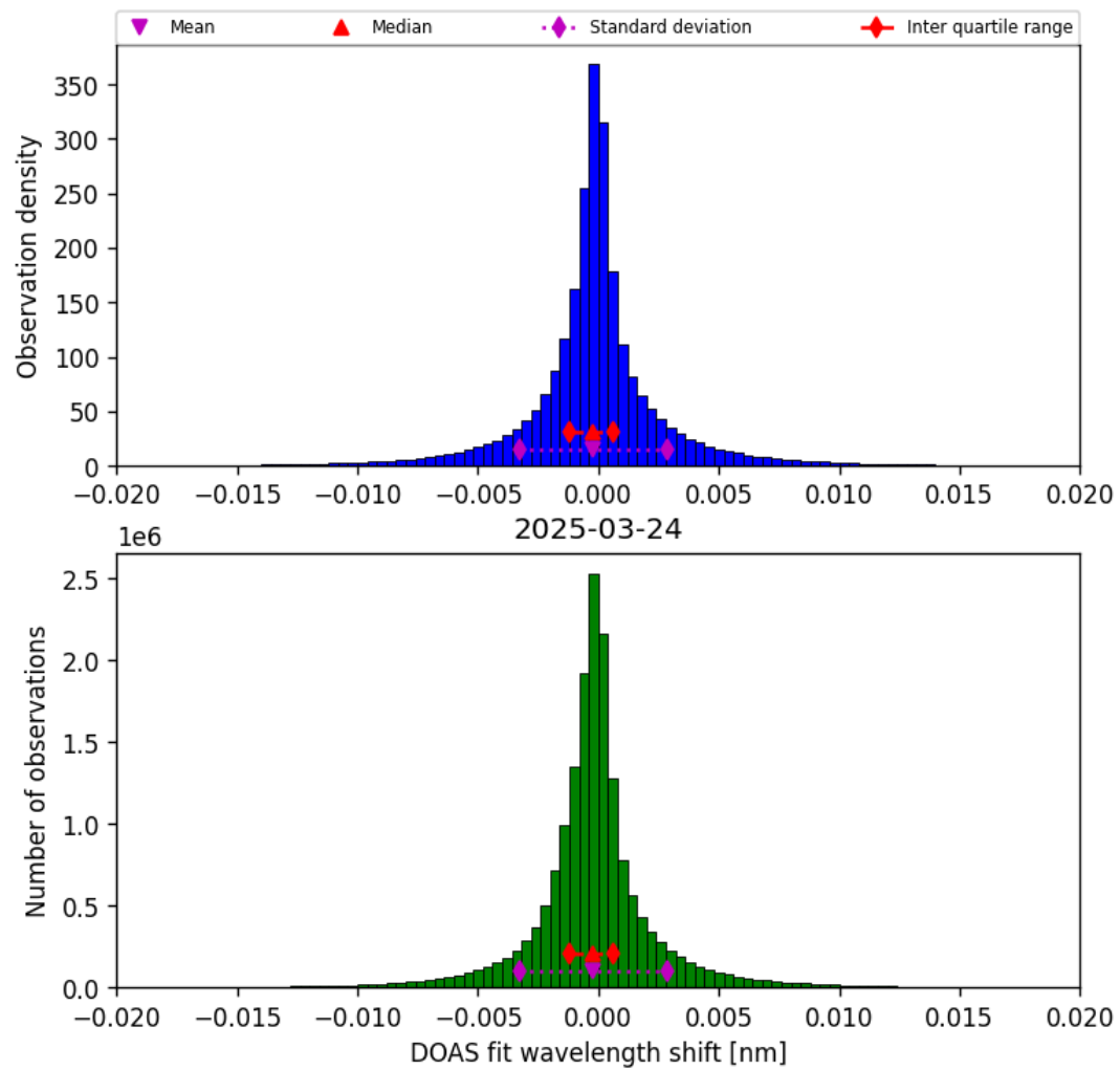
Figure 42: Histogram of “DOAS fit wavelength shift” for 2025-03-24 to 2025-03-25
