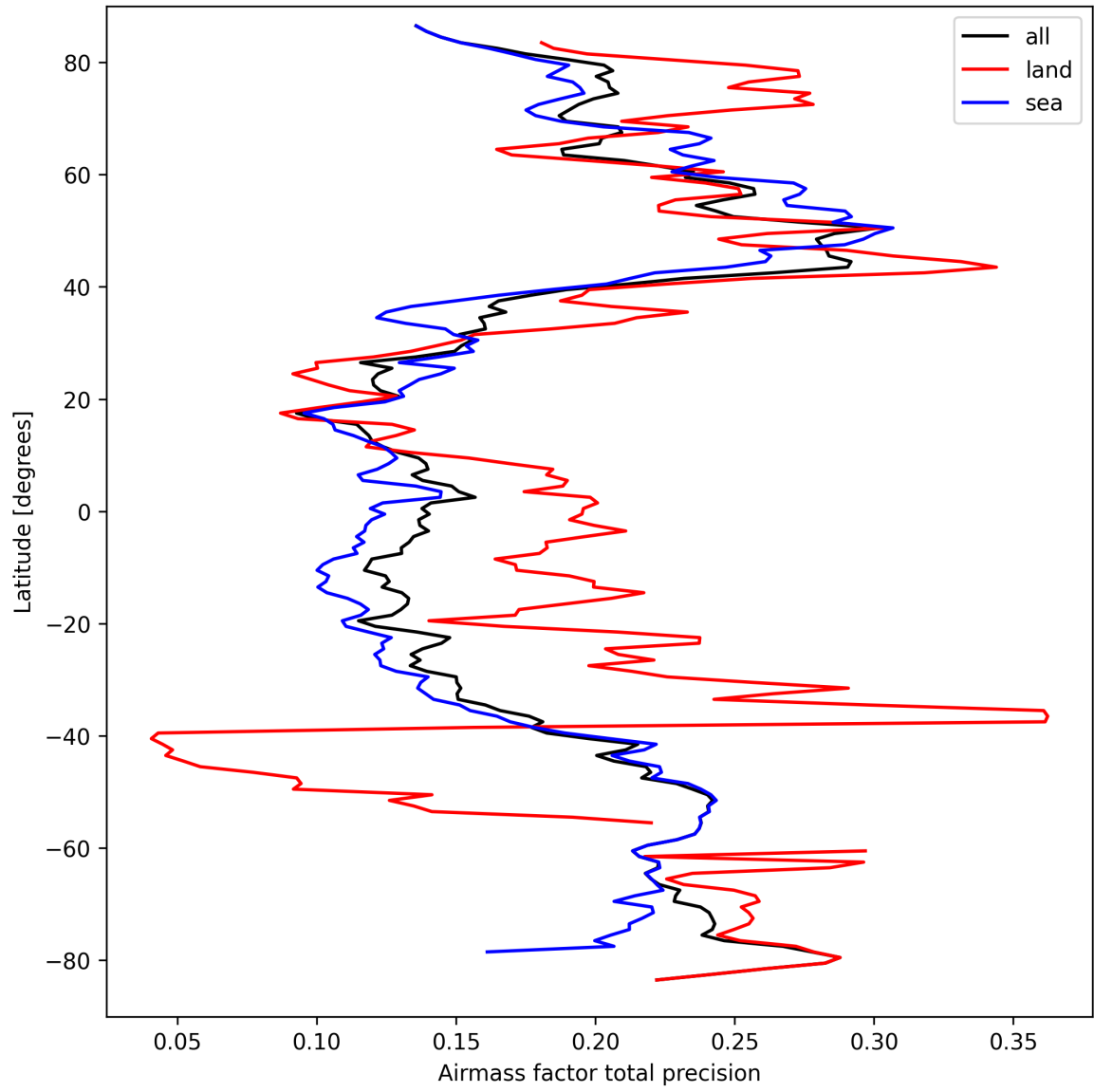
Figure 25: Zonal average of “Airmass factor total precision” for 2025-03-24 to 2025-03-25.
