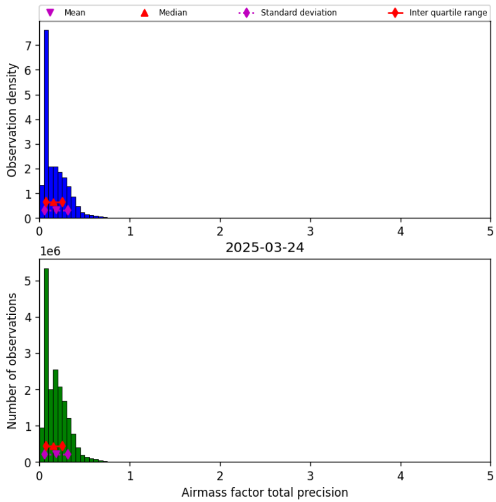
Figure 39: Histogram of “Airmass factor total precision” for 2025-03-24 to 2025-03-25
