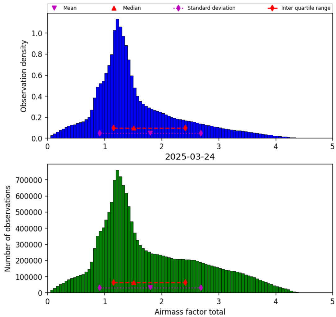
Figure 38: Histogram of “Airmass factor total” for 2025-03-24 to 2025-03-25
