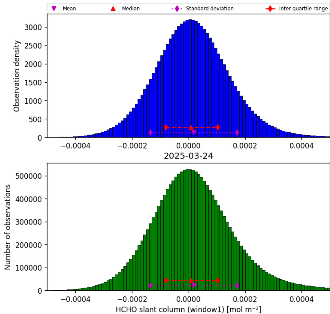
Figure 36: Histogram of “HCHO slant column (window1)” for 2025-03-24 to 2025-03-25
