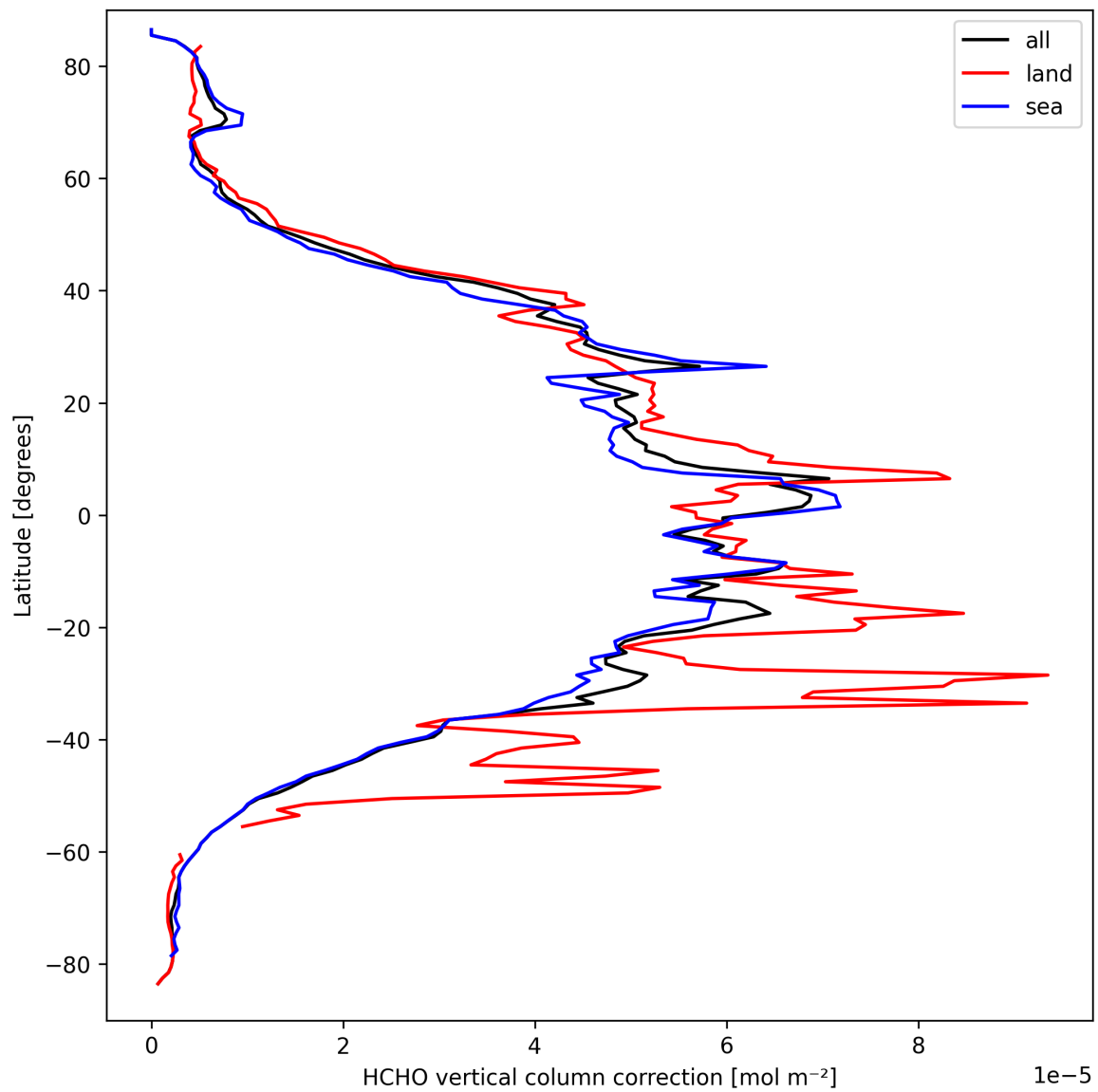
Figure 21: Zonal average of “HCHO vertical column correction” for 2025-03-24 to 2025-03-25.
