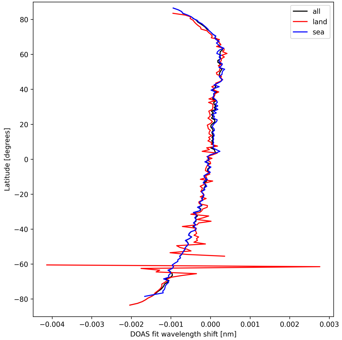
Figure 28: Zonal average of “DOAS fit wavelength shift” for 2025-03-24 to 2025-03-25.
