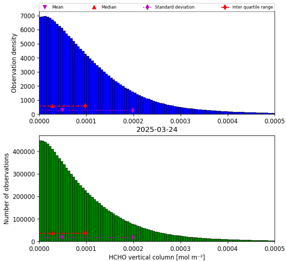
Figure 33: Histogram of “HCHO vertical column” for 2025-03-24 to 2025-03-25
