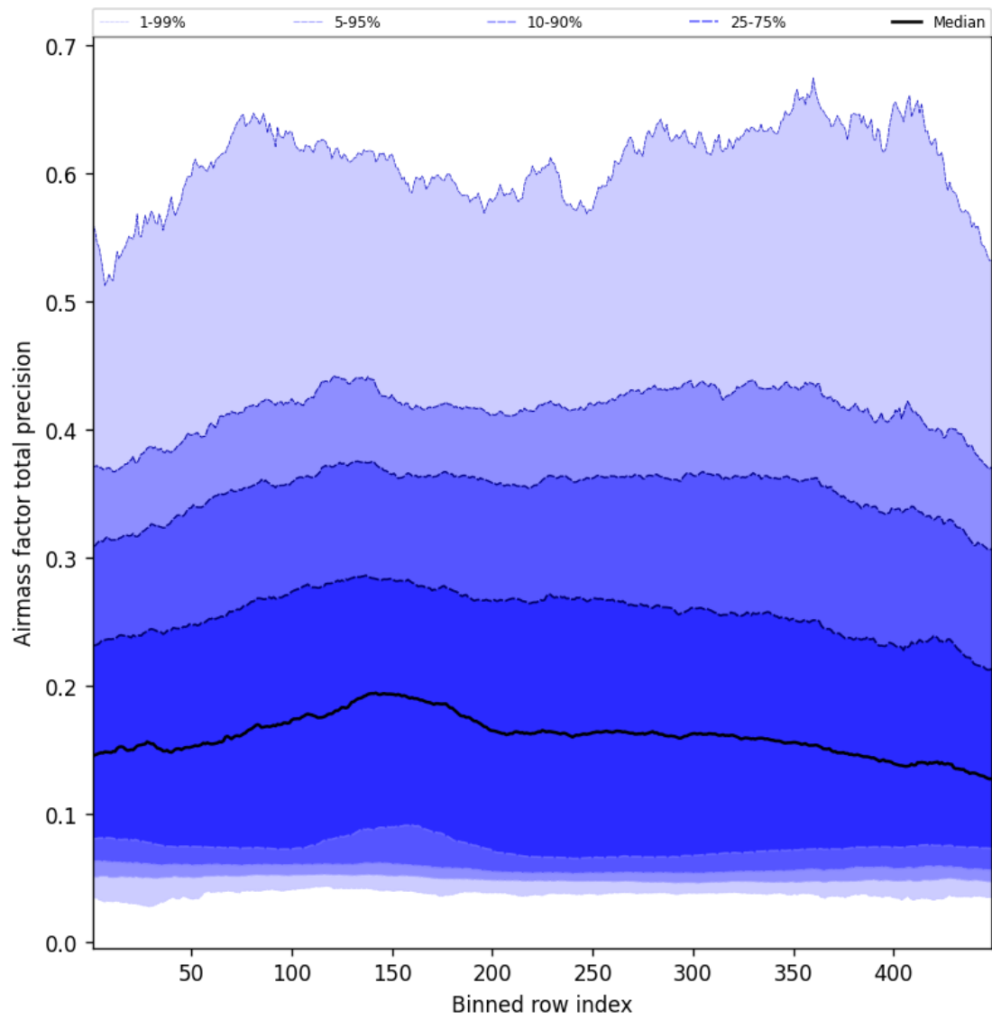
Figure 53: Along track statistics of “Airmass factor total precision” for 2025-03-24 to 2025-03-25
