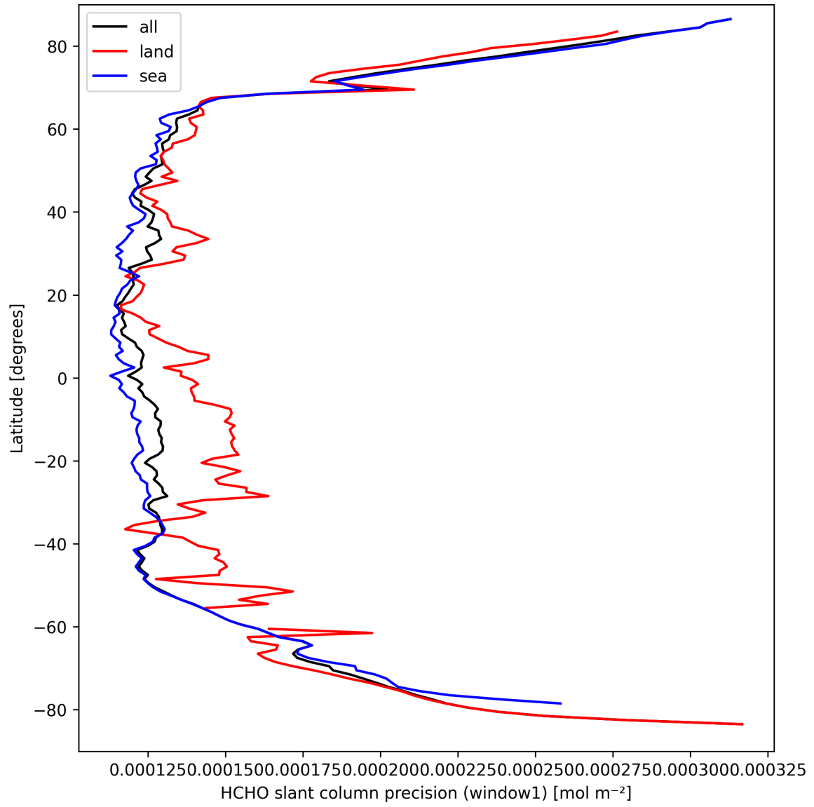
Figure 23: Zonal average of “HCHO slant column precision (window1)” for 2025-03-24 to 2025-03-25.
