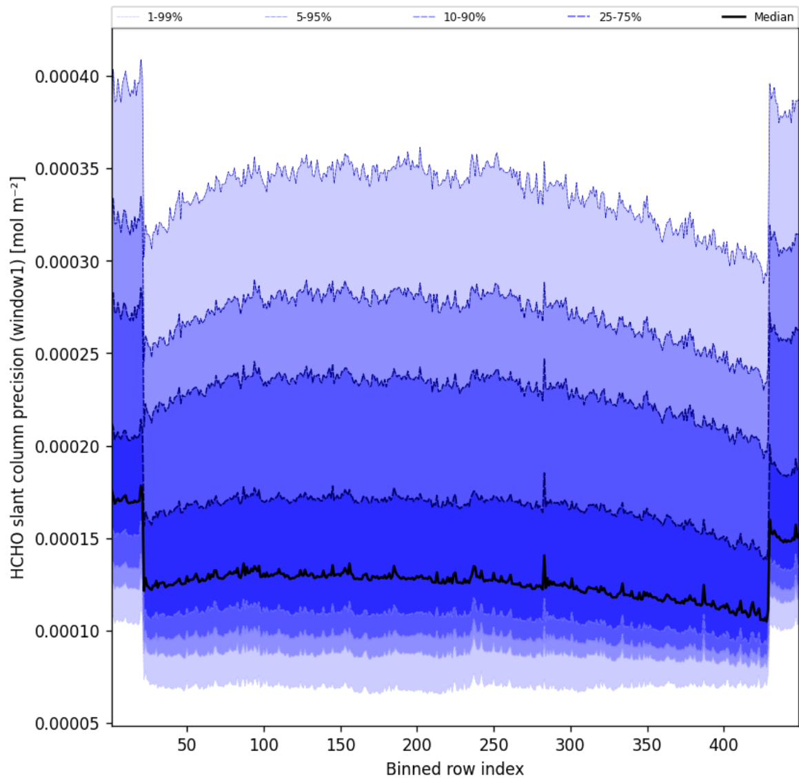
Figure 51: Along track statistics of “HCHO slant column precision (window1)” for 2025-03-24 to 2025-03-25
