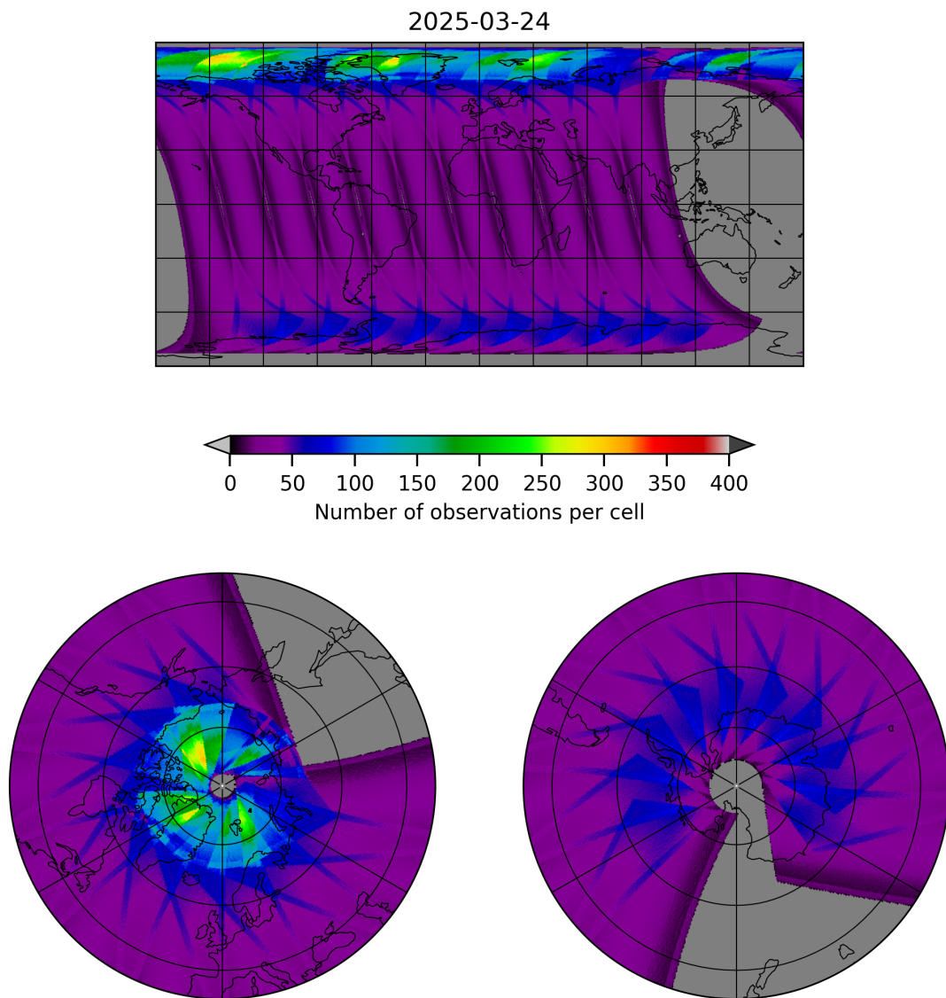
Figure 17: Map of the number of observations for 2025-03-24 to 2025-03-25
