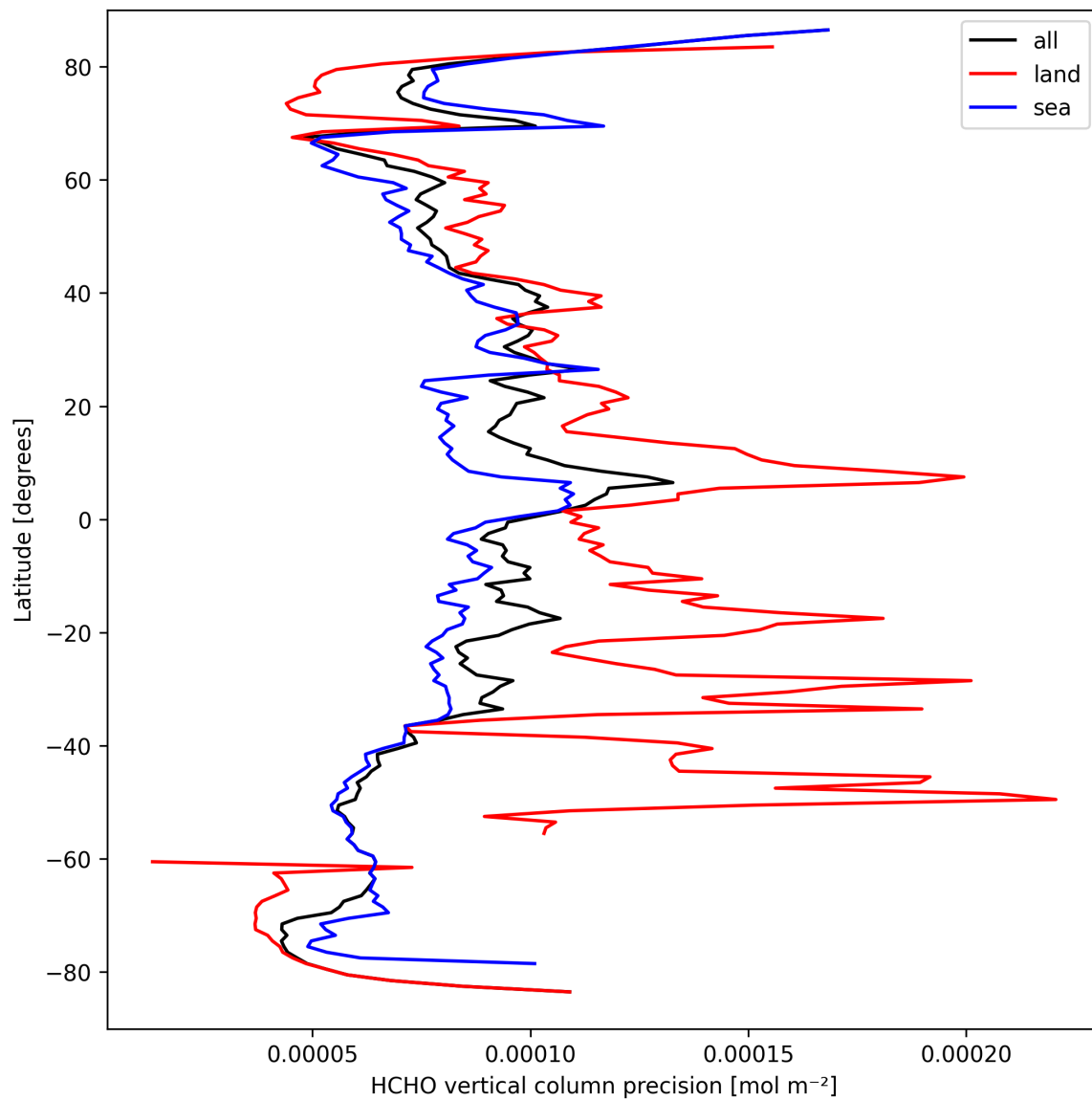
Figure 20: Zonal average of “HCHO vertical column precision” for 2025-03-24 to 2025-03-25.
