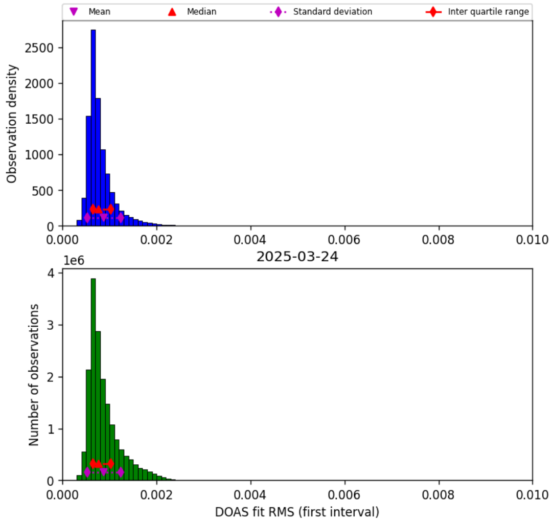
Figure 44: Histogram of “DOAS fit RMS (first interval)” for 2025-03-24 to 2025-03-25
