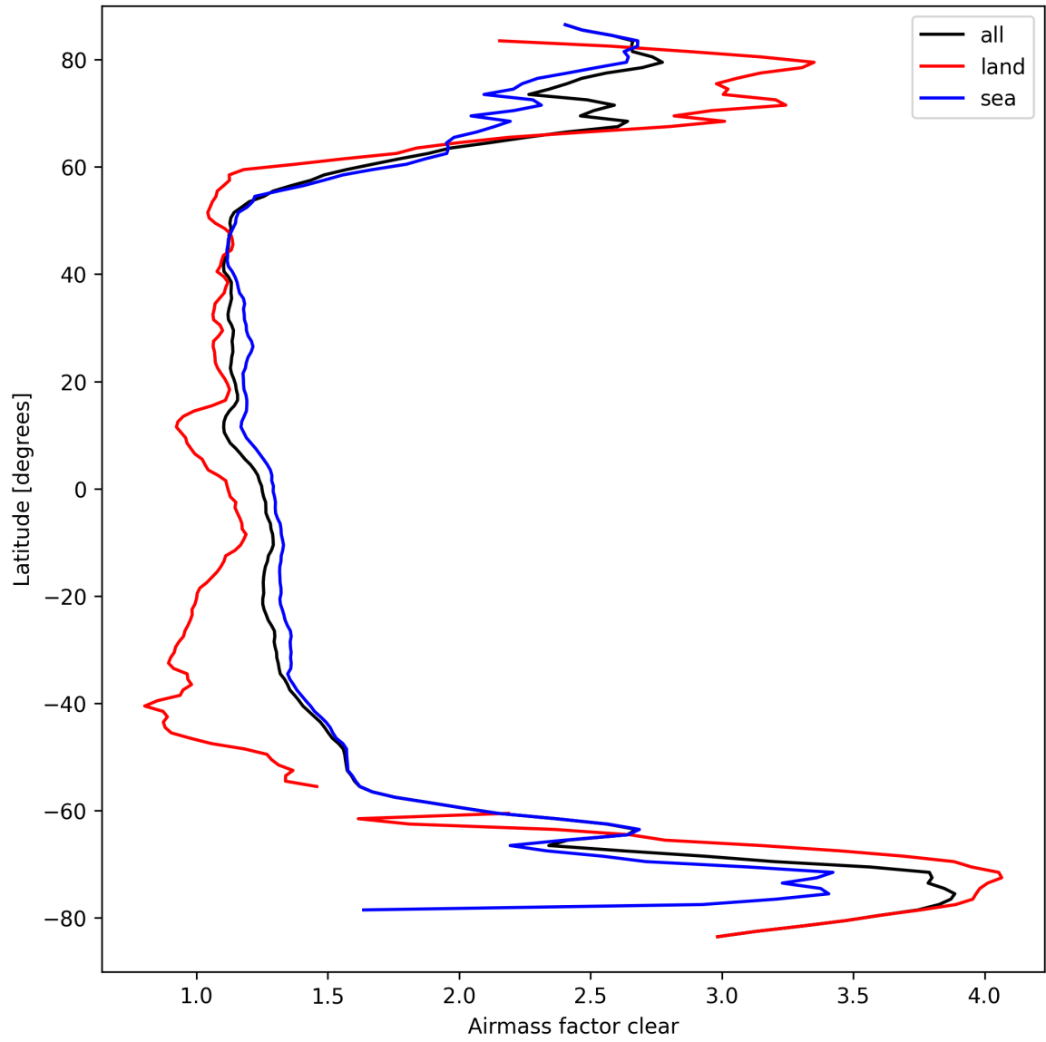
Figure 26: Zonal average of “Airmass factor clear” for 2025-03-24 to 2025-03-25.
