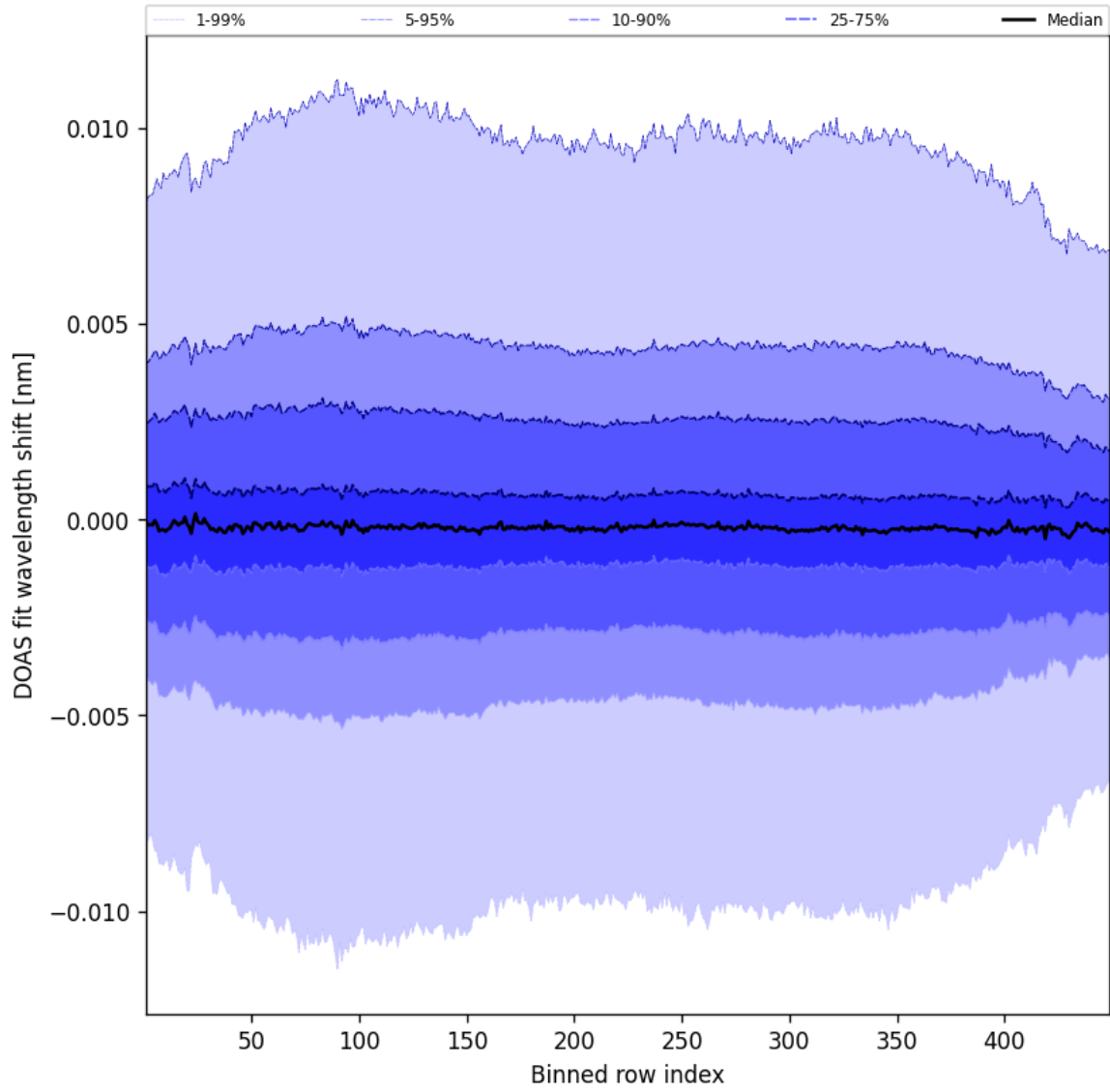
Figure 56: Along track statistics of “DOAS fit wavelength shift” for 2025-03-24 to 2025-03-25
