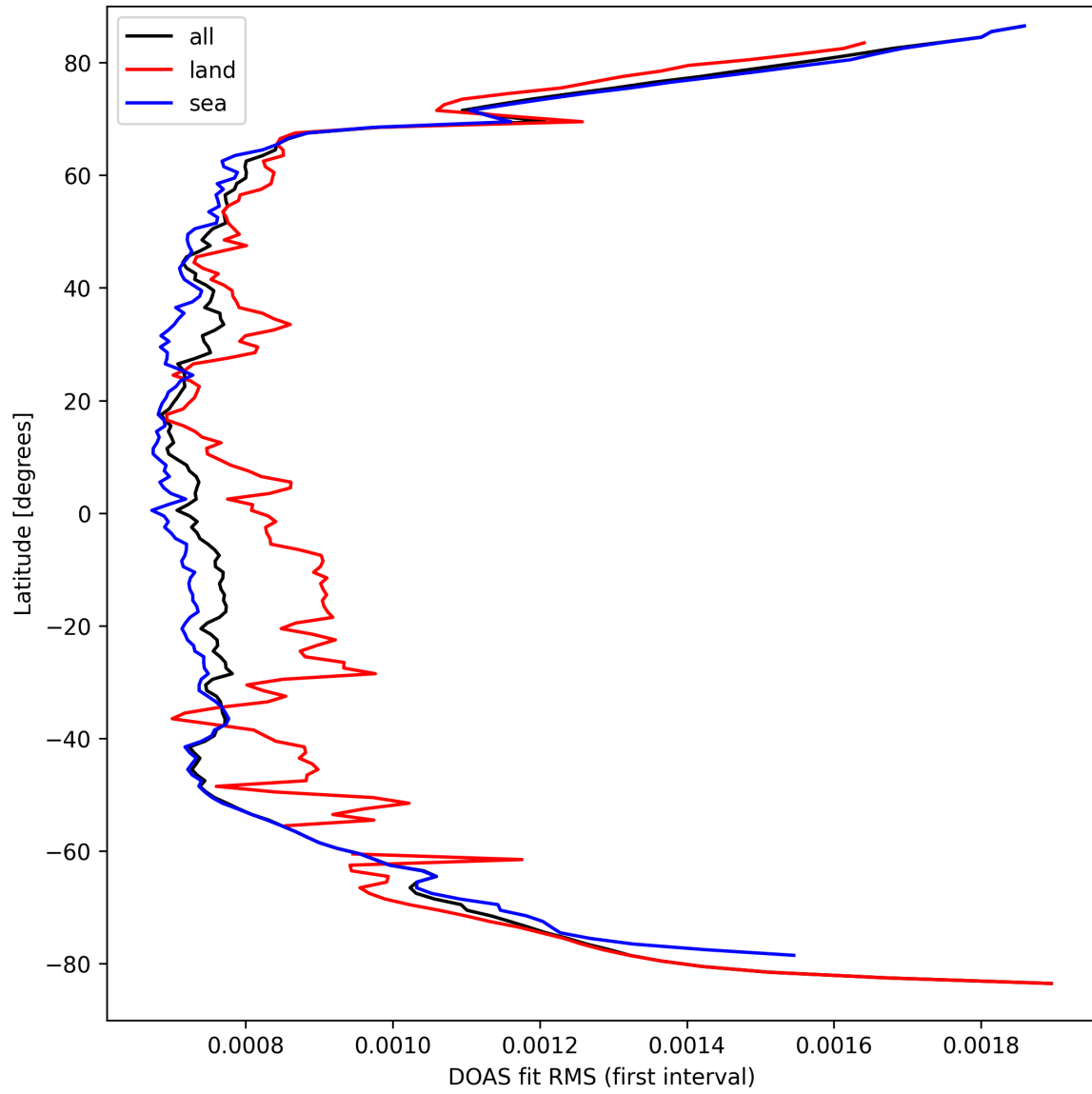
Figure 30: Zonal average of "DOAS fit RMS (first interval)" for 2025-03-24 to 2025-03-25.
