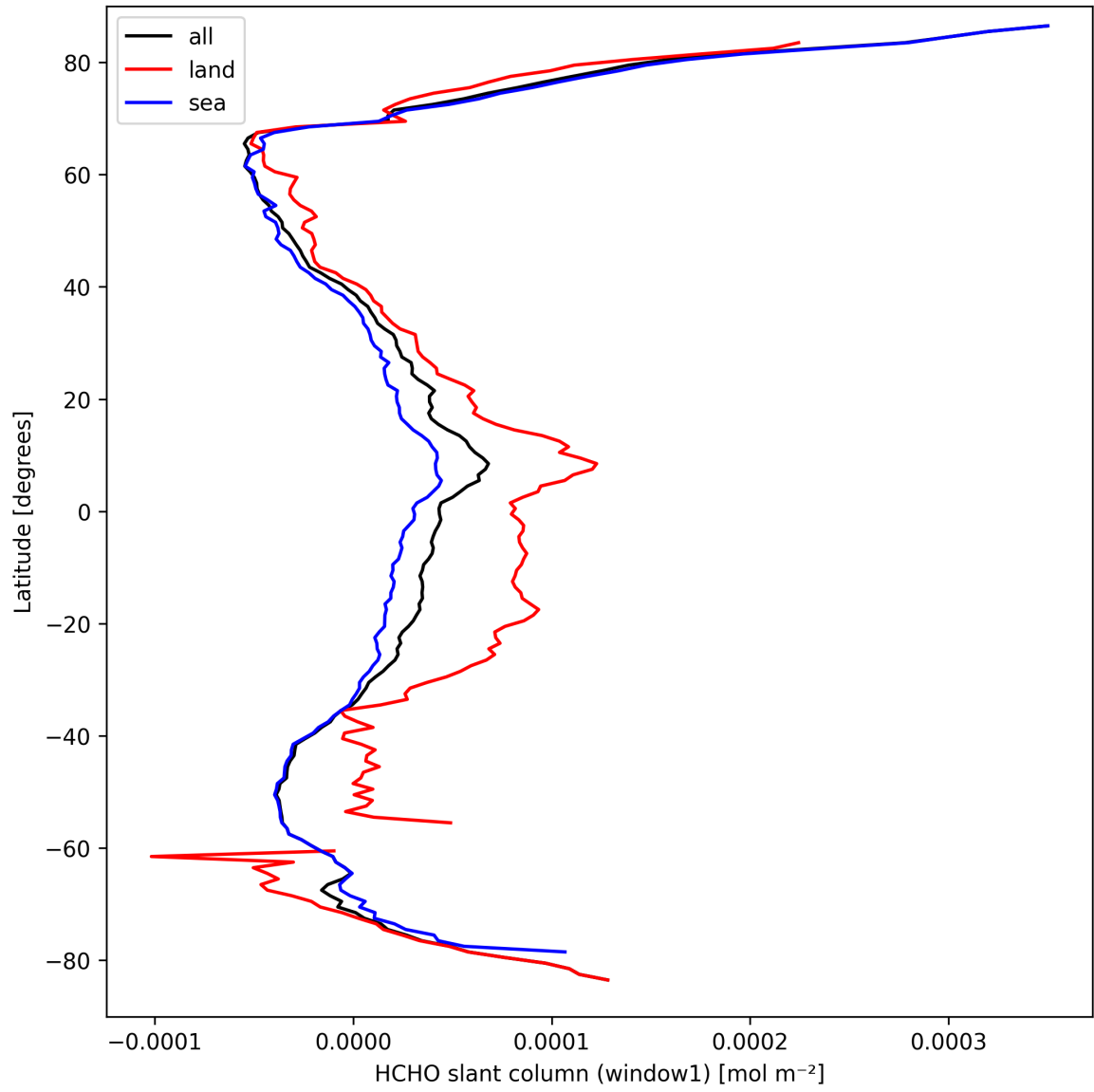
Figure 22: Zonal average of “HCHO slant column (window1)” for 2025-03-24 to 2025-03-25.
