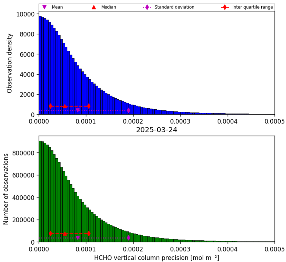
Figure 34: Histogram of “HCHO vertical column precision” for 2025-03-24 to 2025-03-25
