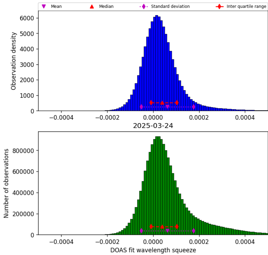
Figure 43: Histogram of “DOAS fit wavelength squeeze” for 2025-03-24 to 2025-03-25
