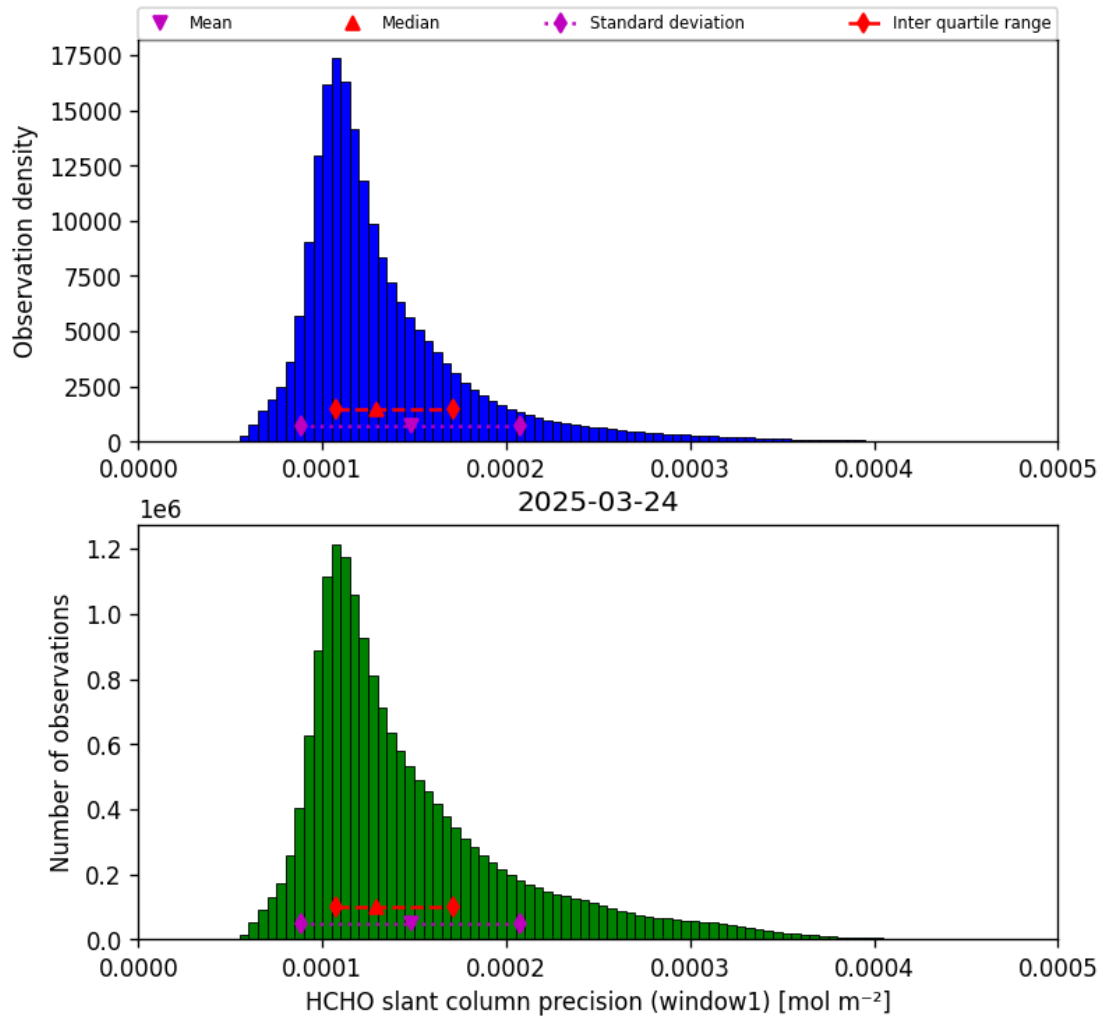
Figure 37: Histogram of “HCHO slant column precision (window1)” for 2025-03-24 to 2025-03-25
