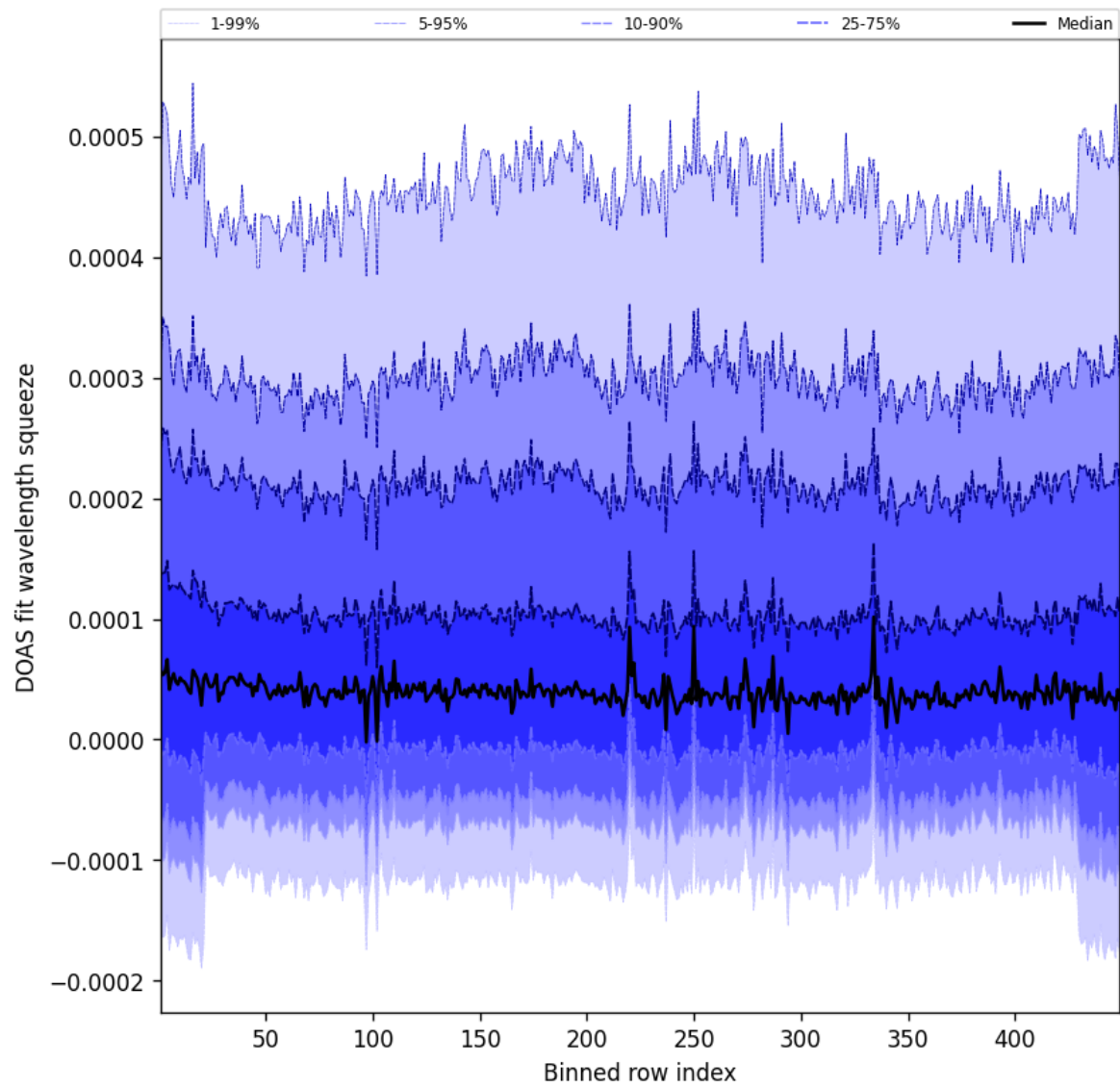
Figure 57: Along track statistics of “DOAS fit wavelength squeeze” for 2025-03-24 to 2025-03-25
