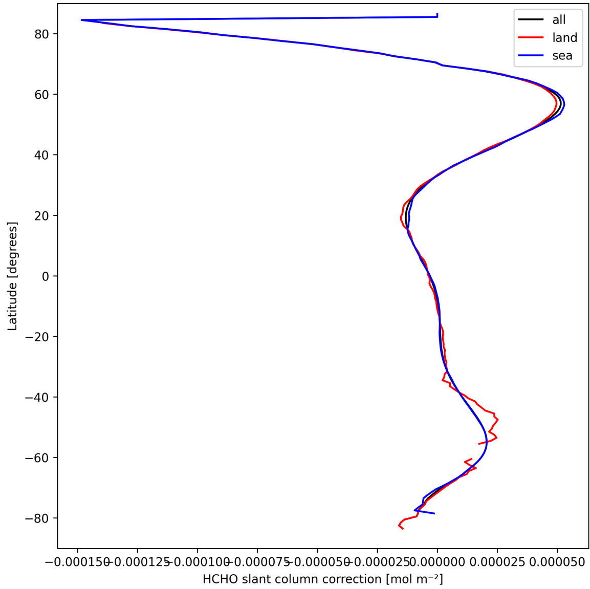
Figure 31: Zonal average of “HCHO slant column correction” for 2025-03-24 to 2025-03-25.
