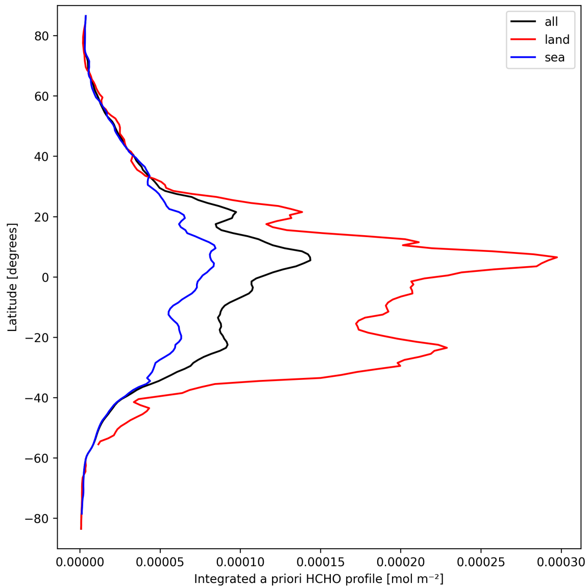
Figure 27: Zonal average of “Integrated a priori HCHO profile” for 2025-03-24 to 2025-03-25.
