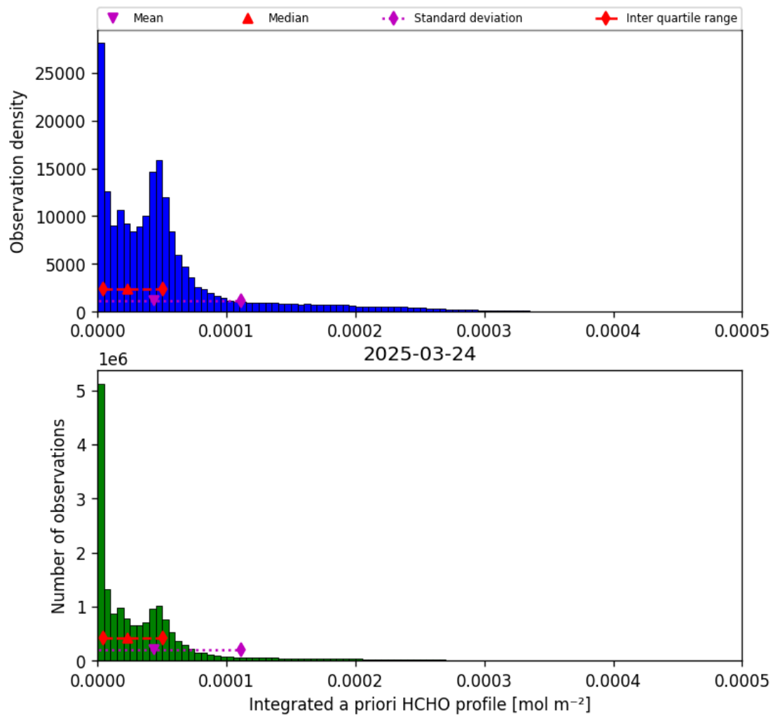
Figure 41: Histogram of “Integrated a priori HCHO profile” for 2025-03-24 to 2025-03-25
