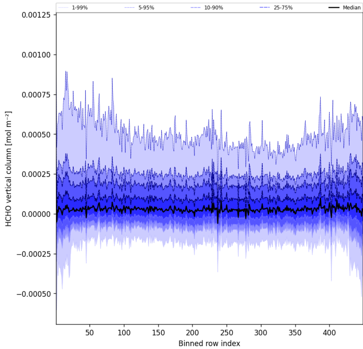
Figure 47: Along track statistics of “HCHO vertical column” for 2025-03-24 to 2025-03-25
