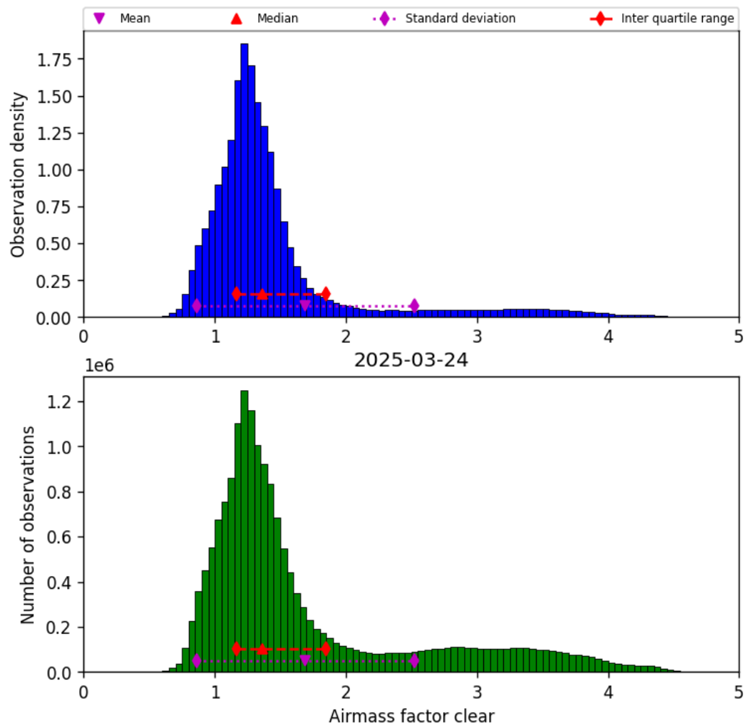
Figure 40: Histogram of “Airmass factor clear” for 2025-03-24 to 2025-03-25
