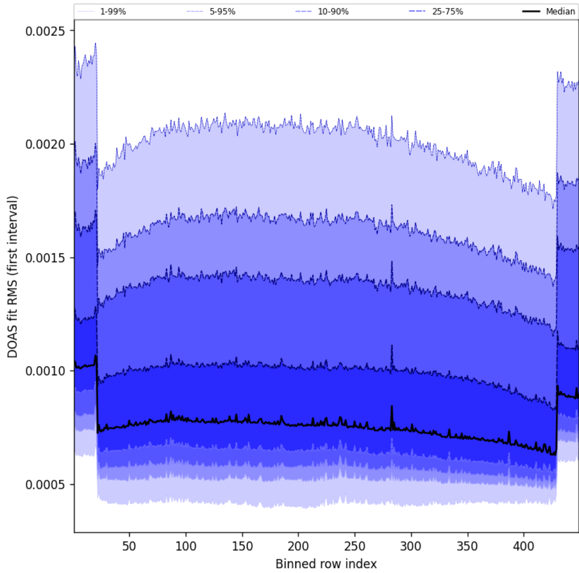
Figure 58: Along track statistics of “DOAS fit RMS (first interval)” for 2025-03-24 to 2025-03-25
