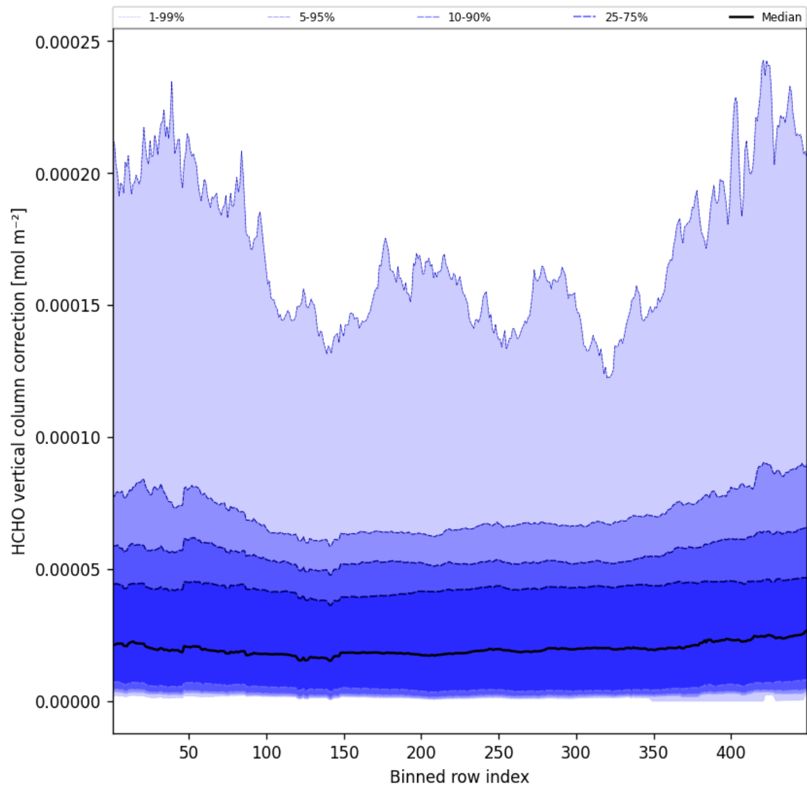
Figure 49: Along track statistics of “HCHO vertical column correction” for 2025-03-24 to 2025-03-25
