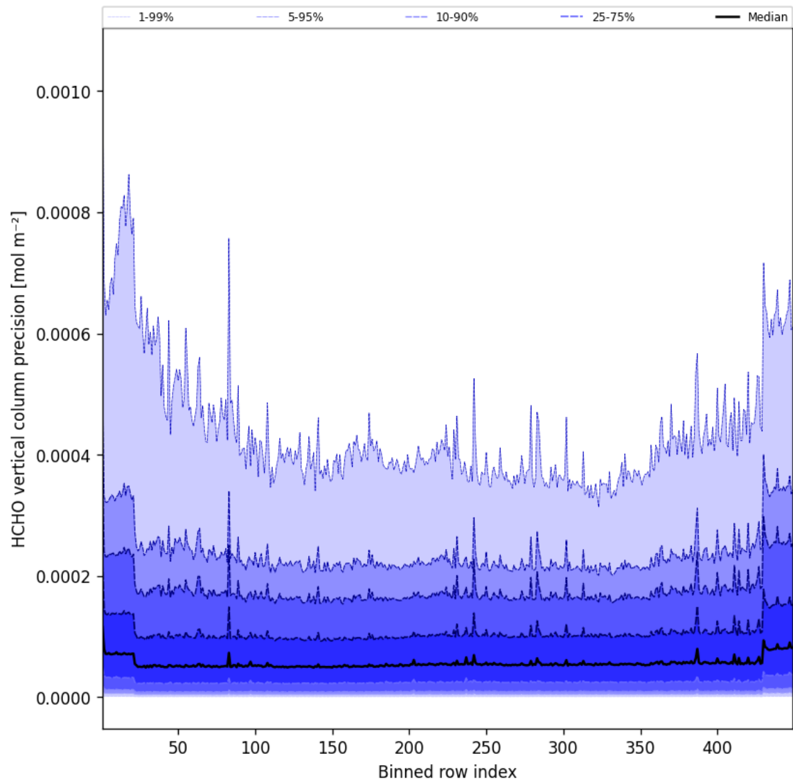
Figure 48: Along track statistics of “HCHO vertical column precision” for 2025-03-24 to 2025-03-25
