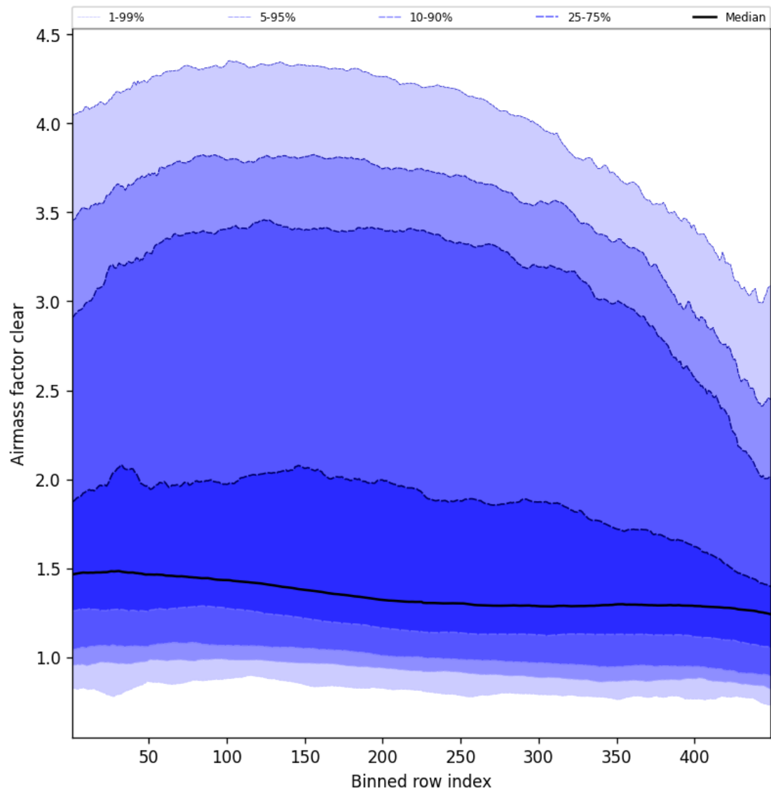
Figure 54: Along track statistics of “Airmass factor clear” for 2025-03-24 to 2025-03-25
