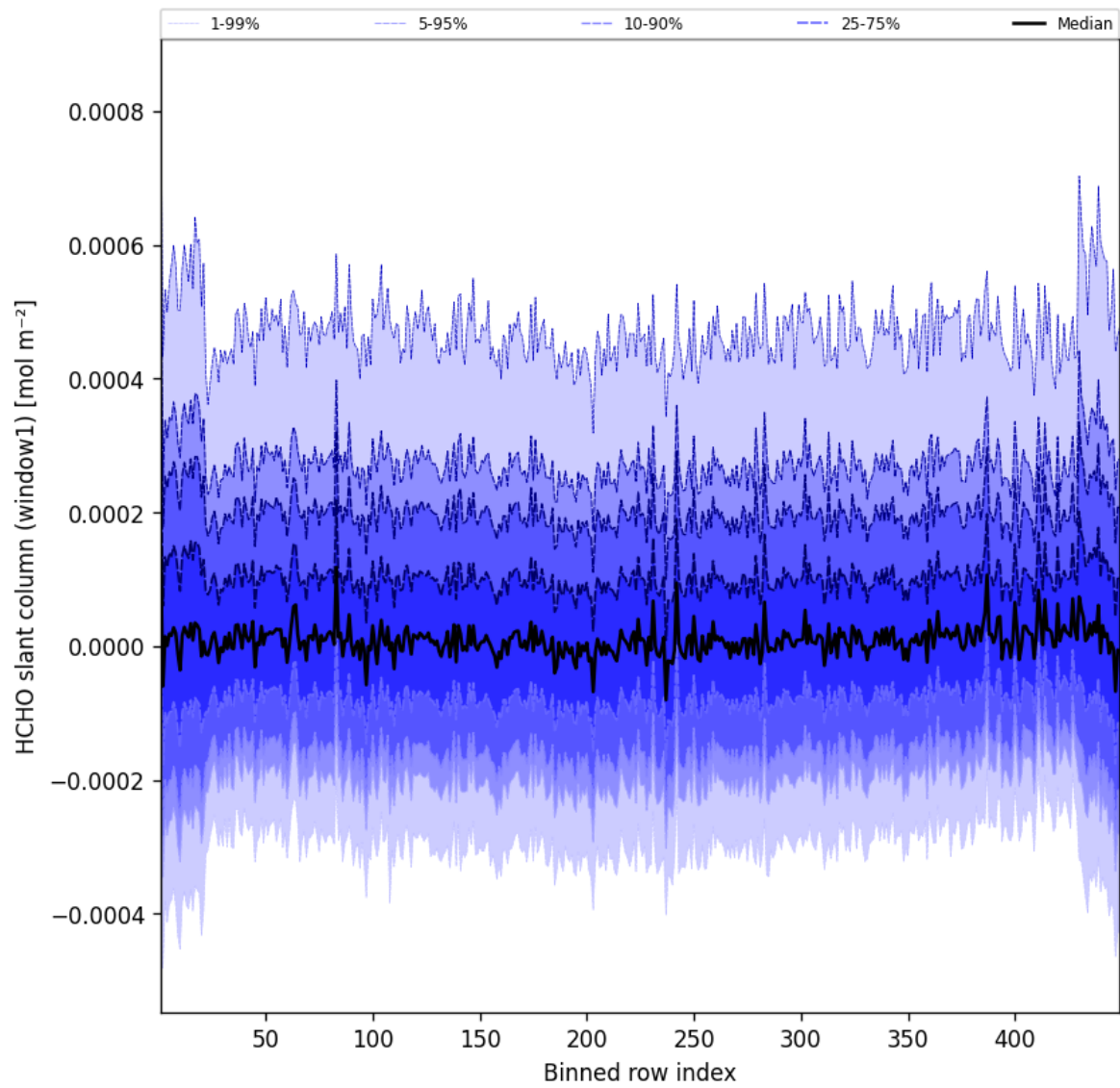
Figure 50: Along track statistics of “HCHO slant column (window1)” for 2025-03-24 to 2025-03-25
