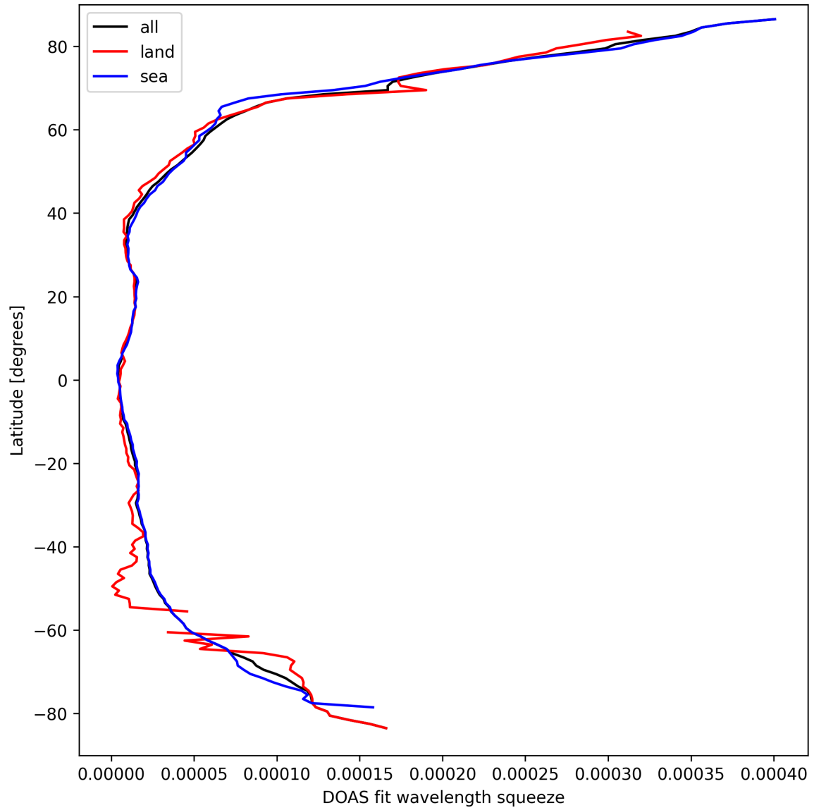
Figure 29: Zonal average of “DOAS fit wavelength squeeze” for 2025-03-24 to 2025-03-25.
