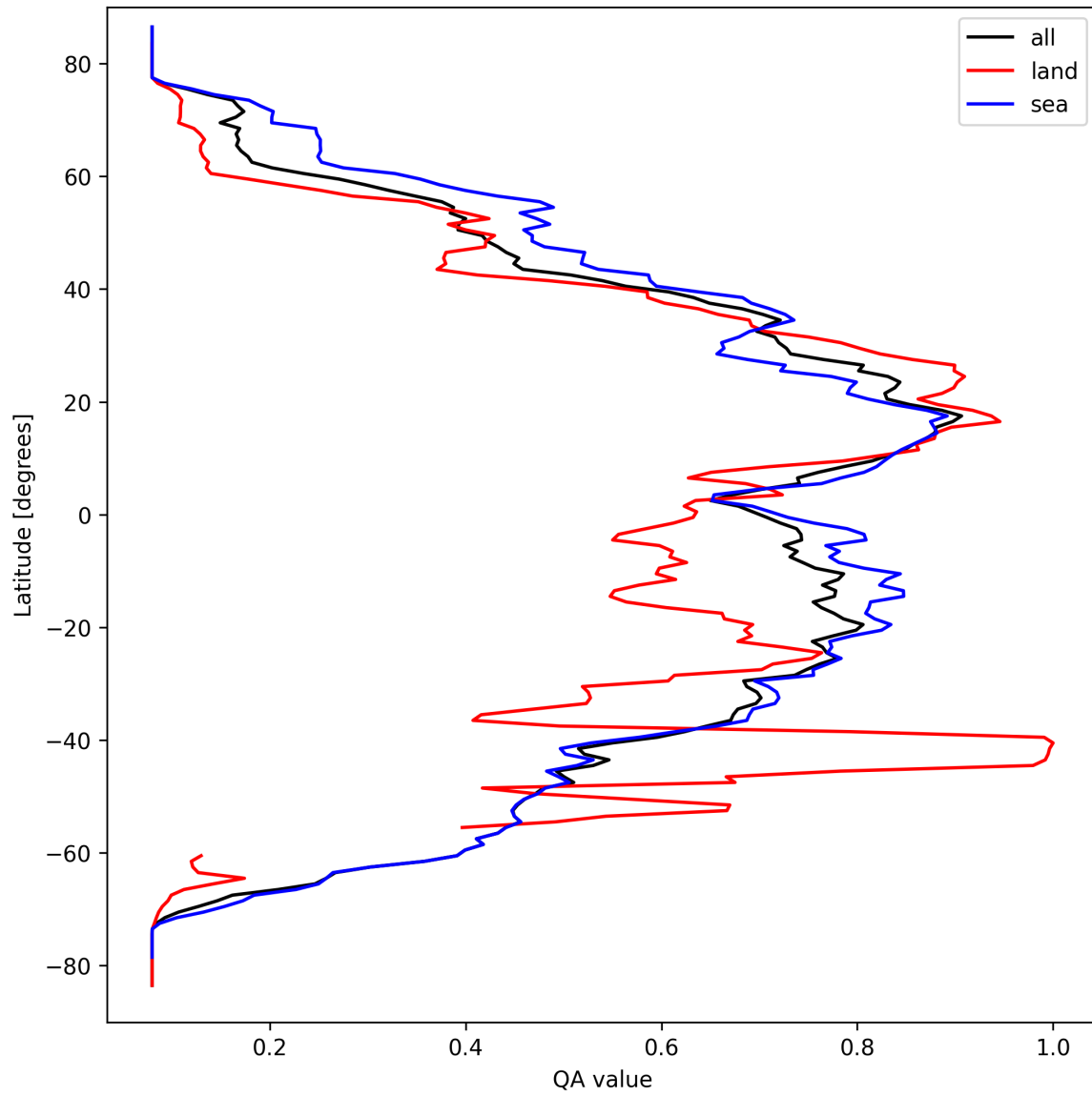
Figure 18: Zonal average of “QA value” for 2025-03-24 to 2025-03-25.
