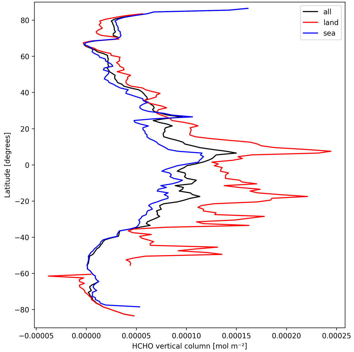
Figure 19: Zonal average of “HCHO vertical column” for 2025-03-24 to 2025-03-25.
