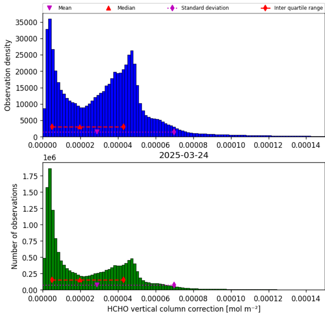
Figure 35: Histogram of “HCHO vertical column correction” for 2025-03-24 to 2025-03-25
