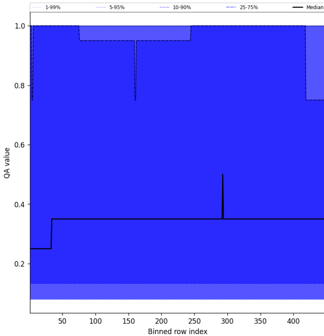
Figure 46: Along track statistics of “QA value” for 2025-03-24 to 2025-03-25
