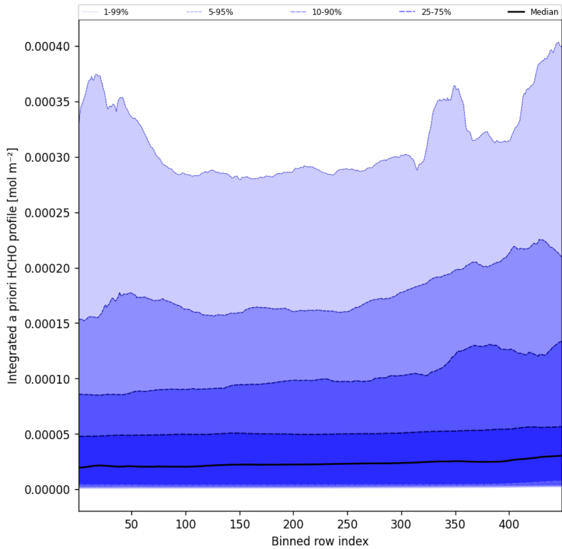
Figure 55: Along track statistics of “Integrated a priori HCHO profile” for 2025-03-24 to 2025-03-25
