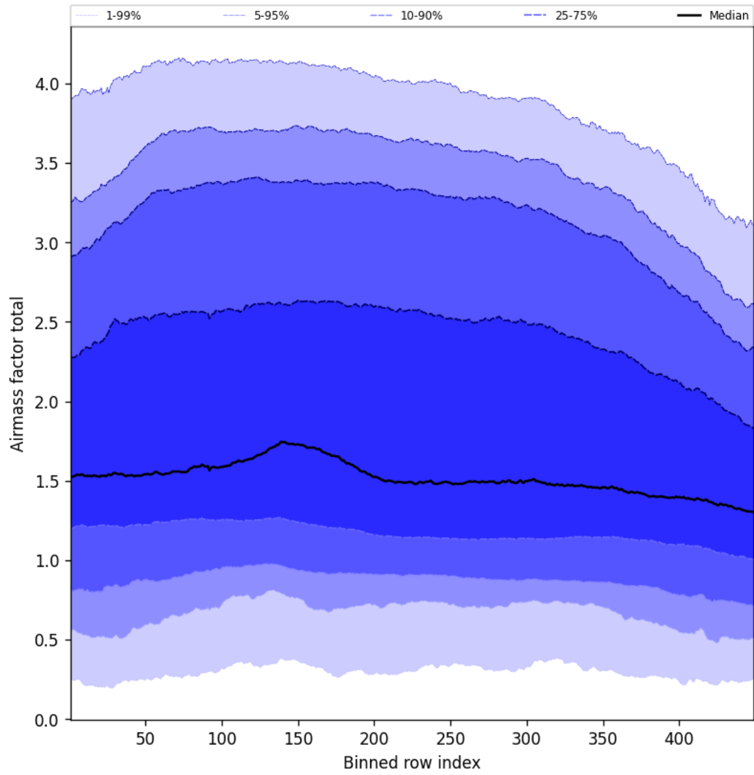
Figure 52: Along track statistics of “Airmass factor total” for 2025-03-24 to 2025-03-25
