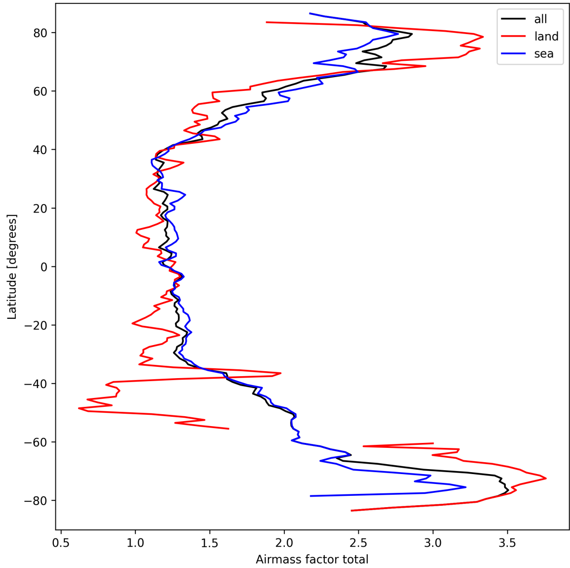
Figure 24: Zonal average of “Airmass factor total” for 2025-03-24 to 2025-03-25.
