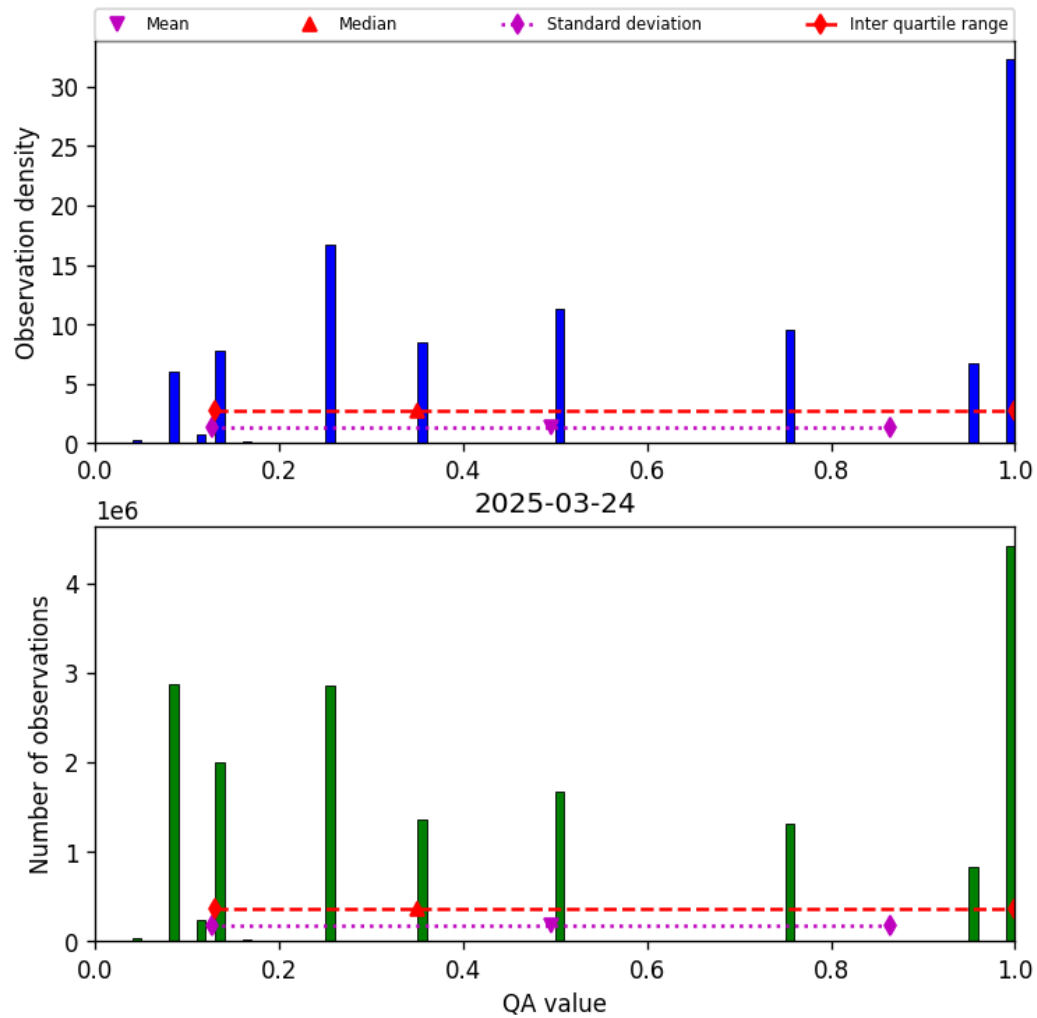
Figure 32: Histogram of “QA value” for 2025-03-24 to 2025-03-25
