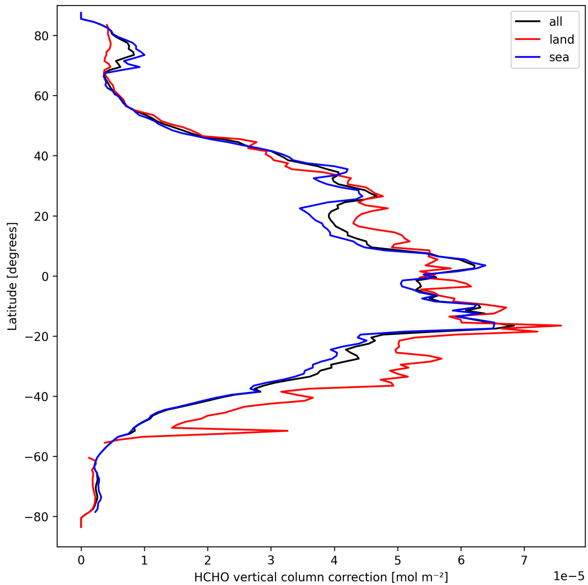
Figure 21: Zonal average of “HCHO vertical column correction” for 2025-03-25 to 2025-03-26.
