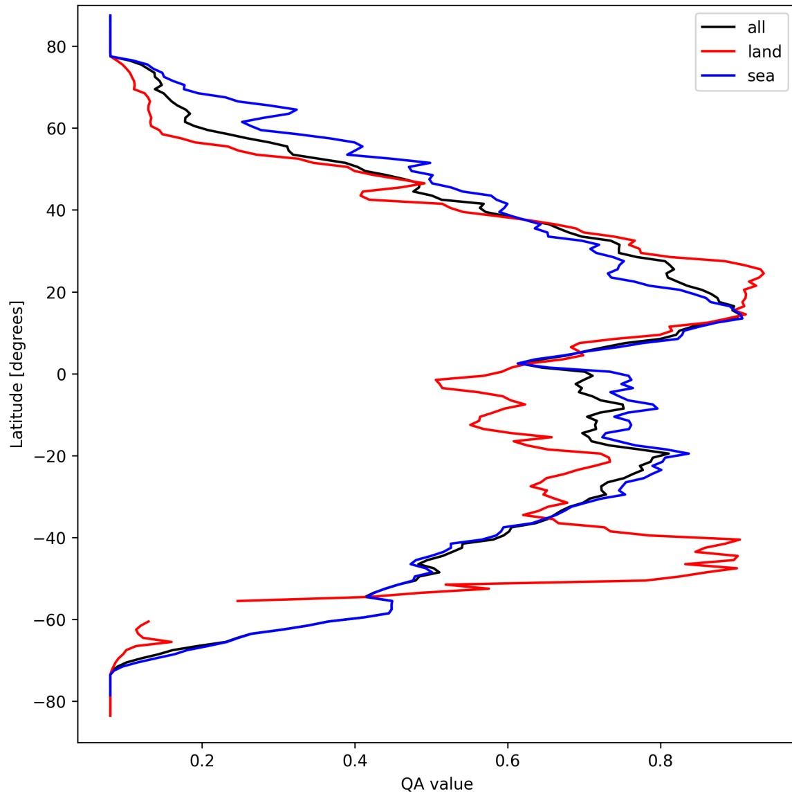
Figure 18: Zonal average of “QA value” for 2025-03-25 to 2025-03-26.
