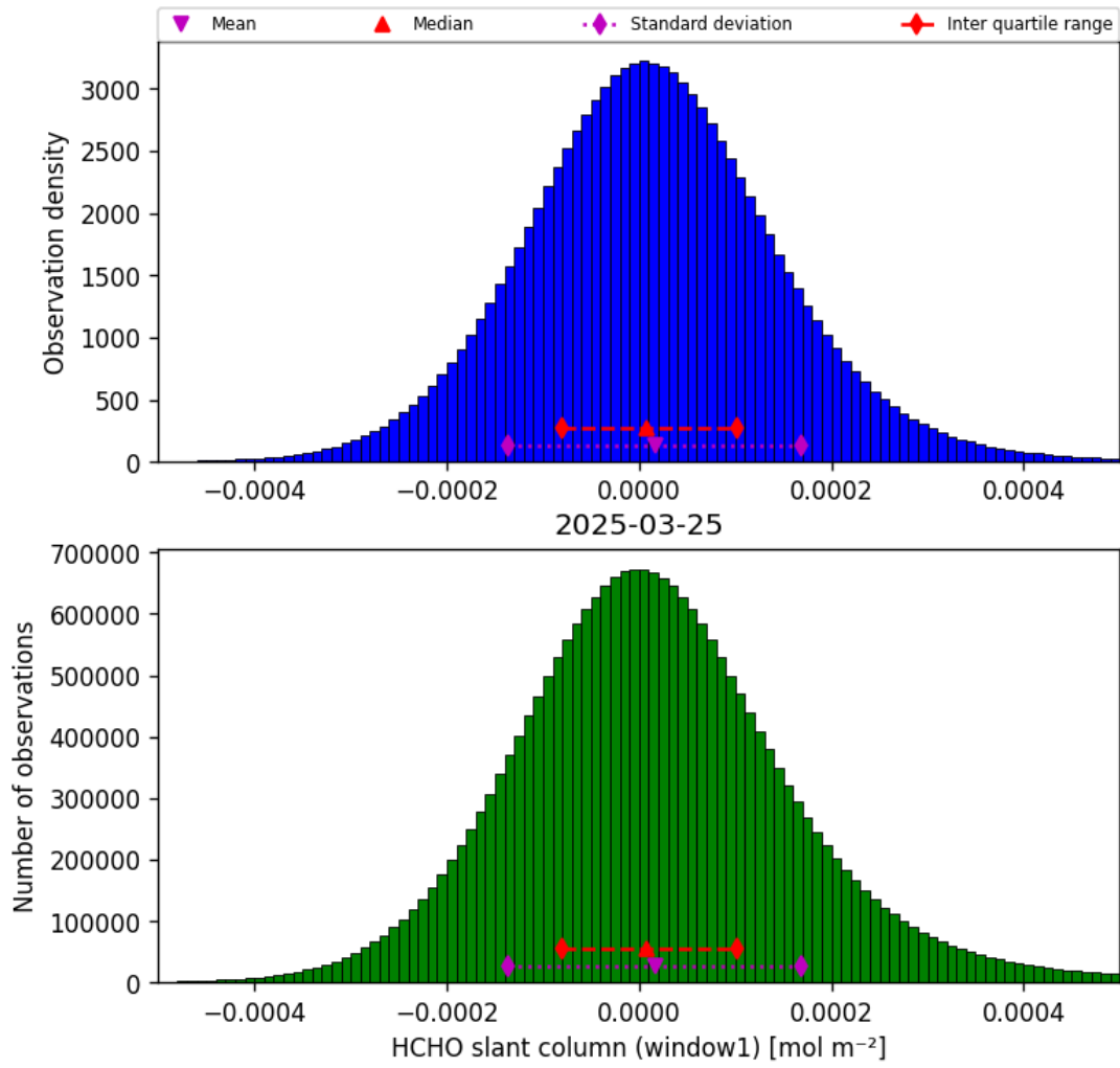
Figure 36: Histogram of “HCHO slant column (window1)” for 2025-03-25 to 2025-03-26
