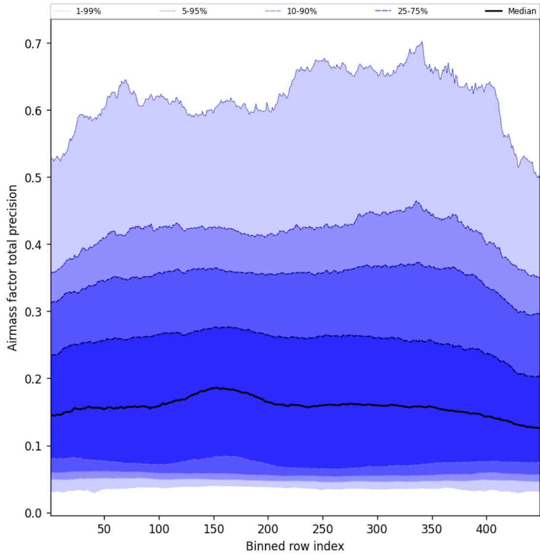
Figure 53: Along track statistics of “Airmass factor total precision” for 2025-03-25 to 2025-03-26
