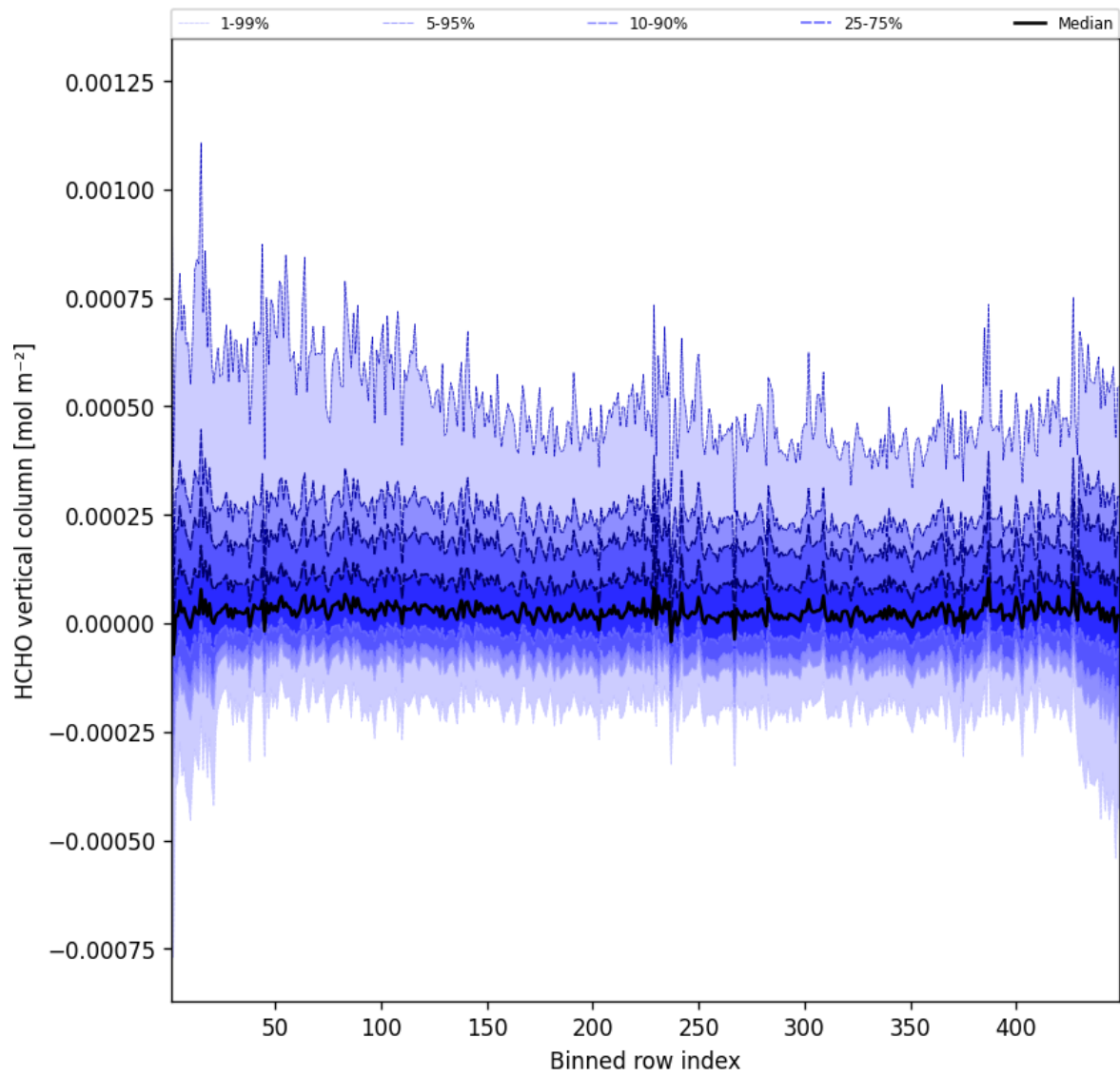
Figure 47: Along track statistics of “HCHO vertical column” for 2025-03-25 to 2025-03-26
