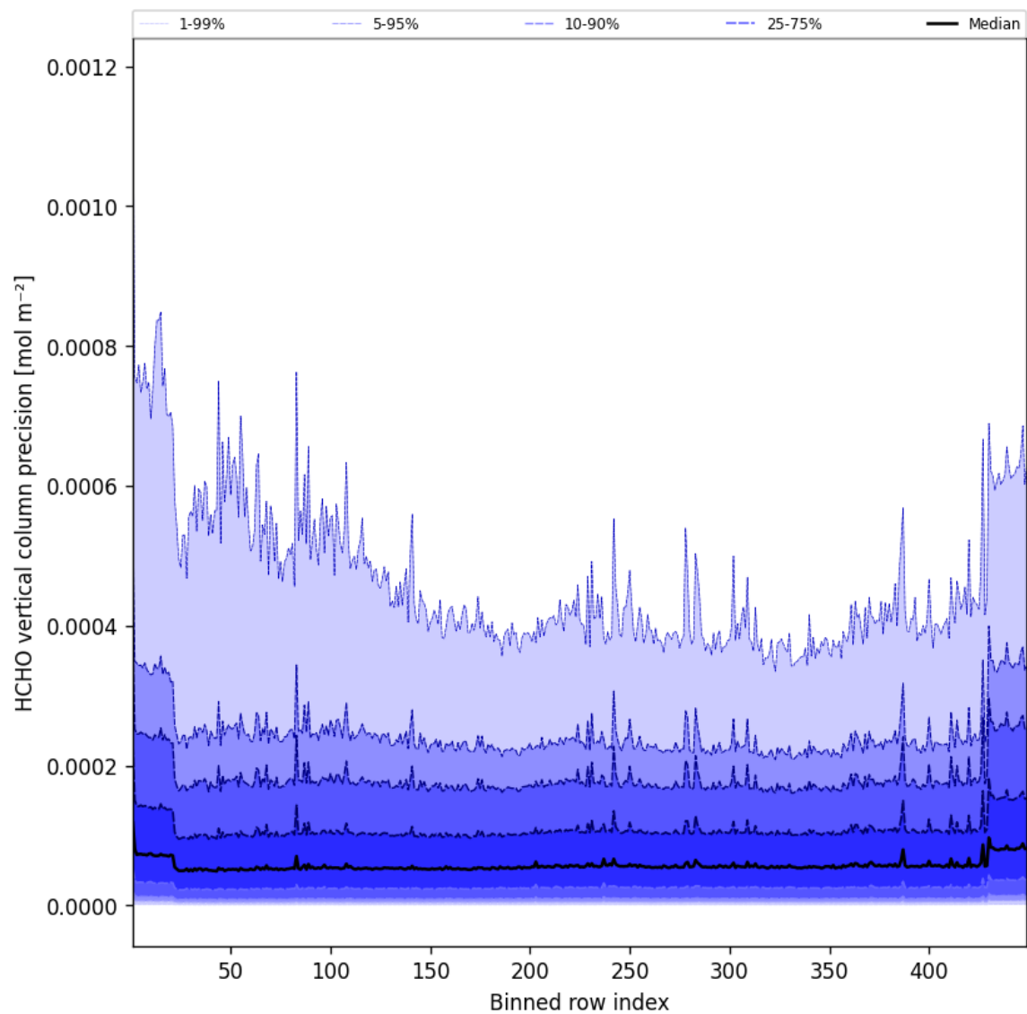
Figure 48: Along track statistics of “HCHO vertical column precision” for 2025-03-25 to 2025-03-26
