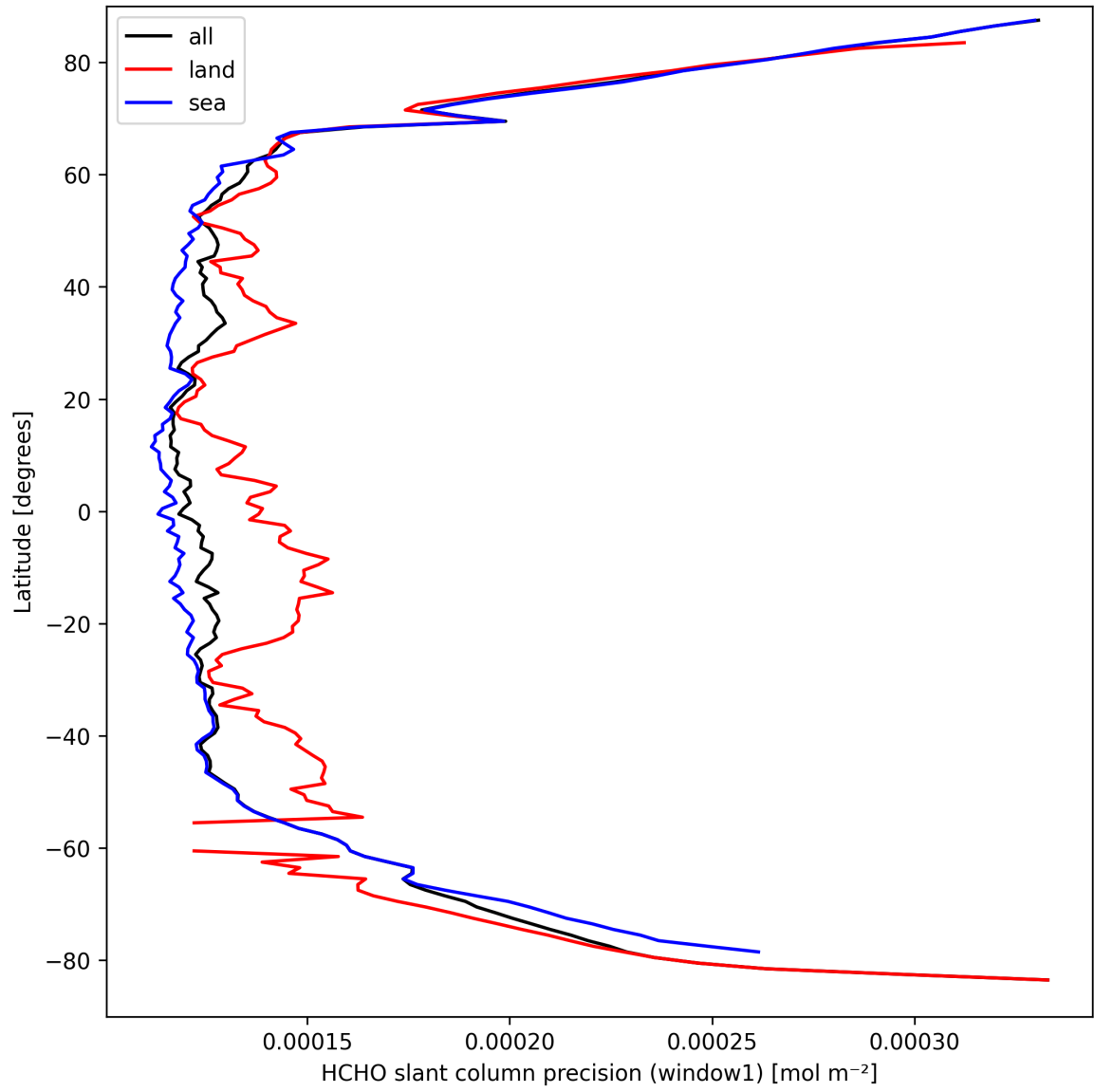
Figure 23: Zonal average of “HCHO slant column precision (window1)” for 2025-03-25 to 2025-03-26.
