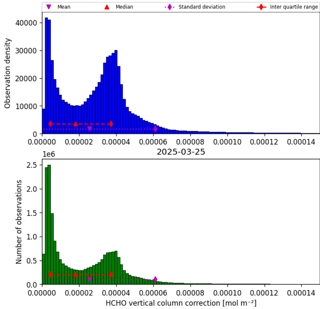
Figure 35: Histogram of “HCHO vertical column correction” for 2025-03-25 to 2025-03-26
