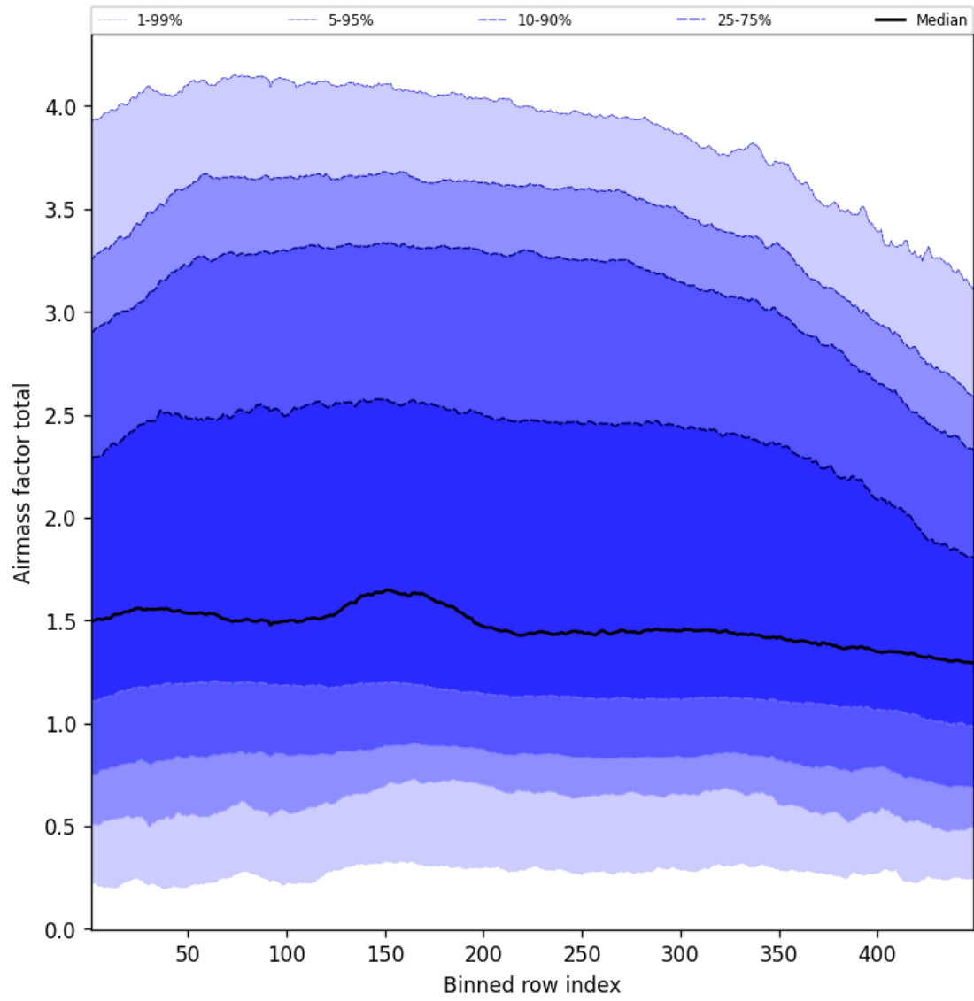
Figure 52: Along track statistics of “Airmass factor total” for 2025-03-25 to 2025-03-26
