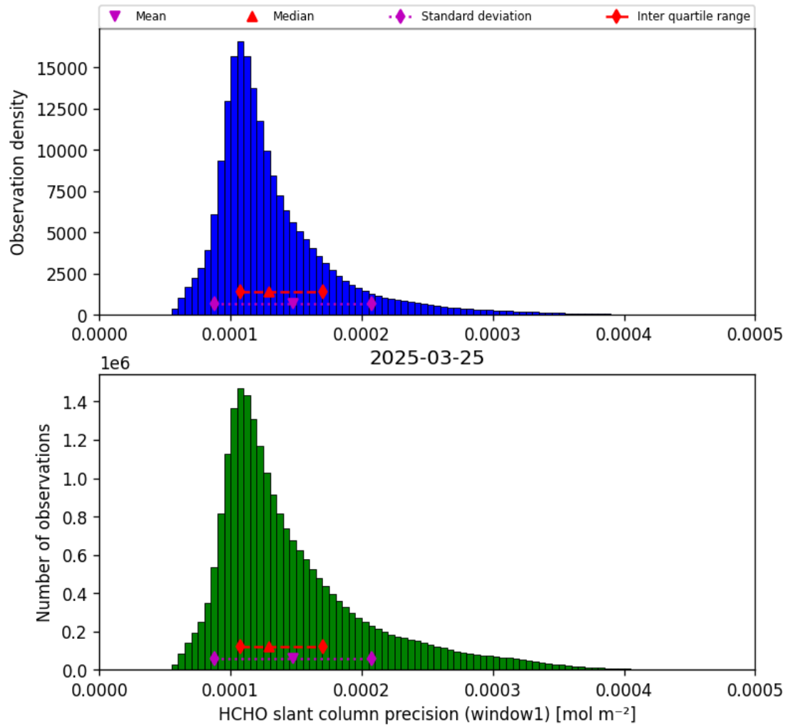
Figure 37: Histogram of “HCHO slant column precision (window1)” for 2025-03-25 to 2025-03-26
