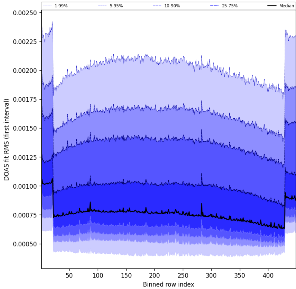
Figure 58: Along track statistics of “DOAS fit RMS (first interval)” for 2025-03-25 to 2025-03-26
