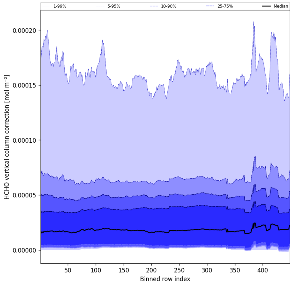
Figure 49: Along track statistics of “HCHO vertical column correction” for 2025-03-25 to 2025-03-26
