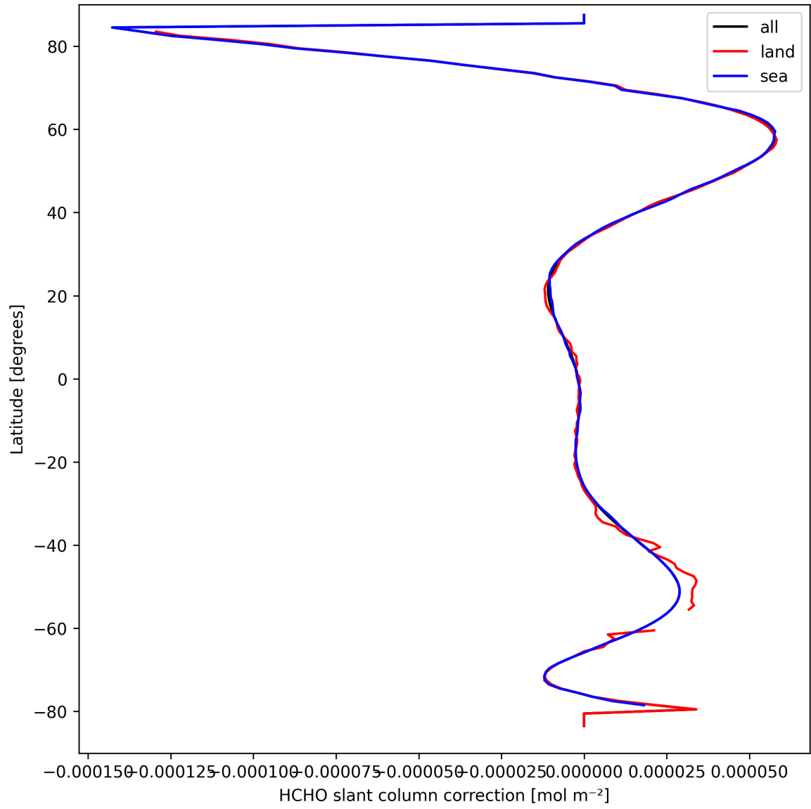
Figure 31: Zonal average of “HCHO slant column correction” for 2025-03-25 to 2025-03-26.
