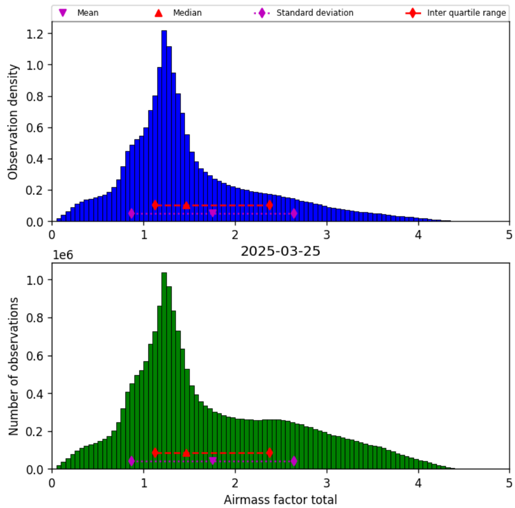
Figure 38: Histogram of “Airmass factor total” for 2025-03-25 to 2025-03-26
