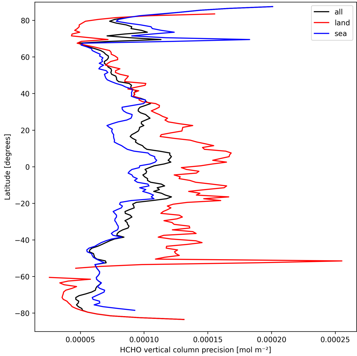
Figure 20: Zonal average of “HCHO vertical column precision” for 2025-03-25 to 2025-03-26.
