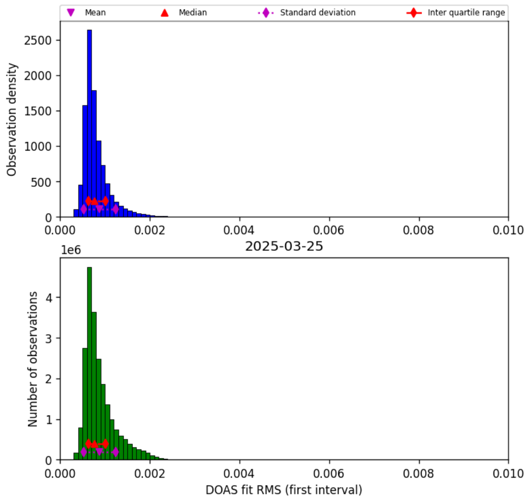
Figure 44: Histogram of “DOAS fit RMS (first interval)” for 2025-03-25 to 2025-03-26
