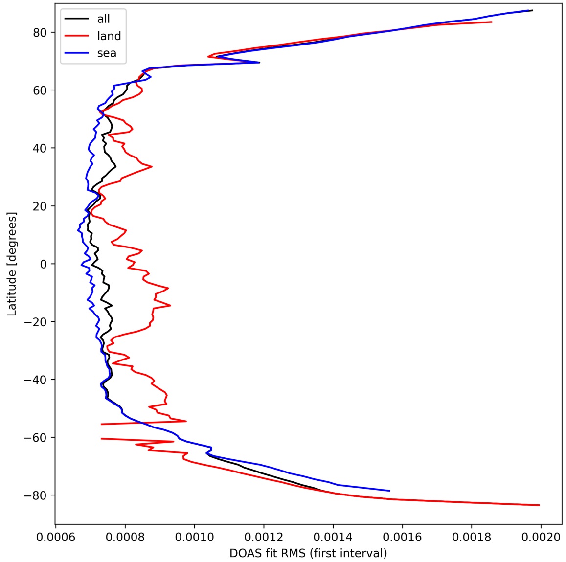
Figure 30: Zonal average of “DOAS fit RMS (first interval)” for 2025-03-25 to 2025-03-26.
