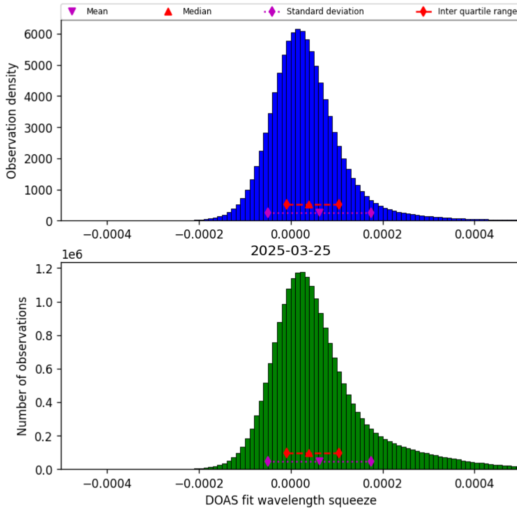
Figure 43: Histogram of “DOAS fit wavelength squeeze” for 2025-03-25 to 2025-03-26
