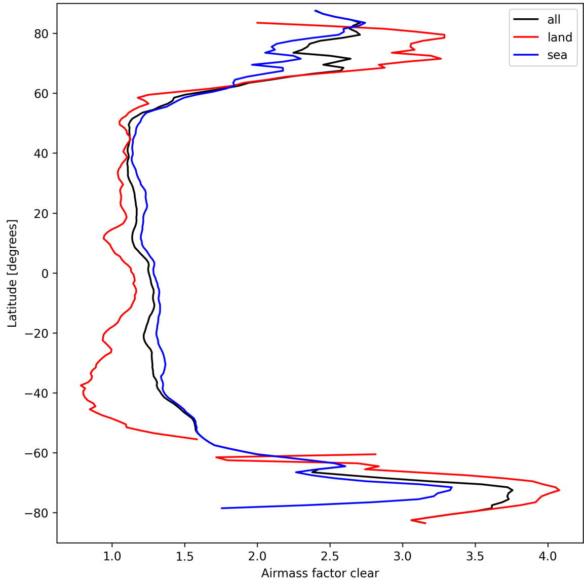
Figure 26: Zonal average of “Airmass factor clear” for 2025-03-25 to 2025-03-26.
