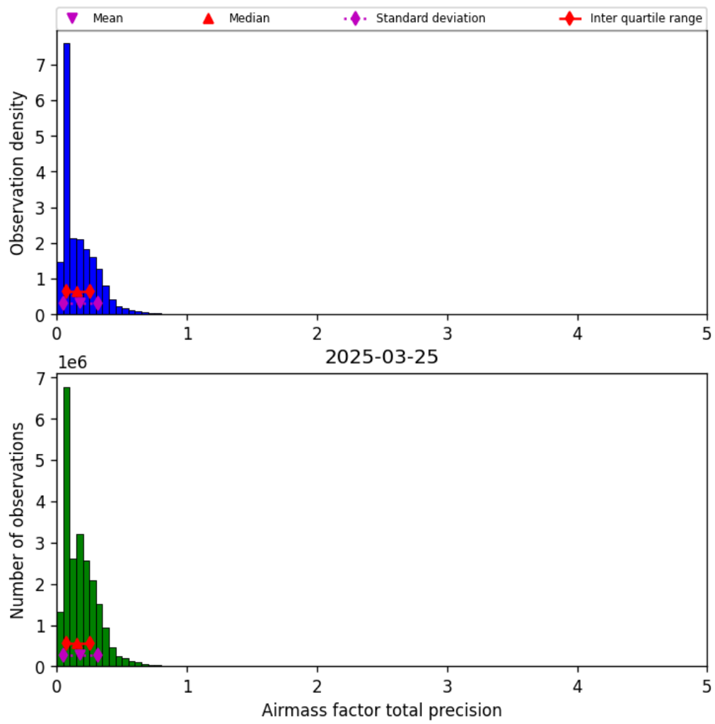
Figure 39: Histogram of “Airmass factor total precision” for 2025-03-25 to 2025-03-26
