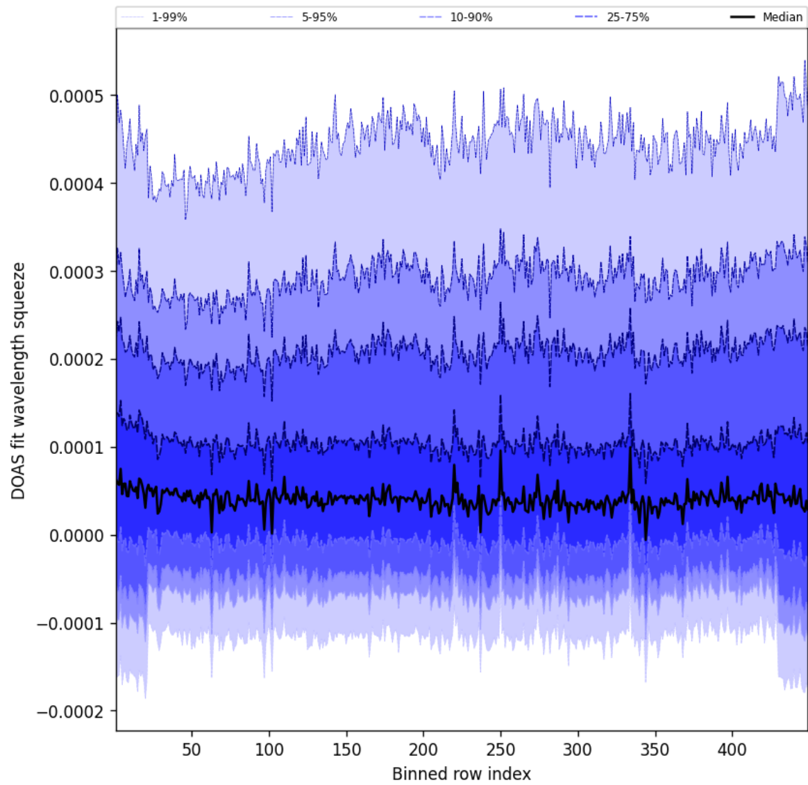
Figure 57: Along track statistics of “DOAS fit wavelength squeeze” for 2025-03-25 to 2025-03-26
