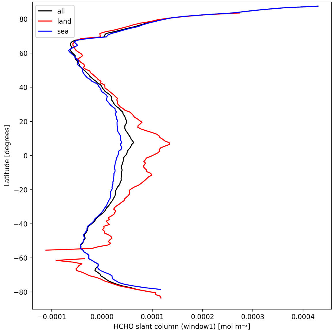
Figure 22: Zonal average of “HCHO slant column (window1)” for 2025-03-25 to 2025-03-26.
