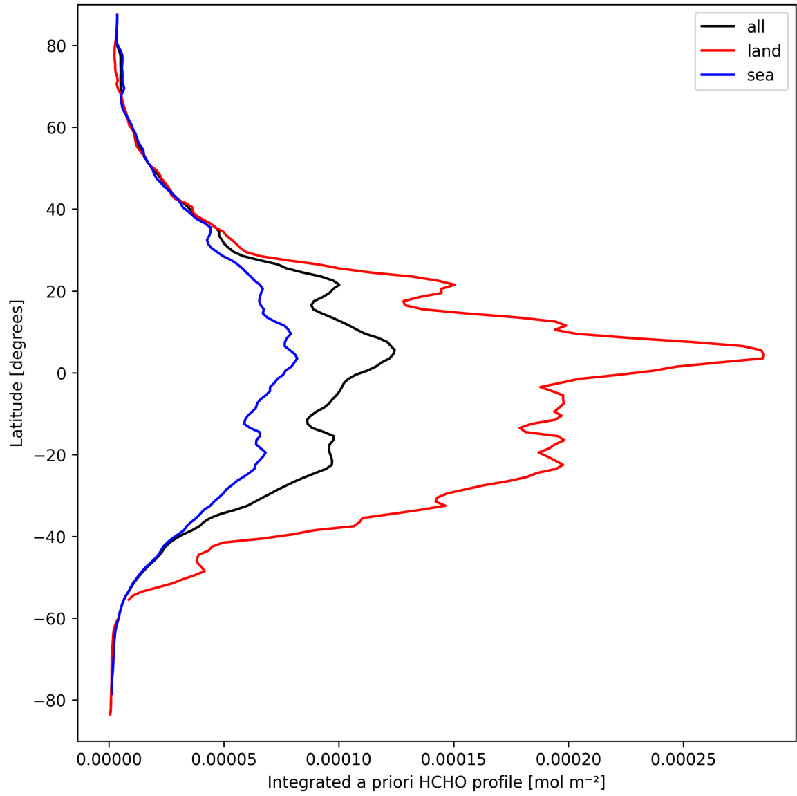
Figure 27: Zonal average of “Integrated a priori HCHO profile” for 2025-03-25 to 2025-03-26.
