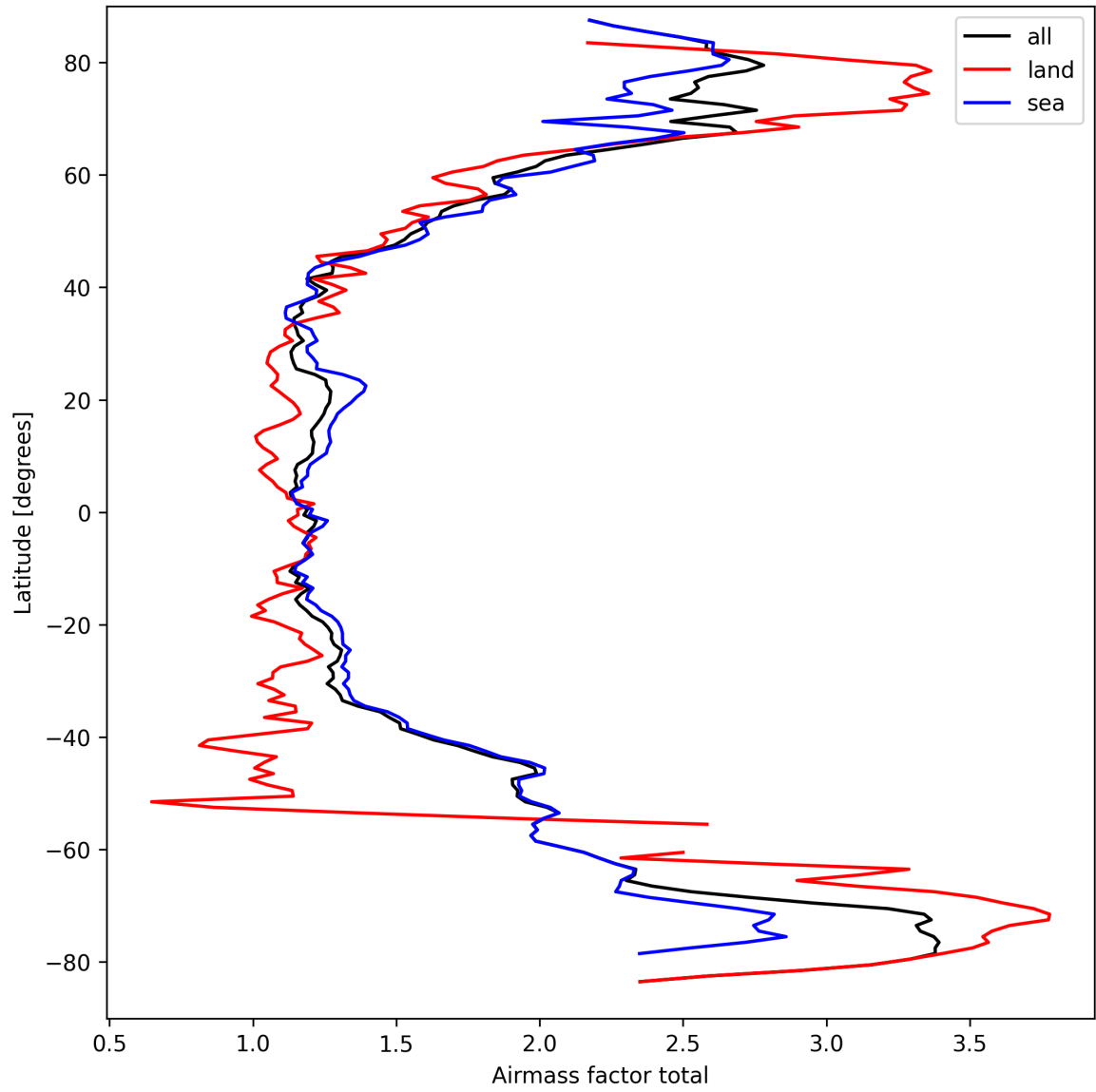
Figure 24: Zonal average of “Airmass factor total” for 2025-03-25 to 2025-03-26.
