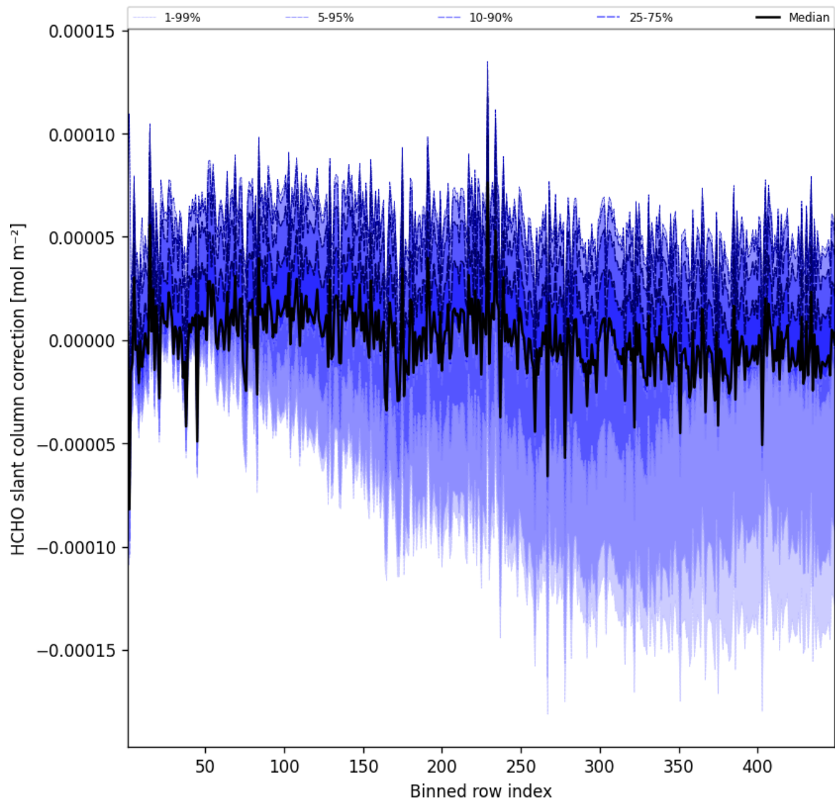
Figure 59: Along track statistics of “HCHO slant column correction” for 2025-03-25 to 2025-03-26
