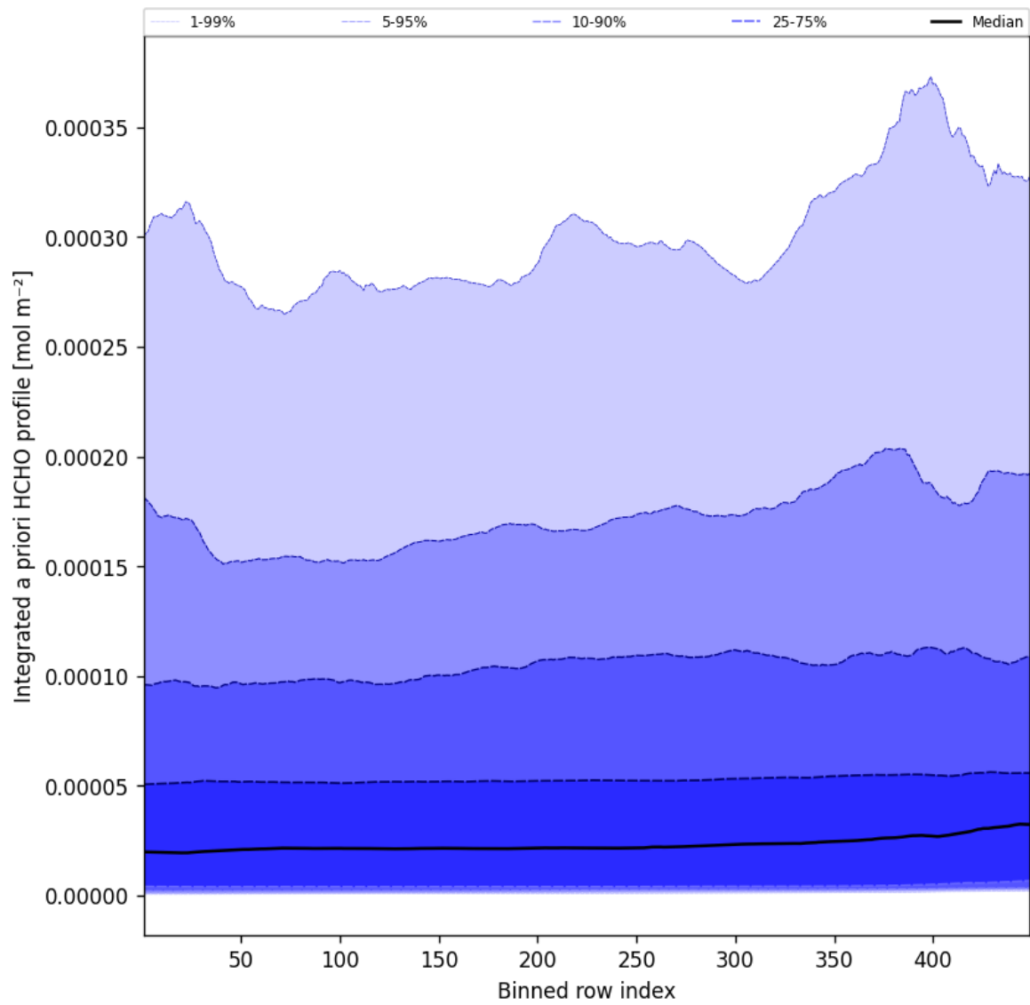
Figure 55: Along track statistics of “Integrated a priori HCHO profile” for 2025-03-25 to 2025-03-26
