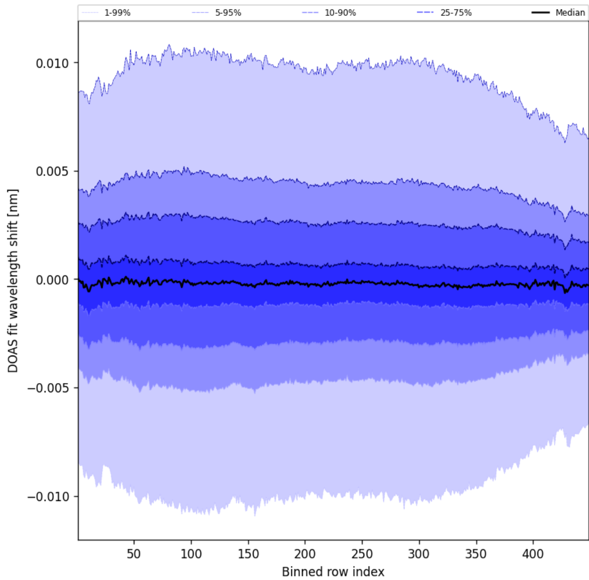
Figure 56: Along track statistics of “DOAS fit wavelength shift” for 2025-03-25 to 2025-03-26
