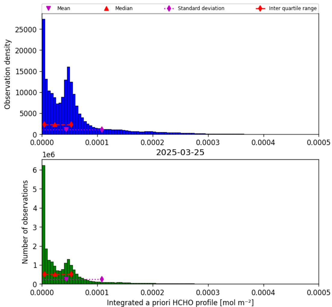
Figure 41: Histogram of “Integrated a priori HCHO profile” for 2025-03-25 to 2025-03-26
