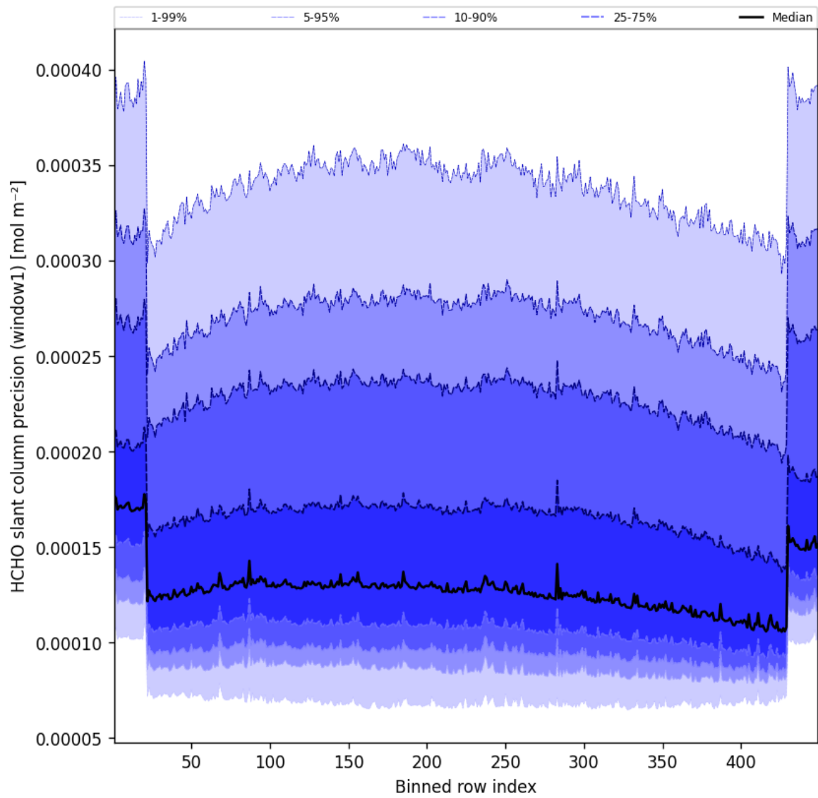
Figure 51: Along track statistics of “HCHO slant column precision (window1)” for 2025-03-25 to 2025-03-26
