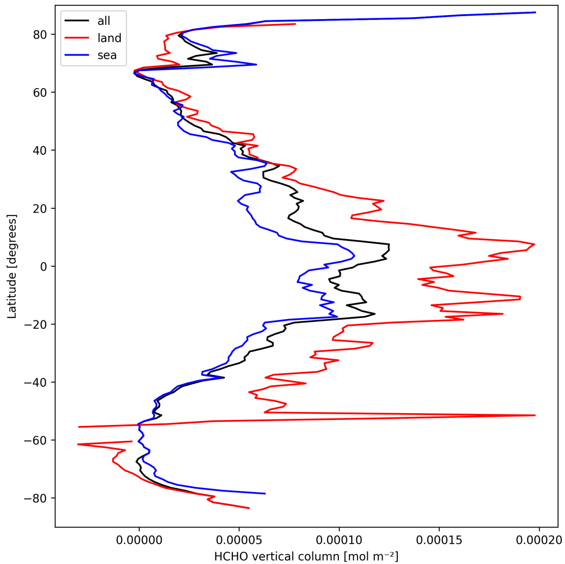
Figure 19: Zonal average of “HCHO vertical column” for 2025-03-25 to 2025-03-26.
