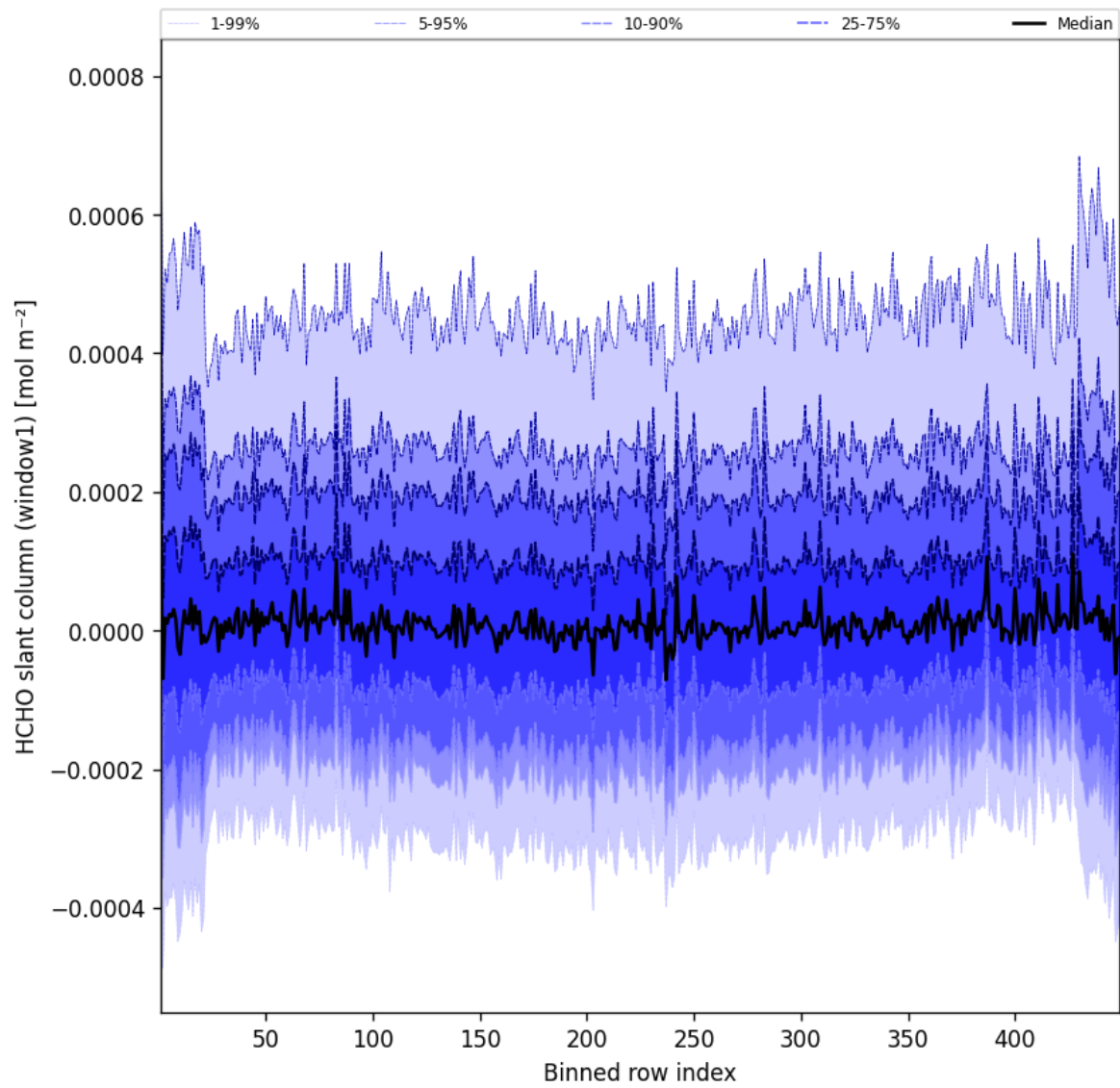
Figure 50: Along track statistics of “HCHO slant column (window1)” for 2025-03-25 to 2025-03-26
