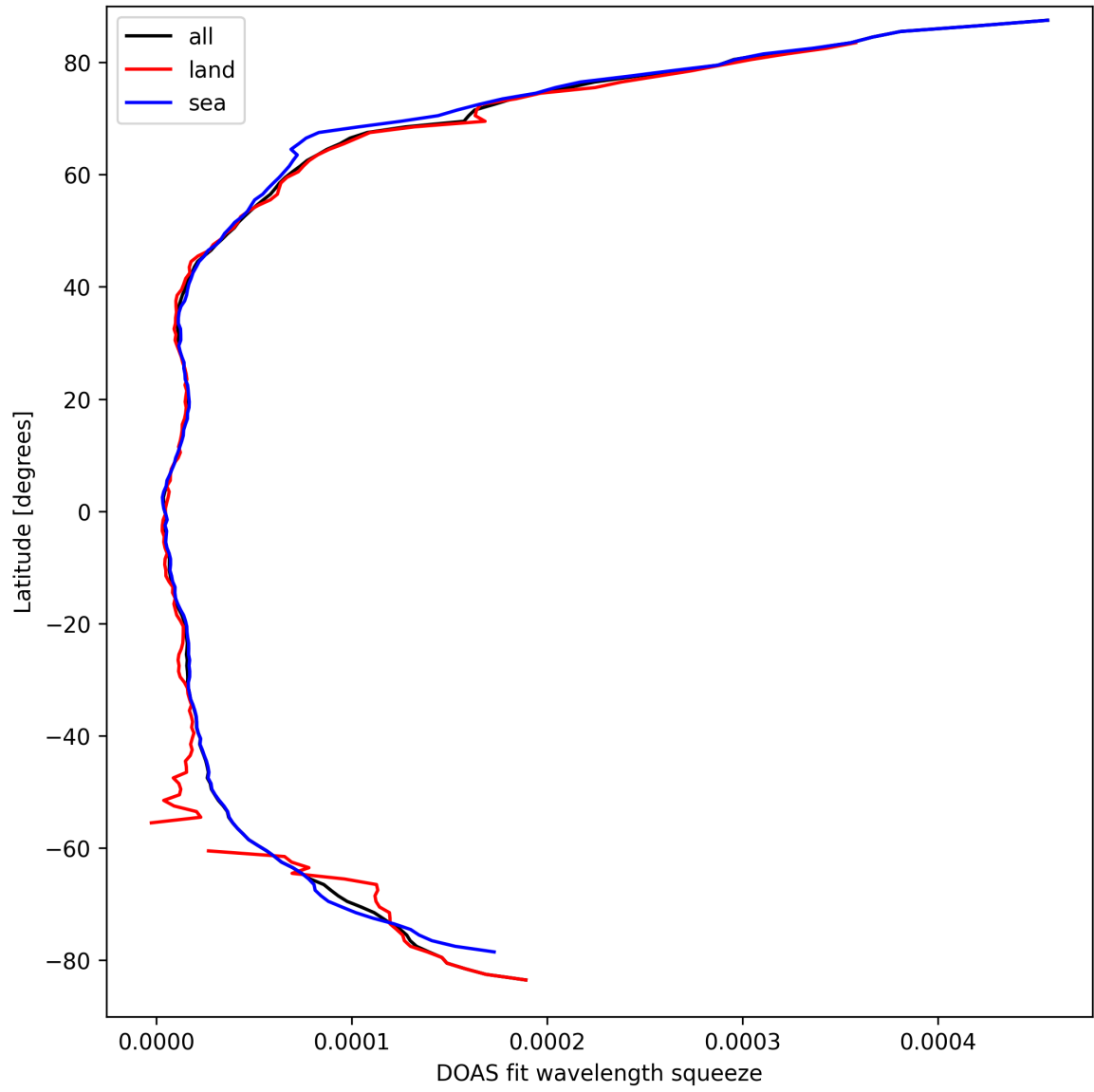
Figure 29: Zonal average of “DOAS fit wavelength squeeze” for 2025-03-25 to 2025-03-26.
