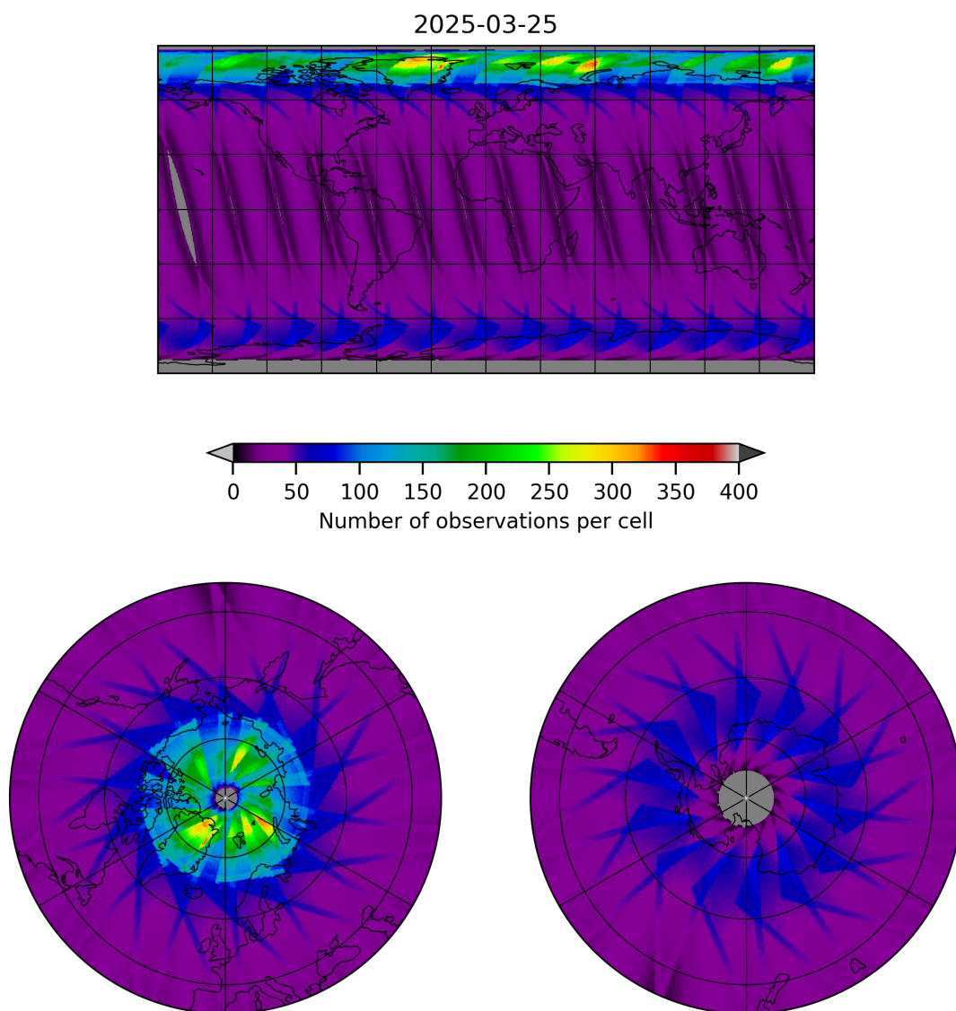
Figure 17: Map of the number of observations for 2025-03-25 to 2025-03-26
