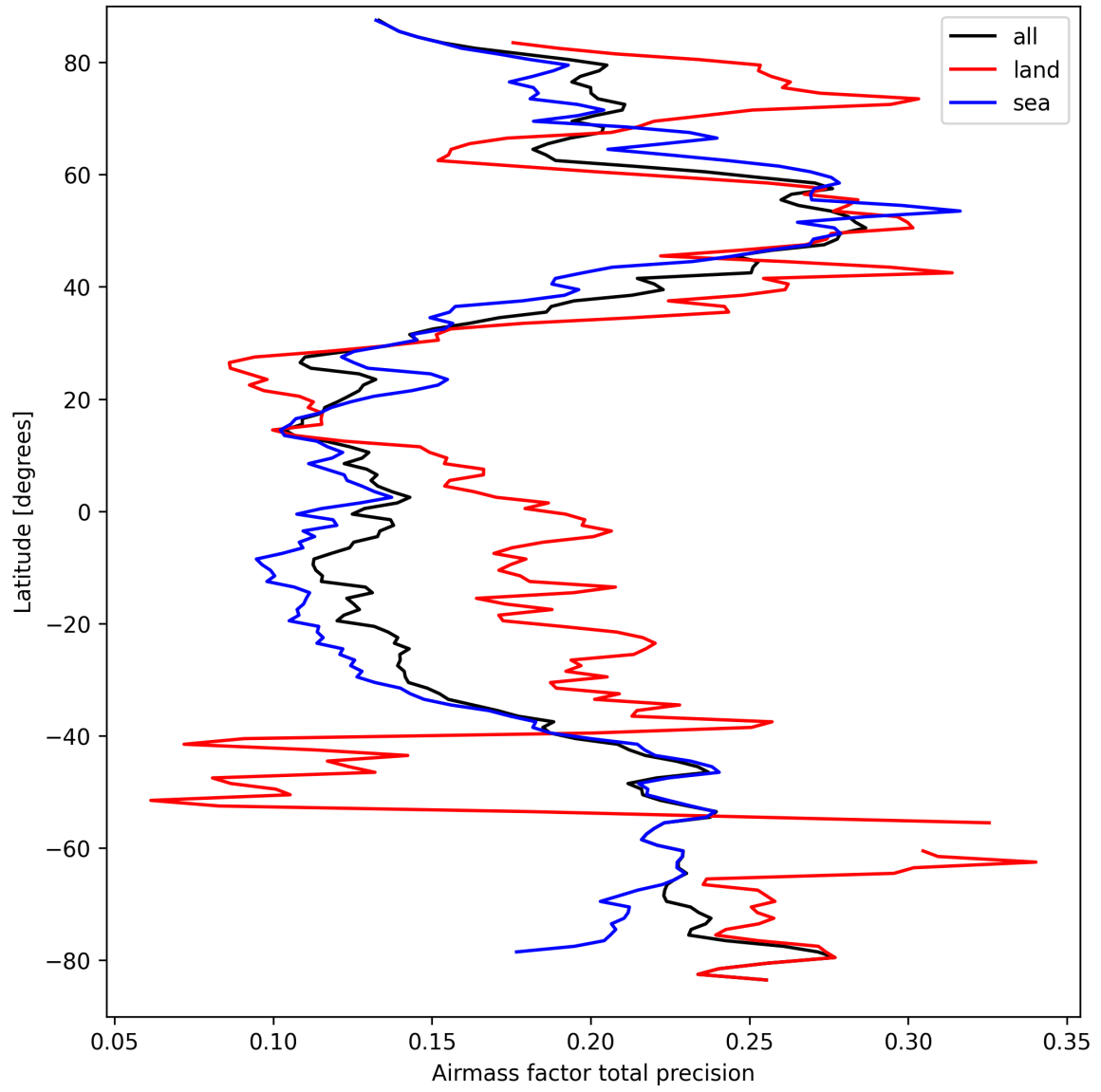
Figure 25: Zonal average of “Airmass factor total precision” for 2025-03-25 to 2025-03-26.
