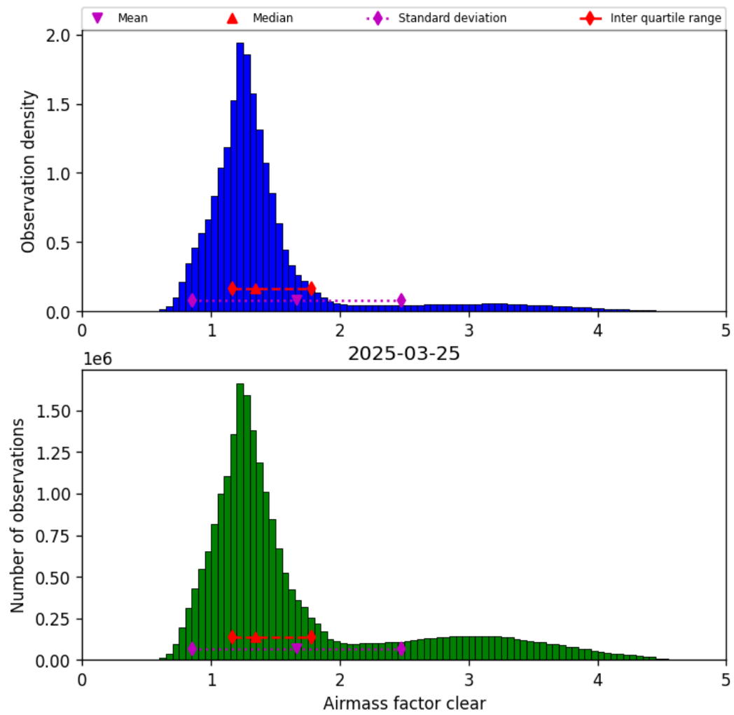
Figure 40: Histogram of “Airmass factor clear” for 2025-03-25 to 2025-03-26
