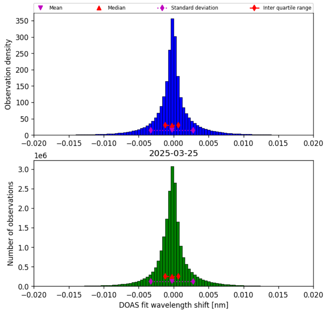
Figure 42: Histogram of “DOAS fit wavelength shift” for 2025-03-25 to 2025-03-26
