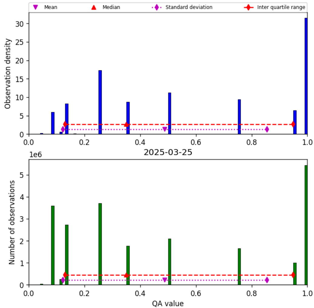
Figure 32: Histogram of “QA value” for 2025-03-25 to 2025-03-26
