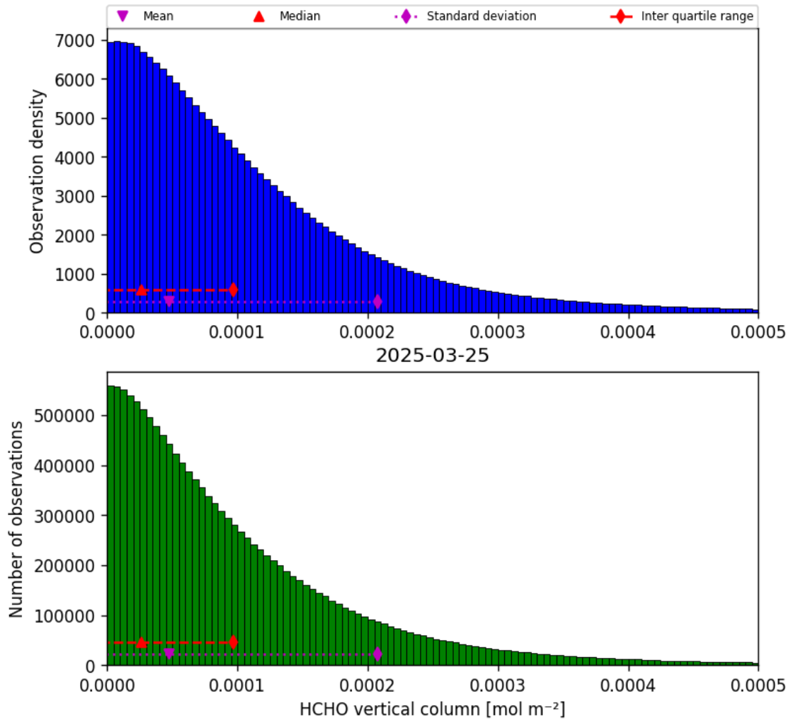
Figure 33: Histogram of “HCHO vertical column” for 2025-03-25 to 2025-03-26
