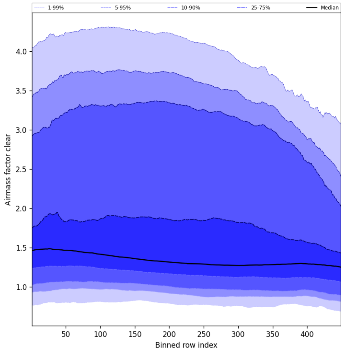
Figure 54: Along track statistics of “Air mass factor clear” for 2025-03-25 to 2025-03-26
