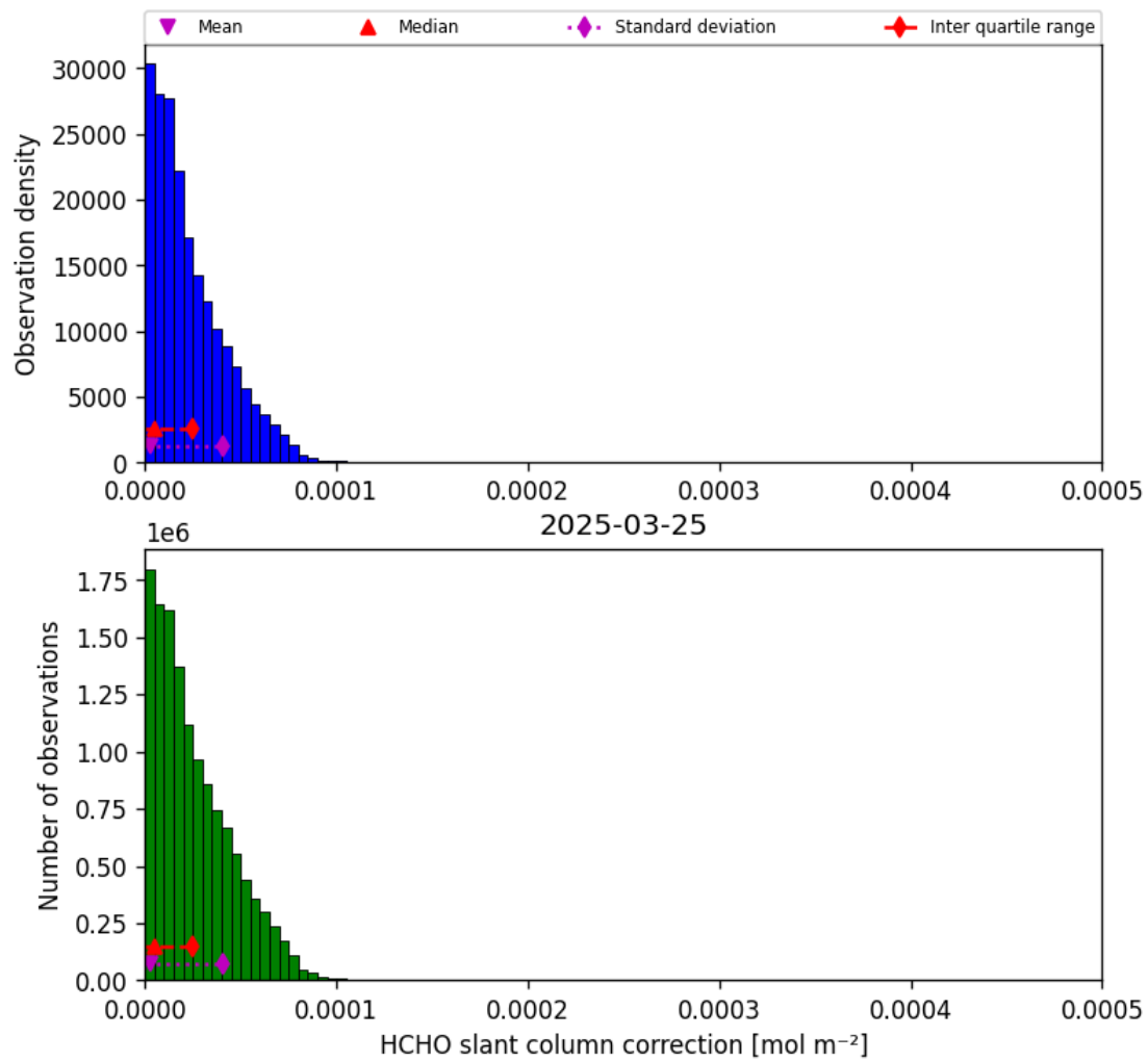
Figure 45: Histogram of “HCHO slant column correction” for 2025-03-25 to 2025-03-26
