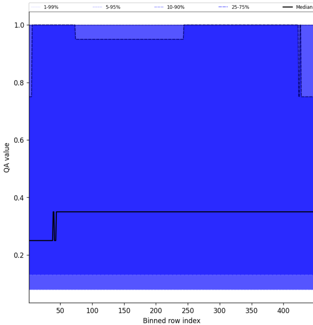
Figure 46: Along track statistics of “QA value” for 2025-03-25 to 2025-03-26
