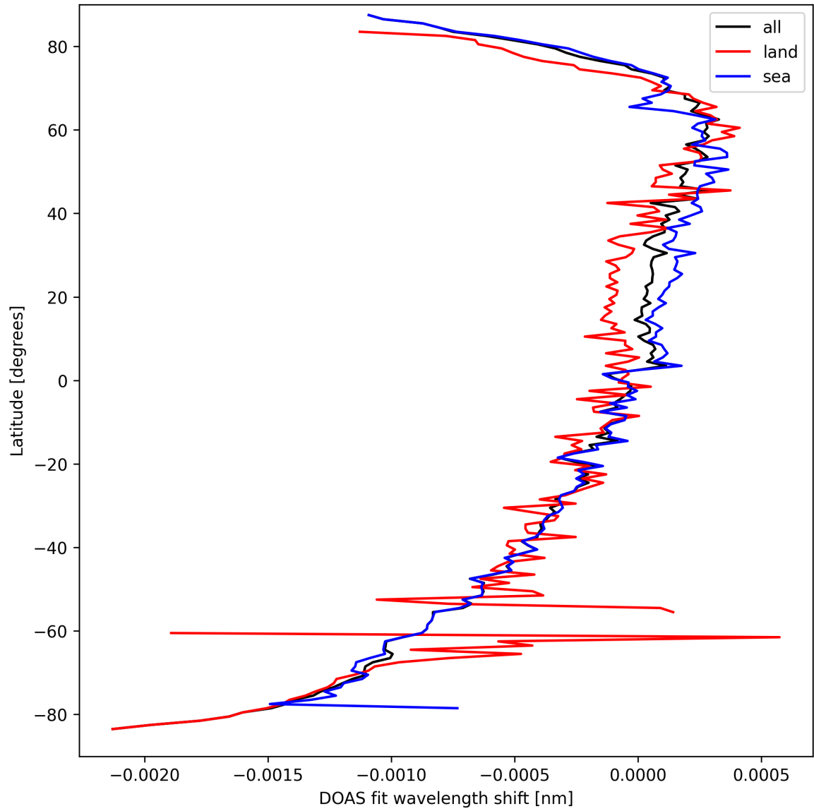
Figure 28: Zonal average of “DOAS fit wavelength shift” for 2025-03-25 to 2025-03-26.
