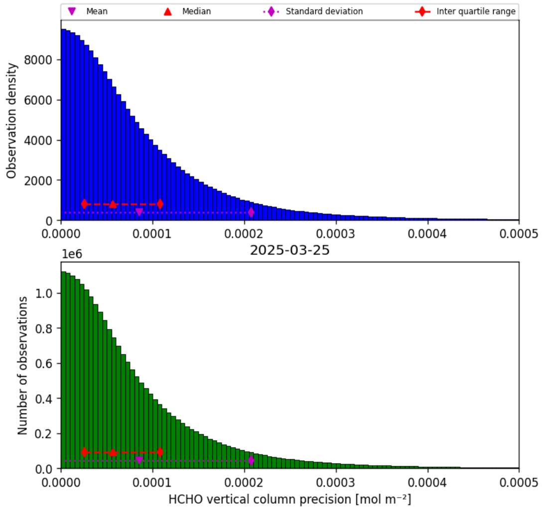
Figure 34: Histogram of “HCHO vertical column precision” for 2025-03-25 to 2025-03-26
