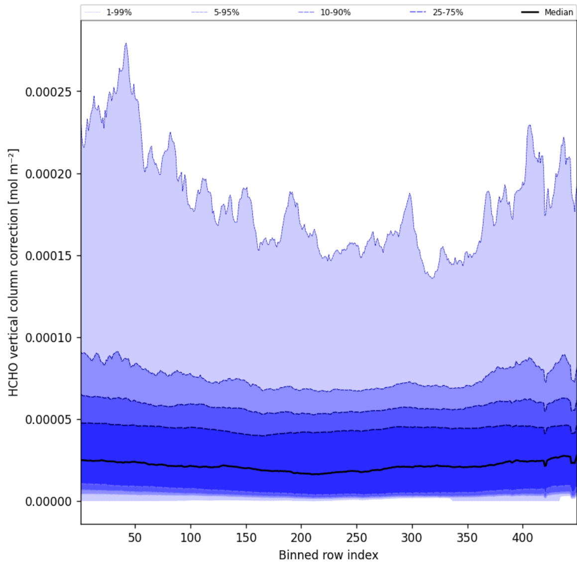
Figure 49: Along track statistics of “HCHO vertical column correction” for 2025-03-26 to 2025-03-26
