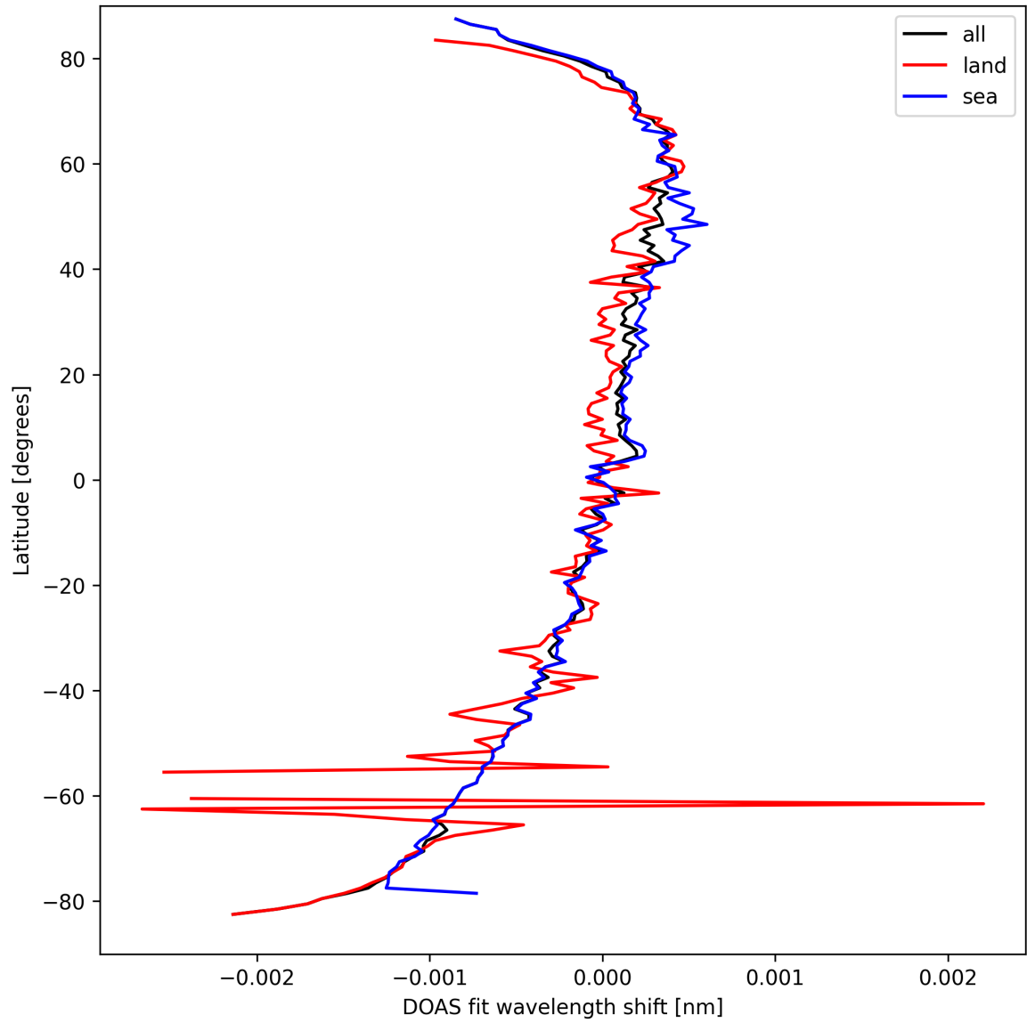
Figure 28: Zonal average of “DOAS fit wavelength shift” for 2025-03-26 to 2025-03-26.
