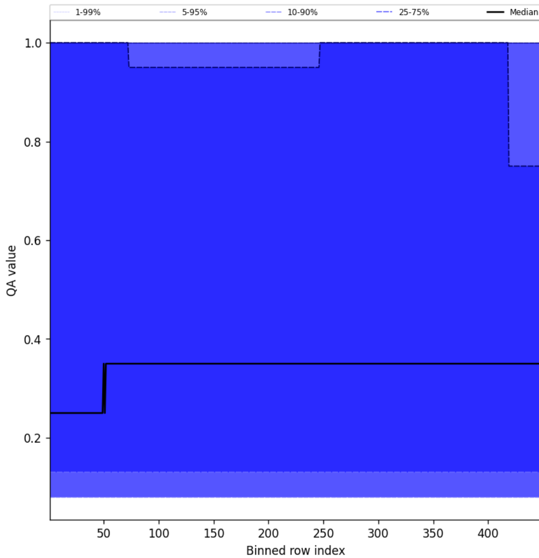
Figure 46: Along track statistics of “QA value” for 2025-03-26 to 2025-03-26
