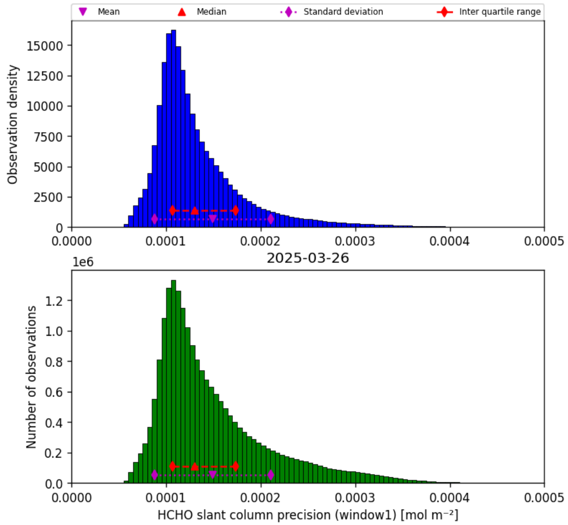
Figure 37: Histogram of “HCHO slant column precision (window1)” for 2025-03-26 to 2025-03-26
