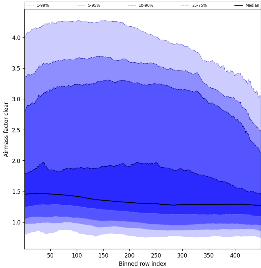
Figure 54: Along track statistics of “Air mass factor clear” for 2025-03-26 to 2025-03-26
