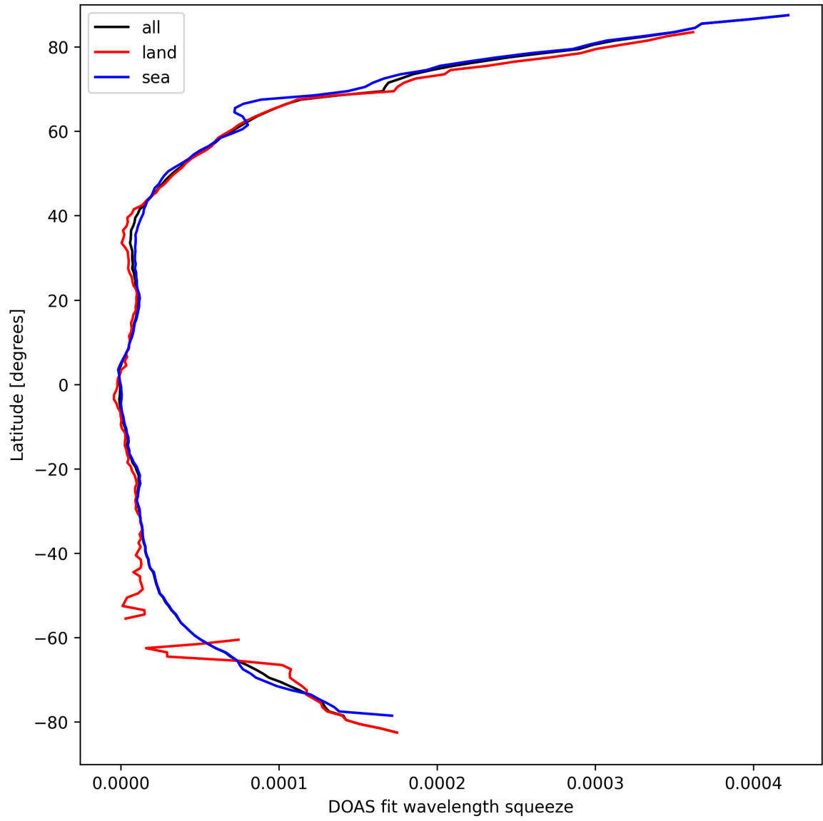
Figure 29: Zonal average of “DOAS fit wavelength squeeze” for 2025-03-26 to 2025-03-26.
