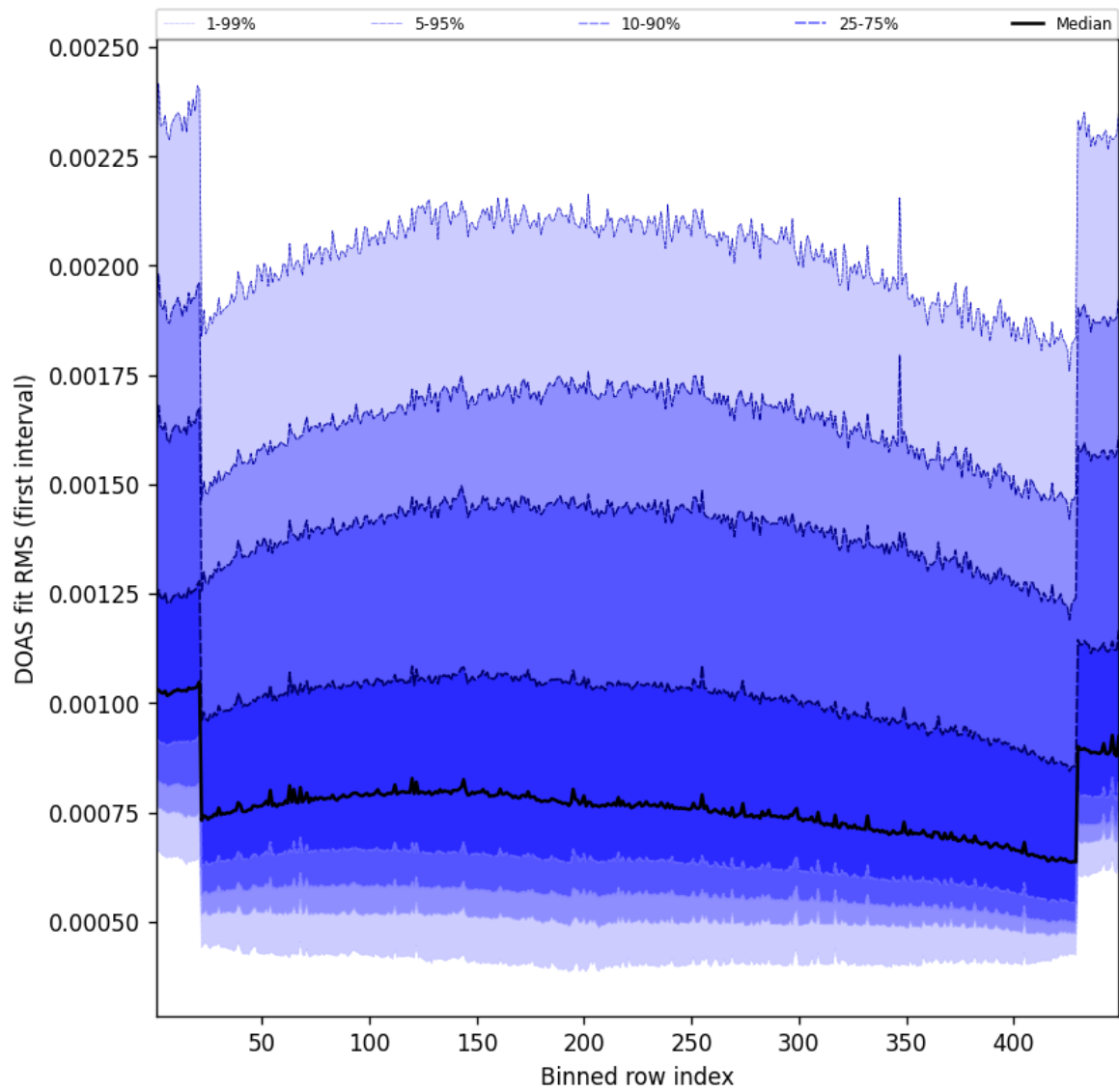
Figure 58: Along track statistics of “DOAS fit RMS (first interval)” for 2025-03-26 to 2025-03-26
