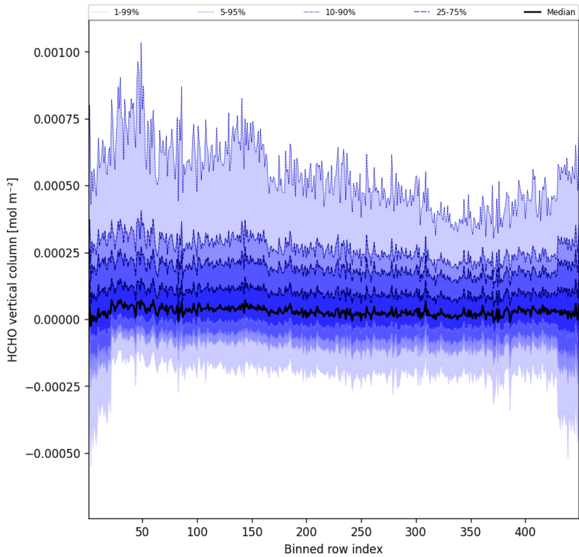
Figure 47: Along track statistics of “HCHO vertical column” for 2025-03-26 to 2025-03-26
