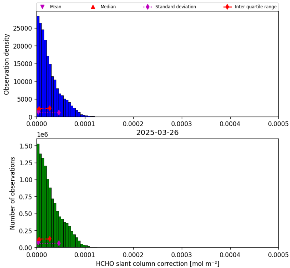
Figure 45: Histogram of “HCHO slant column correction” for 2025-03-26 to 2025-03-26
