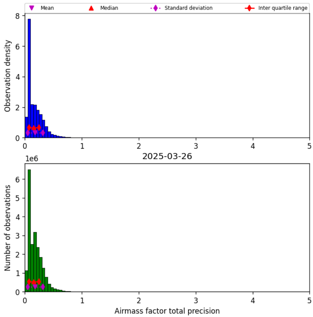
Figure 39: Histogram of “Airmass factor total precision” for 2025-03-26 to 2025-03-26
