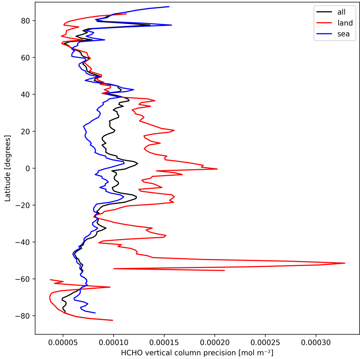
Figure 20: Zonal average of “HCHO vertical column precision” for 2025-03-26 to 2025-03-26.
