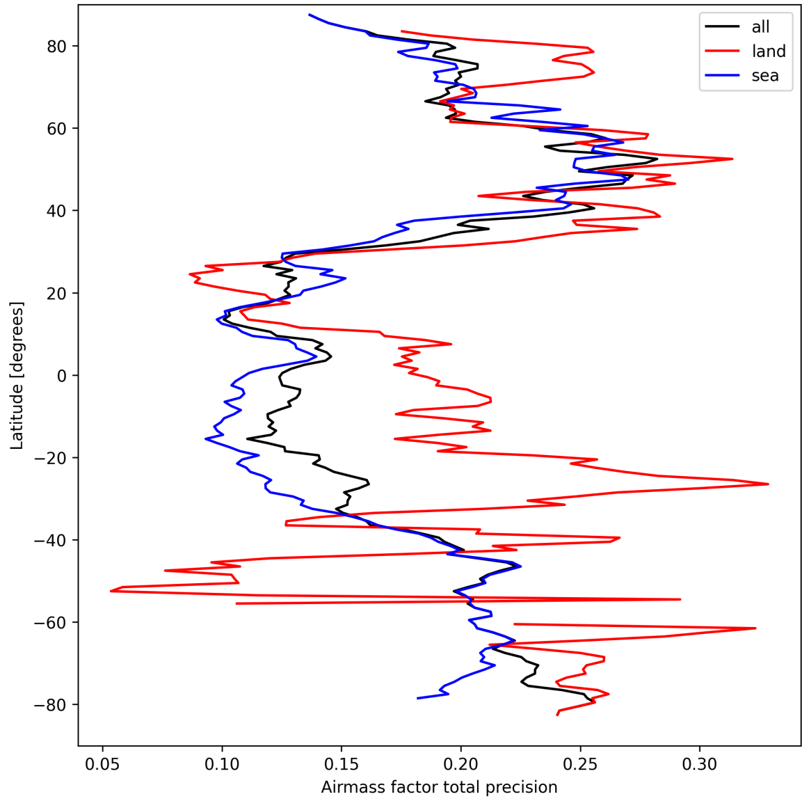
Figure 25: Zonal average of “Airmass factor total precision” for 2025-03-26 to 2025-03-26.
