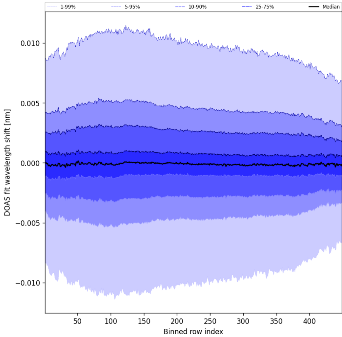
Figure 56: Along track statistics of “DOAS fit wavelength shift” for 2025-03-26 to 2025-03-26
