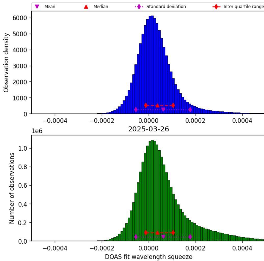
Figure 43: Histogram of “DOAS fit wavelength squeeze” for 2025-03-26 to 2025-03-26
