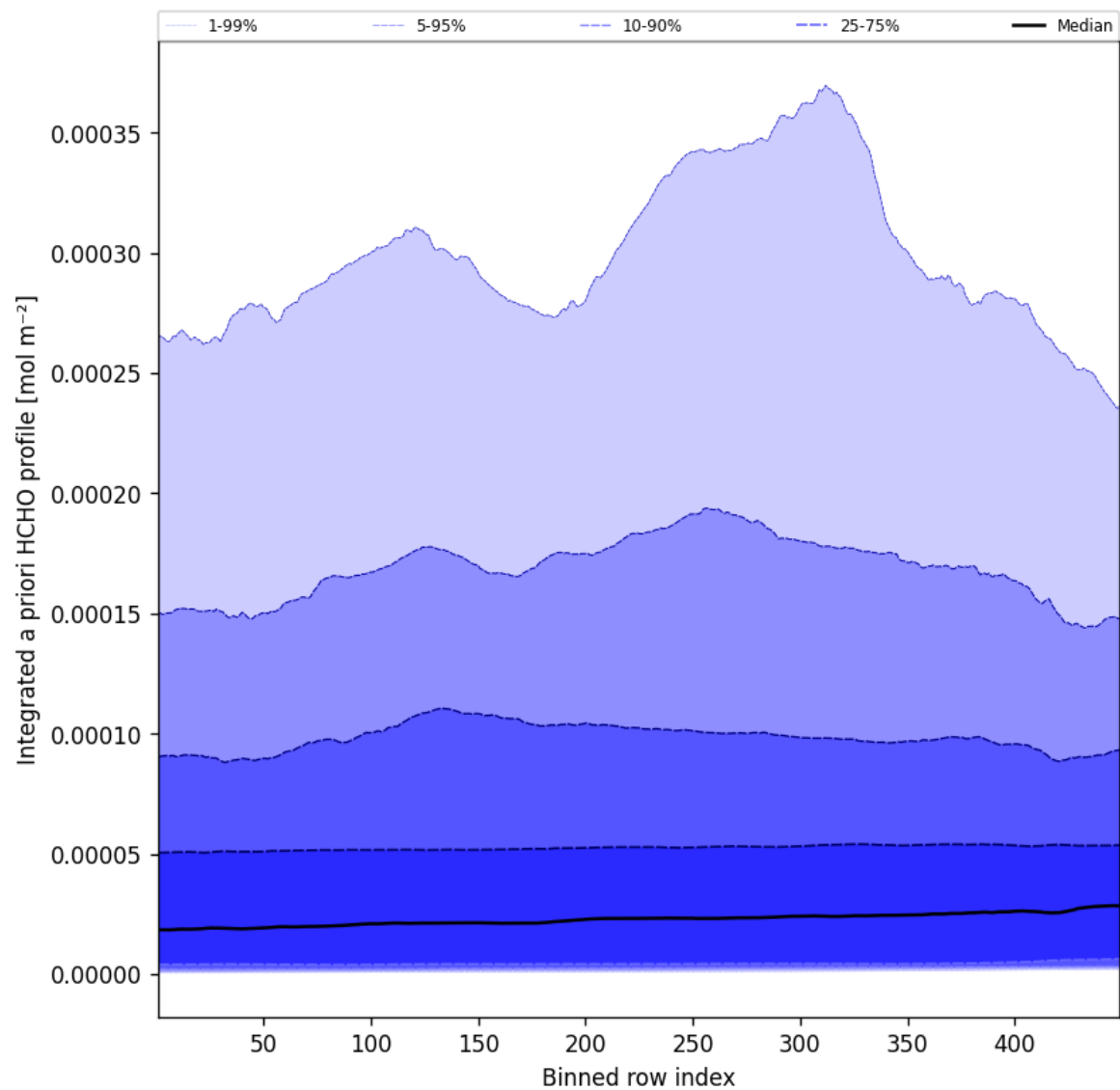
Figure 55: Along track statistics of “Integrated a priori HCHO profile” for 2025-03-26 to 2025-03-26
