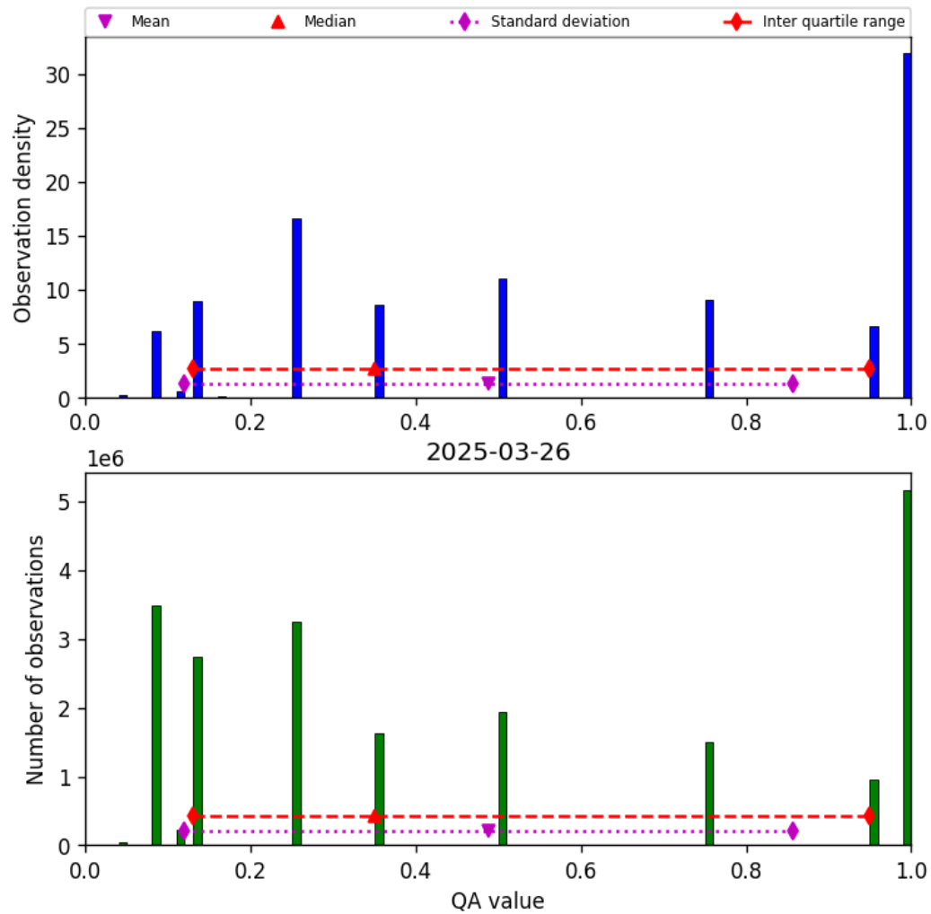
Figure 32: Histogram of “QA value” for 2025-03-26 to 2025-03-26
