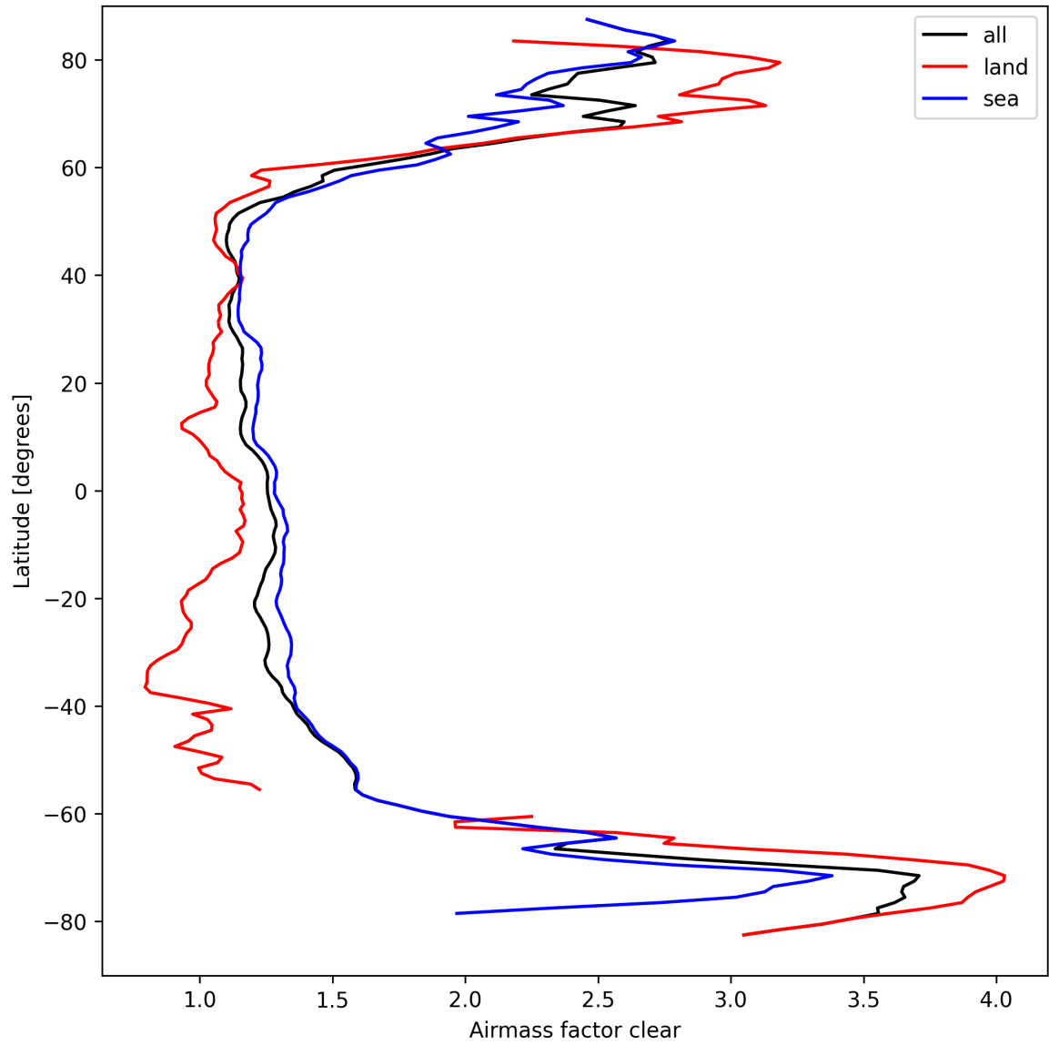
Figure 26: Zonal average of “Airmass factor clear” for 2025-03-26 to 2025-03-26.
