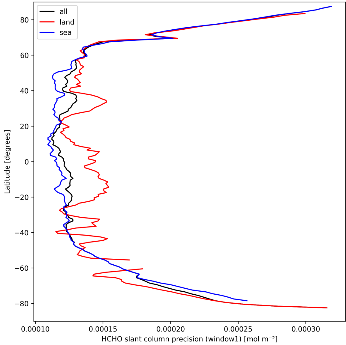
Figure 23: Zonal average of “HCHO slant column precision (window1)” for 2025-03-26 to 2025-03-26.
