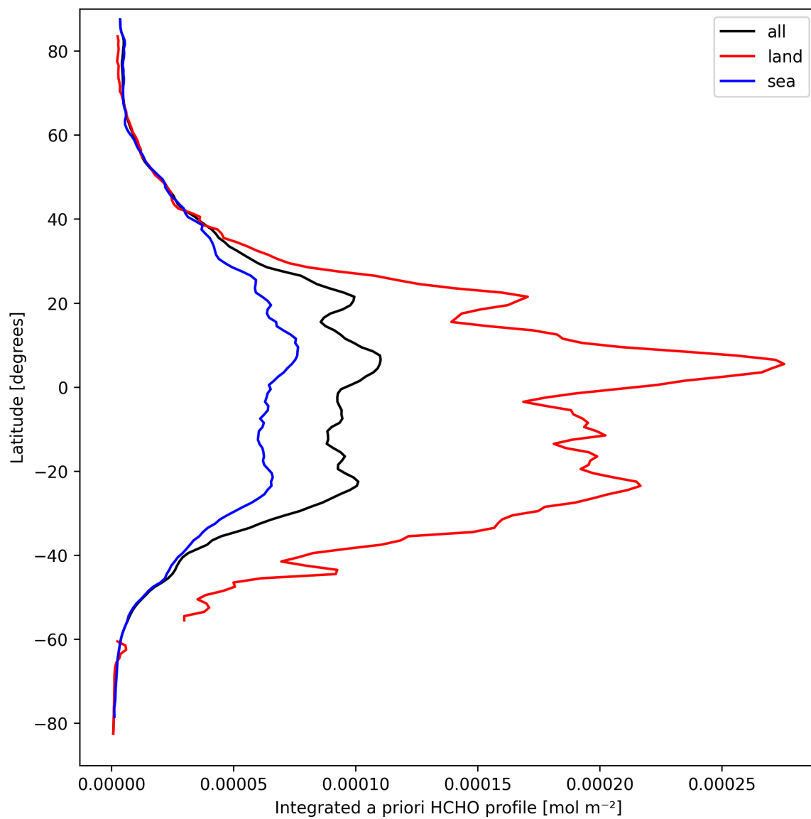
Figure 27: Zonal average of “Integrated a priori HCHO profile” for 2025-03-26 to 2025-03-26.
