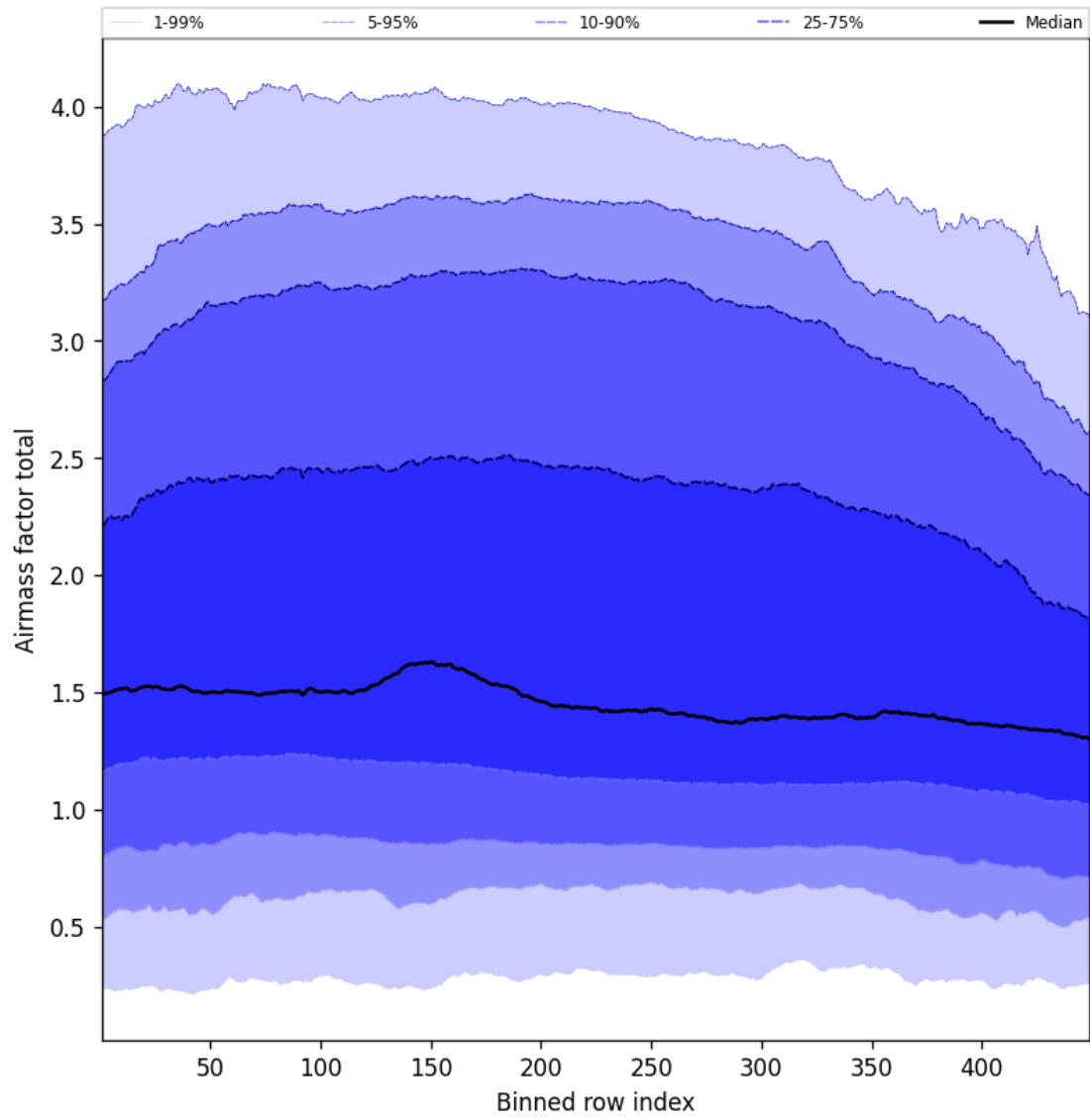
Figure 52: Along track statistics of “Airmass factor total” for 2025-03-26 to 2025-03-26
