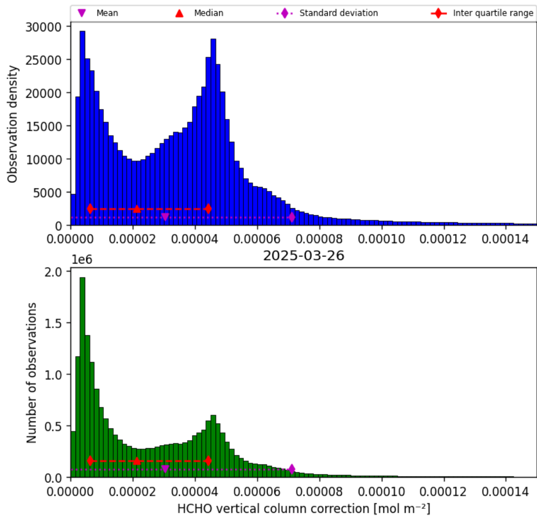
Figure 35: Histogram of “HCHO vertical column correction” for 2025-03-26 to 2025-03-26
