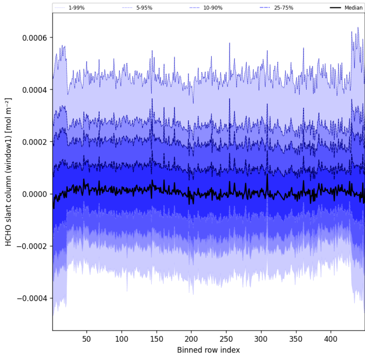
Figure 50: Along track statistics of “HCHO slant column (window1)” for 2025-03-26 to 2025-03-26
