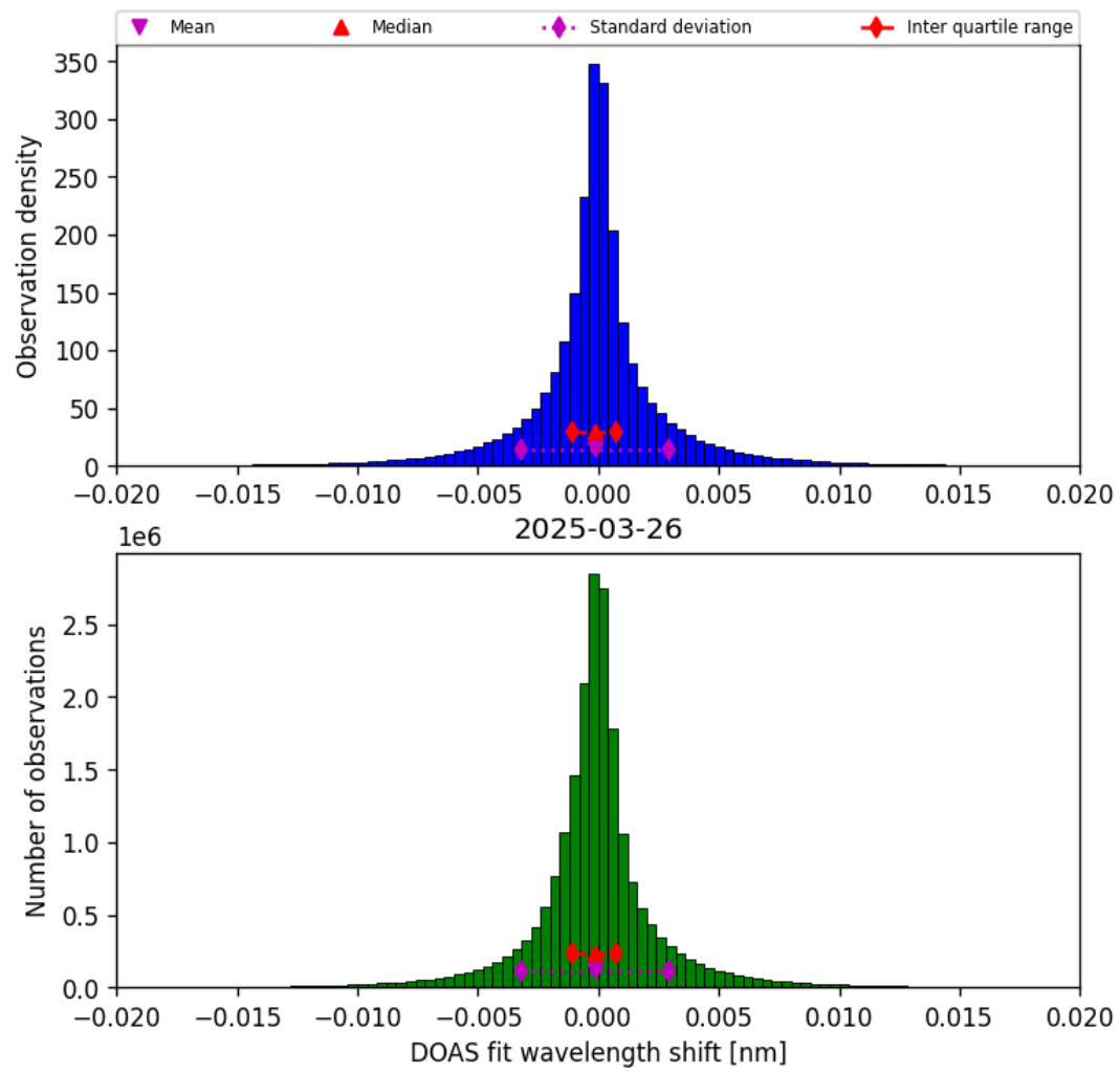
Figure 42: Histogram of “DOAS fit wavelength shift” for 2025-03-26 to 2025-03-26
