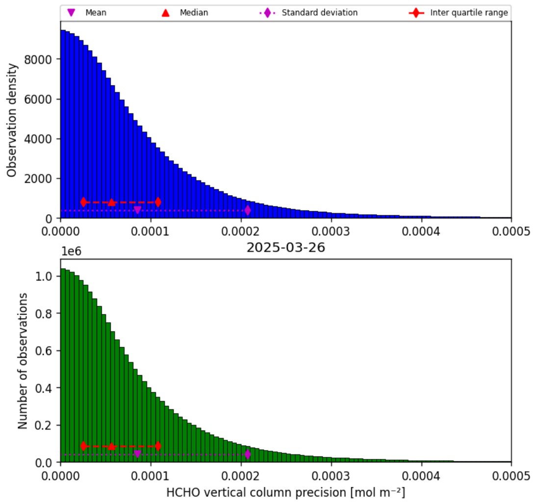
Figure 34: Histogram of “HCHO vertical column precision” for 2025-03-26 to 2025-03-26
