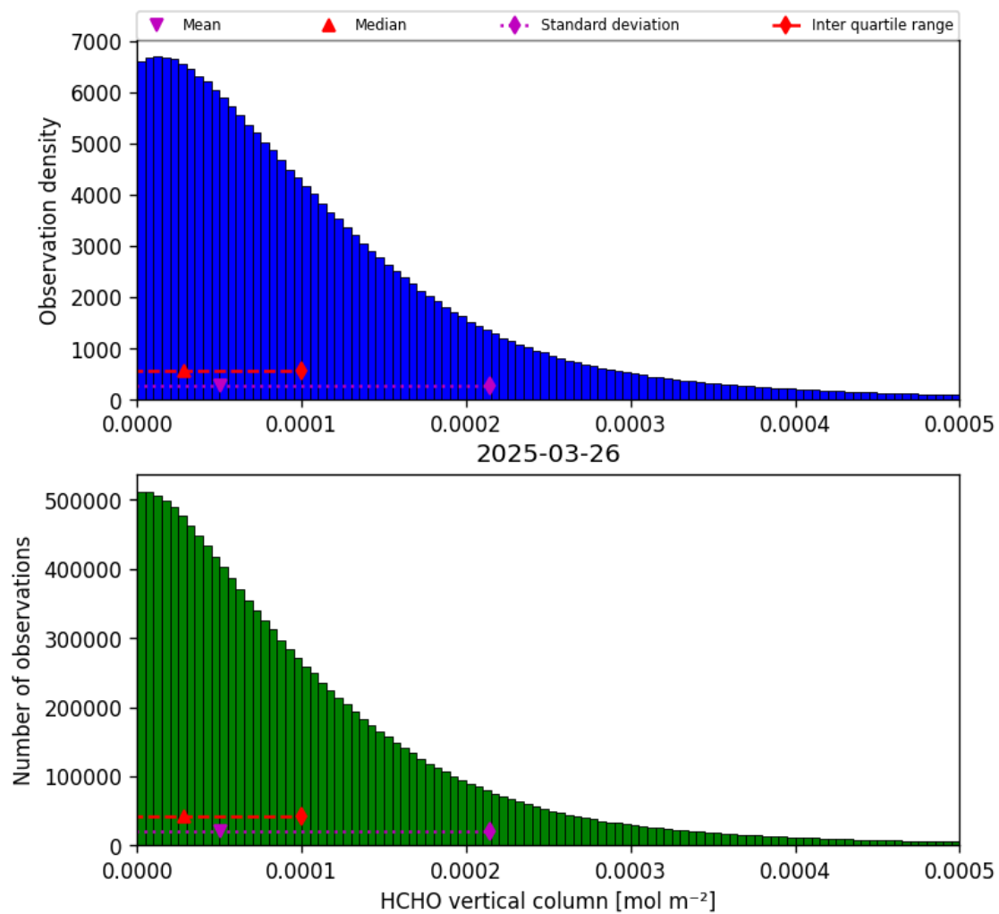
Figure 33: Histogram of “HCHO vertical column” for 2025-03-26 to 2025-03-26
