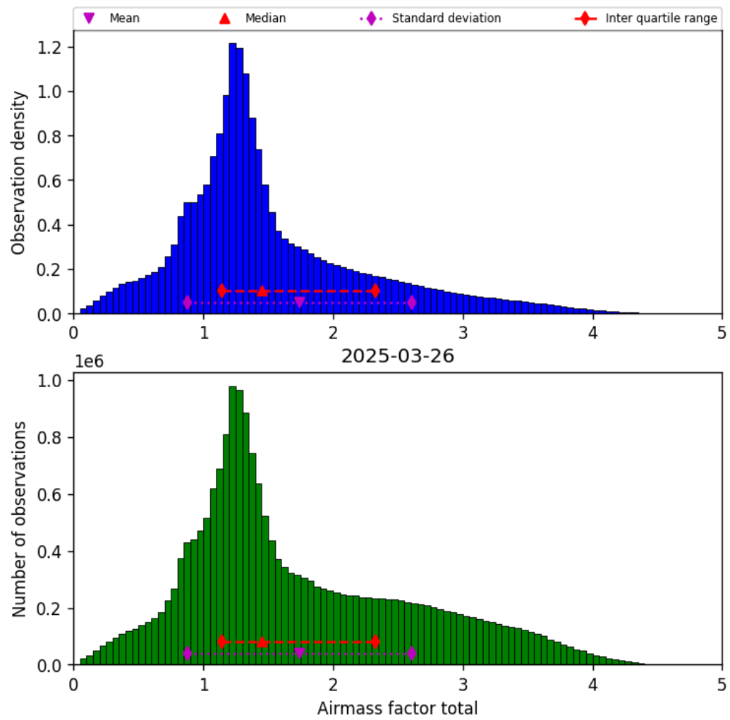
Figure 38: Histogram of “Airmass factor total” for 2025-03-26 to 2025-03-26
