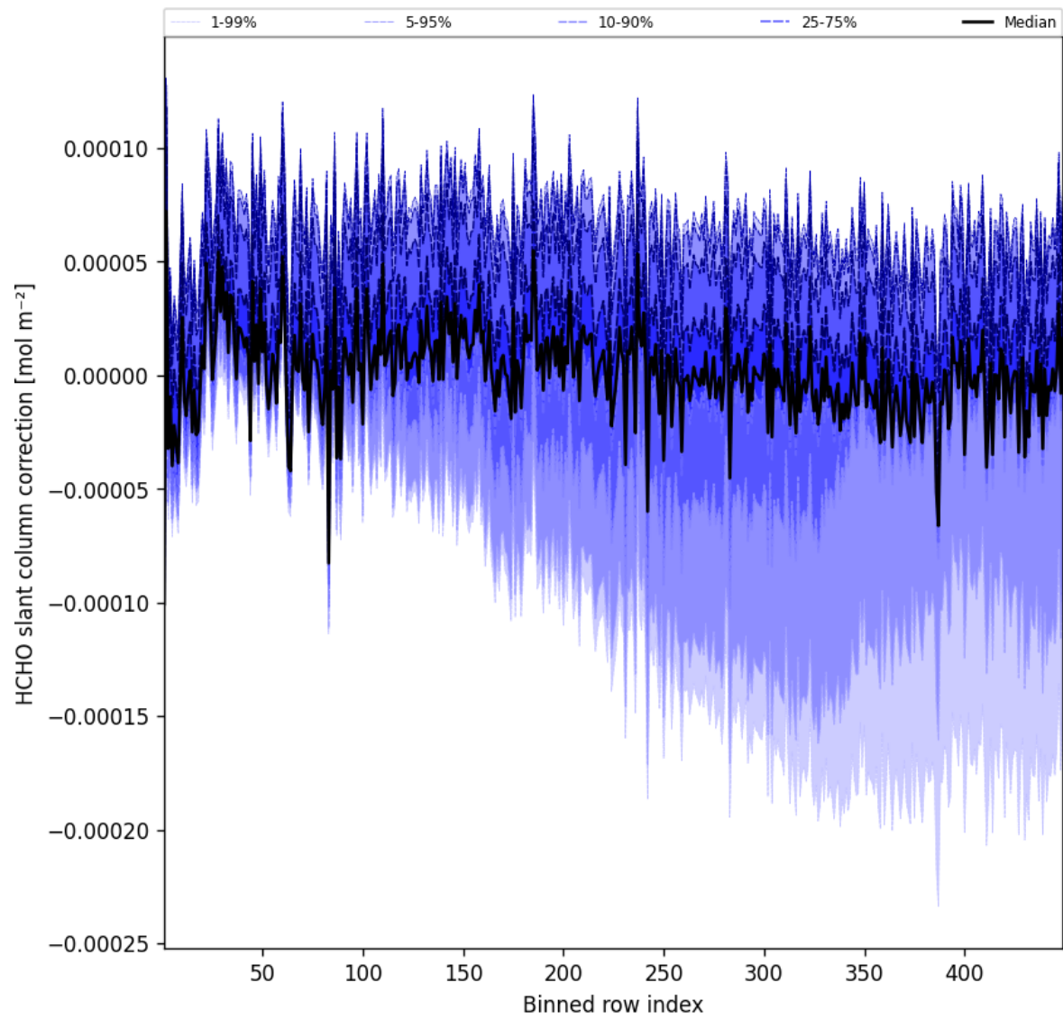
Figure 59: Along track statistics of “HCHO slant column correction” for 2025-03-26 to 2025-03-26
