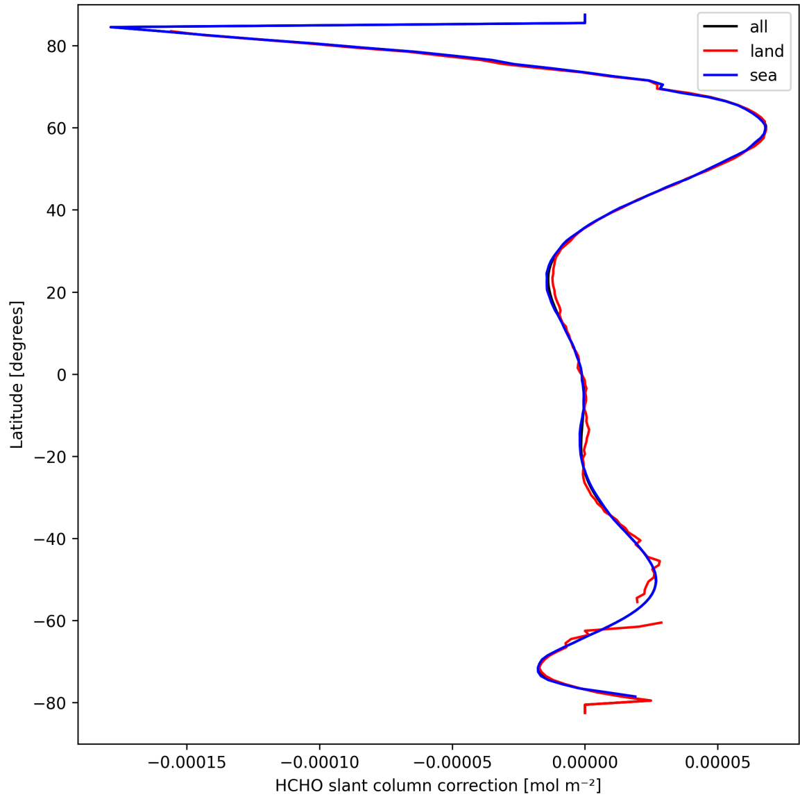
Figure 31: Zonal average of “HCHO slant column correction” for 2025-03-26 to 2025-03-26.
