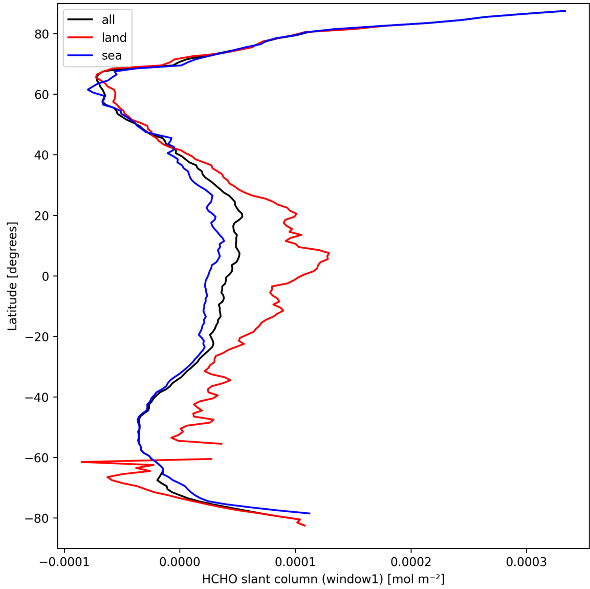
Figure 22: Zonal average of “HCHO slant column (window1)” for 2025-03-26 to 2025-03-26.
