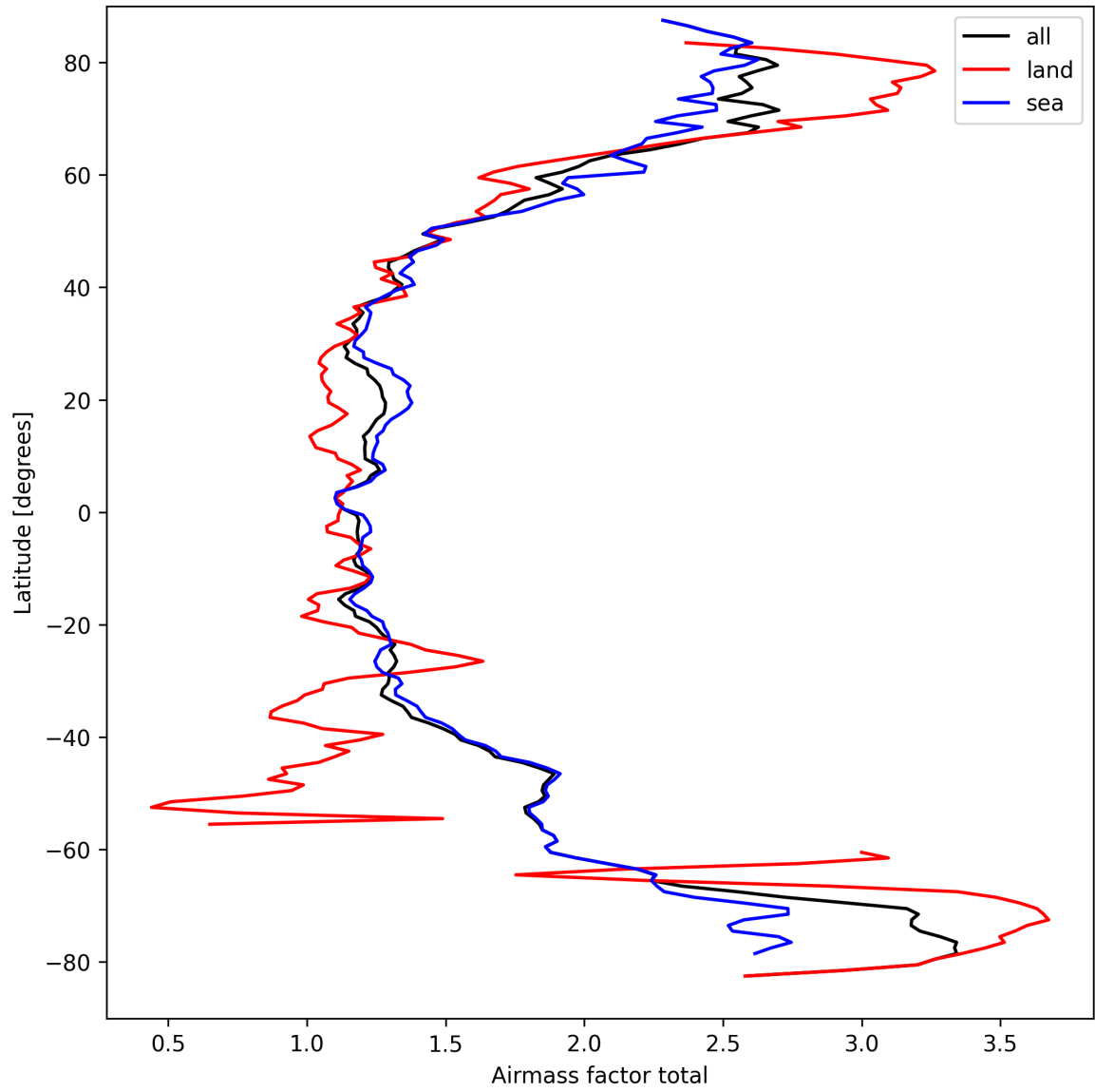
Figure 24: Zonal average of “Airmass factor total” for 2025-03-26 to 2025-03-26.
