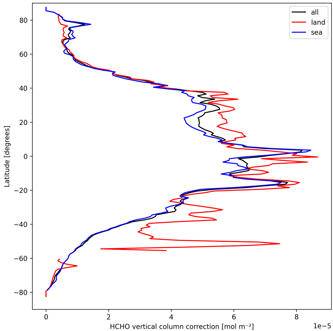
Figure 21: Zonal average of “HCHO vertical column correction” for 2025-03-26 to 2025-03-26.
