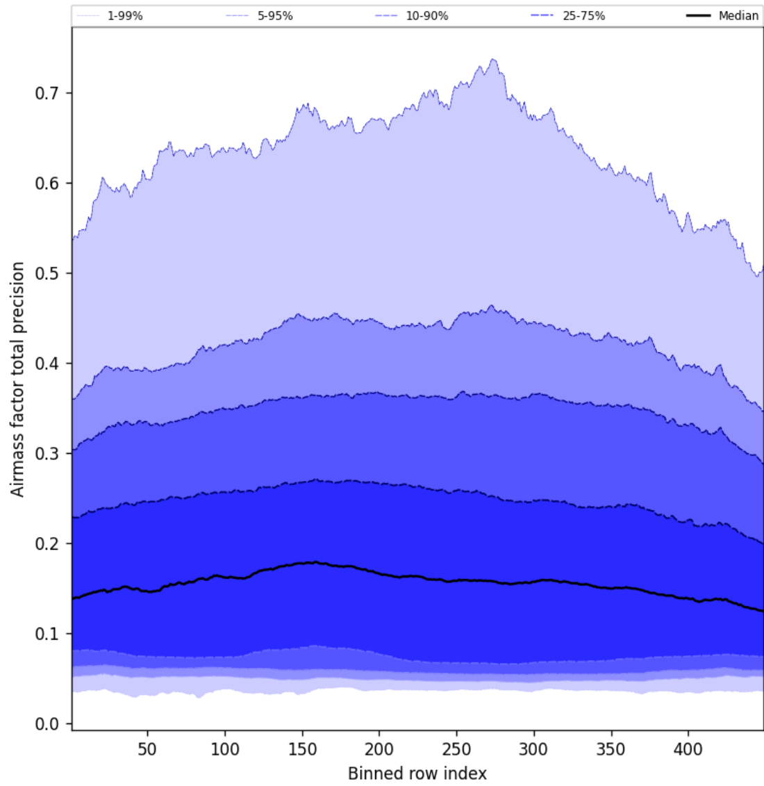
Figure 53: Along track statistics of “Airmass factor total precision” for 2025-03-26 to 2025-03-26
