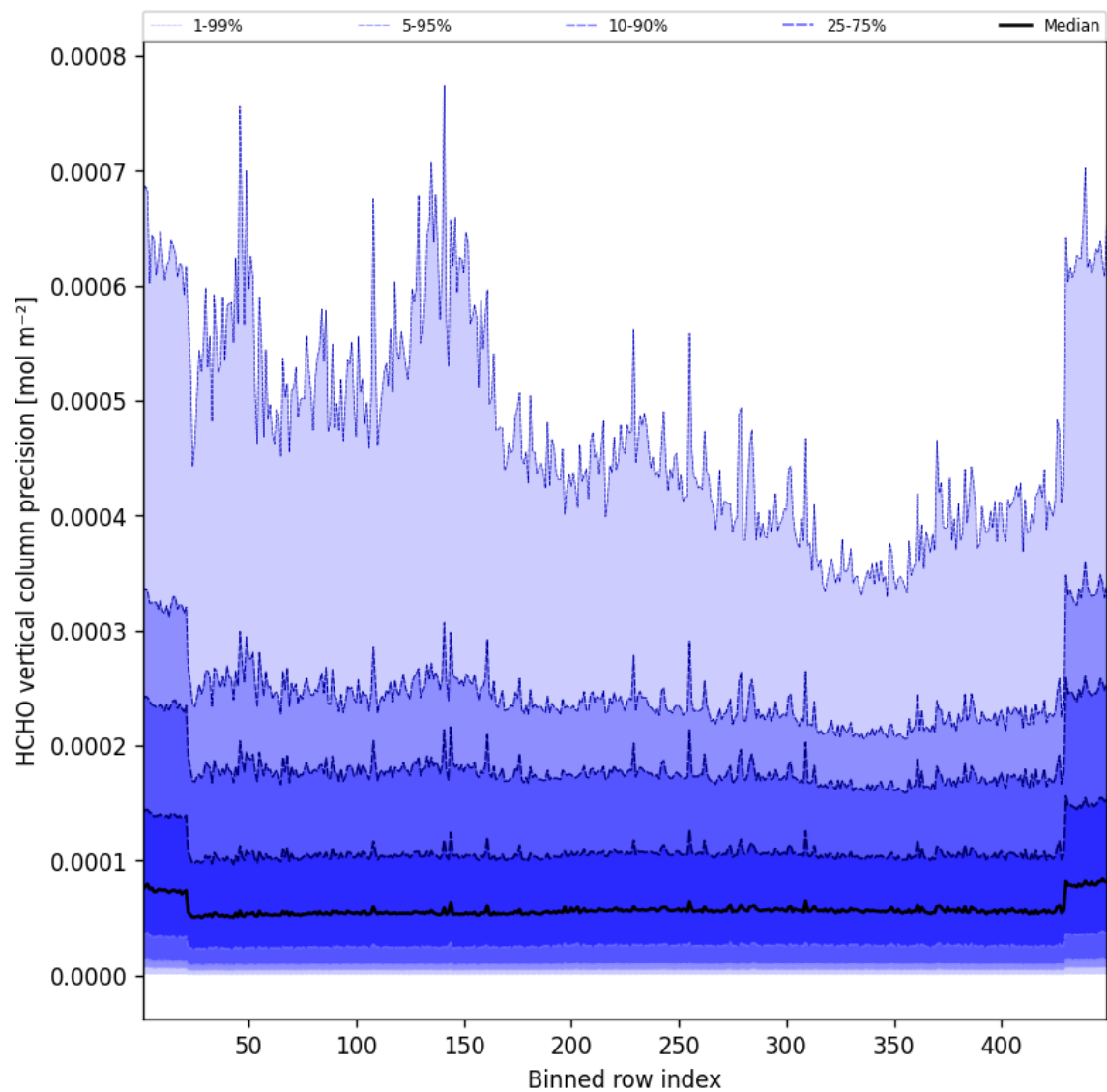
Figure 48: Along track statistics of “HCHO vertical column precision” for 2025-03-26 to 2025-03-26
