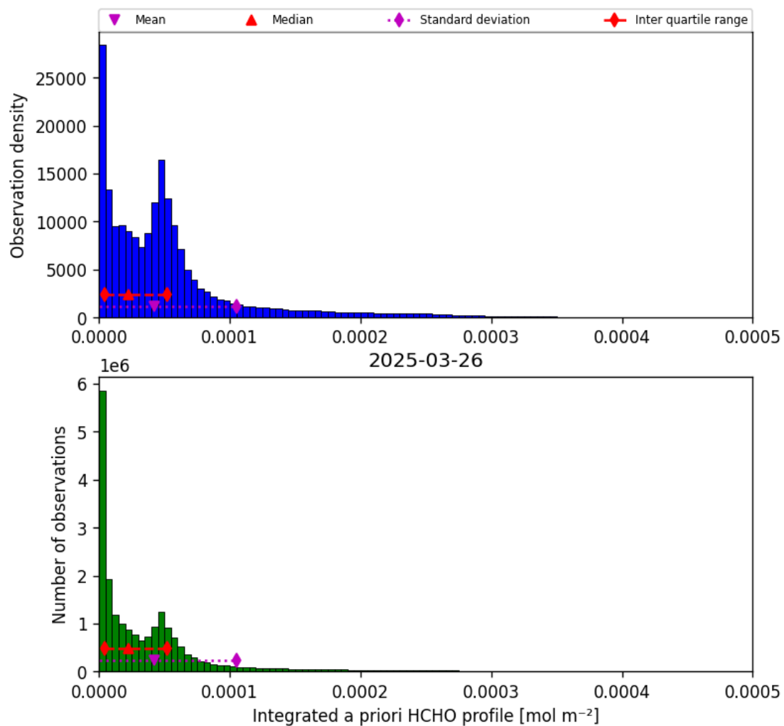
Figure 41: Histogram of “Integrated a priori HCHO profile” for 2025-03-26 to 2025-03-26
