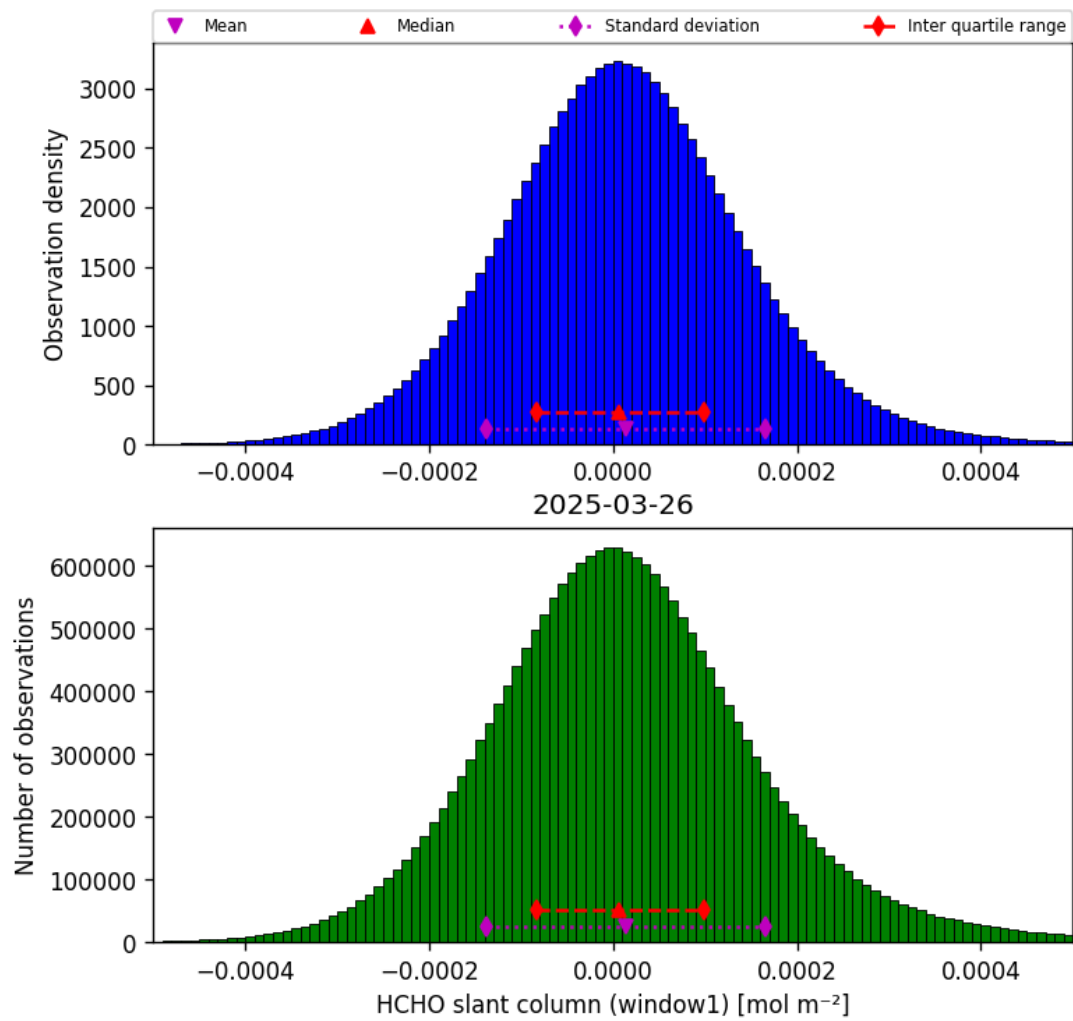
Figure 36: Histogram of “HCHO slant column (window1)” for 2025-03-26 to 2025-03-26
