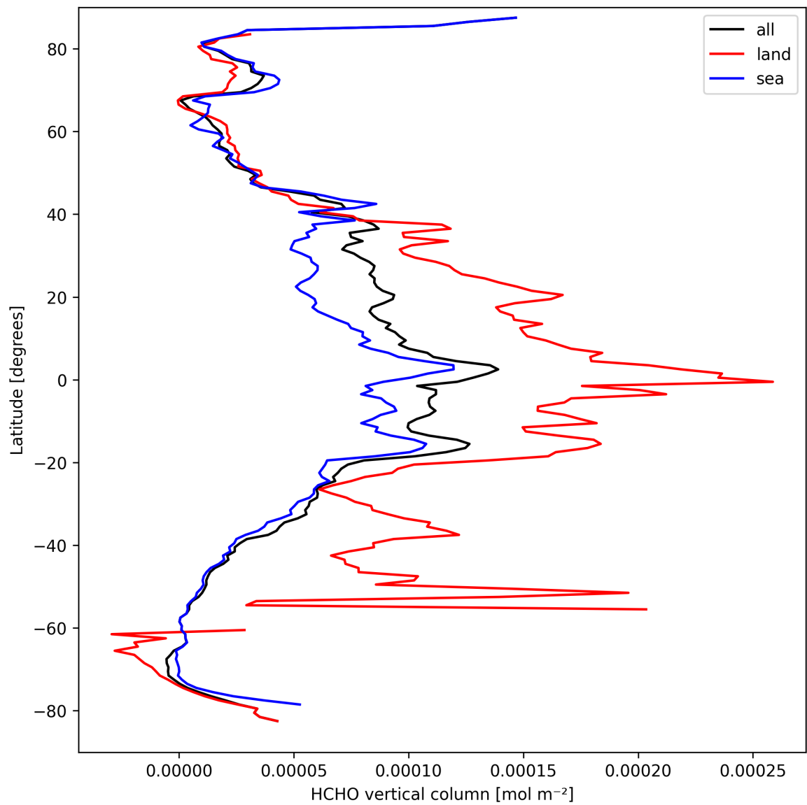
Figure 19: Zonal average of “HCHO vertical column” for 2025-03-26 to 2025-03-26.
