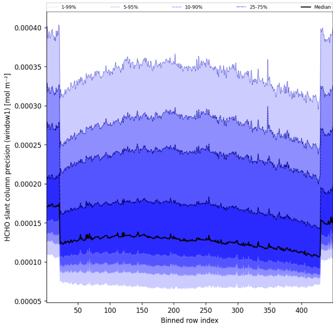
Figure 51: Along track statistics of “HCHO slant column precision (window1)” for 2025-03-26 to 2025-03-26
