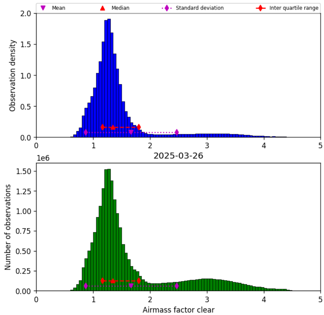
Figure 40: Histogram of “Airmass factor clear” for 2025-03-26 to 2025-03-26
