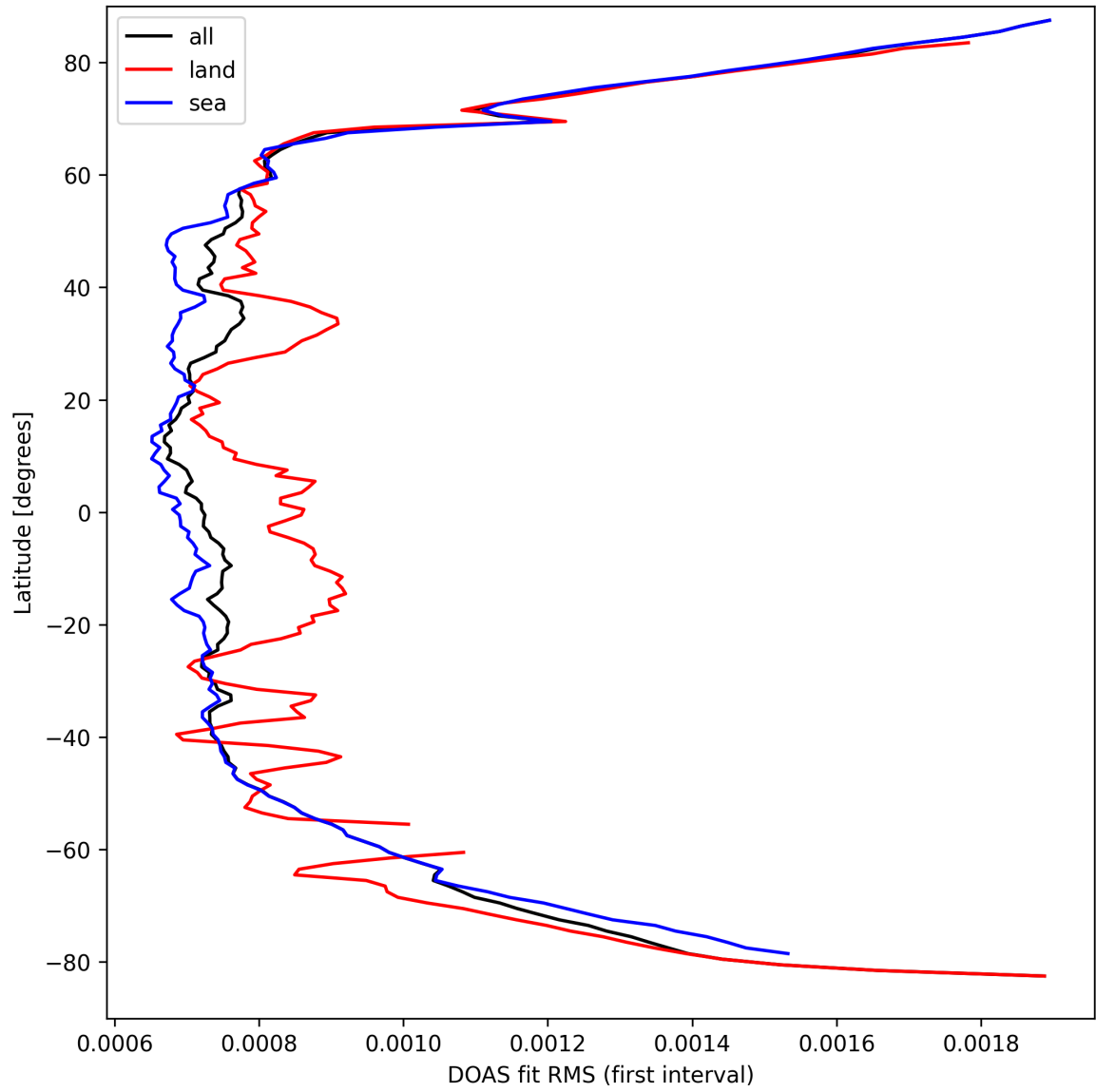
Figure 30: Zonal average of "DOAS fit RMS (first interval)" for 2025-03-26 to 2025-03-26.
