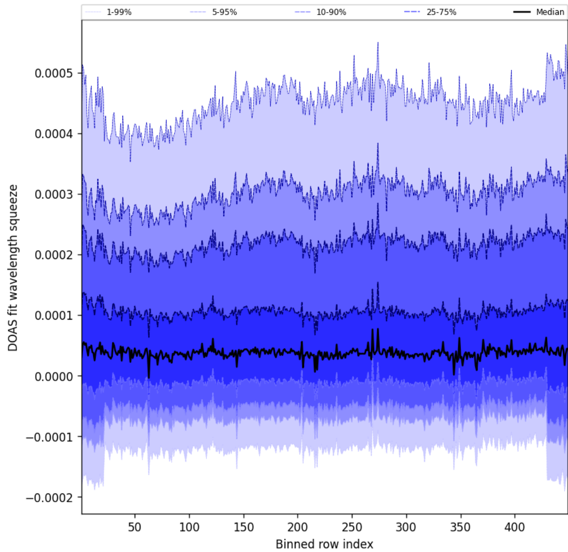
Figure 57: Along track statistics of “DOAS fit wavelength squeeze” for 2025-03-26 to 2025-03-26
