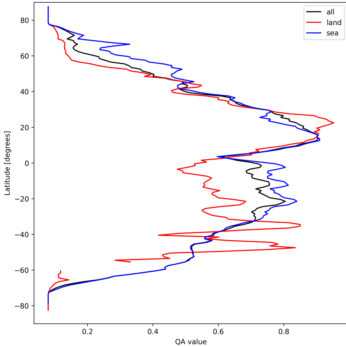
Figure 18: Zonal average of “QA value” for 2025-03-26 to 2025-03-26.
