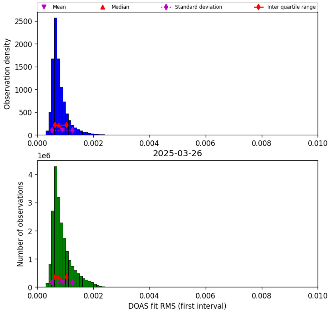
Figure 44: Histogram of “DOAS fit RMS (first interval)” for 2025-03-26 to 2025-03-26
