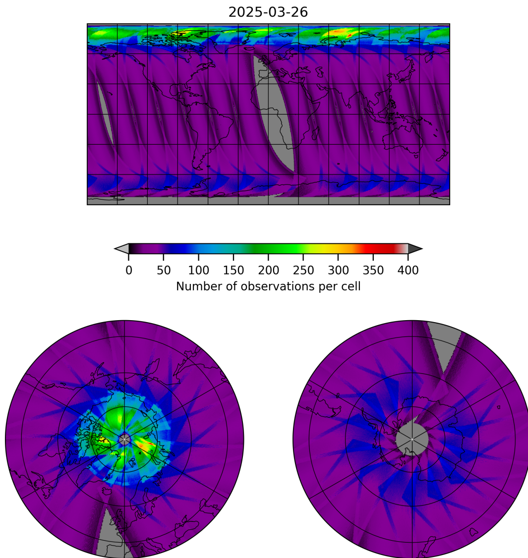
Figure 17: Map of the number of observations for 2025-03-26 to 2025-03-26
