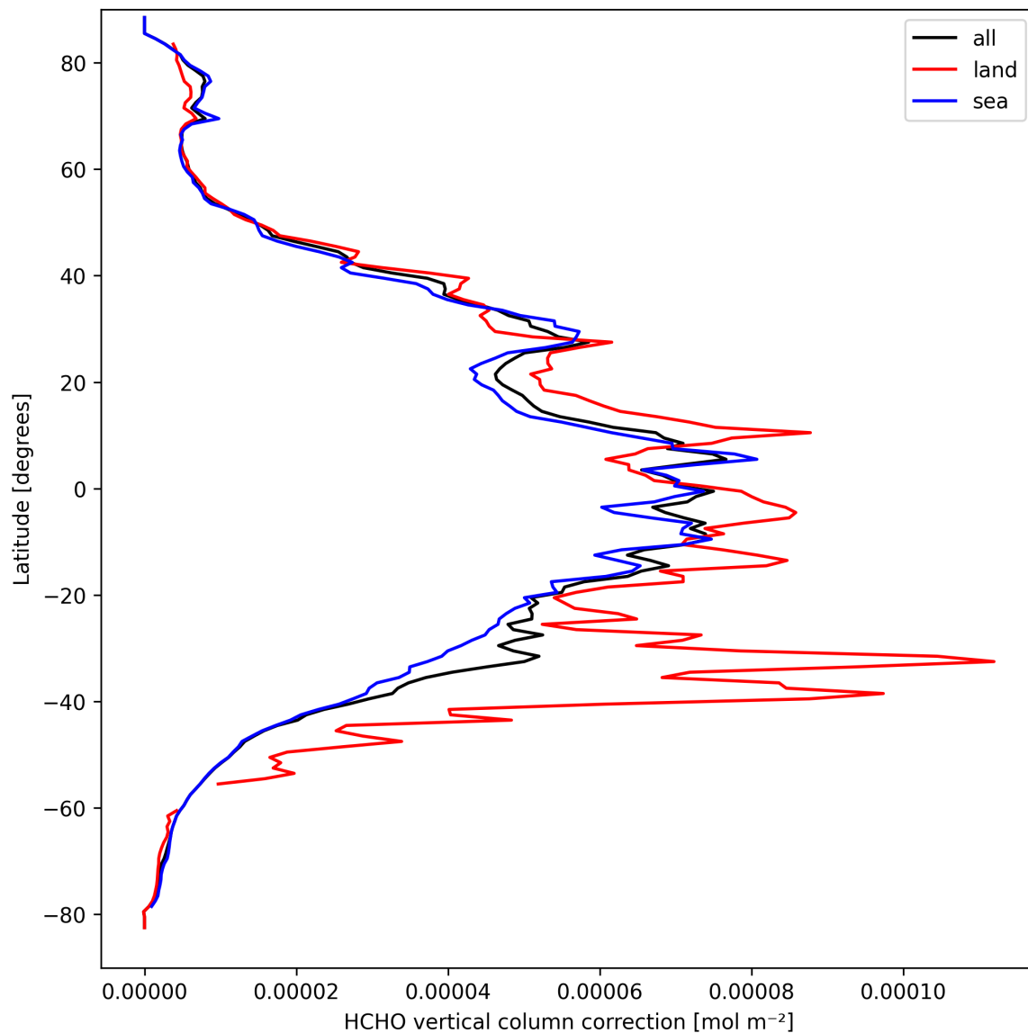
Figure 21: Zonal average of “HCHO vertical column correction” for 2025-03-27 to 2025-03-28.
