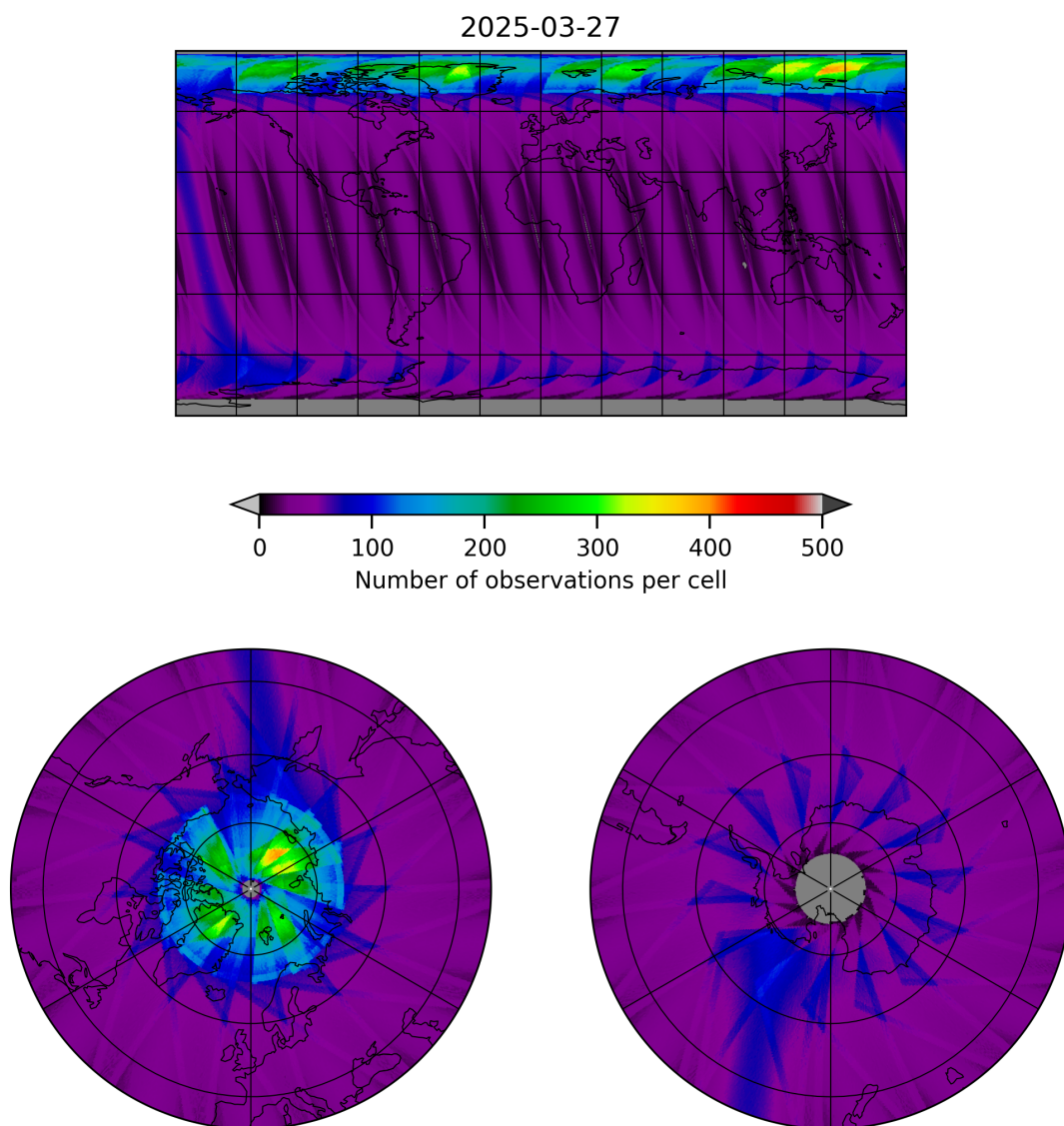
Figure 17: Map of the number of observations for 2025-03-27 to 2025-03-28
