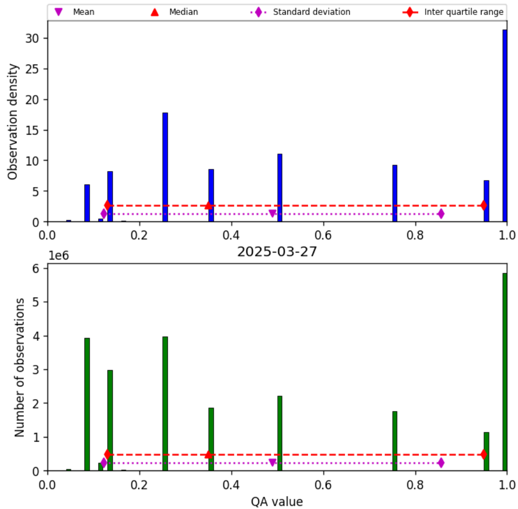
Figure 32: Histogram of “QA value” for 2025-03-27 to 2025-03-28
