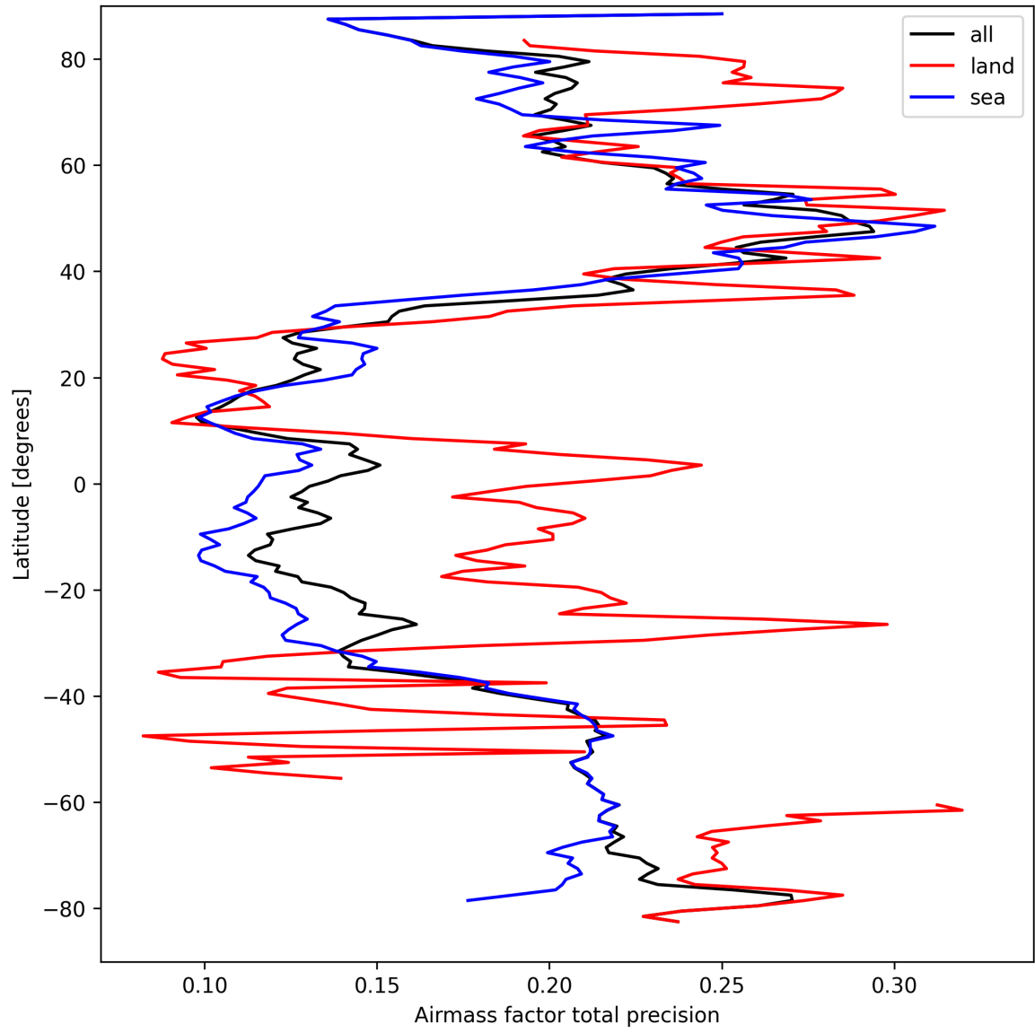
Figure 25: Zonal average of “Airmass factor total precision” for 2025-03-27 to 2025-03-28.
