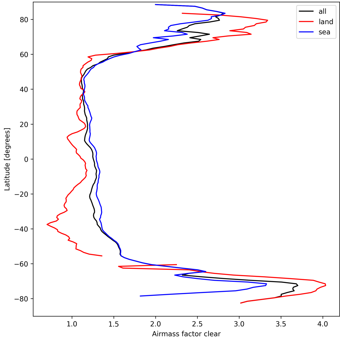
Figure 26: Zonal average of “Airmass factor clear” for 2025-03-27 to 2025-03-28.
