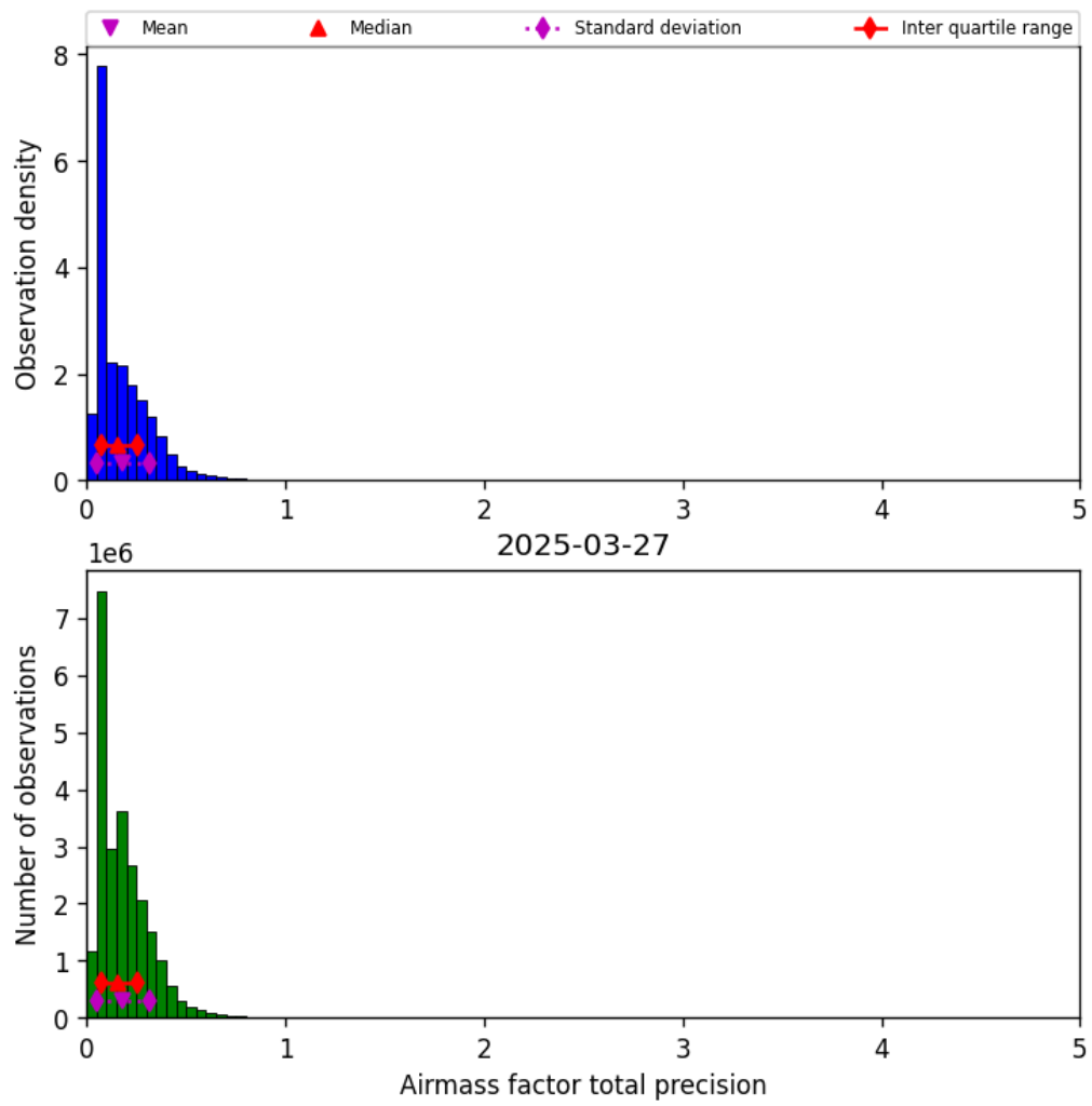
Figure 39: Histogram of “Airmass factor total precision” for 2025-03-27 to 2025-03-28
