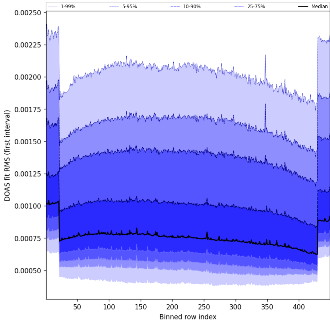
Figure 58: Along track statistics of “DOAS fit RMS (first interval)” for 2025-03-27 to 2025-03-28
