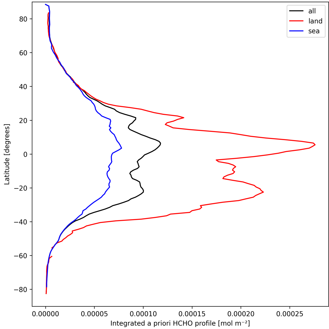
Figure 27: Zonal average of “Integrated a priori HCHO profile” for 2025-03-27 to 2025-03-28.
