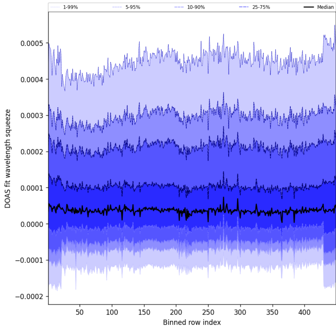
Figure 57: Along track statistics of “DOAS fit wavelength squeeze” for 2025-03-27 to 2025-03-28
