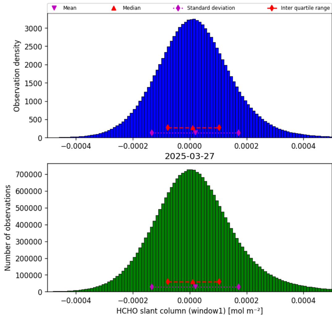
Figure 36: Histogram of “HCHO slant column (window1)” for 2025-03-27 to 2025-03-28
