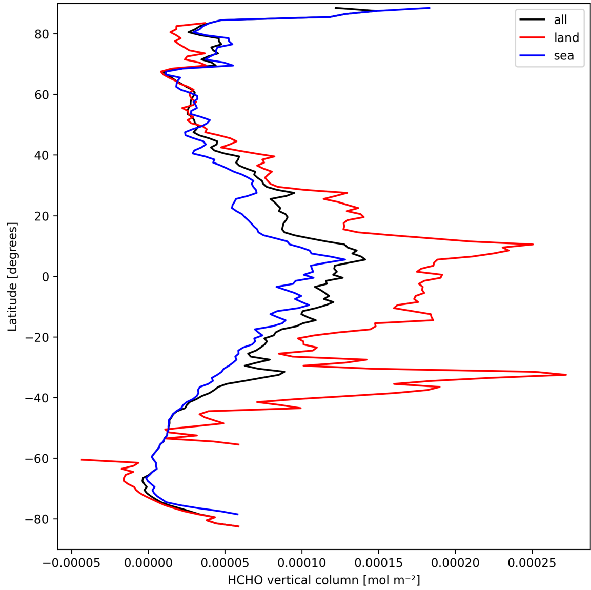
Figure 19: Zonal average of “HCHO vertical column” for 2025-03-27 to 2025-03-28.
