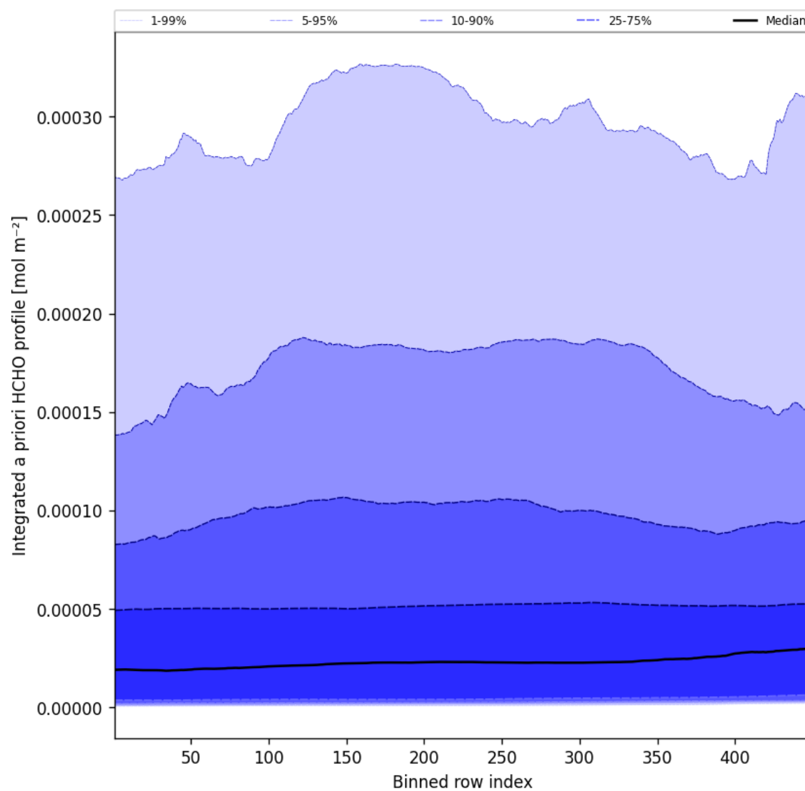
Figure 55: Along track statistics of "Integrated a priori HCHO profile" for 2025-03-27 to 2025-03-28
