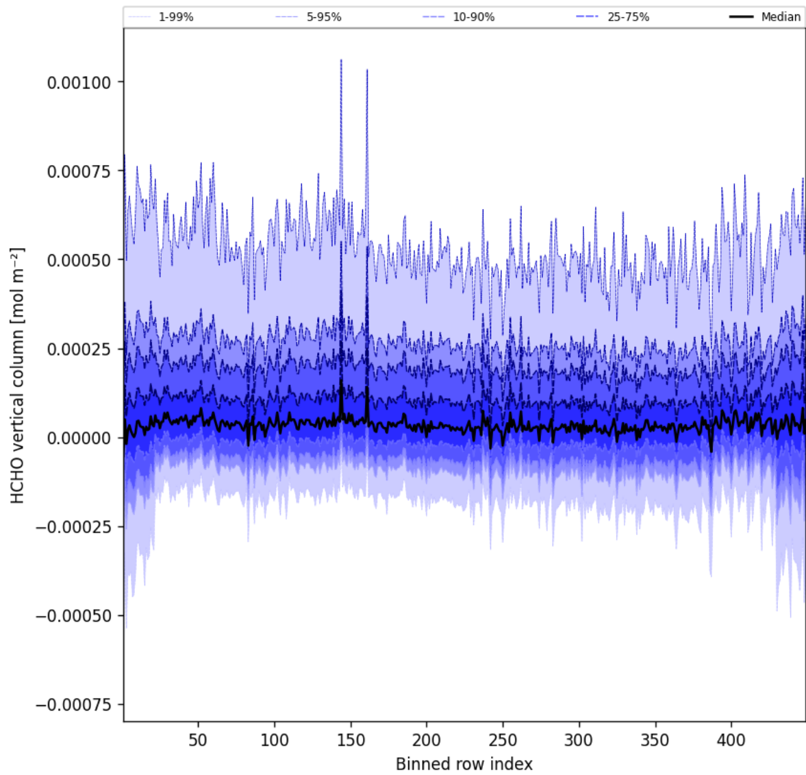
Figure 47: Along track statistics of “HCHO vertical column” for 2025-03-27 to 2025-03-28
