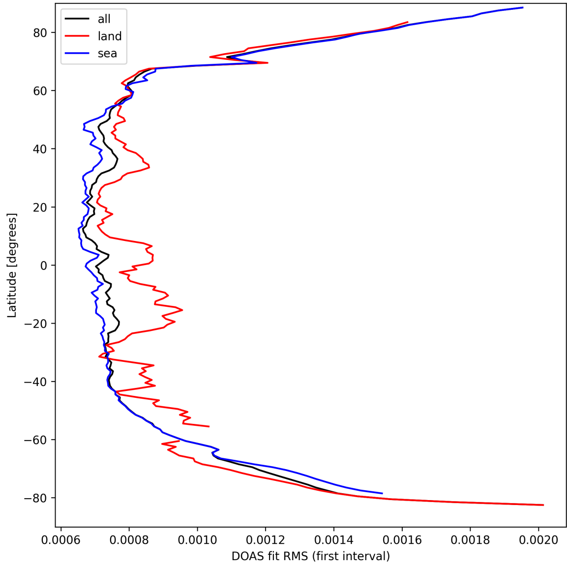
Figure 30: Zonal average of “DOAS fit RMS (first interval)” for 2025-03-27 to 2025-03-28.
