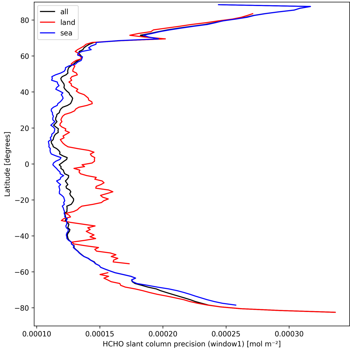
Figure 23: Zonal average of “HCHO slant column precision (window1)” for 2025-03-27 to 2025-03-28.
