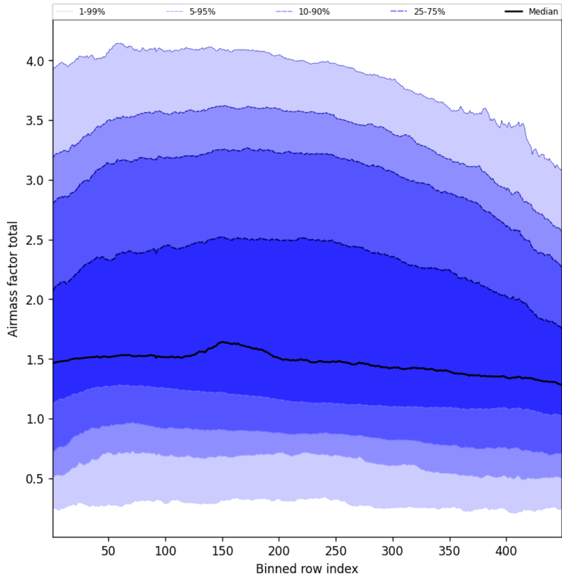
Figure 52: Along track statistics of “Airmass factor total” for 2025-03-27 to 2025-03-28
