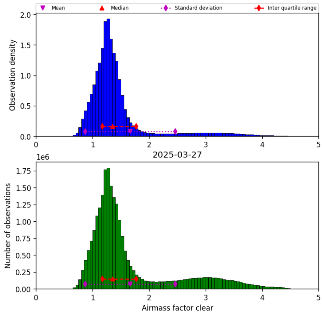
Figure 40: Histogram of “Airmass factor clear” for 2025-03-27 to 2025-03-28
