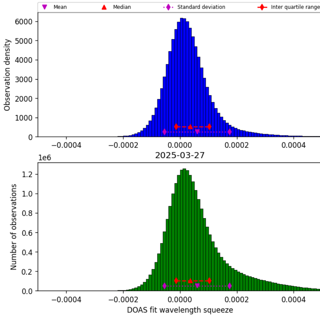
Figure 43: Histogram of “DOAS fit wavelength squeeze” for 2025-03-27 to 2025-03-28
