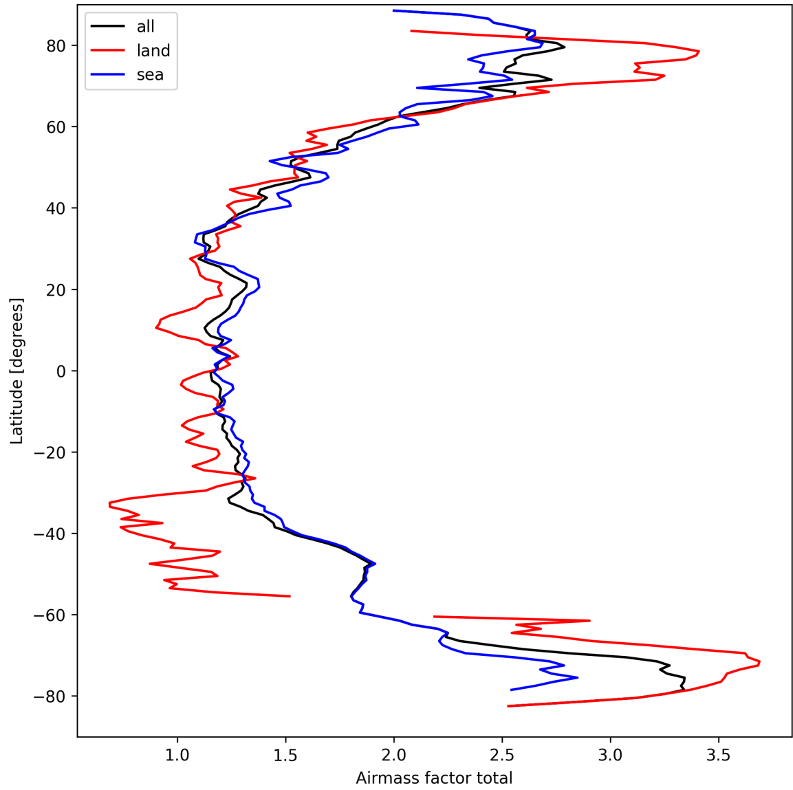
Figure 24: Zonal average of “Airmass factor total” for 2025-03-27 to 2025-03-28.
