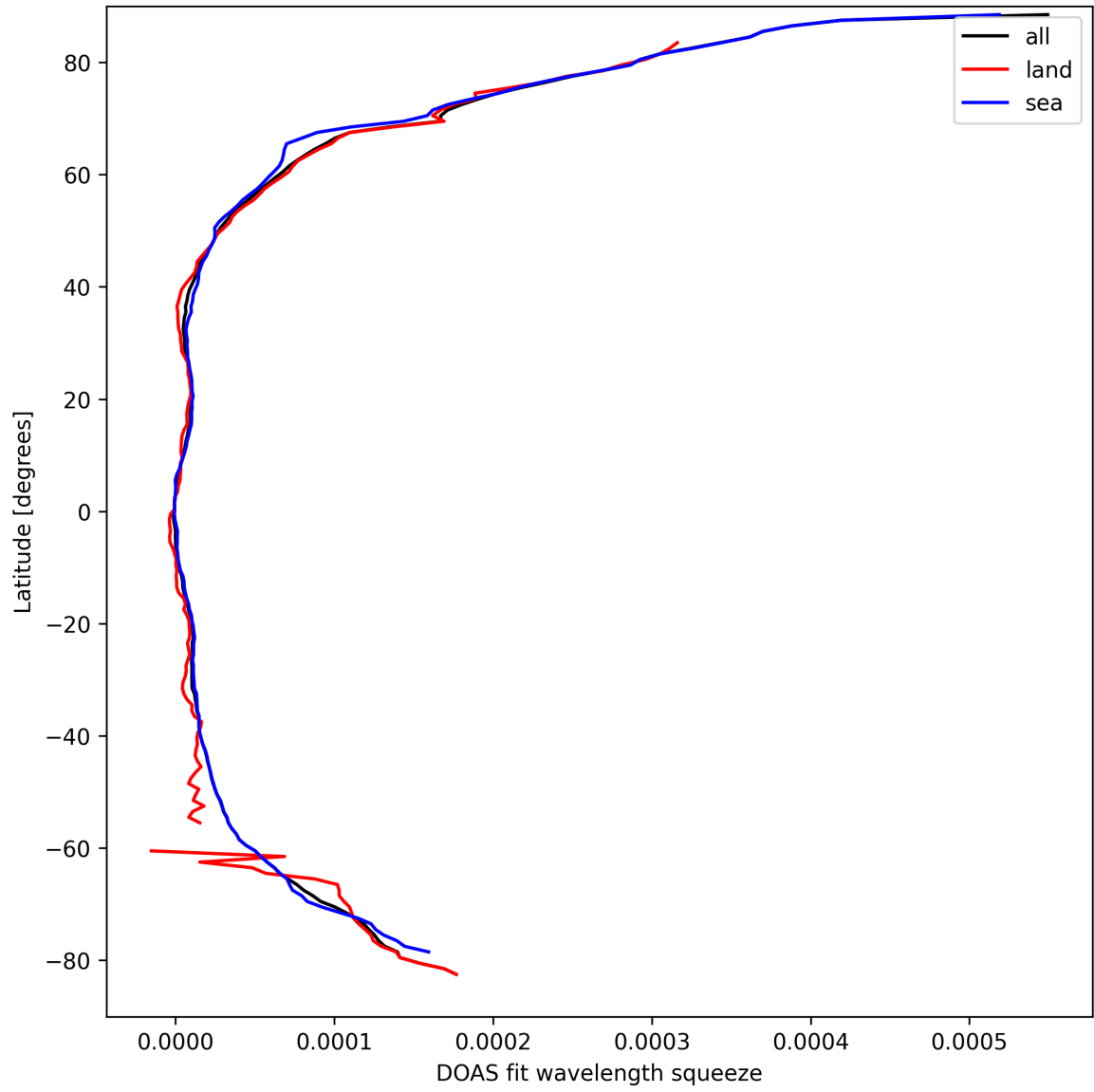
Figure 29: Zonal average of “DOAS fit wavelength squeeze” for 2025-03-27 to 2025-03-28.
