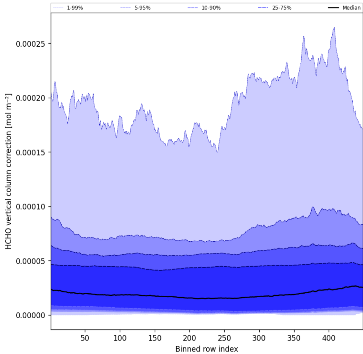
Figure 49: Along track statistics of "HCHO vertical column correction" for 2025-03-27 to 2025-03-28
