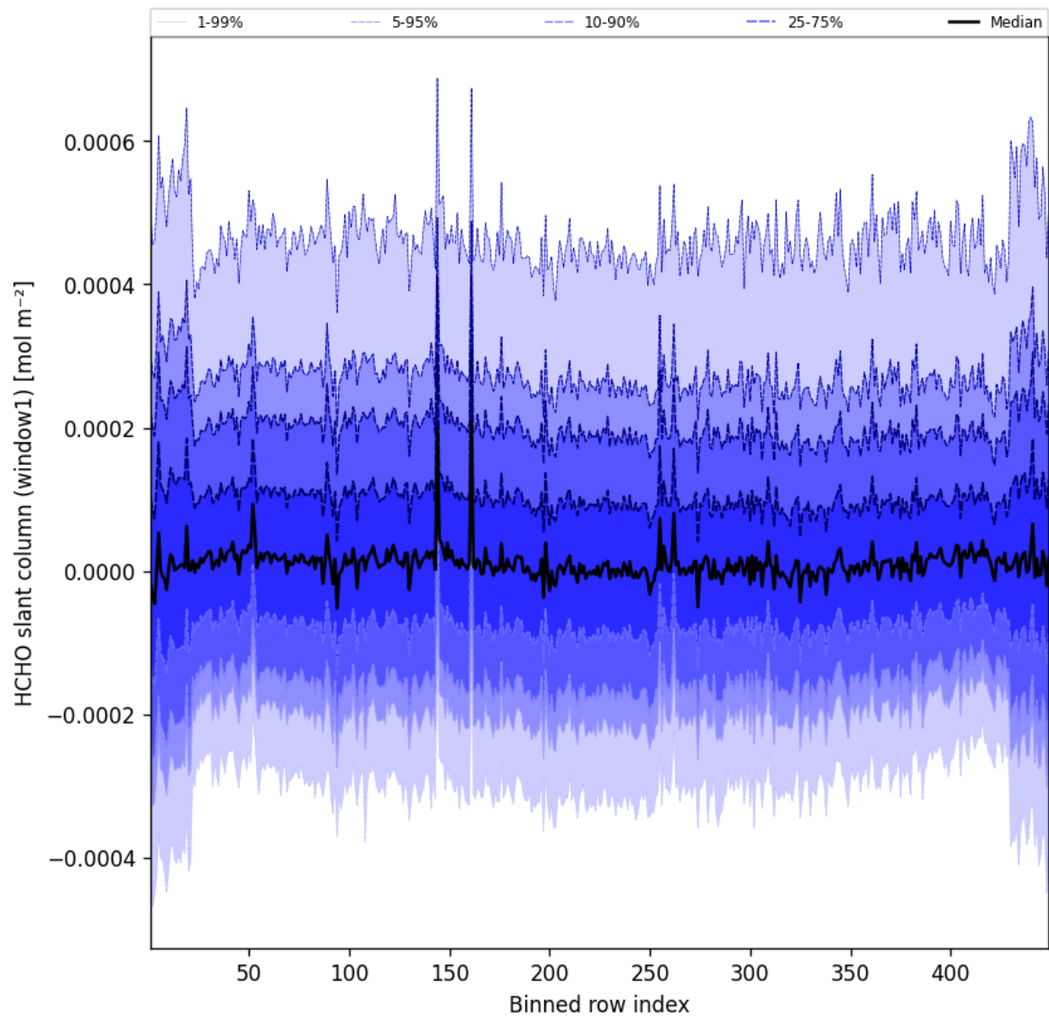
Figure 50: Along track statistics of “HCHO slant column (window1)” for 2025-03-27 to 2025-03-28
