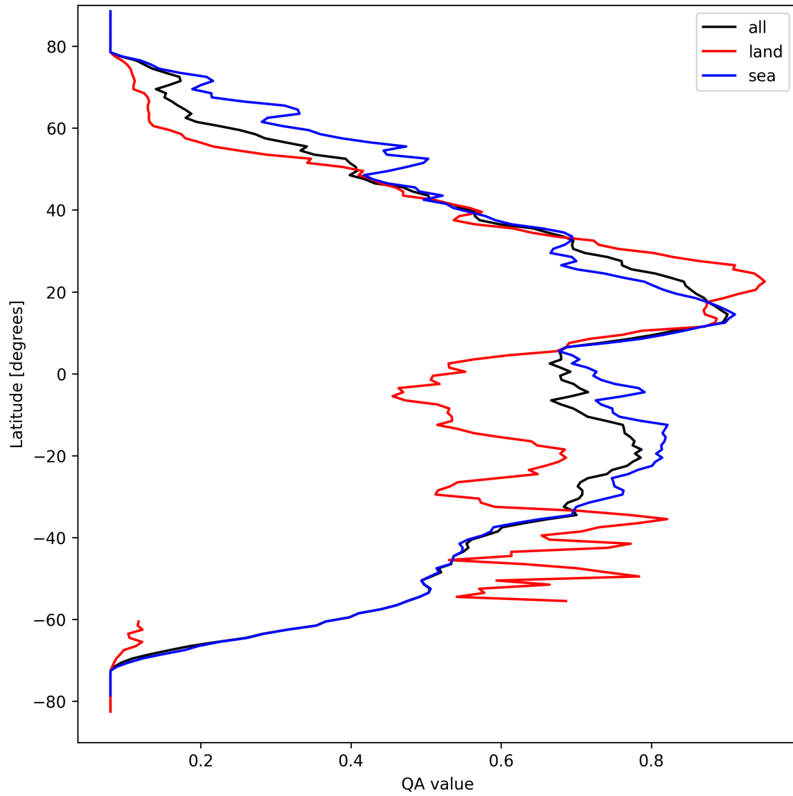
Figure 18: Zonal average of “QA value” for 2025-03-27 to 2025-03-28.
