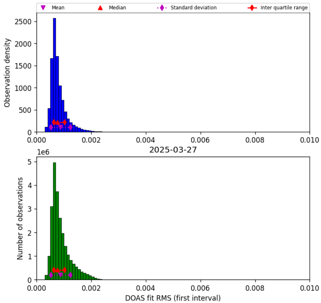
Figure 44: Histogram of “DOAS fit RMS (first interval)” for 2025-03-27 to 2025-03-28
