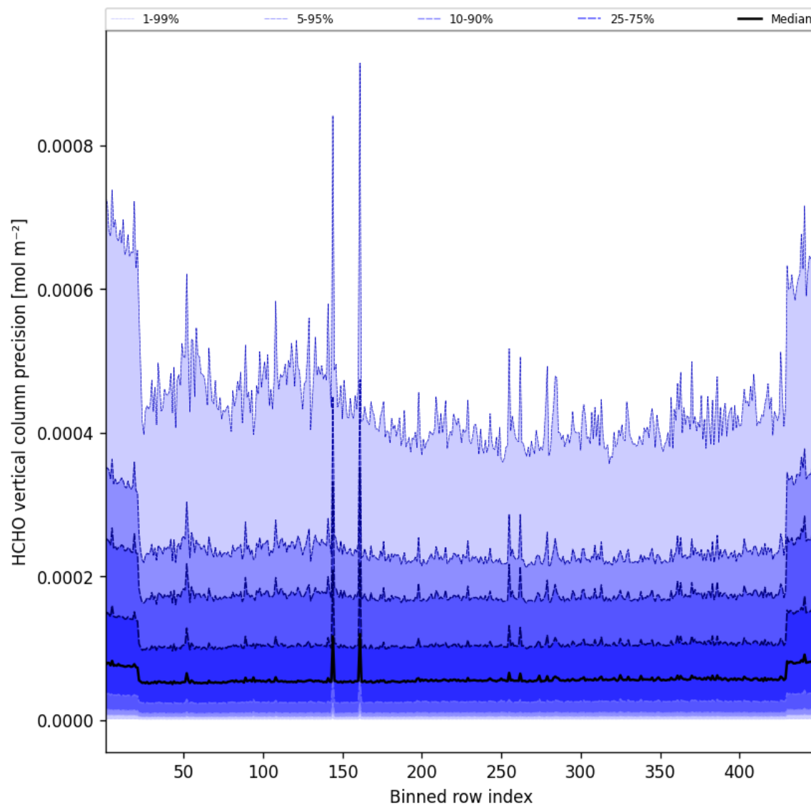
Figure 48: Along track statistics of “HCHO vertical column precision” for 2025-03-27 to 2025-03-28
