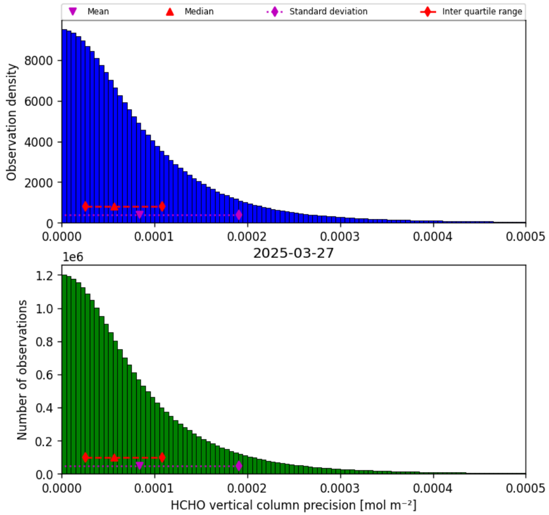
Figure 34: Histogram of “HCHO vertical column precision” for 2025-03-27 to 2025-03-28
