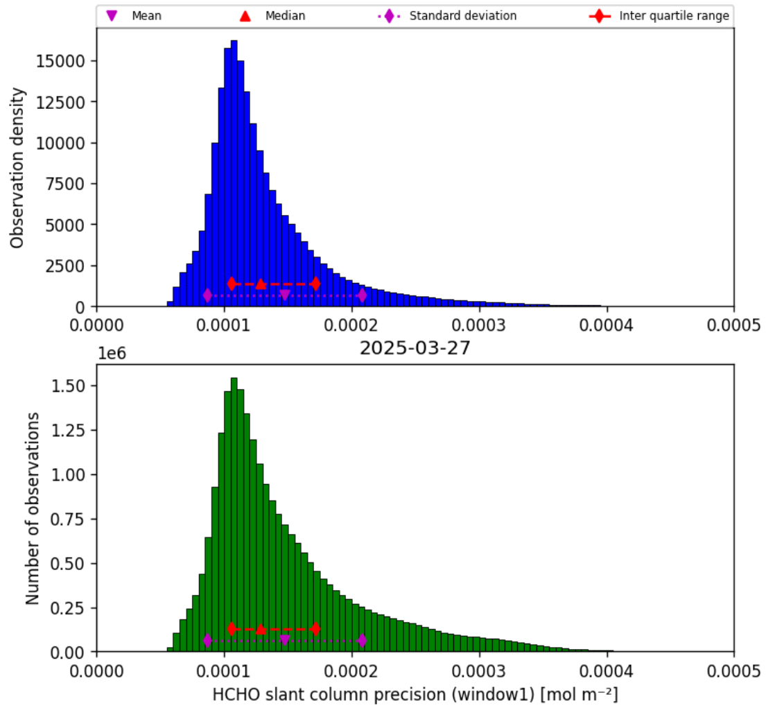
Figure 37: Histogram of “HCHO slant column precision (window1)” for 2025-03-27 to 2025-03-28
