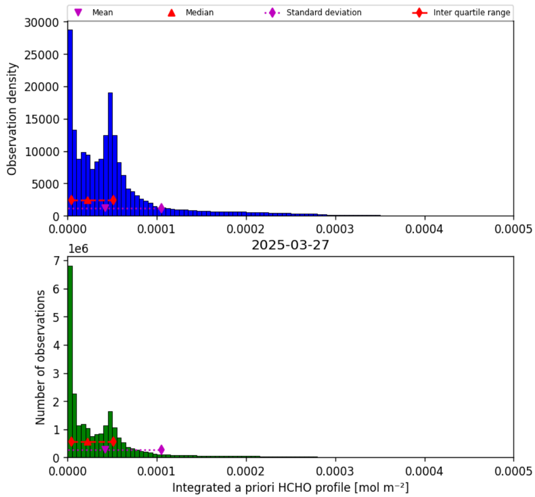
Figure 41: Histogram of “Integrated a priori HCHO profile” for 2025-03-27 to 2025-03-28
