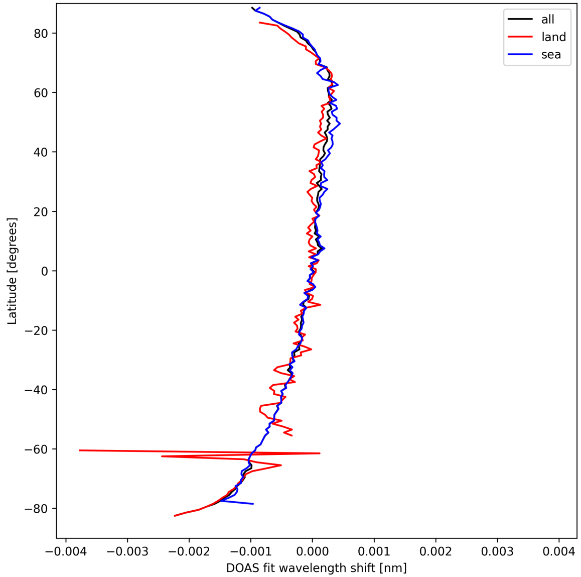
Figure 28: Zonal average of “DOAS fit wavelength shift” for 2025-03-27 to 2025-03-28.
