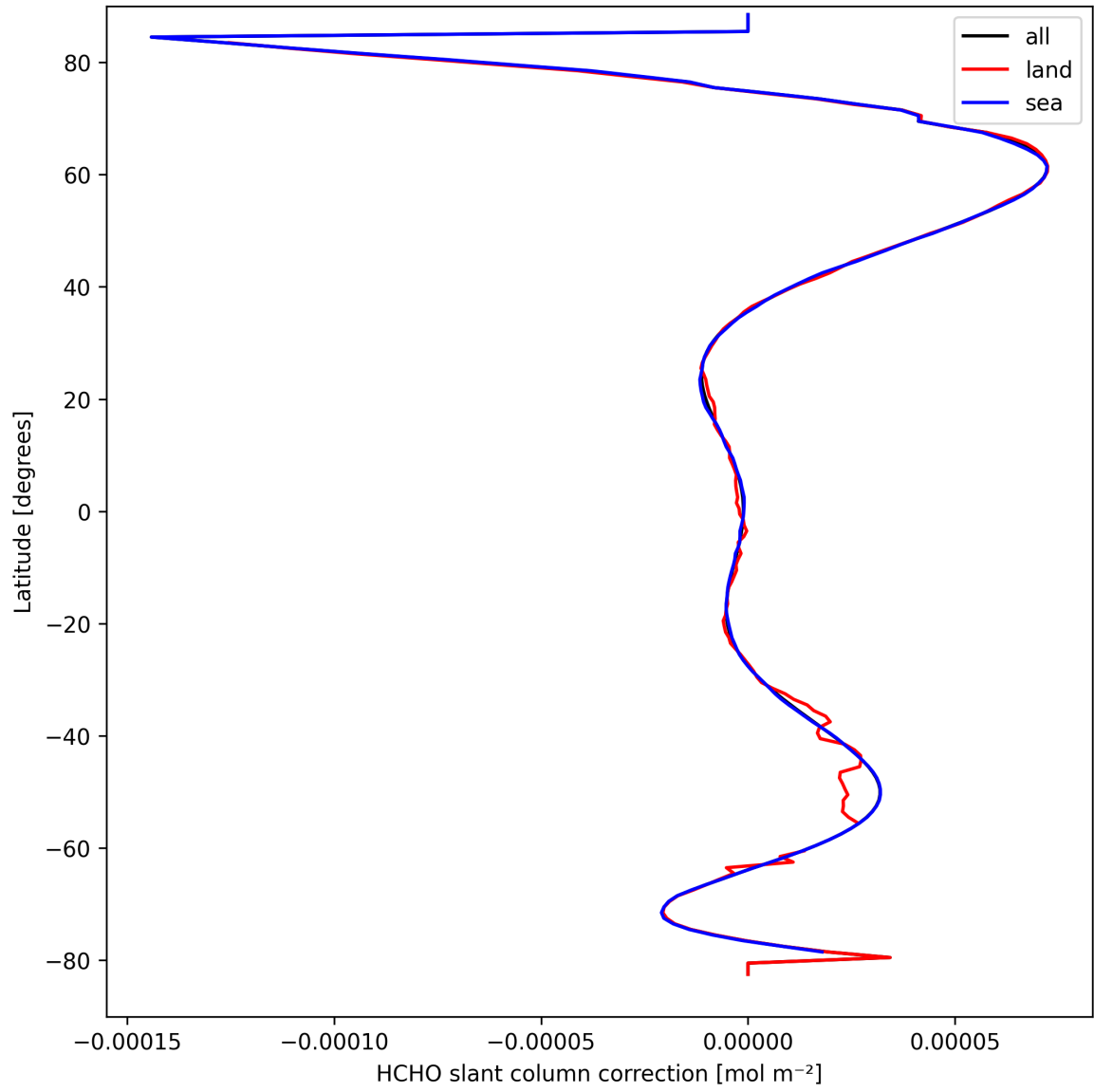
Figure 31: Zonal average of "HCHO slant column correction" for 2025-03-27 to 2025-03-28.
