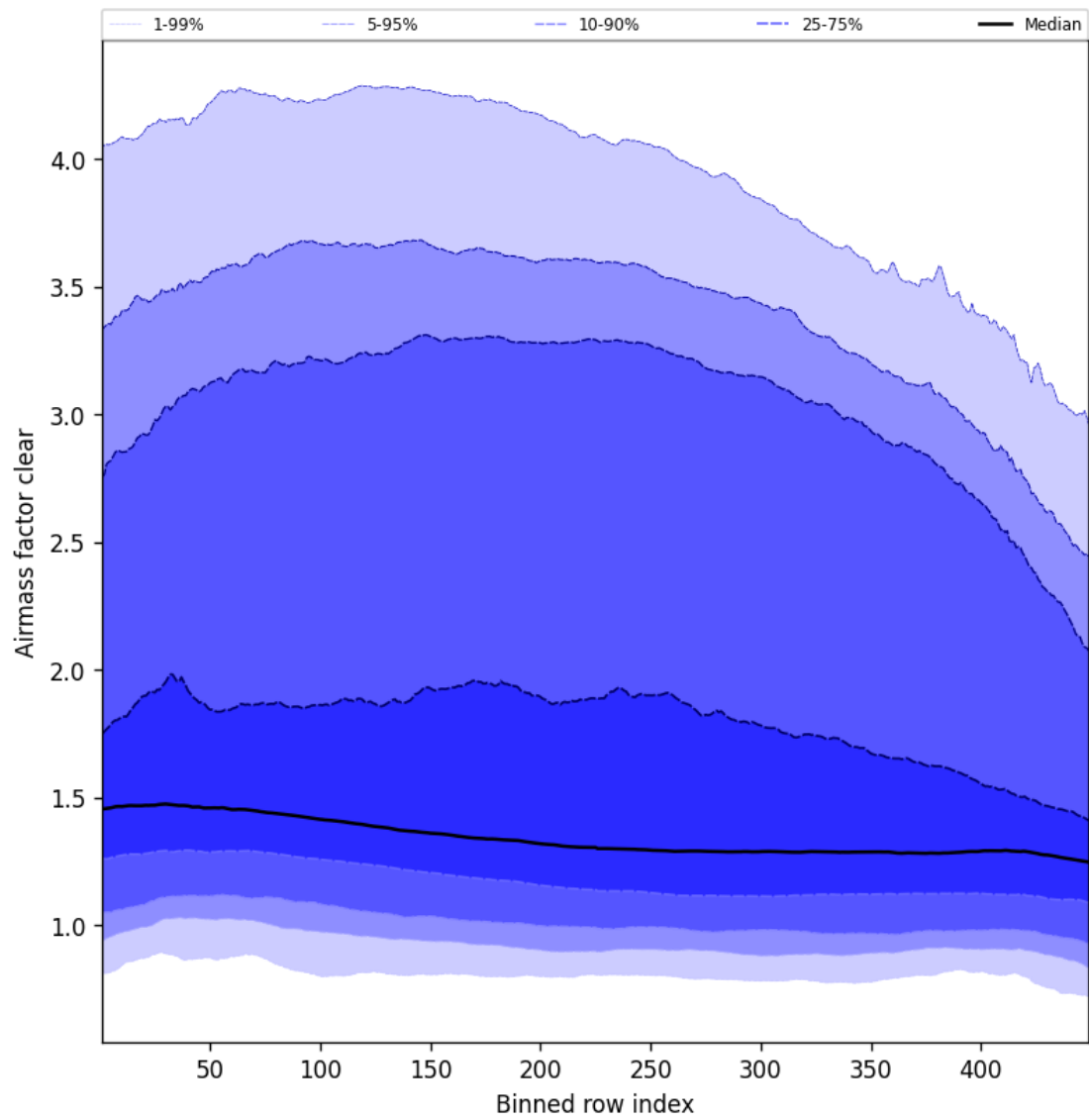
Figure 54: Along track statistics of “Airmass factor clear” for 2025-03-27 to 2025-03-28
