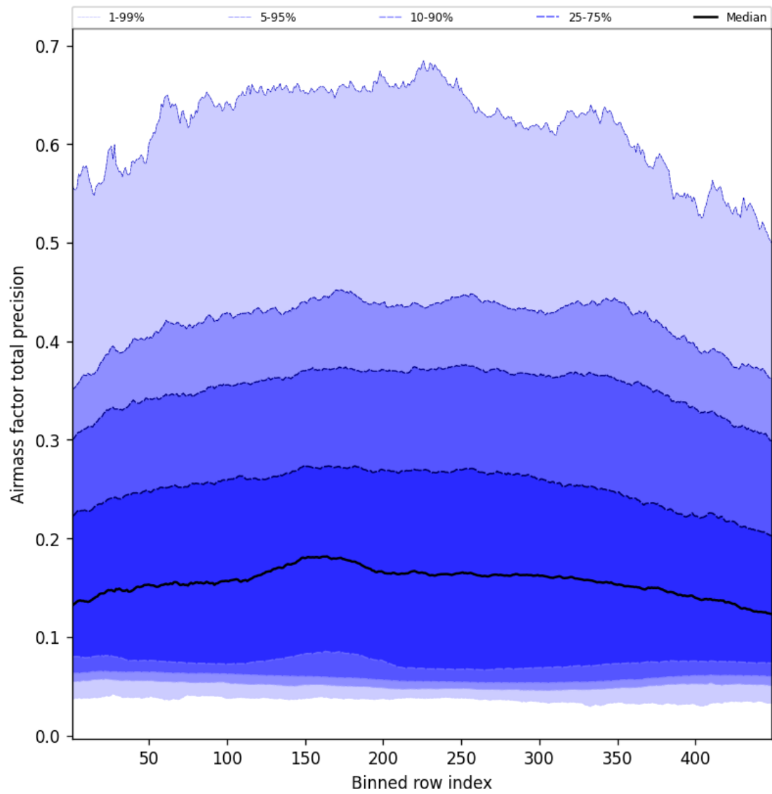
Figure 53: Along track statistics of “Airmass factor total precision” for 2025-03-27 to 2025-03-28
