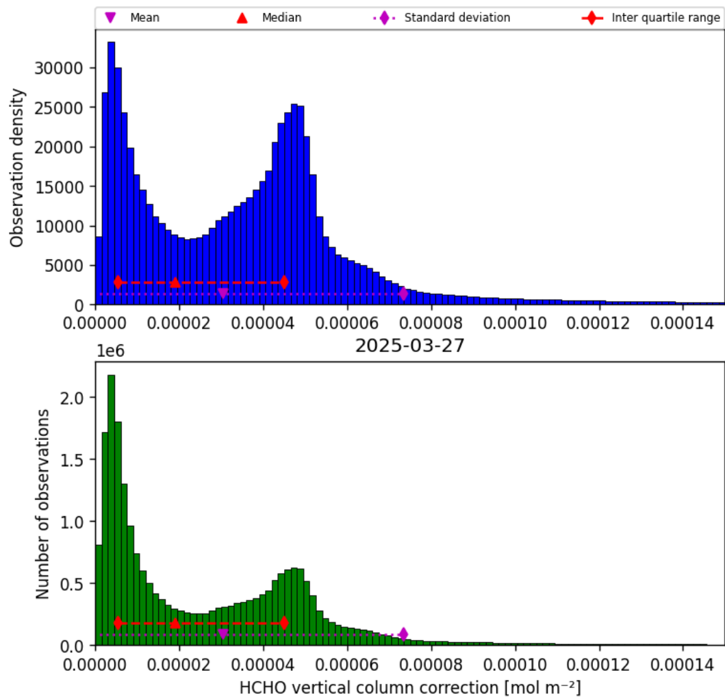
Figure 35: Histogram of “HCHO vertical column correction” for 2025-03-27 to 2025-03-28
