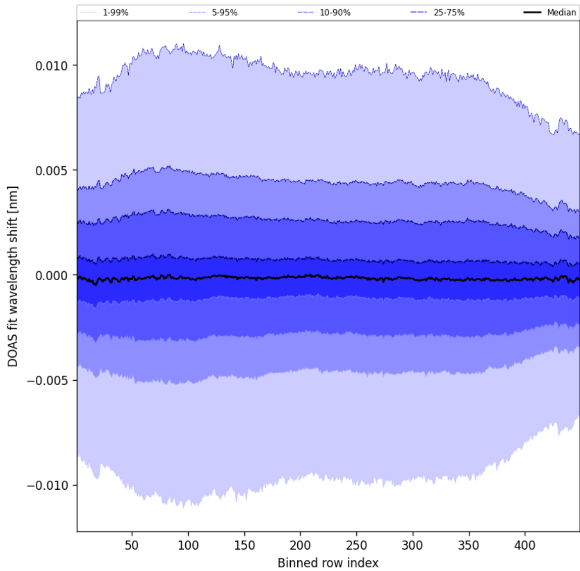
Figure 56: Along track statistics of “DOAS fit wavelength shift” for 2025-03-27 to 2025-03-28
