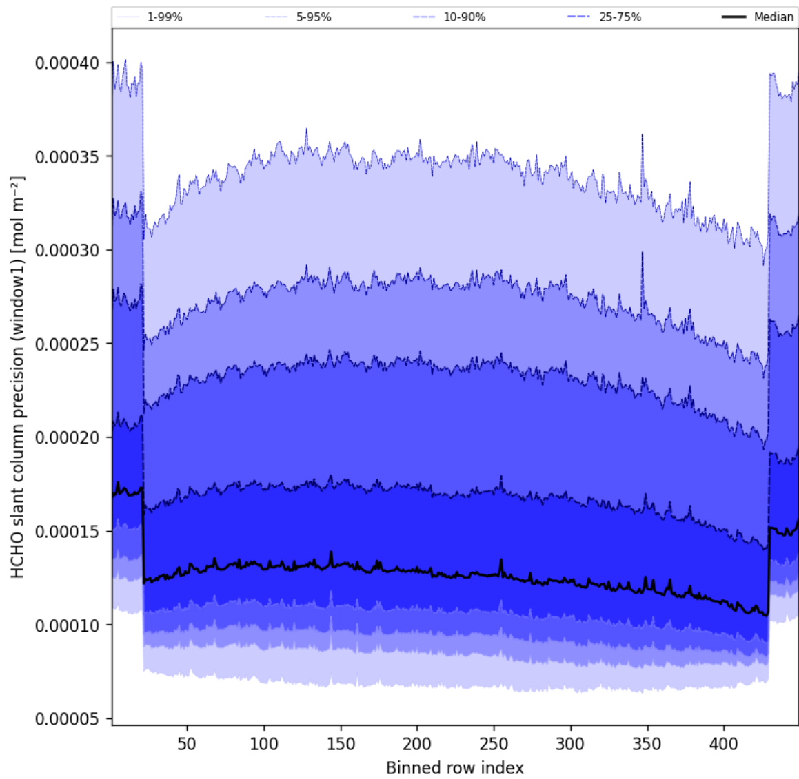
Figure 51: Along track statistics of “HCHO slant column precision (window1)” for 2025-03-27 to 2025-03-28
