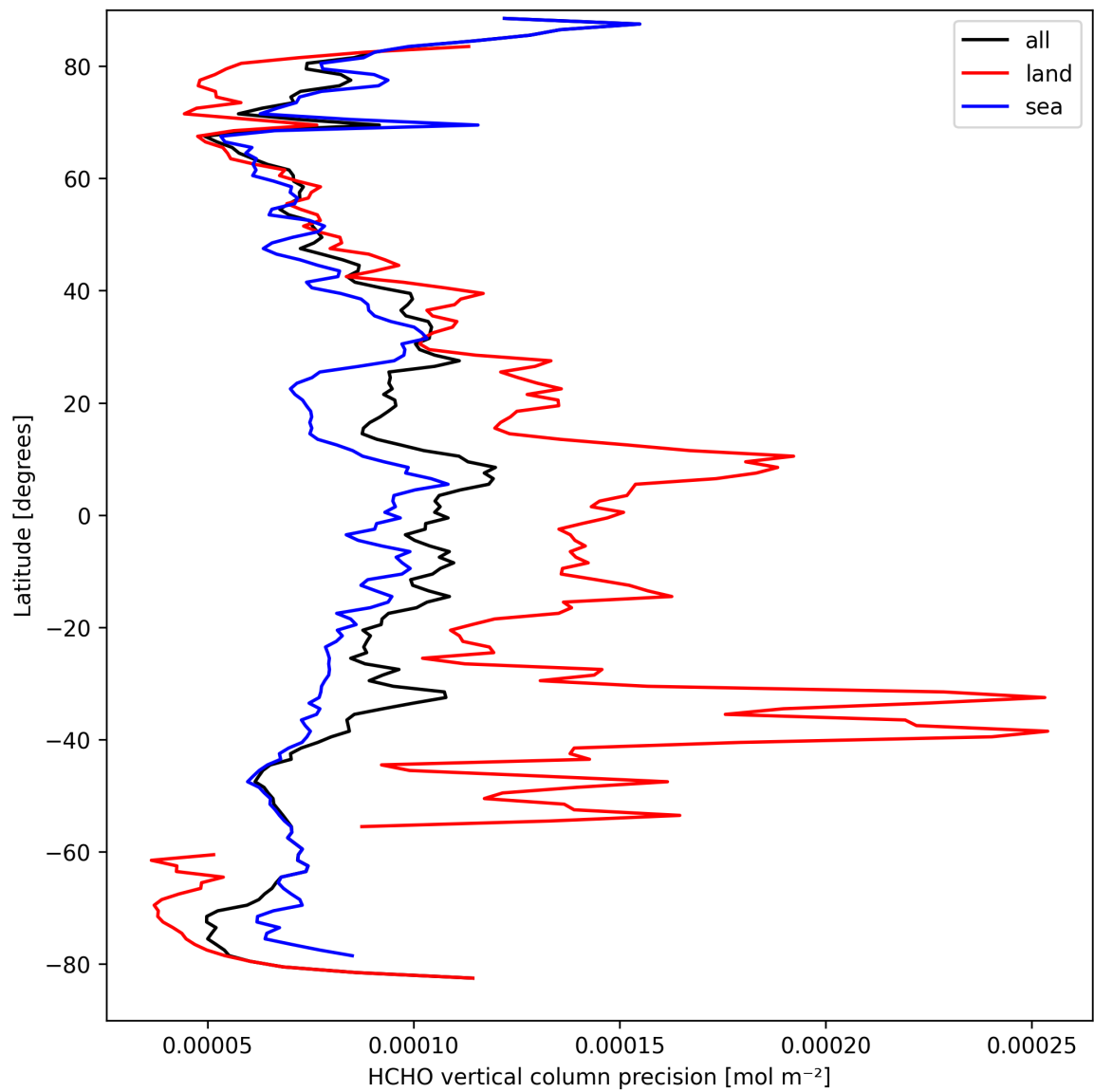
Figure 20: Zonal average of “HCHO vertical column precision” for 2025-03-27 to 2025-03-28.
