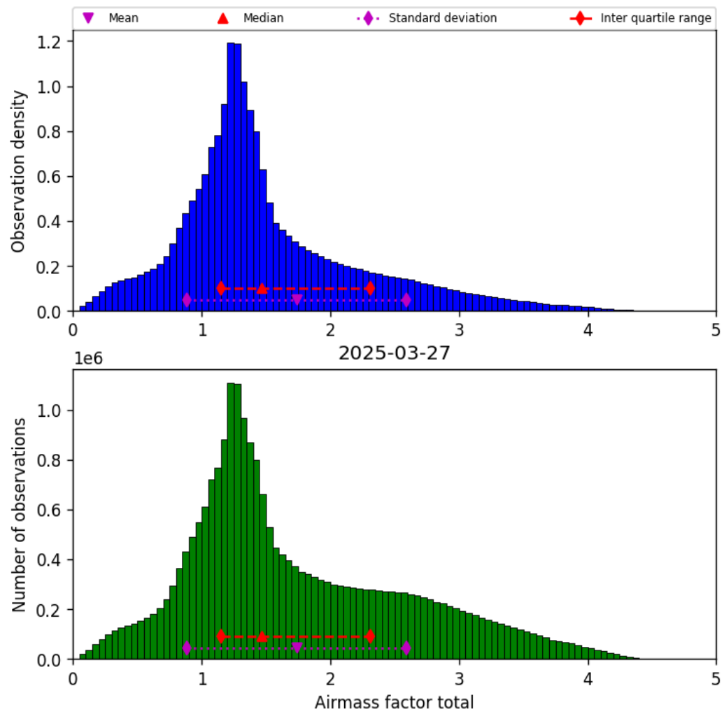
Figure 38: Histogram of “Airmass factor total” for 2025-03-27 to 2025-03-28
