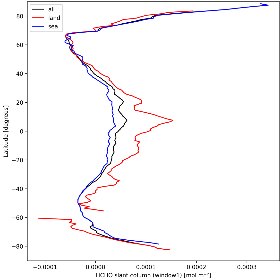
Figure 22: Zonal average of “HCHO slant column (window1)” for 2025-03-27 to 2025-03-28.
