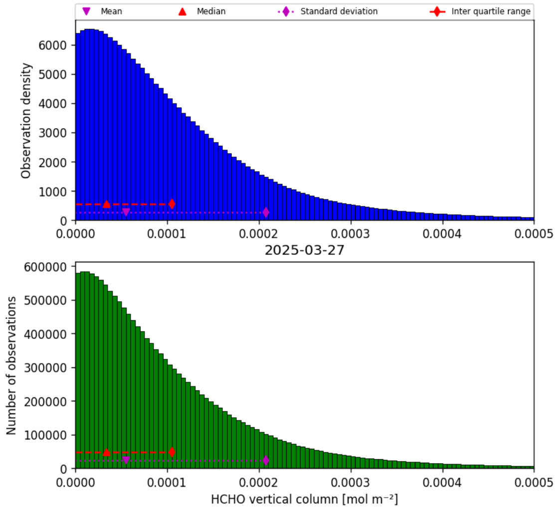
Figure 33: Histogram of “HCHO vertical column” for 2025-03-27 to 2025-03-28
