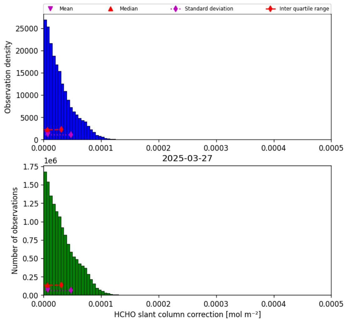
Figure 45: Histogram of “HCHO slant column correction” for 2025-03-27 to 2025-03-28
