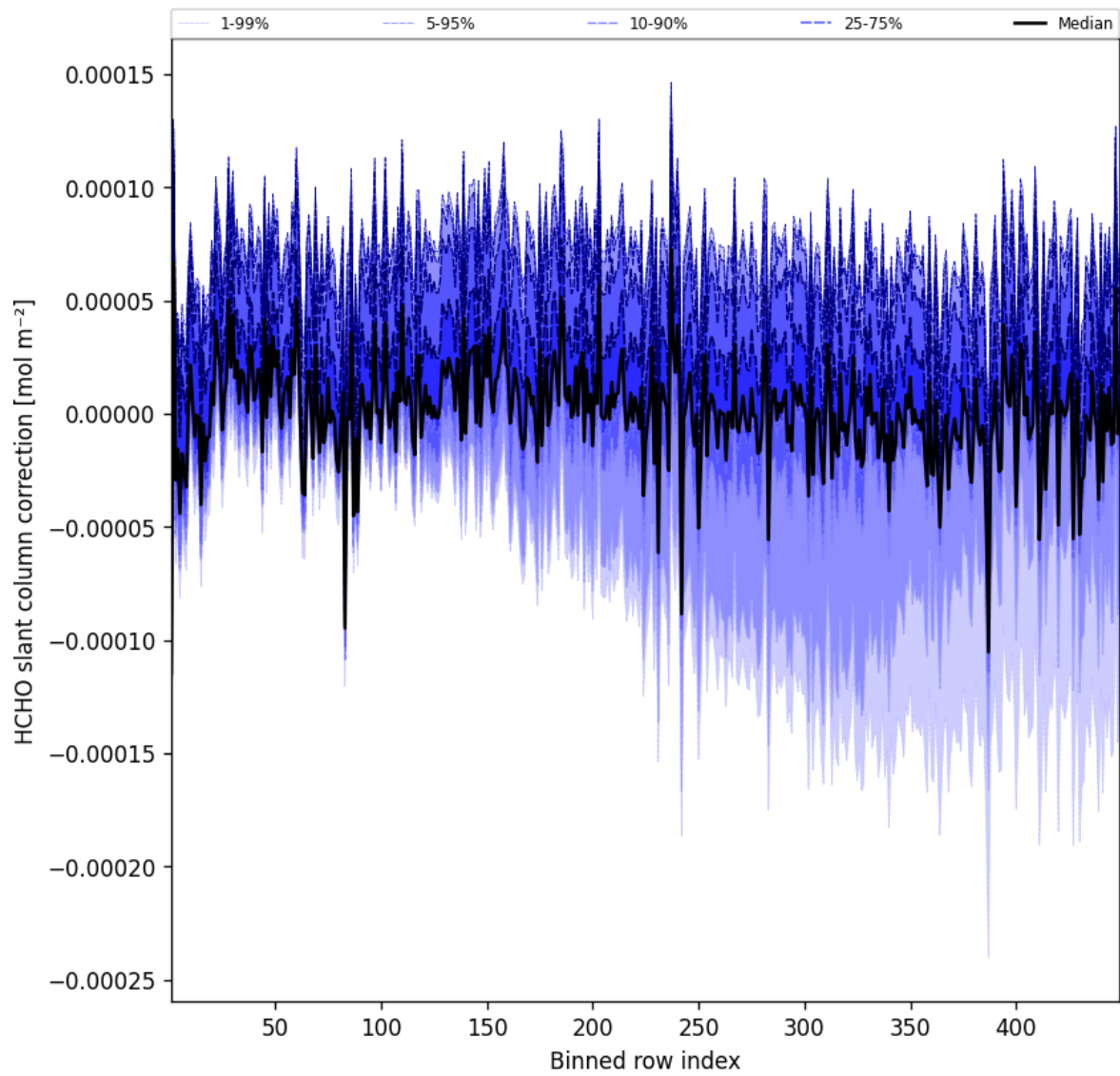
Figure 59: Along track statistics of “HCHO slant column correction” for 2025-03-27 to 2025-03-28
