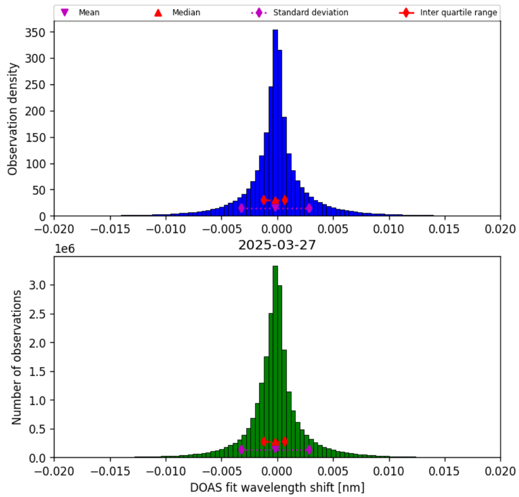
Figure 42: Histogram of “DOAS fit wavelength shift” for 2025-03-27 to 2025-03-28
