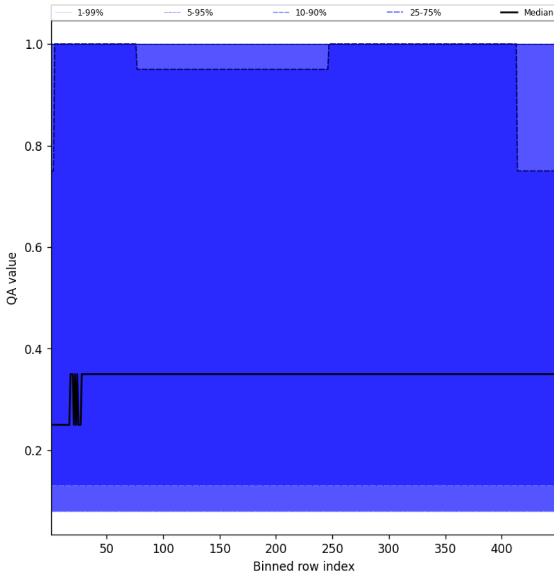
Figure 46: Along track statistics of “QA value” for 2025-03-27 to 2025-03-28
