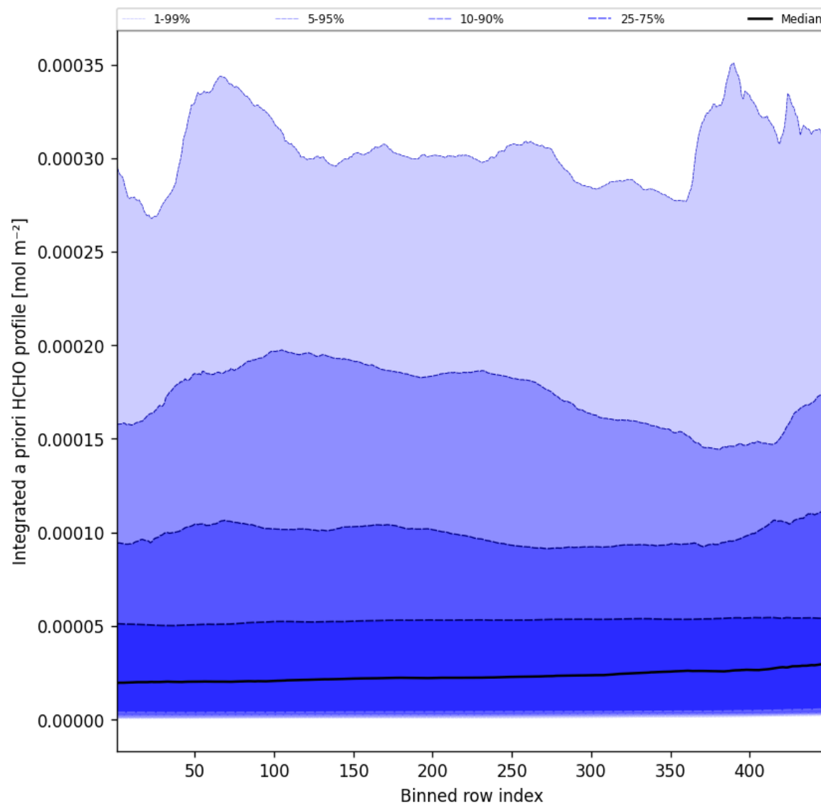
Figure 55: Along track statistics of “Integrated a priori HCHO profile” for 2025-03-28 to 2025-03-29
