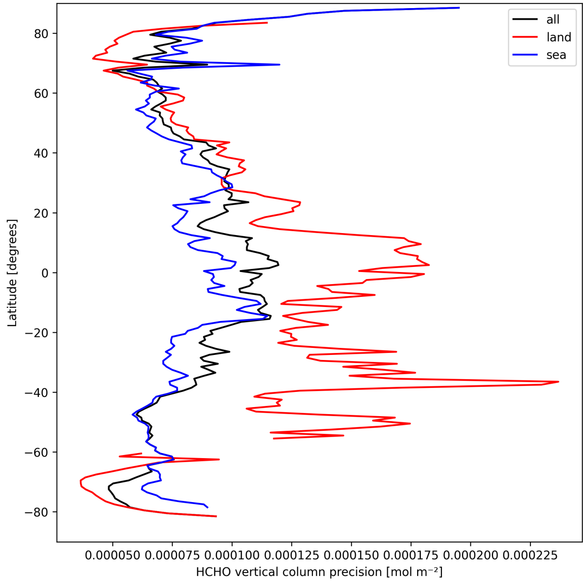
Figure 20: Zonal average of “HCHO vertical column precision” for 2025-03-28 to 2025-03-29.
