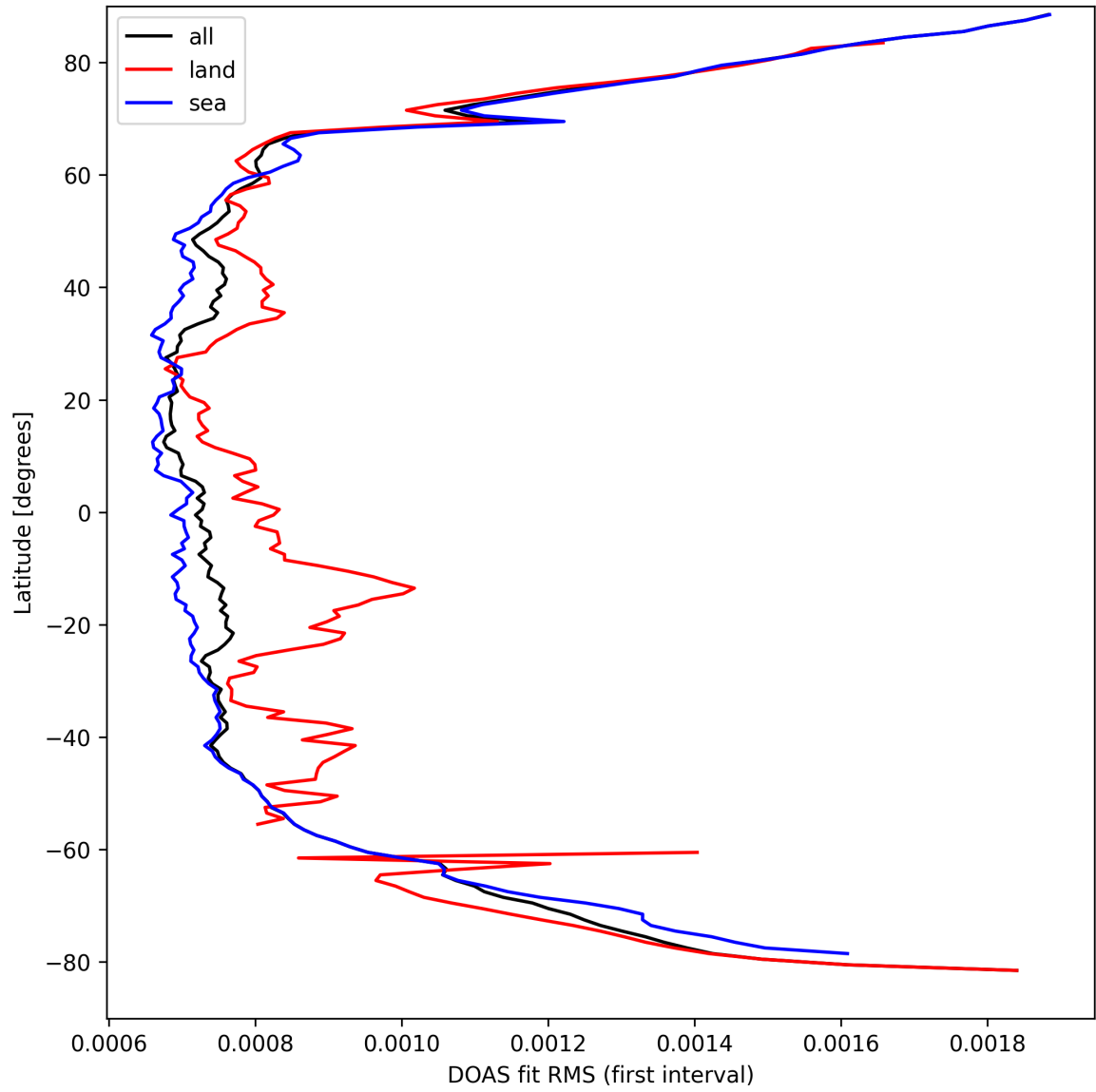
Figure 30: Zonal average of “DOAS fit RMS (first interval)” for 2025-03-28 to 2025-03-29.
