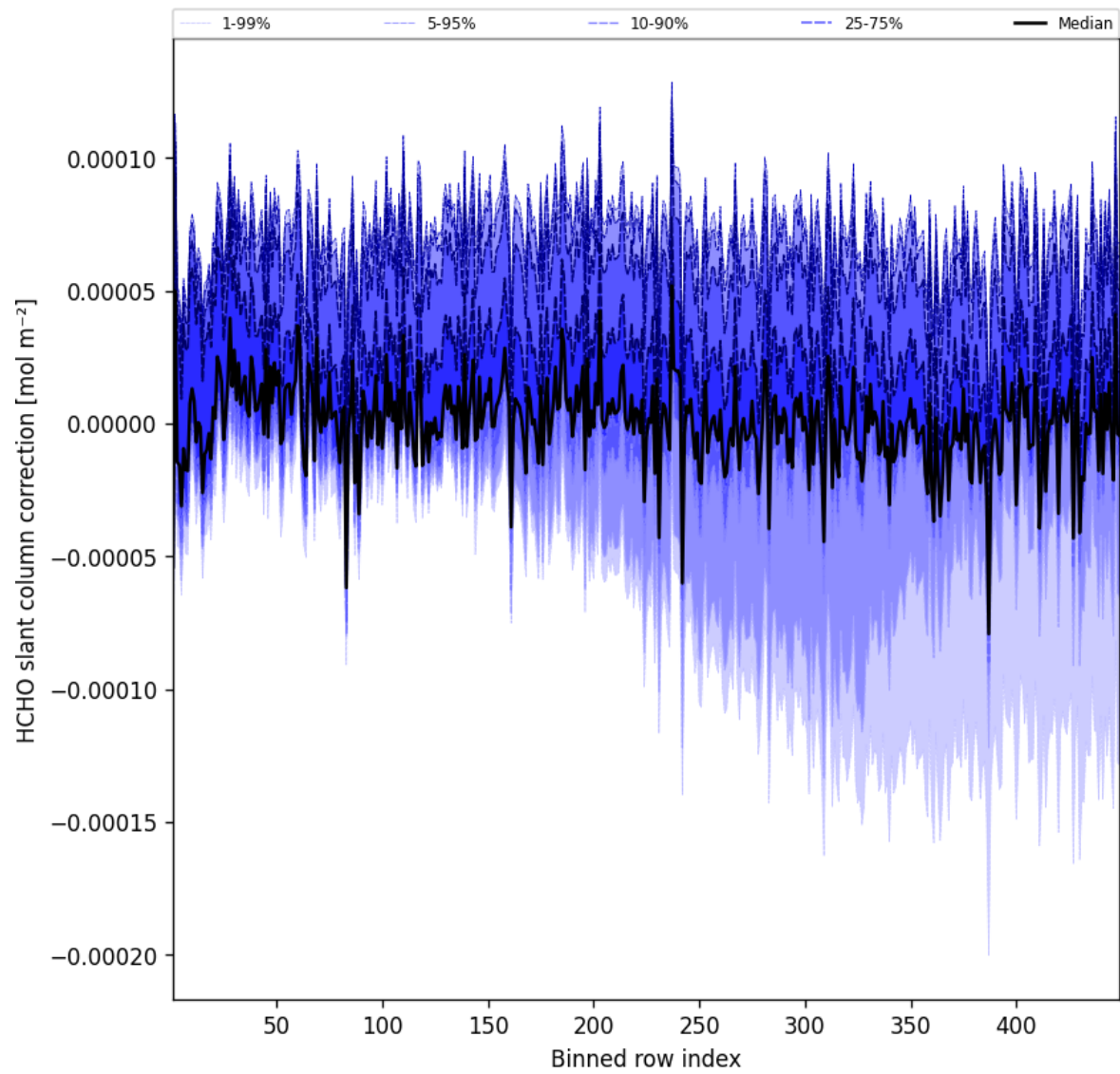
Figure 59: Along track statistics of “HCHO slant column correction” for 2025-03-28 to 2025-03-29
