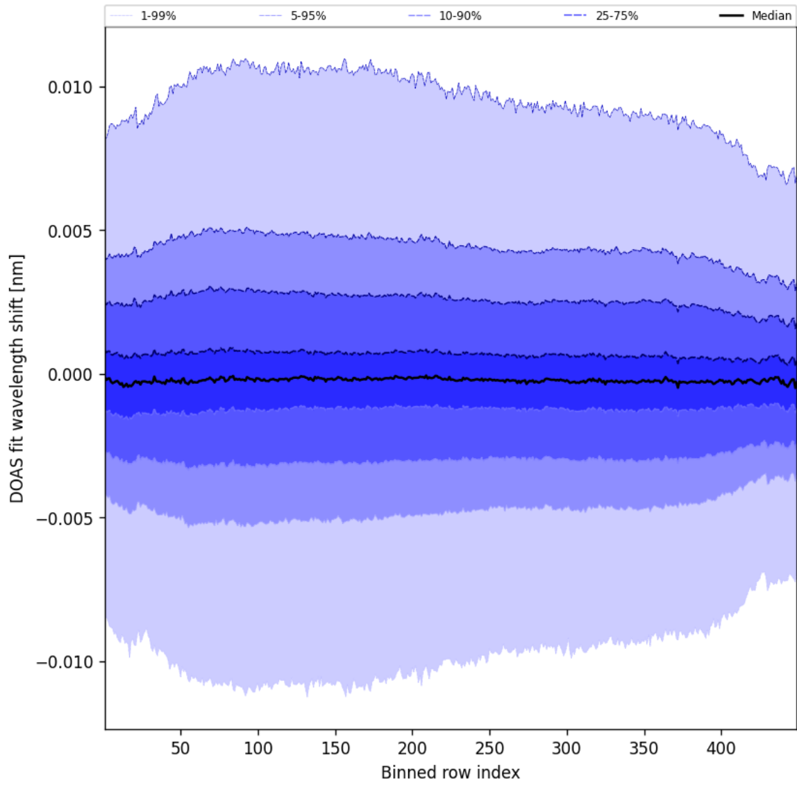
Figure 56: Along track statistics of “DOAS fit wavelength shift” for 2025-03-28 to 2025-03-29
