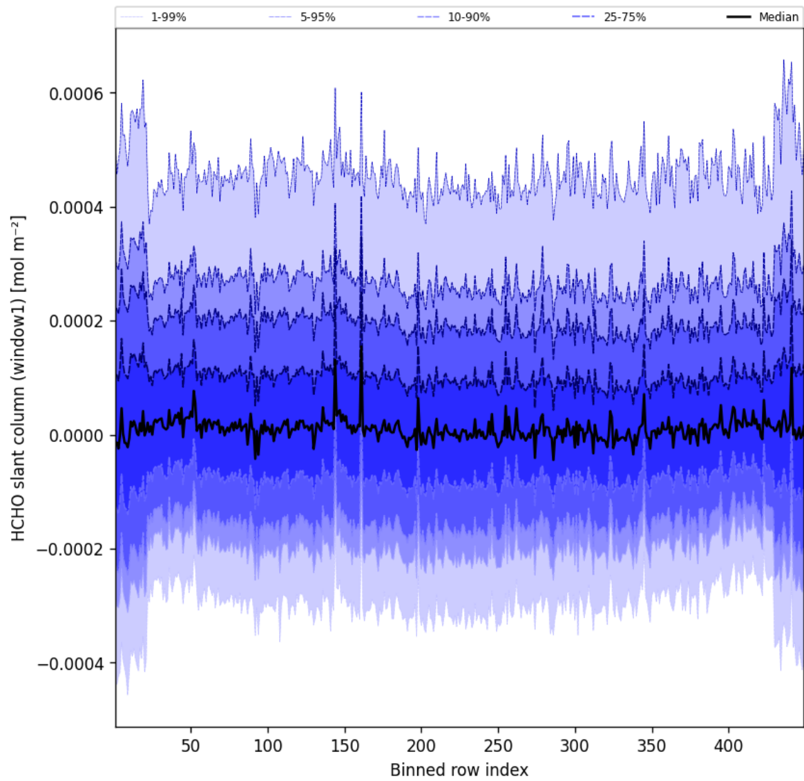
Figure 50: Along track statistics of “HCHO slant column (window1)” for 2025-03-28 to 2025-03-29
