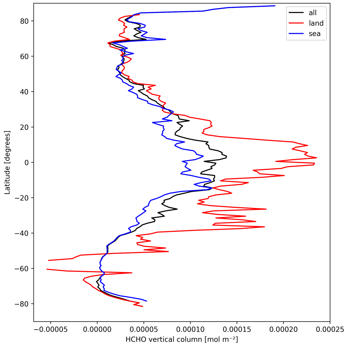
Figure 19: Zonal average of “HCHO vertical column” for 2025-03-28 to 2025-03-29.
