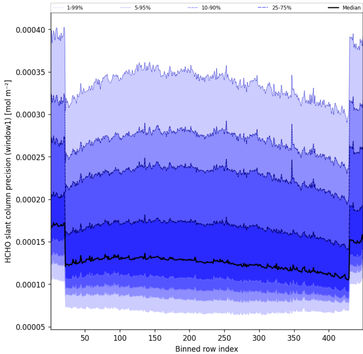
Figure 51: Along track statistics of “HCHO slant column precision (window1)” for 2025-03-28 to 2025-03-29
