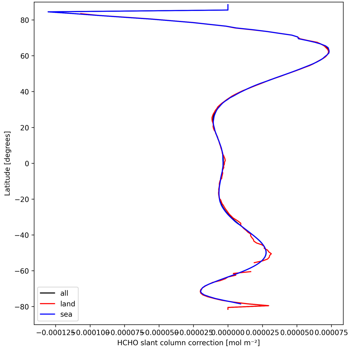
Figure 31: Zonal average of “HCHO slant column correction” for 2025-03-28 to 2025-03-29.
