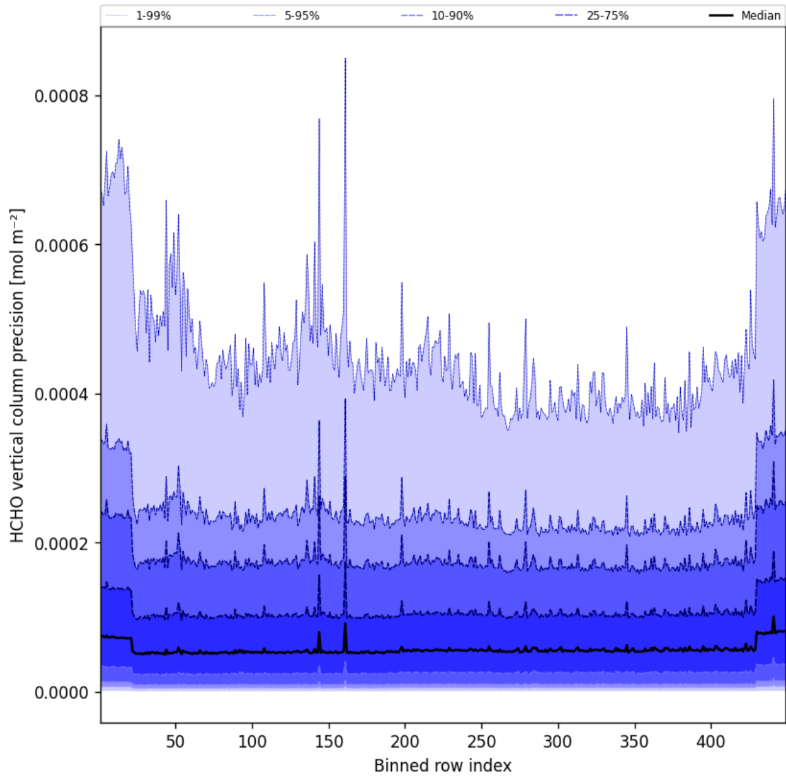
Figure 48: Along track statistics of “HCHO vertical column precision” for 2025-03-28 to 2025-03-29
