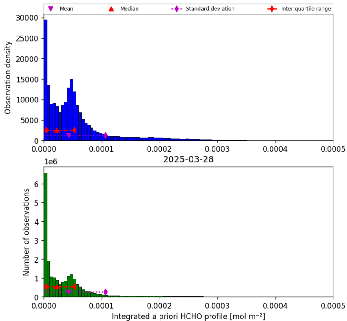
Figure 41: Histogram of “Integrated a priori HCHO profile” for 2025-03-28 to 2025-03-29
