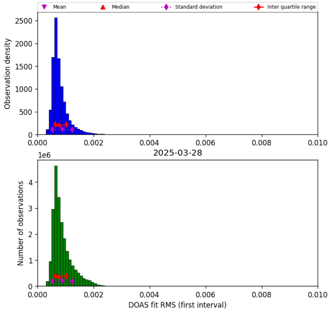
Figure 44: Histogram of “DOAS fit RMS (first interval)” for 2025-03-28 to 2025-03-29
