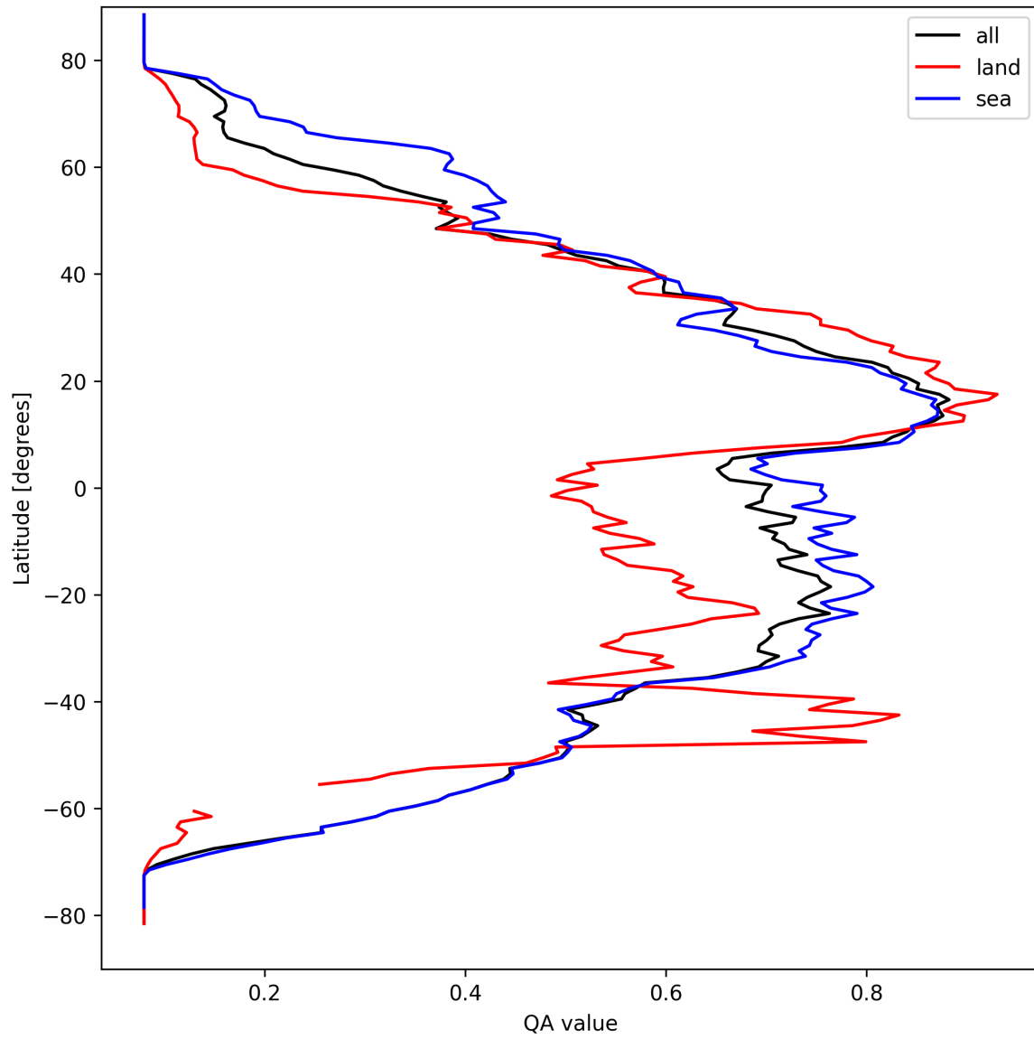
Figure 18: Zonal average of “QA value” for 2025-03-28 to 2025-03-29.
