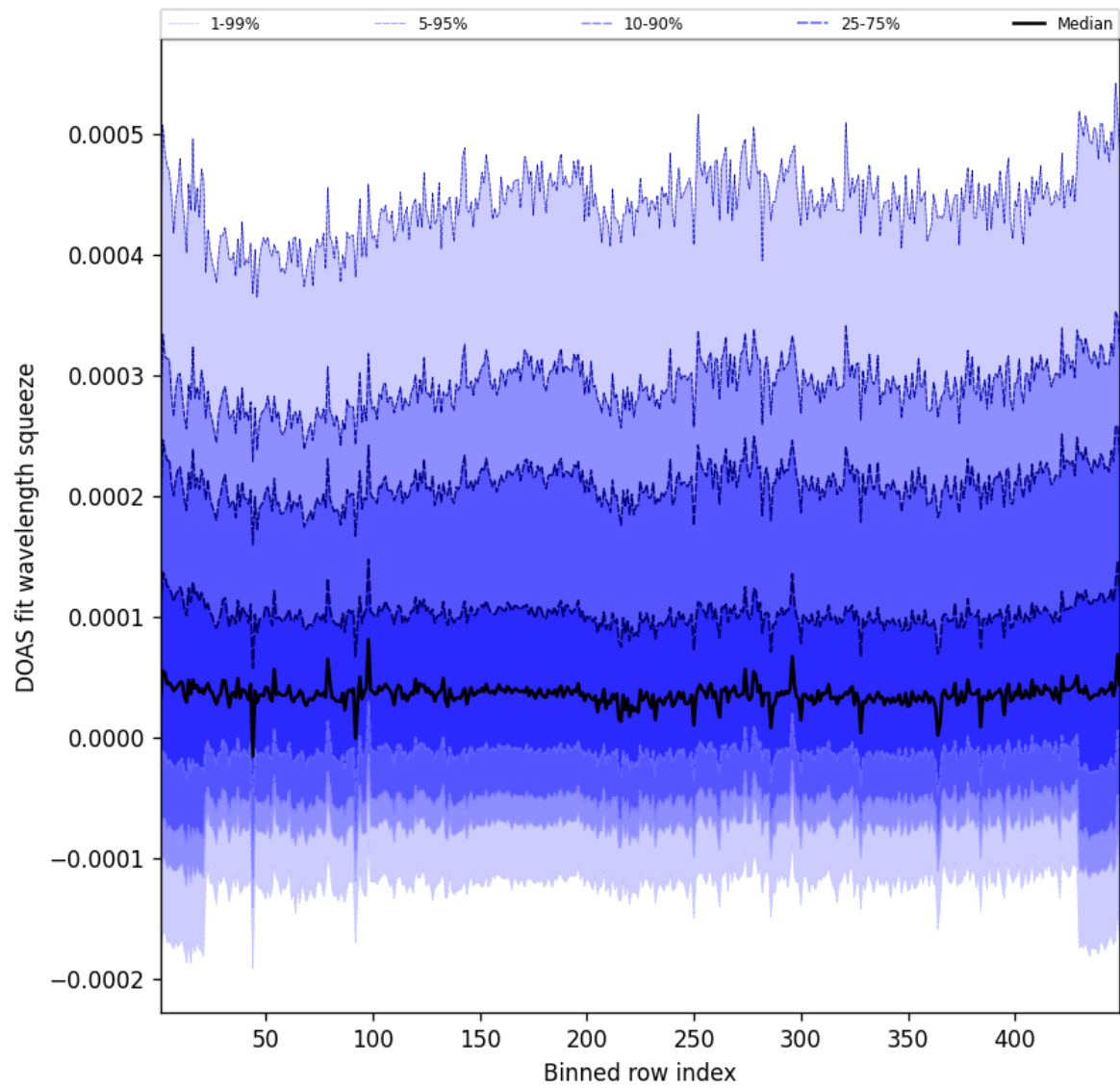
Figure 57: Along track statistics of “DOAS fit wavelength squeeze” for 2025-03-28 to 2025-03-29
