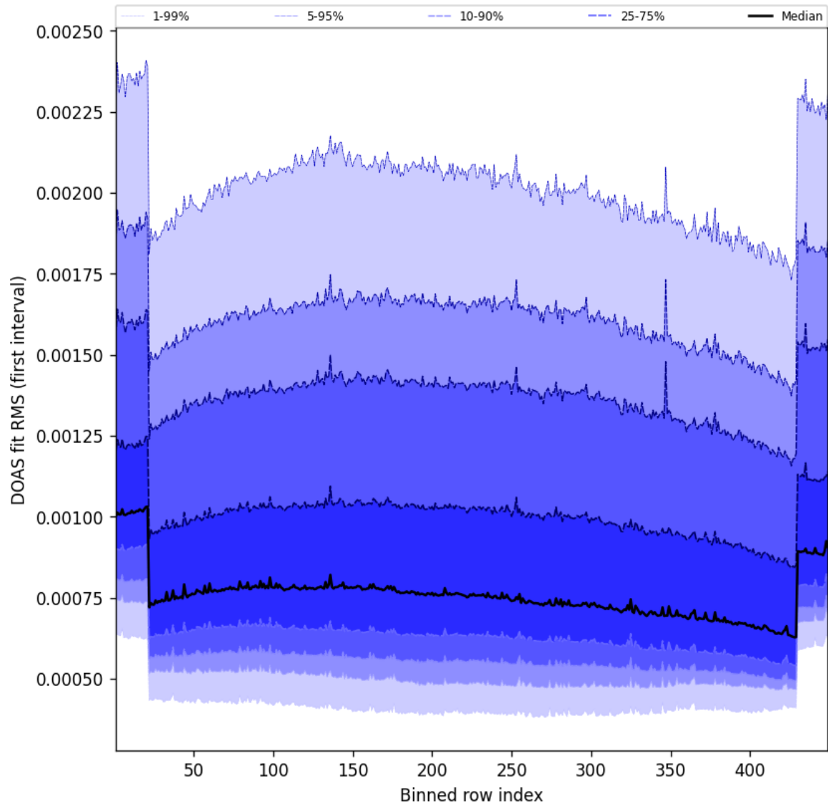
Figure 58: Along track statistics of “DOAS fit RMS (first interval)” for 2025-03-28 to 2025-03-29
