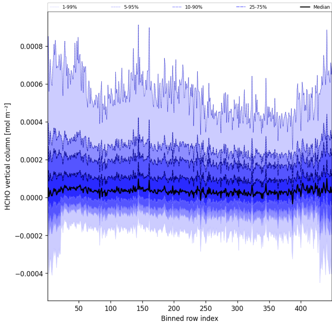
Figure 47: Along track statistics of “HCHO vertical column” for 2025-03-28 to 2025-03-29
