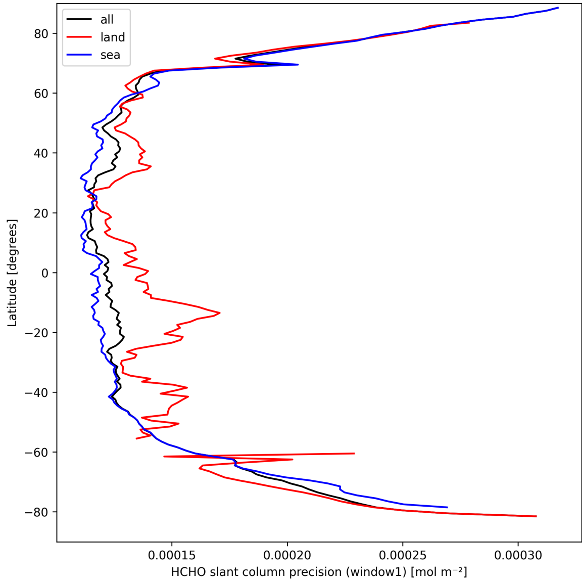
Figure 23: Zonal average of “HCHO slant column precision (window1)” for 2025-03-28 to 2025-03-29.
