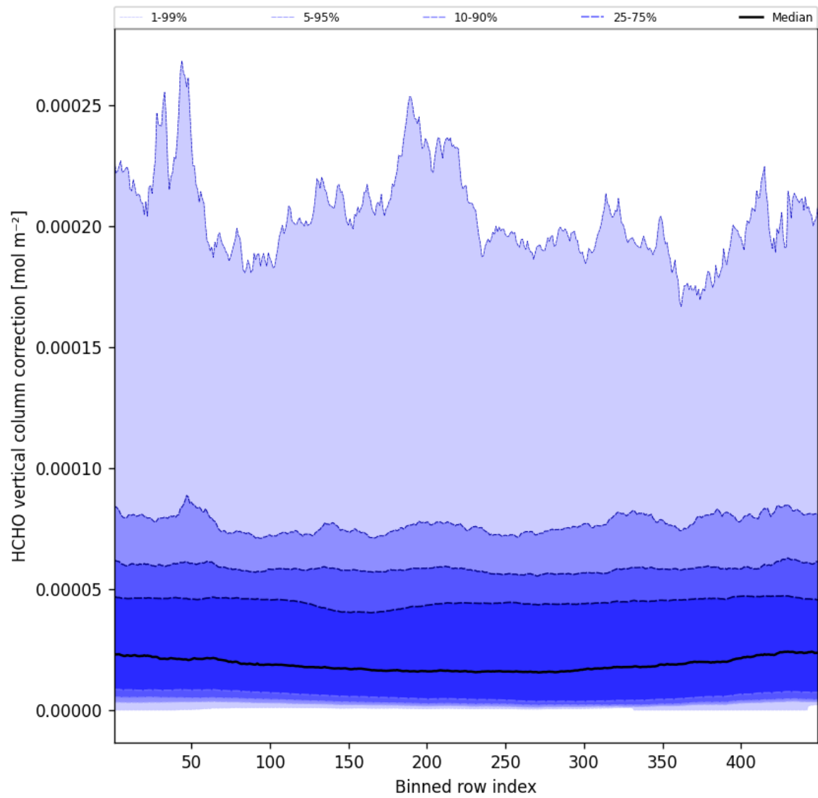
Figure 49: Along track statistics of “HCHO vertical column correction” for 2025-03-28 to 2025-03-29
