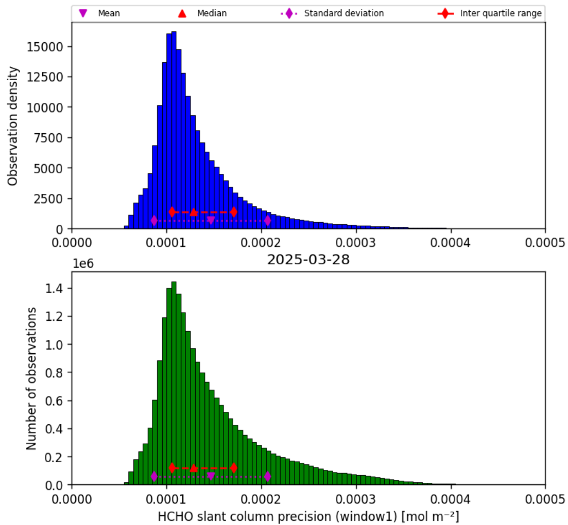
Figure 37: Histogram of “HCHO slant column precision (window1)” for 2025-03-28 to 2025-03-29
