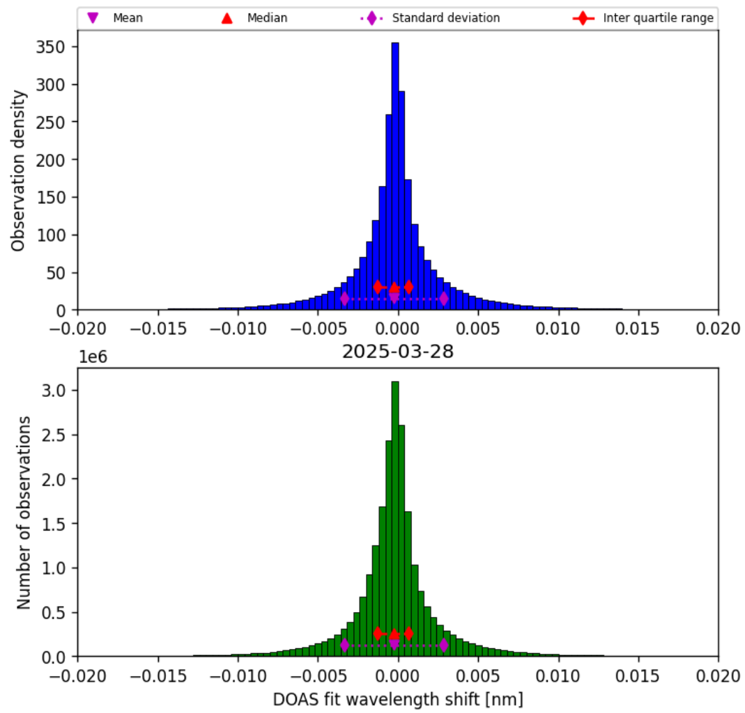
Figure 42: Histogram of “DOAS fit wavelength shift” for 2025-03-28 to 2025-03-29
