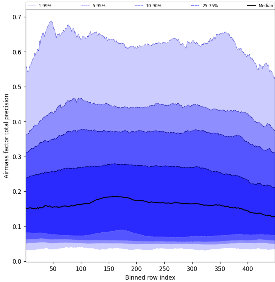
Figure 53: Along track statistics of “Airmass factor total precision” for 2025-03-28 to 2025-03-29
