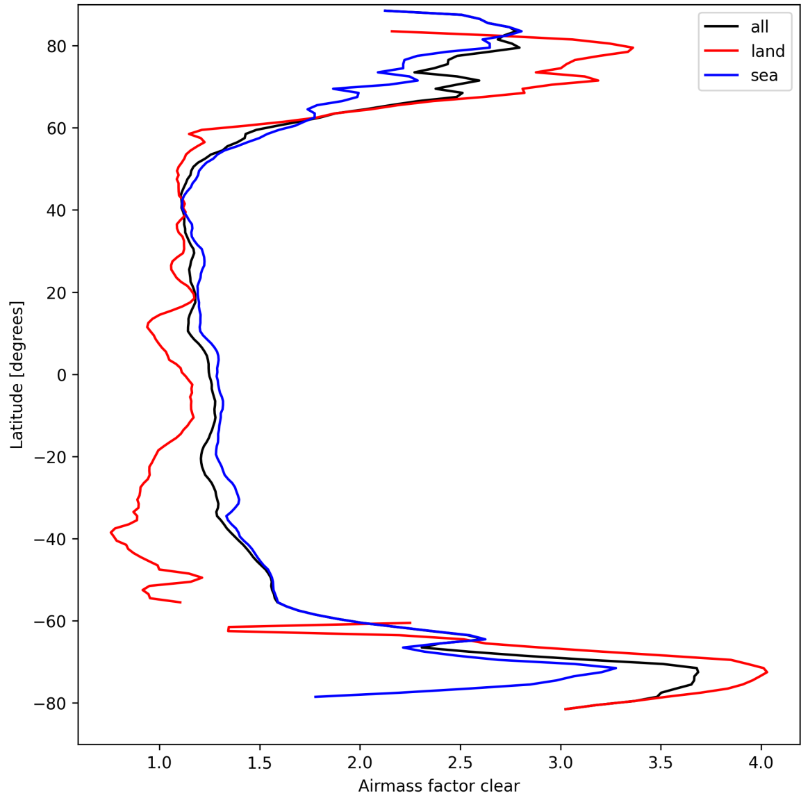
Figure 26: Zonal average of “Airmass factor clear” for 2025-03-28 to 2025-03-29.
