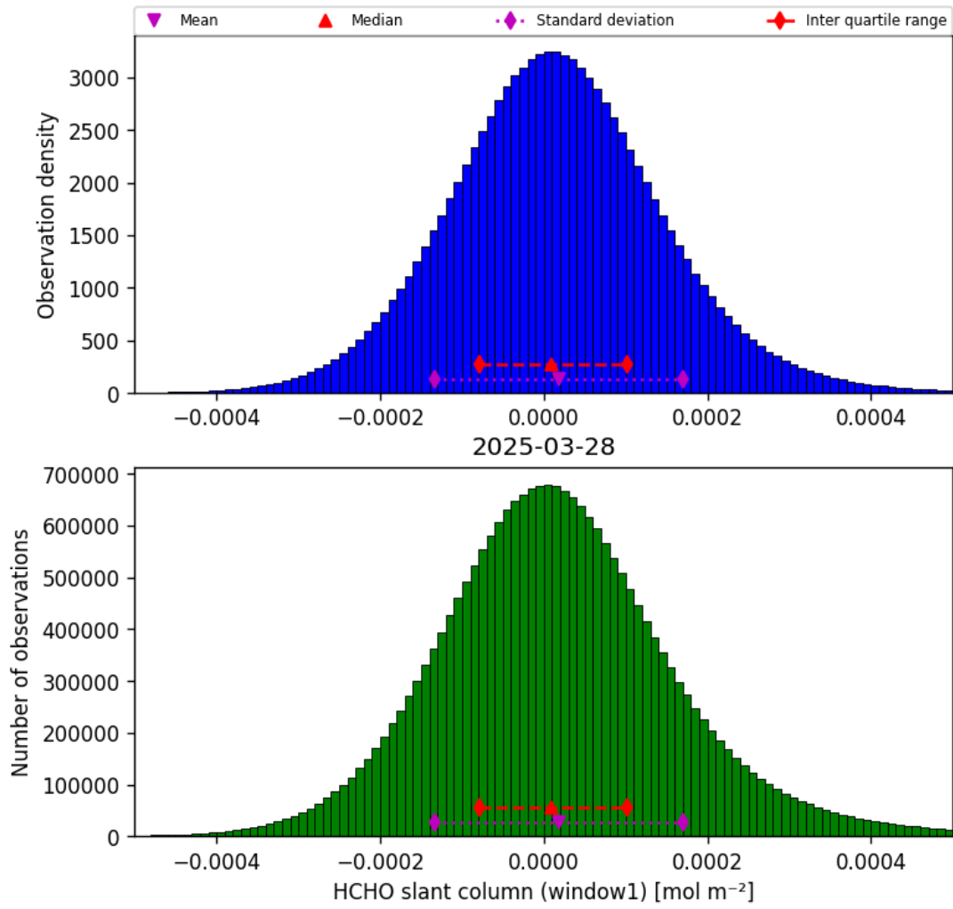
Figure 36: Histogram of “HCHO slant column (window1)” for 2025-03-28 to 2025-03-29
