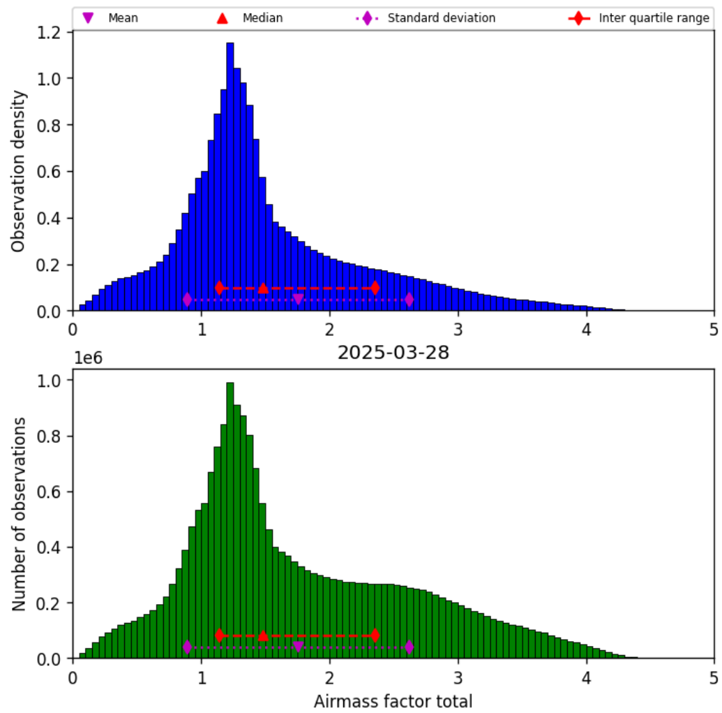
Figure 38: Histogram of “Airmass factor total” for 2025-03-28 to 2025-03-29
