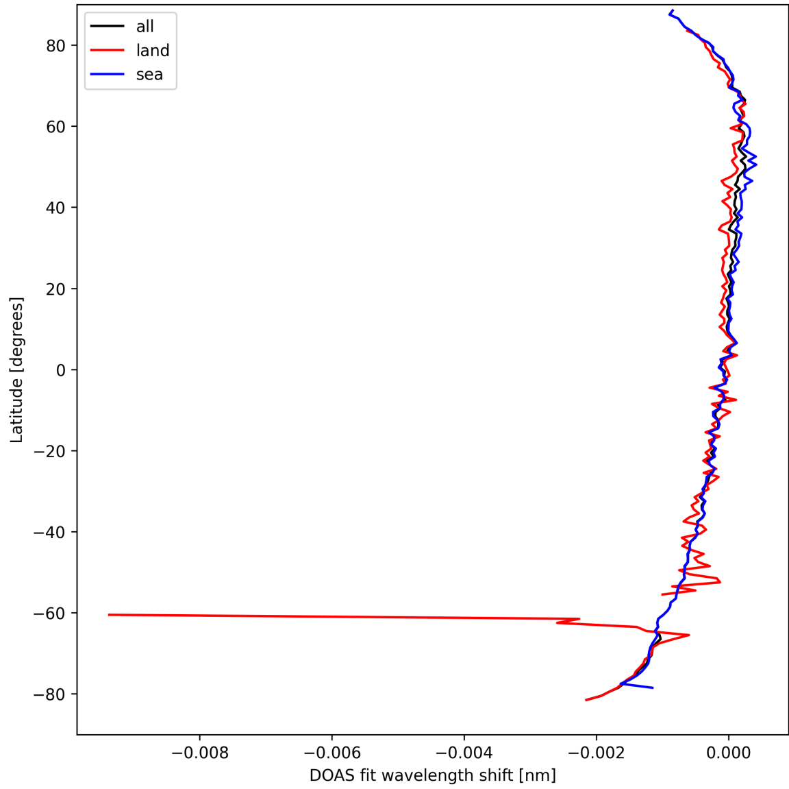
Figure 28: Zonal average of “DOAS fit wavelength shift” for 2025-03-28 to 2025-03-29.
