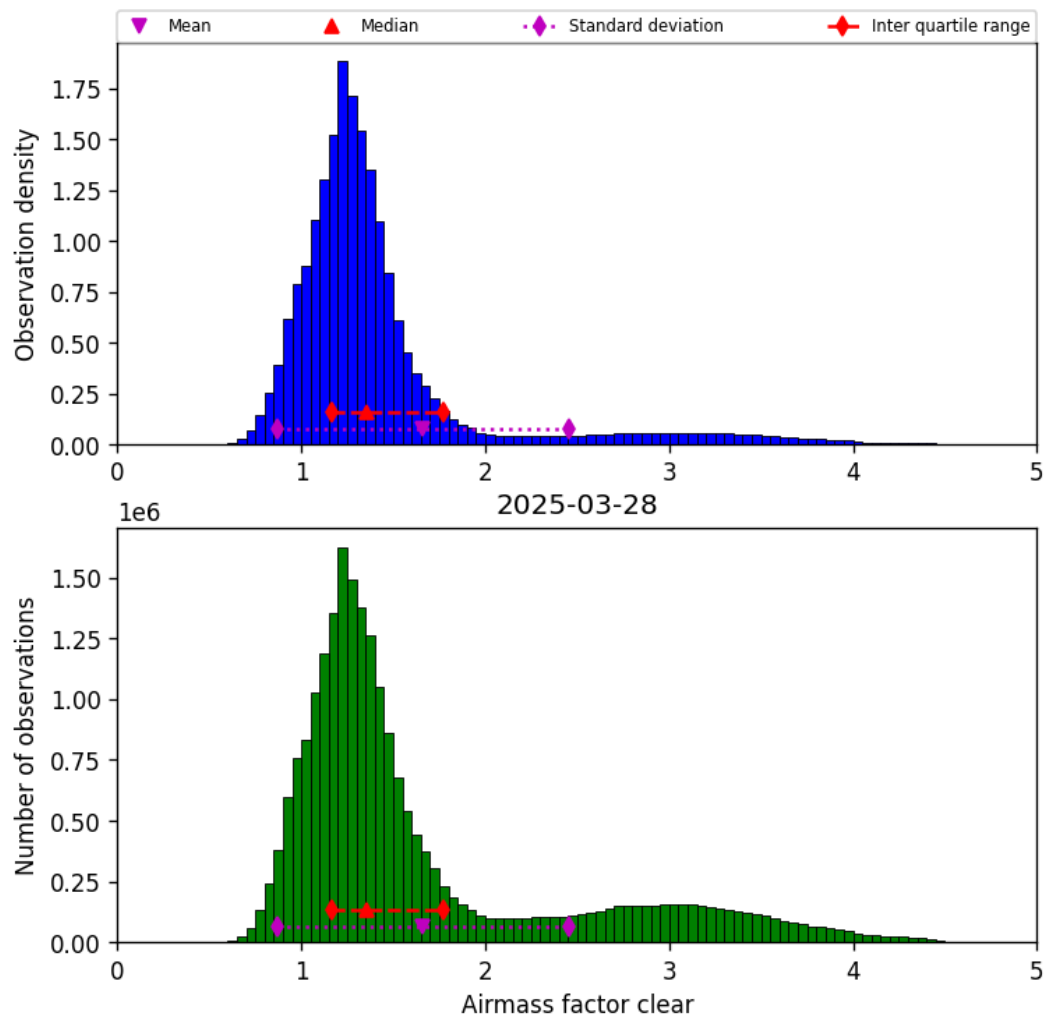
Figure 40: Histogram of “Airmass factor clear” for 2025-03-28 to 2025-03-29
