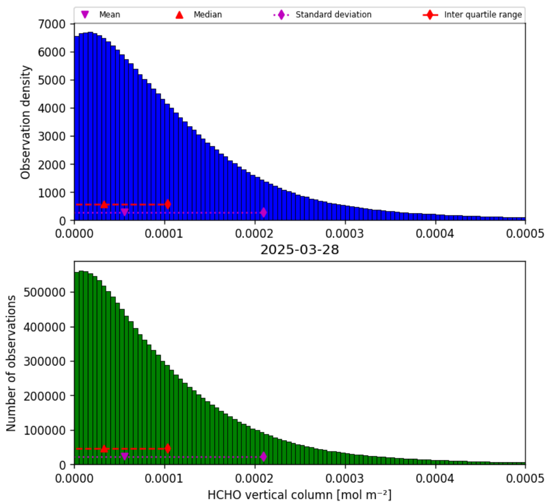
Figure 33: Histogram of “HCHO vertical column” for 2025-03-28 to 2025-03-29
