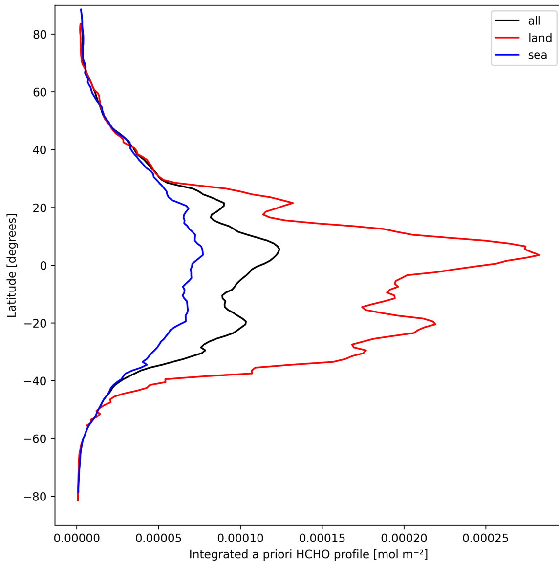
Figure 27: Zonal average of “Integrated a priori HCHO profile” for 2025-03-28 to 2025-03-29.
