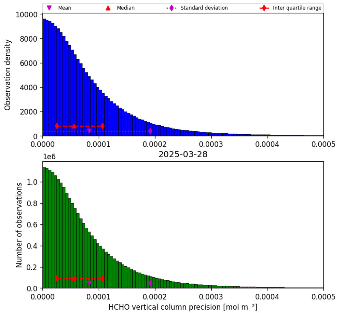
Figure 34: Histogram of “HCHO vertical column precision” for 2025-03-28 to 2025-03-29
