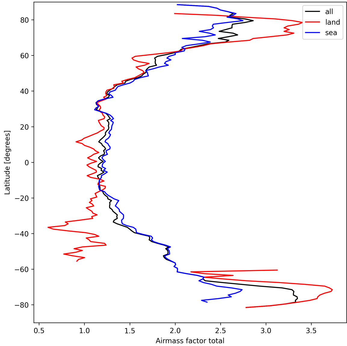
Figure 24: Zonal average of “Airmass factor total” for 2025-03-28 to 2025-03-29.
