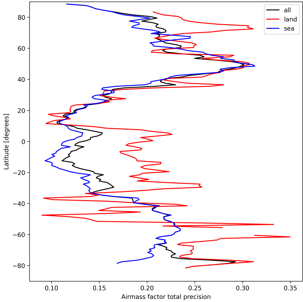
Figure 25: Zonal average of “Airmass factor total precision” for 2025-03-28 to 2025-03-29.
