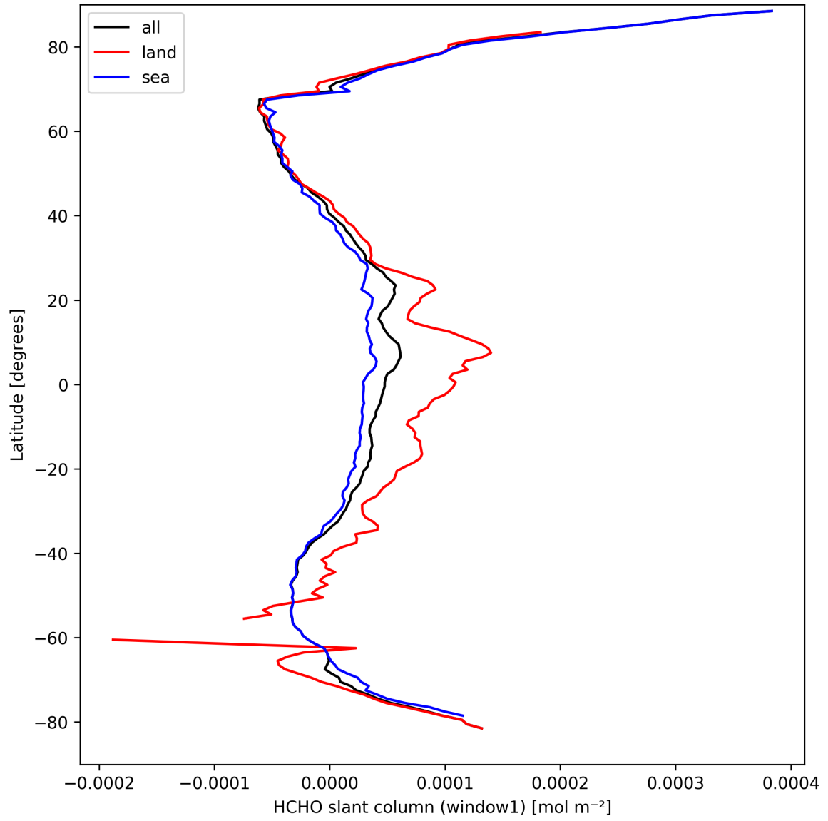
Figure 22: Zonal average of “HCHO slant column (window1)” for 2025-03-28 to 2025-03-29.
