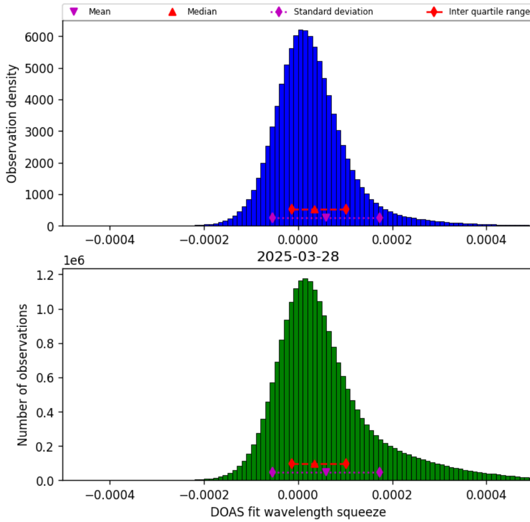
Figure 43: Histogram of “DOAS fit wavelength squeeze” for 2025-03-28 to 2025-03-29
