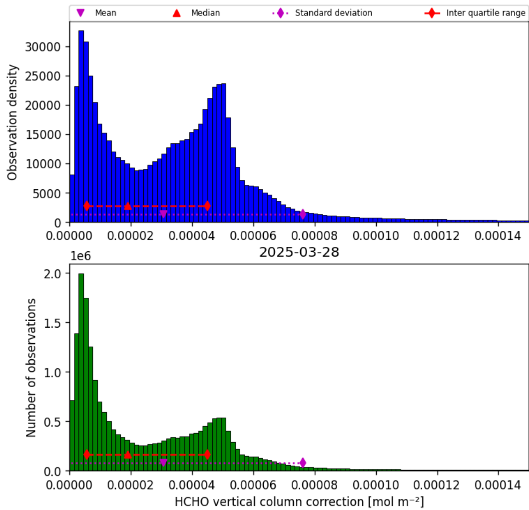
Figure 35: Histogram of “HCHO vertical column correction” for 2025-03-28 to 2025-03-29
