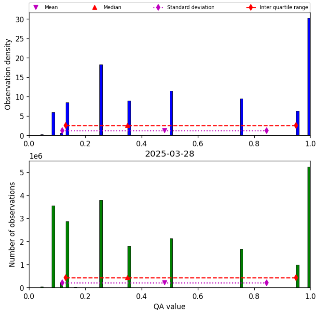
Figure 32: Histogram of “QA value” for 2025-03-28 to 2025-03-29
