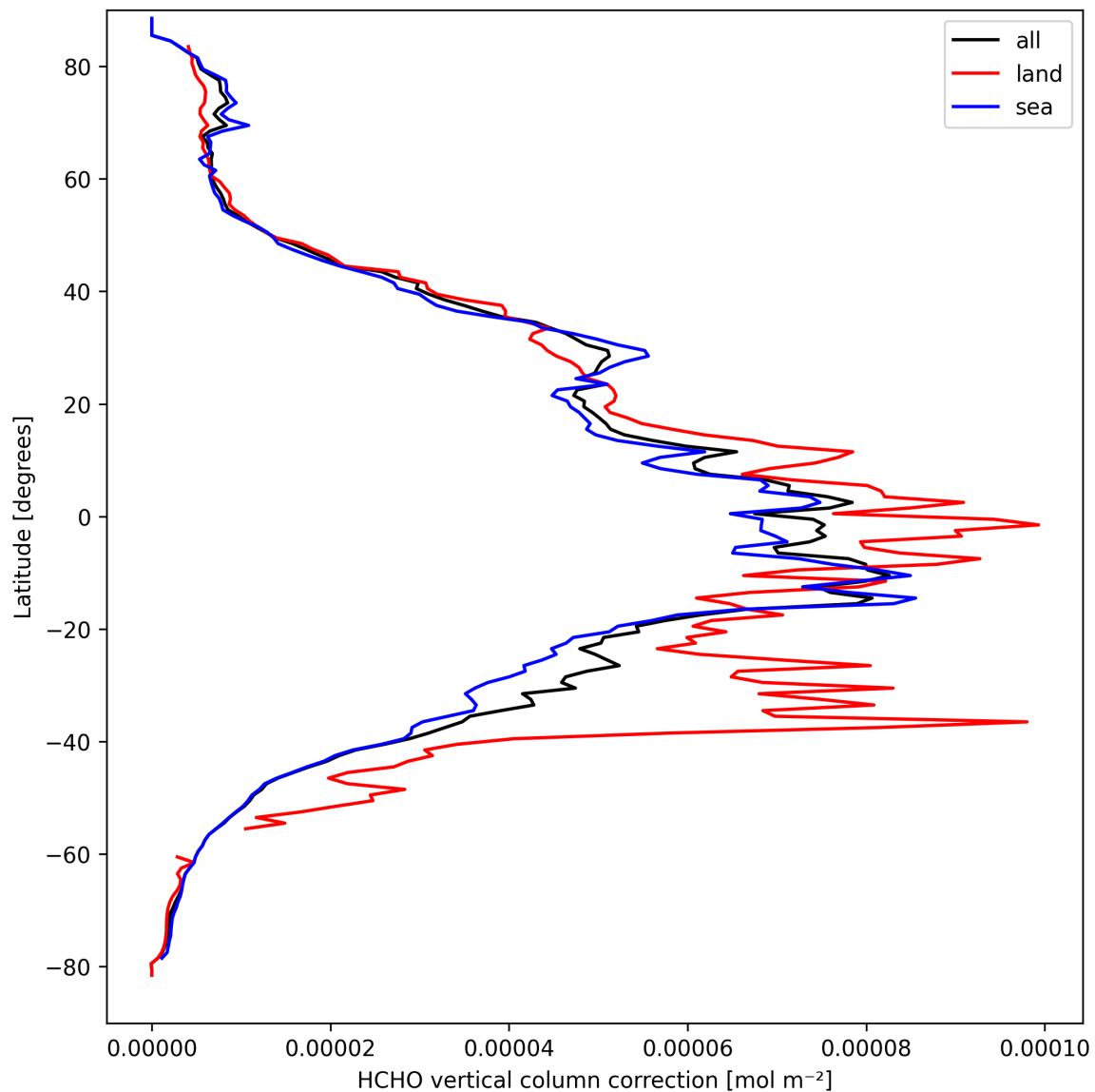
Figure 21: Zonal average of “HCHO vertical column correction” for 2025-03-28 to 2025-03-29.
