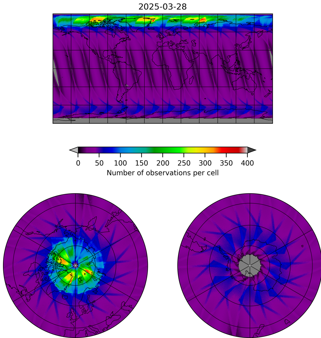
Figure 17: Map of the number of observations for 2025-03-28 to 2025-03-29
