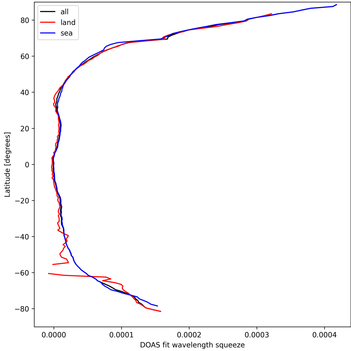
Figure 29: Zonal average of “DOAS fit wavelength squeeze” for 2025-03-28 to 2025-03-29.
