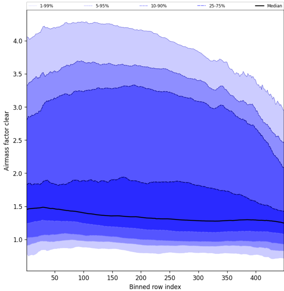
Figure 54: Along track statistics of “Airmass factor clear” for 2025-03-28 to 2025-03-29
