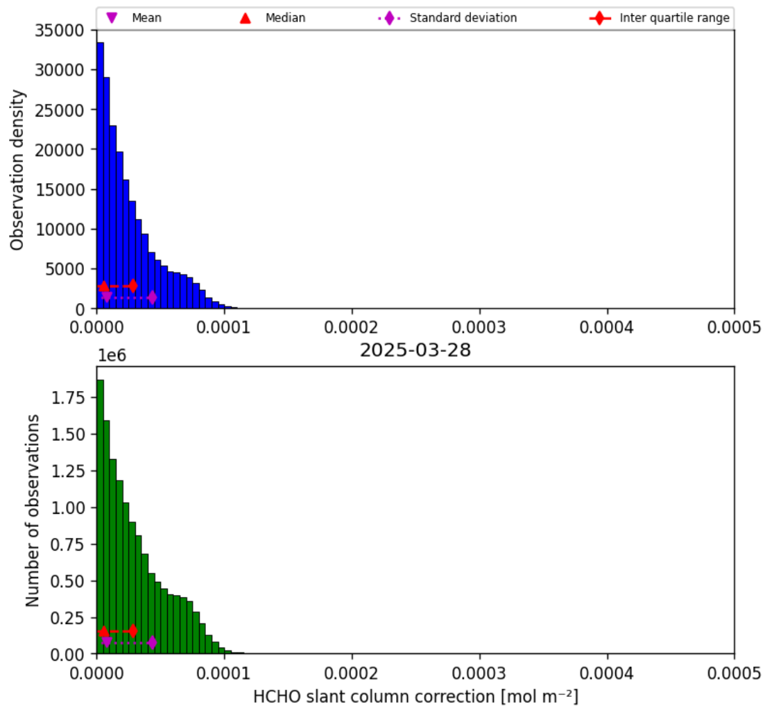
Figure 45: Histogram of “HCHO slant column correction” for 2025-03-28 to 2025-03-29
