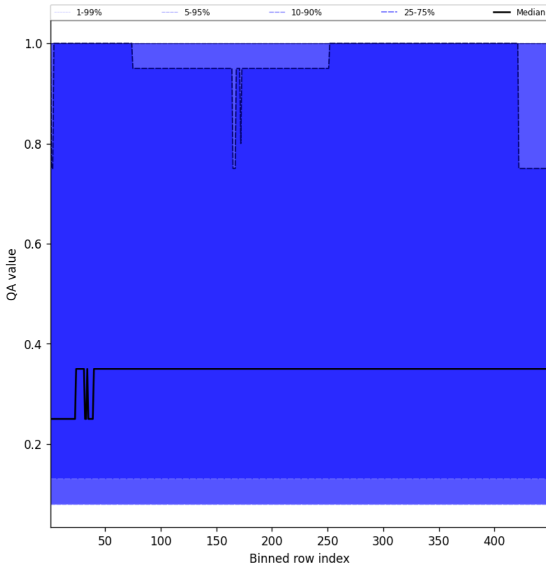
Figure 46: Along track statistics of “QA value” for 2025-03-28 to 2025-03-29
