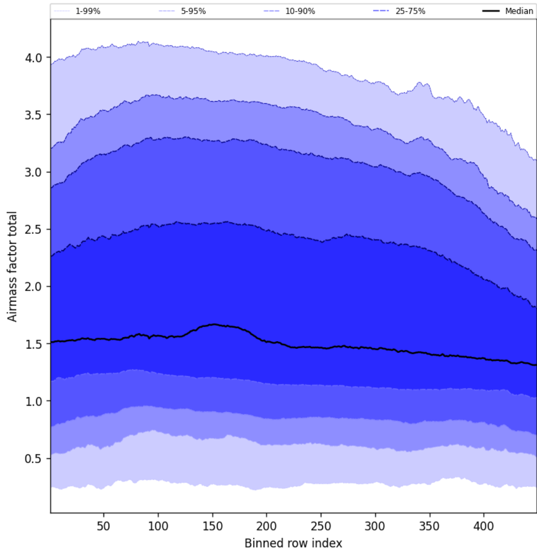
Figure 52: Along track statistics of “Airmass factor total” for 2025-03-28 to 2025-03-29
