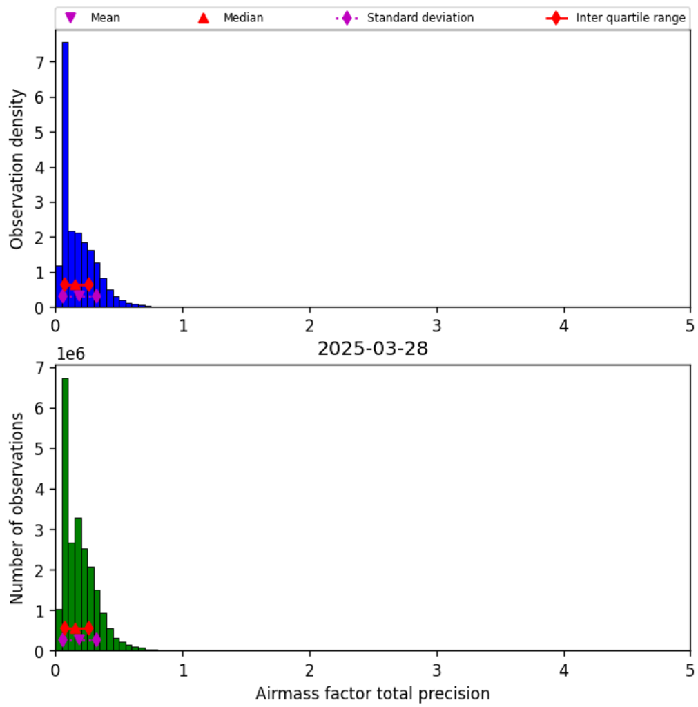
Figure 39: Histogram of “Airmass factor total precision” for 2025-03-28 to 2025-03-29
