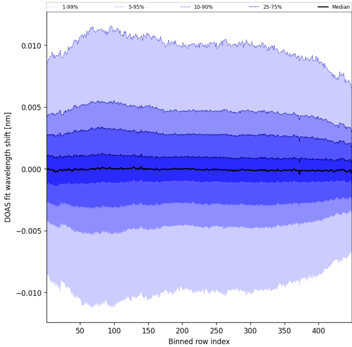
Figure 56: Along track statistics of “DOAS fit wavelength shift” for 2025-03-29 to 2025-03-30
