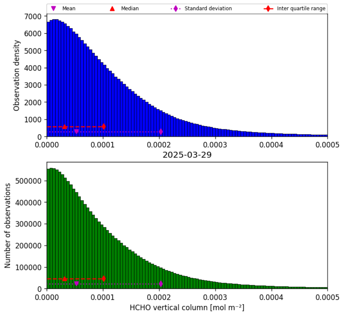
Figure 33: Histogram of “HCHO vertical column” for 2025-03-29 to 2025-03-30
