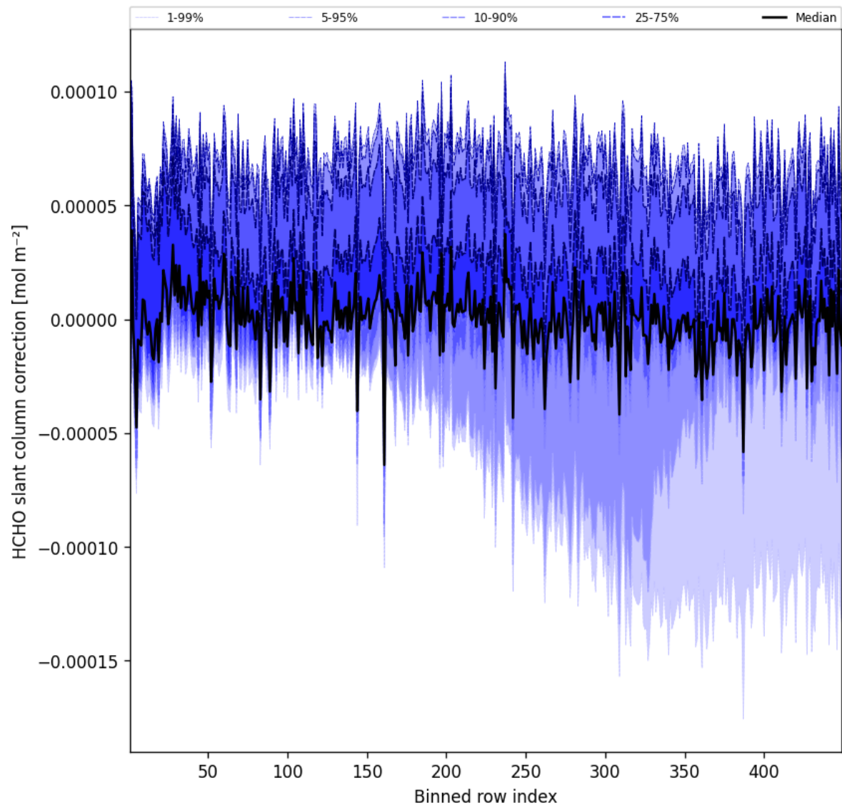
Figure 59: Along track statistics of “HCHO slant column correction” for 2025-03-29 to 2025-03-30
