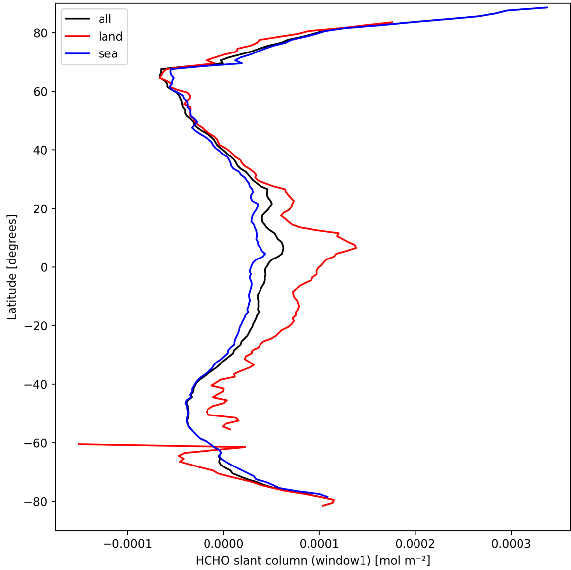
Figure 22: Zonal average of “HCHO slant column (window1)” for 2025-03-29 to 2025-03-30.
