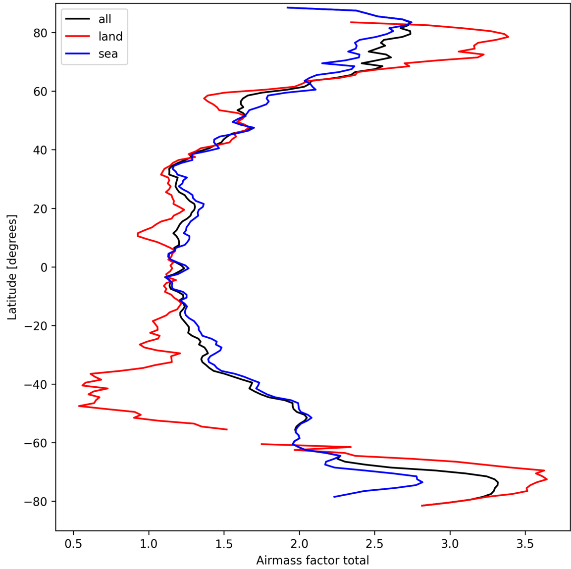
Figure 24: Zonal average of “Airmass factor total” for 2025-03-29 to 2025-03-30.
