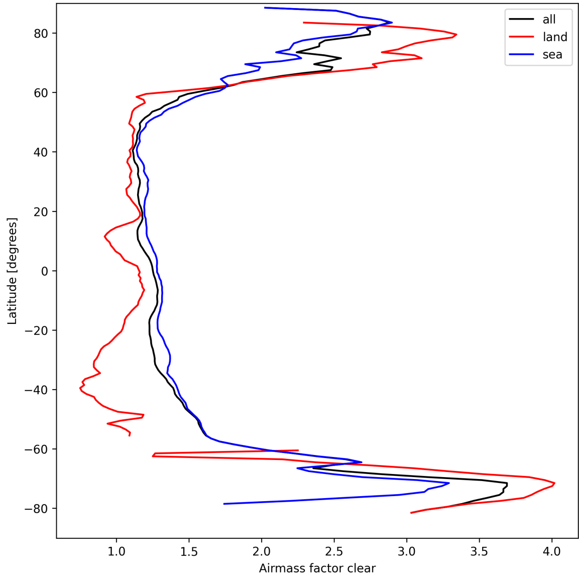
Figure 26: Zonal average of “Airmass factor clear” for 2025-03-29 to 2025-03-30.
