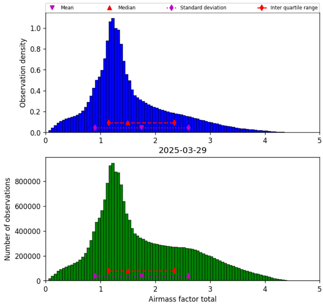
Figure 38: Histogram of “Airmass factor total” for 2025-03-29 to 2025-03-30
