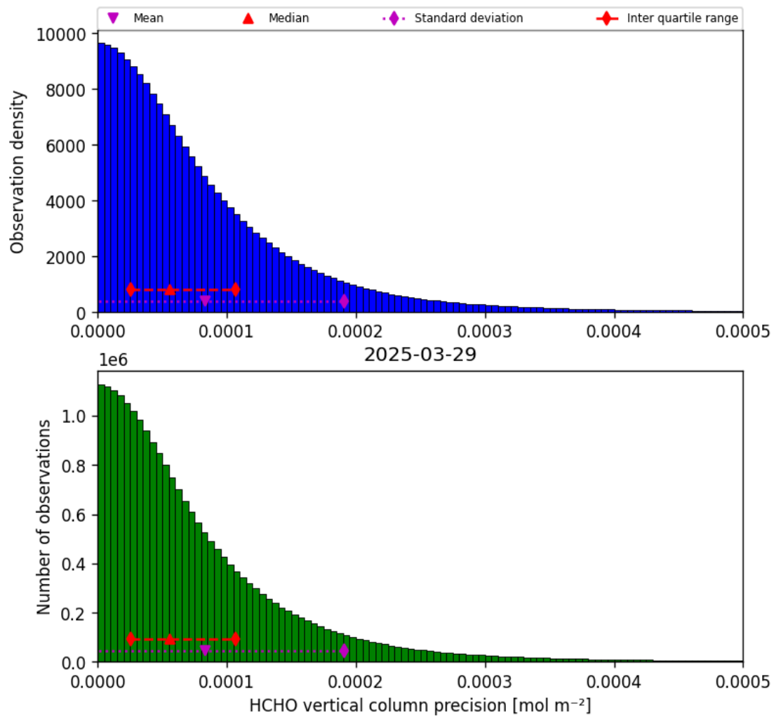
Figure 34: Histogram of “HCHO vertical column precision” for 2025-03-29 to 2025-03-30
