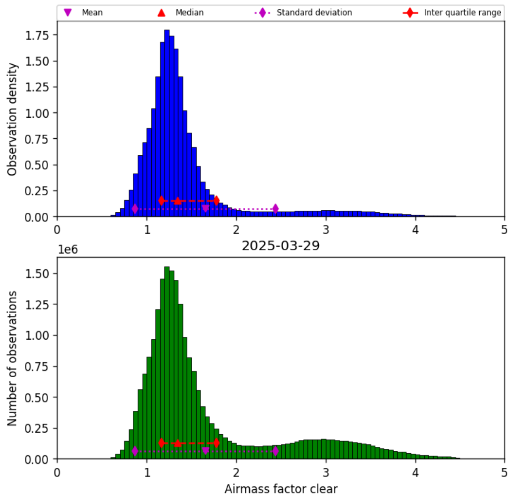
Figure 40: Histogram of “Airmass factor clear” for 2025-03-29 to 2025-03-30
