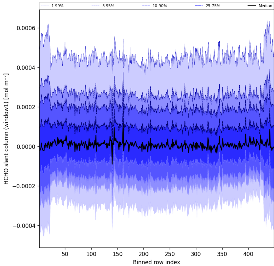
Figure 50: Along track statistics of “HCHO slant column (window1)” for 2025-03-29 to 2025-03-30
