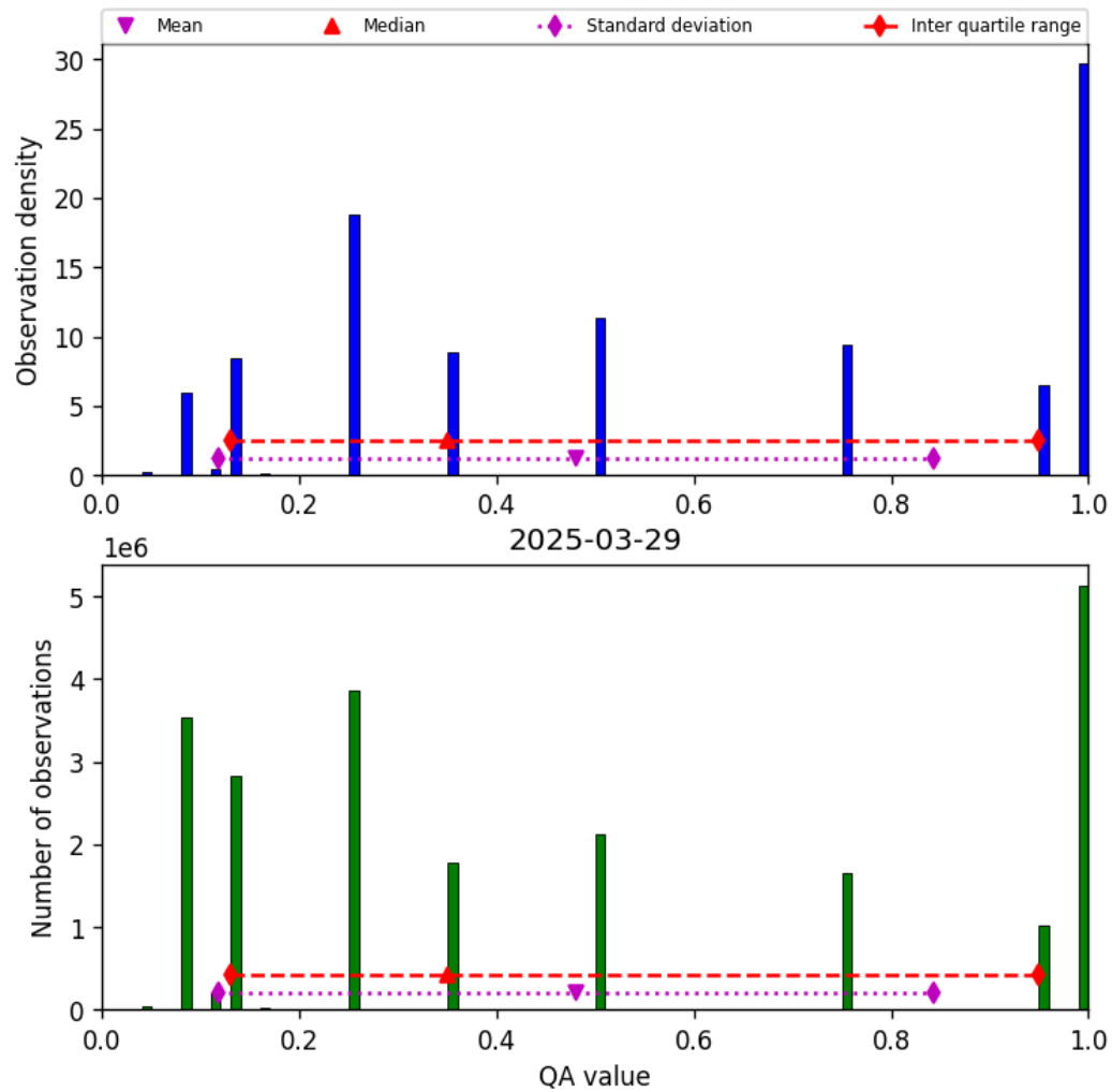
Figure 32: Histogram of “QA value” for 2025-03-29 to 2025-03-30
