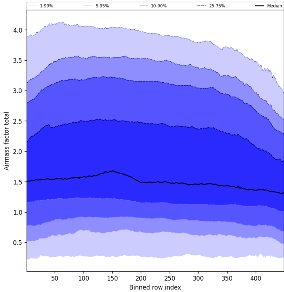
Figure 52: Along track statistics of “Airmass factor total” for 2025-03-29 to 2025-03-30
