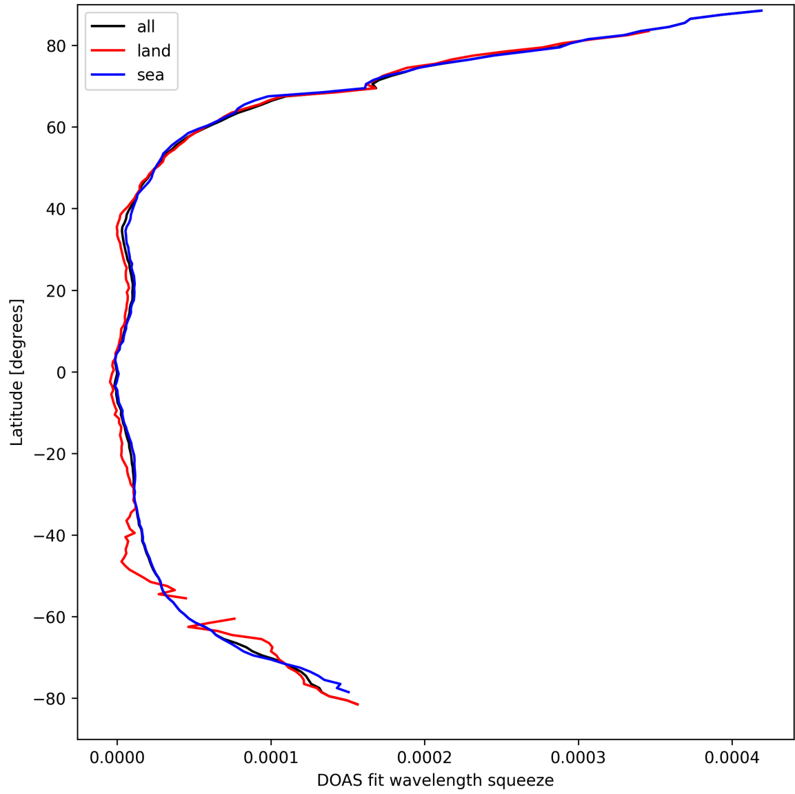
Figure 29: Zonal average of “DOAS fit wavelength squeeze” for 2025-03-29 to 2025-03-30.
