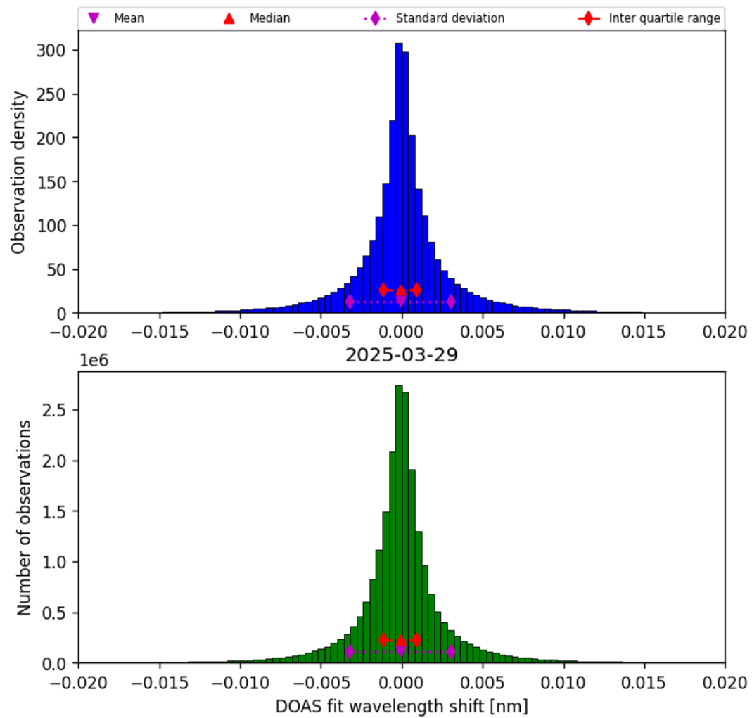
Figure 42: Histogram of “DOAS fit wavelength shift” for 2025-03-29 to 2025-03-30
