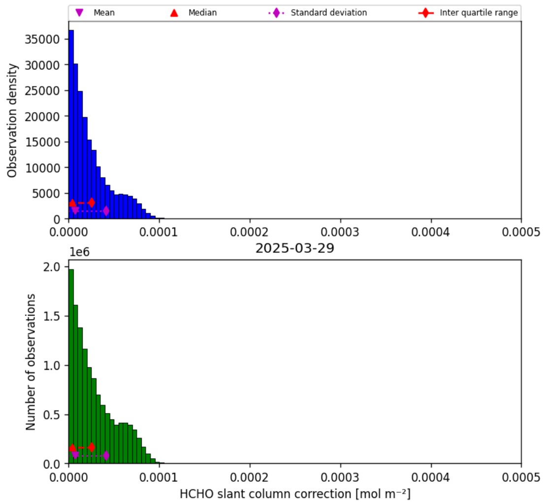
Figure 45: Histogram of “HCHO slant column correction” for 2025-03-29 to 2025-03-30
