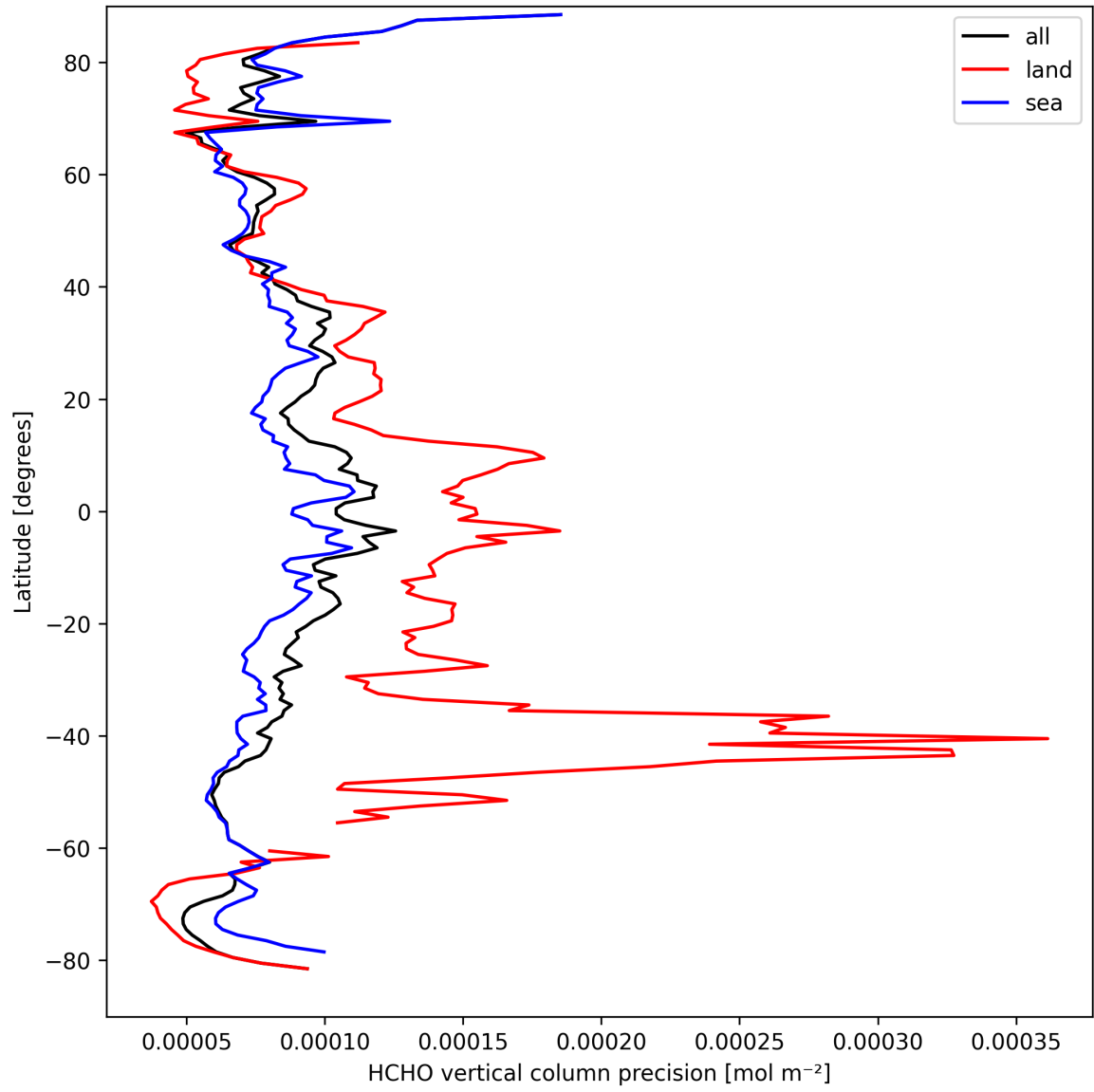
Figure 20: Zonal average of “HCHO vertical column precision” for 2025-03-29 to 2025-03-30.
