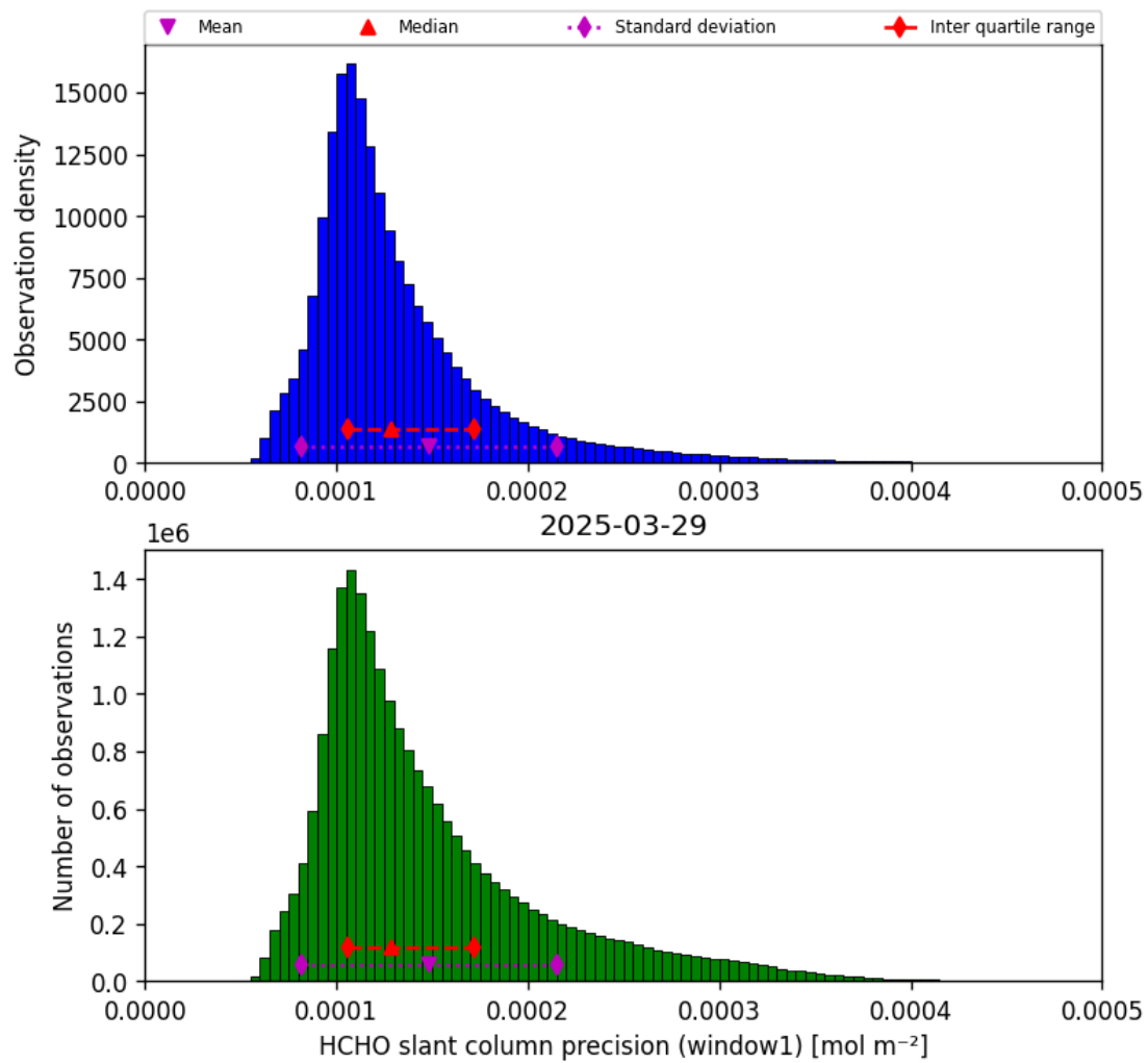
Figure 37: Histogram of “HCHO slant column precision (window1)” for 2025-03-29 to 2025-03-30
