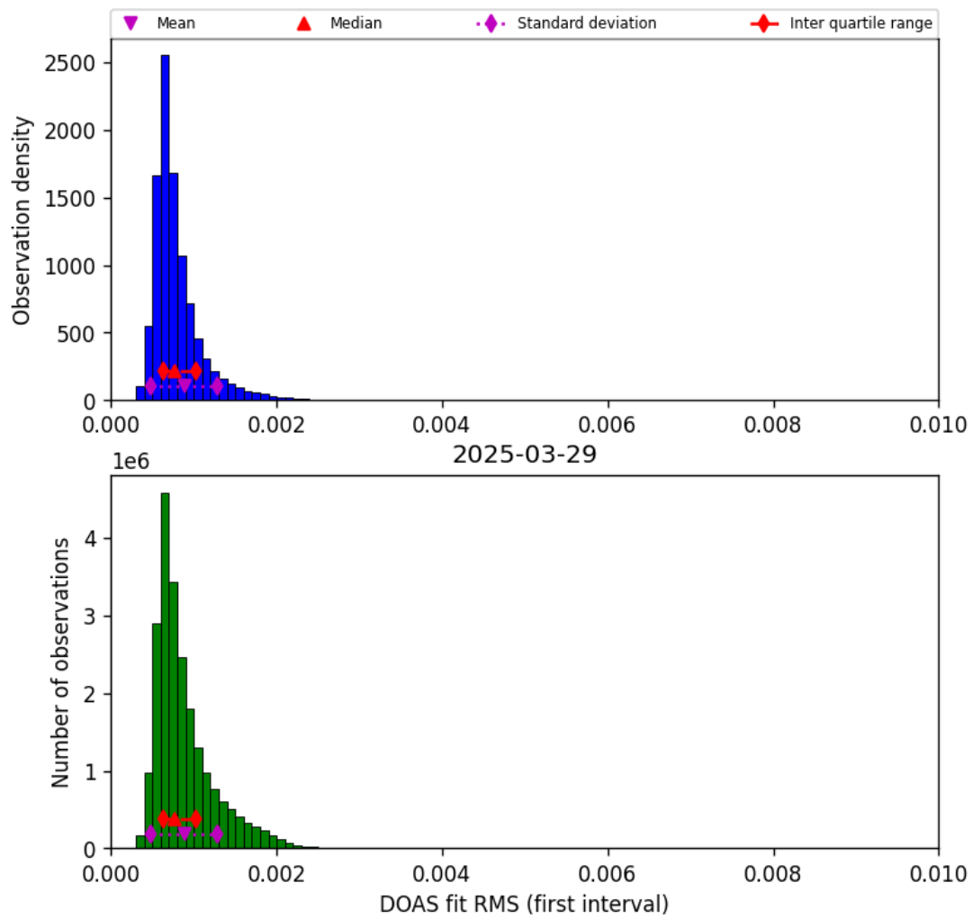
Figure 44: Histogram of “DOAS fit RMS (first interval)” for 2025-03-29 to 2025-03-30
