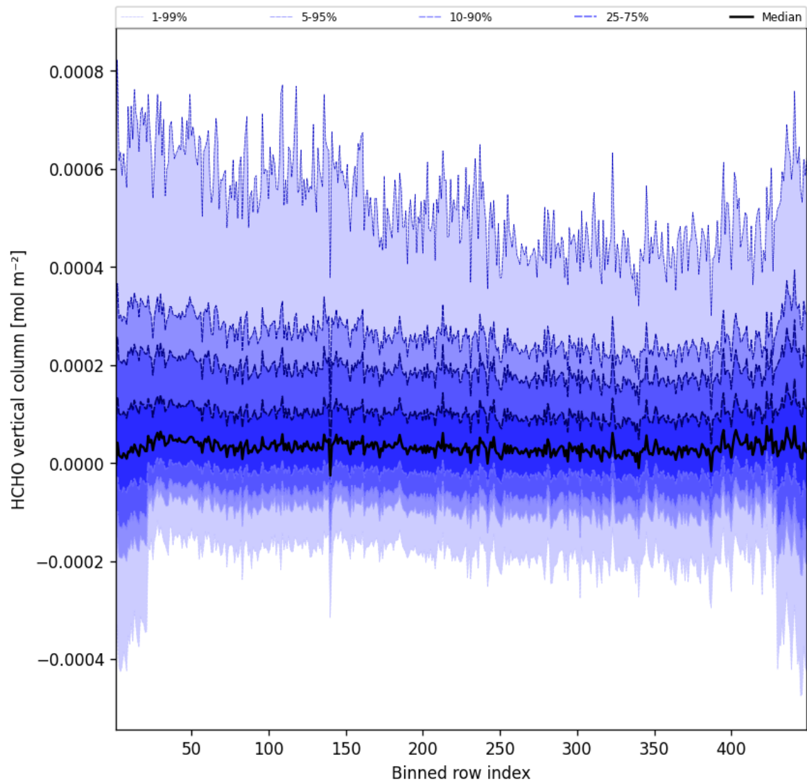
Figure 47: Along track statistics of “HCHO vertical column” for 2025-03-29 to 2025-03-30
