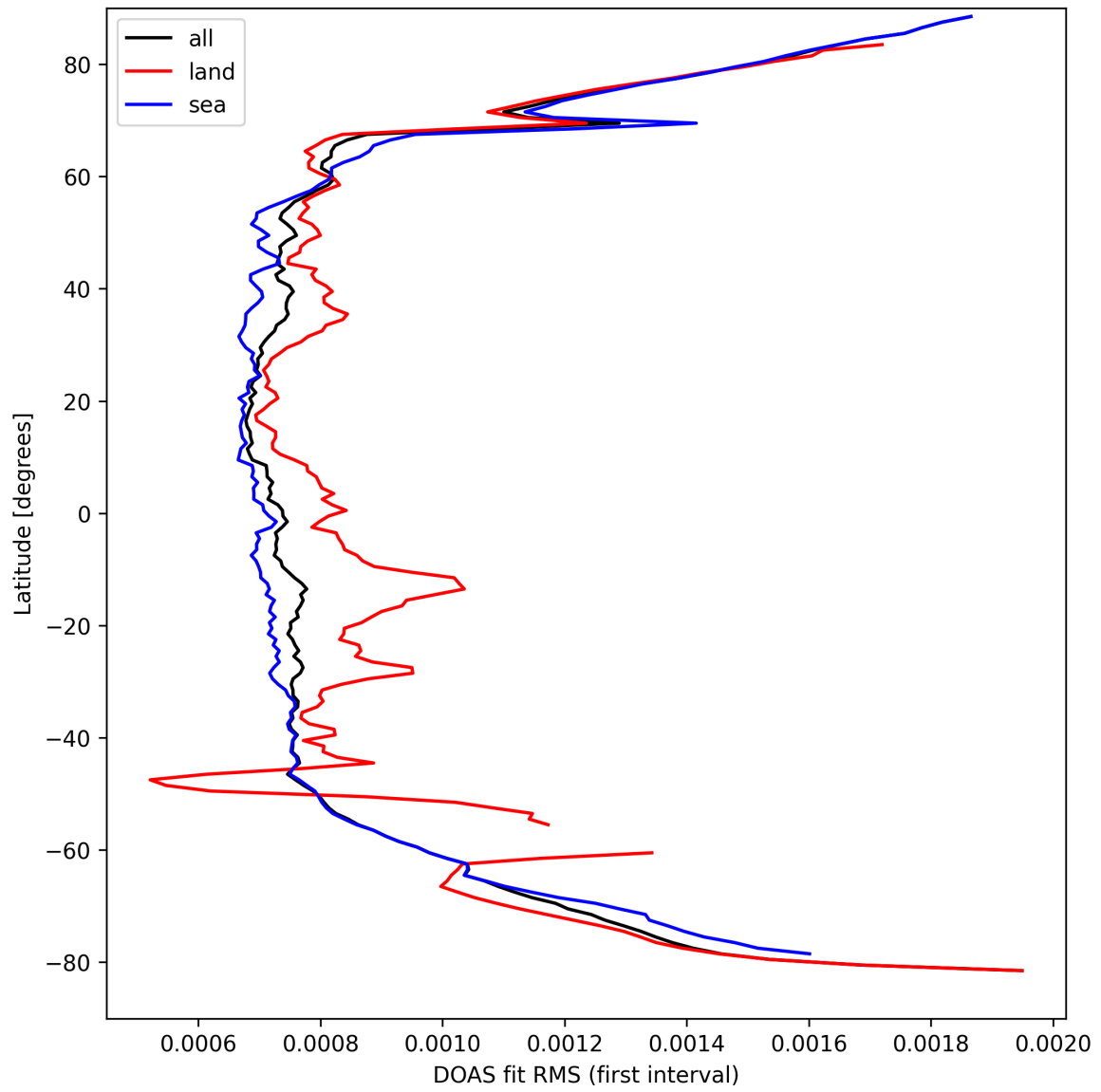
Figure 30: Zonal average of “DOAS fit RMS (first interval)” for 2025-03-29 to 2025-03-30.
