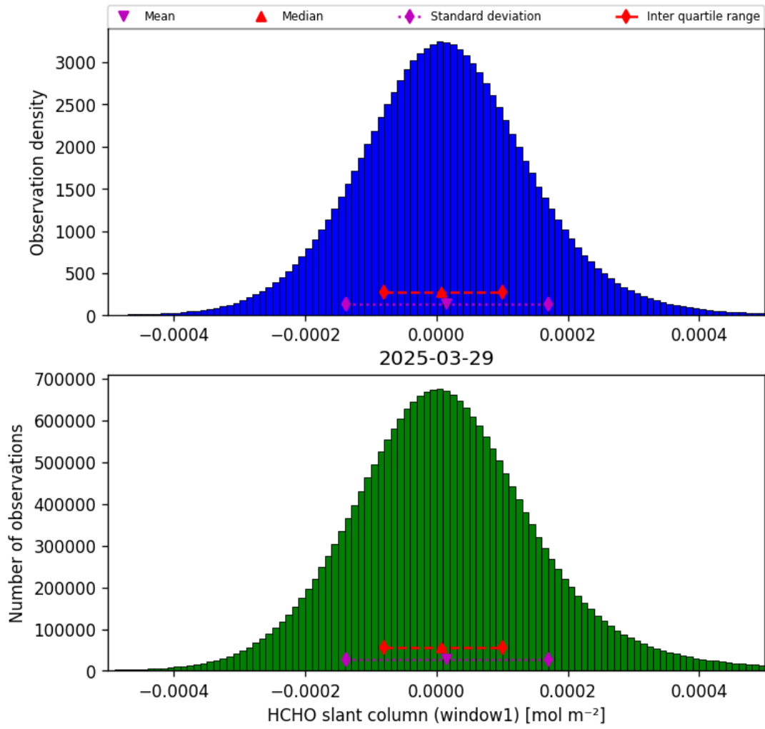
Figure 36: Histogram of “HCHO slant column (window1)” for 2025-03-29 to 2025-03-30
