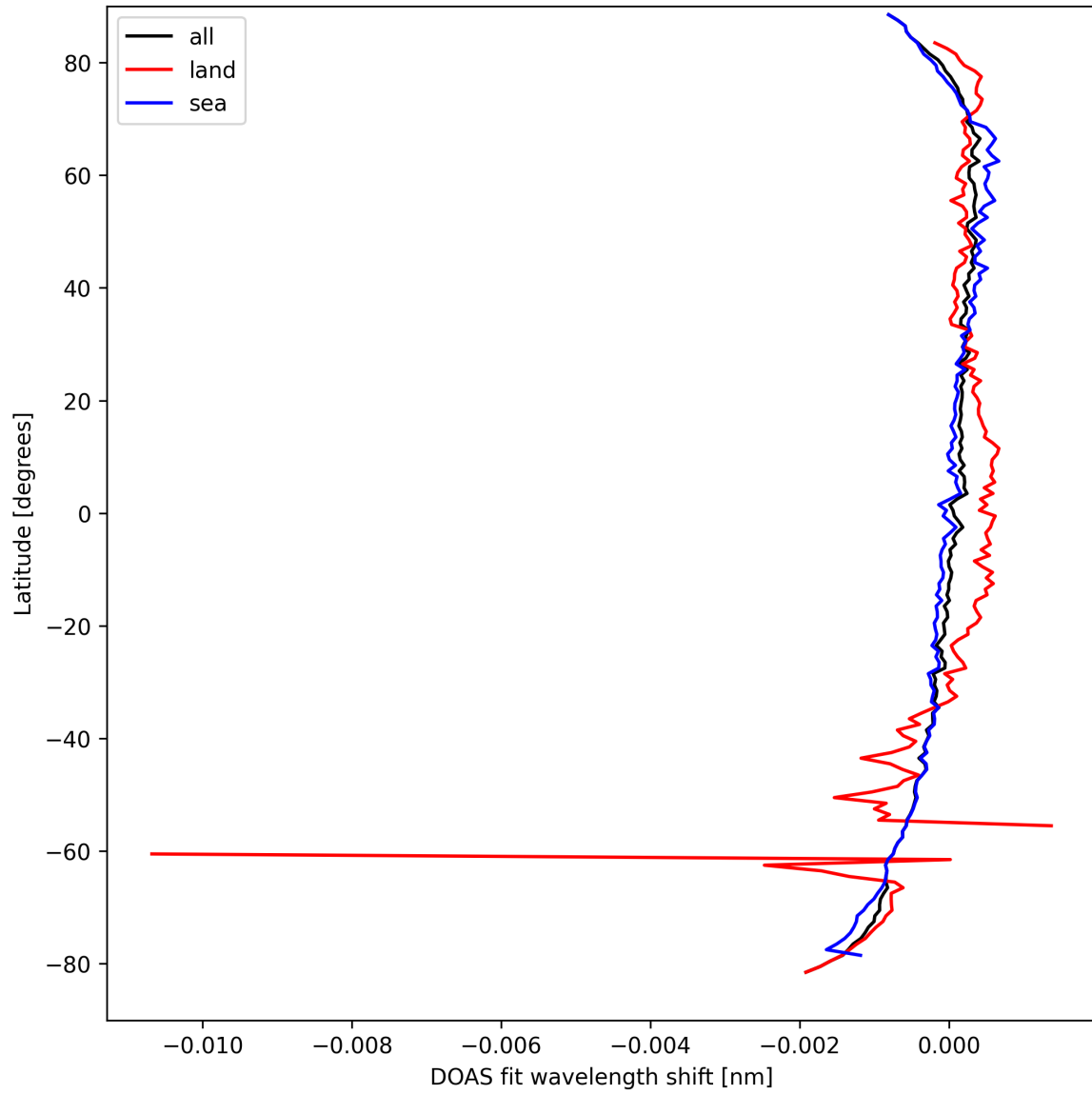
Figure 28: Zonal average of “DOAS fit wavelength shift” for 2025-03-29 to 2025-03-30.
