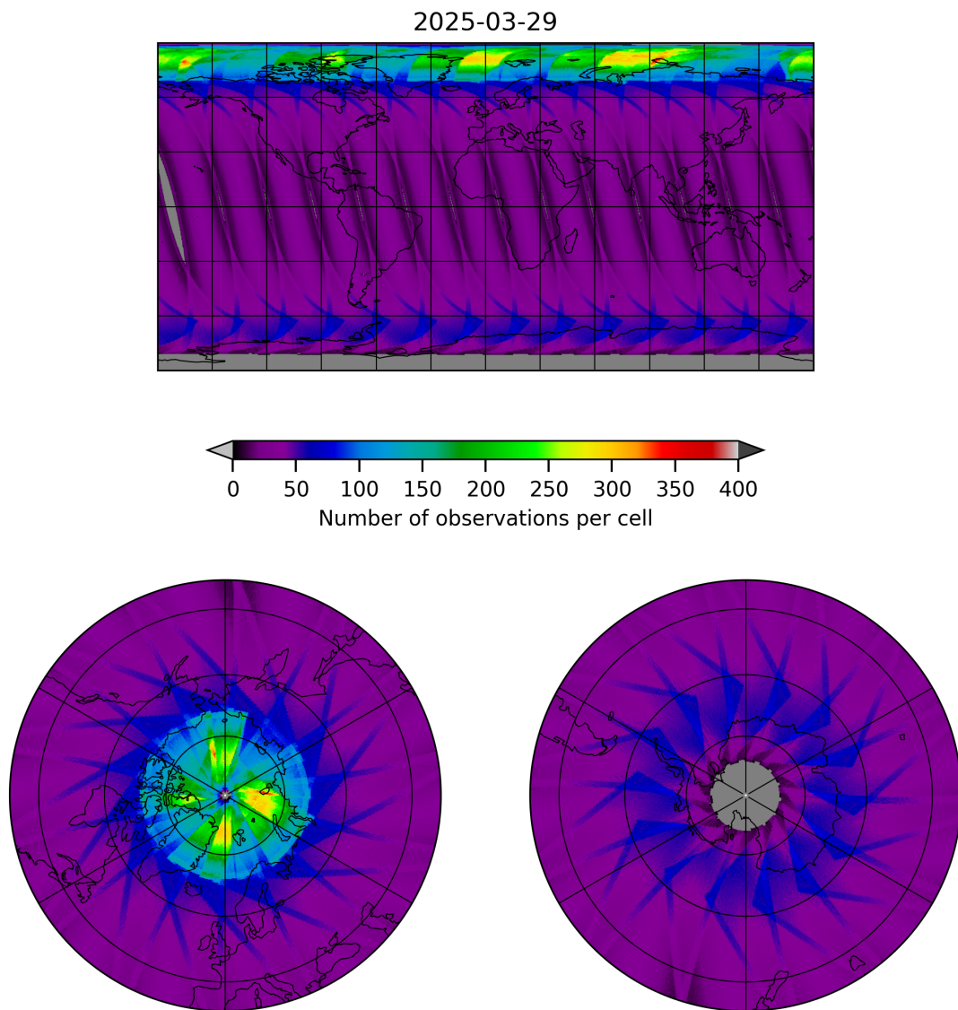
Figure 17: Map of the number of observations for 2025-03-29 to 2025-03-30
