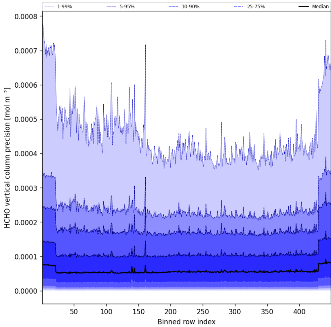
Figure 48: Along track statistics of “HCHO vertical column precision” for 2025-03-29 to 2025-03-30
