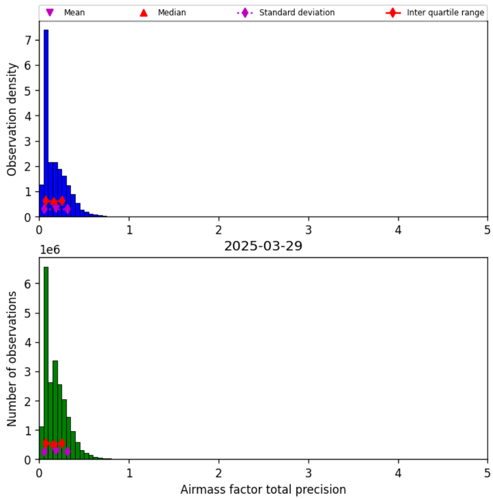
Figure 39: Histogram of “Airmass factor total precision” for 2025-03-29 to 2025-03-30
