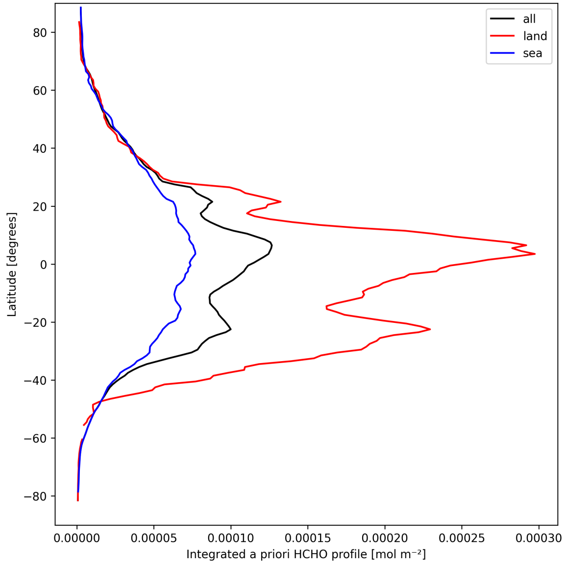
Figure 27: Zonal average of “Integrated a priori HCHO profile” for 2025-03-29 to 2025-03-30.
