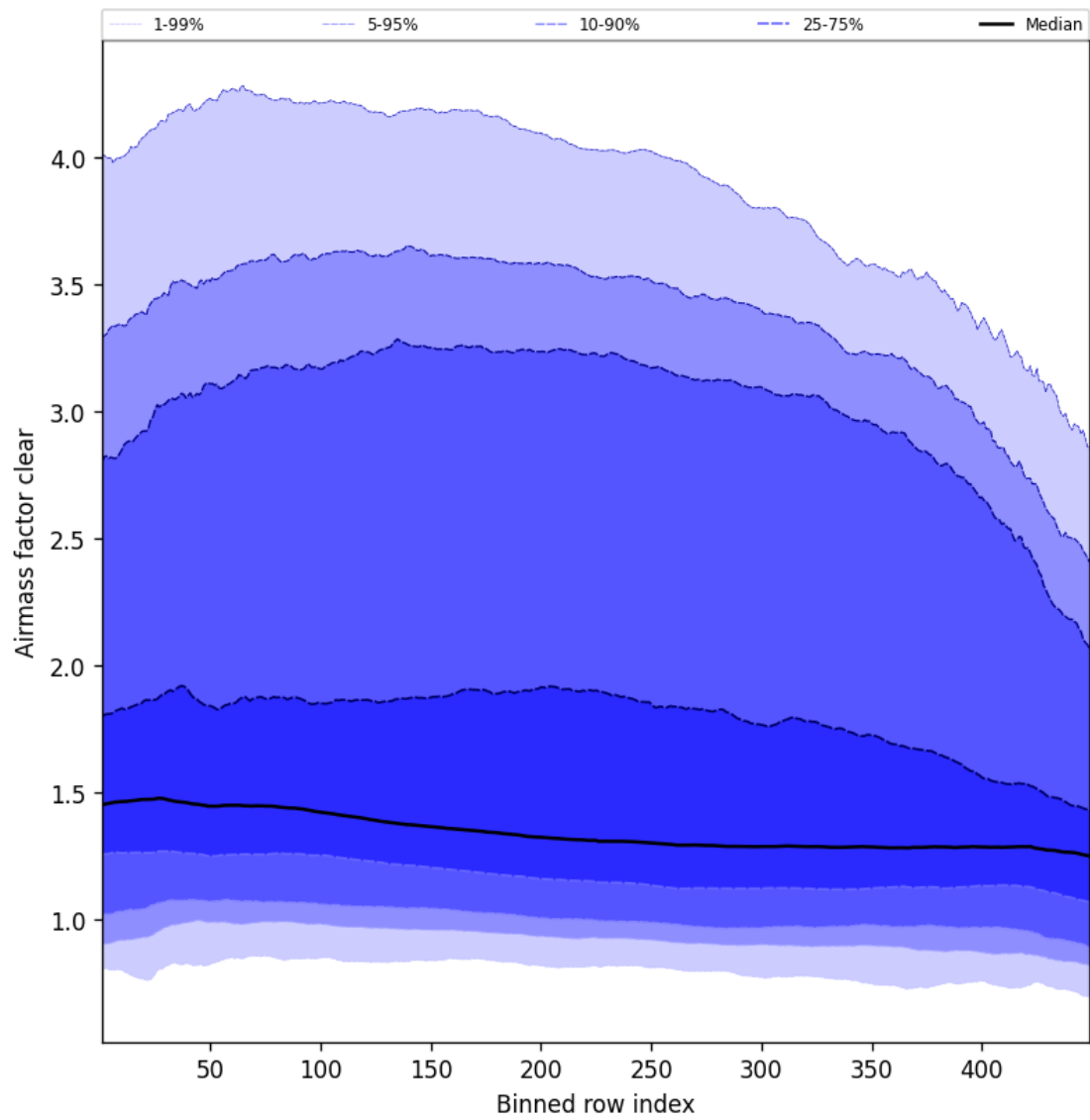
Figure 54: Along track statistics of “Air mass factor clear” for 2025-03-29 to 2025-03-30
