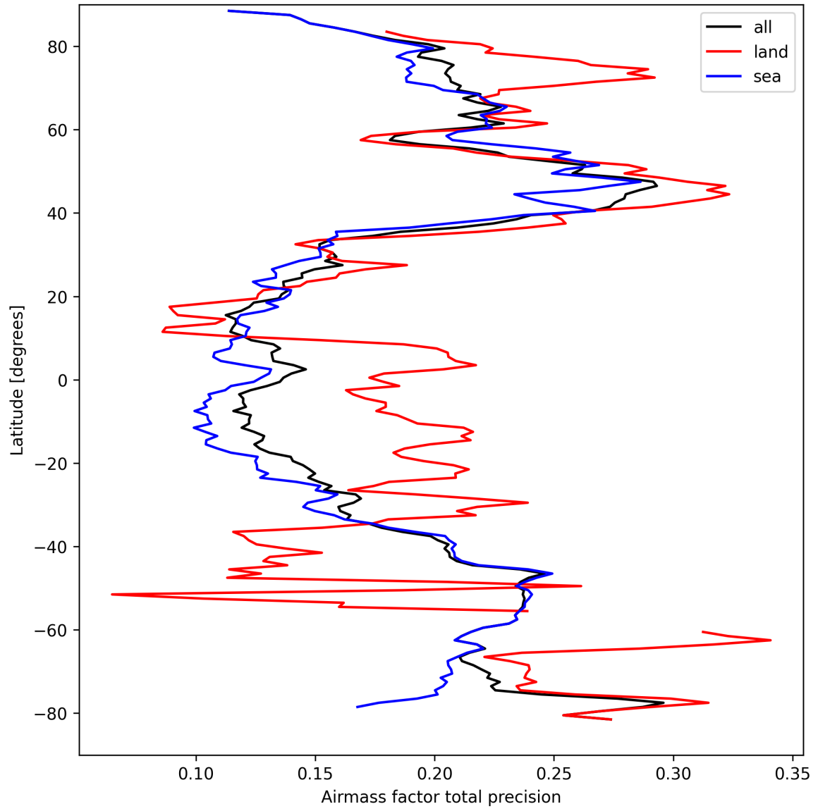
Figure 25: Zonal average of “Airmass factor total precision” for 2025-03-29 to 2025-03-30.
