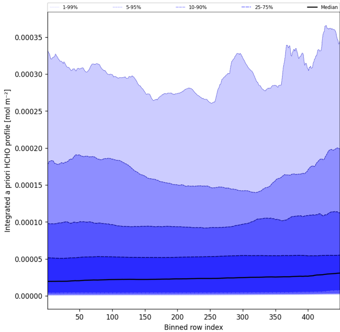
Figure 55: Along track statistics of "Integrated a priori HCHO profile" for 2025-03-29 to 2025-03-30
