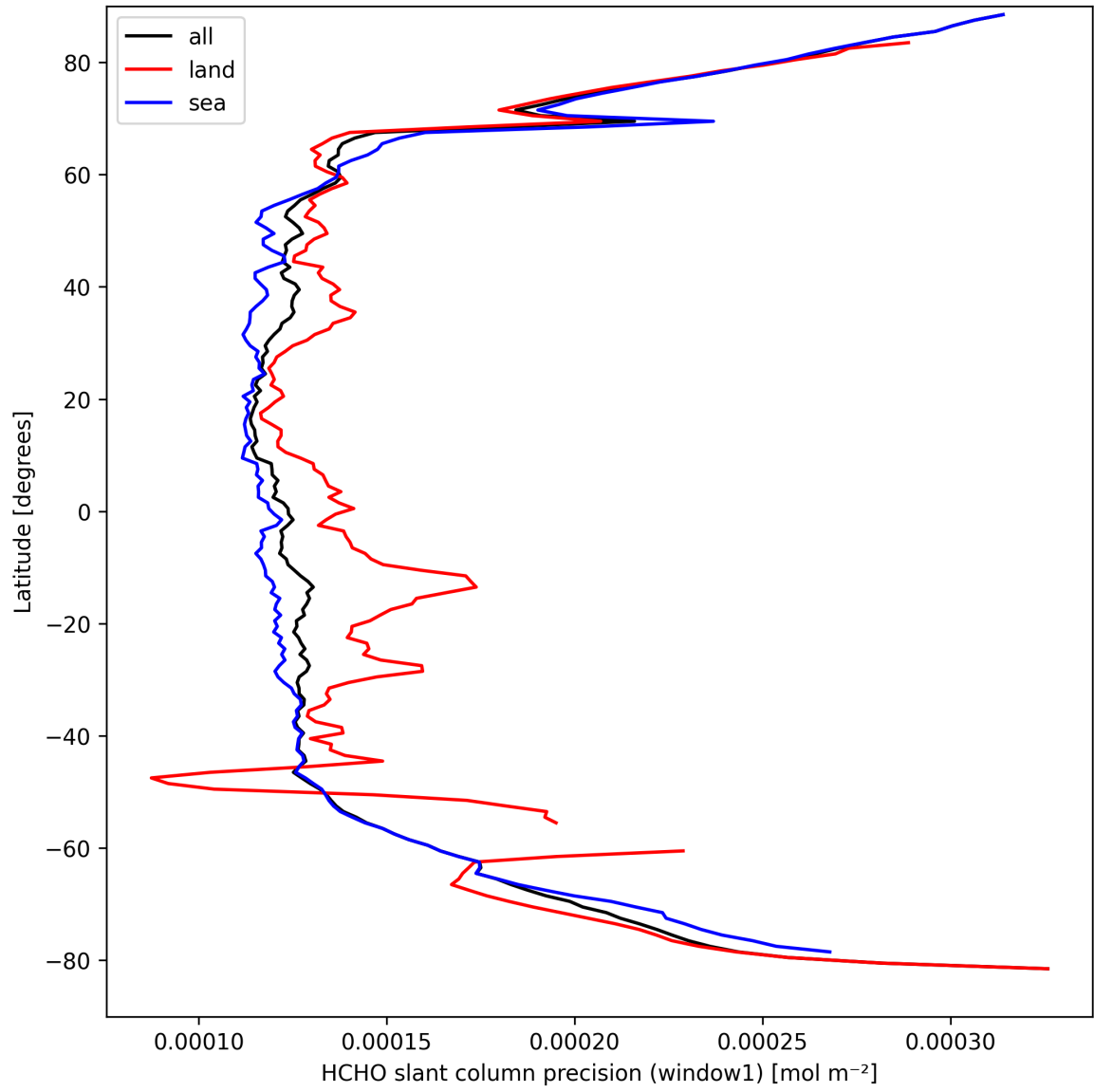
Figure 23: Zonal average of “HCHO slant column precision (window1)” for 2025-03-29 to 2025-03-30.
