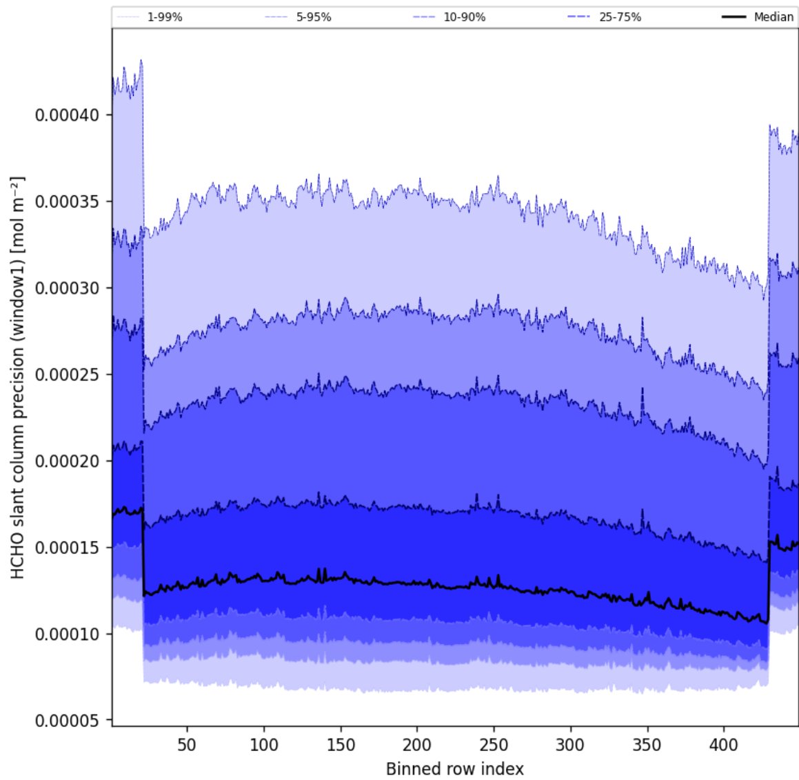
Figure 51: Along track statistics of “HCHO slant column precision (window1)” for 2025-03-29 to 2025-03-30
