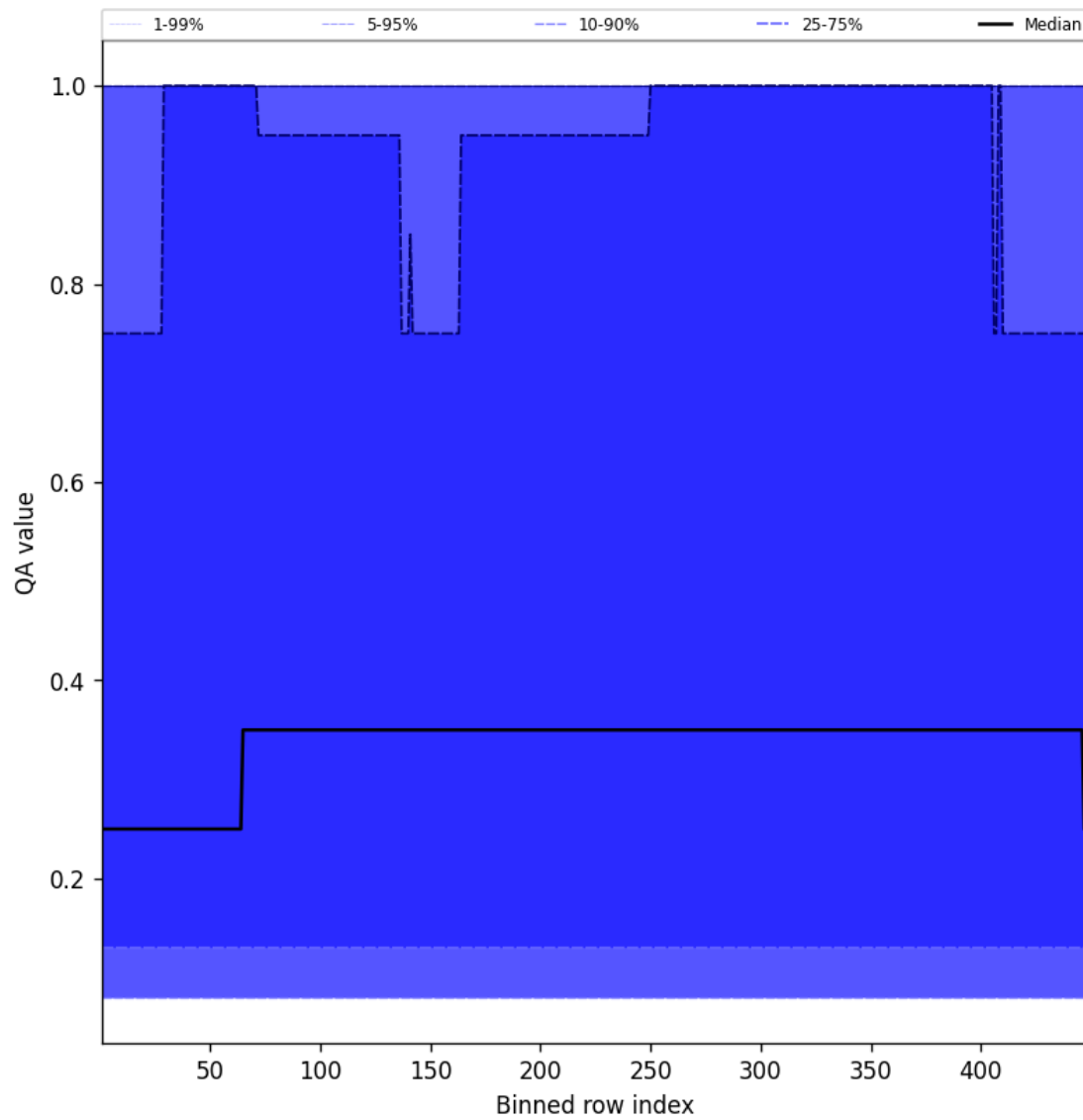
Figure 46: Along track statistics of “QA value” for 2025-03-29 to 2025-03-30
