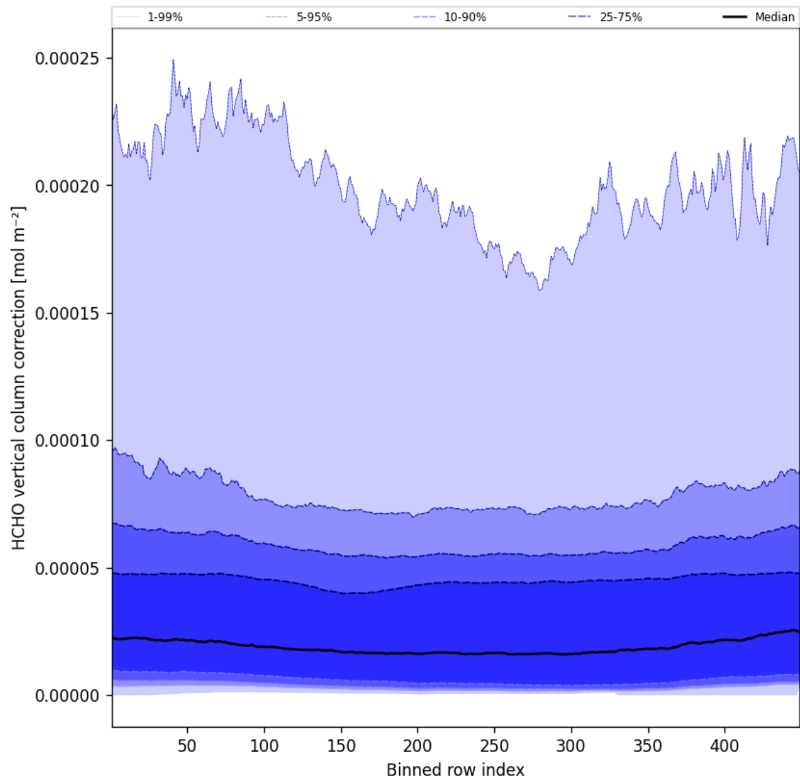
Figure 49: Along track statistics of “HCHO vertical column correction” for 2025-03-29 to 2025-03-30
