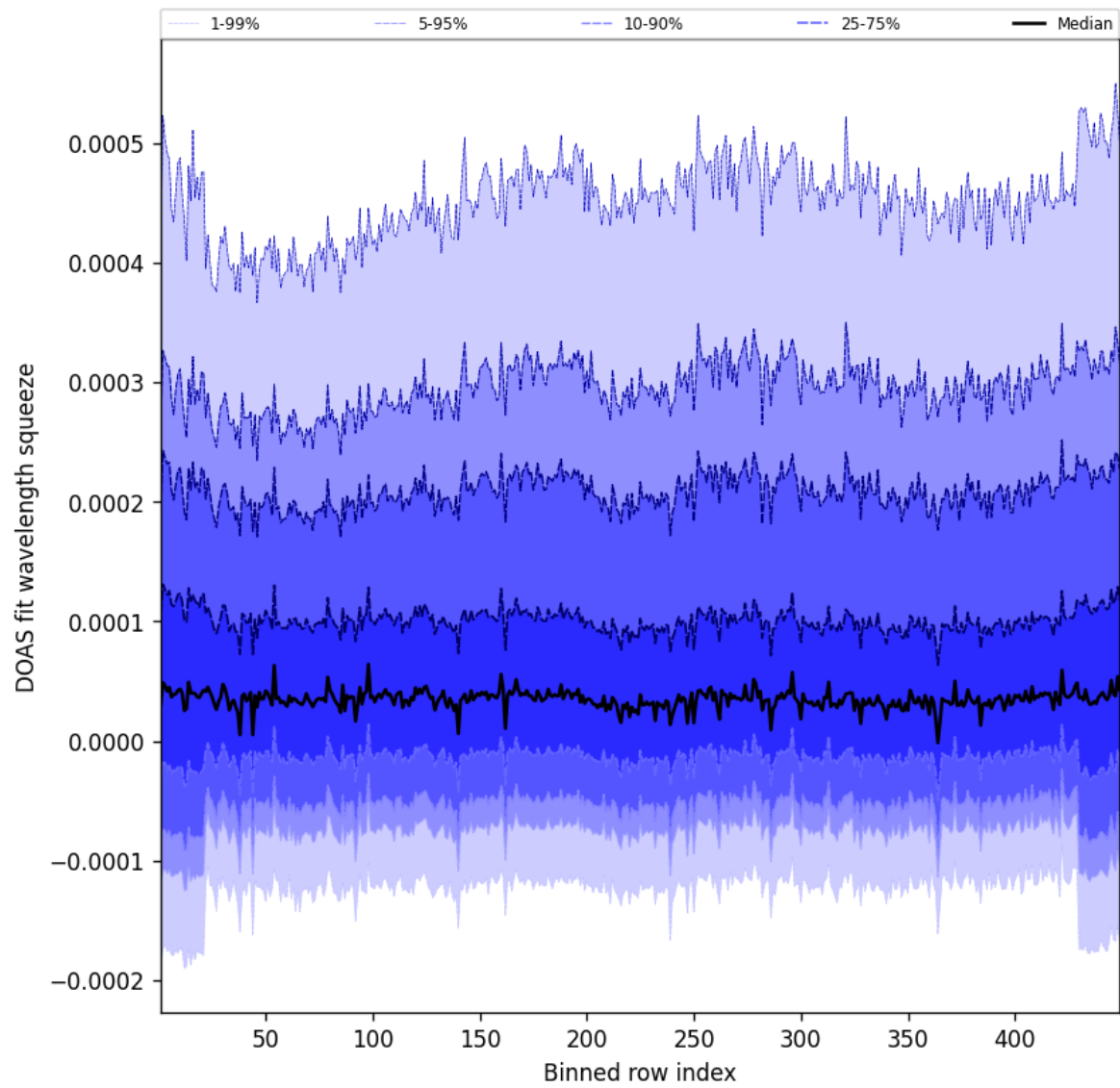
Figure 57: Along track statistics of “DOAS fit wavelength squeeze” for 2025-03-29 to 2025-03-30
