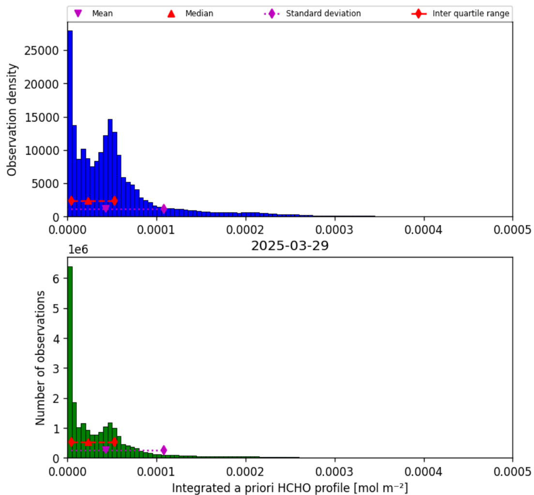
Figure 41: Histogram of “Integrated a priori HCHO profile” for 2025-03-29 to 2025-03-30
