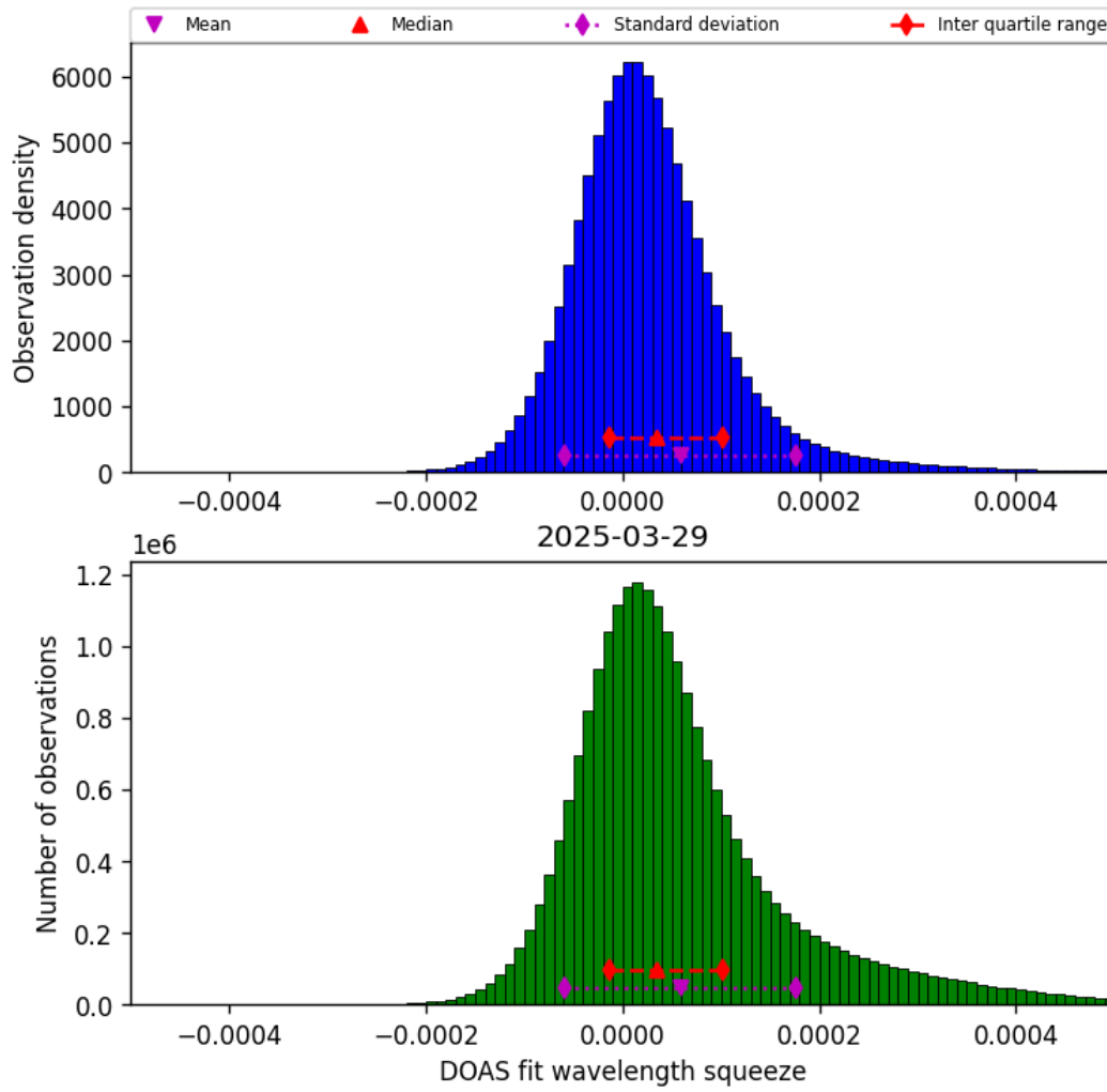
Figure 43: Histogram of “DOAS fit wavelength squeeze” for 2025-03-29 to 2025-03-30
