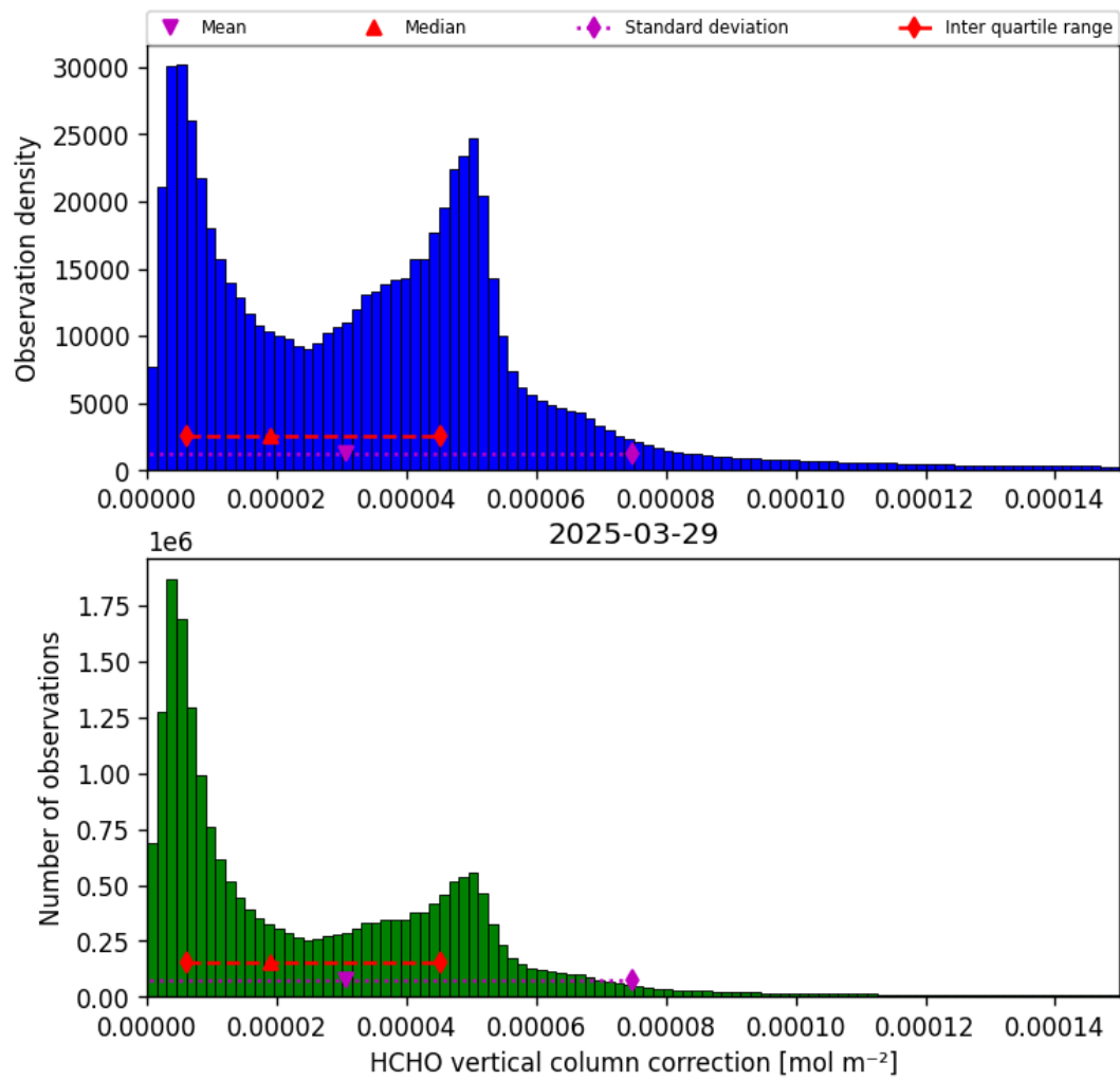
Figure 35: Histogram of “HCHO vertical column correction” for 2025-03-29 to 2025-03-30
