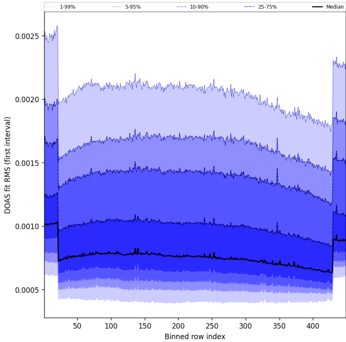
Figure 58: Along track statistics of “DOAS fit RMS (first interval)” for 2025-03-29 to 2025-03-30
