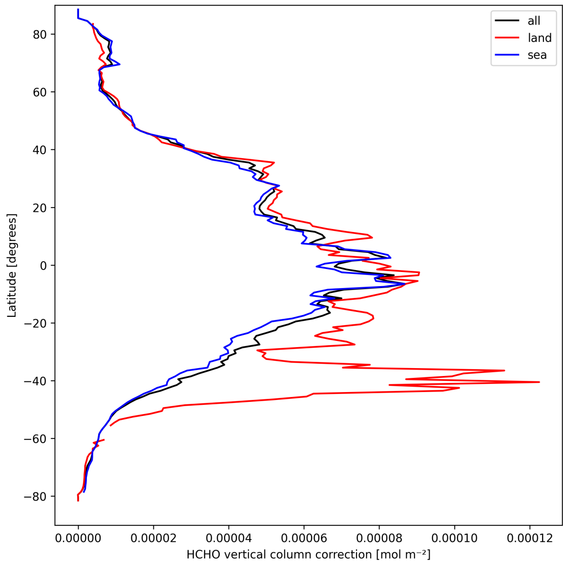
Figure 21: Zonal average of “HCHO vertical column correction” for 2025-03-29 to 2025-03-30.
