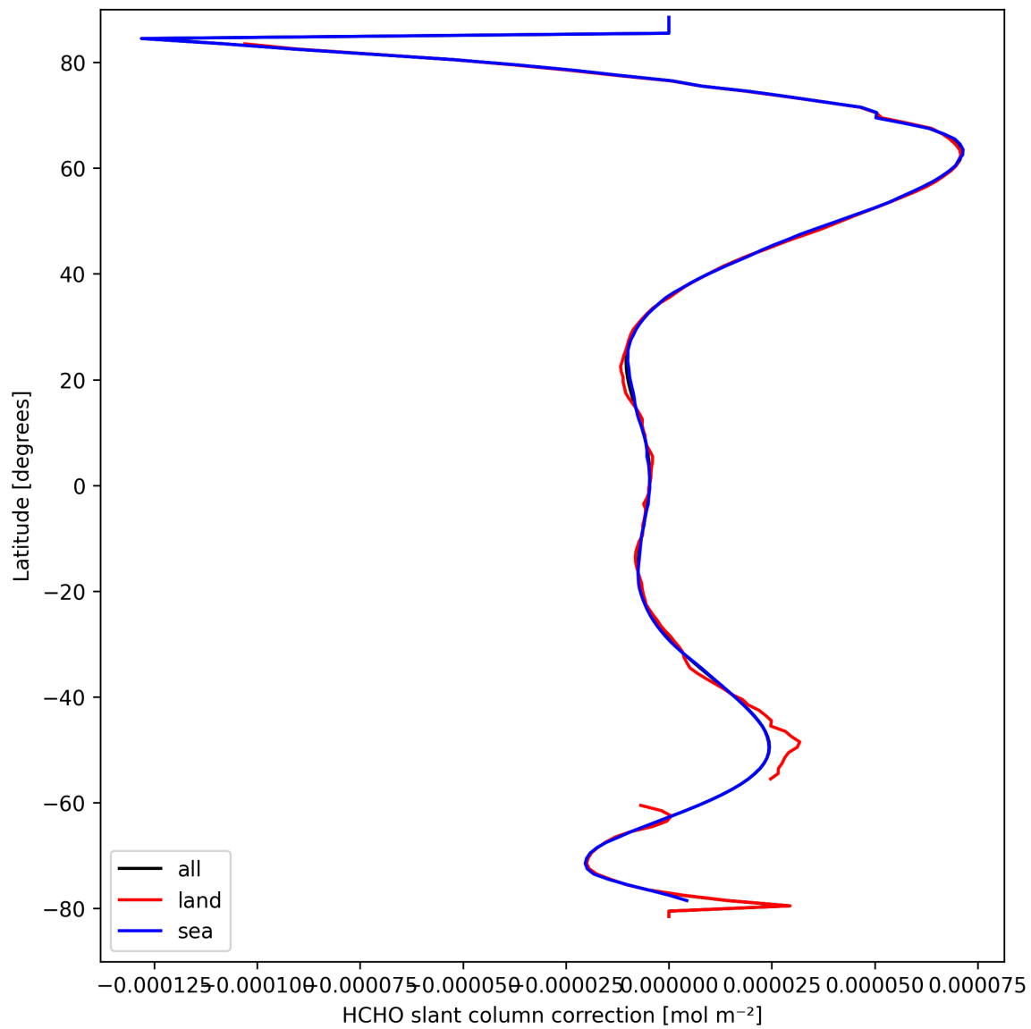
Figure 31: Zonal average of “HCHO slant column correction” for 2025-03-29 to 2025-03-30.
