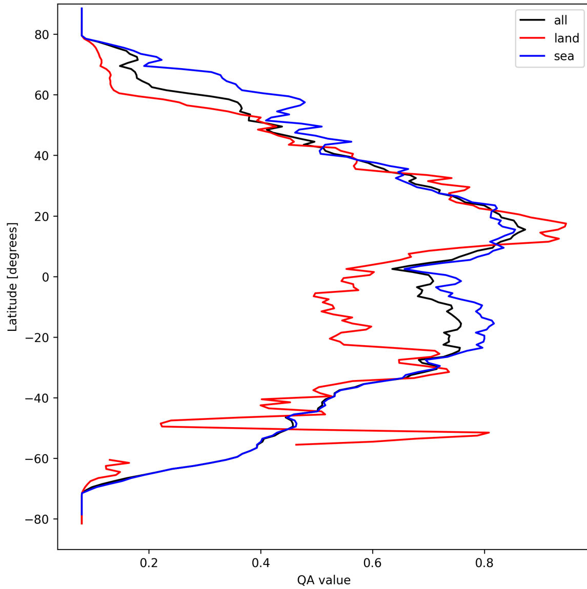
Figure 18: Zonal average of “QA value” for 2025-03-29 to 2025-03-30.
