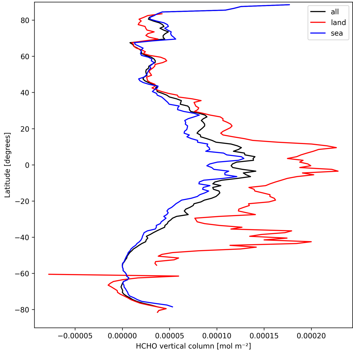
Figure 19: Zonal average of “HCHO vertical column” for 2025-03-29 to 2025-03-30.
