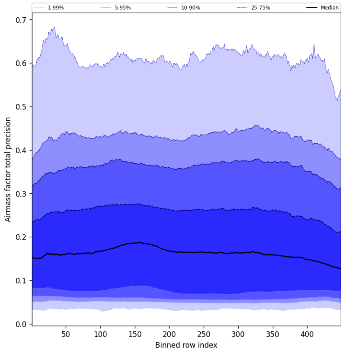
Figure 53: Along track statistics of “Airmass factor total precision” for 2025-03-29 to 2025-03-30
