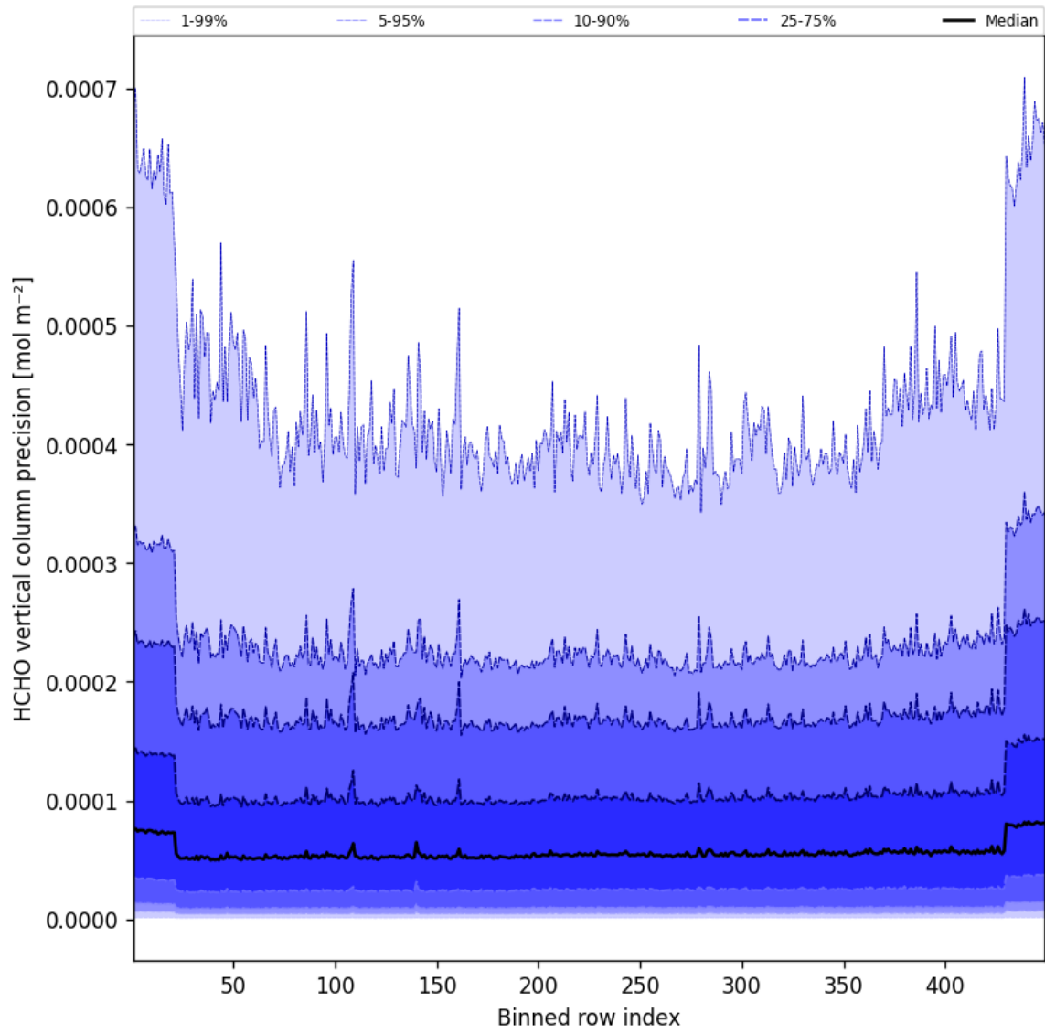
Figure 48: Along track statistics of “HCHO vertical column precision” for 2025-03-30 to 2025-03-31
