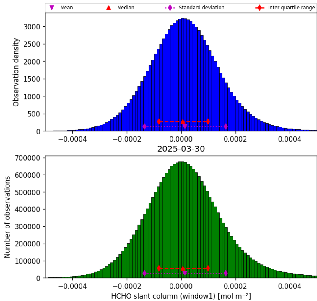
Figure 36: Histogram of “HCHO slant column (window1)” for 2025-03-30 to 2025-03-31
