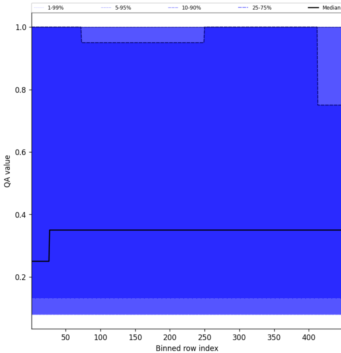
Figure 46: Along track statistics of “QA value” for 2025-03-30 to 2025-03-31
