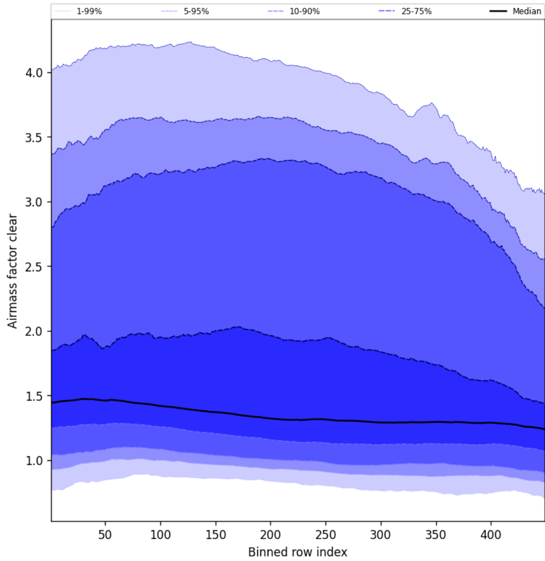
Figure 54: Along track statistics of “Airmass factor clear” for 2025-03-30 to 2025-03-31
