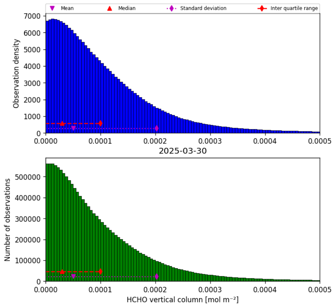
Figure 33: Histogram of “HCHO vertical column” for 2025-03-30 to 2025-03-31
