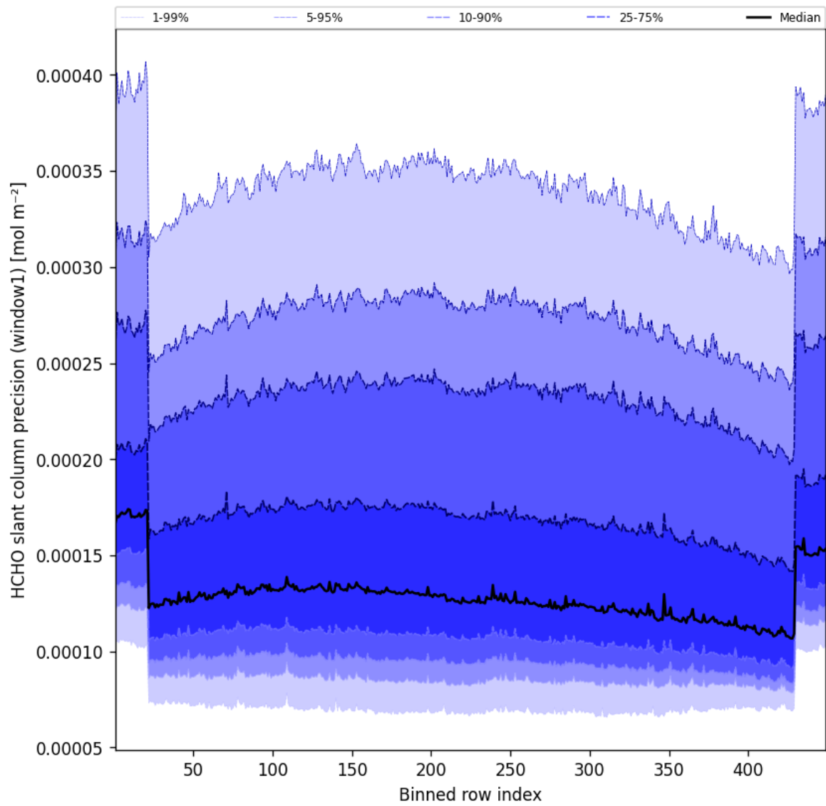
Figure 51: Along track statistics of “HCHO slant column precision (window1)” for 2025-03-30 to 2025-03-31
