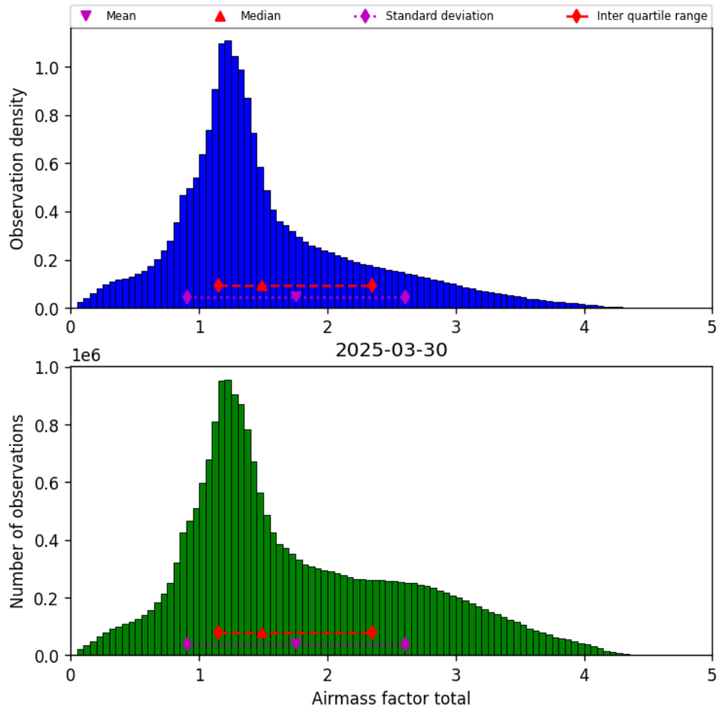
Figure 38: Histogram of “Airmass factor total” for 2025-03-30 to 2025-03-31
