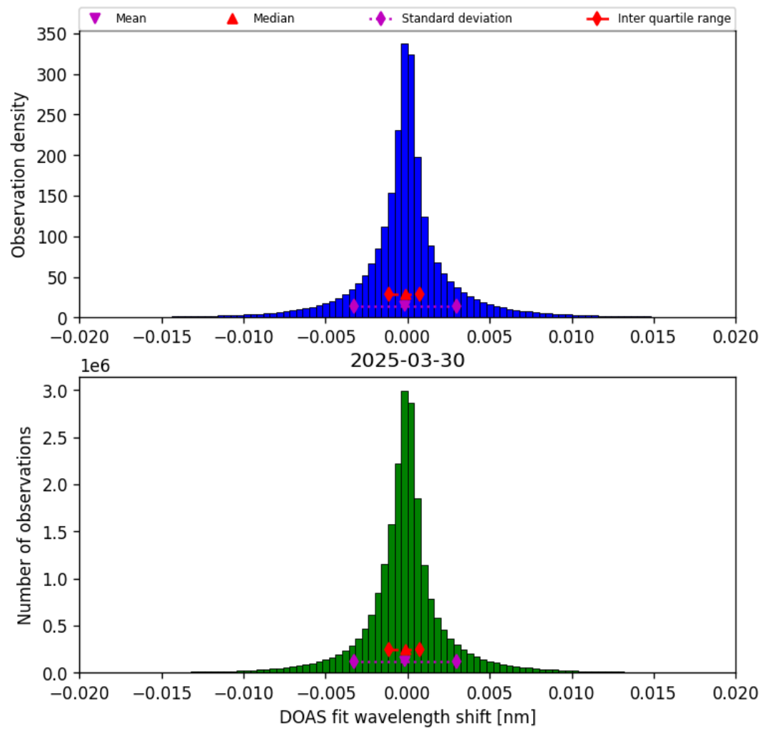
Figure 42: Histogram of “DOAS fit wavelength shift” for 2025-03-30 to 2025-03-31
