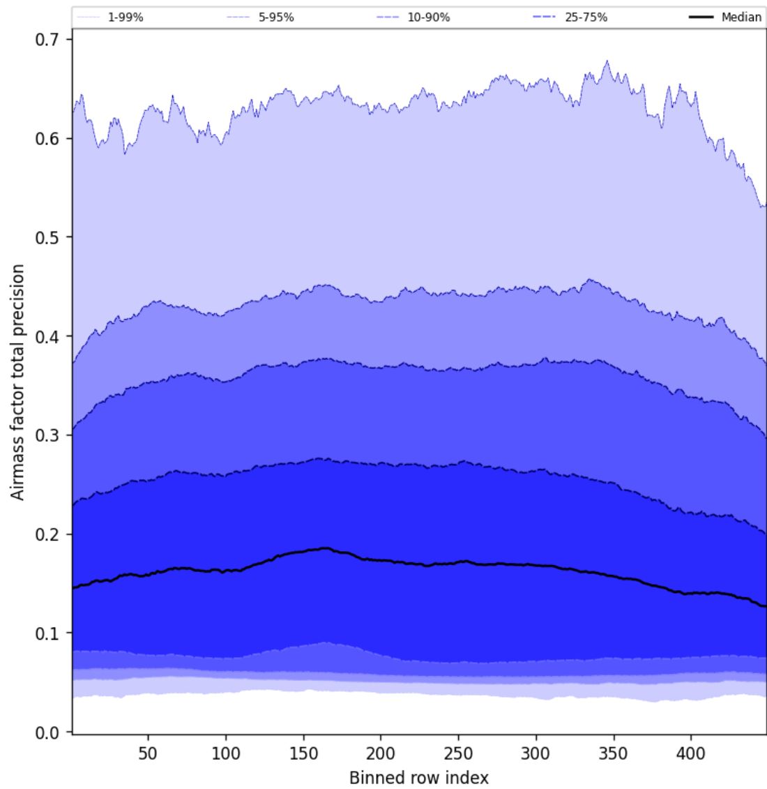
Figure 53: Along track statistics of “Airmass factor total precision” for 2025-03-30 to 2025-03-31
