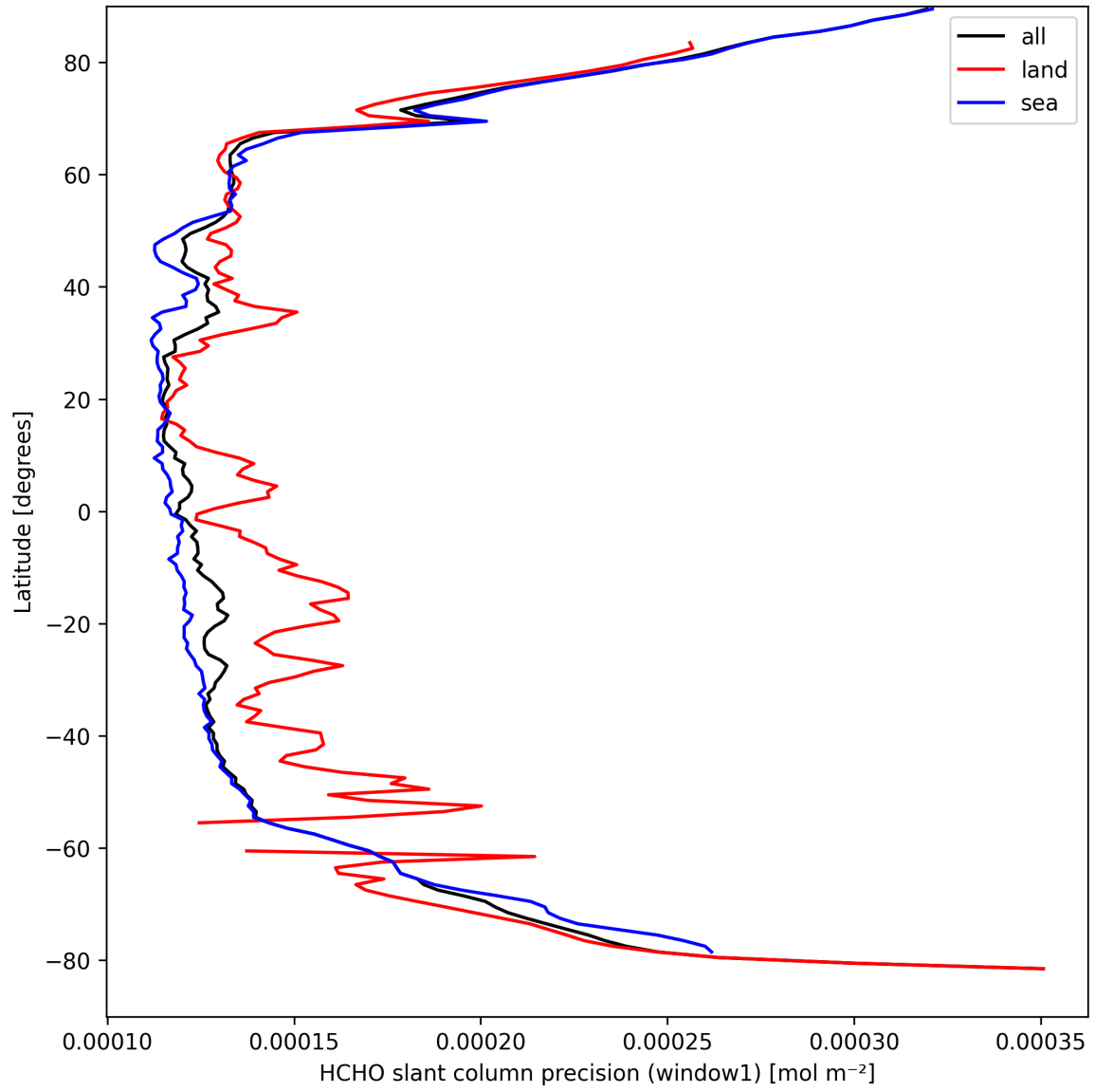
Figure 23: Zonal average of “HCHO slant column precision (window1)” for 2025-03-30 to 2025-03-31.
