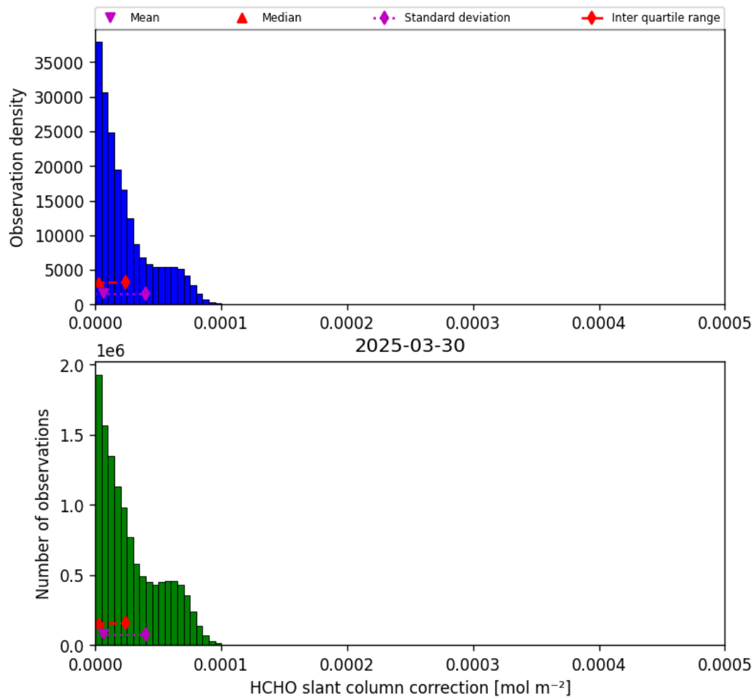
Figure 45: Histogram of “HCHO slant column correction” for 2025-03-30 to 2025-03-31
