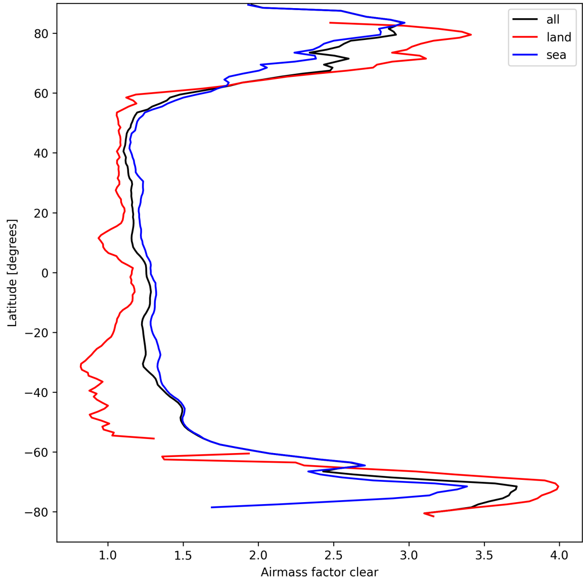
Figure 26: Zonal average of “Airmass factor clear” for 2025-03-30 to 2025-03-31.
