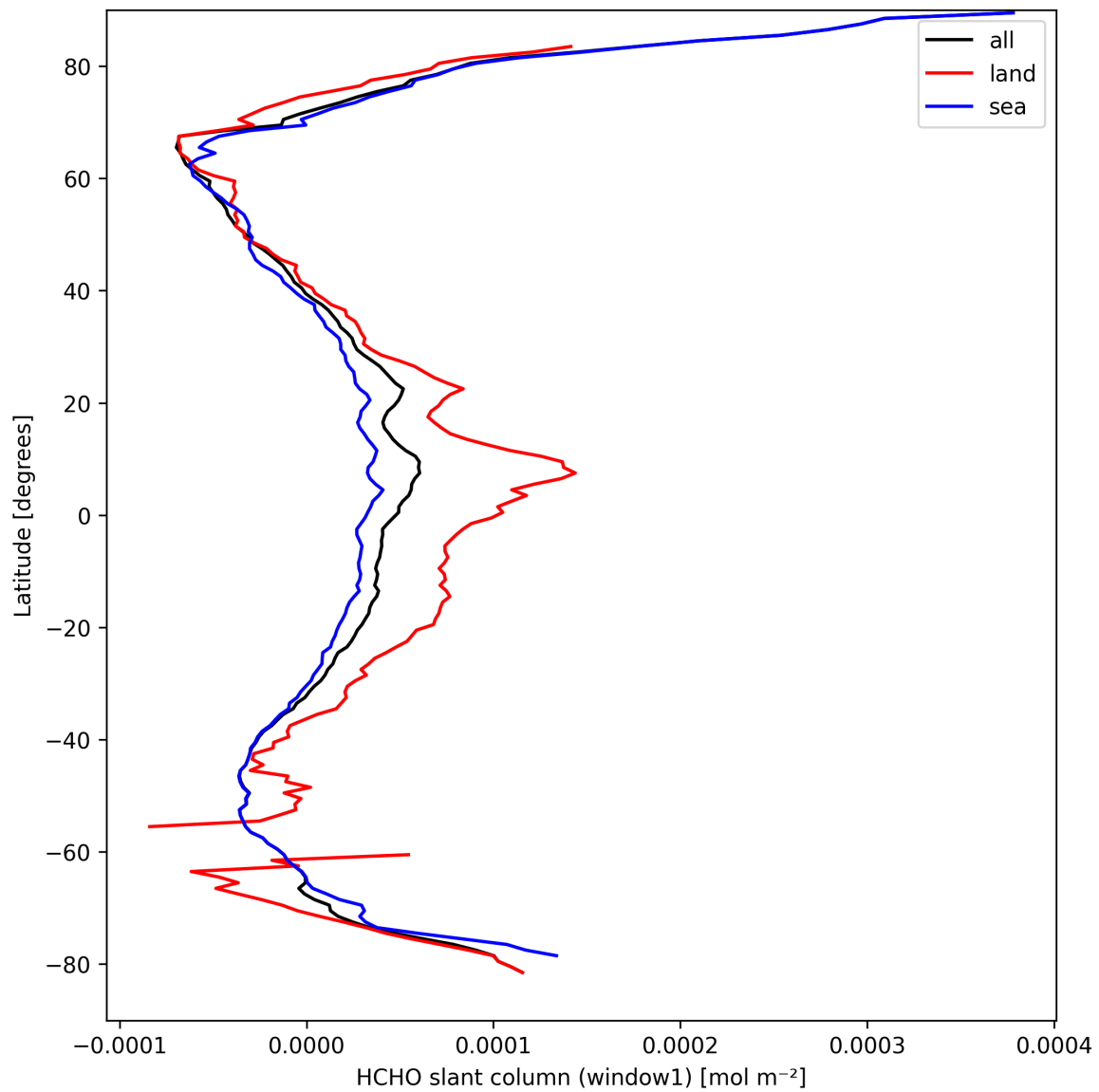
Figure 22: Zonal average of “HCHO slant column (window1)” for 2025-03-30 to 2025-03-31.
