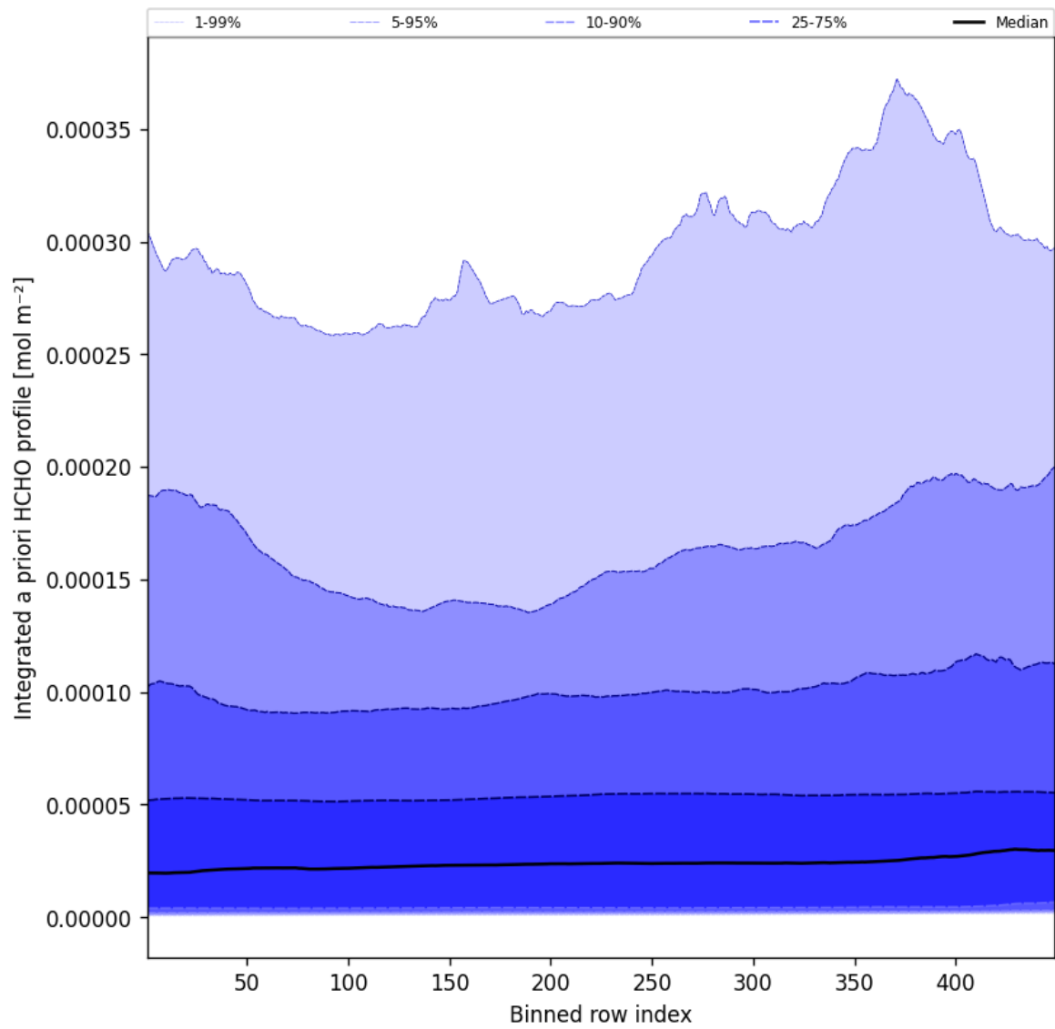
Figure 55: Along track statistics of “Integrated a priori HCHO profile” for 2025-03-30 to 2025-03-31
