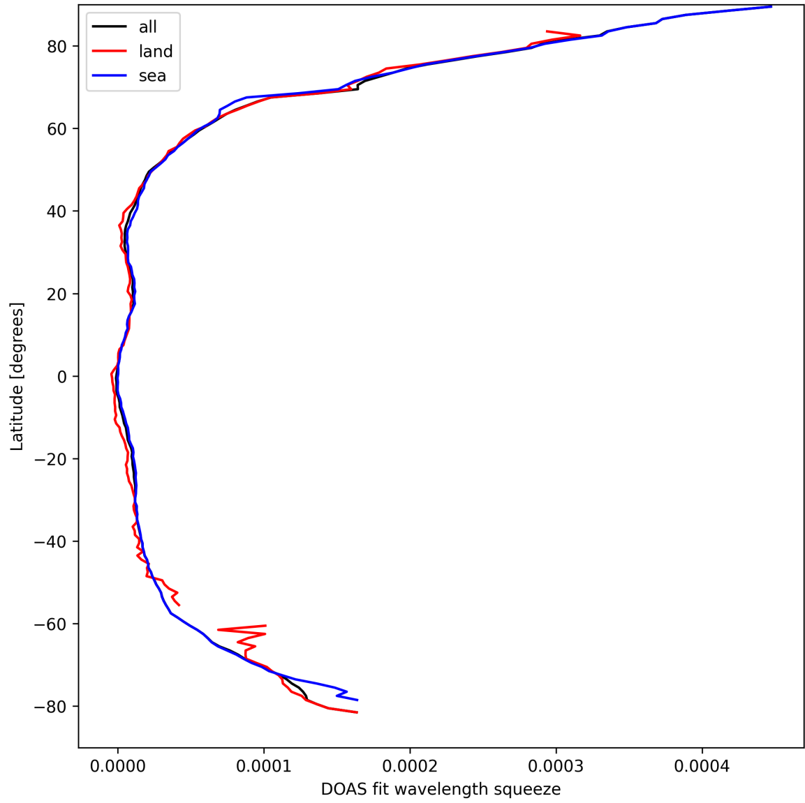
Figure 29: Zonal average of “DOAS fit wavelength squeeze” for 2025-03-30 to 2025-03-31.
