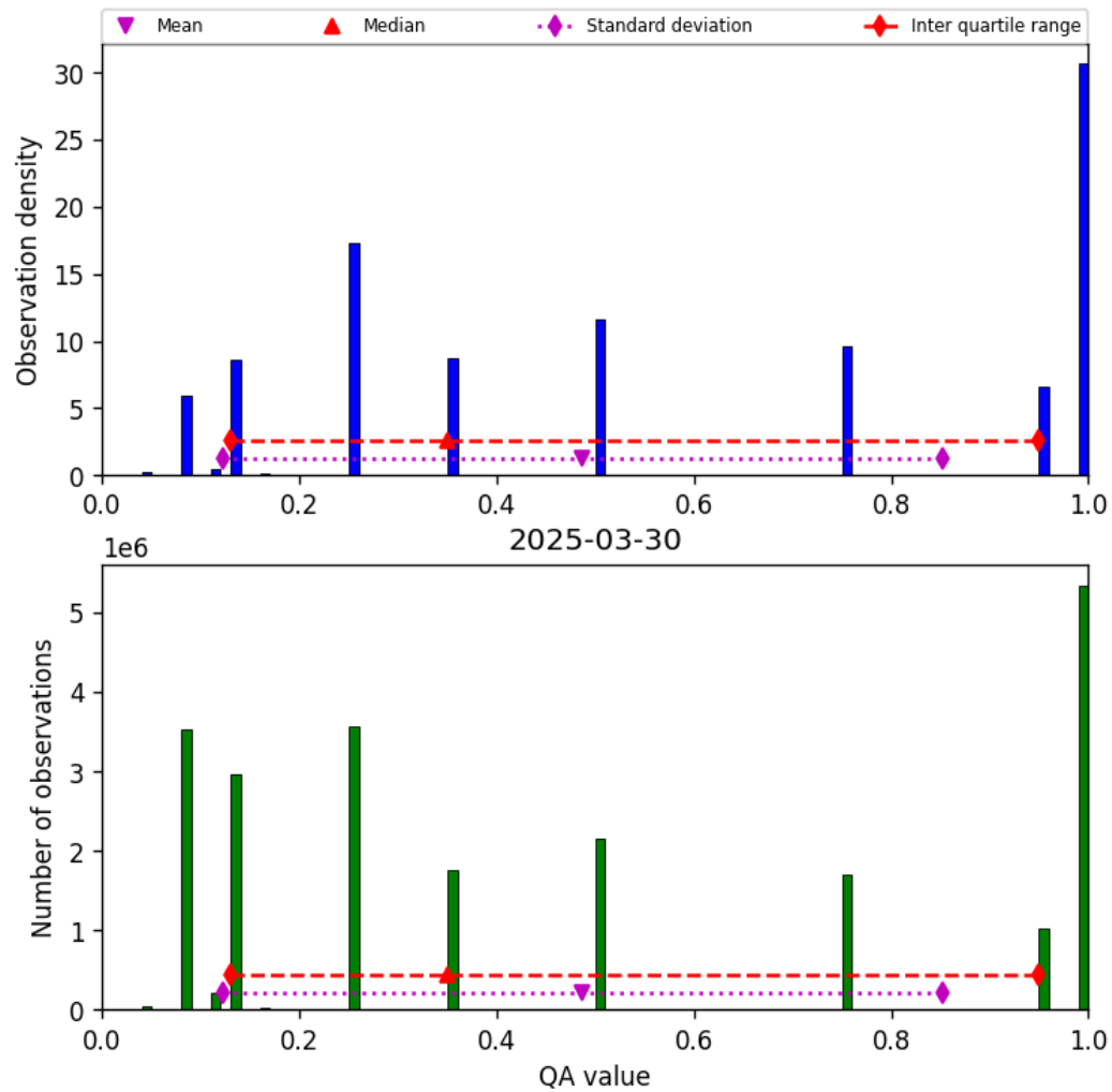
Figure 32: Histogram of “QA value” for 2025-03-30 to 2025-03-31
