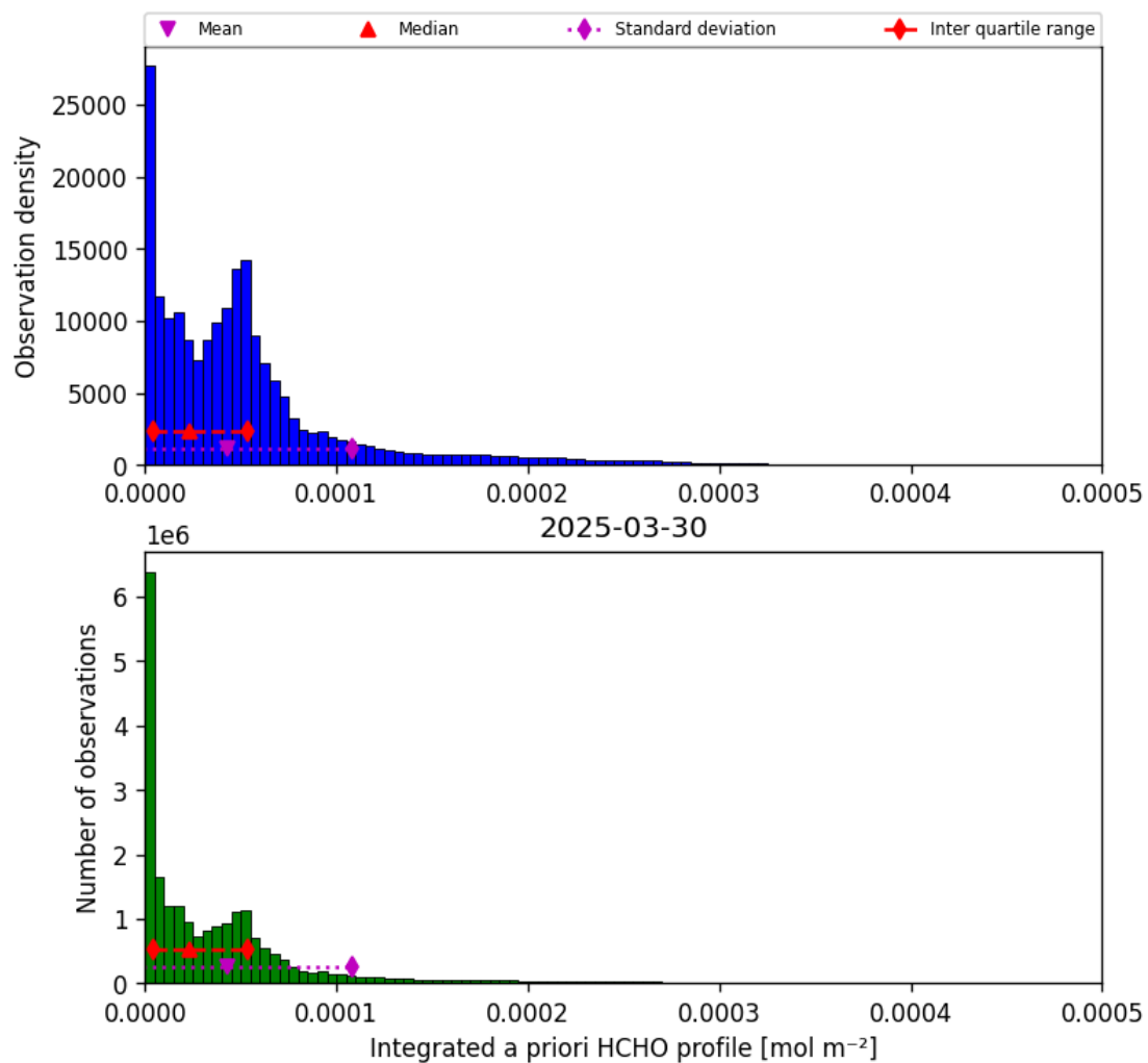
Figure 41: Histogram of “Integrated a priori HCHO profile” for 2025-03-30 to 2025-03-31
