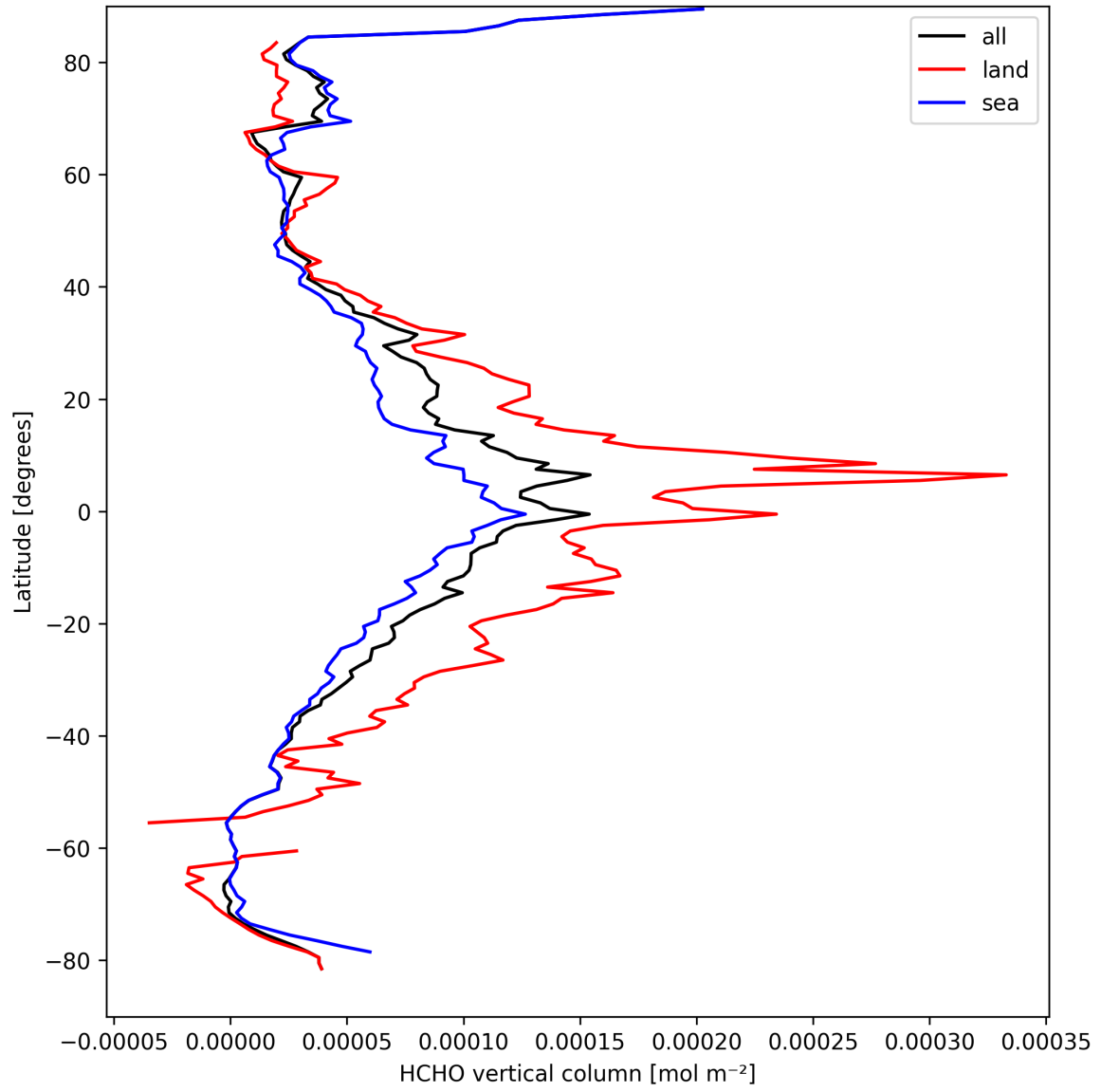
Figure 19: Zonal average of “HCHO vertical column” for 2025-03-30 to 2025-03-31.
