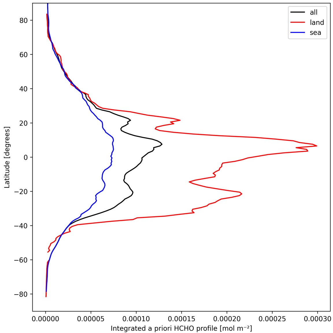
Figure 27: Zonal average of “Integrated a priori HCHO profile” for 2025-03-30 to 2025-03-31.
