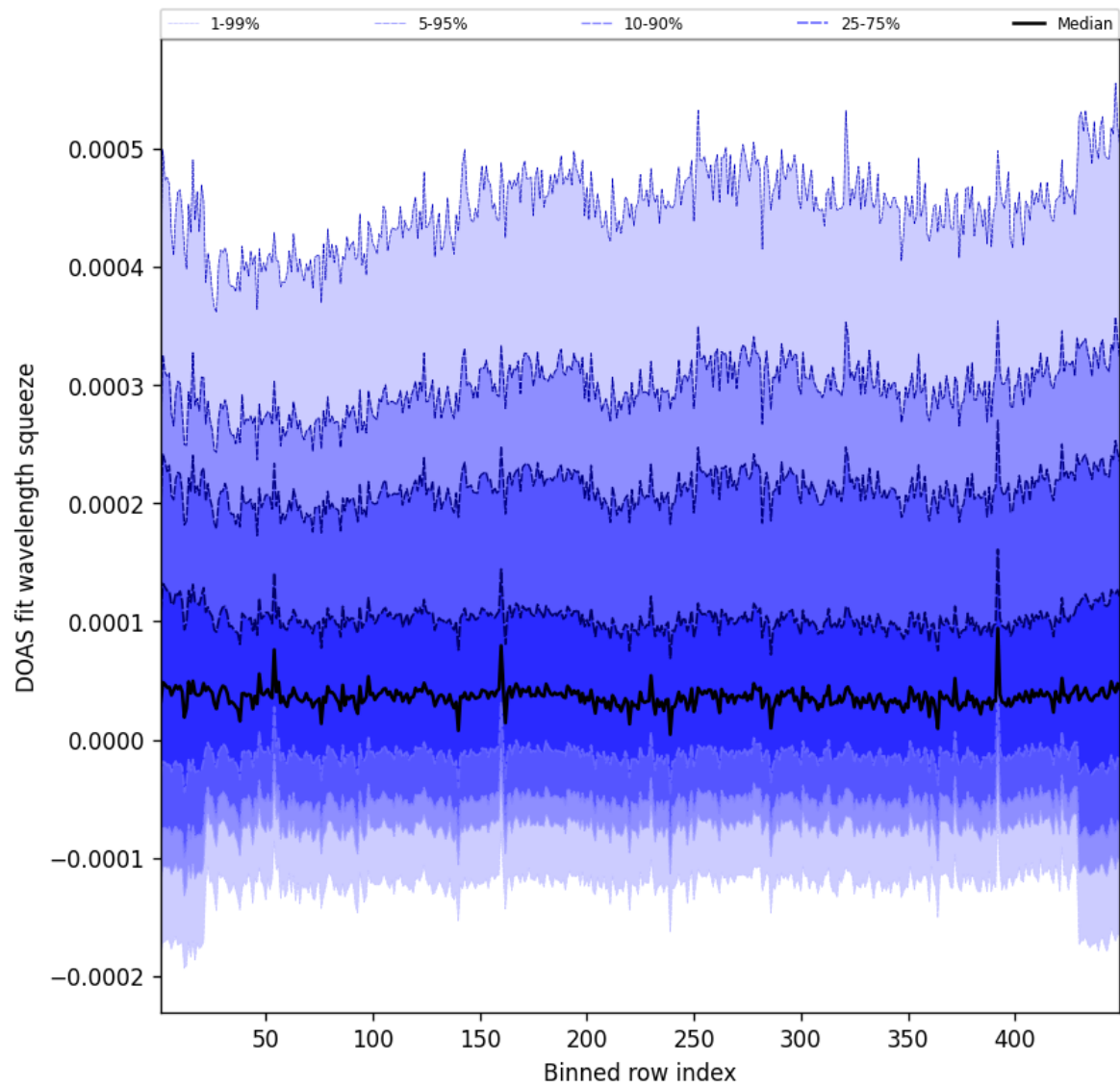
Figure 57: Along track statistics of “DOAS fit wavelength squeeze” for 2025-03-30 to 2025-03-31
