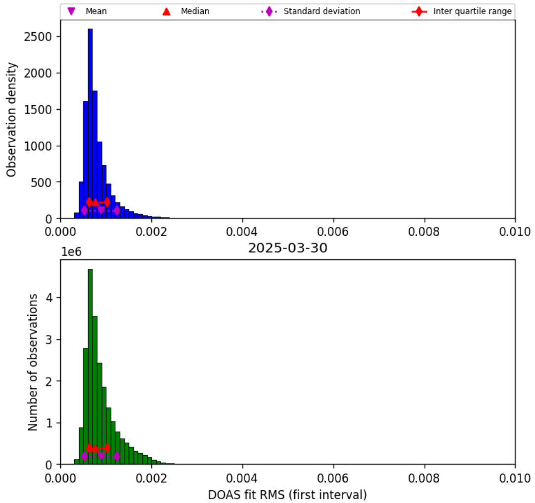
Figure 44: Histogram of “DOAS fit RMS (first interval)” for 2025-03-30 to 2025-03-31
