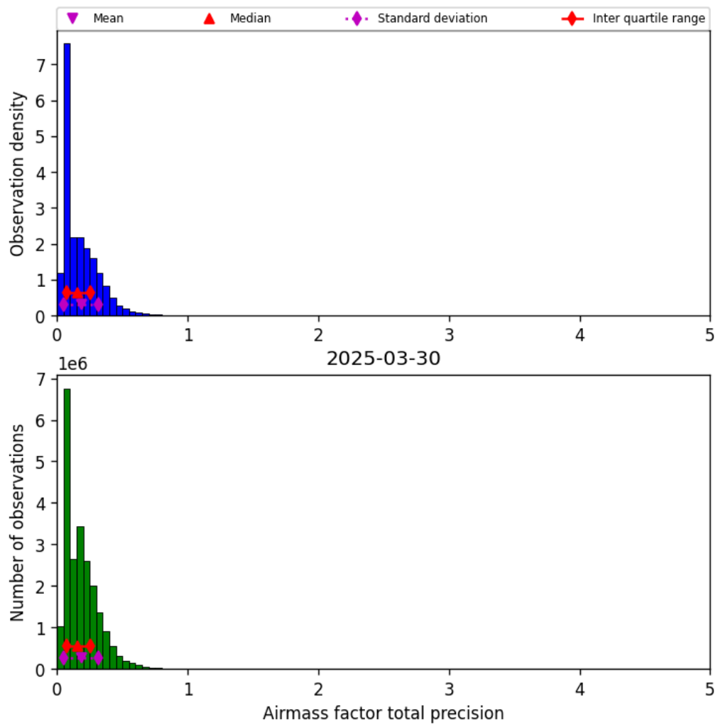
Figure 39: Histogram of “Airmass factor total precision” for 2025-03-30 to 2025-03-31
