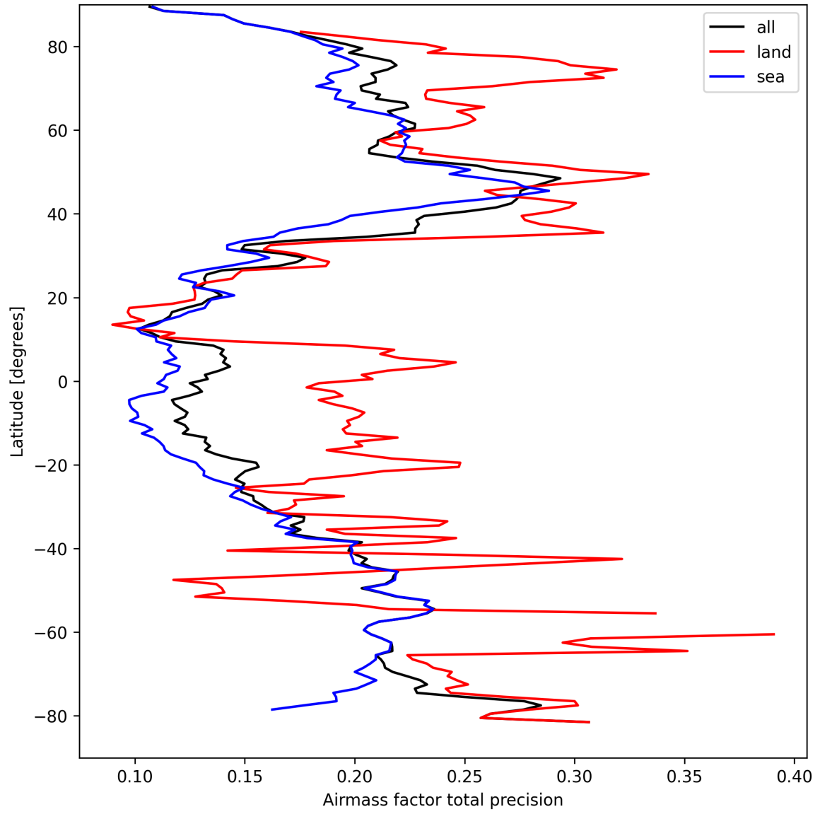
Figure 25: Zonal average of “Airmass factor total precision” for 2025-03-30 to 2025-03-31.
