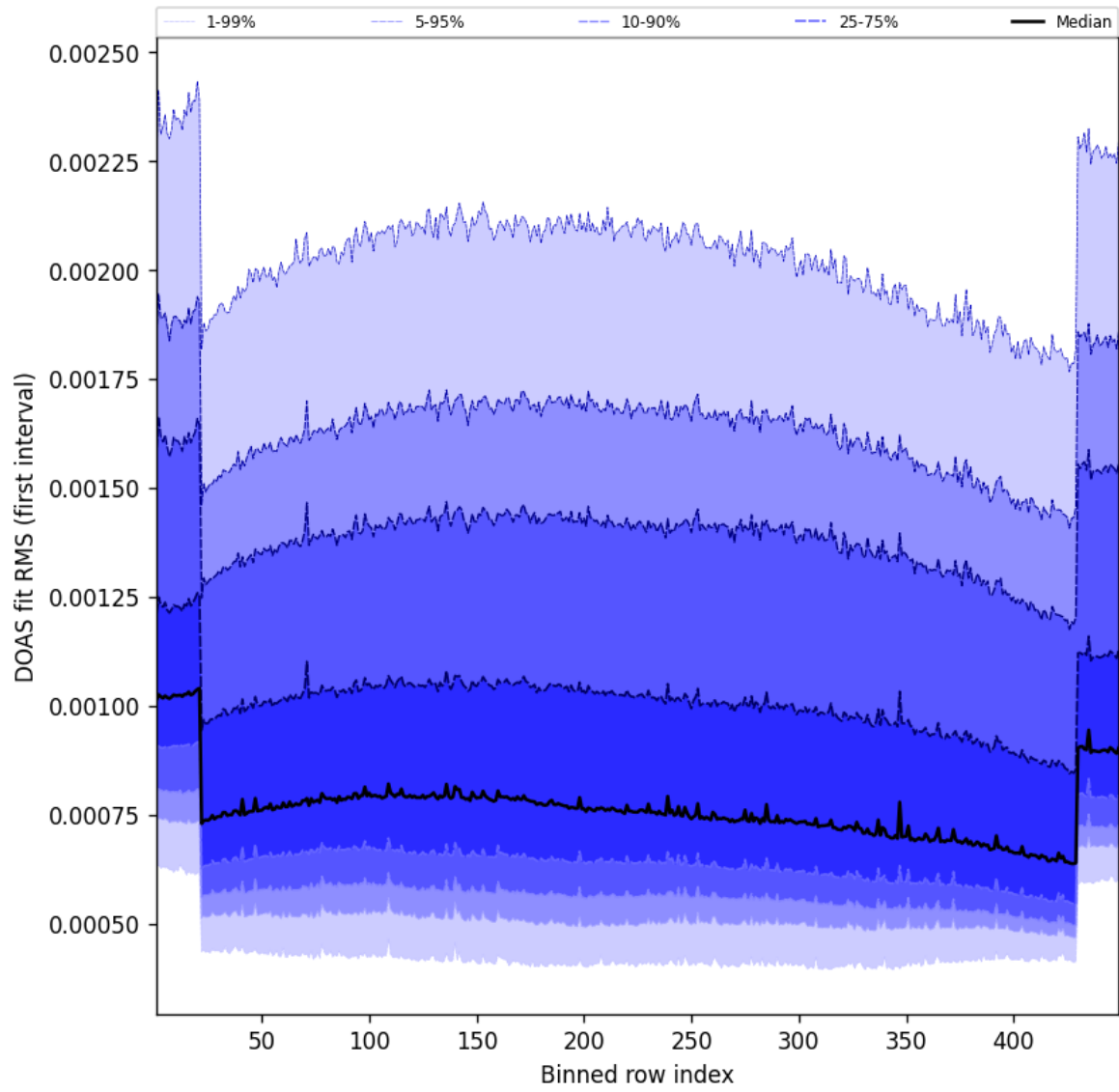
Figure 58: Along track statistics of “DOAS fit RMS (first interval)” for 2025-03-30 to 2025-03-31
