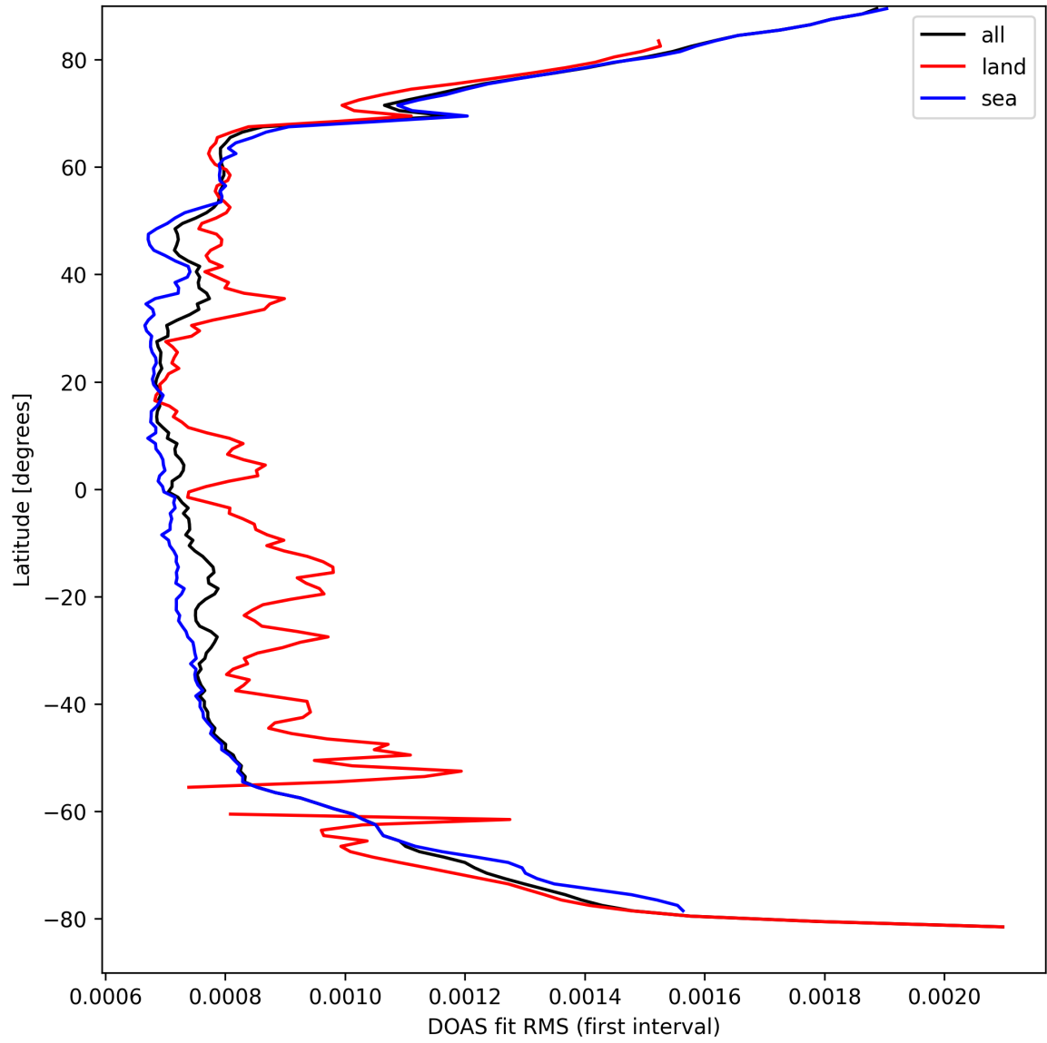
Figure 30: Zonal average of "DOAS fit RMS (first interval)" for 2025-03-30 to 2025-03-31.
