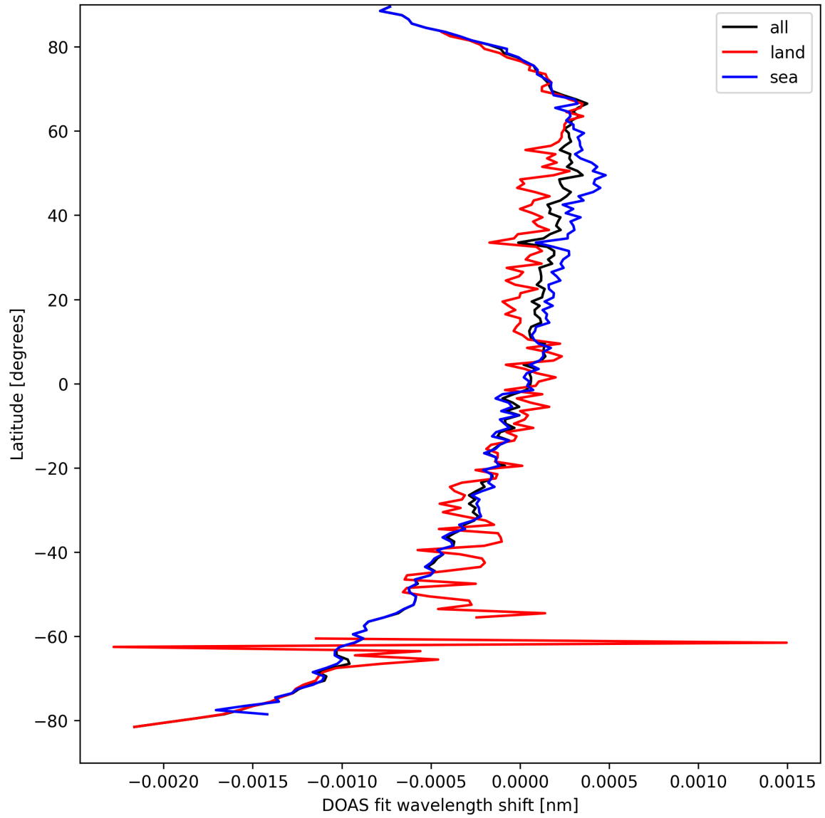
Figure 28: Zonal average of "DOAS fit wavelength shift" for 2025-03-30 to 2025-03-31.
