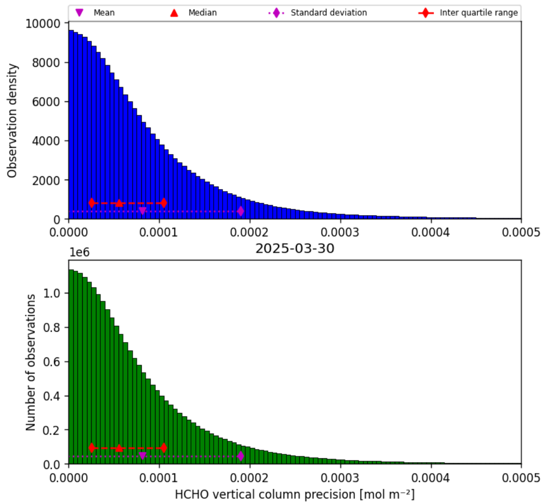
Figure 34: Histogram of “HCHO vertical column precision” for 2025-03-30 to 2025-03-31
