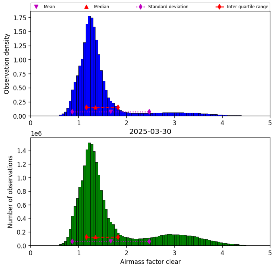
Figure 40: Histogram of “Airmass factor clear” for 2025-03-30 to 2025-03-31
