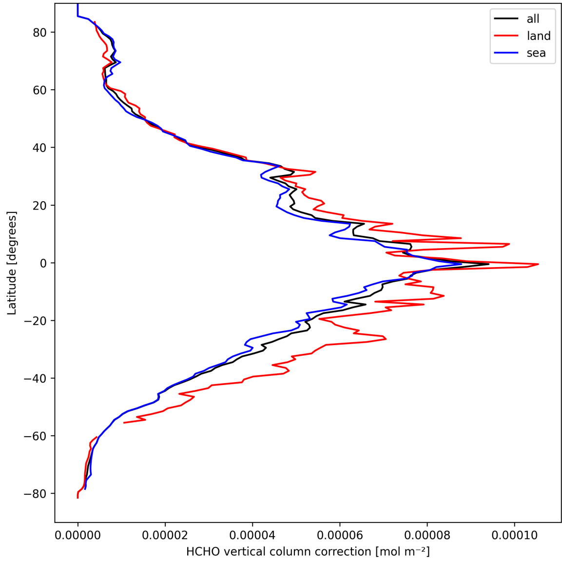
Figure 21: Zonal average of “HCHO vertical column correction” for 2025-03-30 to 2025-03-31.
