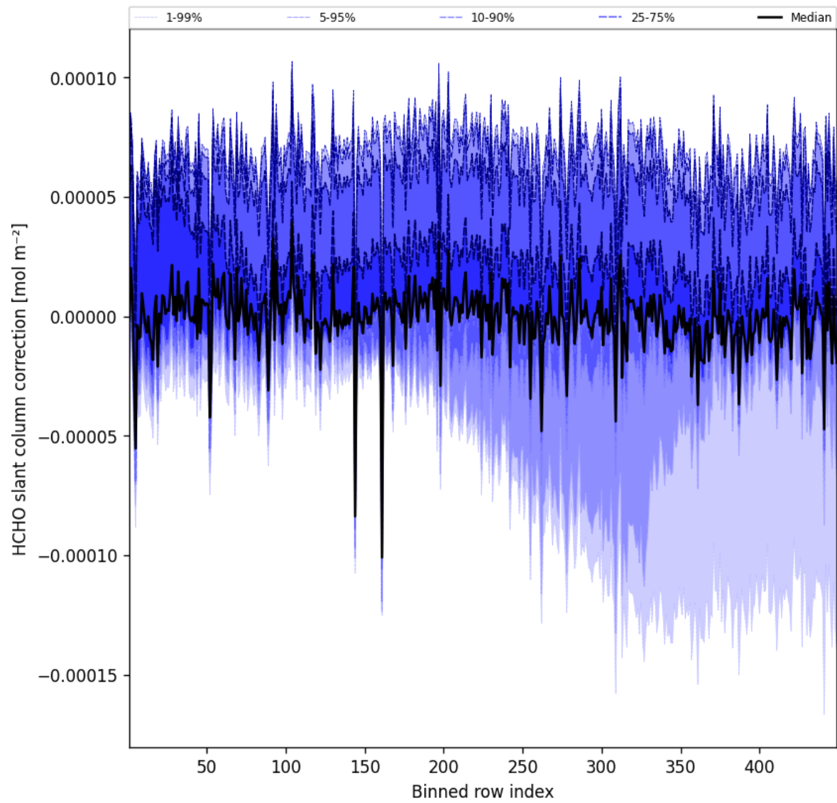
Figure 59: Along track statistics of “HCHO slant column correction” for 2025-03-30 to 2025-03-31
