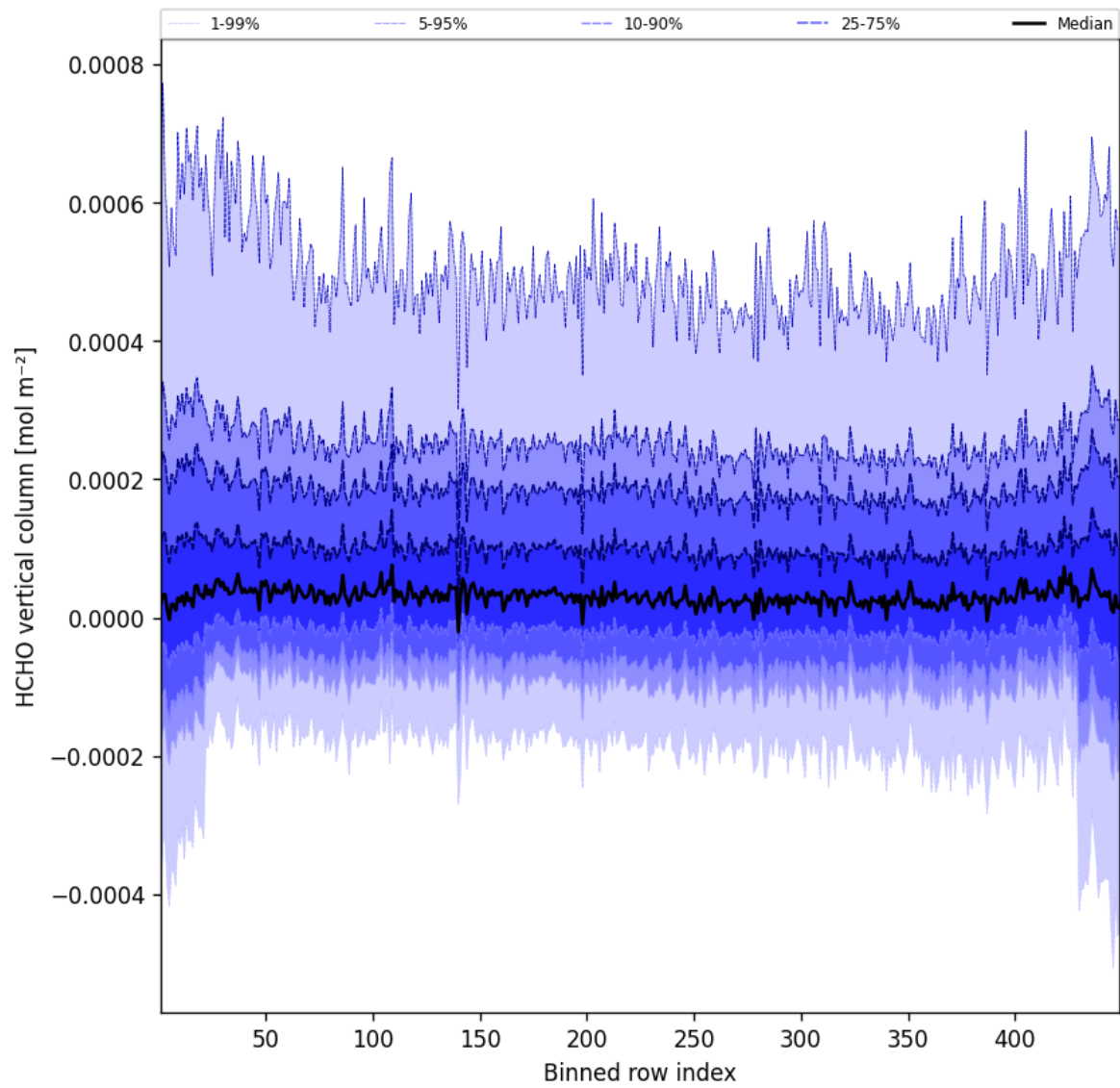
Figure 47: Along track statistics of “HCHO vertical column” for 2025-03-30 to 2025-03-31
