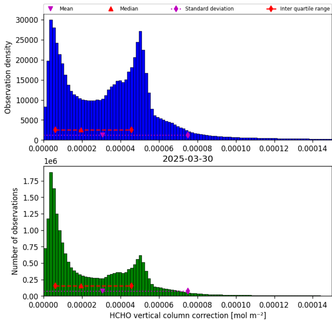
Figure 35: Histogram of “HCHO vertical column correction” for 2025-03-30 to 2025-03-31
