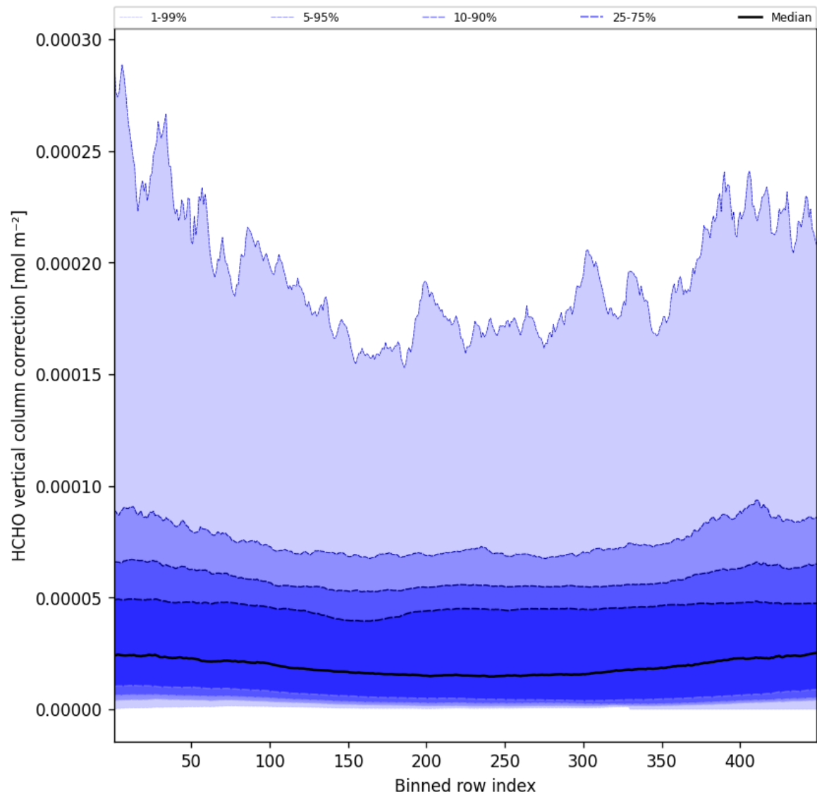
Figure 49: Along track statistics of “HCHO vertical column correction” for 2025-03-30 to 2025-03-31
