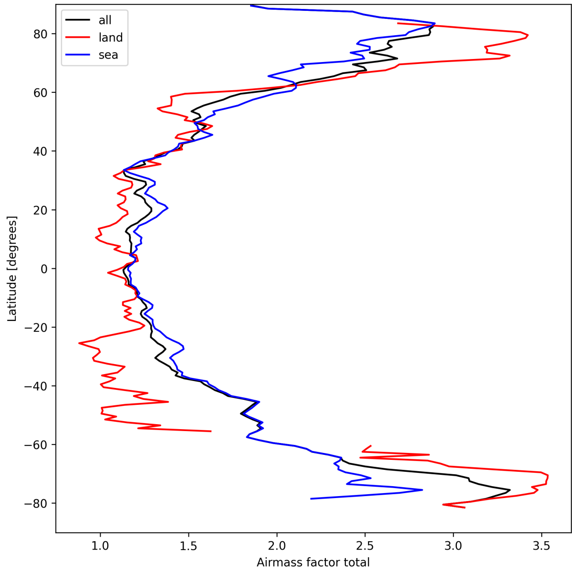
Figure 24: Zonal average of “Airmass factor total” for 2025-03-30 to 2025-03-31.
