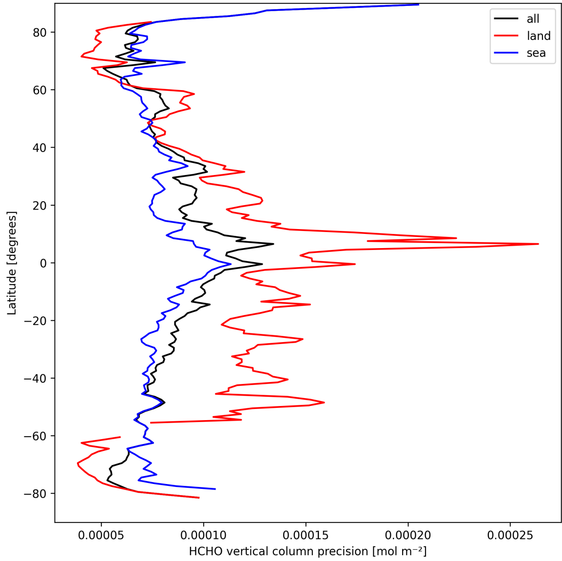
Figure 20: Zonal average of “HCHO vertical column precision” for 2025-03-30 to 2025-03-31.
