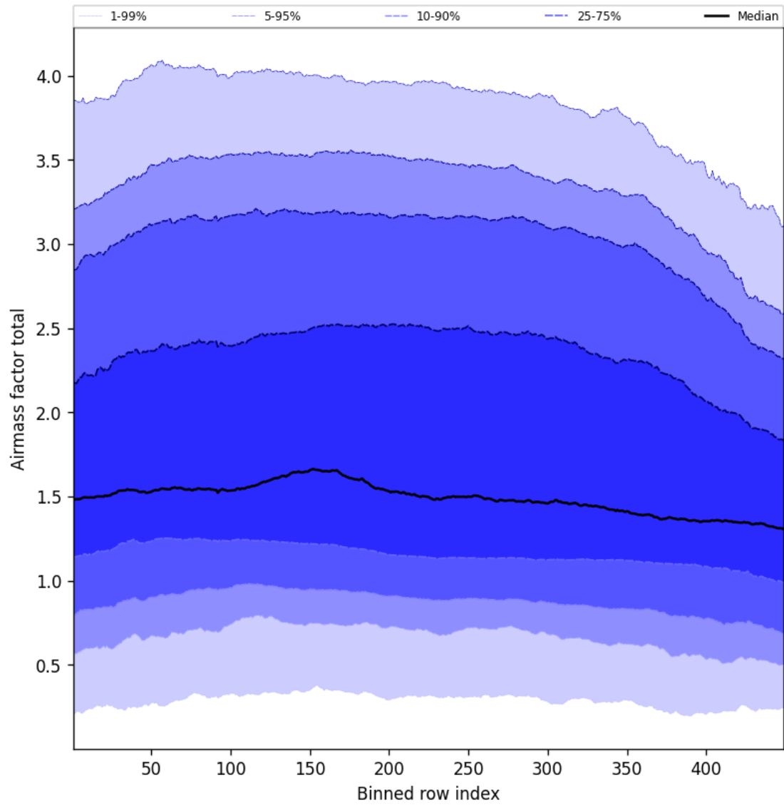
Figure 52: Along track statistics of “Airmass factor total” for 2025-03-30 to 2025-03-31
