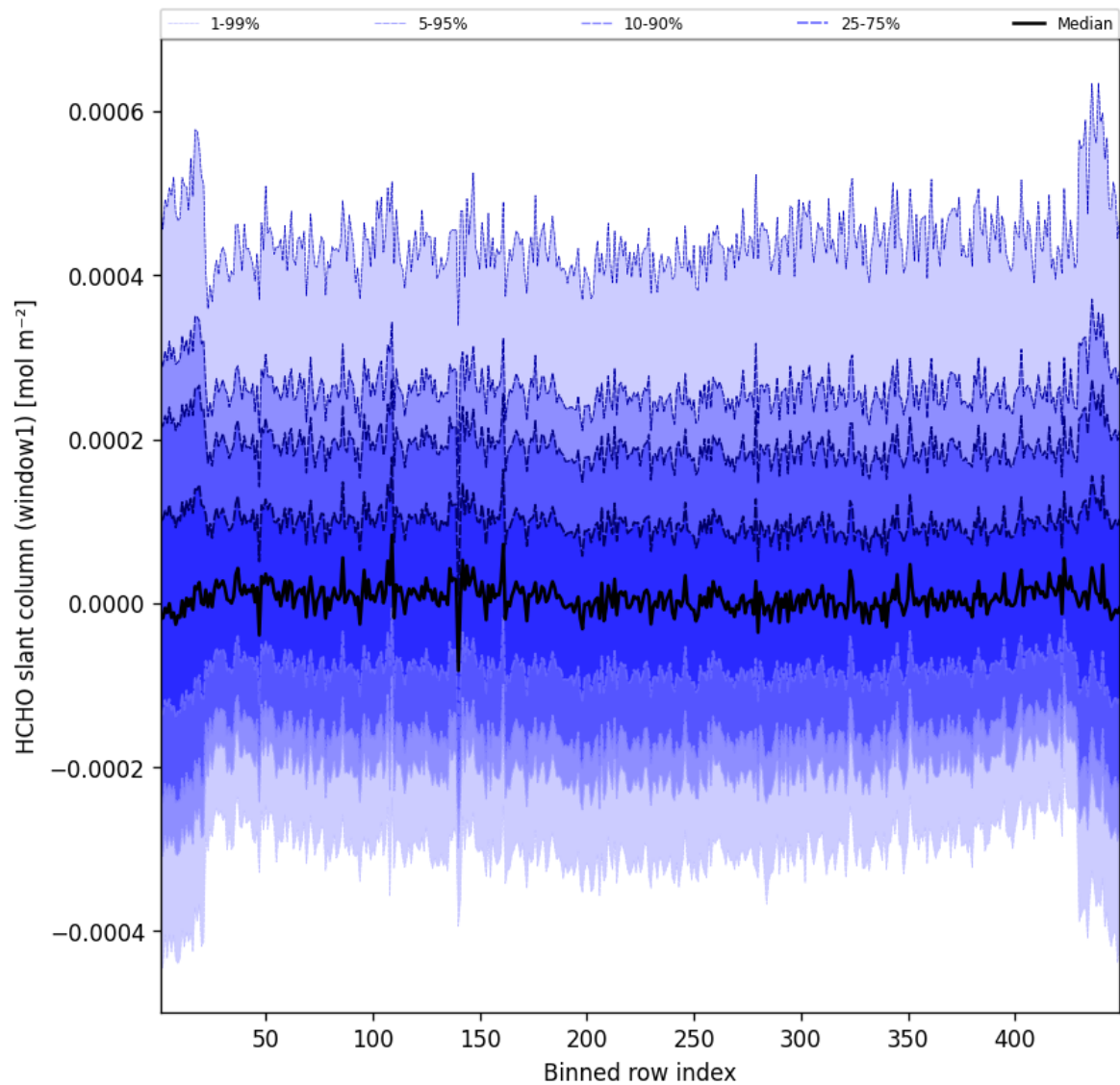
Figure 50: Along track statistics of “HCHO slant column (window1)” for 2025-03-30 to 2025-03-31
