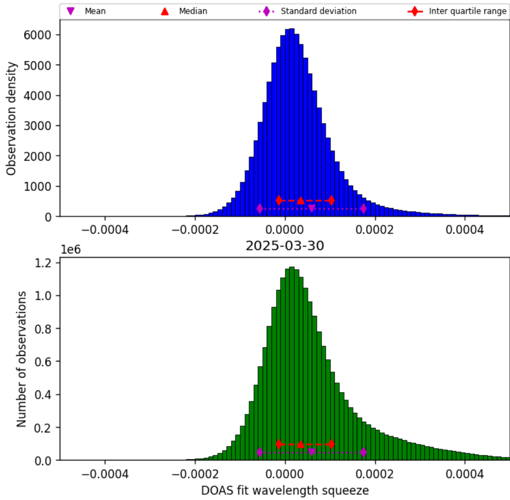
Figure 43: Histogram of “DOAS fit wavelength squeeze” for 2025-03-30 to 2025-03-31
