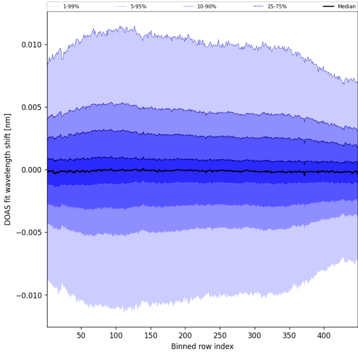
Figure 56: Along track statistics of “DOAS fit wavelength shift” for 2025-03-30 to 2025-03-31
