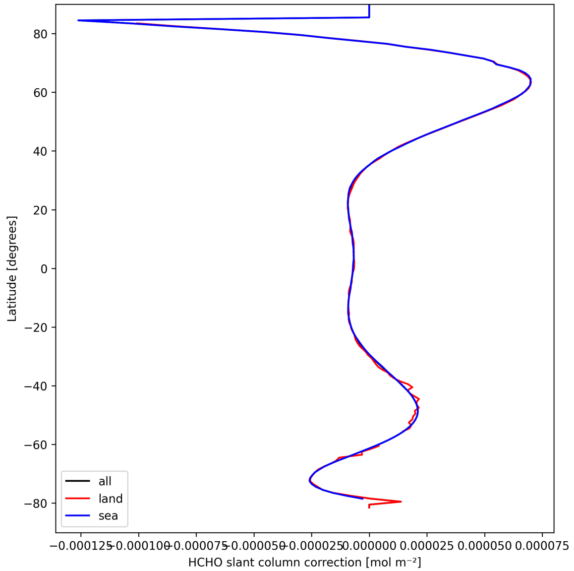
Figure 31: Zonal average of “HCHO slant column correction” for 2025-03-30 to 2025-03-31.
