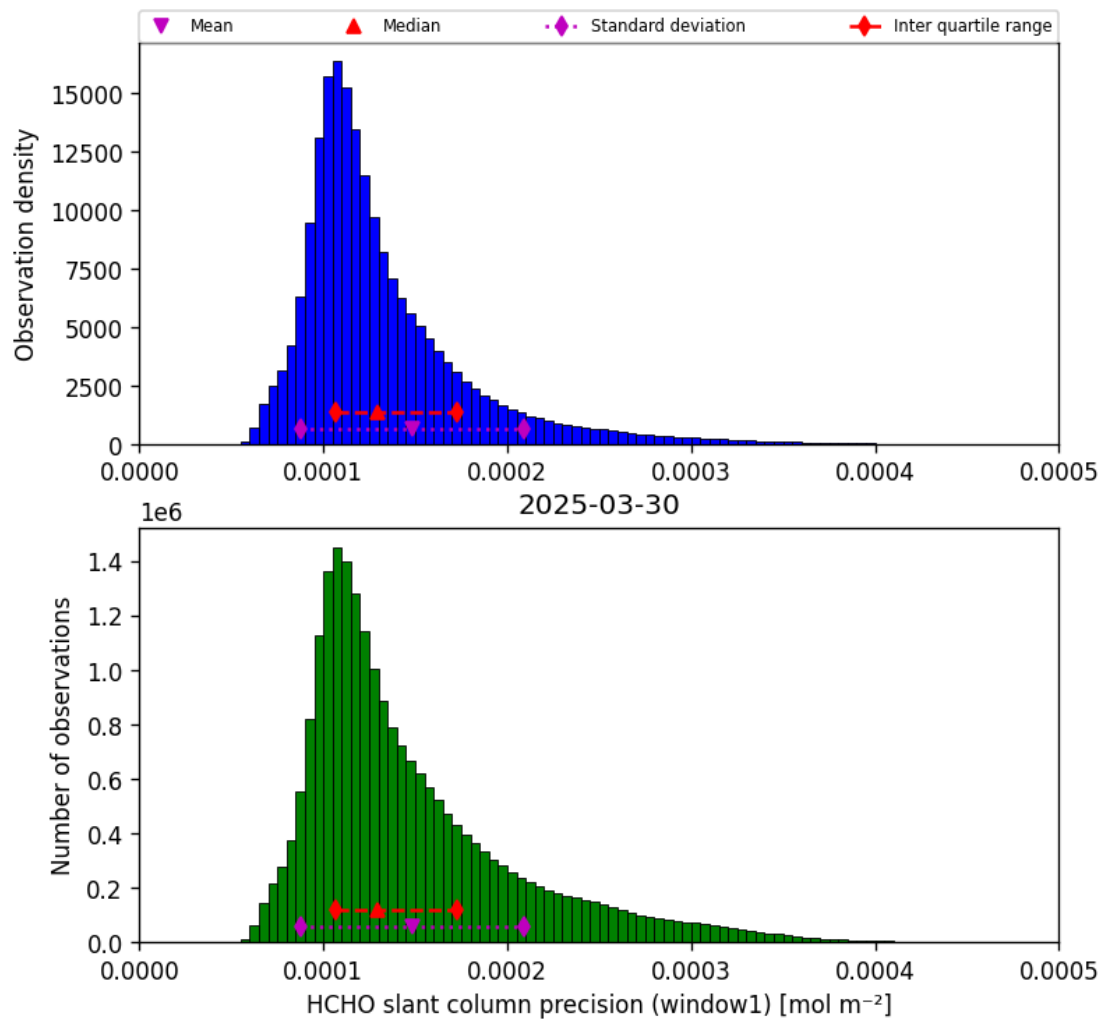
Figure 37: Histogram of “HCHO slant column precision (window1)” for 2025-03-30 to 2025-03-31
