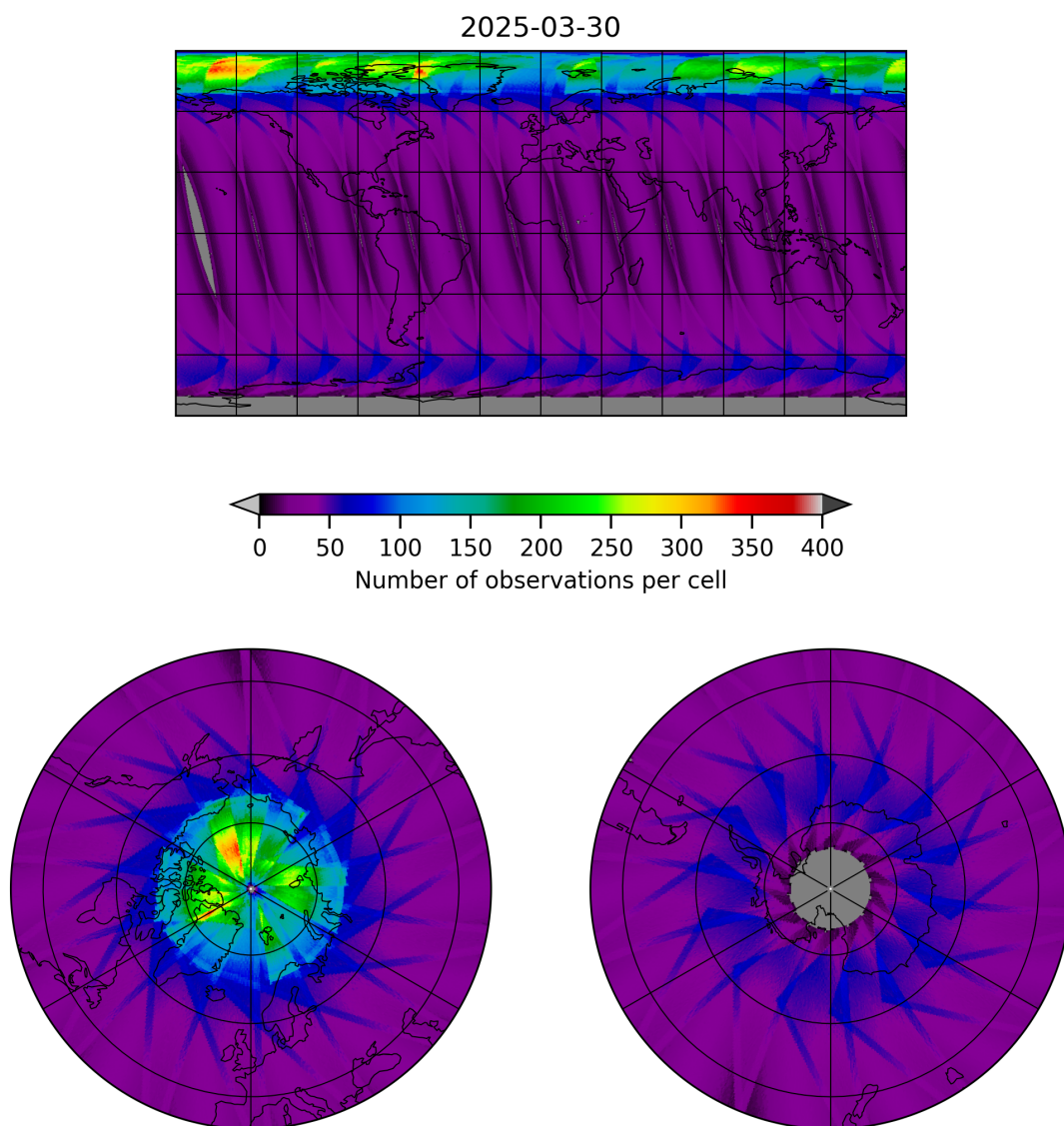
Figure 17: Map of the number of observations for 2025-03-30 to 2025-03-31
