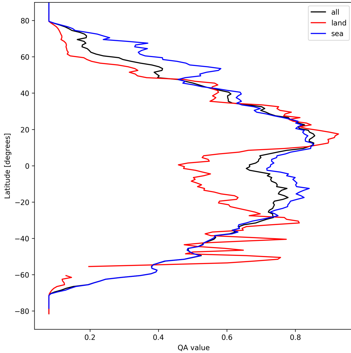
Figure 18: Zonal average of “QA value” for 2025-03-30 to 2025-03-31.
